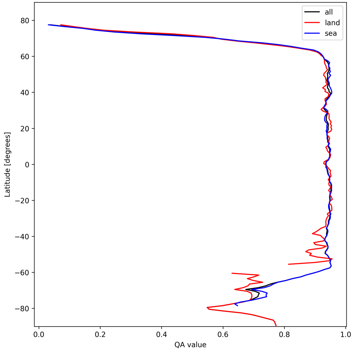
Figure 13: Zonal average of “QA value” for 2024-10-21 to 2024-10-23.
