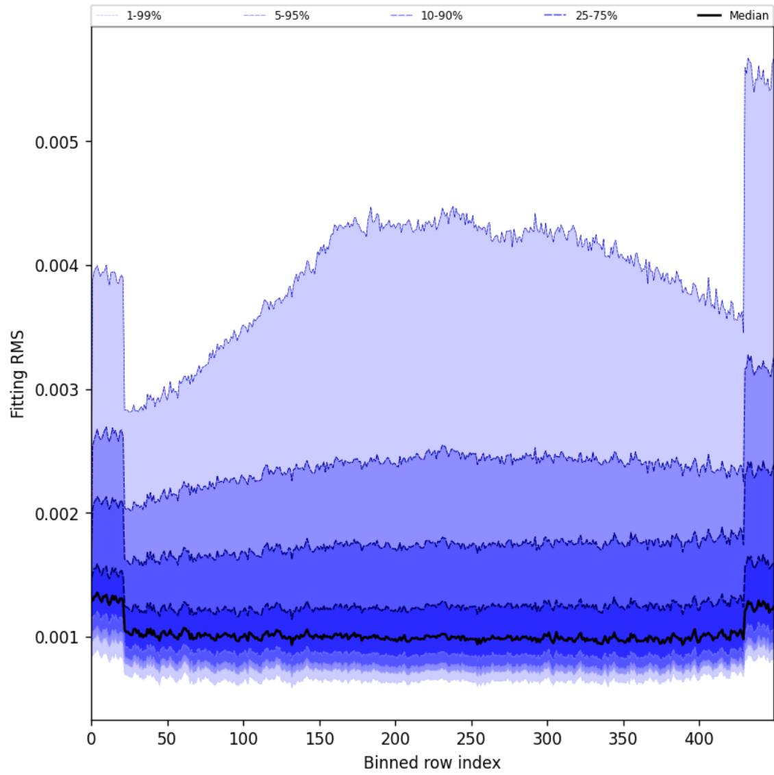
Figure 30: Along track statistics of “Fitting RMS” for 2024-10-21 to 2024-10-23
