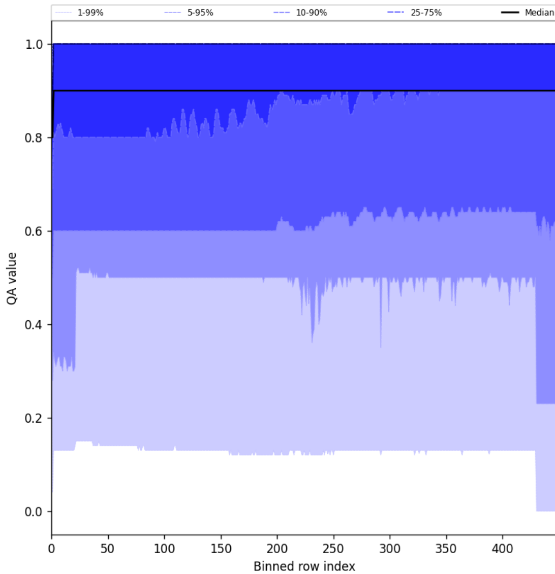
Figure 27: Along track statistics of “QA value” for 2024-10-21 to 2024-10-23
