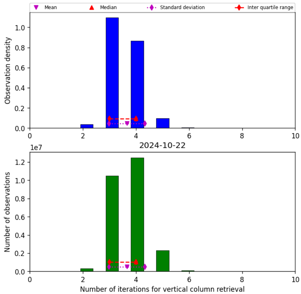
Figure 26: Histogram of “Number of iterations for vertical column retrieval” for 2024-10-21 to 2024-10-23
