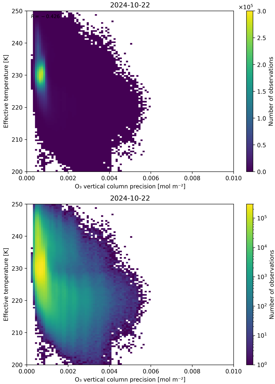
Figure 42: Scatter density plot of “O 3 vertical column precision” against “Effective temperature” for 2024-10-21 to 2024-10-23.
