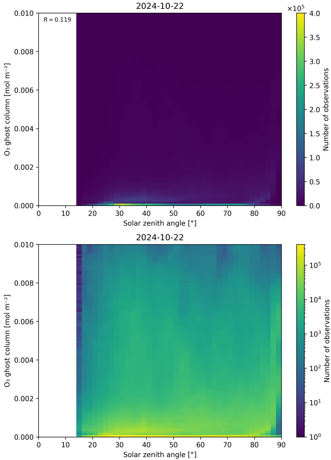
Figure 46: Scatter density plot of “Solar zenith angle” against “O 3 ghost column” for 2024-10-21 to 2024-10-23.
