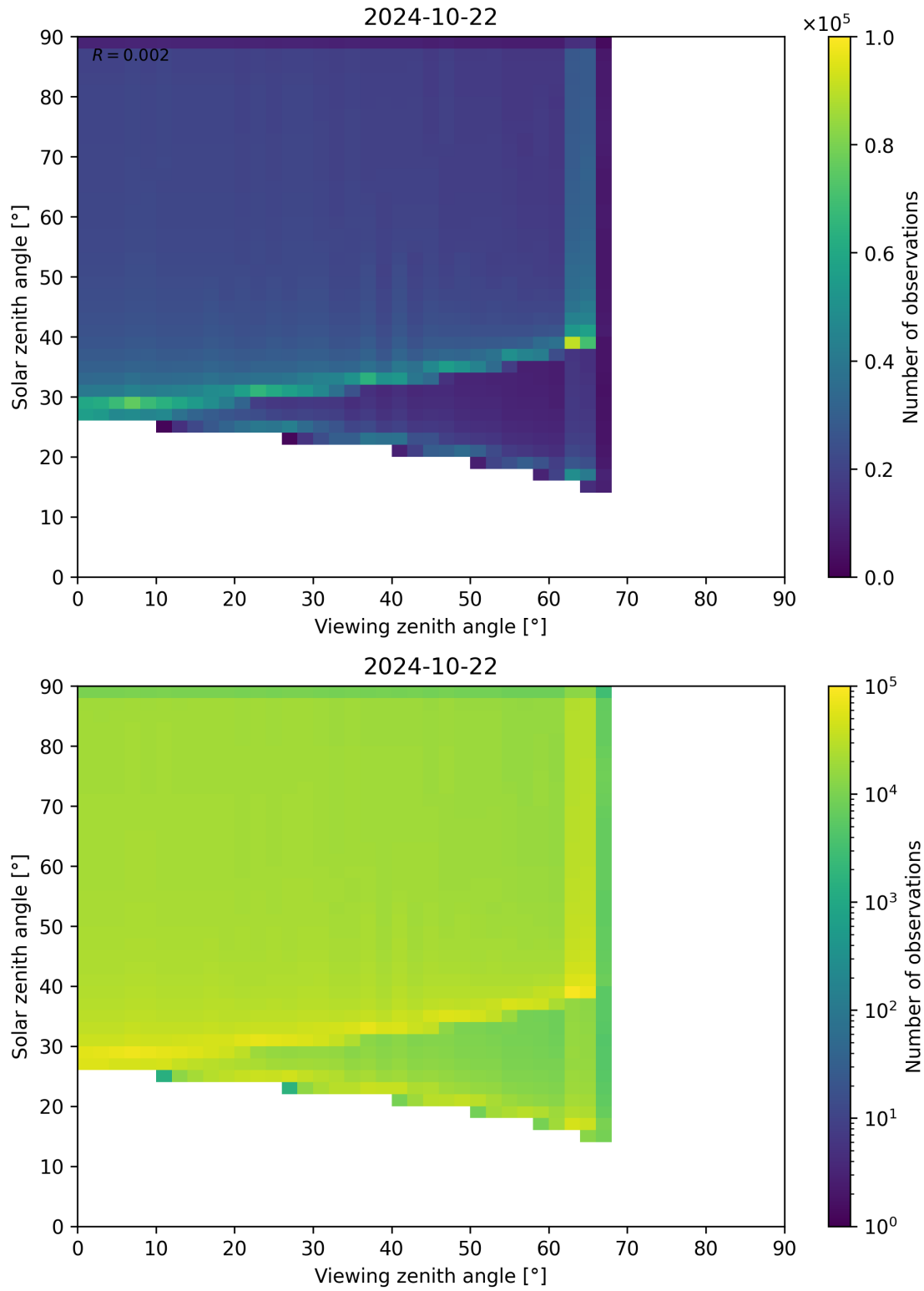
Figure 54: Scatter density plot of “Viewing zenith angle” against “Solar zenith angle” for 2024-10-21 to 2024-10-23.
