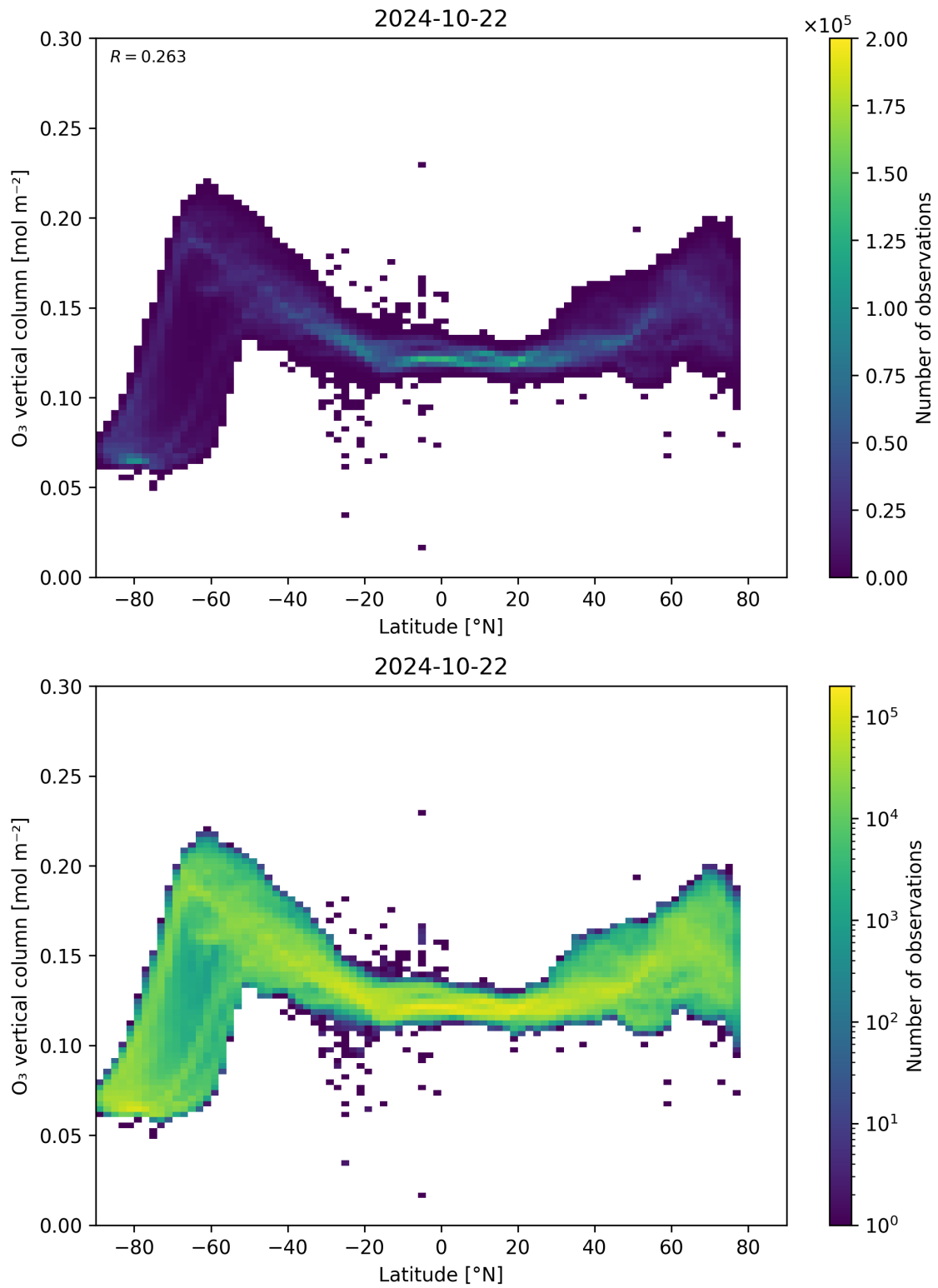
Figure 36: Scatter density plot of “Latitude” against “O 3 vertical column” for 2024-10-21 to 2024-10-23.
