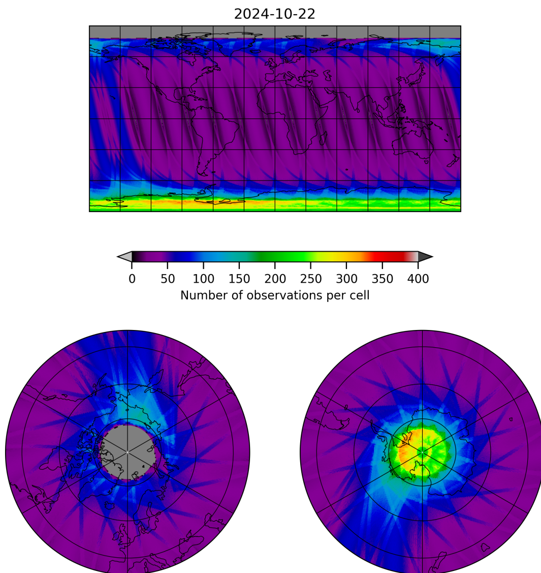
Figure 12: Map of the number of observations for 2024-10-21 to 2024-10-23
