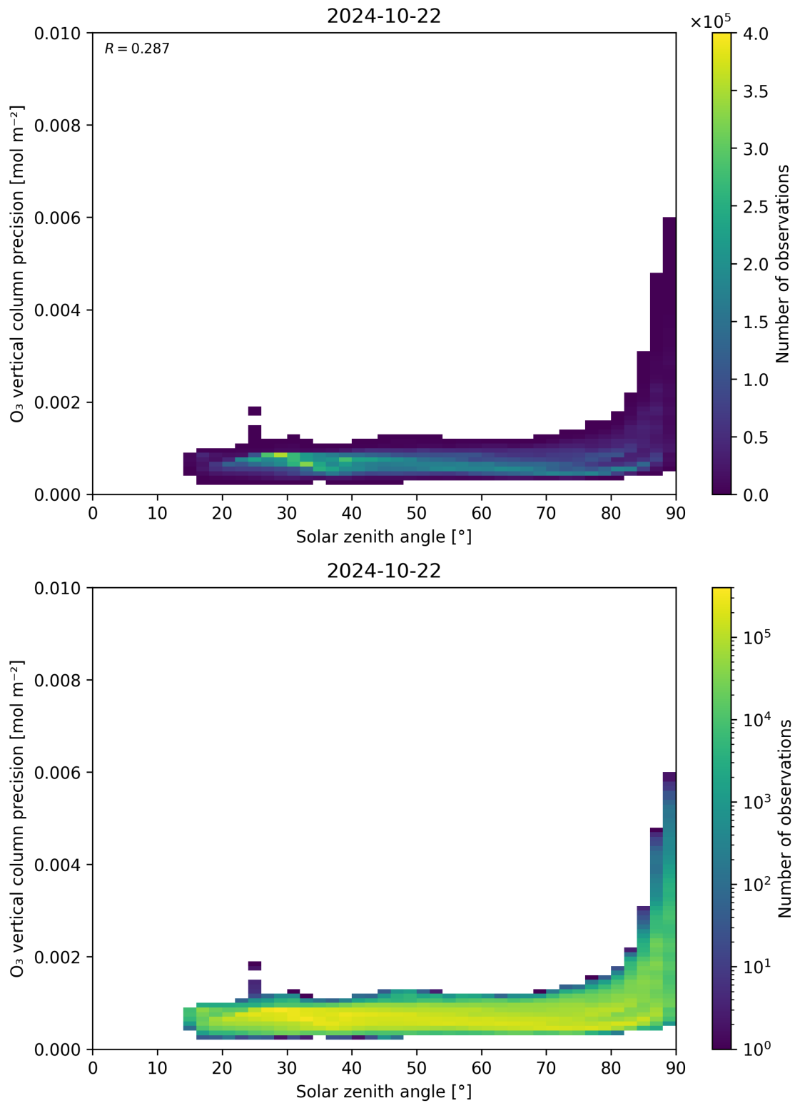
Figure 48: Scatter density plot of “Solar zenith angle” against “O 3 vertical column precision” for 2024-10-21 to 2024-10-23.
