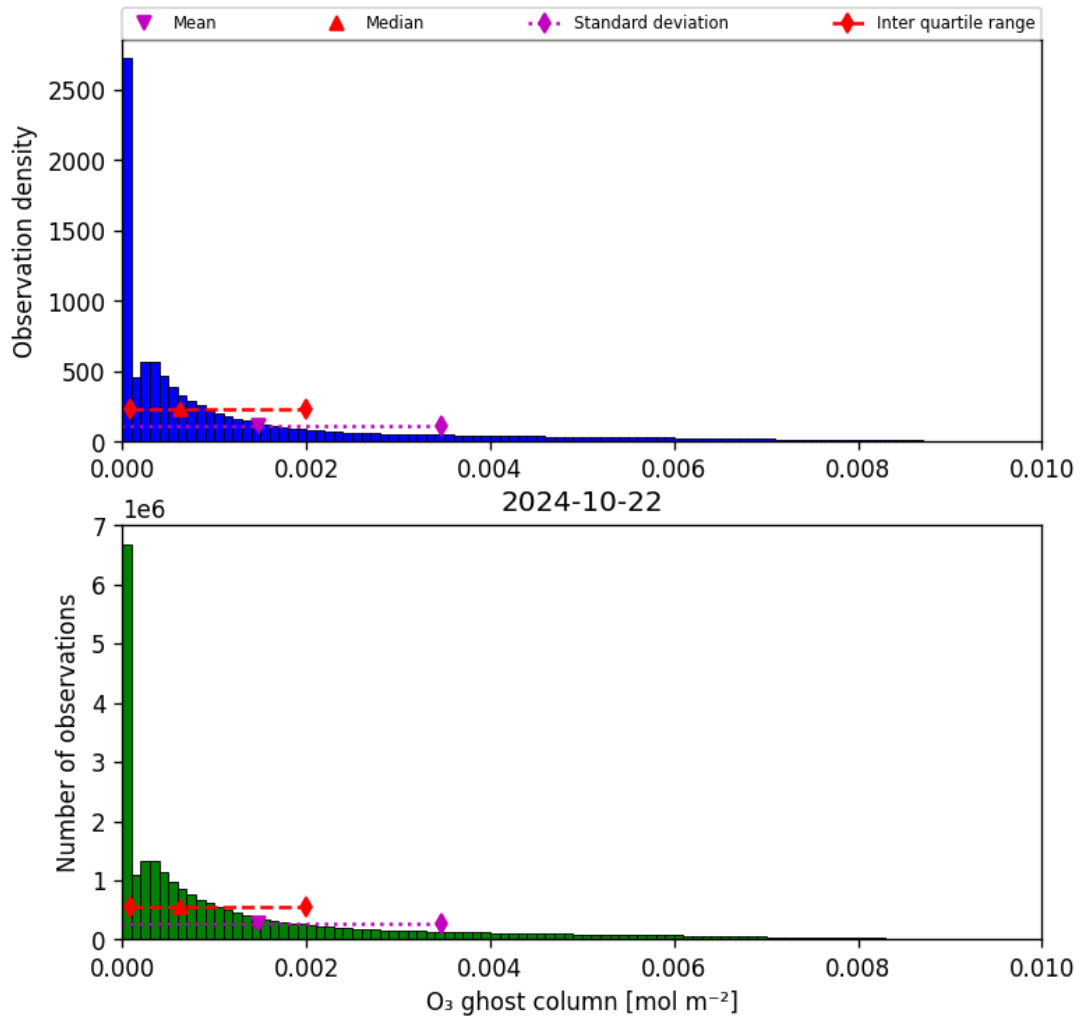
Figure 25: Histogram of “O 3 ghost column” for 2024-10-21 to 2024-10-23
