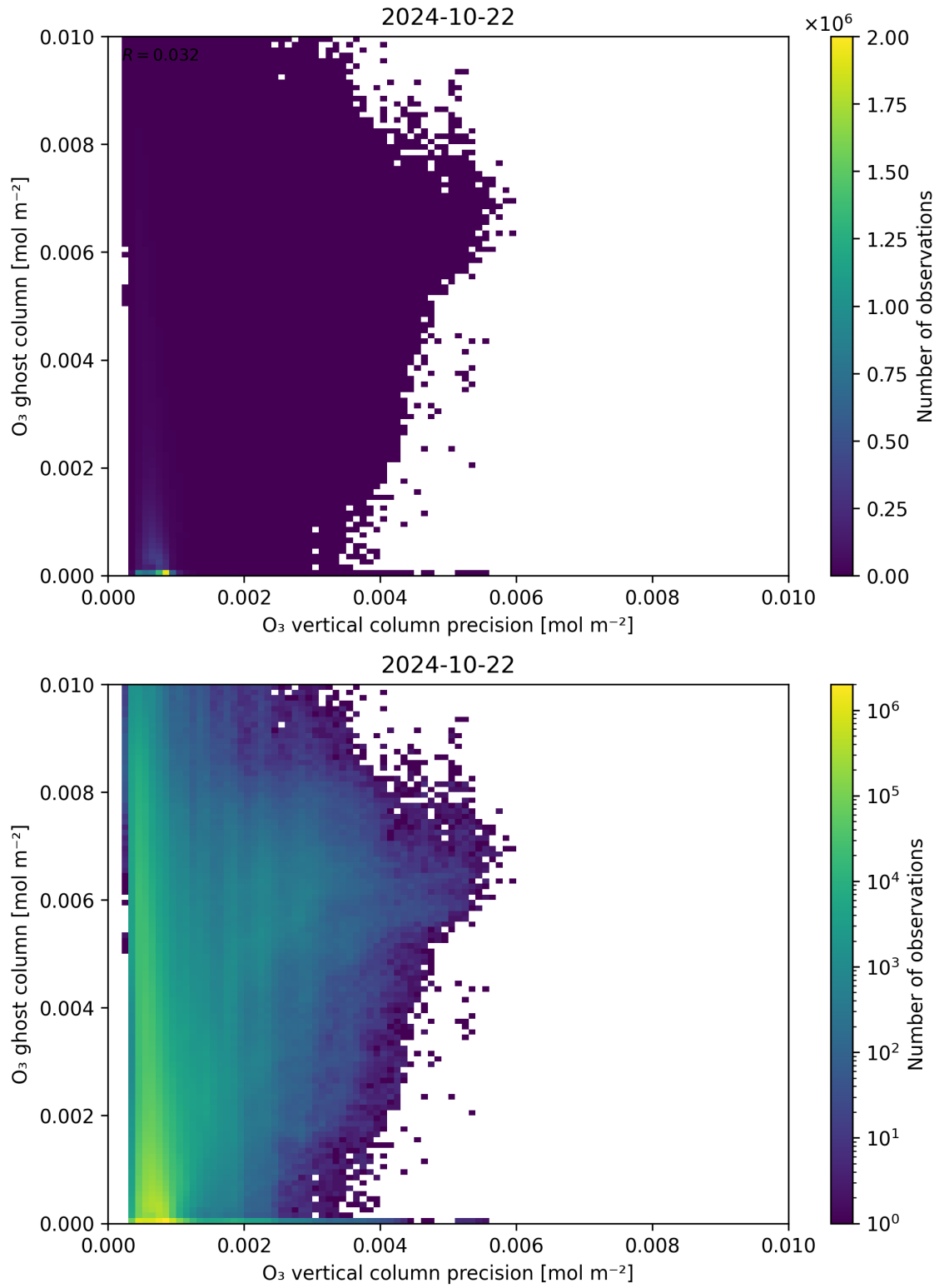
Figure 43: Scatter density plot of “O 3 vertical column precision” against “O 3 ghost column” for 2024-10-21 to 2024-10-23.
