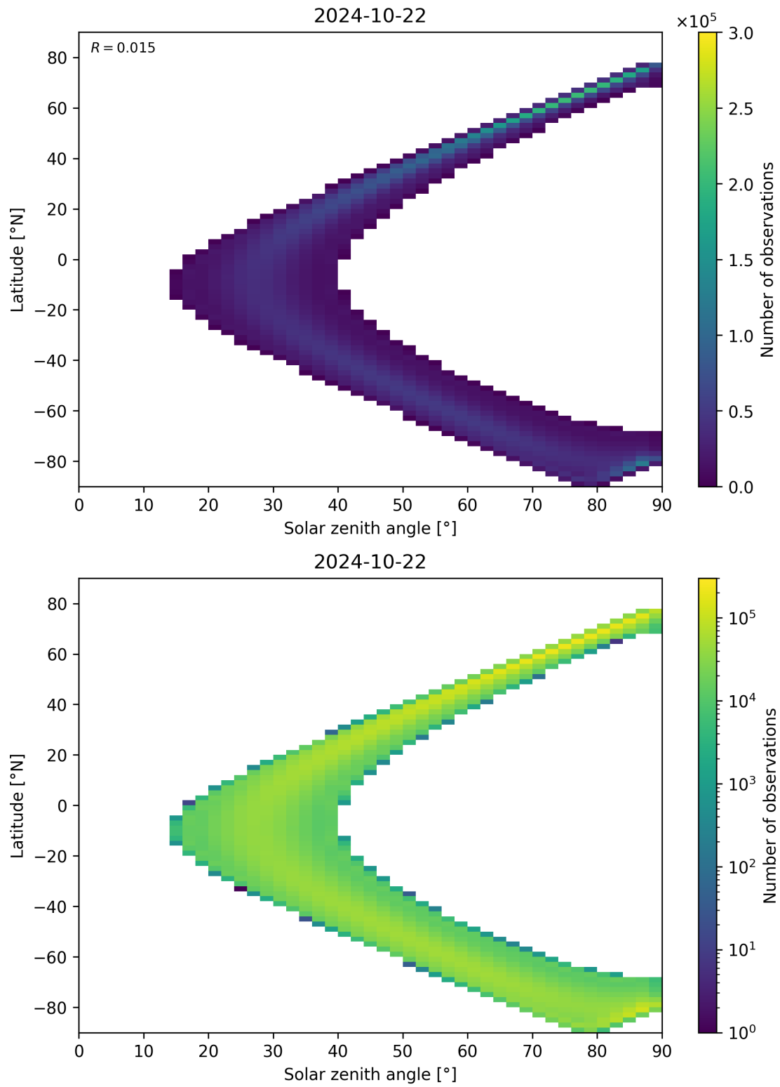
Figure 44: Scatter density plot of “Solar zenith angle” against “Latitude” for 2024-10-21 to 2024-10-23.
