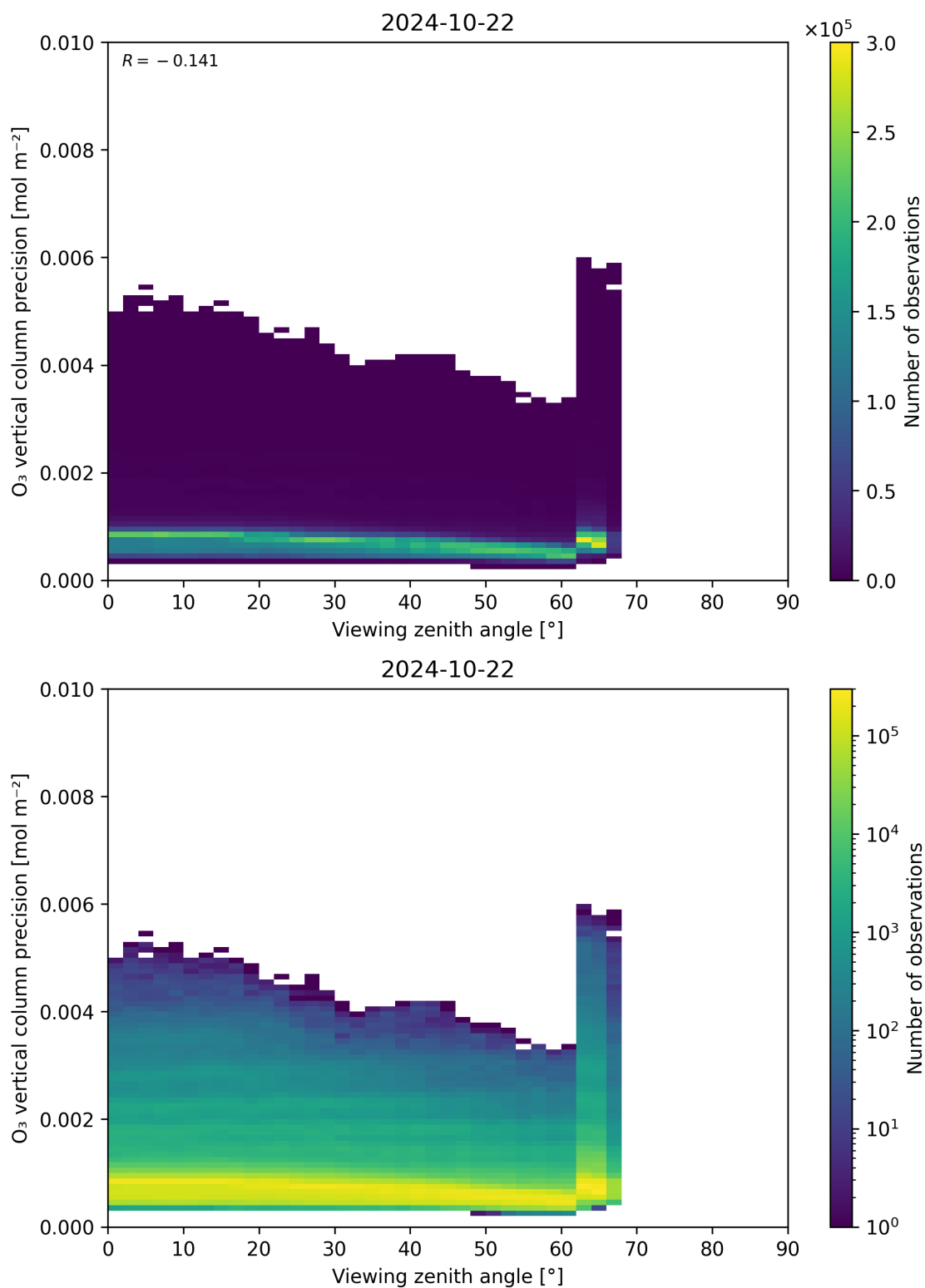
Figure 53: Scatter density plot of “Viewing zenith angle” against “O 3 vertical column precision” for 2024-10-21 to 2024-10-23.
