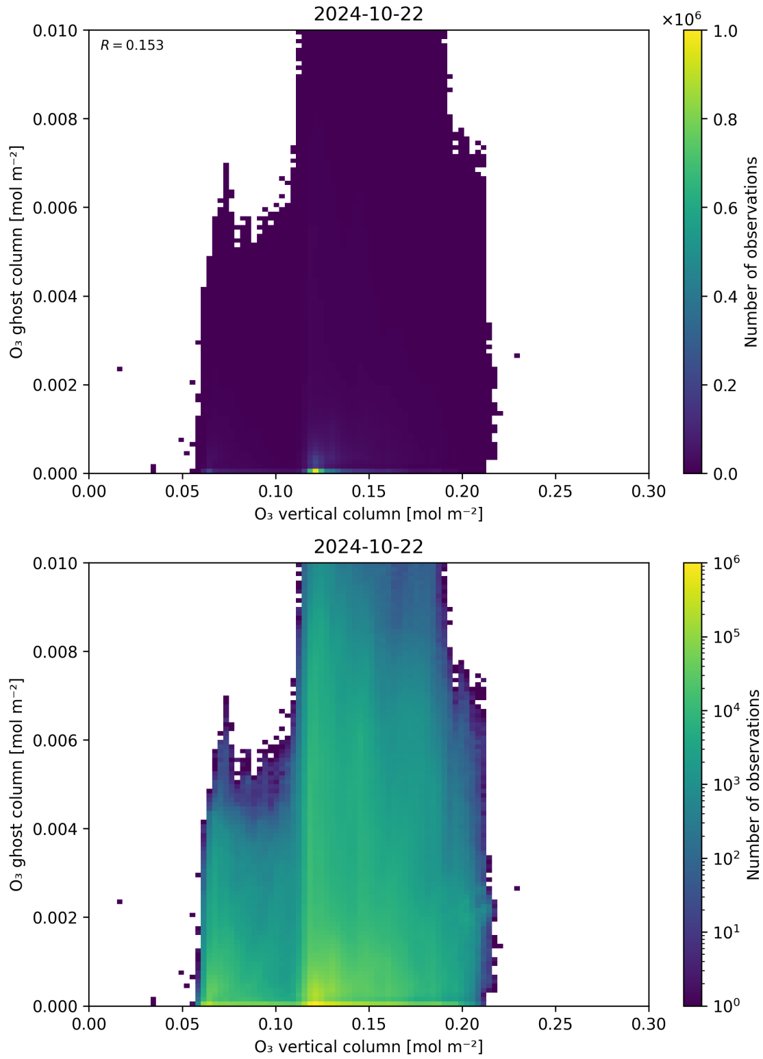
Figure 40: Scatter density plot of “O 3 vertical column” against “O 3 ghost column” for 2024-10-21 to 2024-10-23.
