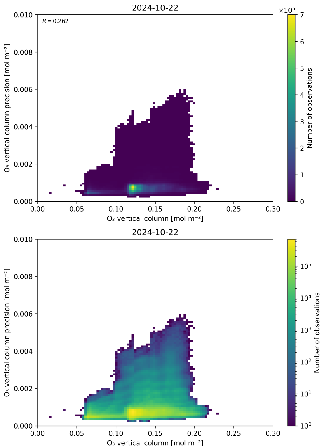
Figure 41: Scatter density plot of “O 3 vertical column” against “O 3 vertical column precision” for 2024-10-21 to 2024-10-23.
