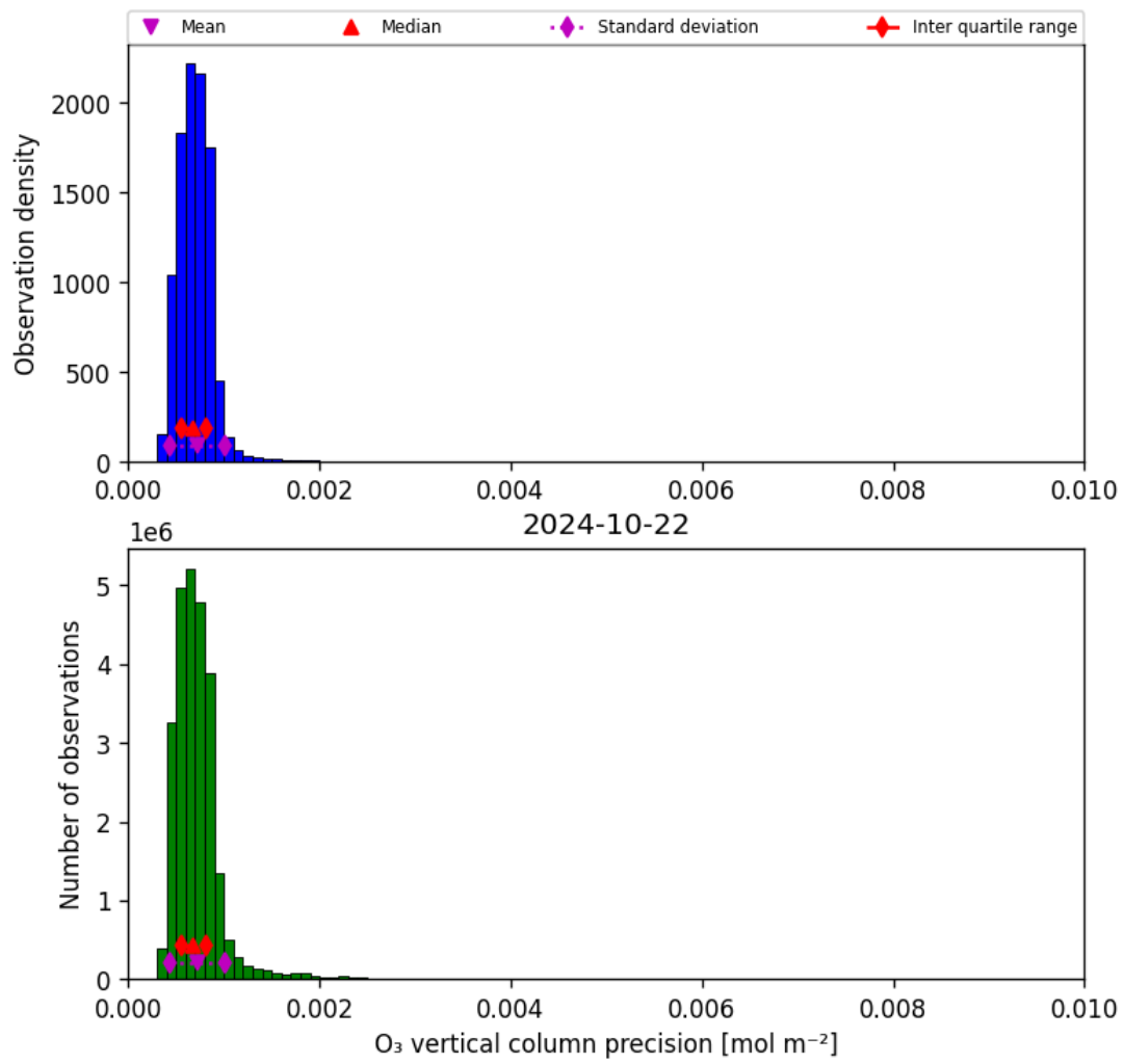
Figure 22: Histogram of "O 3 vertical column precision" for 2024-10-21 to 2024-10-23
