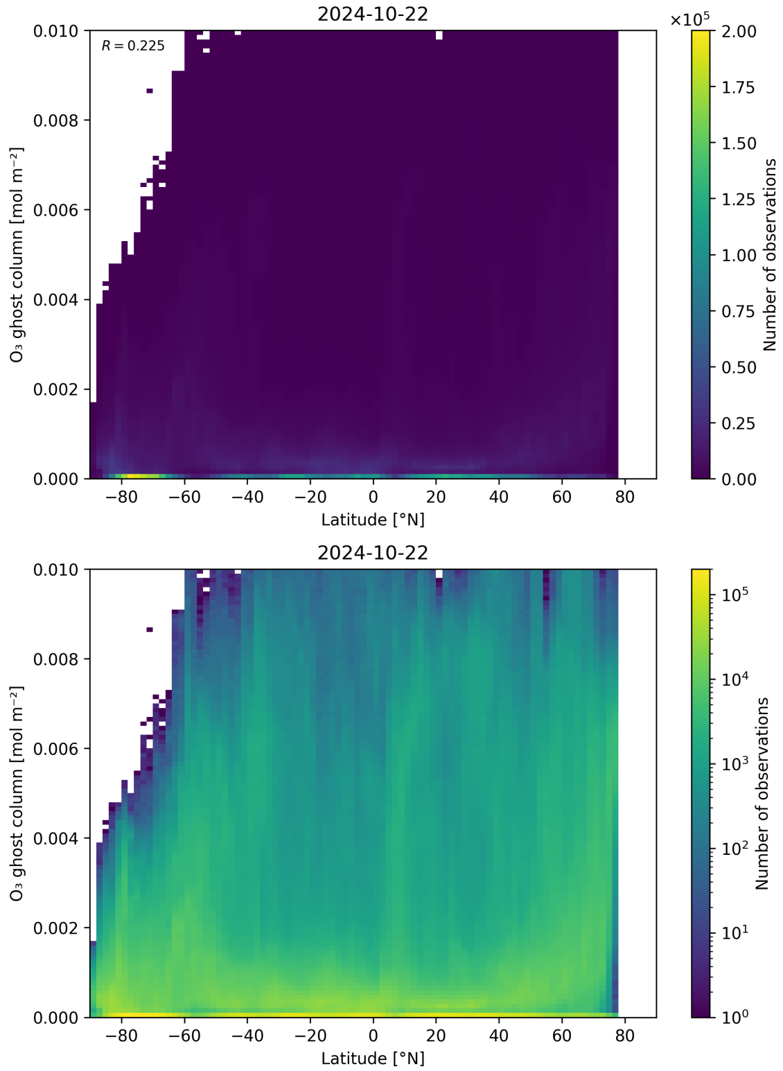
Figure 35: Scatter density plot of “Latitude” against “O 3 ghost column” for 2024-10-21 to 2024-10-23.
