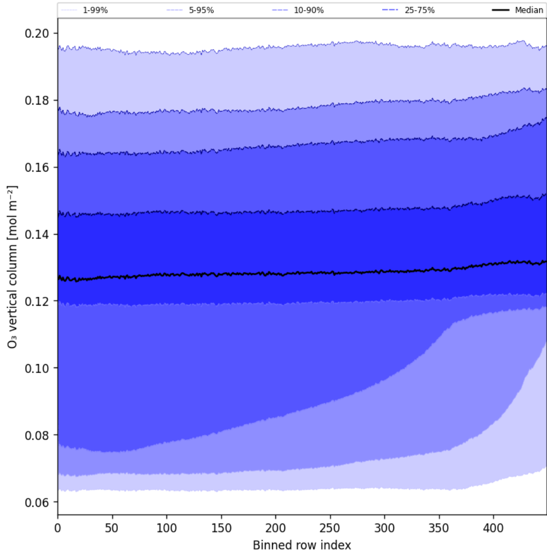
Figure 28: Along track statistics of "O 3 vertical column" for 2024-10-21 to 2024-10-23
