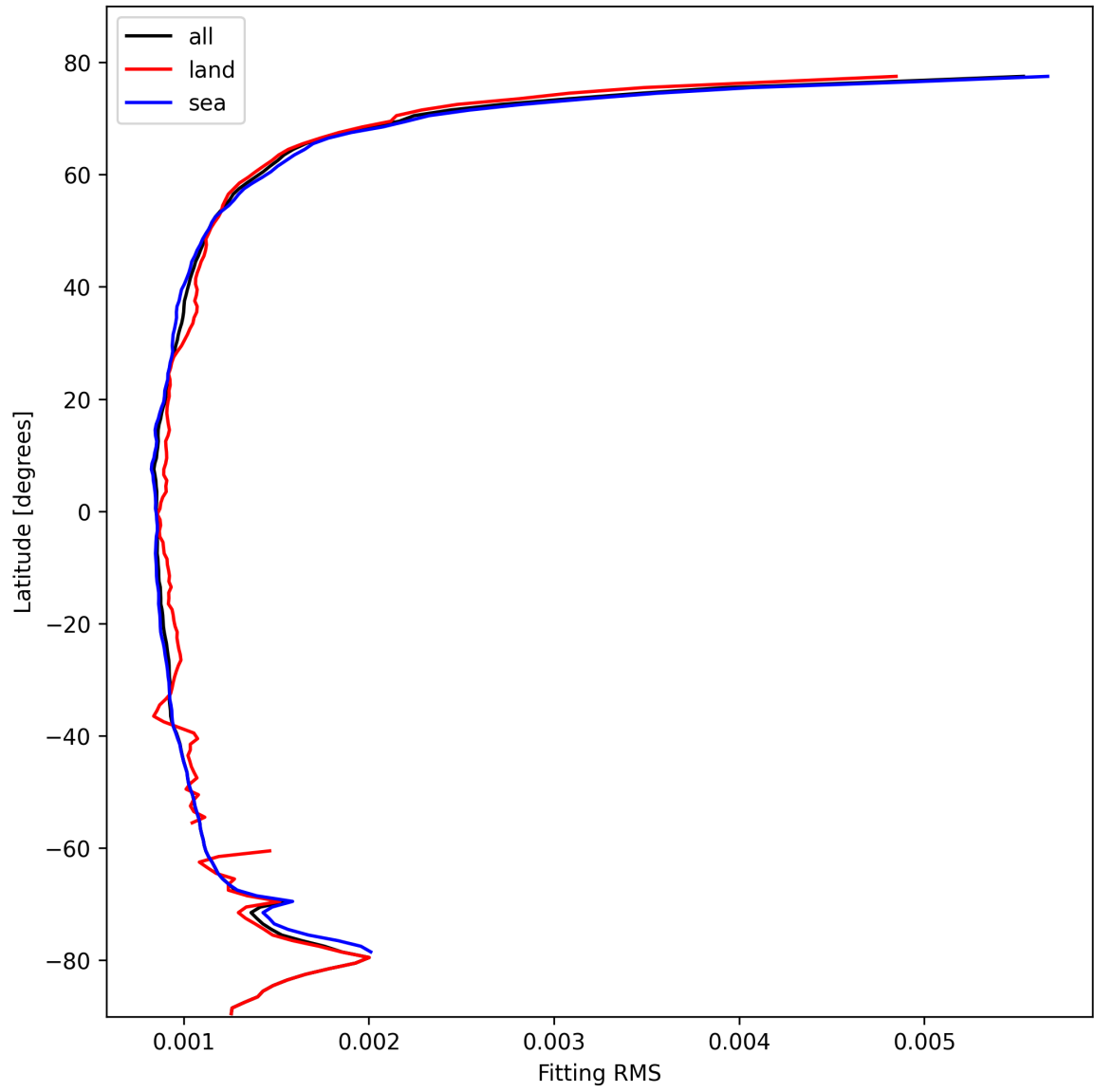
Figure 16: Zonal average of “Fitting RMS” for 2024-10-21 to 2024-10-23.
