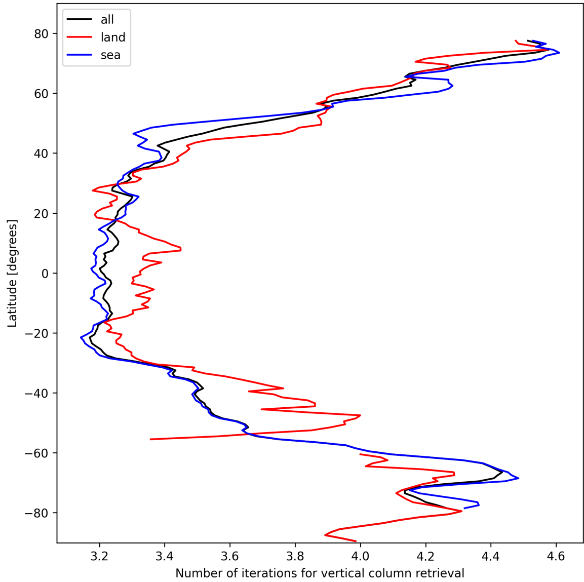
Figure 19: Zonal average of “Number of iterations for vertical column retrieval” for 2024-10-21 to 2024-10-23.
