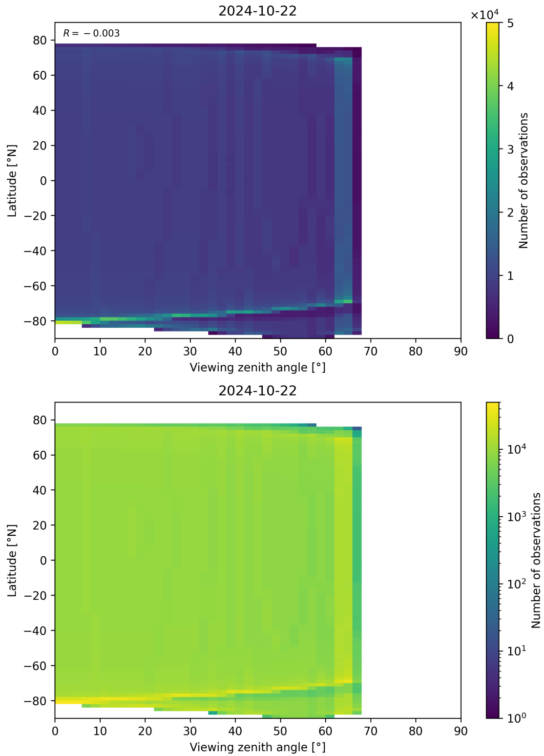
Figure 49: Scatter density plot of “Viewing zenith angle” against “Latitude” for 2024-10-21 to 2024-10-23.
