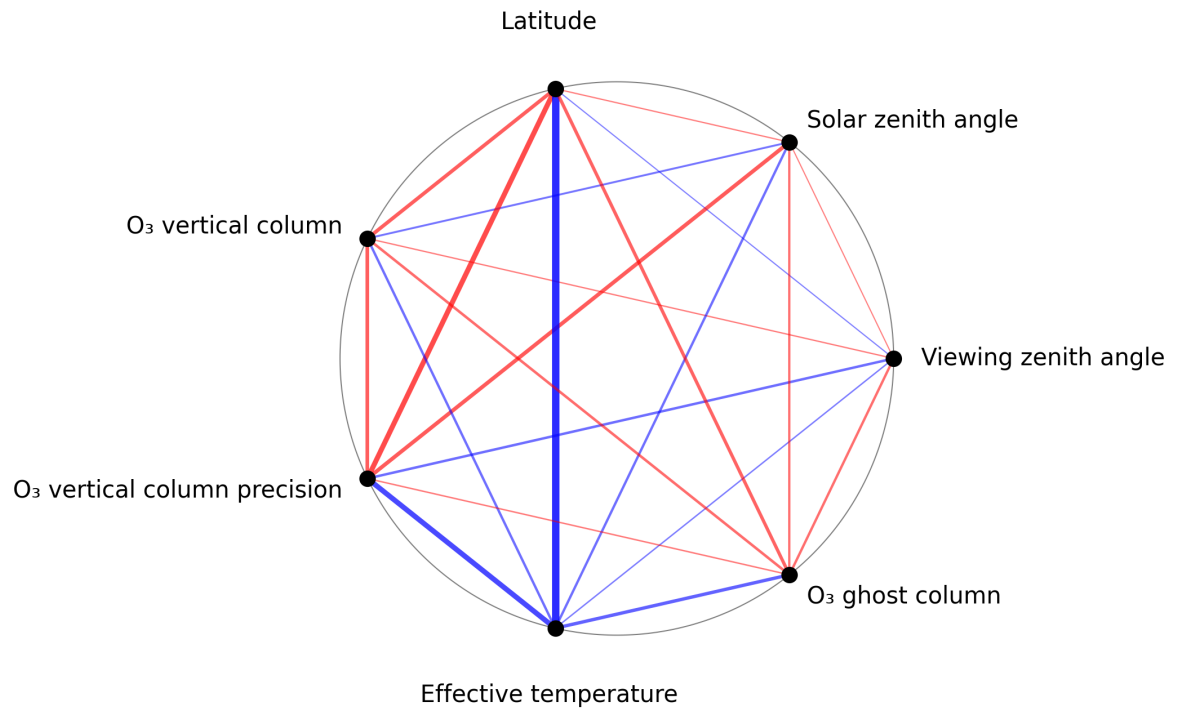
Figure 1: Map of correlation graph for 2024-10-21 to 2024-10-23.
