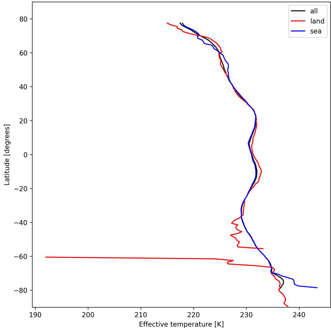
Figure 17: Zonal average of “Effective temperature” for 2024-10-21 to 2024-10-23.
