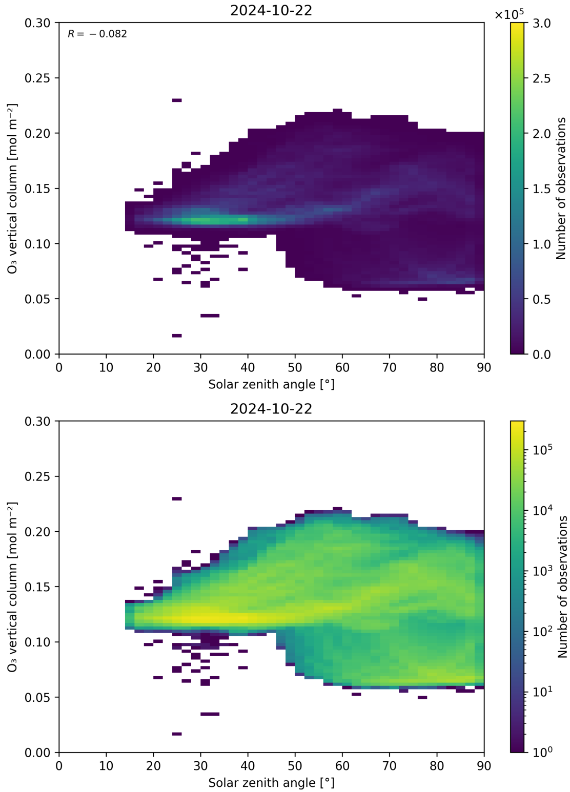
Figure 47: Scatter density plot of “Solar zenith angle” against “O 3 vertical column” for 2024-10-21 to 2024-10-23.
