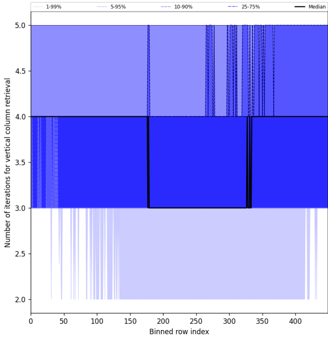
Figure 33: Along track statistics of “Number of iterations for vertical column retrieval” for 2024-10-21 to 2024-10-23
