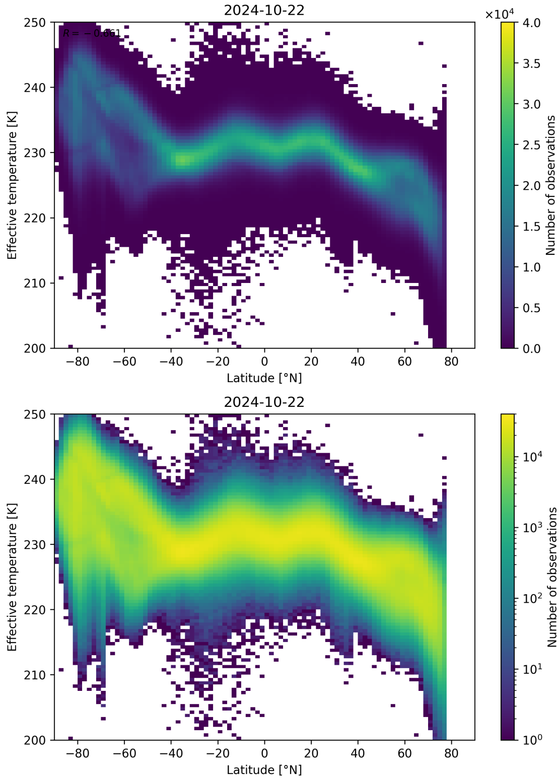
Figure 34: Scatter density plot of “Latitude” against “Effective temperature” for 2024-10-21 to 2024-10-23.
