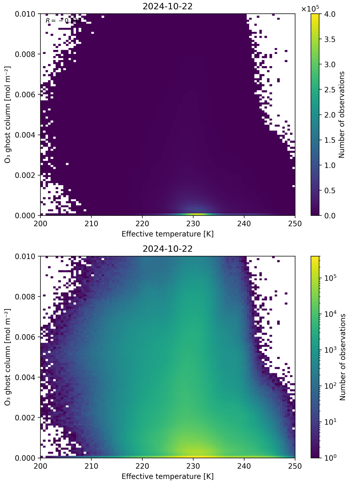
Figure 38: Scatter density plot of “Effective temperature” against “O 3 ghost column” for 2024-10-21 to 2024-10-23.
