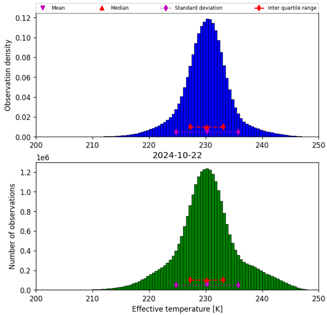
Figure 24: Histogram of “Effective temperature” for 2024-10-21 to 2024-10-23
