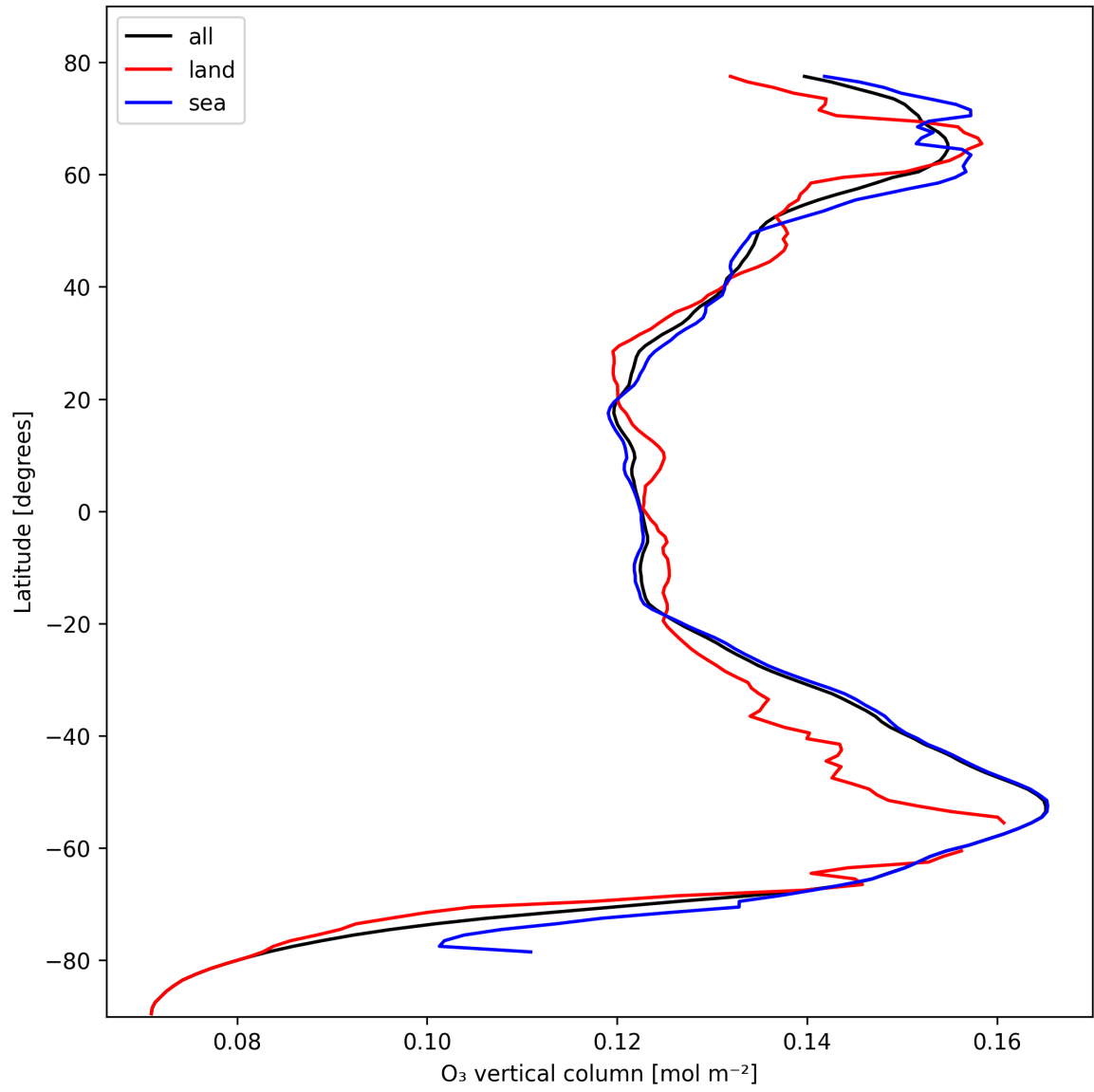
Figure 14: Zonal average of “O 3 vertical column” for 2024-10-21 to 2024-10-23.
