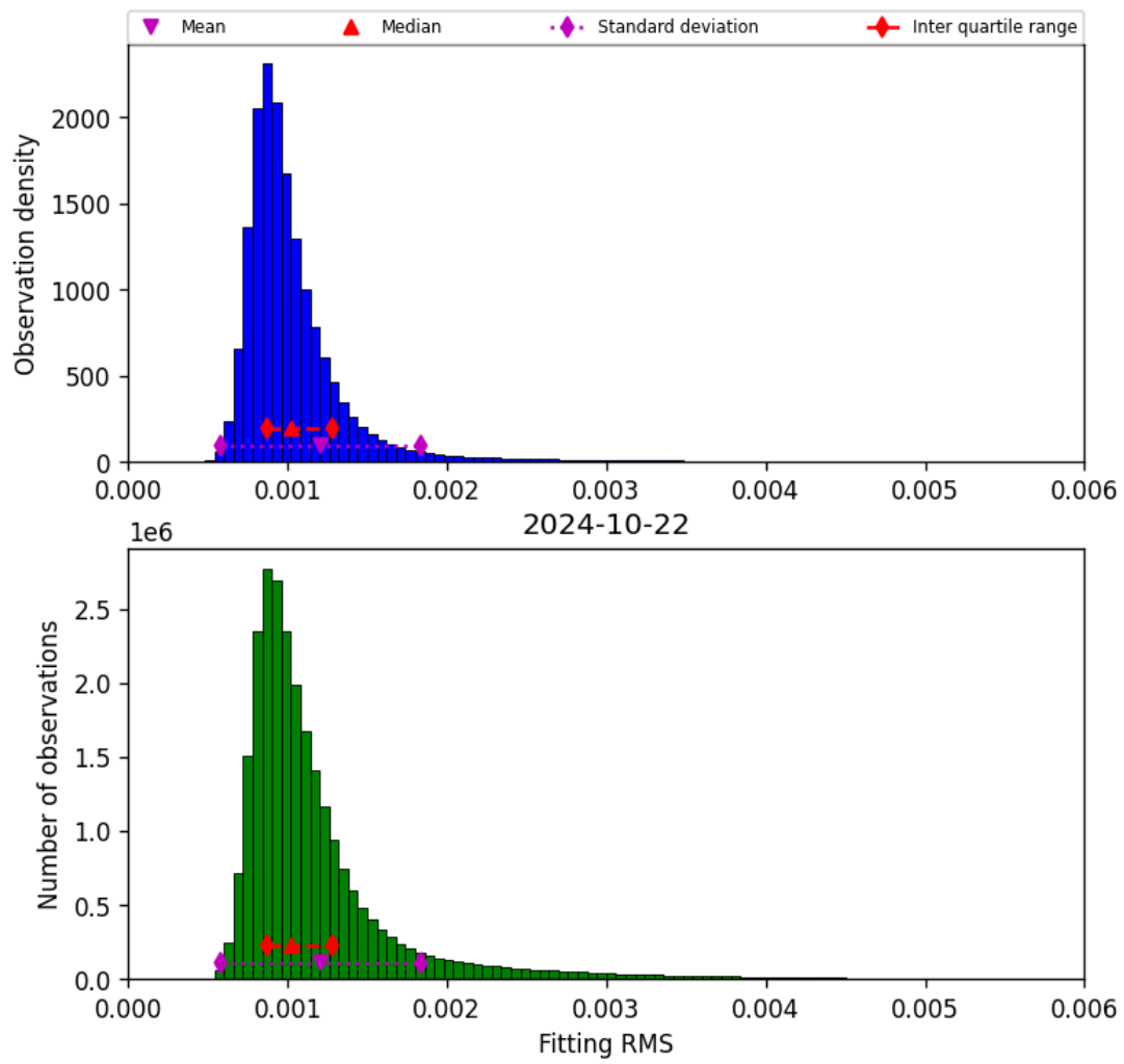
Figure 23: Histogram of “Fitting RMS” for 2024-10-21 to 2024-10-23
