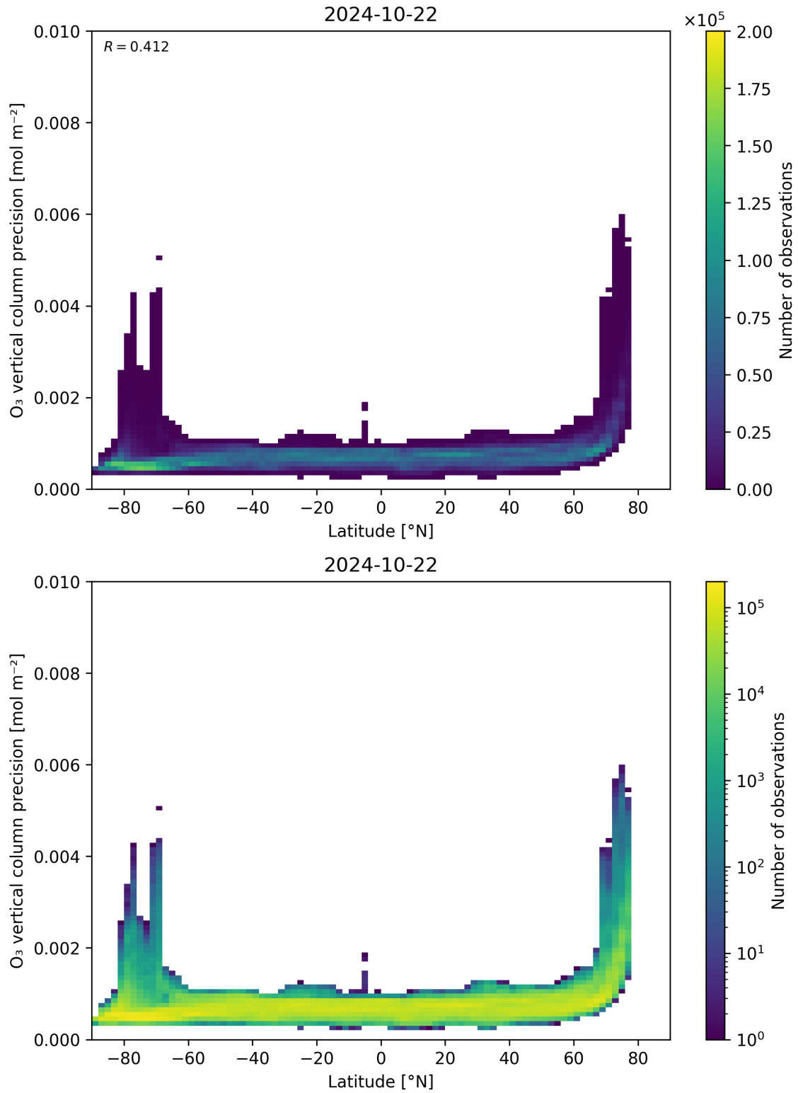
Figure 37: Scatter density plot of “Latitude” against “O 3 vertical column precision” for 2024-10-21 to 2024-10-23.
