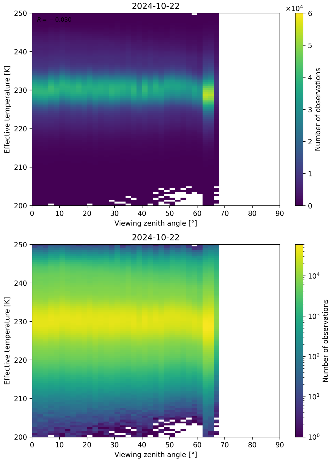
Figure 50: Scatter density plot of “Viewing zenith angle” against “Effective temperature” for 2024-10-21 to 2024-10-23.
