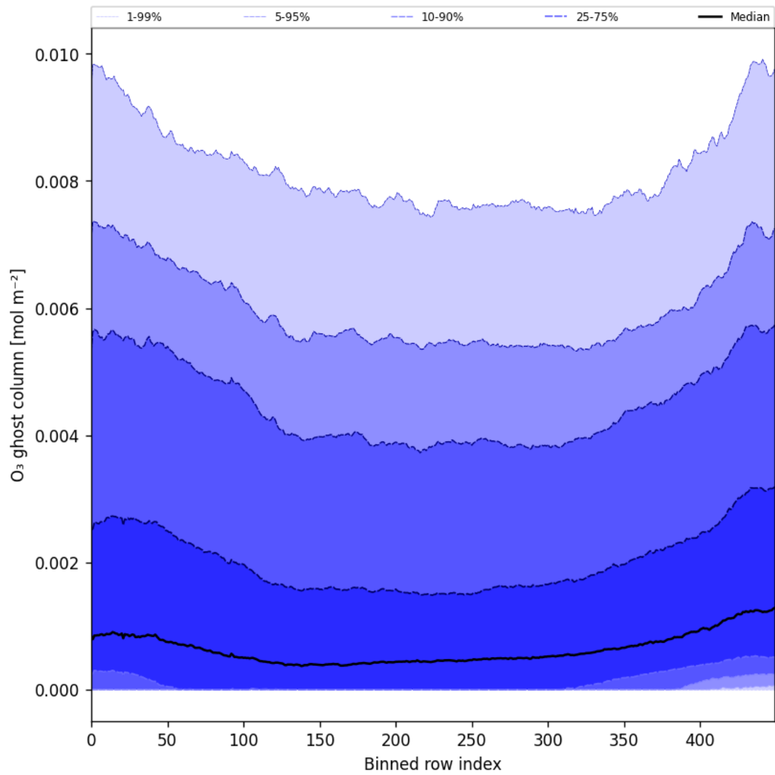
Figure 32: Along track statistics of “O 3 ghost column” for 2024-10-21 to 2024-10-23
