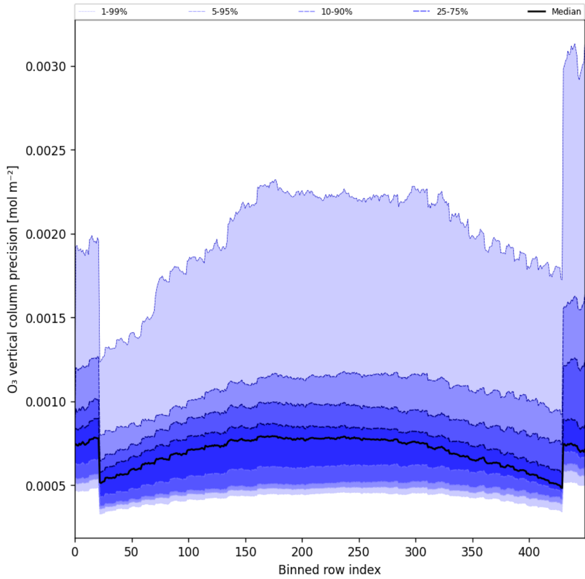
Figure 29: Along track statistics of “O 3 vertical column precision” for 2024-10-21 to 2024-10-23
