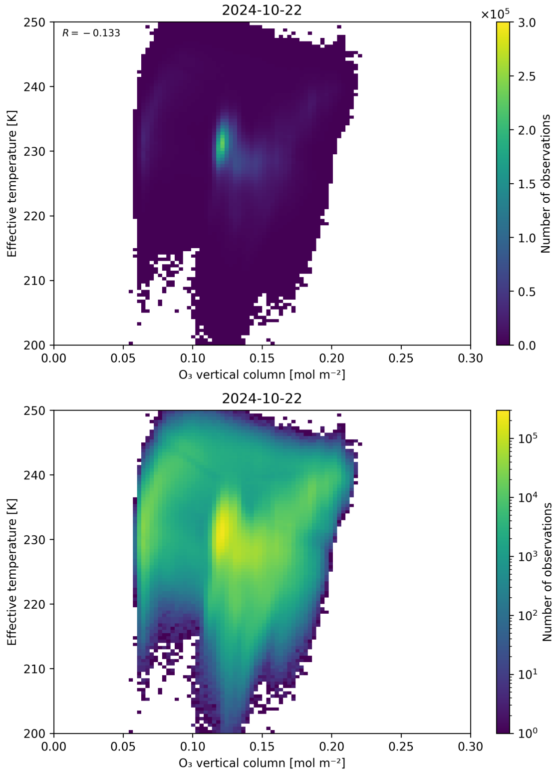
Figure 39: Scatter density plot of “O 3 vertical column” against “Effective temperature” for 2024-10-21 to 2024-10-23.
