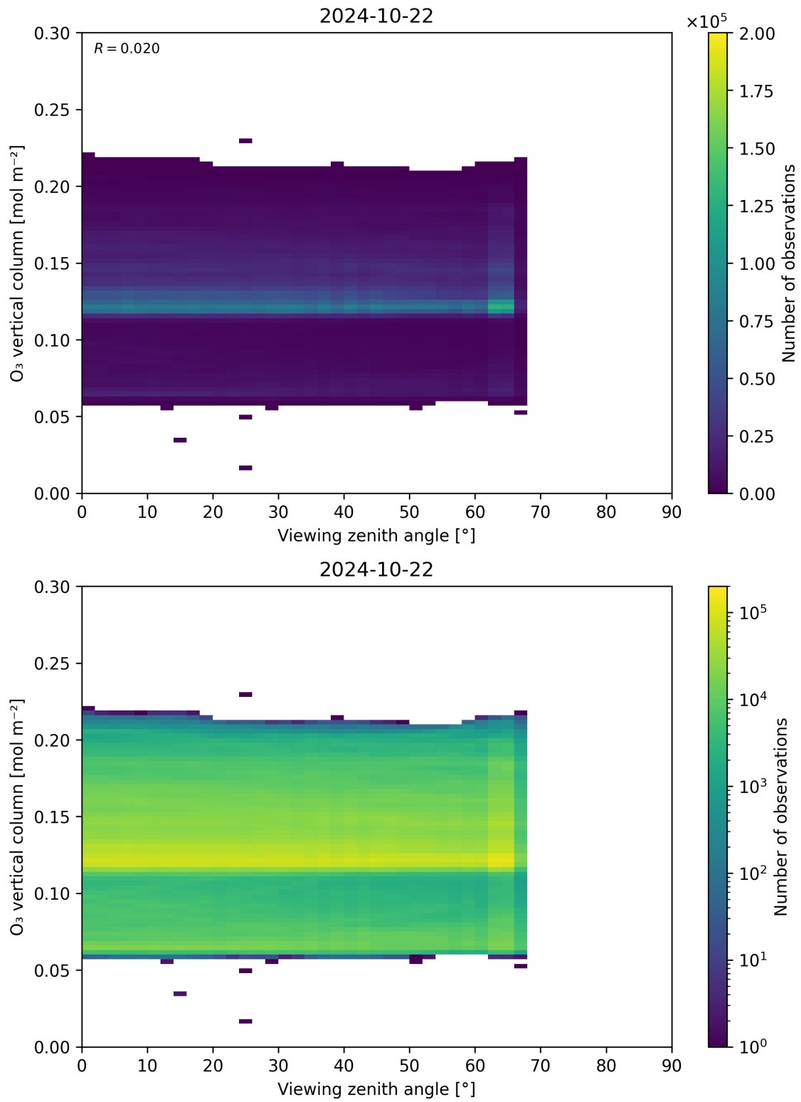
Figure 52: Scatter density plot of “Viewing zenith angle” against “O 3 vertical column” for 2024-10-21 to 2024-10-23.
