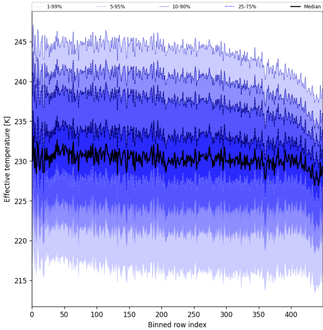
Figure 31: Along track statistics of “Effective temperature” for 2024-10-21 to 2024-10-23
