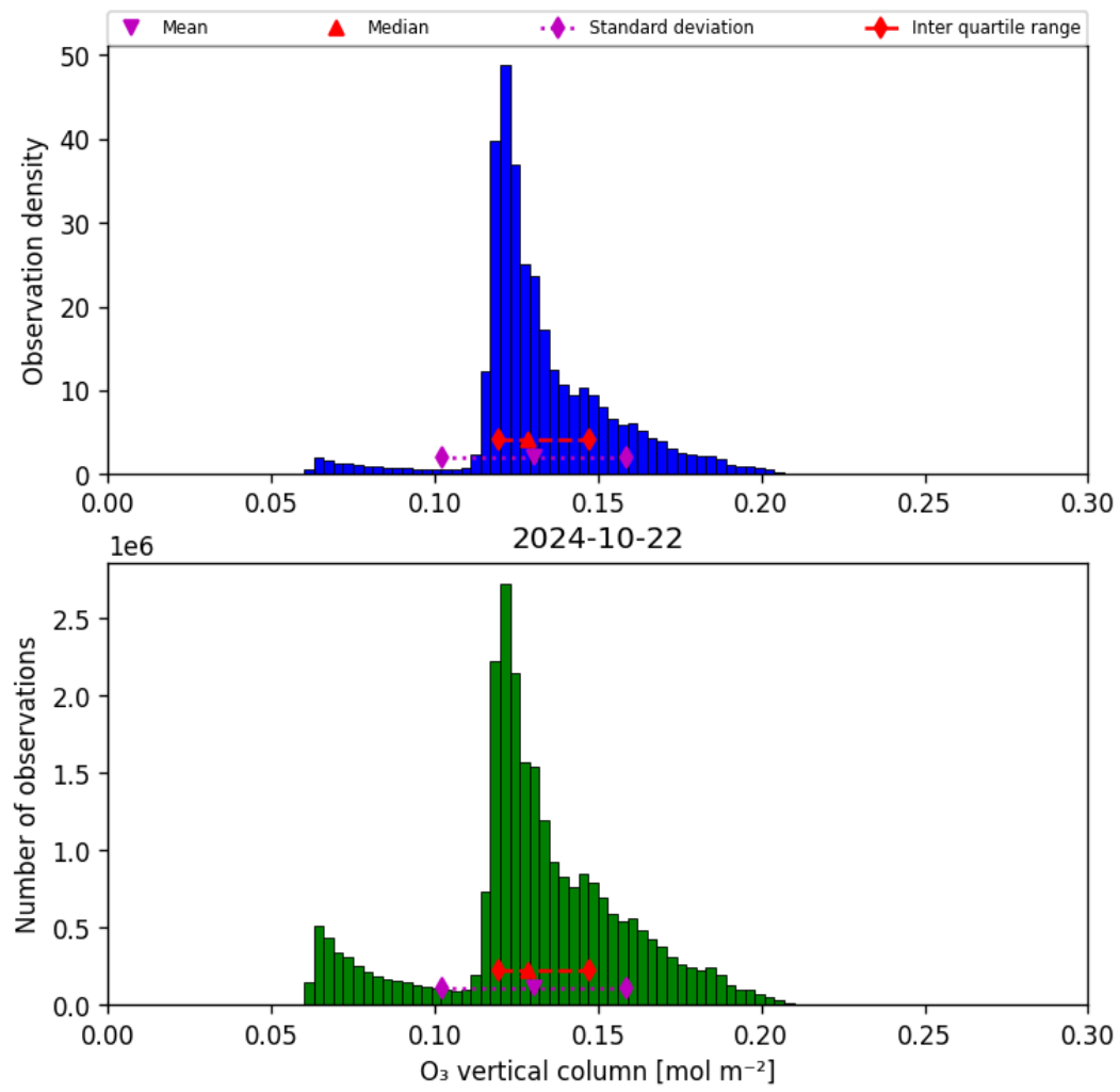
Figure 21: Histogram of “O 3 vertical column” for 2024-10-21 to 2024-10-23
