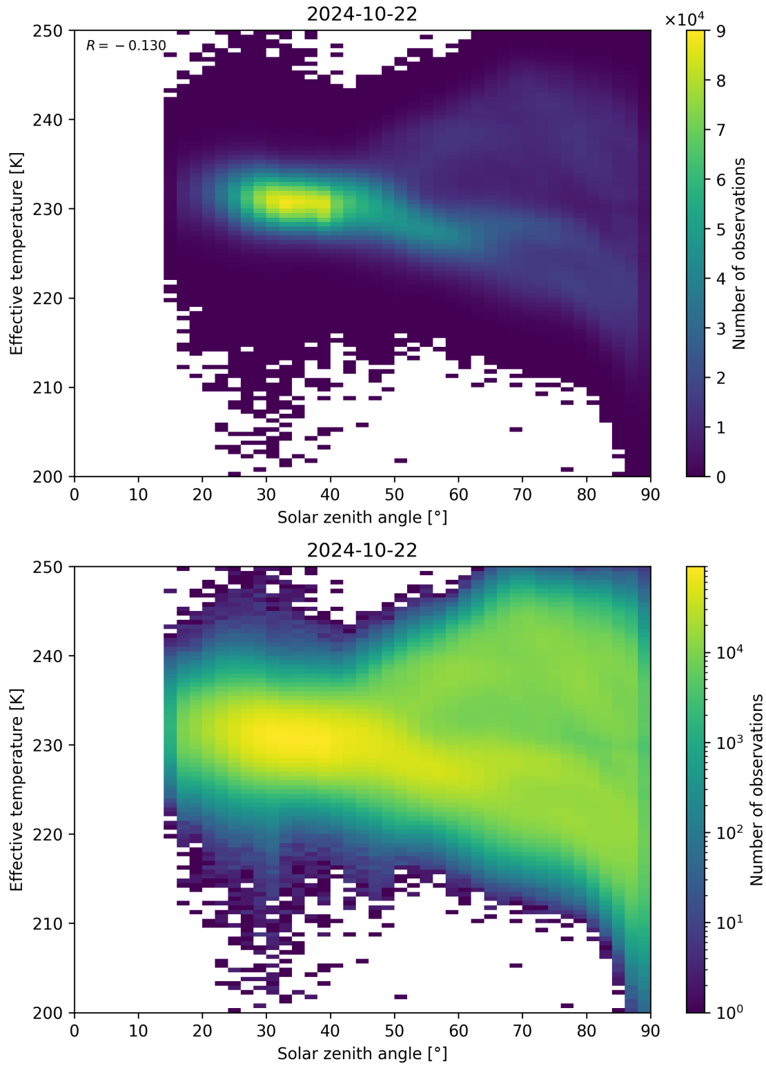
Figure 45: Scatter density plot of “Solar zenith angle” against “Effective temperature” for 2024-10-21 to 2024-10-23.
