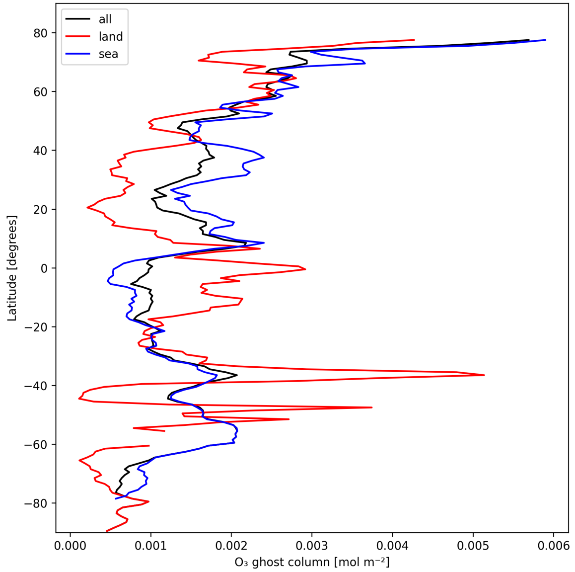
Figure 18: Zonal average of "O 3 ghost column" for 2024-10-21 to 2024-10-23.
