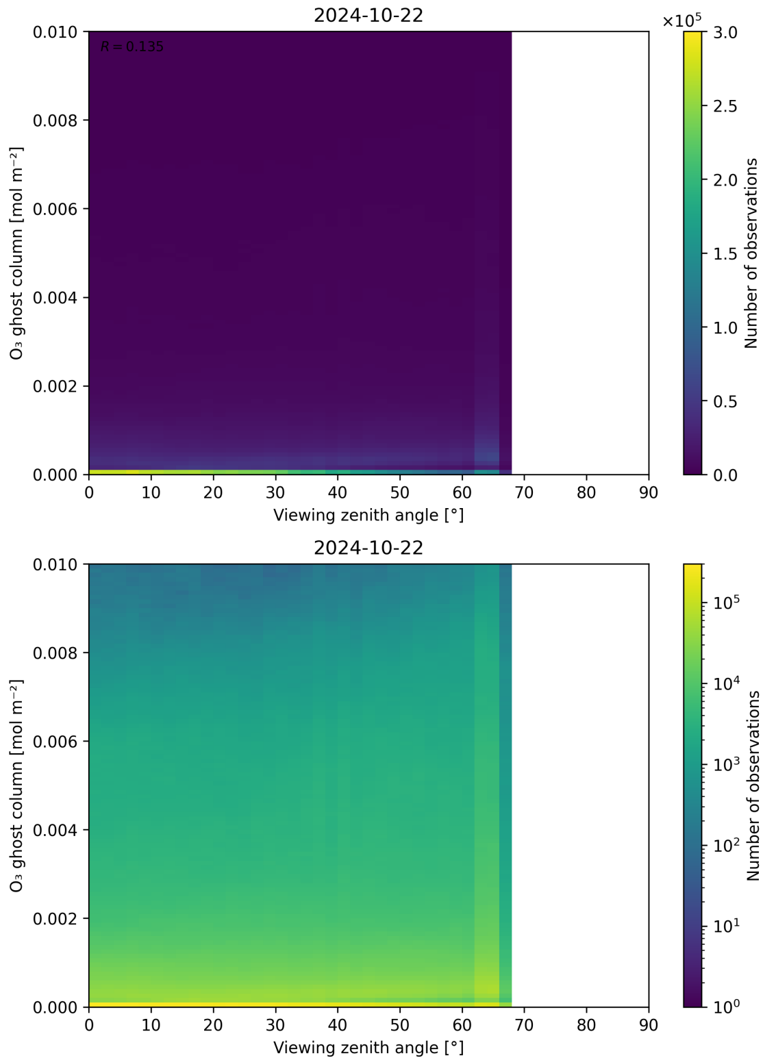
Figure 51: Scatter density plot of “Viewing zenith angle” against “O 3 ghost column” for 2024-10-21 to 2024-10-23.
