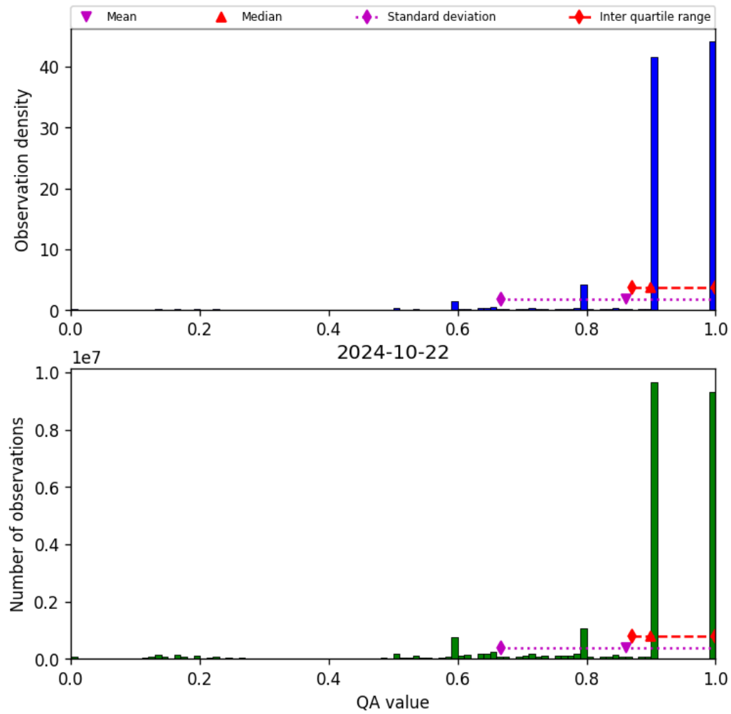
Figure 20: Histogram of “QA value” for 2024-10-21 to 2024-10-23
