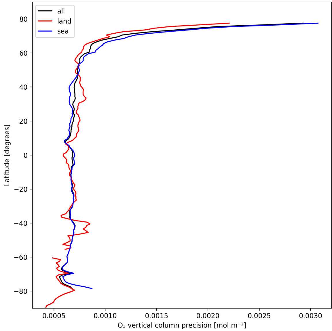
Figure 15: Zonal average of “O 3 vertical column precision” for 2024-10-21 to 2024-10-23.
