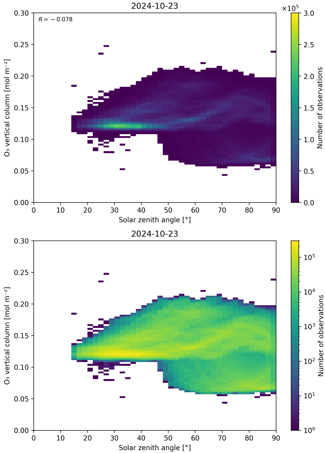
Figure 47: Scatter density plot of “Solar zenith angle” against “O 3 vertical column” for 2024-10-22 to 2024-10-24.
