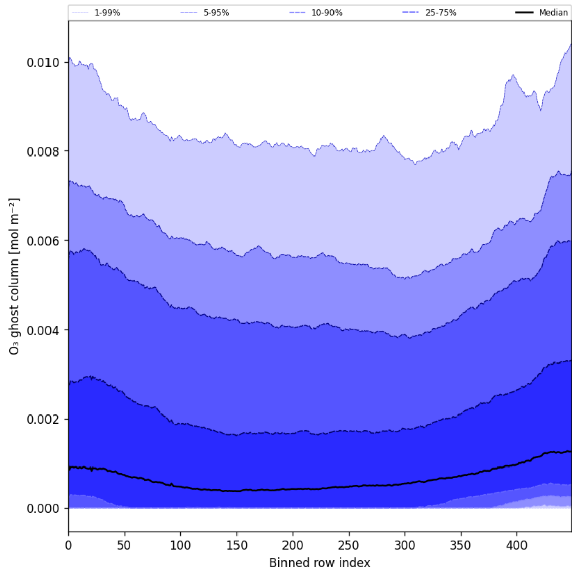
Figure 32: Along track statistics of “O 3 ghost column” for 2024-10-22 to 2024-10-24
