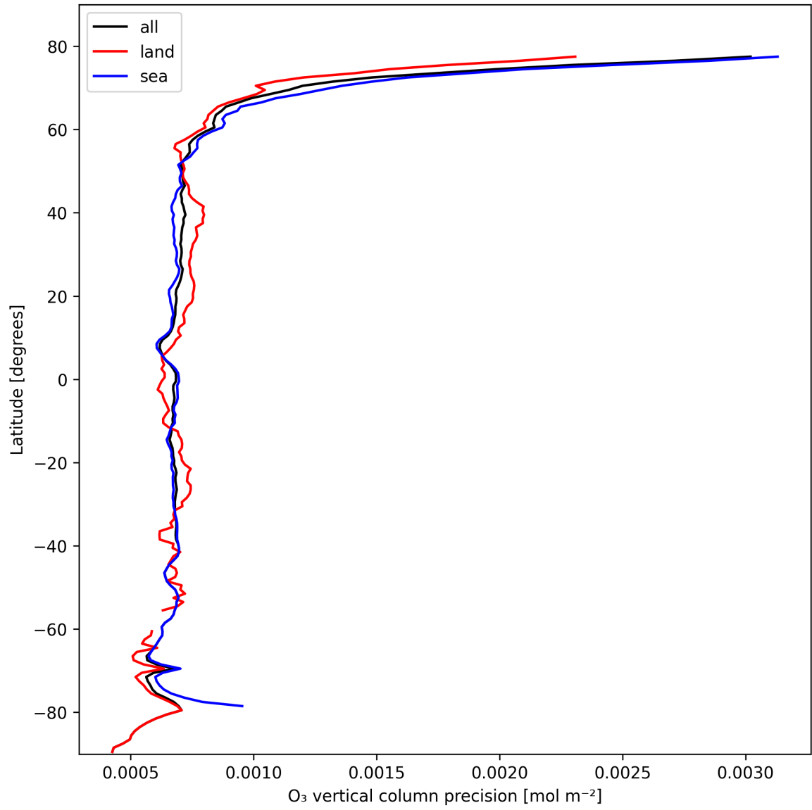
Figure 15: Zonal average of “O 3 vertical column precision” for 2024-10-22 to 2024-10-24.
