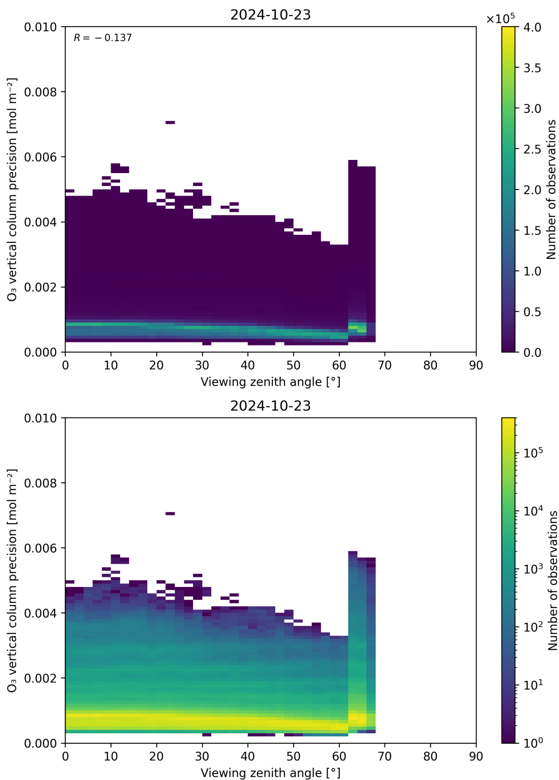
Figure 53: Scatter density plot of “Viewing zenith angle” against “O 3 vertical column precision” for 2024-10-22 to 2024-10-24.
