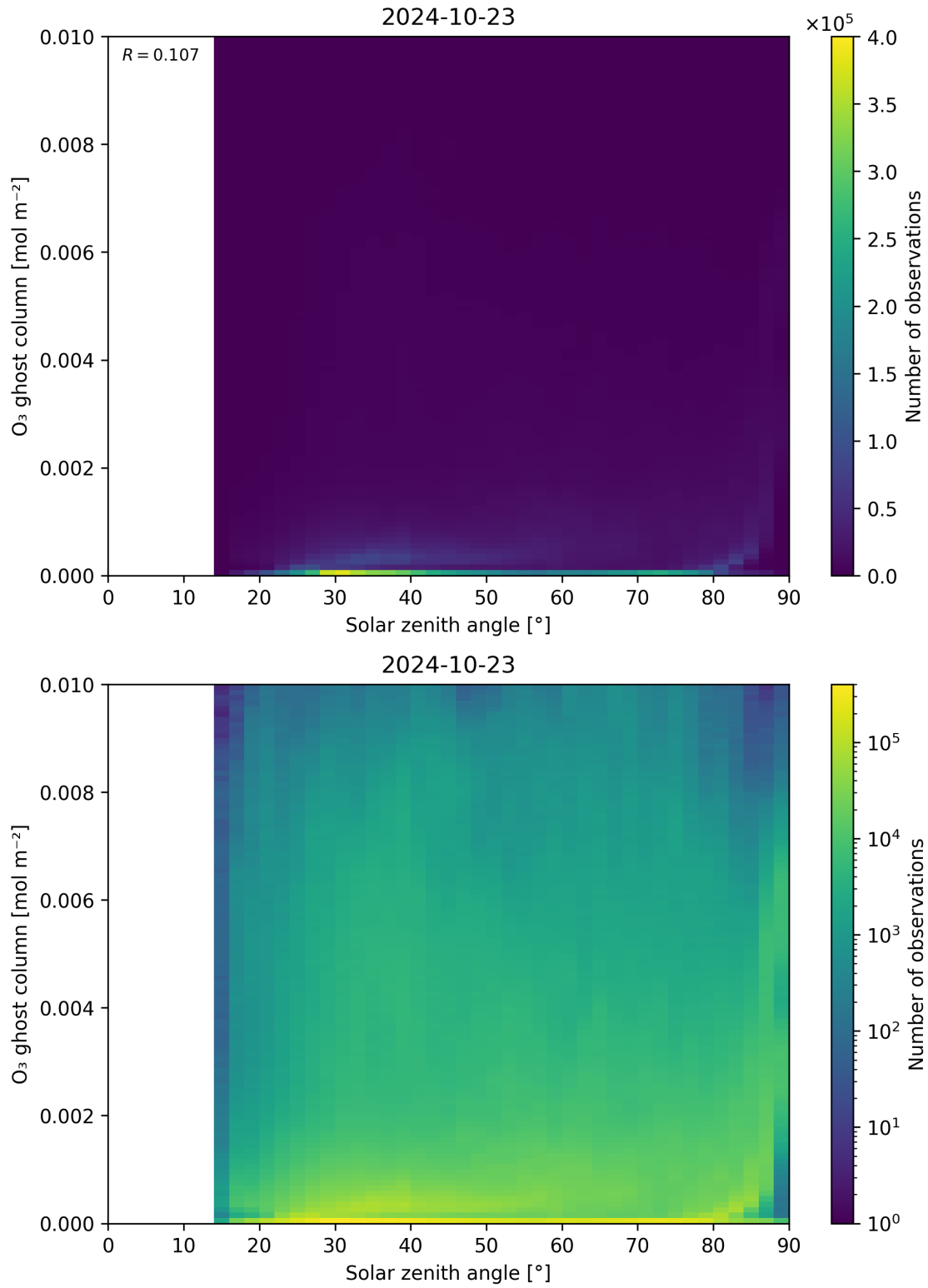
Figure 46: Scatter density plot of “Solar zenith angle” against “O 3 ghost column” for 2024-10-22 to 2024-10-24.
