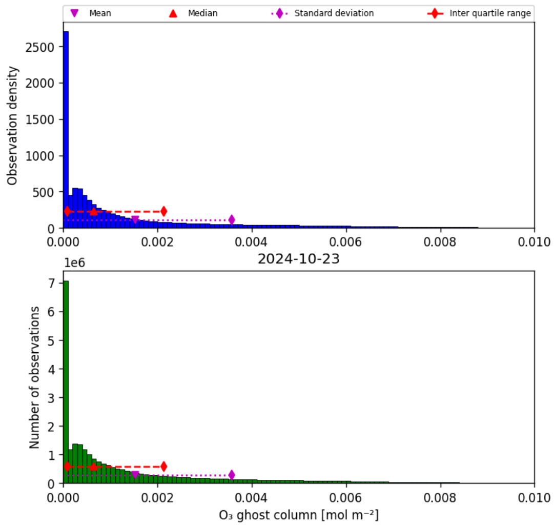
Figure 25: Histogram of “O 3 ghost column” for 2024-10-22 to 2024-10-24
