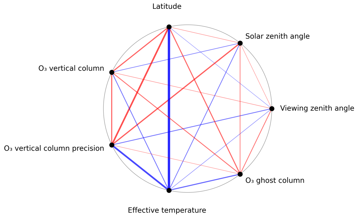
Figure 1: Map of correlation graph for 2024-10-22 to 2024-10-24.
