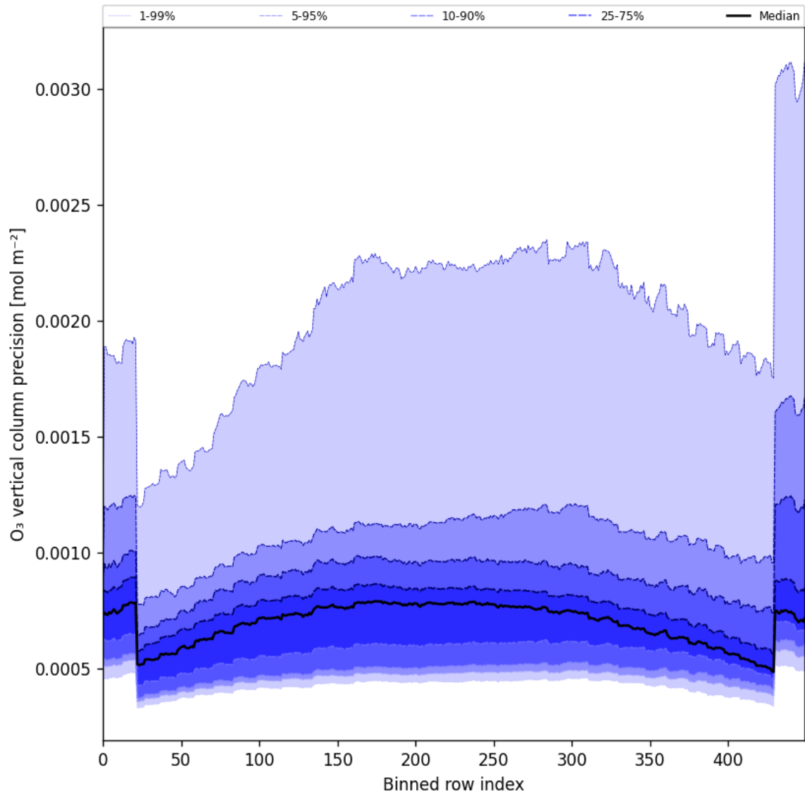
Figure 29: Along track statistics of “O 3 vertical column precision” for 2024-10-22 to 2024-10-24
