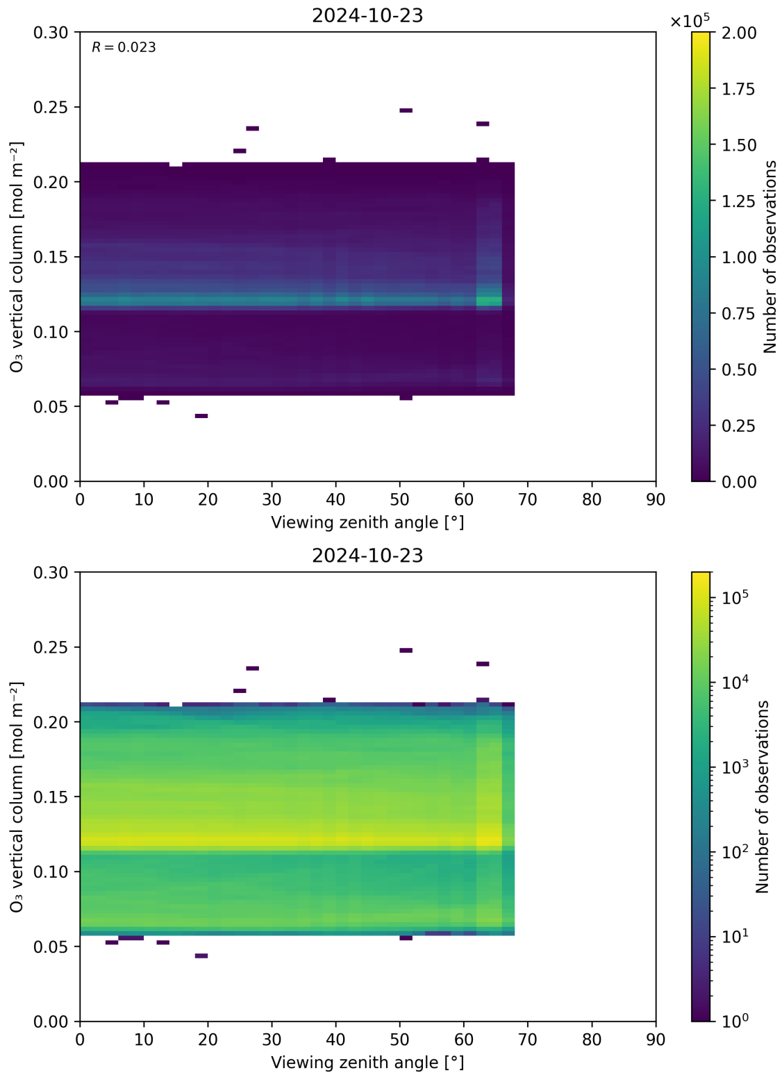
Figure 52: Scatter density plot of “Viewing zenith angle” against “O 3 vertical column” for 2024-10-22 to 2024-10-24.
