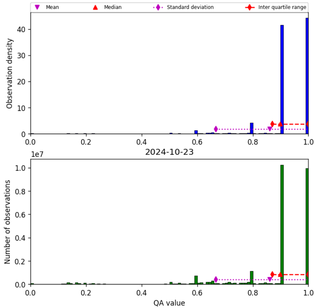
Figure 20: Histogram of “QA value” for 2024-10-22 to 2024-10-24
