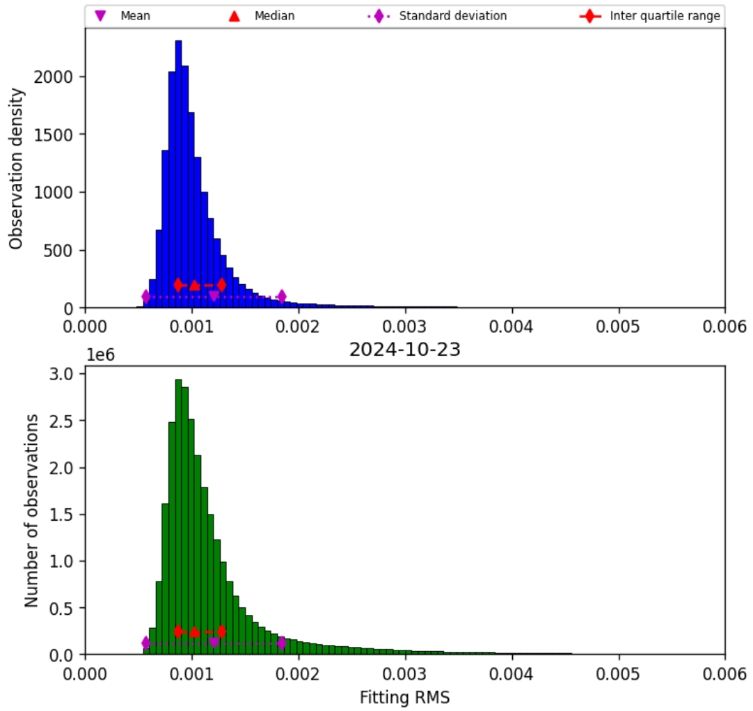
Figure 23: Histogram of “Fitting RMS” for 2024-10-22 to 2024-10-24
