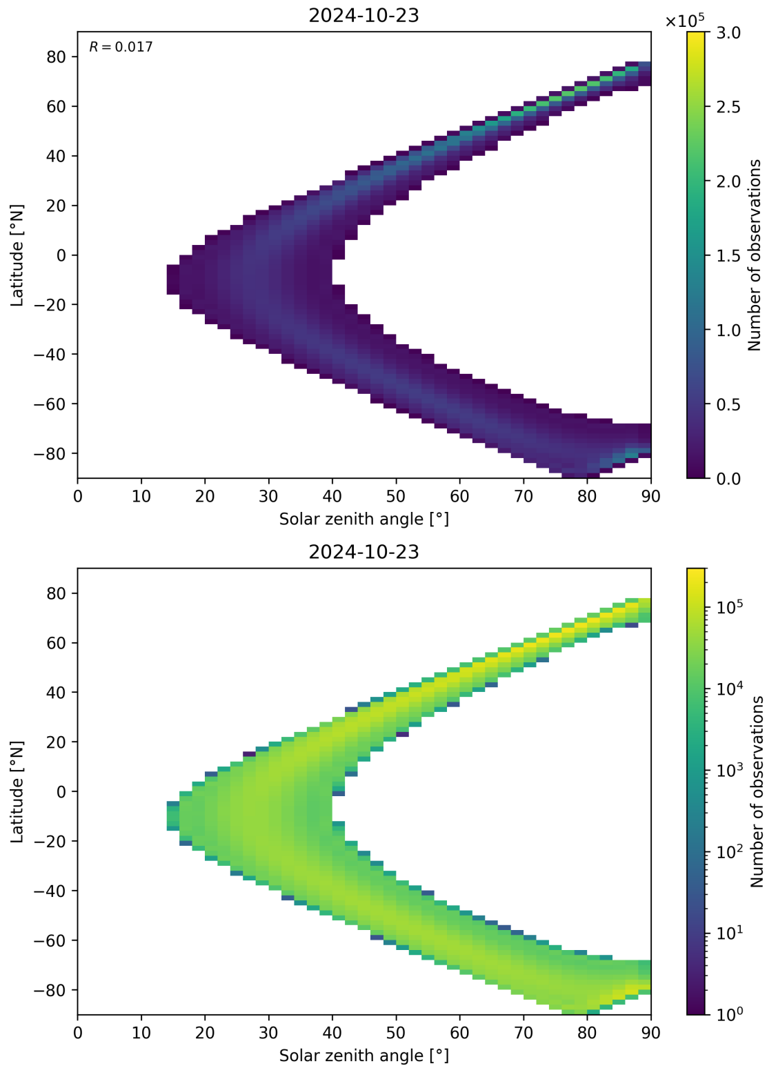
Figure 44: Scatter density plot of “Solar zenith angle” against “Latitude” for 2024-10-22 to 2024-10-24.
