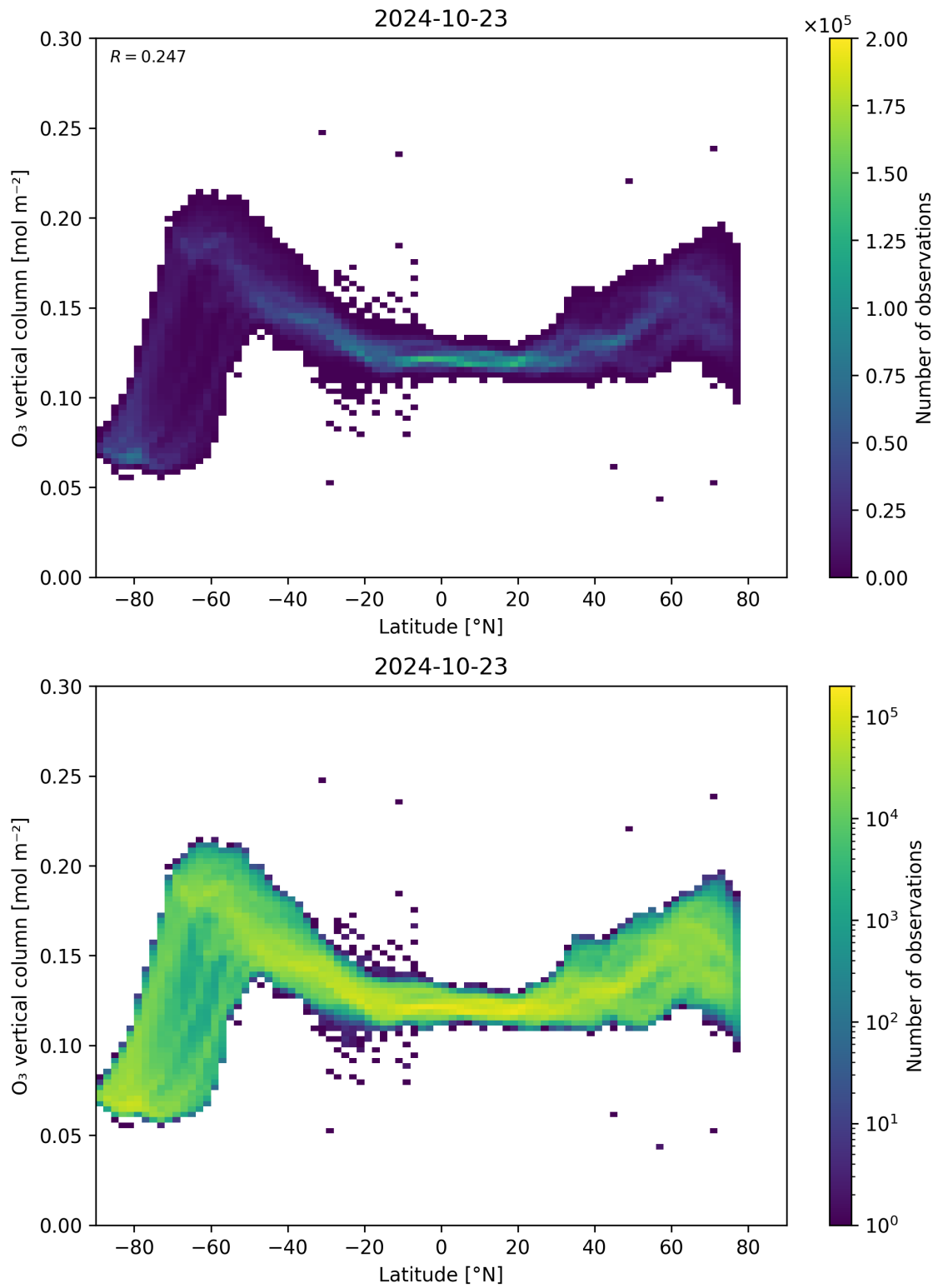
Figure 36: Scatter density plot of “Latitude” against “O 3 vertical column” for 2024-10-22 to 2024-10-24.
