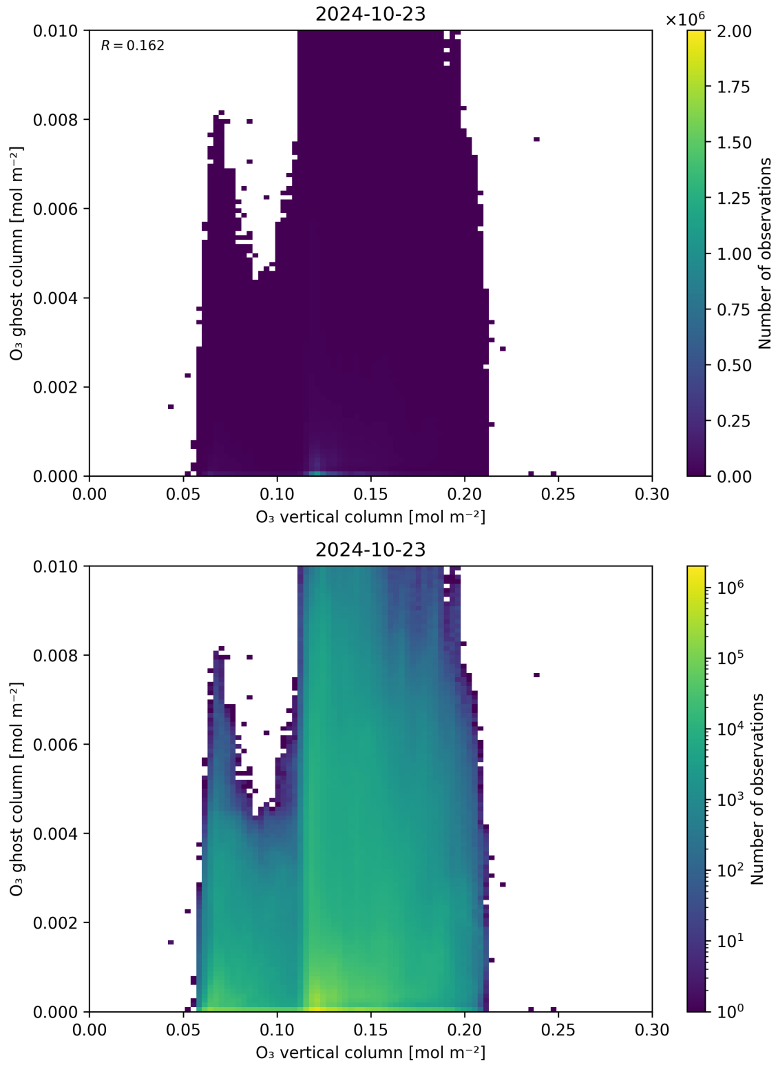
Figure 40: Scatter density plot of “O 3 vertical column” against “O 3 ghost column” for 2024-10-22 to 2024-10-24.
