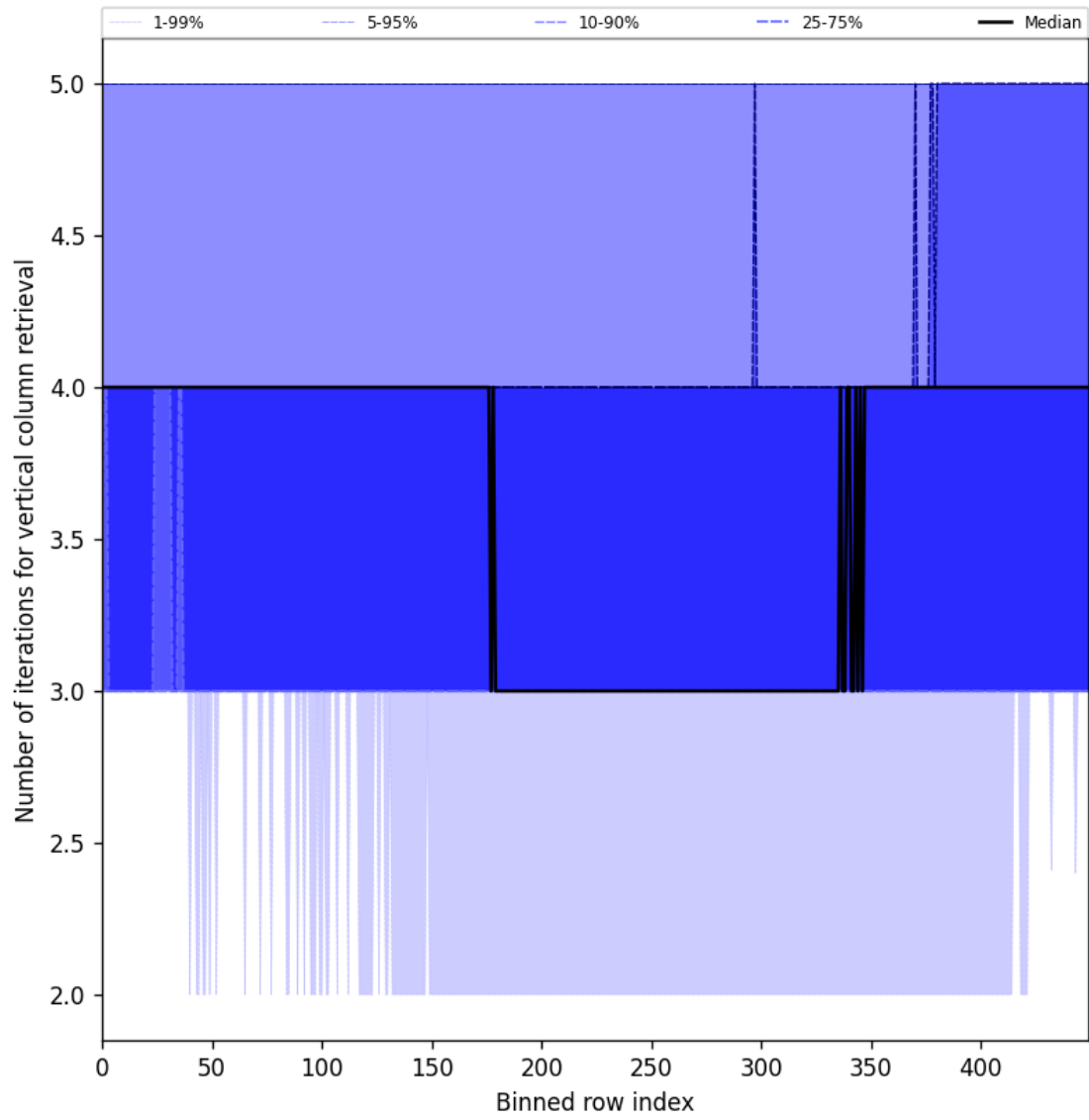
Figure 33: Along track statistics of “Number of iterations for vertical column retrieval” for 2024-10-22 to 2024-10-24
