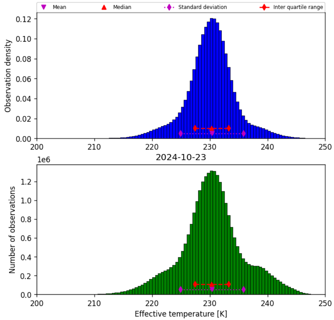
Figure 24: Histogram of “Effective temperature” for 2024-10-22 to 2024-10-24
