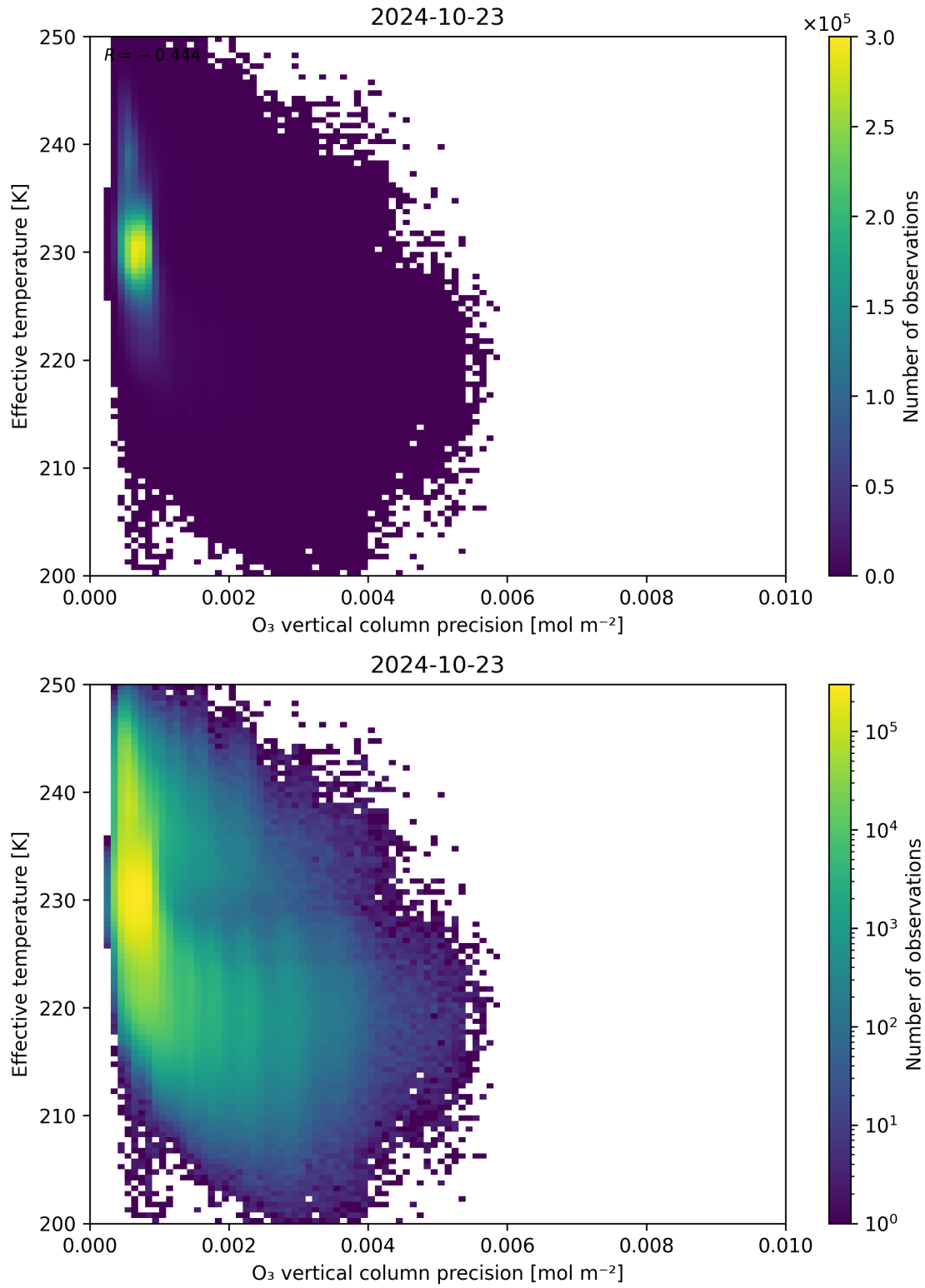
Figure 42: Scatter density plot of “ O_3 vertical column precision” against “Effective temperature” for 2024-10-22 to 2024-10-24.
