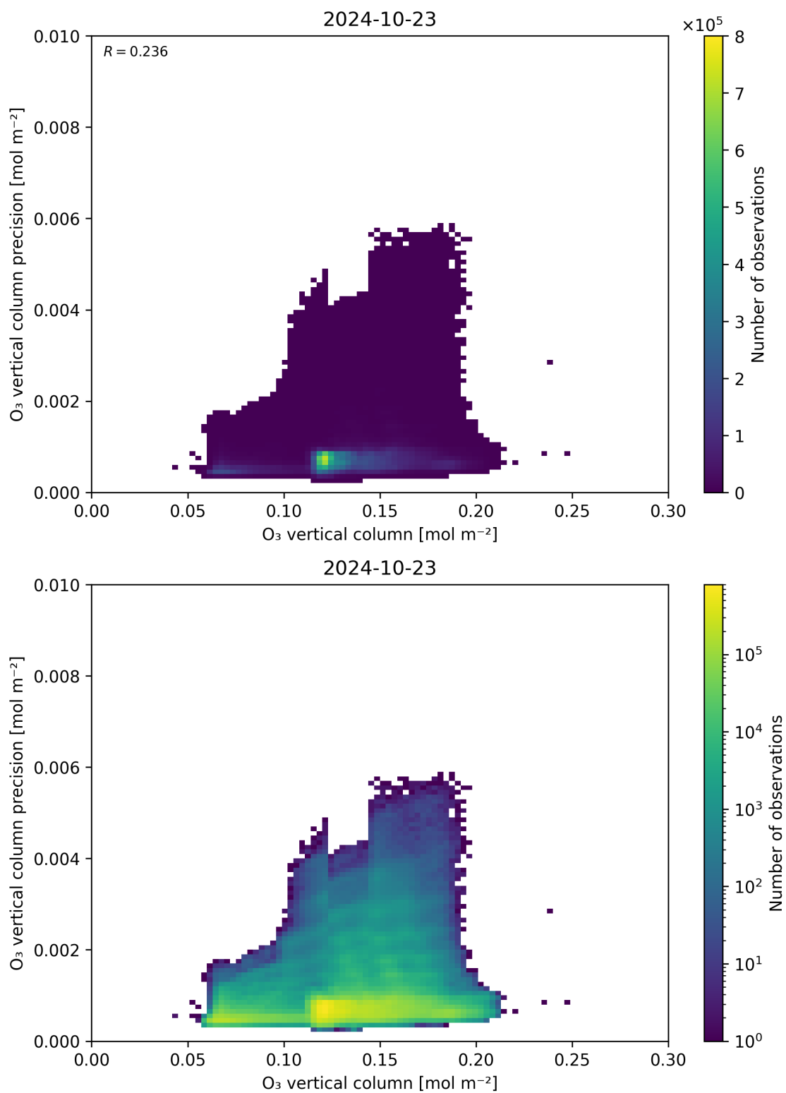
Figure 41: Scatter density plot of “O 3 vertical column” against “O 3 vertical column precision” for 2024-10-22 to 2024-10-24.
