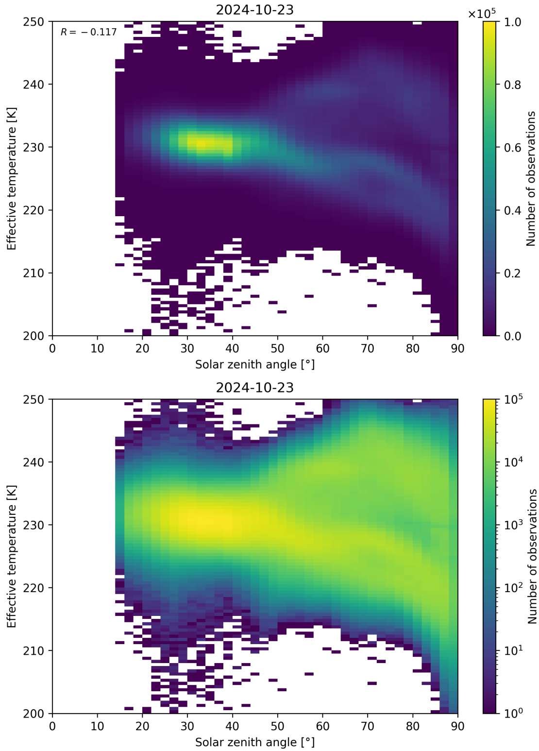
Figure 45: Scatter density plot of “Solar zenith angle” against “Effective temperature” for 2024-10-22 to 2024-10-24.
