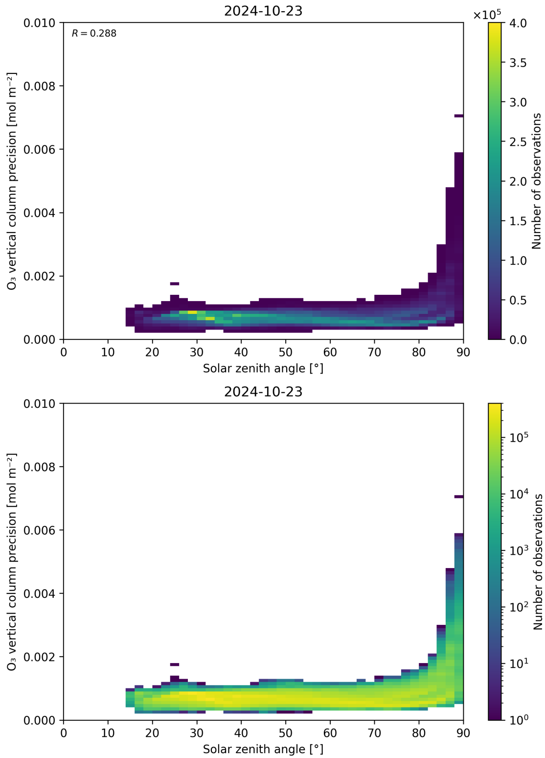
Figure 48: Scatter density plot of “Solar zenith angle” against “O 3 vertical column precision” for 2024-10-22 to 2024-10-24.
