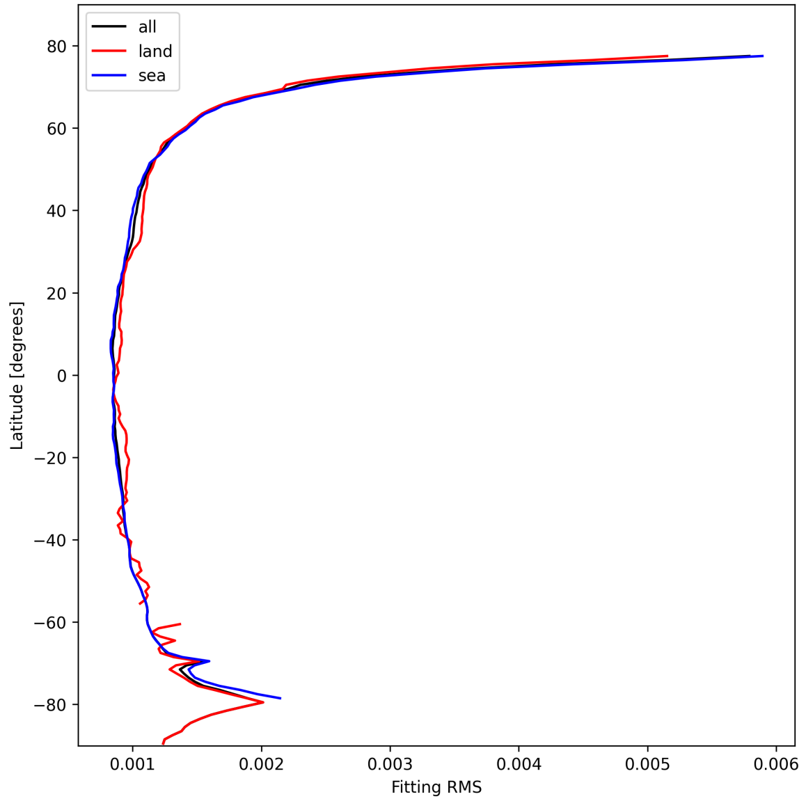
Figure 16: Zonal average of “Fitting RMS” for 2024-10-22 to 2024-10-24.
