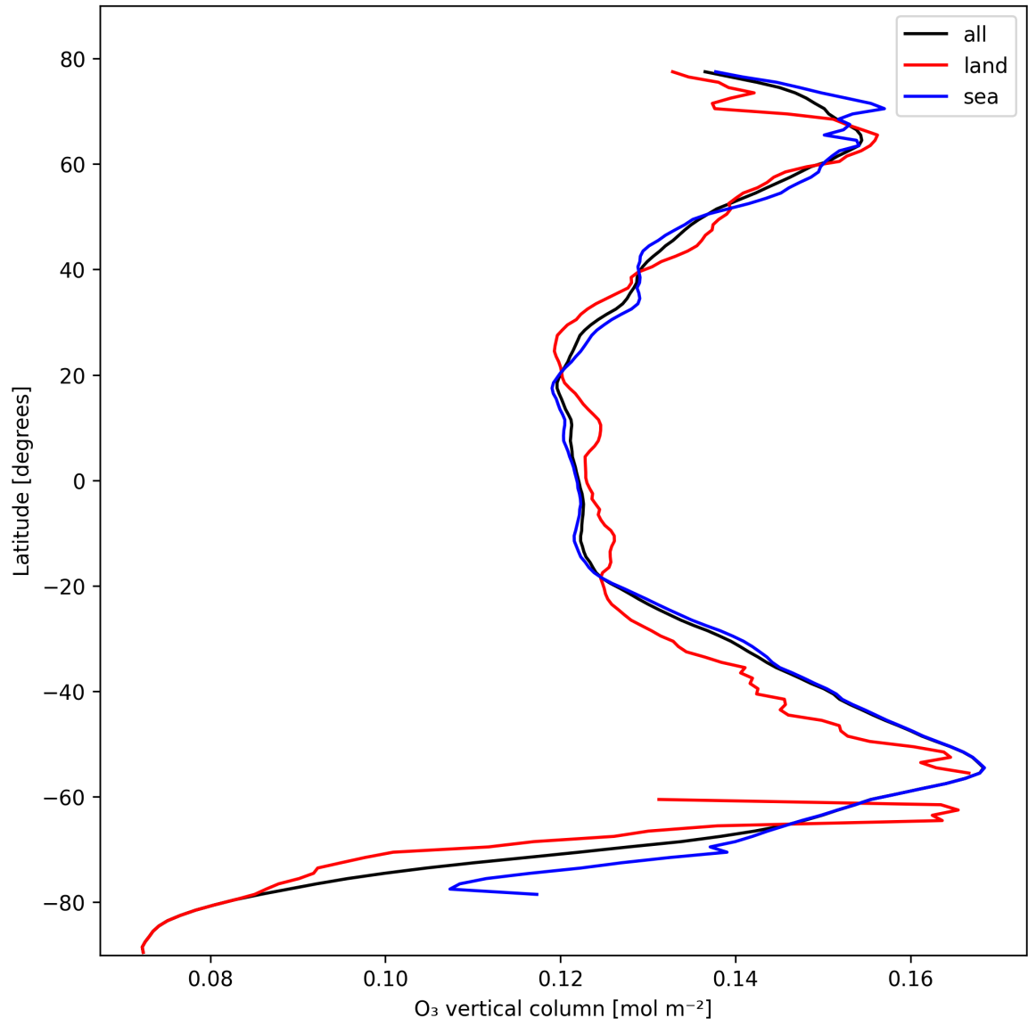
Figure 14: Zonal average of “O 3 vertical column” for 2024-10-22 to 2024-10-24.
