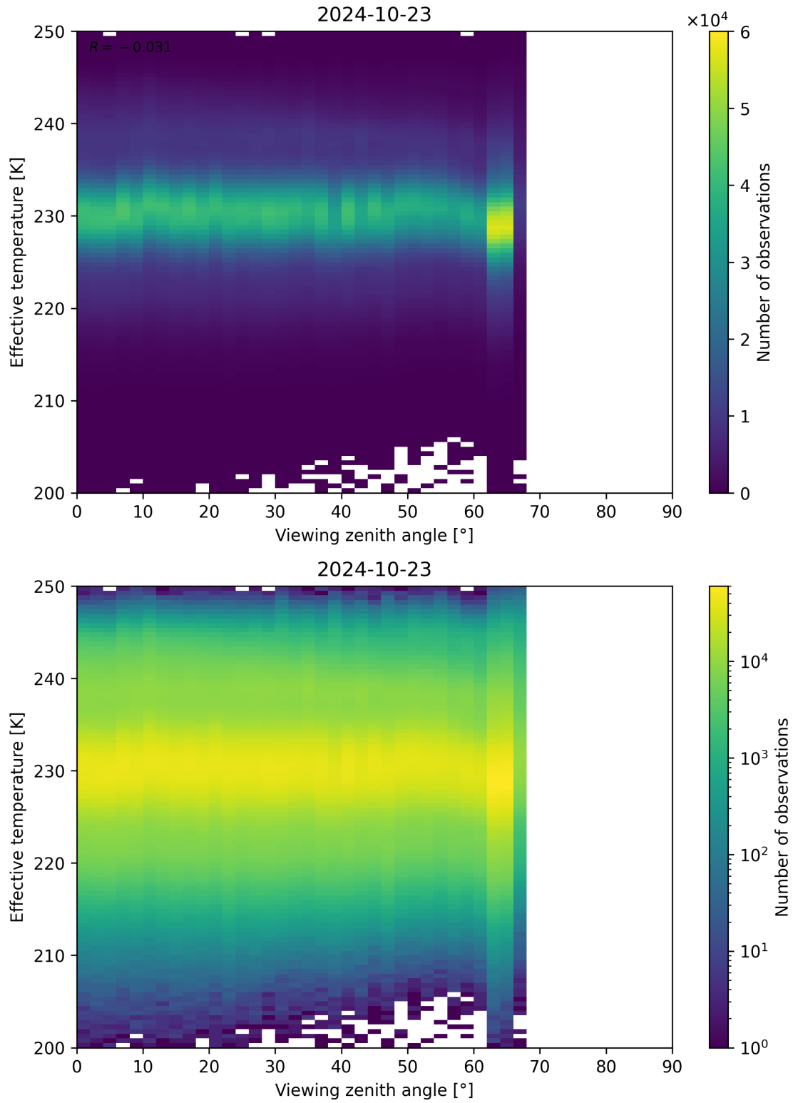
Figure 50: Scatter density plot of “Viewing zenith angle” against “Effective temperature” for 2024-10-22 to 2024-10-24.
