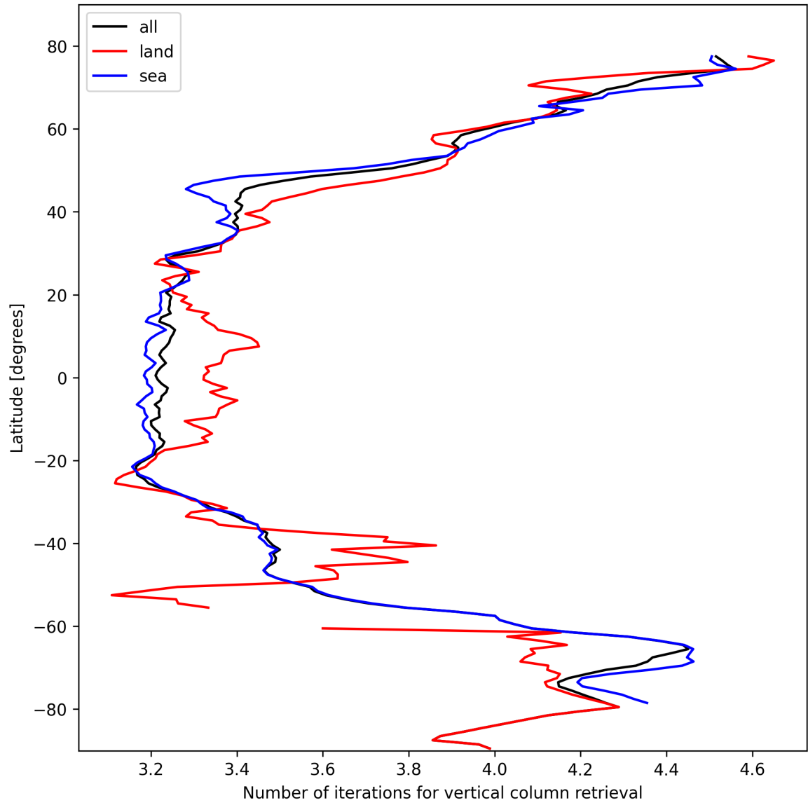
Figure 19: Zonal average of “Number of iterations for vertical column retrieval” for 2024-10-22 to 2024-10-24.
