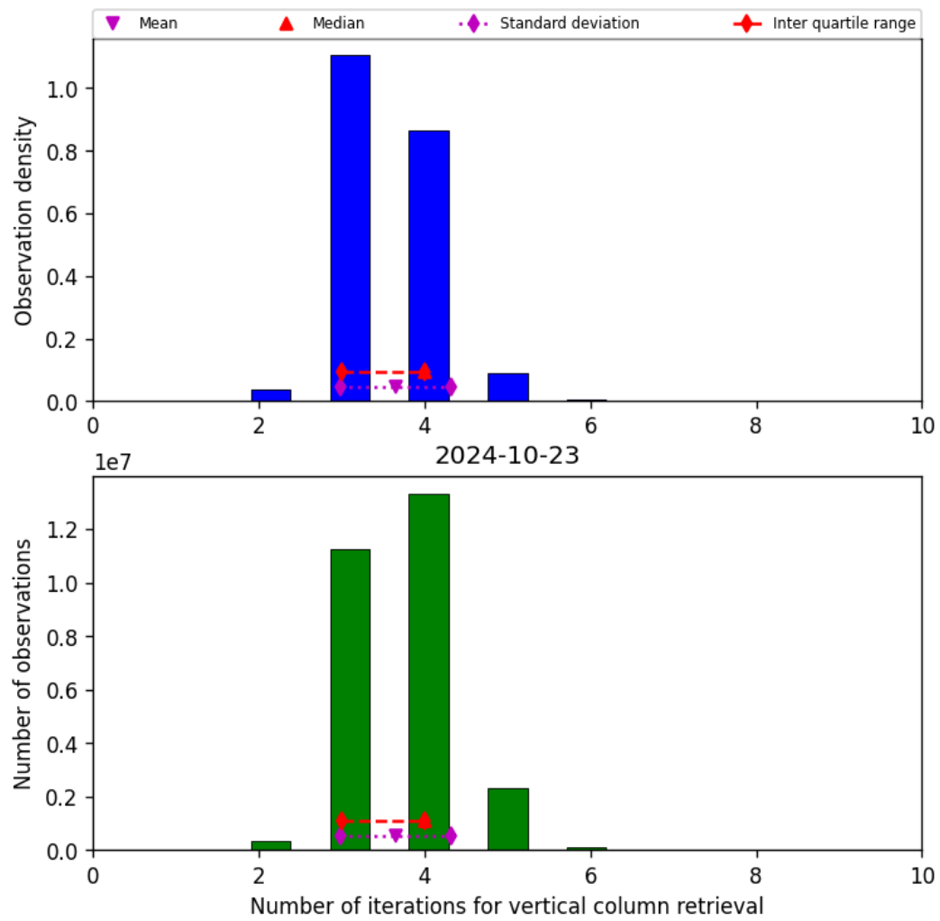
Figure 26: Histogram of “Number of iterations for vertical column retrieval” for 2024-10-22 to 2024-10-24
