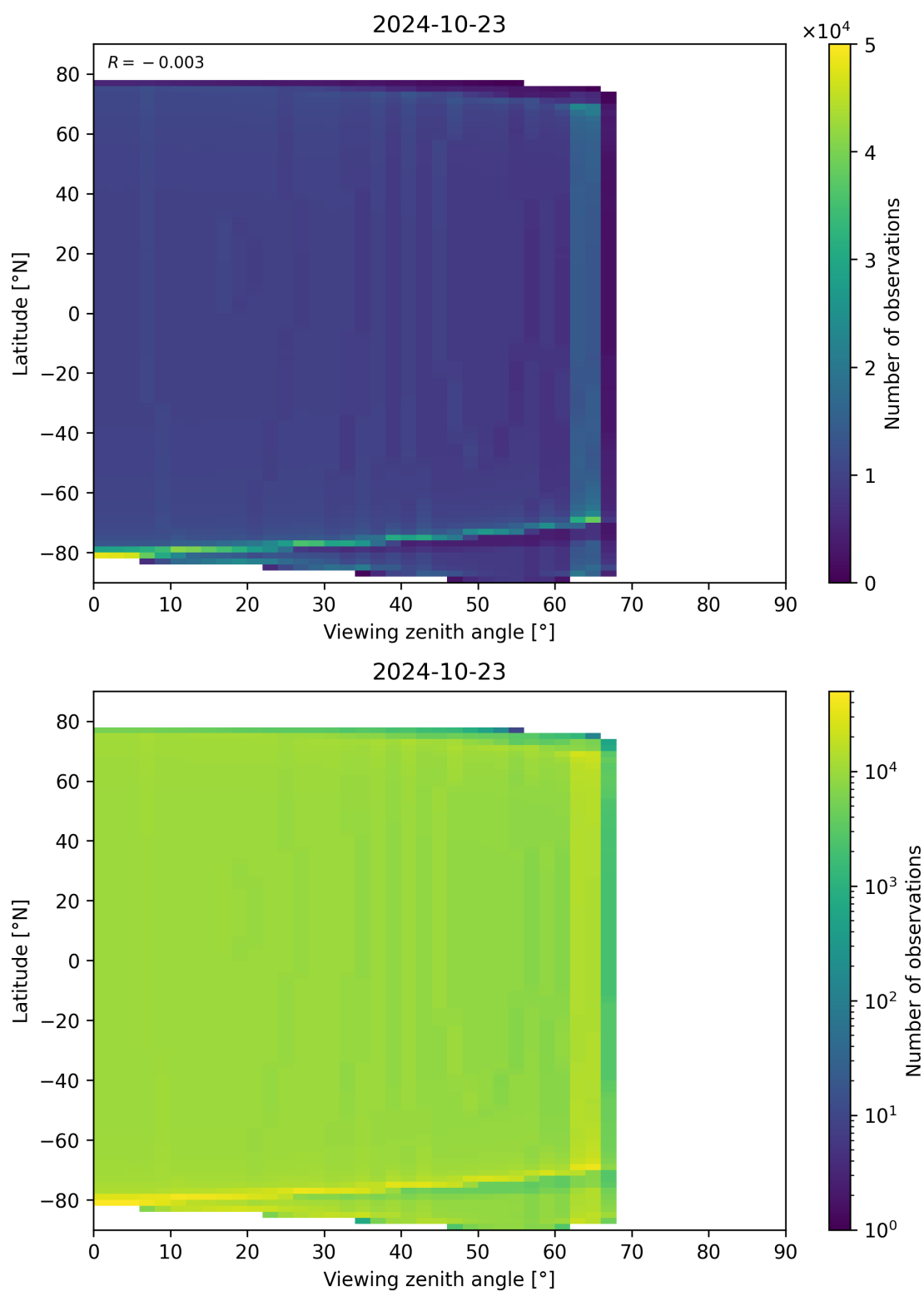
Figure 49: Scatter density plot of “Viewing zenith angle” against “Latitude” for 2024-10-22 to 2024-10-24.
