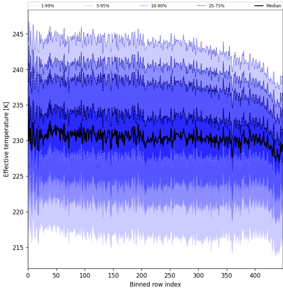
Figure 31: Along track statistics of “Effective temperature” for 2024-10-22 to 2024-10-24
