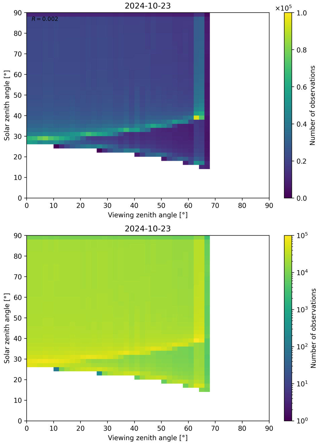
Figure 54: Scatter density plot of “Viewing zenith angle” against “Solar zenith angle” for 2024-10-22 to 2024-10-24.
