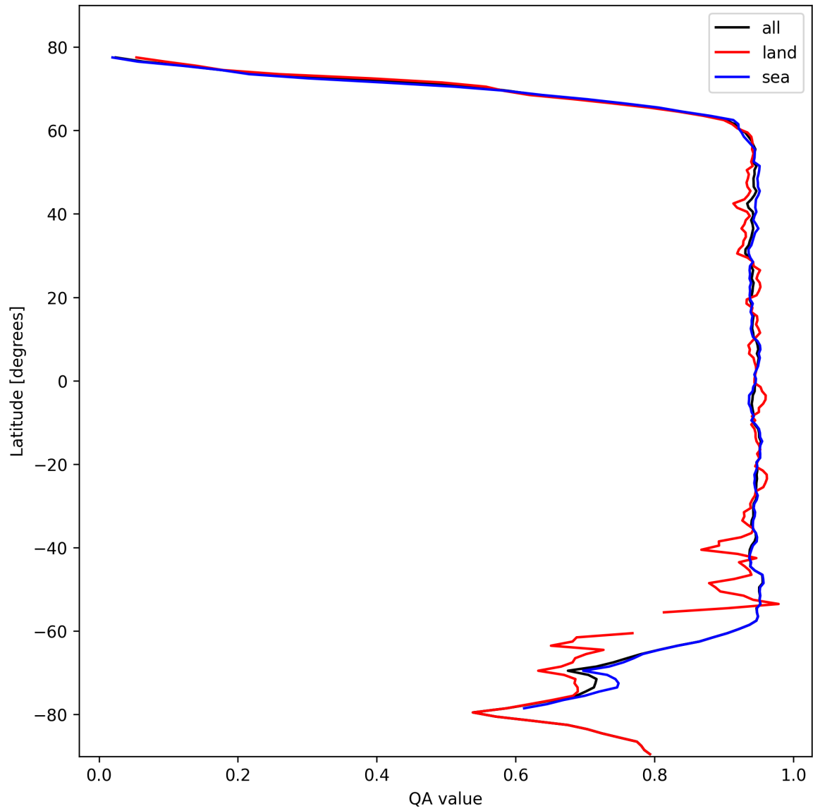
Figure 13: Zonal average of “QA value” for 2024-10-22 to 2024-10-24.
