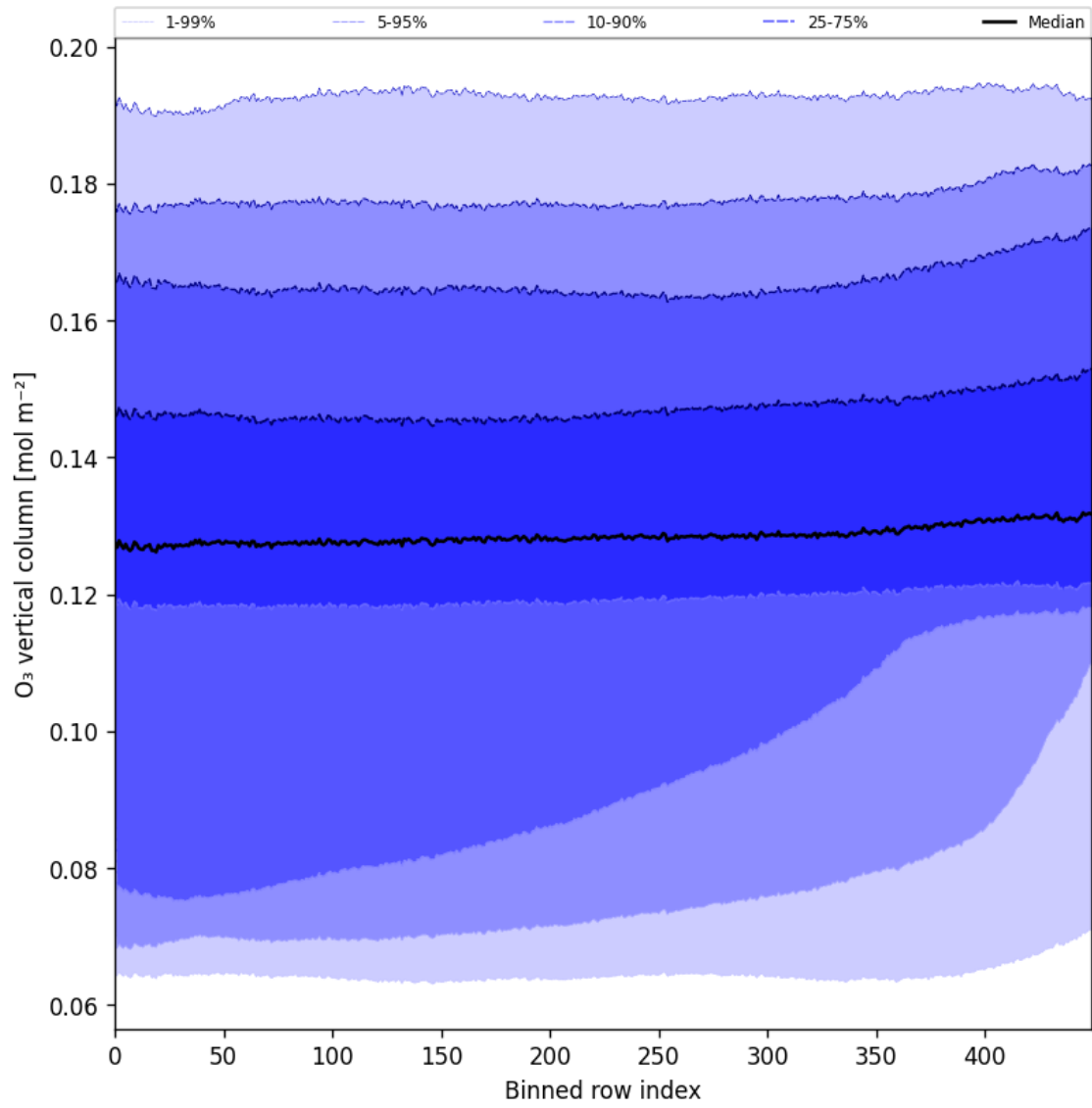
Figure 28: Along track statistics of “O 3 vertical column” for 2024-10-22 to 2024-10-24
