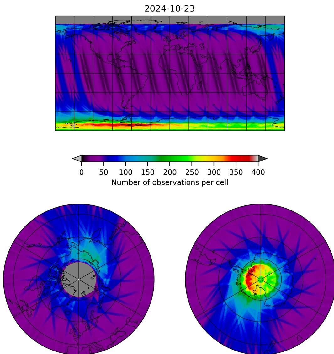
Figure 12: Map of the number of observations for 2024-10-22 to 2024-10-24
