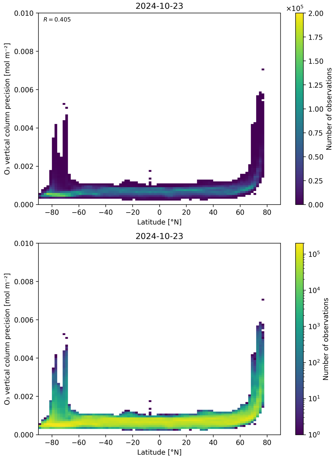
Figure 37: Scatter density plot of “Latitude” against “O 3 vertical column precision” for 2024-10-22 to 2024-10-24.
