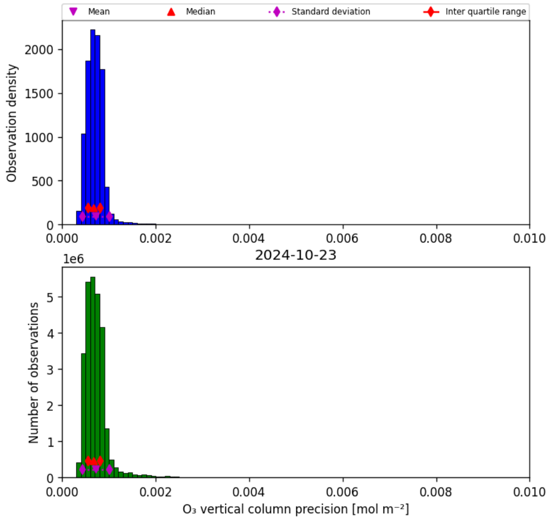
Figure 22: Histogram of “O 3 vertical column precision” for 2024-10-22 to 2024-10-24
