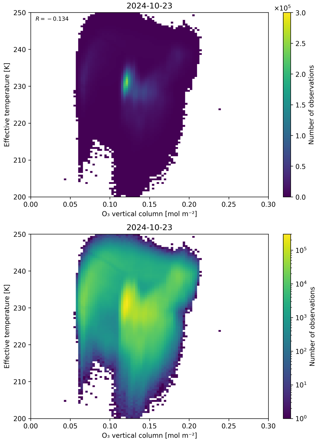
Figure 39: Scatter density plot of “O 3 vertical column” against “Effective temperature” for 2024-10-22 to 2024-10-24.
