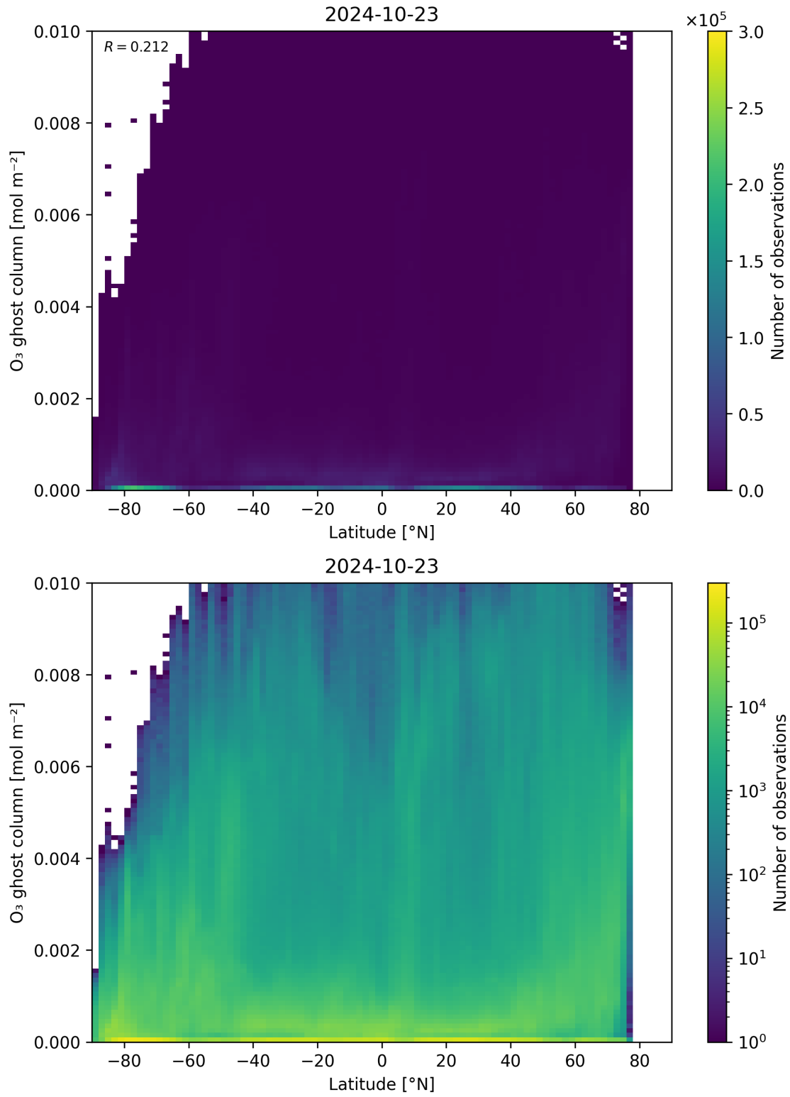
Figure 35: Scatter density plot of “Latitude” against “O 3 ghost column” for 2024-10-22 to 2024-10-24.
