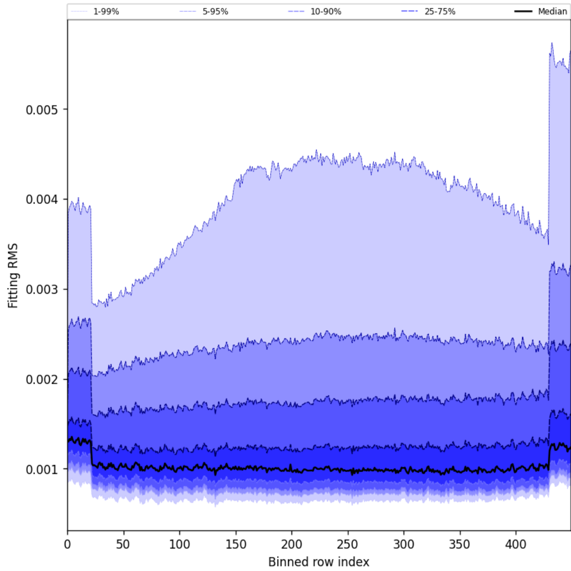
Figure 30: Along track statistics of “Fitting RMS” for 2024-10-22 to 2024-10-24
