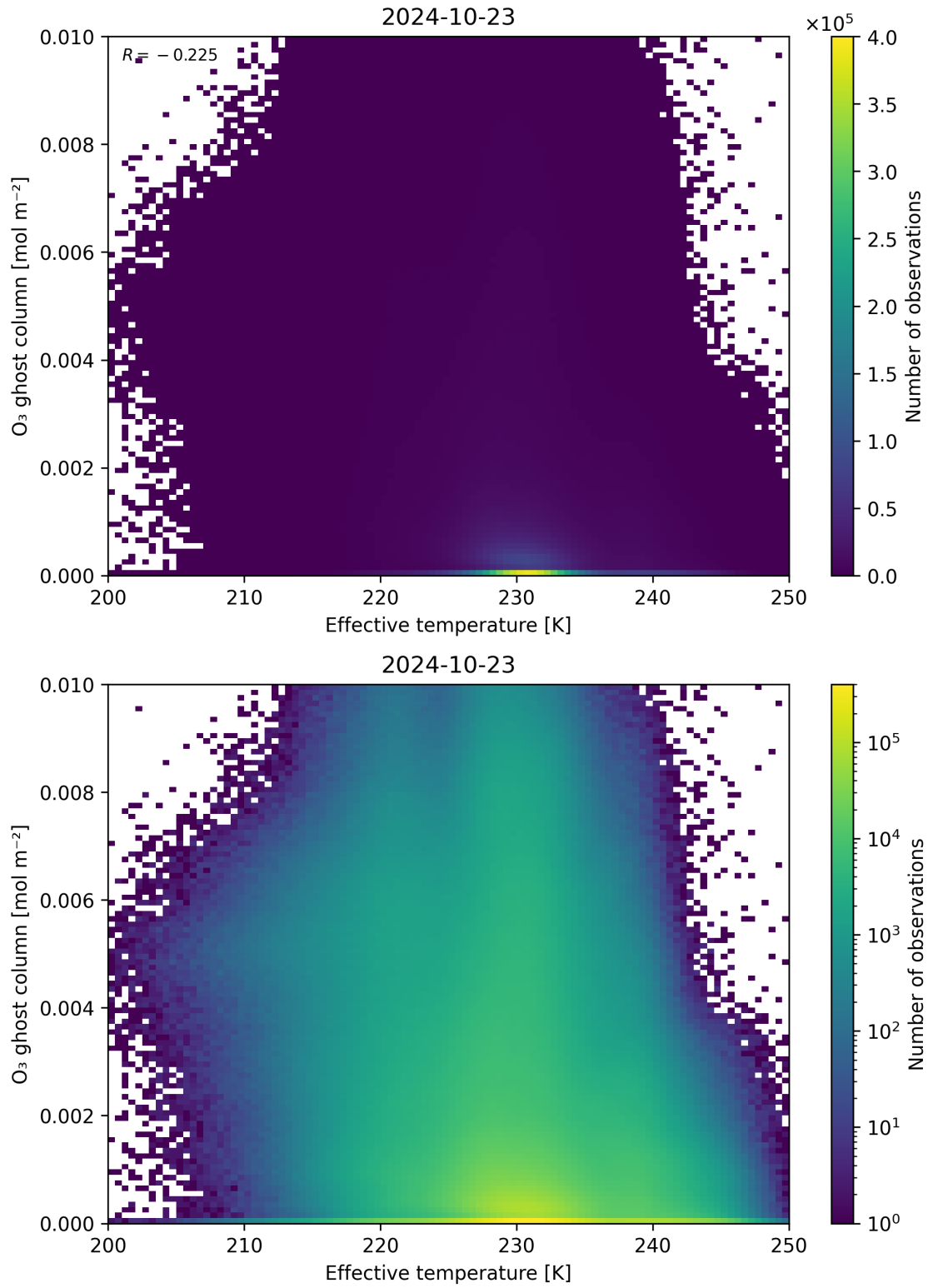
Figure 38: Scatter density plot of “Effective temperature” against “O 3 ghost column” for 2024-10-22 to 2024-10-24.
