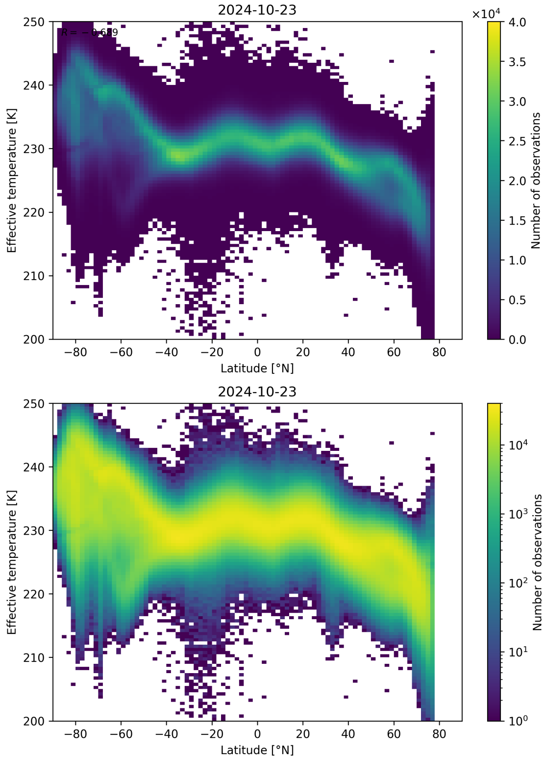
Figure 34: Scatter density plot of “Latitude” against “Effective temperature” for 2024-10-22 to 2024-10-24.
