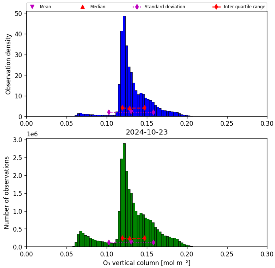
Figure 21: Histogram of “O 3 vertical column” for 2024-10-22 to 2024-10-24
