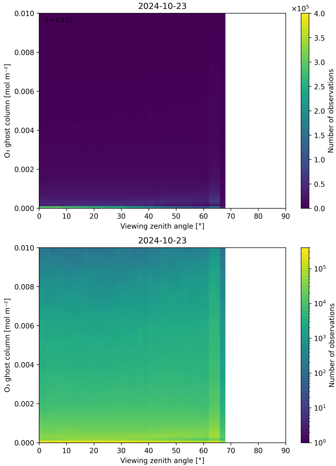
Figure 51: Scatter density plot of “Viewing zenith angle” against “O 3 ghost column” for 2024-10-22 to 2024-10-24.
