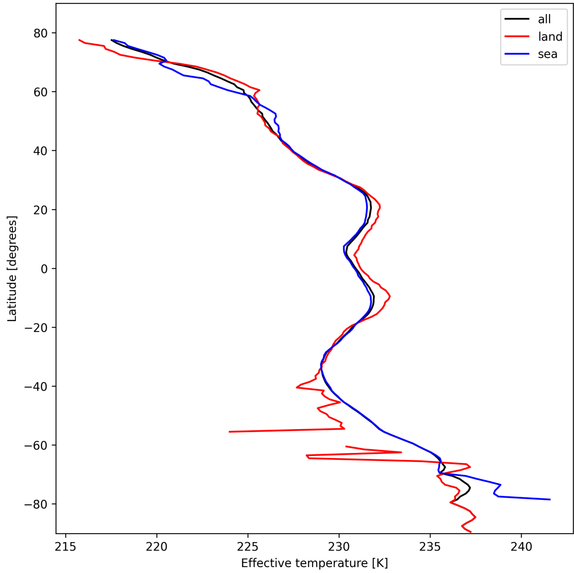
Figure 17: Zonal average of “Effective temperature” for 2024-10-22 to 2024-10-24.
