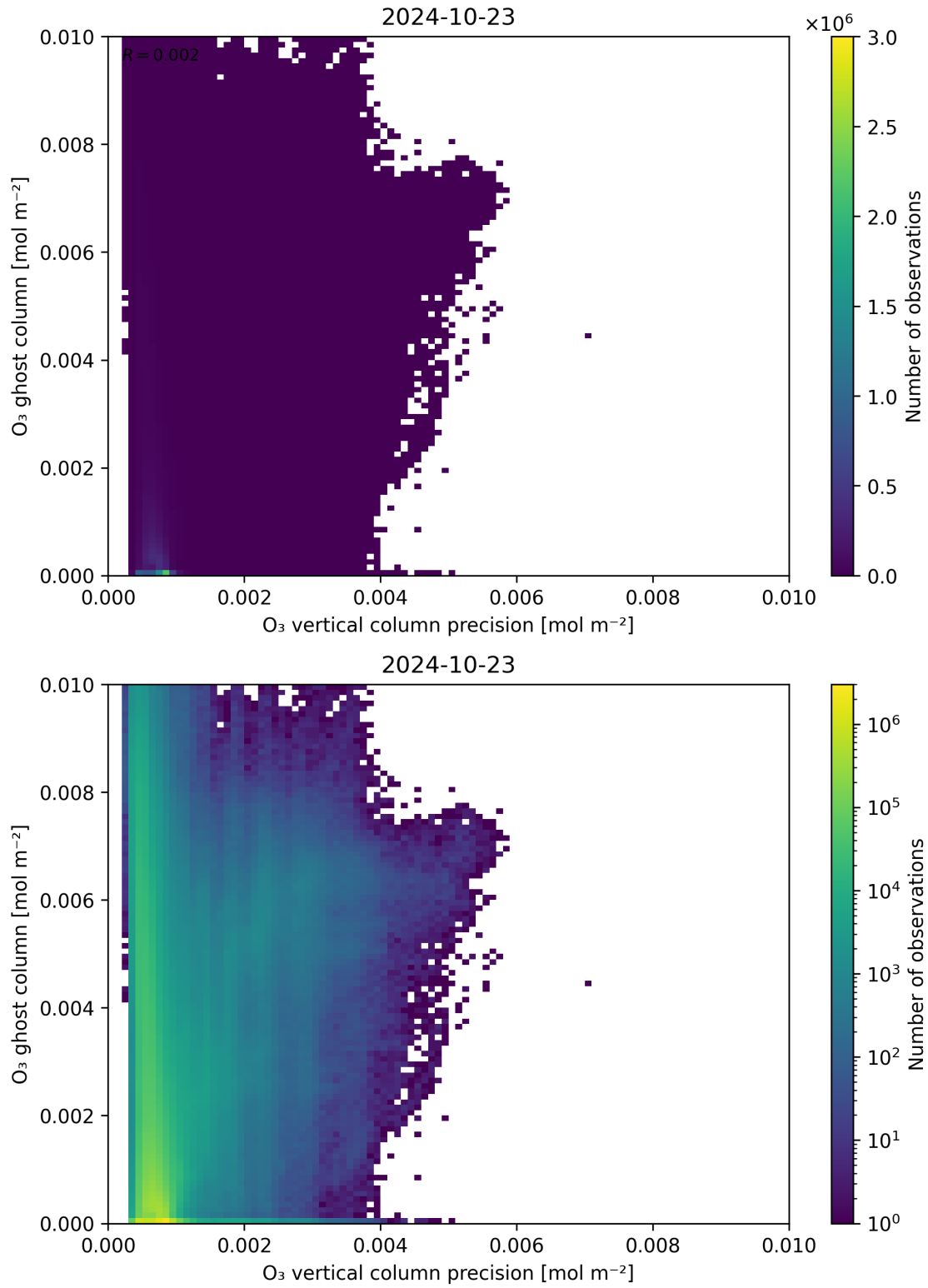
Figure 43: Scatter density plot of “ \text{O}_3 vertical column precision” against “ \text{O}_3 ghost column” for 2024-10-22 to 2024-10-24.
