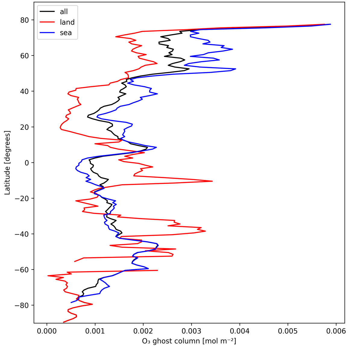
Figure 18: Zonal average of “O 3 ghost column” for 2024-10-22 to 2024-10-24.
