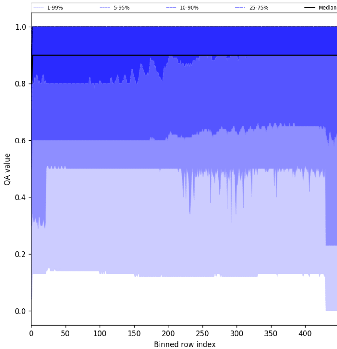
Figure 27: Along track statistics of “QA value” for 2024-10-22 to 2024-10-24
