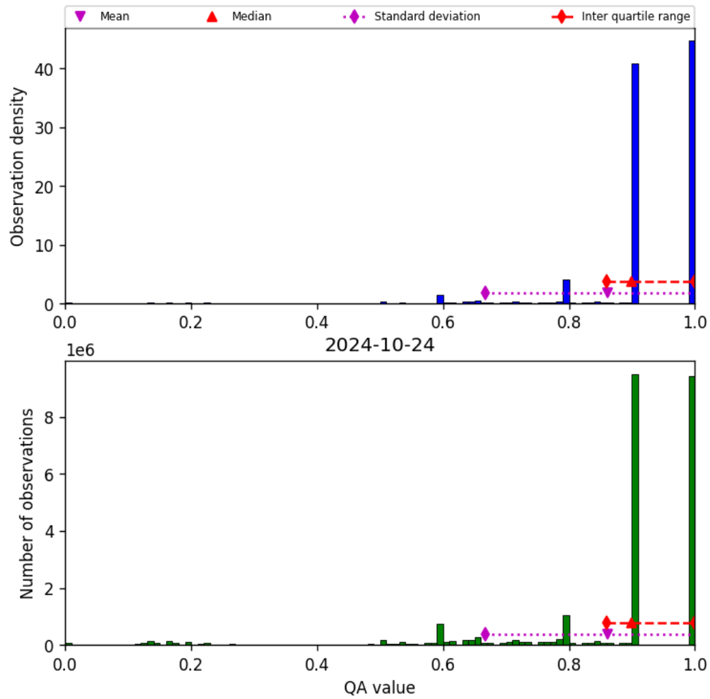
Figure 20: Histogram of “QA value” for 2024-10-24 to 2024-10-25
