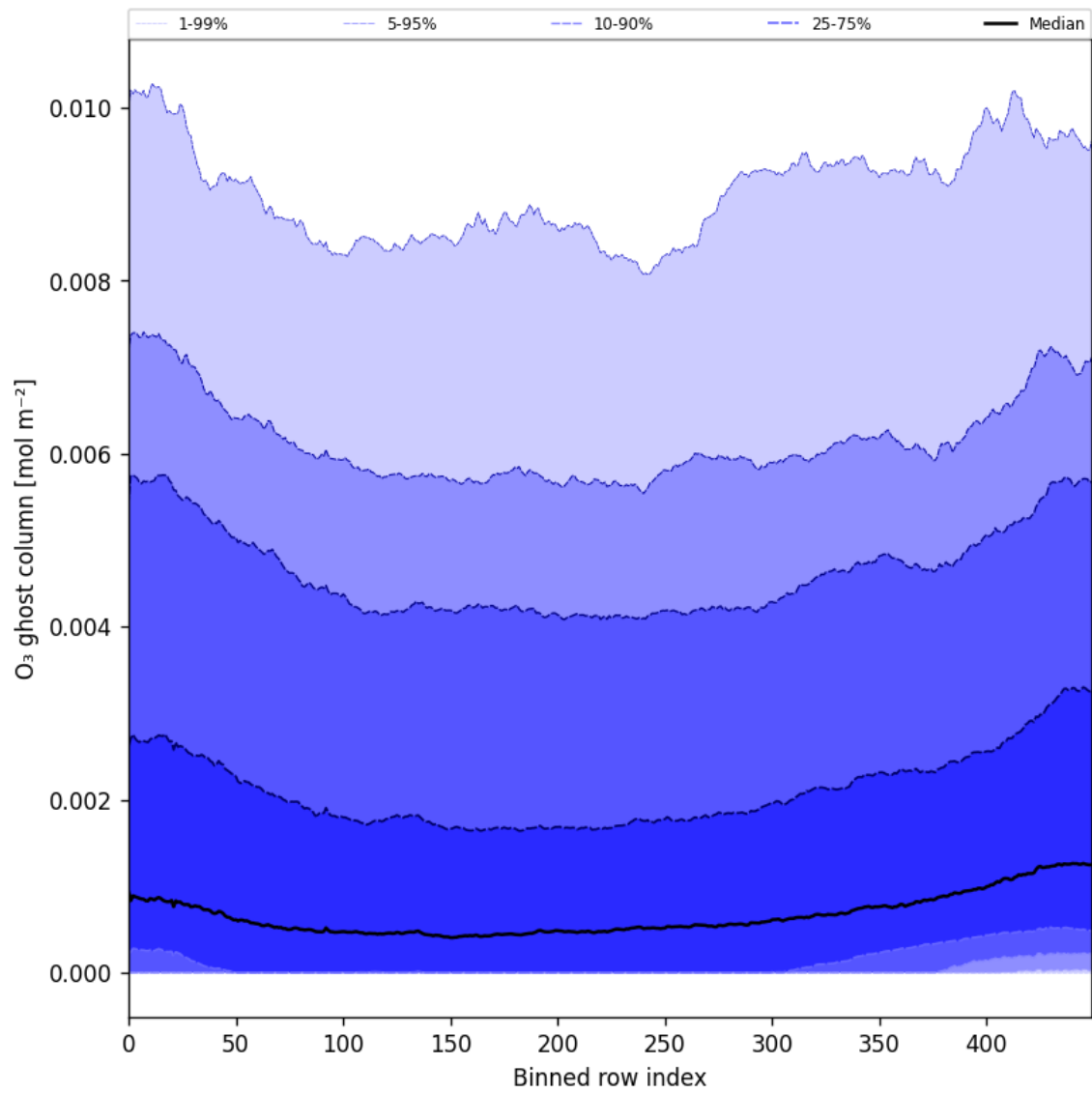
Figure 32: Along track statistics of “O 3 ghost column” for 2024-10-24 to 2024-10-25
