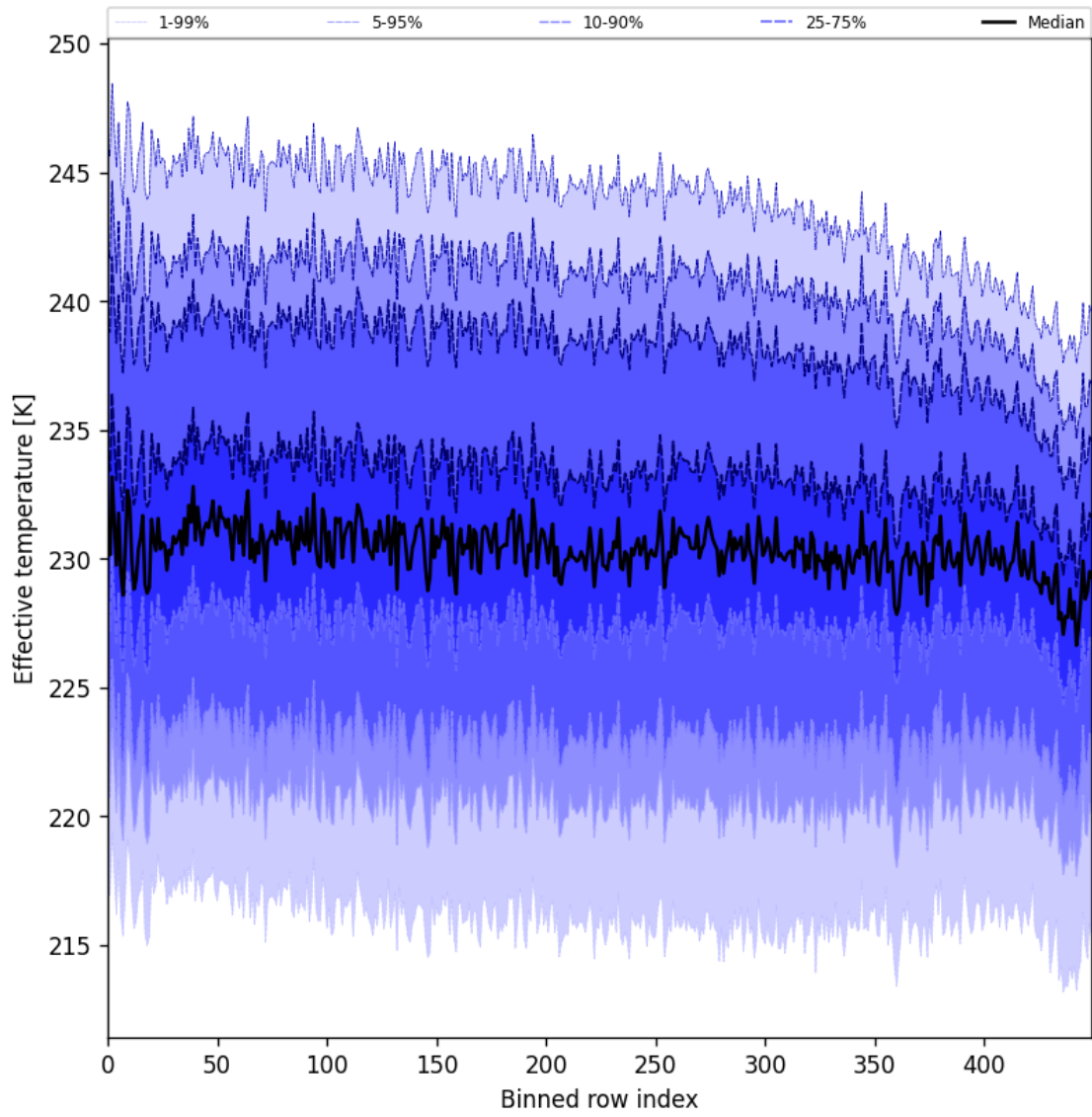
Figure 31: Along track statistics of “Effective temperature” for 2024-10-24 to 2024-10-25
