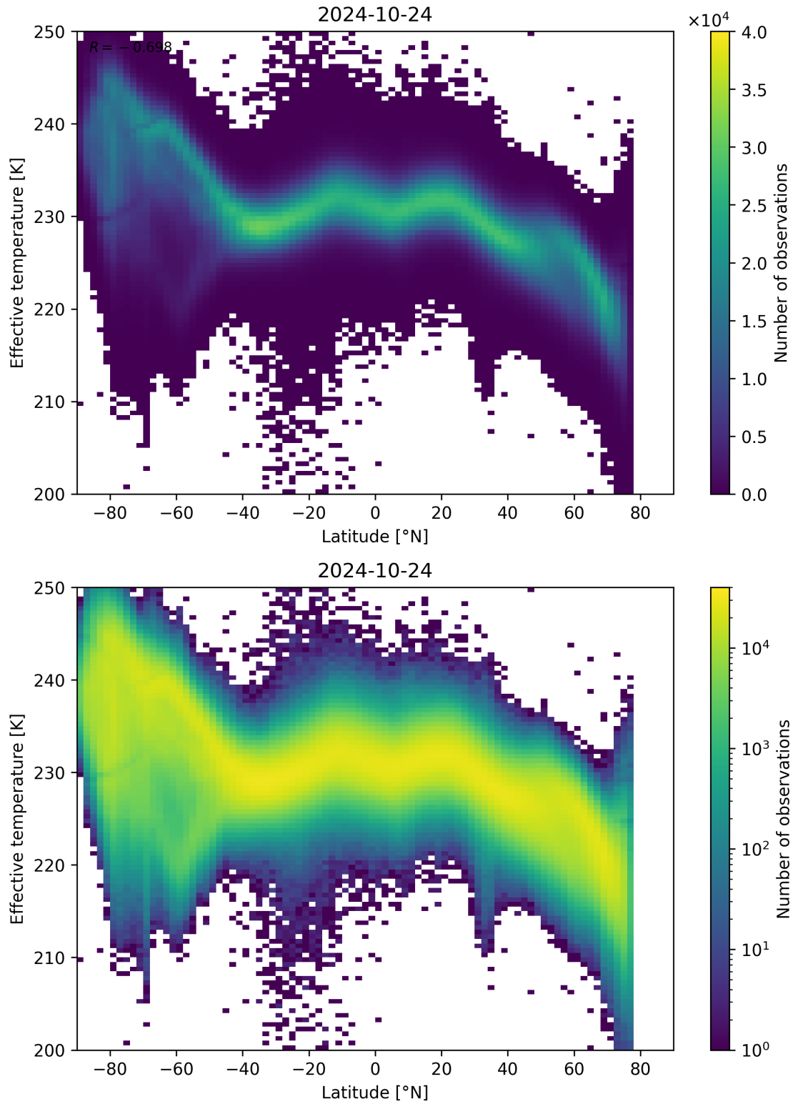
Figure 34: Scatter density plot of “Latitude” against “Effective temperature” for 2024-10-24 to 2024-10-25.
