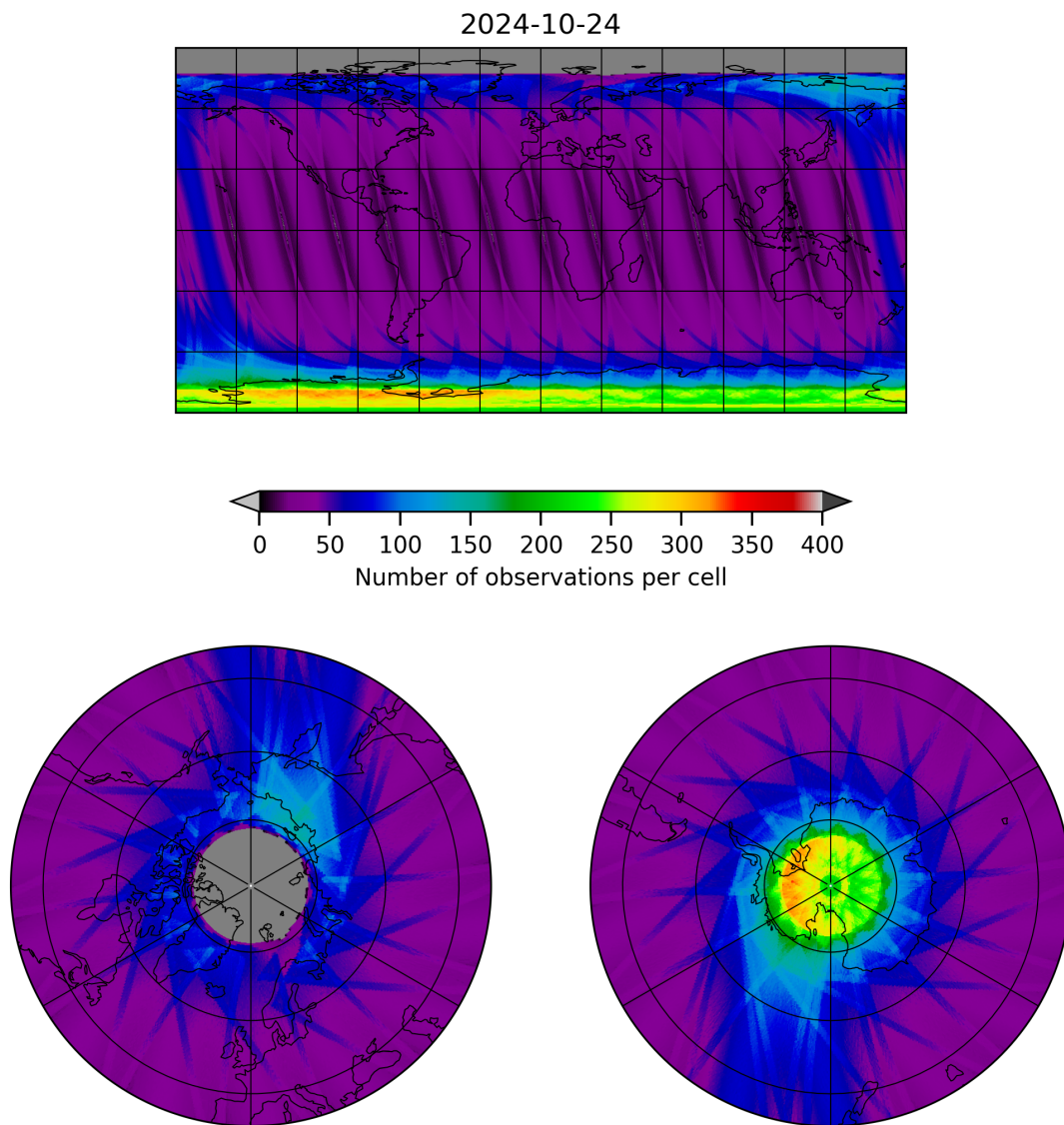
Figure 12: Map of the number of observations for 2024-10-24 to 2024-10-25
