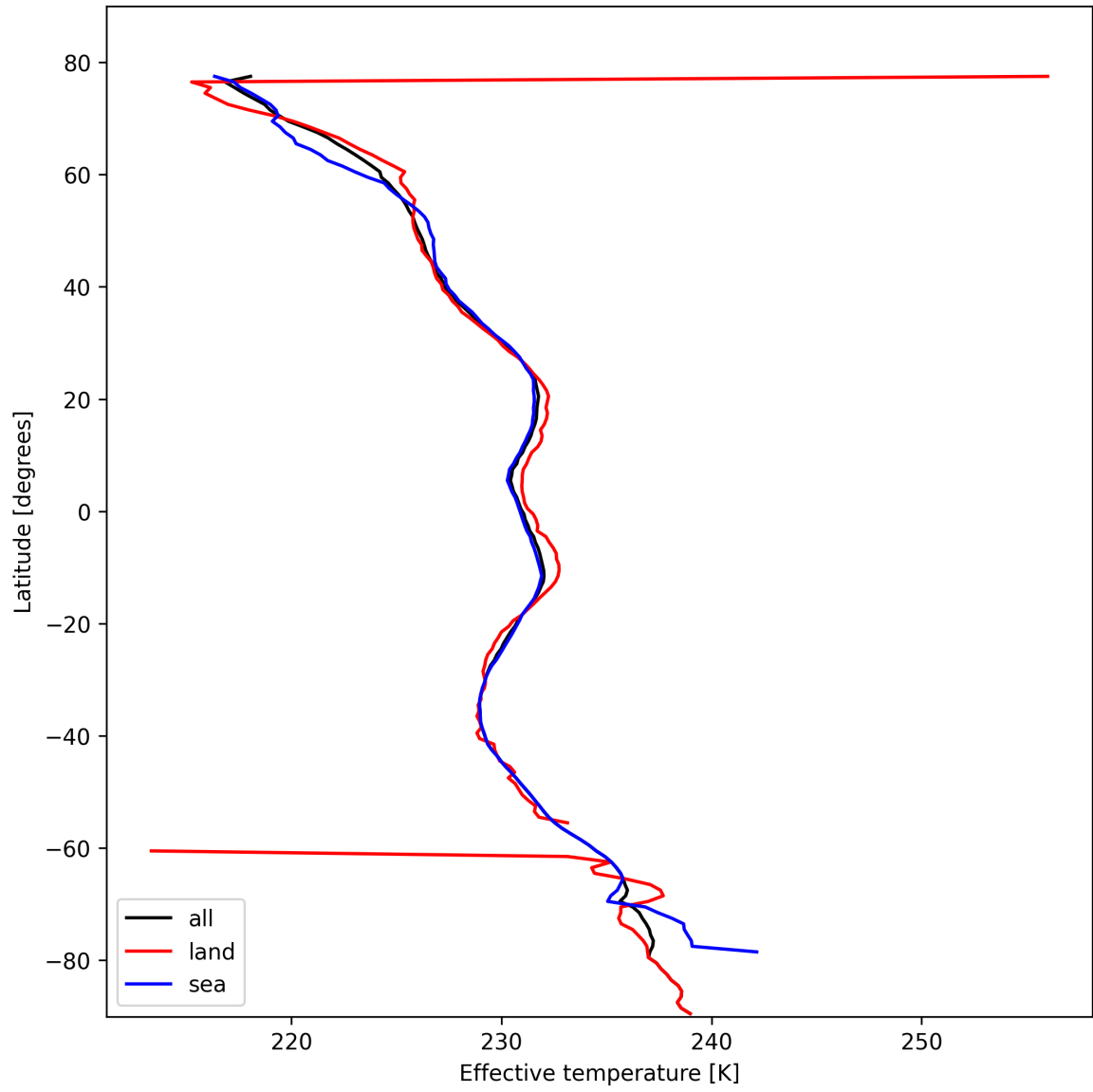
Figure 17: Zonal average of "Effective temperature" for 2024-10-24 to 2024-10-25.
