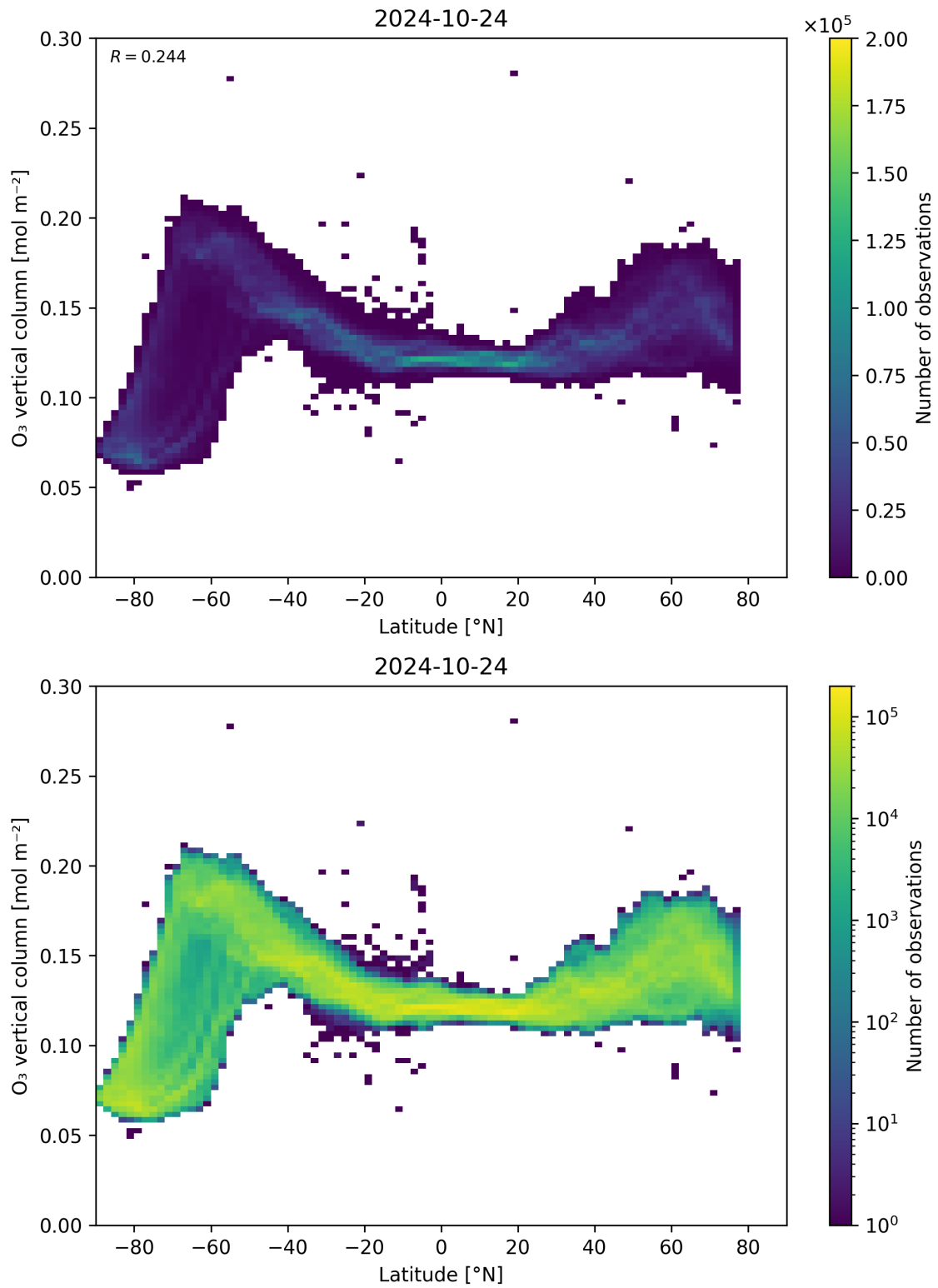
Figure 36: Scatter density plot of “Latitude” against “O 3 vertical column” for 2024-10-24 to 2024-10-25.
