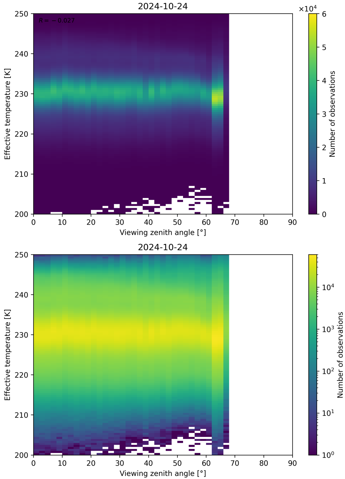
Figure 50: Scatter density plot of “Viewing zenith angle” against “Effective temperature” for 2024-10-24 to 2024-10-25.
