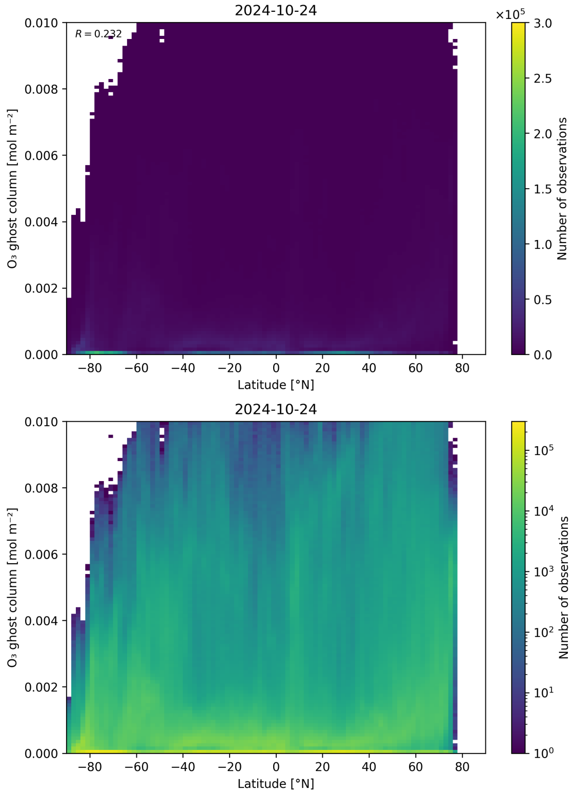
Figure 35: Scatter density plot of “Latitude” against “O 3 ghost column” for 2024-10-24 to 2024-10-25.
