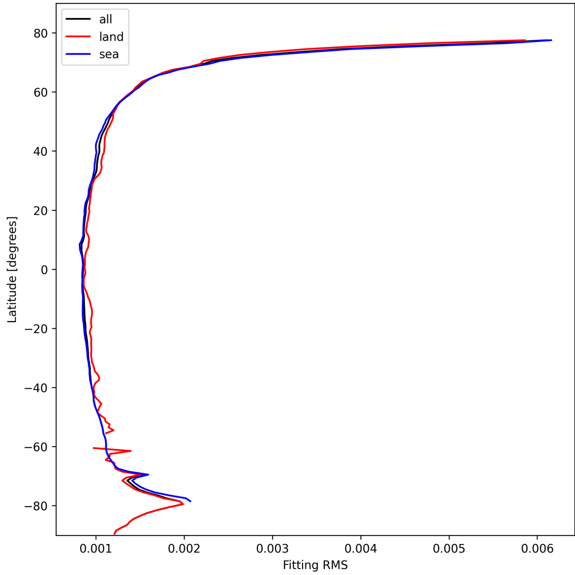
Figure 16: Zonal average of “Fitting RMS” for 2024-10-24 to 2024-10-25.
