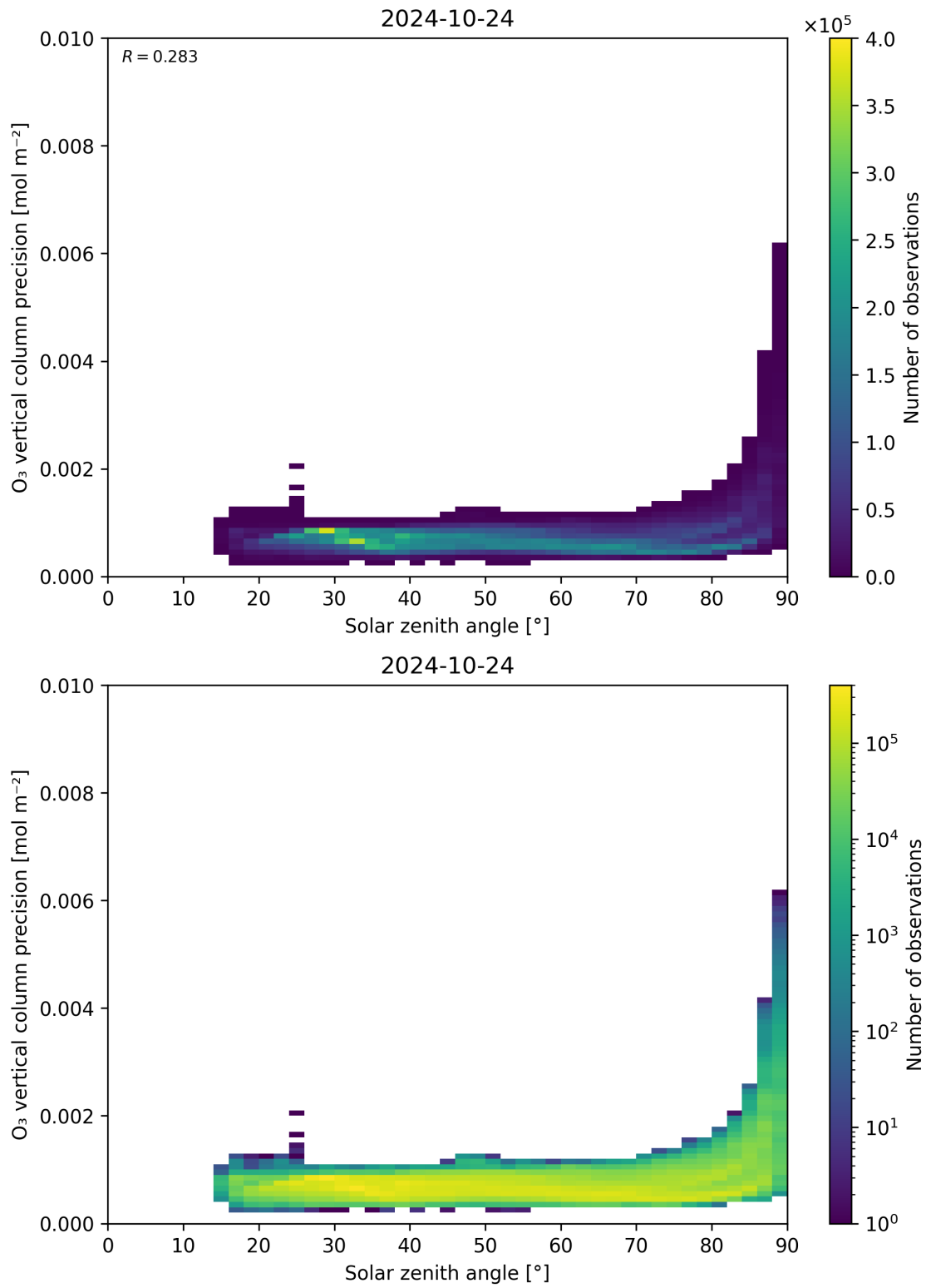
Figure 48: Scatter density plot of “Solar zenith angle” against “O 3 vertical column precision” for 2024-10-24 to 2024-10-25.
