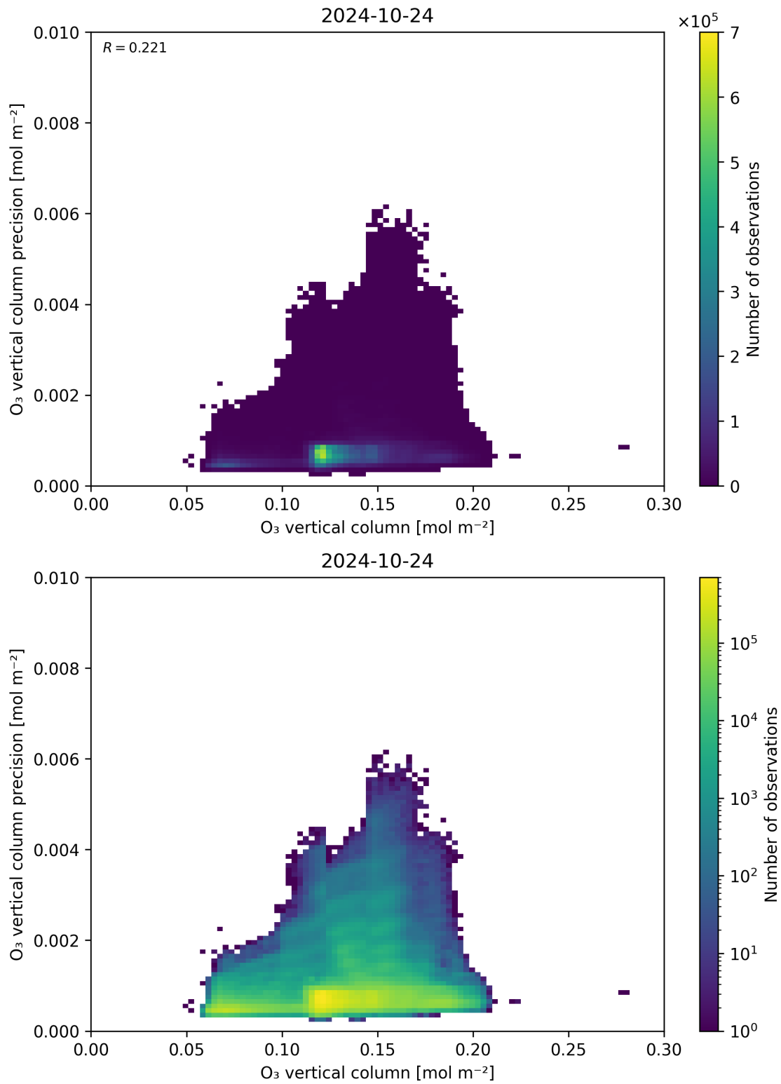
Figure 41: Scatter density plot of “O 3 vertical column” against “O 3 vertical column precision” for 2024-10-24 to 2024-10-25.
