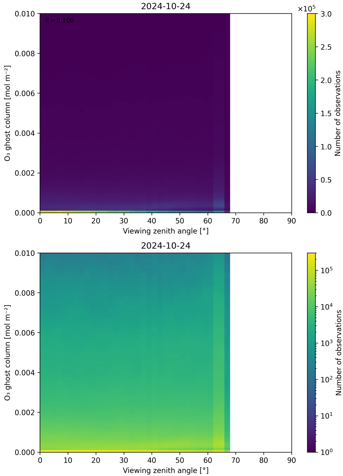
Figure 51: Scatter density plot of “Viewing zenith angle” against “O 3 ghost column” for 2024-10-24 to 2024-10-25.
