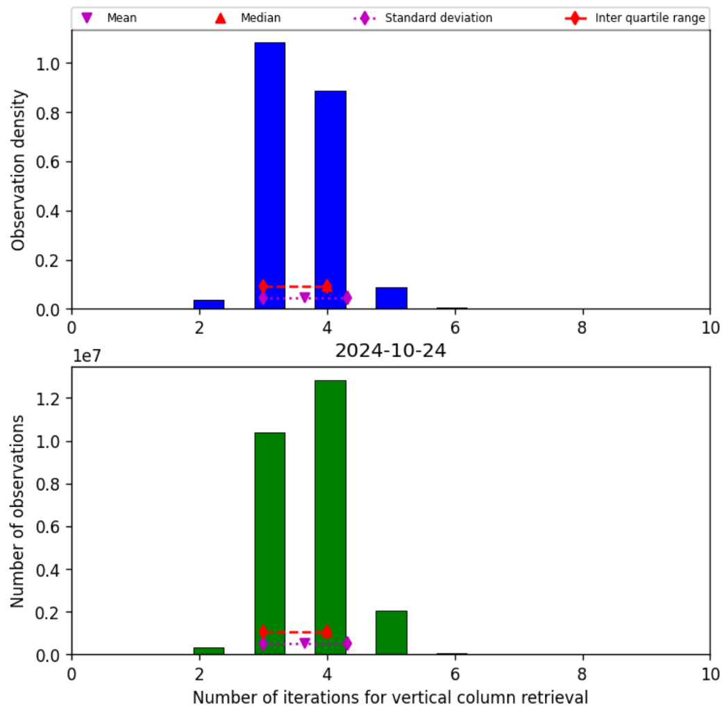
Figure 26: Histogram of “Number of iterations for vertical column retrieval” for 2024-10-24 to 2024-10-25
