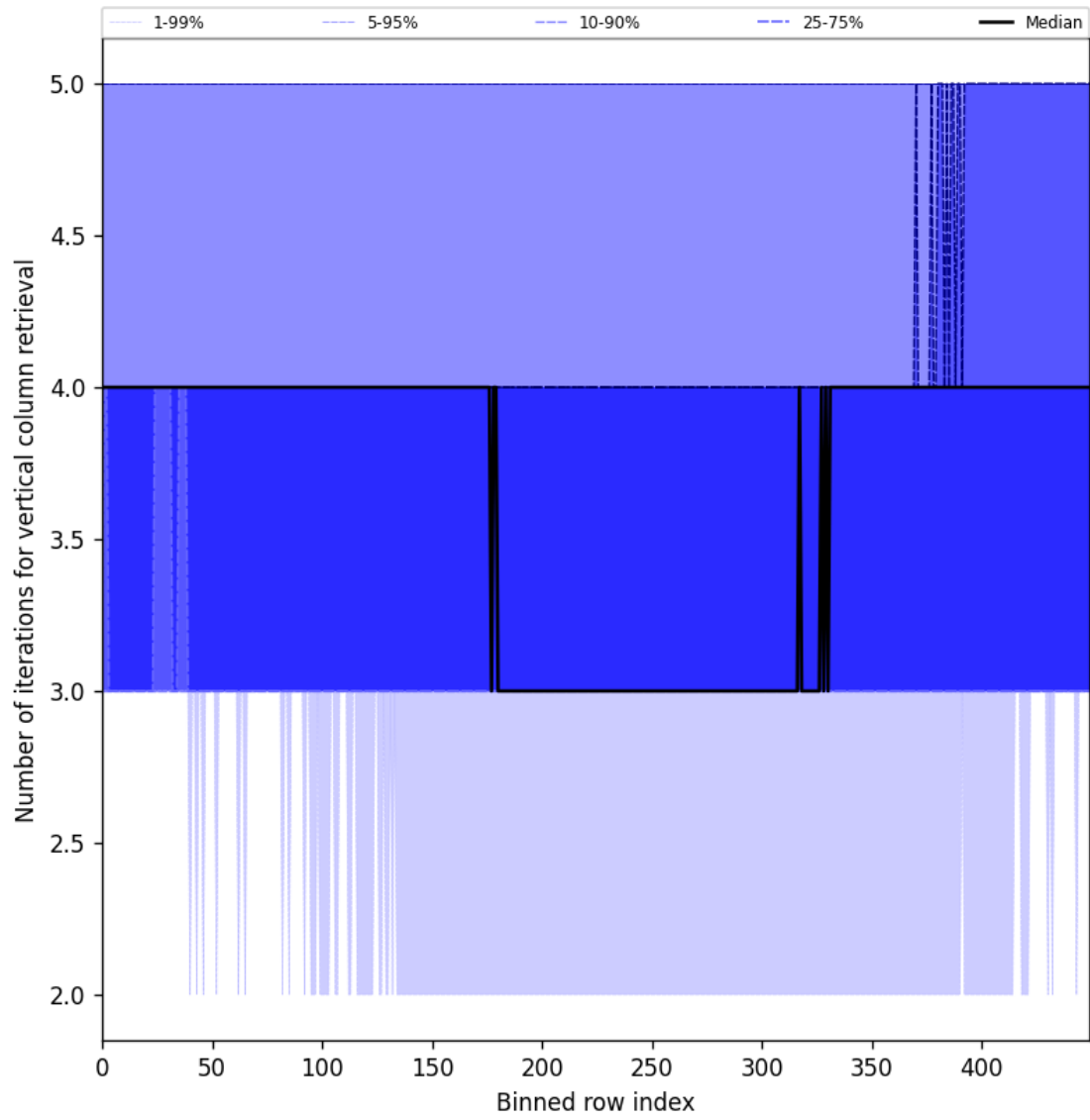
Figure 33: Along track statistics of “Number of iterations for vertical column retrieval” for 2024-10-24 to 2024-10-25
