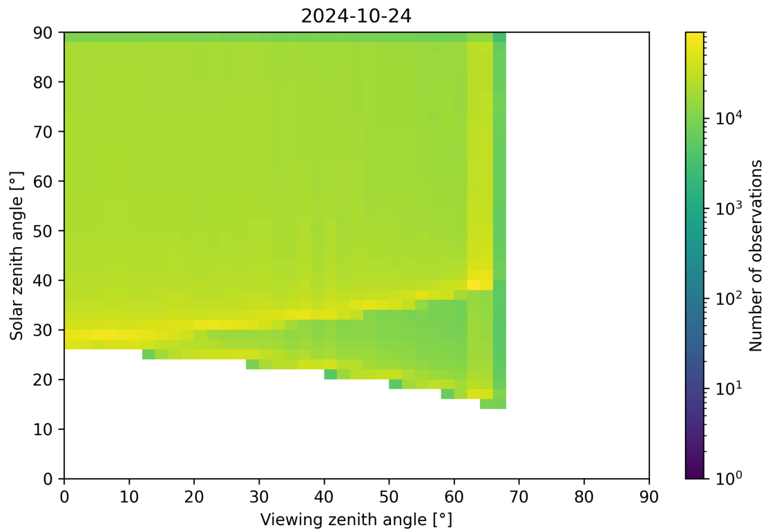
Figure 54: Scatter density plot of “Viewing zenith angle” against “Solar zenith angle” for 2024-10-24 to 2024-10-25.
