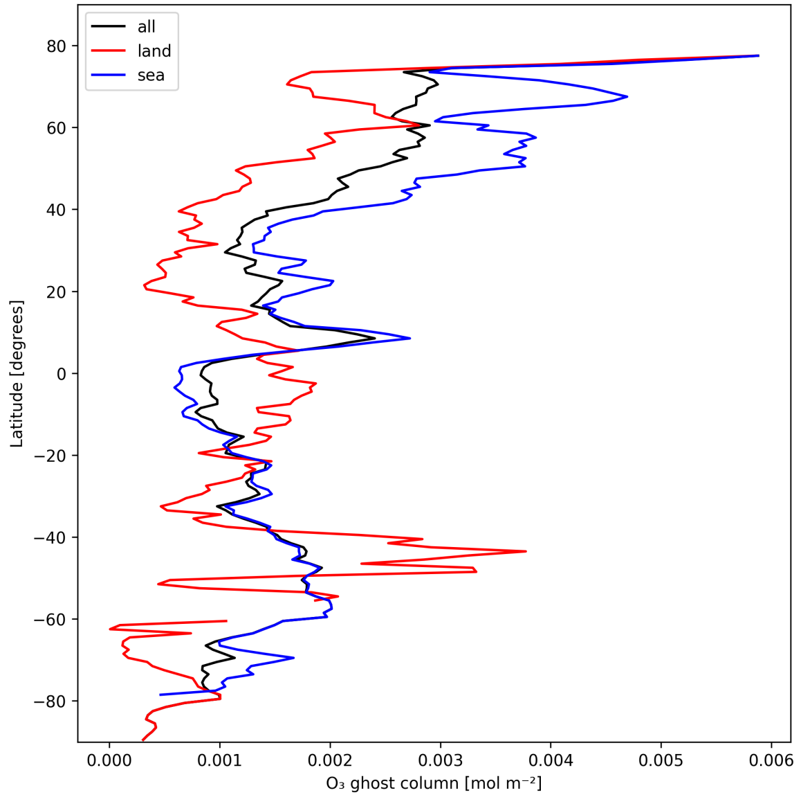
Figure 18: Zonal average of “O 3 ghost column” for 2024-10-24 to 2024-10-25.
