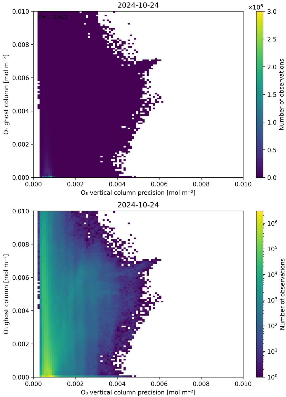
Figure 43: Scatter density plot of “O 3 vertical column precision” against “O 3 ghost column” for 2024-10-24 to 2024-10-25.
