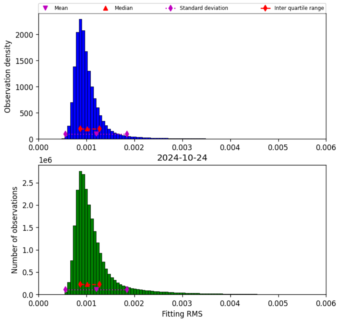
Figure 23: Histogram of “Fitting RMS” for 2024-10-24 to 2024-10-25
