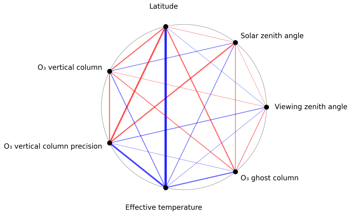
Figure 1: Map of correlation graph for 2024-10-24 to 2024-10-25.
