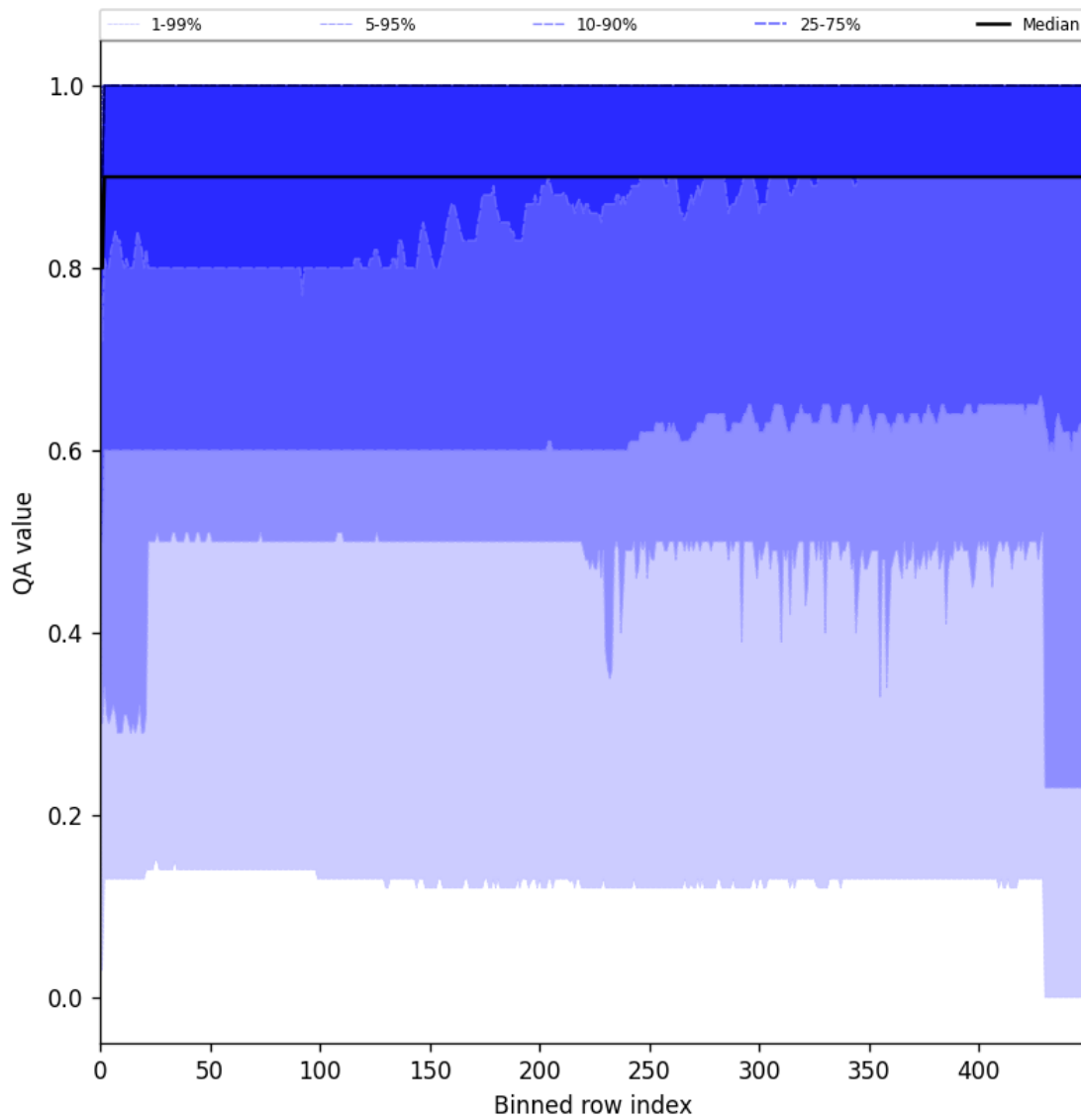
Figure 27: Along track statistics of “QA value” for 2024-10-24 to 2024-10-25
