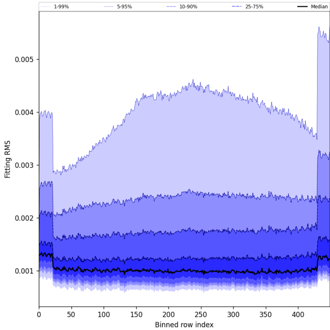
Figure 30: Along track statistics of “Fitting RMS” for 2024-10-24 to 2024-10-25
