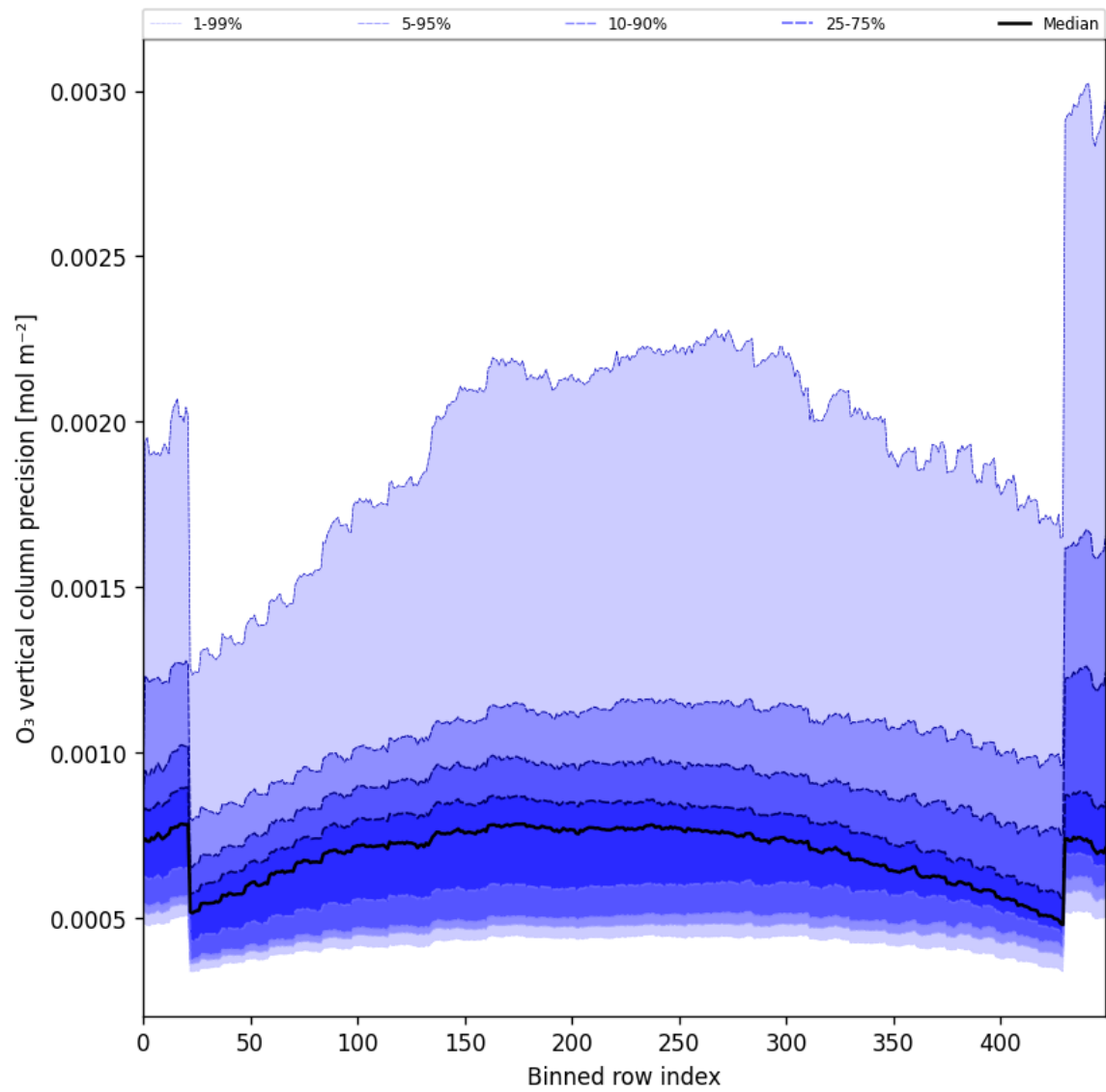
Figure 29: Along track statistics of “O 3 vertical column precision” for 2024-10-24 to 2024-10-25
