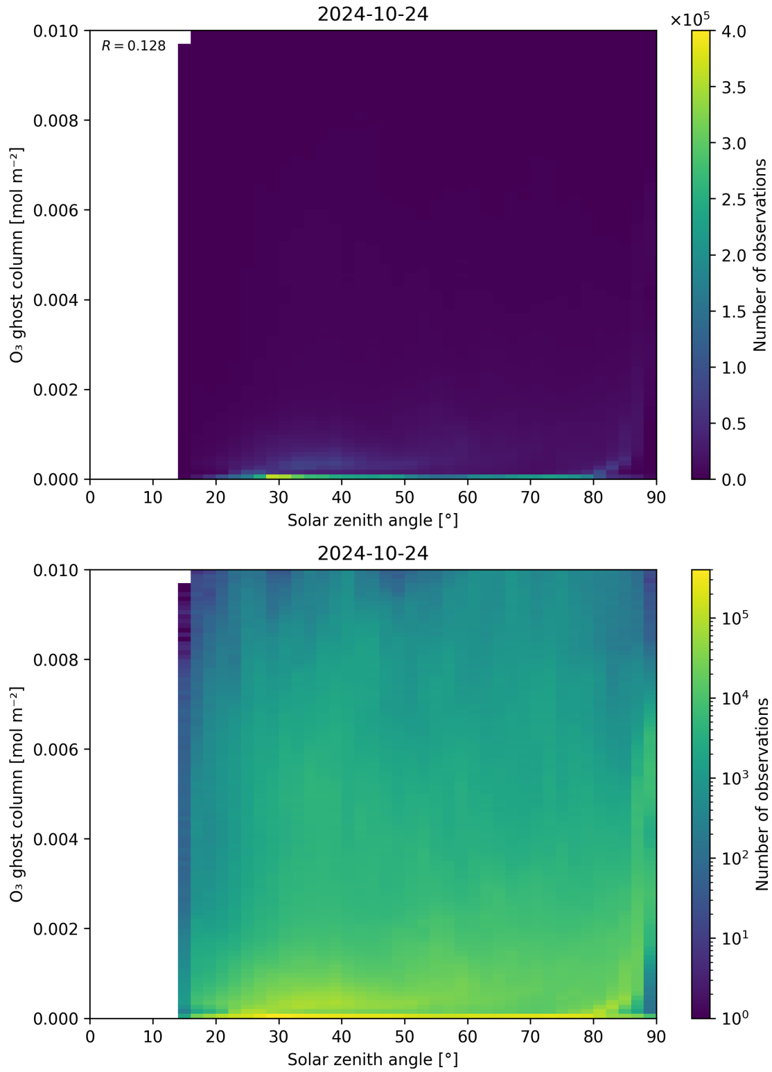
Figure 46: Scatter density plot of “Solar zenith angle” against “O 3 ghost column” for 2024-10-24 to 2024-10-25.
