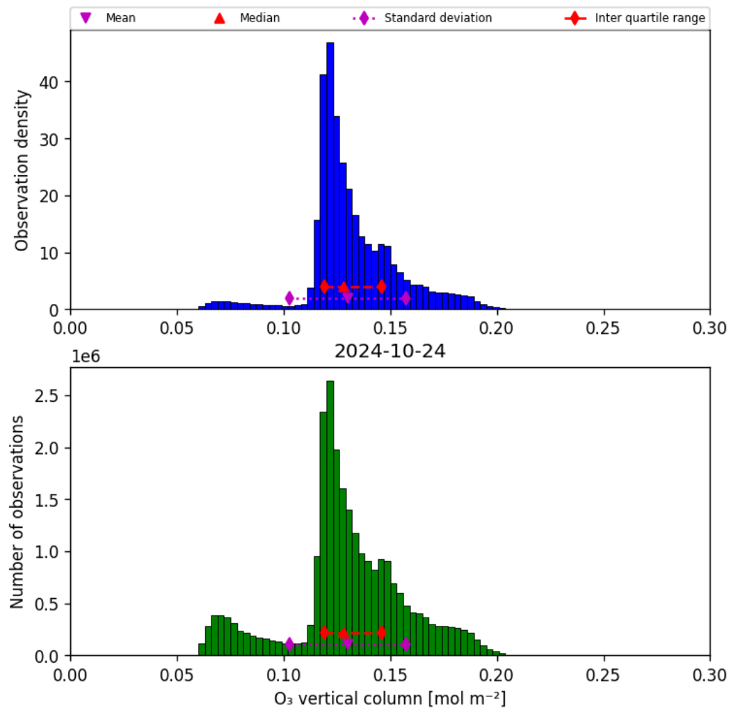
Figure 21: Histogram of “O 3 vertical column” for 2024-10-24 to 2024-10-25
