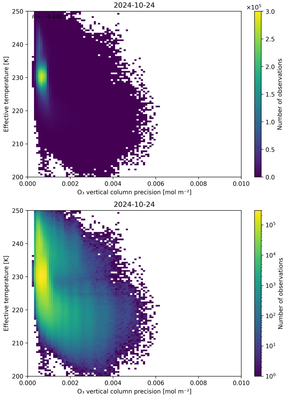
Figure 42: Scatter density plot of “ \text{O}_3 vertical column precision” against “Effective temperature” for 2024-10-24 to 2024-10-25.
