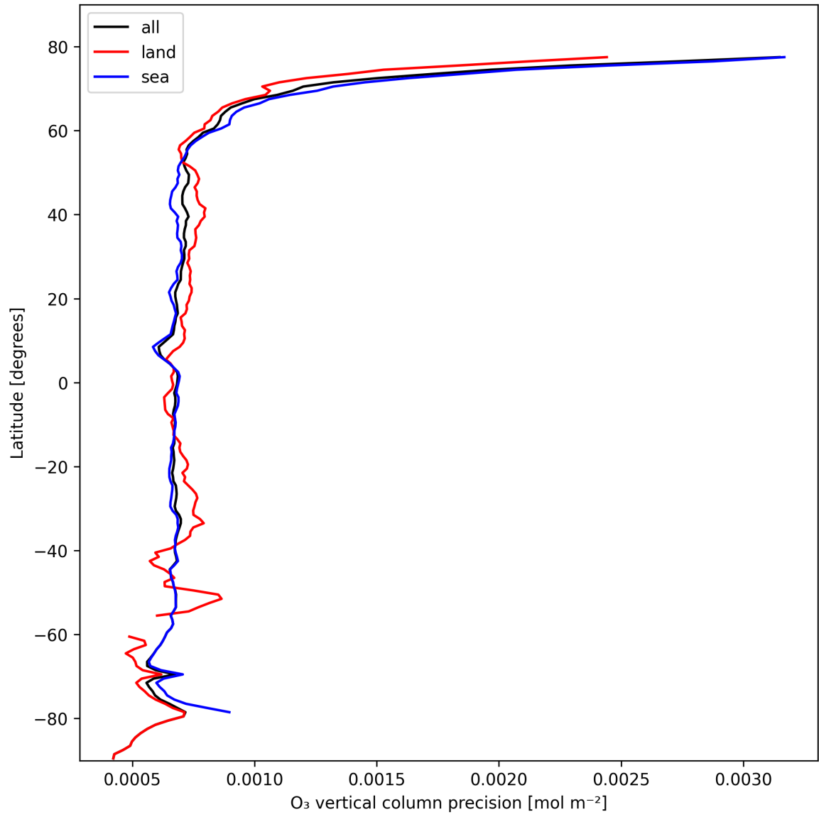
Figure 15: Zonal average of “O 3 vertical column precision” for 2024-10-24 to 2024-10-25.
