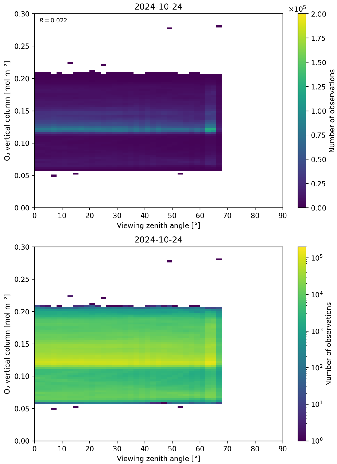
Figure 52: Scatter density plot of “Viewing zenith angle” against “O 3 vertical column” for 2024-10-24 to 2024-10-25.
