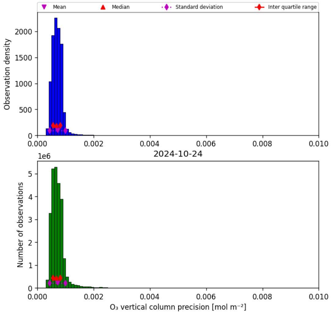
Figure 22: Histogram of “O 3 vertical column precision” for 2024-10-24 to 2024-10-25
