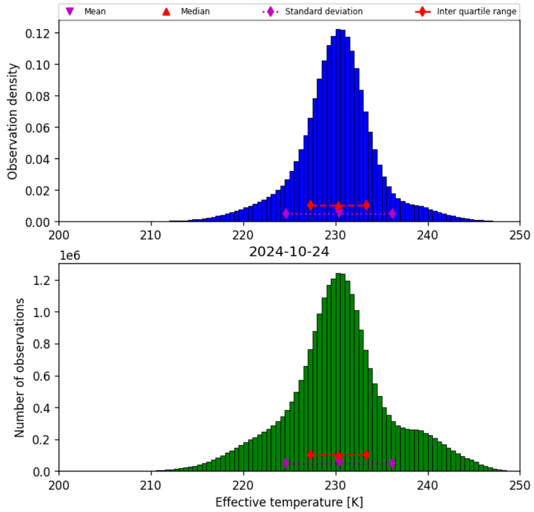
Figure 24: Histogram of “Effective temperature” for 2024-10-24 to 2024-10-25
