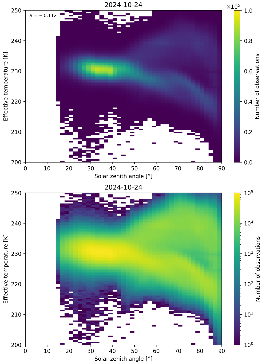
Figure 45: Scatter density plot of “Solar zenith angle” against “Effective temperature” for 2024-10-24 to 2024-10-25.
