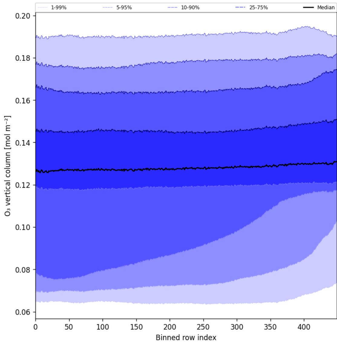
Figure 28: Along track statistics of “O 3 vertical column” for 2024-10-24 to 2024-10-25
