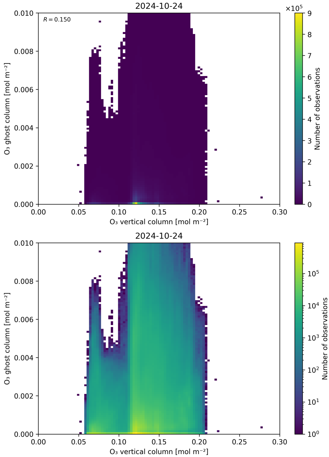
Figure 40: Scatter density plot of “O 3 vertical column” against “O 3 ghost column” for 2024-10-24 to 2024-10-25.
