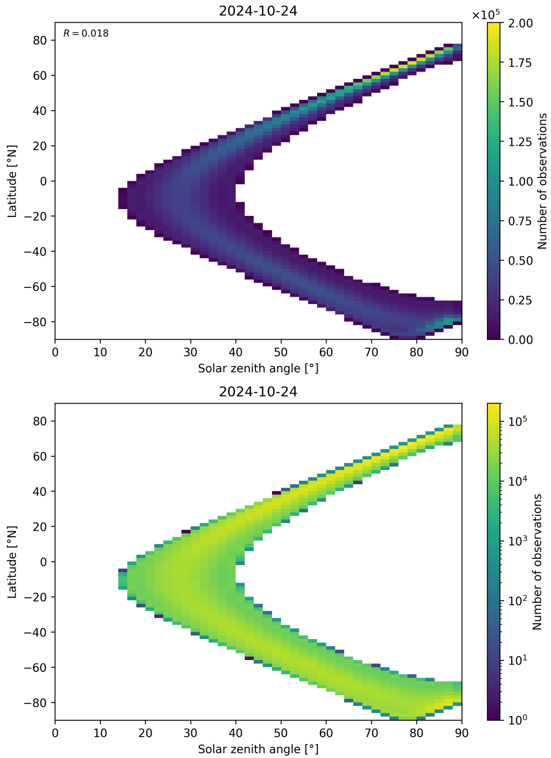
Figure 44: Scatter density plot of “Solar zenith angle” against “Latitude” for 2024-10-24 to 2024-10-25.
