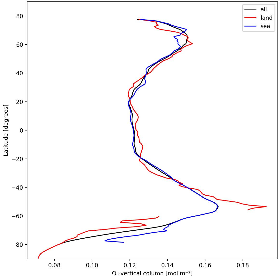
Figure 14: Zonal average of “O 3 vertical column” for 2024-10-24 to 2024-10-25.
