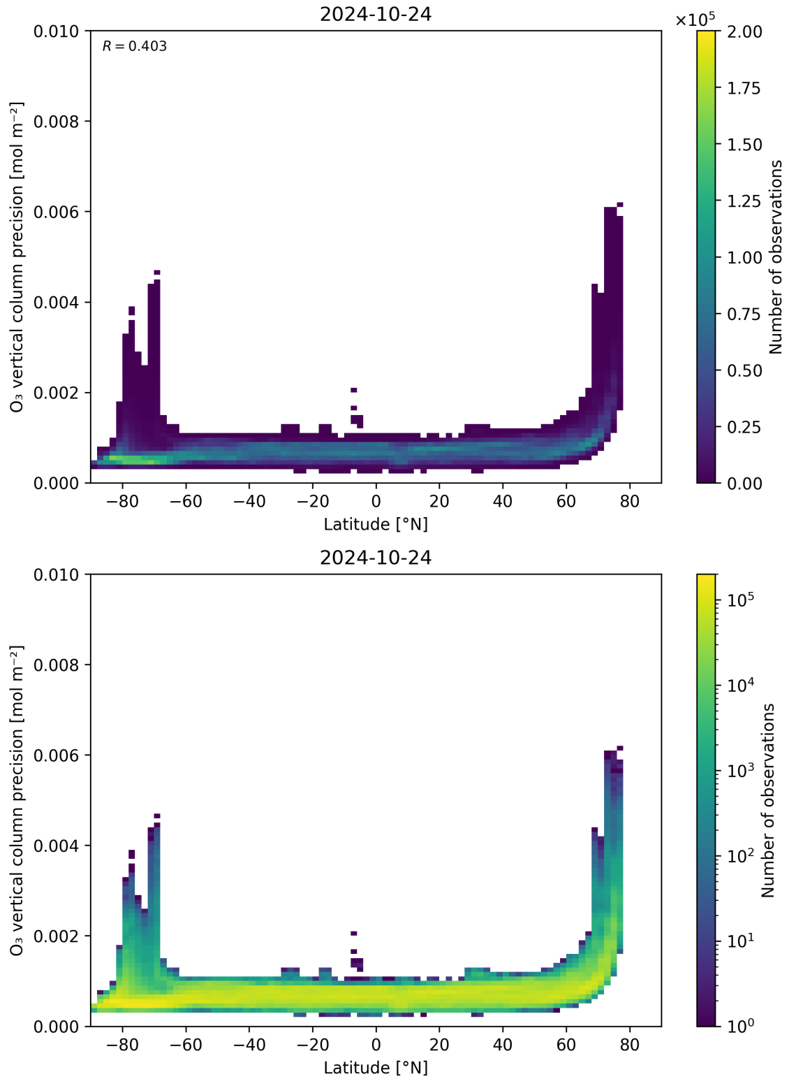
Figure 37: Scatter density plot of “Latitude” against “O 3 vertical column precision” for 2024-10-24 to 2024-10-25.
