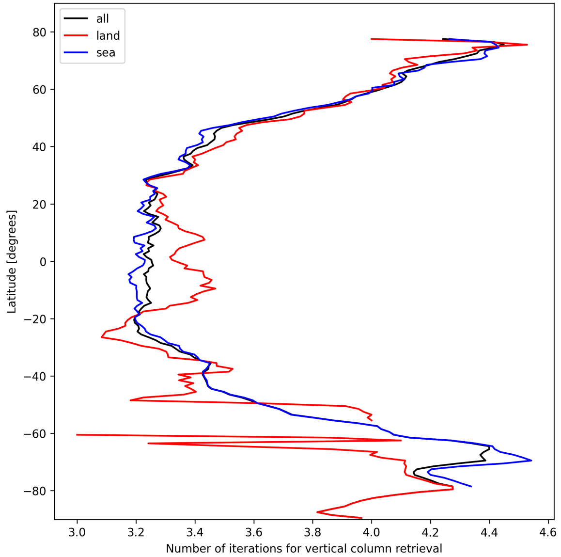
Figure 19: Zonal average of “Number of iterations for vertical column retrieval” for 2024-10-24 to 2024-10-25.
