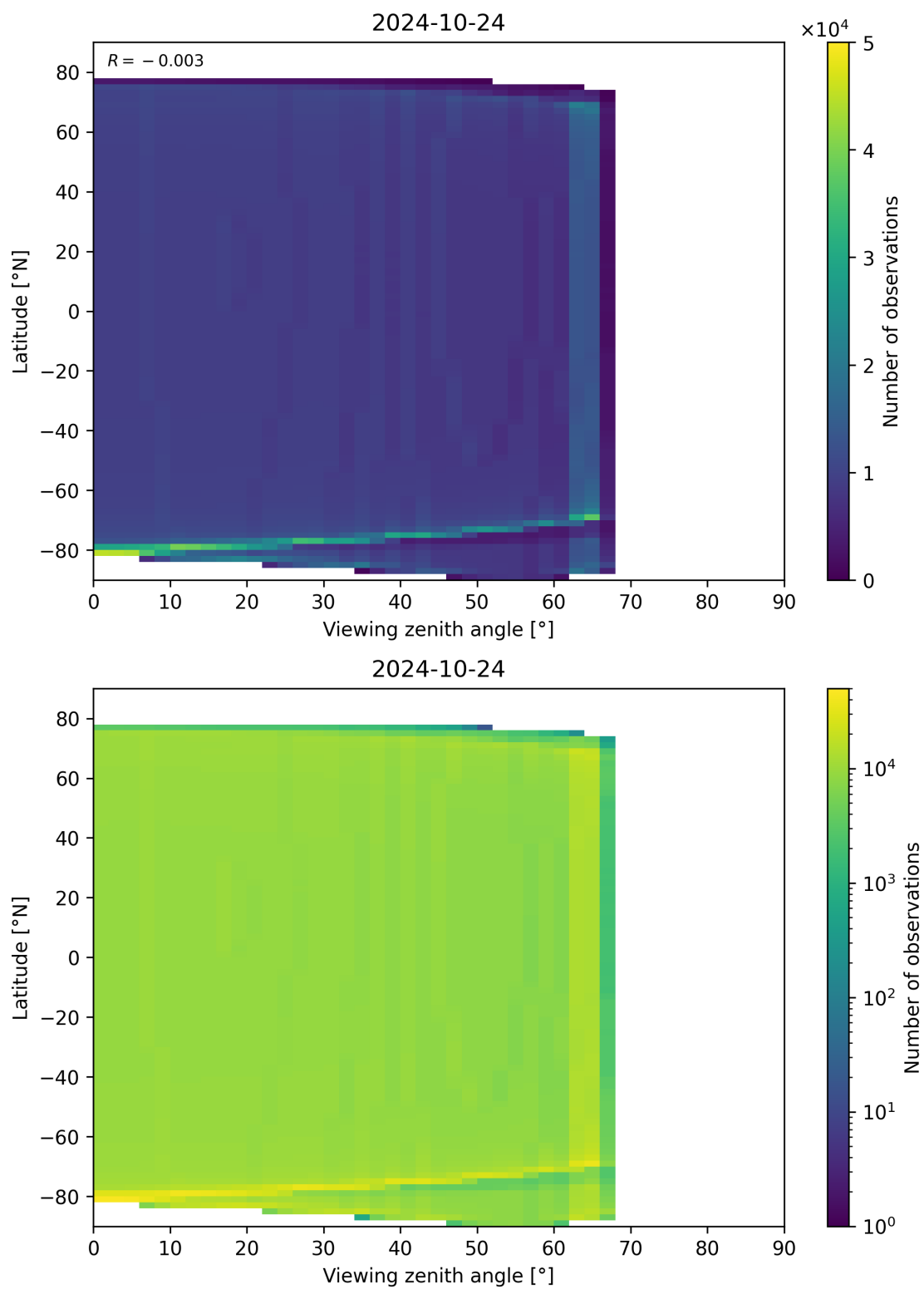
Figure 49: Scatter density plot of “Viewing zenith angle” against “Latitude” for 2024-10-24 to 2024-10-25.
