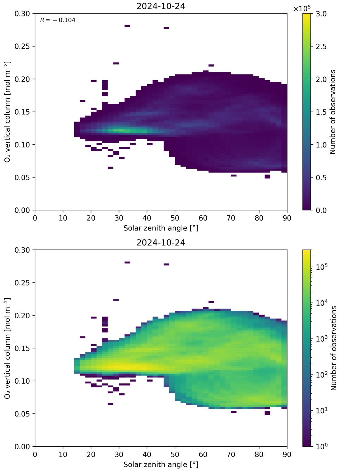
Figure 47: Scatter density plot of “Solar zenith angle” against “O 3 vertical column” for 2024-10-24 to 2024-10-25.
