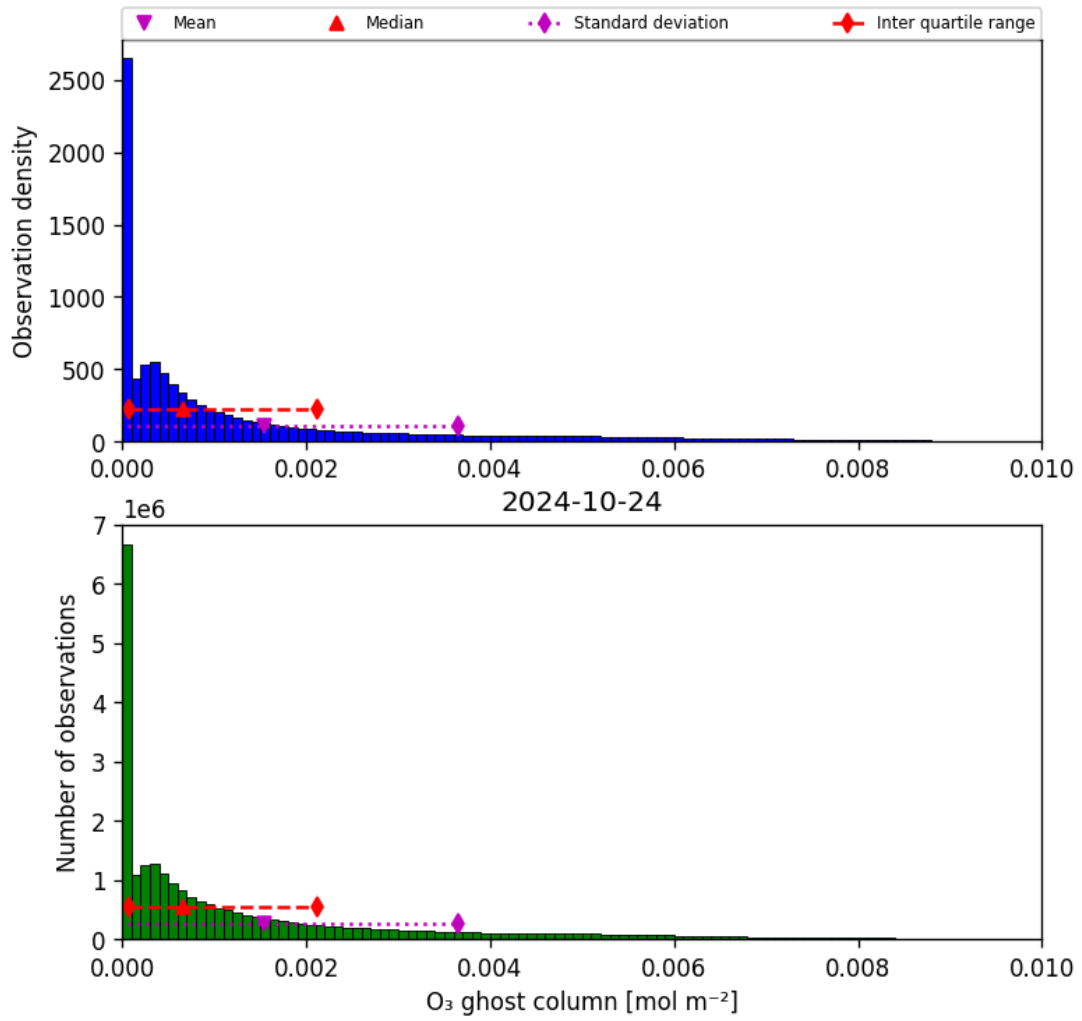
Figure 25: Histogram of “O 3 ghost column” for 2024-10-24 to 2024-10-25
