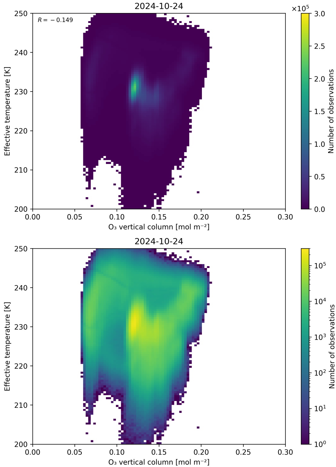
Figure 39: Scatter density plot of “O 3 vertical column” against “Effective temperature” for 2024-10-24 to 2024-10-25.
