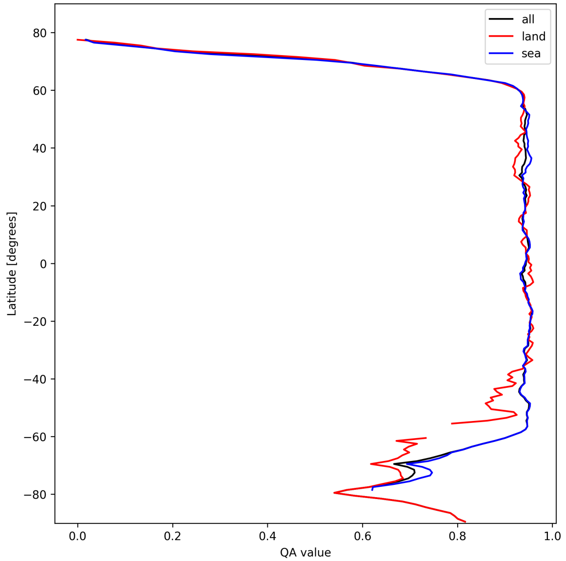
Figure 13: Zonal average of “QA value” for 2024-10-24 to 2024-10-25.
