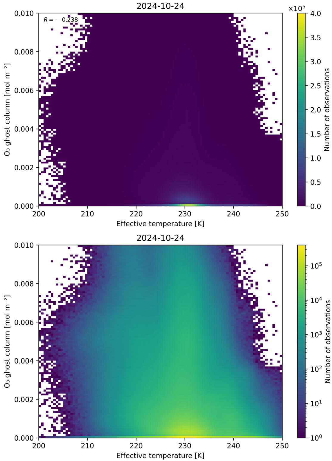
Figure 38: Scatter density plot of “Effective temperature” against “O 3 ghost column” for 2024-10-24 to 2024-10-25.
