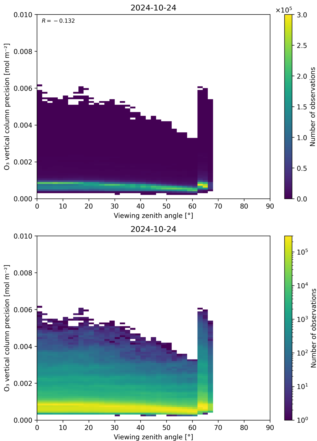
Figure 53: Scatter density plot of “Viewing zenith angle” against “O 3 vertical column precision” for 2024-10-24 to 2024-10-25.
