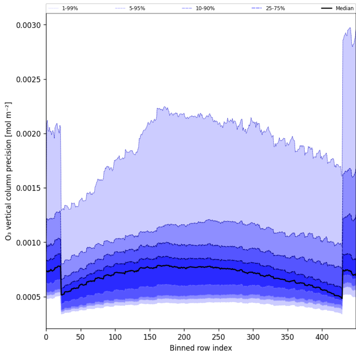
Figure 29: Along track statistics of “O 3 vertical column precision” for 2024-10-24 to 2024-10-26
