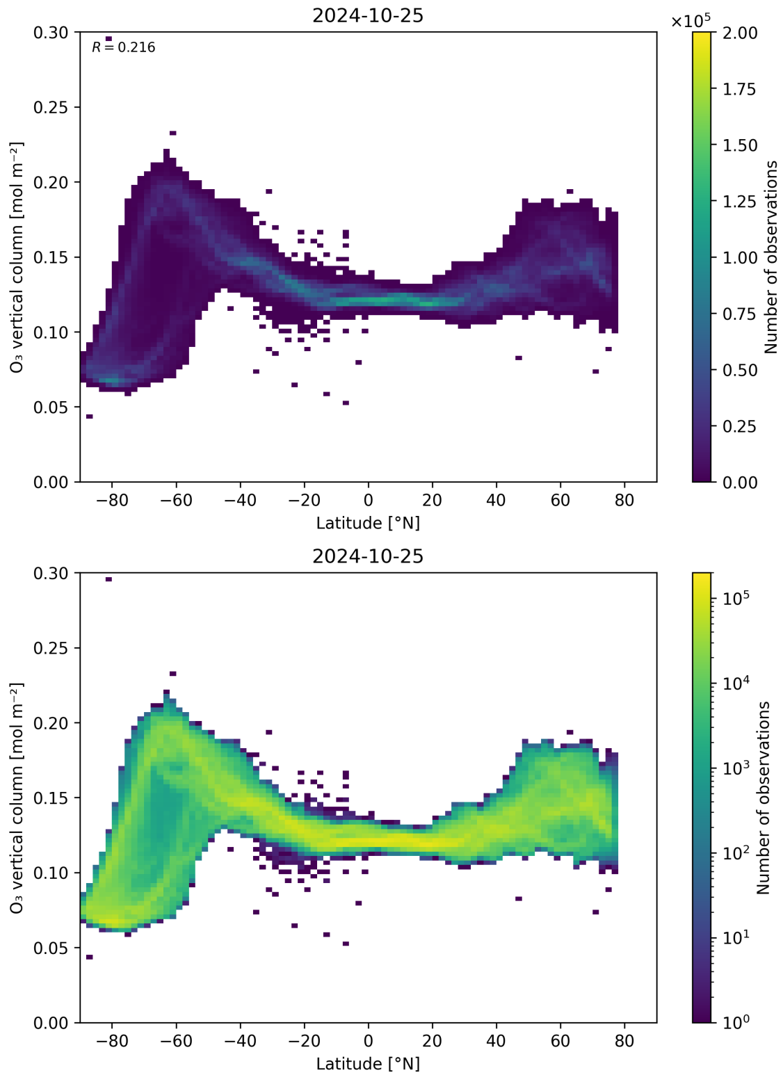
Figure 36: Scatter density plot of “Latitude” against “O 3 vertical column” for 2024-10-24 to 2024-10-26.
