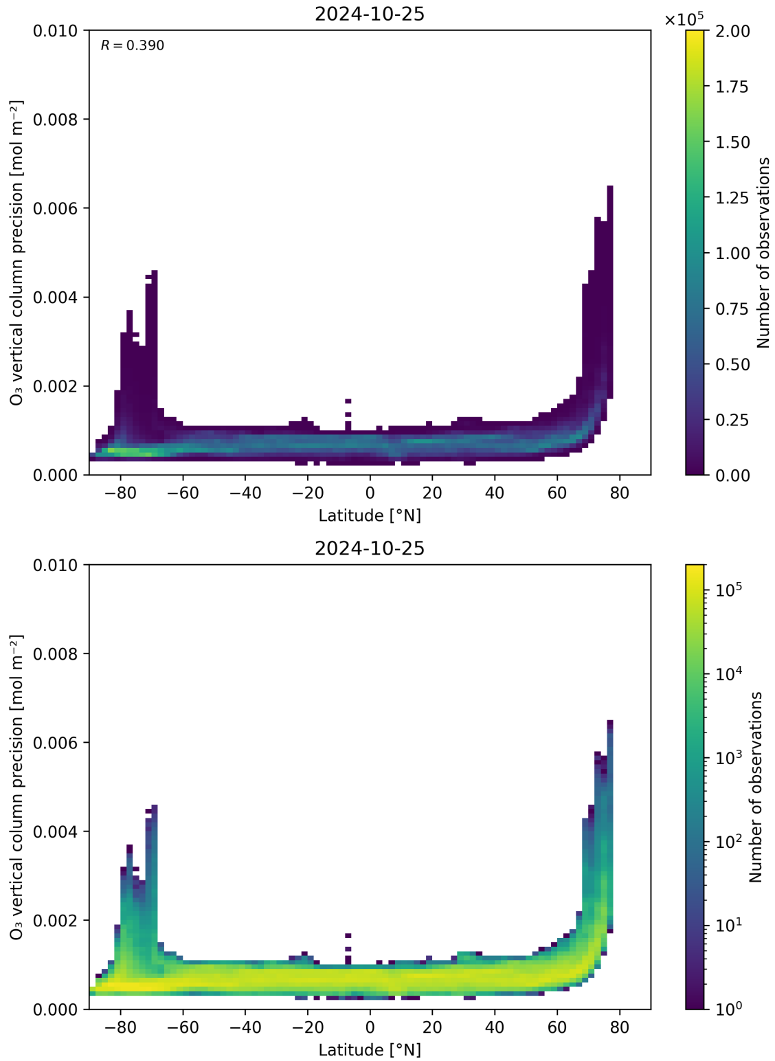
Figure 37: Scatter density plot of “Latitude” against “O 3 vertical column precision” for 2024-10-24 to 2024-10-26.
