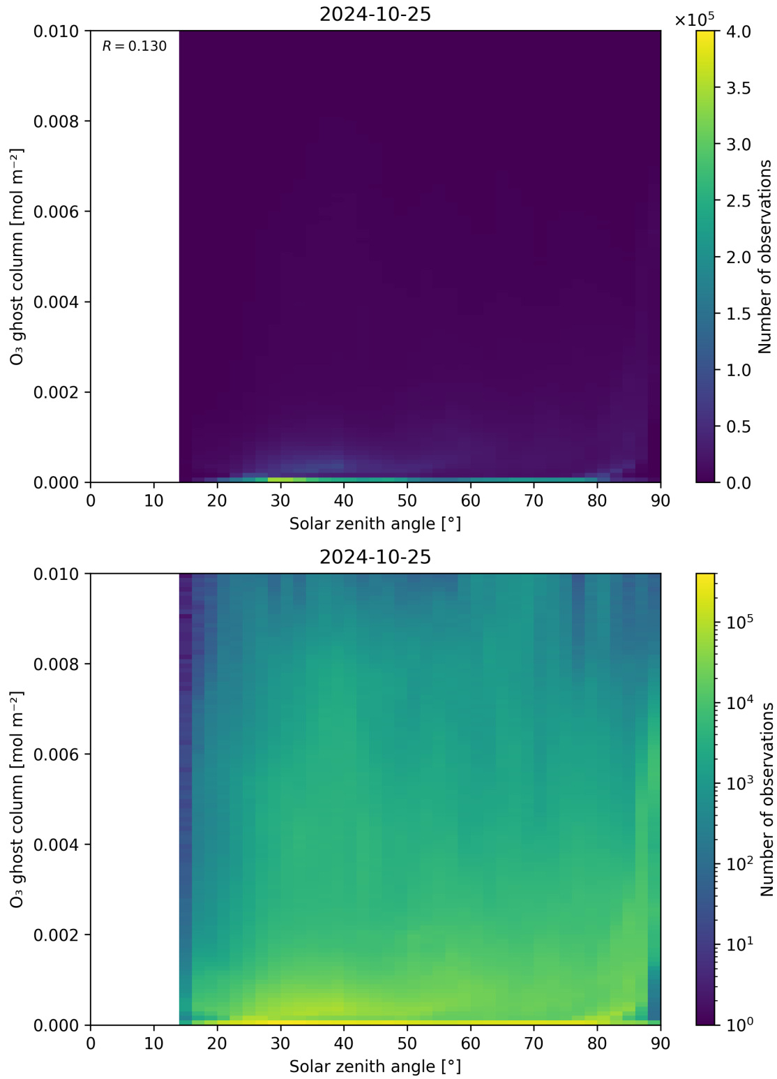
Figure 46: Scatter density plot of “Solar zenith angle” against “O 3 ghost column” for 2024-10-24 to 2024-10-26.
