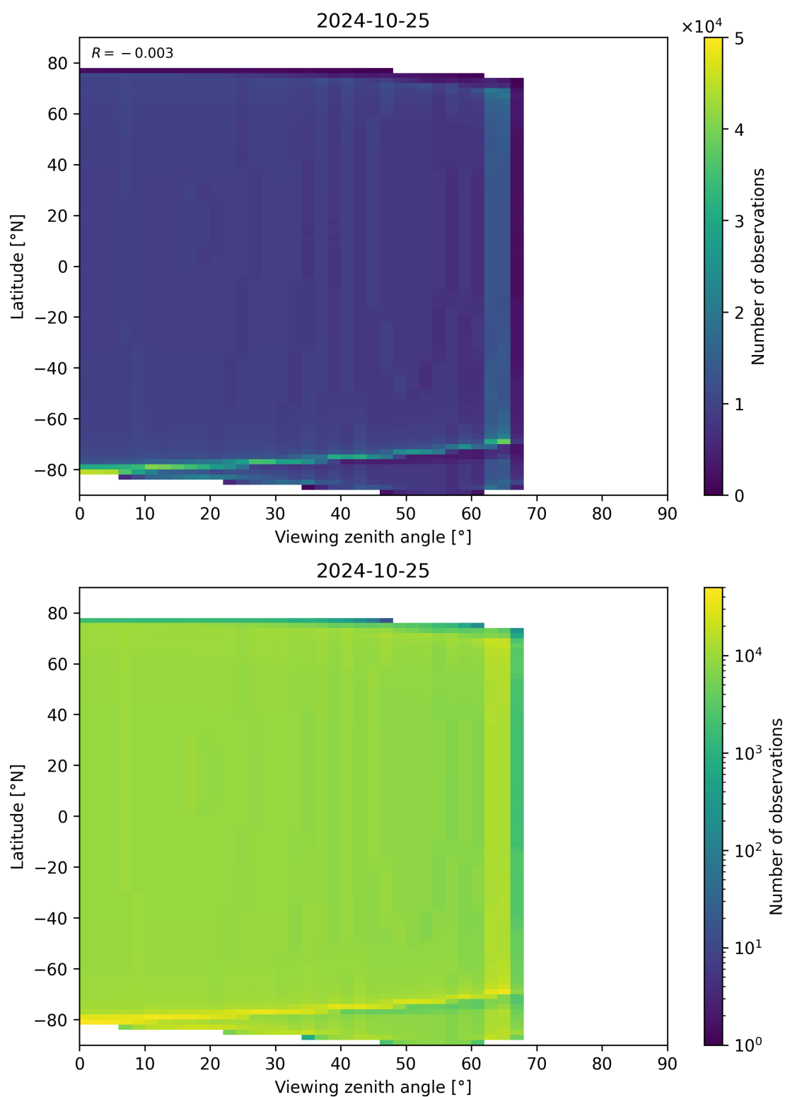
Figure 49: Scatter density plot of “Viewing zenith angle” against “Latitude” for 2024-10-24 to 2024-10-26.
