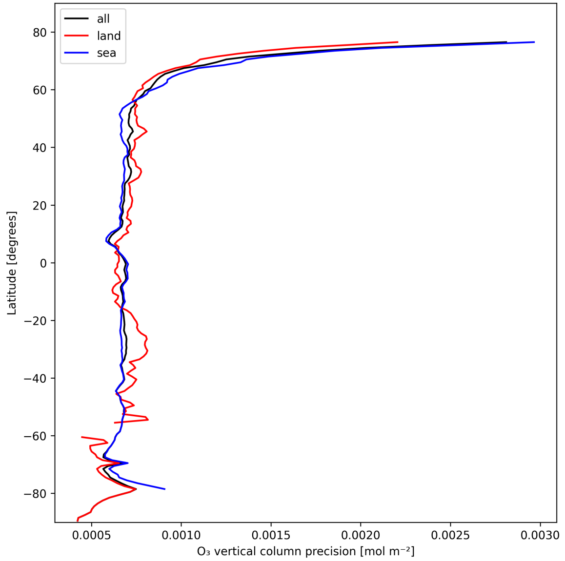
Figure 15: Zonal average of “O 3 vertical column precision” for 2024-10-24 to 2024-10-26.
