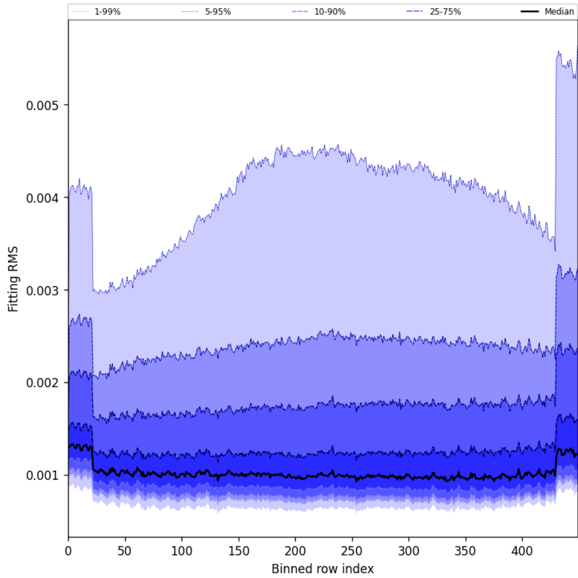
Figure 30: Along track statistics of “Fitting RMS” for 2024-10-24 to 2024-10-26
