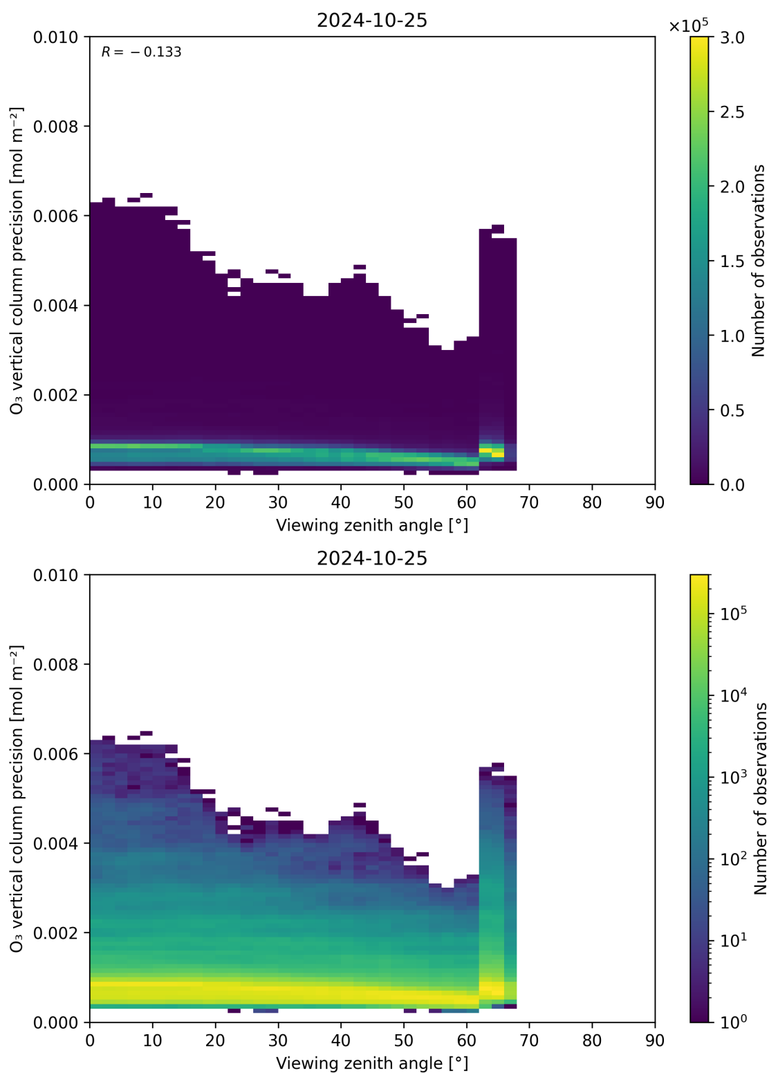
Figure 53: Scatter density plot of “Viewing zenith angle” against “O 3 vertical column precision” for 2024-10-24 to 2024-10-26.
