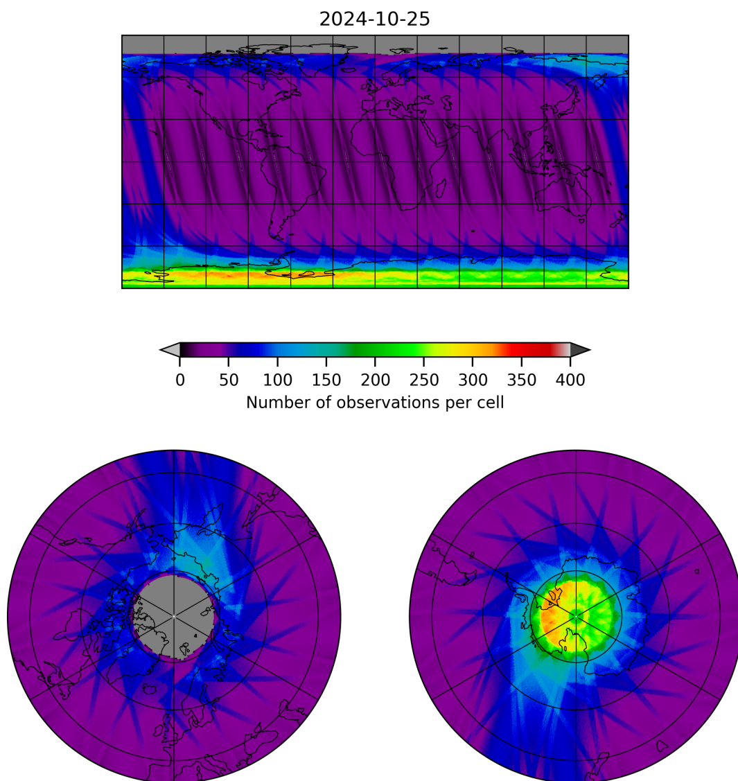
Figure 12: Map of the number of observations for 2024-10-24 to 2024-10-26
