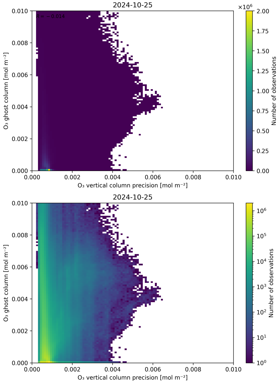
Figure 43: Scatter density plot of “O 3 vertical column precision” against “O 3 ghost column” for 2024-10-24 to 2024-10-26.
