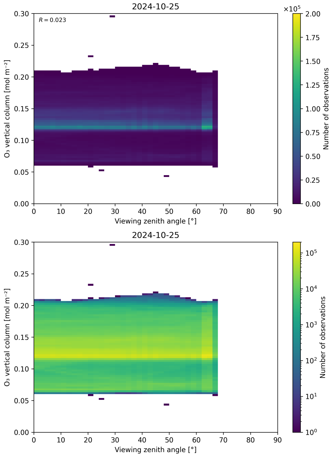
Figure 52: Scatter density plot of “Viewing zenith angle” against “O 3 vertical column” for 2024-10-24 to 2024-10-26.
