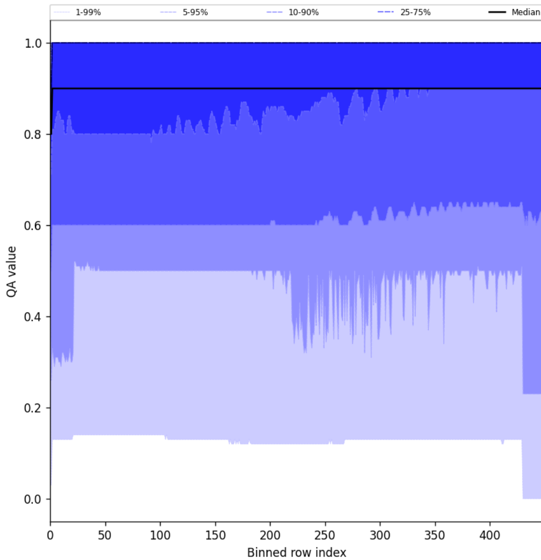
Figure 27: Along track statistics of “QA value” for 2024-10-24 to 2024-10-26
