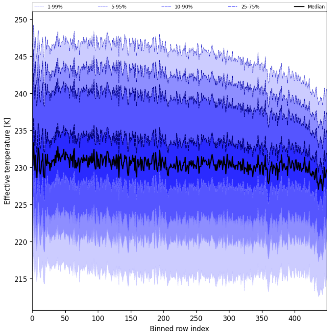
Figure 31: Along track statistics of “Effective temperature” for 2024-10-24 to 2024-10-26
