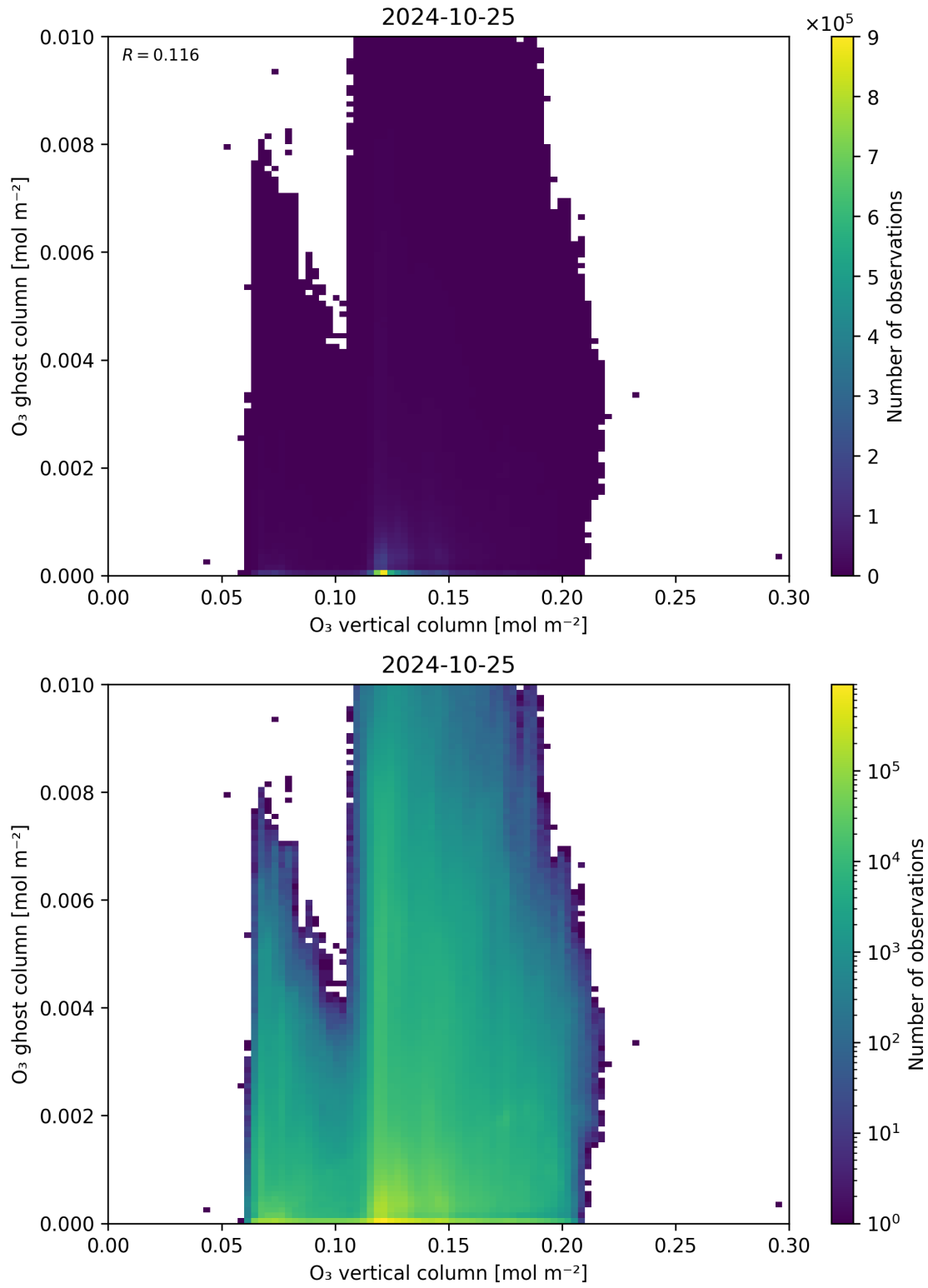
Figure 40: Scatter density plot of “O 3 vertical column” against “O 3 ghost column” for 2024-10-24 to 2024-10-26.
