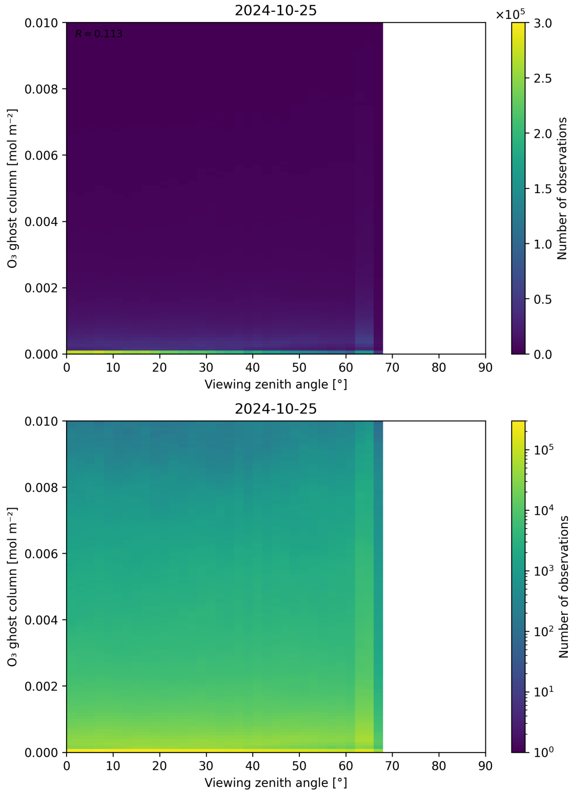
Figure 51: Scatter density plot of “Viewing zenith angle” against “O 3 ghost column” for 2024-10-24 to 2024-10-26.
