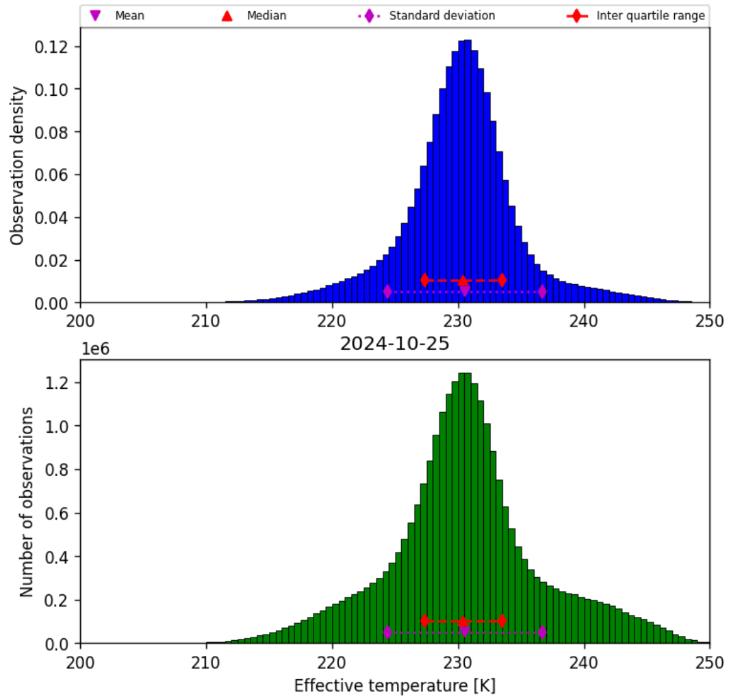
Figure 24: Histogram of “Effective temperature” for 2024-10-24 to 2024-10-26
