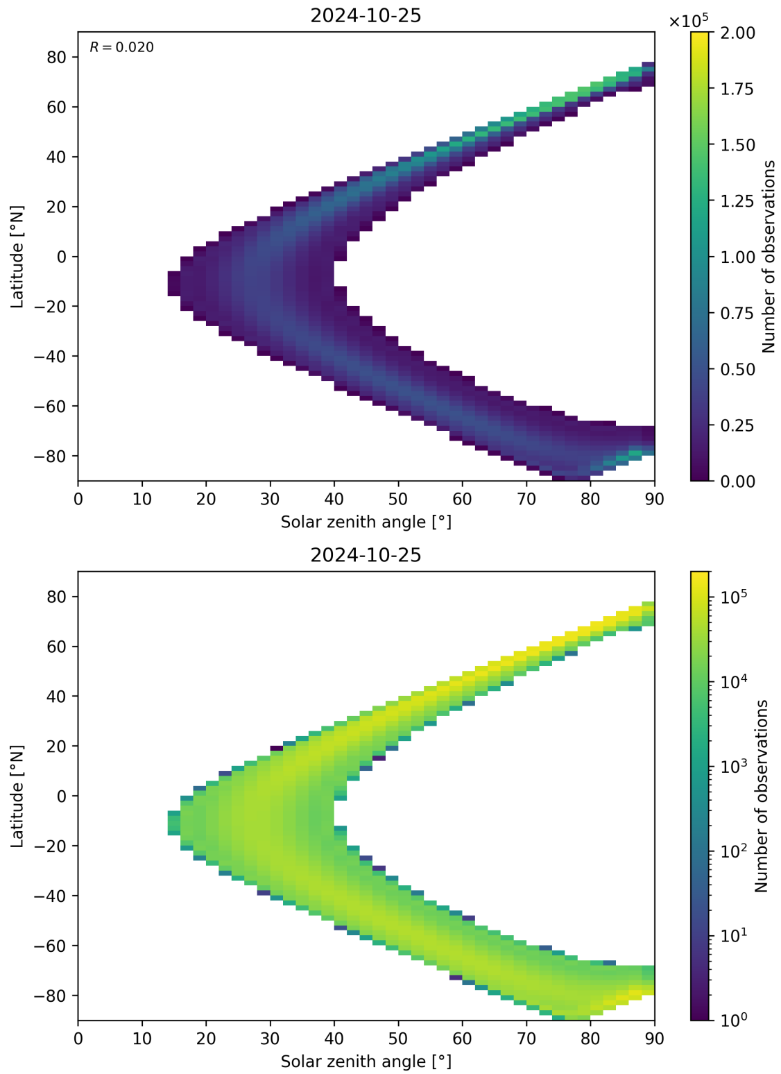
Figure 44: Scatter density plot of “Solar zenith angle” against “Latitude” for 2024-10-24 to 2024-10-26.
