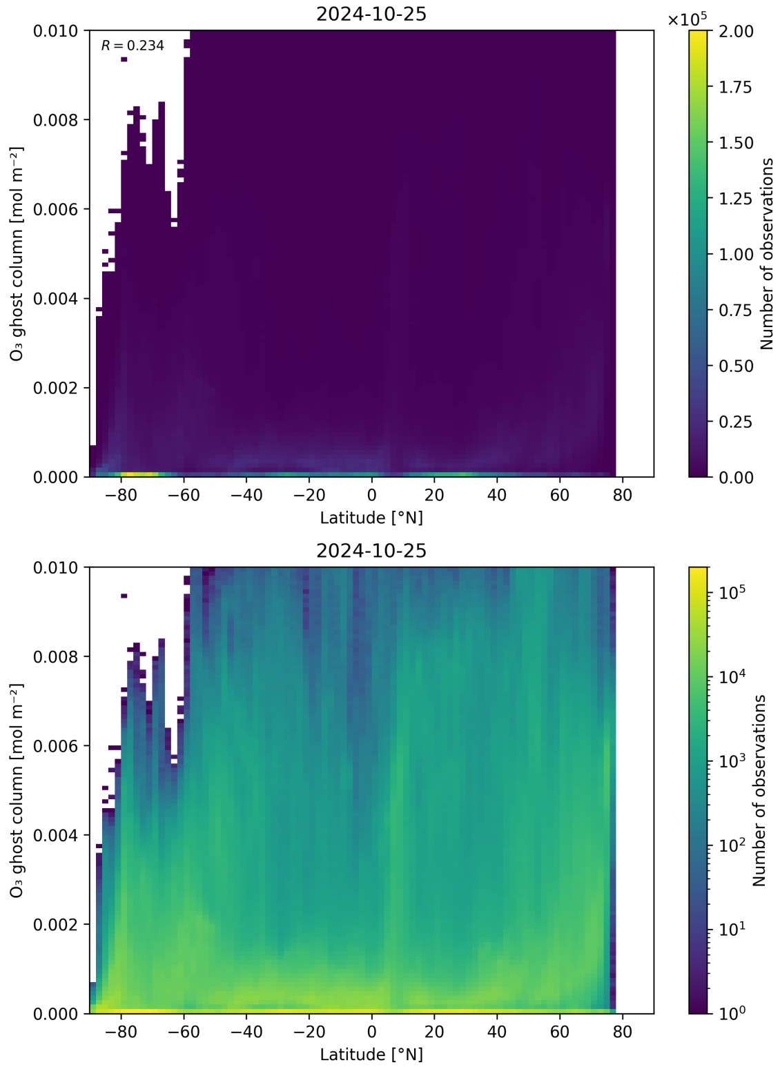
Figure 35: Scatter density plot of “Latitude” against “O 3 ghost column” for 2024-10-24 to 2024-10-26.
