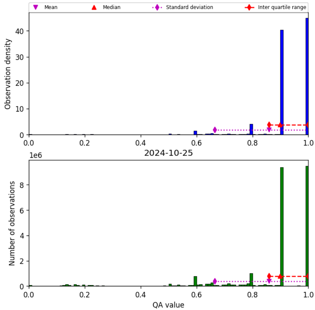
Figure 20: Histogram of “QA value” for 2024-10-24 to 2024-10-26
