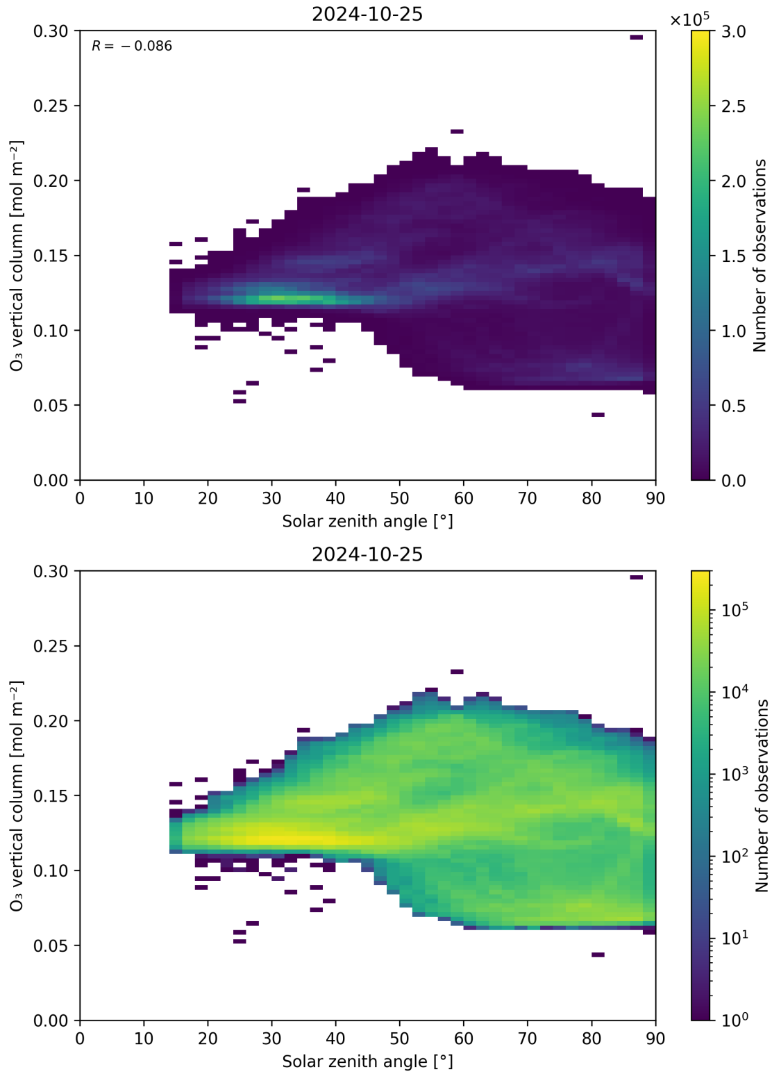
Figure 47: Scatter density plot of “Solar zenith angle” against “O 3 vertical column” for 2024-10-24 to 2024-10-26.
