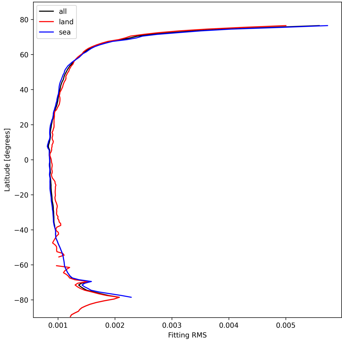
Figure 16: Zonal average of “Fitting RMS” for 2024-10-24 to 2024-10-26.
