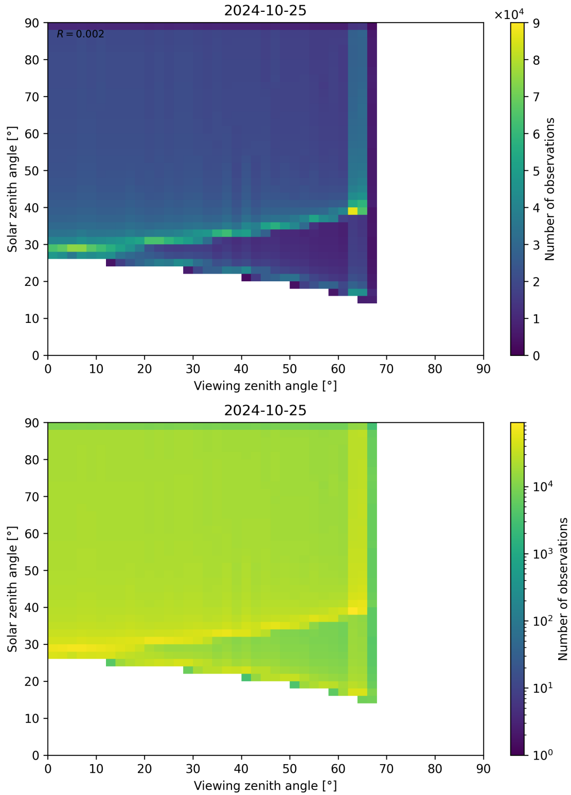
Figure 54: Scatter density plot of “Viewing zenith angle” against “Solar zenith angle” for 2024-10-24 to 2024-10-26.
