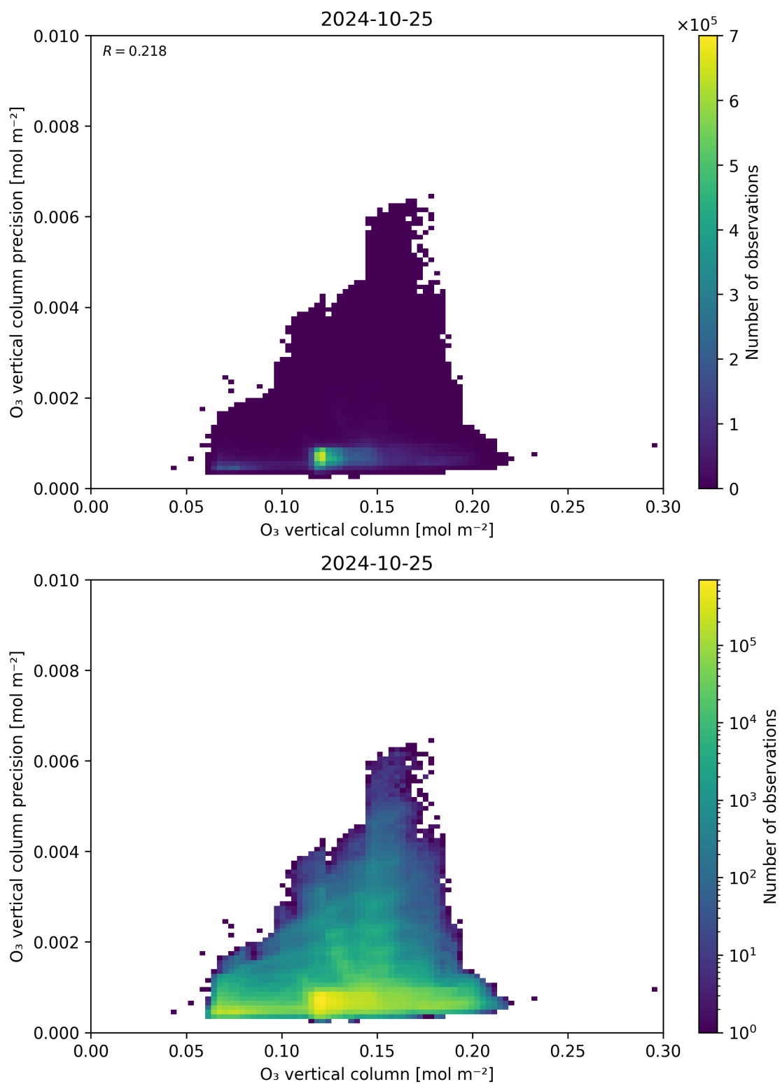
Figure 41: Scatter density plot of “O 3 vertical column” against “O 3 vertical column precision” for 2024-10-24 to 2024-10-26.
