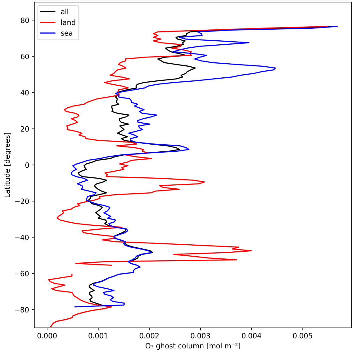
Figure 18: Zonal average of "O 3 ghost column" for 2024-10-24 to 2024-10-26.
