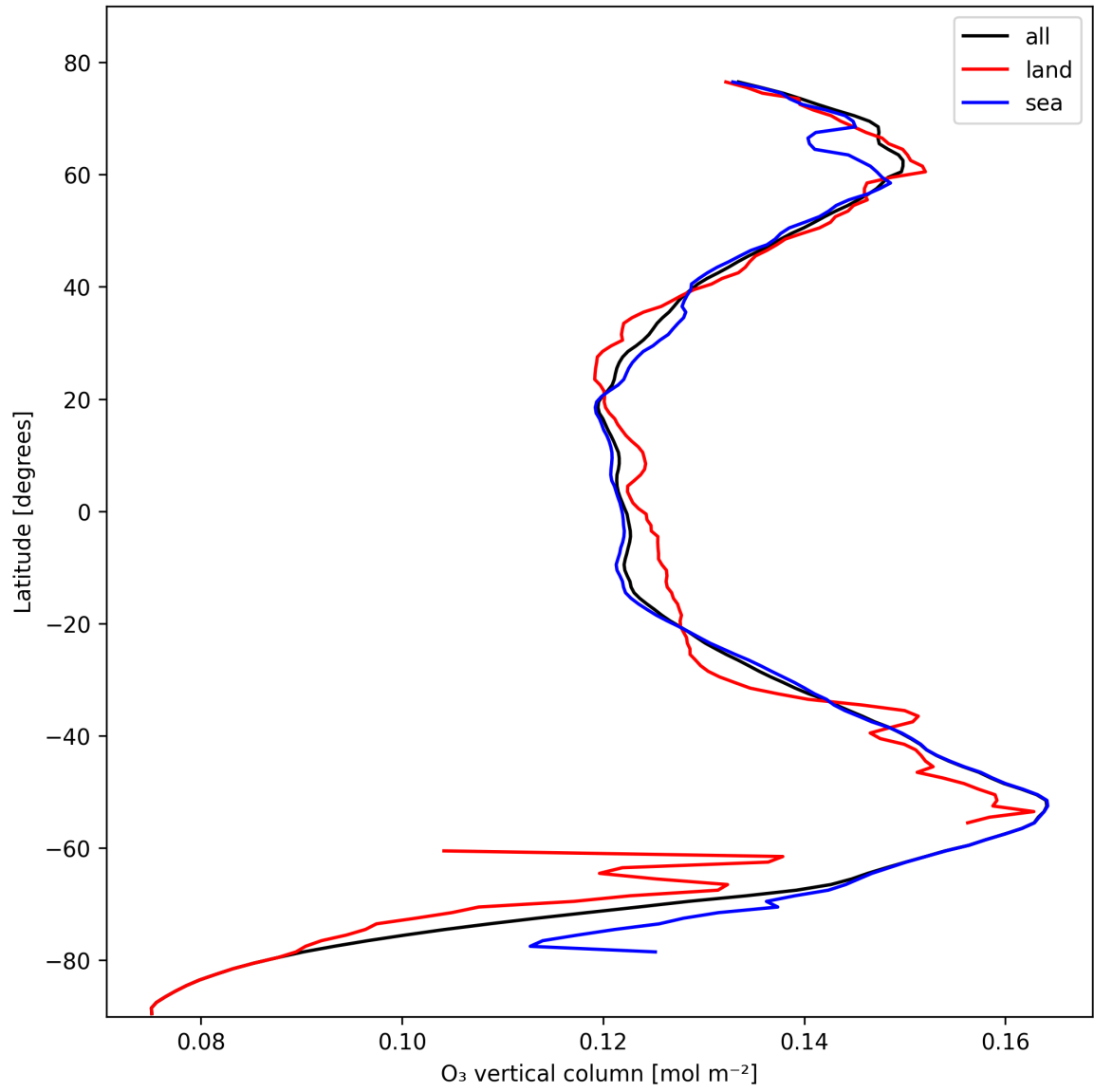
Figure 14: Zonal average of “O 3 vertical column” for 2024-10-24 to 2024-10-26.
