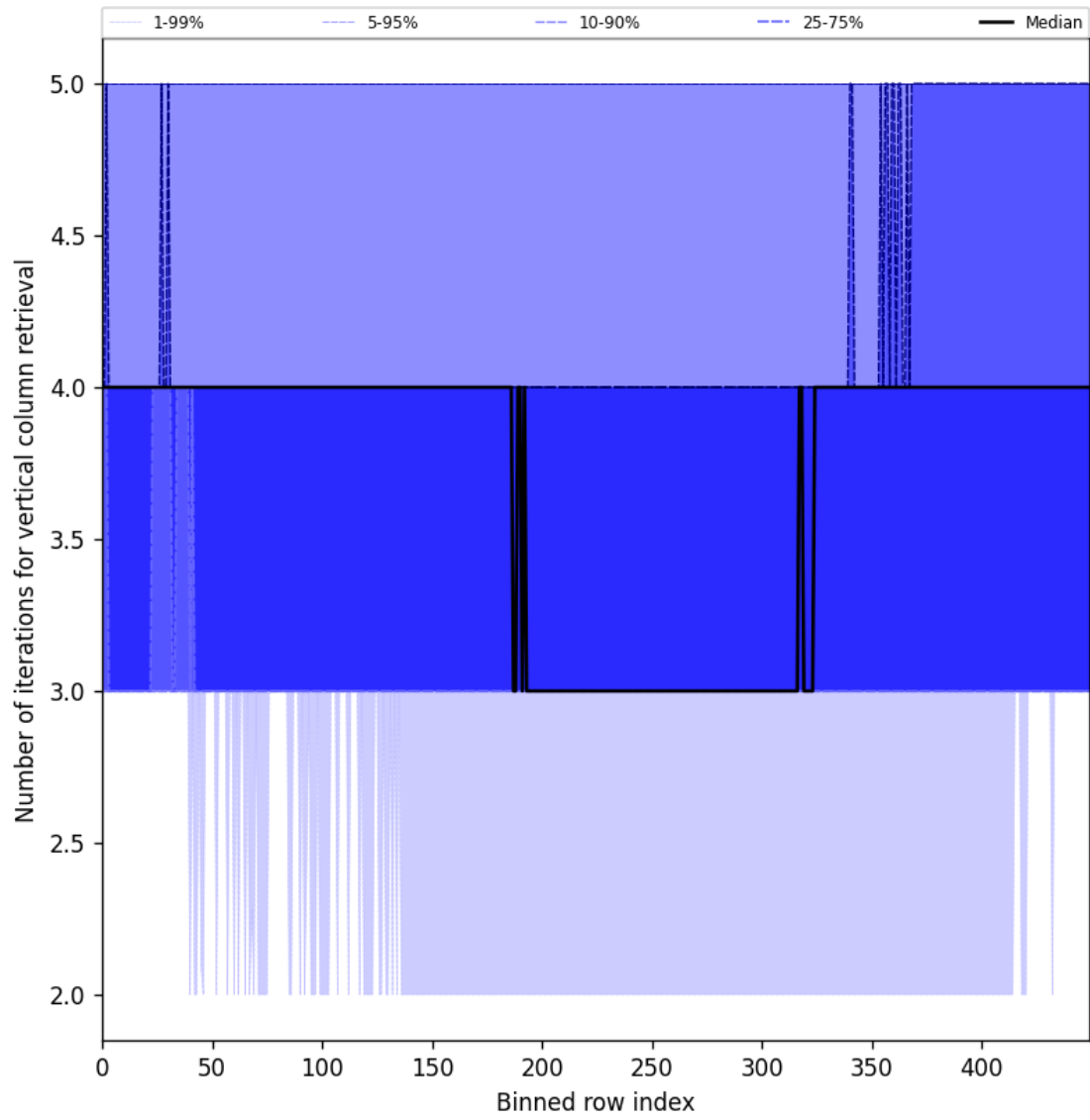
Figure 33: Along track statistics of “Number of iterations for vertical column retrieval” for 2024-10-24 to 2024-10-26
