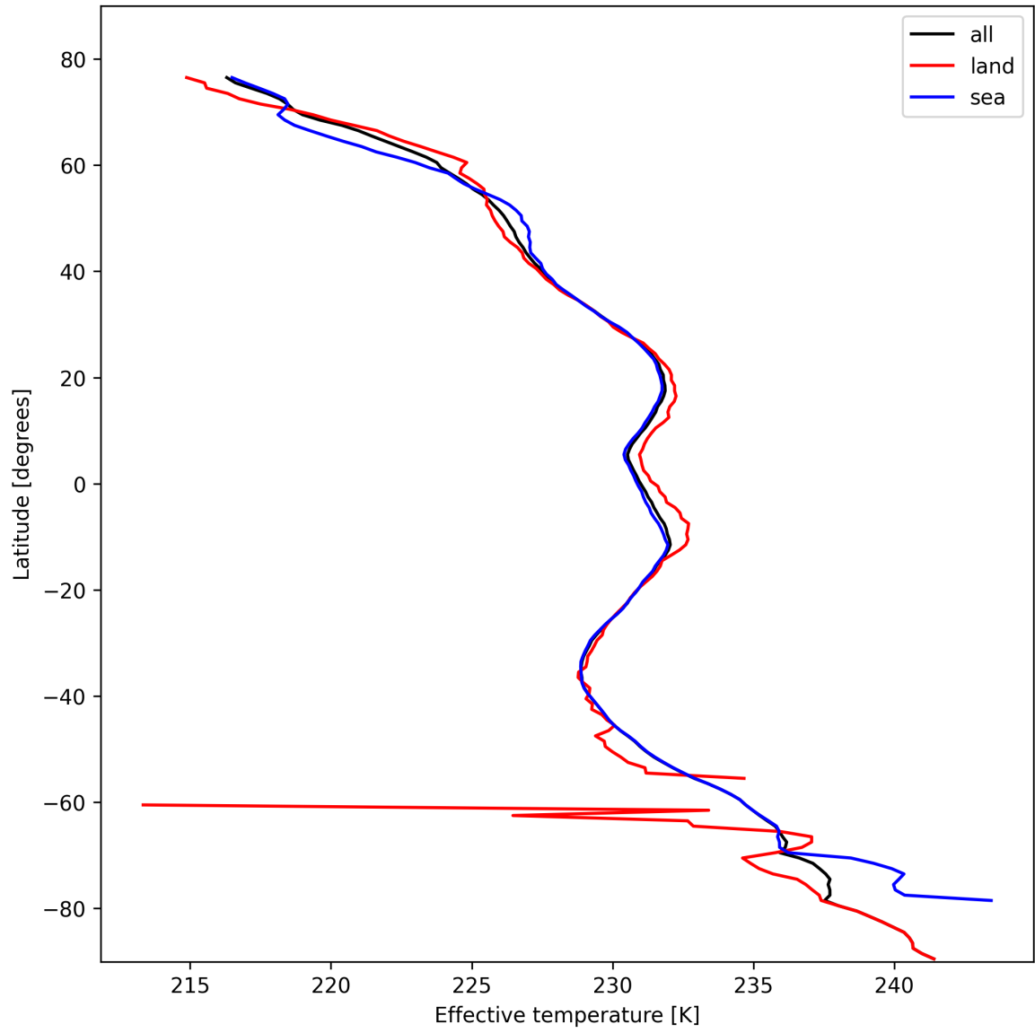
Figure 17: Zonal average of "Effective temperature" for 2024-10-24 to 2024-10-26.
