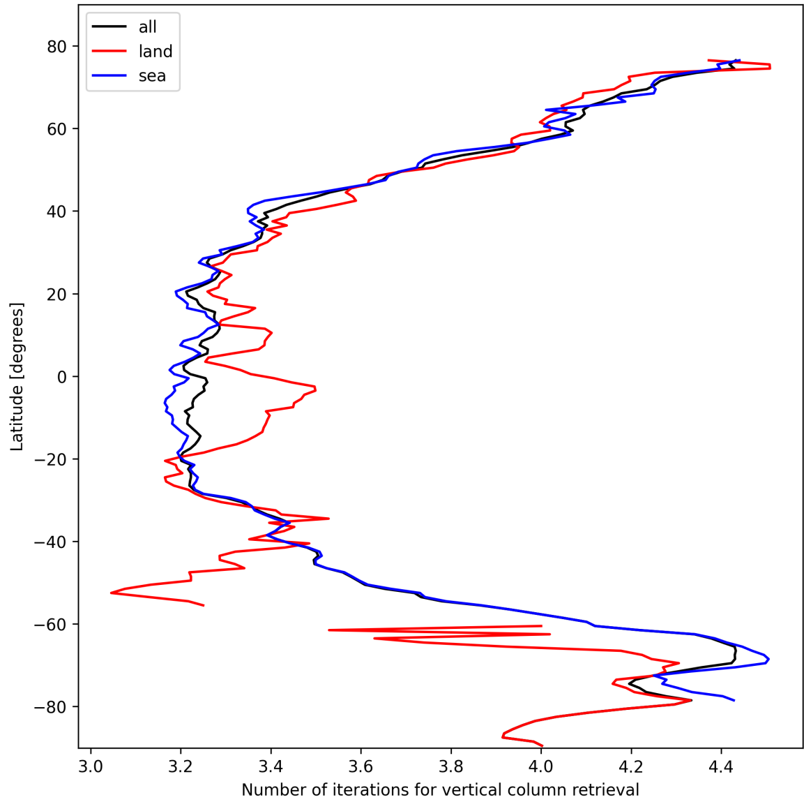
Figure 19: Zonal average of “Number of iterations for vertical column retrieval” for 2024-10-24 to 2024-10-26.
