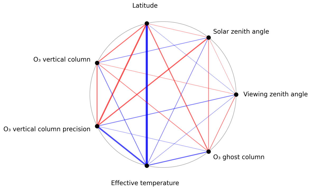
Figure 1: Map of correlation graph for 2024-10-24 to 2024-10-26.
