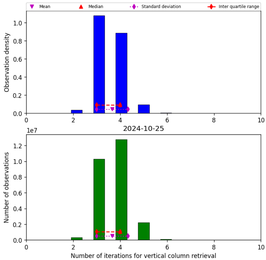
Figure 26: Histogram of “Number of iterations for vertical column retrieval” for 2024-10-24 to 2024-10-26
