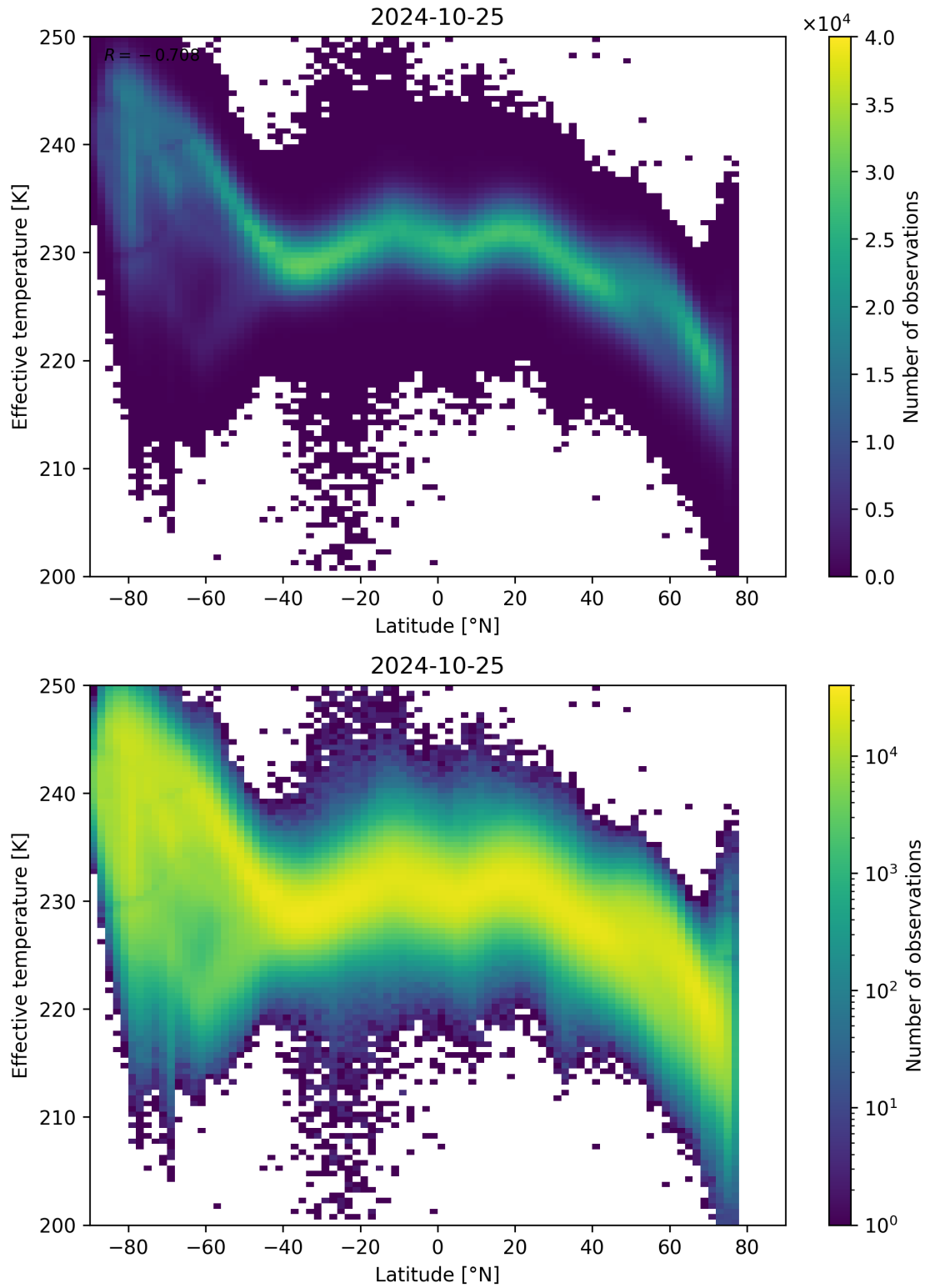
Figure 34: Scatter density plot of “Latitude” against “Effective temperature” for 2024-10-24 to 2024-10-26.
