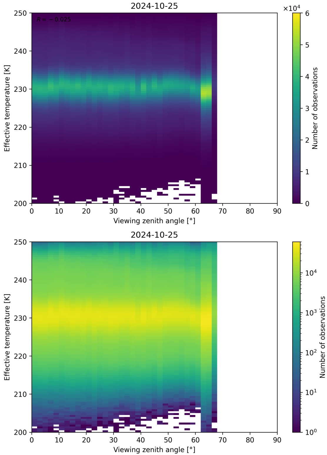
Figure 50: Scatter density plot of “Viewing zenith angle” against “Effective temperature” for 2024-10-24 to 2024-10-26.
