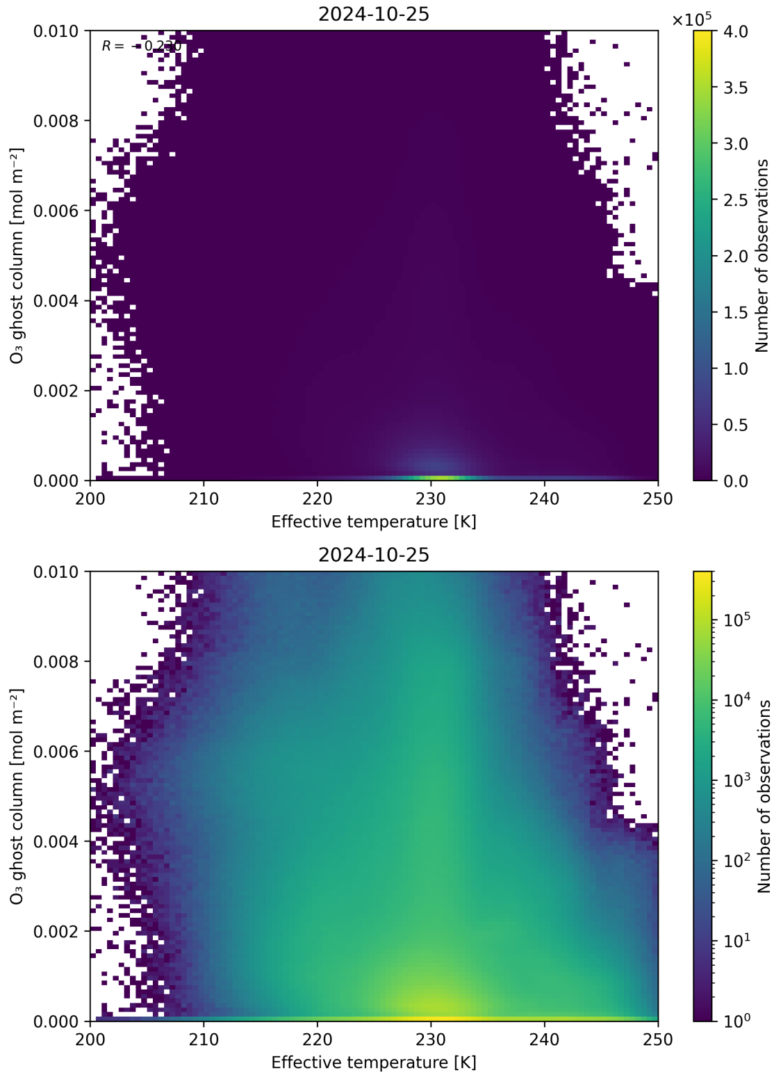
Figure 38: Scatter density plot of “Effective temperature” against “O 3 ghost column” for 2024-10-24 to 2024-10-26.
