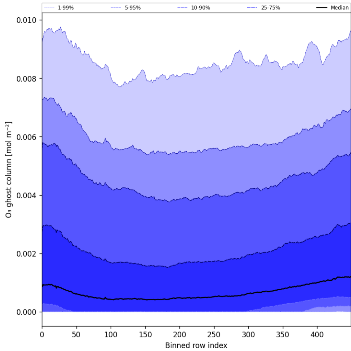
Figure 32: Along track statistics of "O 3 ghost column" for 2024-10-24 to 2024-10-26
