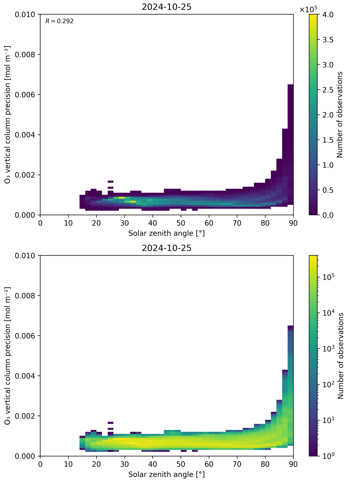
Figure 48: Scatter density plot of “Solar zenith angle” against “O 3 vertical column precision” for 2024-10-24 to 2024-10-26.
