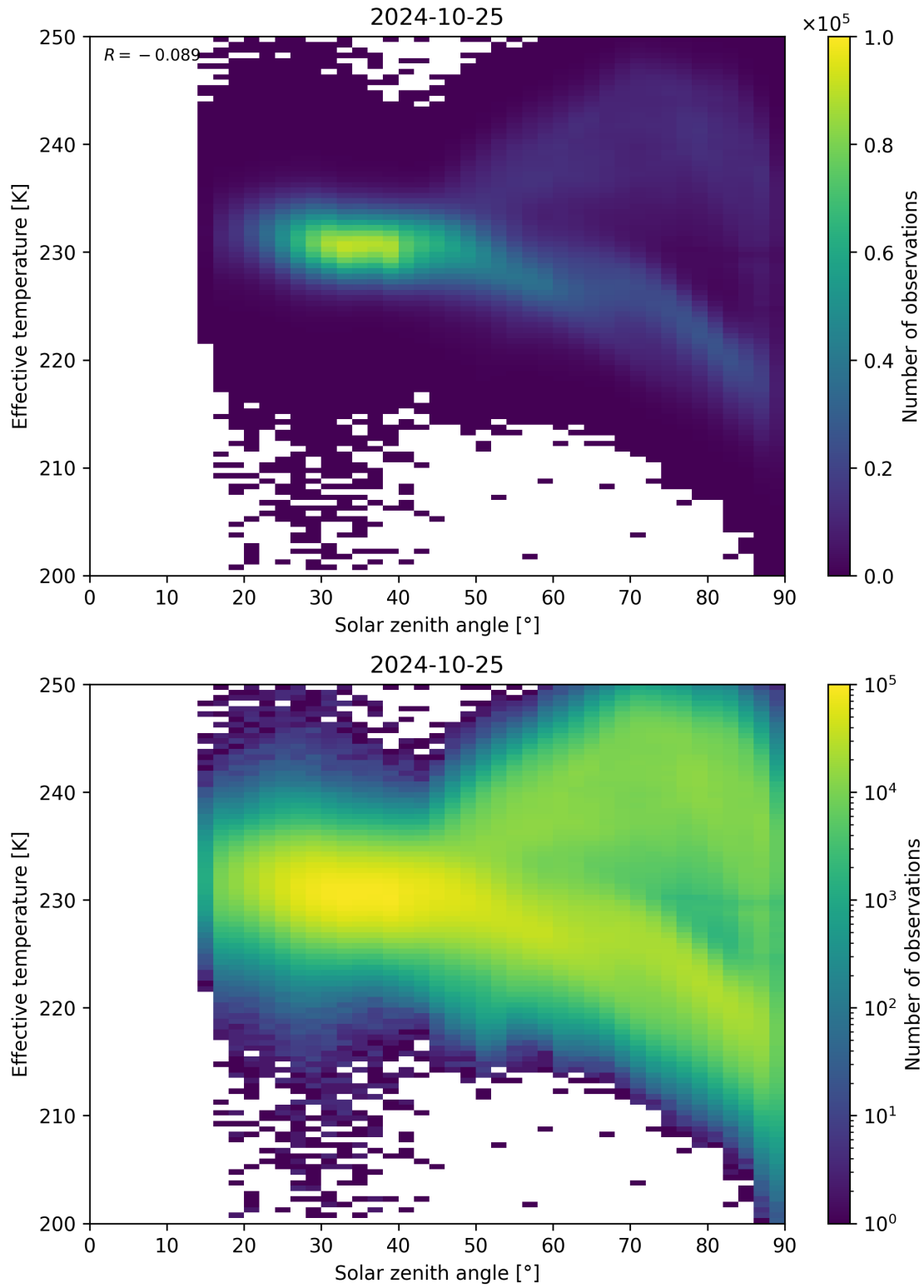
Figure 45: Scatter density plot of “Solar zenith angle” against “Effective temperature” for 2024-10-24 to 2024-10-26.
