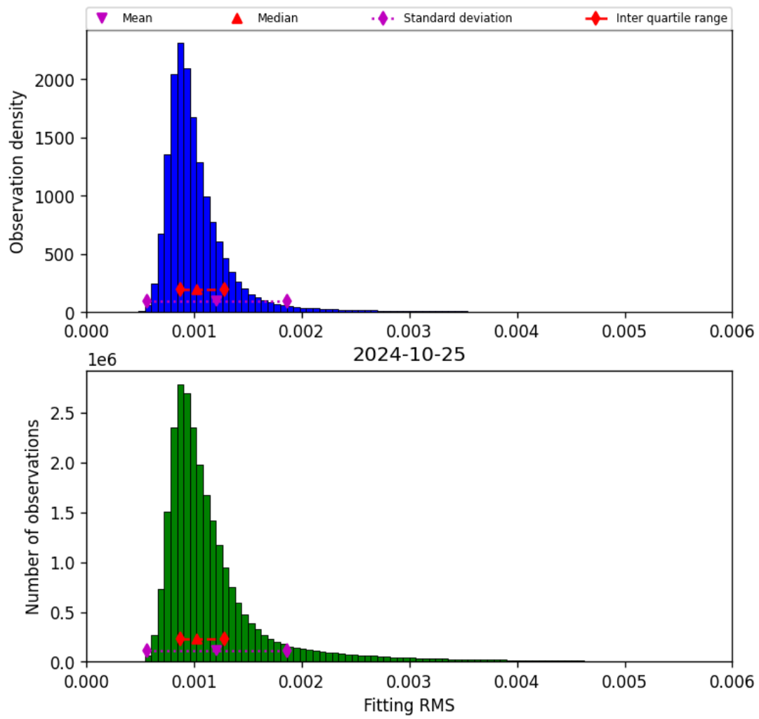
Figure 23: Histogram of “Fitting RMS” for 2024-10-24 to 2024-10-26
