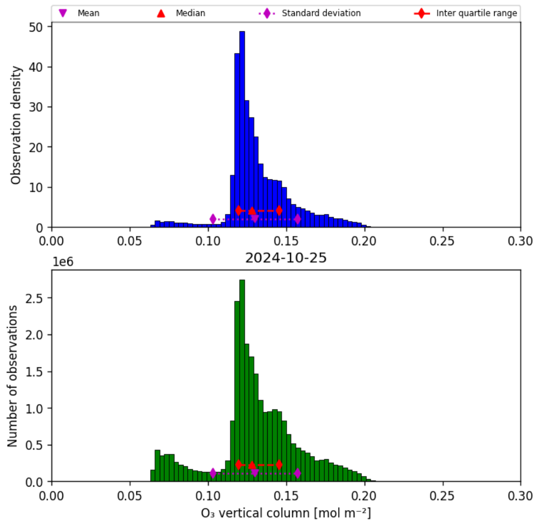
Figure 21: Histogram of “O 3 vertical column” for 2024-10-24 to 2024-10-26
