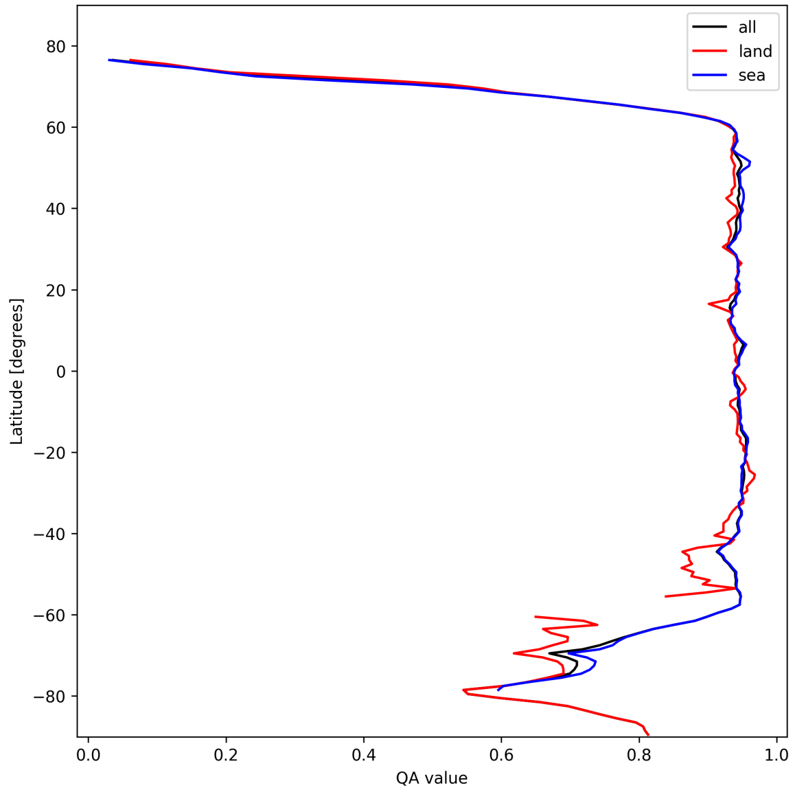
Figure 13: Zonal average of “QA value” for 2024-10-24 to 2024-10-26.
