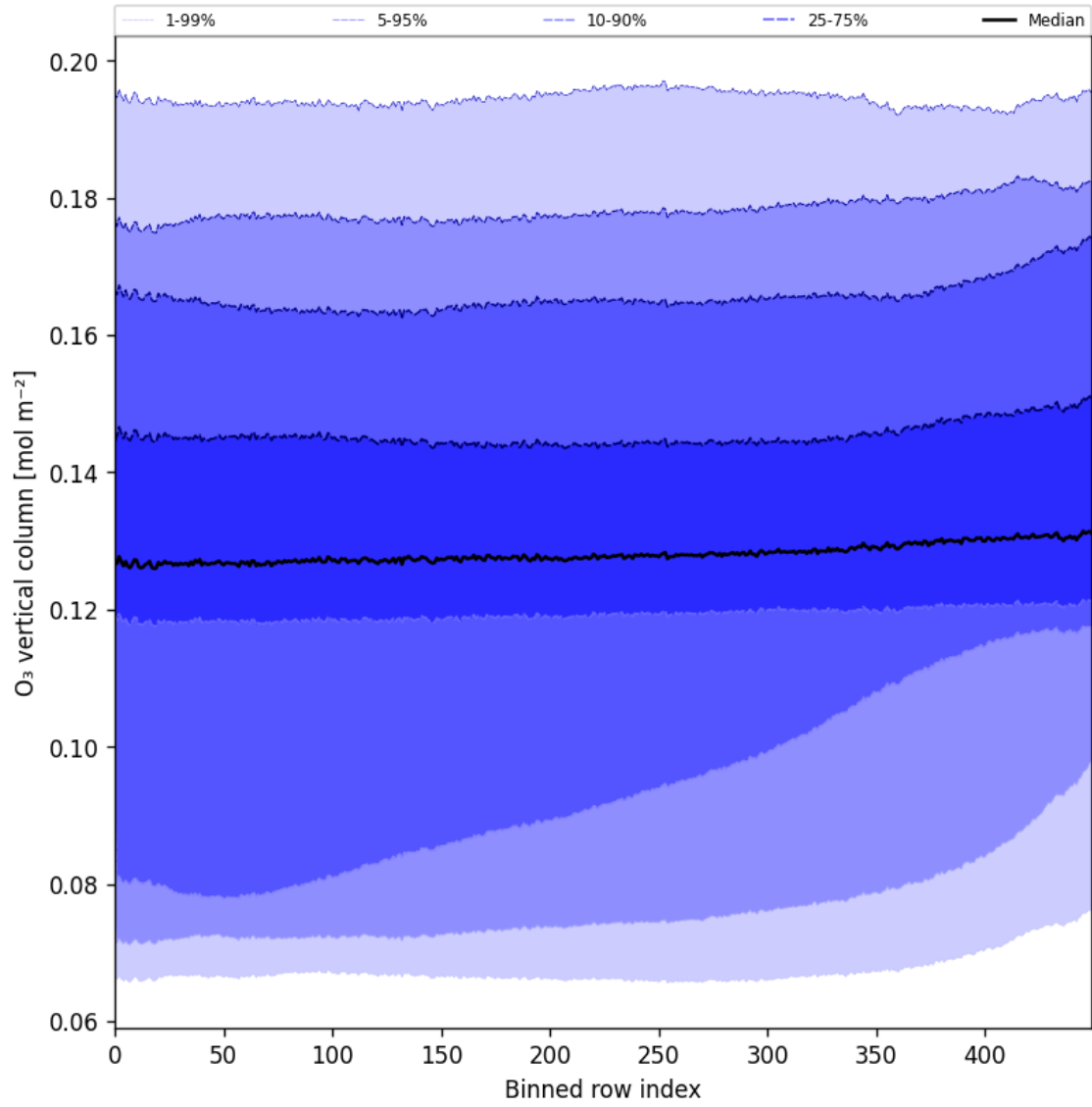
Figure 28: Along track statistics of “O 3 vertical column” for 2024-10-24 to 2024-10-26
