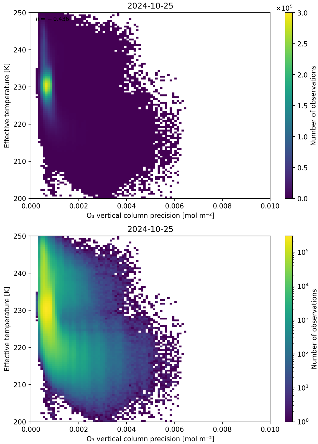
Figure 42: Scatter density plot of “O 3 vertical column precision” against “Effective temperature” for 2024-10-24 to 2024-10-26.
