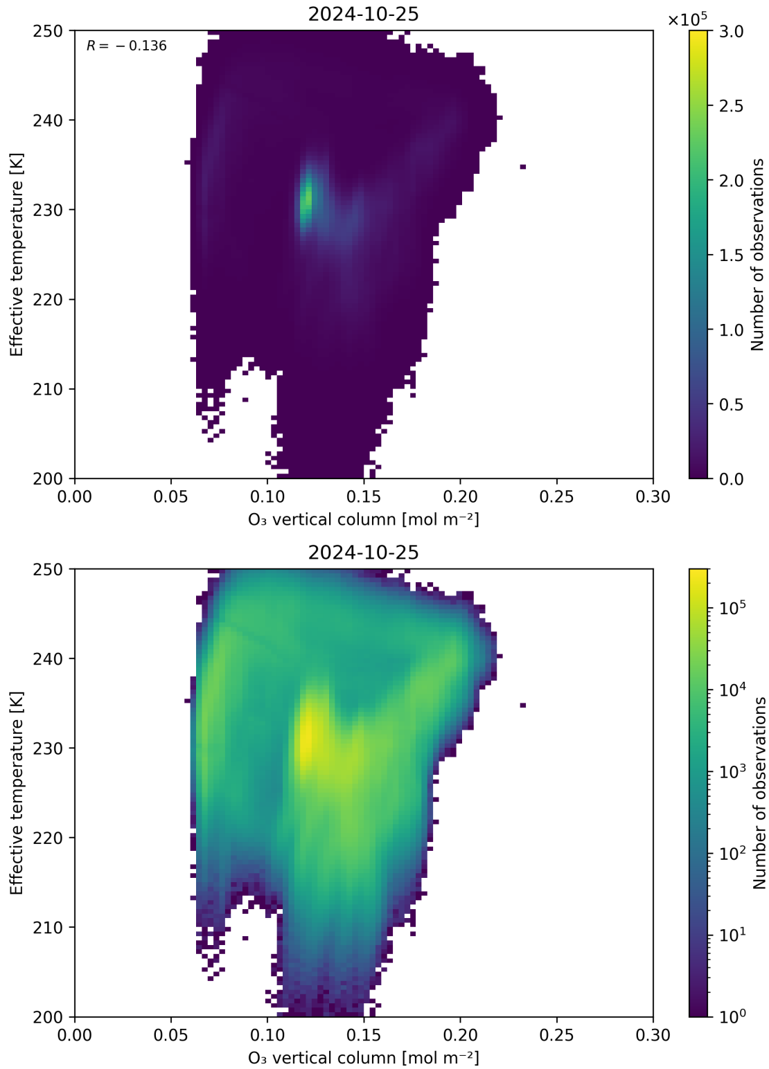
Figure 39: Scatter density plot of “O 3 vertical column” against “Effective temperature” for 2024-10-24 to 2024-10-26.
