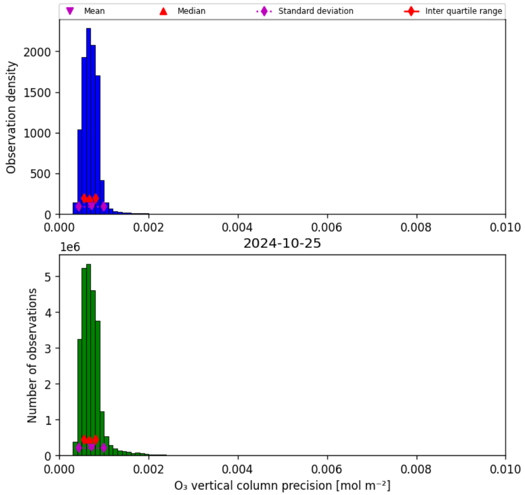
Figure 22: Histogram of “O 3 vertical column precision” for 2024-10-24 to 2024-10-26
