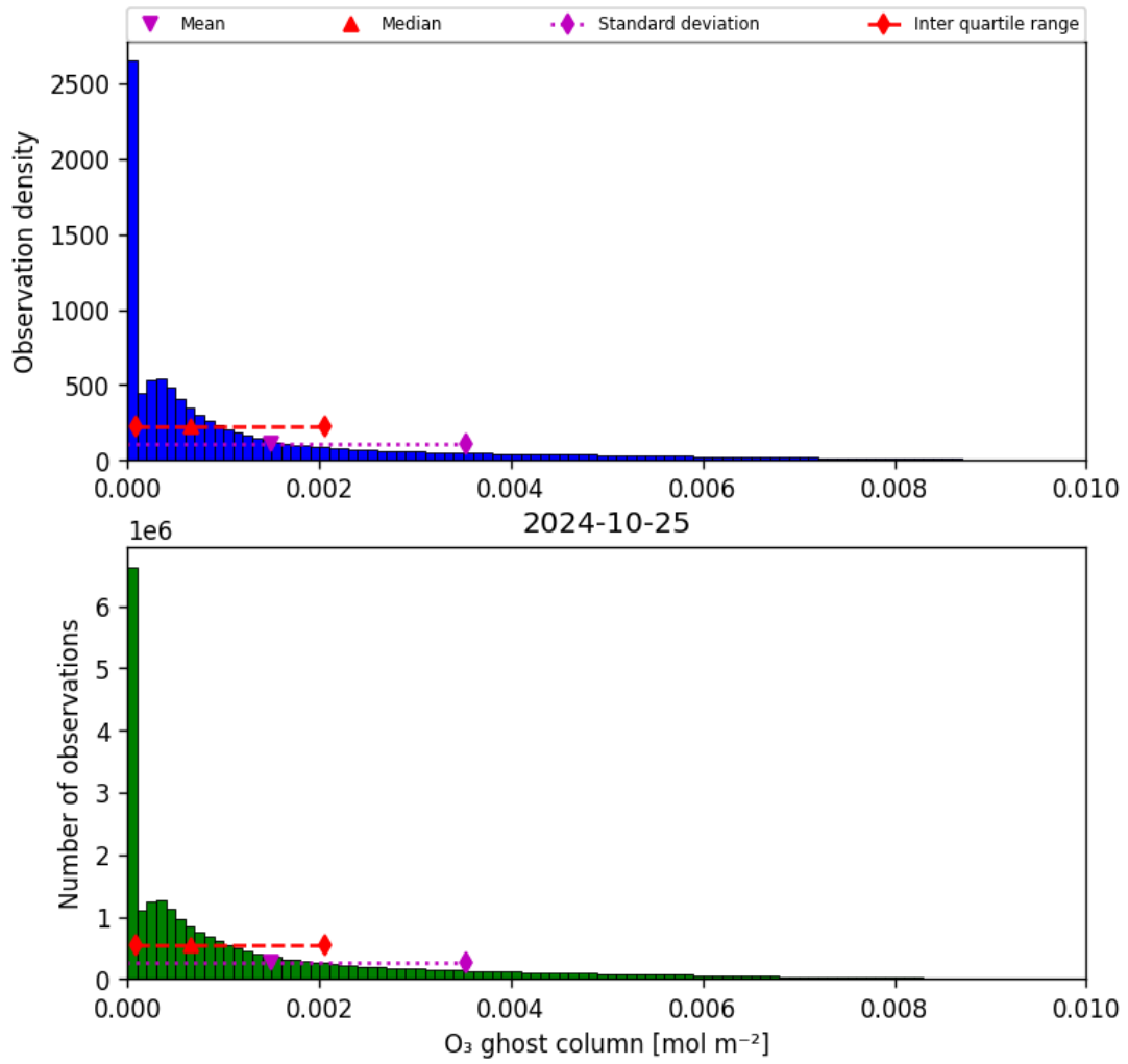
Figure 25: Histogram of “O 3 ghost column” for 2024-10-24 to 2024-10-26
