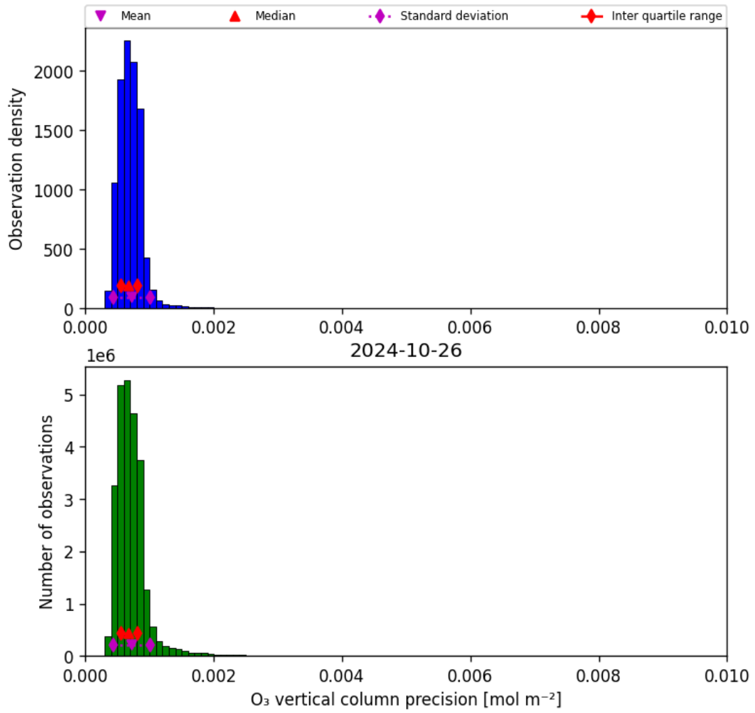
Figure 22: Histogram of “O 3 vertical column precision” for 2024-10-25 to 2024-10-27
