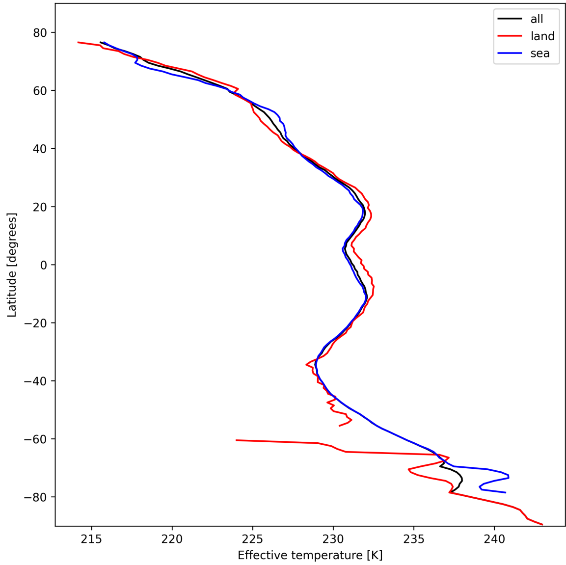
Figure 17: Zonal average of “Effective temperature” for 2024-10-25 to 2024-10-27.
