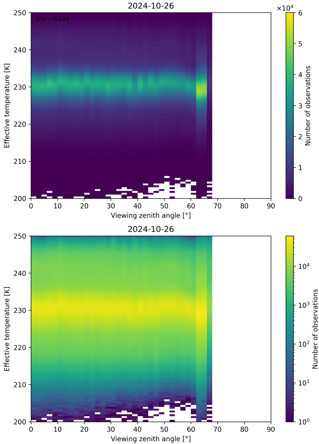
Figure 50: Scatter density plot of “Viewing zenith angle” against “Effective temperature” for 2024-10-25 to 2024-10-27.
