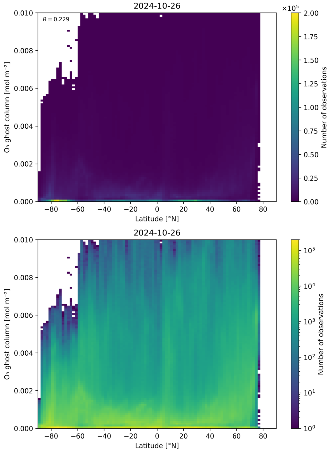
Figure 35: Scatter density plot of “Latitude” against “O 3 ghost column” for 2024-10-25 to 2024-10-27.
