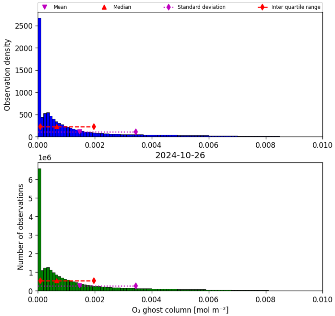
Figure 25: Histogram of “O 3 ghost column” for 2024-10-25 to 2024-10-27
