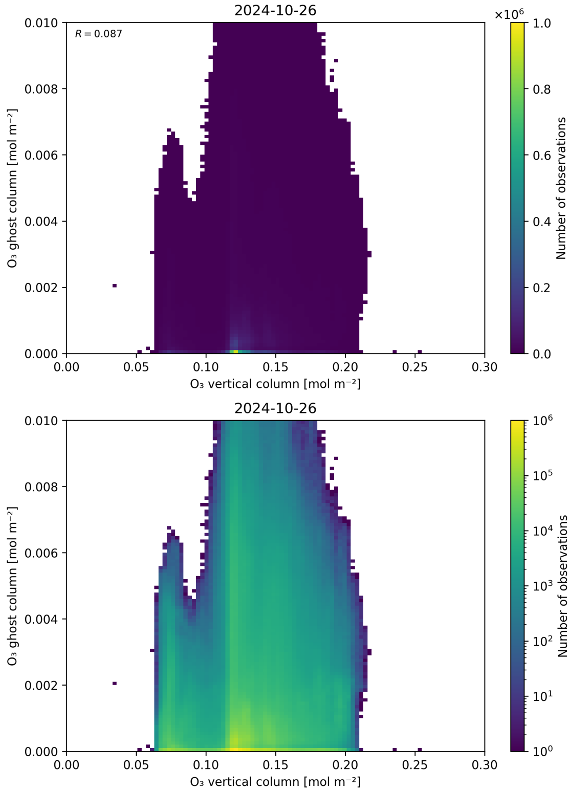
Figure 40: Scatter density plot of “O 3 vertical column” against “O 3 ghost column” for 2024-10-25 to 2024-10-27.
