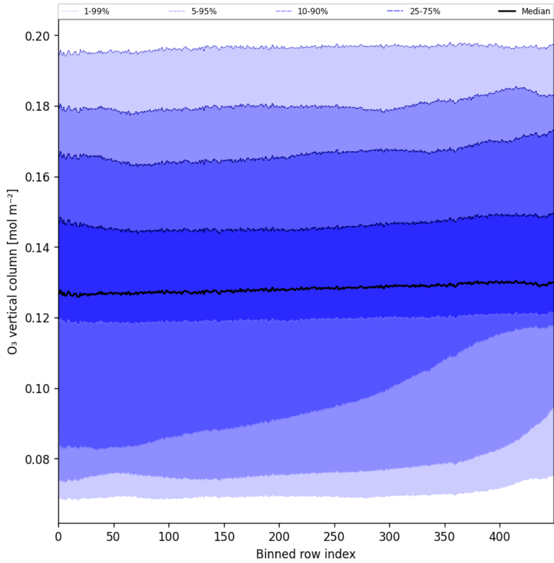
Figure 28: Along track statistics of “O 3 vertical column” for 2024-10-25 to 2024-10-27
