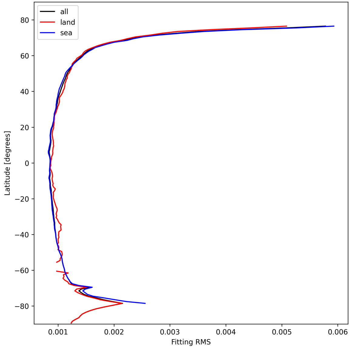
Figure 16: Zonal average of “Fitting RMS” for 2024-10-25 to 2024-10-27.
