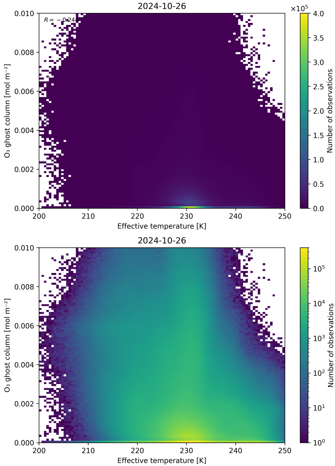
Figure 38: Scatter density plot of “Effective temperature” against “O 3 ghost column” for 2024-10-25 to 2024-10-27.
