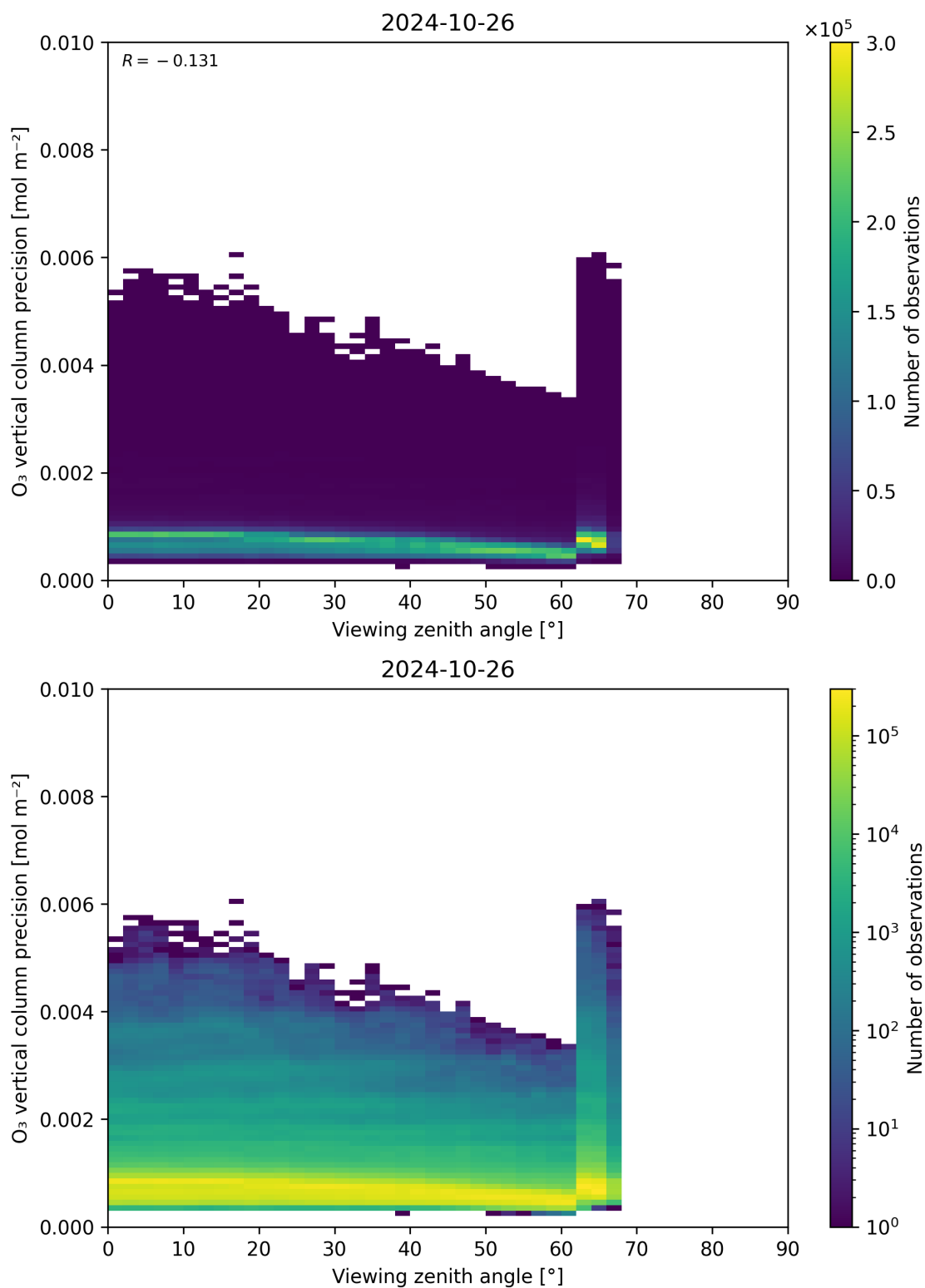
Figure 53: Scatter density plot of “Viewing zenith angle” against “O 3 vertical column precision” for 2024-10-25 to 2024-10-27.
