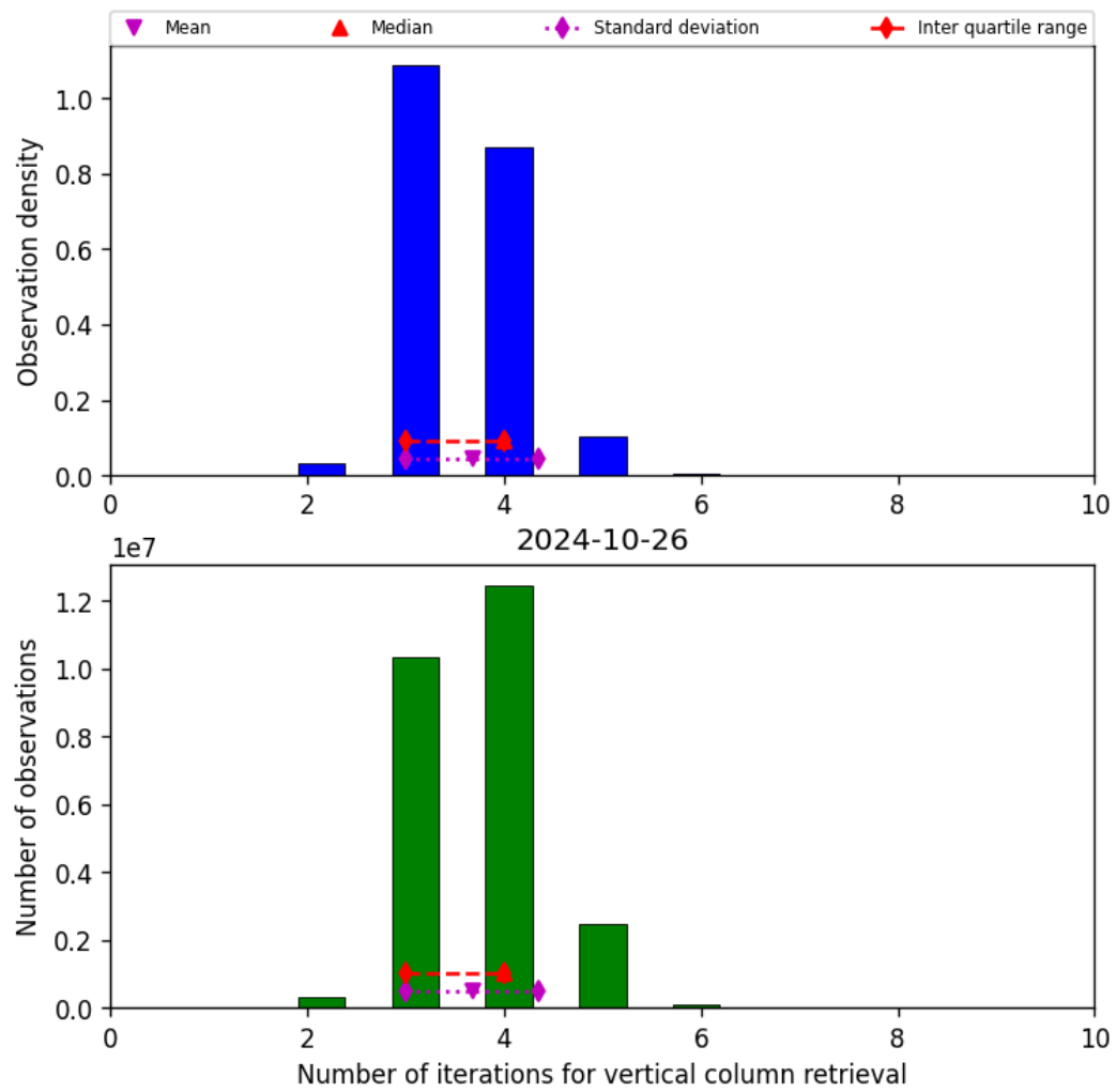
Figure 26: Histogram of “Number of iterations for vertical column retrieval” for 2024-10-25 to 2024-10-27
