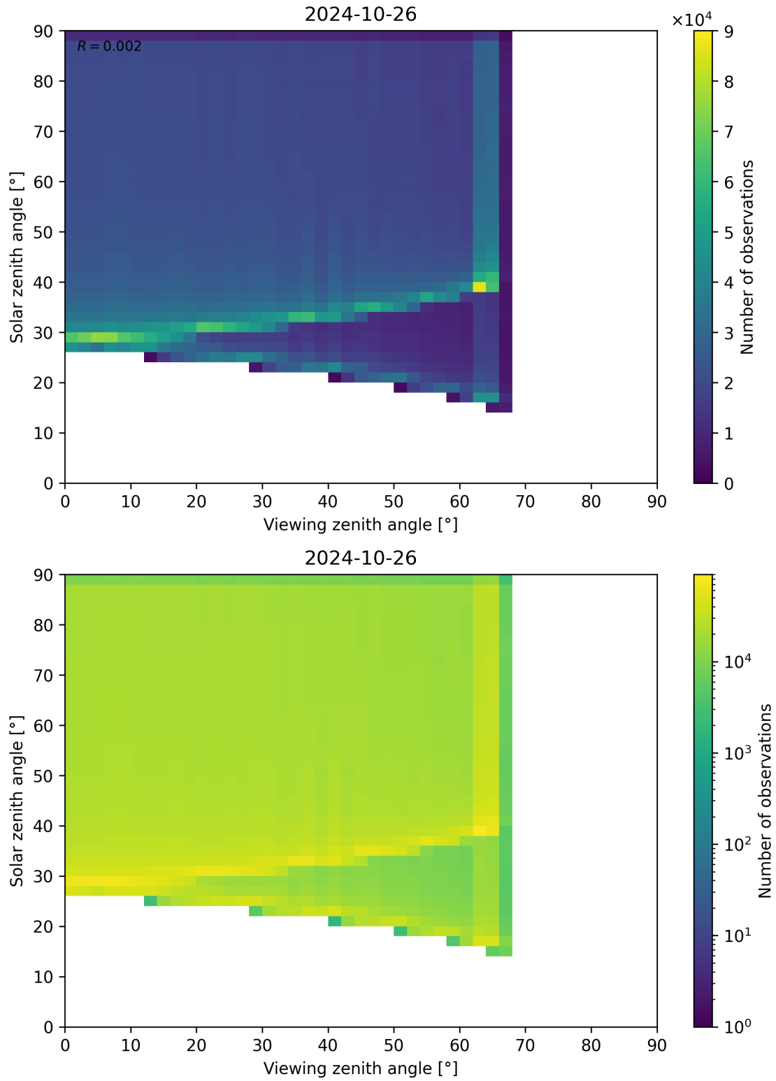
Figure 54: Scatter density plot of “Viewing zenith angle” against “Solar zenith angle” for 2024-10-25 to 2024-10-27.
