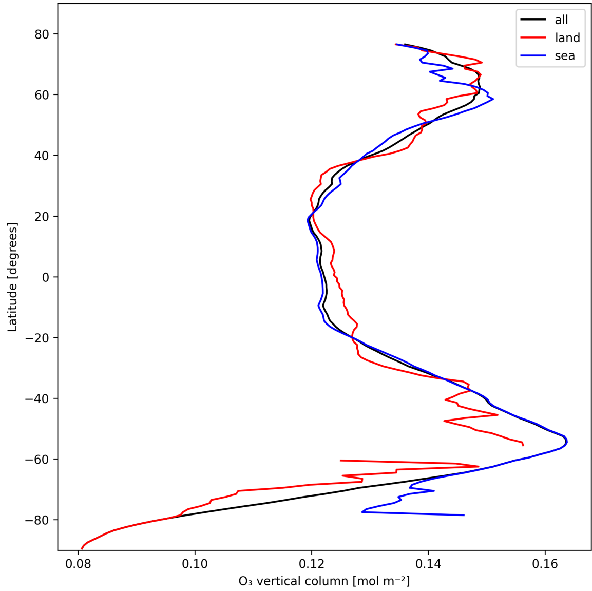
Figure 14: Zonal average of “O 3 vertical column” for 2024-10-25 to 2024-10-27.
