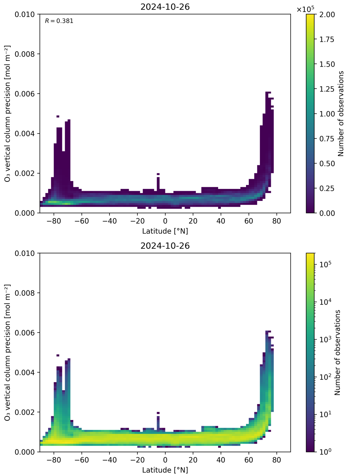
Figure 37: Scatter density plot of “Latitude” against “O 3 vertical column precision” for 2024-10-25 to 2024-10-27.
