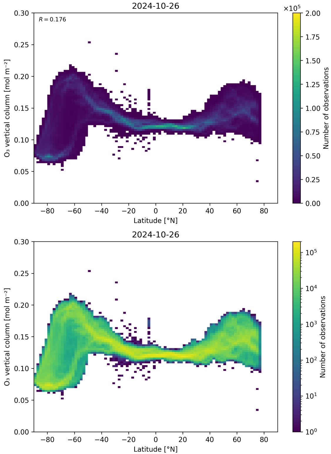
Figure 36: Scatter density plot of “Latitude” against “O 3 vertical column” for 2024-10-25 to 2024-10-27.
