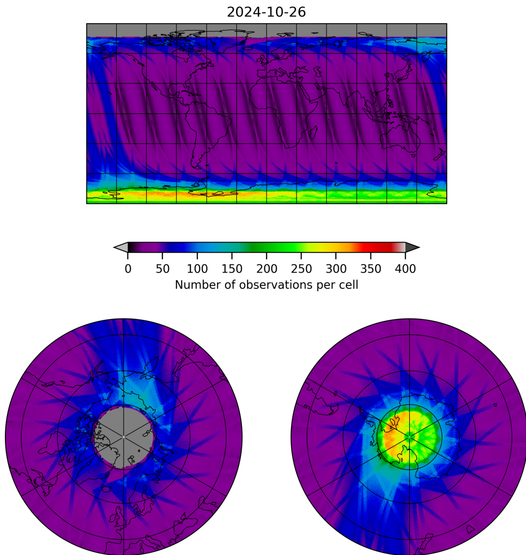
Figure 12: Map of the number of observations for 2024-10-25 to 2024-10-27
