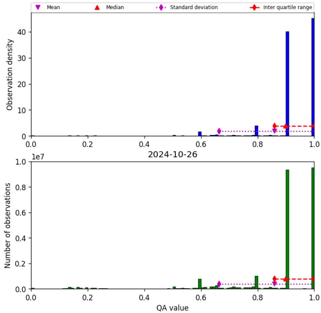
Figure 20: Histogram of “QA value” for 2024-10-25 to 2024-10-27
