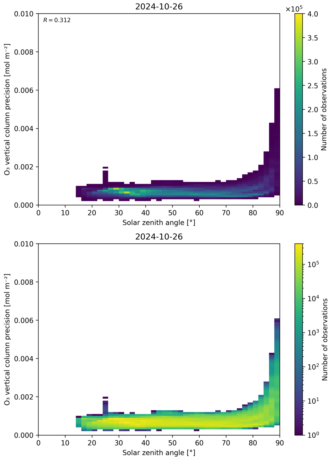
Figure 48: Scatter density plot of “Solar zenith angle” against “O 3 vertical column precision” for 2024-10-25 to 2024-10-27.
