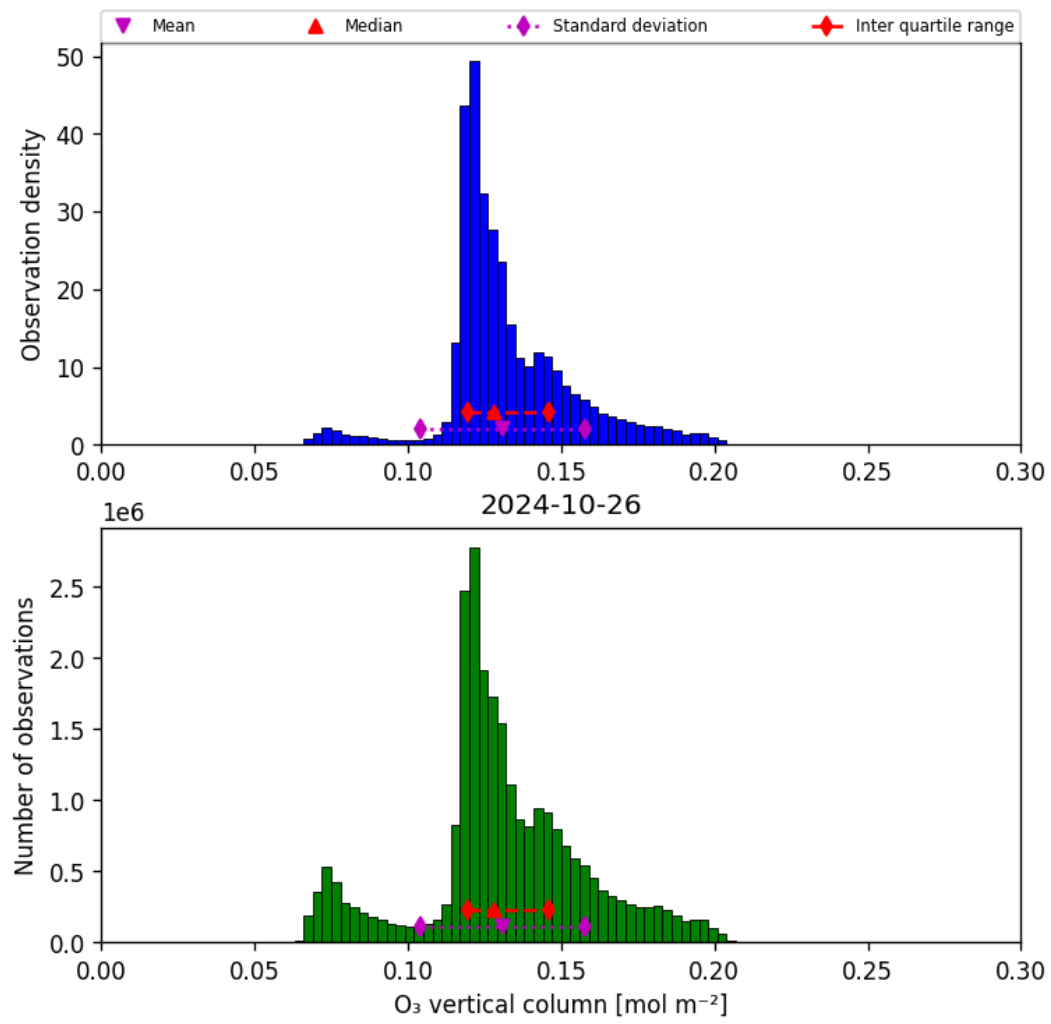
Figure 21: Histogram of “O 3 vertical column” for 2024-10-25 to 2024-10-27
