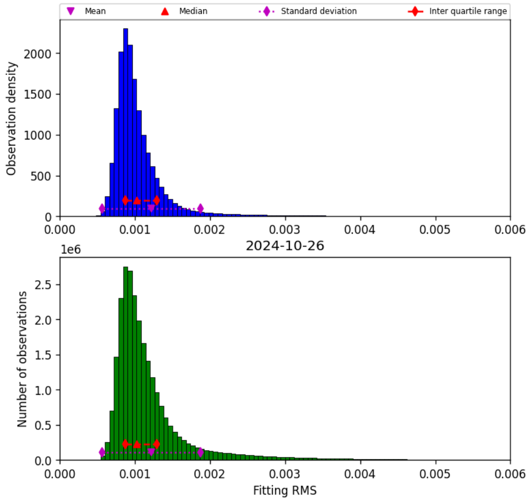
Figure 23: Histogram of “Fitting RMS” for 2024-10-25 to 2024-10-27
