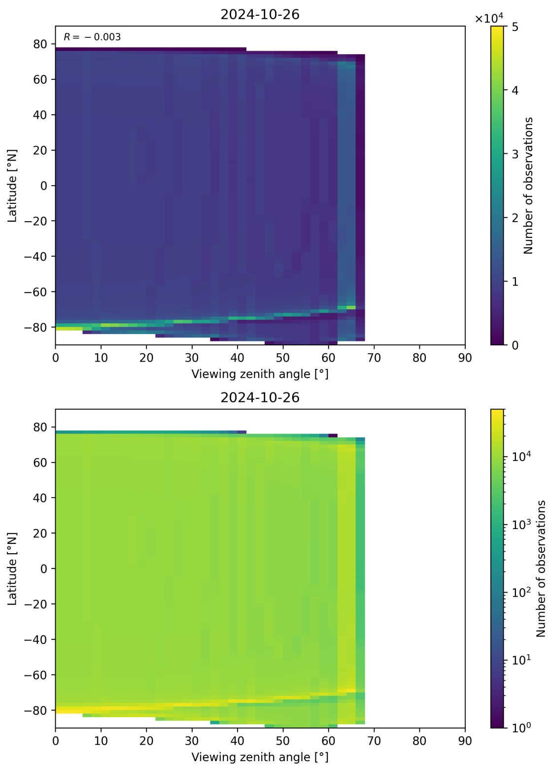
Figure 49: Scatter density plot of “Viewing zenith angle” against “Latitude” for 2024-10-25 to 2024-10-27.
