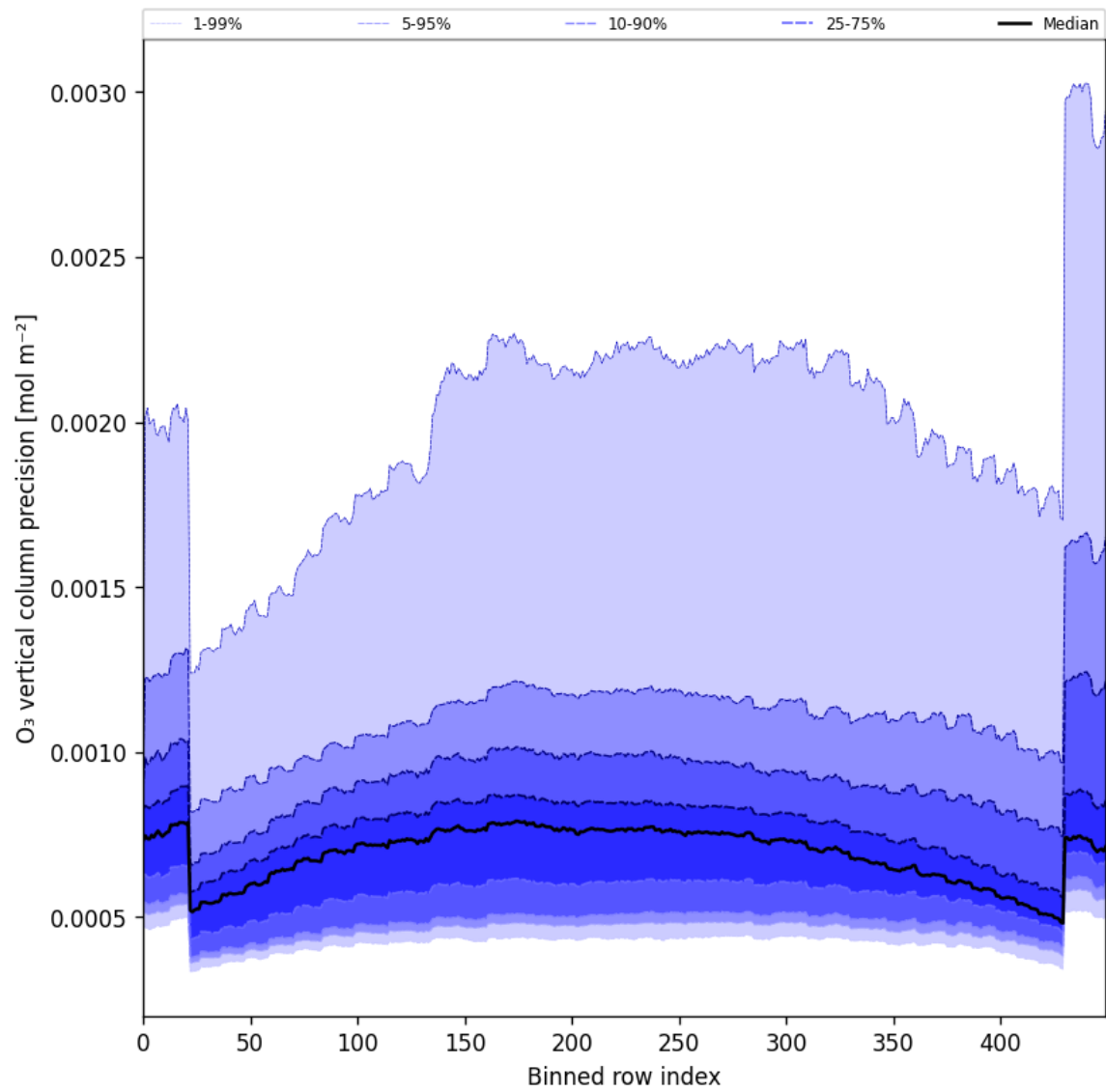
Figure 29: Along track statistics of “O 3 vertical column precision” for 2024-10-25 to 2024-10-27
