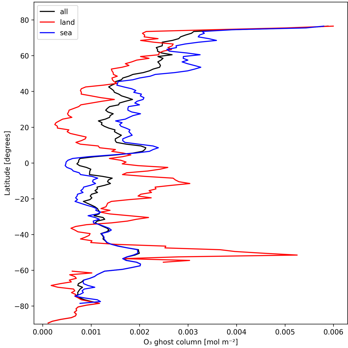
Figure 18: Zonal average of "O 3 ghost column" for 2024-10-25 to 2024-10-27.
