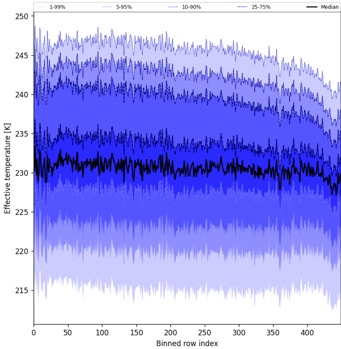
Figure 31: Along track statistics of “Effective temperature” for 2024-10-25 to 2024-10-27
