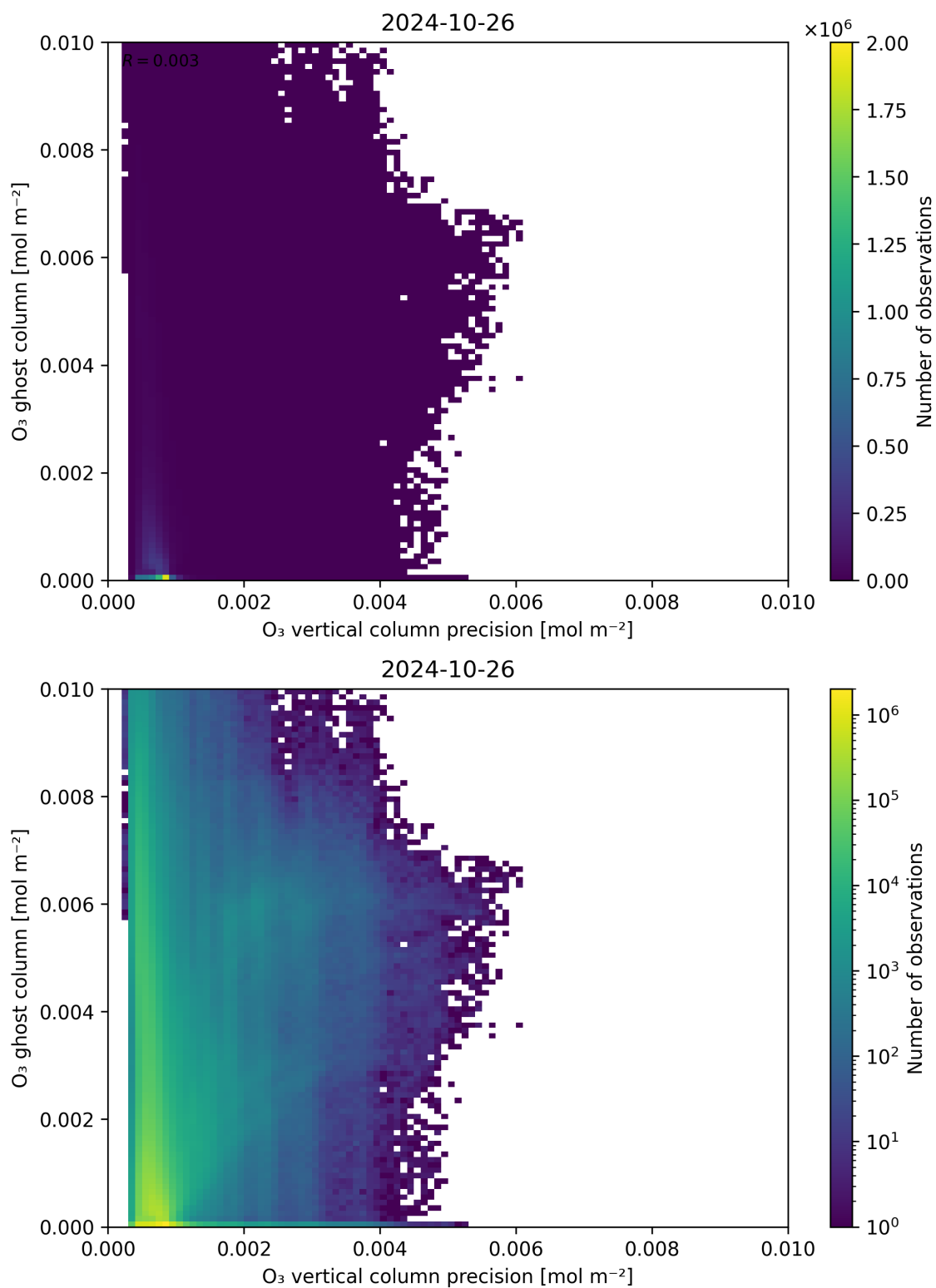
Figure 43: Scatter density plot of “ \text{O}_3 vertical column precision” against “ \text{O}_3 ghost column” for 2024-10-25 to 2024-10-27.
