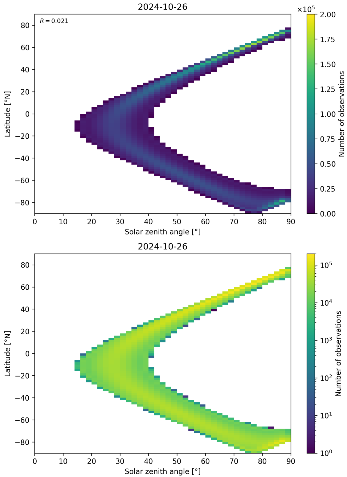
Figure 44: Scatter density plot of “Solar zenith angle” against “Latitude” for 2024-10-25 to 2024-10-27.
