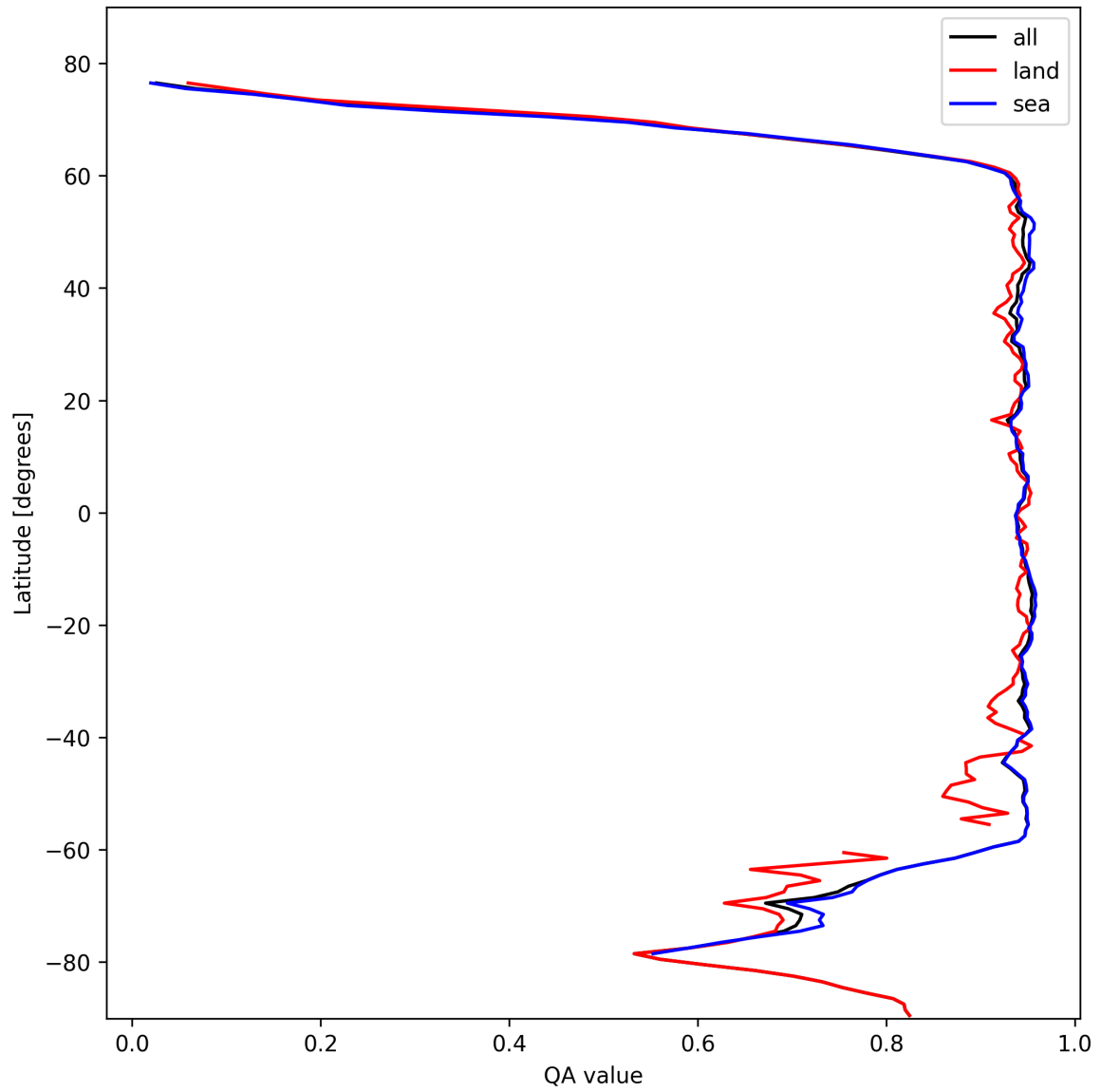
Figure 13: Zonal average of “QA value” for 2024-10-25 to 2024-10-27.
