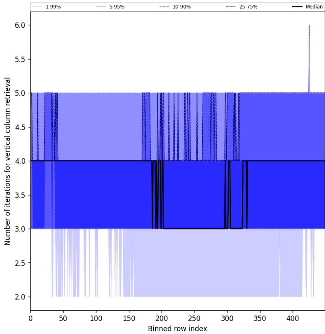
Figure 33: Along track statistics of “Number of iterations for vertical column retrieval” for 2024-10-25 to 2024-10-27
