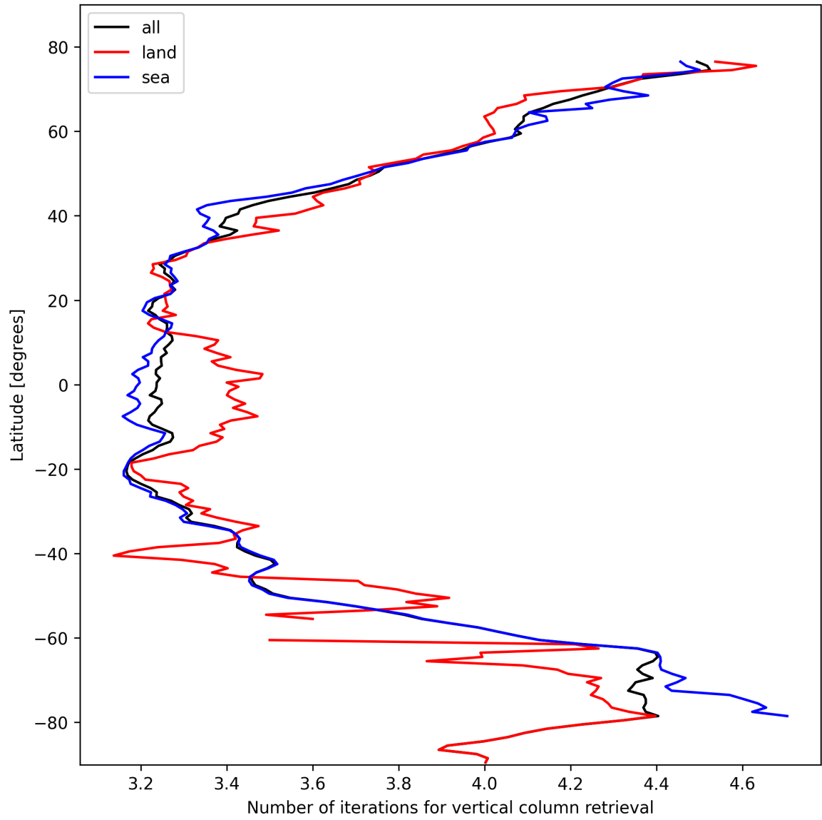
Figure 19: Zonal average of “Number of iterations for vertical column retrieval” for 2024-10-25 to 2024-10-27.
