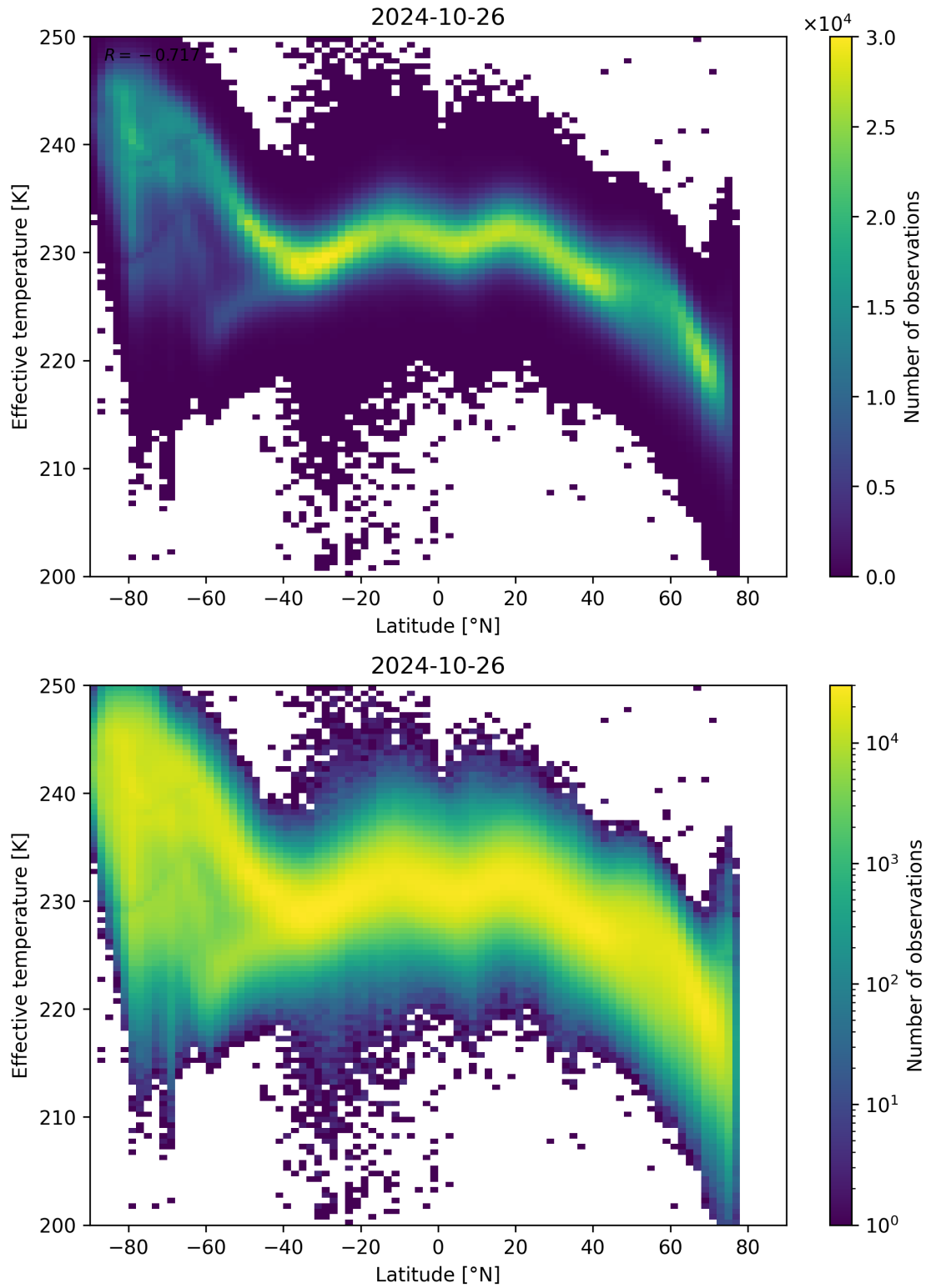
Figure 34: Scatter density plot of “Latitude” against “Effective temperature” for 2024-10-25 to 2024-10-27.
