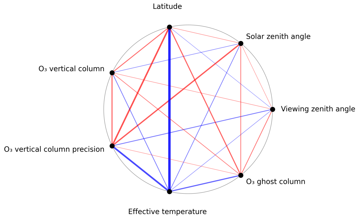
Figure 1: Map of correlation graph for 2024-10-25 to 2024-10-27.
