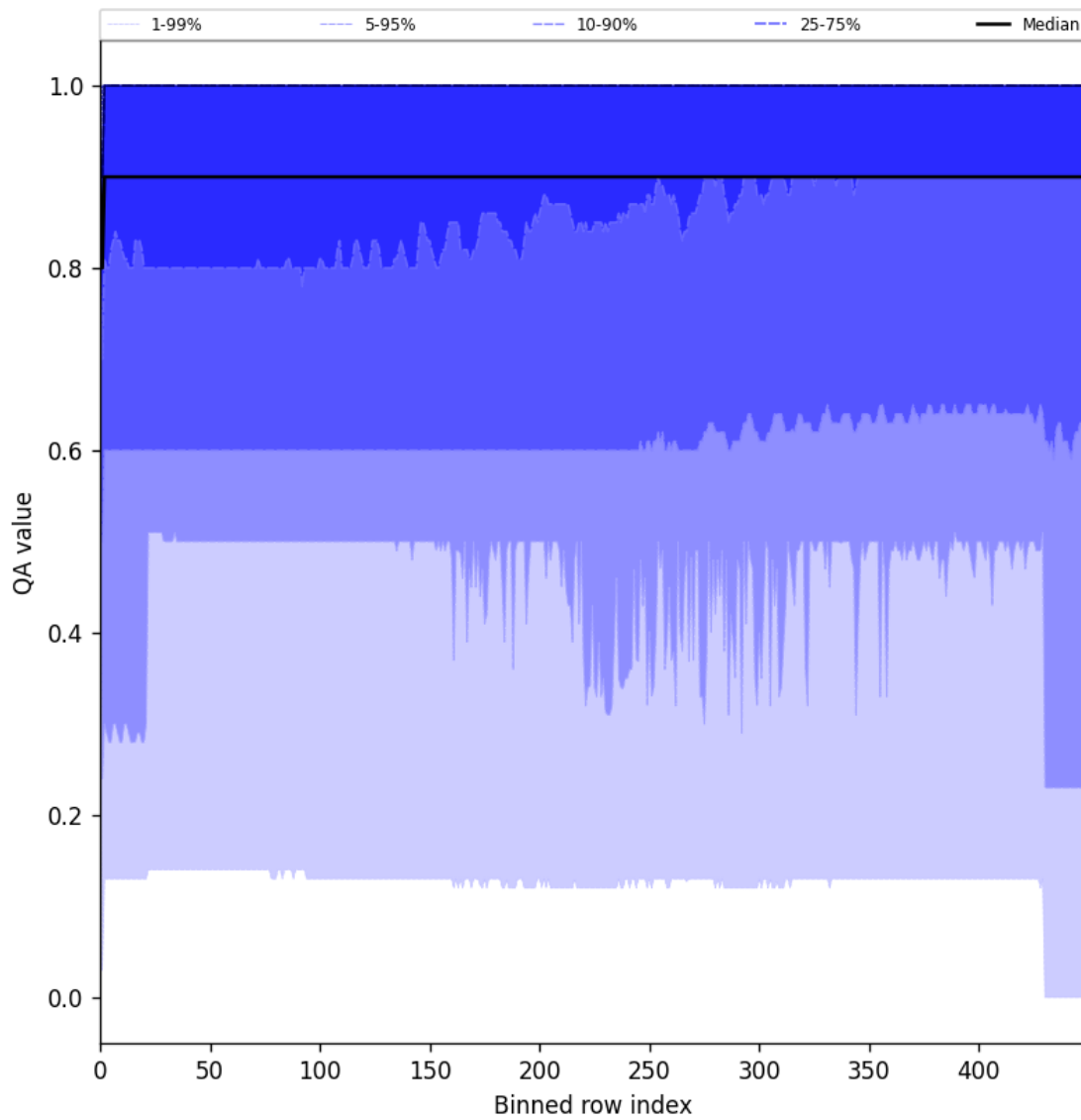
Figure 27: Along track statistics of “QA value” for 2024-10-25 to 2024-10-27
