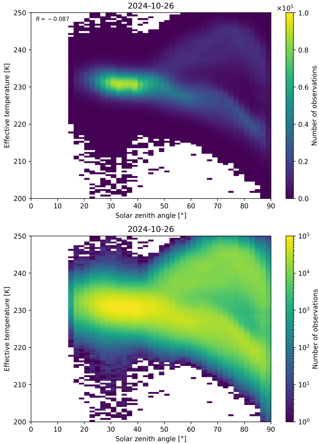
Figure 45: Scatter density plot of “Solar zenith angle” against “Effective temperature” for 2024-10-25 to 2024-10-27.
