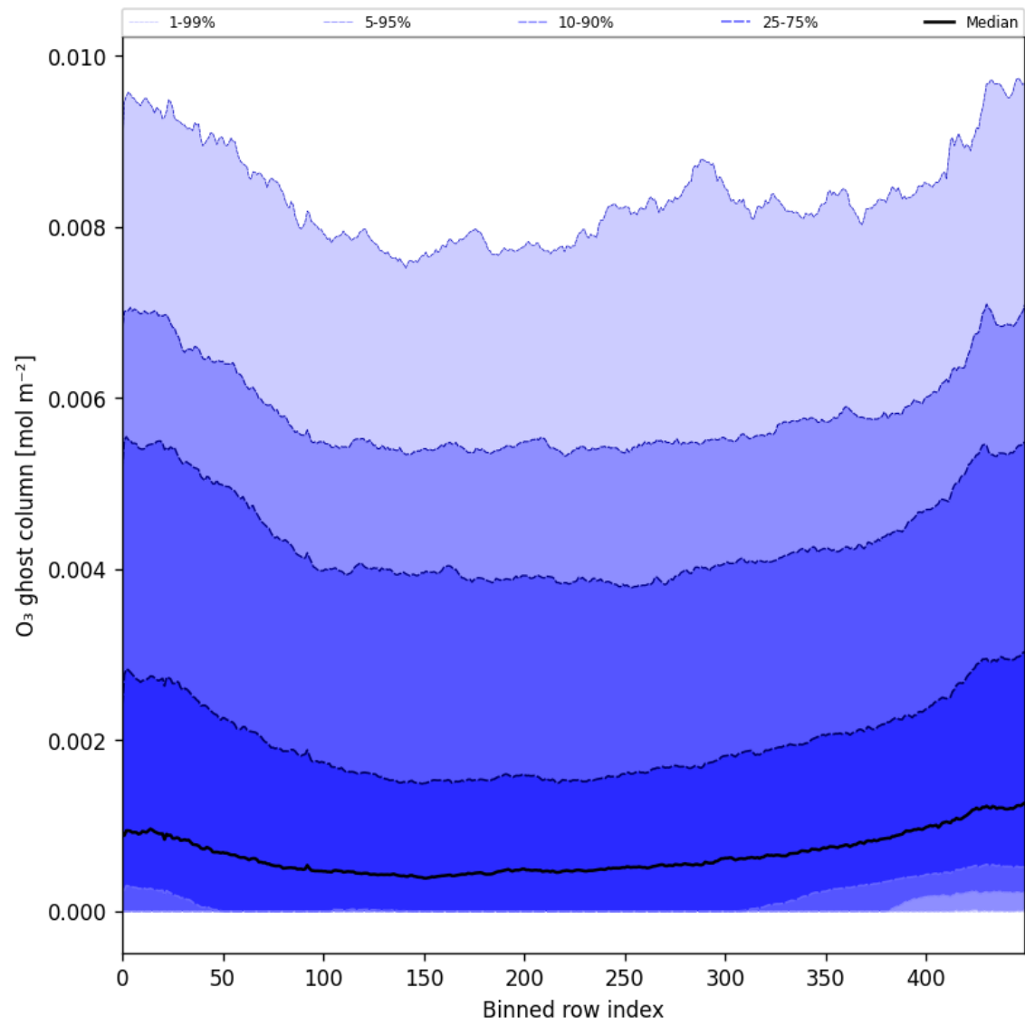
Figure 32: Along track statistics of “O 3 ghost column” for 2024-10-25 to 2024-10-27
