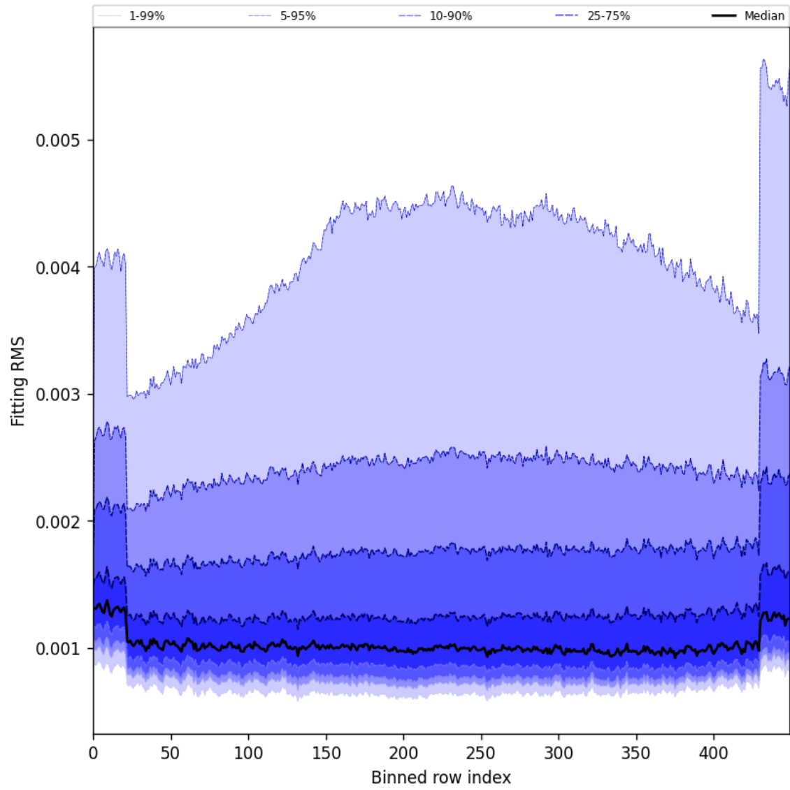
Figure 30: Along track statistics of “Fitting RMS” for 2024-10-25 to 2024-10-27
