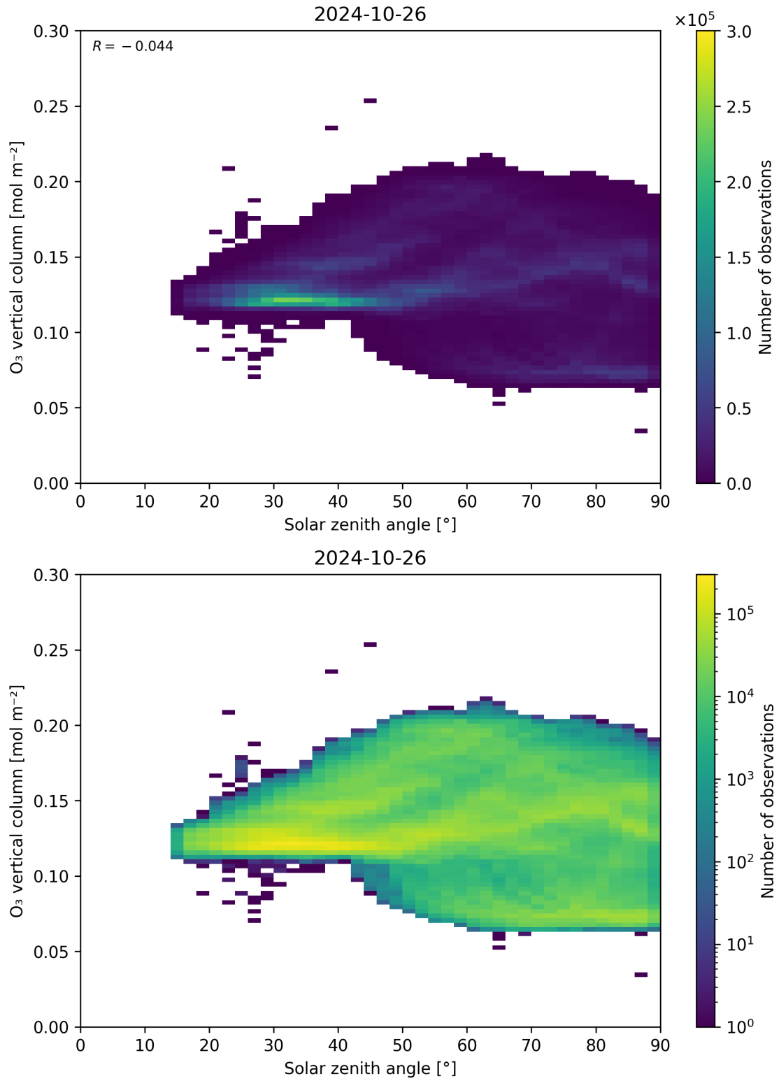
Figure 47: Scatter density plot of “Solar zenith angle” against “O 3 vertical column” for 2024-10-25 to 2024-10-27.
