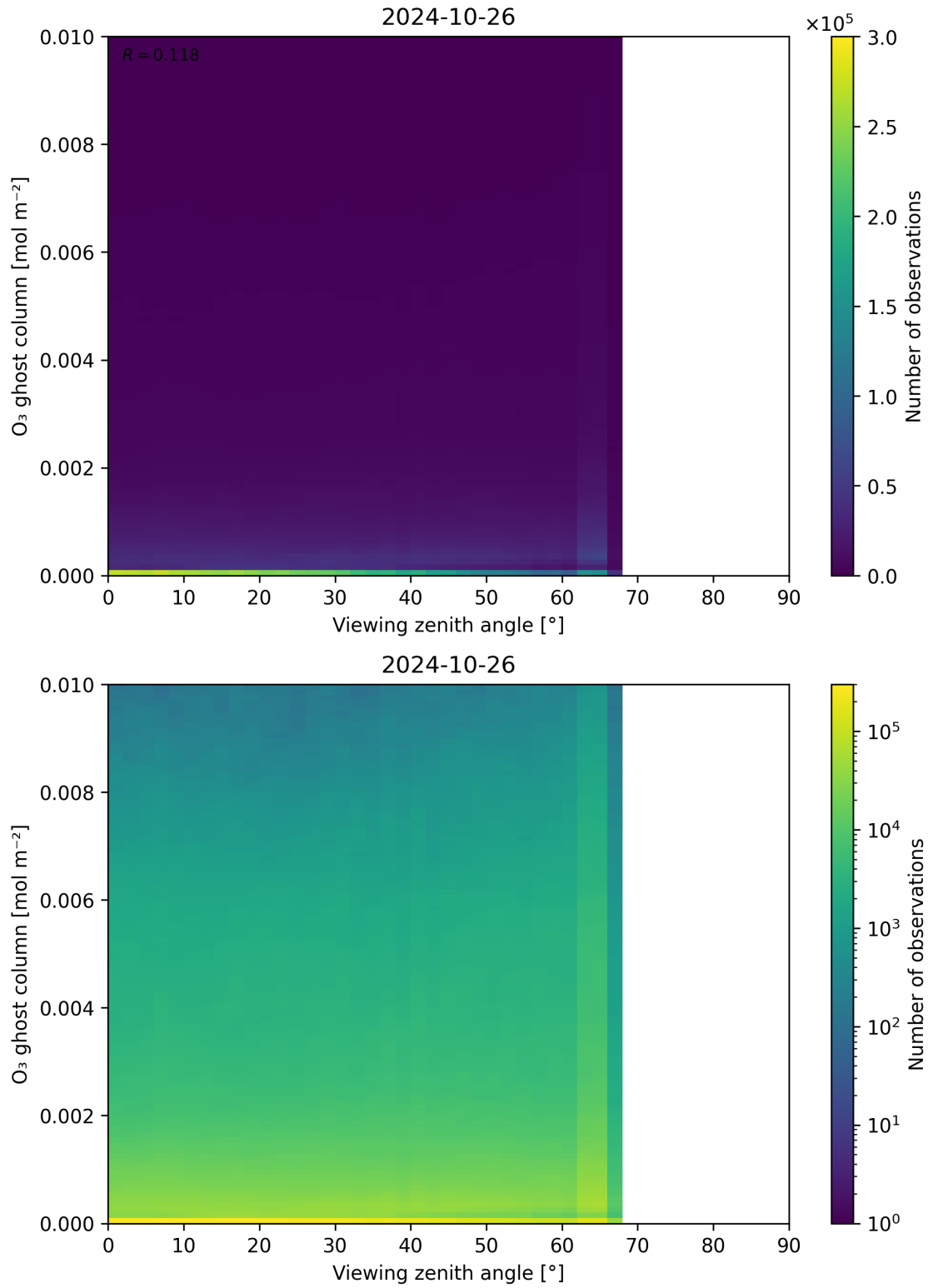
Figure 51: Scatter density plot of “Viewing zenith angle” against “O 3 ghost column” for 2024-10-25 to 2024-10-27.
