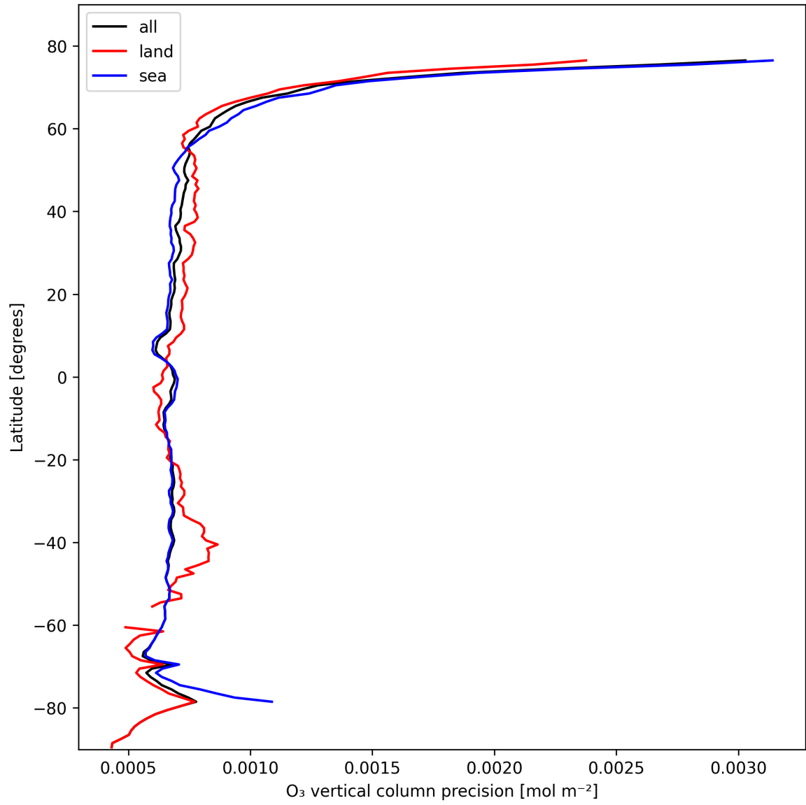
Figure 15: Zonal average of “O 3 vertical column precision” for 2024-10-25 to 2024-10-27.
