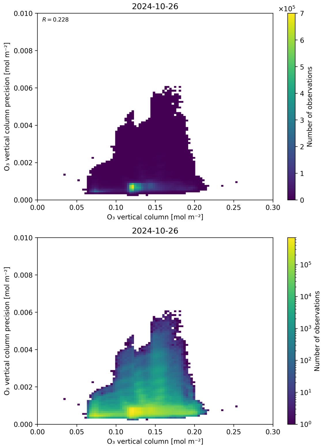
Figure 41: Scatter density plot of “O 3 vertical column” against “O 3 vertical column precision” for 2024-10-25 to 2024-10-27.
