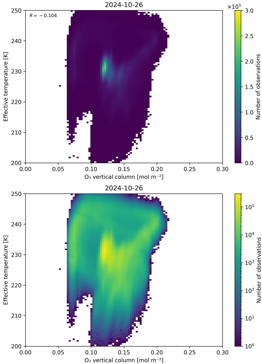
Figure 39: Scatter density plot of “O 3 vertical column” against “Effective temperature” for 2024-10-25 to 2024-10-27.
