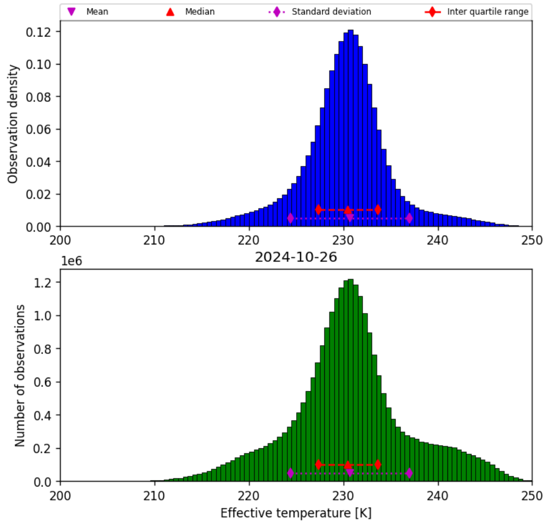
Figure 24: Histogram of “Effective temperature” for 2024-10-25 to 2024-10-27
