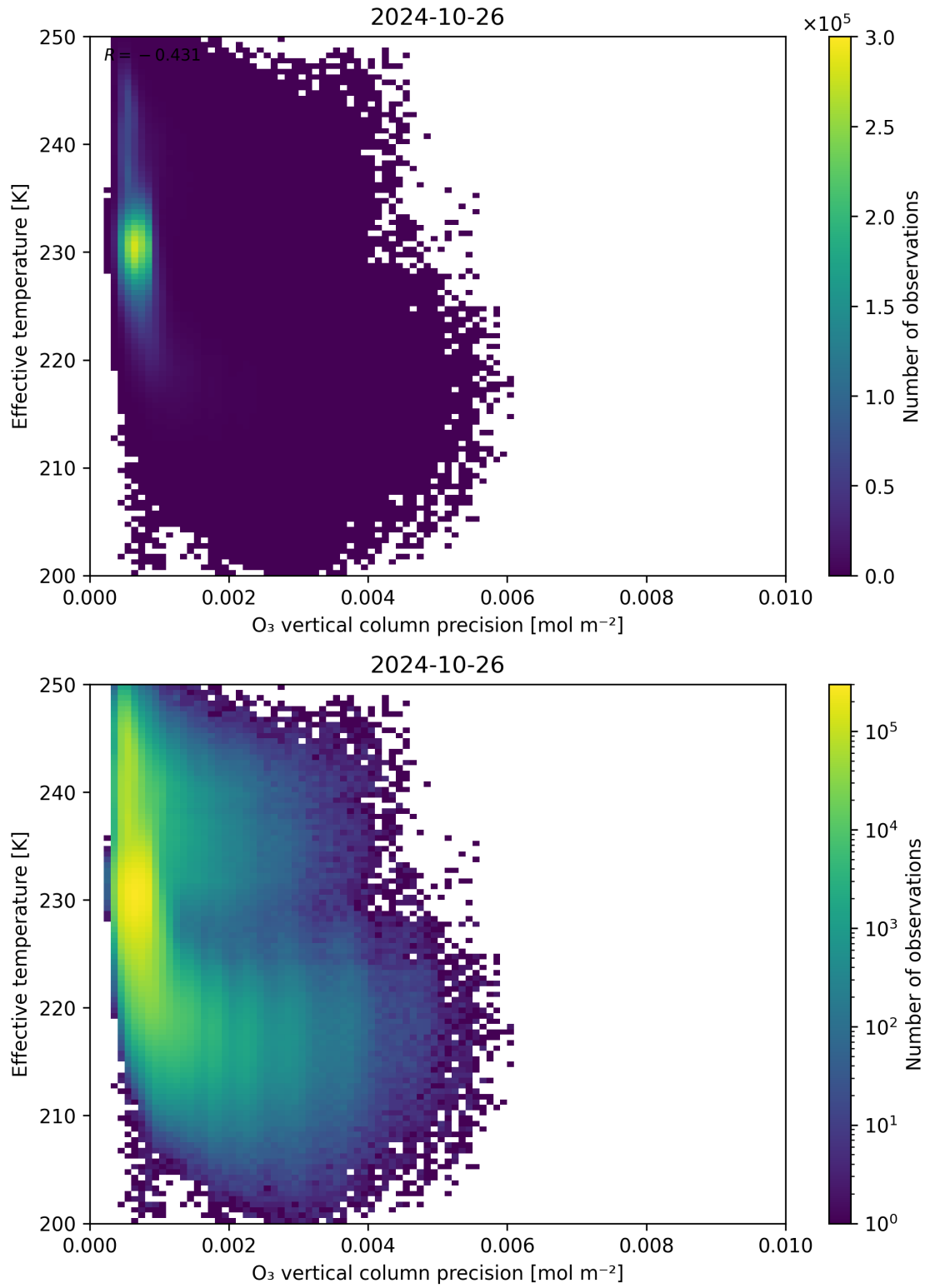
Figure 42: Scatter density plot of “ O_3 vertical column precision” against “Effective temperature” for 2024-10-25 to 2024-10-27.
