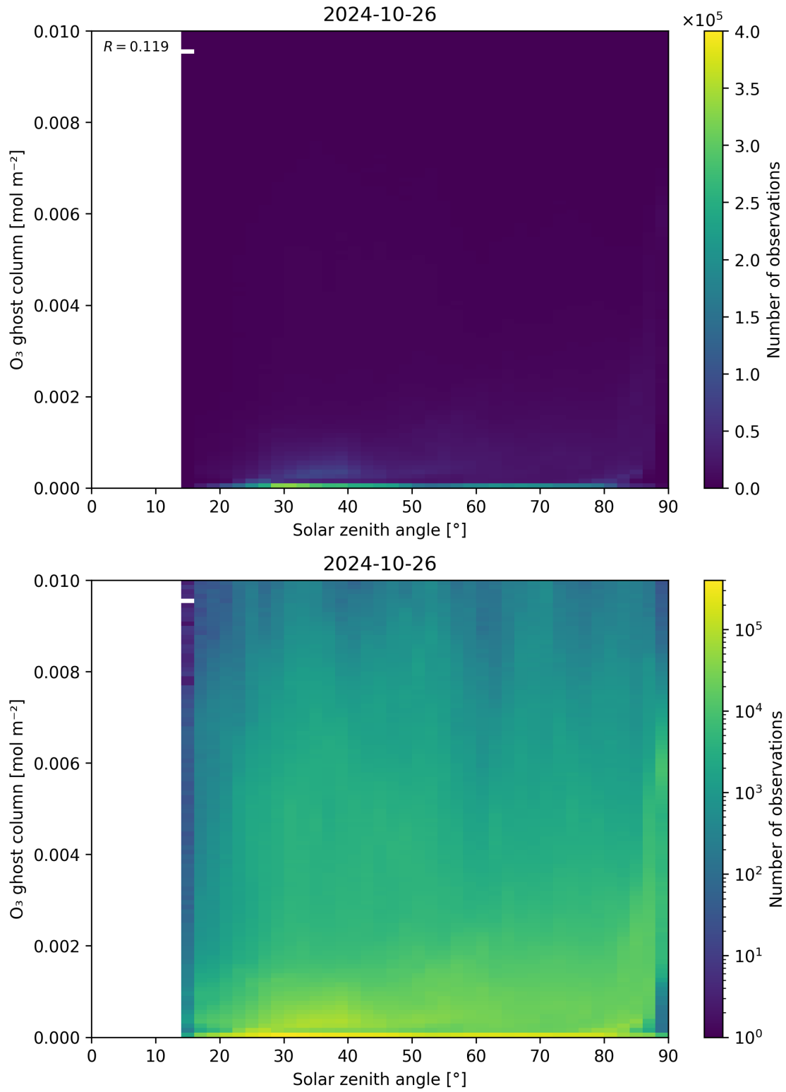
Figure 46: Scatter density plot of “Solar zenith angle” against “O 3 ghost column” for 2024-10-25 to 2024-10-27.
