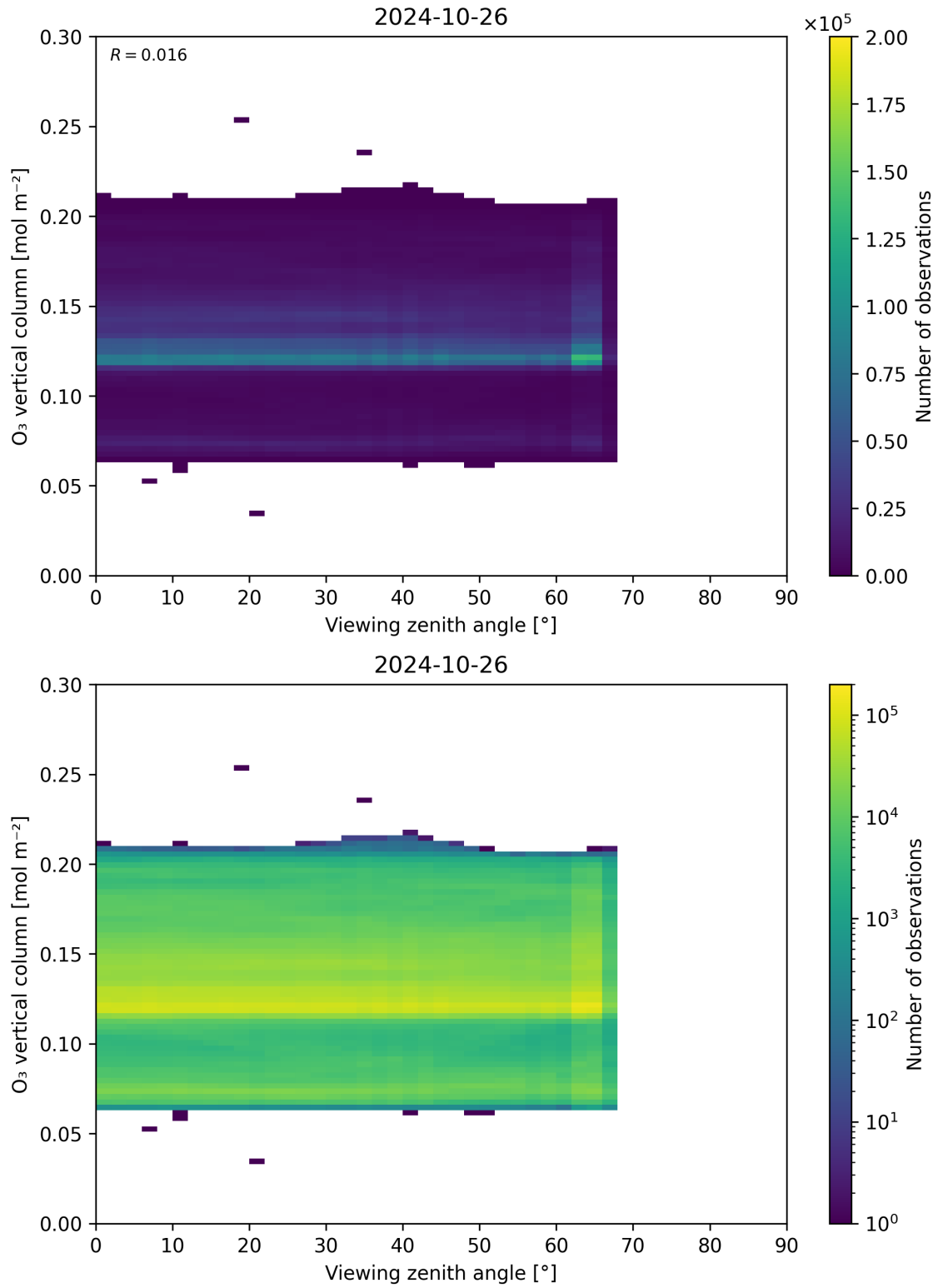
Figure 52: Scatter density plot of “Viewing zenith angle” against “O 3 vertical column” for 2024-10-25 to 2024-10-27.
