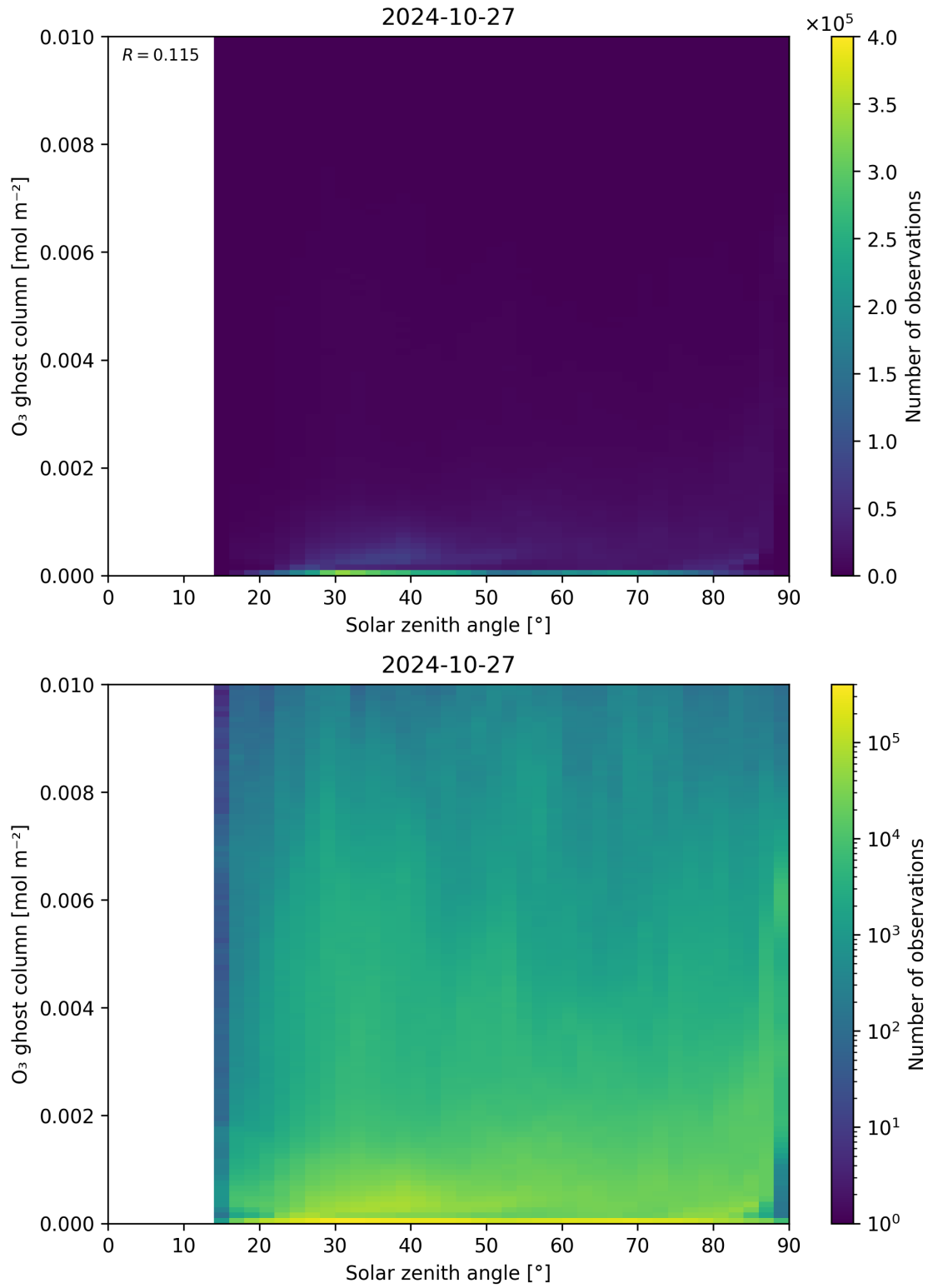
Figure 46: Scatter density plot of “Solar zenith angle” against “O 3 ghost column” for 2024-10-26 to 2024-10-28.
