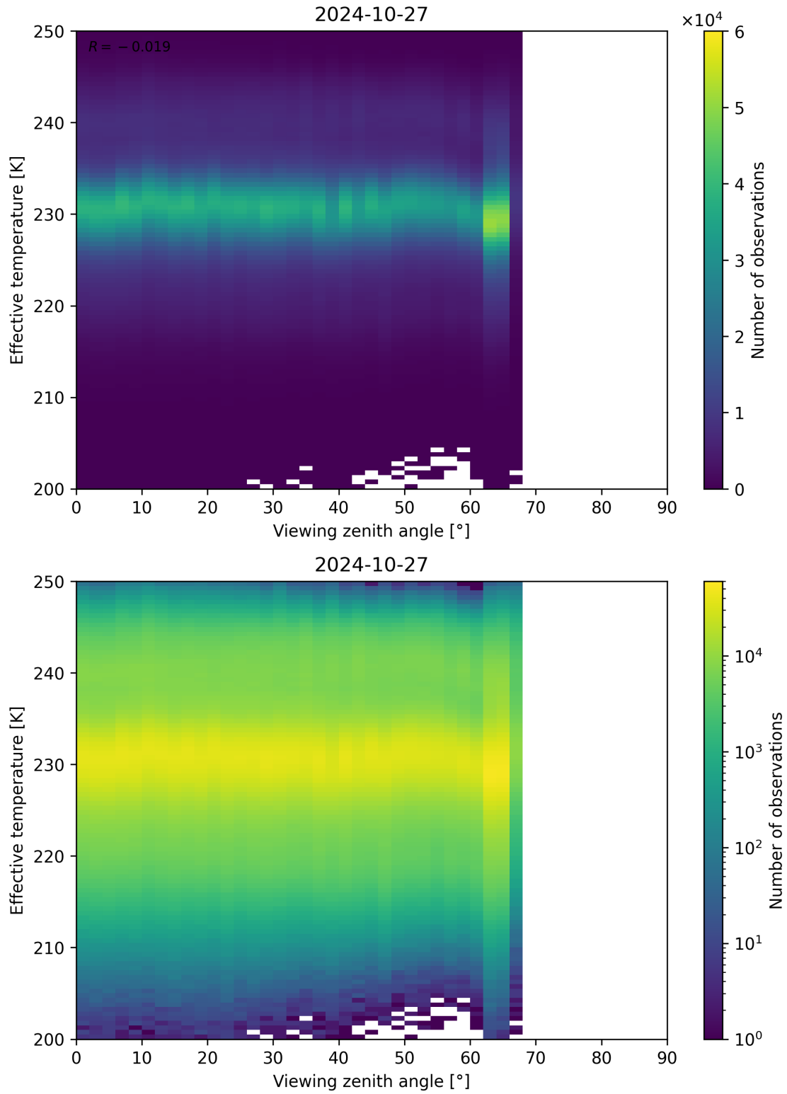
Figure 50: Scatter density plot of “Viewing zenith angle” against “Effective temperature” for 2024-10-26 to 2024-10-28.
