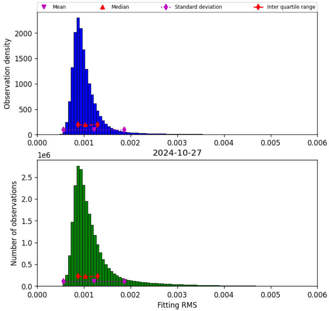
Figure 23: Histogram of “Fitting RMS” for 2024-10-26 to 2024-10-28
