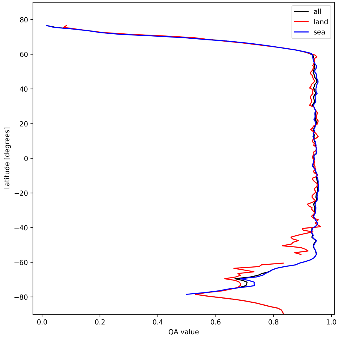
Figure 13: Zonal average of “QA value” for 2024-10-26 to 2024-10-28.
