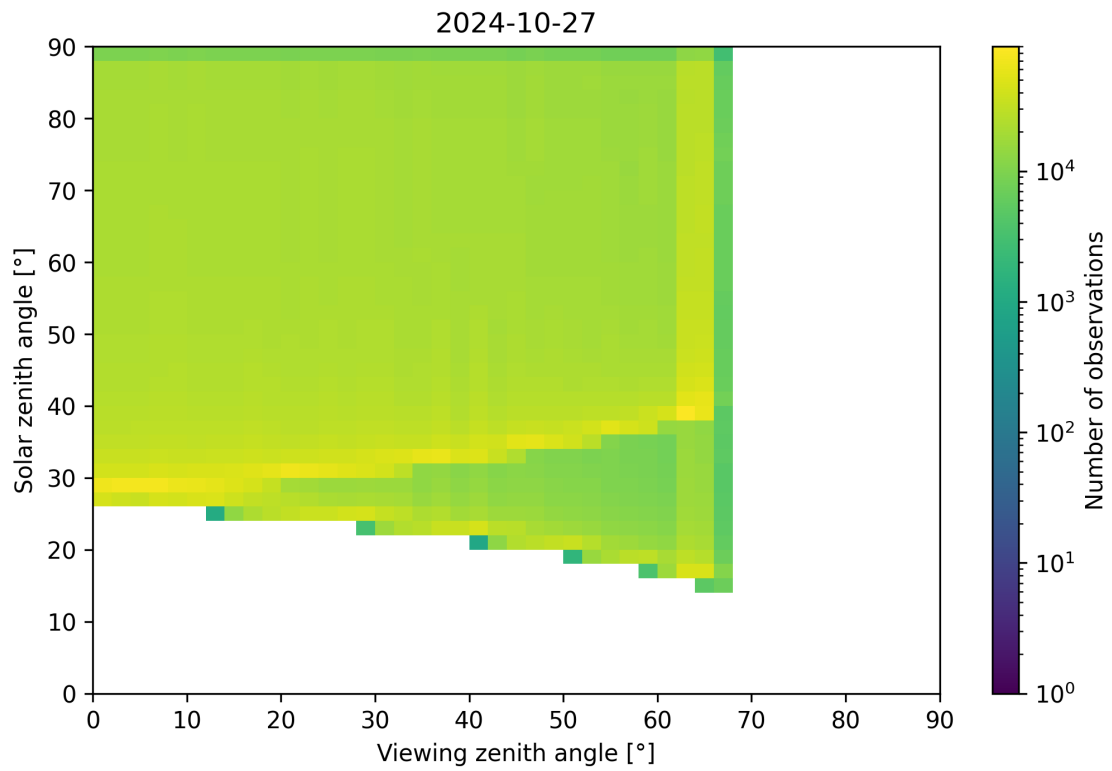
Figure 54: Scatter density plot of “Viewing zenith angle” against “Solar zenith angle” for 2024-10-26 to 2024-10-28.
