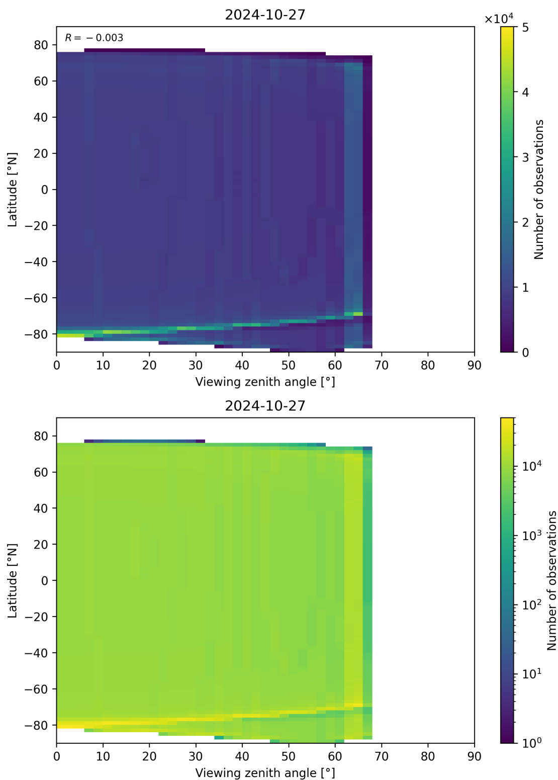
Figure 49: Scatter density plot of “Viewing zenith angle” against “Latitude” for 2024-10-26 to 2024-10-28.
