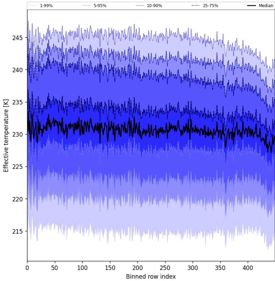
Figure 31: Along track statistics of “Effective temperature” for 2024-10-26 to 2024-10-28
