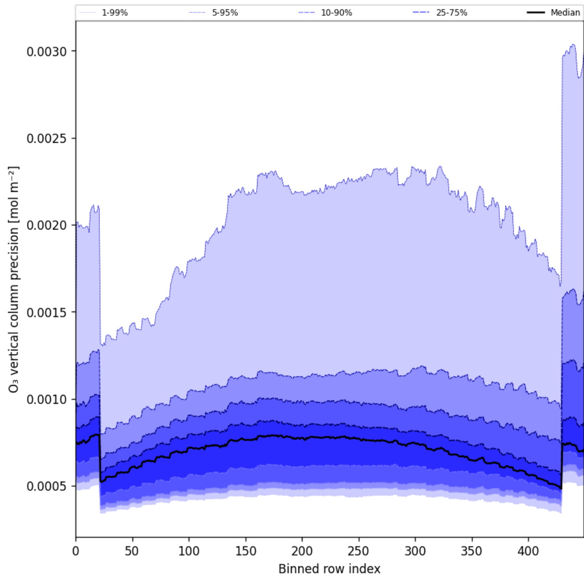
Figure 29: Along track statistics of “O 3 vertical column precision” for 2024-10-26 to 2024-10-28
