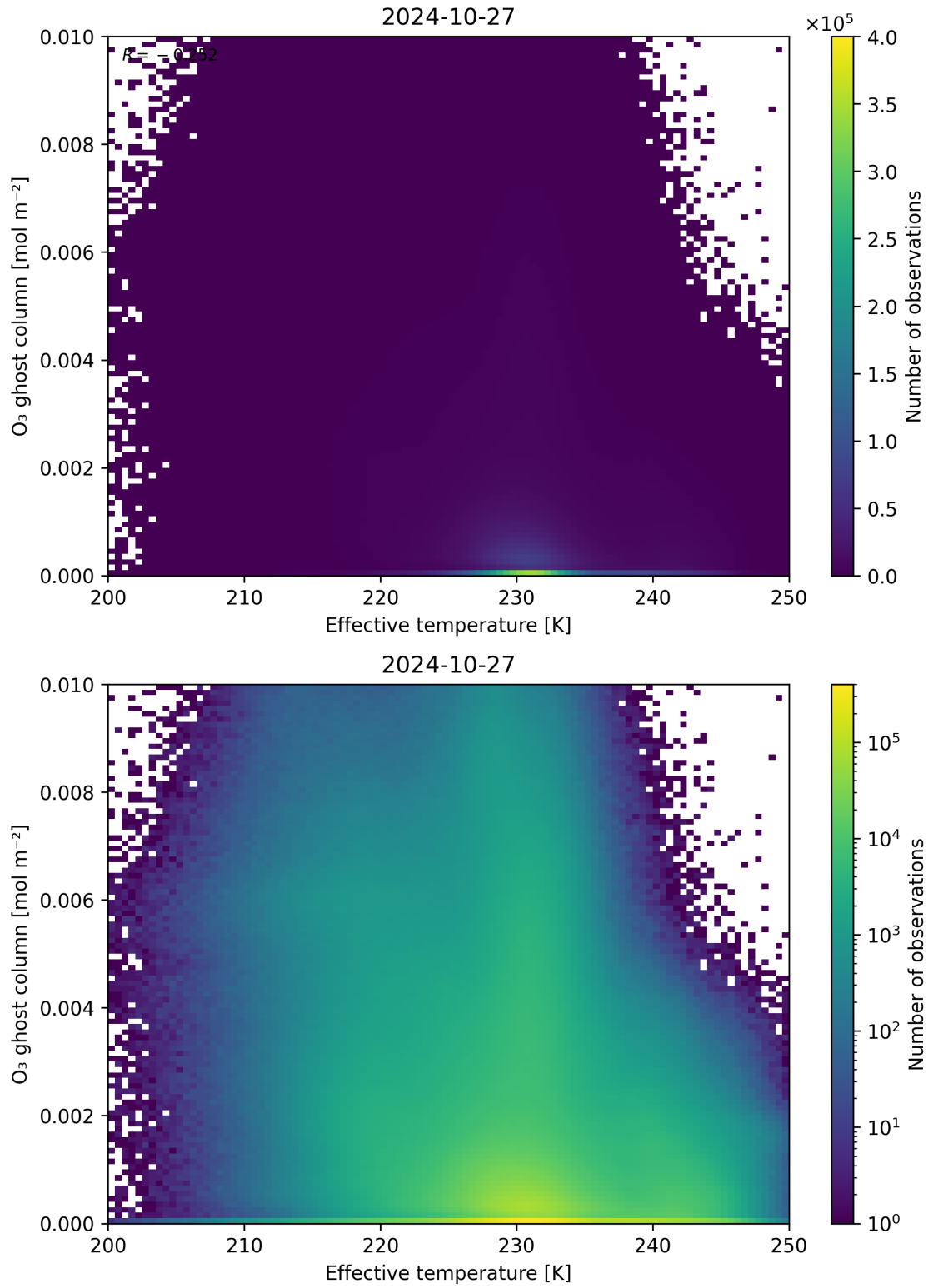
Figure 38: Scatter density plot of “Effective temperature” against “O 3 ghost column” for 2024-10-26 to 2024-10-28.
