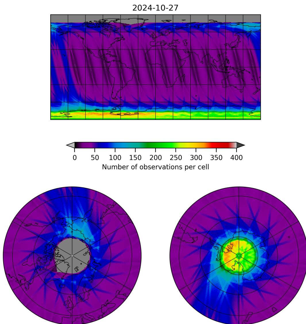
Figure 12: Map of the number of observations for 2024-10-26 to 2024-10-28
