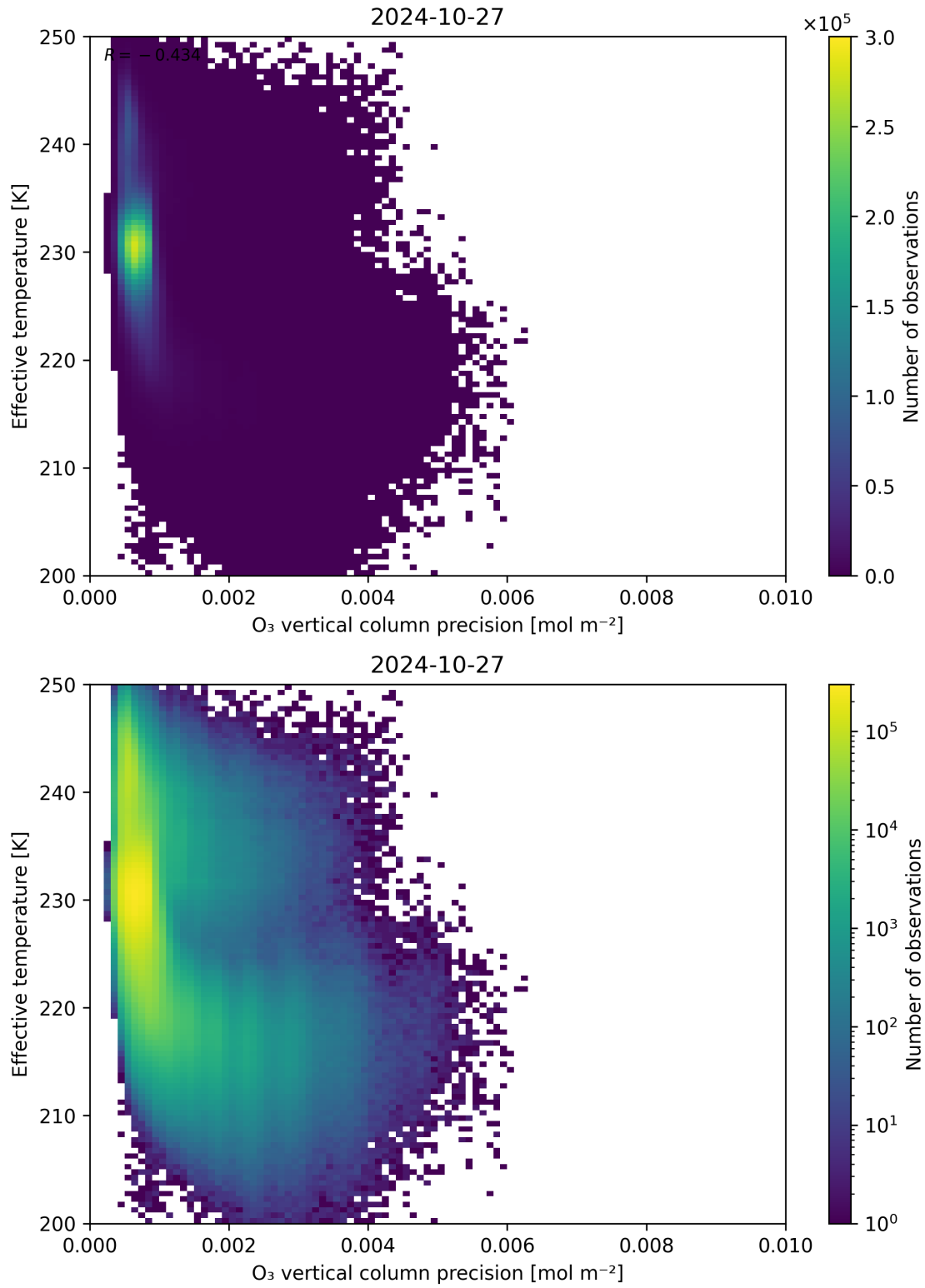
Figure 42: Scatter density plot of “ O_3 vertical column precision” against “Effective temperature” for 2024-10-26 to 2024-10-28.
