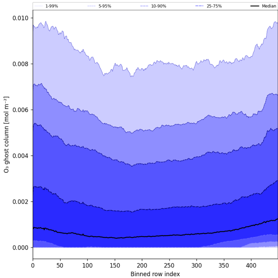
Figure 32: Along track statistics of “O 3 ghost column” for 2024-10-26 to 2024-10-28
