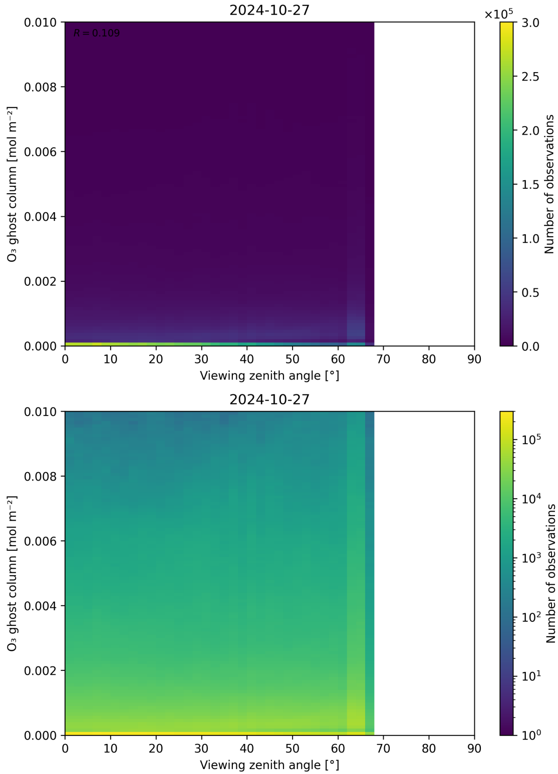
Figure 51: Scatter density plot of “Viewing zenith angle” against “O 3 ghost column” for 2024-10-26 to 2024-10-28.
