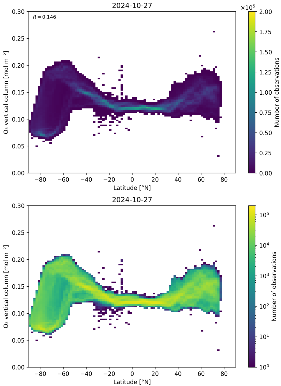
Figure 36: Scatter density plot of “Latitude” against “O 3 vertical column” for 2024-10-26 to 2024-10-28.
