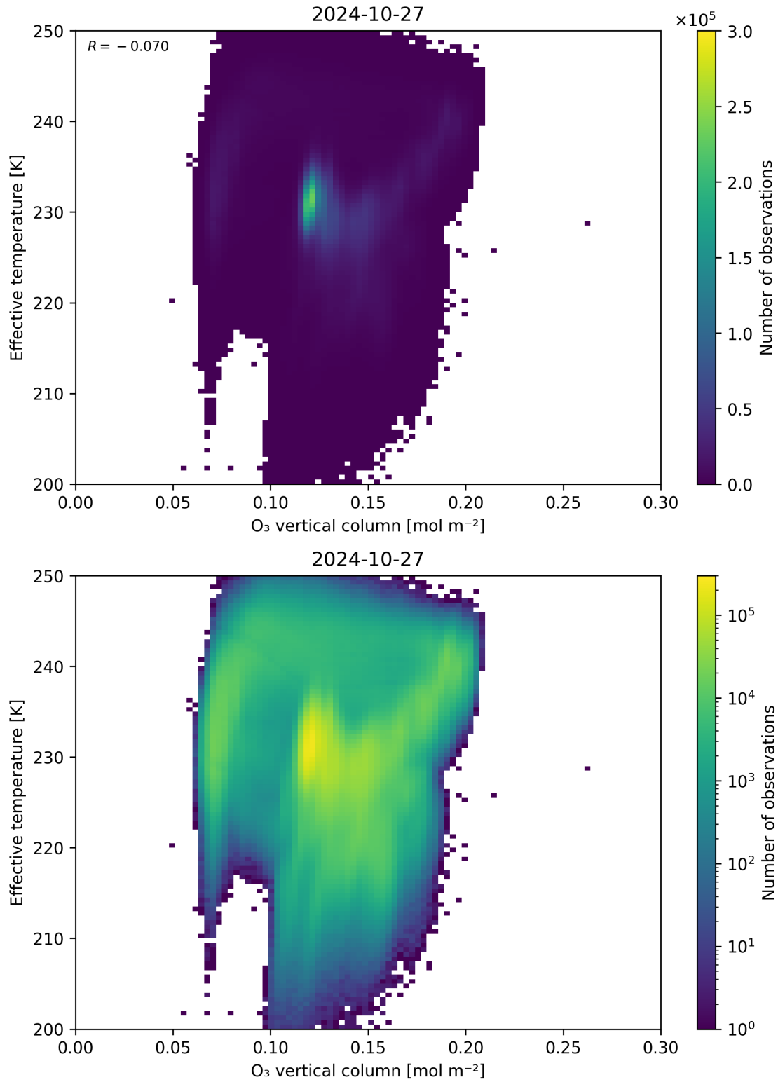
Figure 39: Scatter density plot of “O 3 vertical column” against “Effective temperature” for 2024-10-26 to 2024-10-28.
