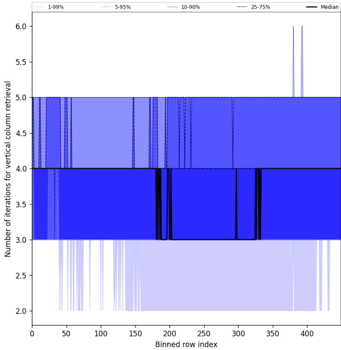
Figure 33: Along track statistics of “Number of iterations for vertical column retrieval” for 2024-10-26 to 2024-10-28
