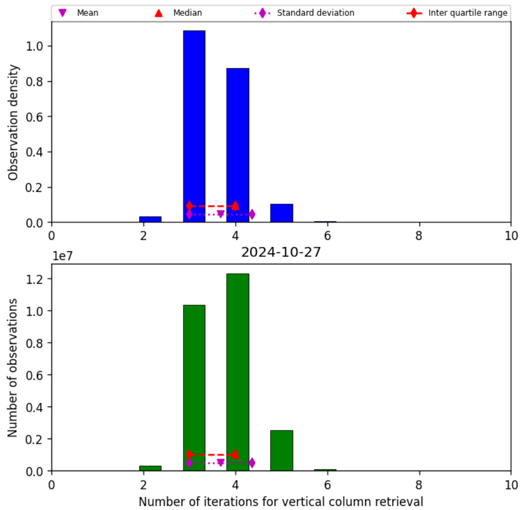
Figure 26: Histogram of “Number of iterations for vertical column retrieval” for 2024-10-26 to 2024-10-28
