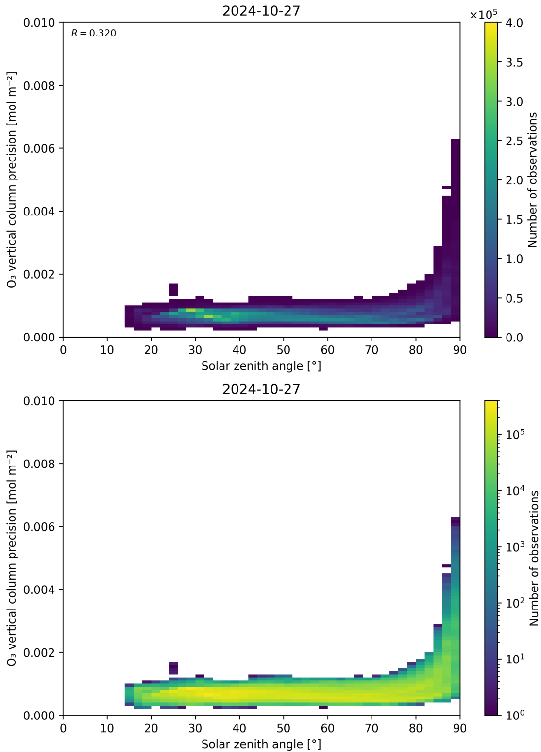
Figure 48: Scatter density plot of “Solar zenith angle” against “O 3 vertical column precision” for 2024-10-26 to 2024-10-28.
