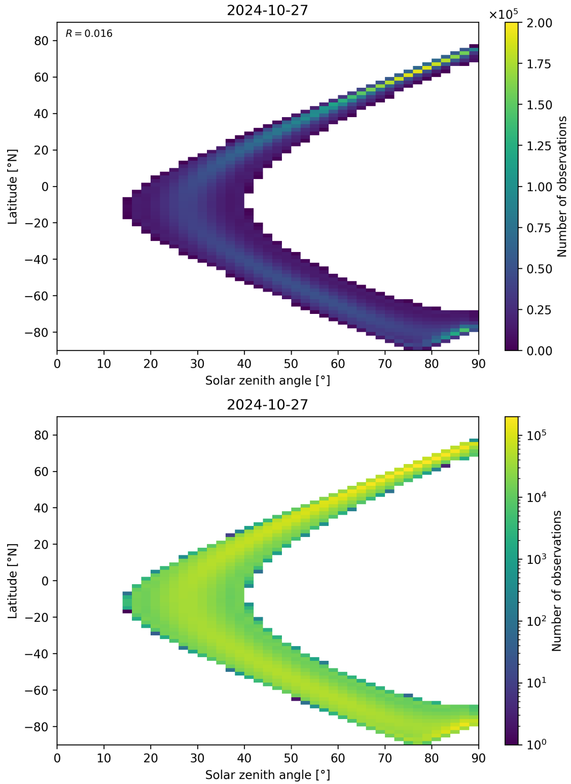
Figure 44: Scatter density plot of “Solar zenith angle” against “Latitude” for 2024-10-26 to 2024-10-28.
