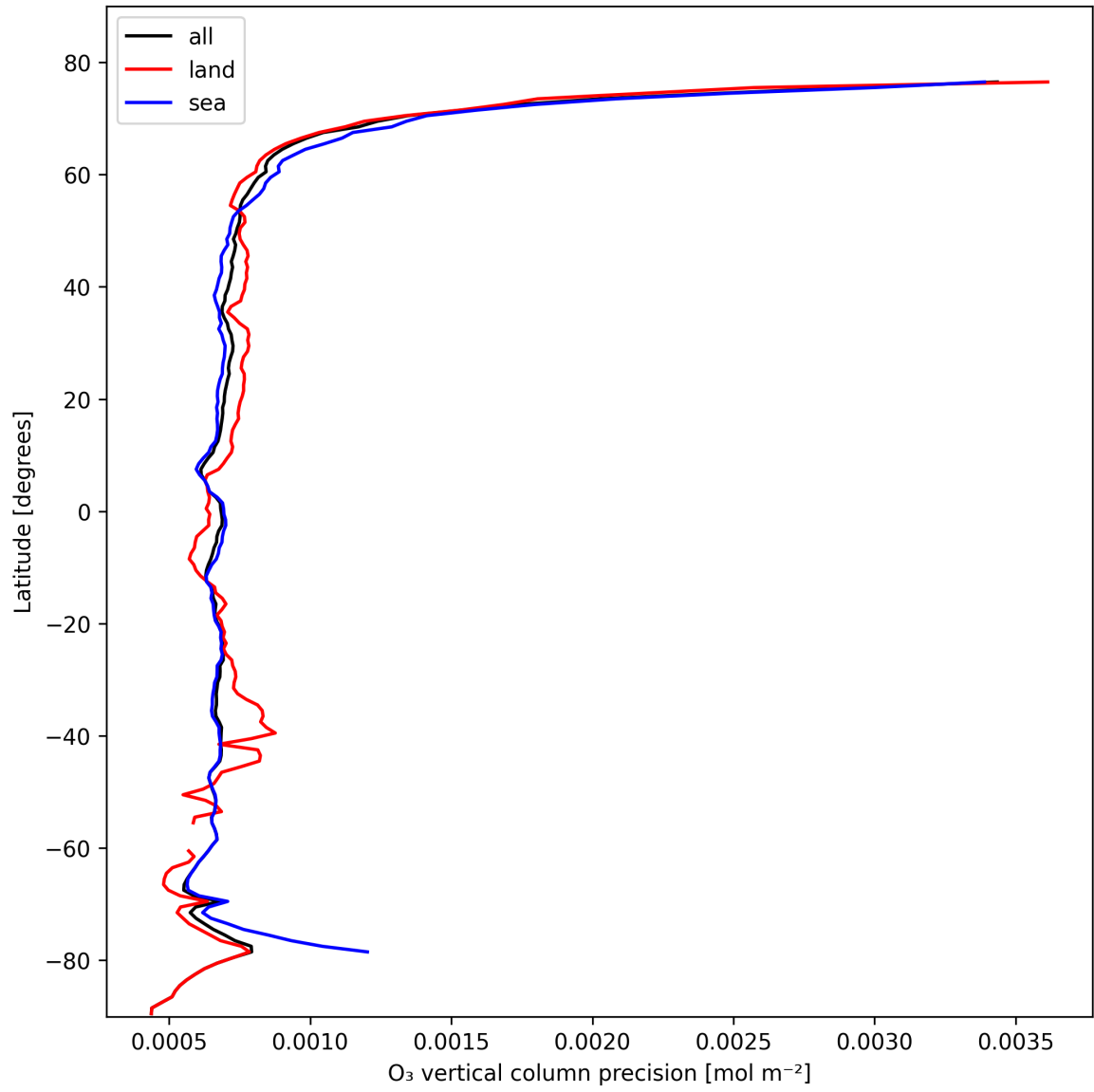
Figure 15: Zonal average of “O 3 vertical column precision” for 2024-10-26 to 2024-10-28.
