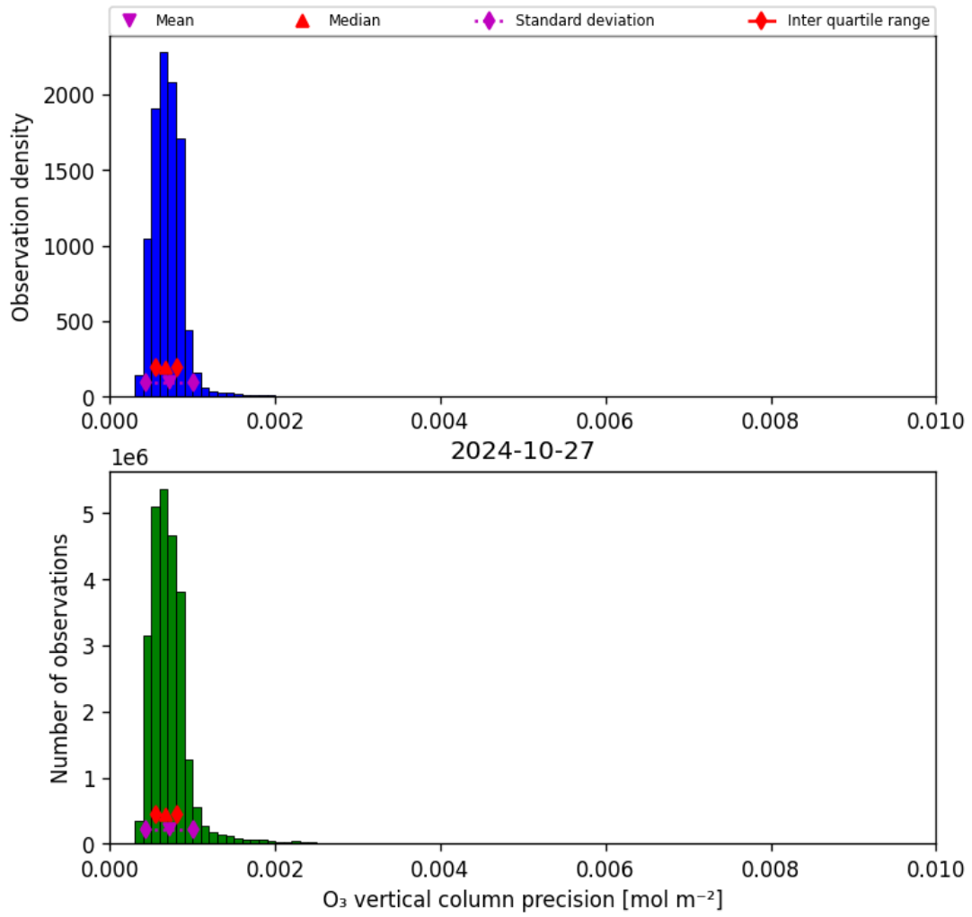
Figure 22: Histogram of “O 3 vertical column precision” for 2024-10-26 to 2024-10-28
