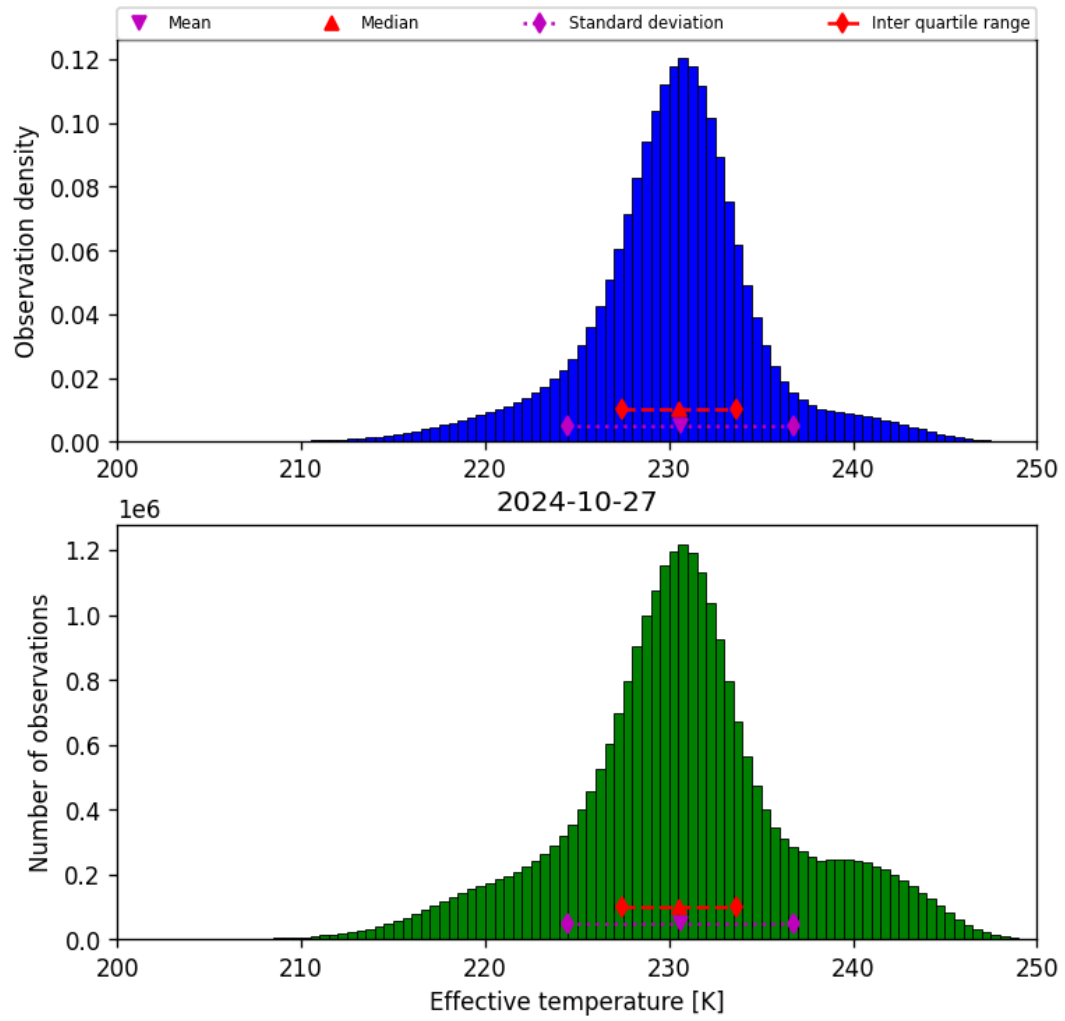
Figure 24: Histogram of “Effective temperature” for 2024-10-26 to 2024-10-28
