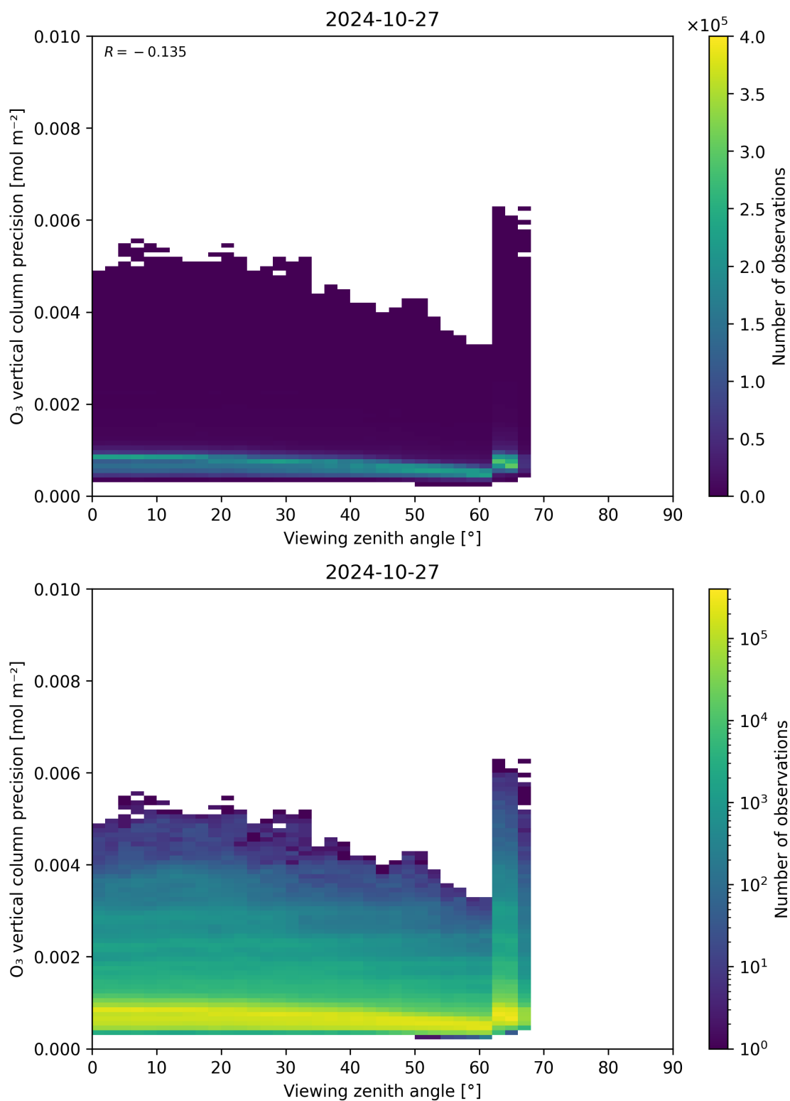
Figure 53: Scatter density plot of “Viewing zenith angle” against “O 3 vertical column precision” for 2024-10-26 to 2024-10-28.
