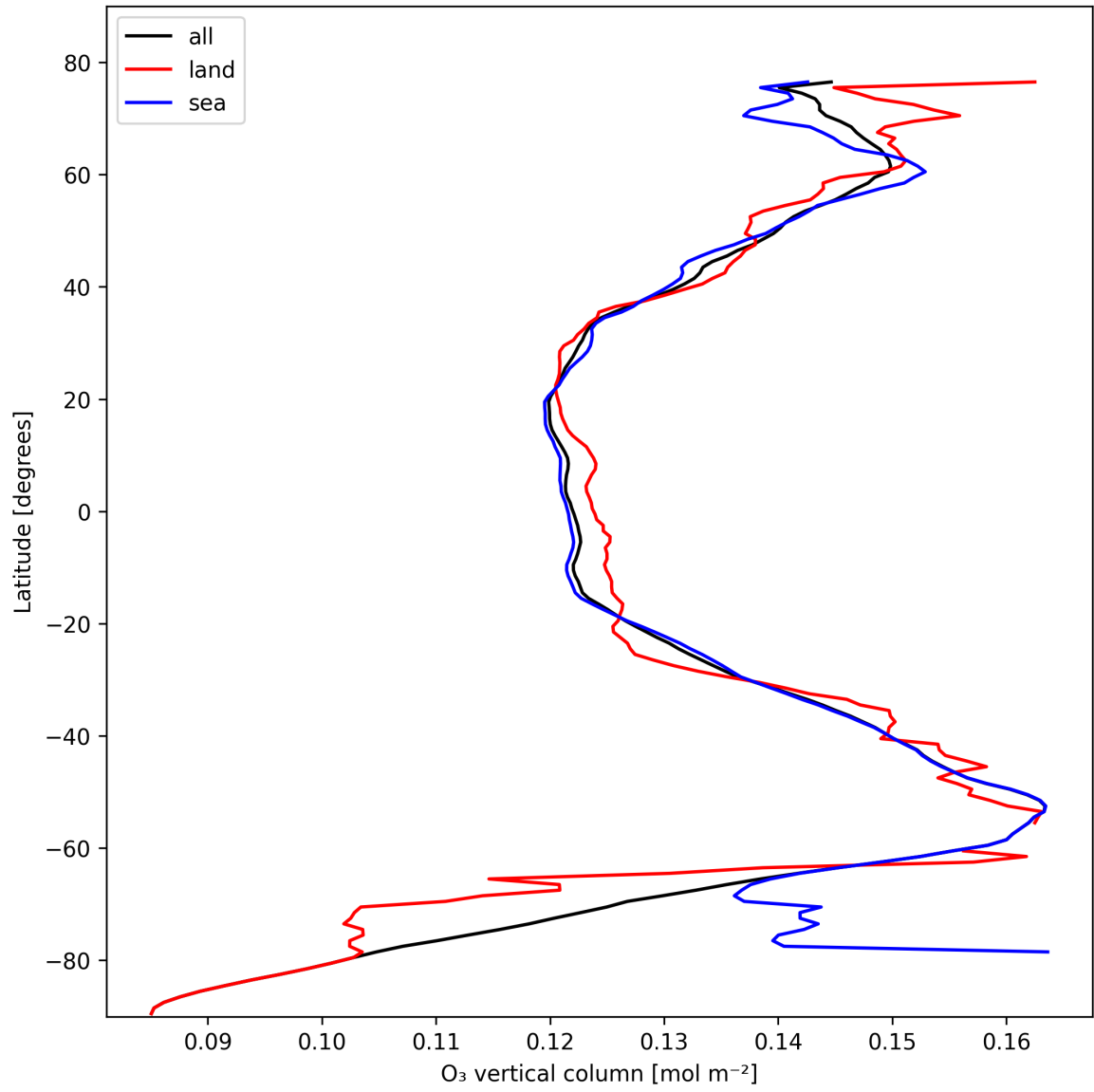
Figure 14: Zonal average of “O 3 vertical column” for 2024-10-26 to 2024-10-28.
