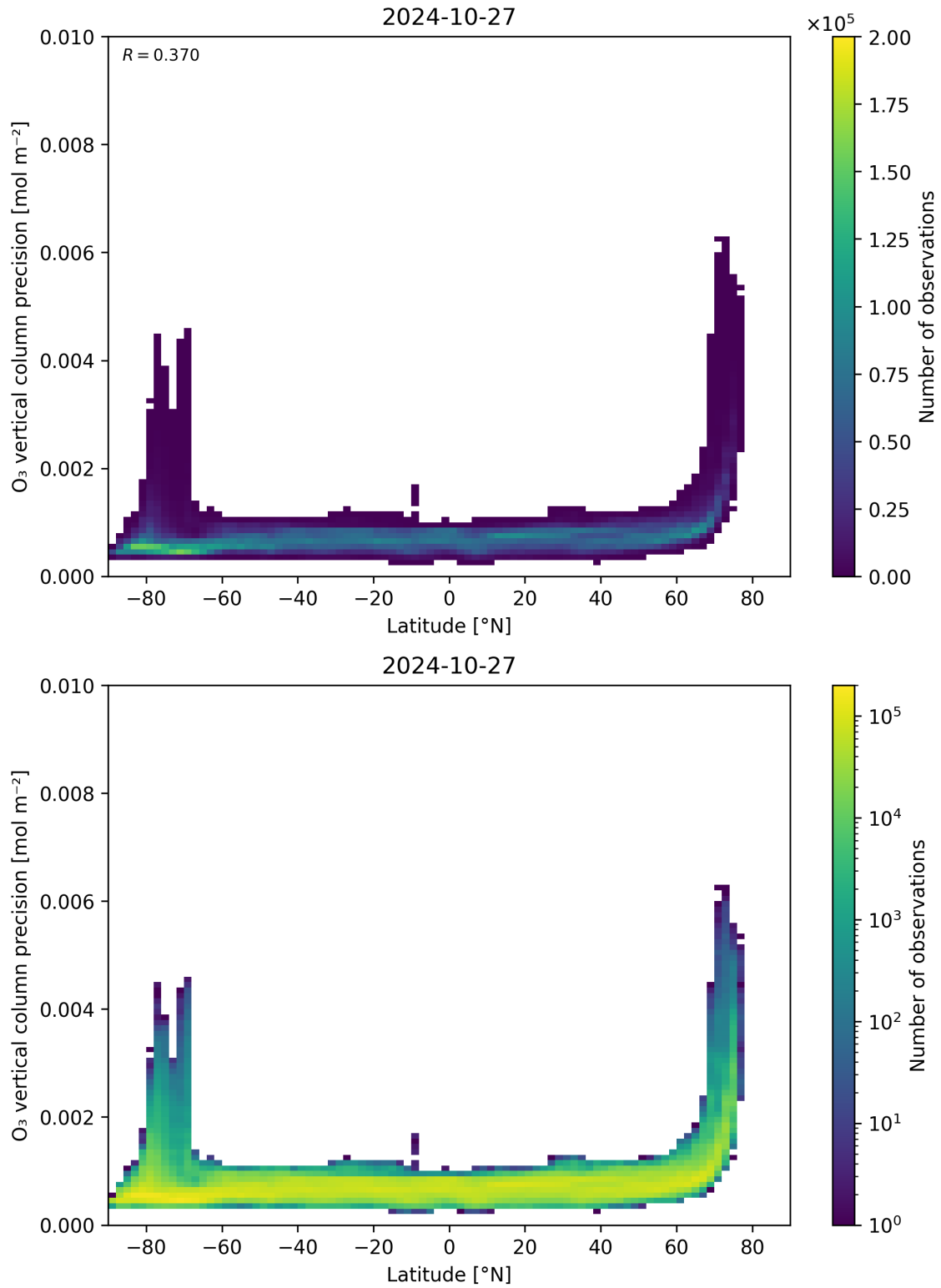
Figure 37: Scatter density plot of “Latitude” against “O 3 vertical column precision” for 2024-10-26 to 2024-10-28.
