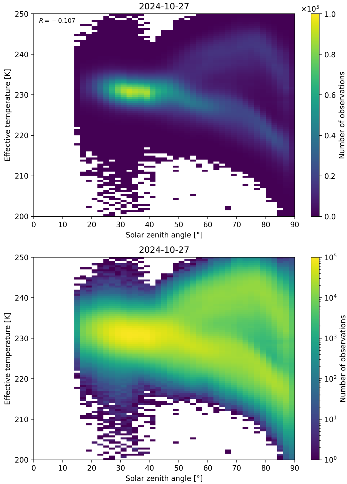
Figure 45: Scatter density plot of “Solar zenith angle” against “Effective temperature” for 2024-10-26 to 2024-10-28.
