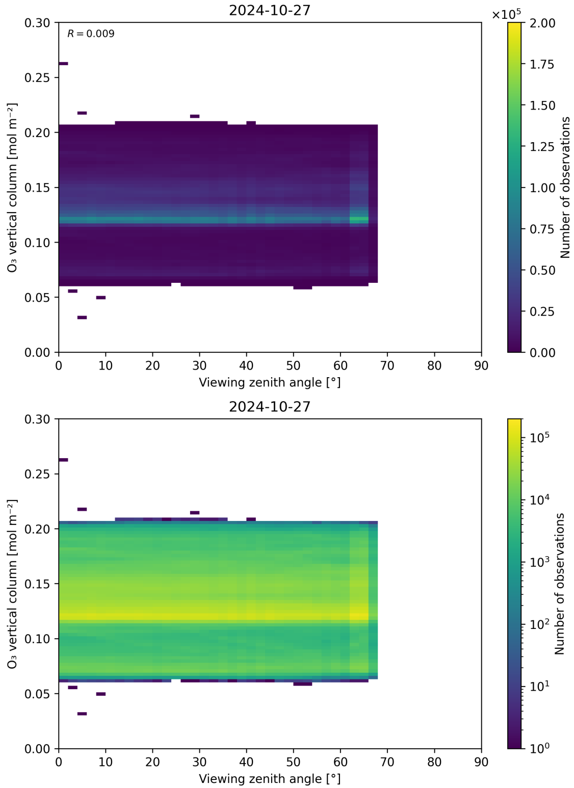
Figure 52: Scatter density plot of “Viewing zenith angle” against “O 3 vertical column” for 2024-10-26 to 2024-10-28.
