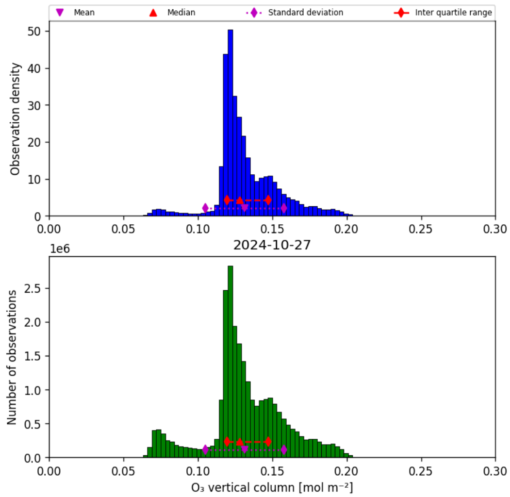
Figure 21: Histogram of “O 3 vertical column” for 2024-10-26 to 2024-10-28
