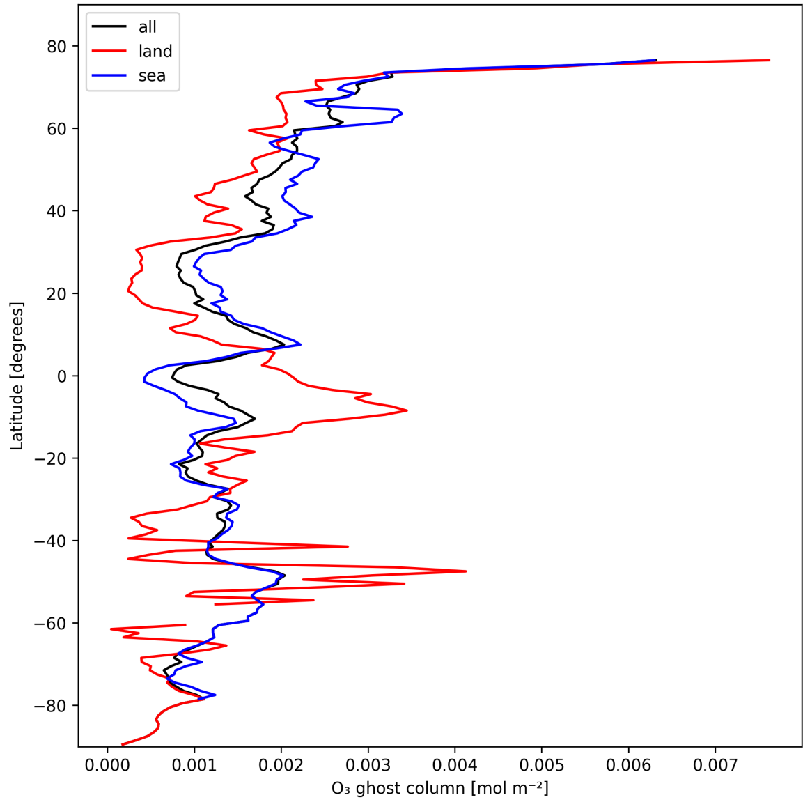
Figure 18: Zonal average of "O 3 ghost column" for 2024-10-26 to 2024-10-28.
