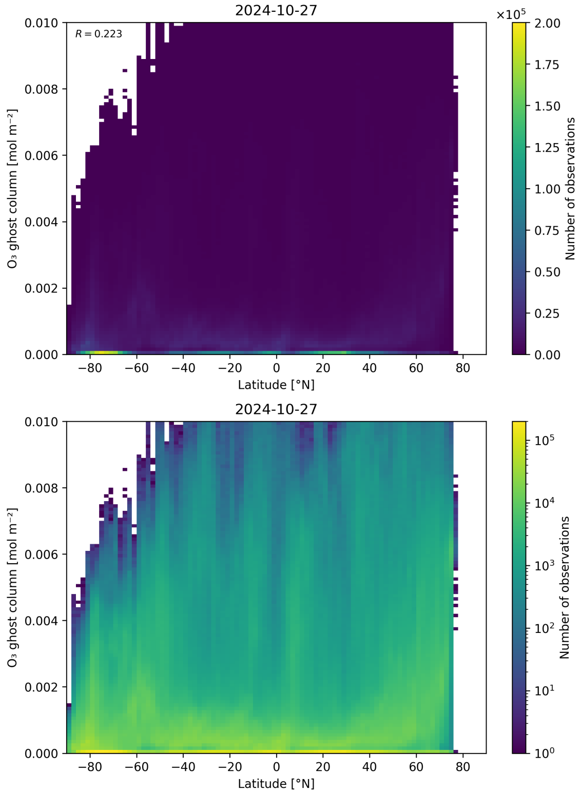
Figure 35: Scatter density plot of “Latitude” against “O 3 ghost column” for 2024-10-26 to 2024-10-28.
