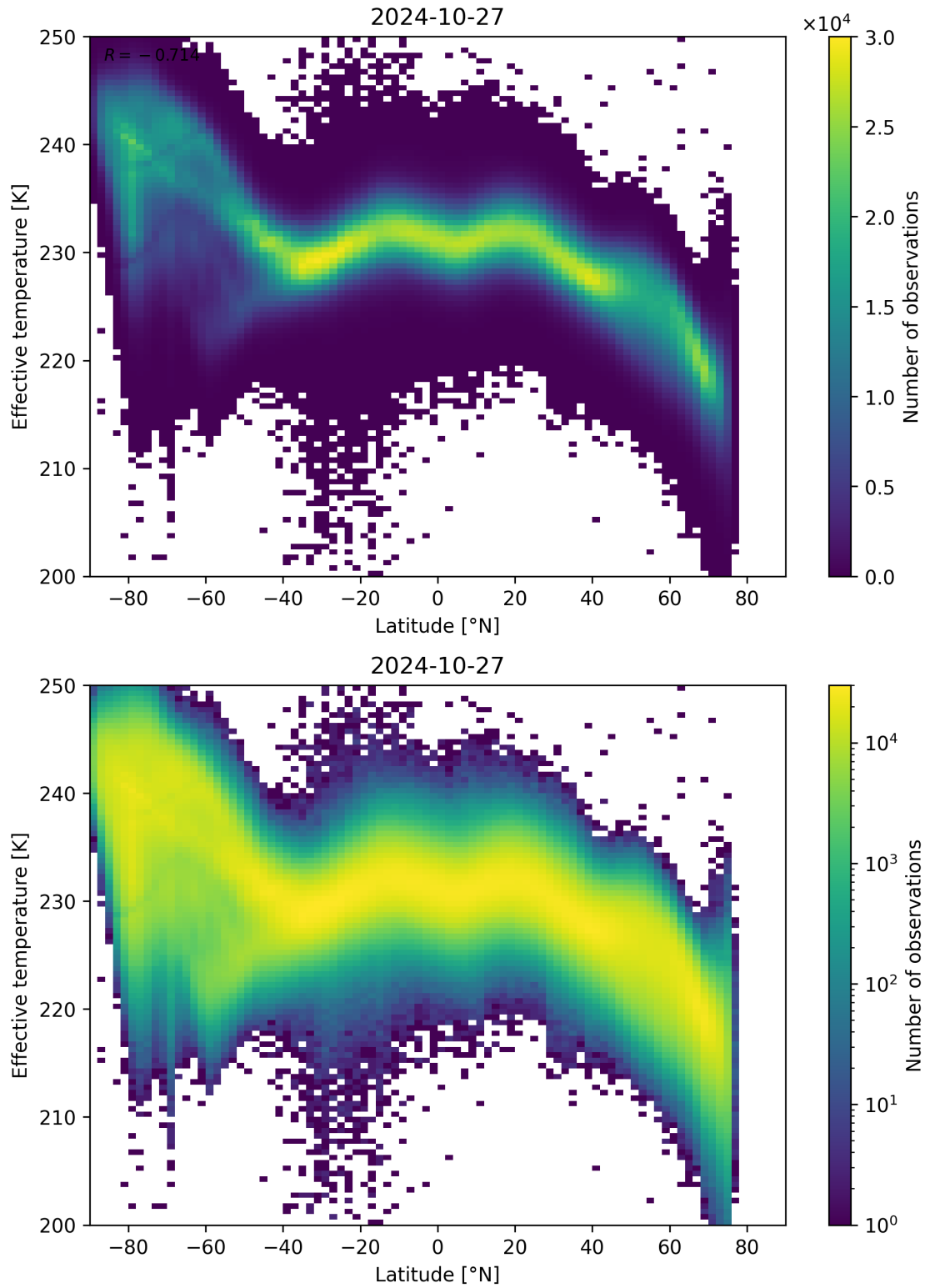
Figure 34: Scatter density plot of “Latitude” against “Effective temperature” for 2024-10-26 to 2024-10-28.
