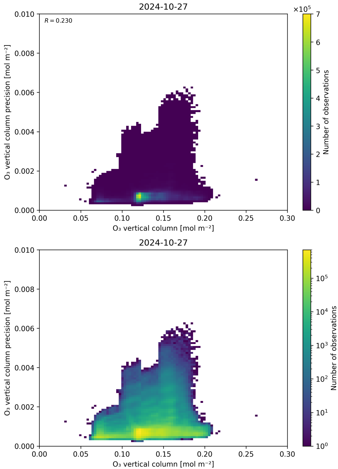
Figure 41: Scatter density plot of “O 3 vertical column” against “O 3 vertical column precision” for 2024-10-26 to 2024-10-28.
