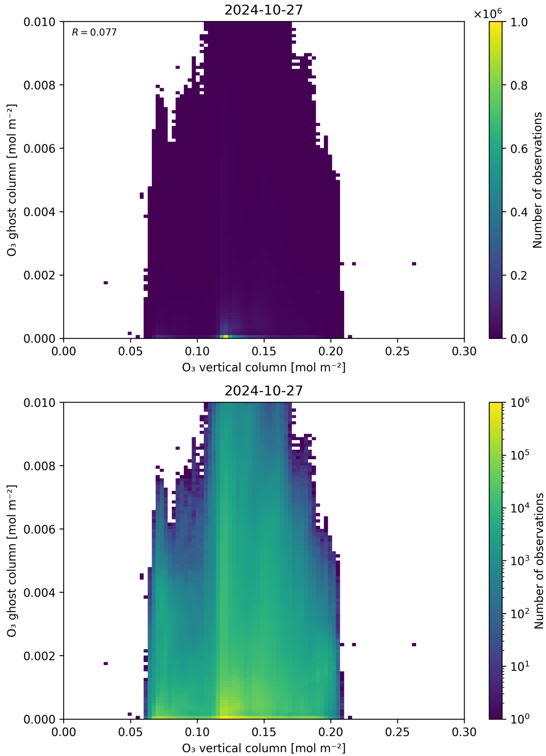
Figure 40: Scatter density plot of “O 3 vertical column” against “O 3 ghost column” for 2024-10-26 to 2024-10-28.
