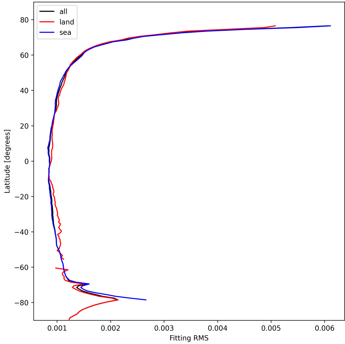
Figure 16: Zonal average of “Fitting RMS” for 2024-10-26 to 2024-10-28.
