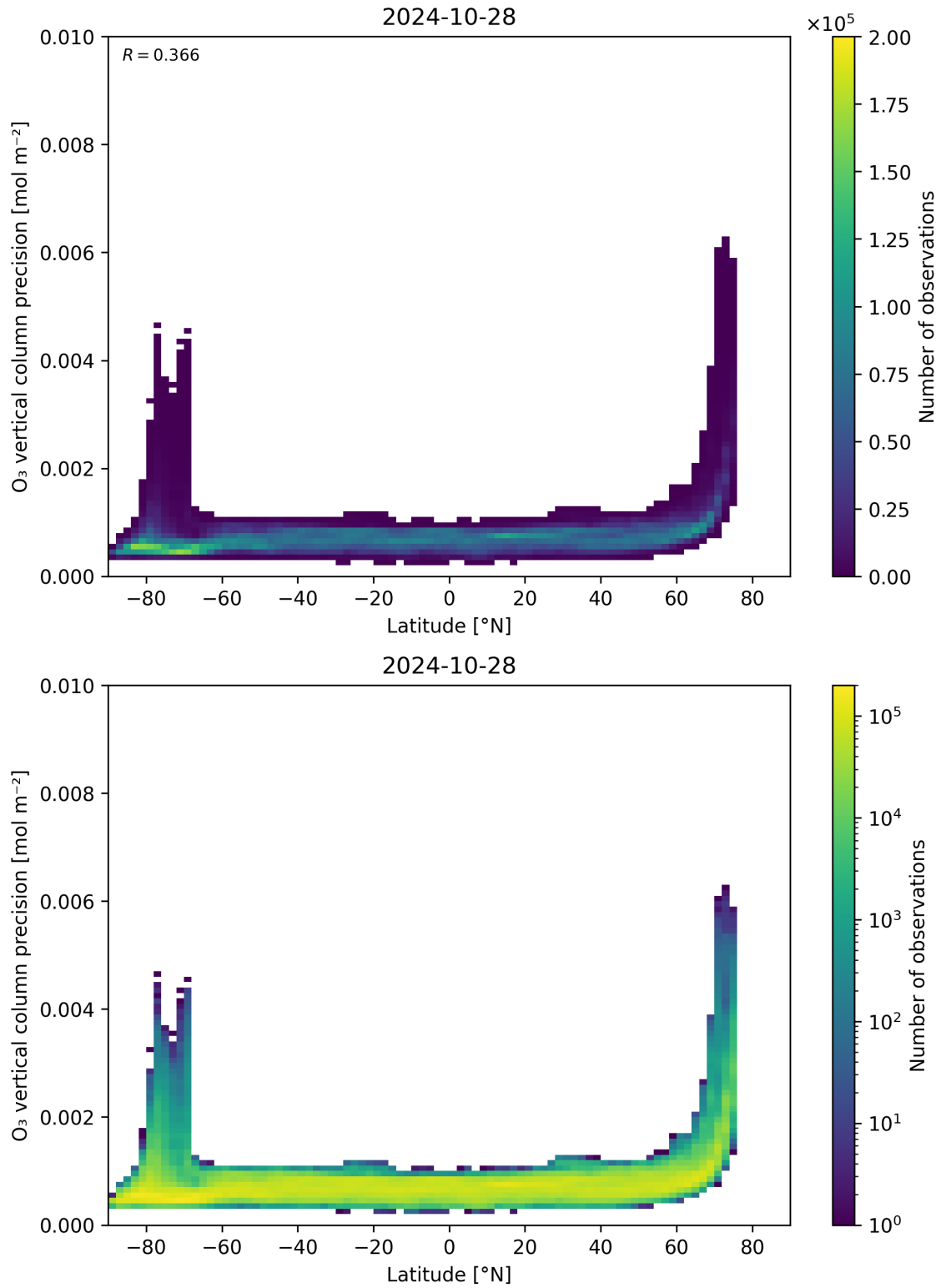
Figure 37: Scatter density plot of “Latitude” against “O 3 vertical column precision” for 2024-10-27 to 2024-10-29.
