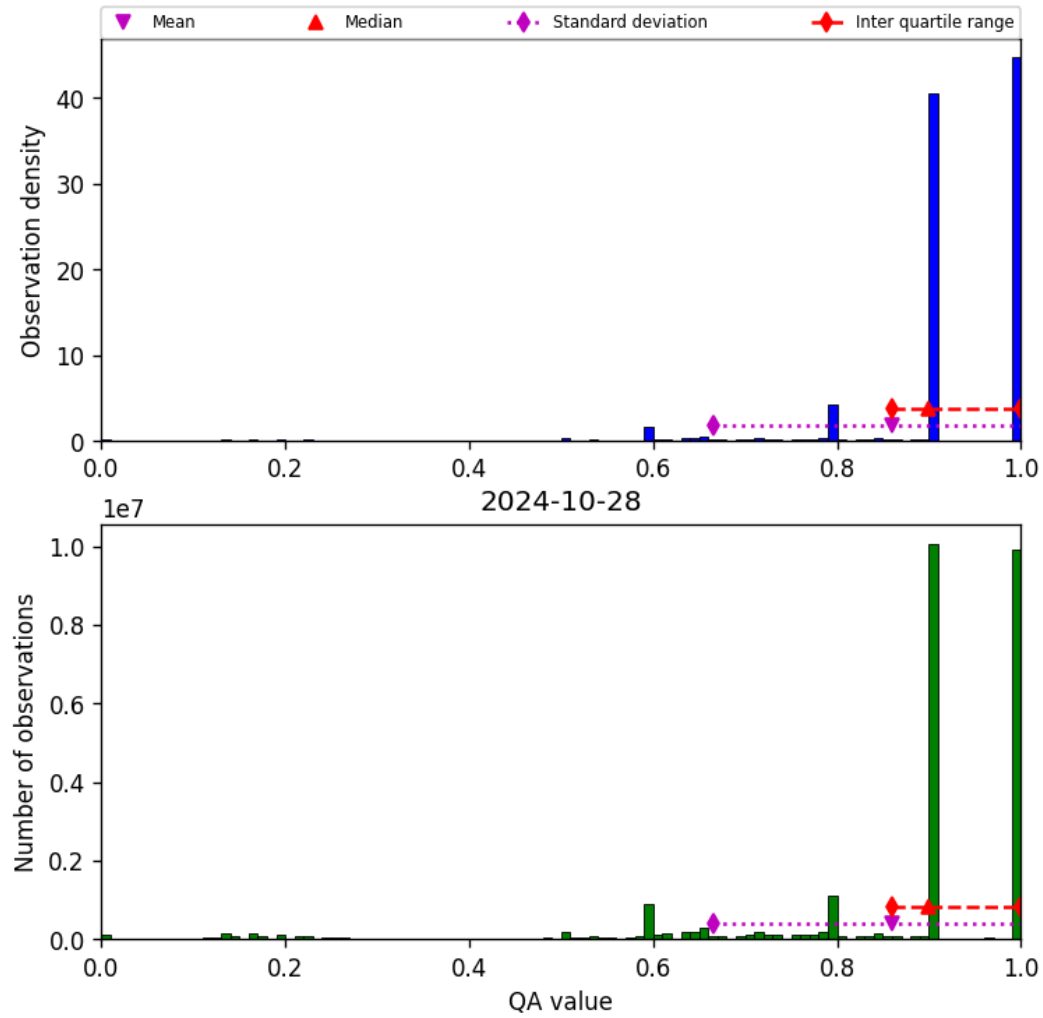
Figure 20: Histogram of “QA value” for 2024-10-27 to 2024-10-29
