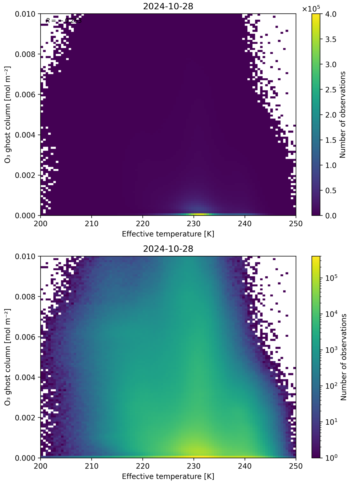
Figure 38: Scatter density plot of “Effective temperature” against “O 3 ghost column” for 2024-10-27 to 2024-10-29.
