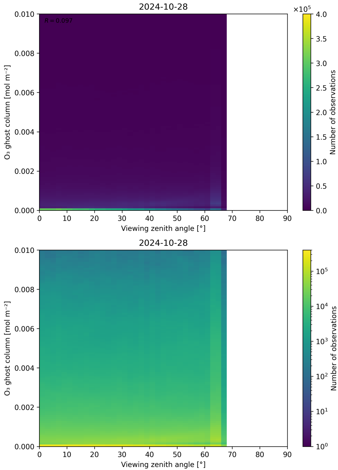
Figure 51: Scatter density plot of “Viewing zenith angle” against “O 3 ghost column” for 2024-10-27 to 2024-10-29.
