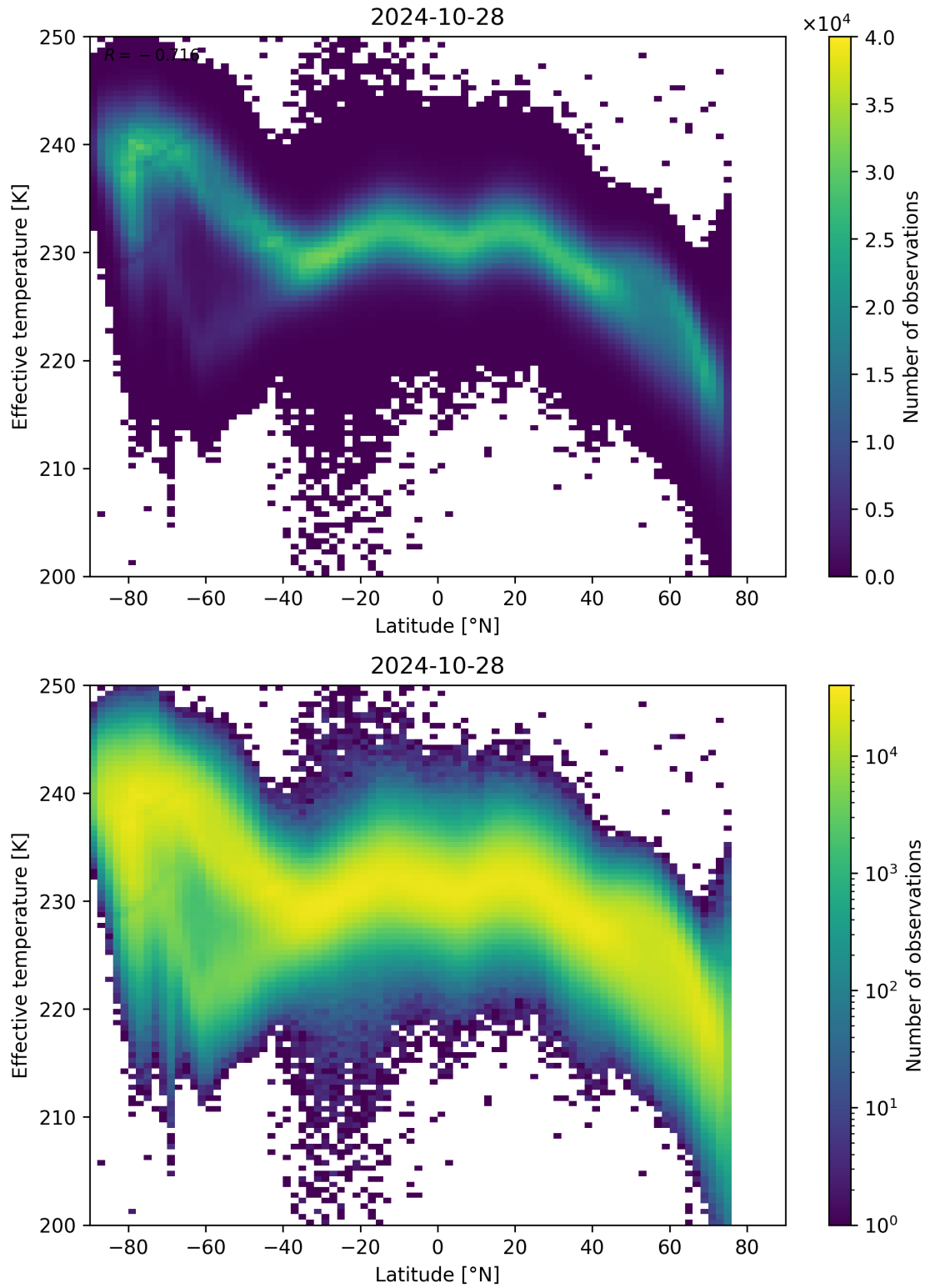
Figure 34: Scatter density plot of “Latitude” against “Effective temperature” for 2024-10-27 to 2024-10-29.
