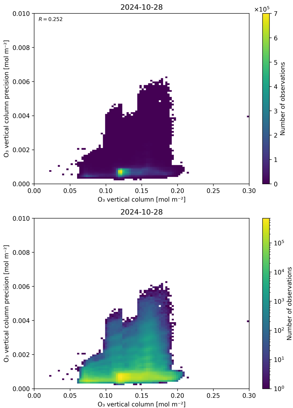
Figure 41: Scatter density plot of “O 3 vertical column” against “O 3 vertical column precision” for 2024-10-27 to 2024-10-29.
