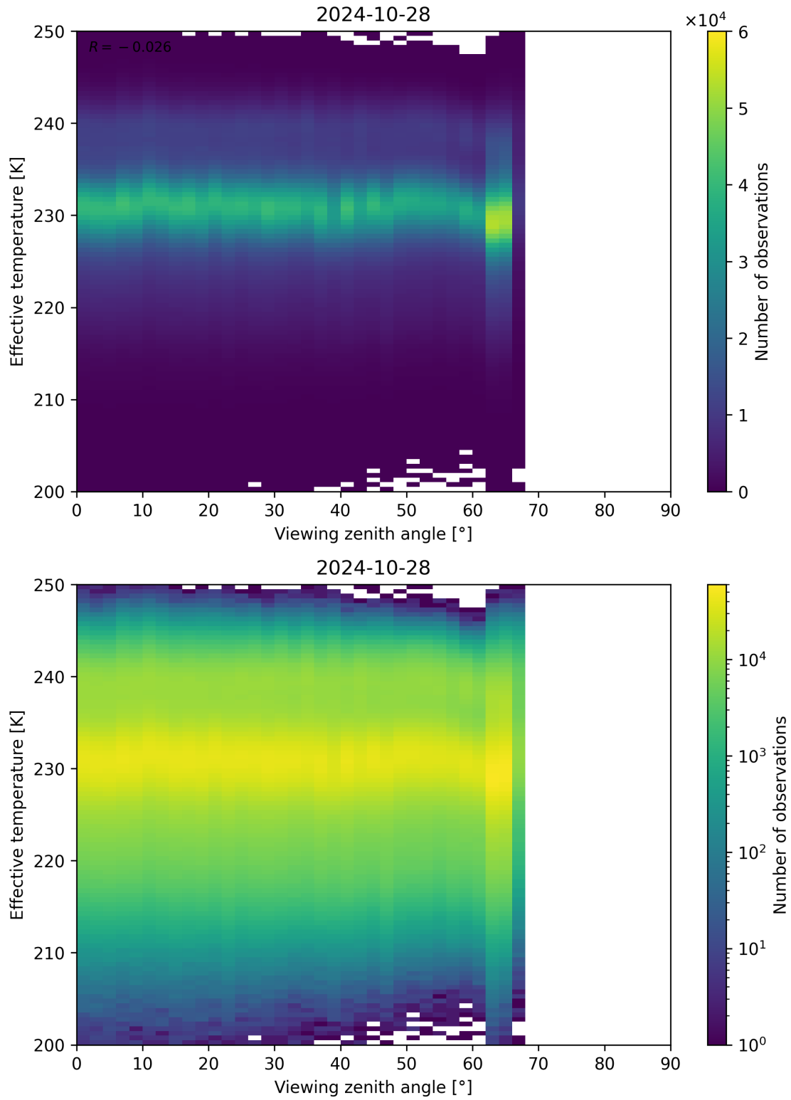
Figure 50: Scatter density plot of “Viewing zenith angle” against “Effective temperature” for 2024-10-27 to 2024-10-29.
