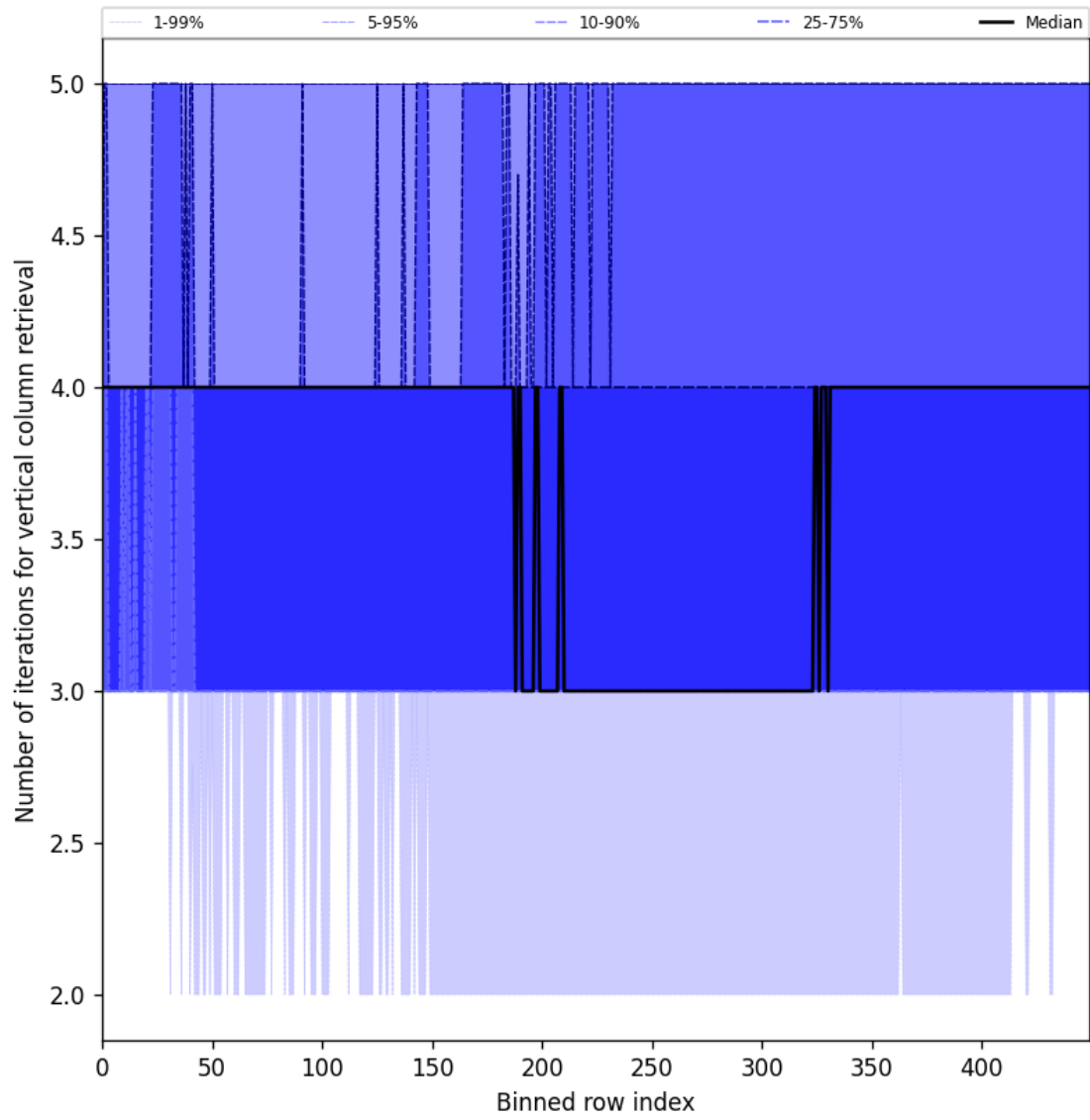
Figure 33: Along track statistics of “Number of iterations for vertical column retrieval” for 2024-10-27 to 2024-10-29
