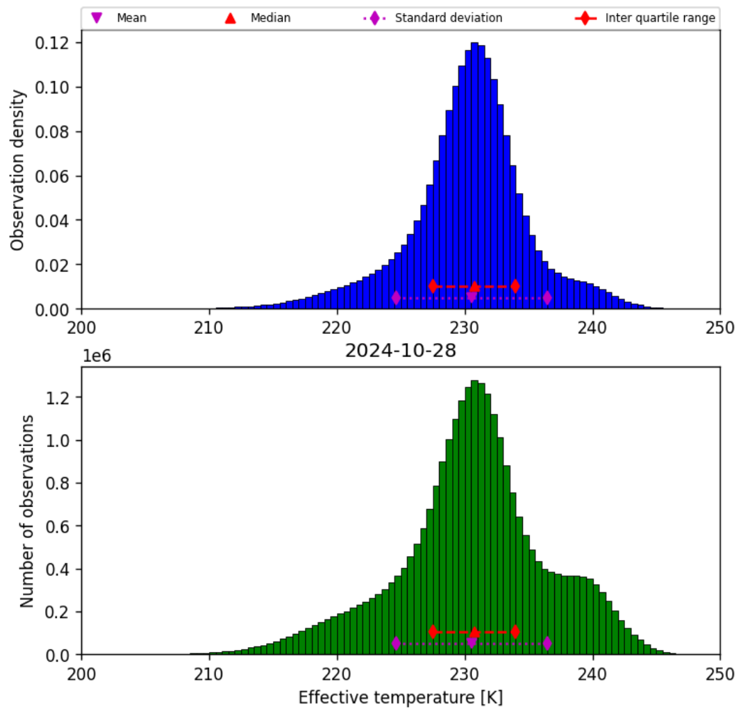
Figure 24: Histogram of “Effective temperature” for 2024-10-27 to 2024-10-29
