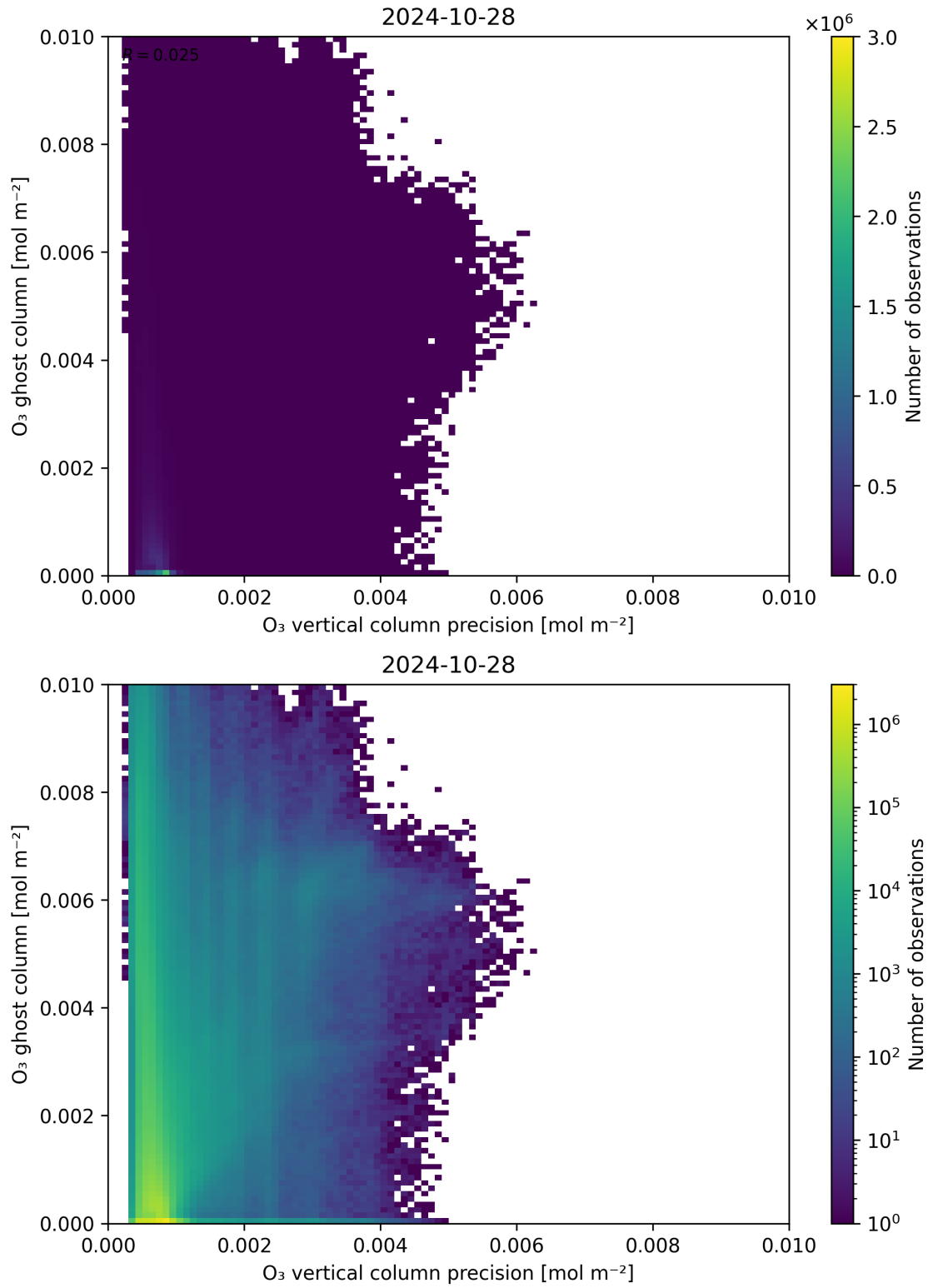
Figure 43: Scatter density plot of “ \text{O}_3 vertical column precision” against “ \text{O}_3 ghost column” for 2024-10-27 to 2024-10-29.
