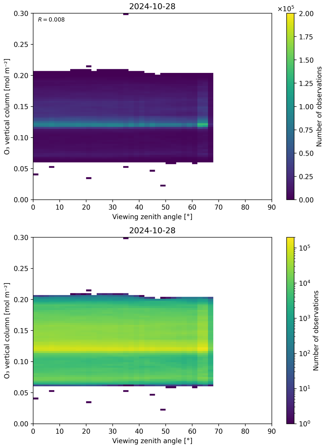
Figure 52: Scatter density plot of “Viewing zenith angle” against “O 3 vertical column” for 2024-10-27 to 2024-10-29.
