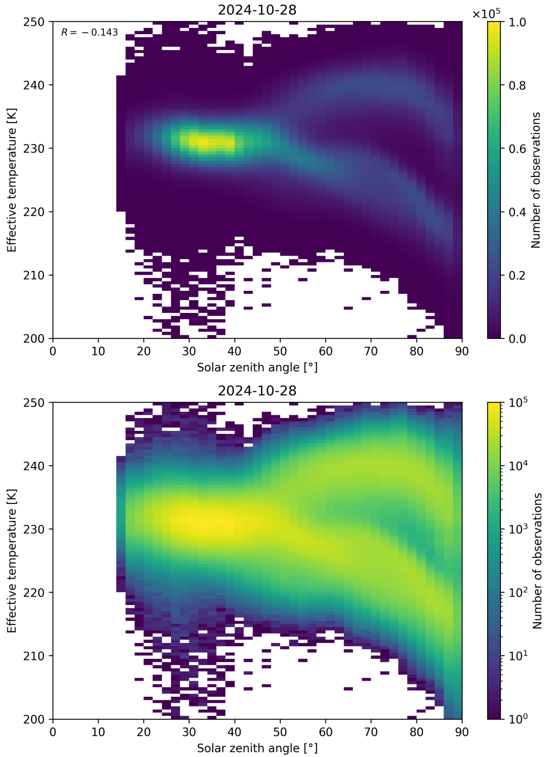
Figure 45: Scatter density plot of “Solar zenith angle” against “Effective temperature” for 2024-10-27 to 2024-10-29.
