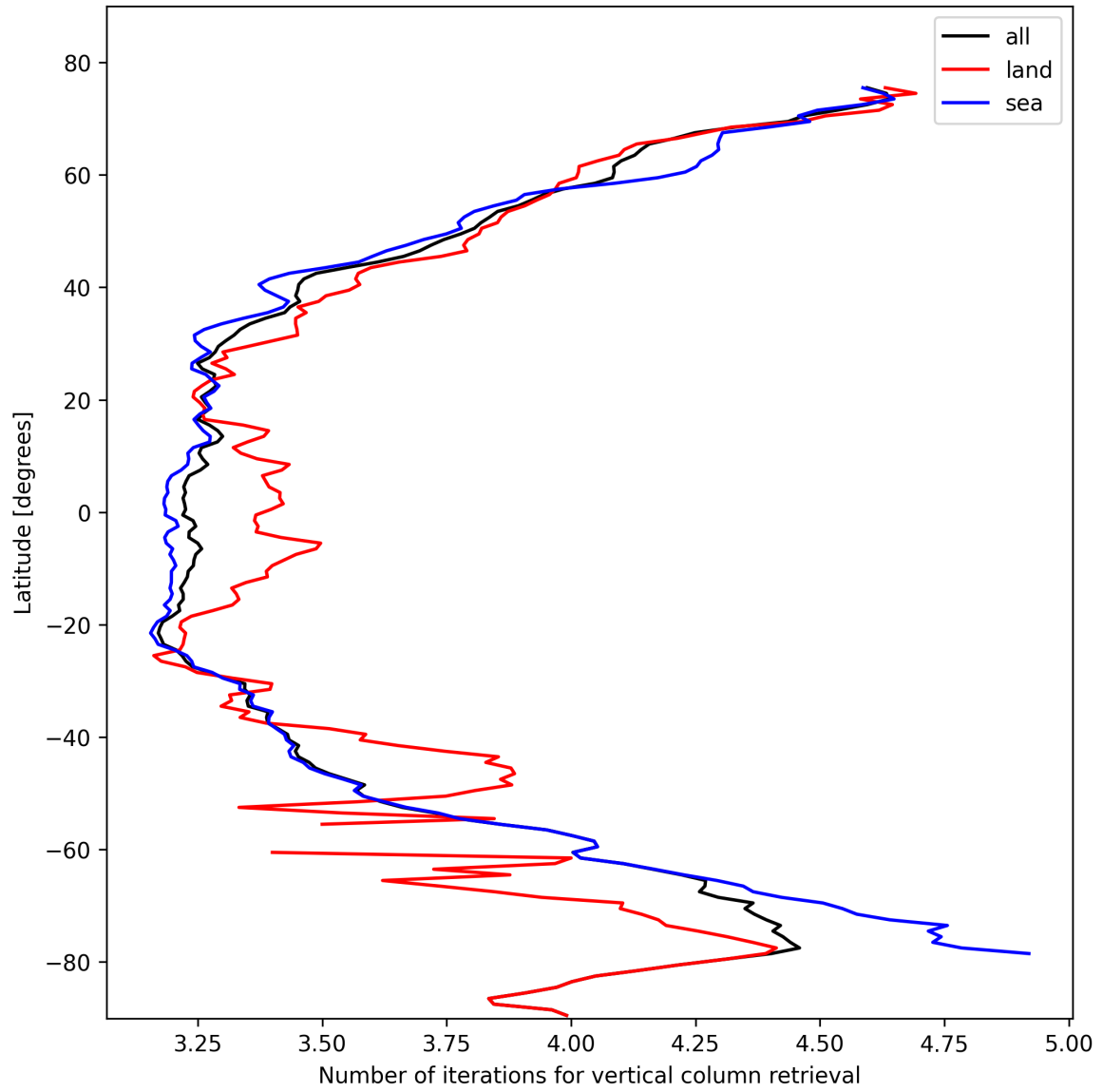
Figure 19: Zonal average of “Number of iterations for vertical column retrieval” for 2024-10-27 to 2024-10-29.
