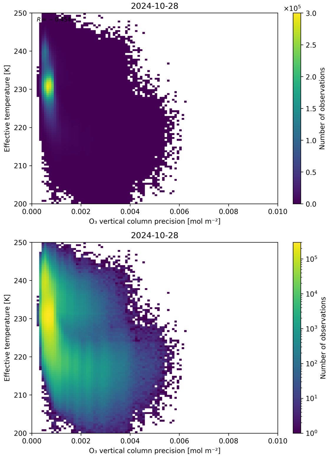
Figure 42: Scatter density plot of “ O_3 vertical column precision” against “Effective temperature” for 2024-10-27 to 2024-10-29.
