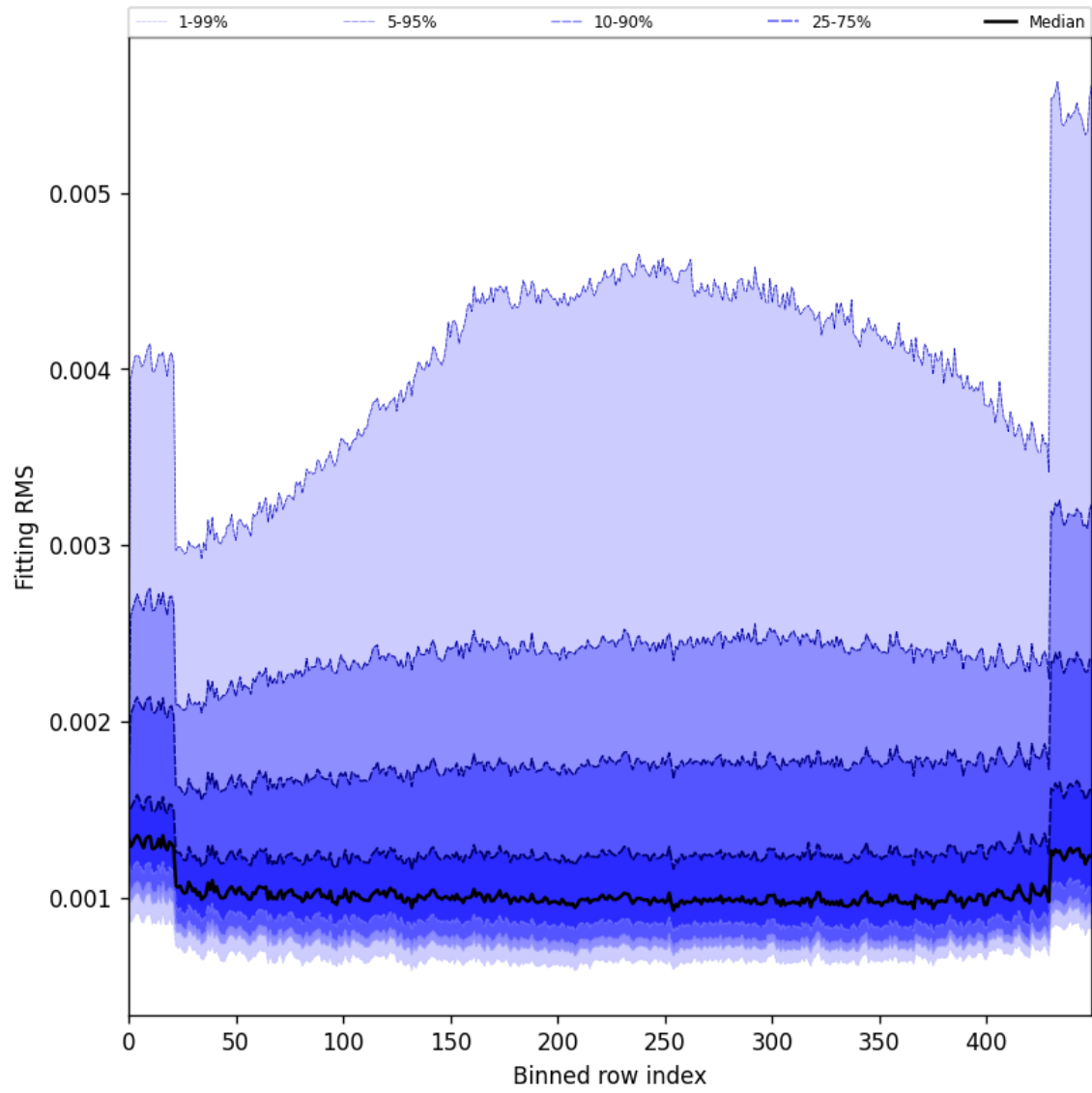
Figure 30: Along track statistics of “Fitting RMS” for 2024-10-27 to 2024-10-29
