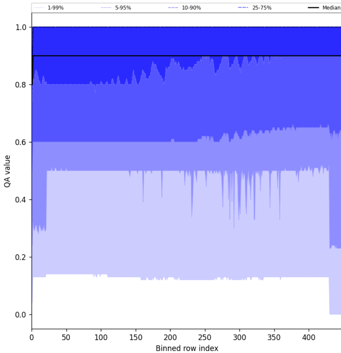
Figure 27: Along track statistics of “QA value” for 2024-10-27 to 2024-10-29
