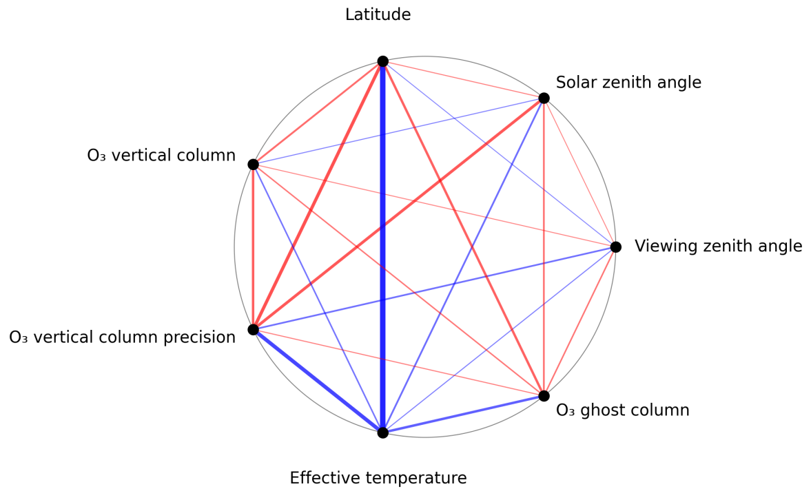
Figure 1: Map of correlation graph for 2024-10-27 to 2024-10-29.
