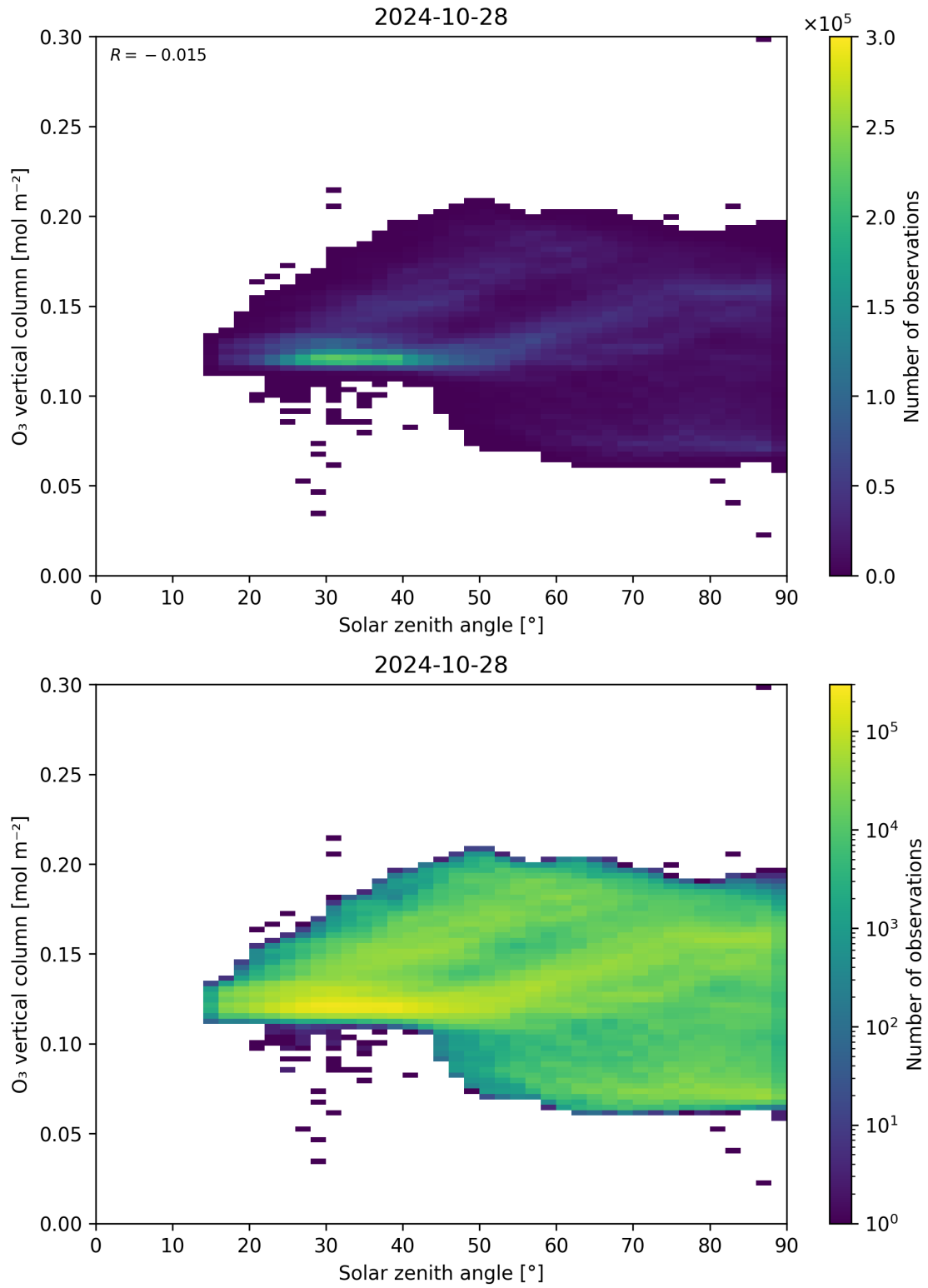
Figure 47: Scatter density plot of “Solar zenith angle” against “O 3 vertical column” for 2024-10-27 to 2024-10-29.
