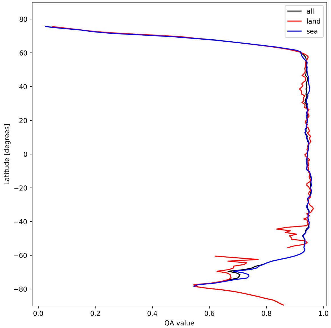
Figure 13: Zonal average of “QA value” for 2024-10-27 to 2024-10-29.
