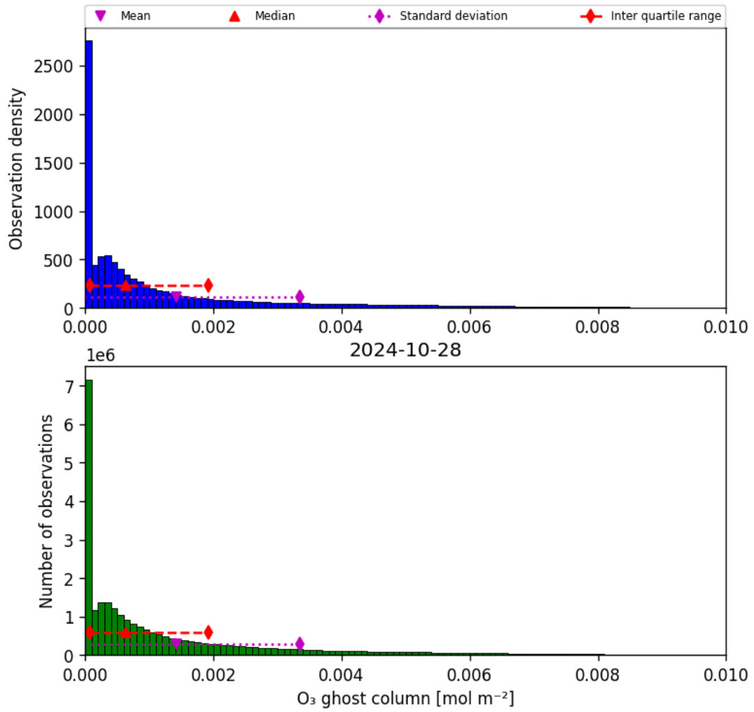
Figure 25: Histogram of “O 3 ghost column” for 2024-10-27 to 2024-10-29
