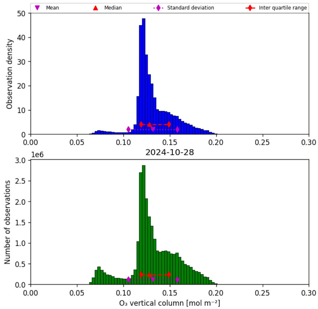
Figure 21: Histogram of “O 3 vertical column” for 2024-10-27 to 2024-10-29
