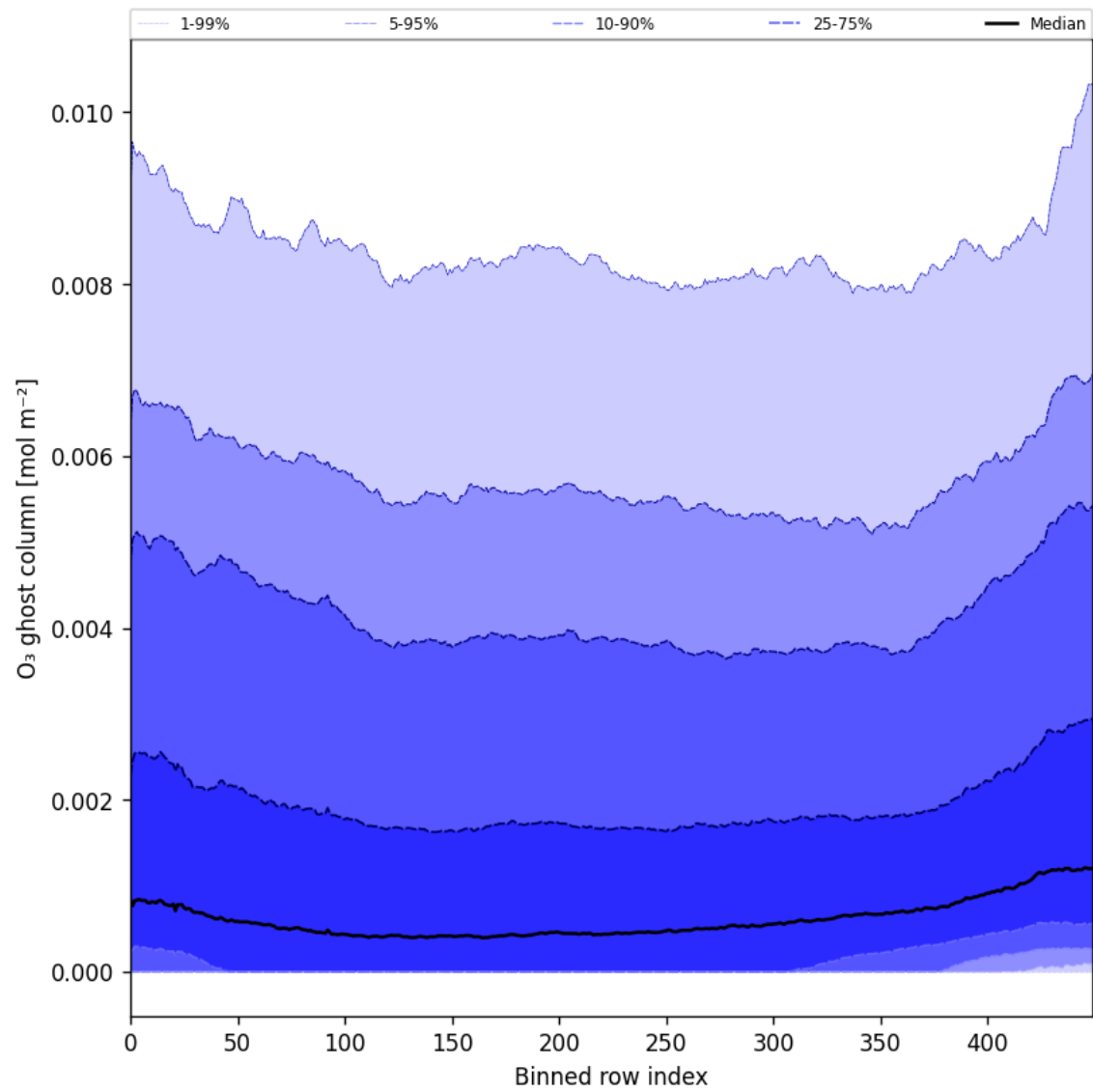
Figure 32: Along track statistics of “O 3 ghost column” for 2024-10-27 to 2024-10-29
