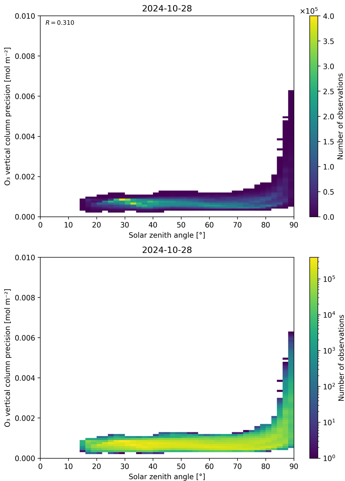
Figure 48: Scatter density plot of “Solar zenith angle” against “O 3 vertical column precision” for 2024-10-27 to 2024-10-29.
