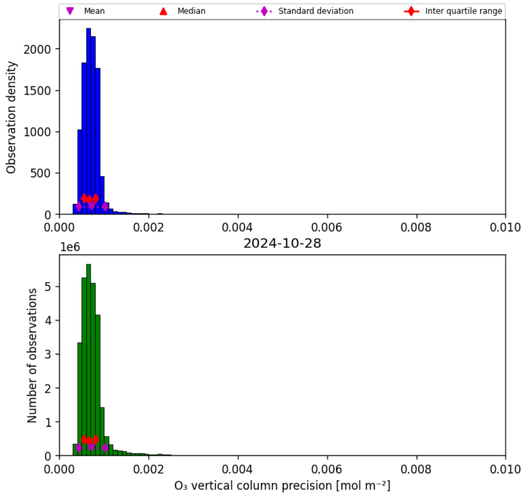
Figure 22: Histogram of “O 3 vertical column precision” for 2024-10-27 to 2024-10-29
