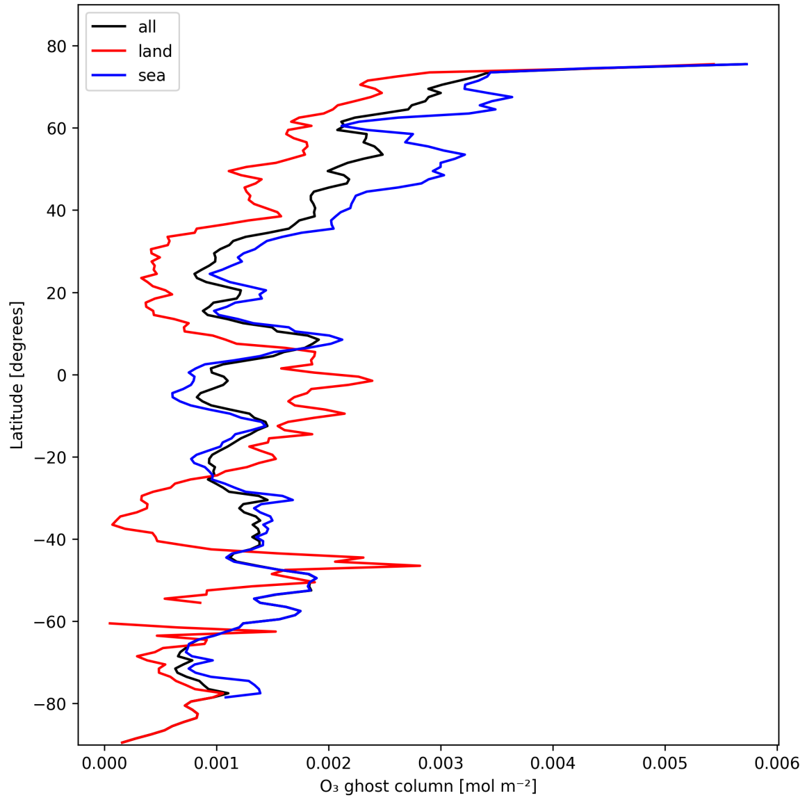
Figure 18: Zonal average of "O 3 ghost column" for 2024-10-27 to 2024-10-29.
