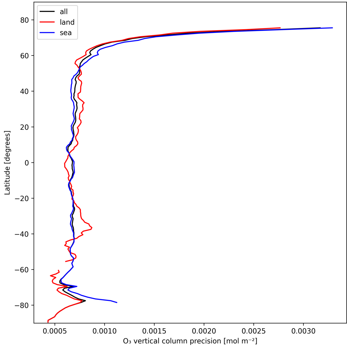
Figure 15: Zonal average of “O 3 vertical column precision” for 2024-10-27 to 2024-10-29.
