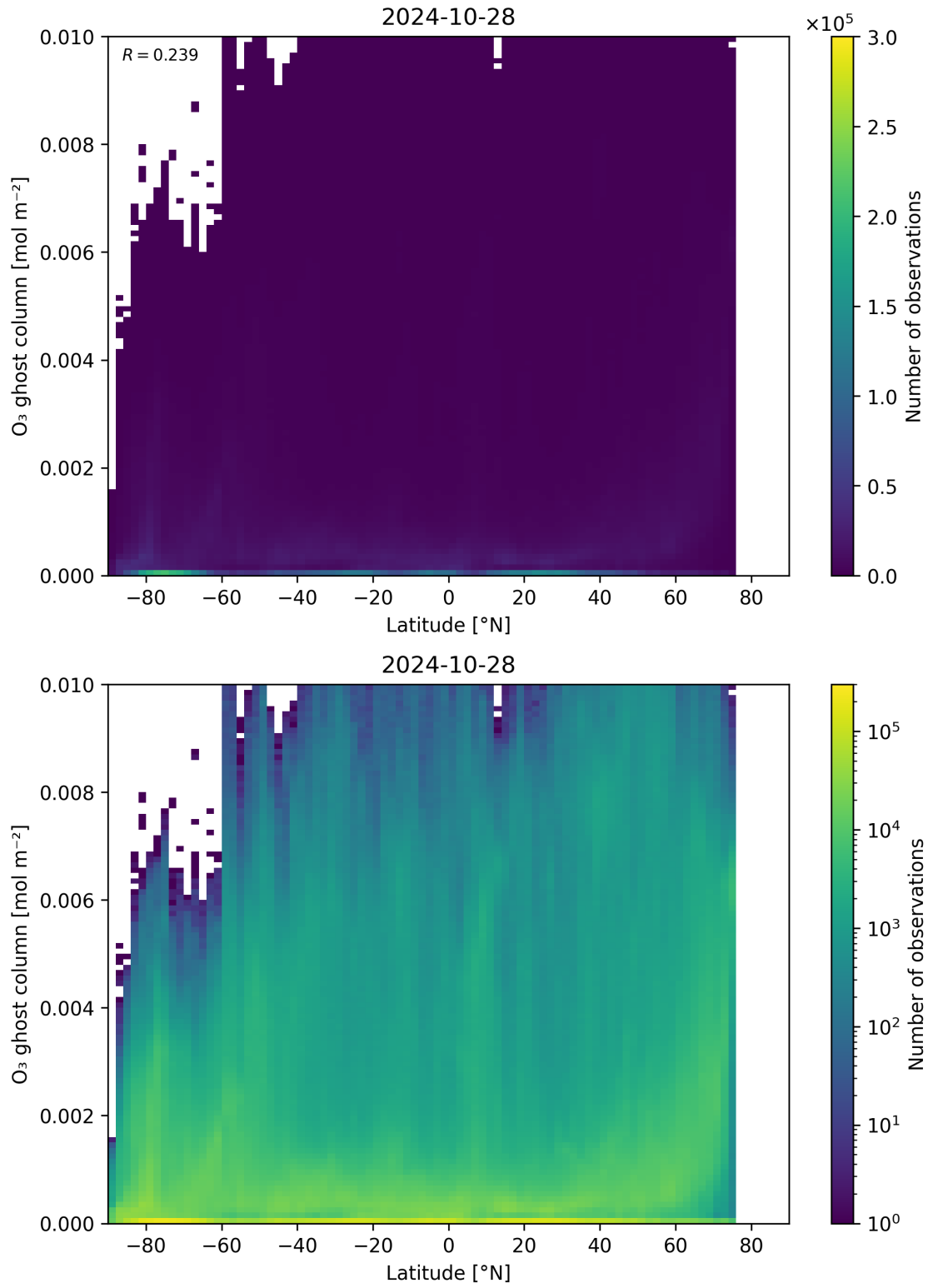
Figure 35: Scatter density plot of “Latitude” against “O 3 ghost column” for 2024-10-27 to 2024-10-29.
