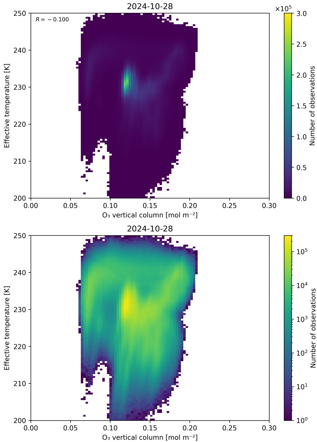
Figure 39: Scatter density plot of “O 3 vertical column” against “Effective temperature” for 2024-10-27 to 2024-10-29.
