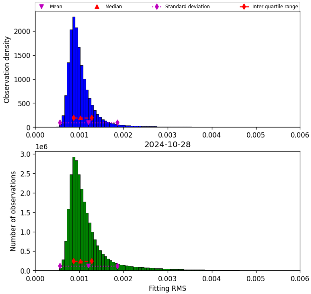
Figure 23: Histogram of “Fitting RMS” for 2024-10-27 to 2024-10-29
