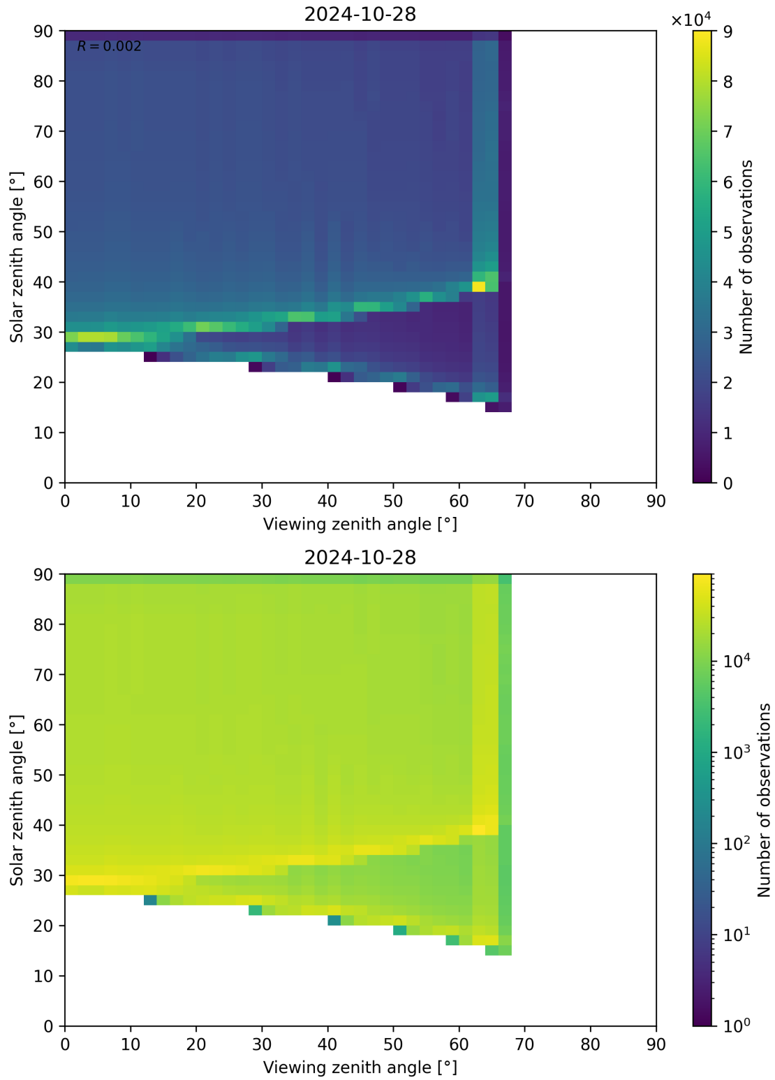
Figure 54: Scatter density plot of “Viewing zenith angle” against “Solar zenith angle” for 2024-10-27 to 2024-10-29.
