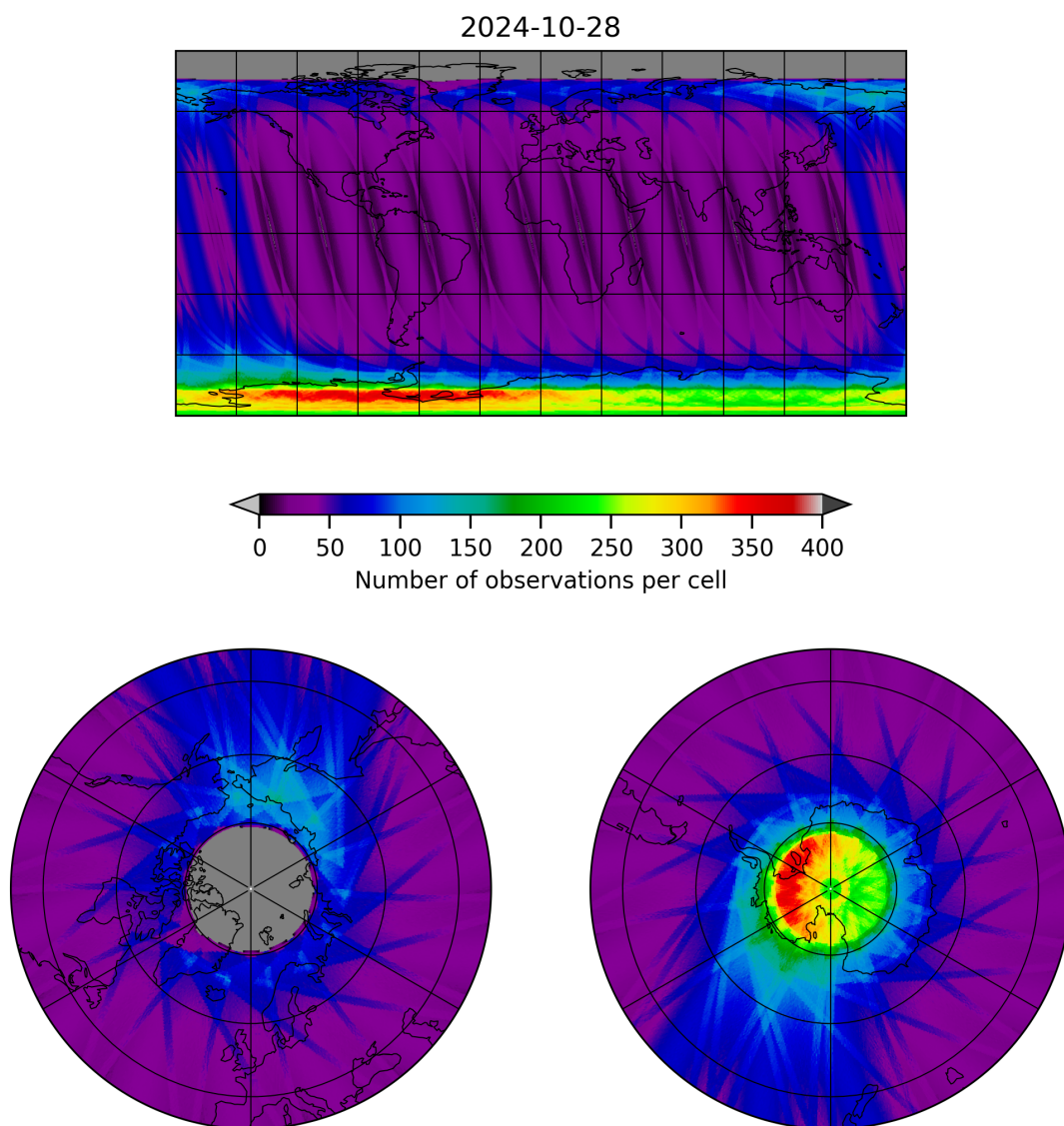
Figure 12: Map of the number of observations for 2024-10-27 to 2024-10-29
