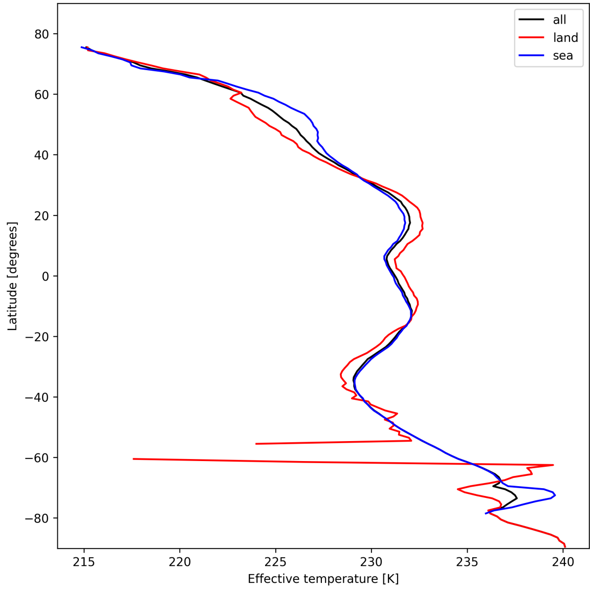
Figure 17: Zonal average of “Effective temperature” for 2024-10-27 to 2024-10-29.
