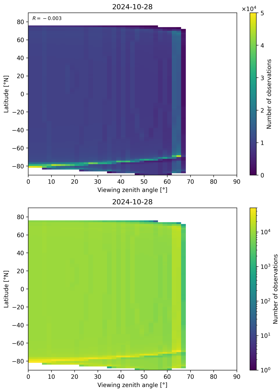
Figure 49: Scatter density plot of “Viewing zenith angle” against “Latitude” for 2024-10-27 to 2024-10-29.
