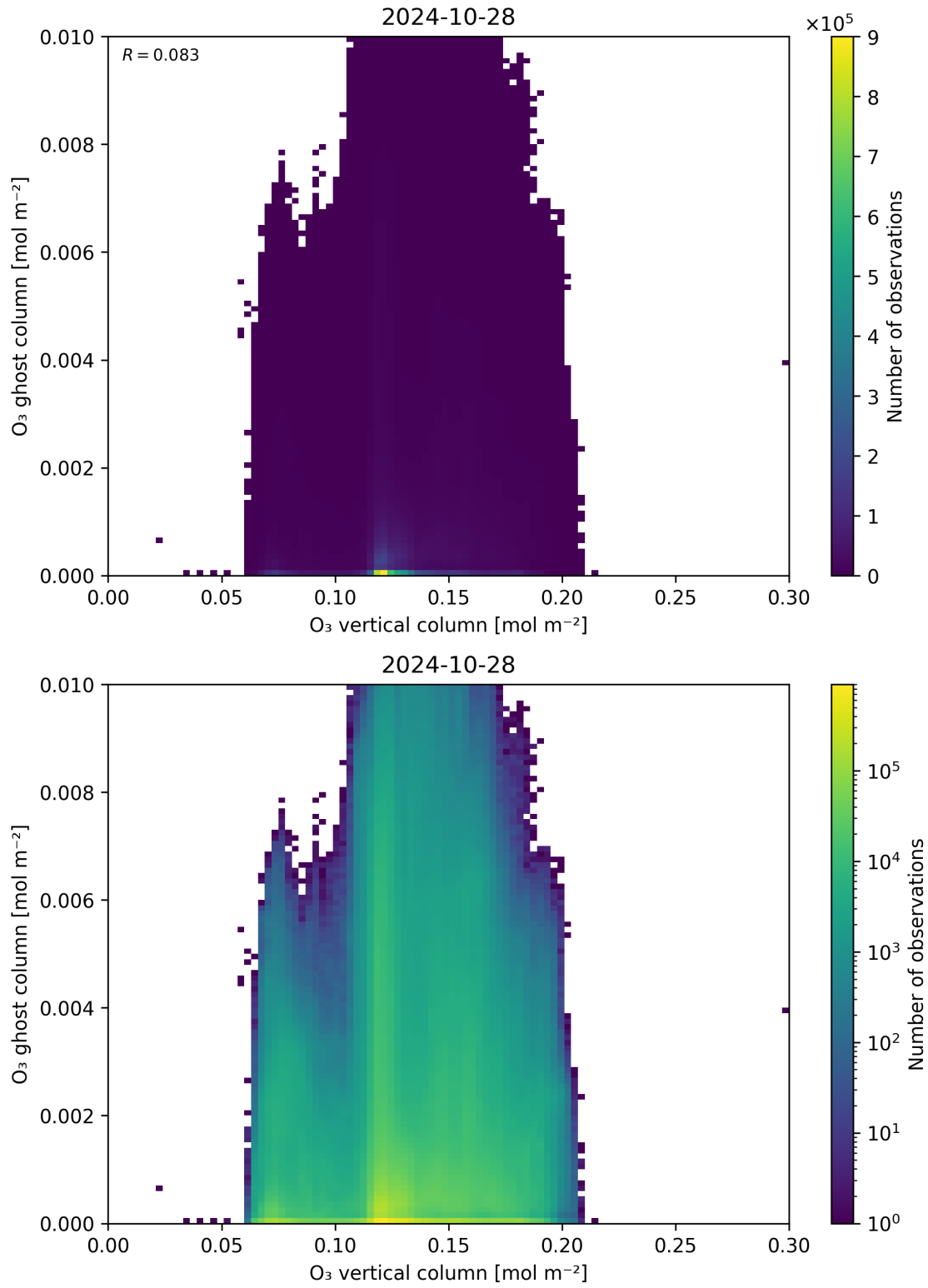
Figure 40: Scatter density plot of “O 3 vertical column” against “O 3 ghost column” for 2024-10-27 to 2024-10-29.
