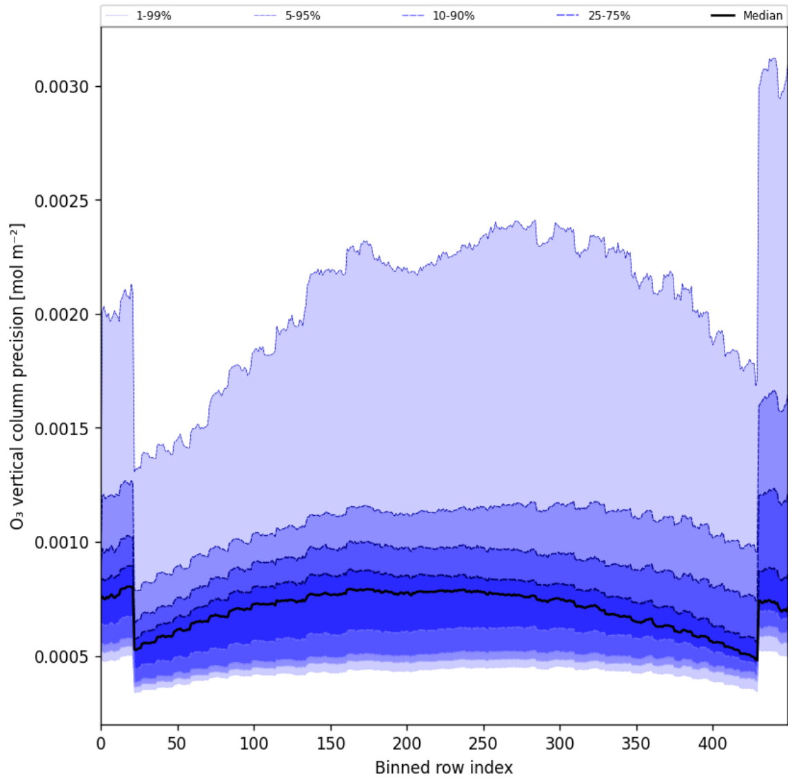
Figure 29: Along track statistics of “O 3 vertical column precision” for 2024-10-27 to 2024-10-29
