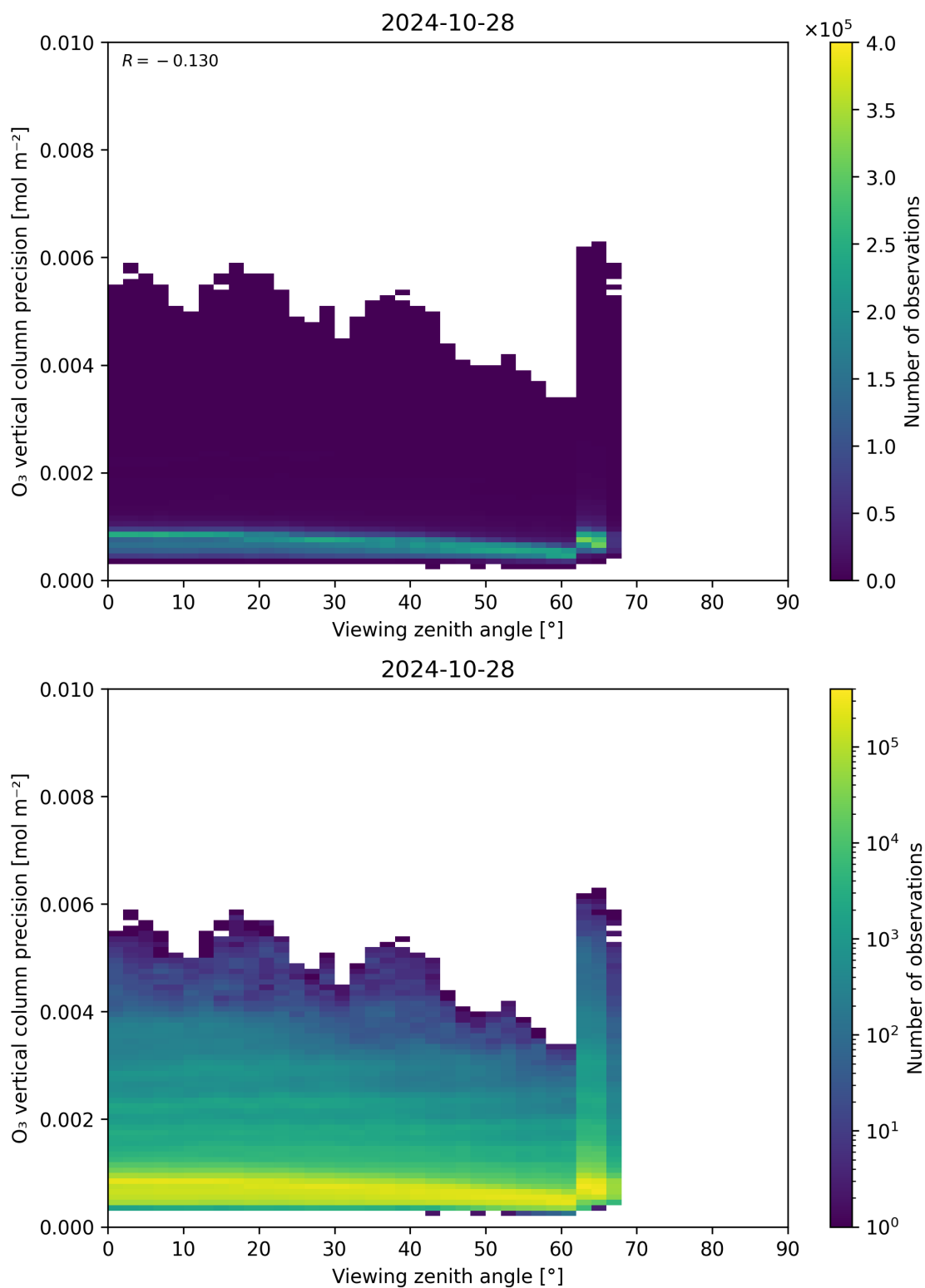
Figure 53: Scatter density plot of “Viewing zenith angle” against “O 3 vertical column precision” for 2024-10-27 to 2024-10-29.
