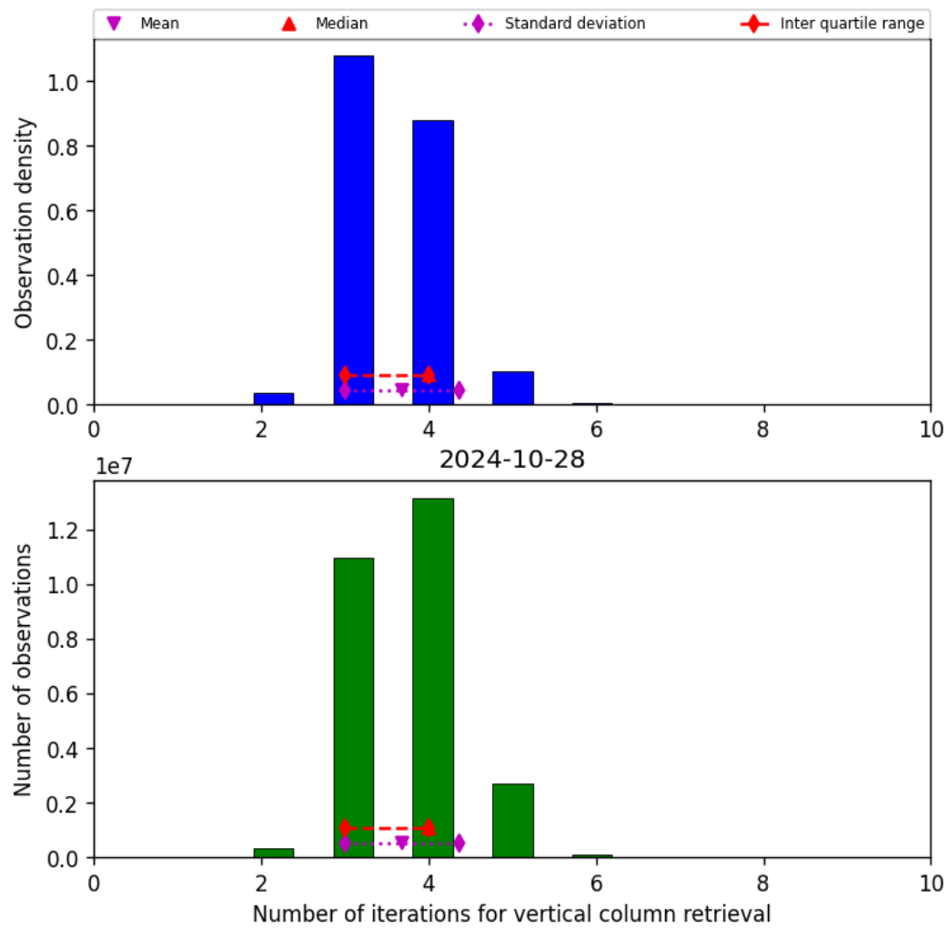
Figure 26: Histogram of “Number of iterations for vertical column retrieval” for 2024-10-27 to 2024-10-29
