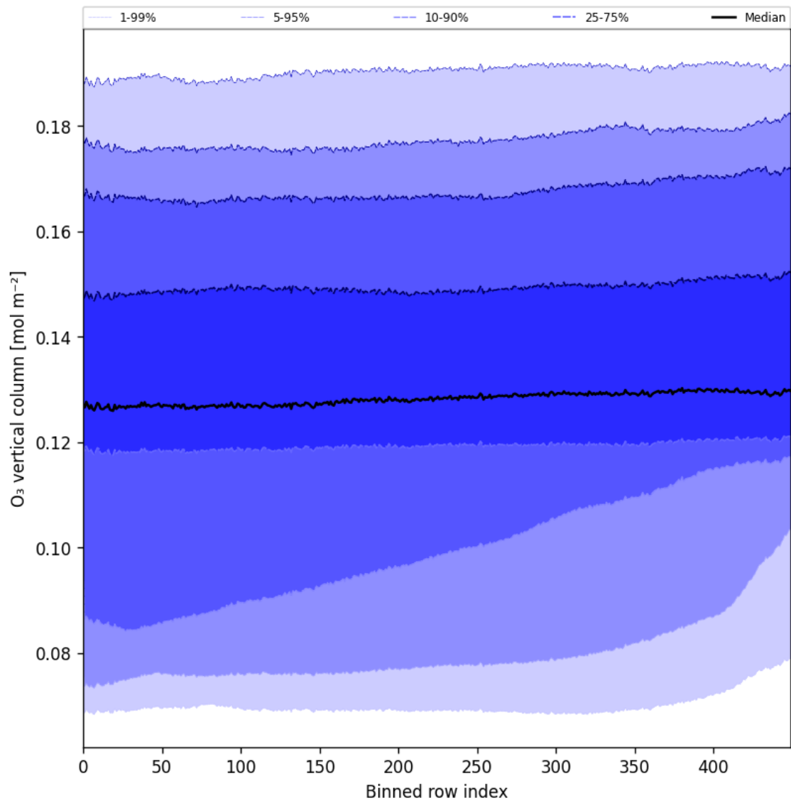
Figure 28: Along track statistics of “O 3 vertical column” for 2024-10-27 to 2024-10-29
