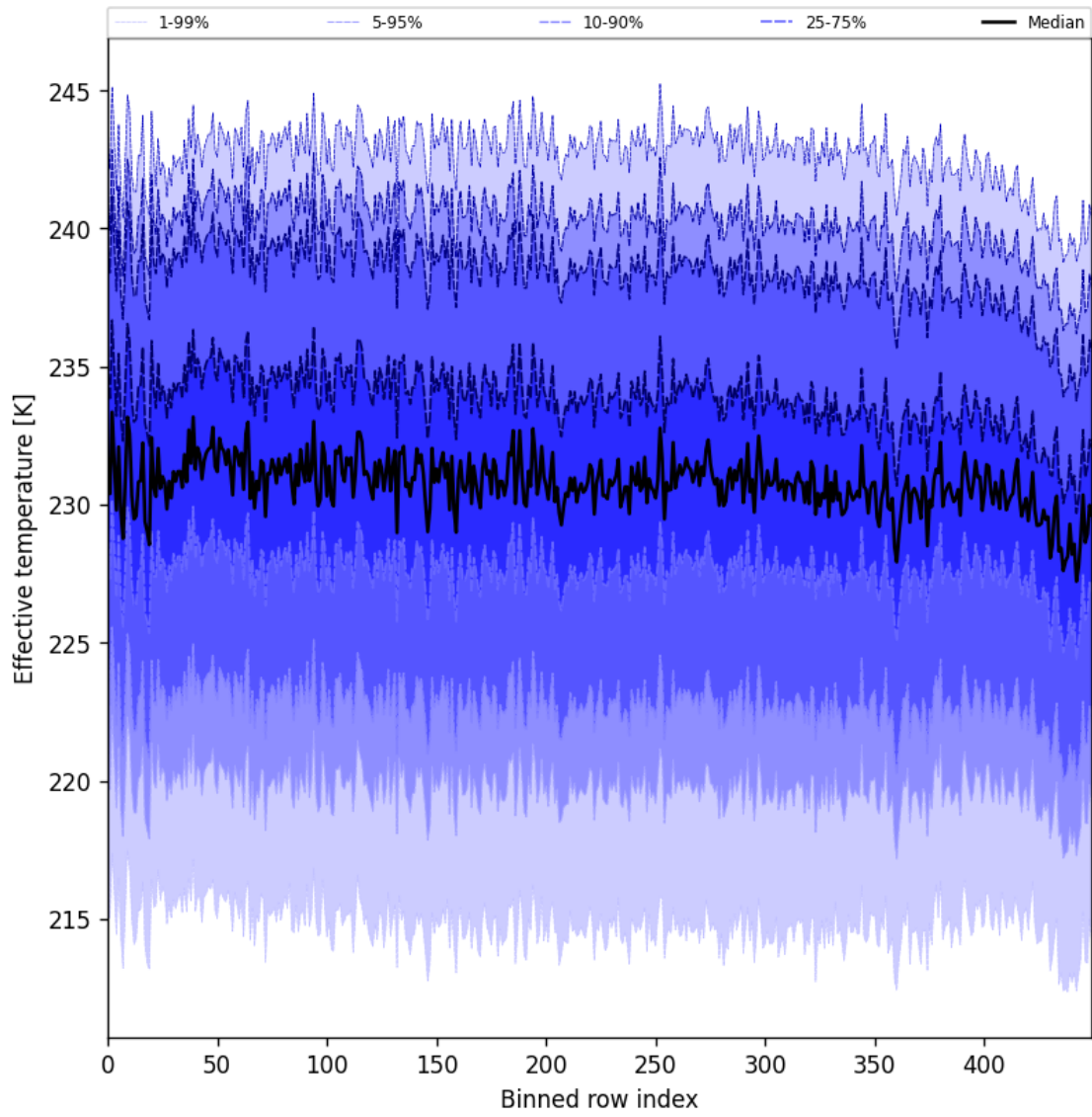
Figure 31: Along track statistics of “Effective temperature” for 2024-10-27 to 2024-10-29
