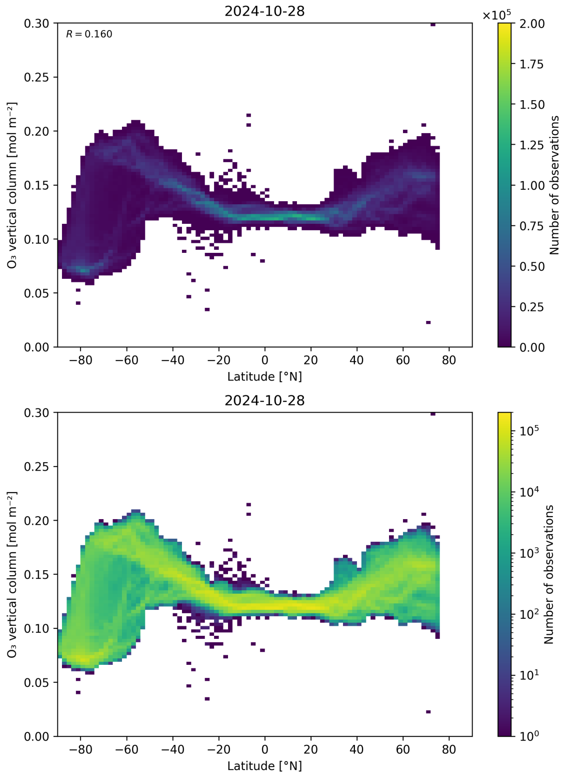
Figure 36: Scatter density plot of “Latitude” against “O 3 vertical column” for 2024-10-27 to 2024-10-29.
