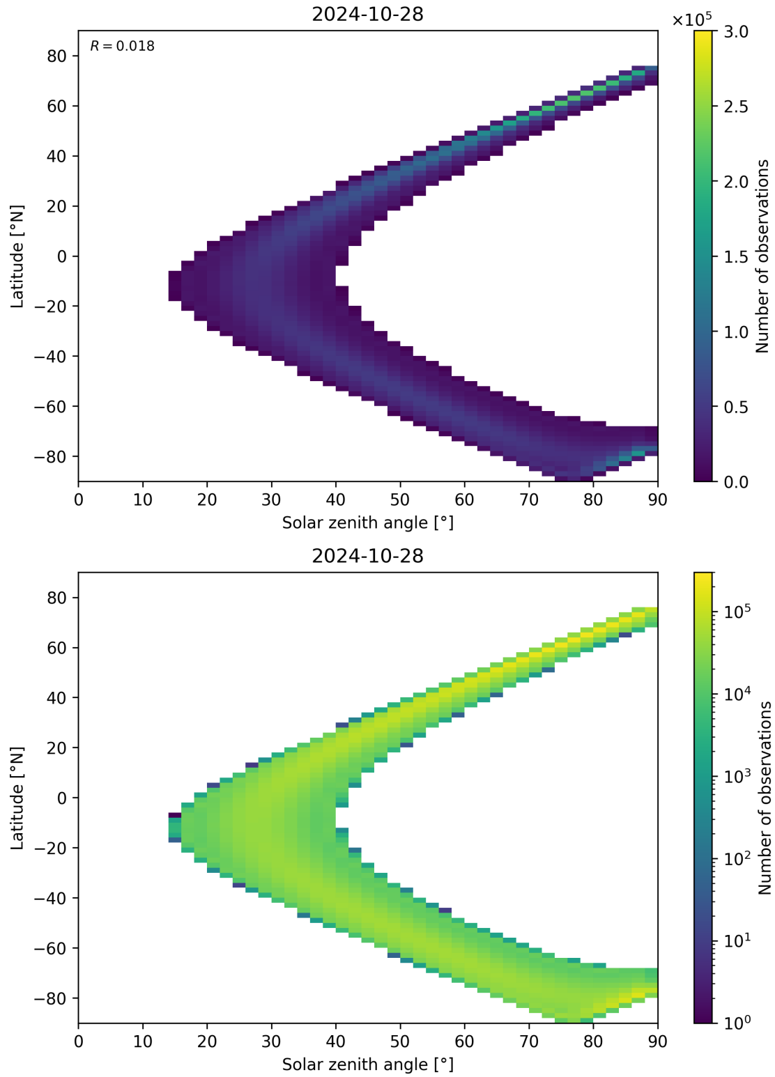
Figure 44: Scatter density plot of “Solar zenith angle” against “Latitude” for 2024-10-27 to 2024-10-29.
