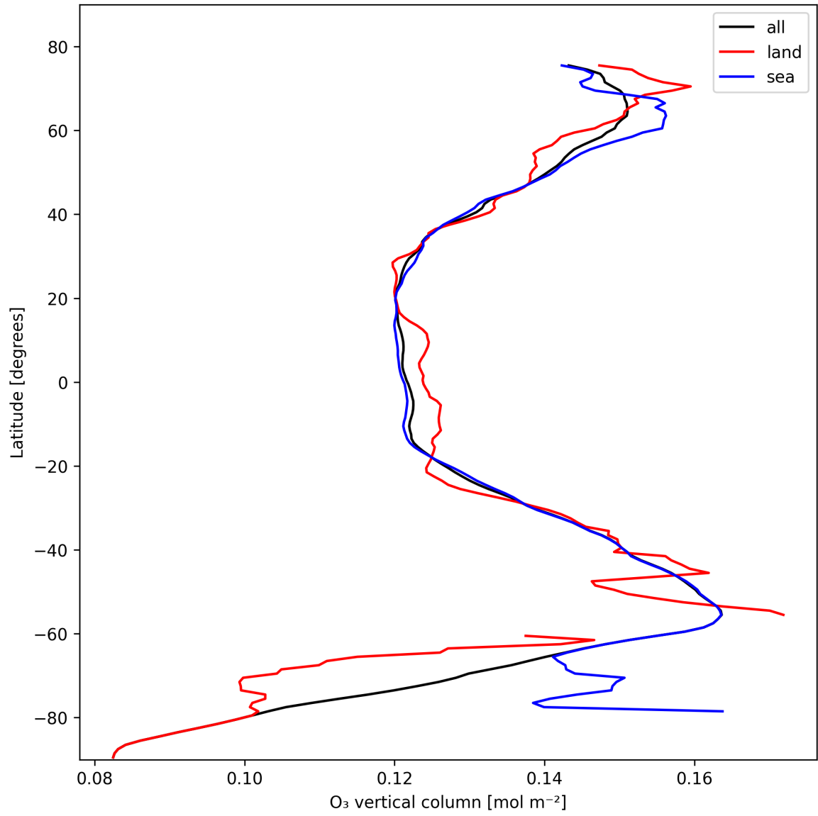
Figure 14: Zonal average of “O 3 vertical column” for 2024-10-27 to 2024-10-29.
