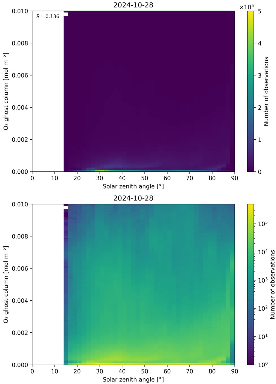
Figure 46: Scatter density plot of “Solar zenith angle” against “O 3 ghost column” for 2024-10-27 to 2024-10-29.
