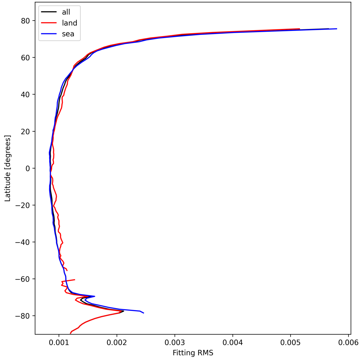
Figure 16: Zonal average of “Fitting RMS” for 2024-10-27 to 2024-10-29.
