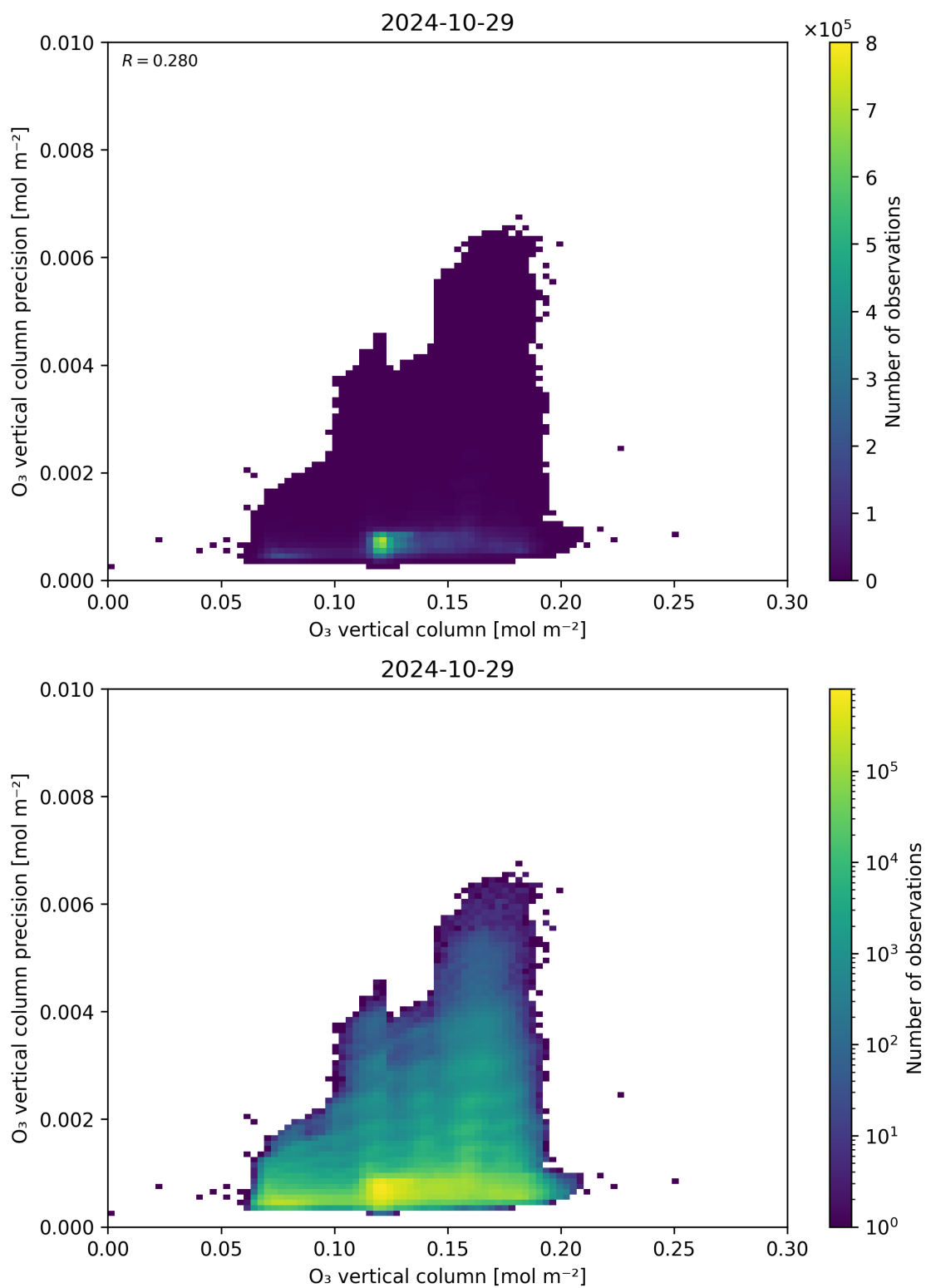
Figure 41: Scatter density plot of “O 3 vertical column” against “O 3 vertical column precision” for 2024-10-29 to 2024-10-30.
