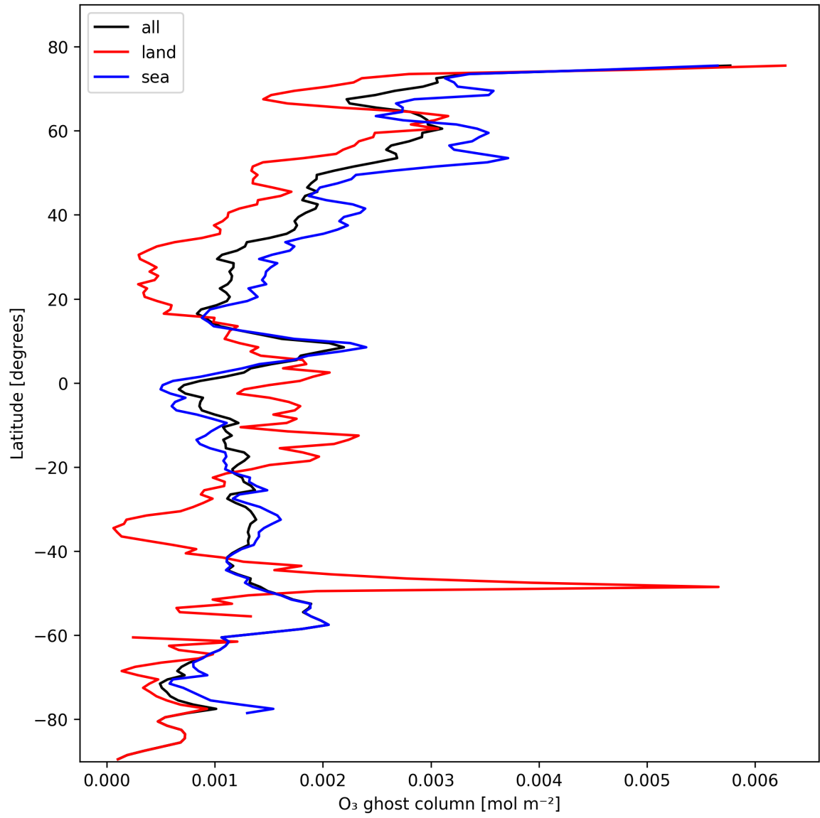
Figure 18: Zonal average of "O 3 ghost column" for 2024-10-29 to 2024-10-30.
