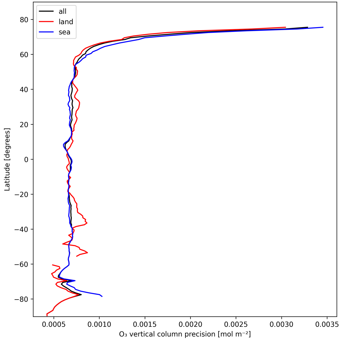
Figure 15: Zonal average of “O 3 vertical column precision” for 2024-10-29 to 2024-10-30.
