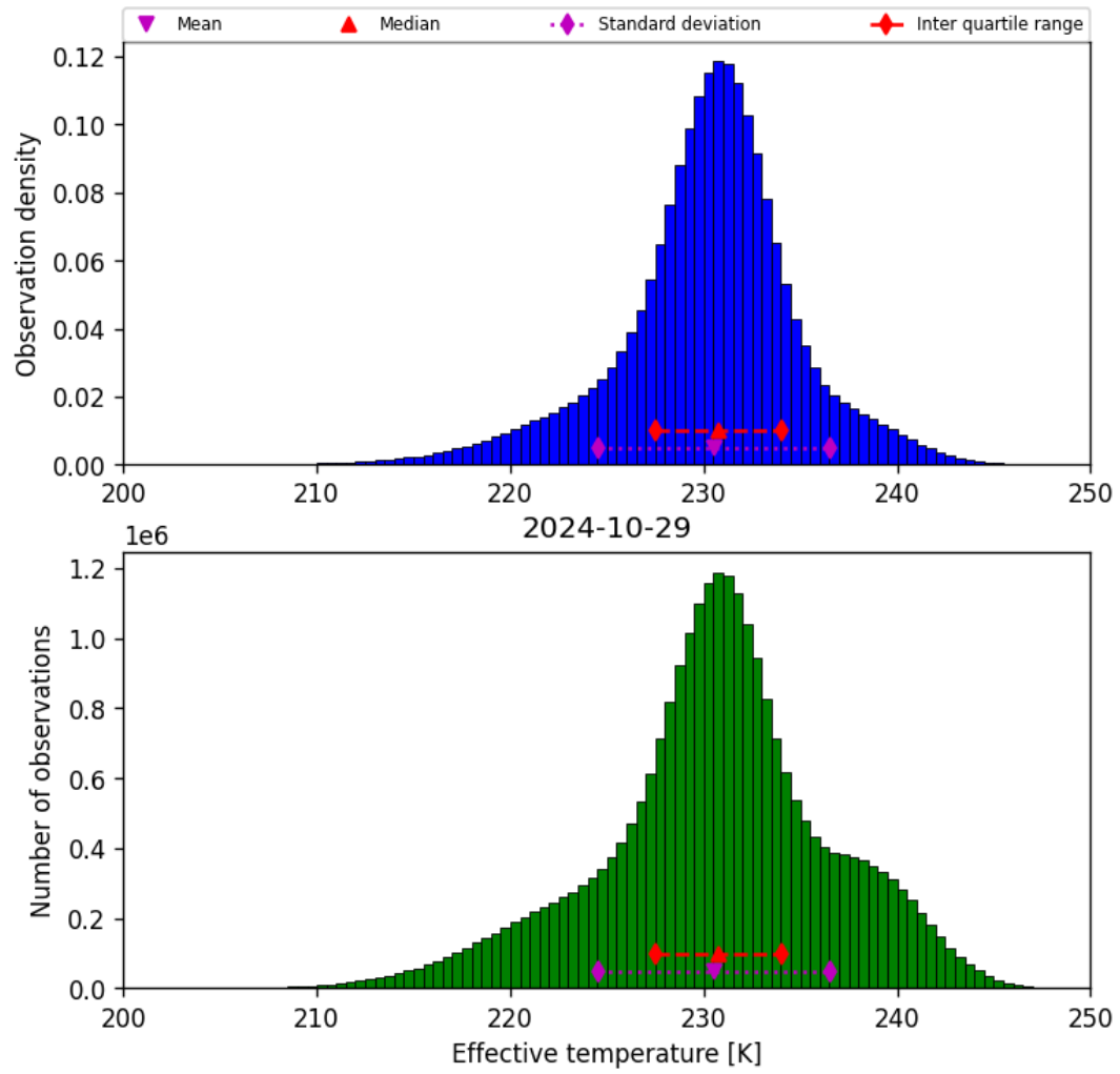
Figure 24: Histogram of “Effective temperature” for 2024-10-29 to 2024-10-30
