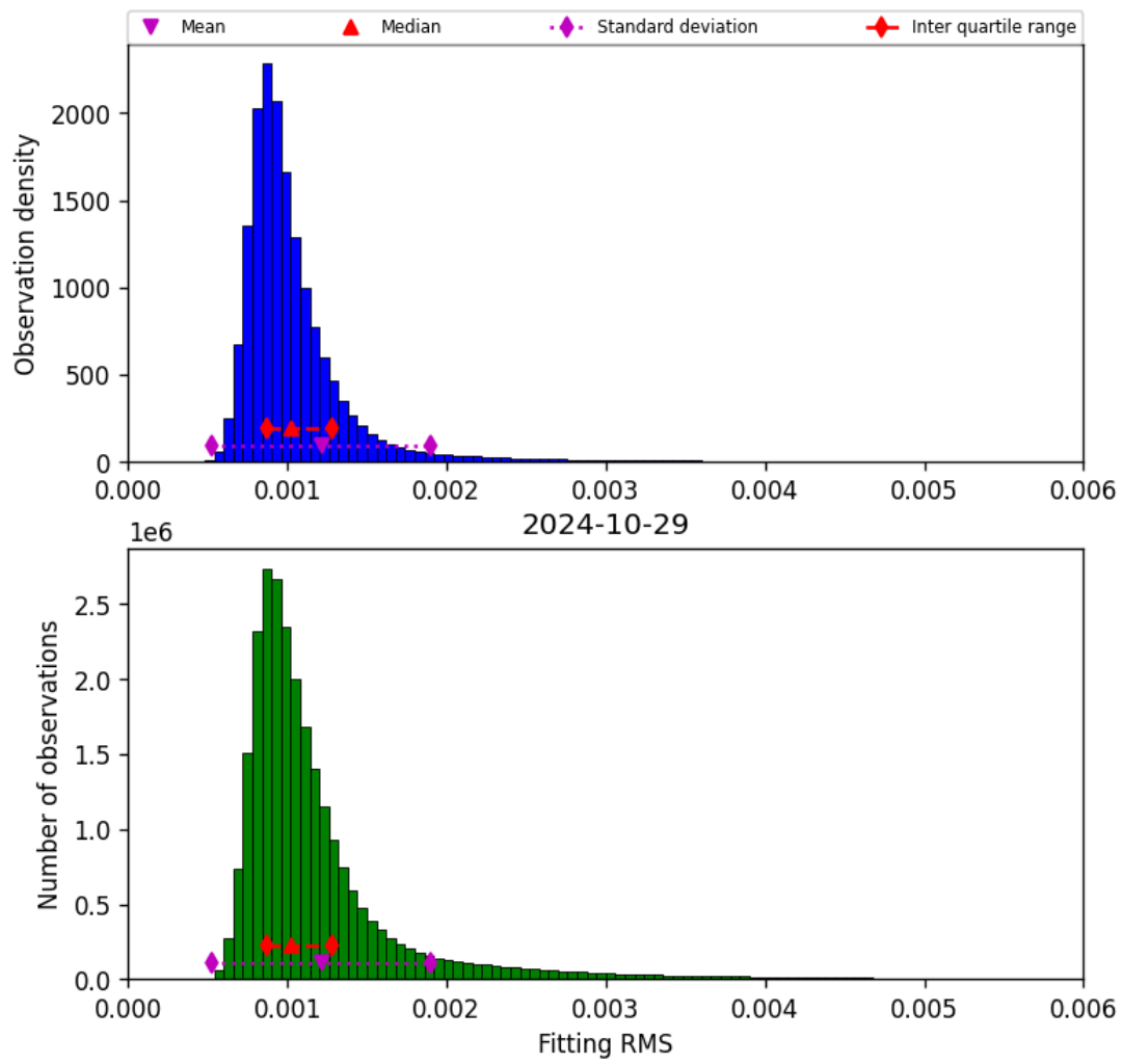
Figure 23: Histogram of “Fitting RMS” for 2024-10-29 to 2024-10-30
