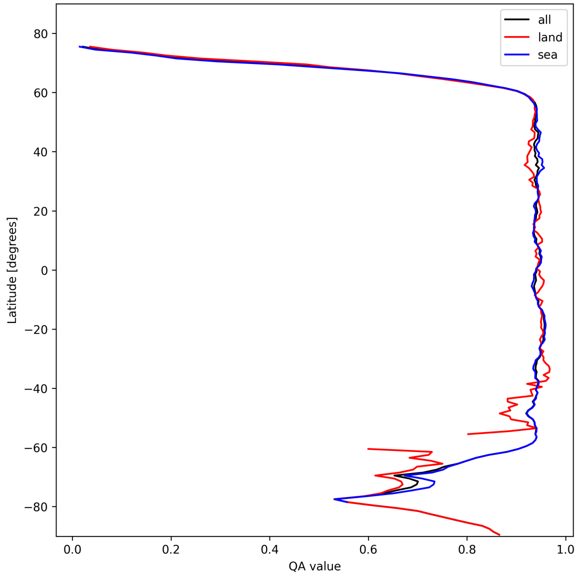
Figure 13: Zonal average of “QA value” for 2024-10-29 to 2024-10-30.
