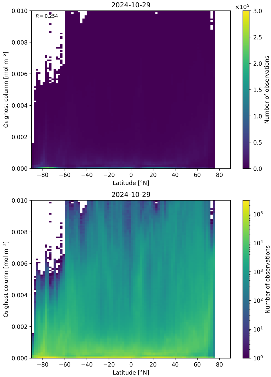
Figure 35: Scatter density plot of “Latitude” against “O 3 ghost column” for 2024-10-29 to 2024-10-30.
