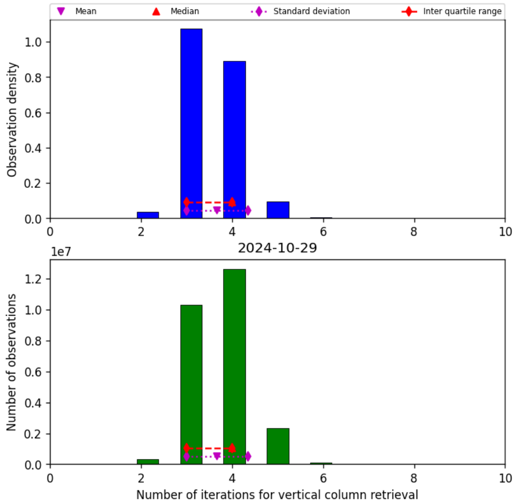
Figure 26: Histogram of “Number of iterations for vertical column retrieval” for 2024-10-29 to 2024-10-30
