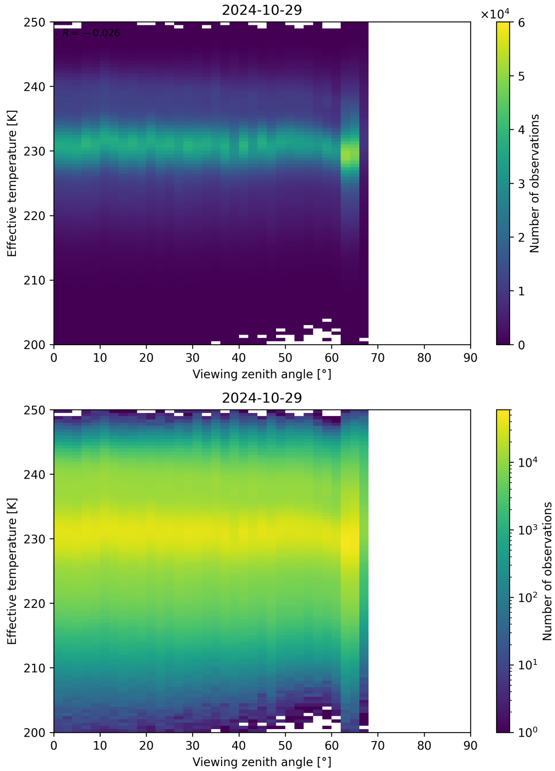
Figure 50: Scatter density plot of “Viewing zenith angle” against “Effective temperature” for 2024-10-29 to 2024-10-30.
