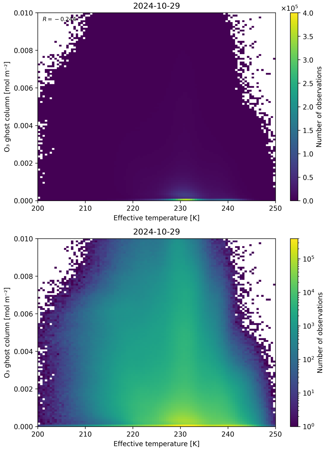
Figure 38: Scatter density plot of “Effective temperature” against “O 3 ghost column” for 2024-10-29 to 2024-10-30.
