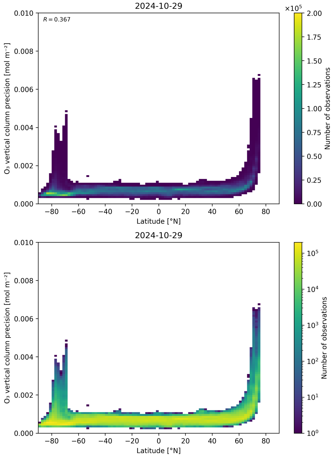
Figure 37: Scatter density plot of “Latitude” against “O 3 vertical column precision” for 2024-10-29 to 2024-10-30.
