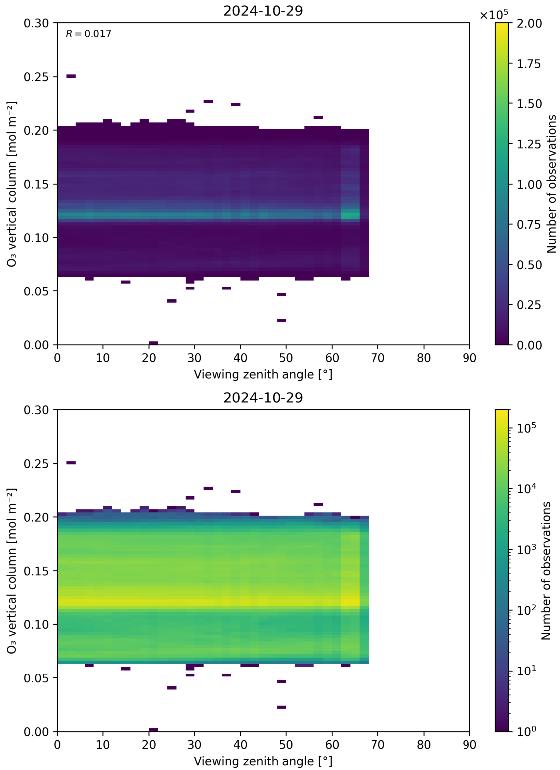
Figure 52: Scatter density plot of “Viewing zenith angle” against “O 3 vertical column” for 2024-10-29 to 2024-10-30.
