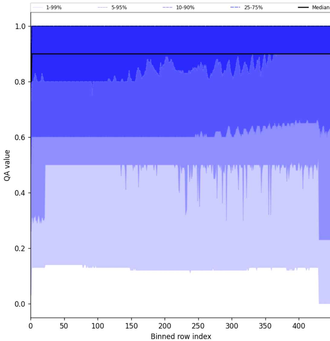
Figure 27: Along track statistics of “QA value” for 2024-10-29 to 2024-10-30
