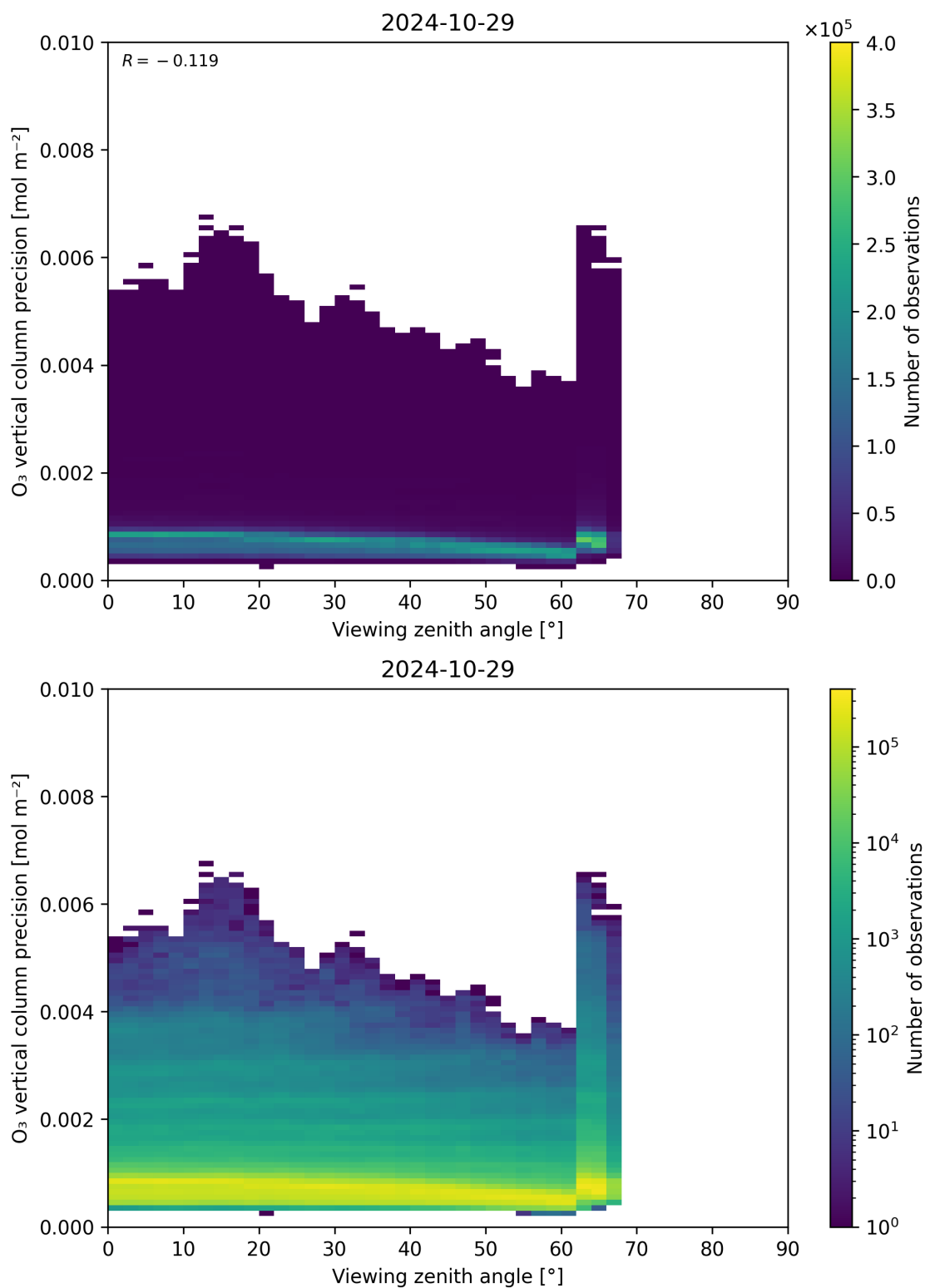
Figure 53: Scatter density plot of “Viewing zenith angle” against “O 3 vertical column precision” for 2024-10-29 to 2024-10-30.
