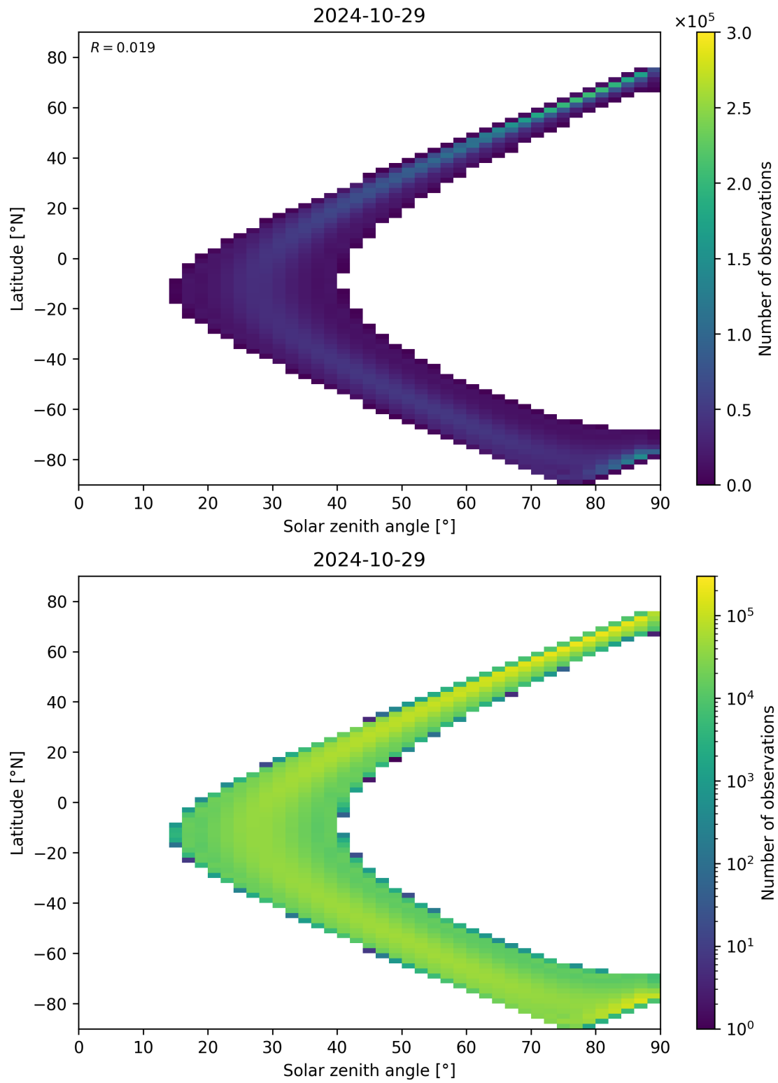
Figure 44: Scatter density plot of “Solar zenith angle” against “Latitude” for 2024-10-29 to 2024-10-30.
