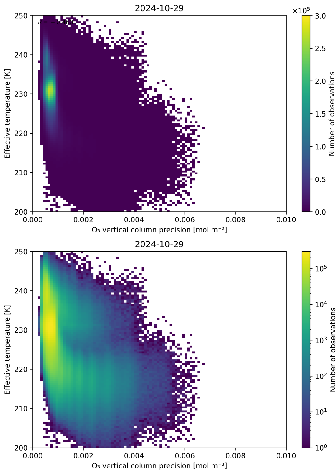
Figure 42: Scatter density plot of “ O_3 vertical column precision” against “Effective temperature” for 2024-10-29 to 2024-10-30.
