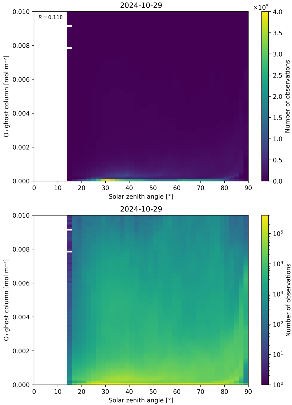
Figure 46: Scatter density plot of “Solar zenith angle” against “O 3 ghost column” for 2024-10-29 to 2024-10-30.
