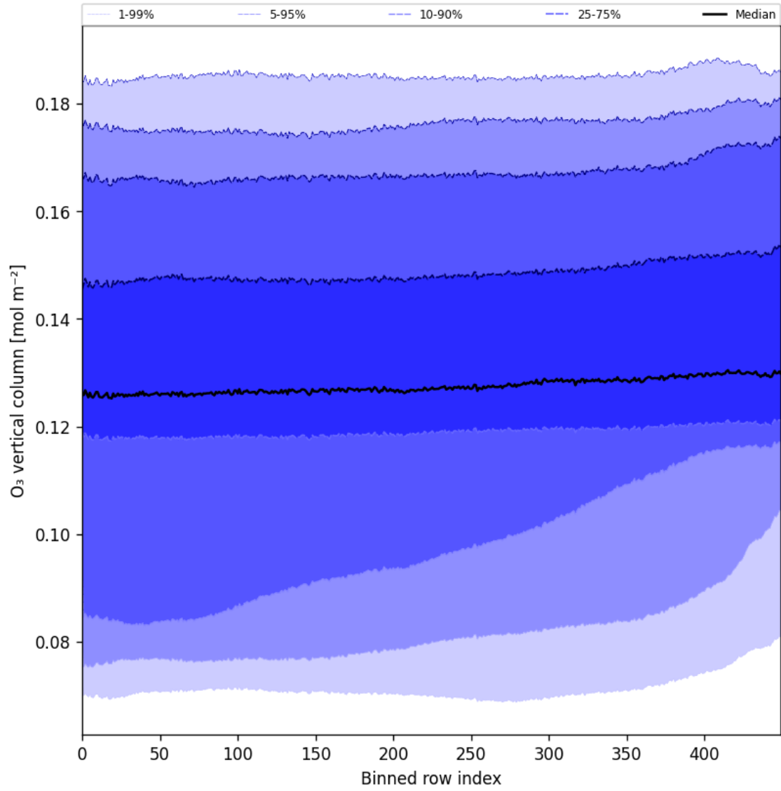
Figure 28: Along track statistics of “O 3 vertical column” for 2024-10-29 to 2024-10-30
