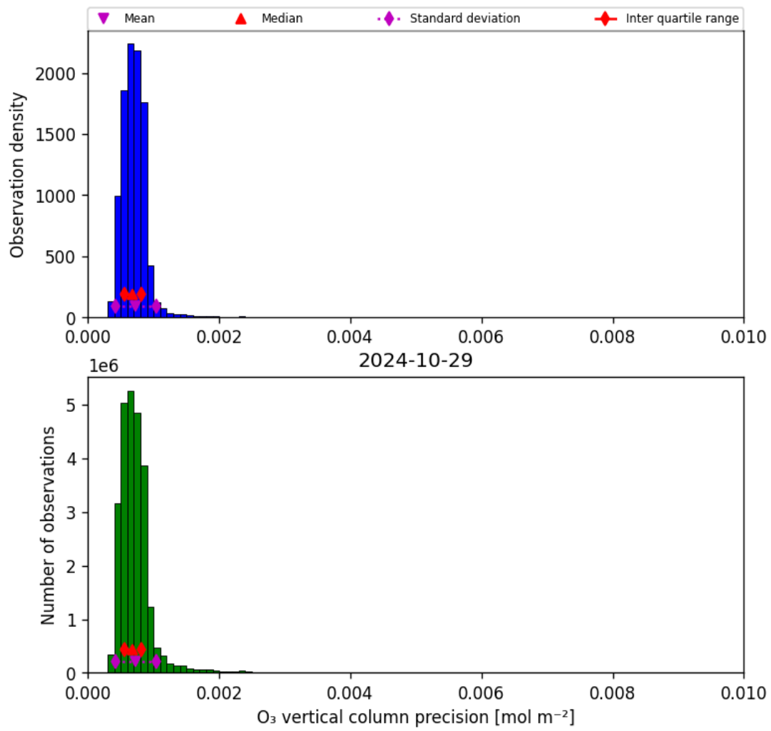
Figure 22: Histogram of “O 3 vertical column precision” for 2024-10-29 to 2024-10-30
