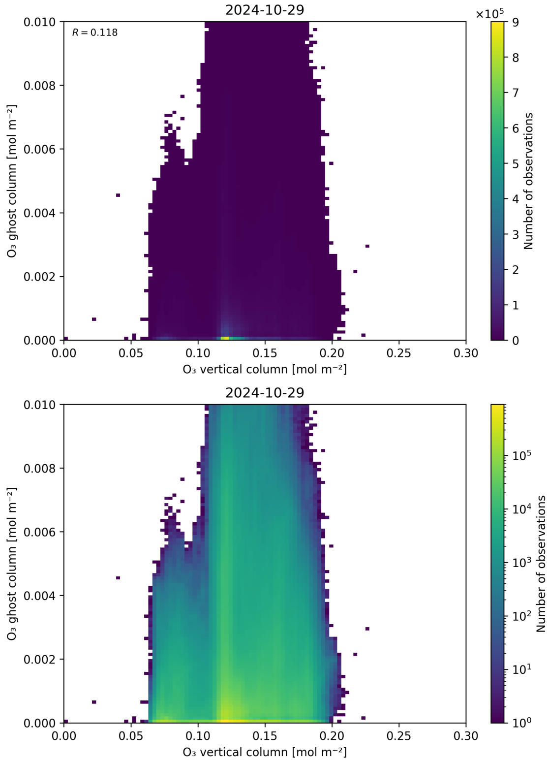
Figure 40: Scatter density plot of “O 3 vertical column” against “O 3 ghost column” for 2024-10-29 to 2024-10-30.
