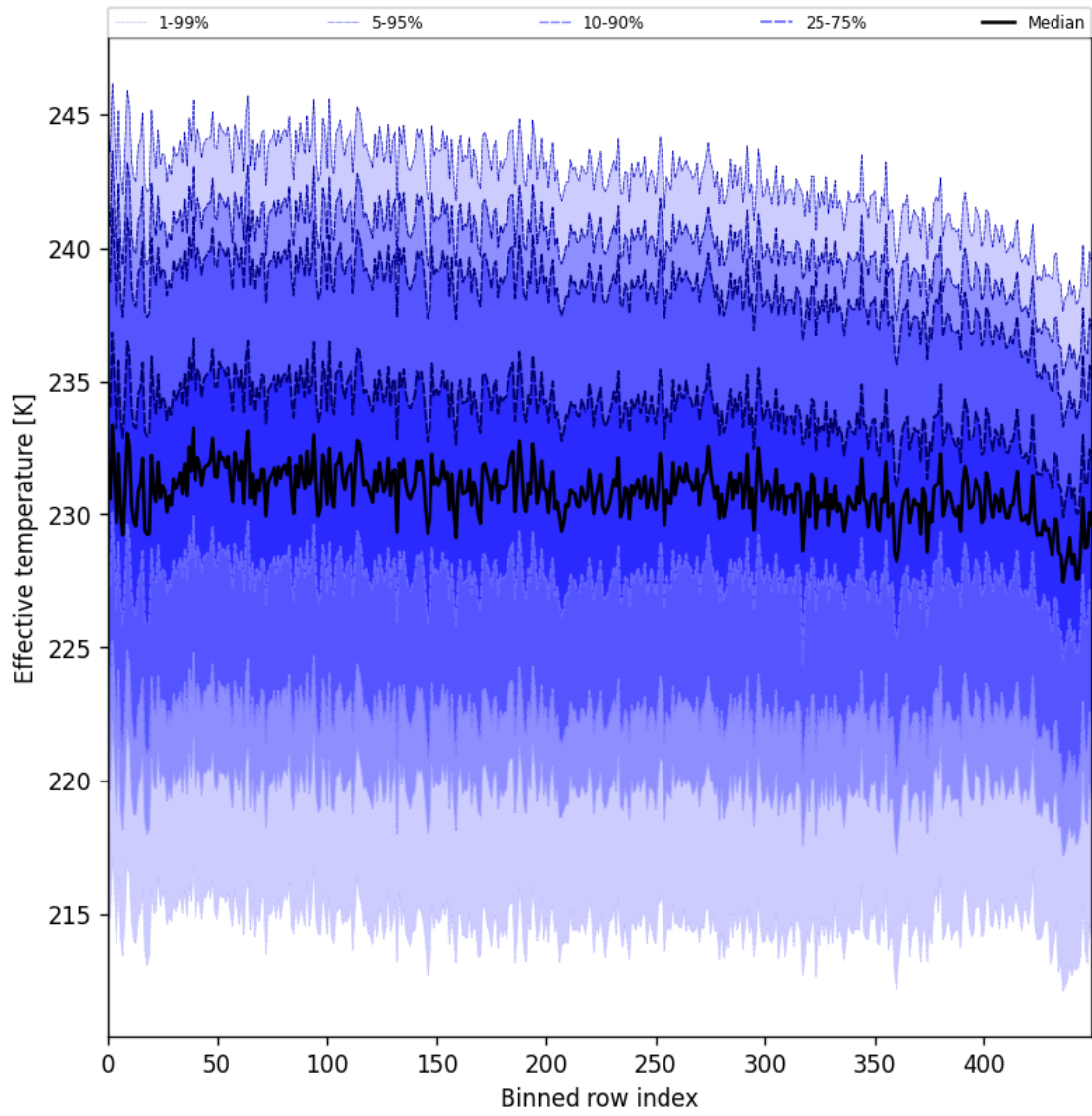
Figure 31: Along track statistics of “Effective temperature” for 2024-10-29 to 2024-10-30
