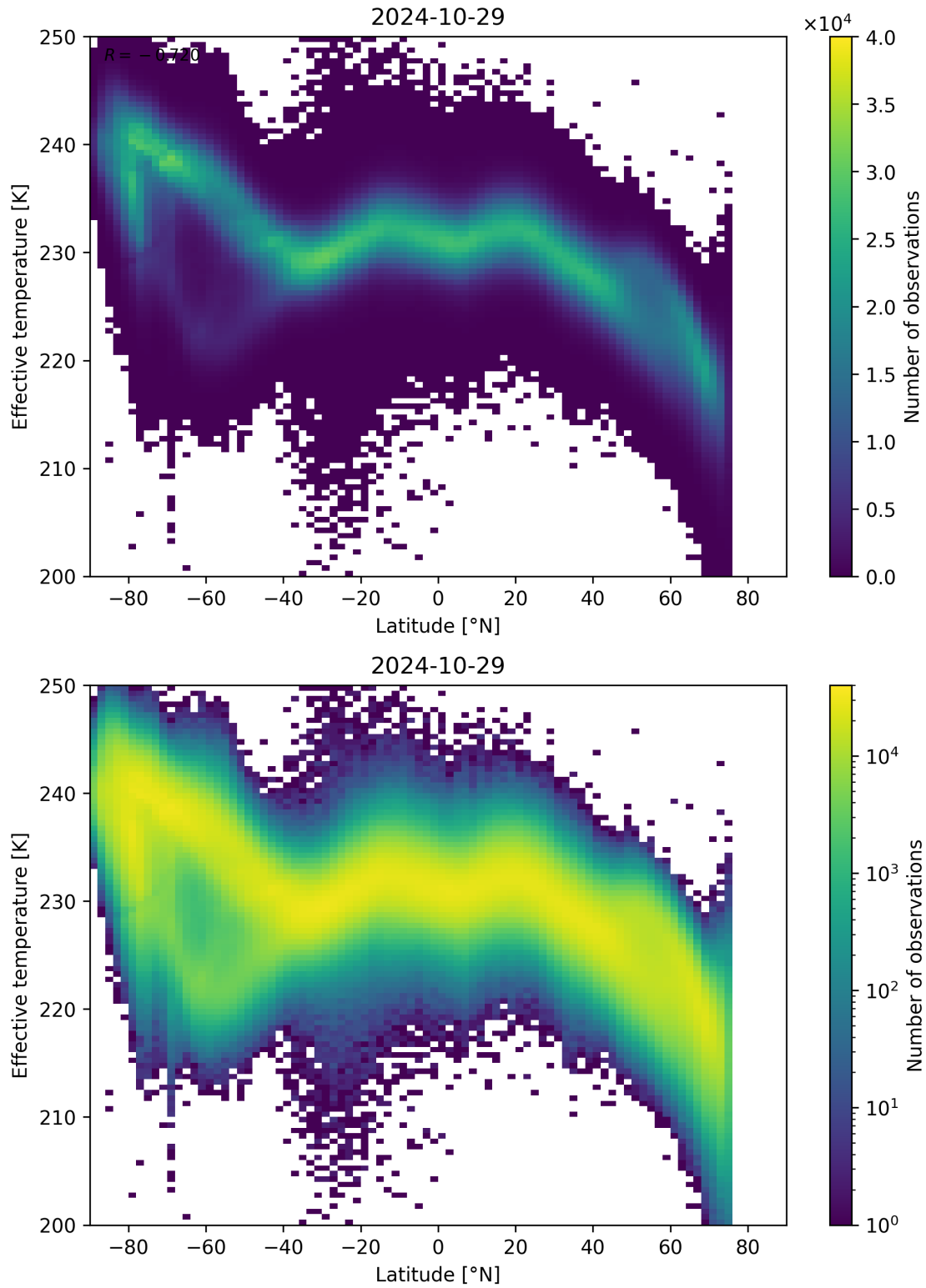
Figure 34: Scatter density plot of “Latitude” against “Effective temperature” for 2024-10-29 to 2024-10-30.
