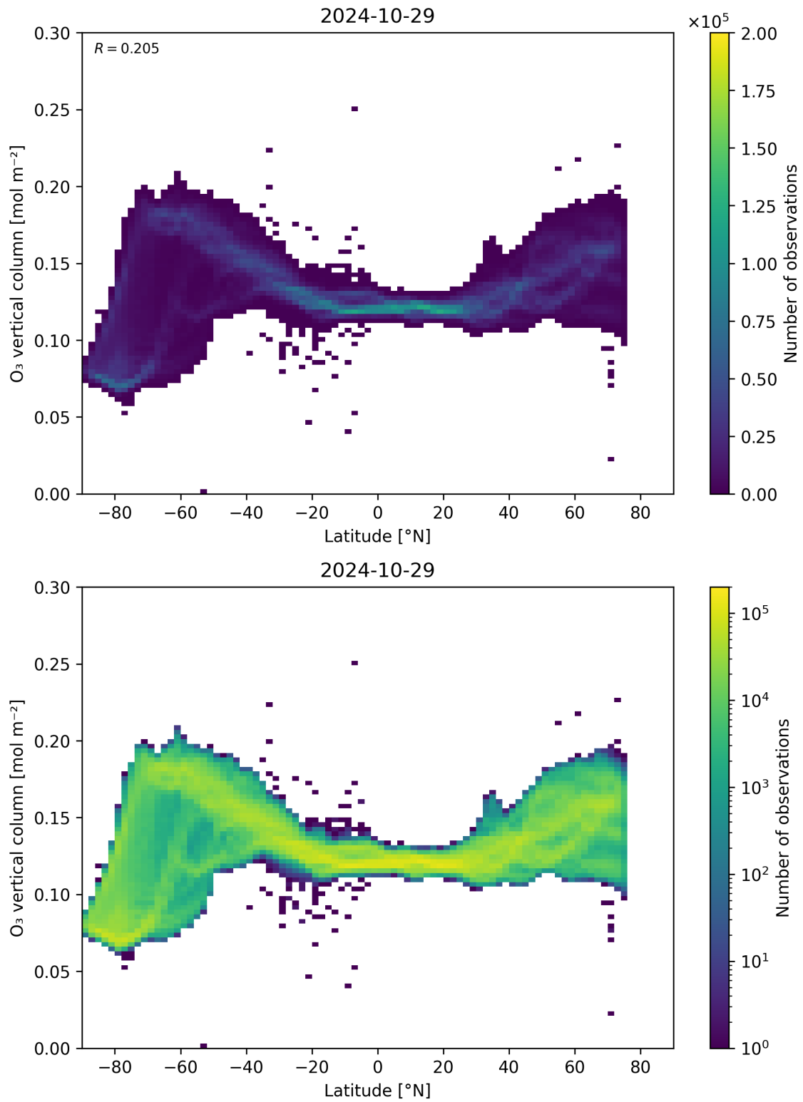
Figure 36: Scatter density plot of “Latitude” against “O 3 vertical column” for 2024-10-29 to 2024-10-30.
