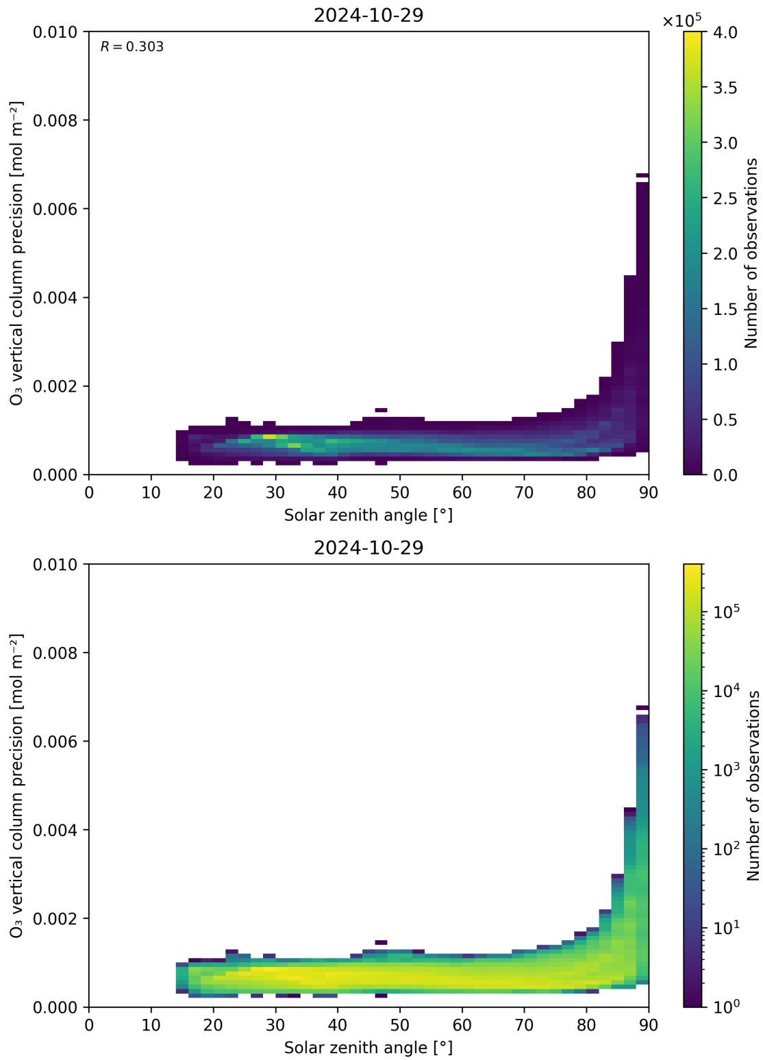
Figure 48: Scatter density plot of “Solar zenith angle” against “O 3 vertical column precision” for 2024-10-29 to 2024-10-30.
