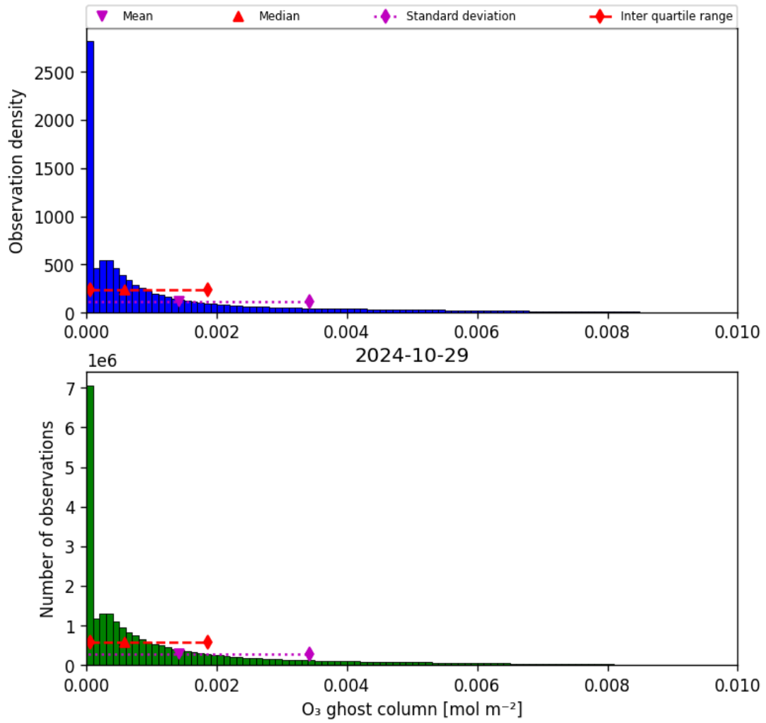
Figure 25: Histogram of “O 3 ghost column” for 2024-10-29 to 2024-10-30
