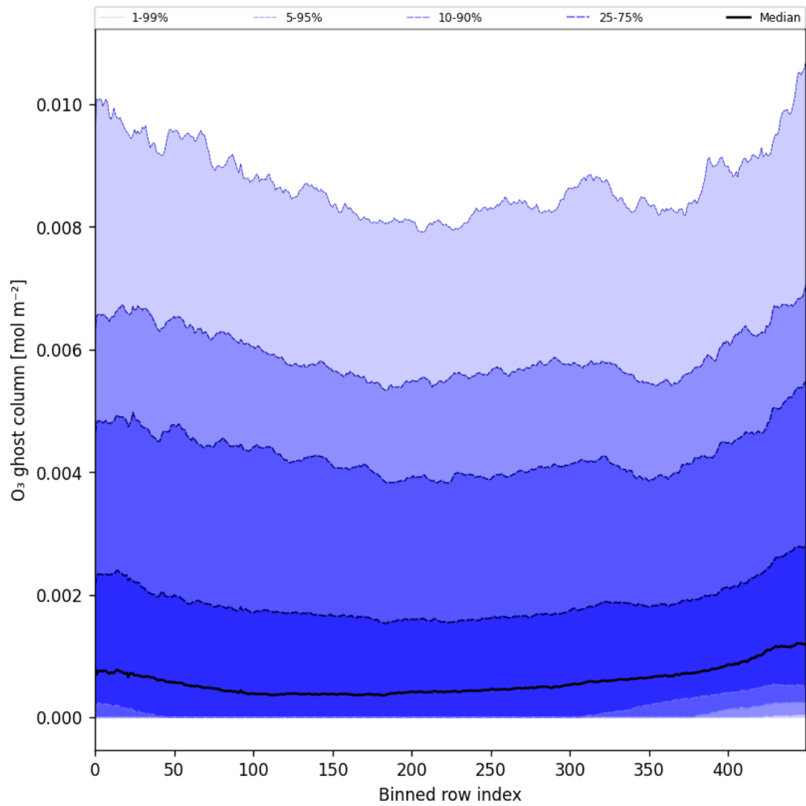
Figure 32: Along track statistics of “O 3 ghost column” for 2024-10-29 to 2024-10-30
