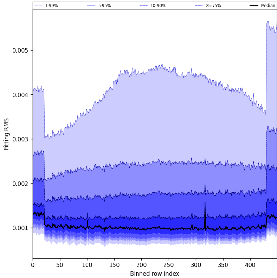
Figure 30: Along track statistics of “Fitting RMS” for 2024-10-29 to 2024-10-30
