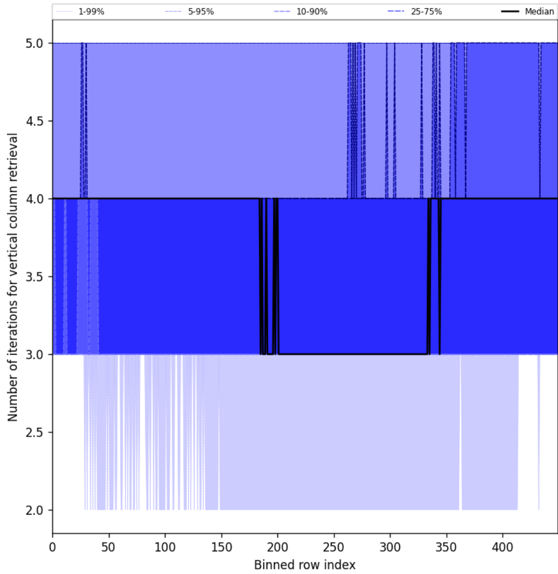
Figure 33: Along track statistics of “Number of iterations for vertical column retrieval” for 2024-10-29 to 2024-10-30
