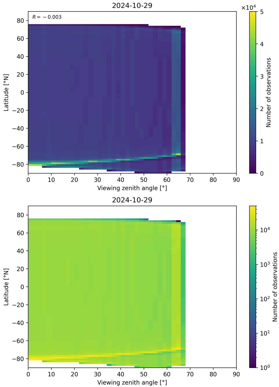
Figure 49: Scatter density plot of “Viewing zenith angle” against “Latitude” for 2024-10-29 to 2024-10-30.
