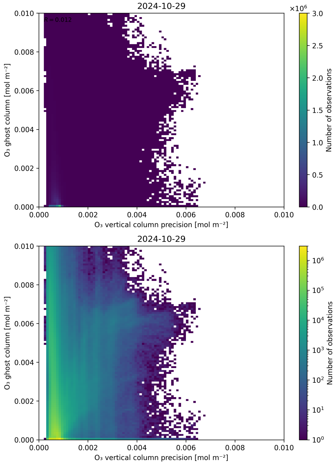
Figure 43: Scatter density plot of “ \text{O}_3 vertical column precision” against “ \text{O}_3 ghost column” for 2024-10-29 to 2024-10-30.
