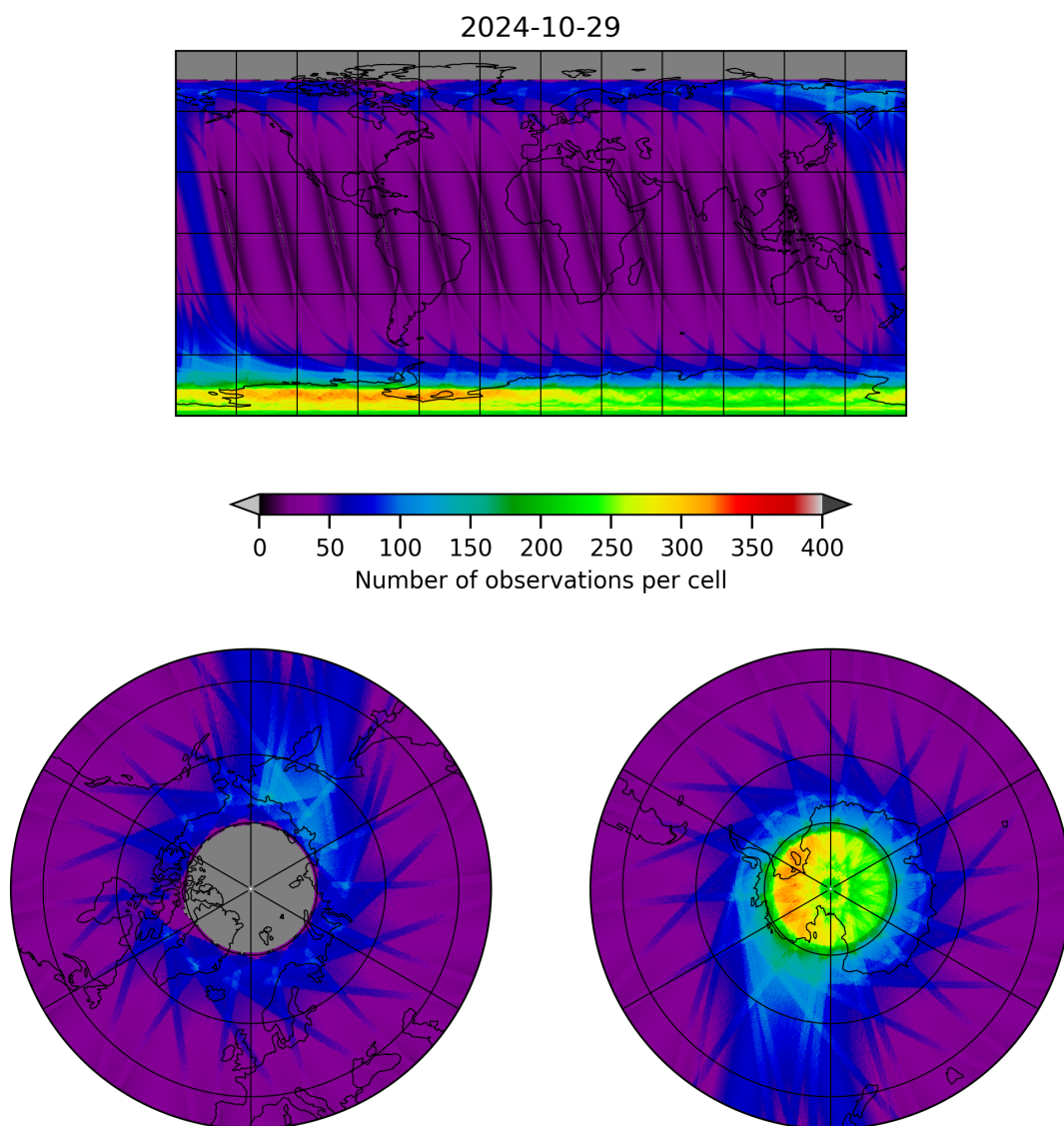
Figure 12: Map of the number of observations for 2024-10-29 to 2024-10-30
