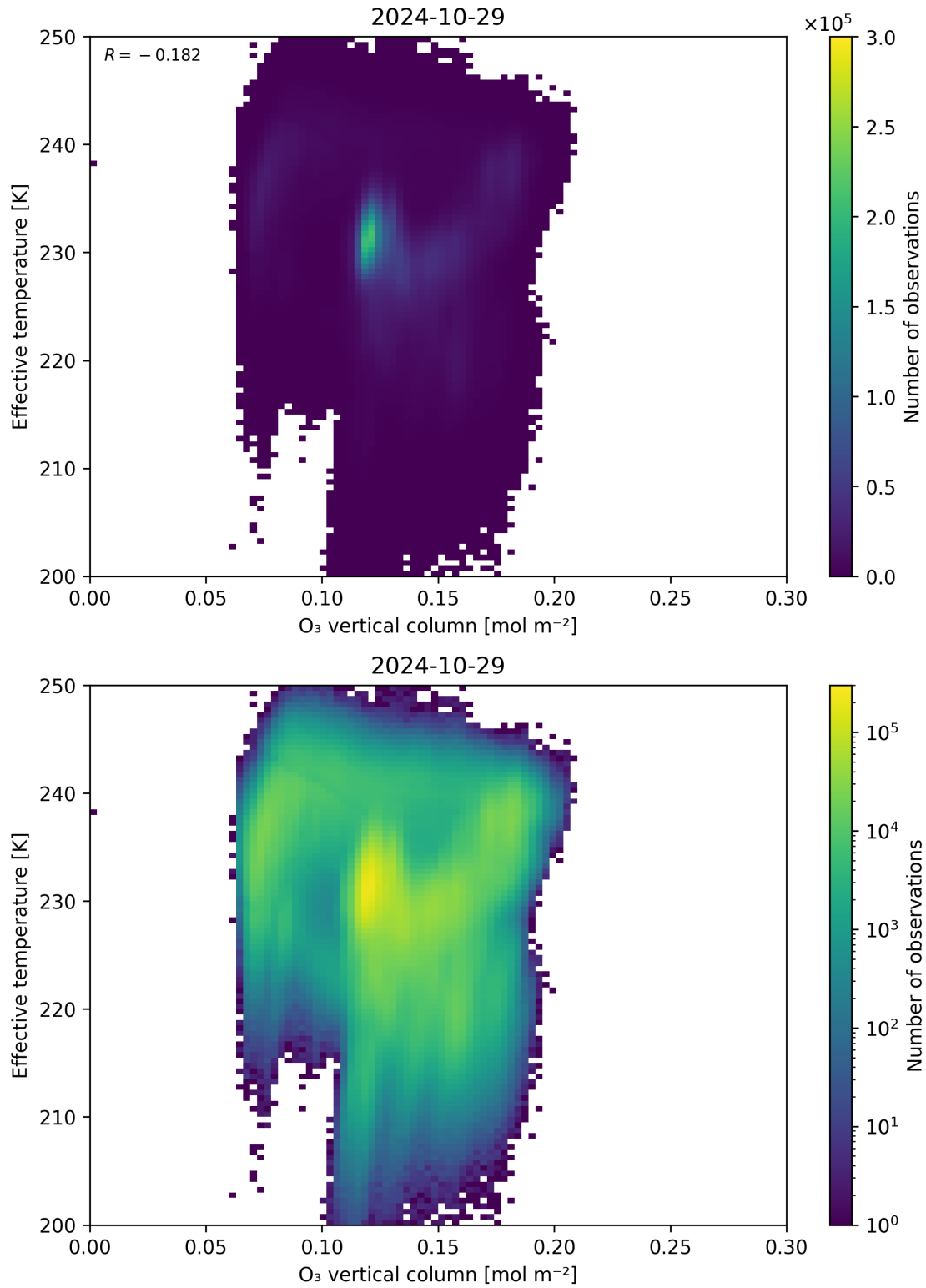
Figure 39: Scatter density plot of “O 3 vertical column” against “Effective temperature” for 2024-10-29 to 2024-10-30.
