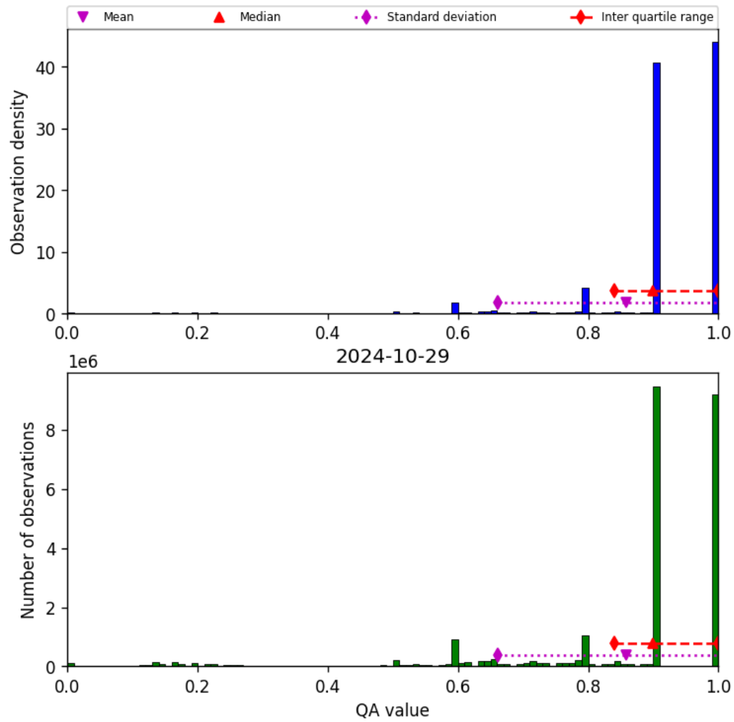
Figure 20: Histogram of “QA value” for 2024-10-29 to 2024-10-30
