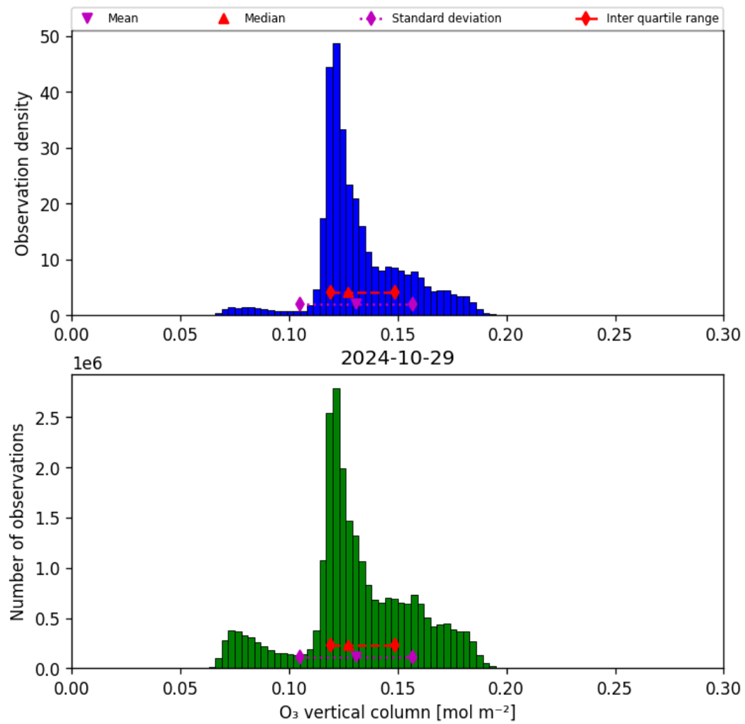
Figure 21: Histogram of “O 3 vertical column” for 2024-10-29 to 2024-10-30
