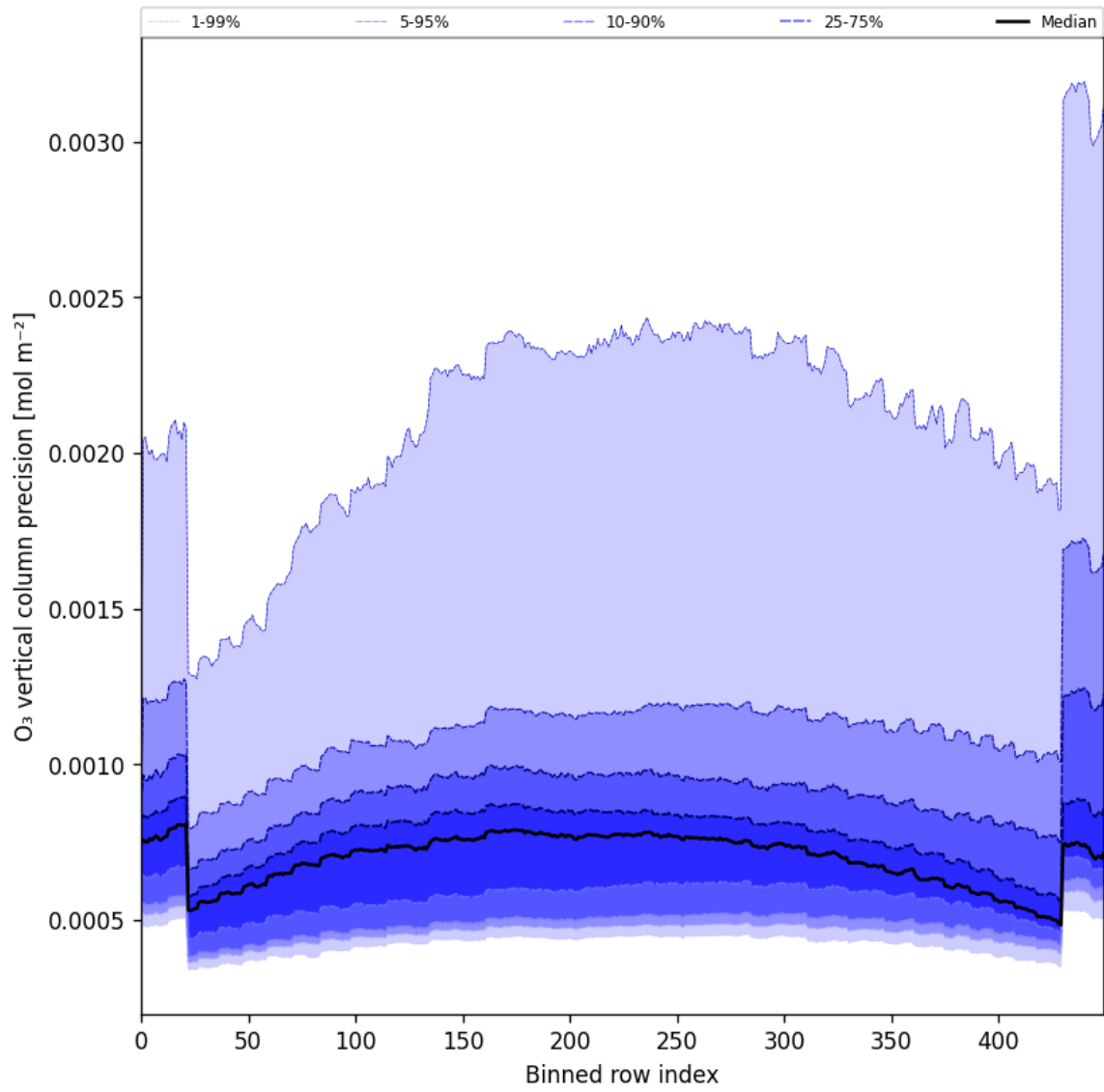
Figure 29: Along track statistics of “O 3 vertical column precision” for 2024-10-29 to 2024-10-30
