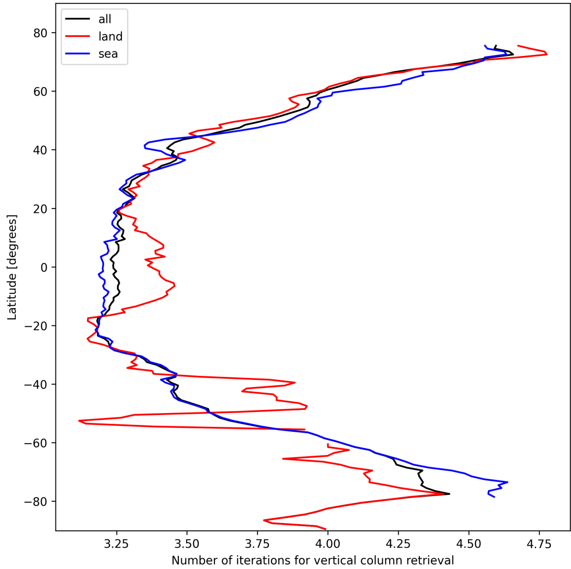
Figure 19: Zonal average of “Number of iterations for vertical column retrieval” for 2024-10-29 to 2024-10-30.
