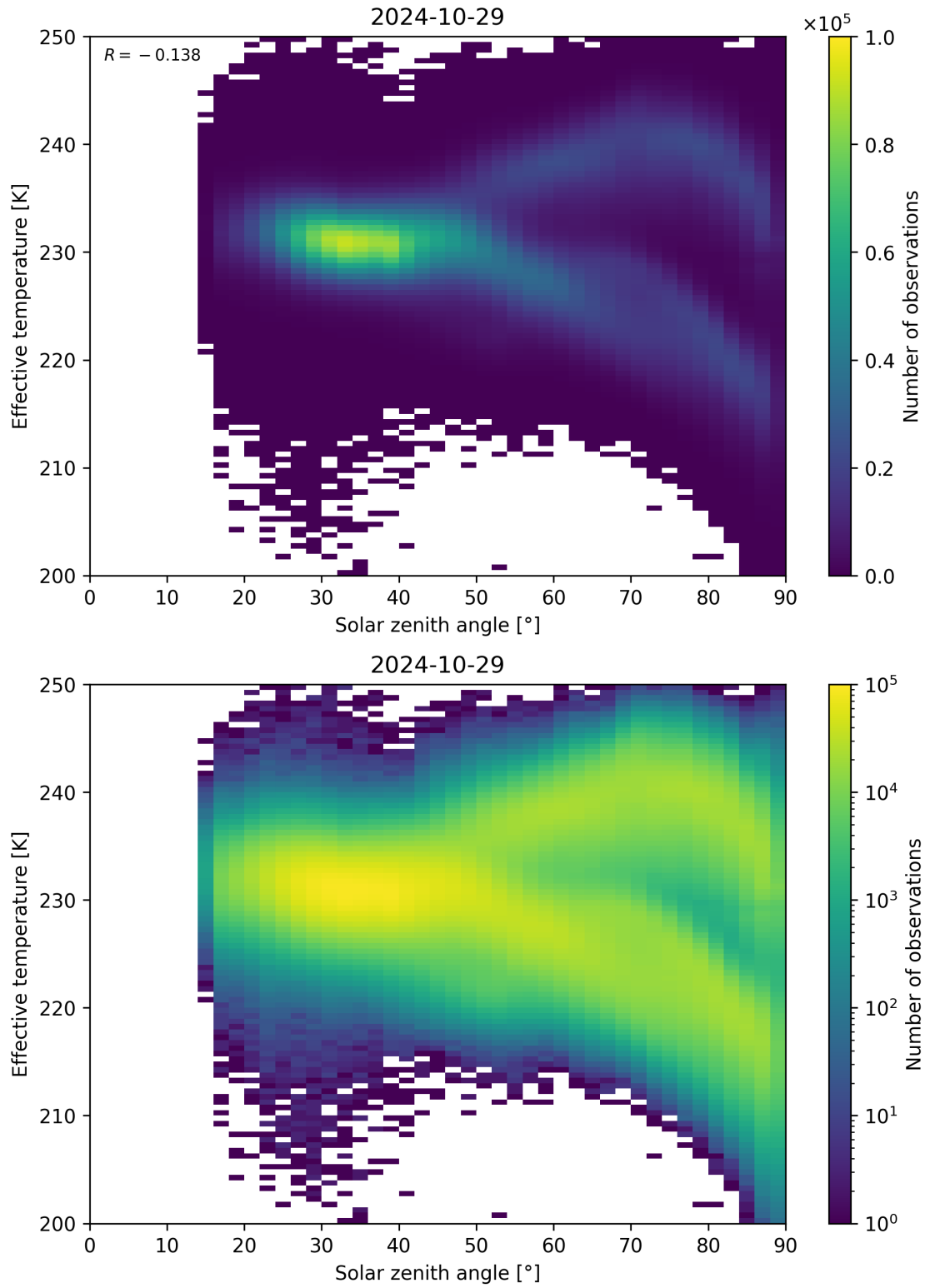
Figure 45: Scatter density plot of “Solar zenith angle” against “Effective temperature” for 2024-10-29 to 2024-10-30.
