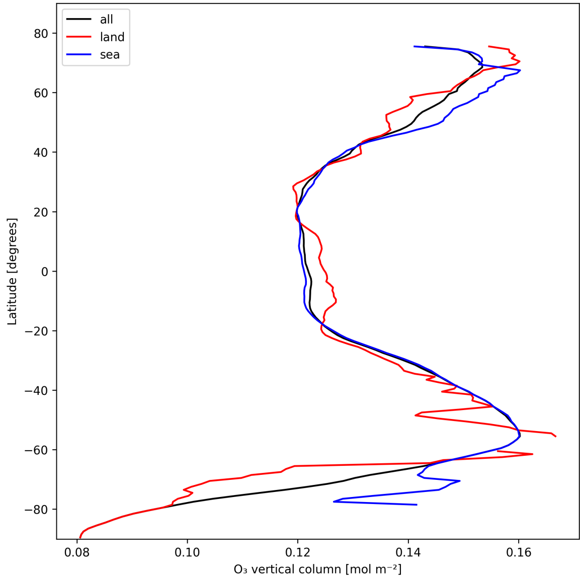
Figure 14: Zonal average of “O 3 vertical column” for 2024-10-29 to 2024-10-30.
