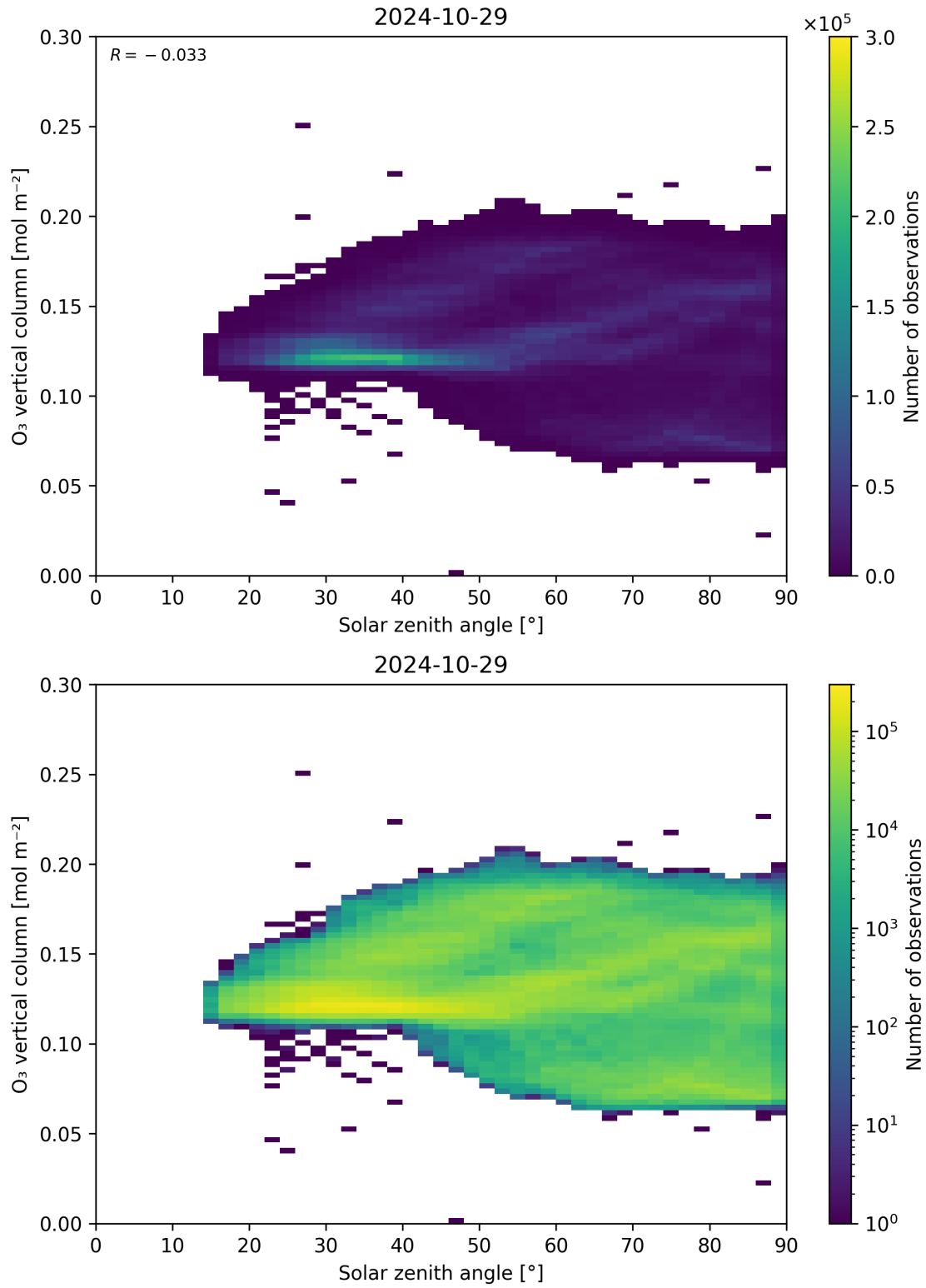
Figure 47: Scatter density plot of “Solar zenith angle” against “O 3 vertical column” for 2024-10-29 to 2024-10-30.
