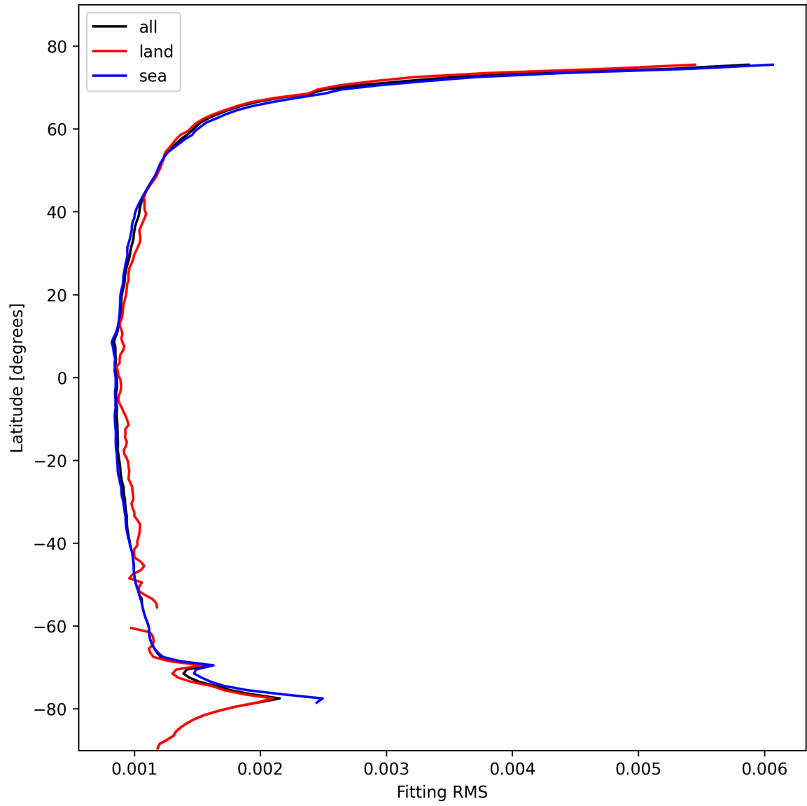
Figure 16: Zonal average of “Fitting RMS” for 2024-10-29 to 2024-10-30.
