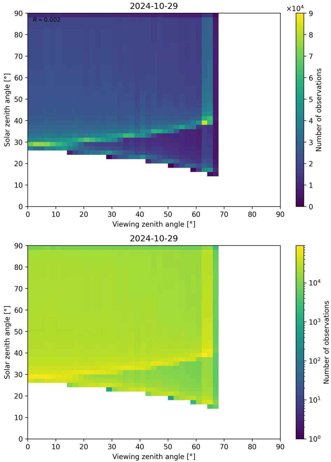
Figure 54: Scatter density plot of “Viewing zenith angle” against “Solar zenith angle” for 2024-10-29 to 2024-10-30.
