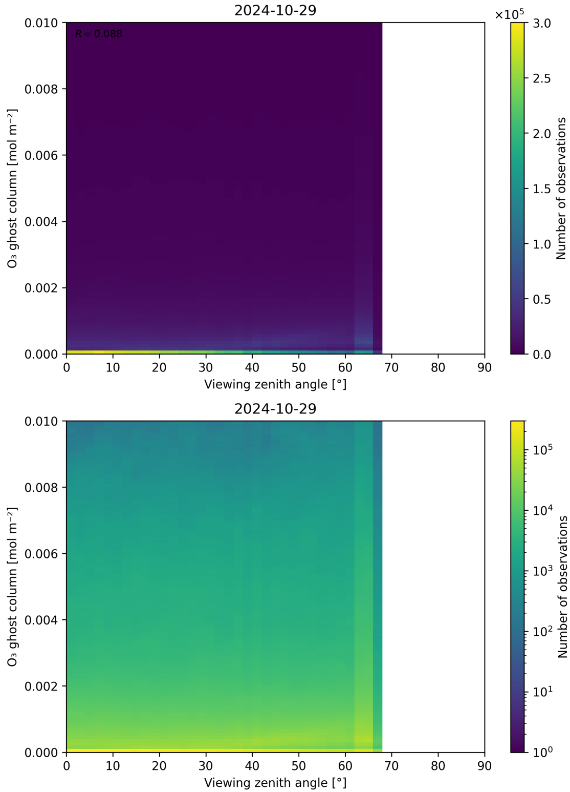
Figure 51: Scatter density plot of “Viewing zenith angle” against “O 3 ghost column” for 2024-10-29 to 2024-10-30.
