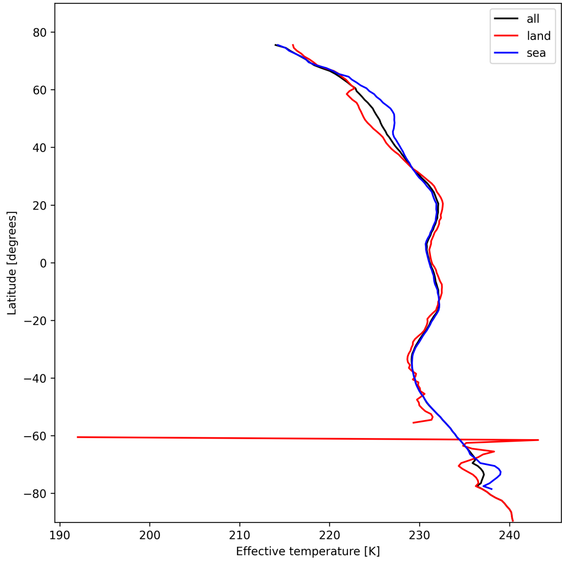
Figure 17: Zonal average of “Effective temperature” for 2024-10-29 to 2024-10-30.
