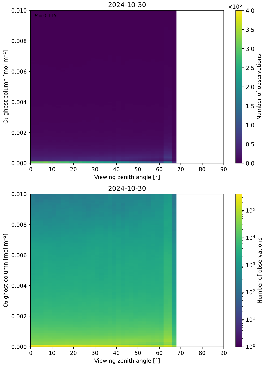
Figure 51: Scatter density plot of “Viewing zenith angle” against “O 3 ghost column” for 2024-10-30 to 2024-10-31.
