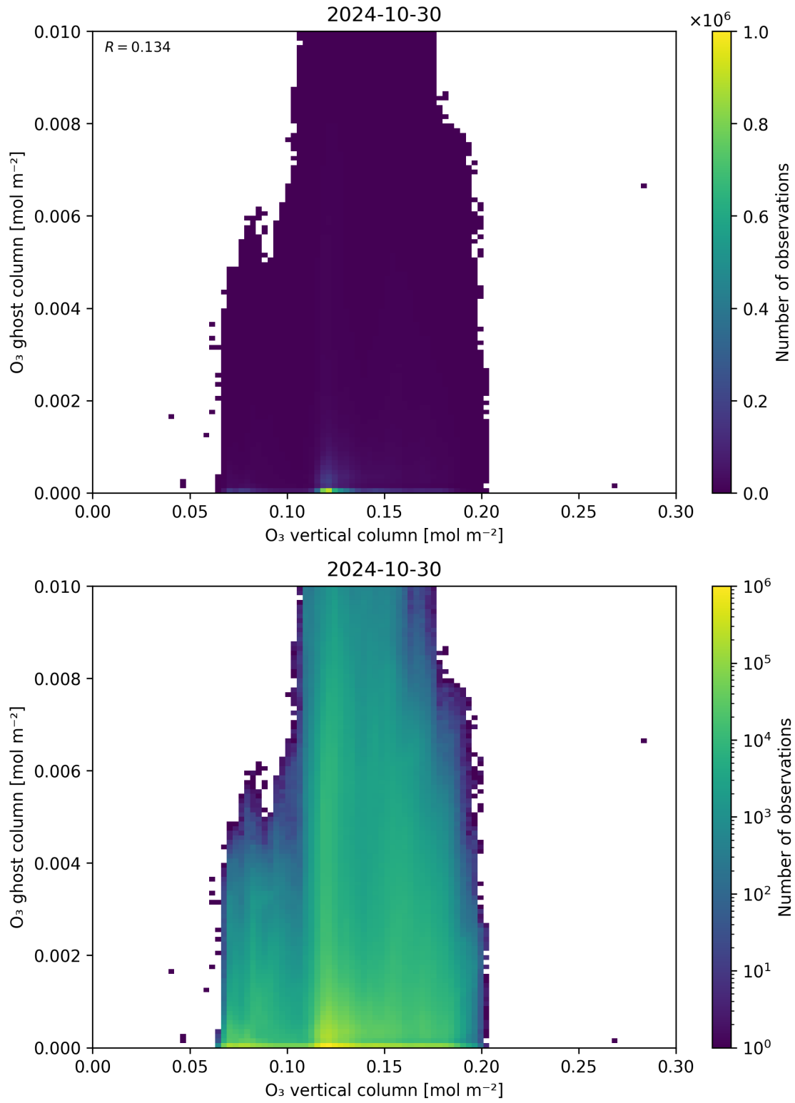
Figure 40: Scatter density plot of “O 3 vertical column” against “O 3 ghost column” for 2024-10-30 to 2024-10-31.
