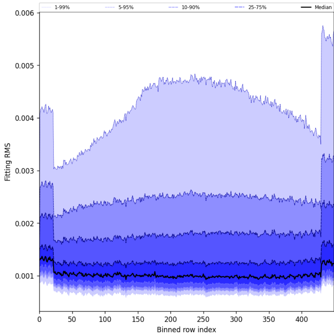
Figure 30: Along track statistics of “Fitting RMS” for 2024-10-30 to 2024-10-31
