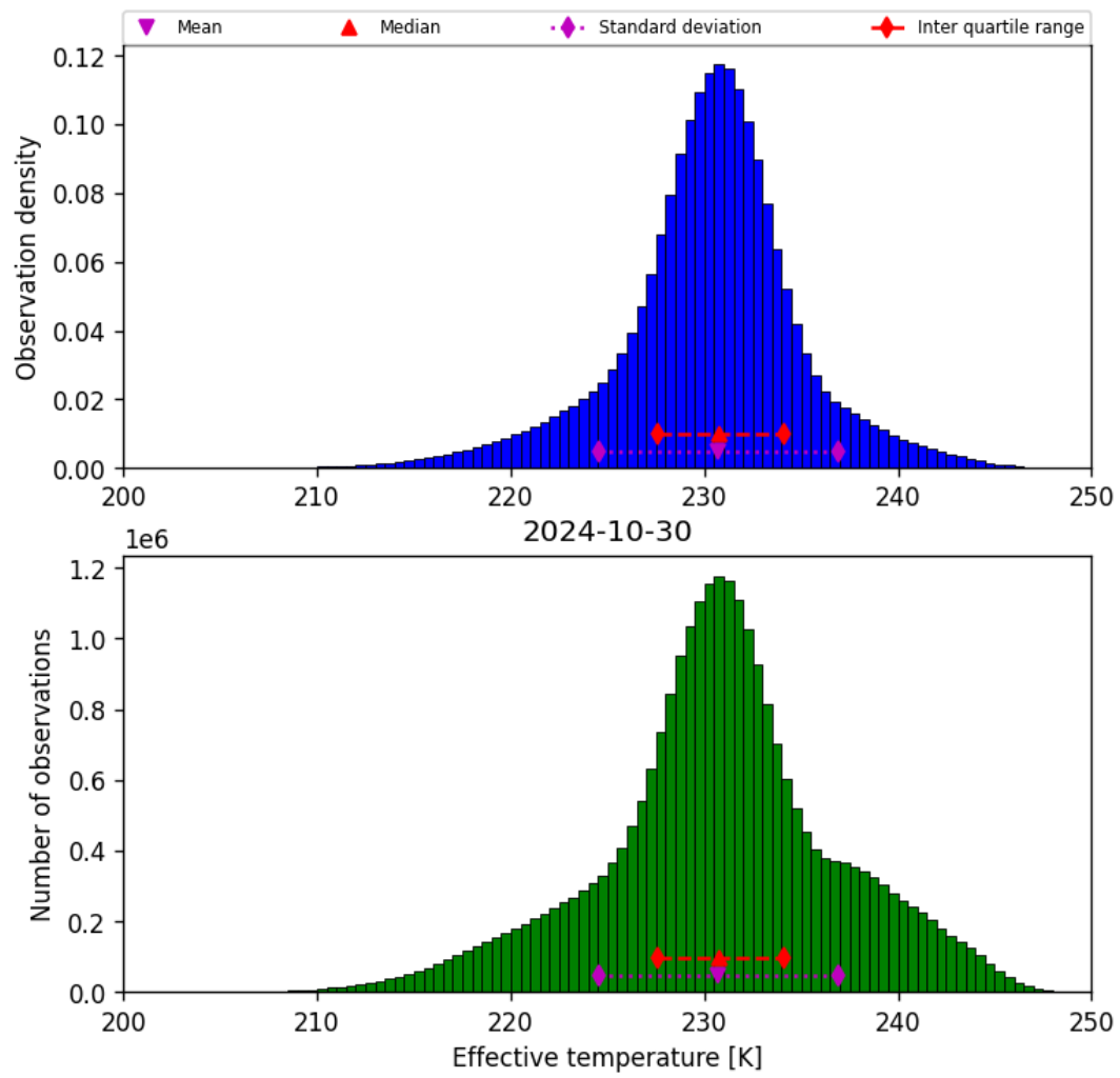
Figure 24: Histogram of “Effective temperature” for 2024-10-30 to 2024-10-31
