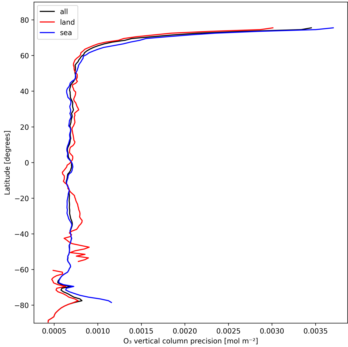
Figure 15: Zonal average of "O 3 vertical column precision" for 2024-10-30 to 2024-10-31.
