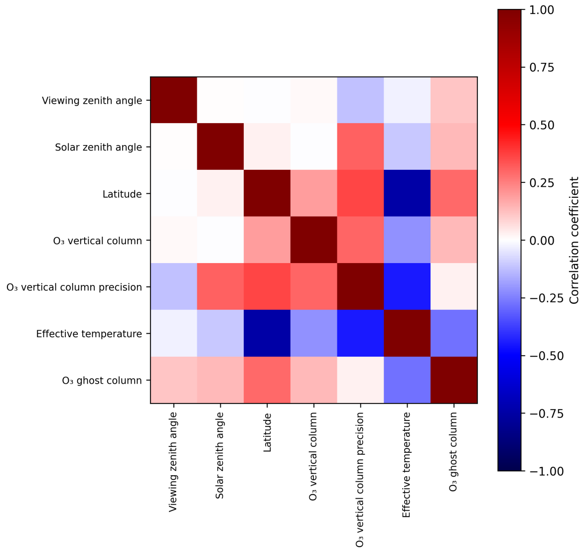
Figure 2: Map of correlation matrix for 2024-10-30 to 2024-10-31.
