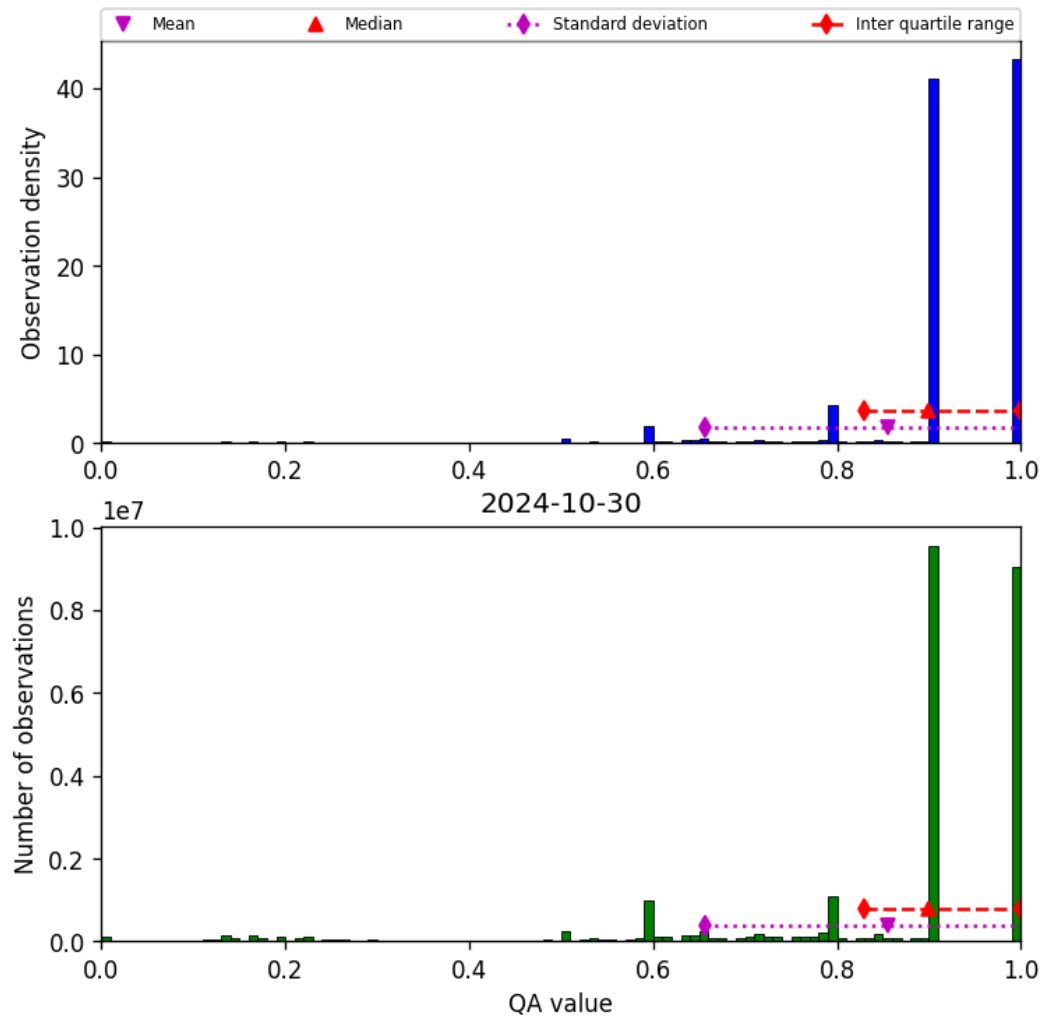
Figure 20: Histogram of “QA value” for 2024-10-30 to 2024-10-31
