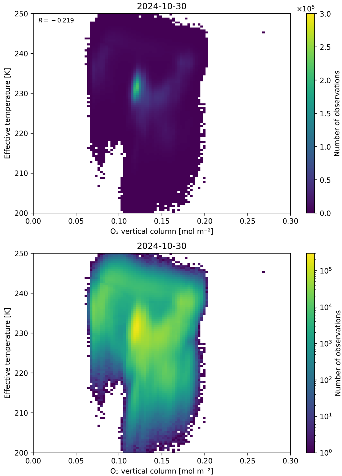
Figure 39: Scatter density plot of “O 3 vertical column” against “Effective temperature” for 2024-10-30 to 2024-10-31.
