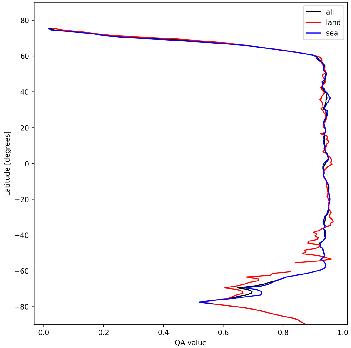
Figure 13: Zonal average of “QA value” for 2024-10-30 to 2024-10-31.
