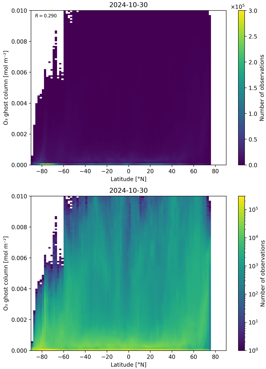
Figure 35: Scatter density plot of “Latitude” against “O 3 ghost column” for 2024-10-30 to 2024-10-31.
