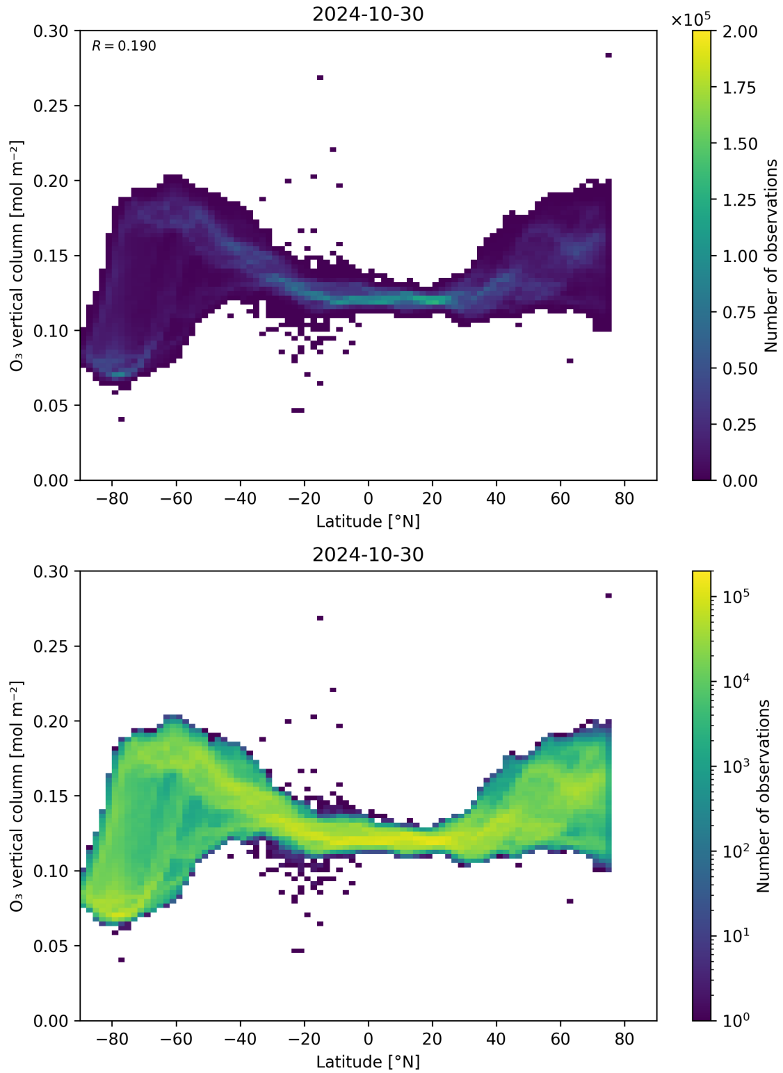
Figure 36: Scatter density plot of “Latitude” against “O 3 vertical column” for 2024-10-30 to 2024-10-31.
