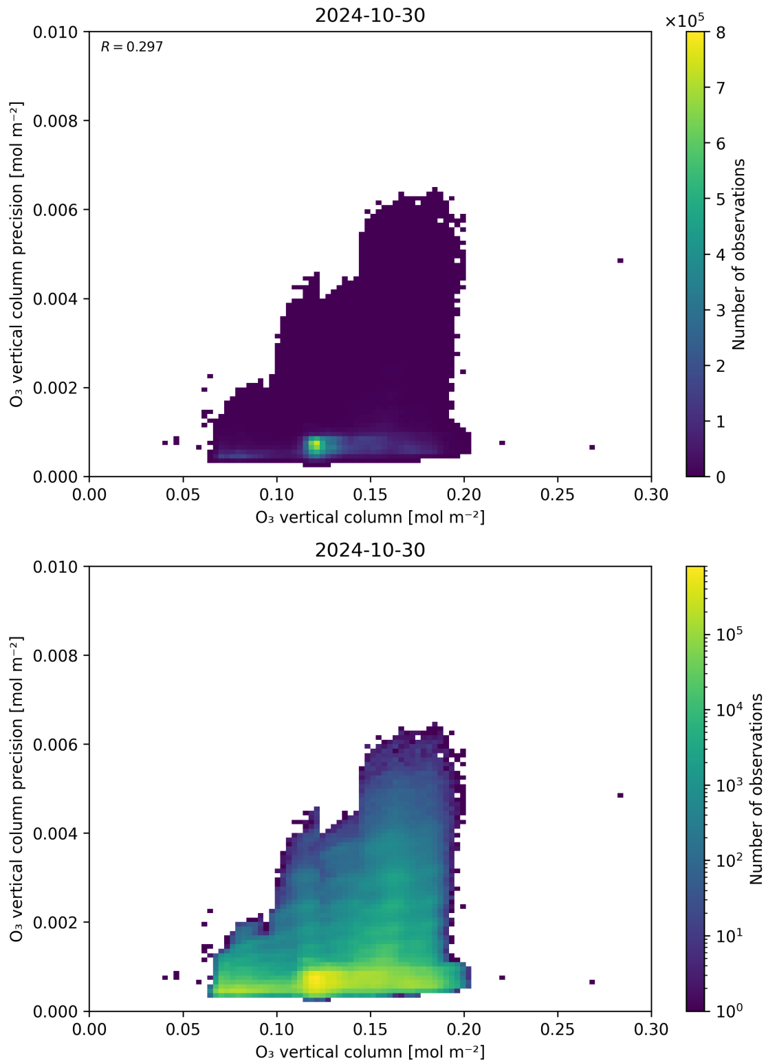
Figure 41: Scatter density plot of “O 3 vertical column” against “O 3 vertical column precision” for 2024-10-30 to 2024-10-31.
