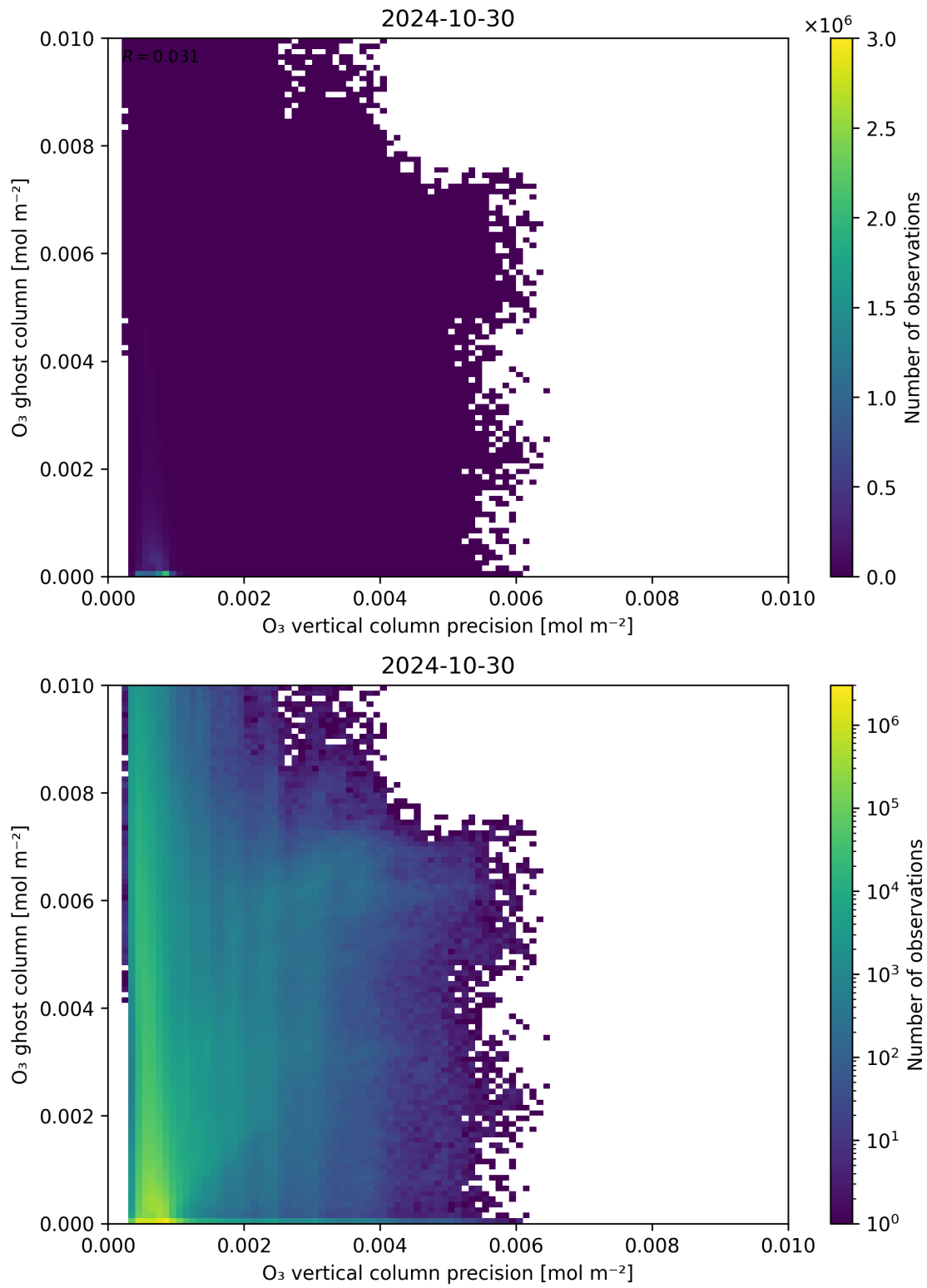
Figure 43: Scatter density plot of “ O_3 vertical column precision” against “ O_3 ghost column” for 2024-10-30 to 2024-10-31.
