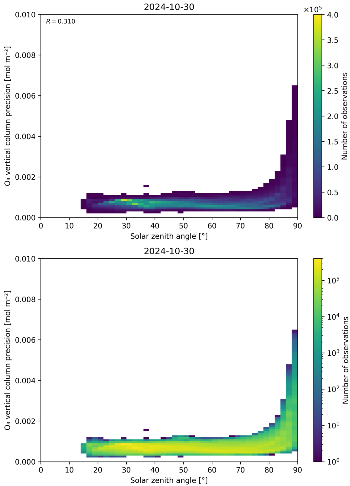
Figure 48: Scatter density plot of “Solar zenith angle” against “O 3 vertical column precision” for 2024-10-30 to 2024-10-31.
