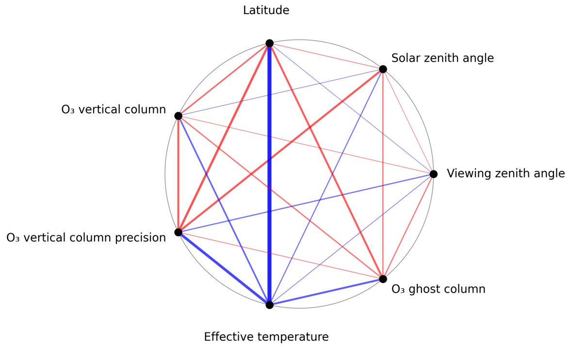
Figure 1: Map of correlation graph for 2024-10-30 to 2024-10-31.
