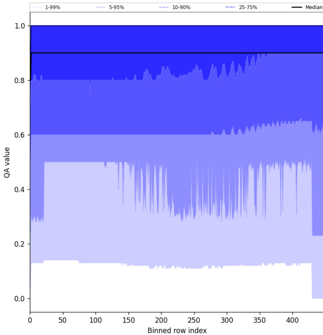
Figure 27: Along track statistics of “QA value” for 2024-10-30 to 2024-10-31
