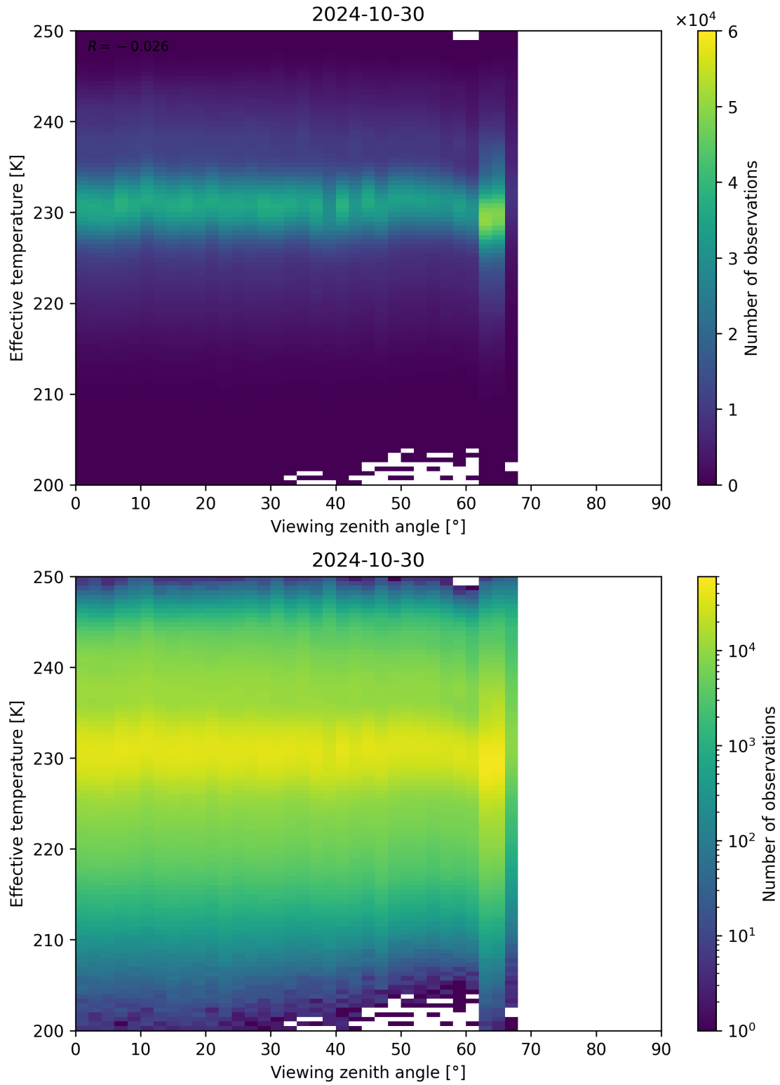
Figure 50: Scatter density plot of “Viewing zenith angle” against “Effective temperature” for 2024-10-30 to 2024-10-31.
