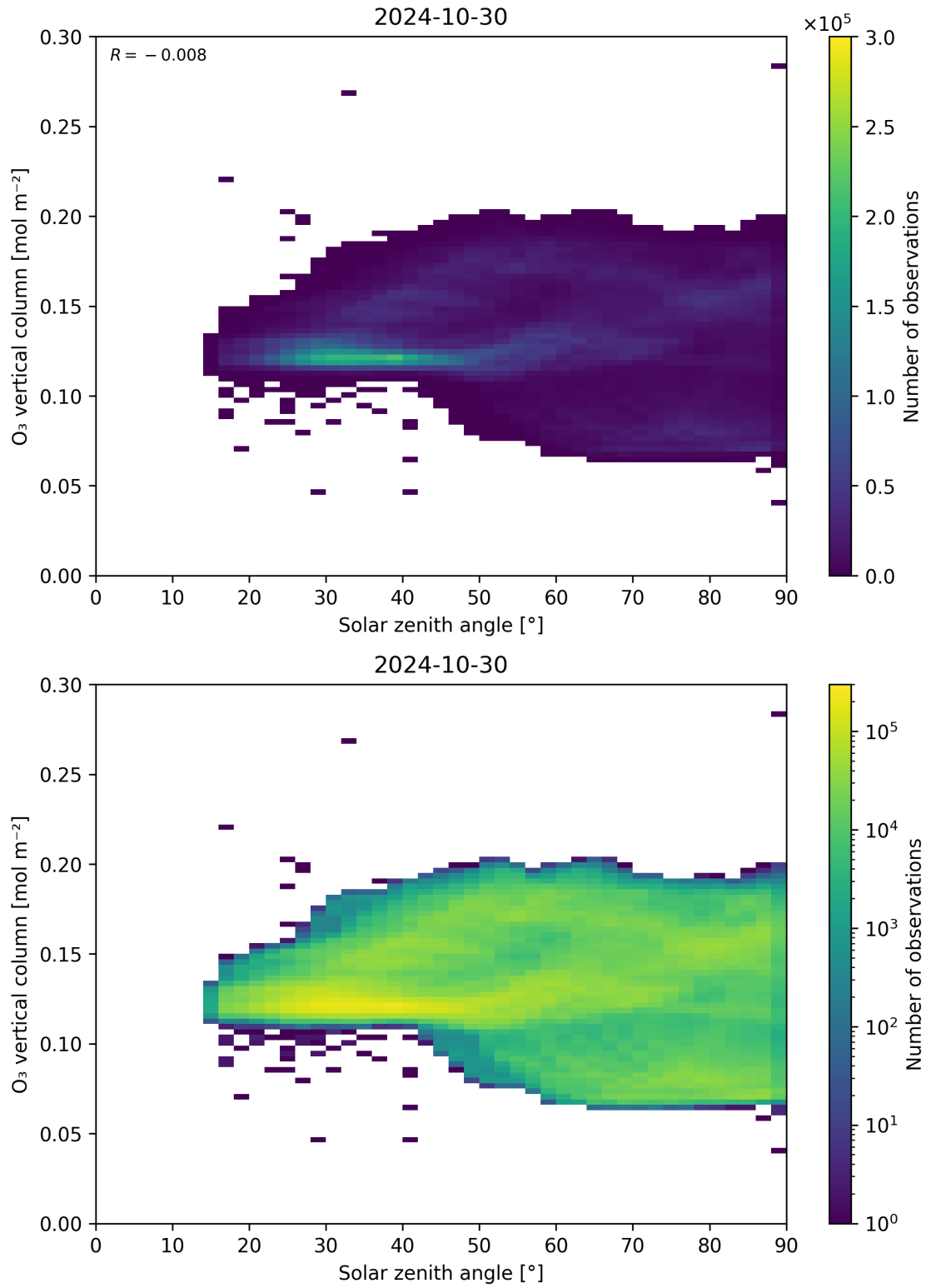
Figure 47: Scatter density plot of “Solar zenith angle” against “O 3 vertical column” for 2024-10-30 to 2024-10-31.
