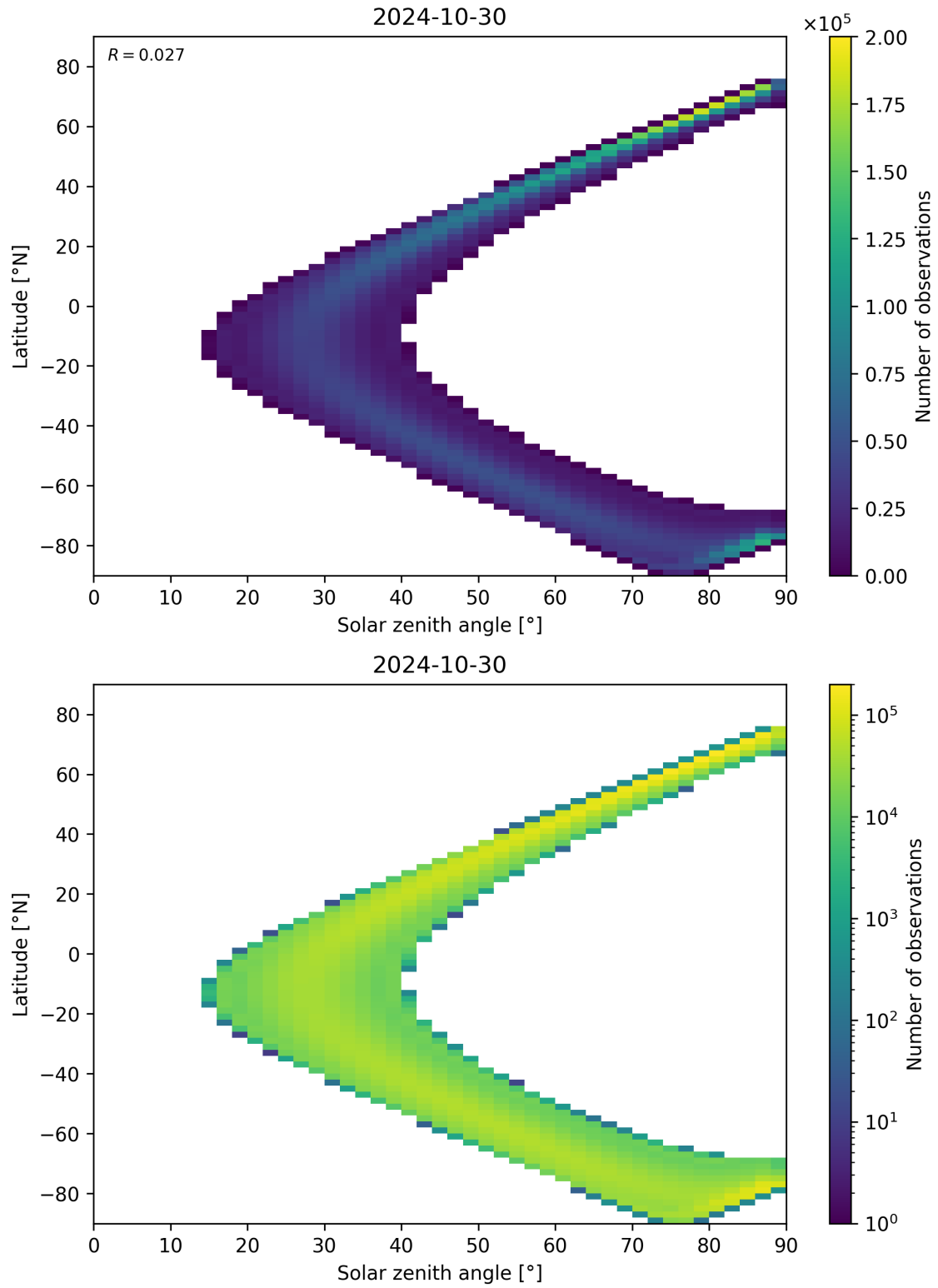
Figure 44: Scatter density plot of “Solar zenith angle” against “Latitude” for 2024-10-30 to 2024-10-31.
