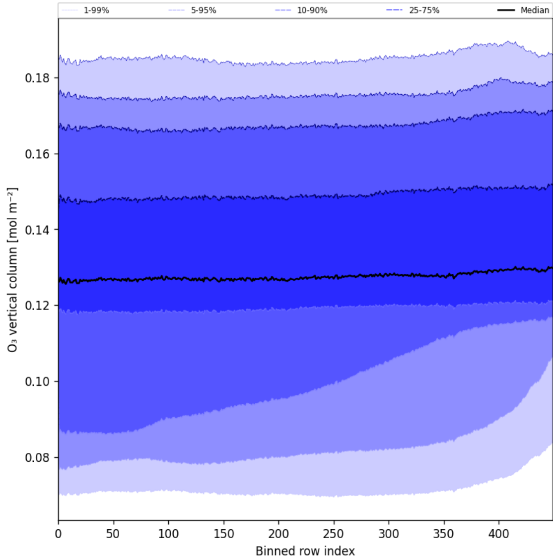
Figure 28: Along track statistics of “O 3 vertical column” for 2024-10-30 to 2024-10-31
