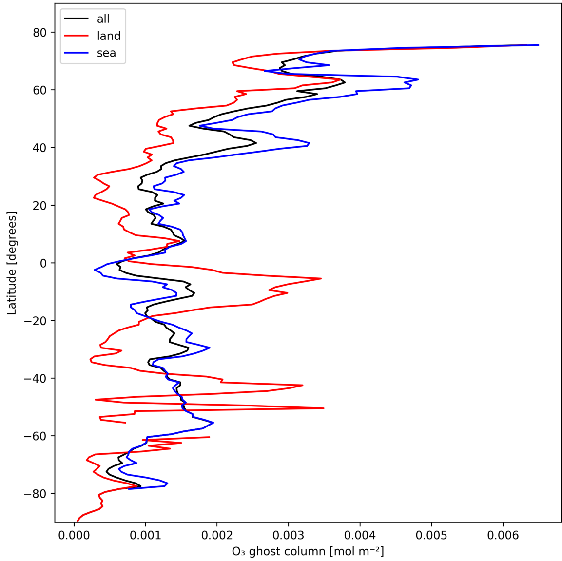
Figure 18: Zonal average of "O 3 ghost column" for 2024-10-30 to 2024-10-31.
