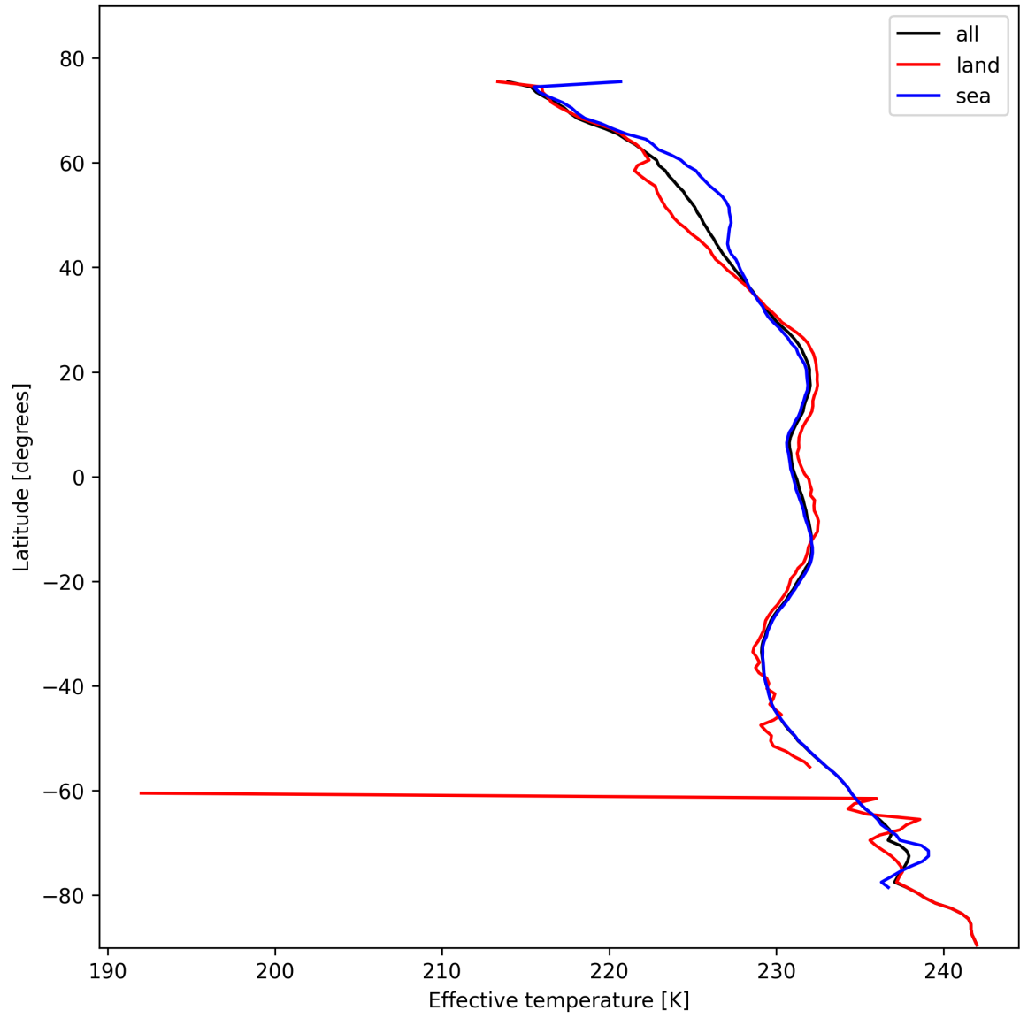
Figure 17: Zonal average of “Effective temperature” for 2024-10-30 to 2024-10-31.
