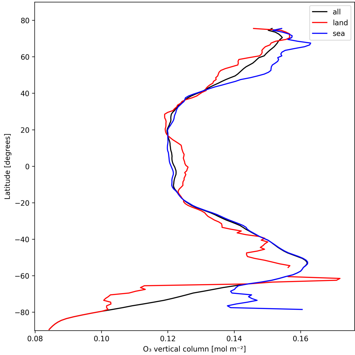
Figure 14: Zonal average of “O 3 vertical column” for 2024-10-30 to 2024-10-31.
