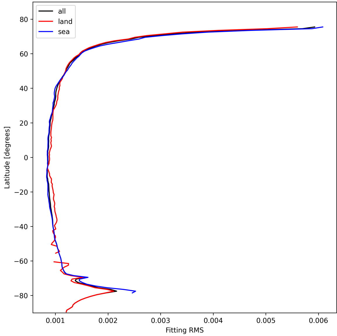
Figure 16: Zonal average of “Fitting RMS” for 2024-10-30 to 2024-10-31.
