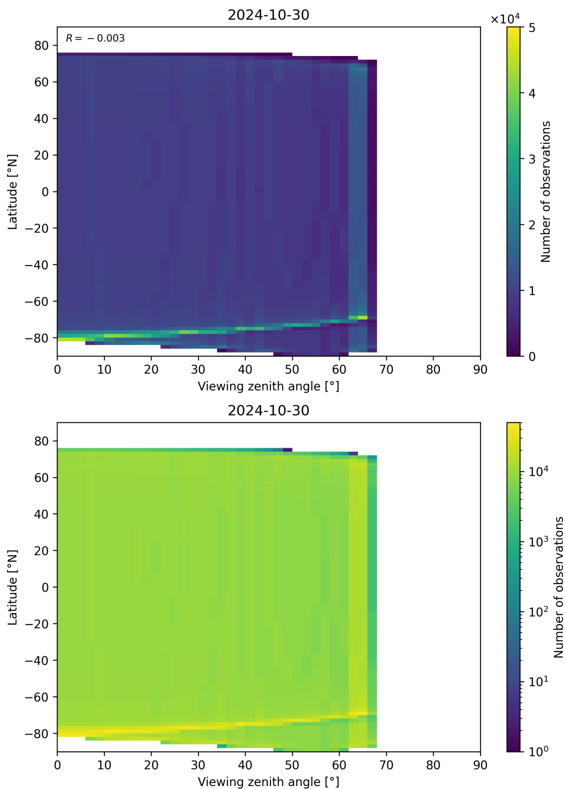
Figure 49: Scatter density plot of “Viewing zenith angle” against “Latitude” for 2024-10-30 to 2024-10-31.
