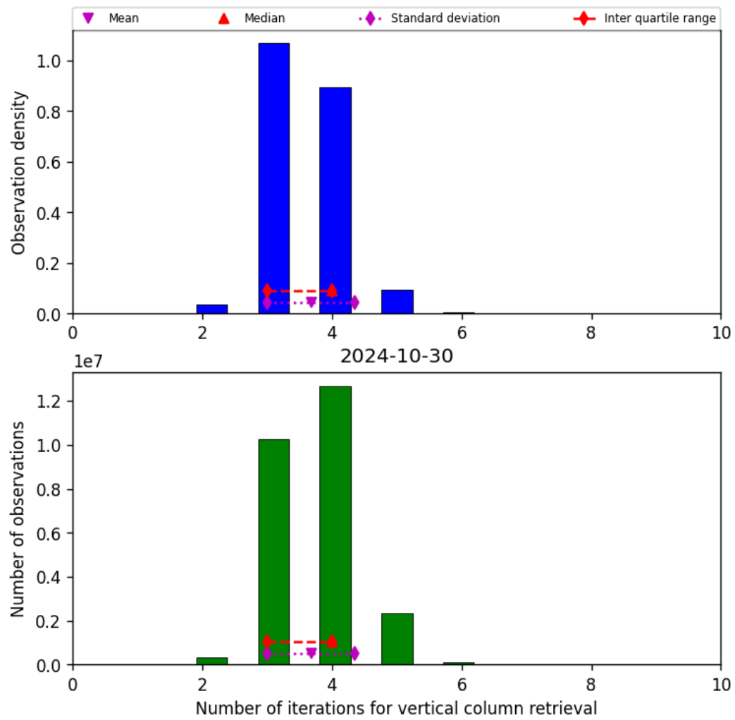
Figure 26: Histogram of "Number of iterations for vertical column retrieval" for 2024-10-30 to 2024-10-31
