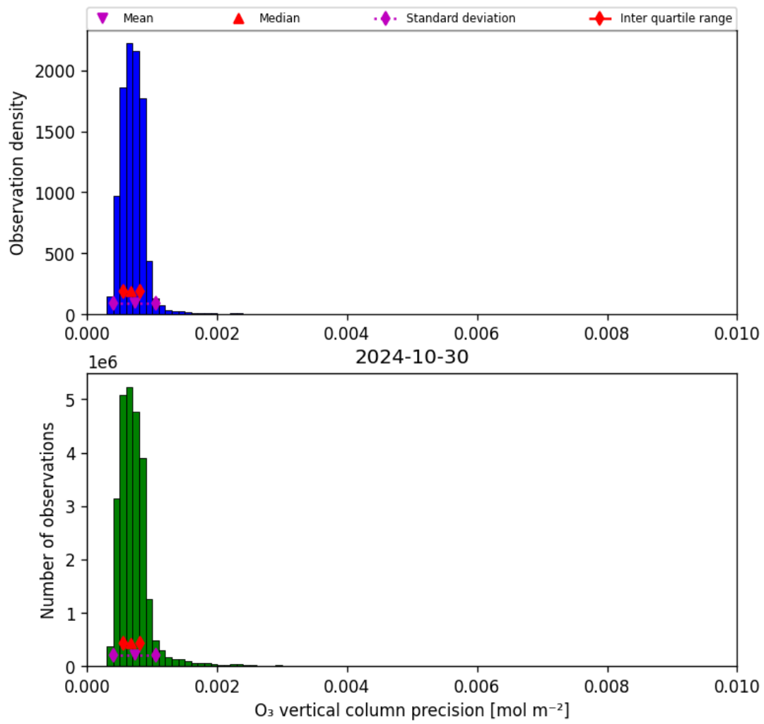
Figure 22: Histogram of “O 3 vertical column precision” for 2024-10-30 to 2024-10-31
