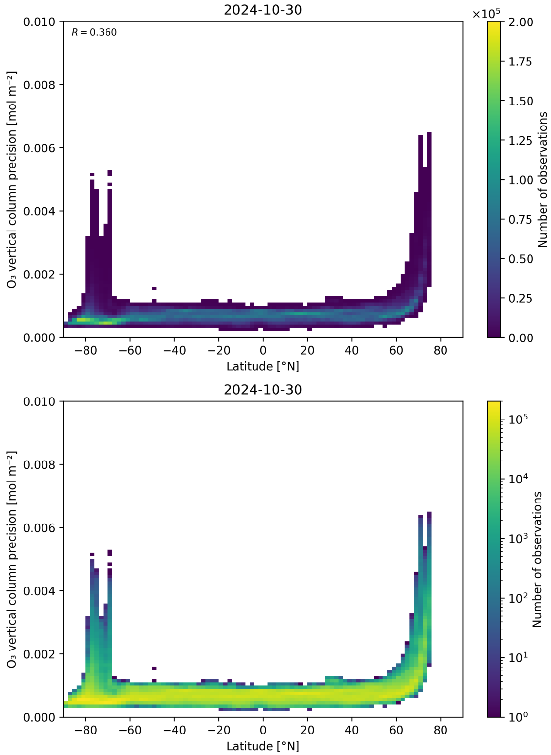
Figure 37: Scatter density plot of “Latitude” against “O 3 vertical column precision” for 2024-10-30 to 2024-10-31.
