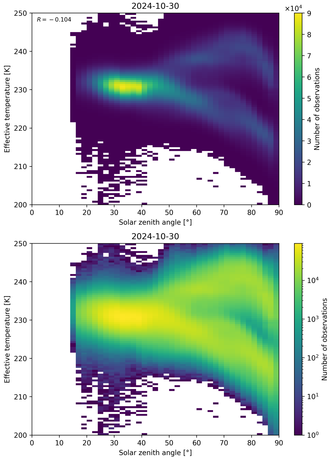
Figure 45: Scatter density plot of “Solar zenith angle” against “Effective temperature” for 2024-10-30 to 2024-10-31.
