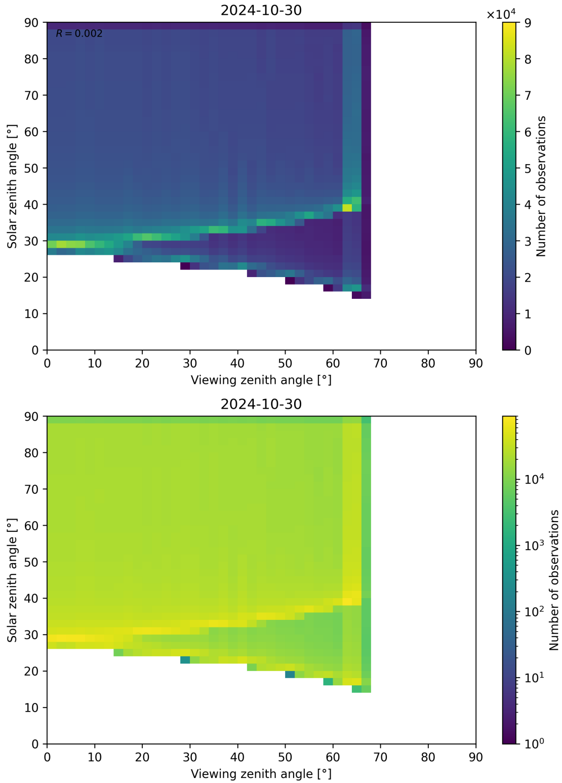
Figure 54: Scatter density plot of “Viewing zenith angle” against “Solar zenith angle” for 2024-10-30 to 2024-10-31.
