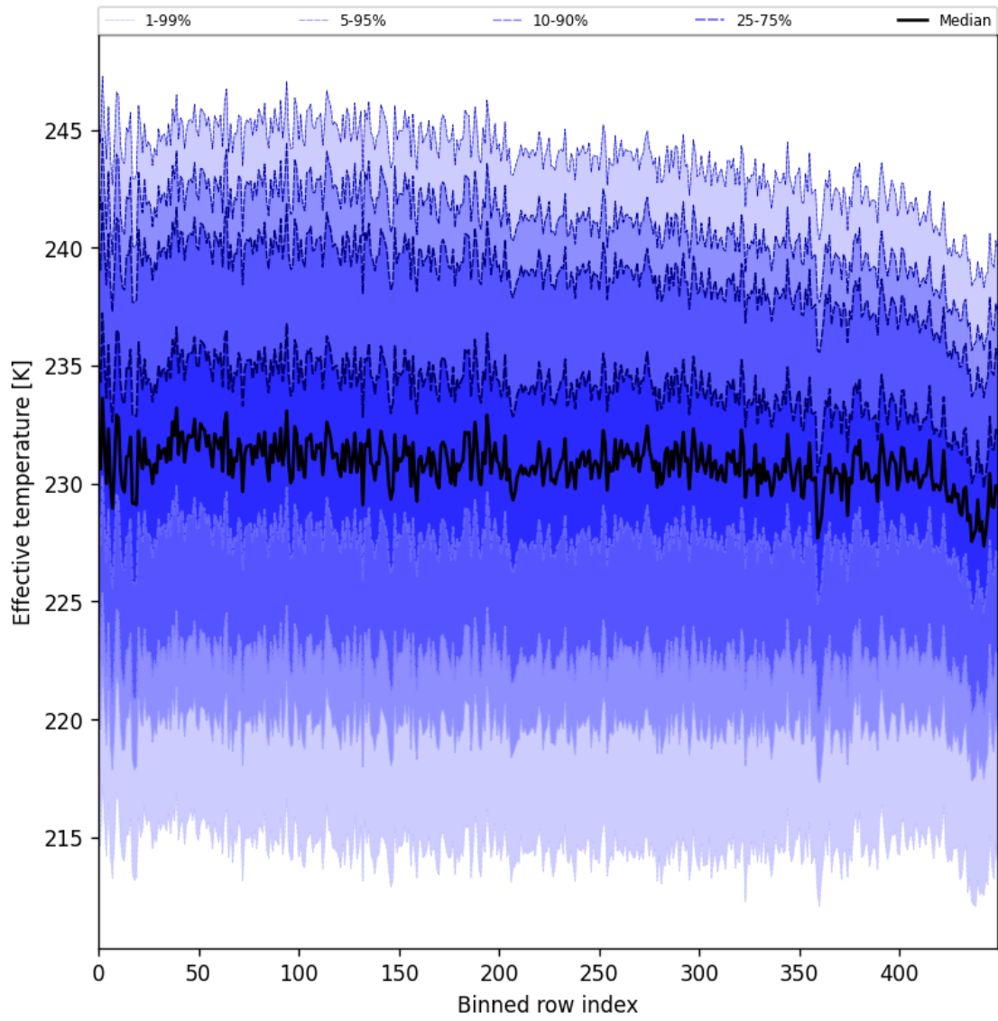
Figure 31: Along track statistics of “Effective temperature” for 2024-10-30 to 2024-10-31
