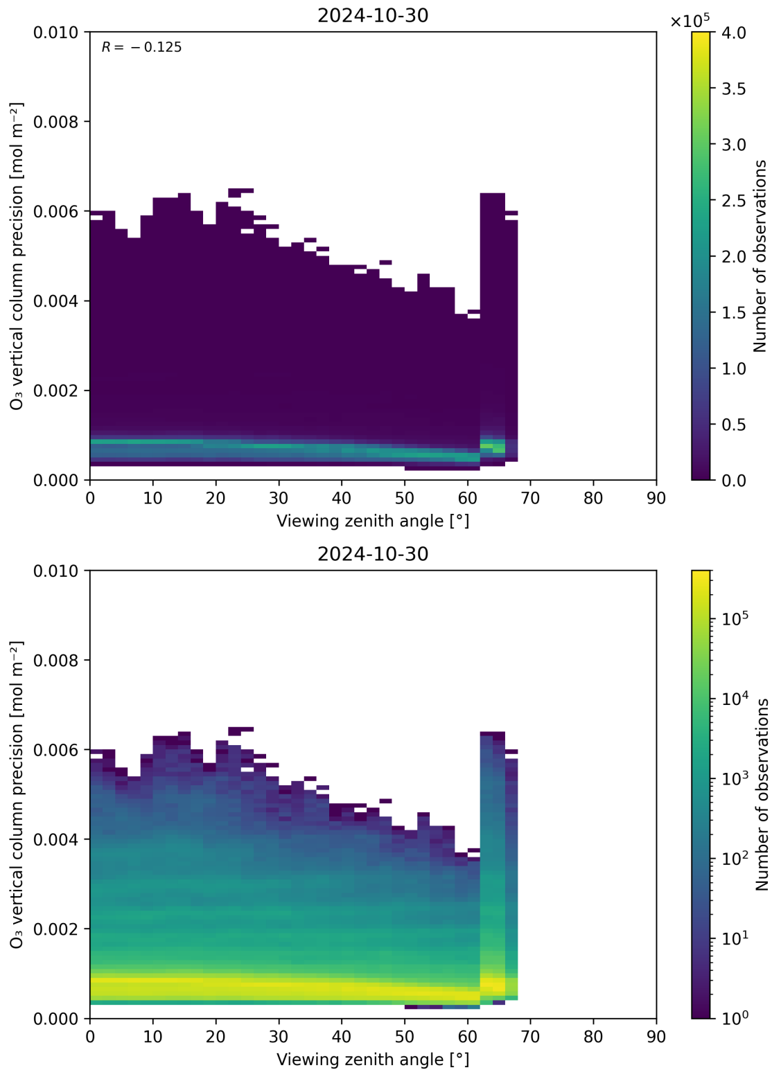
Figure 53: Scatter density plot of “Viewing zenith angle” against “O 3 vertical column precision” for 2024-10-30 to 2024-10-31.
