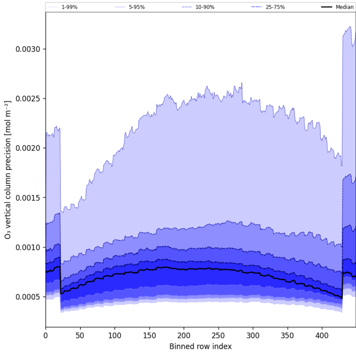
Figure 29: Along track statistics of “O 3 vertical column precision” for 2024-10-30 to 2024-10-31
