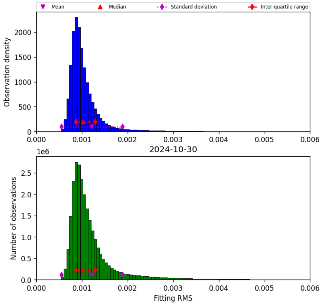
Figure 23: Histogram of “Fitting RMS” for 2024-10-30 to 2024-10-31
