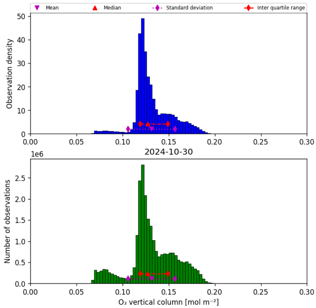
Figure 21: Histogram of “O 3 vertical column” for 2024-10-30 to 2024-10-31
