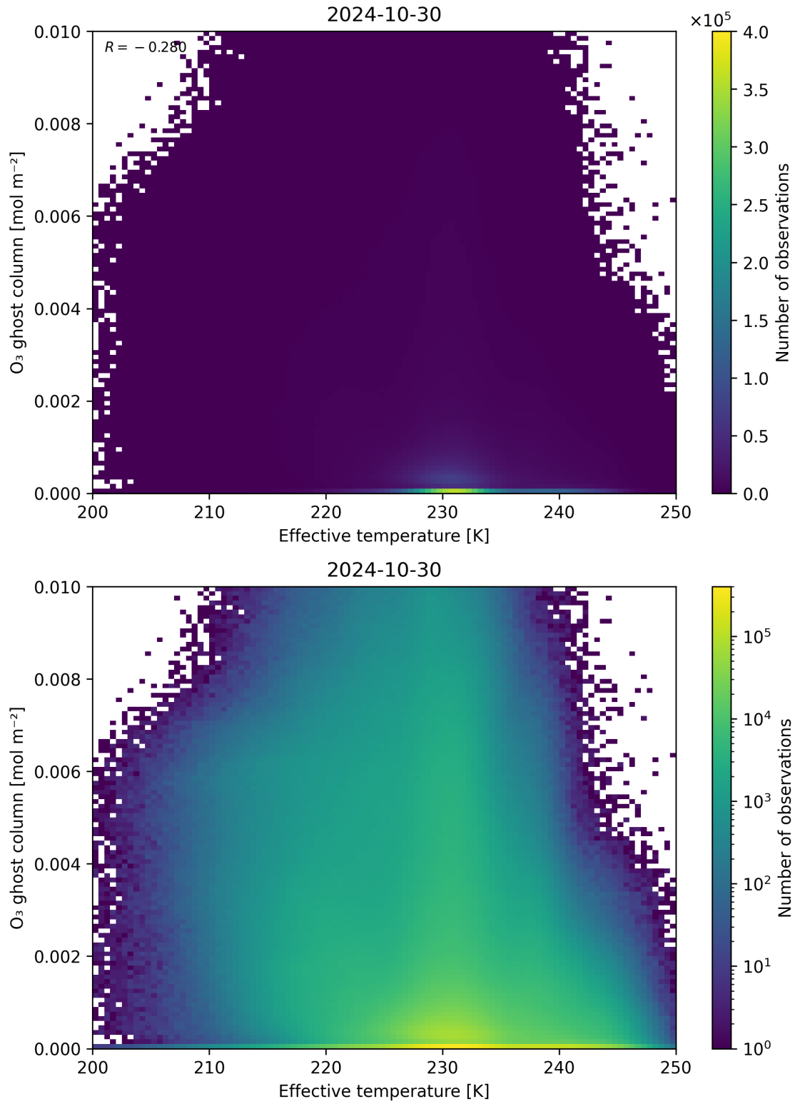
Figure 38: Scatter density plot of “Effective temperature” against “O 3 ghost column” for 2024-10-30 to 2024-10-31.
