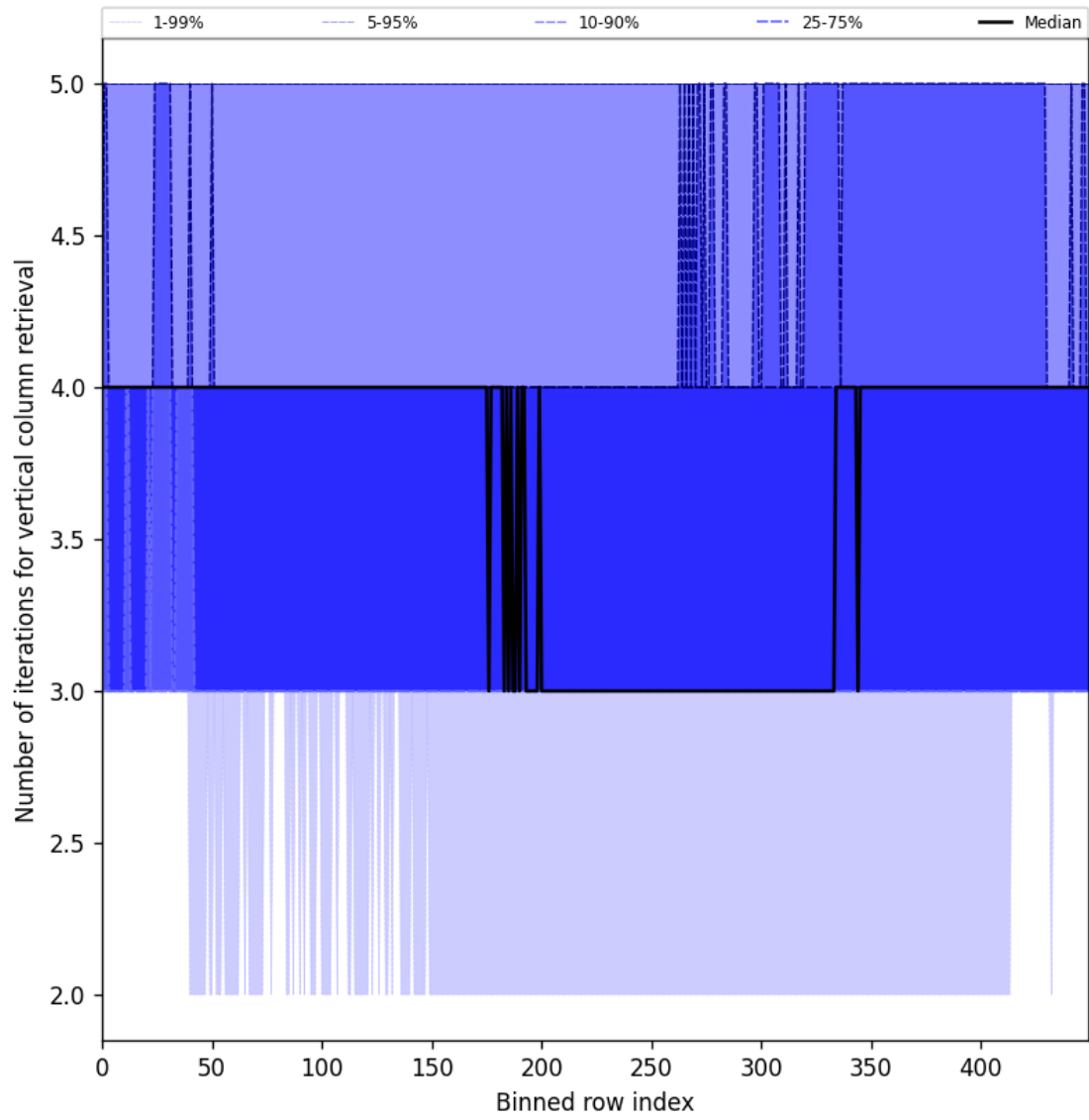
Figure 33: Along track statistics of “Number of iterations for vertical column retrieval” for 2024-10-30 to 2024-10-31
