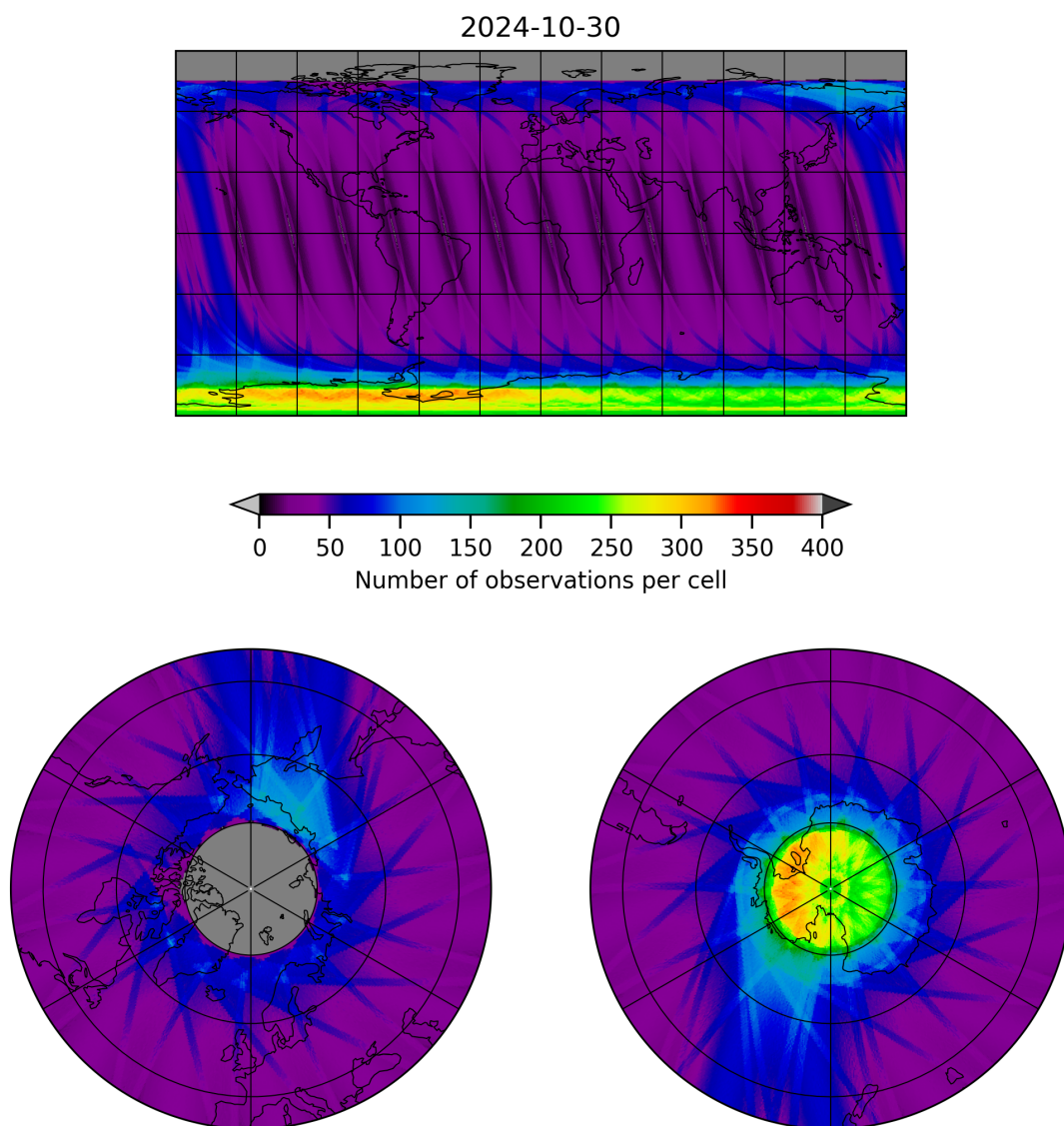
Figure 12: Map of the number of observations for 2024-10-30 to 2024-10-31
