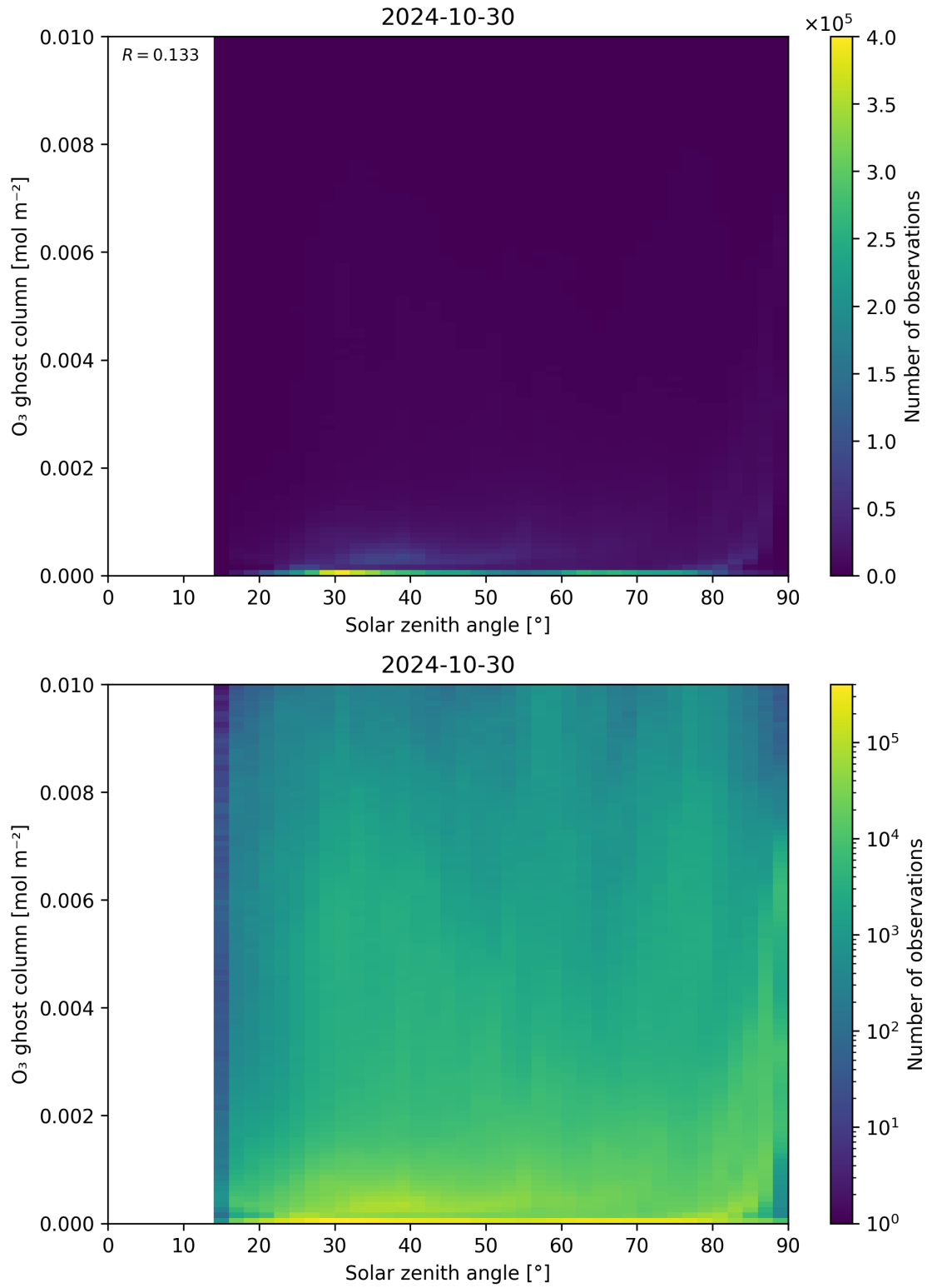
Figure 46: Scatter density plot of “Solar zenith angle” against “O 3 ghost column” for 2024-10-30 to 2024-10-31.
