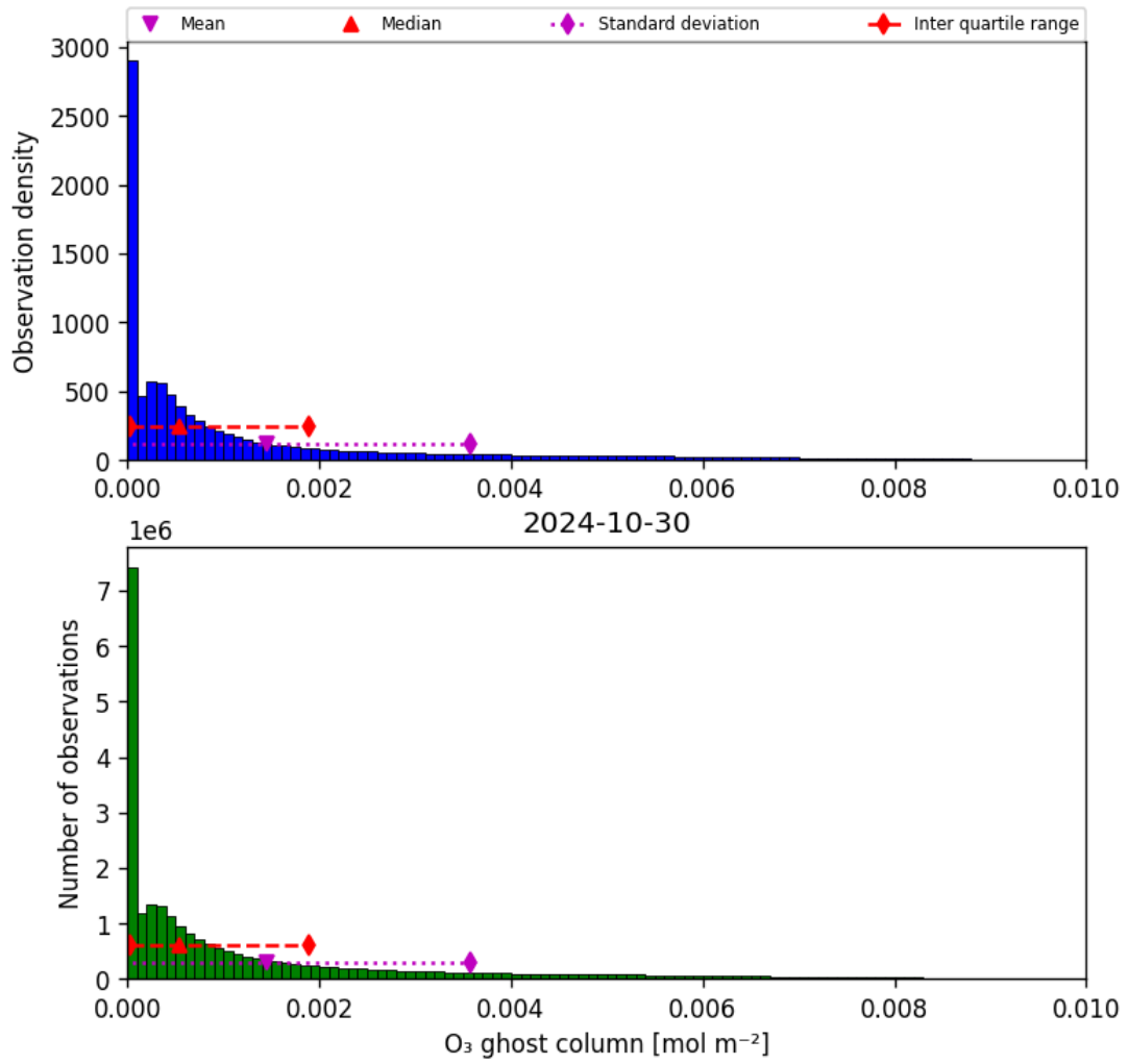
Figure 25: Histogram of “O 3 ghost column” for 2024-10-30 to 2024-10-31
