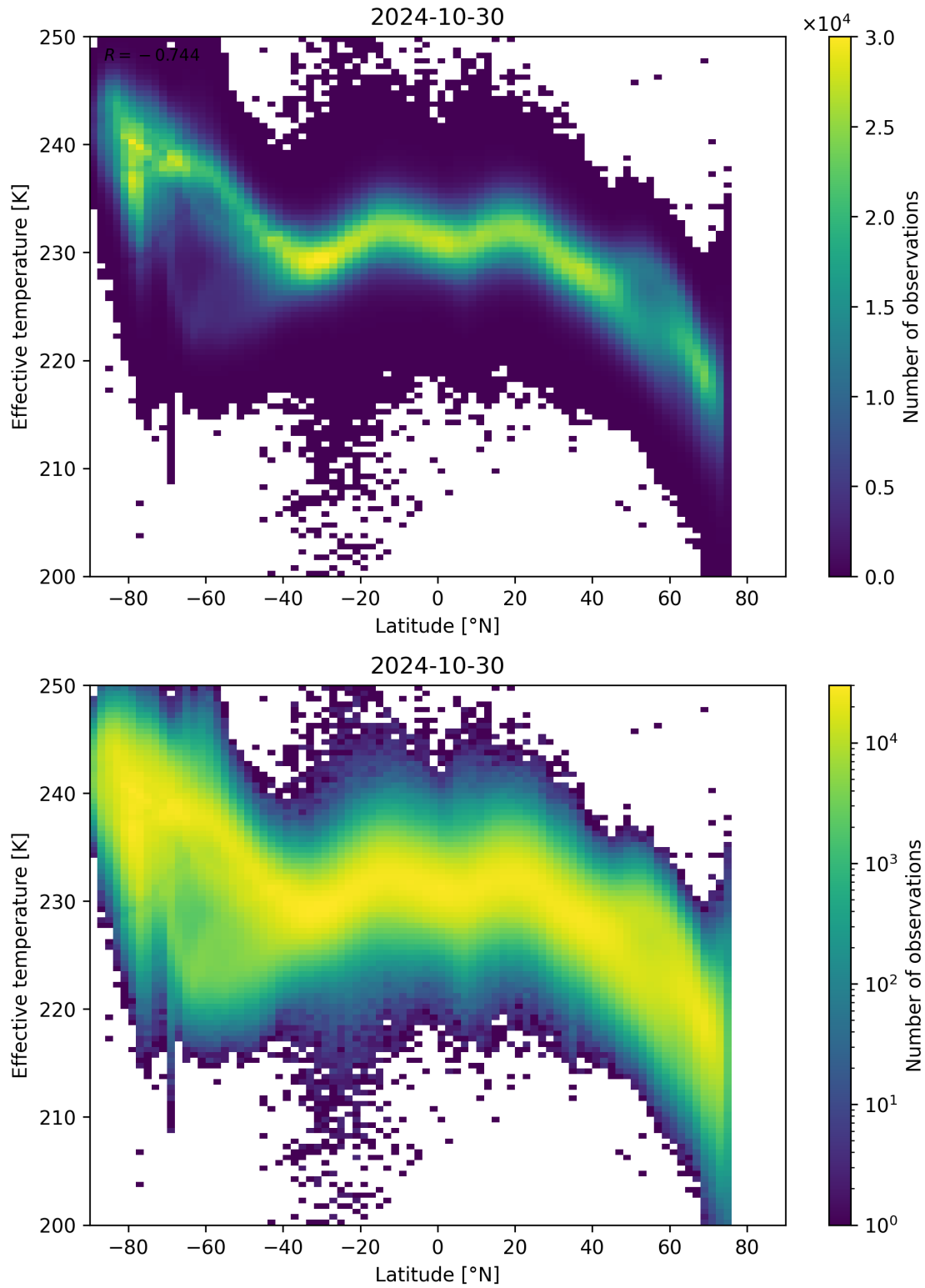
Figure 34: Scatter density plot of “Latitude” against “Effective temperature” for 2024-10-30 to 2024-10-31.
