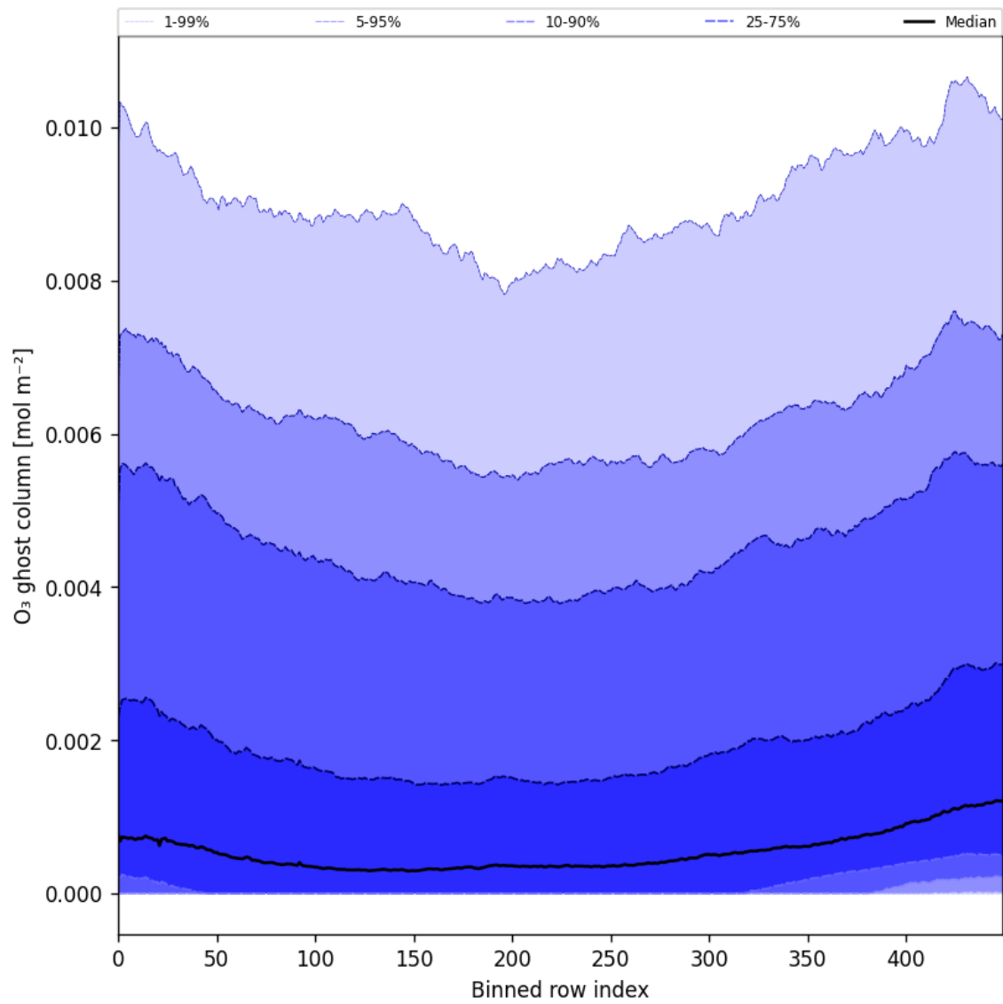
Figure 32: Along track statistics of “O 3 ghost column” for 2024-10-30 to 2024-10-31
