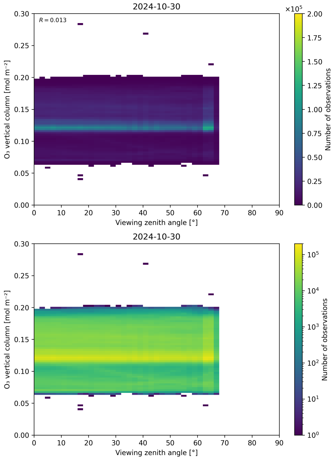
Figure 52: Scatter density plot of “Viewing zenith angle” against “O 3 vertical column” for 2024-10-30 to 2024-10-31.
