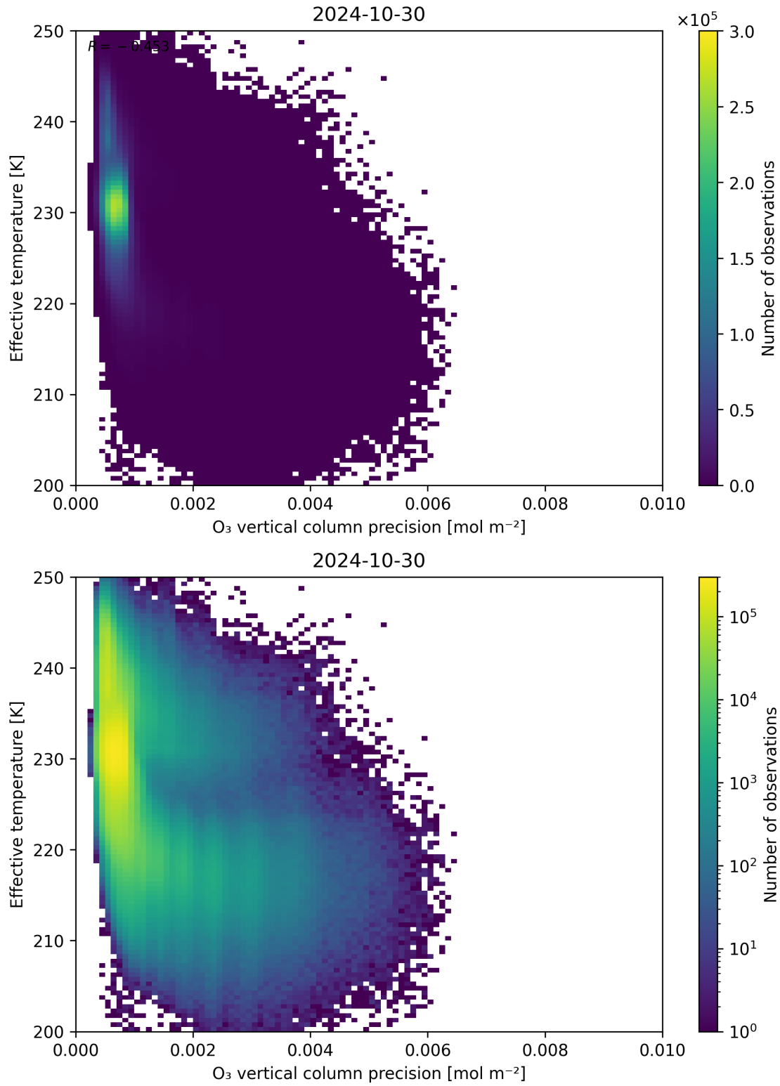
Figure 42: Scatter density plot of “O 3 vertical column precision” against “Effective temperature” for 2024-10-30 to 2024-10-31.
