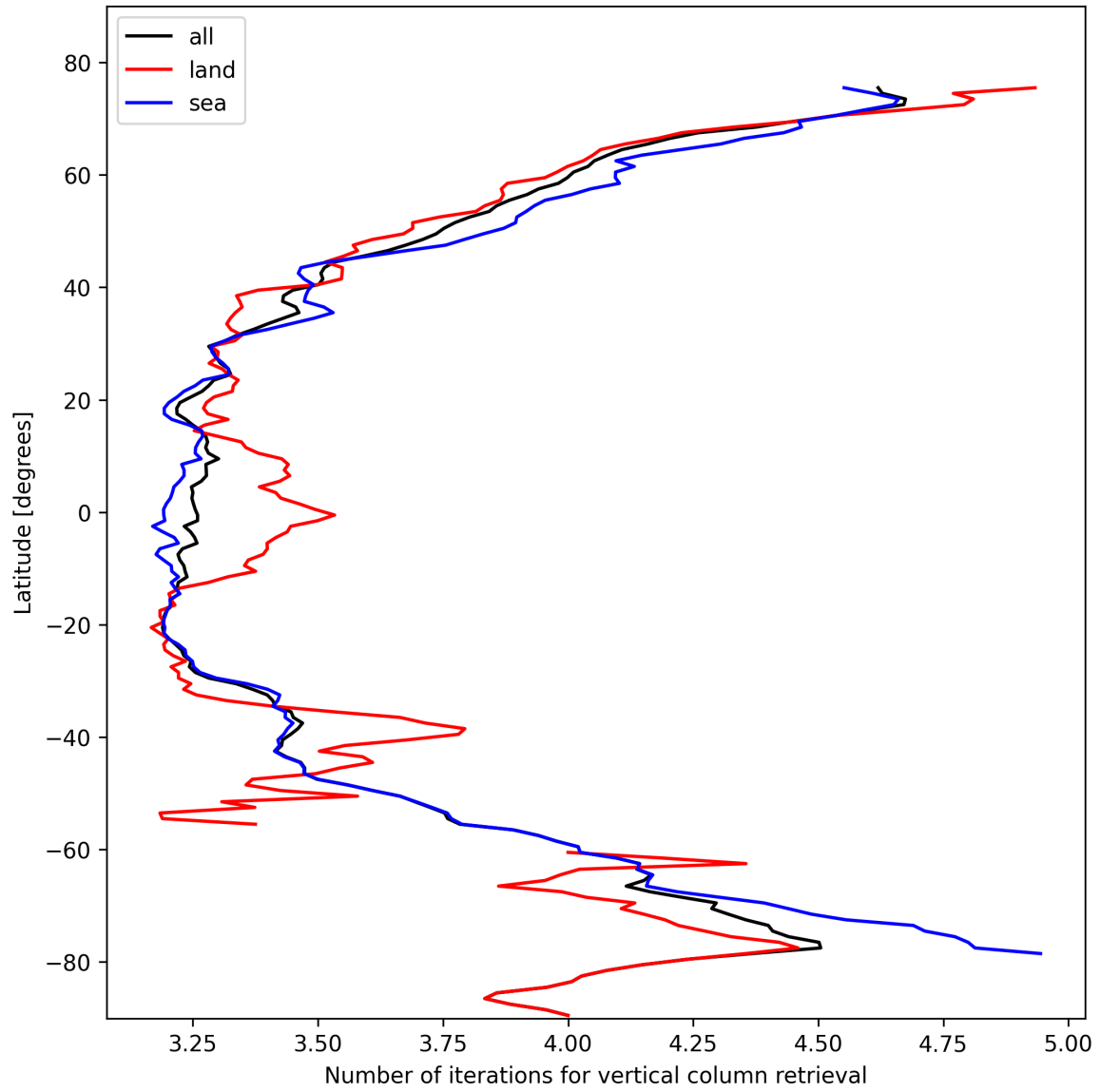
Figure 19: Zonal average of “Number of iterations for vertical column retrieval” for 2024-10-30 to 2024-10-31.
