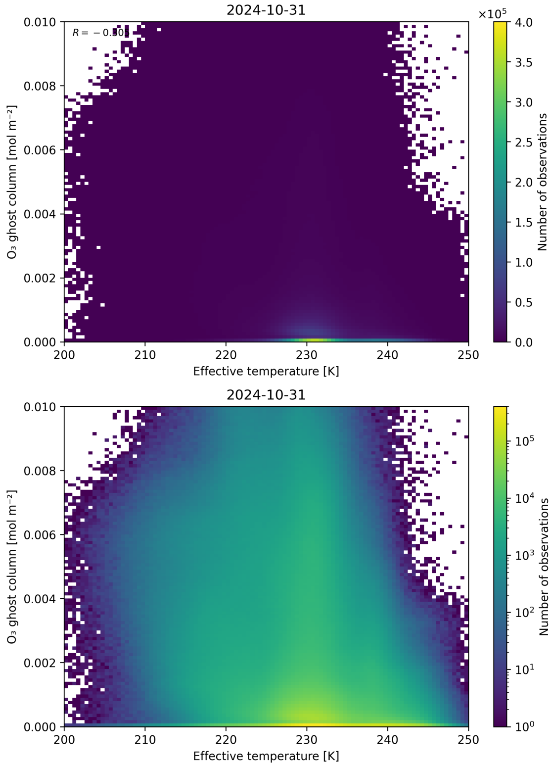
Figure 38: Scatter density plot of “Effective temperature” against “O 3 ghost column” for 2024-10-30 to 2024-11-01.
