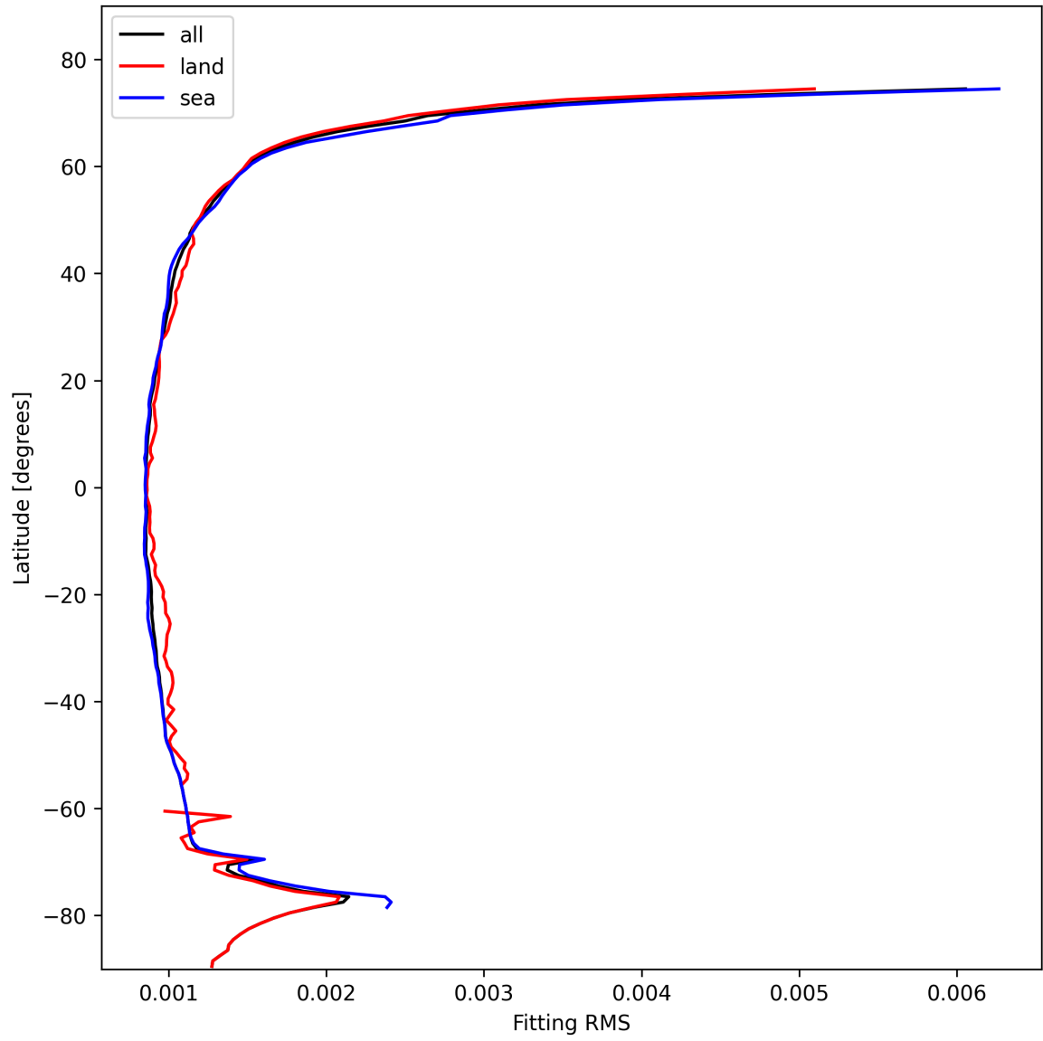
Figure 16: Zonal average of “Fitting RMS” for 2024-10-30 to 2024-11-01.
