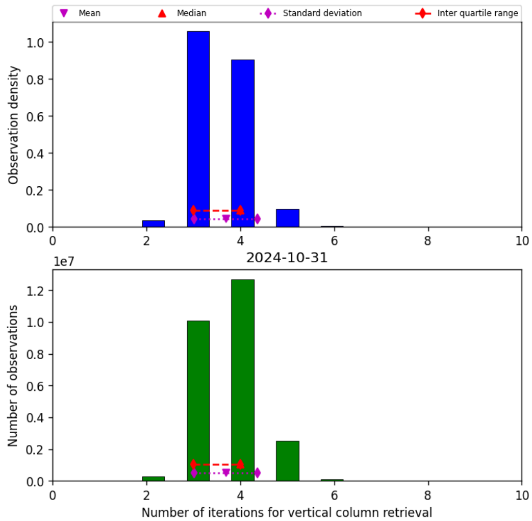
Figure 26: Histogram of “Number of iterations for vertical column retrieval” for 2024-10-30 to 2024-11-01
