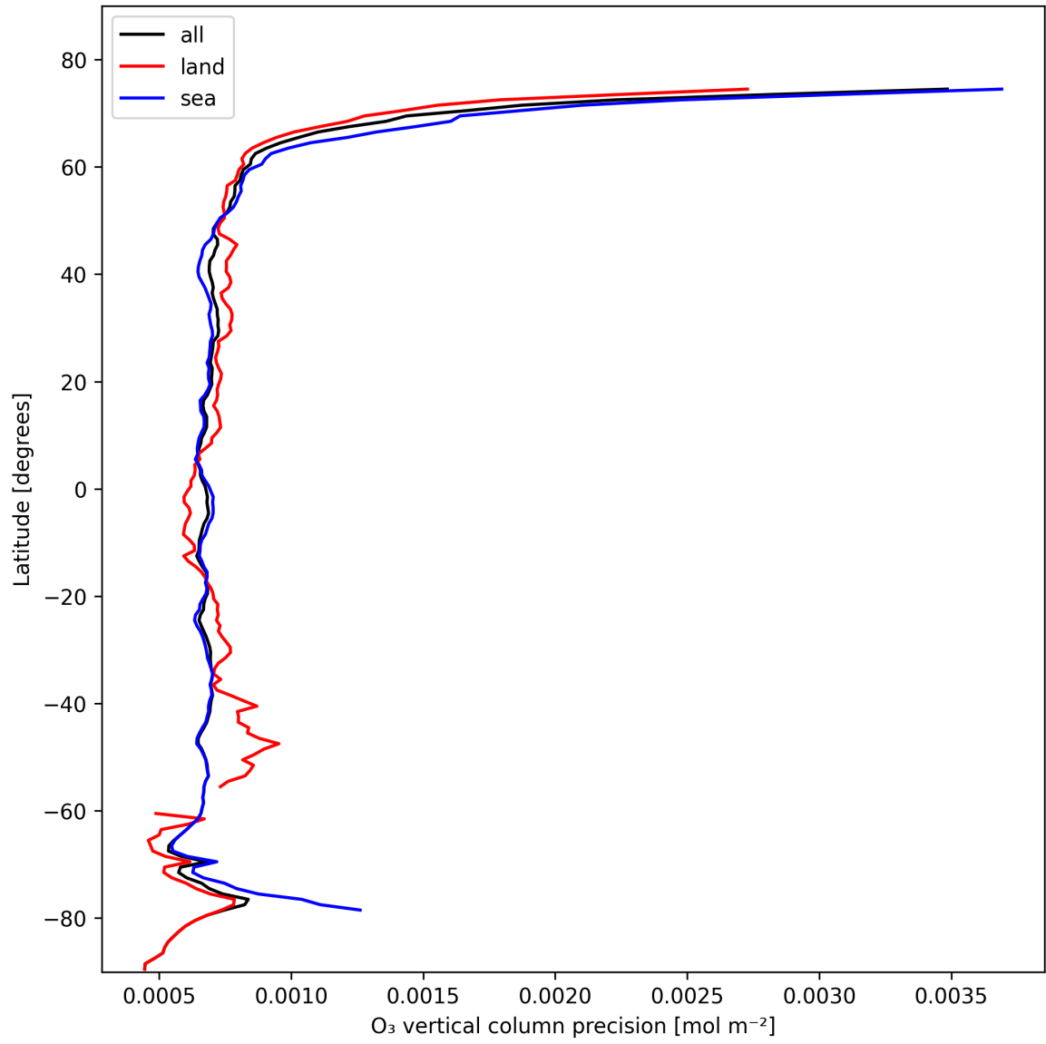
Figure 15: Zonal average of “O 3 vertical column precision” for 2024-10-30 to 2024-11-01.
