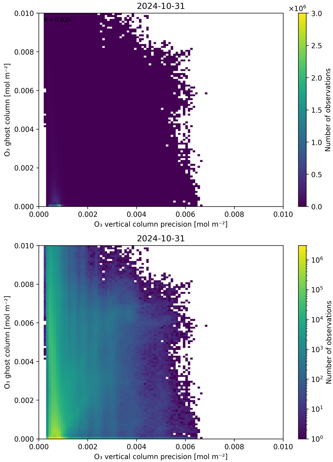
Figure 43: Scatter density plot of “O 3 vertical column precision” against “O 3 ghost column” for 2024-10-30 to 2024-11-01.
