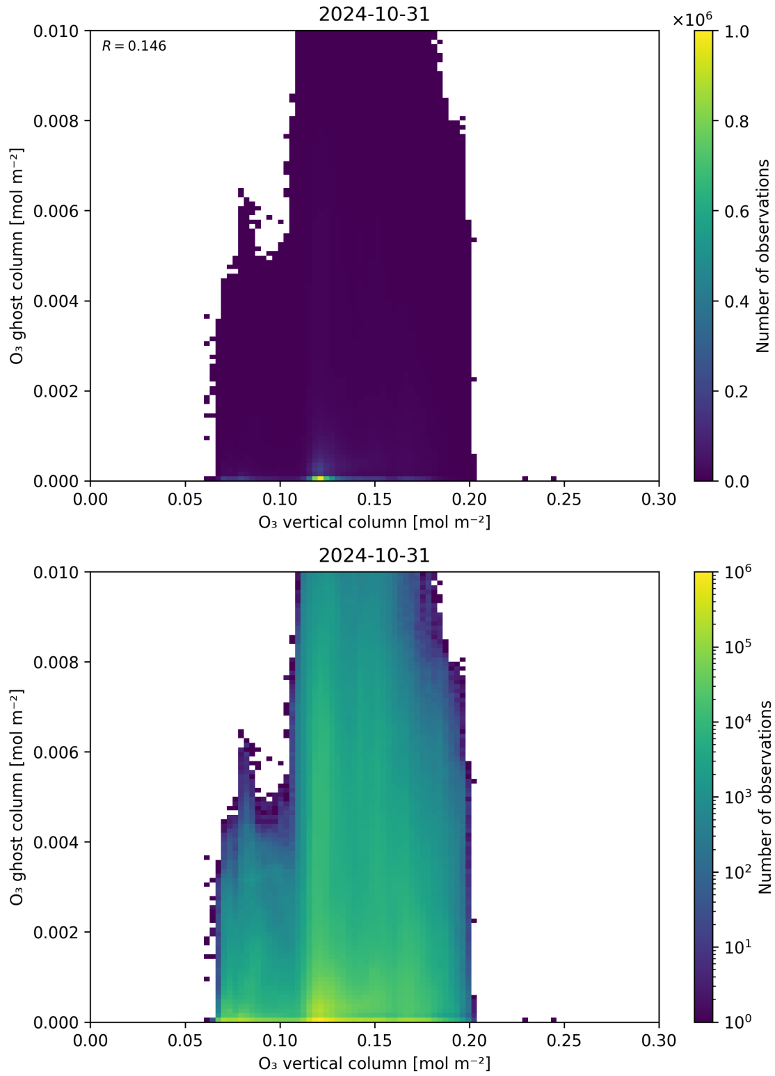
Figure 40: Scatter density plot of “O 3 vertical column” against “O 3 ghost column” for 2024-10-30 to 2024-11-01.
