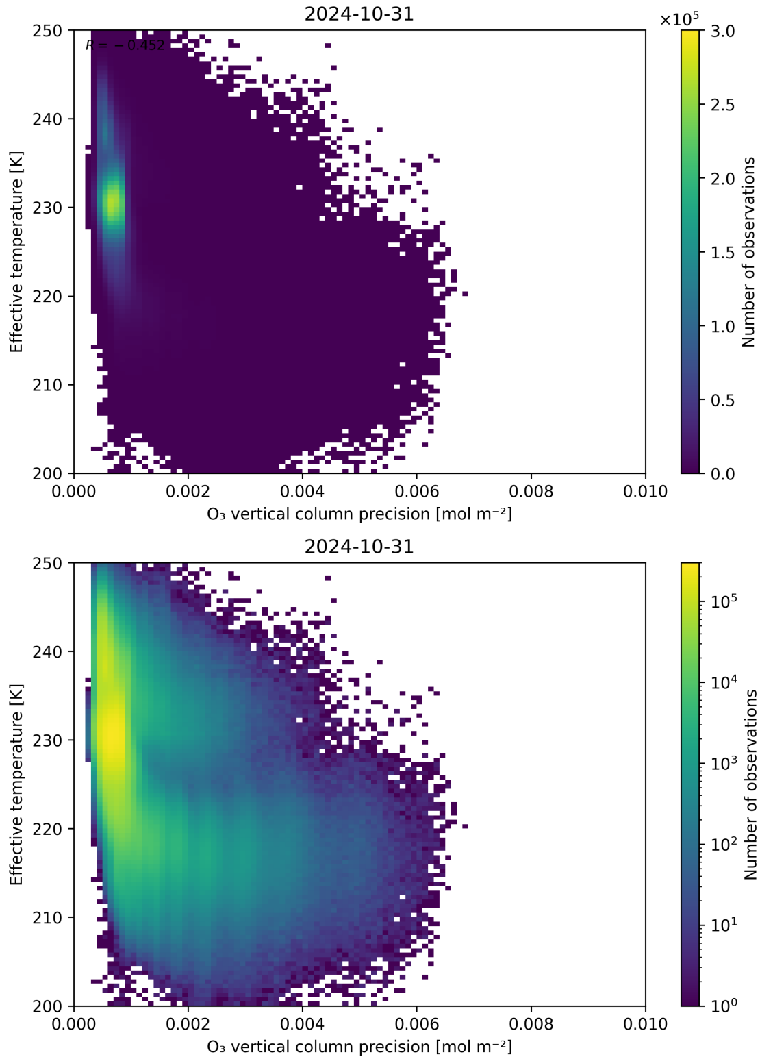
Figure 42: Scatter density plot of “O 3 vertical column precision” against “Effective temperature” for 2024-10-30 to 2024-11-01.
