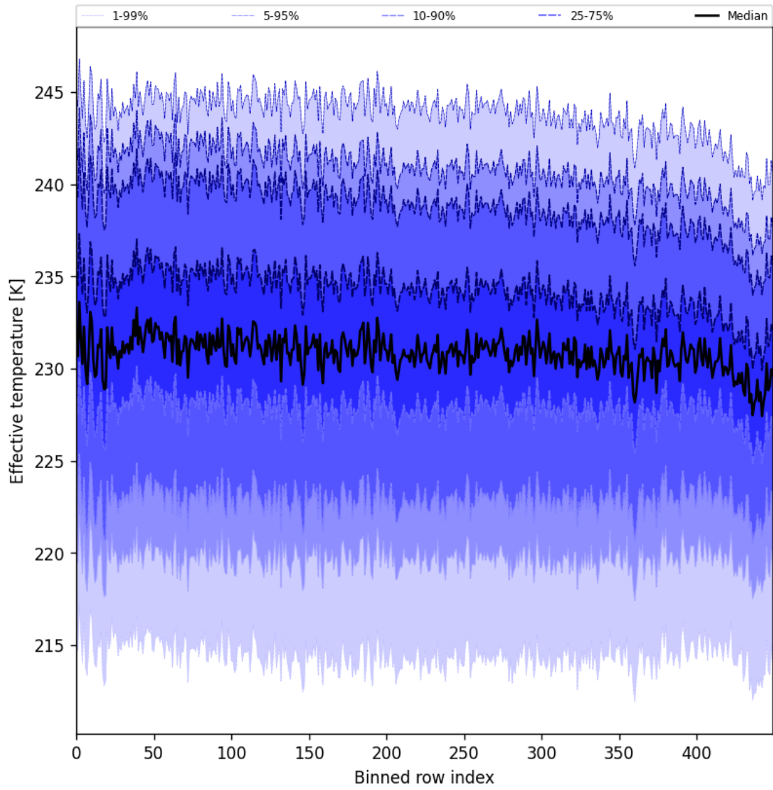
Figure 31: Along track statistics of “Effective temperature” for 2024-10-30 to 2024-11-01
