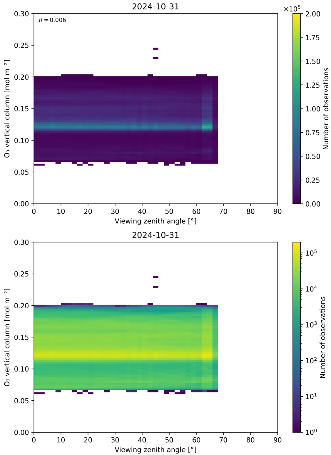
Figure 52: Scatter density plot of “Viewing zenith angle” against “O 3 vertical column” for 2024-10-30 to 2024-11-01.
