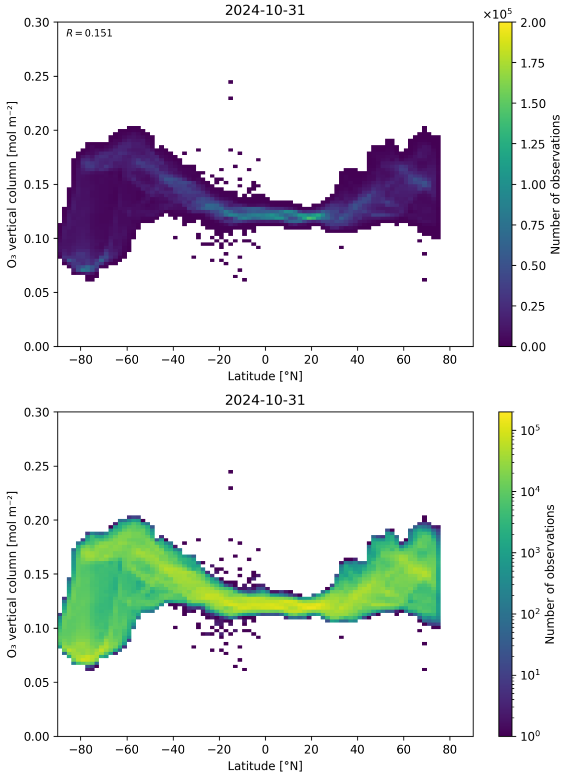
Figure 36: Scatter density plot of “Latitude” against “O 3 vertical column” for 2024-10-30 to 2024-11-01.
