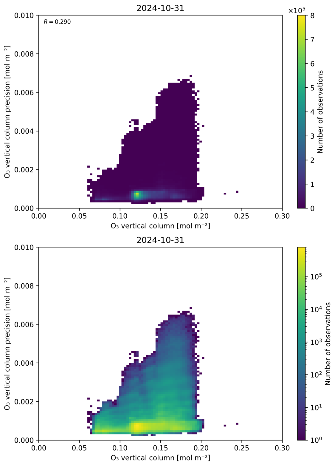
Figure 41: Scatter density plot of “O 3 vertical column” against “O 3 vertical column precision” for 2024-10-30 to 2024-11-01.
