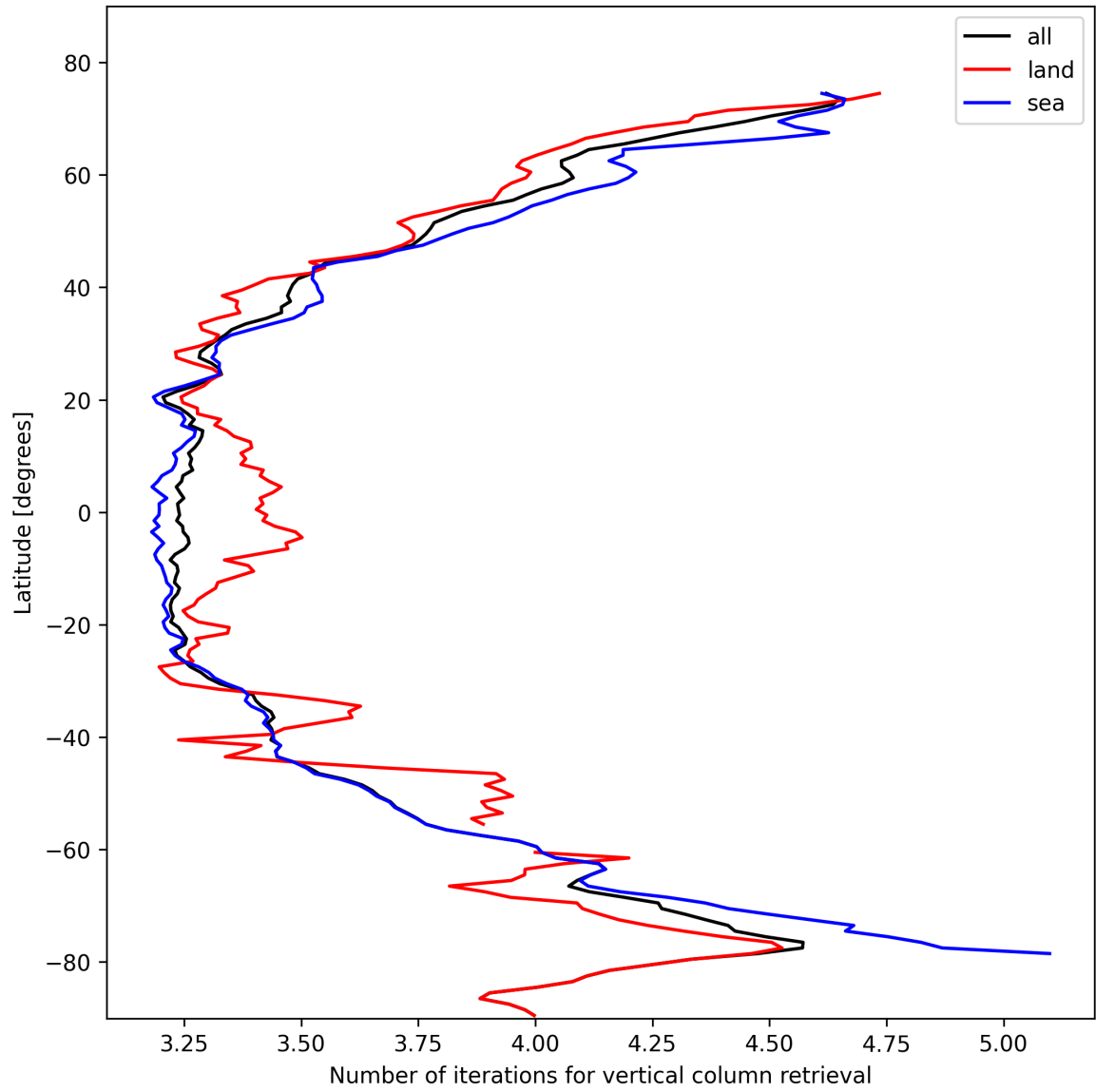
Figure 19: Zonal average of “Number of iterations for vertical column retrieval” for 2024-10-30 to 2024-11-01.
