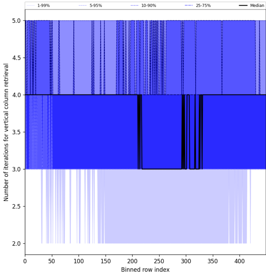
Figure 33: Along track statistics of “Number of iterations for vertical column retrieval” for 2024-10-30 to 2024-11-01
