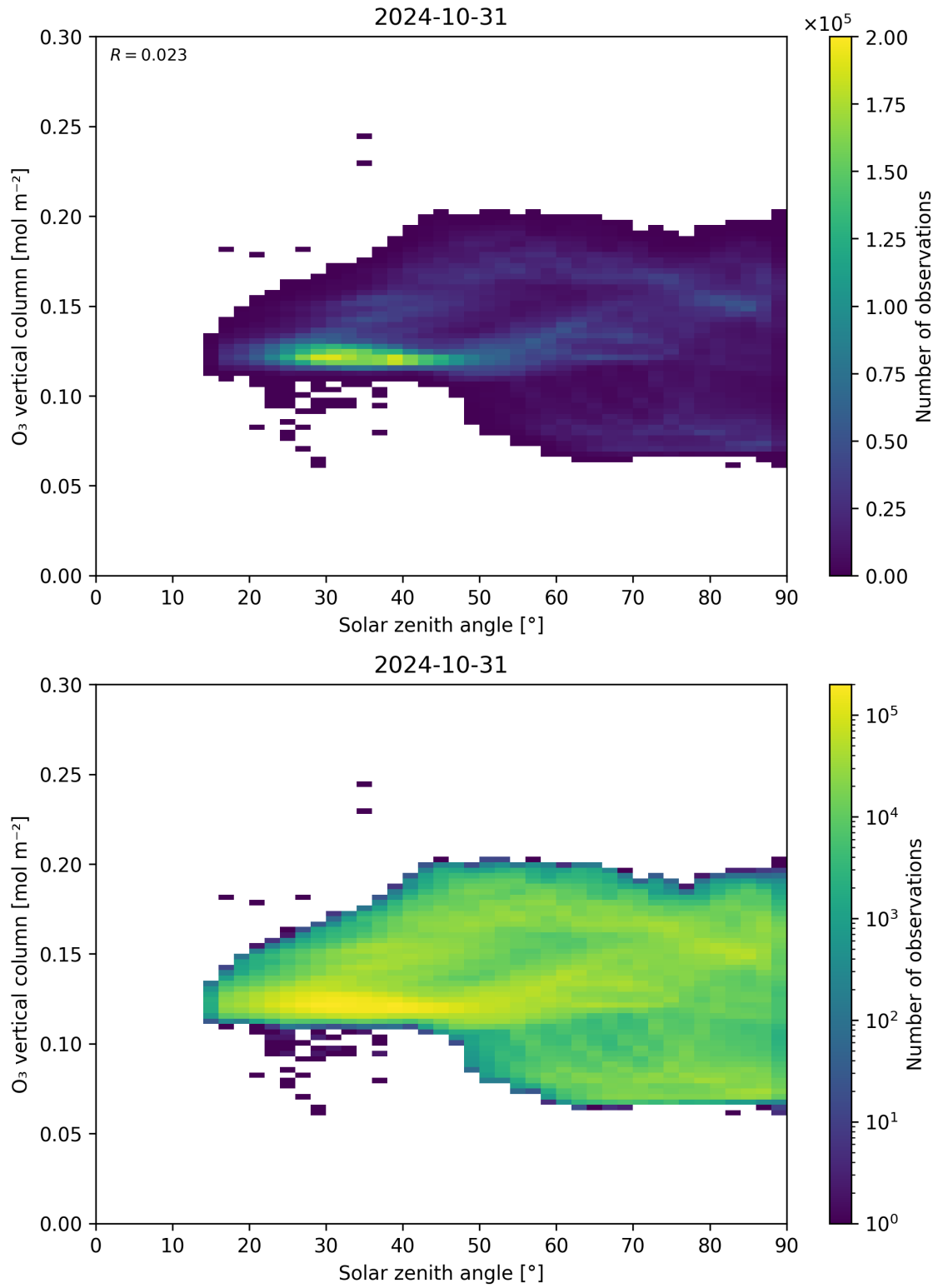
Figure 47: Scatter density plot of “Solar zenith angle” against “O 3 vertical column” for 2024-10-30 to 2024-11-01.
