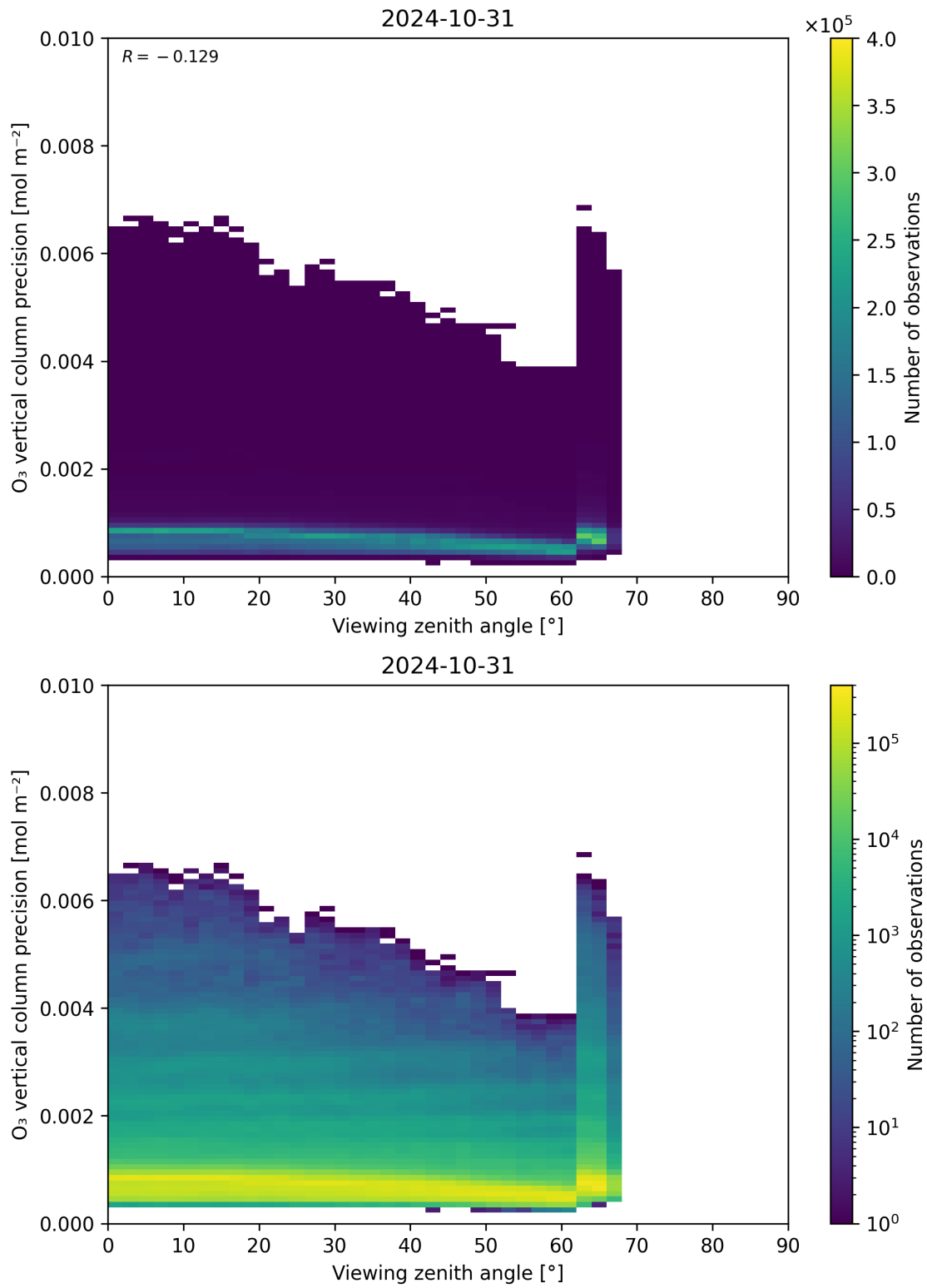
Figure 53: Scatter density plot of “Viewing zenith angle” against “O 3 vertical column precision” for 2024-10-30 to 2024-11-01.
