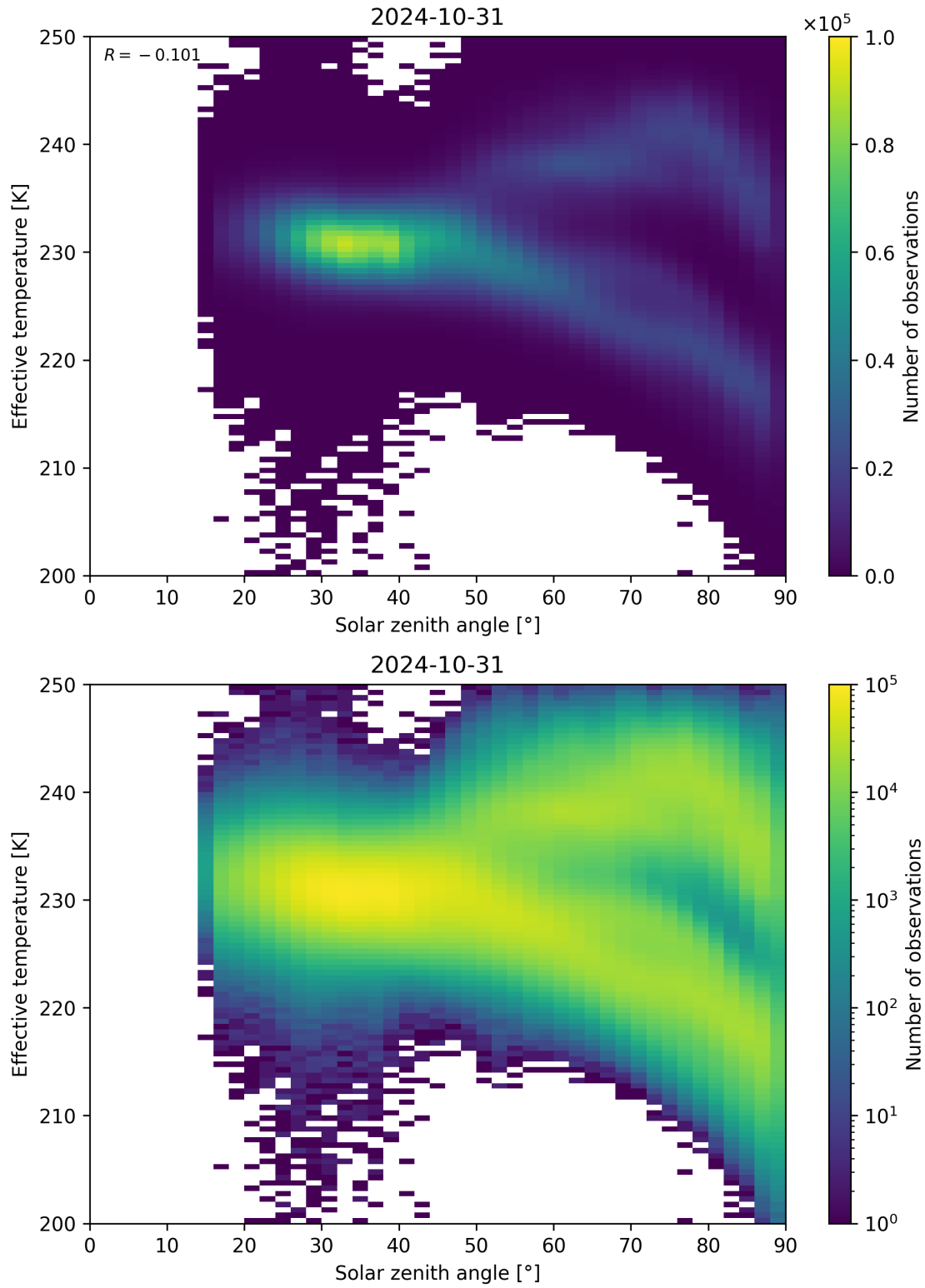
Figure 45: Scatter density plot of “Solar zenith angle” against “Effective temperature” for 2024-10-30 to 2024-11-01.
