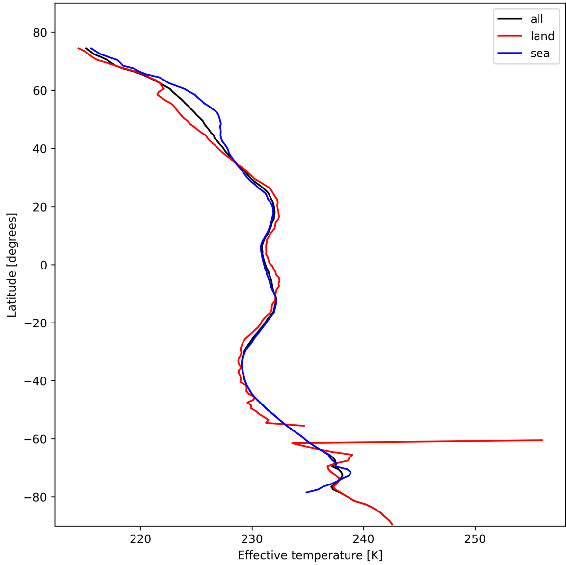
Figure 17: Zonal average of “Effective temperature” for 2024-10-30 to 2024-11-01.
