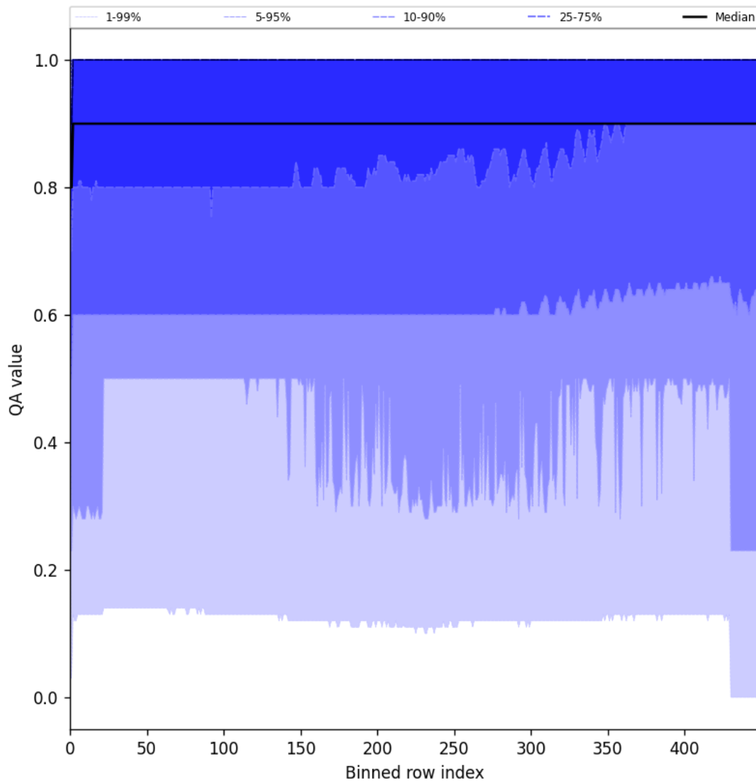
Figure 27: Along track statistics of “QA value” for 2024-10-30 to 2024-11-01
