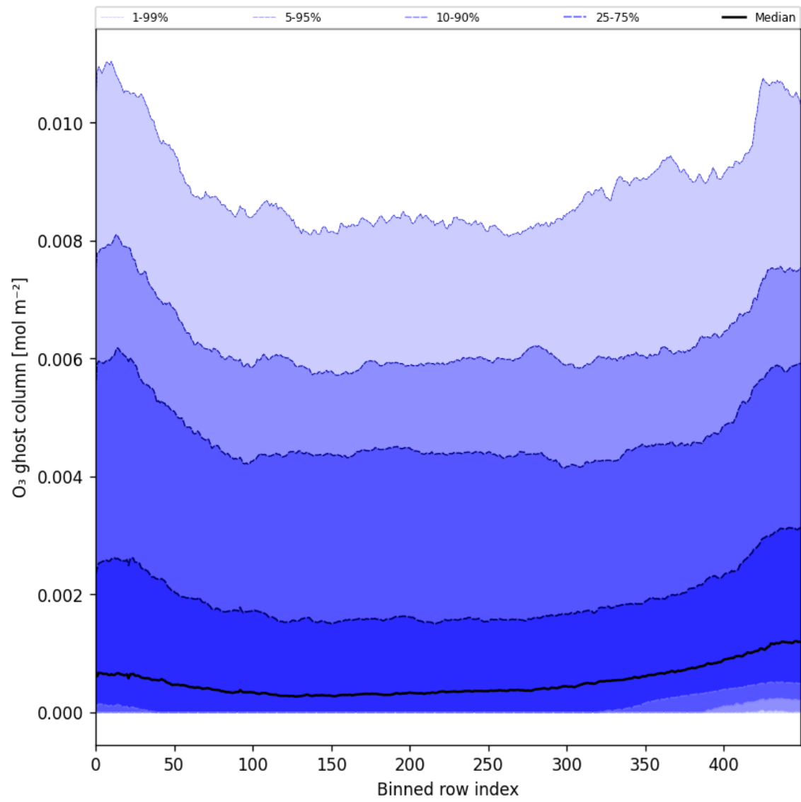
Figure 32: Along track statistics of “O 3 ghost column” for 2024-10-30 to 2024-11-01
