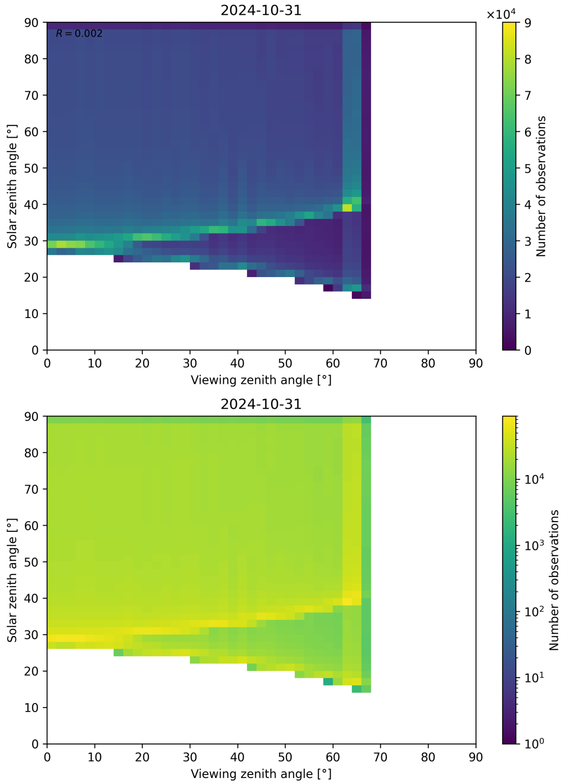
Figure 54: Scatter density plot of “Viewing zenith angle” against “Solar zenith angle” for 2024-10-30 to 2024-11-01.
