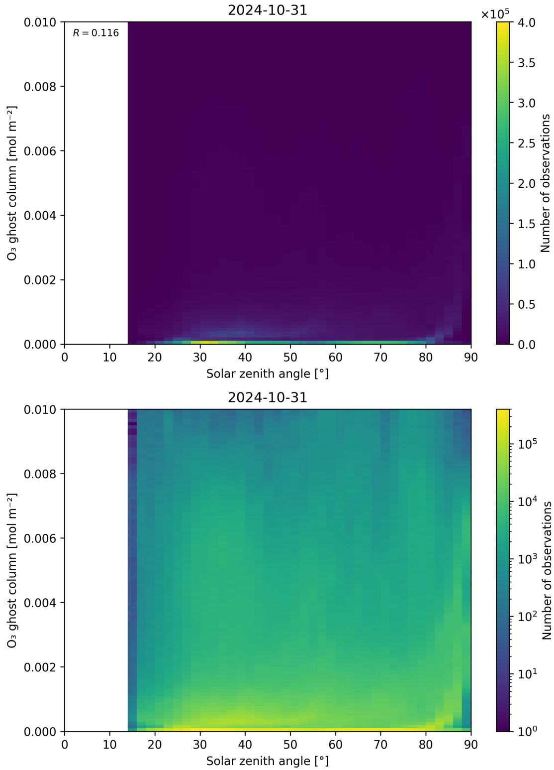
Figure 46: Scatter density plot of “Solar zenith angle” against “O 3 ghost column” for 2024-10-30 to 2024-11-01.
