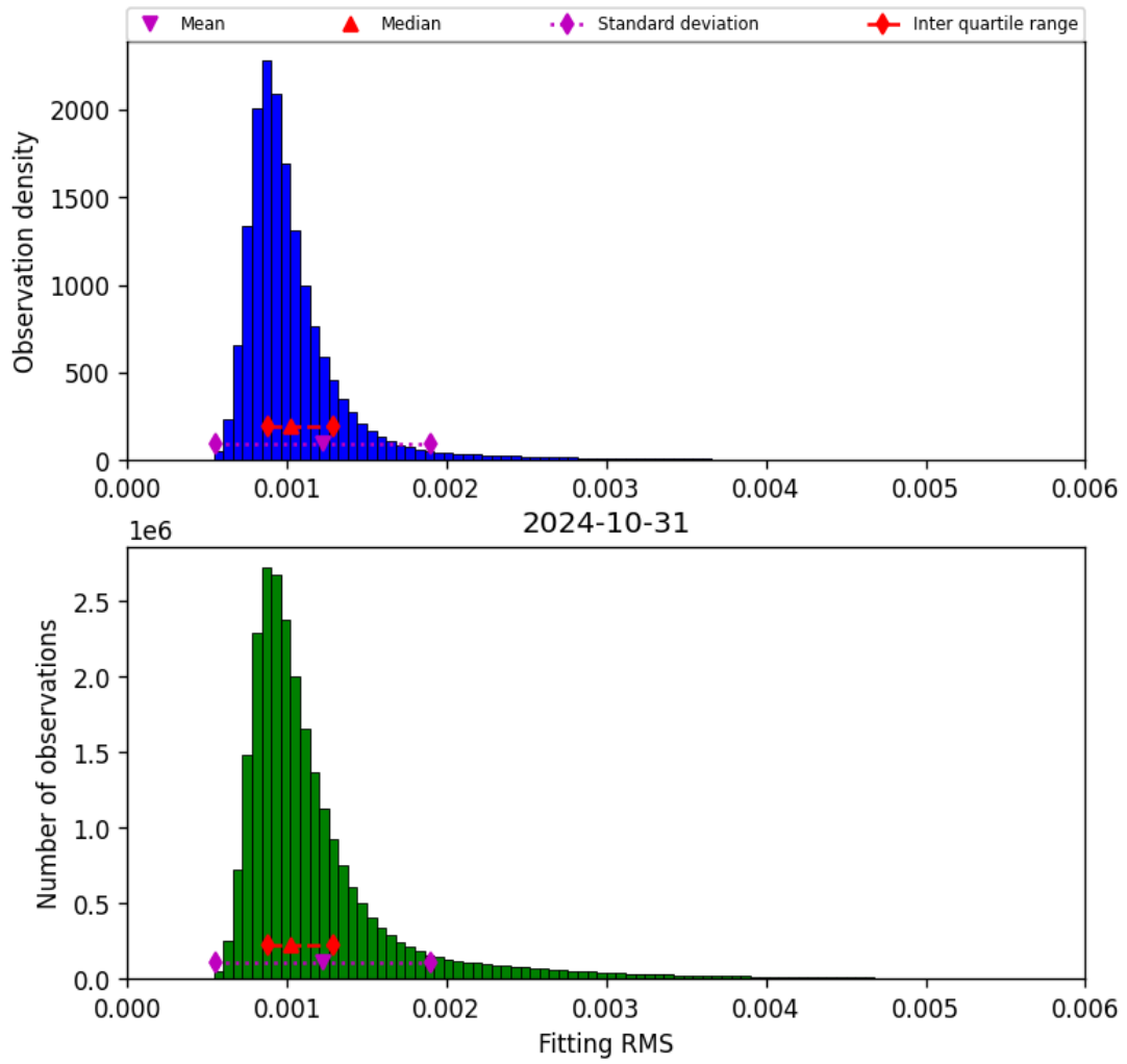
Figure 23: Histogram of “Fitting RMS” for 2024-10-30 to 2024-11-01
