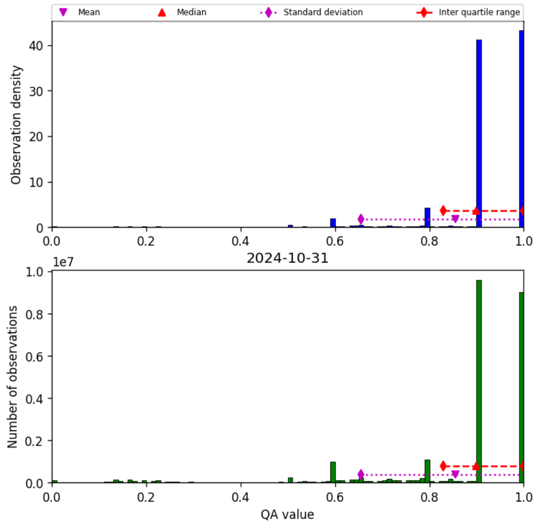
Figure 20: Histogram of “QA value” for 2024-10-30 to 2024-11-01
