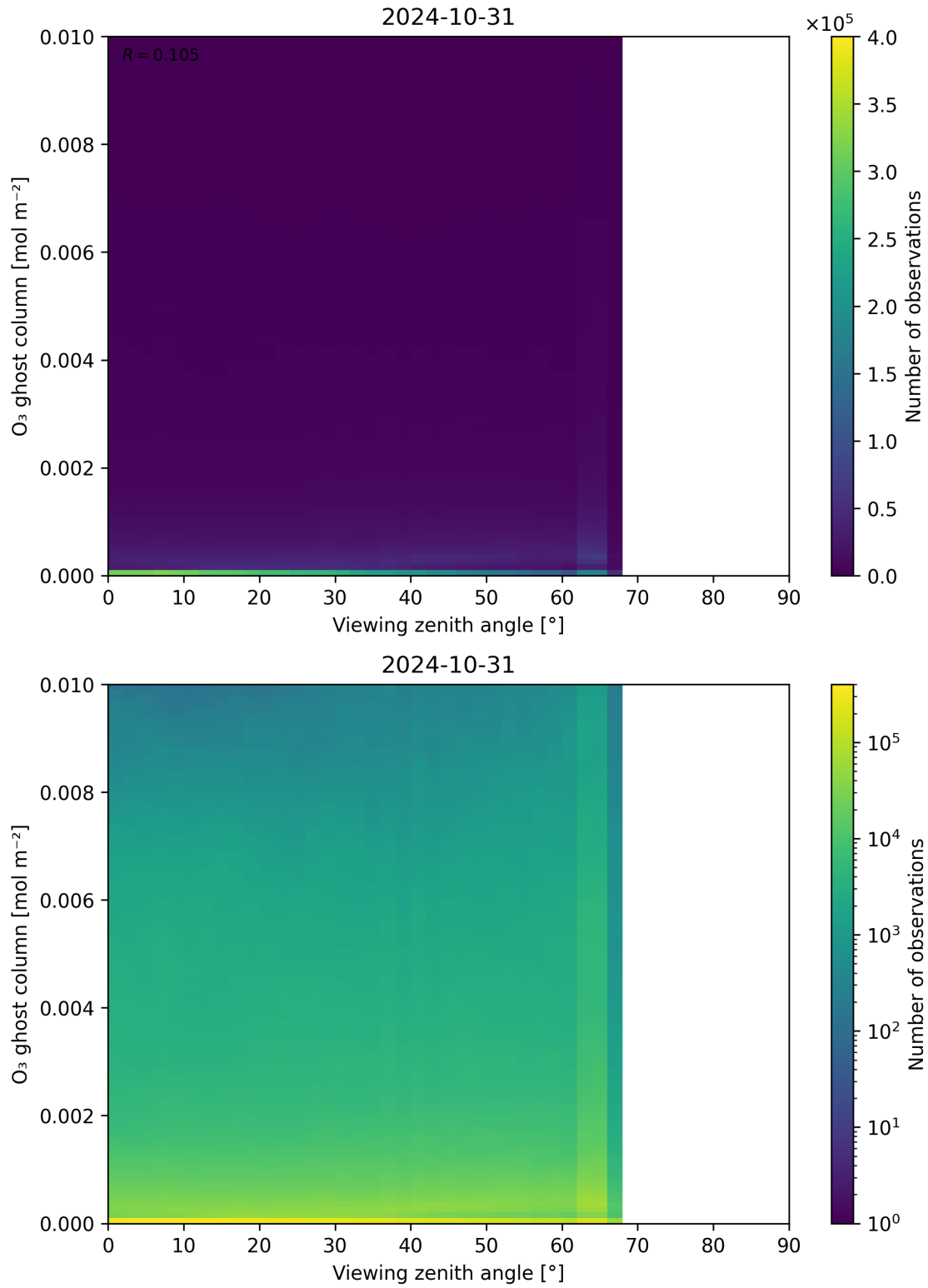
Figure 51: Scatter density plot of “Viewing zenith angle” against “O 3 ghost column” for 2024-10-30 to 2024-11-01.
