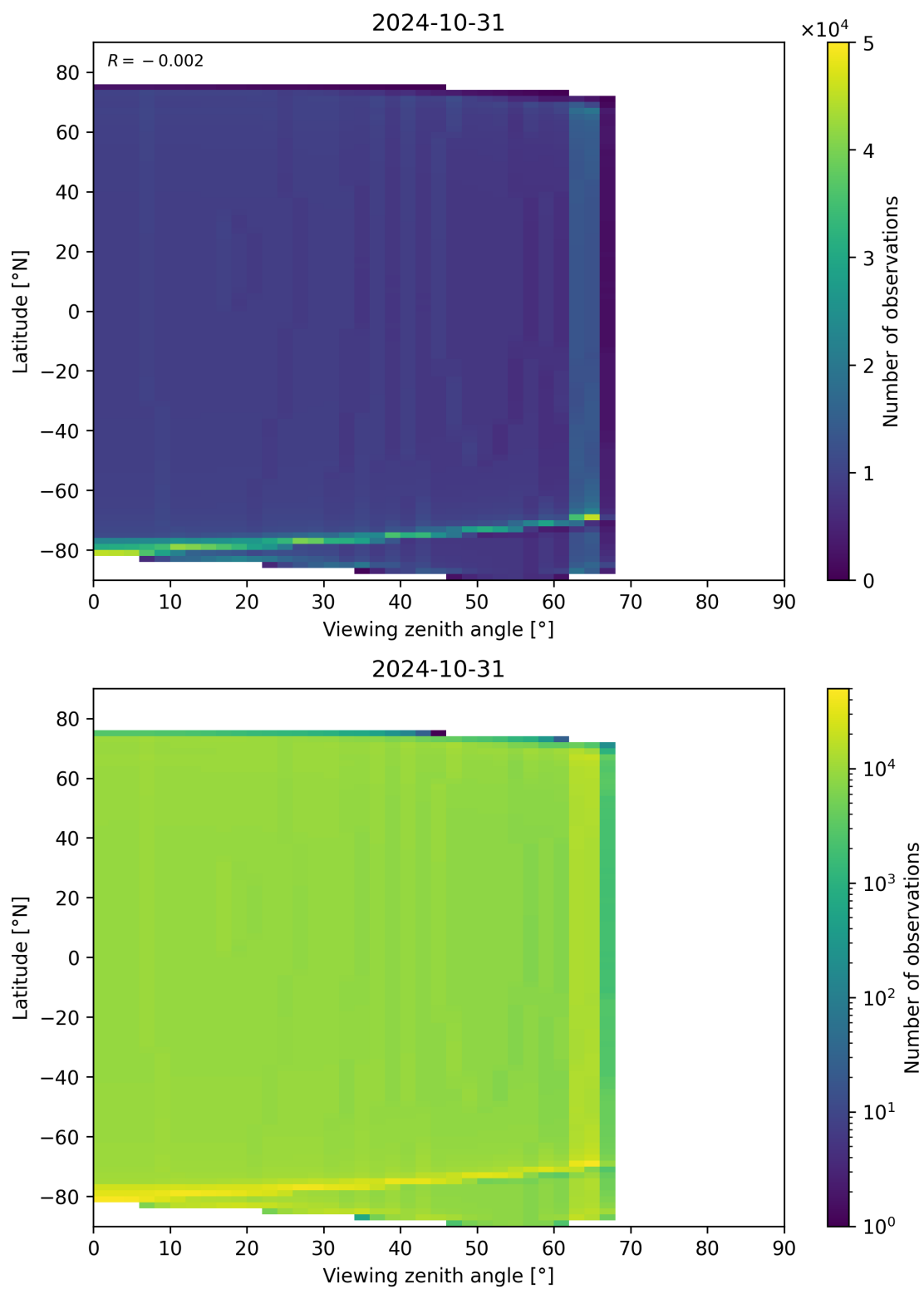
Figure 49: Scatter density plot of “Viewing zenith angle” against “Latitude” for 2024-10-30 to 2024-11-01.
