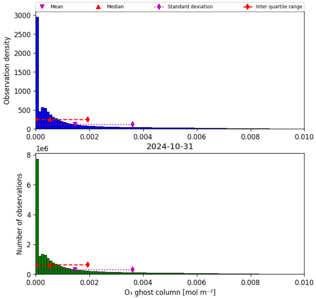
Figure 25: Histogram of “O 3 ghost column” for 2024-10-30 to 2024-11-01
