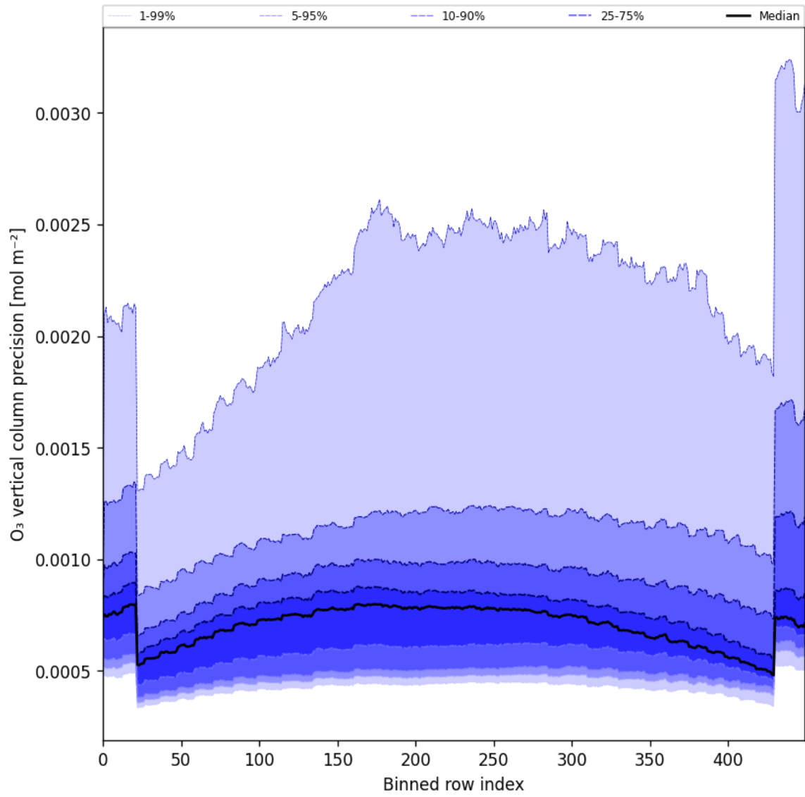
Figure 29: Along track statistics of “O 3 vertical column precision” for 2024-10-30 to 2024-11-01
