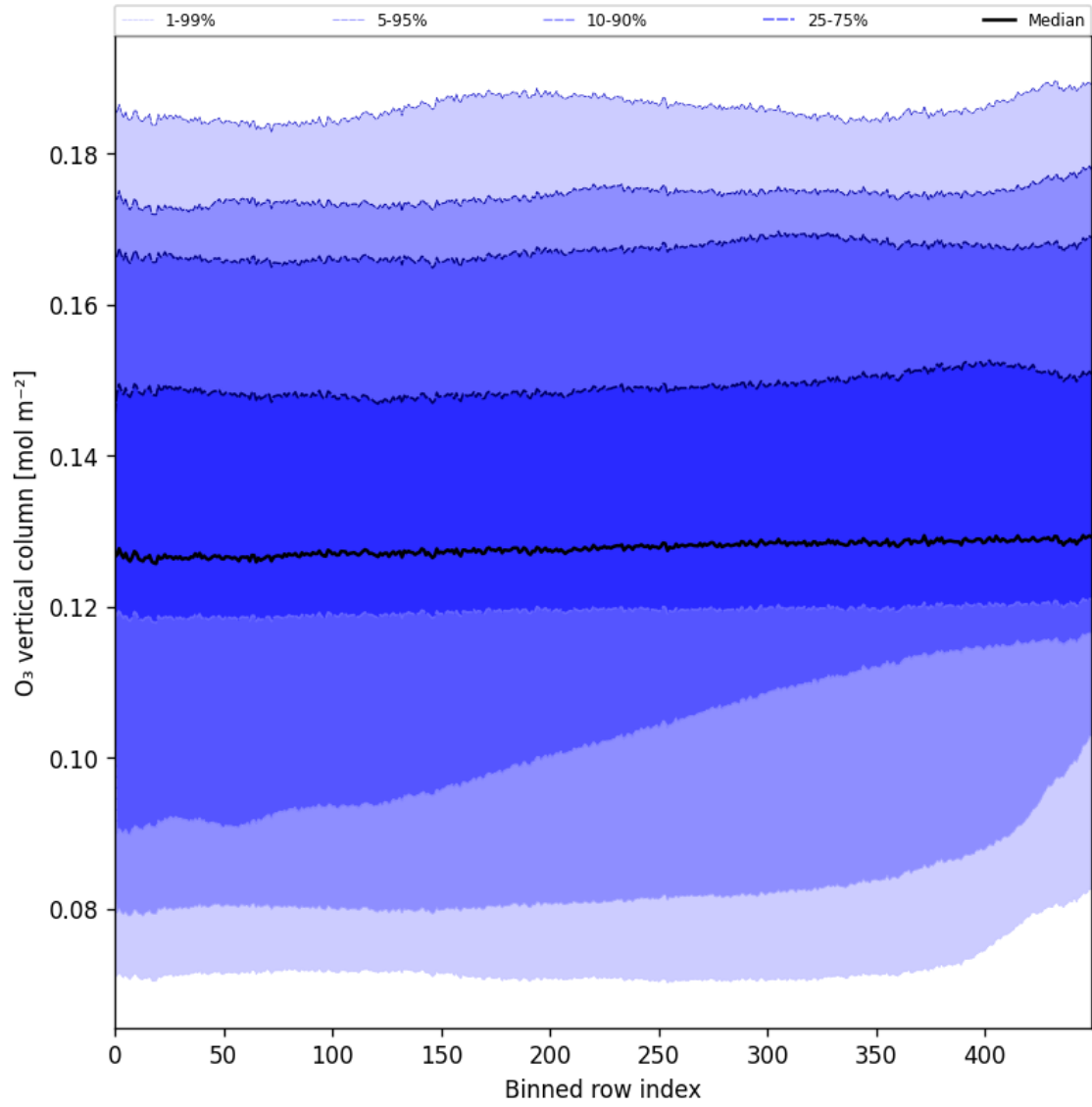
Figure 28: Along track statistics of “O 3 vertical column” for 2024-10-30 to 2024-11-01
