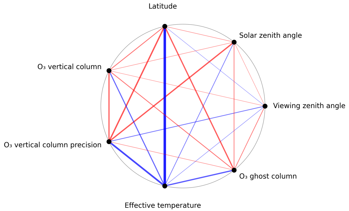
Figure 1: Map of correlation graph for 2024-10-30 to 2024-11-01.
