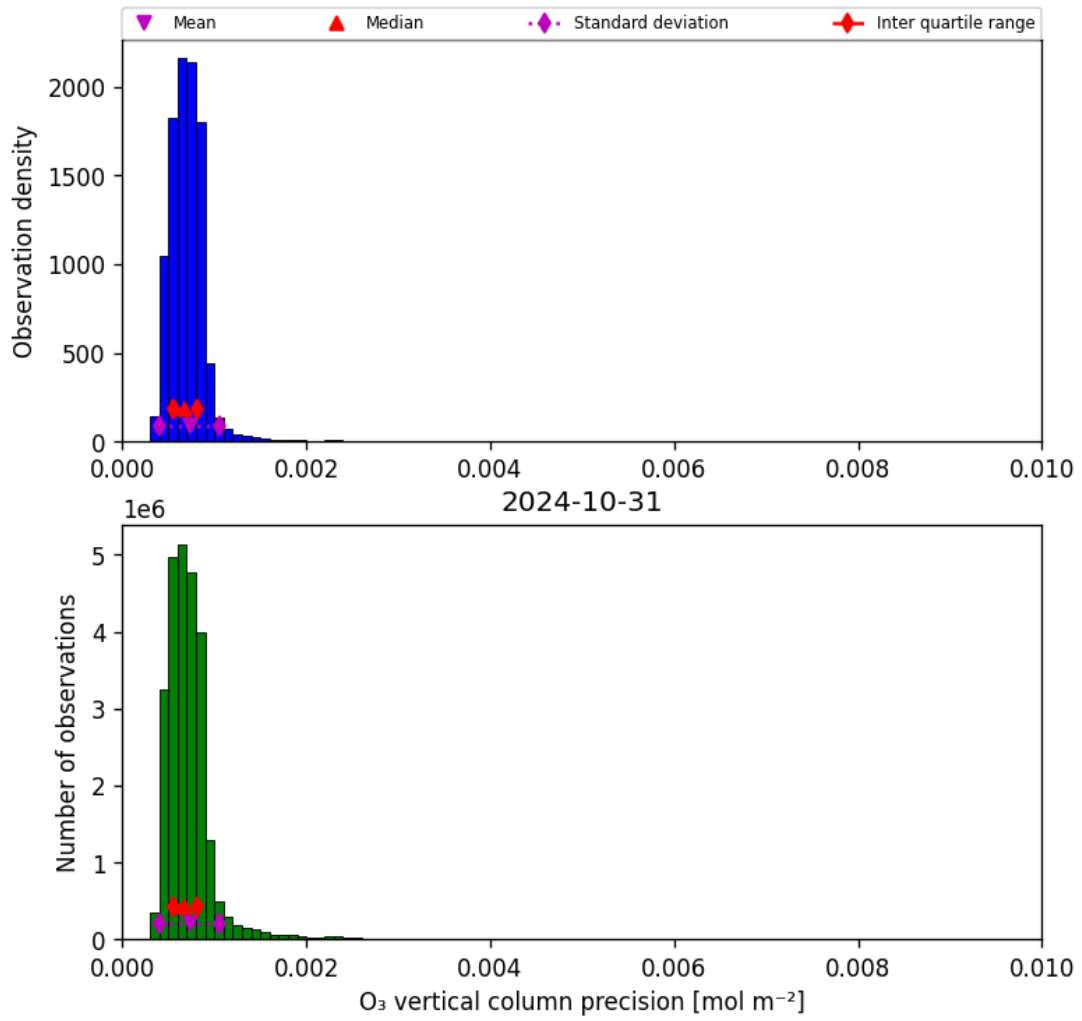
Figure 22: Histogram of “O 3 vertical column precision” for 2024-10-30 to 2024-11-01
