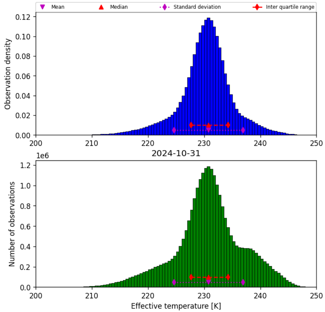
Figure 24: Histogram of “Effective temperature” for 2024-10-30 to 2024-11-01
