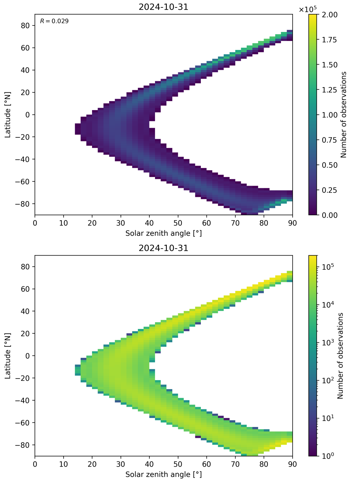
Figure 44: Scatter density plot of “Solar zenith angle” against “Latitude” for 2024-10-30 to 2024-11-01.
