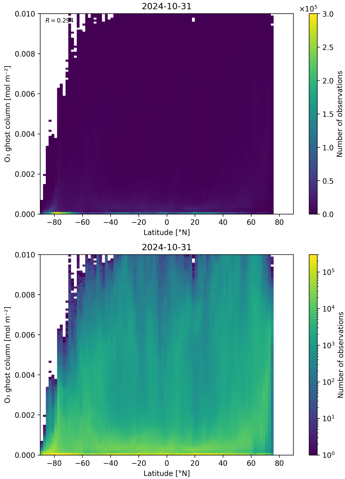
Figure 35: Scatter density plot of “Latitude” against “O 3 ghost column” for 2024-10-30 to 2024-11-01.
