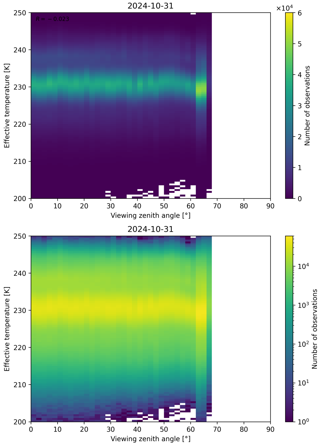
Figure 50: Scatter density plot of “Viewing zenith angle” against “Effective temperature” for 2024-10-30 to 2024-11-01.
