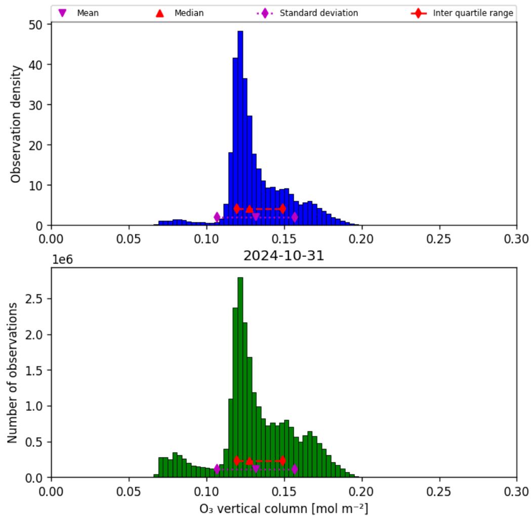
Figure 21: Histogram of “O 3 vertical column” for 2024-10-30 to 2024-11-01
