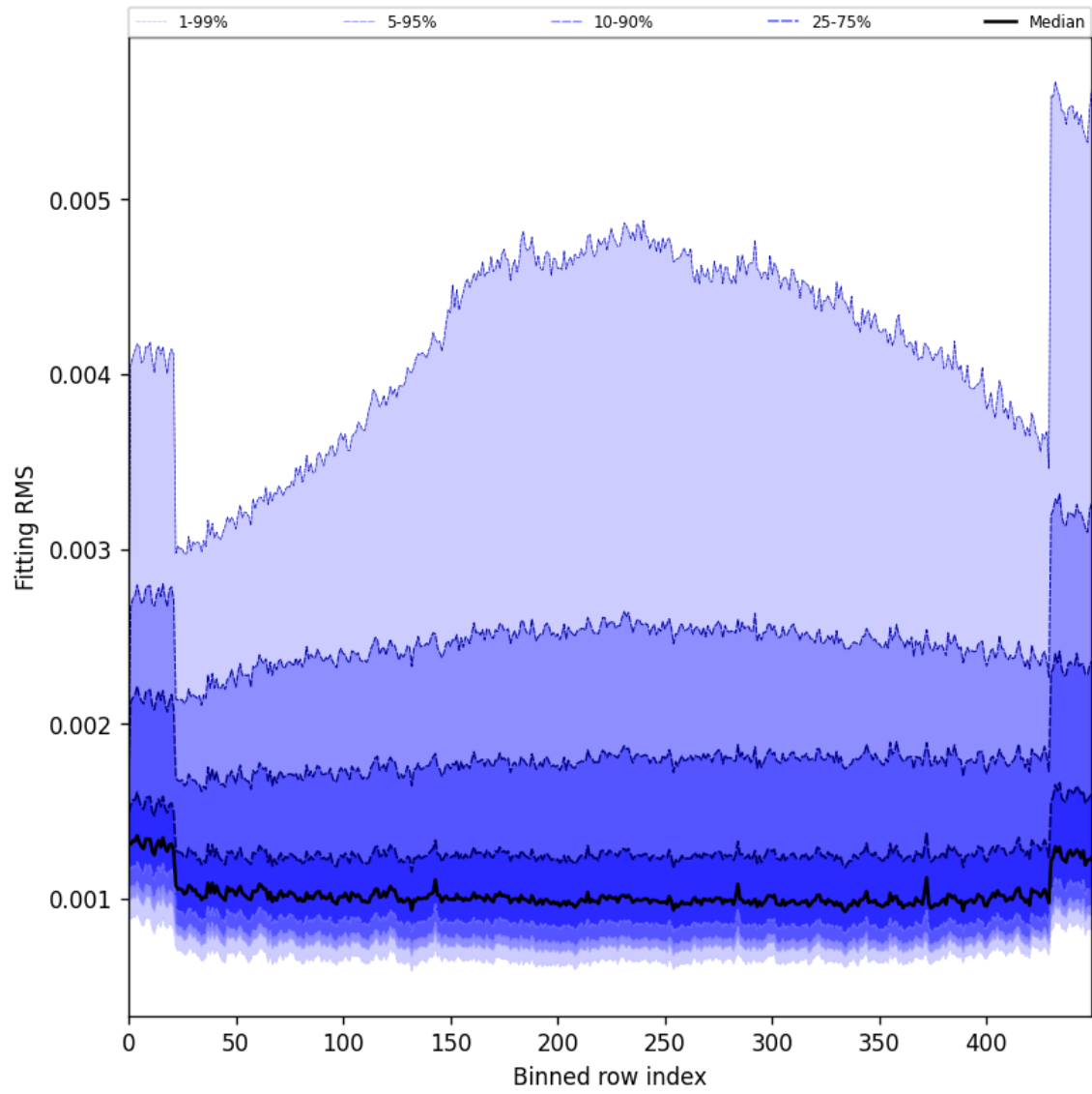
Figure 30: Along track statistics of “Fitting RMS” for 2024-10-30 to 2024-11-01
