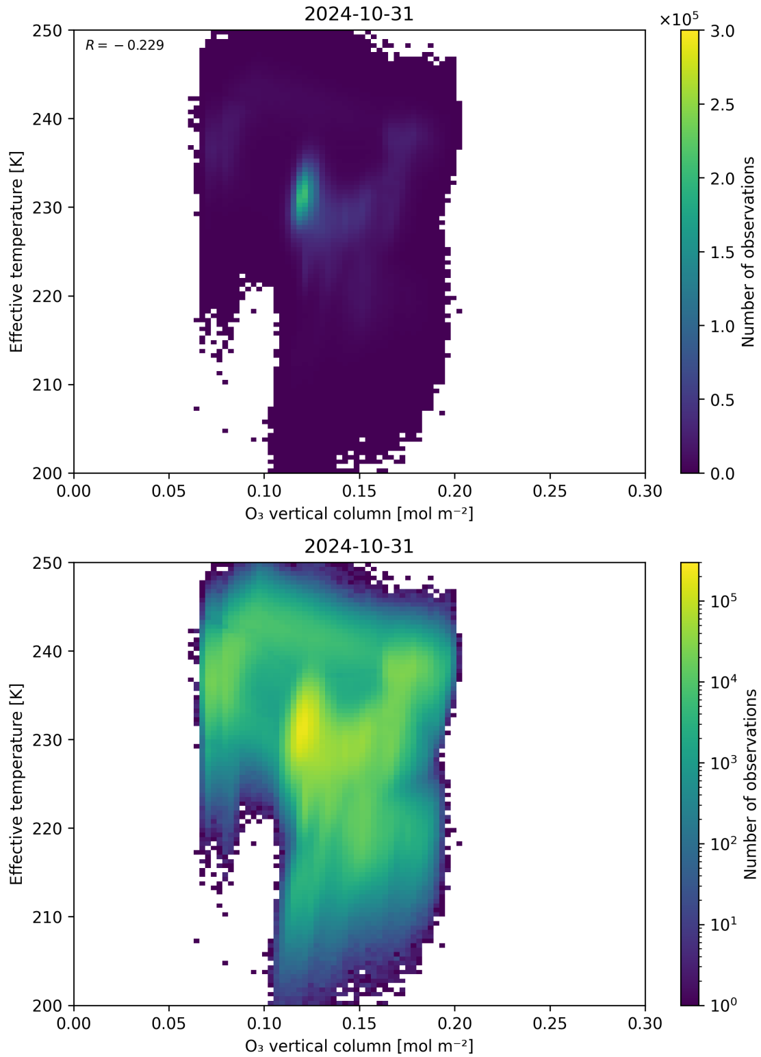
Figure 39: Scatter density plot of “O 3 vertical column” against “Effective temperature” for 2024-10-30 to 2024-11-01.
