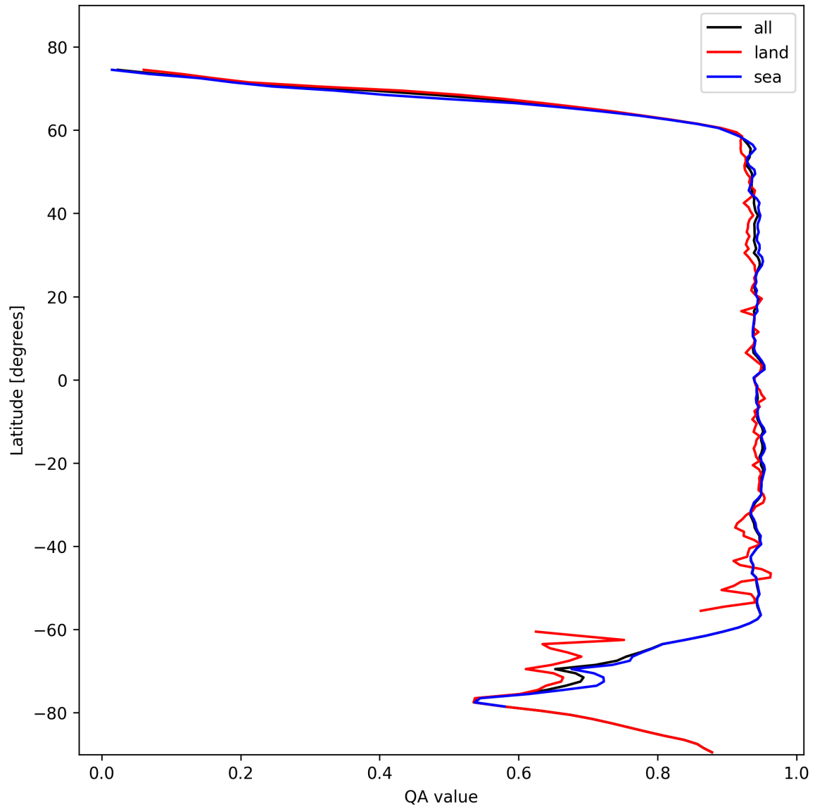
Figure 13: Zonal average of “QA value” for 2024-10-30 to 2024-11-01.
