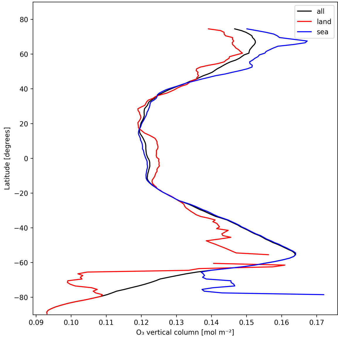
Figure 14: Zonal average of “O 3 vertical column” for 2024-10-30 to 2024-11-01.
