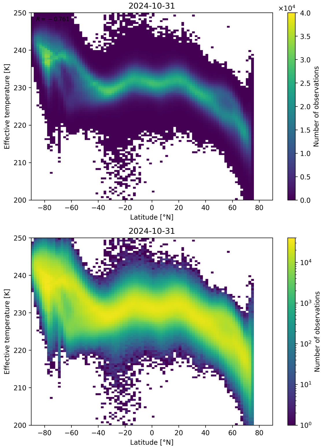
Figure 34: Scatter density plot of “Latitude” against “Effective temperature” for 2024-10-30 to 2024-11-01.
