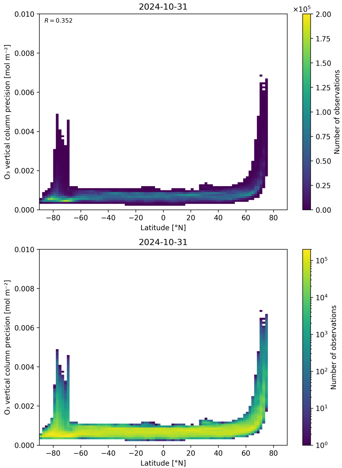
Figure 37: Scatter density plot of “Latitude” against “O 3 vertical column precision” for 2024-10-30 to 2024-11-01.
