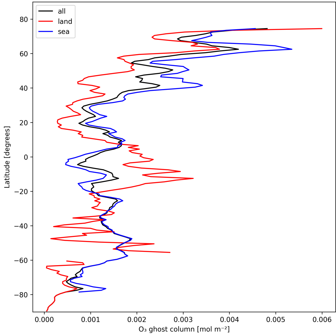
Figure 18: Zonal average of “O 3 ghost column” for 2024-10-30 to 2024-11-01.
