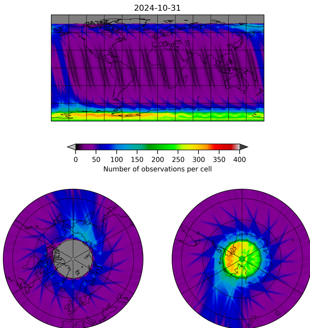
Figure 12: Map of the number of observations for 2024-10-30 to 2024-11-01
