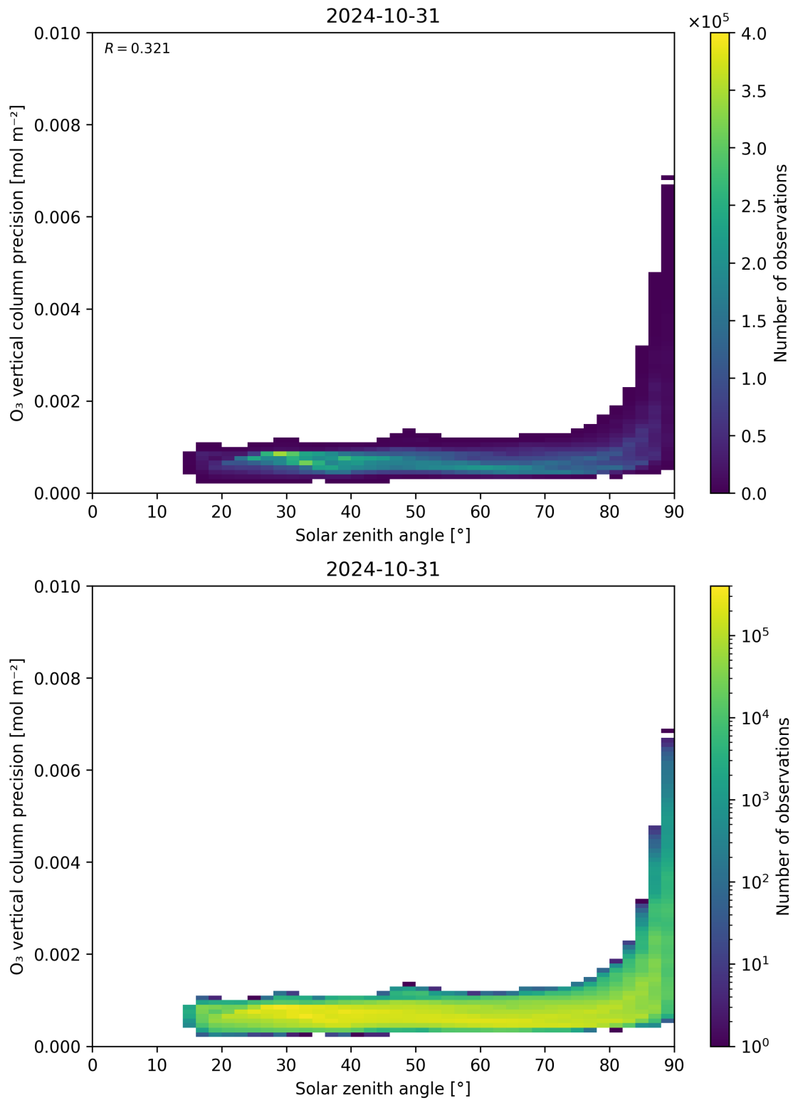
Figure 48: Scatter density plot of “Solar zenith angle” against “O 3 vertical column precision” for 2024-10-30 to 2024-11-01.
