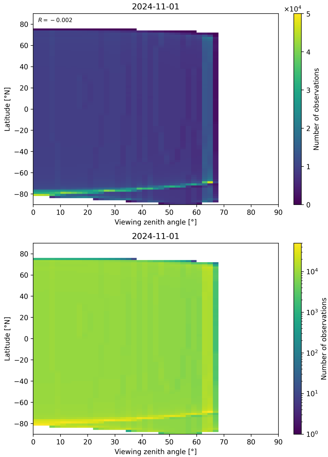
Figure 49: Scatter density plot of “Viewing zenith angle” against “Latitude” for 2024-10-31 to 2024-11-02.
