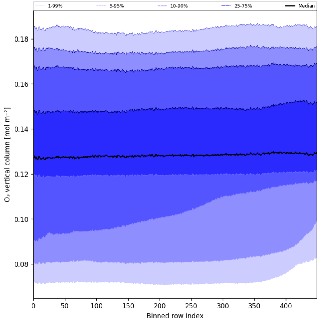
Figure 28: Along track statistics of “O 3 vertical column” for 2024-10-31 to 2024-11-02
