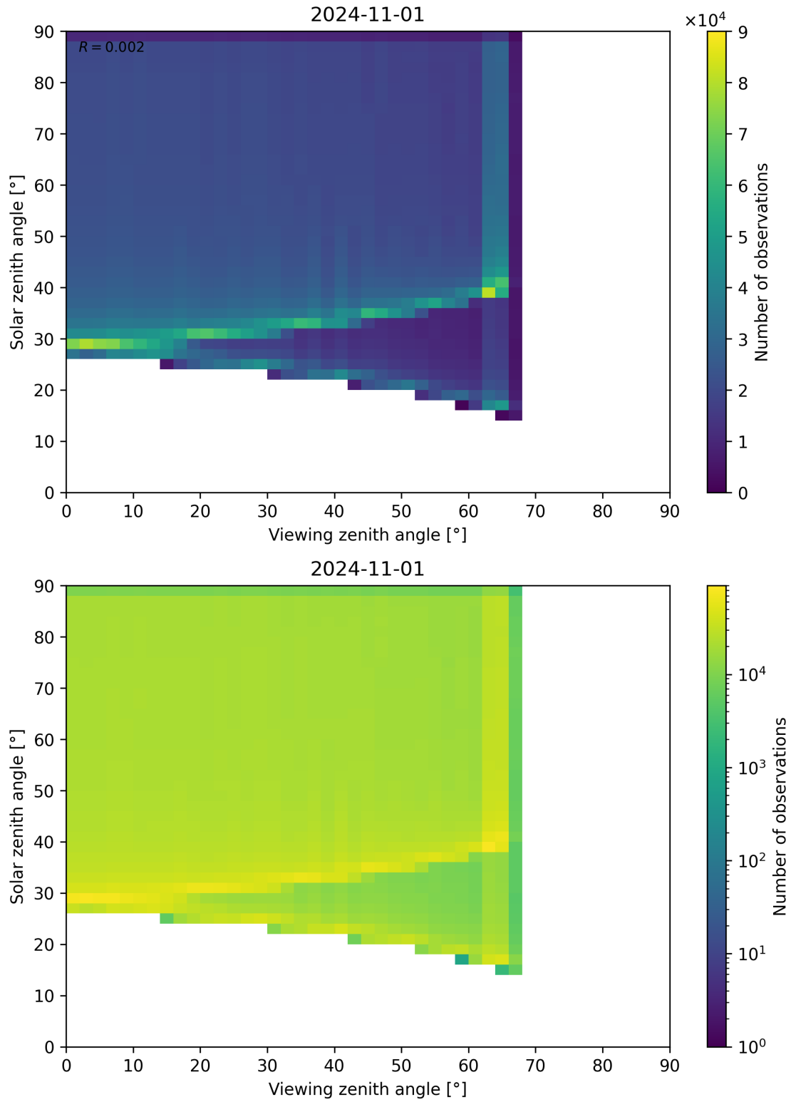
Figure 54: Scatter density plot of “Viewing zenith angle” against “Solar zenith angle” for 2024-10-31 to 2024-11-02.
