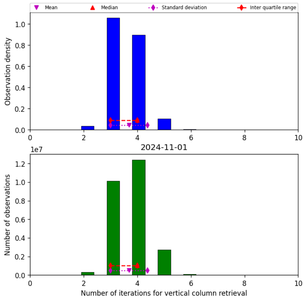
Figure 26: Histogram of “Number of iterations for vertical column retrieval” for 2024-10-31 to 2024-11-02
