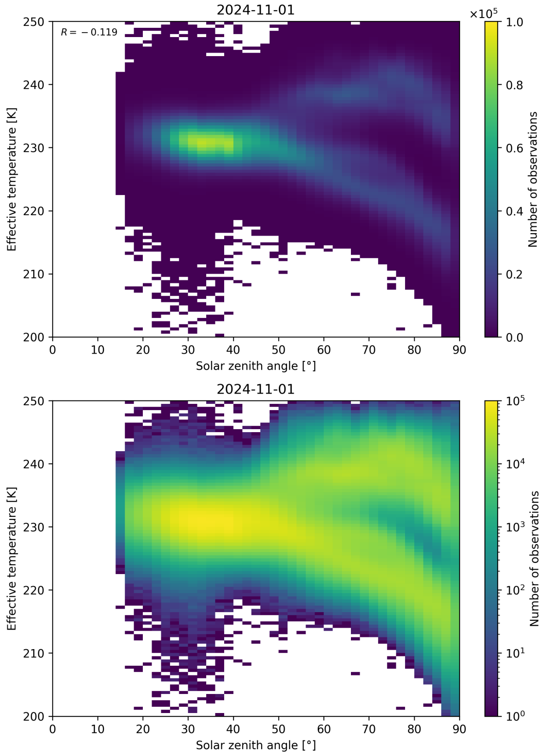
Figure 45: Scatter density plot of “Solar zenith angle” against “Effective temperature” for 2024-10-31 to 2024-11-02.
