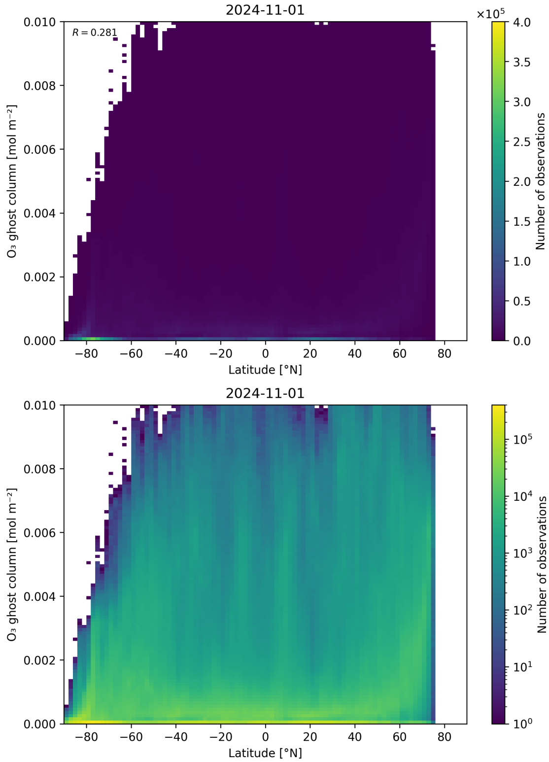
Figure 35: Scatter density plot of “Latitude” against “O 3 ghost column” for 2024-10-31 to 2024-11-02.
