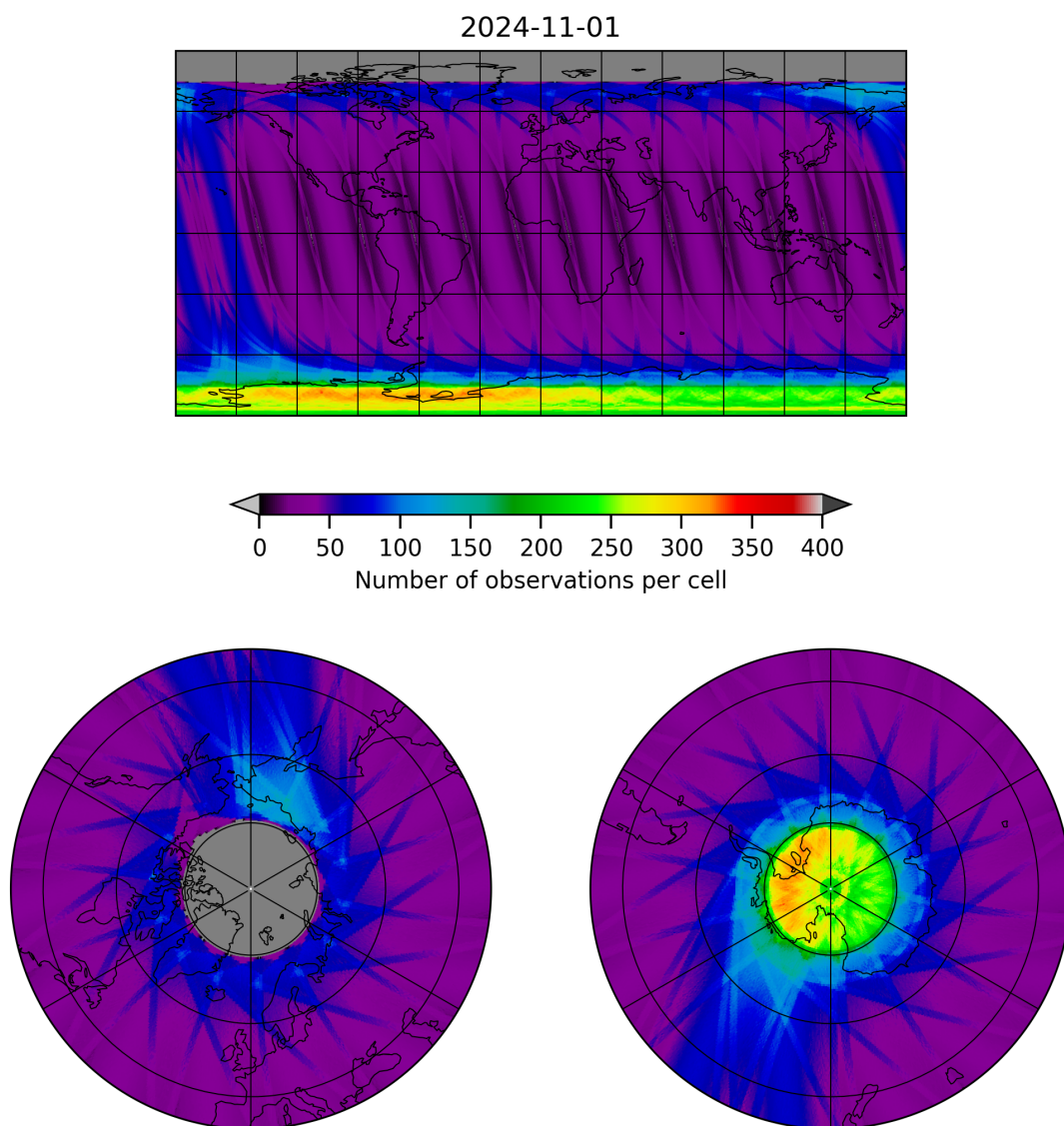
Figure 12: Map of the number of observations for 2024-10-31 to 2024-11-02
