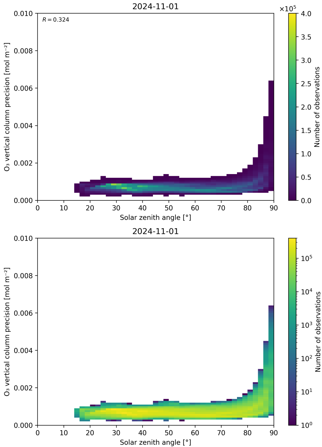
Figure 48: Scatter density plot of “Solar zenith angle” against “O 3 vertical column precision” for 2024-10-31 to 2024-11-02.
