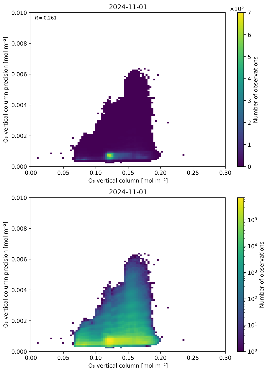
Figure 41: Scatter density plot of “O 3 vertical column” against “O 3 vertical column precision” for 2024-10-31 to 2024-11-02.
