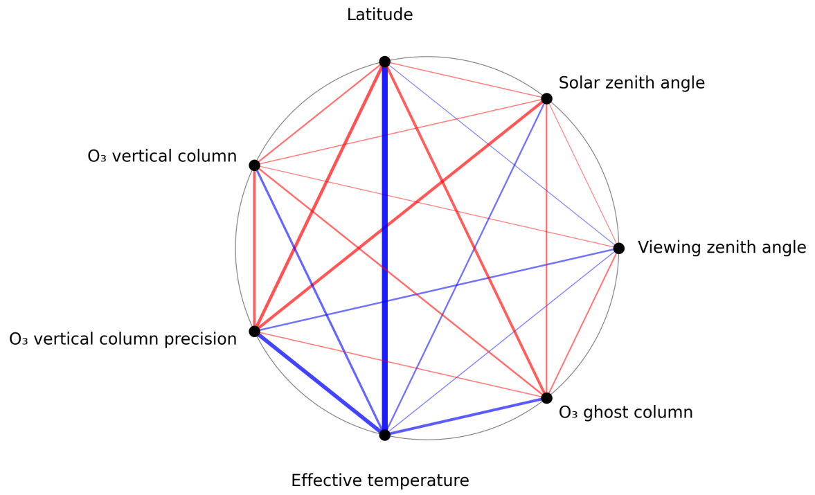
Figure 1: Map of correlation graph for 2024-10-31 to 2024-11-02.
