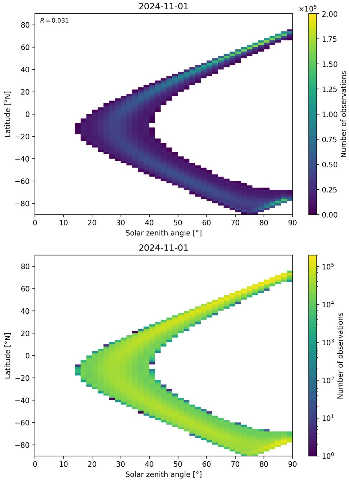
Figure 44: Scatter density plot of “Solar zenith angle” against “Latitude” for 2024-10-31 to 2024-11-02.
