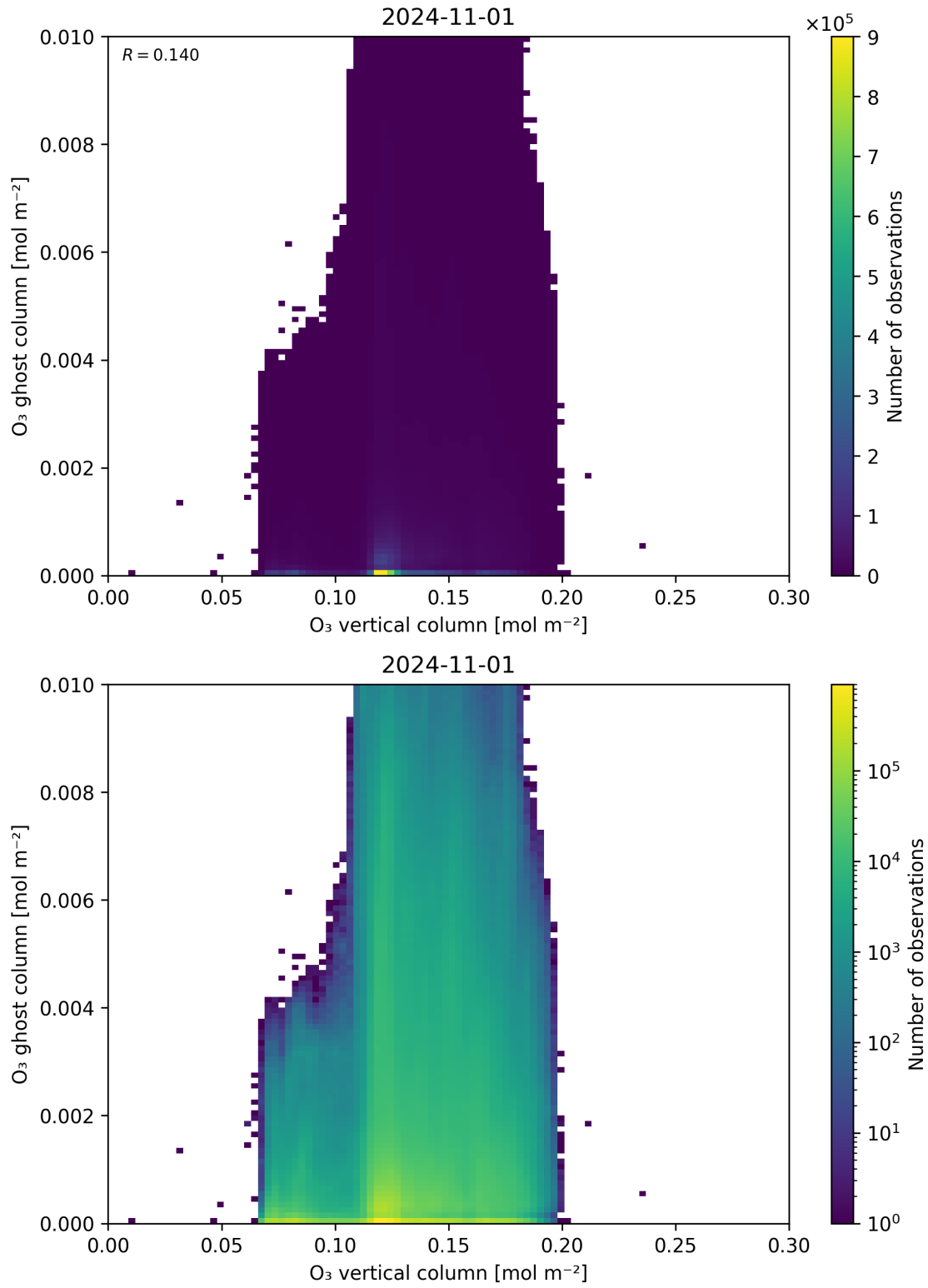
Figure 40: Scatter density plot of “O 3 vertical column” against “O 3 ghost column” for 2024-10-31 to 2024-11-02.
