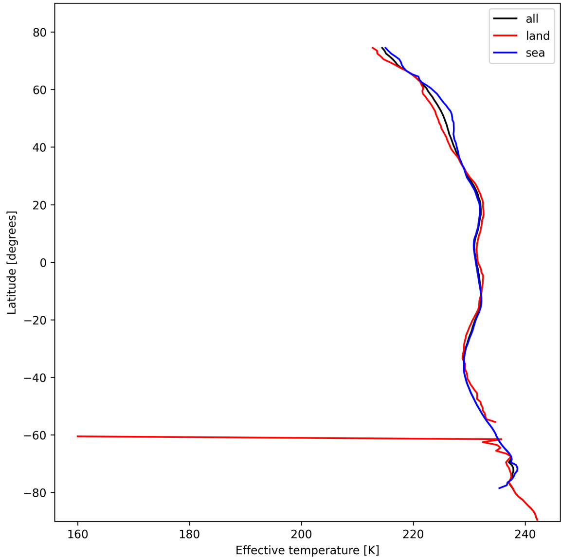
Figure 17: Zonal average of “Effective temperature” for 2024-10-31 to 2024-11-02.
