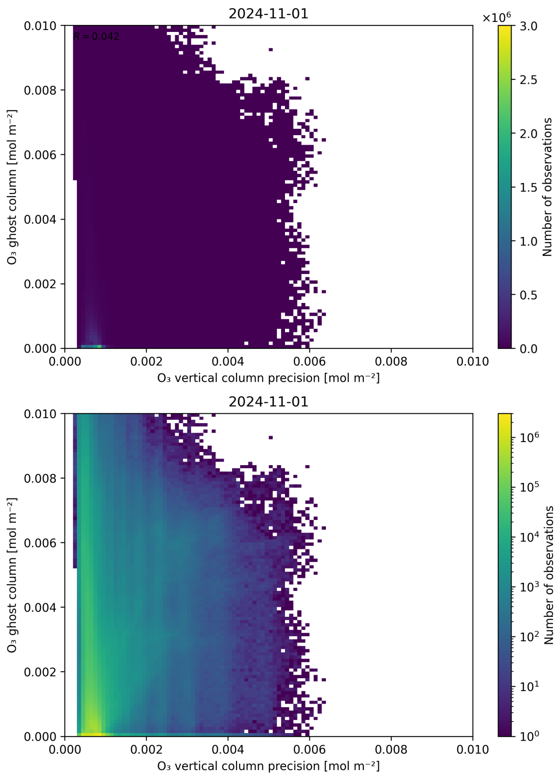
Figure 43: Scatter density plot of “O 3 vertical column precision” against “O 3 ghost column” for 2024-10-31 to 2024-11-02.
