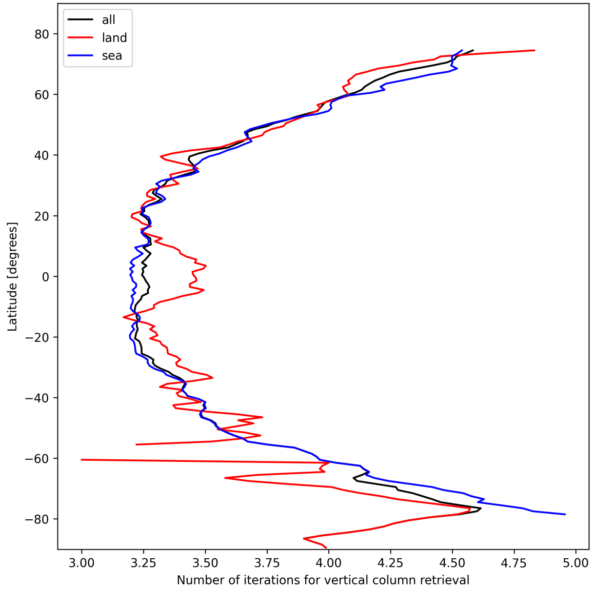
Figure 19: Zonal average of “Number of iterations for vertical column retrieval” for 2024-10-31 to 2024-11-02.
