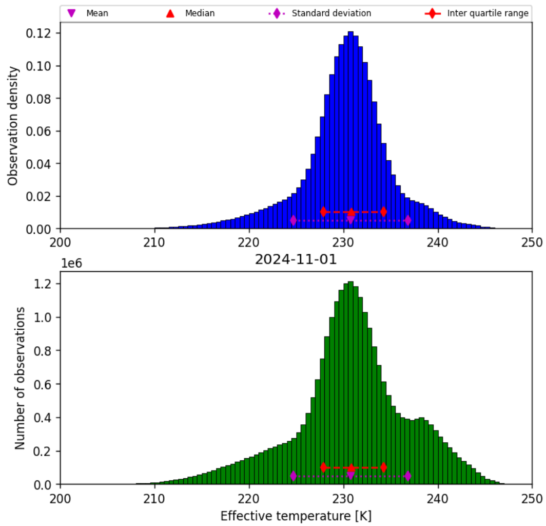
Figure 24: Histogram of “Effective temperature” for 2024-10-31 to 2024-11-02
