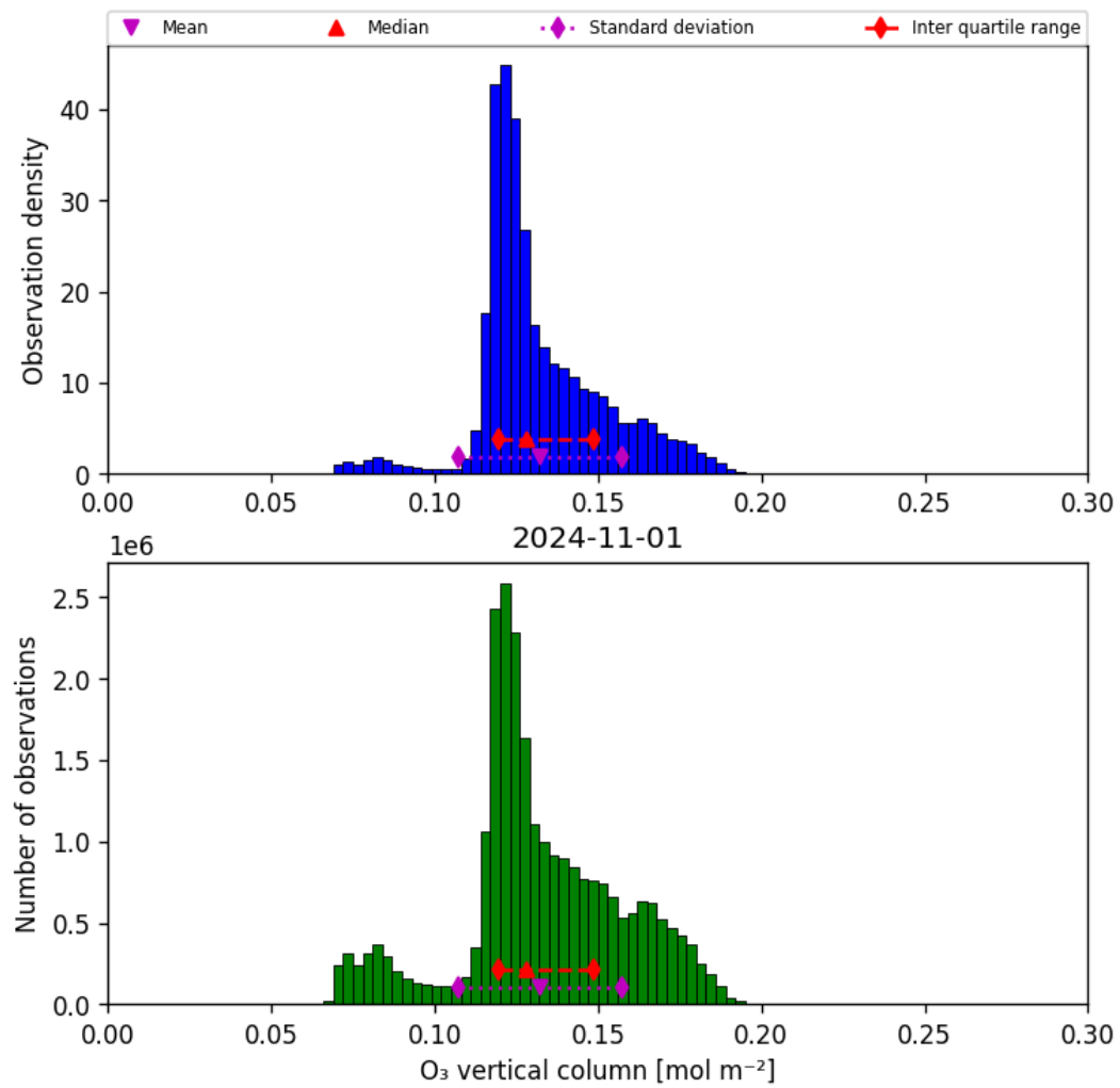
Figure 21: Histogram of “O 3 vertical column” for 2024-10-31 to 2024-11-02
