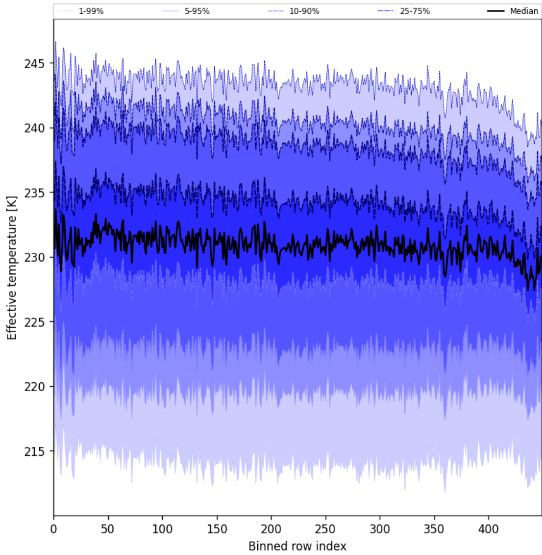
Figure 31: Along track statistics of “Effective temperature” for 2024-10-31 to 2024-11-02
