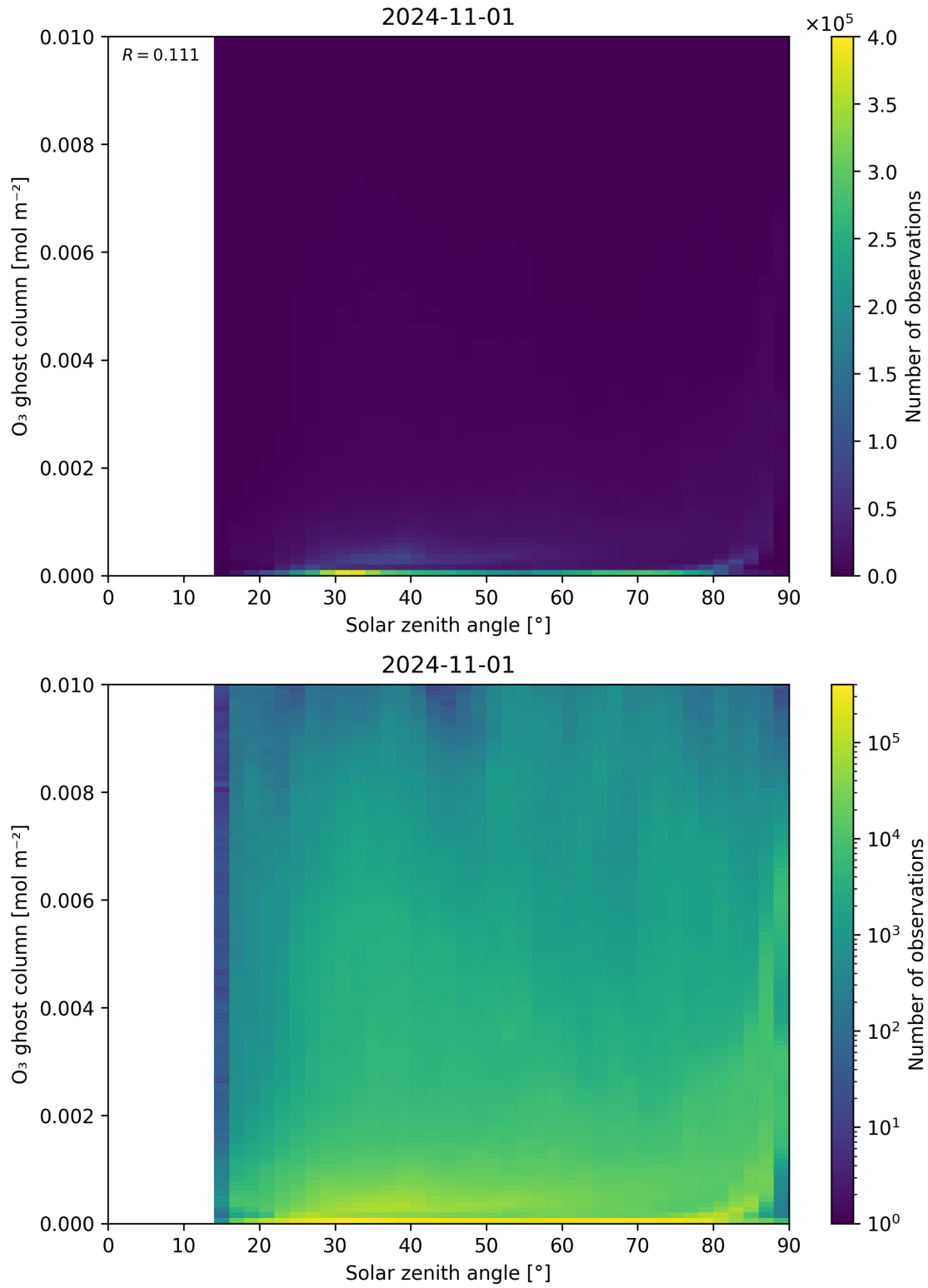
Figure 46: Scatter density plot of “Solar zenith angle” against “O 3 ghost column” for 2024-10-31 to 2024-11-02.
