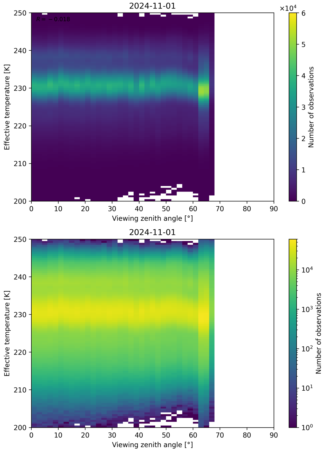
Figure 50: Scatter density plot of “Viewing zenith angle” against “Effective temperature” for 2024-10-31 to 2024-11-02.
