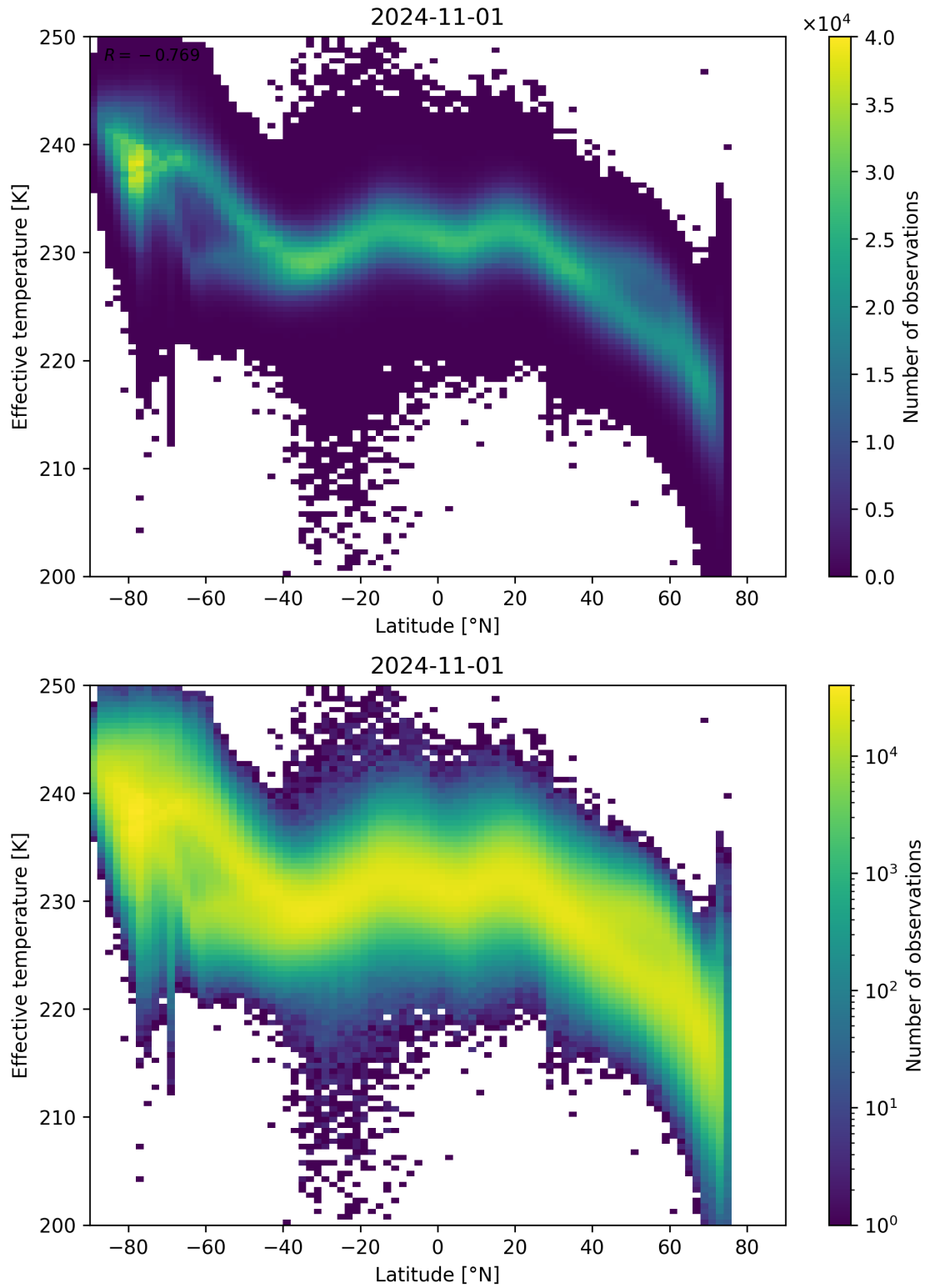
Figure 34: Scatter density plot of “Latitude” against “Effective temperature” for 2024-10-31 to 2024-11-02.
