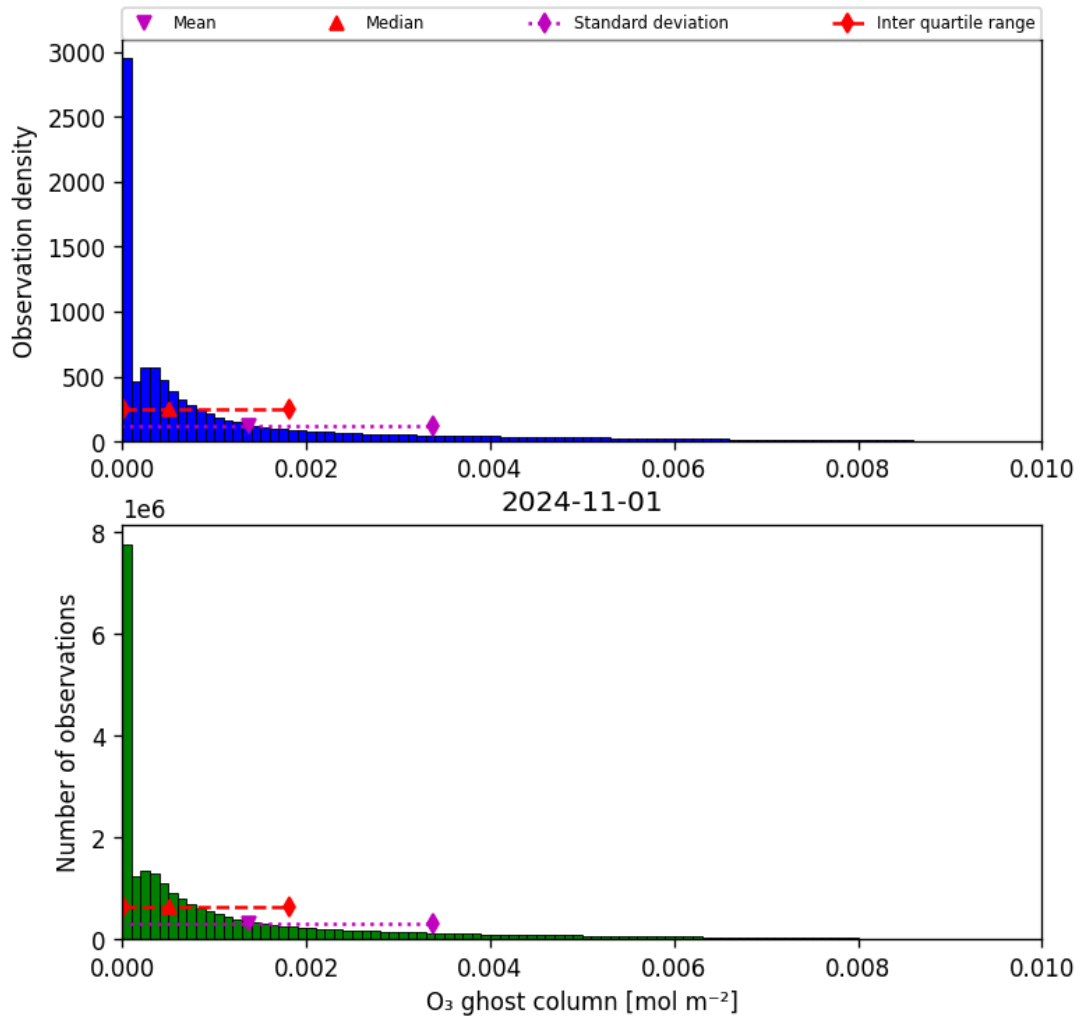
Figure 25: Histogram of “O 3 ghost column” for 2024-10-31 to 2024-11-02
