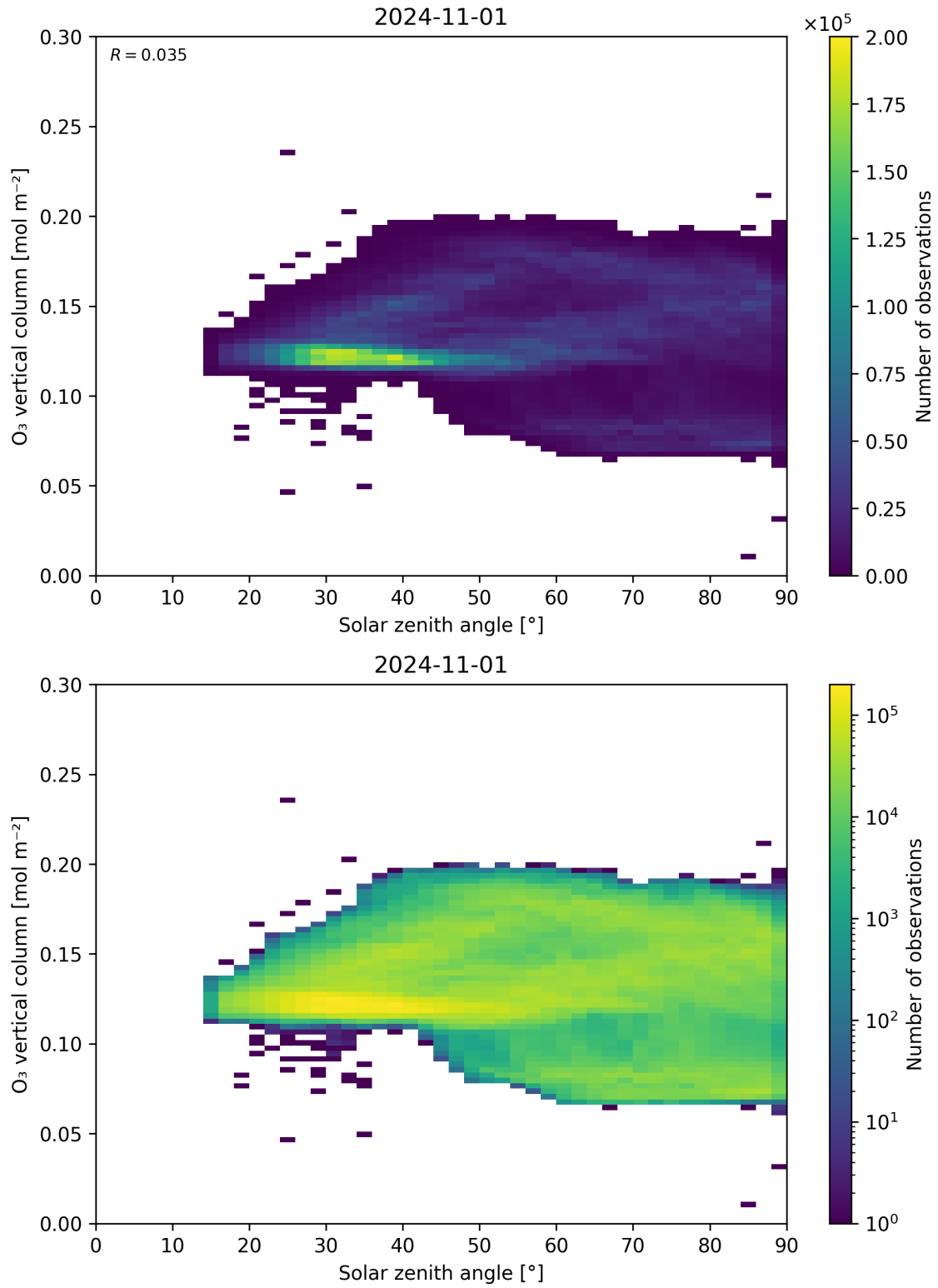
Figure 47: Scatter density plot of “Solar zenith angle” against “O 3 vertical column” for 2024-10-31 to 2024-11-02.
