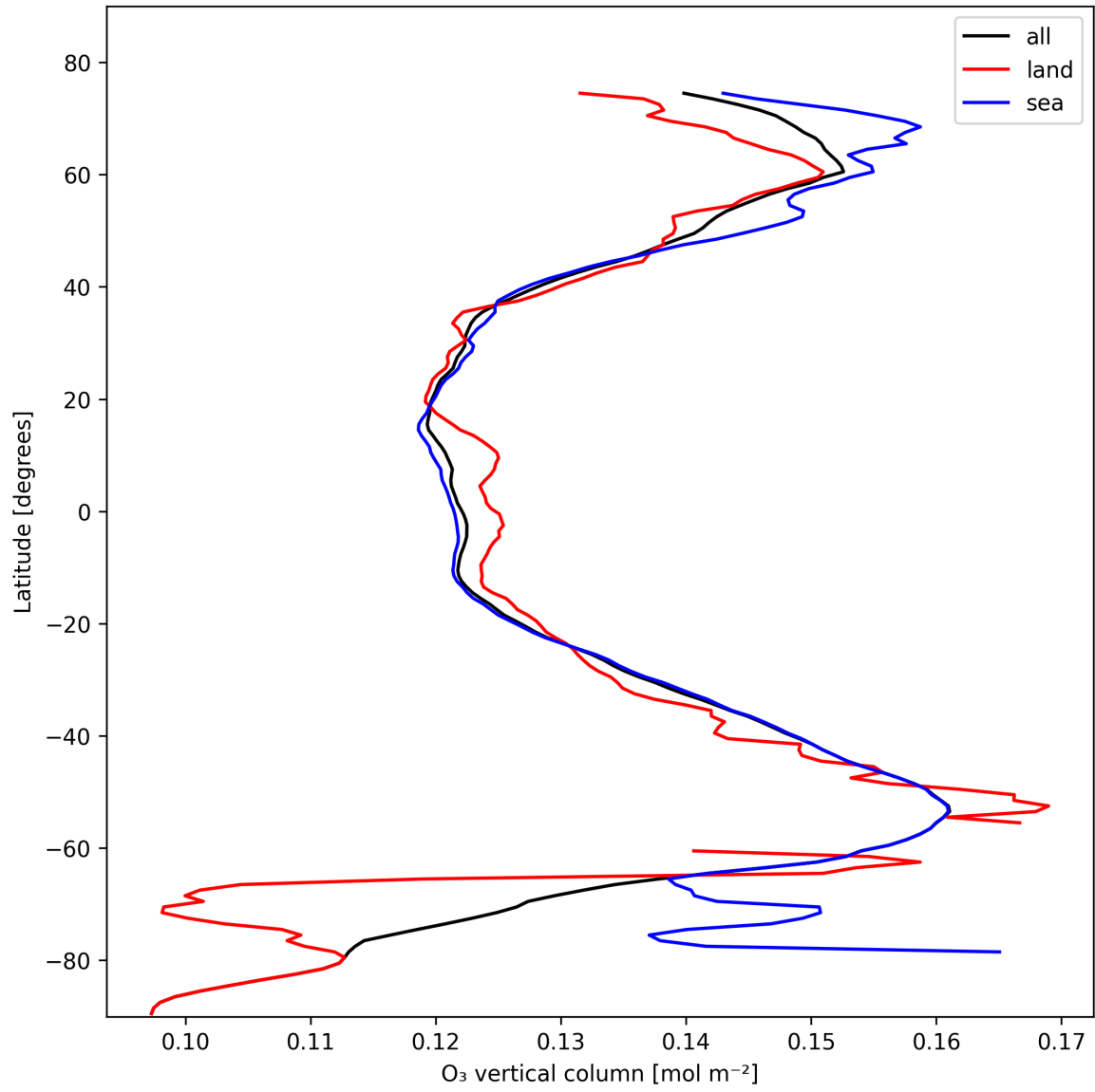
Figure 14: Zonal average of “O 3 vertical column” for 2024-10-31 to 2024-11-02.
