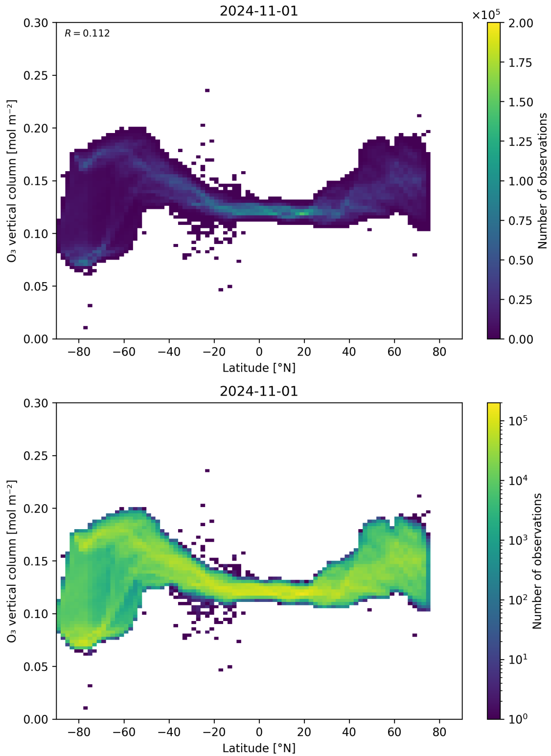
Figure 36: Scatter density plot of “Latitude” against “O 3 vertical column” for 2024-10-31 to 2024-11-02.
