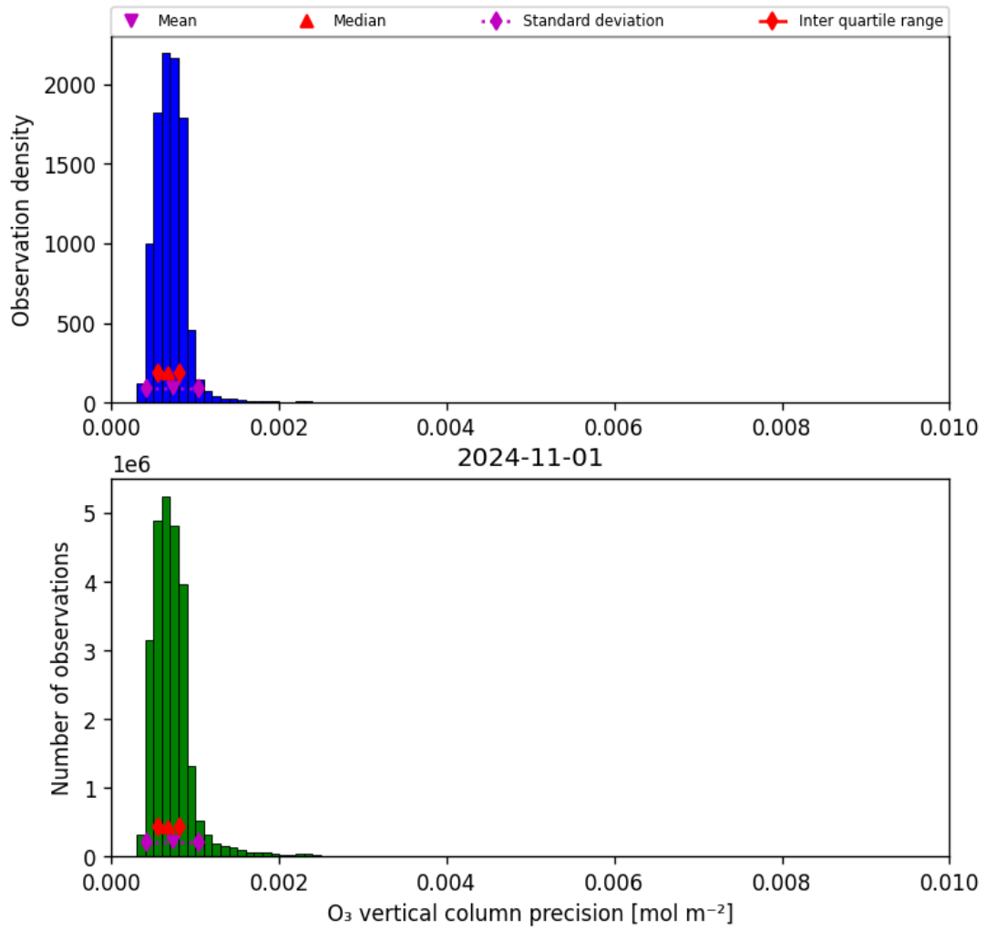
Figure 22: Histogram of “O 3 vertical column precision” for 2024-10-31 to 2024-11-02
