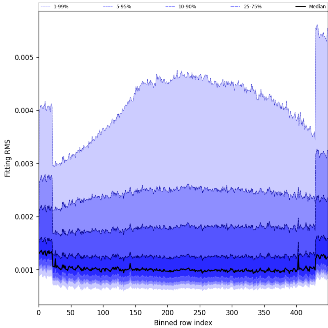
Figure 30: Along track statistics of “Fitting RMS” for 2024-10-31 to 2024-11-02
