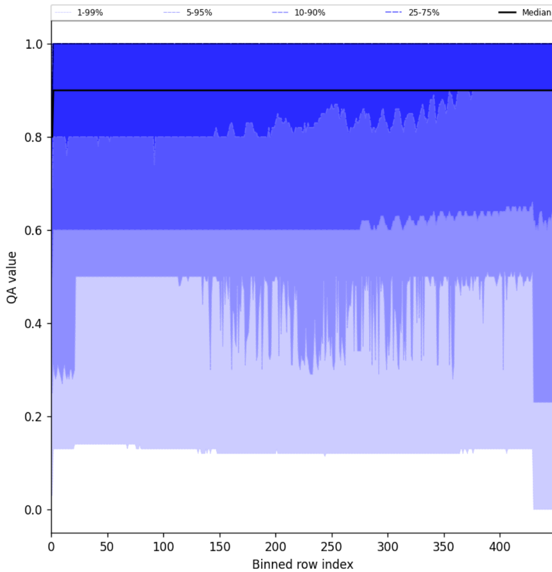
Figure 27: Along track statistics of “QA value” for 2024-10-31 to 2024-11-02
