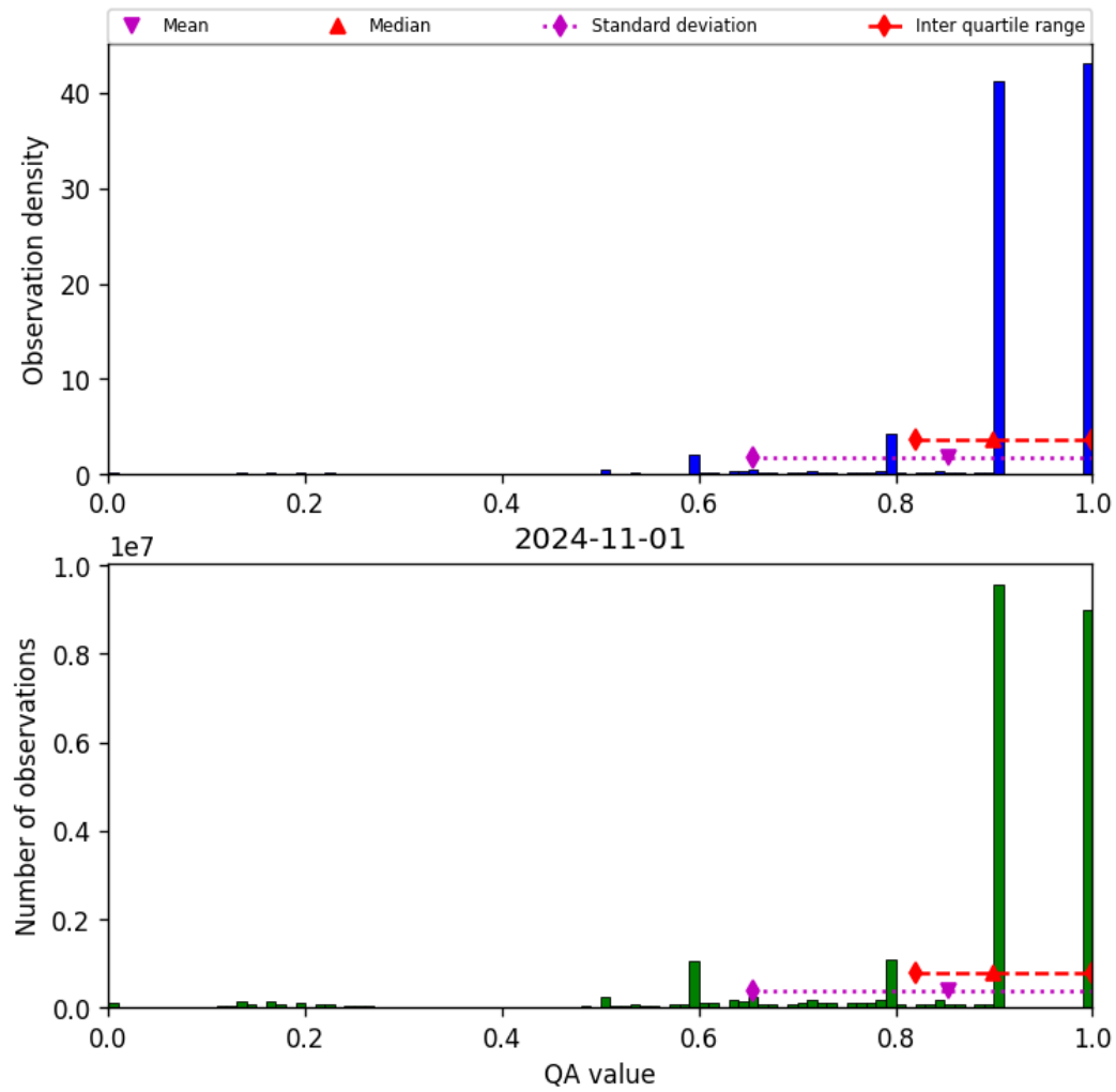
Figure 20: Histogram of “QA value” for 2024-10-31 to 2024-11-02
