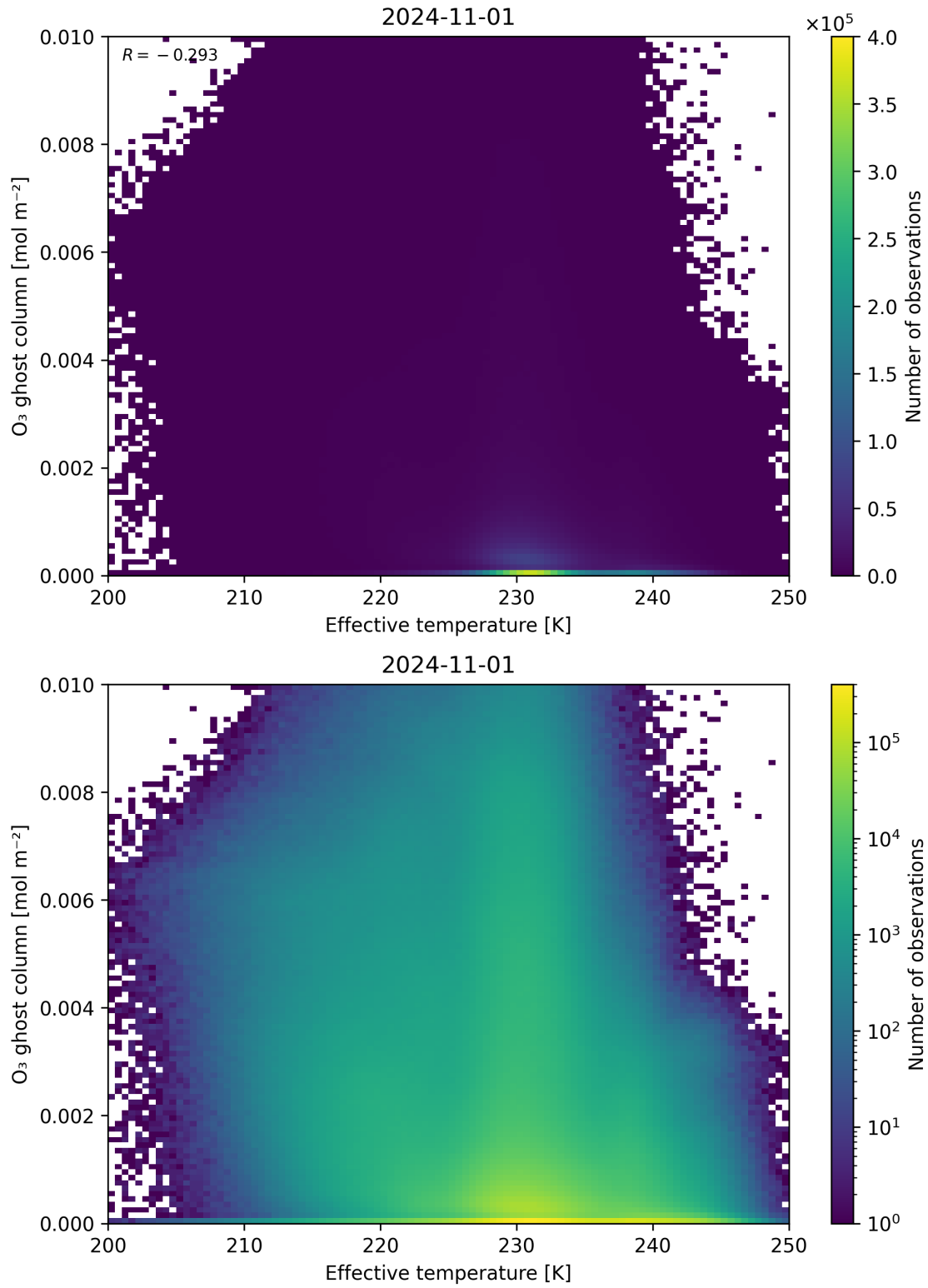
Figure 38: Scatter density plot of “Effective temperature” against “O 3 ghost column” for 2024-10-31 to 2024-11-02.
