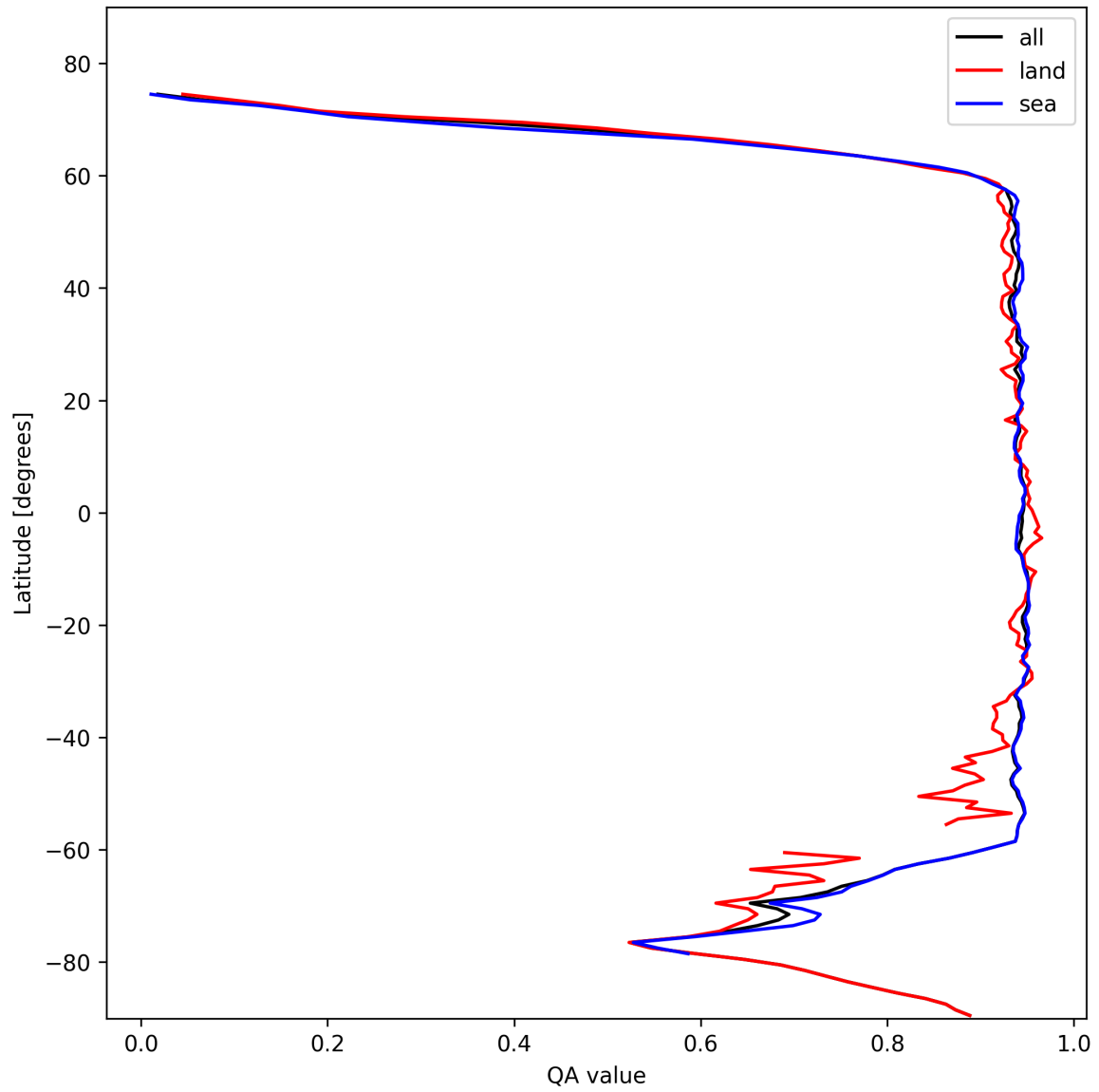
Figure 13: Zonal average of “QA value” for 2024-10-31 to 2024-11-02.
