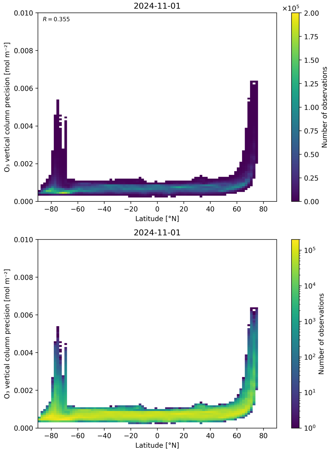
Figure 37: Scatter density plot of “Latitude” against “O 3 vertical column precision” for 2024-10-31 to 2024-11-02.
