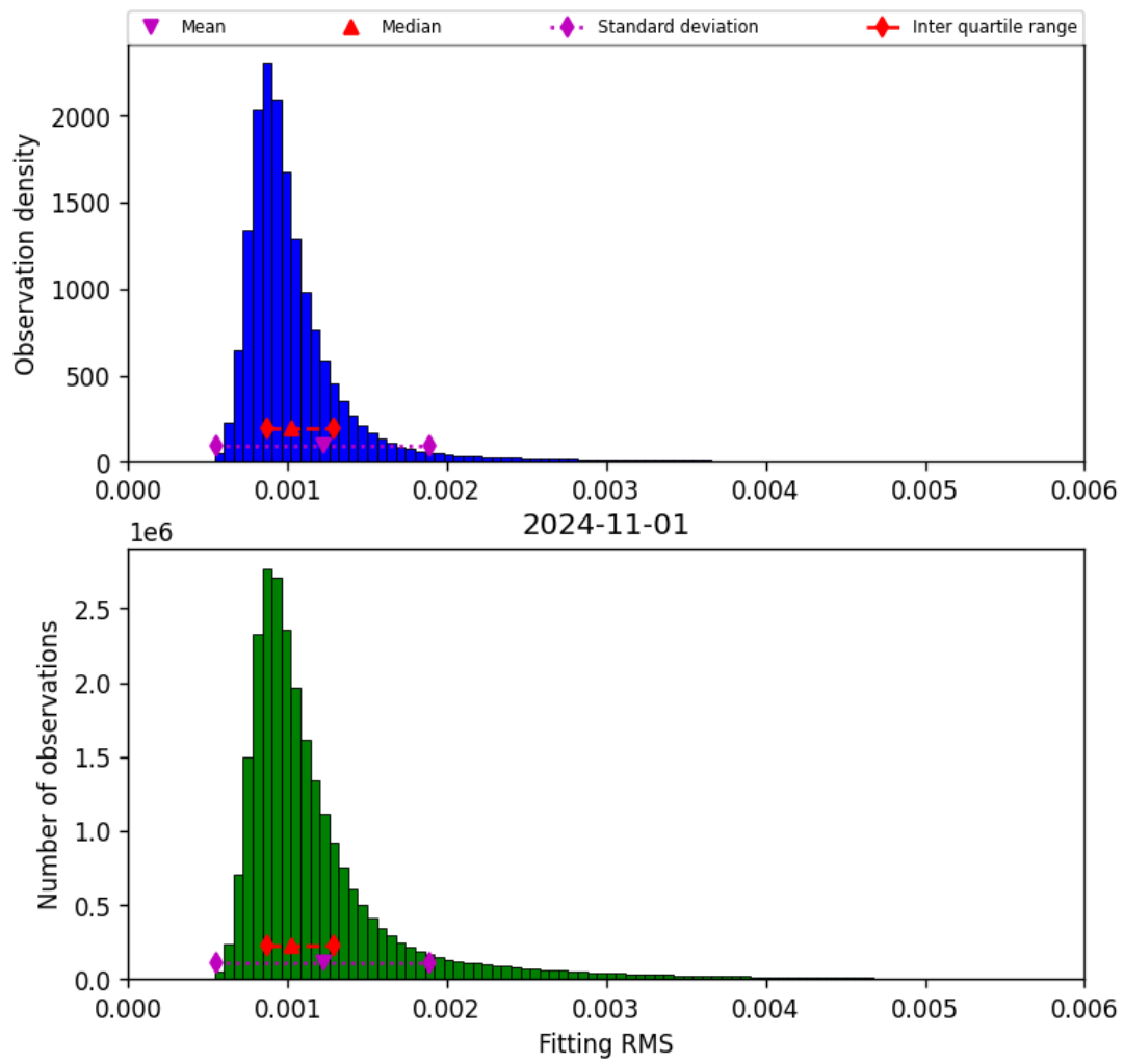
Figure 23: Histogram of “Fitting RMS” for 2024-10-31 to 2024-11-02
