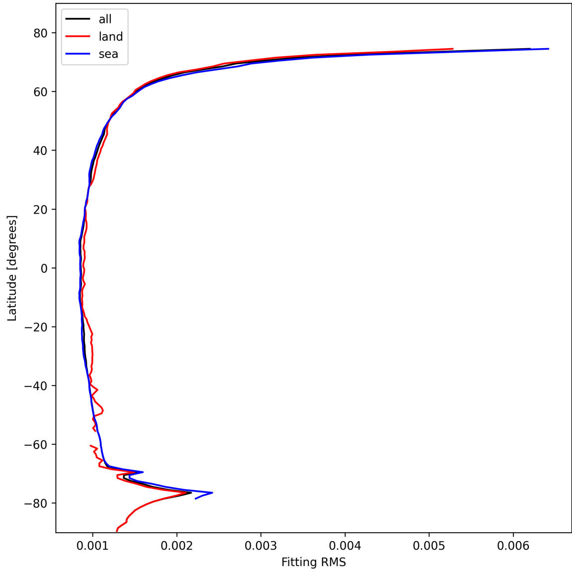
Figure 16: Zonal average of “Fitting RMS” for 2024-10-31 to 2024-11-02.
