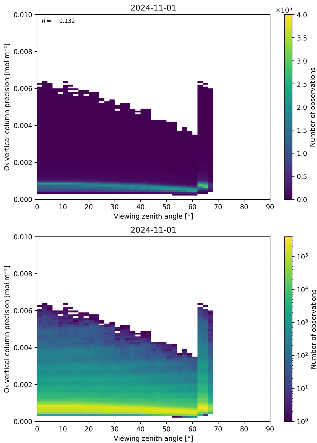
Figure 53: Scatter density plot of “Viewing zenith angle” against “O 3 vertical column precision” for 2024-10-31 to 2024-11-02.
