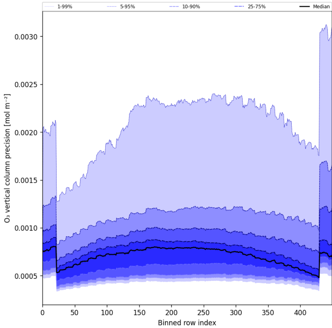
Figure 29: Along track statistics of “O 3 vertical column precision” for 2024-10-31 to 2024-11-02
