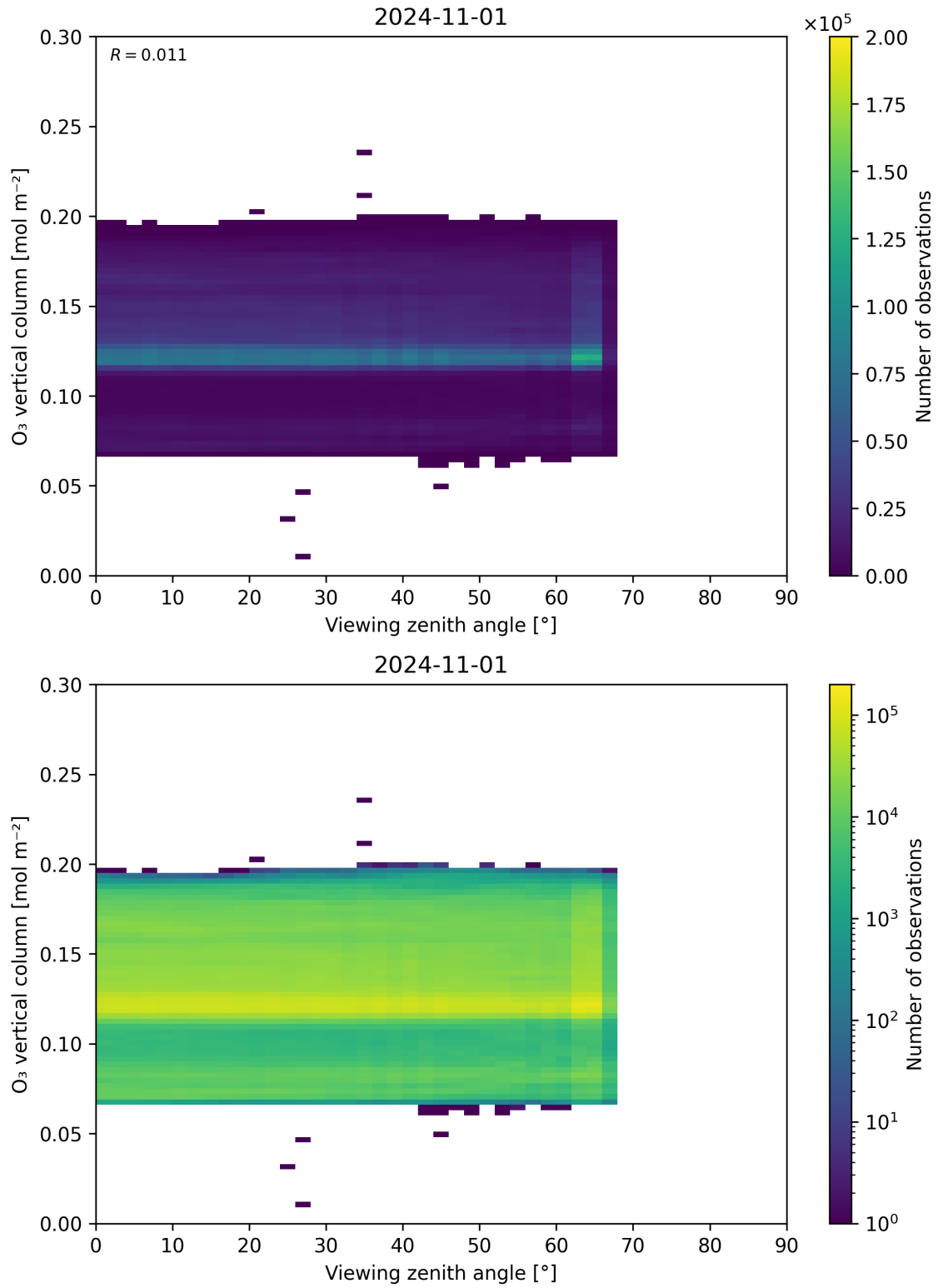
Figure 52: Scatter density plot of “Viewing zenith angle” against “O 3 vertical column” for 2024-10-31 to 2024-11-02.
