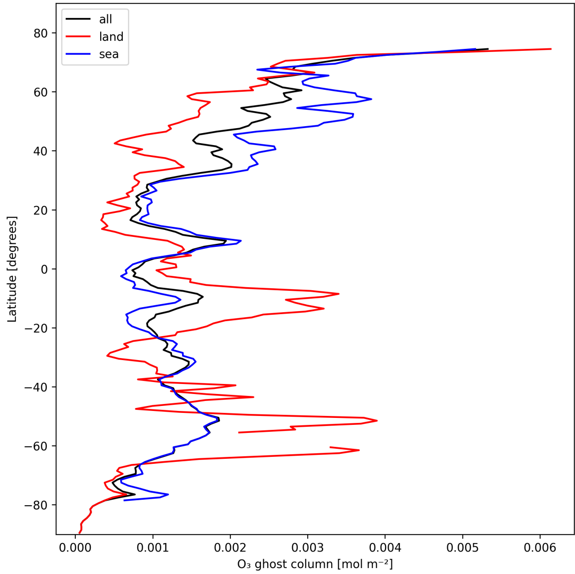
Figure 18: Zonal average of "O 3 ghost column" for 2024-10-31 to 2024-11-02.
