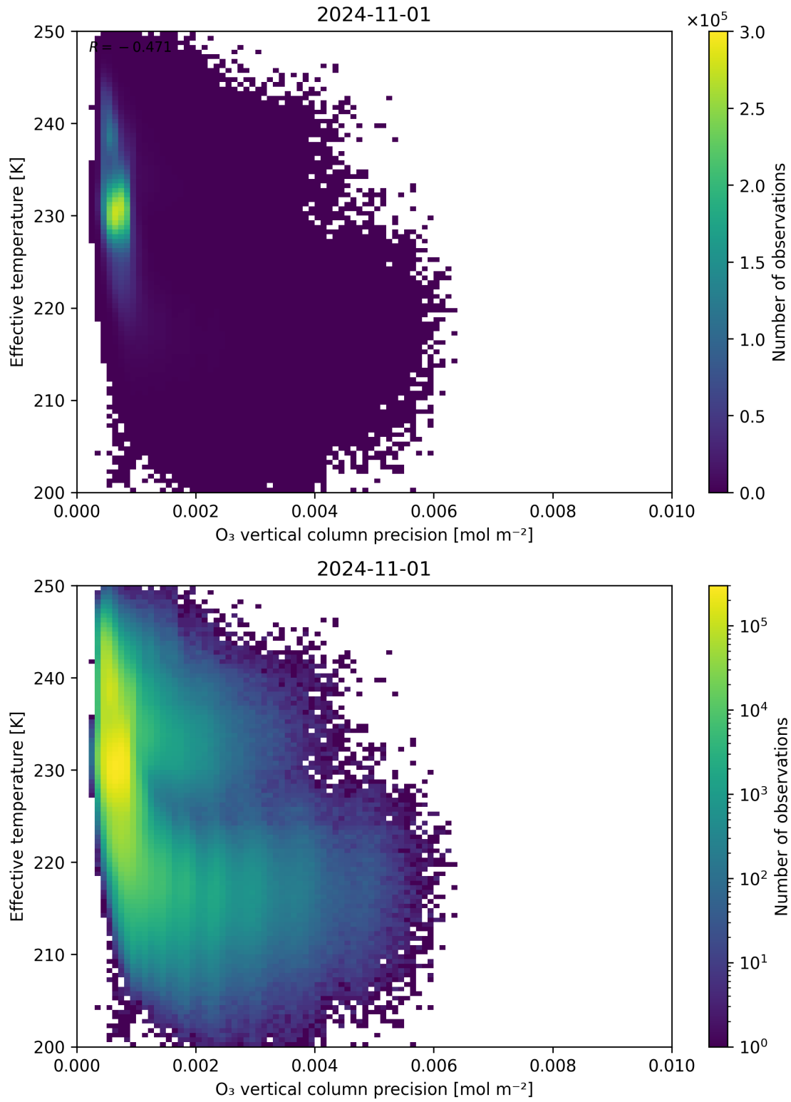
Figure 42: Scatter density plot of “ O_3 vertical column precision” against “Effective temperature” for 2024-10-31 to 2024-11-02.
