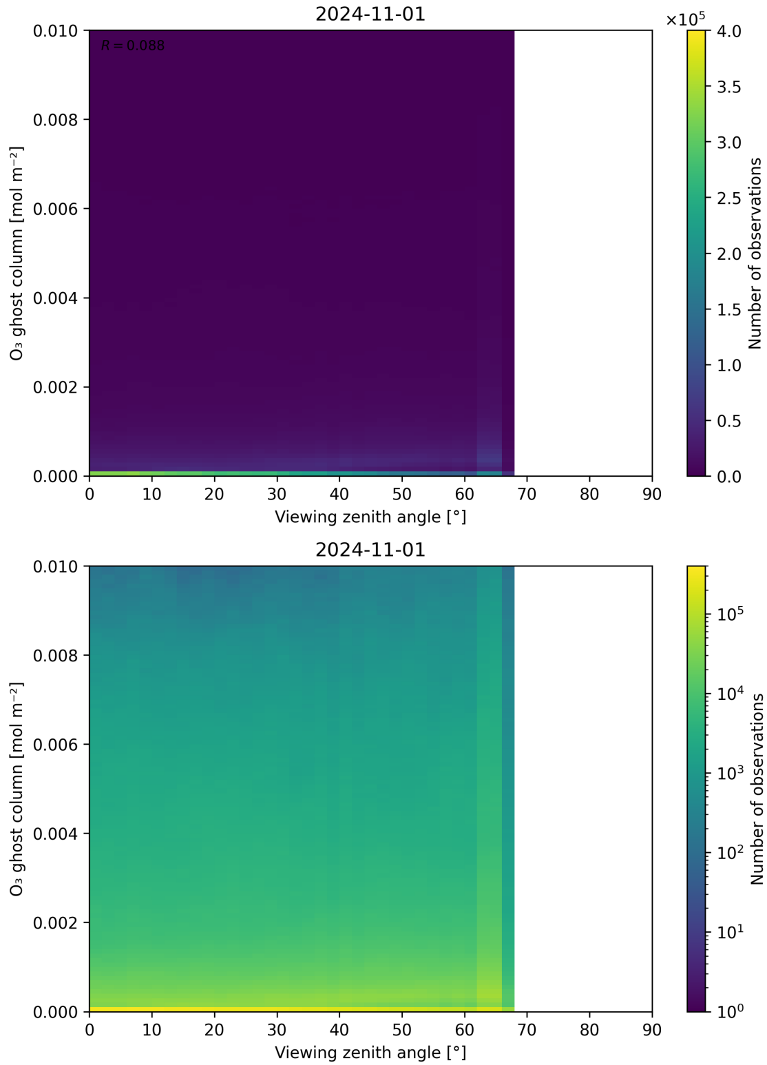
Figure 51: Scatter density plot of “Viewing zenith angle” against “O 3 ghost column” for 2024-10-31 to 2024-11-02.
