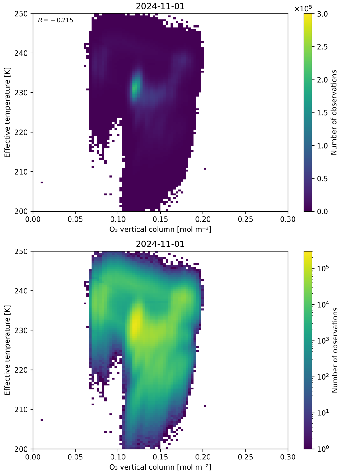
Figure 39: Scatter density plot of “O 3 vertical column” against “Effective temperature” for 2024-10-31 to 2024-11-02.
