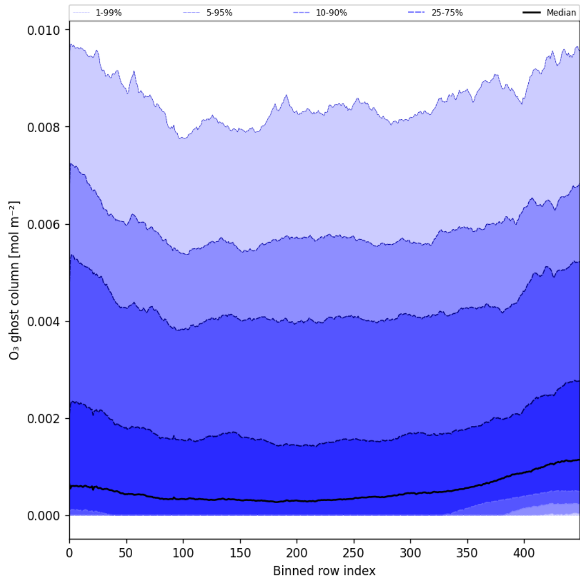
Figure 32: Along track statistics of “O 3 ghost column” for 2024-10-31 to 2024-11-02
