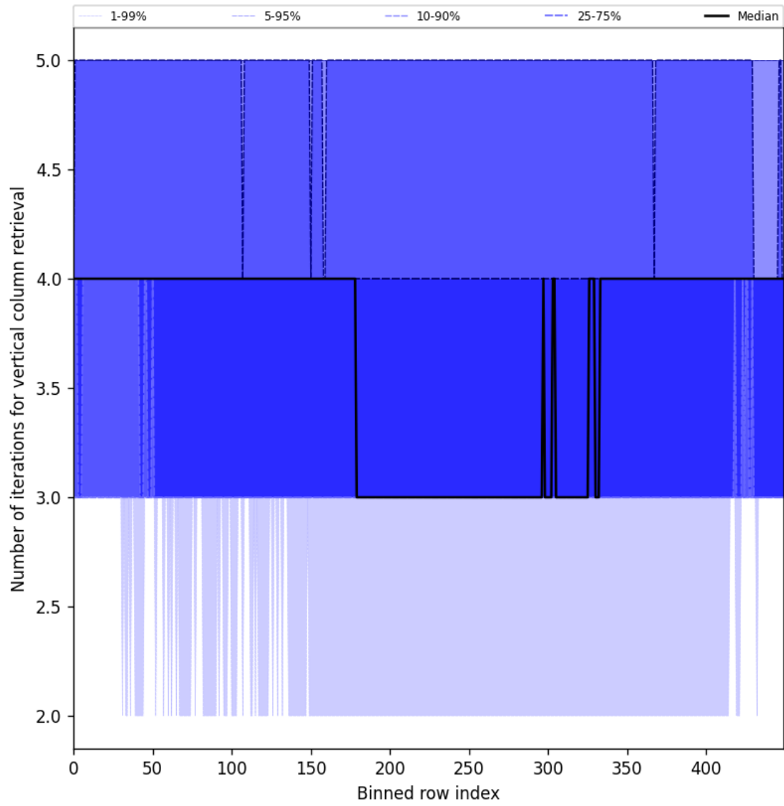
Figure 33: Along track statistics of “Number of iterations for vertical column retrieval” for 2024-10-31 to 2024-11-02
