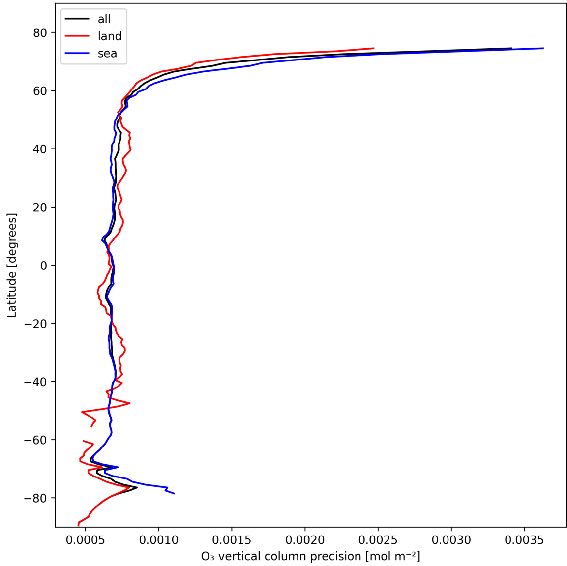
Figure 15: Zonal average of “O 3 vertical column precision” for 2024-10-31 to 2024-11-02.
