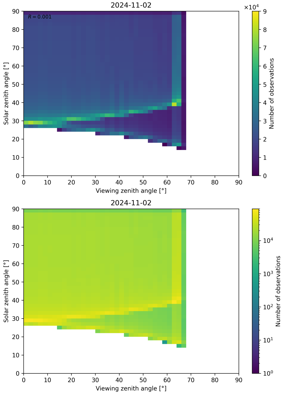
Figure 54: Scatter density plot of “Viewing zenith angle” against “Solar zenith angle” for 2024-11-01 to 2024-11-03.
