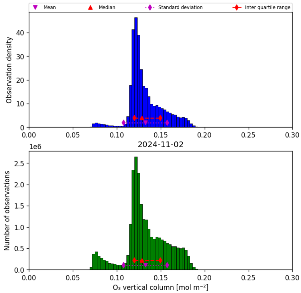
Figure 21: Histogram of “O 3 vertical column” for 2024-11-01 to 2024-11-03
