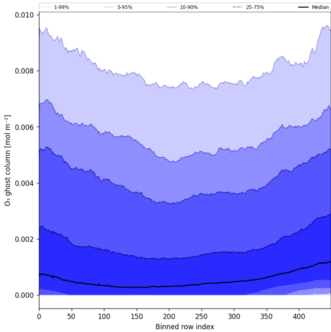
Figure 32: Along track statistics of “O 3 ghost column” for 2024-11-01 to 2024-11-03
