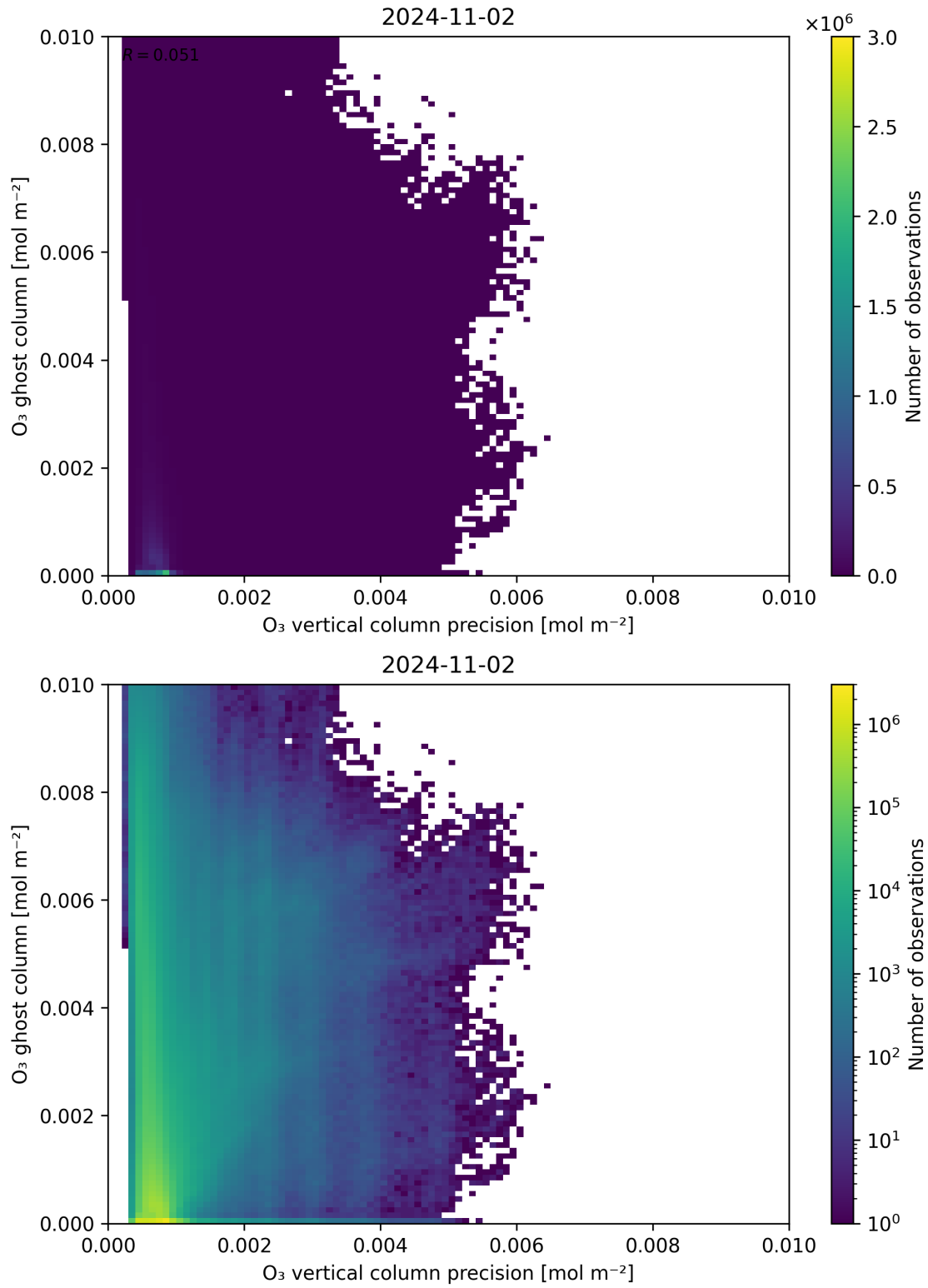
Figure 43: Scatter density plot of “ \text{O}_3 vertical column precision” against “ \text{O}_3 ghost column” for 2024-11-01 to 2024-11-03.
