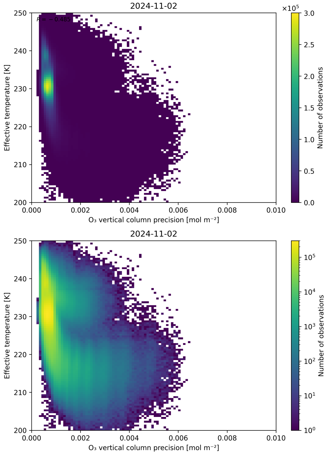
Figure 42: Scatter density plot of “O 3 vertical column precision” against “Effective temperature” for 2024-11-01 to 2024-11-03.
