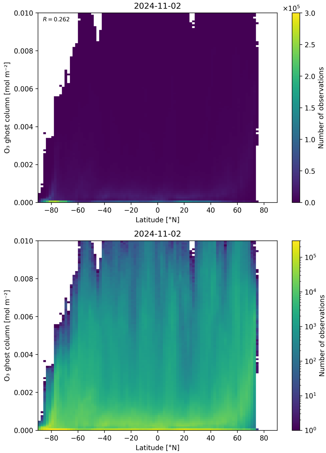
Figure 35: Scatter density plot of “Latitude” against “O 3 ghost column” for 2024-11-01 to 2024-11-03.
