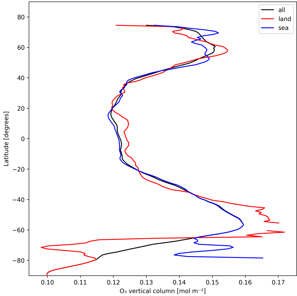
Figure 14: Zonal average of “O 3 vertical column” for 2024-11-01 to 2024-11-03.
