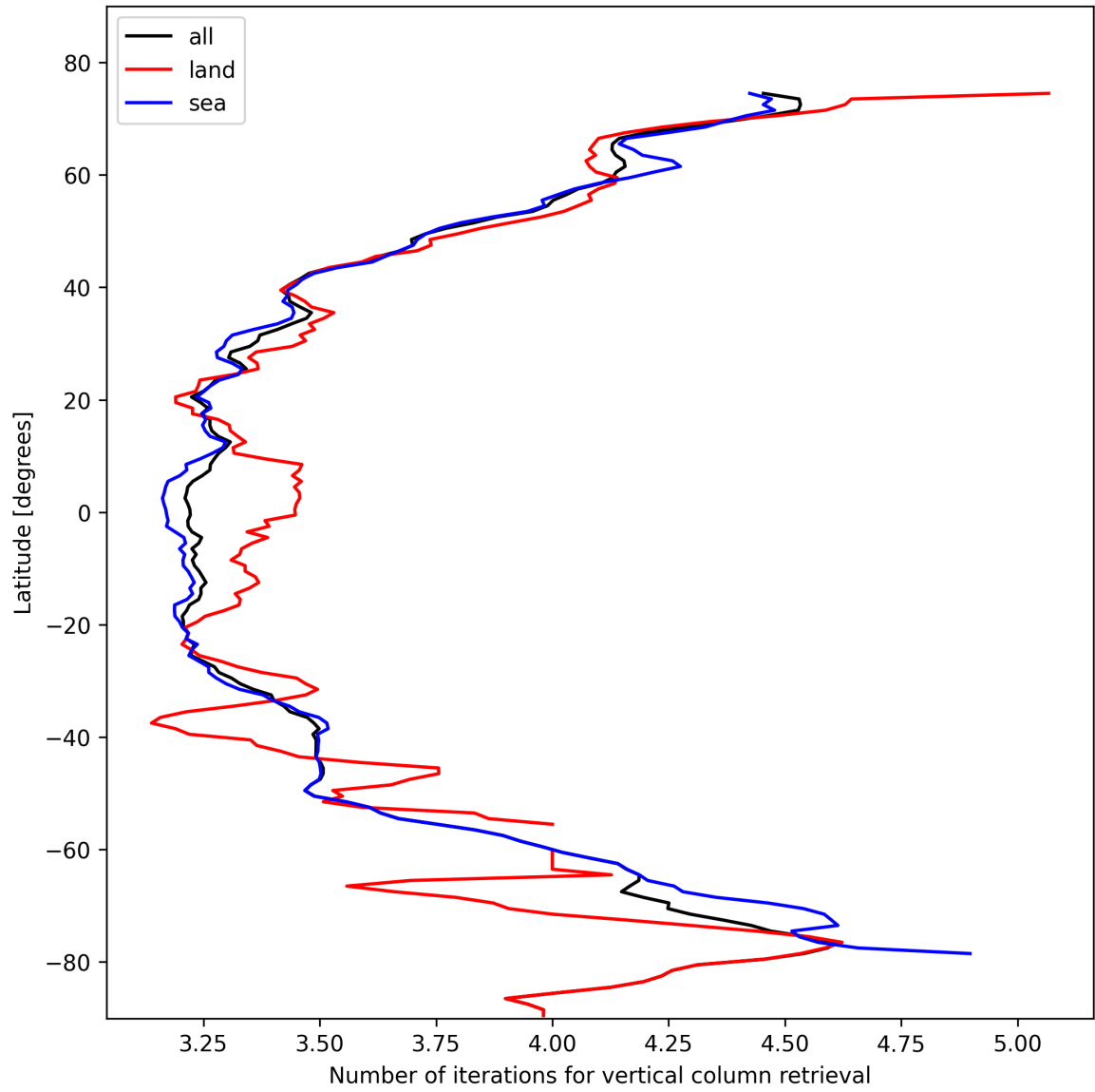
Figure 19: Zonal average of “Number of iterations for vertical column retrieval” for 2024-11-01 to 2024-11-03.
