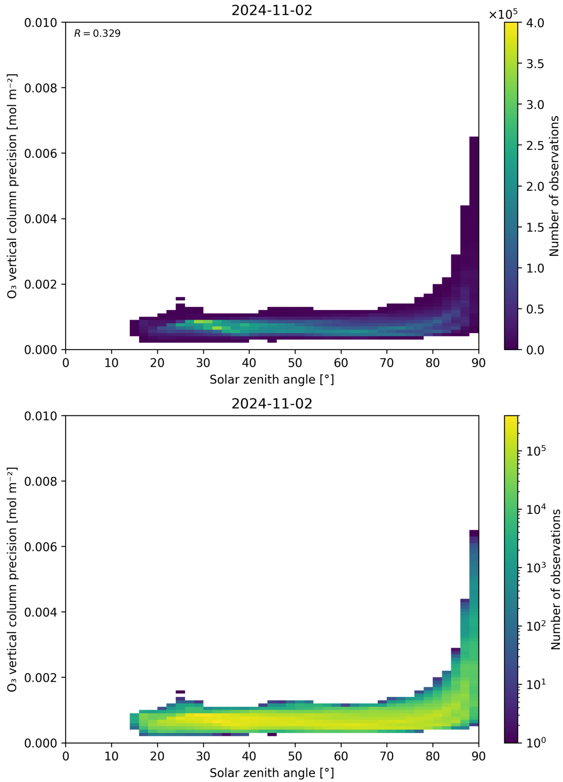
Figure 48: Scatter density plot of “Solar zenith angle” against “O 3 vertical column precision” for 2024-11-01 to 2024-11-03.
