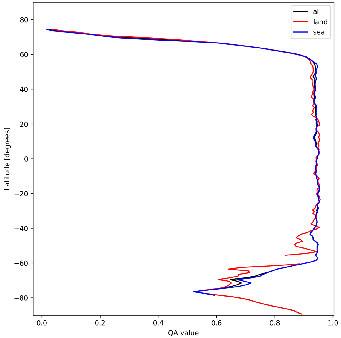
Figure 13: Zonal average of “QA value” for 2024-11-01 to 2024-11-03.
