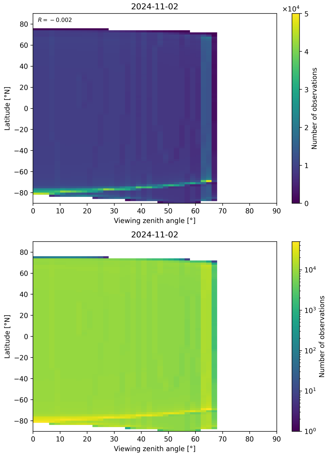
Figure 49: Scatter density plot of “Viewing zenith angle” against “Latitude” for 2024-11-01 to 2024-11-03.
