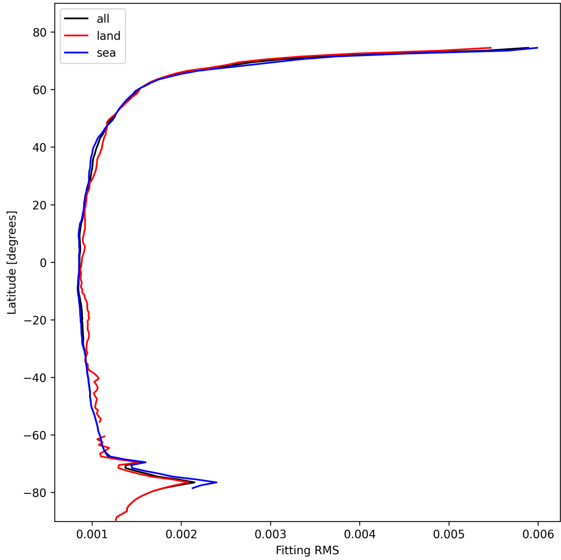
Figure 16: Zonal average of “Fitting RMS” for 2024-11-01 to 2024-11-03.
