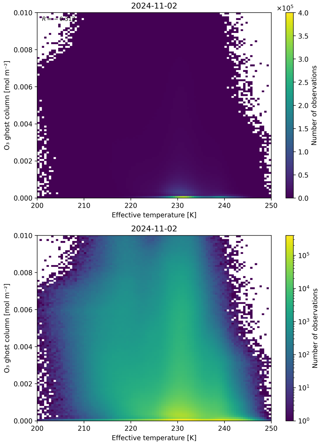
Figure 38: Scatter density plot of “Effective temperature” against “O 3 ghost column” for 2024-11-01 to 2024-11-03.
