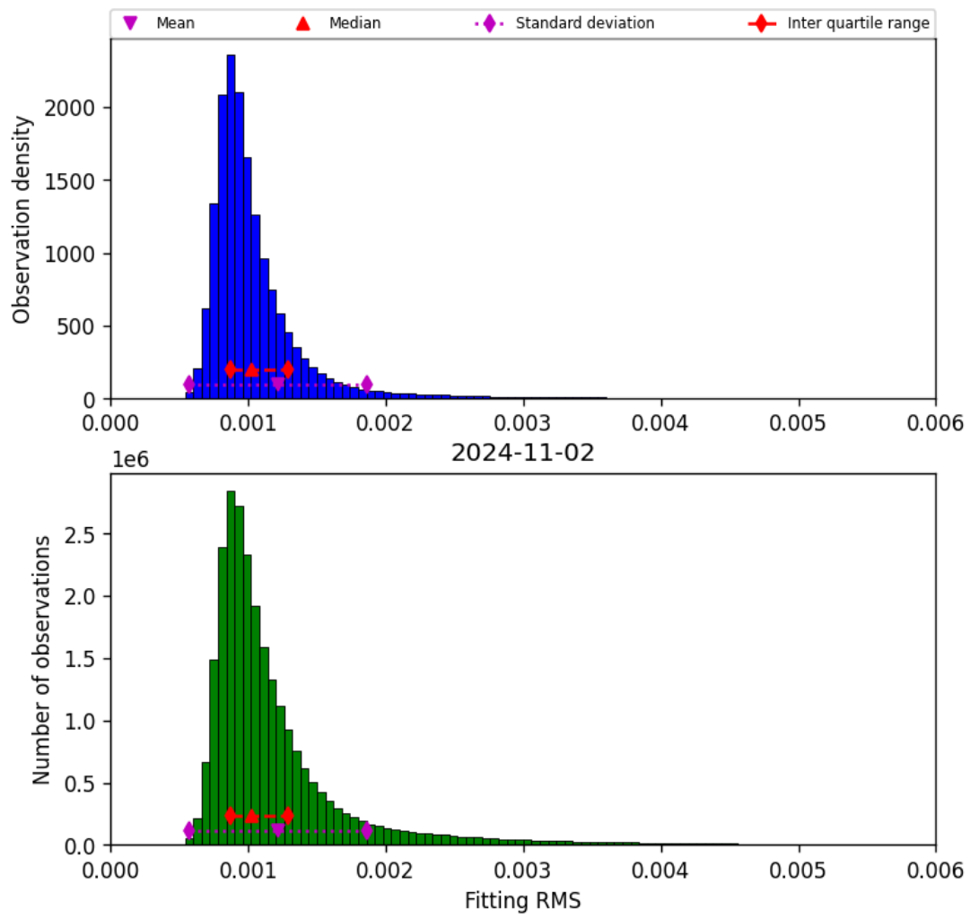
Figure 23: Histogram of “Fitting RMS” for 2024-11-01 to 2024-11-03
