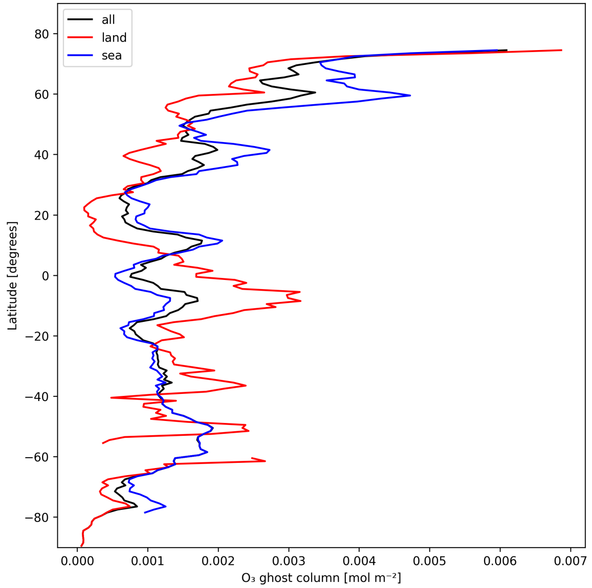
Figure 18: Zonal average of "O 3 ghost column" for 2024-11-01 to 2024-11-03.
