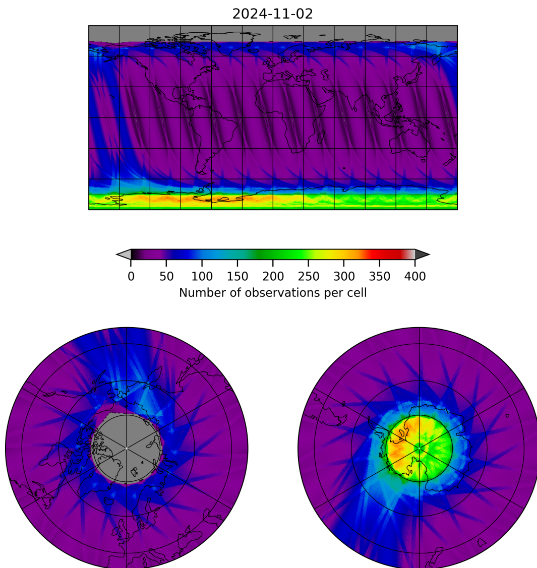
Figure 12: Map of the number of observations for 2024-11-01 to 2024-11-03
