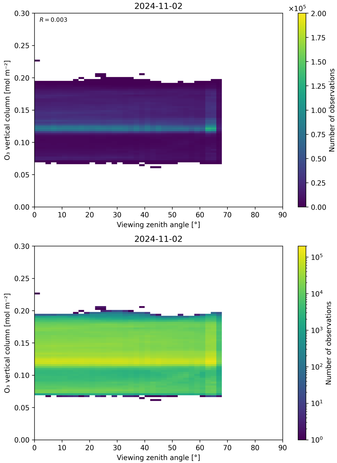
Figure 52: Scatter density plot of “Viewing zenith angle” against “O 3 vertical column” for 2024-11-01 to 2024-11-03.
