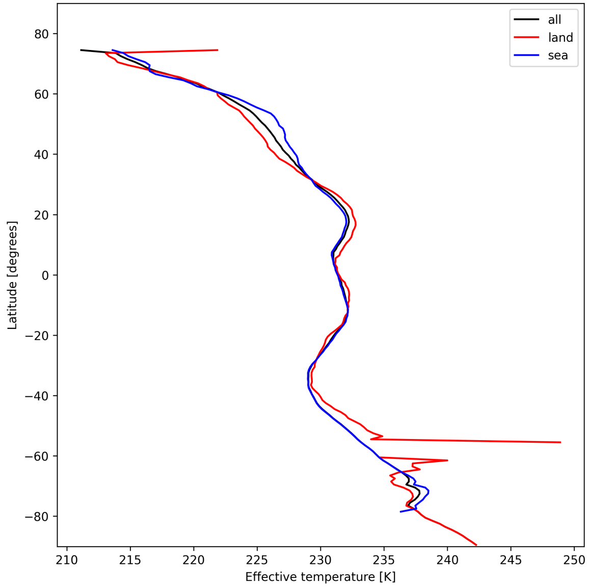
Figure 17: Zonal average of “Effective temperature” for 2024-11-01 to 2024-11-03.
