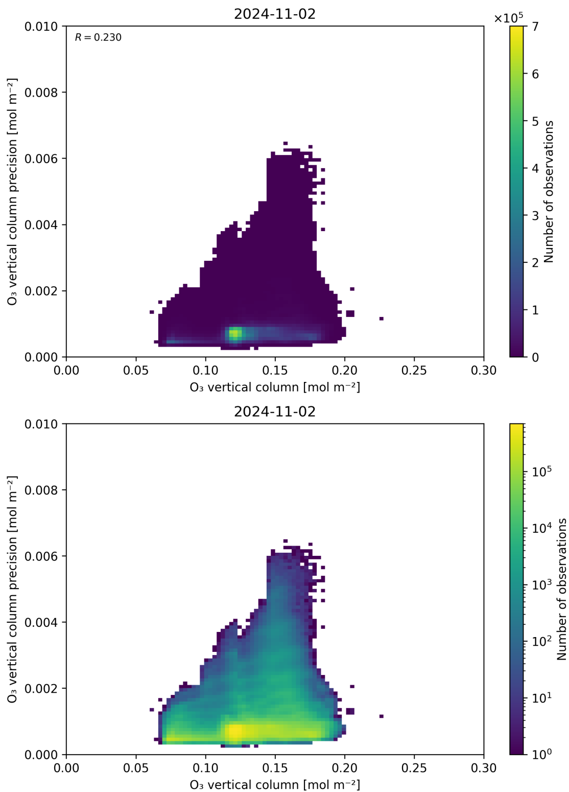
Figure 41: Scatter density plot of “O 3 vertical column” against “O 3 vertical column precision” for 2024-11-01 to 2024-11-03.
