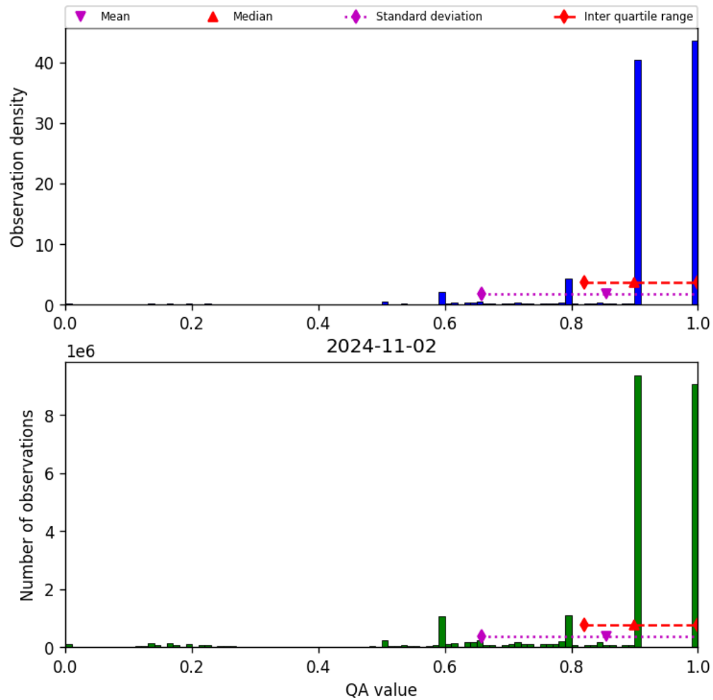
Figure 20: Histogram of “QA value” for 2024-11-01 to 2024-11-03
