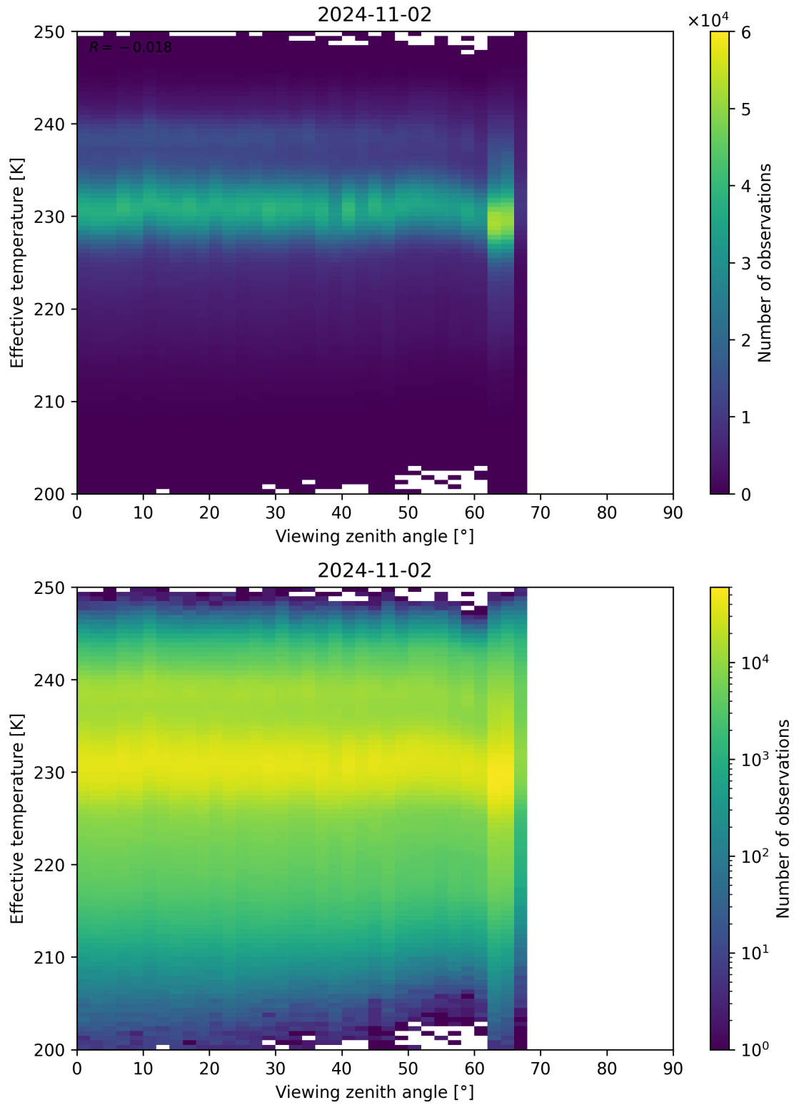
Figure 50: Scatter density plot of “Viewing zenith angle” against “Effective temperature” for 2024-11-01 to 2024-11-03.
