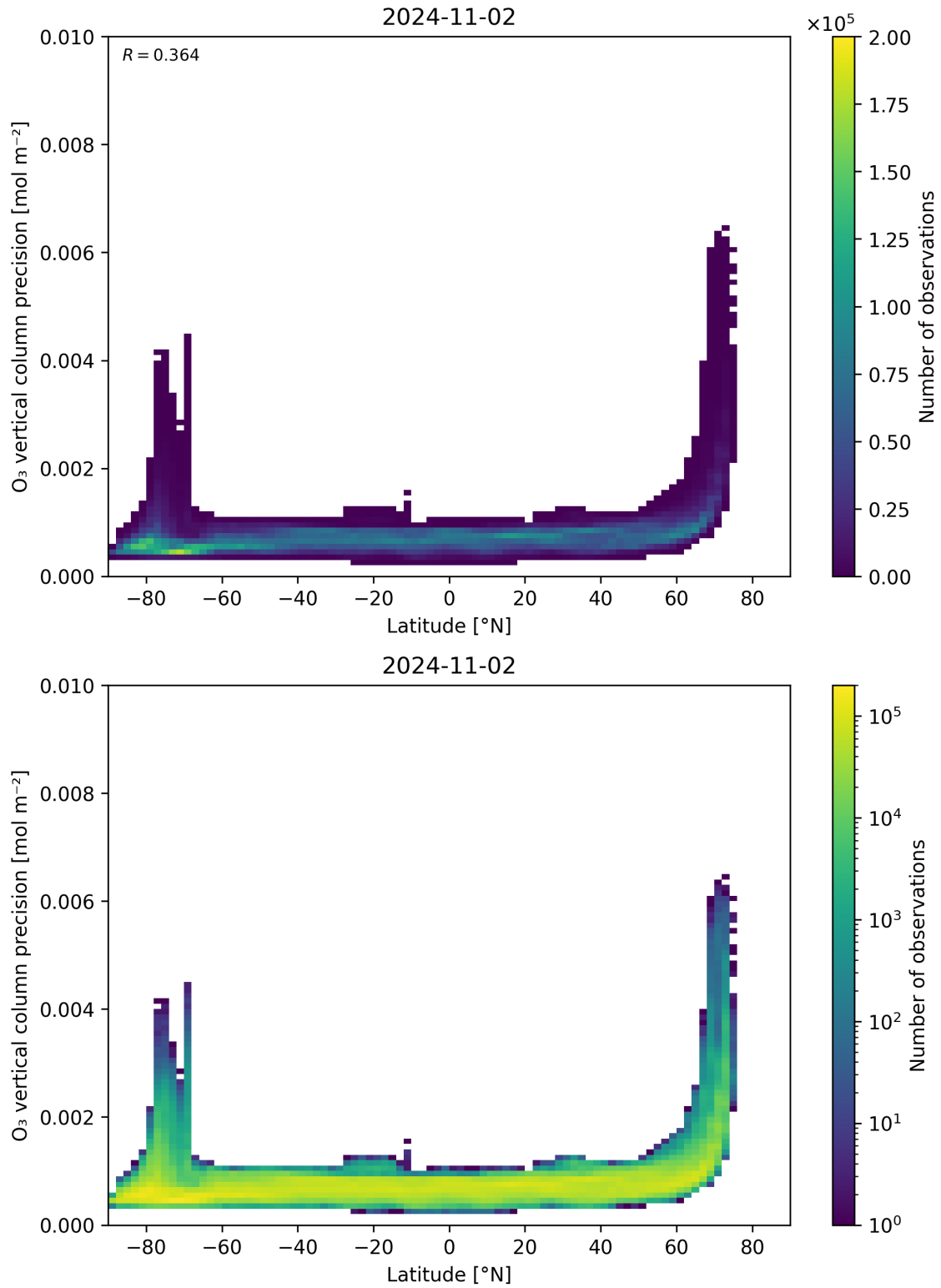
Figure 37: Scatter density plot of “Latitude” against “O 3 vertical column precision” for 2024-11-01 to 2024-11-03.
