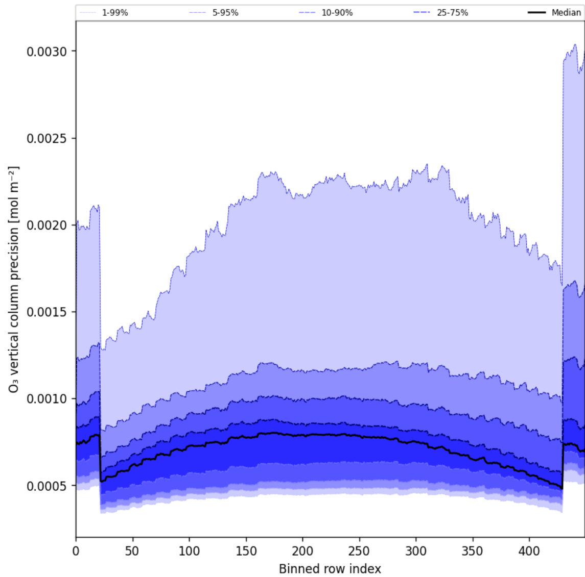
Figure 29: Along track statistics of “O 3 vertical column precision” for 2024-11-01 to 2024-11-03
