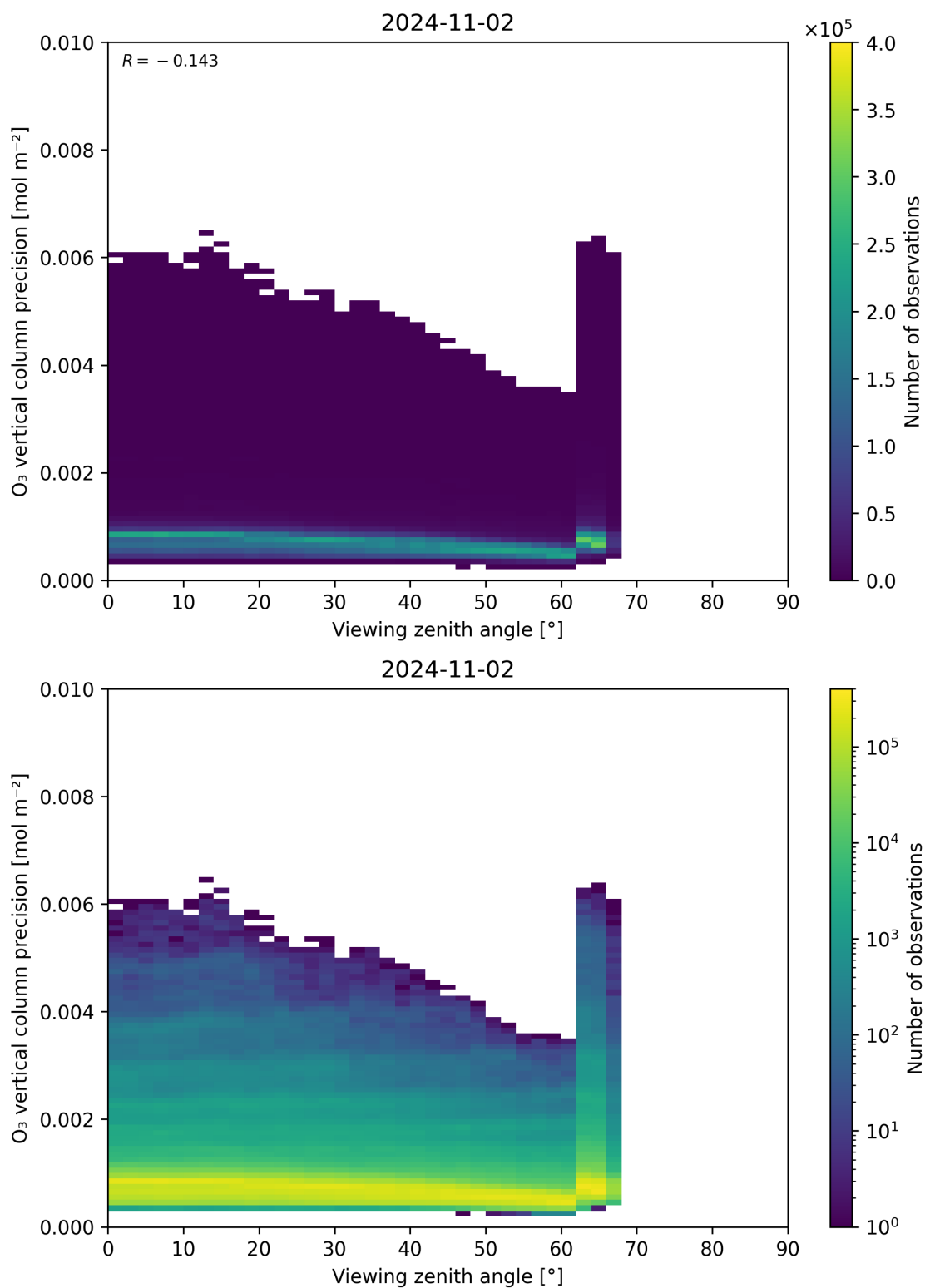
Figure 53: Scatter density plot of “Viewing zenith angle” against “O 3 vertical column precision” for 2024-11-01 to 2024-11-03.
