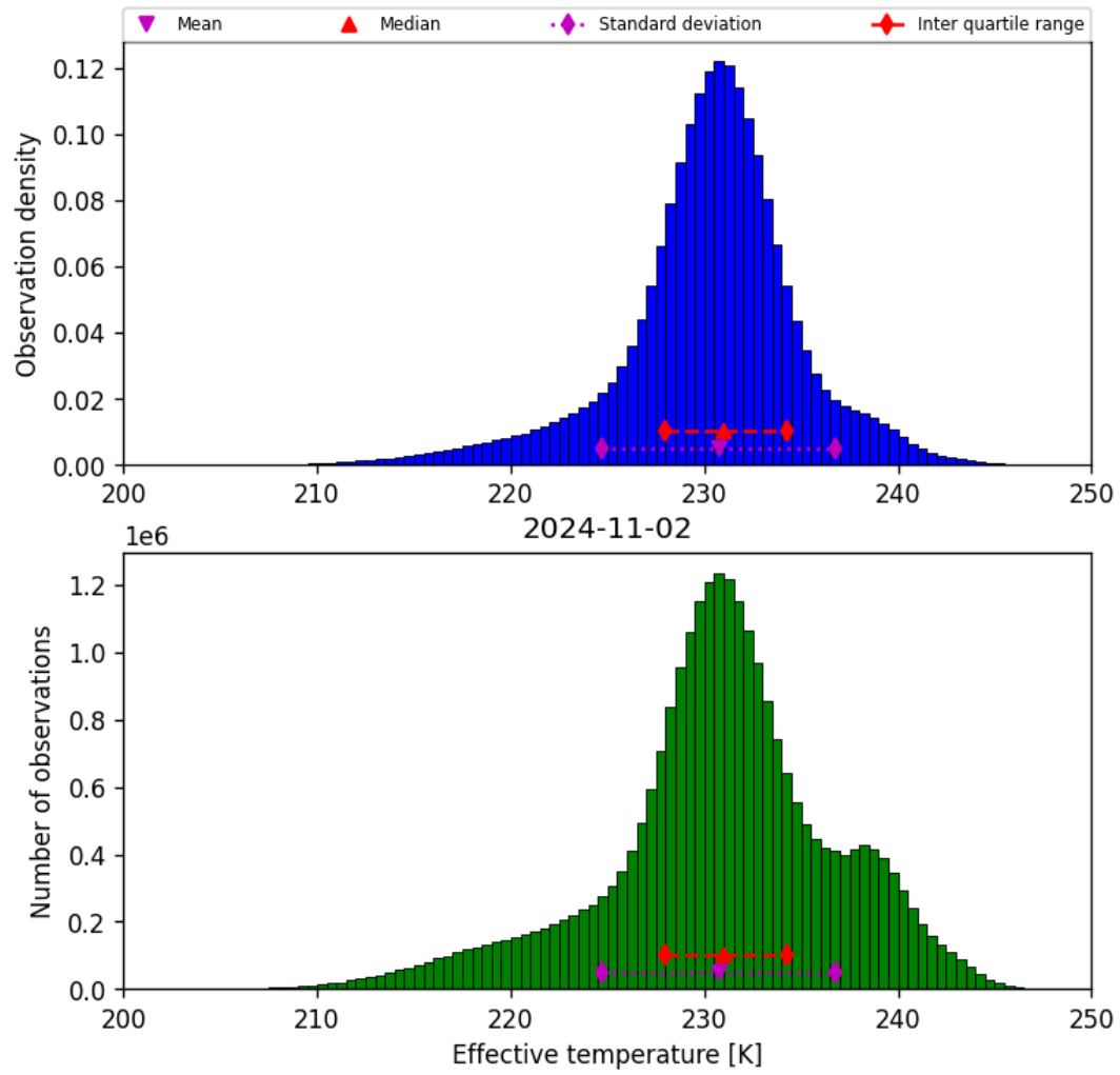
Figure 24: Histogram of “Effective temperature” for 2024-11-01 to 2024-11-03
