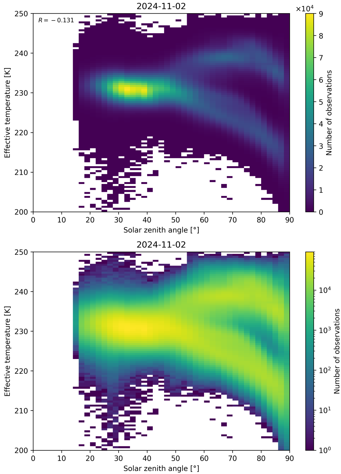
Figure 45: Scatter density plot of “Solar zenith angle” against “Effective temperature” for 2024-11-01 to 2024-11-03.
