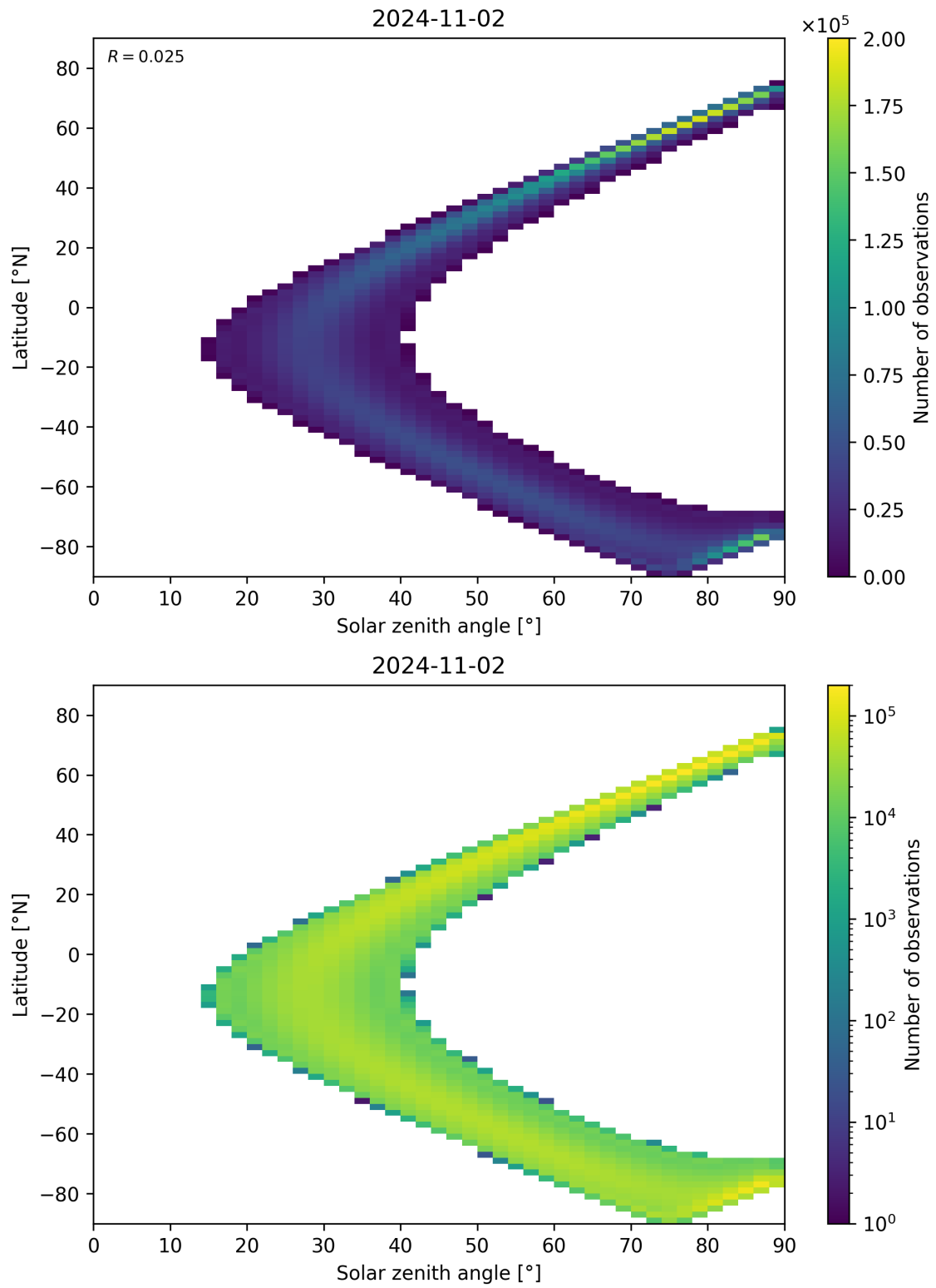
Figure 44: Scatter density plot of “Solar zenith angle” against “Latitude” for 2024-11-01 to 2024-11-03.
