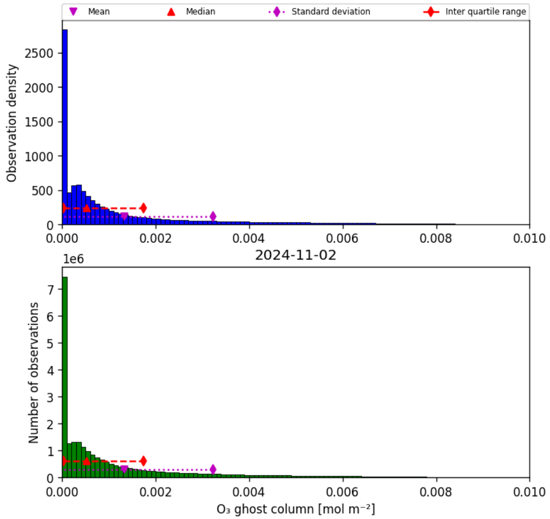
Figure 25: Histogram of “O 3 ghost column” for 2024-11-01 to 2024-11-03
