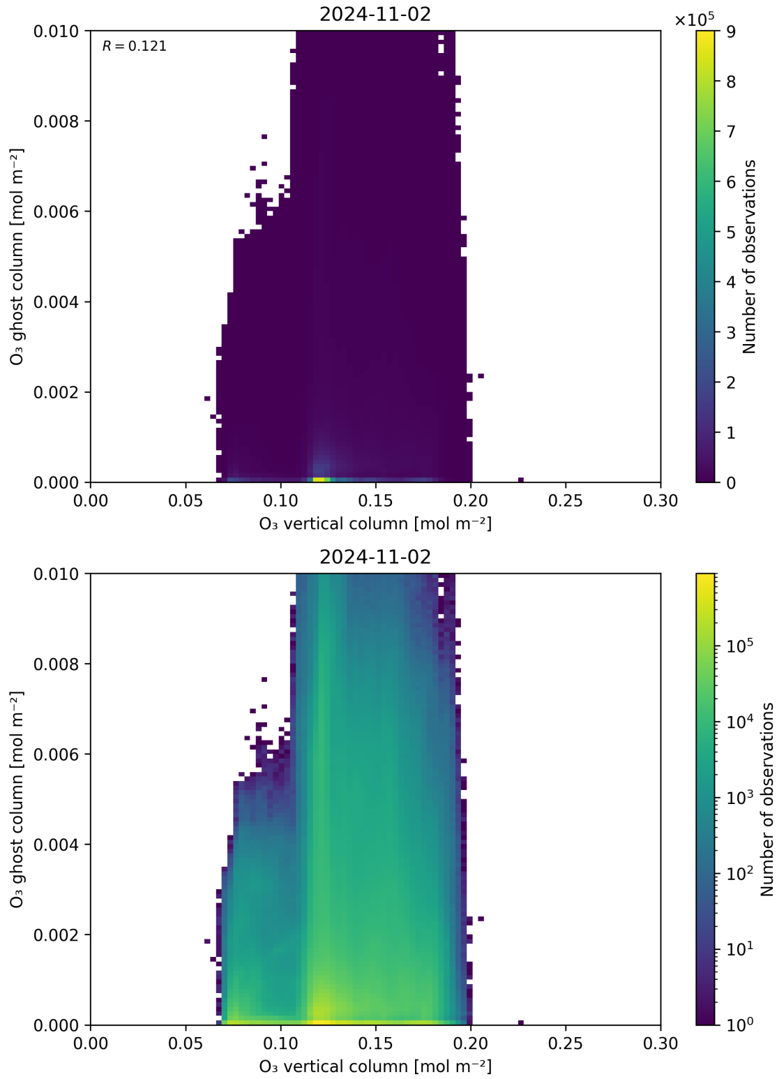
Figure 40: Scatter density plot of “O 3 vertical column” against “O 3 ghost column” for 2024-11-01 to 2024-11-03.
