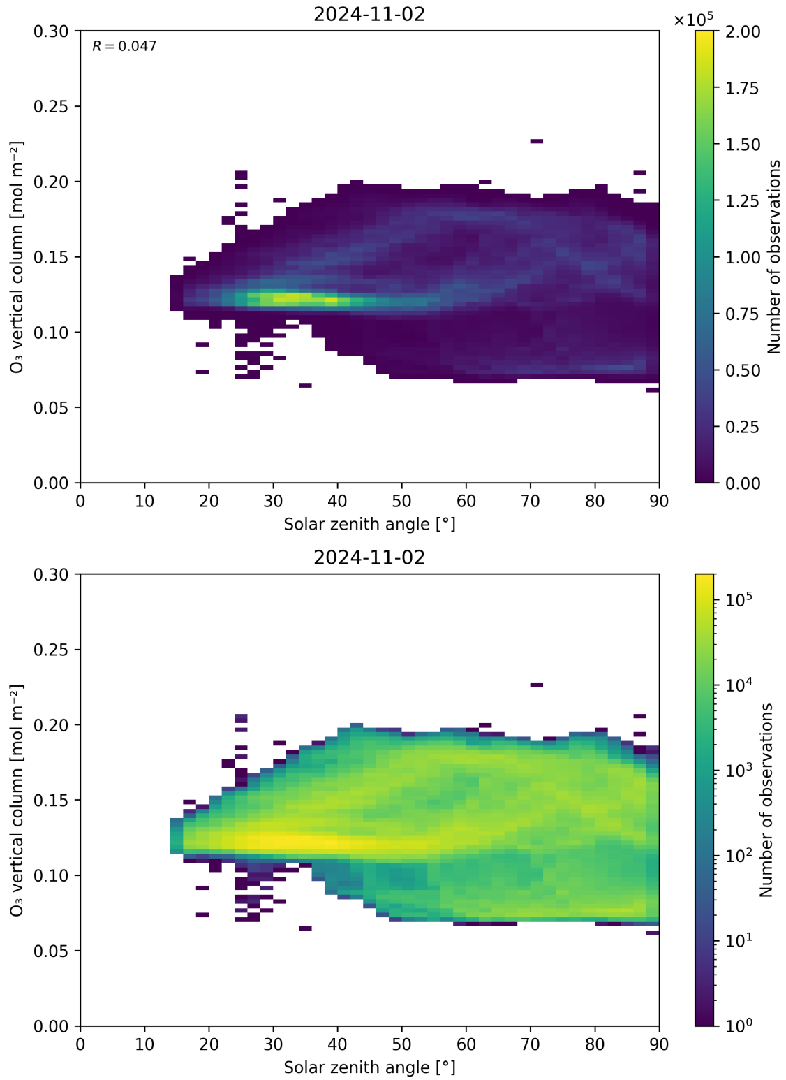
Figure 47: Scatter density plot of “Solar zenith angle” against “O 3 vertical column” for 2024-11-01 to 2024-11-03.
