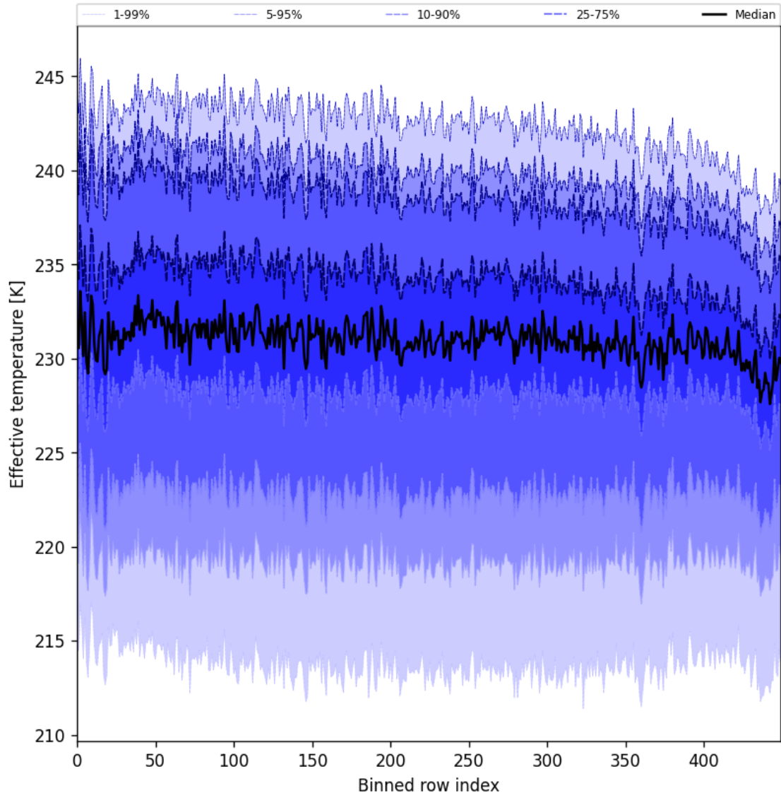
Figure 31: Along track statistics of “Effective temperature” for 2024-11-01 to 2024-11-03
