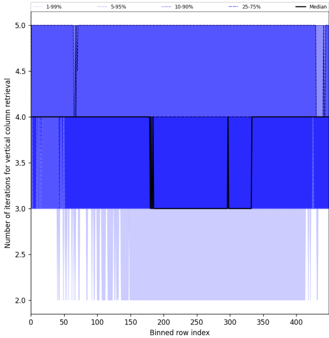
Figure 33: Along track statistics of “Number of iterations for vertical column retrieval” for 2024-11-01 to 2024-11-03
