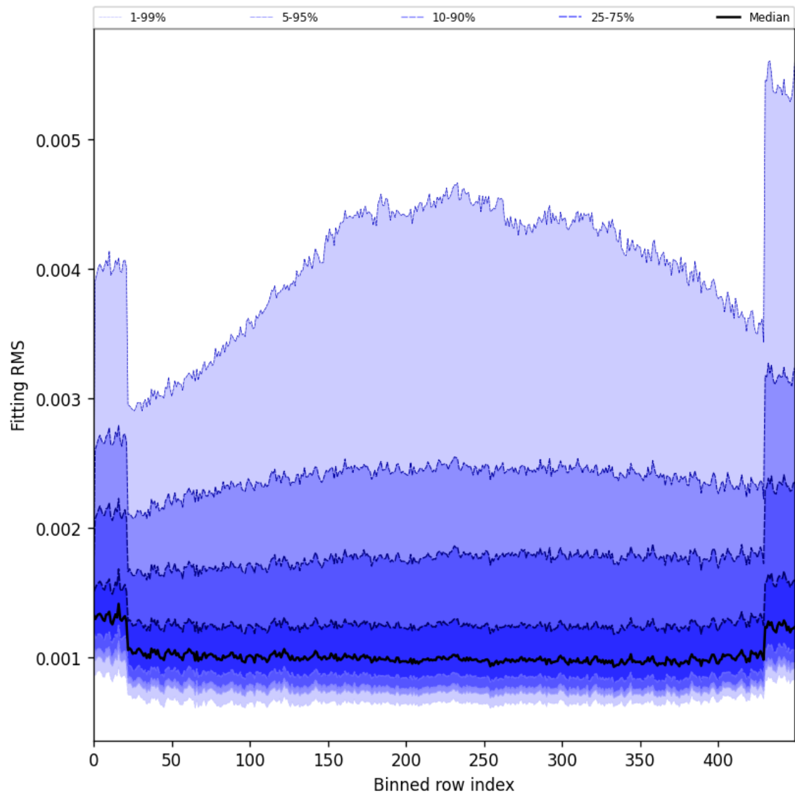
Figure 30: Along track statistics of “Fitting RMS” for 2024-11-01 to 2024-11-03
