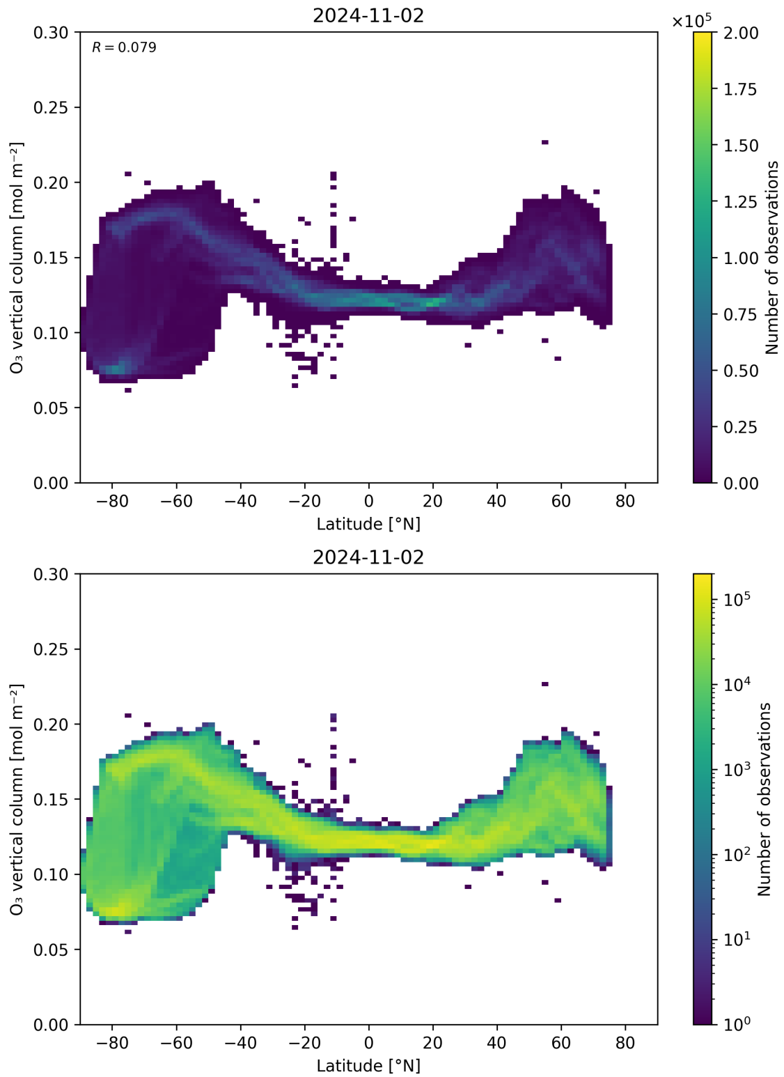
Figure 36: Scatter density plot of “Latitude” against “O 3 vertical column” for 2024-11-01 to 2024-11-03.
