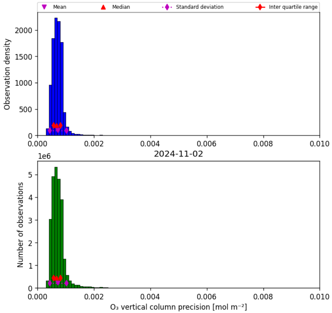
Figure 22: Histogram of “O 3 vertical column precision” for 2024-11-01 to 2024-11-03
