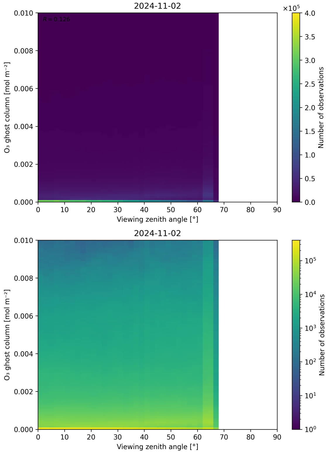
Figure 51: Scatter density plot of “Viewing zenith angle” against “O 3 ghost column” for 2024-11-01 to 2024-11-03.
