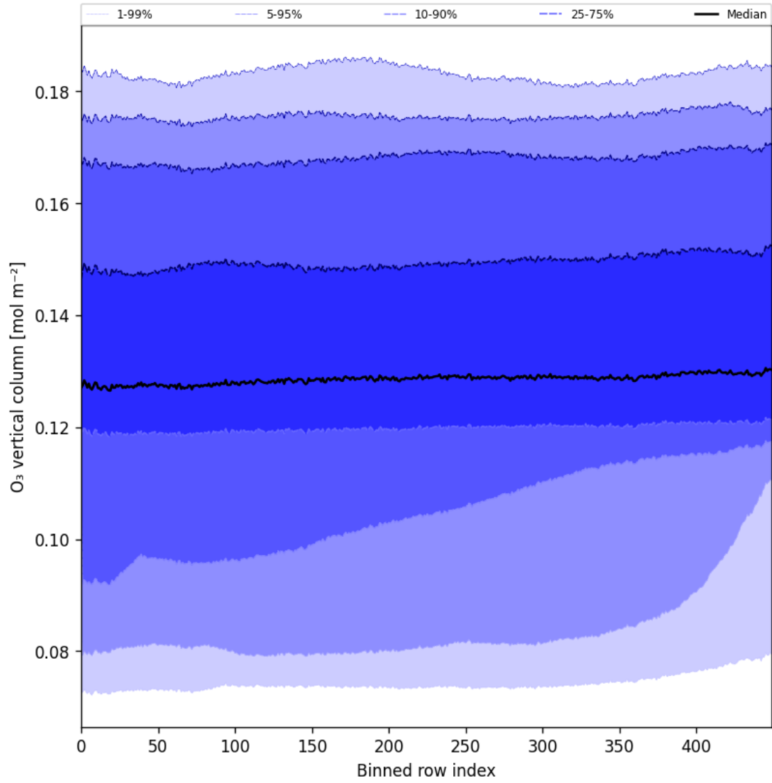
Figure 28: Along track statistics of “O 3 vertical column” for 2024-11-01 to 2024-11-03
