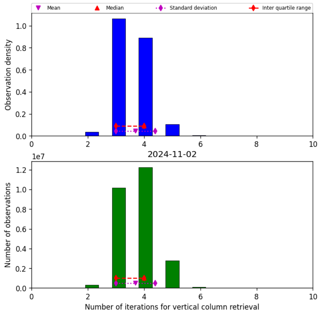
Figure 26: Histogram of “Number of iterations for vertical column retrieval” for 2024-11-01 to 2024-11-03
