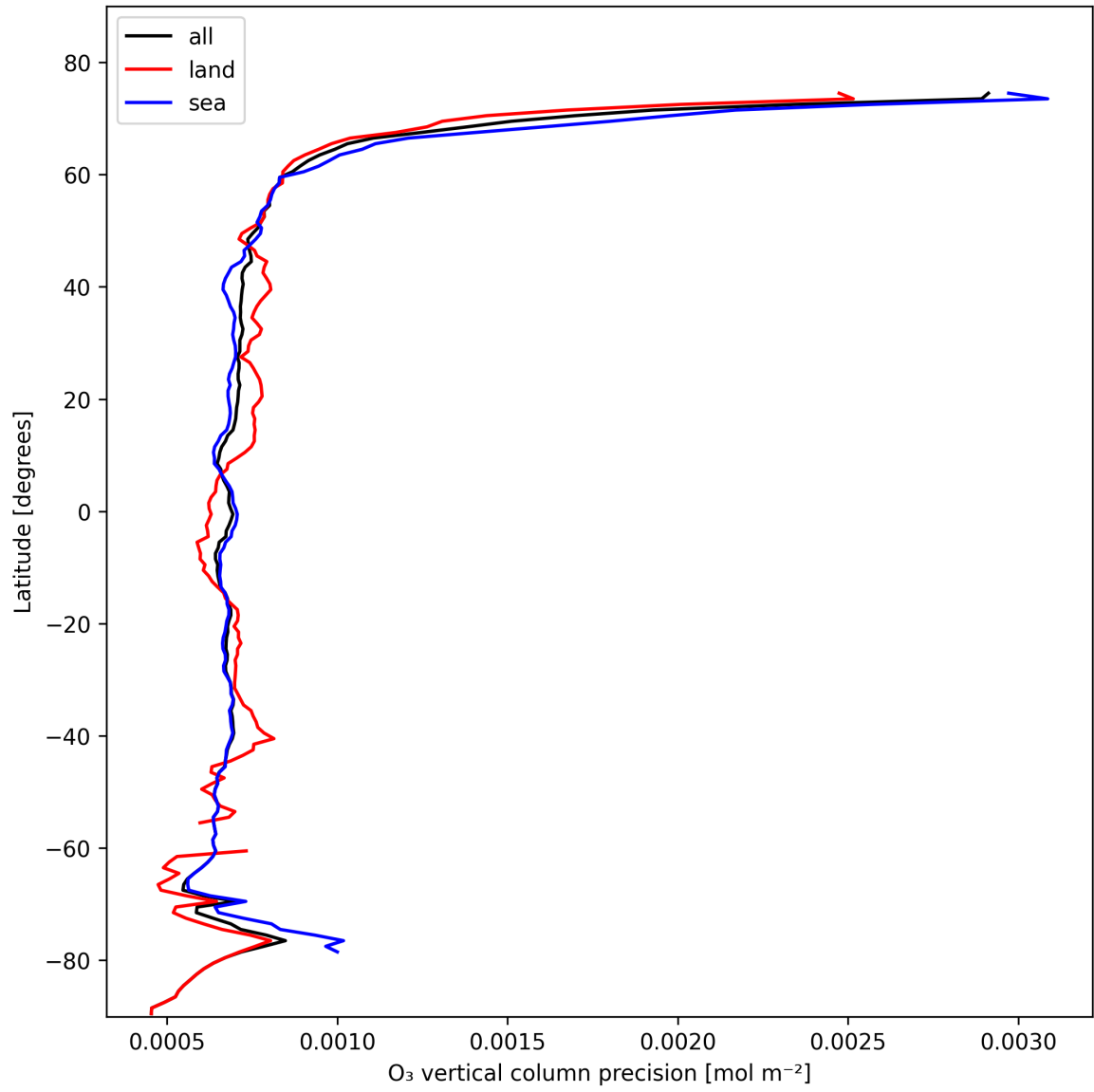
Figure 15: Zonal average of “O 3 vertical column precision” for 2024-11-01 to 2024-11-03.
