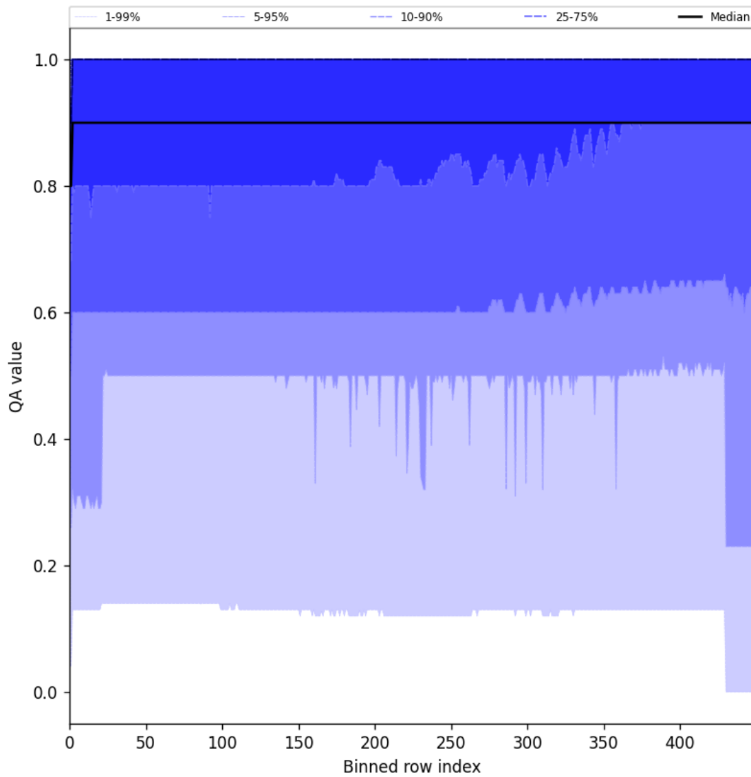
Figure 27: Along track statistics of “QA value” for 2024-11-01 to 2024-11-03
