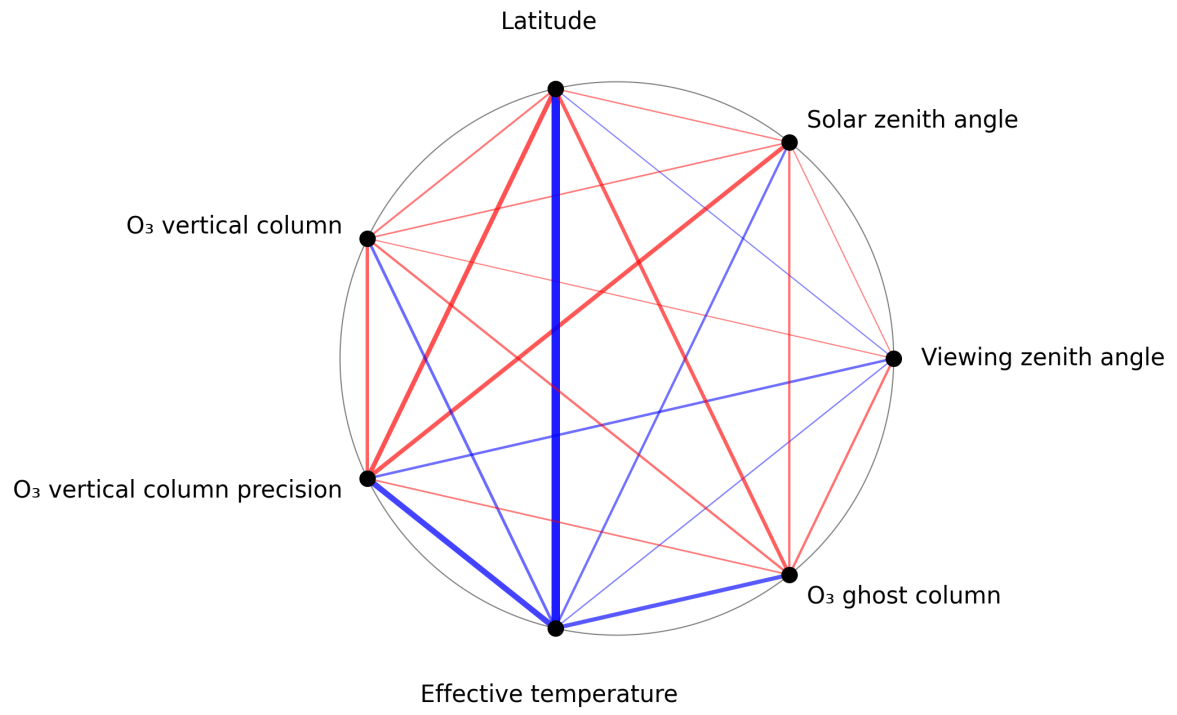
Figure 1: Map of correlation graph for 2024-11-01 to 2024-11-03.
