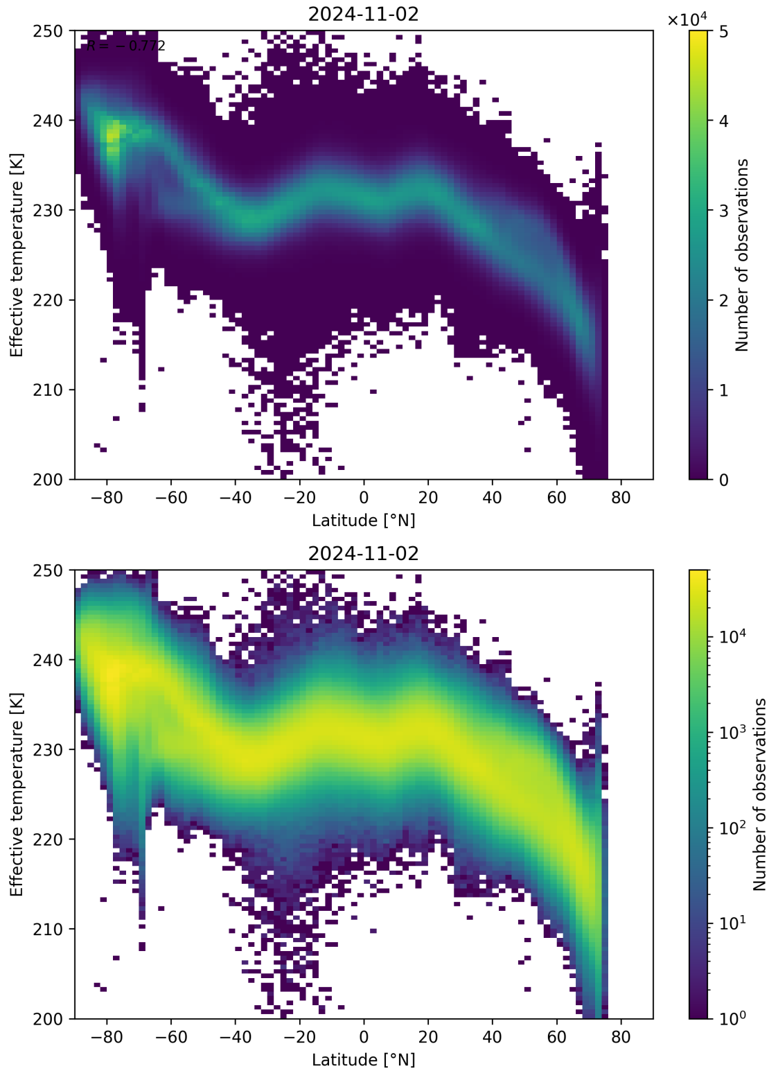
Figure 34: Scatter density plot of “Latitude” against “Effective temperature” for 2024-11-01 to 2024-11-03.
