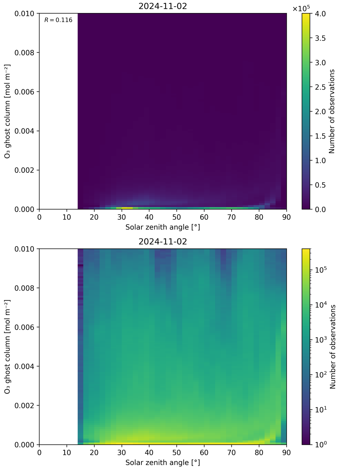
Figure 46: Scatter density plot of “Solar zenith angle” against “O 3 ghost column” for 2024-11-01 to 2024-11-03.
