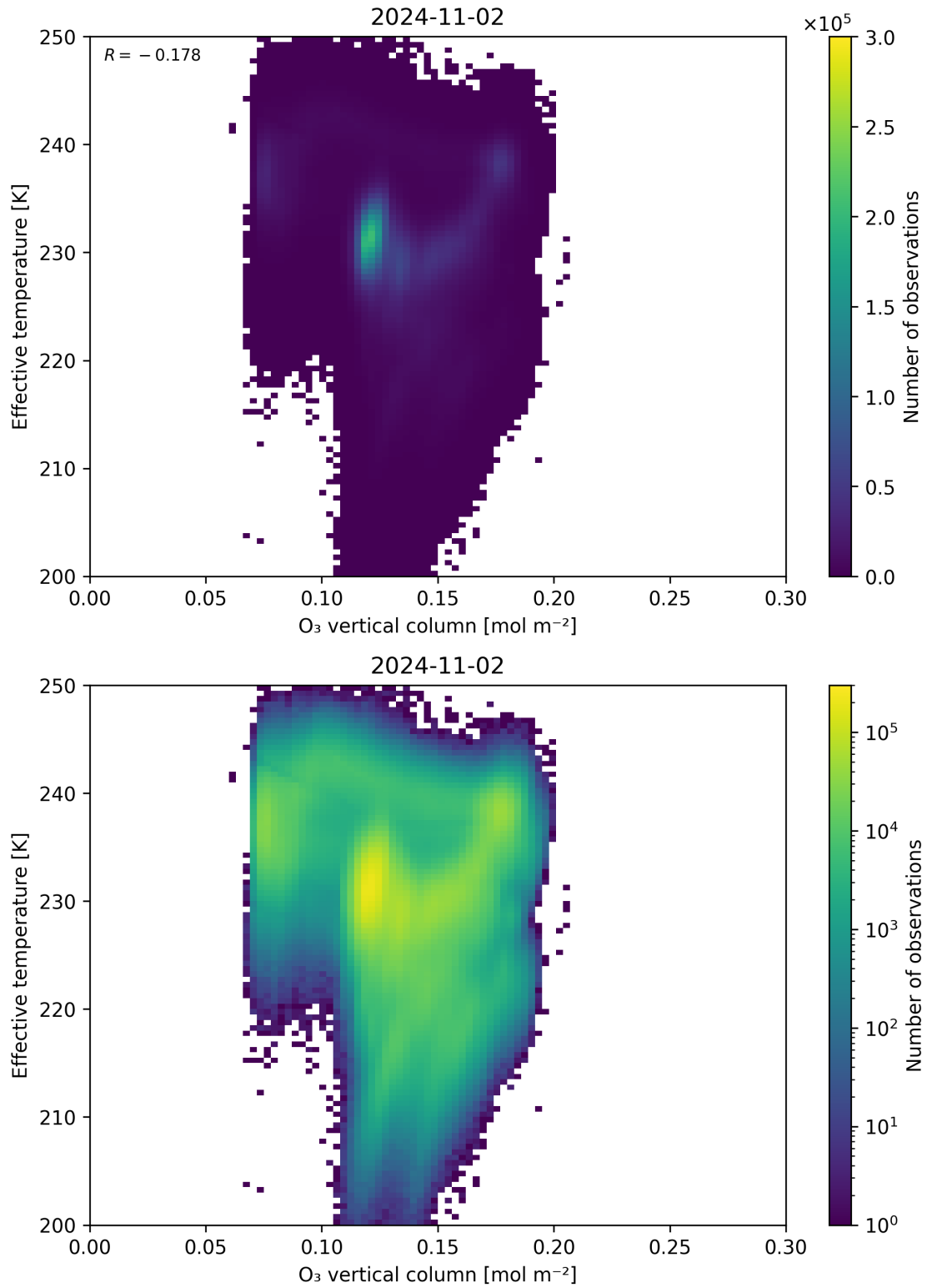
Figure 39: Scatter density plot of “O 3 vertical column” against “Effective temperature” for 2024-11-01 to 2024-11-03.
