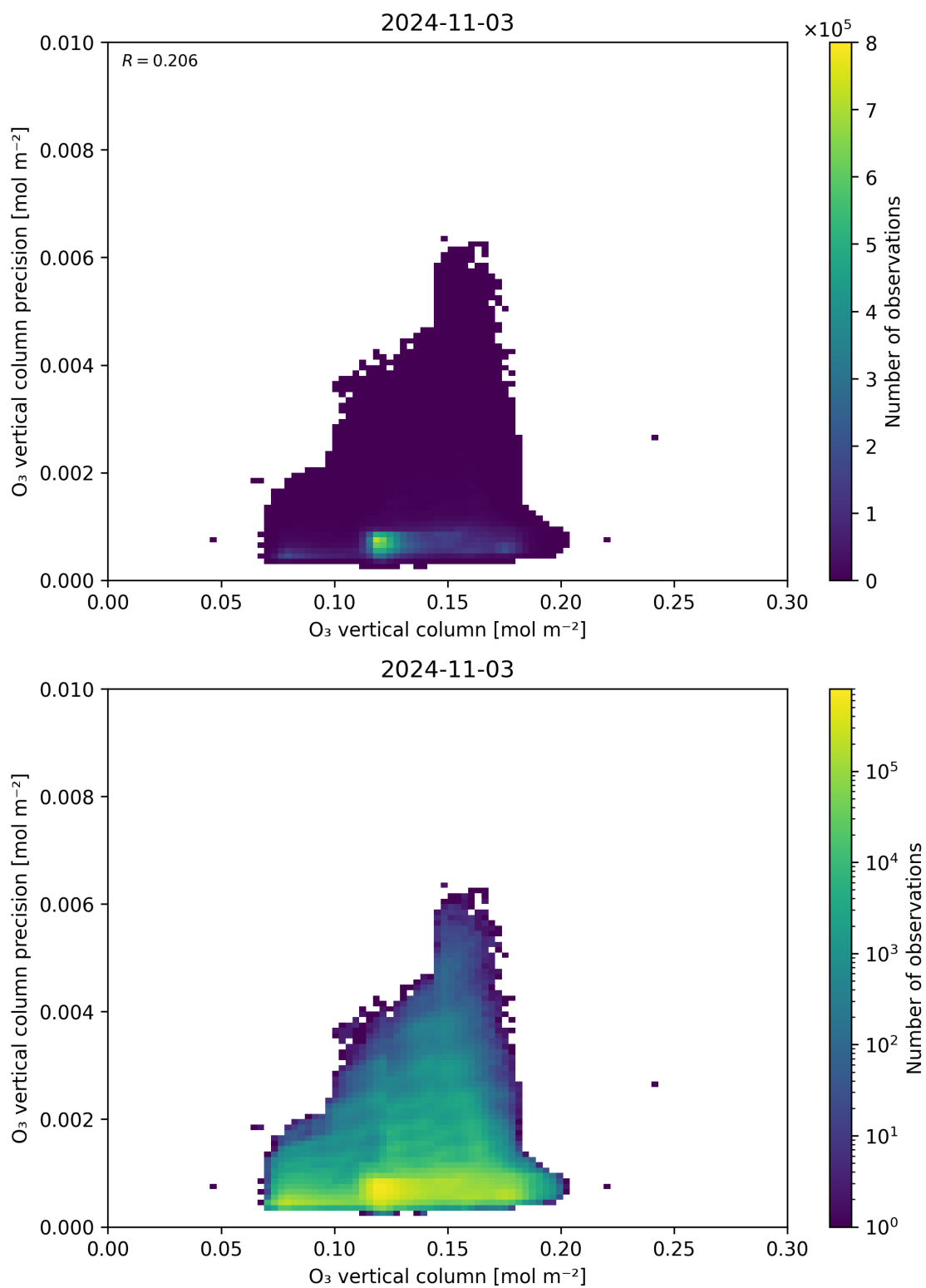
Figure 41: Scatter density plot of “O 3 vertical column” against “O 3 vertical column precision” for 2024-11-02 to 2024-11-04.
