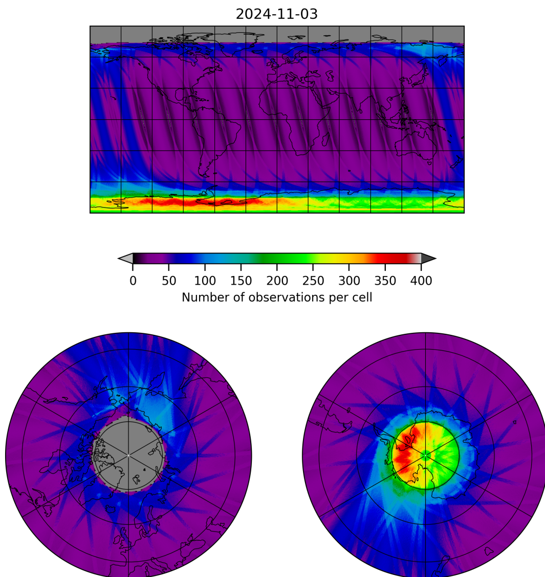
Figure 12: Map of the number of observations for 2024-11-02 to 2024-11-04
