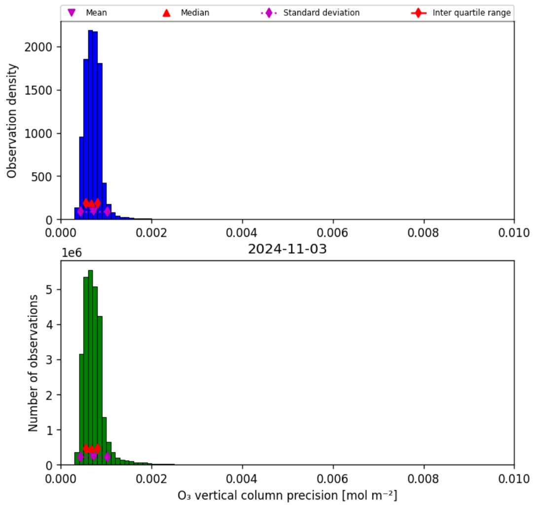
Figure 22: Histogram of “O 3 vertical column precision” for 2024-11-02 to 2024-11-04
