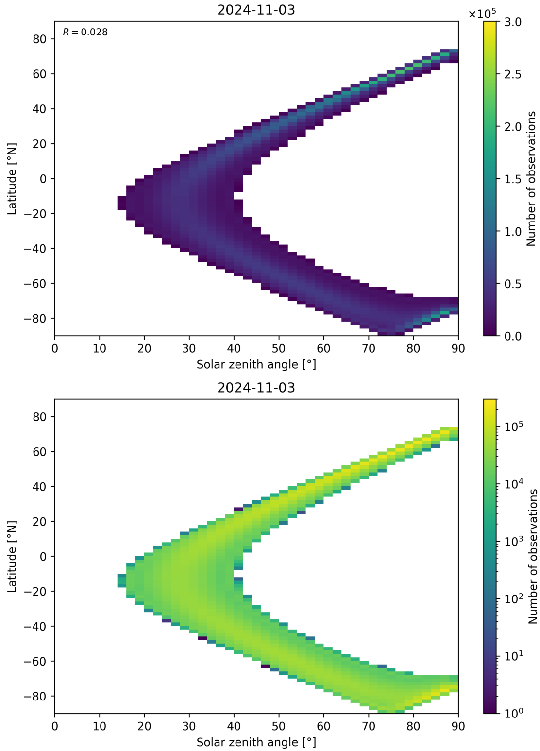
Figure 44: Scatter density plot of “Solar zenith angle” against “Latitude” for 2024-11-02 to 2024-11-04.
