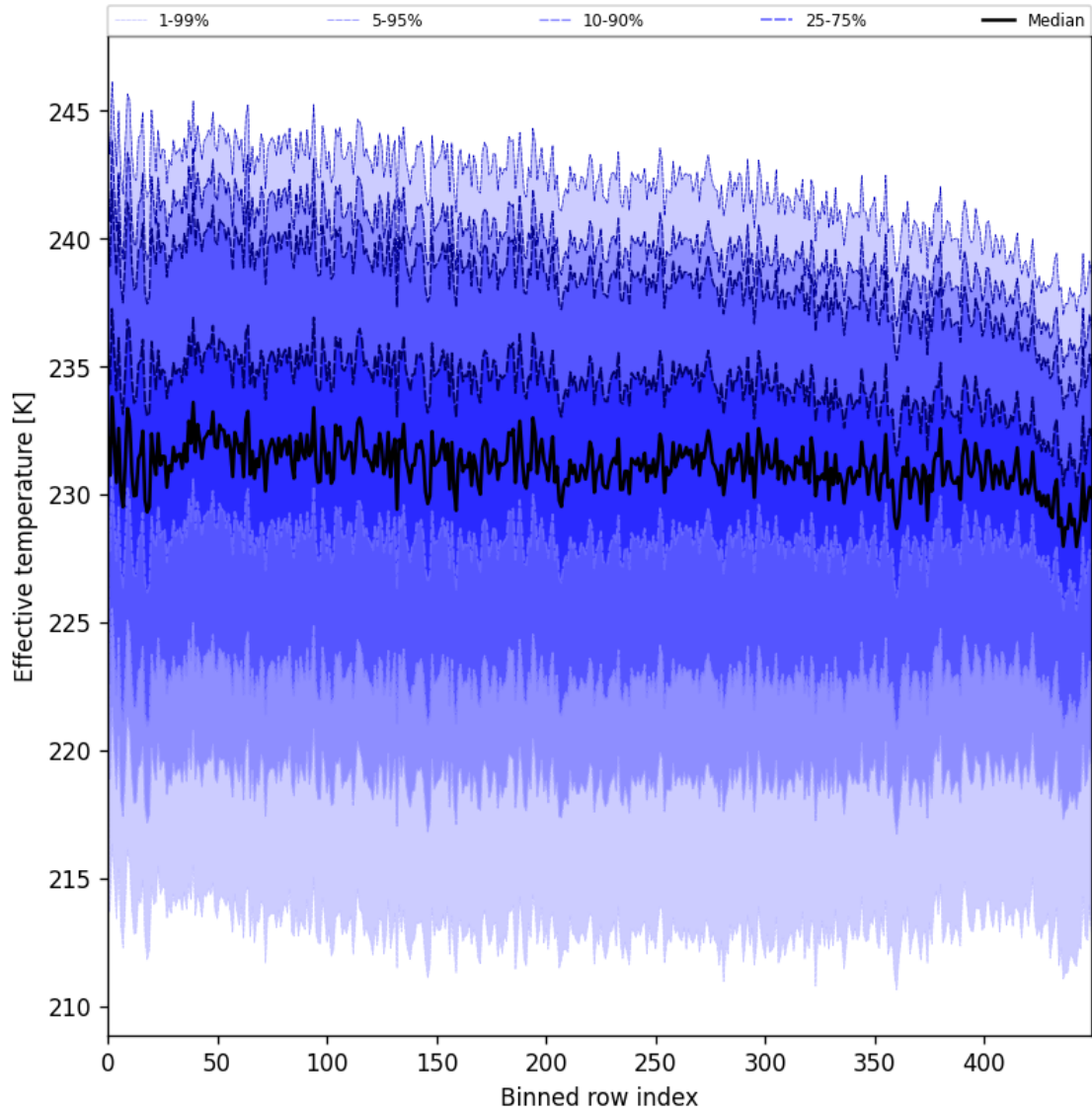
Figure 31: Along track statistics of “Effective temperature” for 2024-11-02 to 2024-11-04
