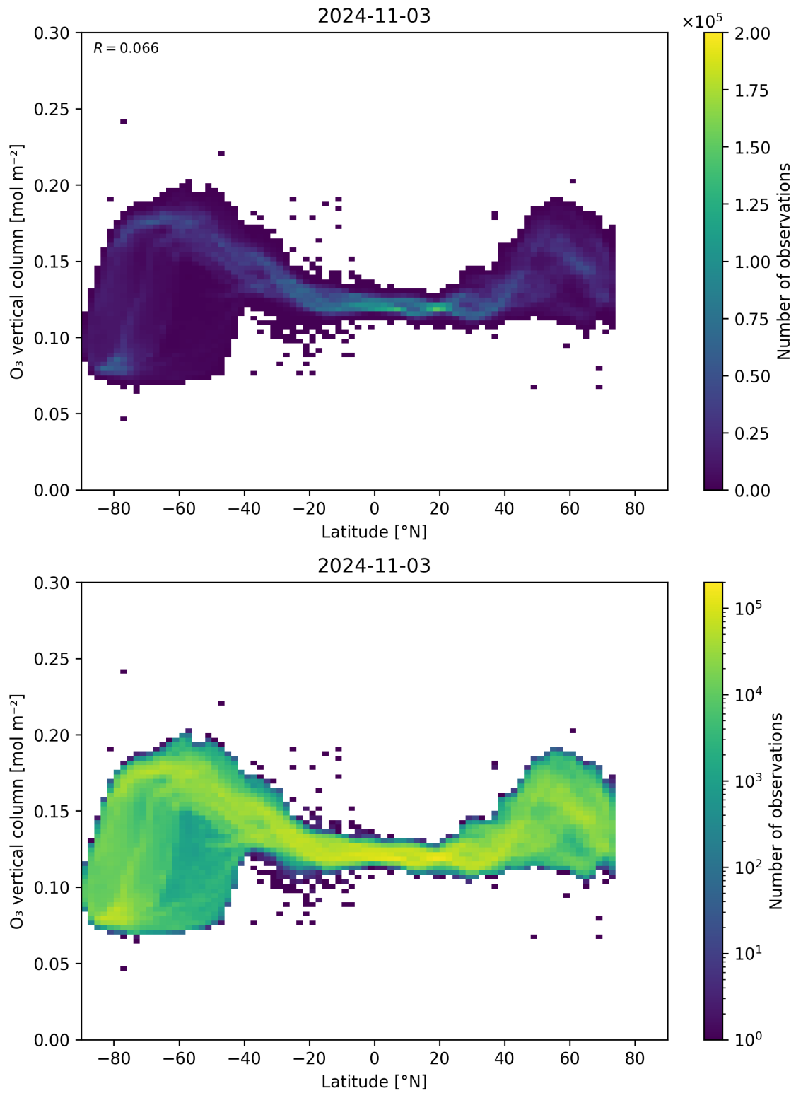
Figure 36: Scatter density plot of “Latitude” against “O 3 vertical column” for 2024-11-02 to 2024-11-04.
