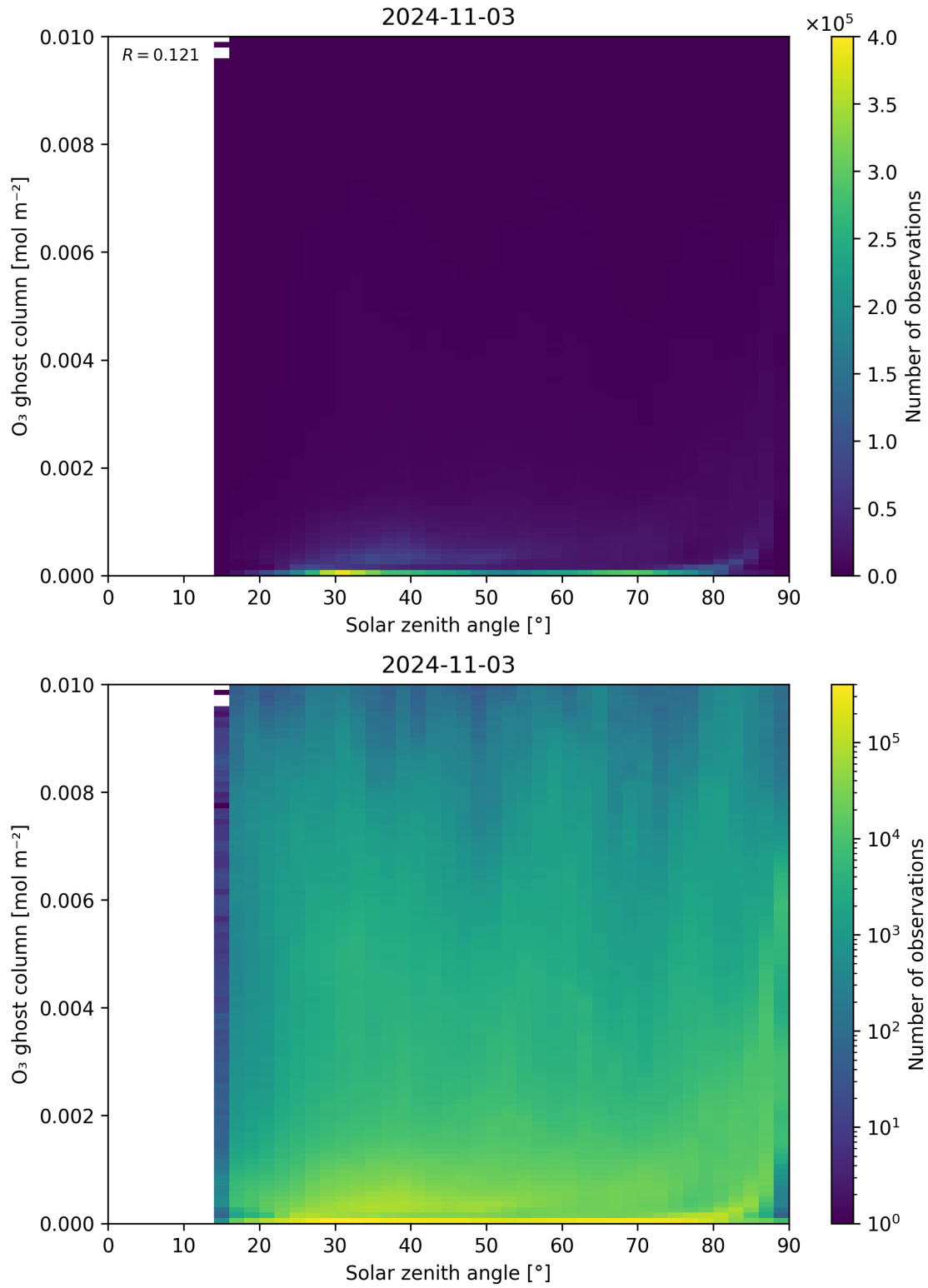
Figure 46: Scatter density plot of “Solar zenith angle” against “O 3 ghost column” for 2024-11-02 to 2024-11-04.
