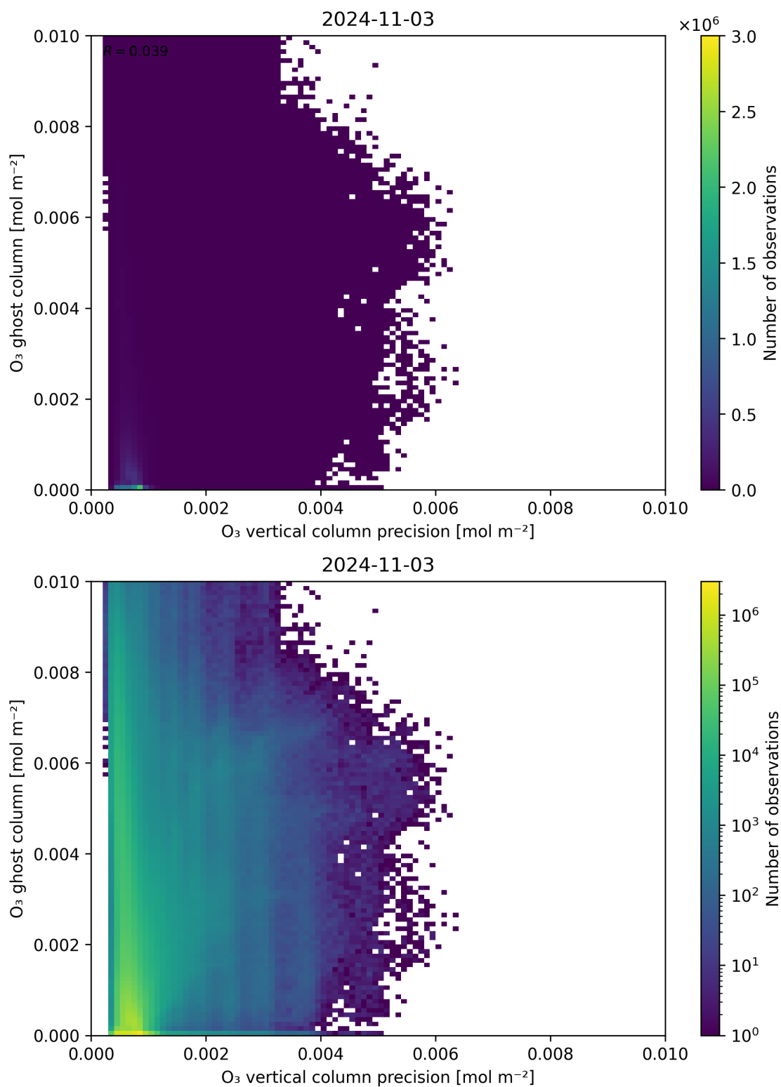
Figure 43: Scatter density plot of “ \text{O}_3 vertical column precision” against “ \text{O}_3 ghost column” for 2024-11-02 to 2024-11-04.
