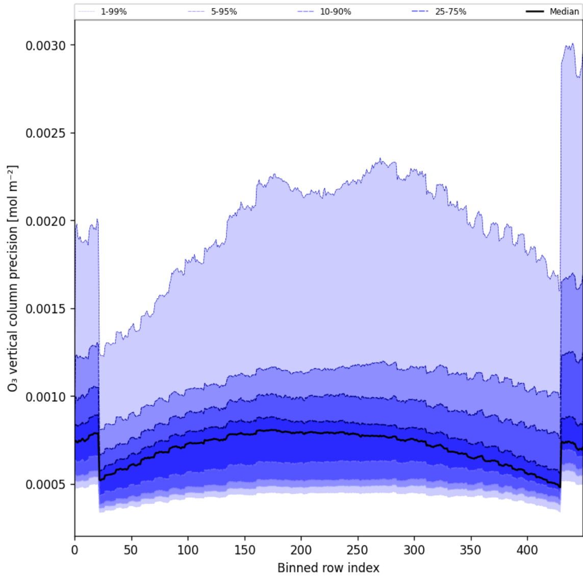
Figure 29: Along track statistics of “O 3 vertical column precision” for 2024-11-02 to 2024-11-04
