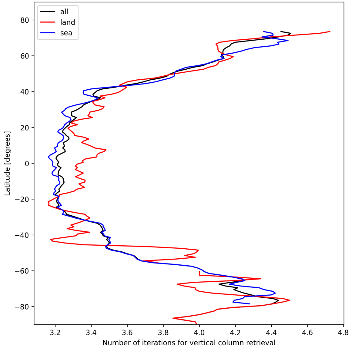
Figure 19: Zonal average of “Number of iterations for vertical column retrieval” for 2024-11-02 to 2024-11-04.
