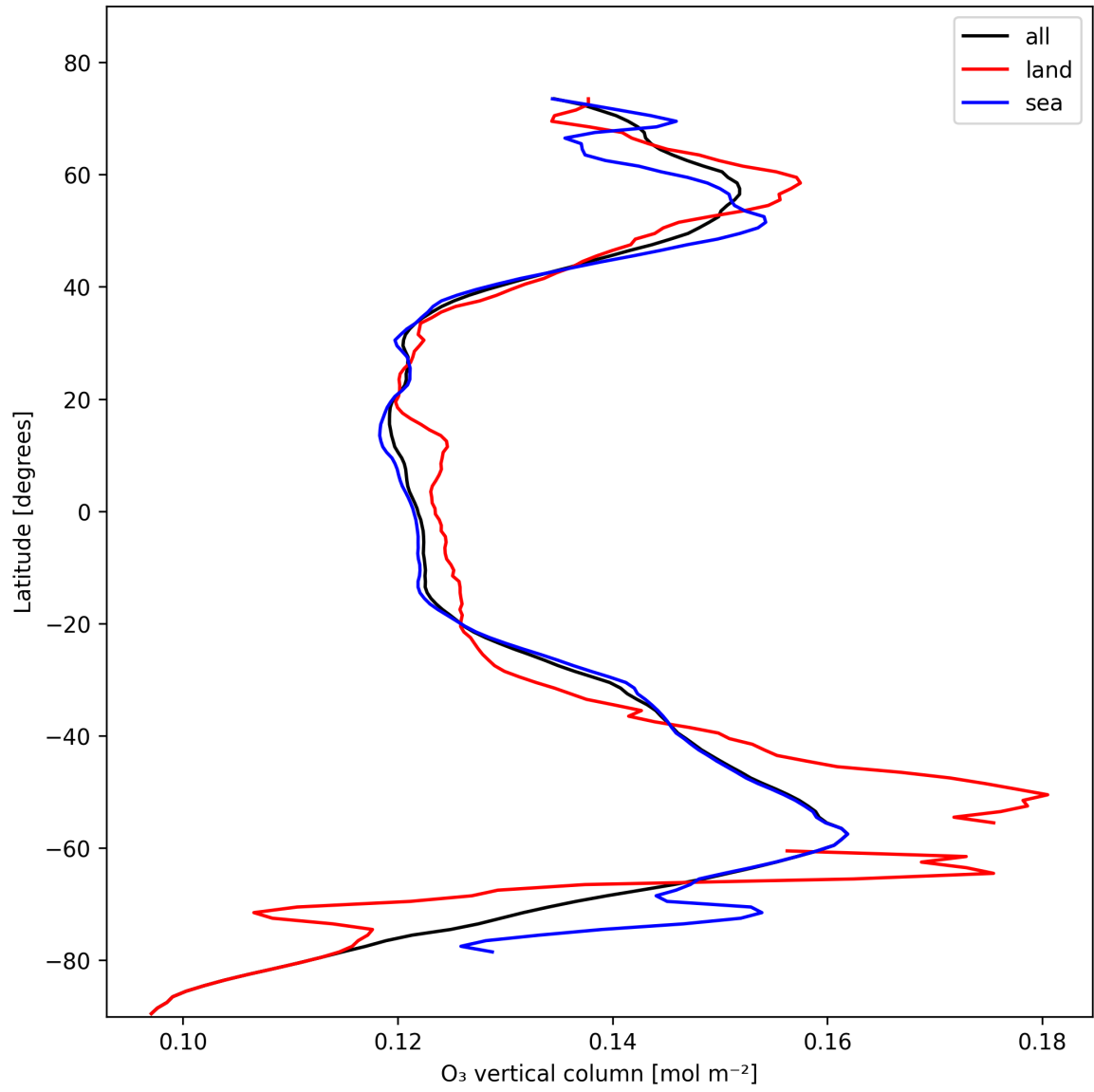
Figure 14: Zonal average of “O 3 vertical column” for 2024-11-02 to 2024-11-04.
