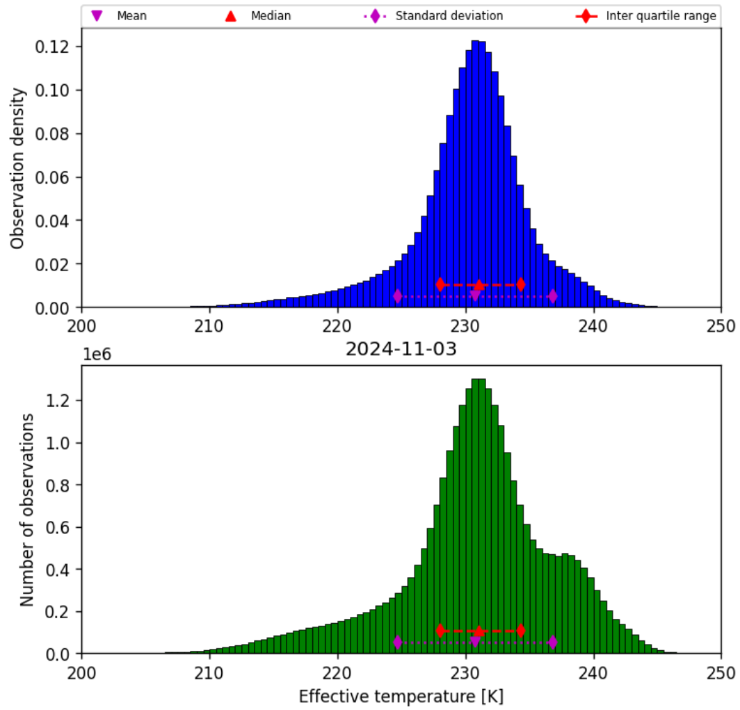
Figure 24: Histogram of “Effective temperature” for 2024-11-02 to 2024-11-04
