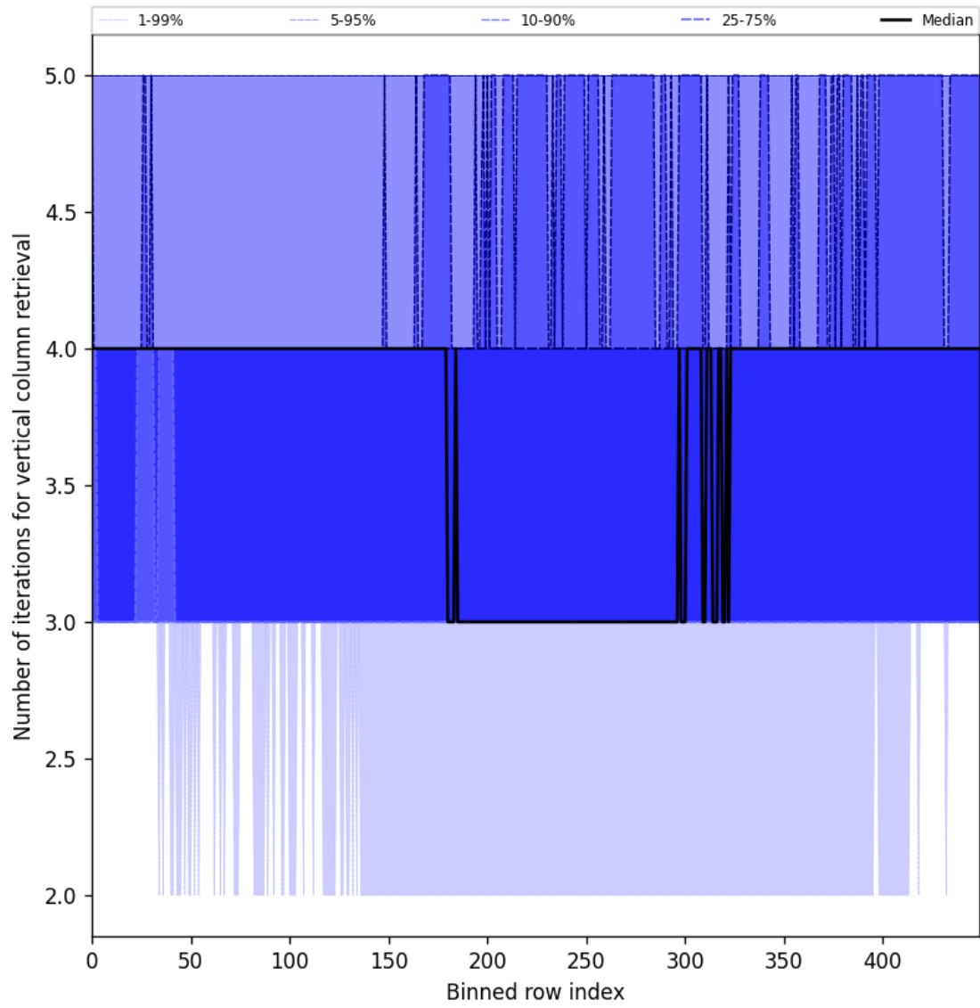
Figure 33: Along track statistics of “Number of iterations for vertical column retrieval” for 2024-11-02 to 2024-11-04
