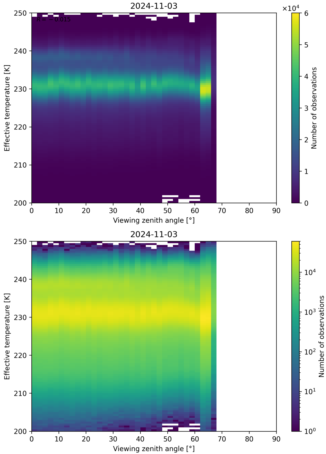
Figure 50: Scatter density plot of “Viewing zenith angle” against “Effective temperature” for 2024-11-02 to 2024-11-04.
