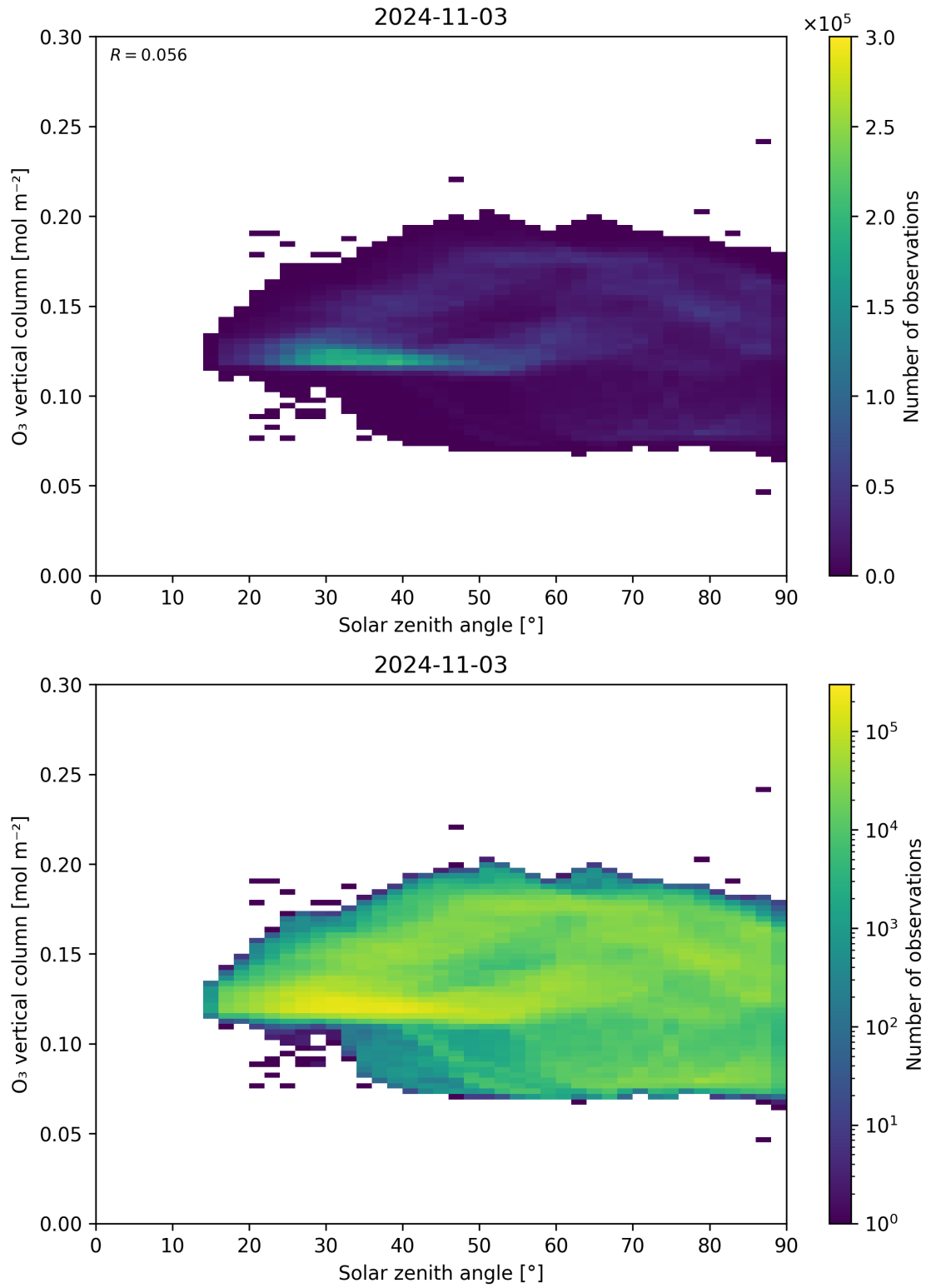
Figure 47: Scatter density plot of “Solar zenith angle” against “O 3 vertical column” for 2024-11-02 to 2024-11-04.
