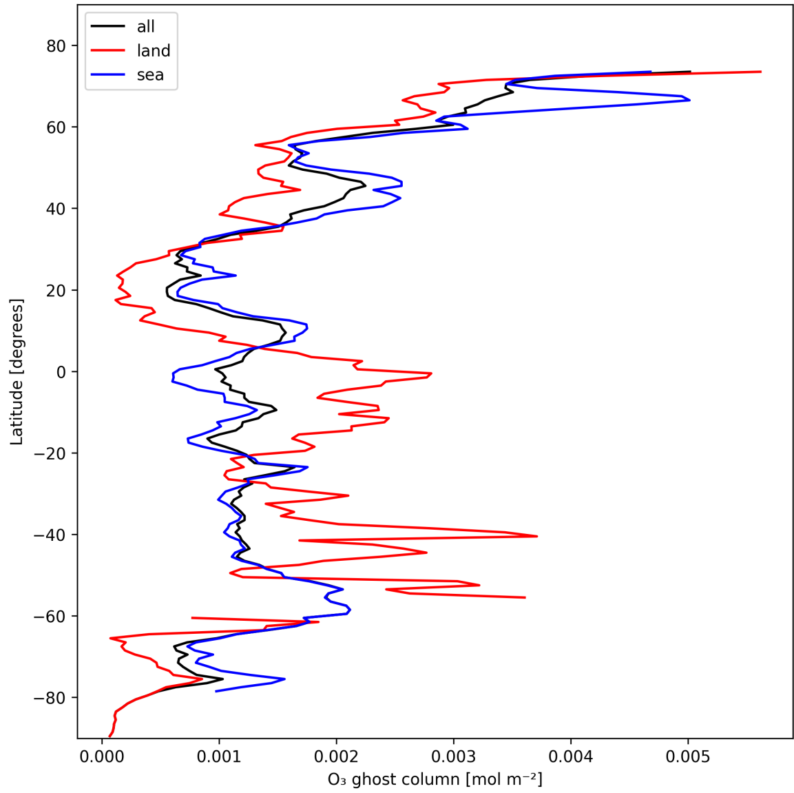
Figure 18: Zonal average of "O 3 ghost column" for 2024-11-02 to 2024-11-04.
