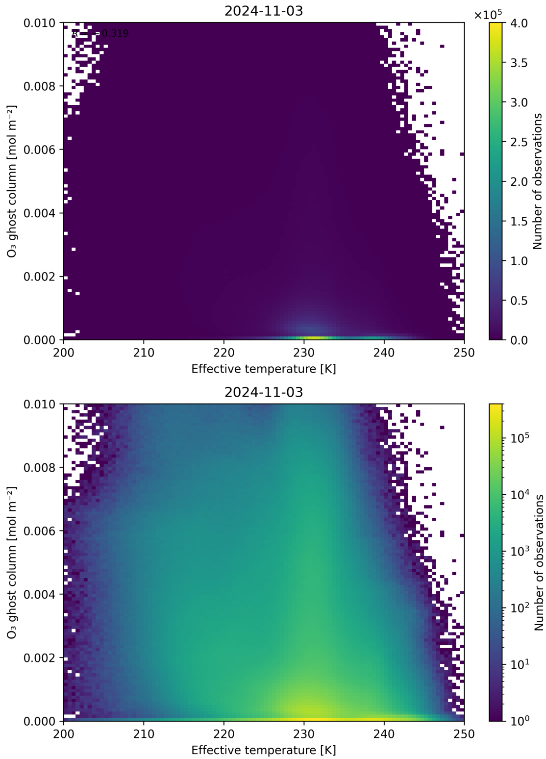
Figure 38: Scatter density plot of “Effective temperature” against “O 3 ghost column” for 2024-11-02 to 2024-11-04.
