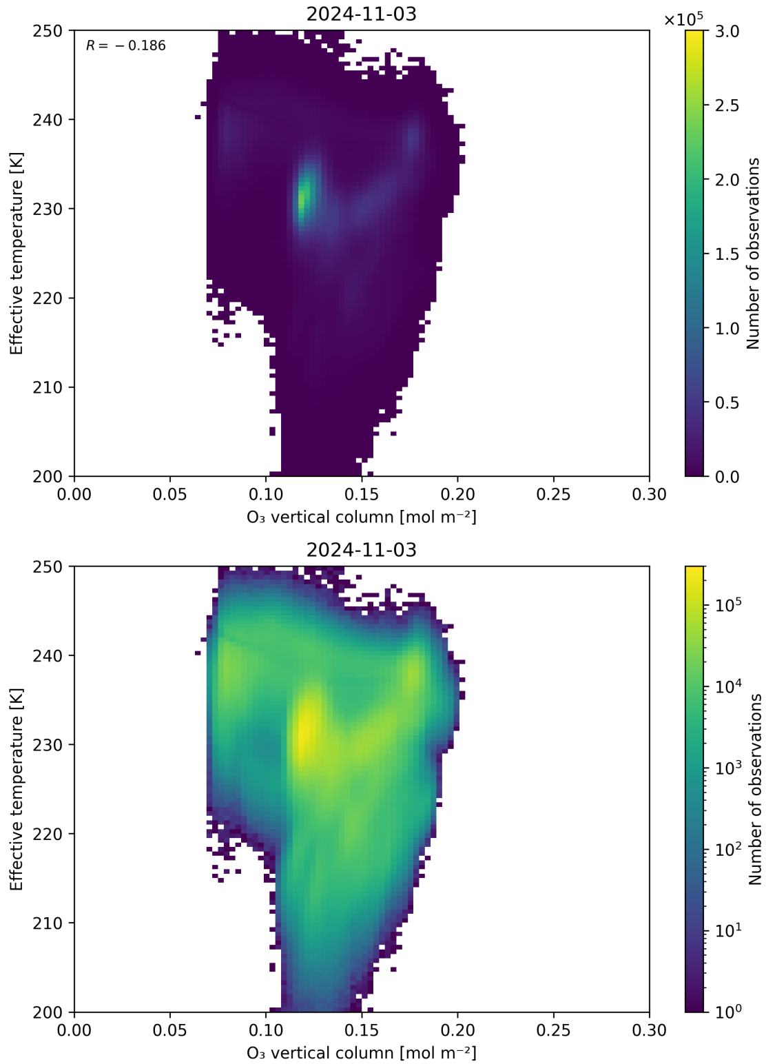
Figure 39: Scatter density plot of “O 3 vertical column” against “Effective temperature” for 2024-11-02 to 2024-11-04.
