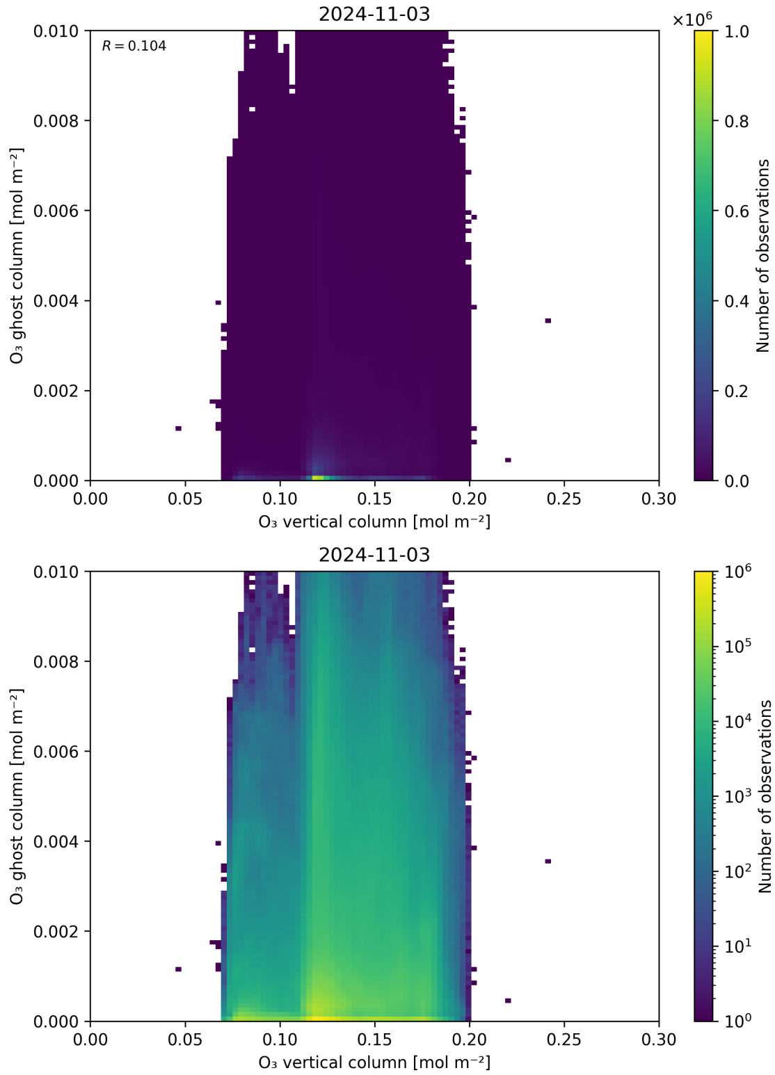
Figure 40: Scatter density plot of “O 3 vertical column” against “O 3 ghost column” for 2024-11-02 to 2024-11-04.
