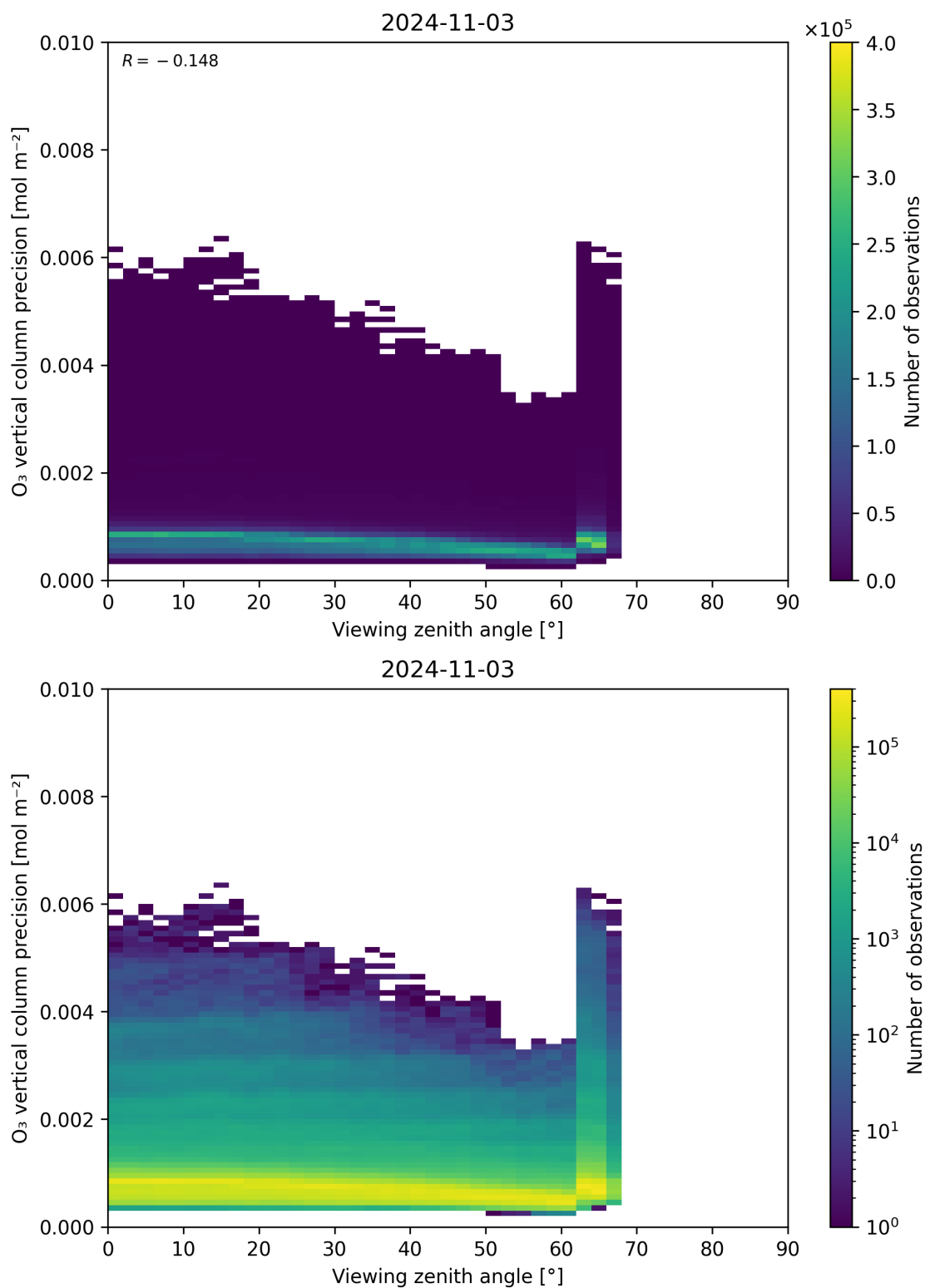
Figure 53: Scatter density plot of “Viewing zenith angle” against “O 3 vertical column precision” for 2024-11-02 to 2024-11-04.
