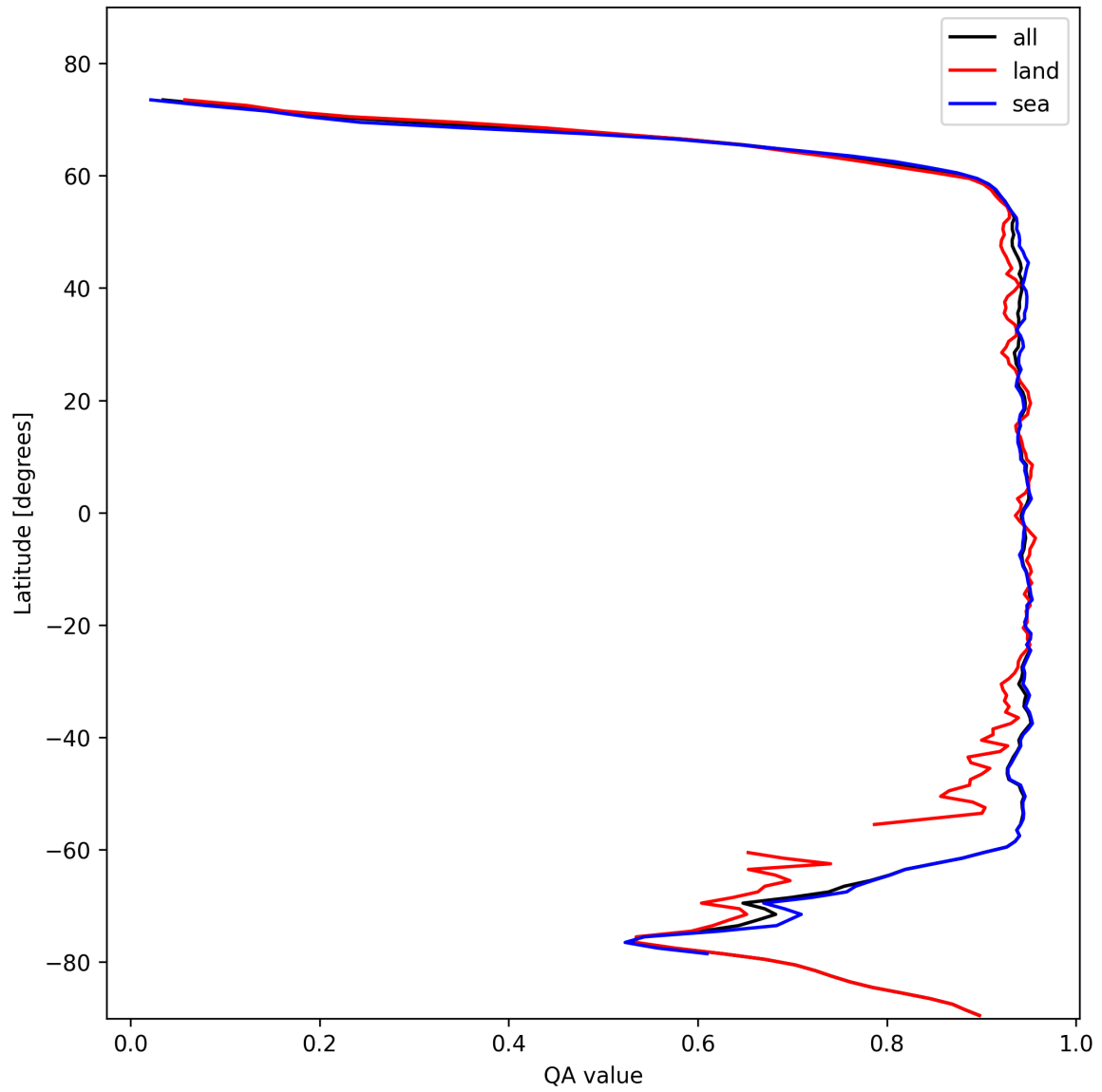
Figure 13: Zonal average of “QA value” for 2024-11-02 to 2024-11-04.
