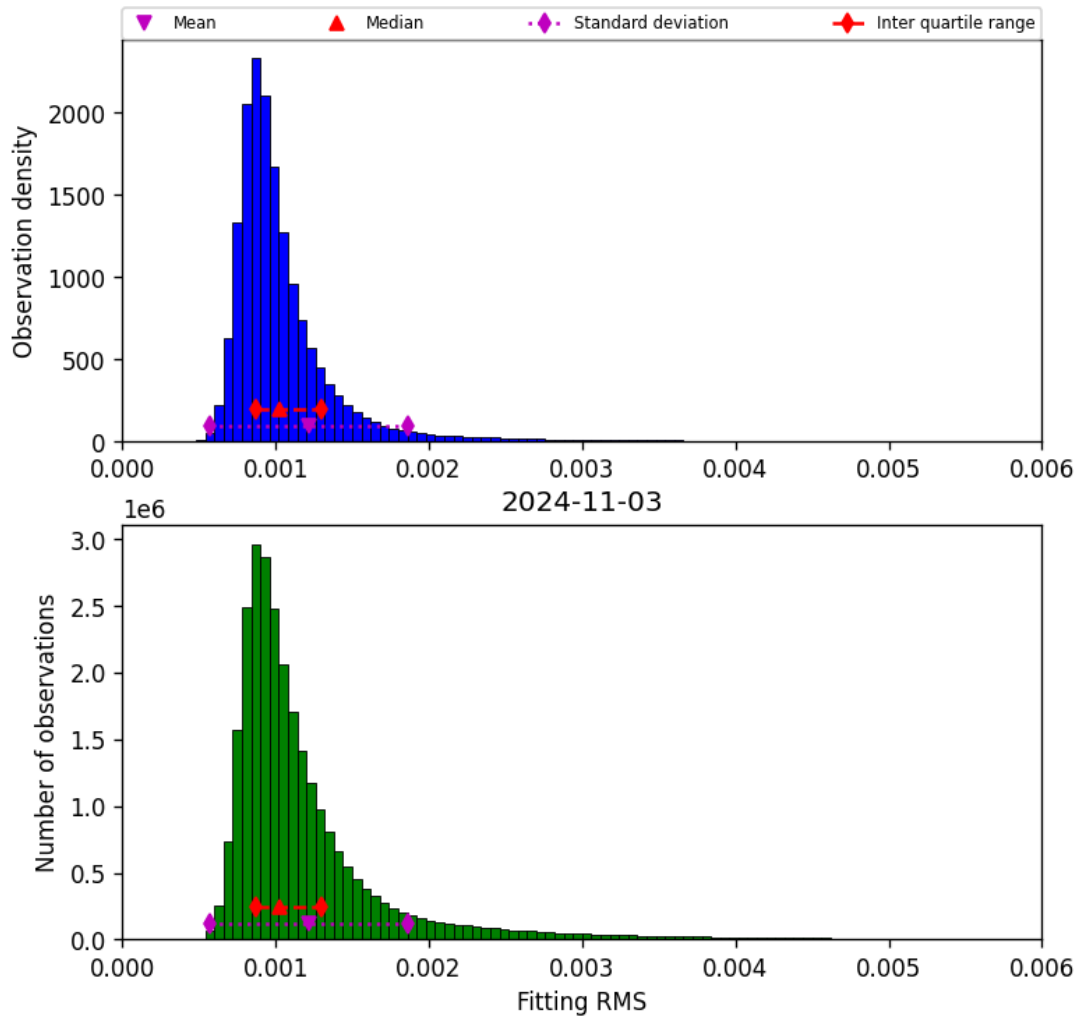
Figure 23: Histogram of “Fitting RMS” for 2024-11-02 to 2024-11-04
