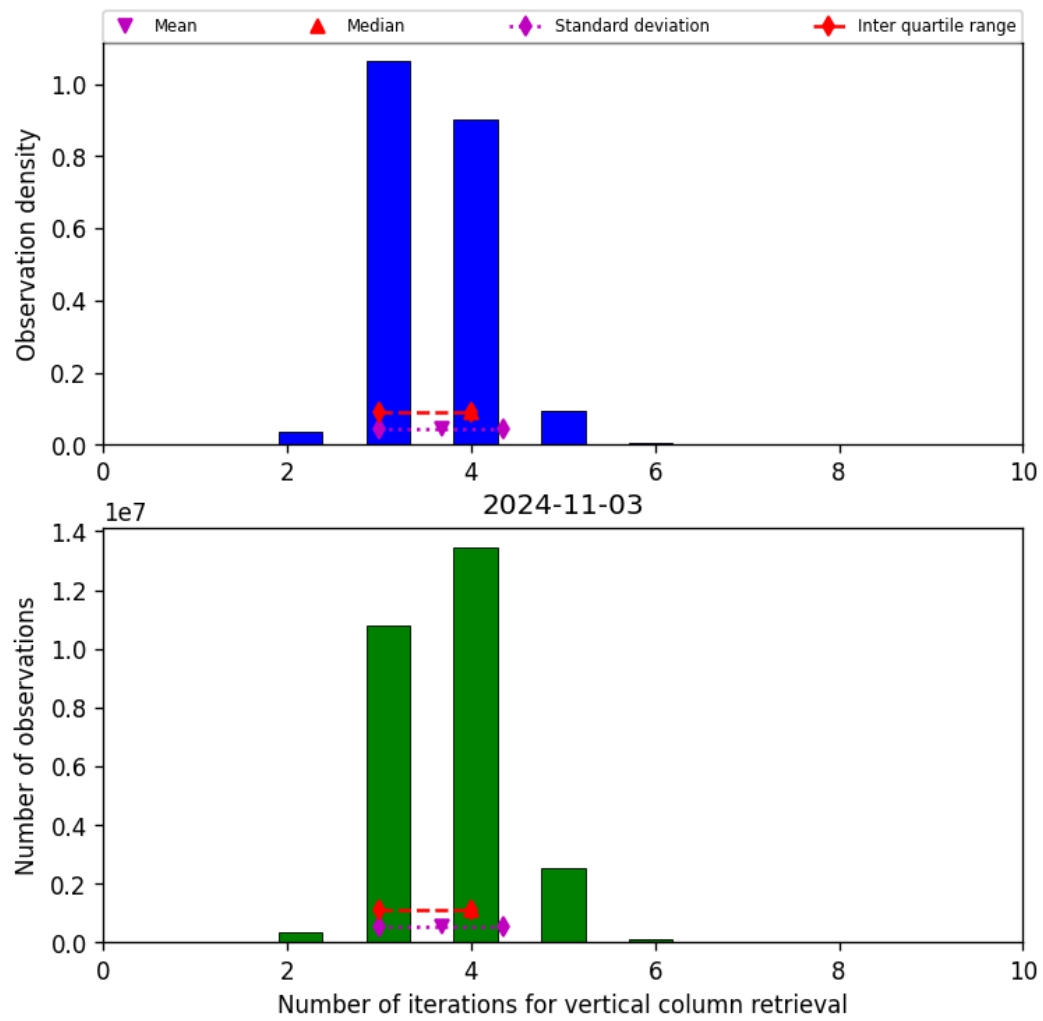
Figure 26: Histogram of “Number of iterations for vertical column retrieval” for 2024-11-02 to 2024-11-04
