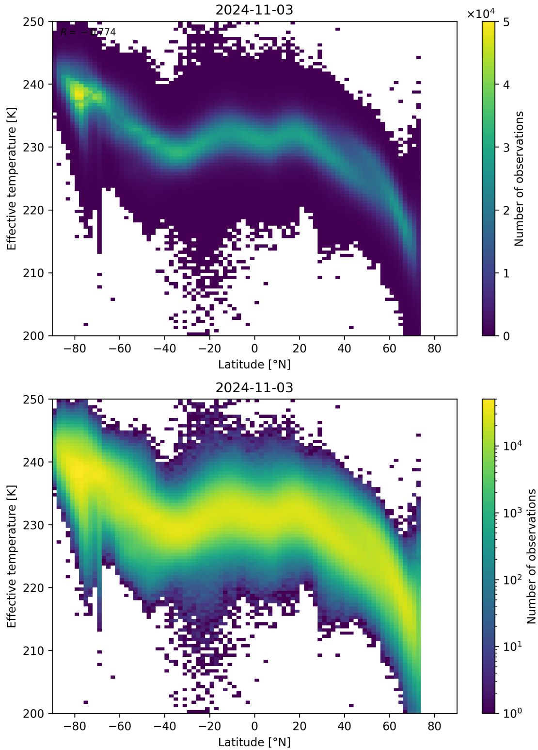
Figure 34: Scatter density plot of “Latitude” against “Effective temperature” for 2024-11-02 to 2024-11-04.
