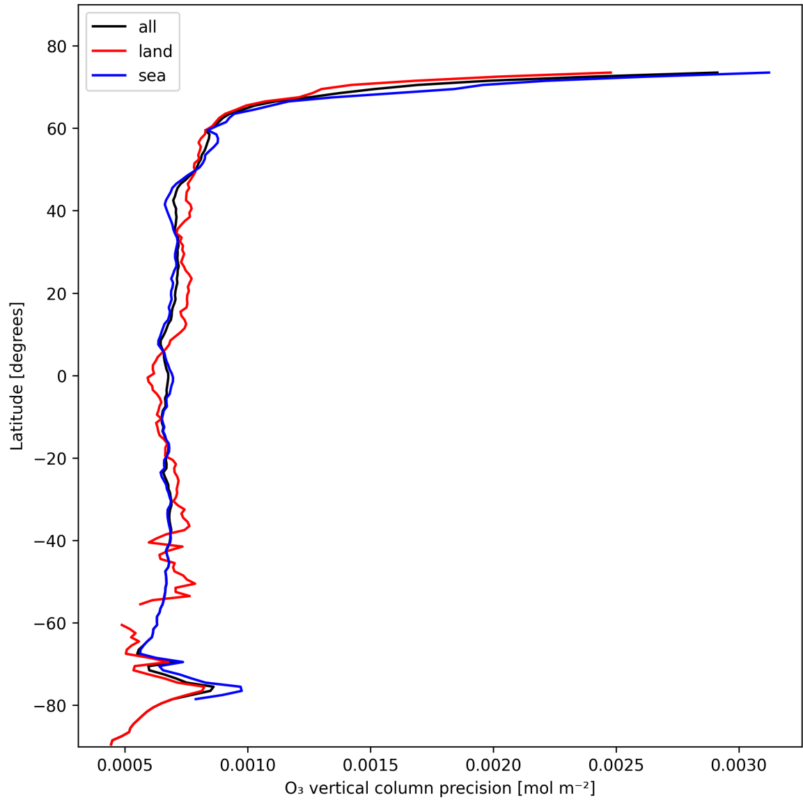
Figure 15: Zonal average of “O 3 vertical column precision” for 2024-11-02 to 2024-11-04.
