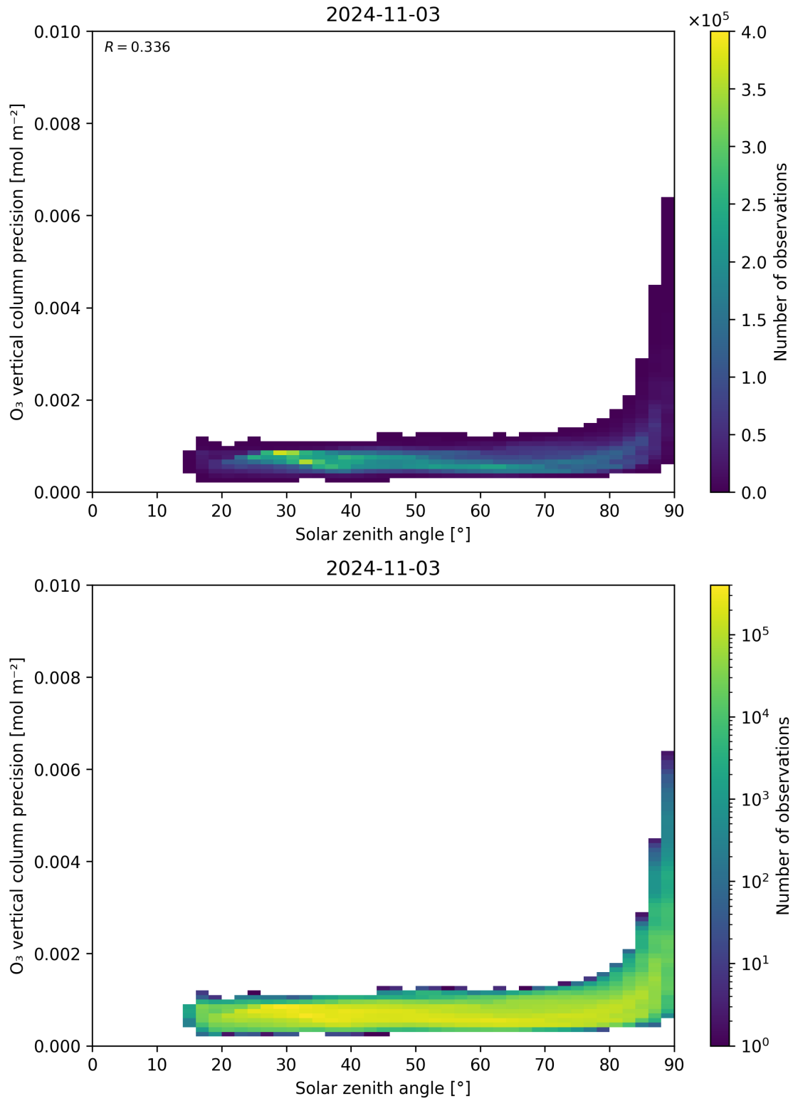
Figure 48: Scatter density plot of “Solar zenith angle” against “O 3 vertical column precision” for 2024-11-02 to 2024-11-04.
