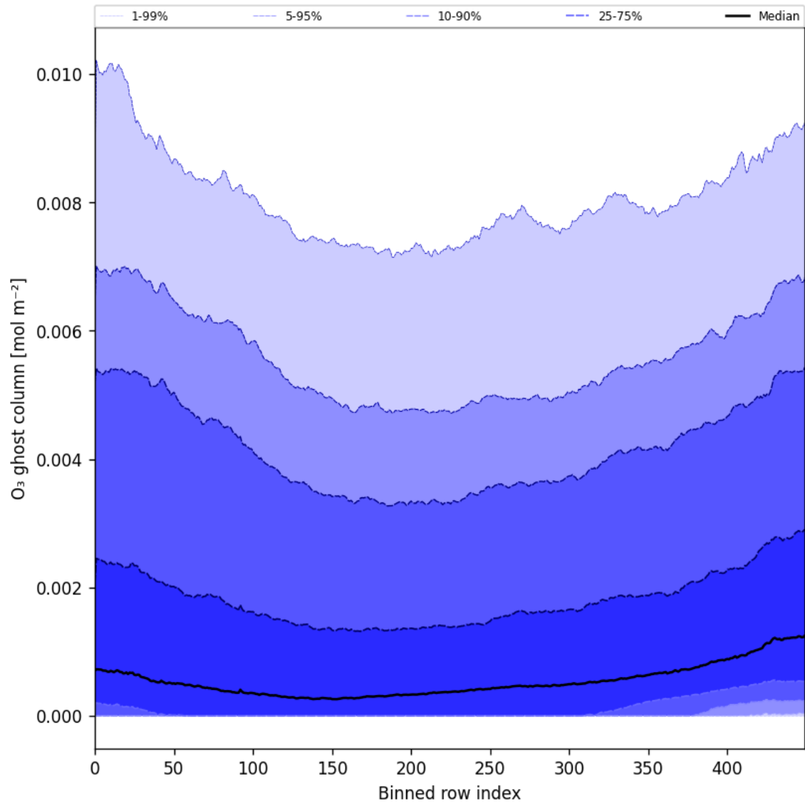
Figure 32: Along track statistics of "O 3 ghost column" for 2024-11-02 to 2024-11-04
