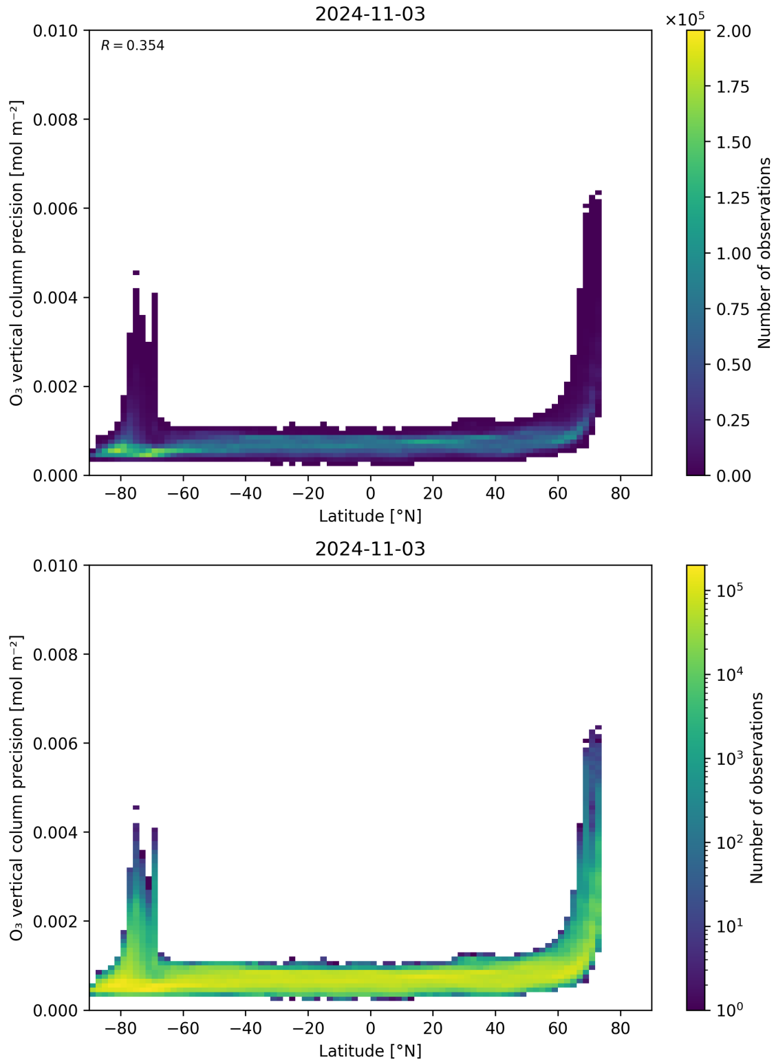
Figure 37: Scatter density plot of “Latitude” against “O 3 vertical column precision” for 2024-11-02 to 2024-11-04.
