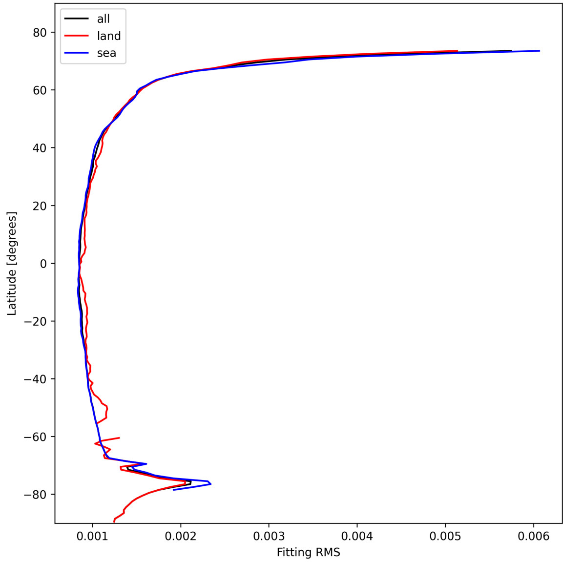
Figure 16: Zonal average of “Fitting RMS” for 2024-11-02 to 2024-11-04.
