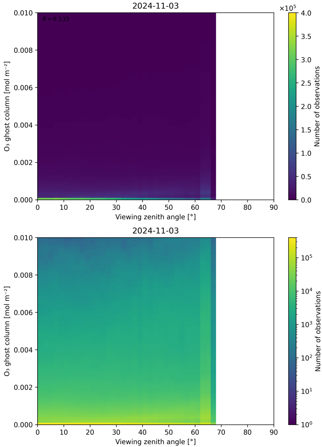
Figure 51: Scatter density plot of “Viewing zenith angle” against “O 3 ghost column” for 2024-11-02 to 2024-11-04.
