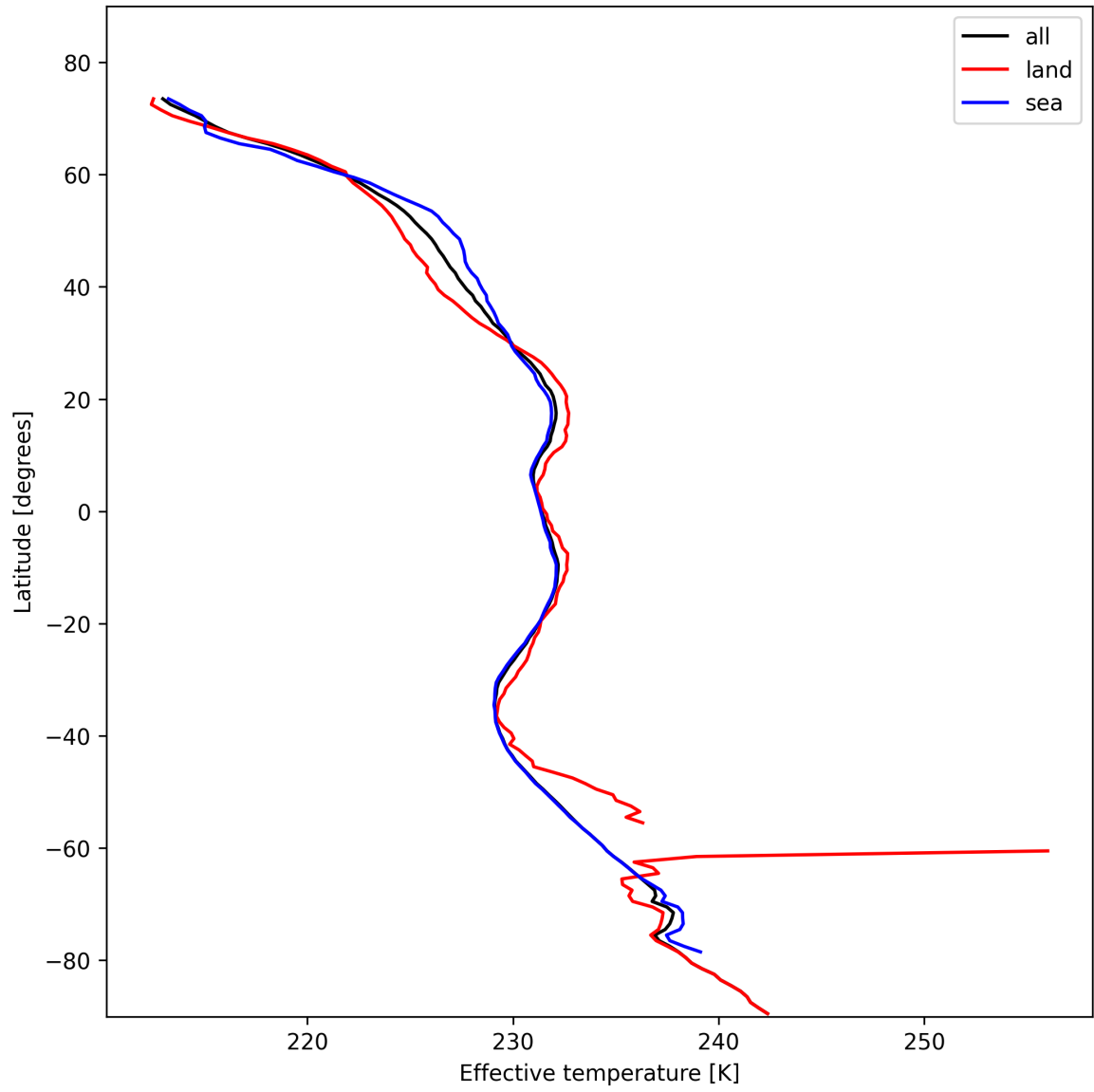
Figure 17: Zonal average of "Effective temperature" for 2024-11-02 to 2024-11-04.
