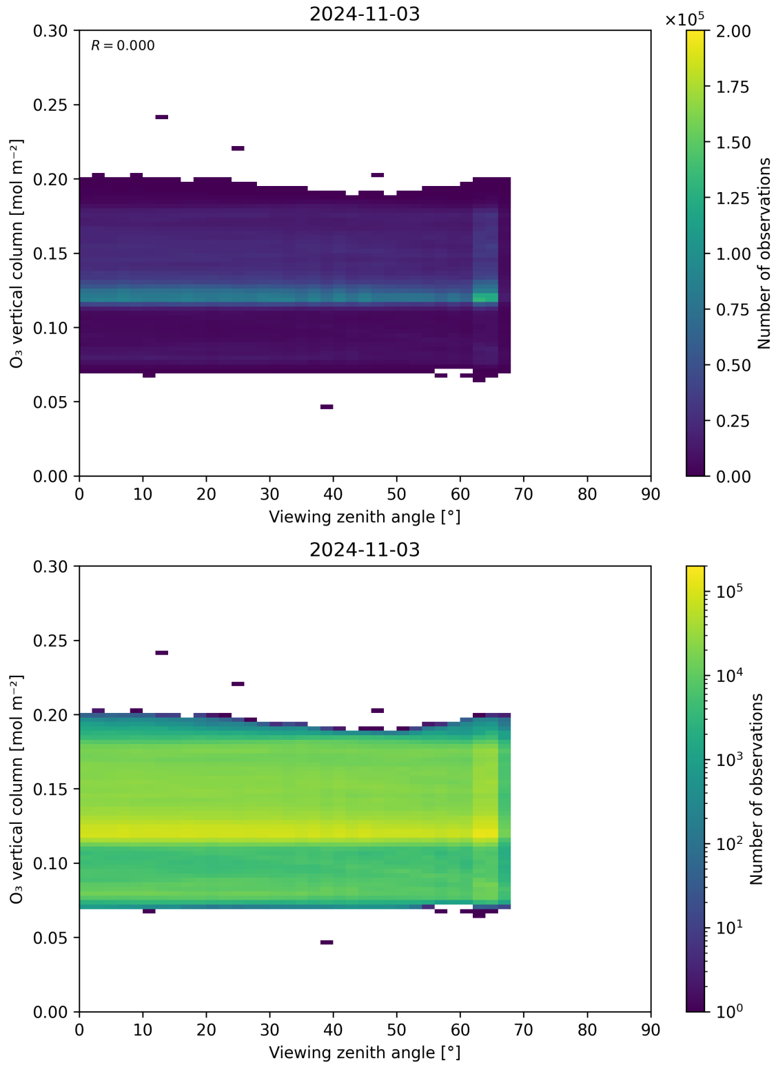
Figure 52: Scatter density plot of “Viewing zenith angle” against “O 3 vertical column” for 2024-11-02 to 2024-11-04.
