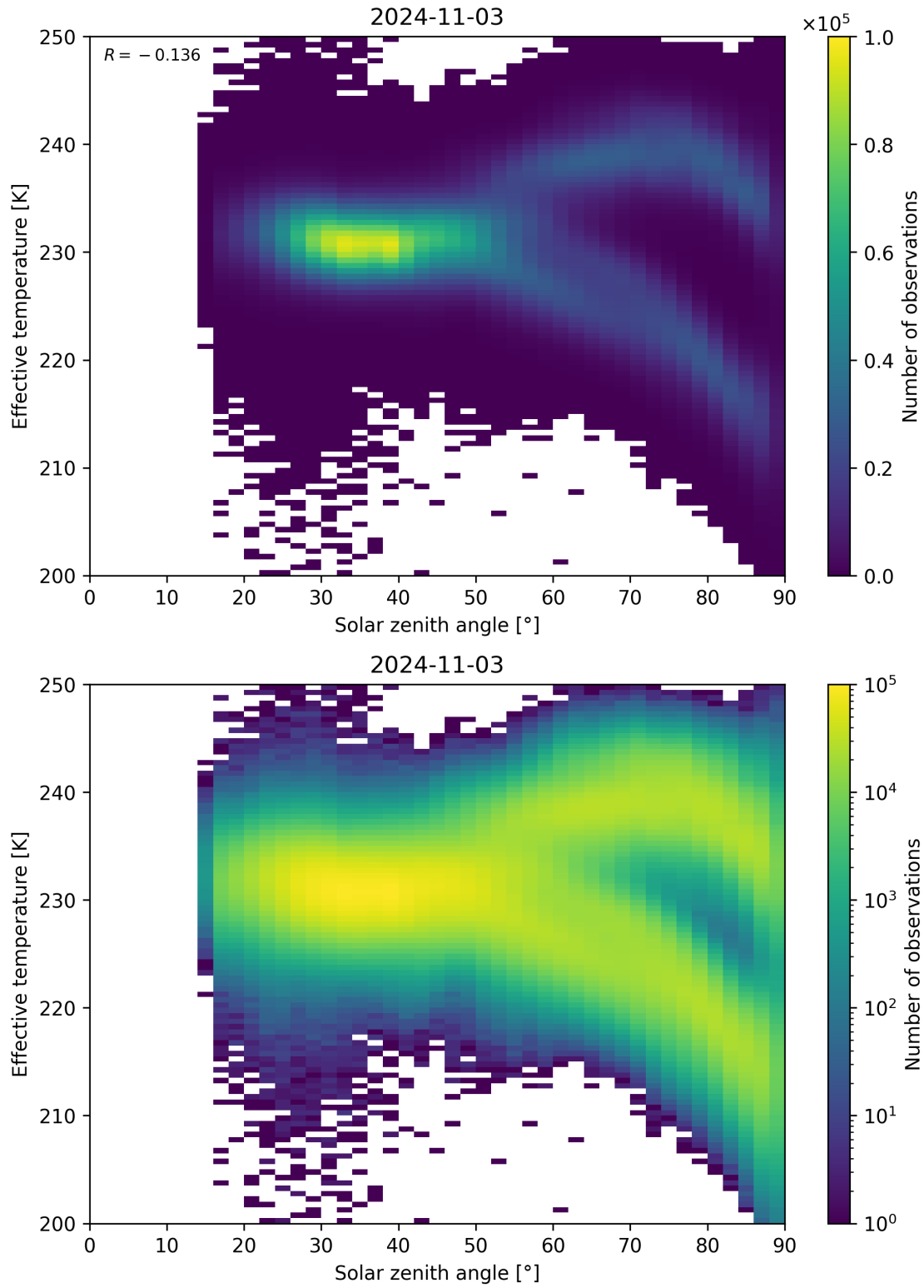
Figure 45: Scatter density plot of “Solar zenith angle” against “Effective temperature” for 2024-11-02 to 2024-11-04.
