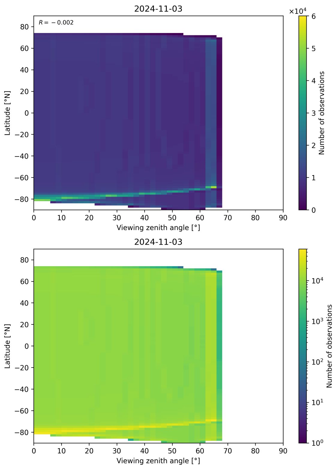
Figure 49: Scatter density plot of “Viewing zenith angle” against “Latitude” for 2024-11-02 to 2024-11-04.
