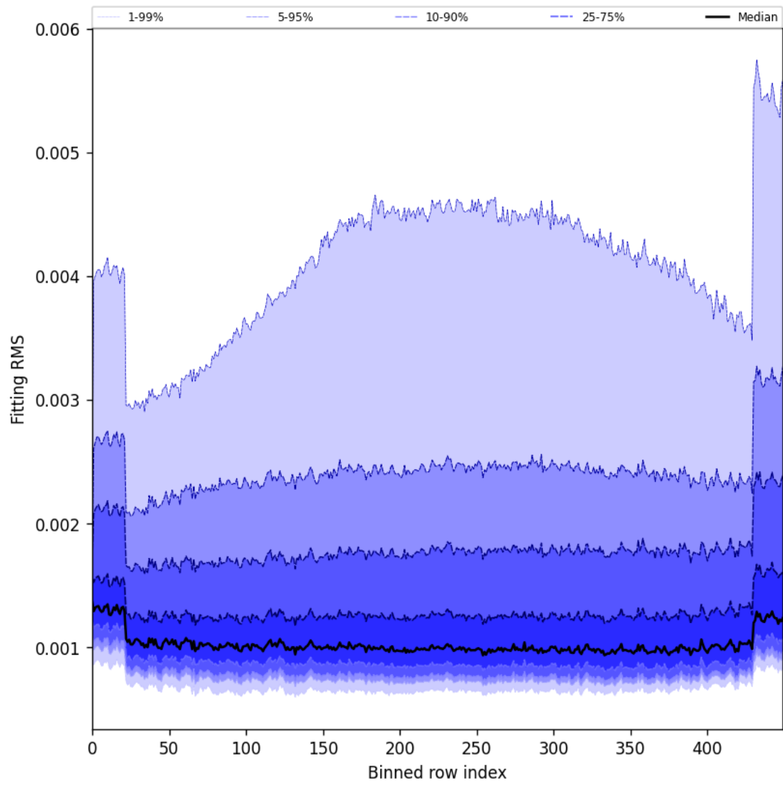
Figure 30: Along track statistics of “Fitting RMS” for 2024-11-02 to 2024-11-04
