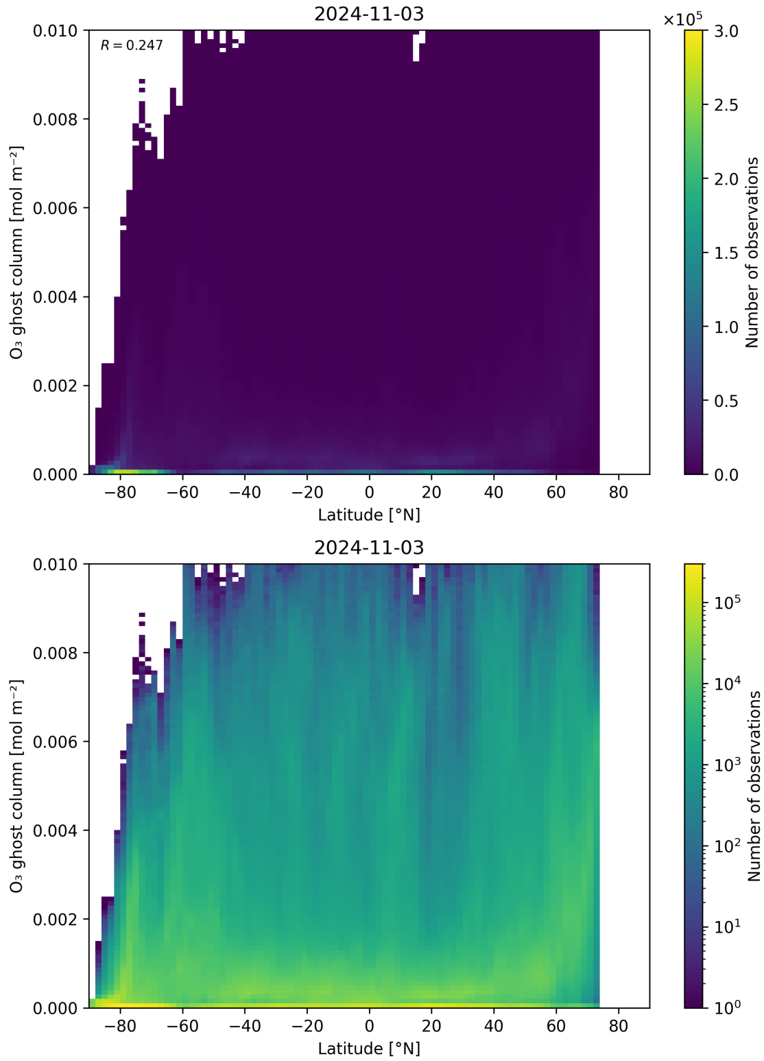
Figure 35: Scatter density plot of “Latitude” against “O 3 ghost column” for 2024-11-02 to 2024-11-04.
