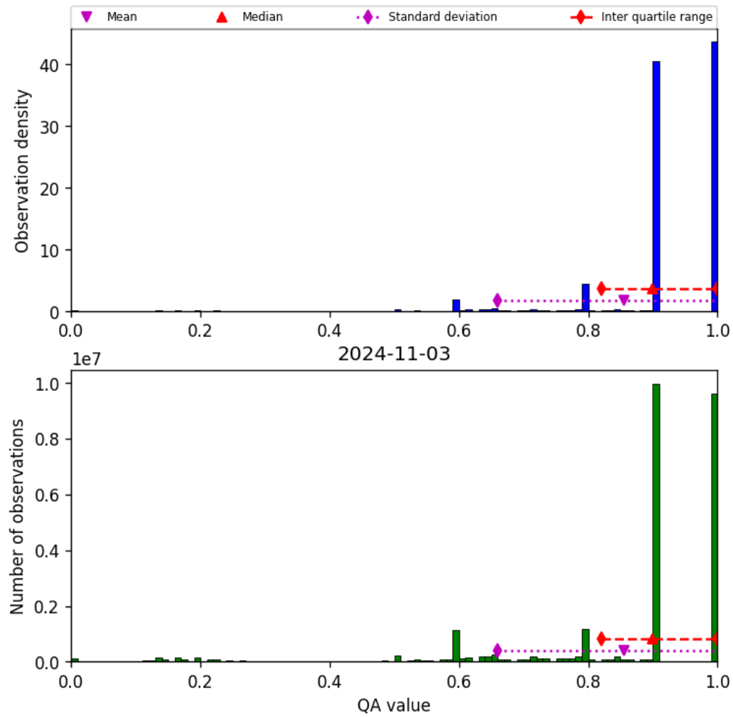
Figure 20: Histogram of “QA value” for 2024-11-02 to 2024-11-04
