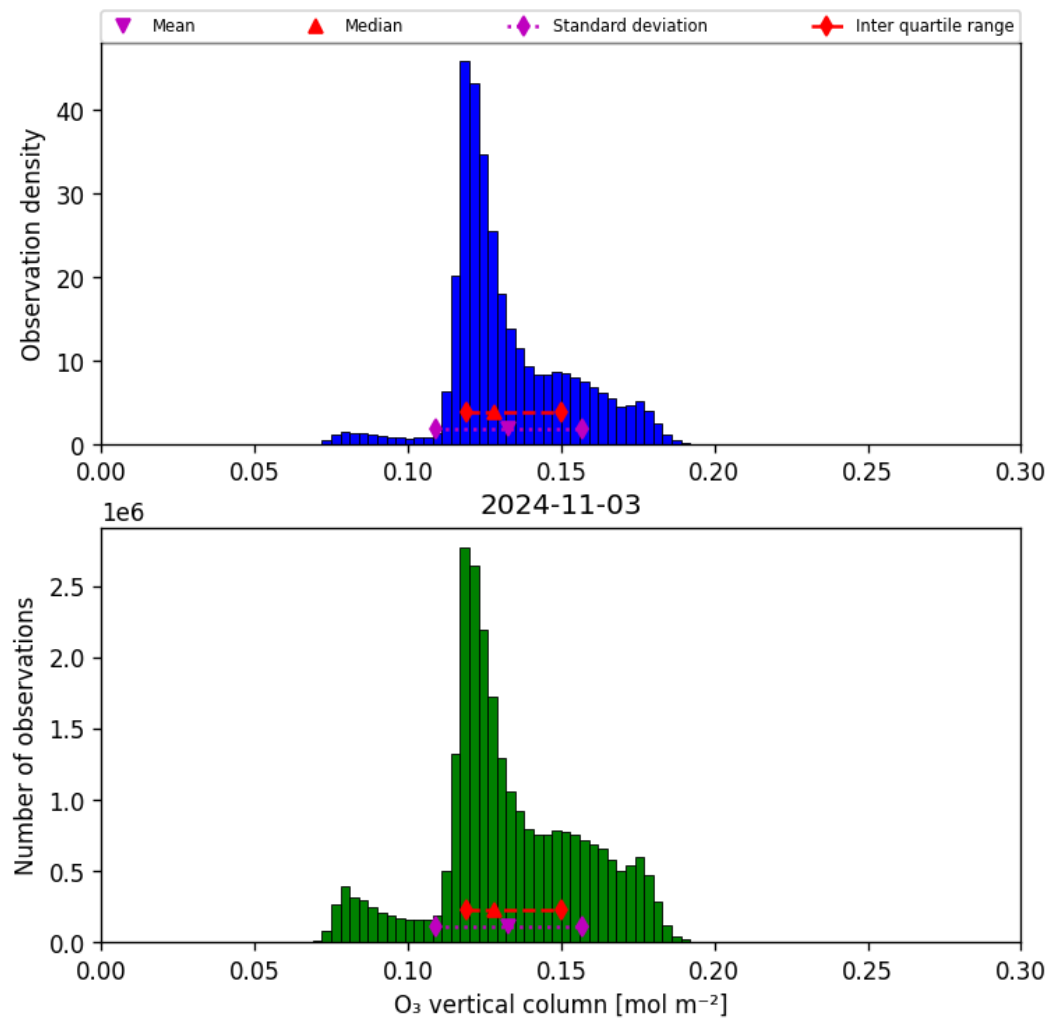
Figure 21: Histogram of “O 3 vertical column” for 2024-11-02 to 2024-11-04
