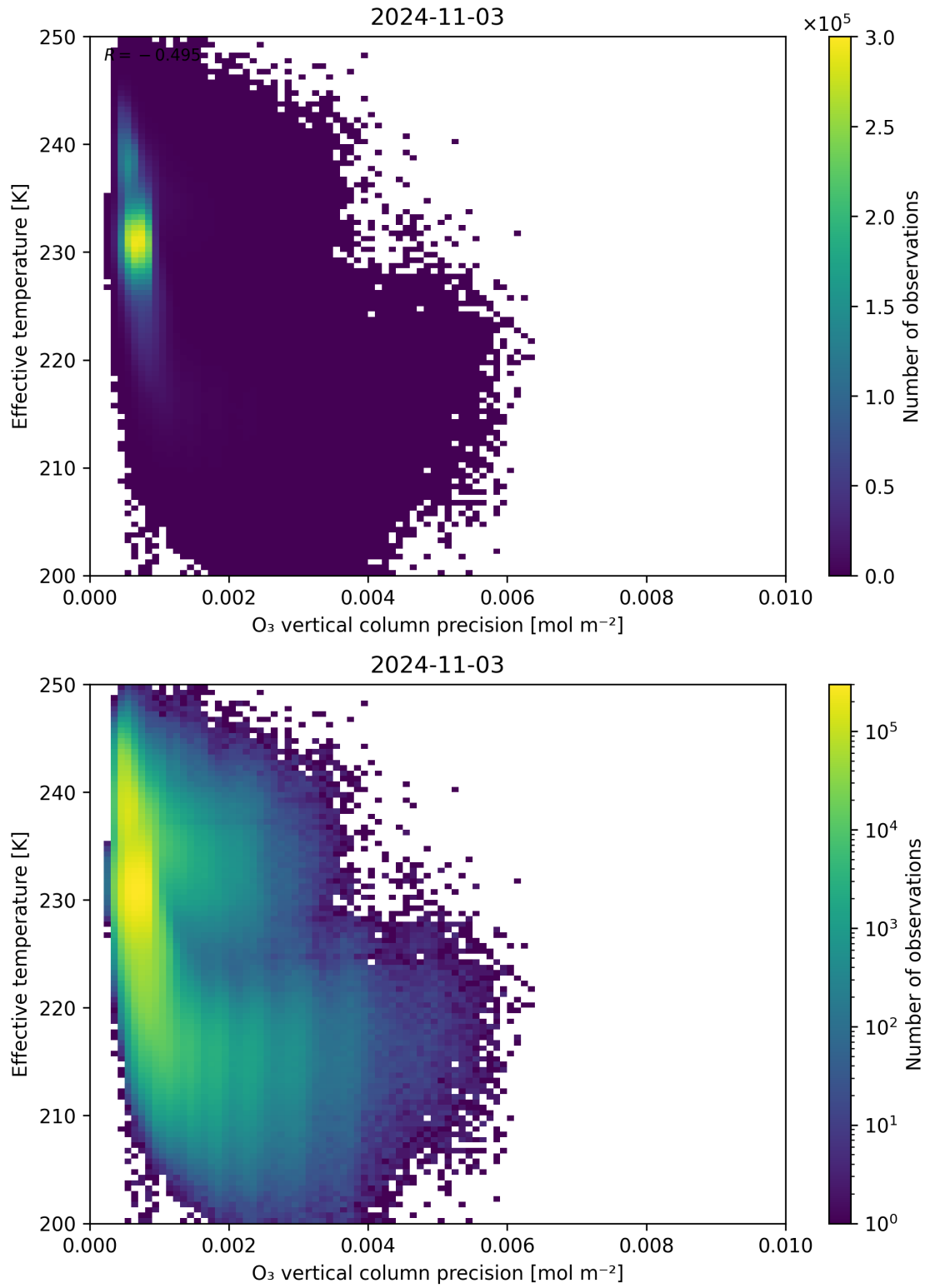
Figure 42: Scatter density plot of “O 3 vertical column precision” against “Effective temperature” for 2024-11-02 to 2024-11-04.
