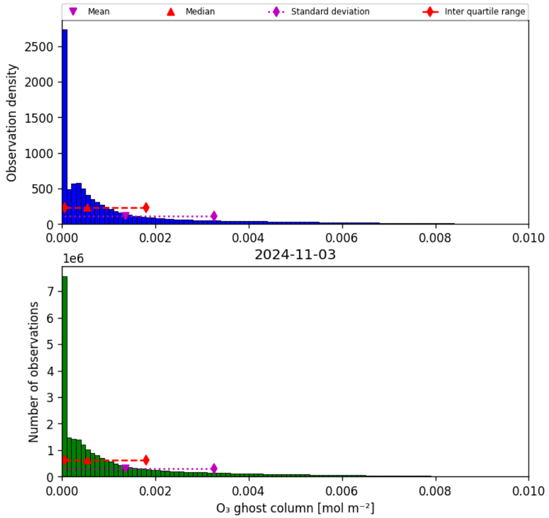
Figure 25: Histogram of “O 3 ghost column” for 2024-11-02 to 2024-11-04
