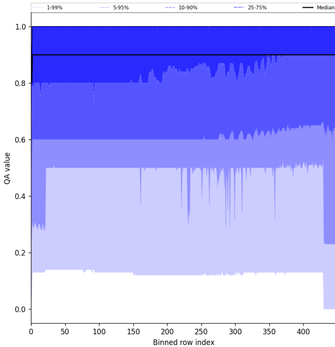
Figure 27: Along track statistics of “QA value” for 2024-11-02 to 2024-11-04
