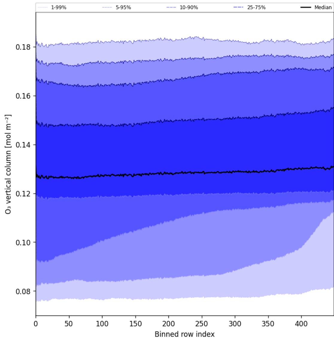
Figure 28: Along track statistics of “O 3 vertical column” for 2024-11-02 to 2024-11-04
