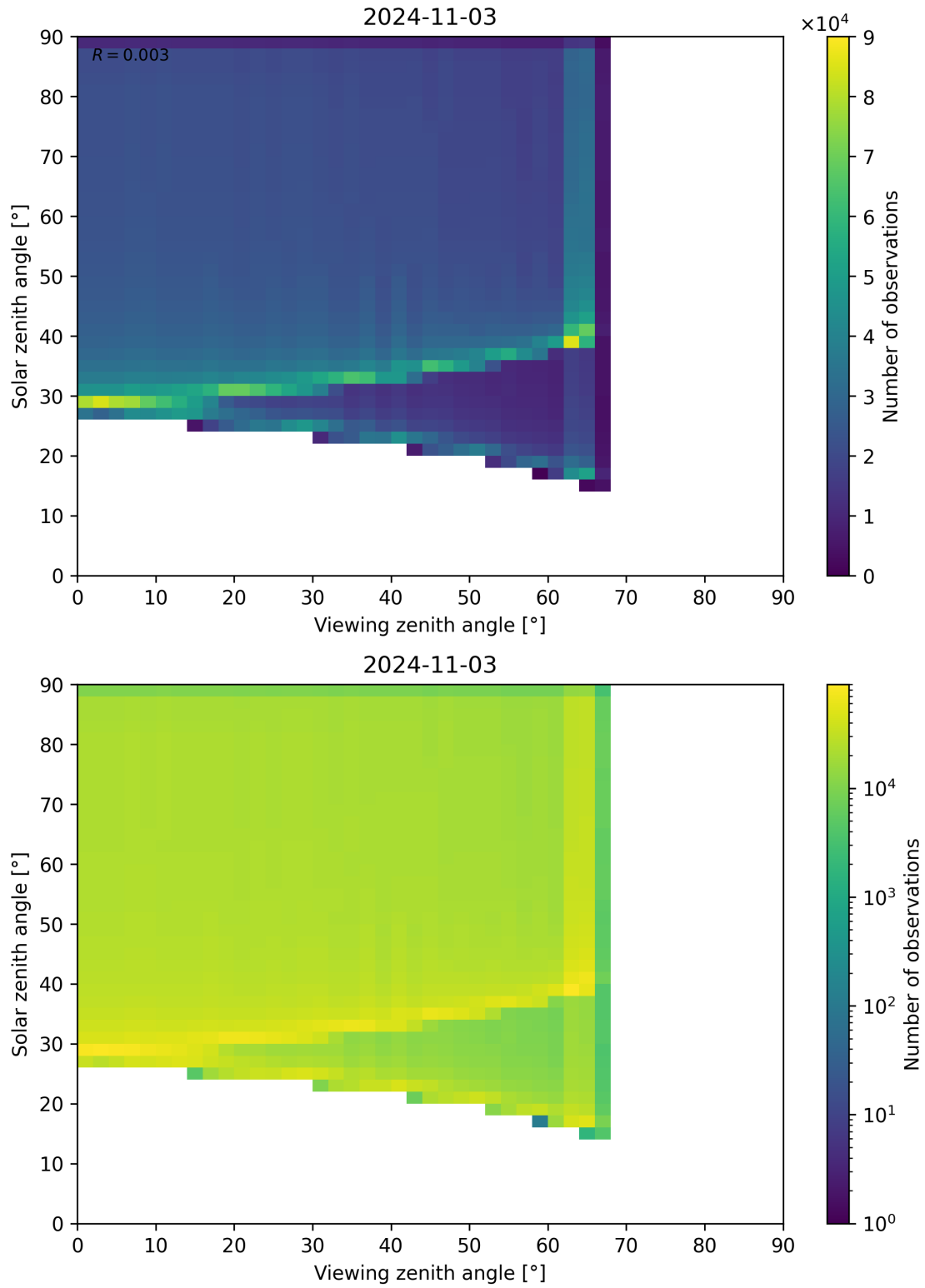
Figure 54: Scatter density plot of “Viewing zenith angle” against “Solar zenith angle” for 2024-11-02 to 2024-11-04.
