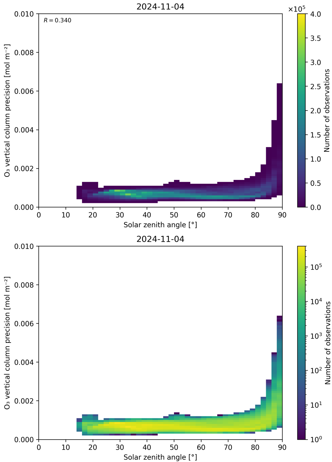
Figure 48: Scatter density plot of “Solar zenith angle” against “O 3 vertical column precision” for 2024-11-04 to 2024-11-05.
