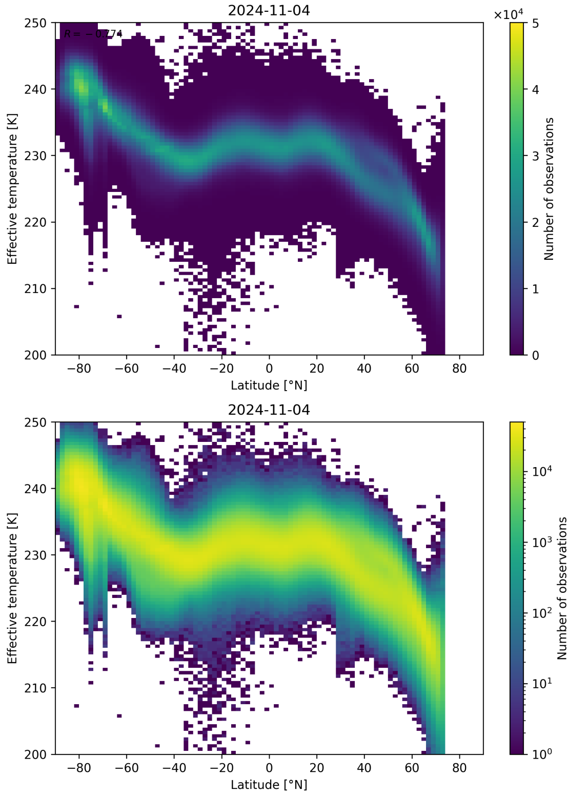
Figure 34: Scatter density plot of “Latitude” against “Effective temperature” for 2024-11-04 to 2024-11-05.
