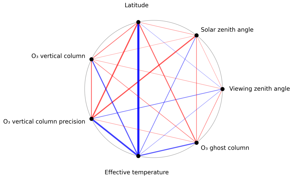
Figure 1: Map of correlation graph for 2024-11-04 to 2024-11-05.
