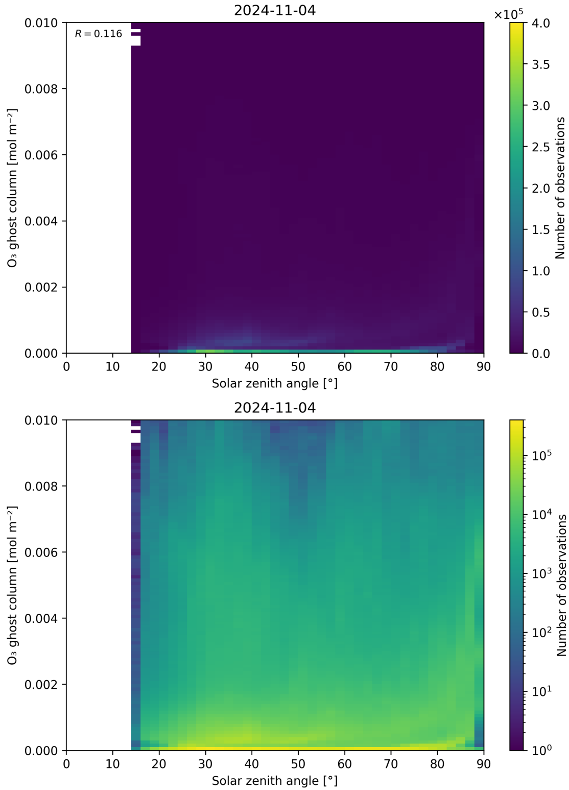
Figure 46: Scatter density plot of “Solar zenith angle” against “O 3 ghost column” for 2024-11-04 to 2024-11-05.
