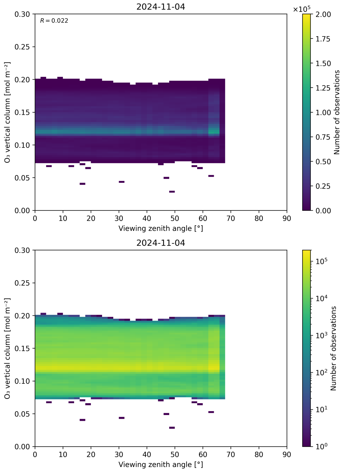
Figure 52: Scatter density plot of “Viewing zenith angle” against “O 3 vertical column” for 2024-11-04 to 2024-11-05.
