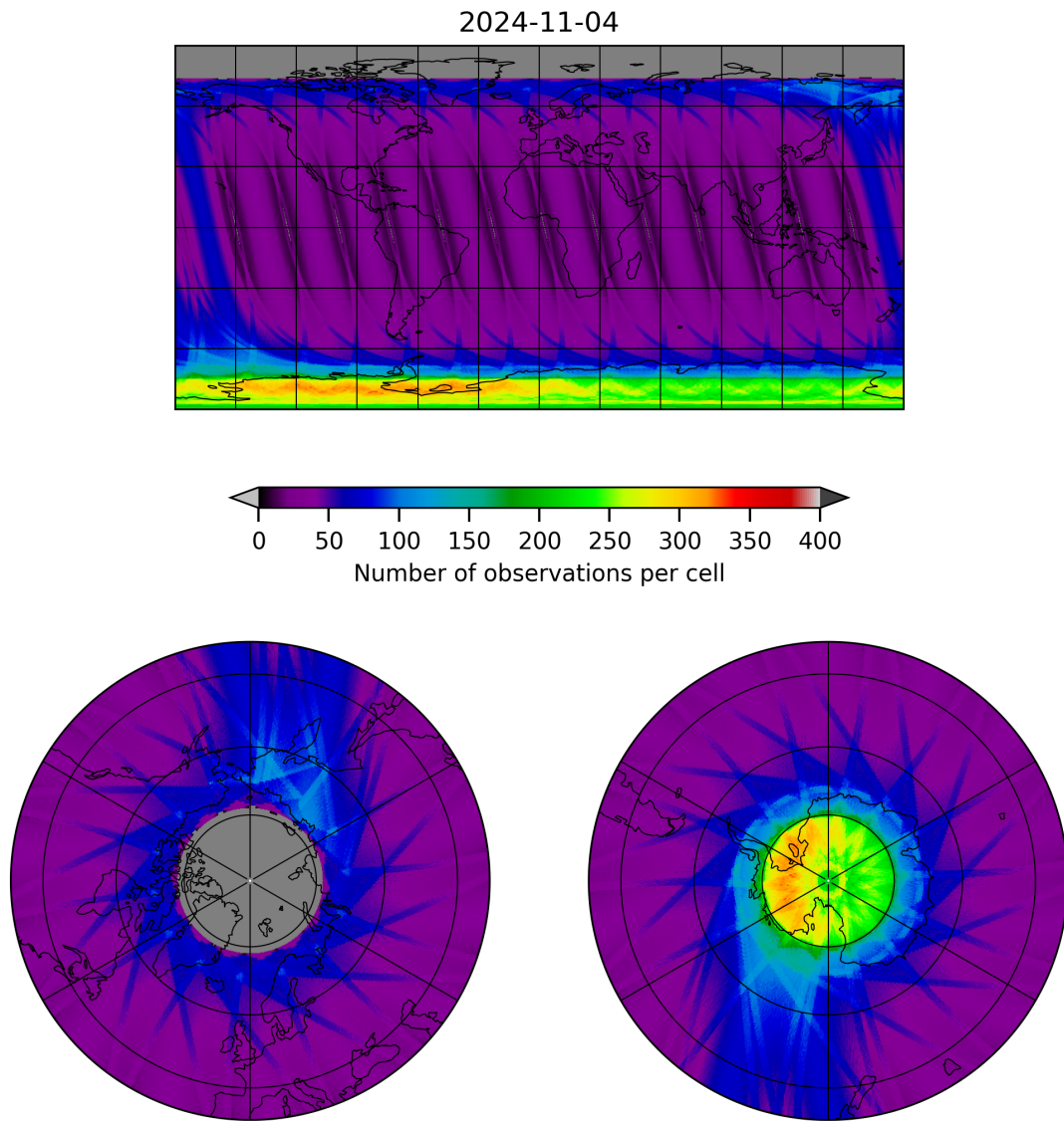
Figure 12: Map of the number of observations for 2024-11-04 to 2024-11-05
