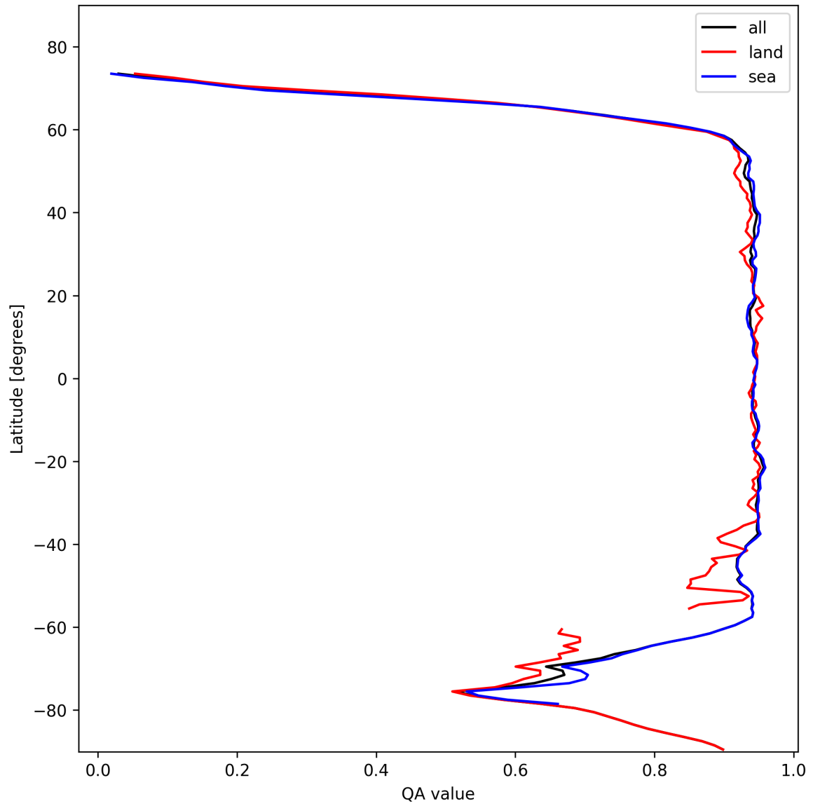
Figure 13: Zonal average of “QA value” for 2024-11-04 to 2024-11-05.
