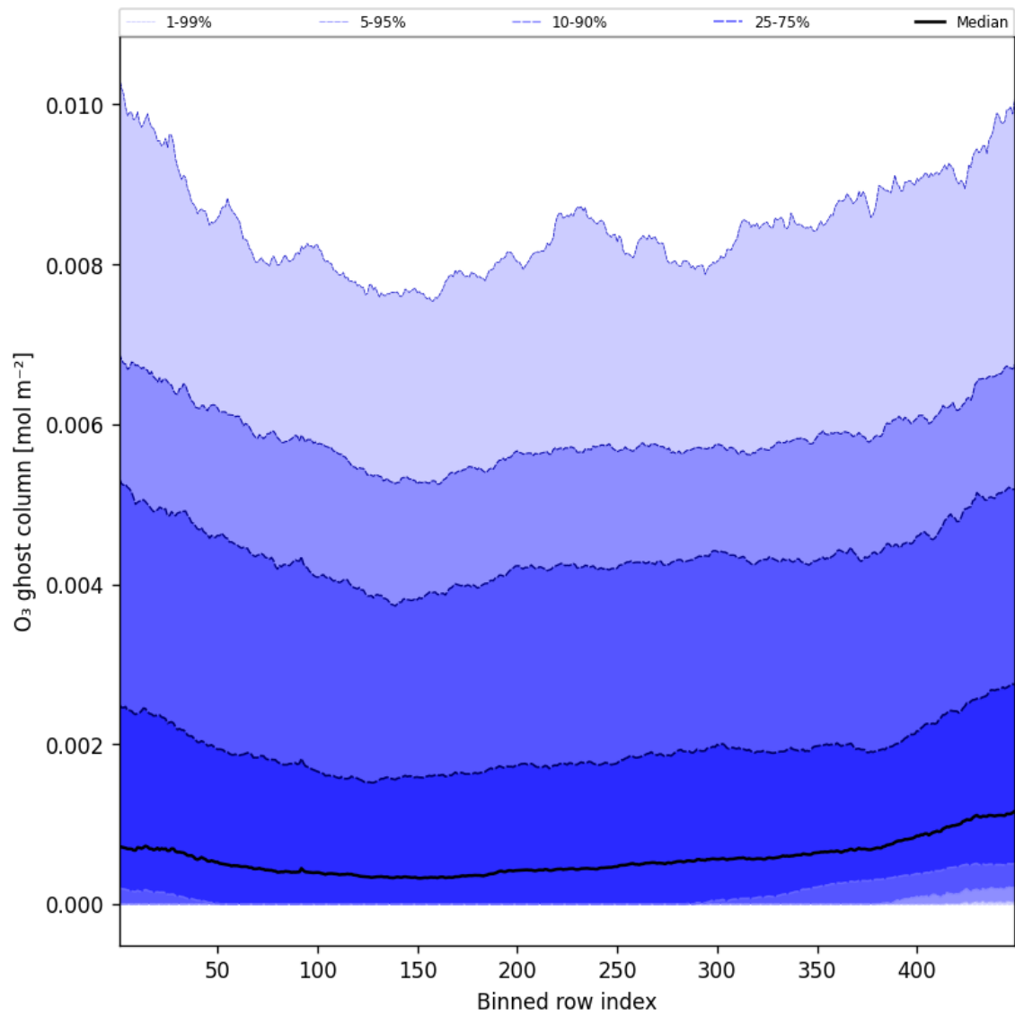
Figure 32: Along track statistics of “O 3 ghost column” for 2024-11-04 to 2024-11-05
