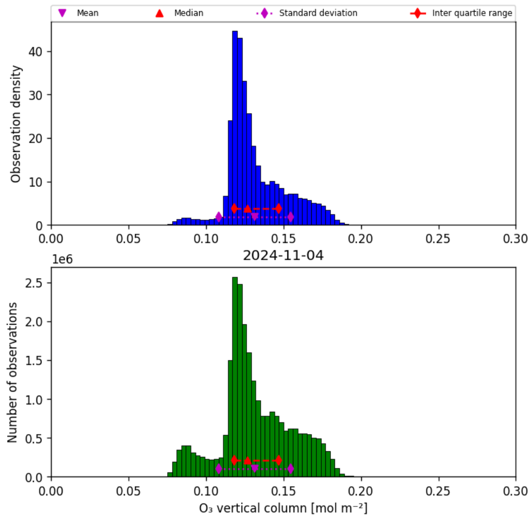
Figure 21: Histogram of “O 3 vertical column” for 2024-11-04 to 2024-11-05
