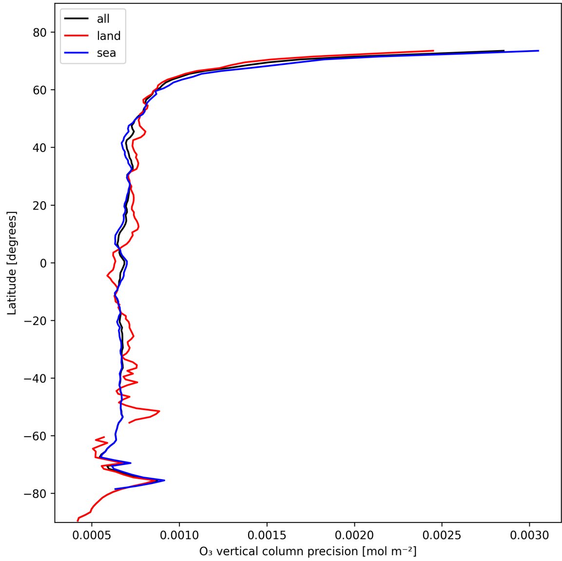
Figure 15: Zonal average of “O 3 vertical column precision” for 2024-11-04 to 2024-11-05.
