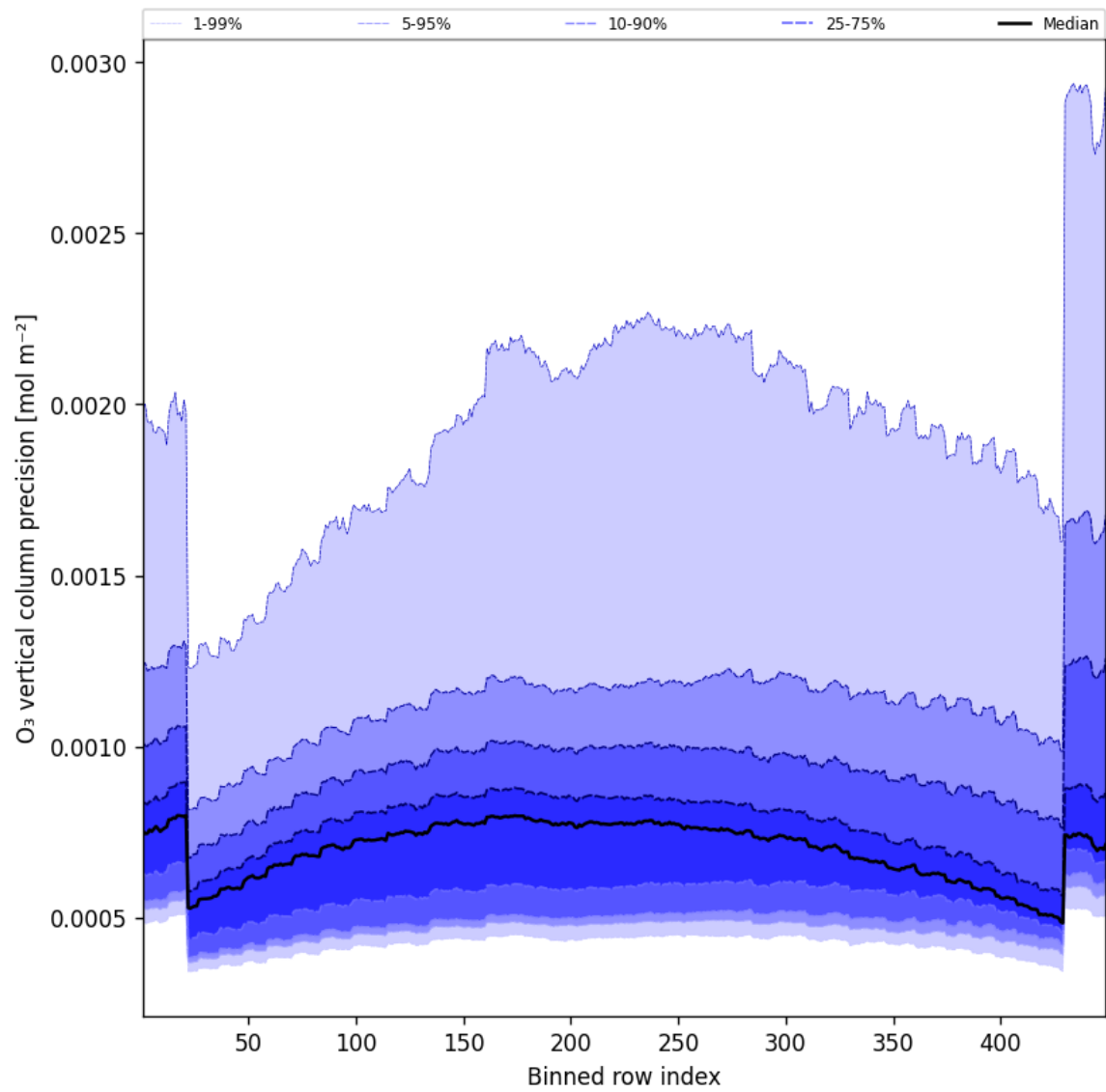
Figure 29: Along track statistics of “O 3 vertical column precision” for 2024-11-04 to 2024-11-05
