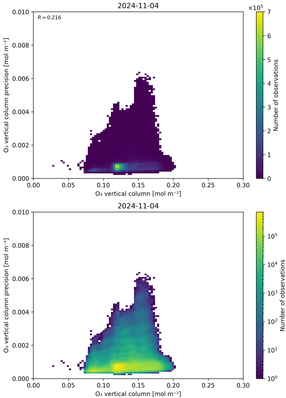
Figure 41: Scatter density plot of “O 3 vertical column” against “O 3 vertical column precision” for 2024-11-04 to 2024-11-05.
