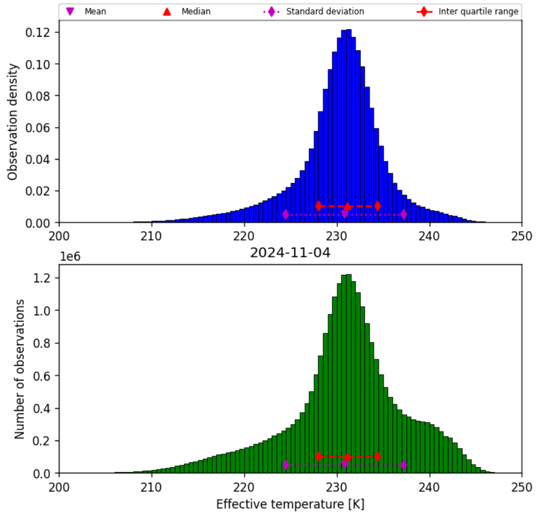
Figure 24: Histogram of “Effective temperature” for 2024-11-04 to 2024-11-05
