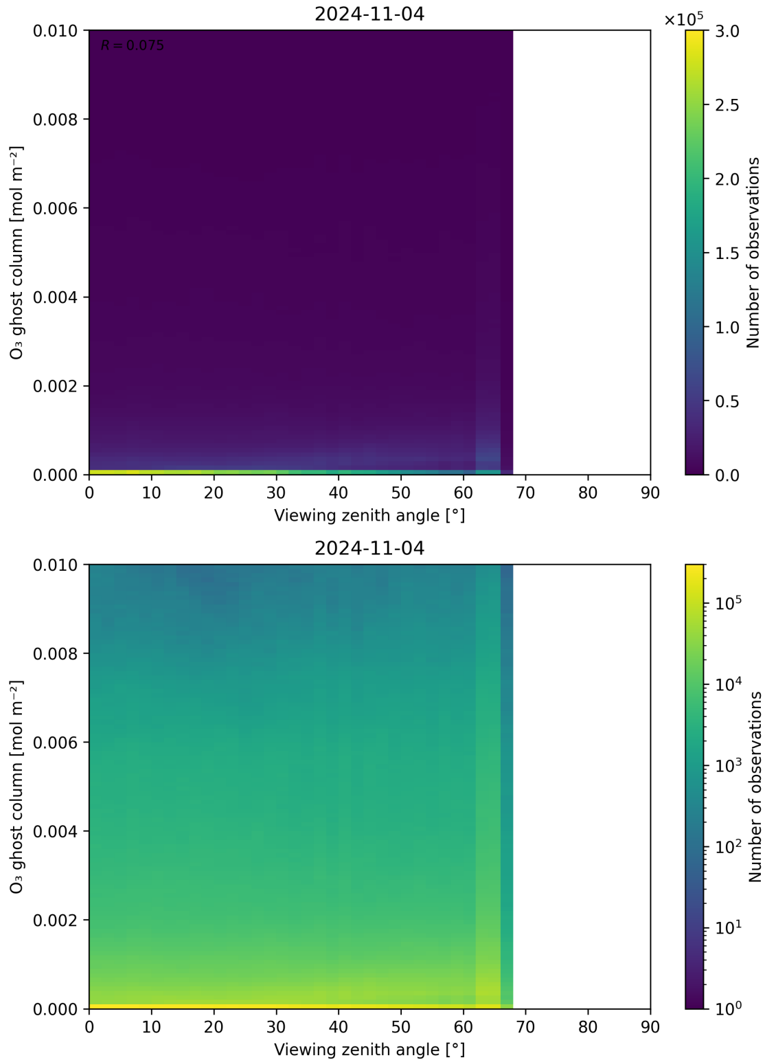
Figure 51: Scatter density plot of “Viewing zenith angle” against “O 3 ghost column” for 2024-11-04 to 2024-11-05.
