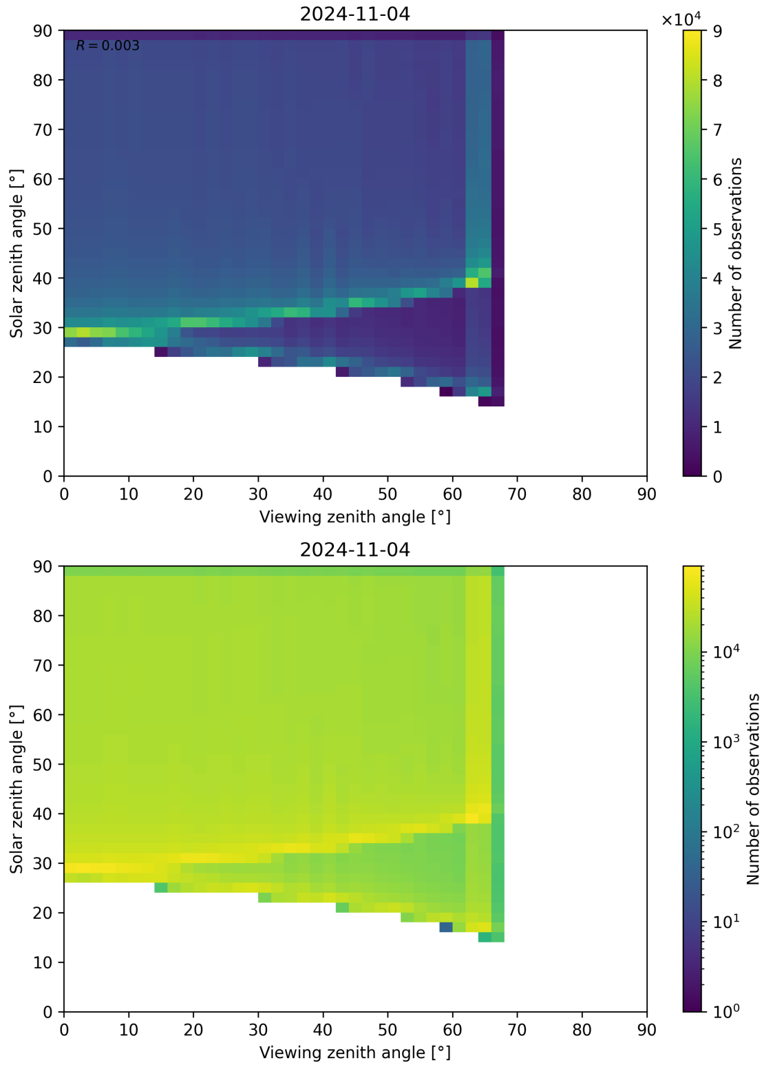
Figure 54: Scatter density plot of “Viewing zenith angle” against “Solar zenith angle” for 2024-11-04 to 2024-11-05.
