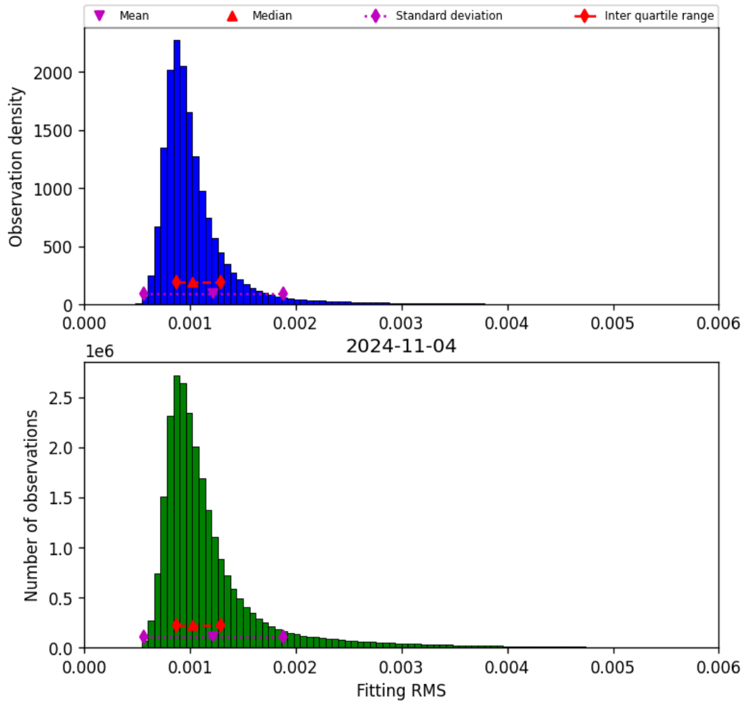
Figure 23: Histogram of “Fitting RMS” for 2024-11-04 to 2024-11-05
