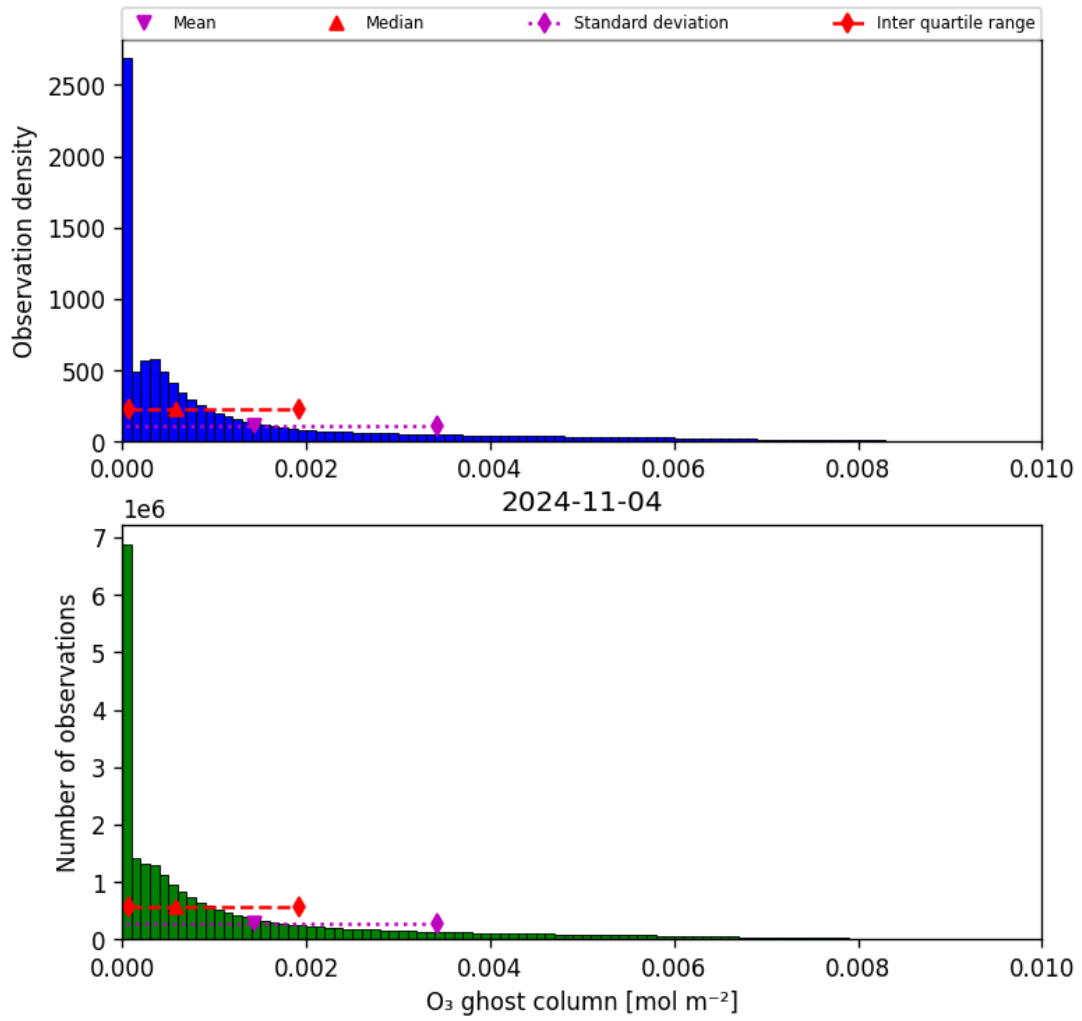
Figure 25: Histogram of “O 3 ghost column” for 2024-11-04 to 2024-11-05
