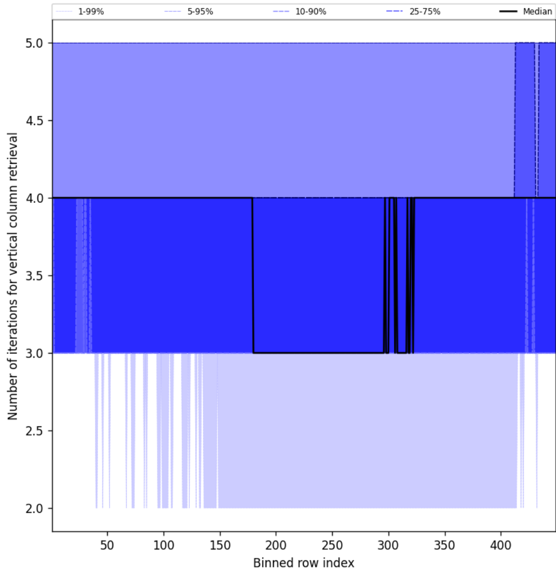
Figure 33: Along track statistics of “Number of iterations for vertical column retrieval” for 2024-11-04 to 2024-11-05
