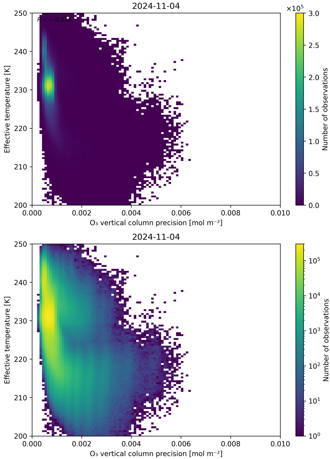
Figure 42: Scatter density plot of “O 3 vertical column precision” against “Effective temperature” for 2024-11-04 to 2024-11-05.
