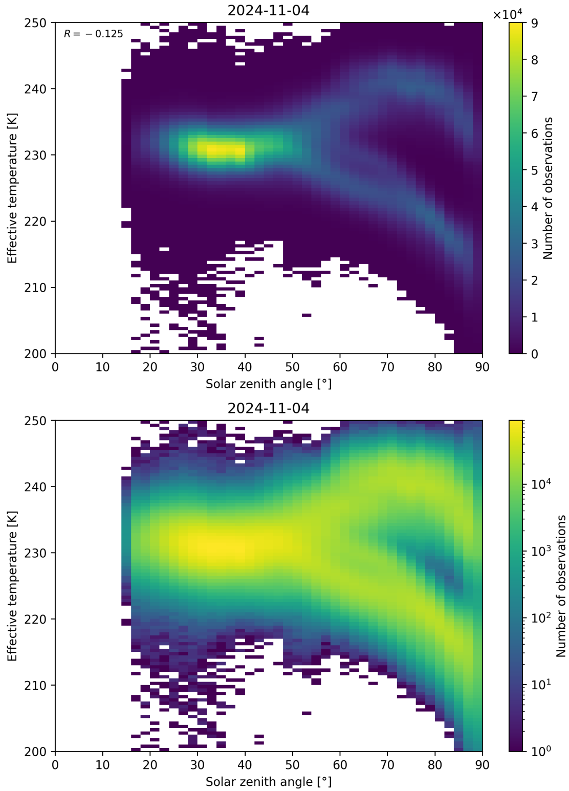
Figure 45: Scatter density plot of “Solar zenith angle” against “Effective temperature” for 2024-11-04 to 2024-11-05.
