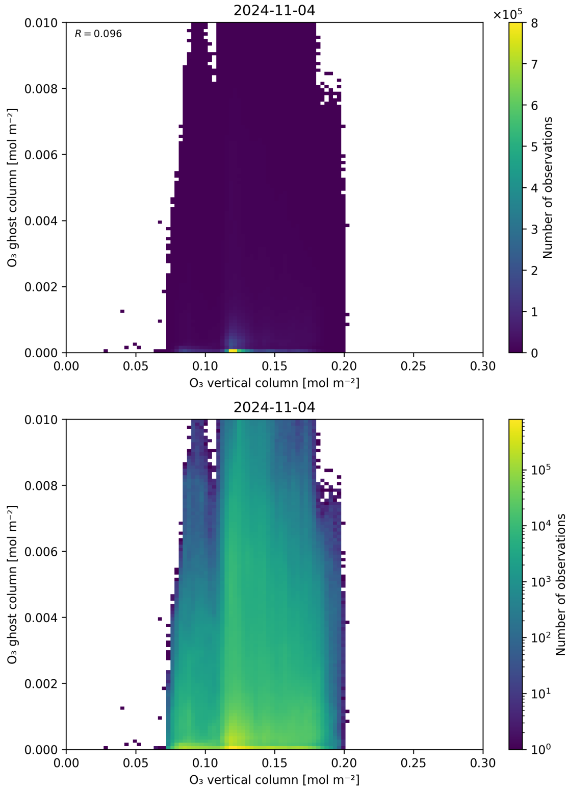
Figure 40: Scatter density plot of “O 3 vertical column” against “O 3 ghost column” for 2024-11-04 to 2024-11-05.
