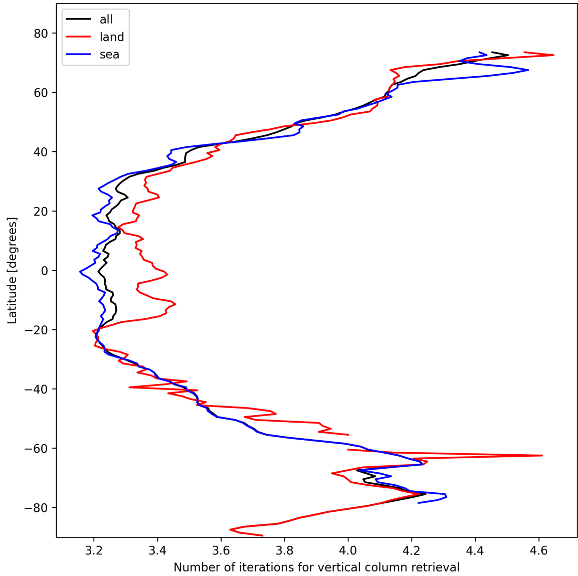
Figure 19: Zonal average of “Number of iterations for vertical column retrieval” for 2024-11-04 to 2024-11-05.
