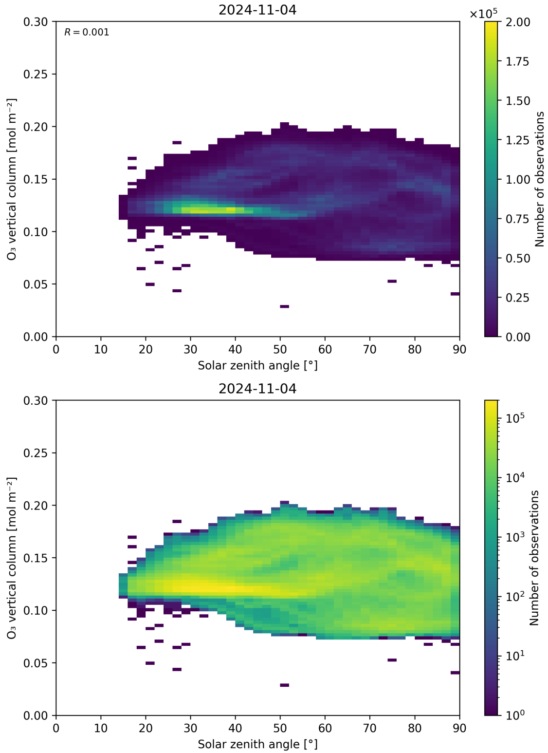
Figure 47: Scatter density plot of “Solar zenith angle” against “O 3 vertical column” for 2024-11-04 to 2024-11-05.
