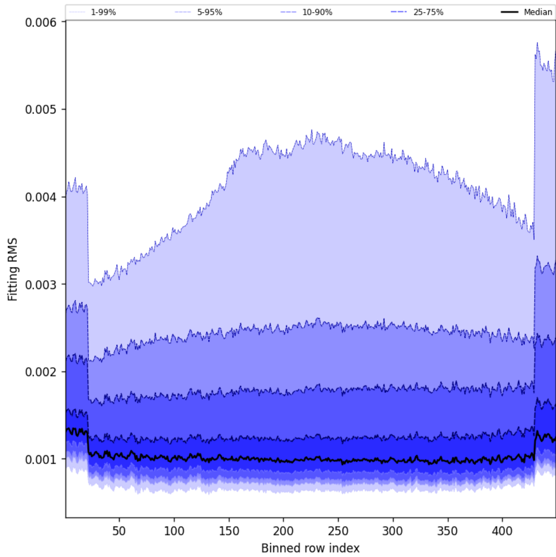
Figure 30: Along track statistics of “Fitting RMS” for 2024-11-04 to 2024-11-05
