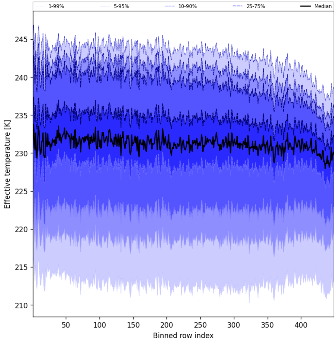
Figure 31: Along track statistics of “Effective temperature” for 2024-11-04 to 2024-11-05
