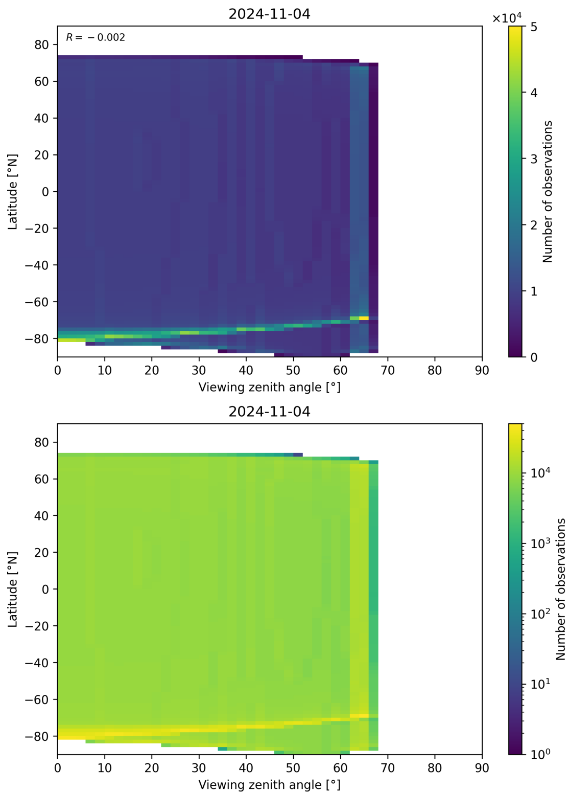
Figure 49: Scatter density plot of “Viewing zenith angle” against “Latitude” for 2024-11-04 to 2024-11-05.
