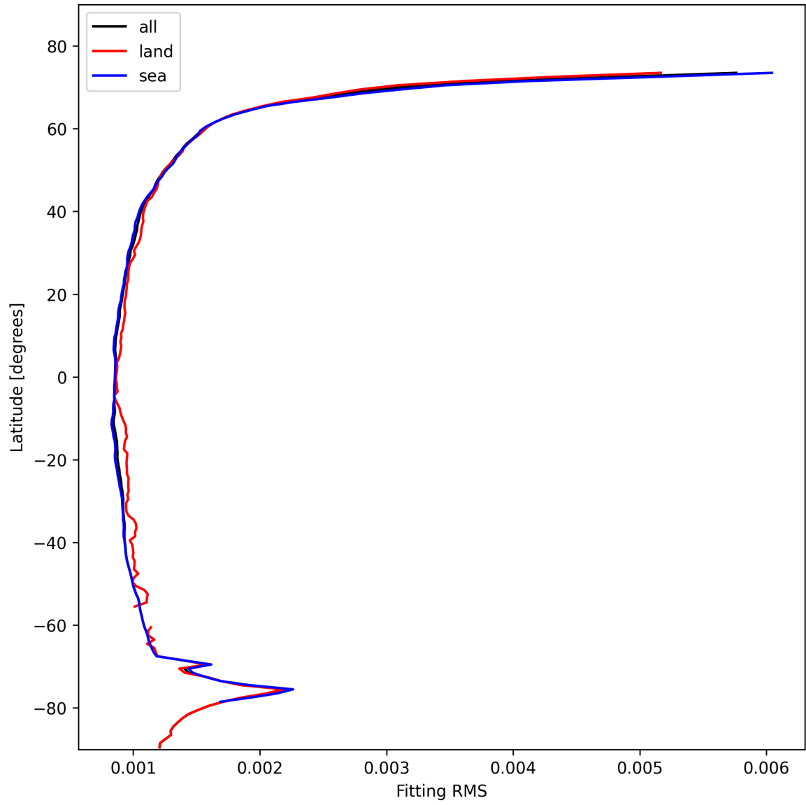
Figure 16: Zonal average of “Fitting RMS” for 2024-11-04 to 2024-11-05.
