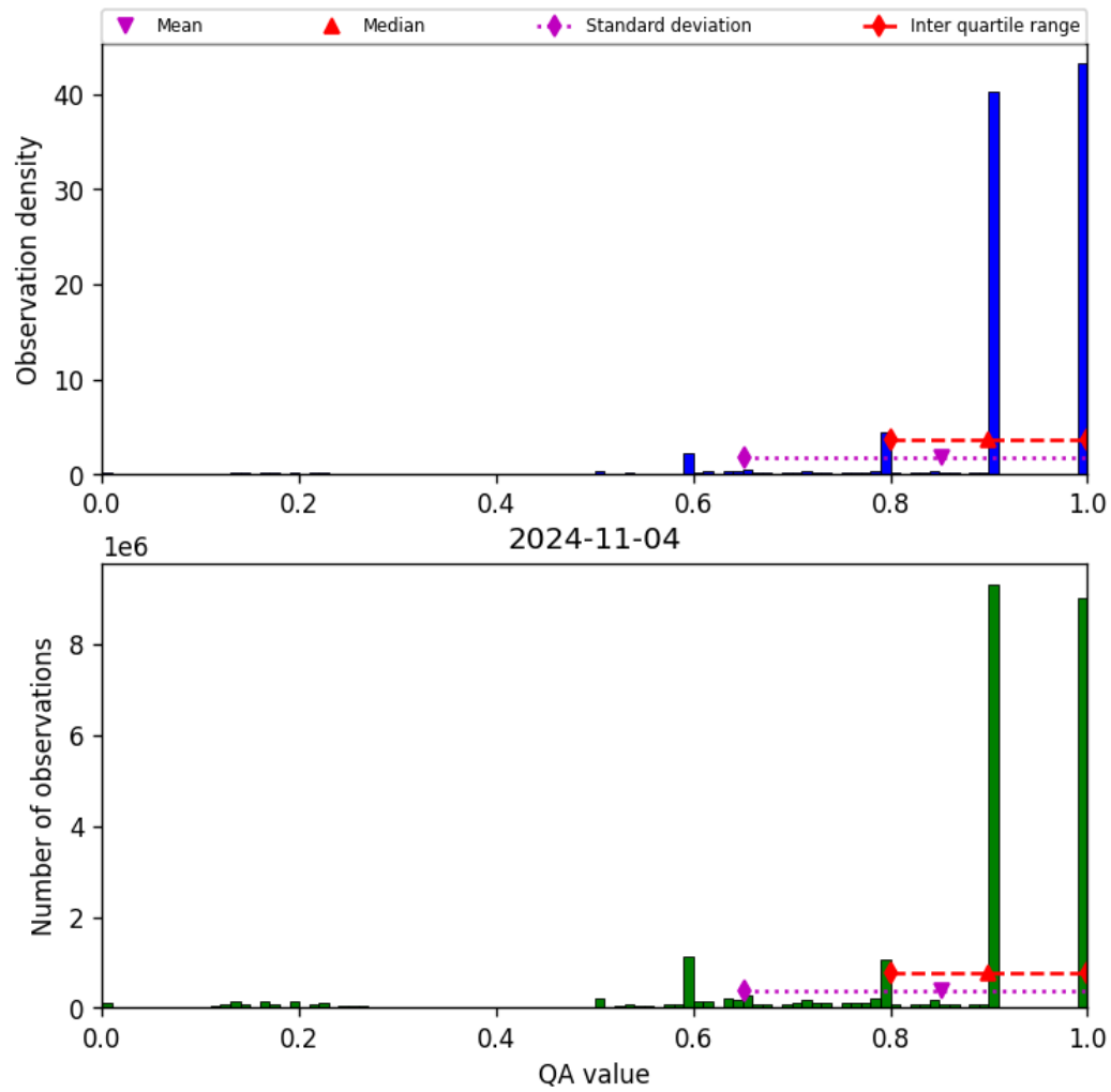
Figure 20: Histogram of “QA value” for 2024-11-04 to 2024-11-05
