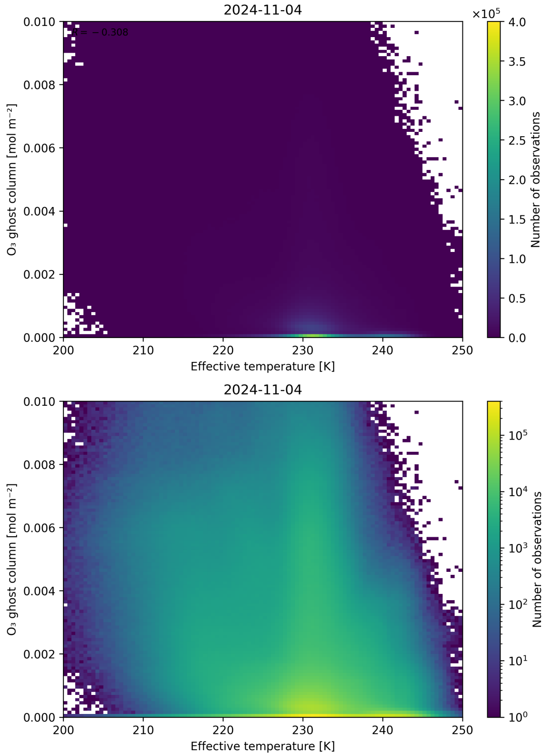
Figure 38: Scatter density plot of “Effective temperature” against “O 3 ghost column” for 2024-11-04 to 2024-11-05.
