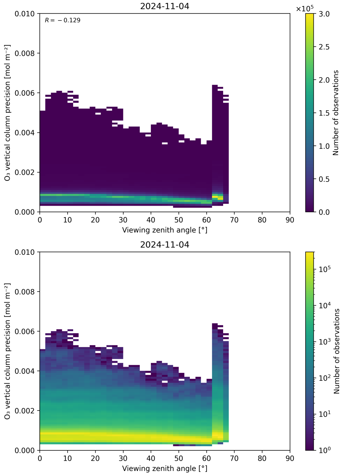
Figure 53: Scatter density plot of “Viewing zenith angle” against “O 3 vertical column precision” for 2024-11-04 to 2024-11-05.
