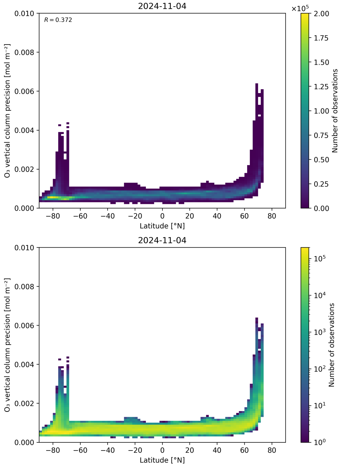
Figure 37: Scatter density plot of “Latitude” against “O 3 vertical column precision” for 2024-11-04 to 2024-11-05.
