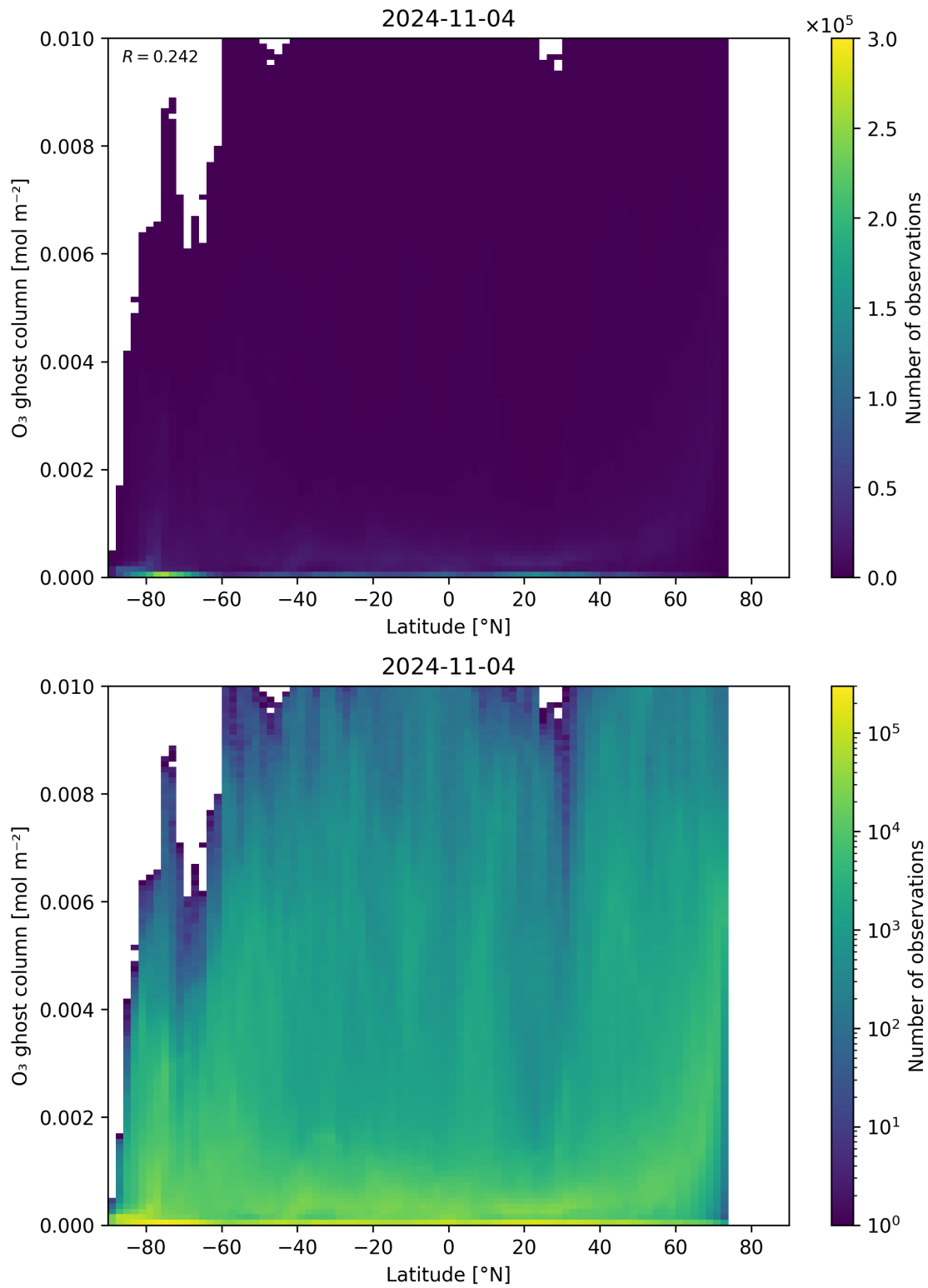
Figure 35: Scatter density plot of “Latitude” against “O 3 ghost column” for 2024-11-04 to 2024-11-05.
