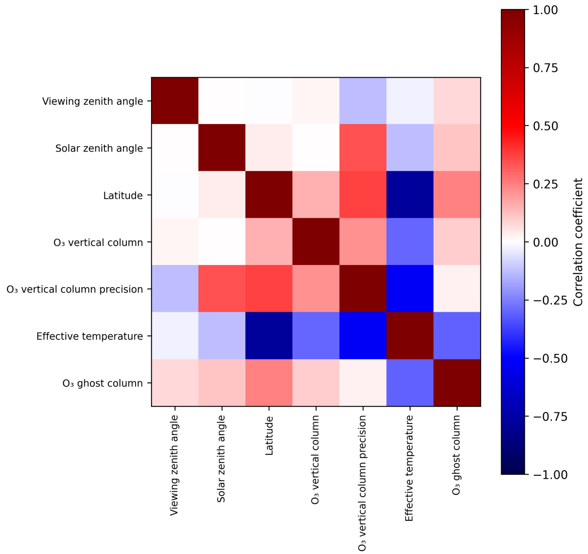
Figure 2: Map of correlation matrix for 2024-11-04 to 2024-11-05.
