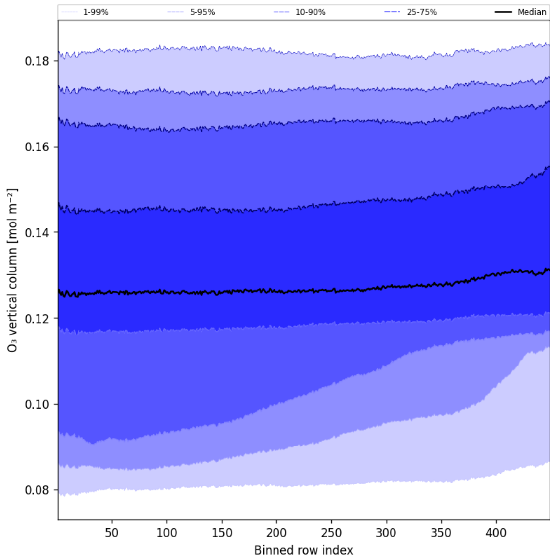
Figure 28: Along track statistics of “O 3 vertical column” for 2024-11-04 to 2024-11-05
