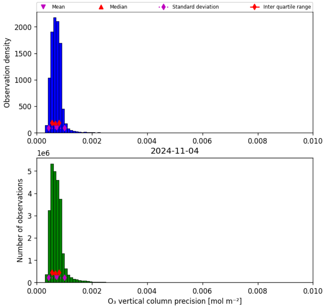
Figure 22: Histogram of “O 3 vertical column precision” for 2024-11-04 to 2024-11-05
