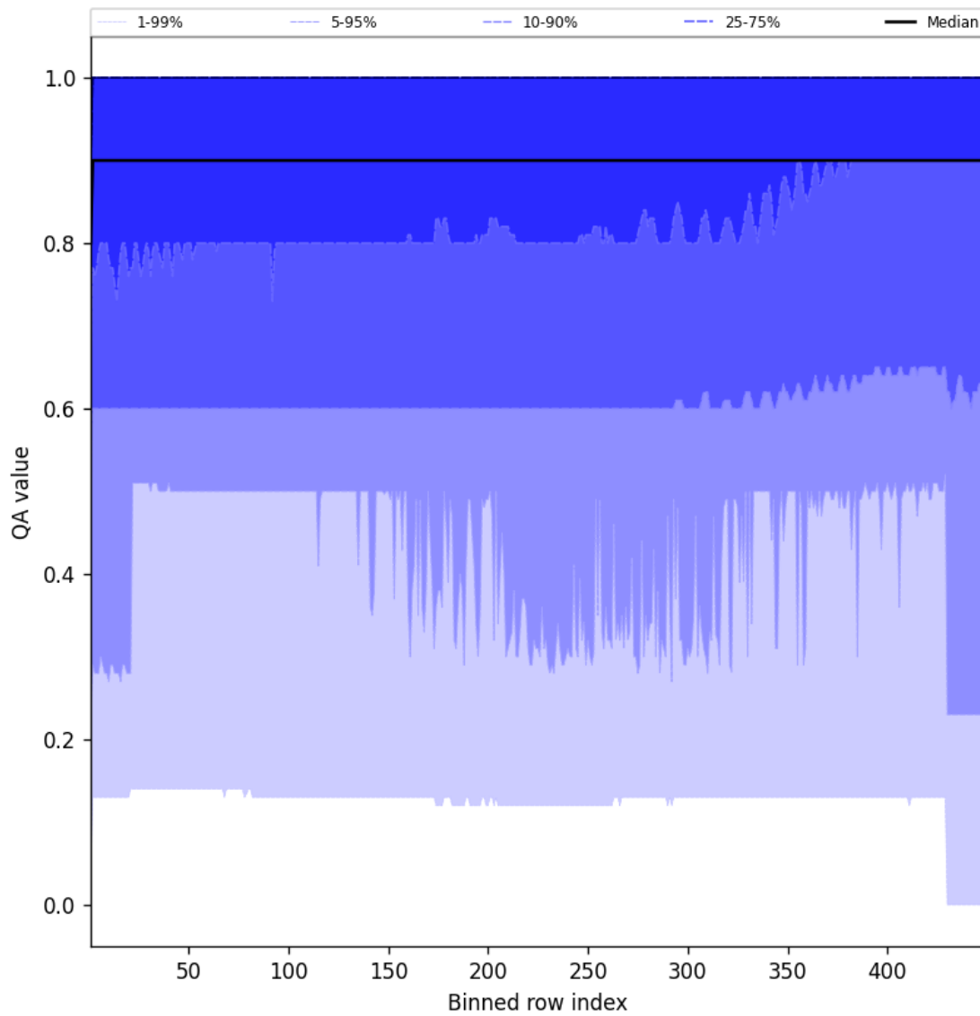
Figure 27: Along track statistics of “QA value” for 2024-11-04 to 2024-11-05
