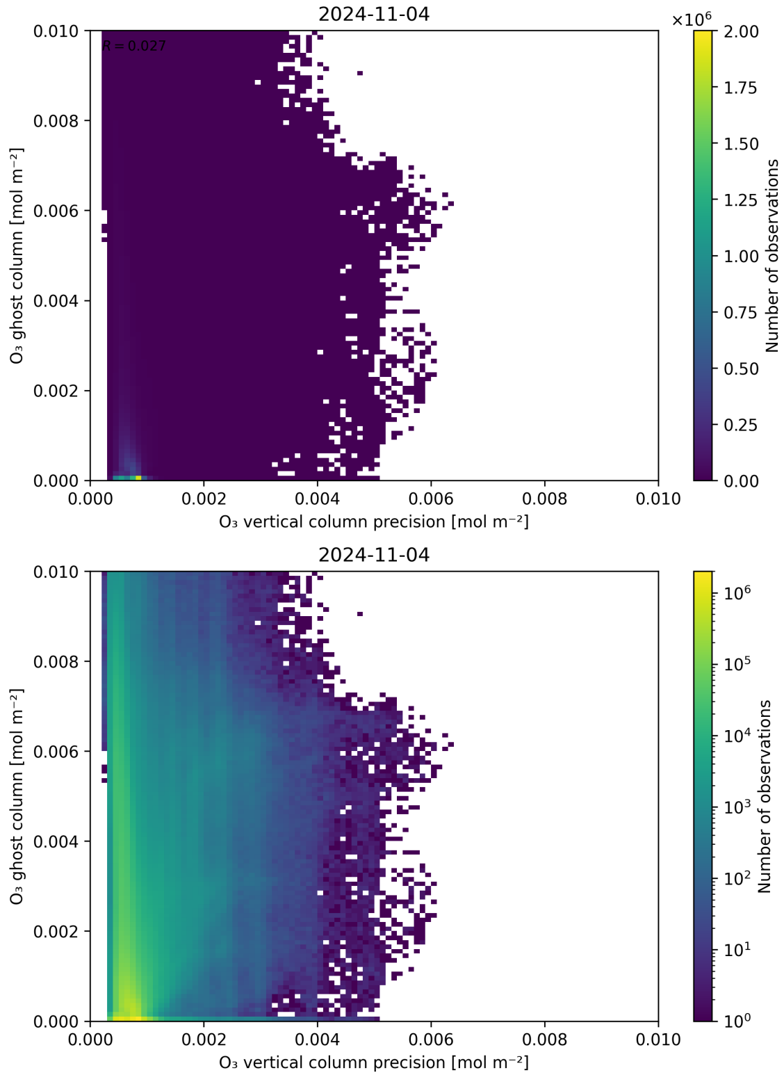
Figure 43: Scatter density plot of “ \text{O}_3 vertical column precision” against “ \text{O}_3 ghost column” for 2024-11-04 to 2024-11-05.
