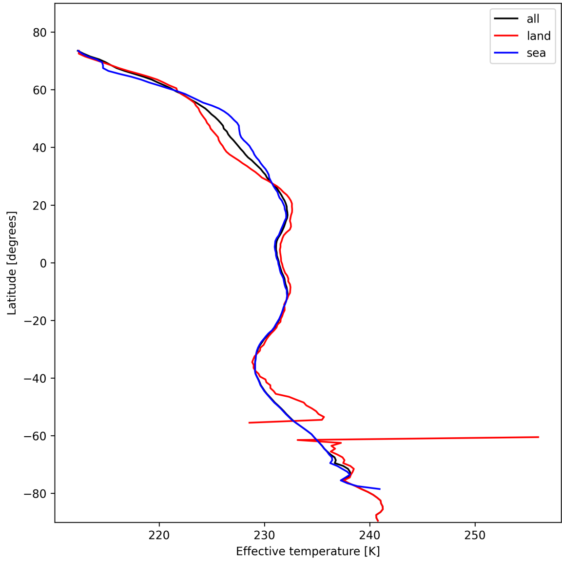
Figure 17: Zonal average of “Effective temperature” for 2024-11-04 to 2024-11-05.
