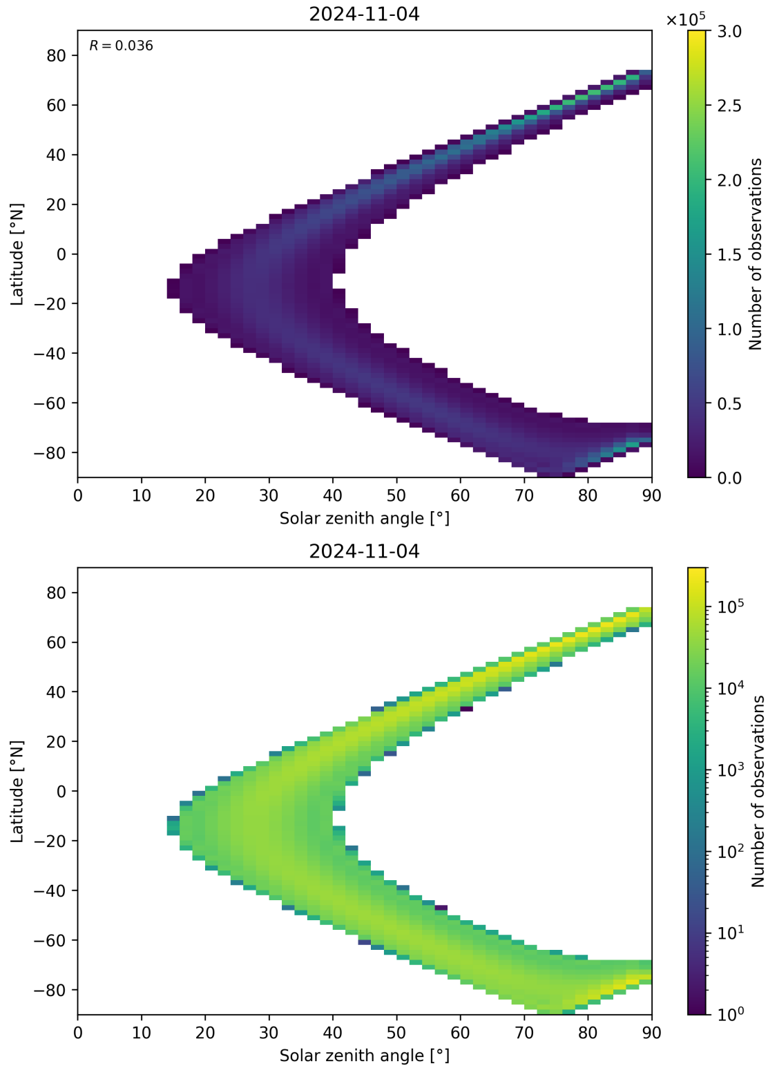
Figure 44: Scatter density plot of “Solar zenith angle” against “Latitude” for 2024-11-04 to 2024-11-05.
