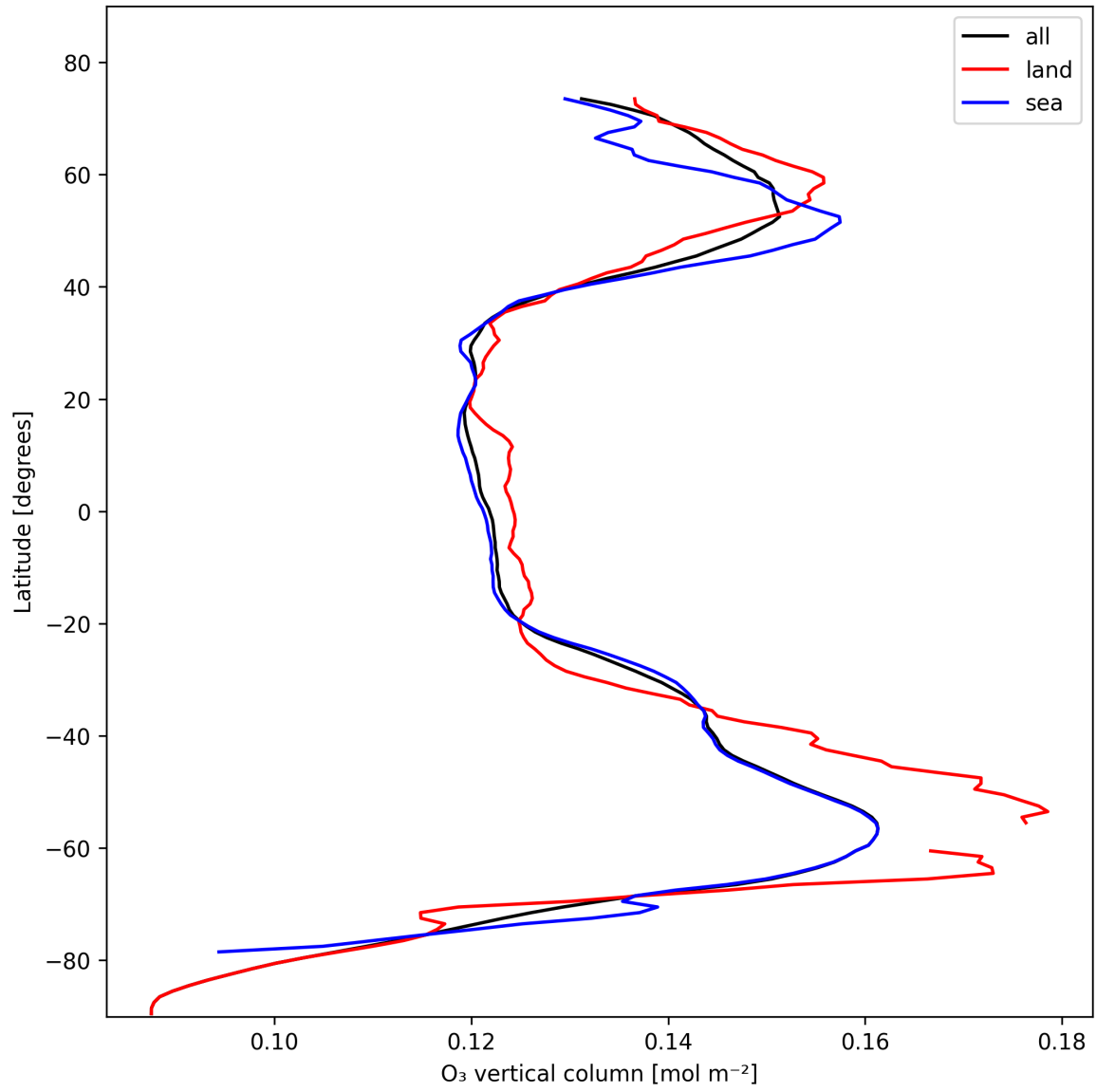
Figure 14: Zonal average of “O 3 vertical column” for 2024-11-04 to 2024-11-05.
