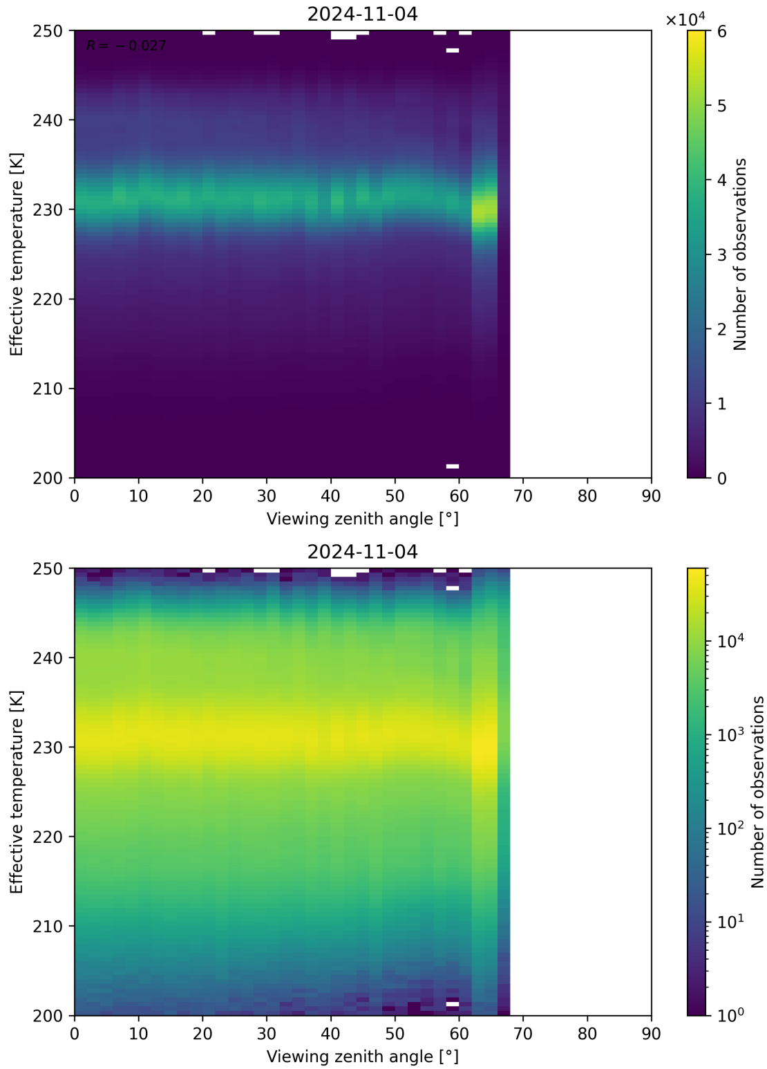
Figure 50: Scatter density plot of “Viewing zenith angle” against “Effective temperature” for 2024-11-04 to 2024-11-05.
