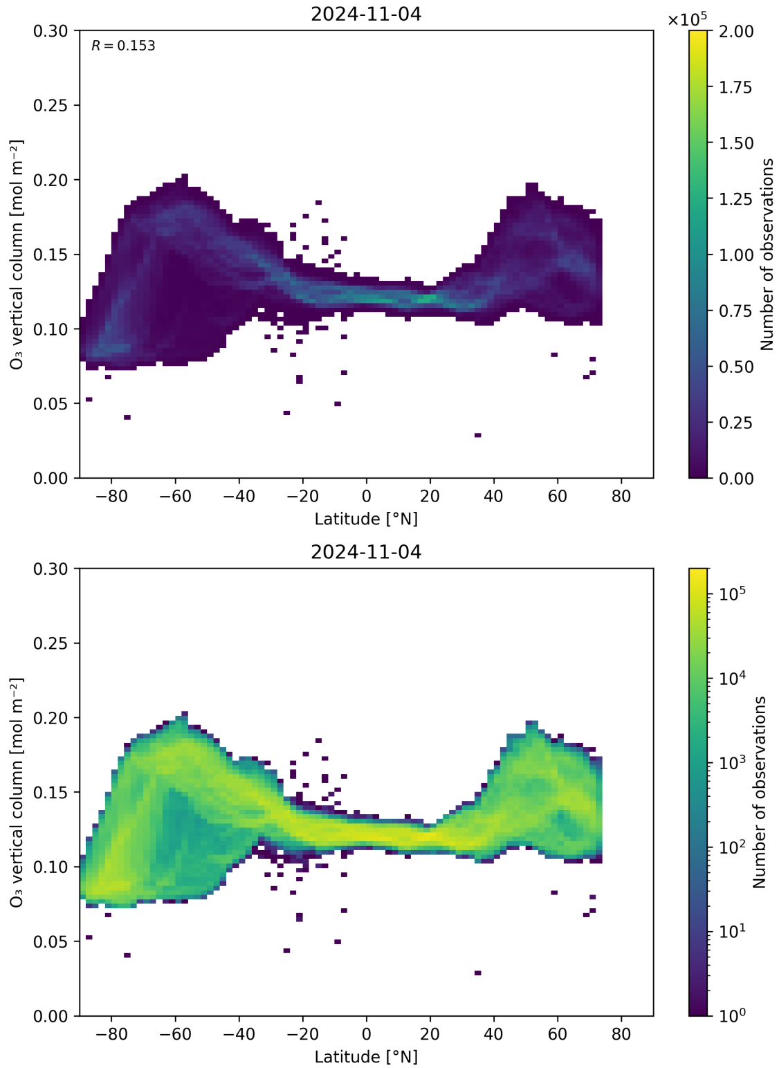
Figure 36: Scatter density plot of “Latitude” against “O 3 vertical column” for 2024-11-04 to 2024-11-05.
