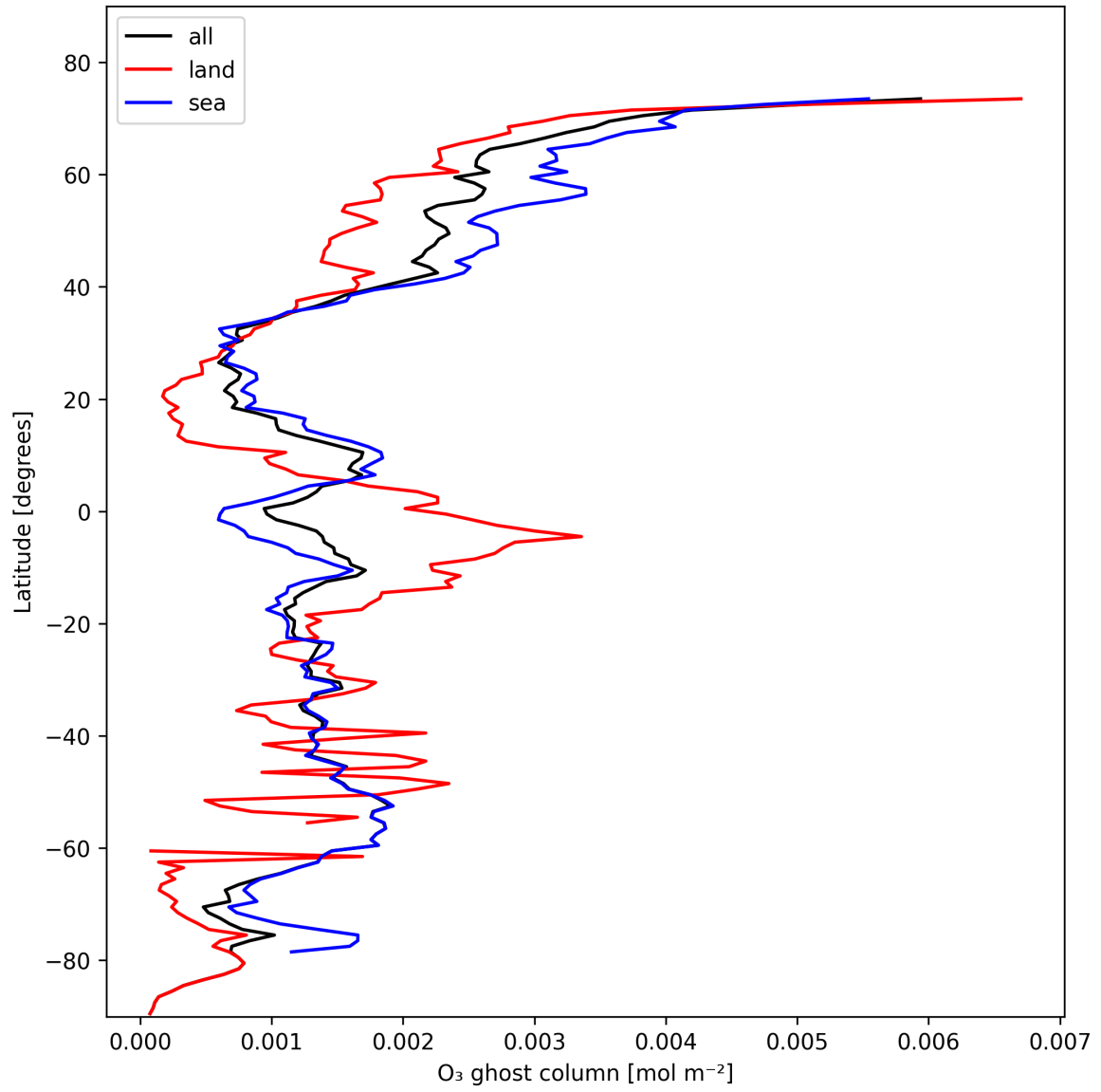
Figure 18: Zonal average of "O 3 ghost column" for 2024-11-04 to 2024-11-05.
