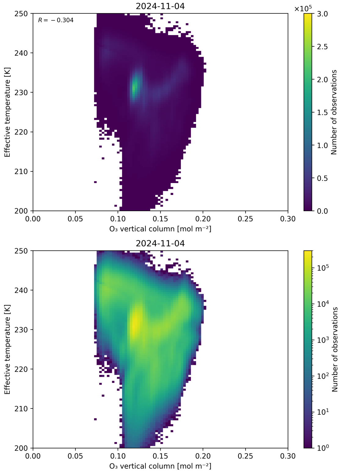
Figure 39: Scatter density plot of “O 3 vertical column” against “Effective temperature” for 2024-11-04 to 2024-11-05.
