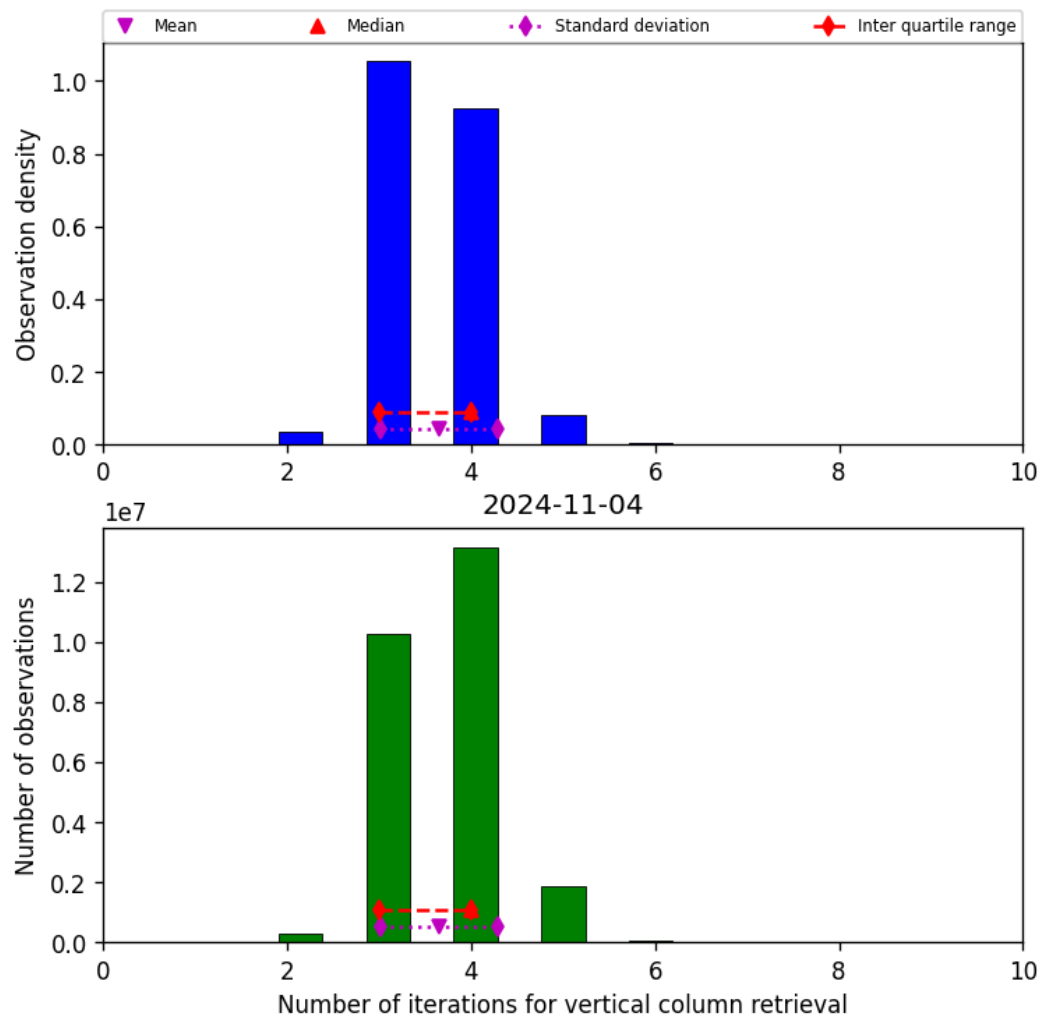
Figure 26: Histogram of “Number of iterations for vertical column retrieval” for 2024-11-04 to 2024-11-05
