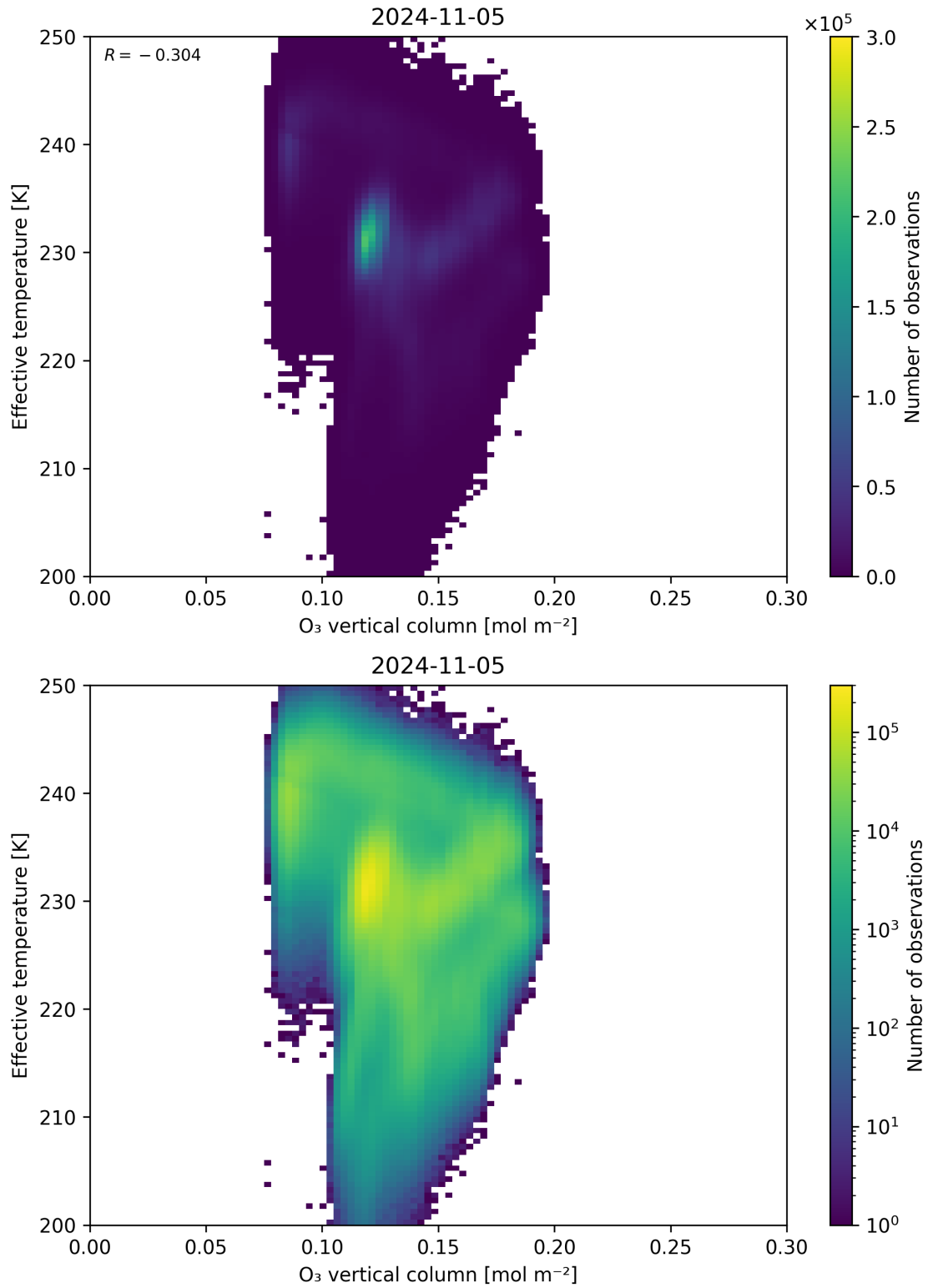
Figure 39: Scatter density plot of “O 3 vertical column” against “Effective temperature” for 2024-11-04 to 2024-11-06.
