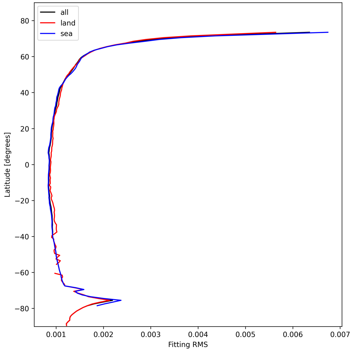
Figure 16: Zonal average of “Fitting RMS” for 2024-11-04 to 2024-11-06.
