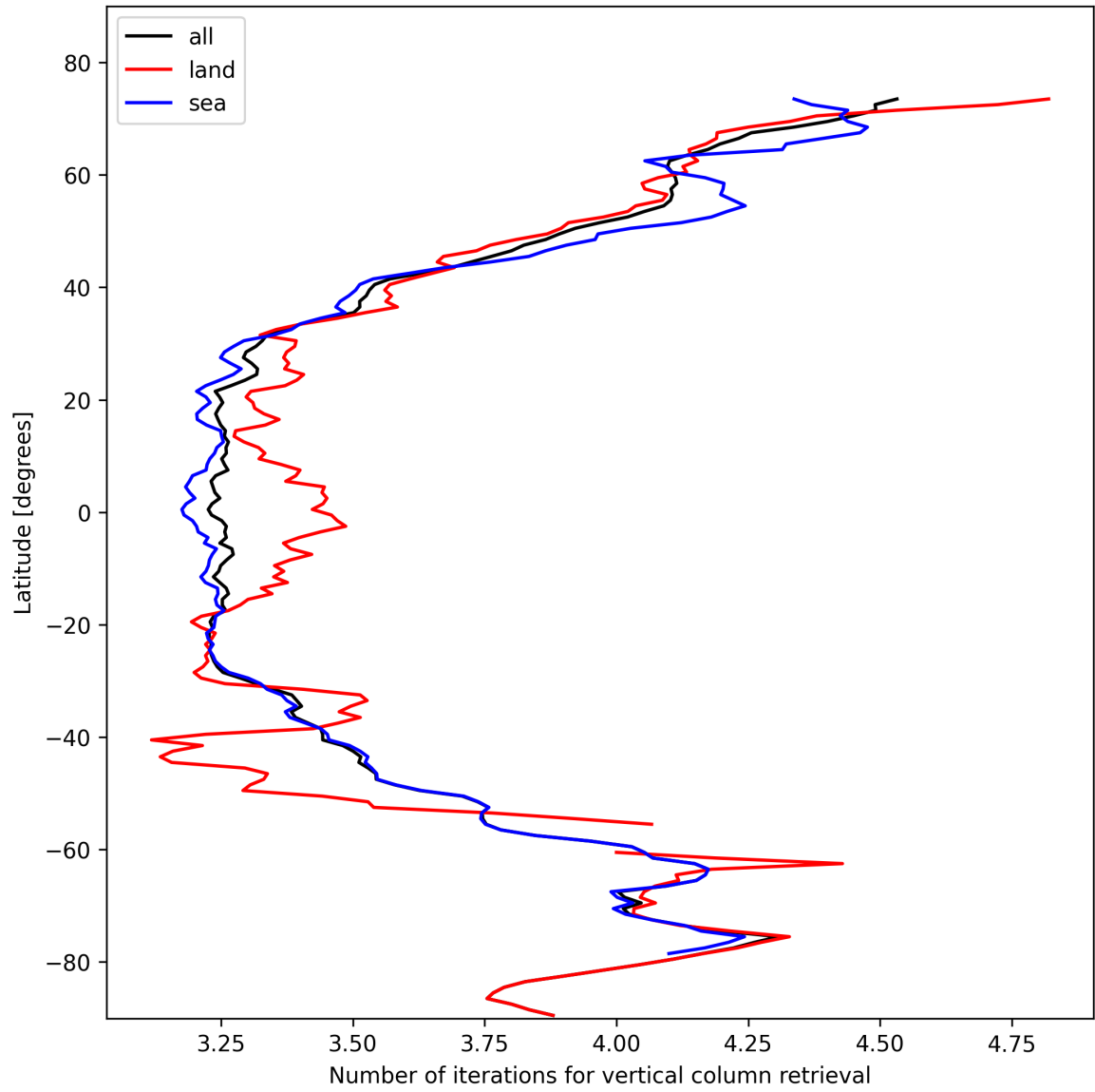
Figure 19: Zonal average of “Number of iterations for vertical column retrieval” for 2024-11-04 to 2024-11-06.
