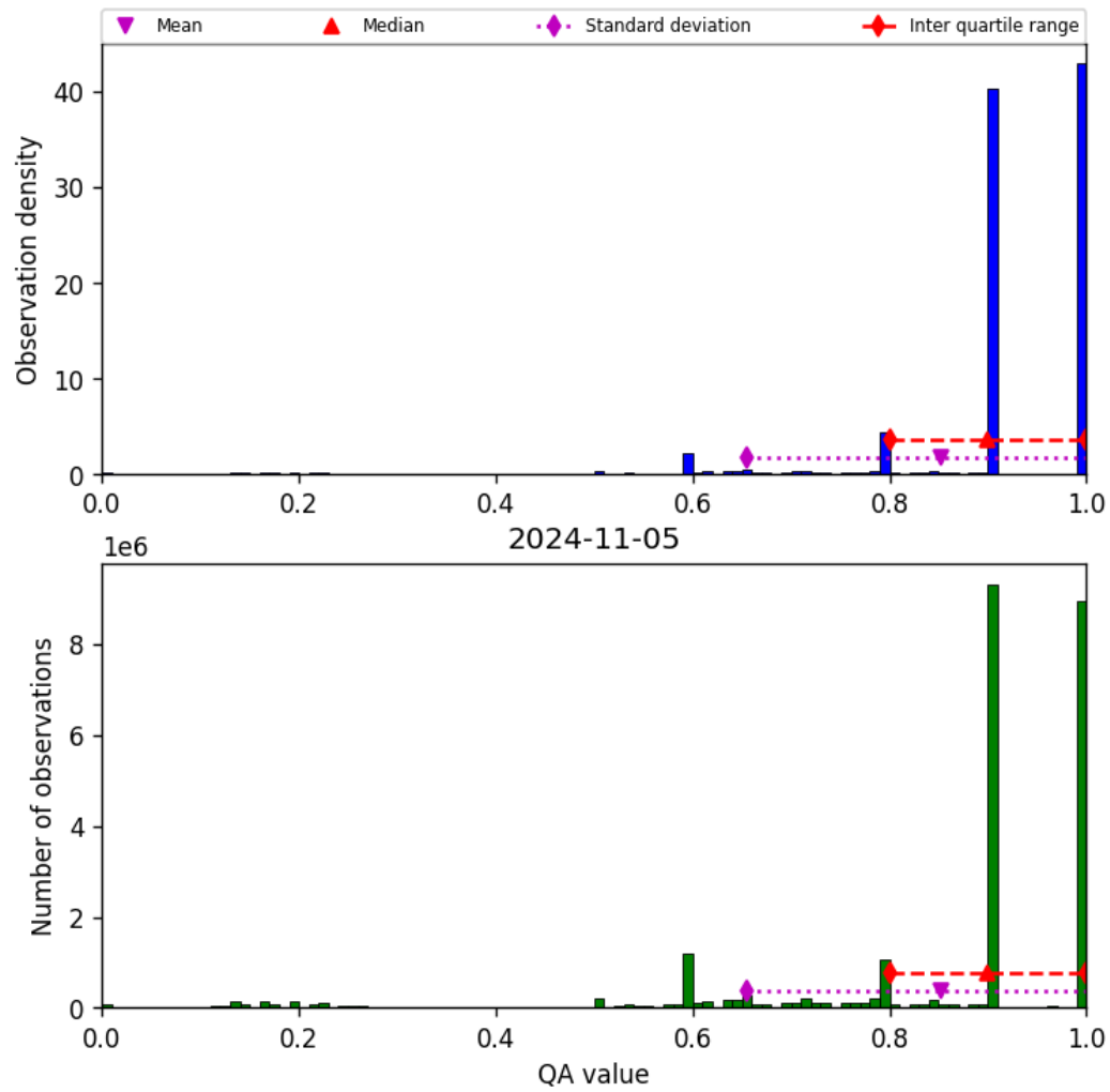
Figure 20: Histogram of “QA value” for 2024-11-04 to 2024-11-06
