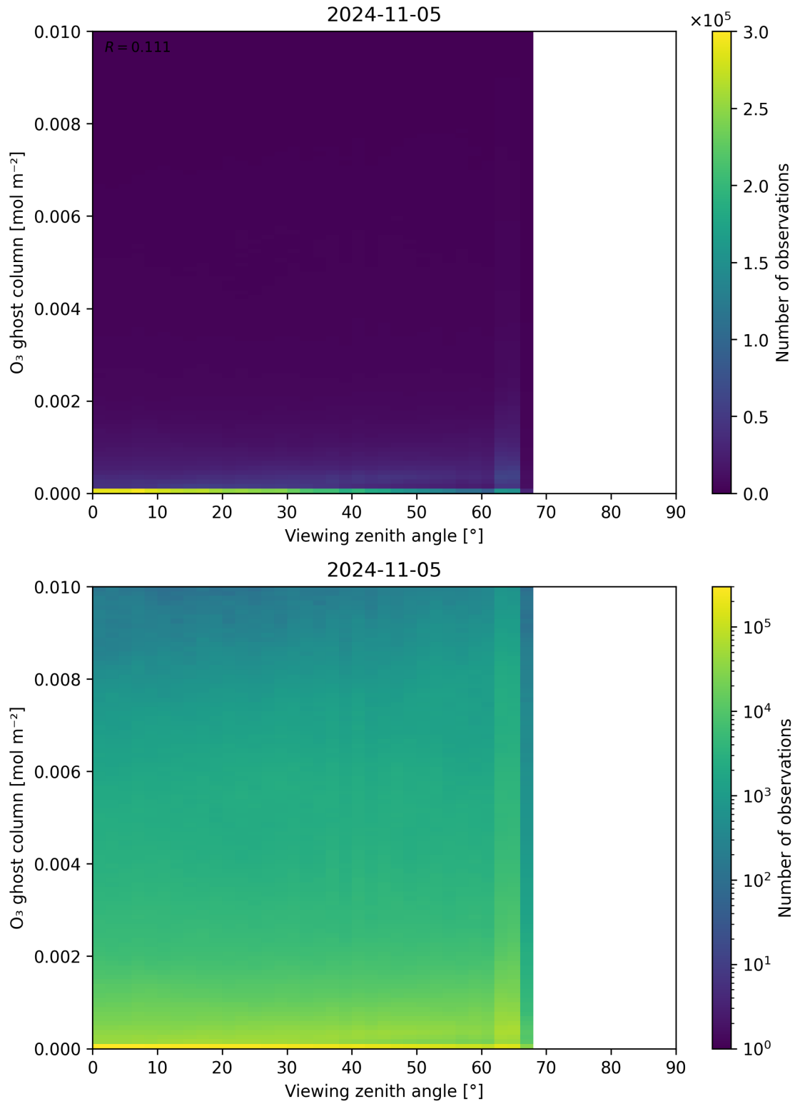
Figure 51: Scatter density plot of “Viewing zenith angle” against “O 3 ghost column” for 2024-11-04 to 2024-11-06.
