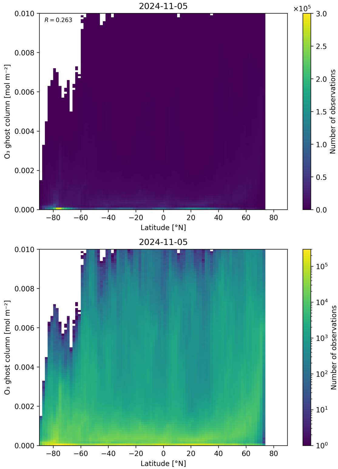
Figure 35: Scatter density plot of “Latitude” against “O 3 ghost column” for 2024-11-04 to 2024-11-06.
