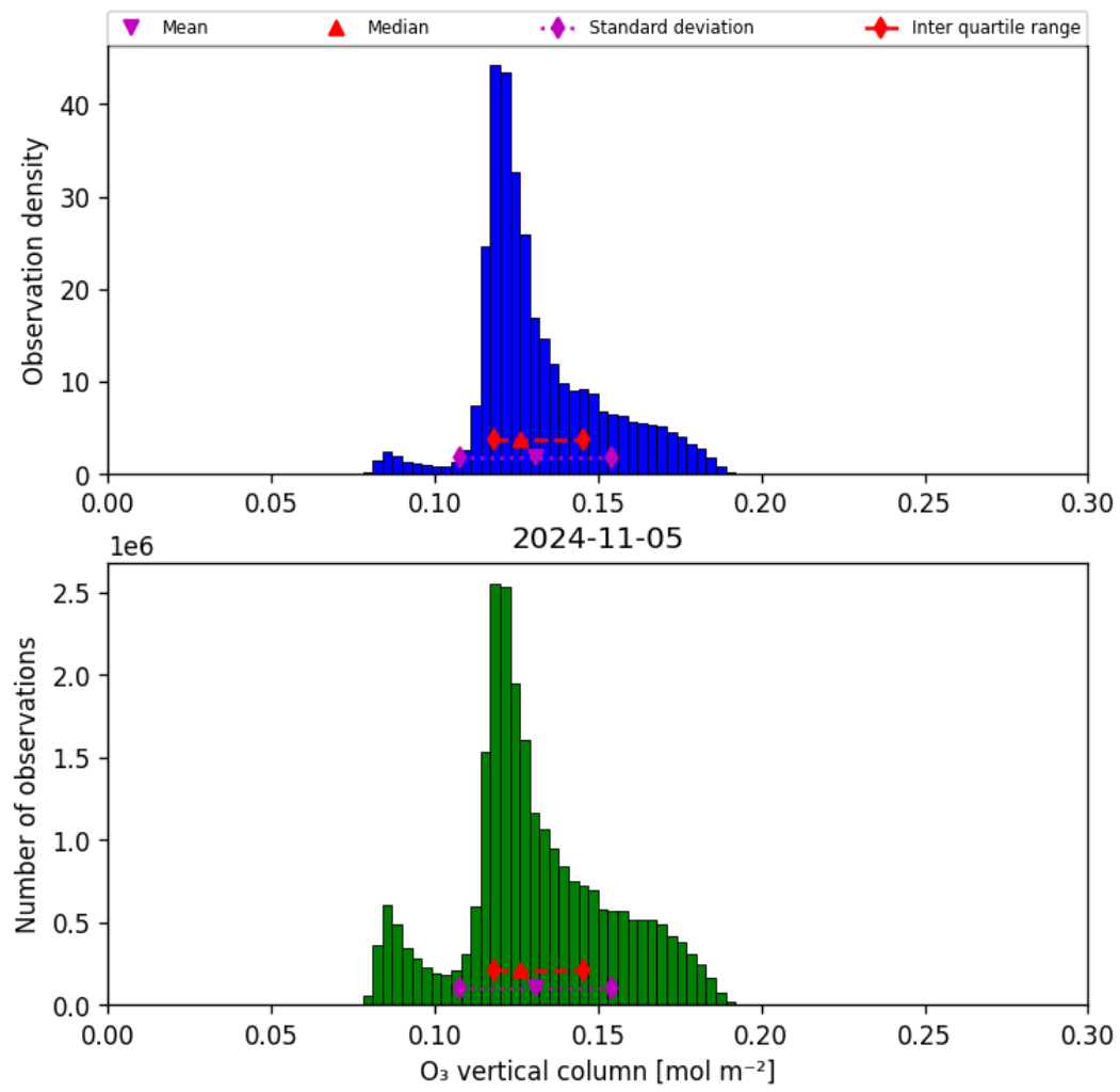
Figure 21: Histogram of “O 3 vertical column” for 2024-11-04 to 2024-11-06
