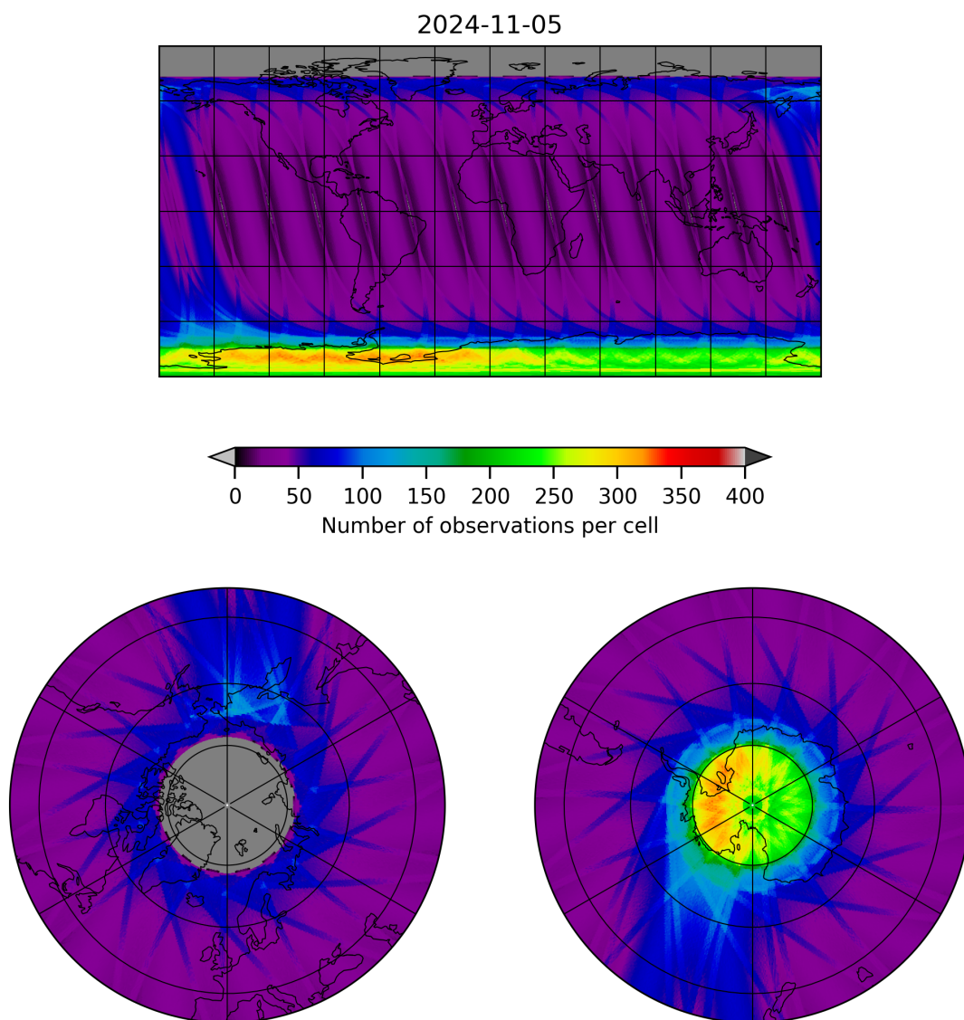
Figure 12: Map of the number of observations for 2024-11-04 to 2024-11-06
