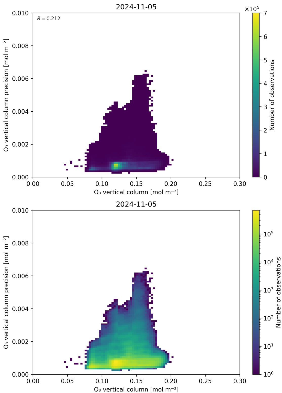
Figure 41: Scatter density plot of “O 3 vertical column” against “O 3 vertical column precision” for 2024-11-04 to 2024-11-06.
