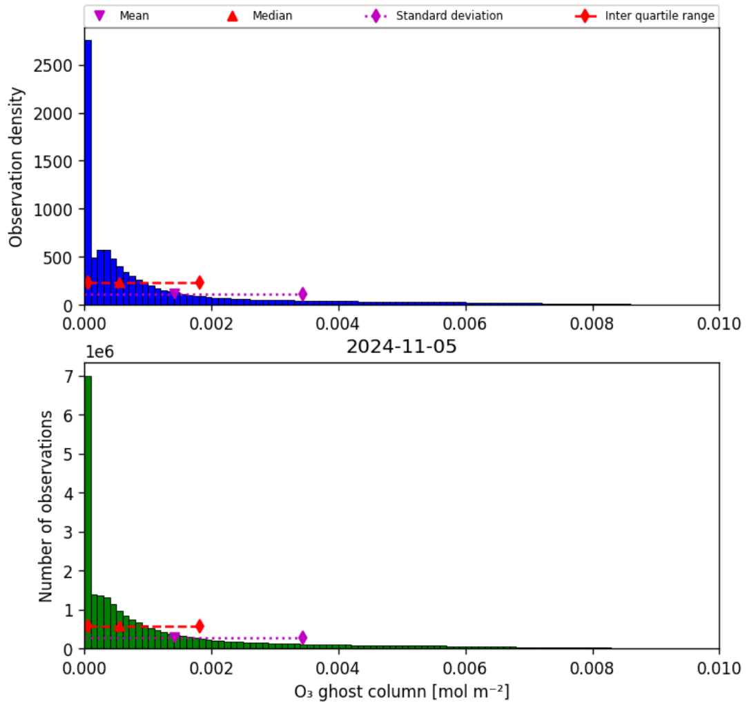
Figure 25: Histogram of “O 3 ghost column” for 2024-11-04 to 2024-11-06
