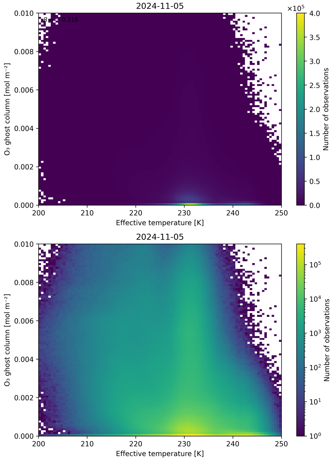
Figure 38: Scatter density plot of “Effective temperature” against “O 3 ghost column” for 2024-11-04 to 2024-11-06.
