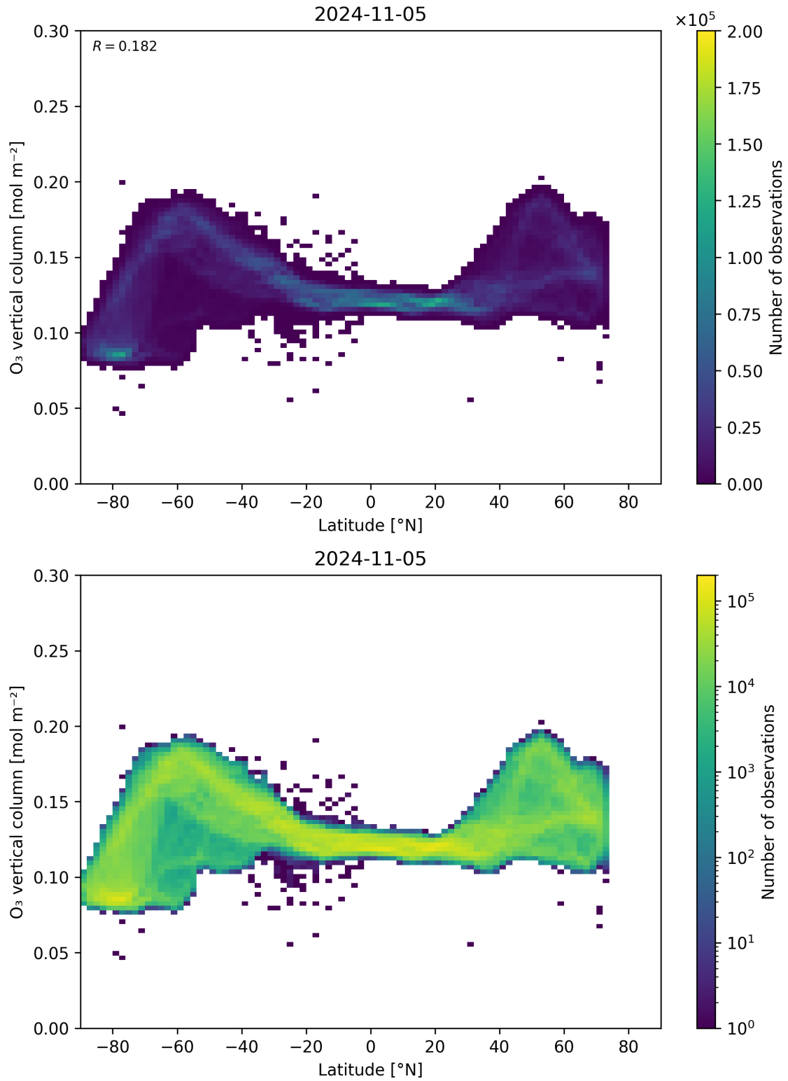
Figure 36: Scatter density plot of “Latitude” against “O 3 vertical column” for 2024-11-04 to 2024-11-06.
