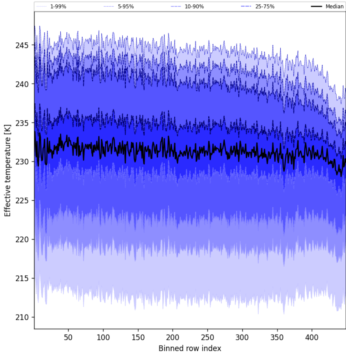
Figure 31: Along track statistics of “Effective temperature” for 2024-11-04 to 2024-11-06
