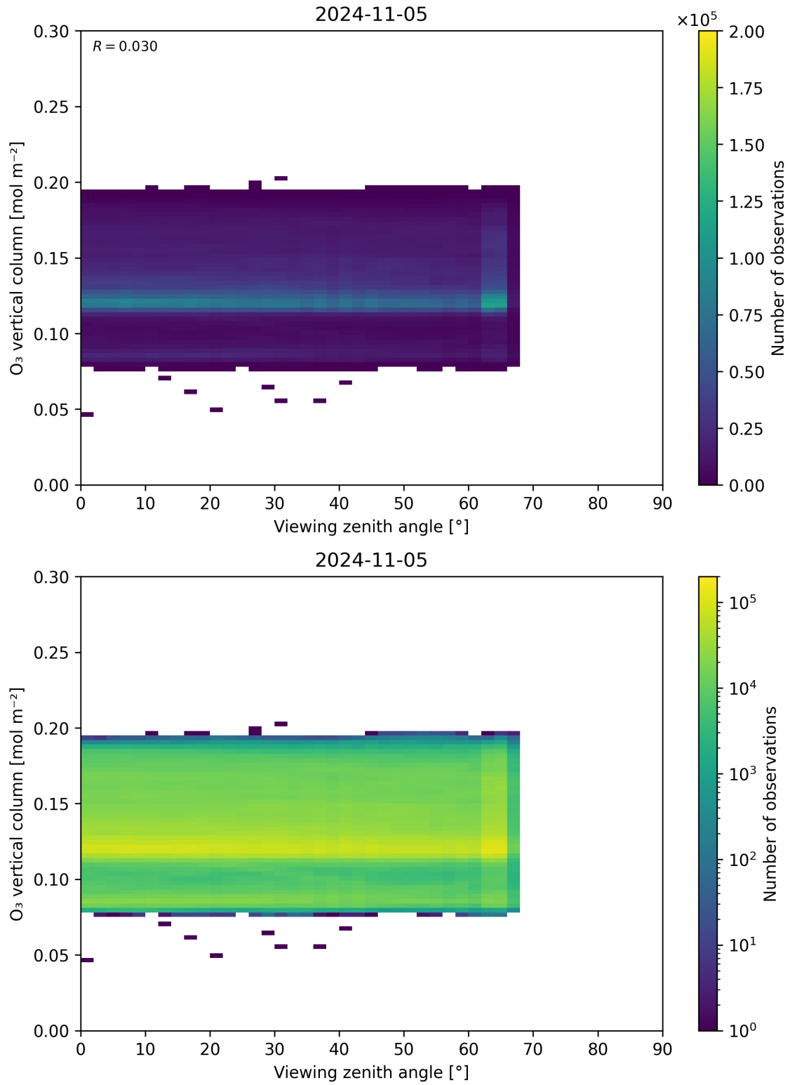
Figure 52: Scatter density plot of “Viewing zenith angle” against “O 3 vertical column” for 2024-11-04 to 2024-11-06.
