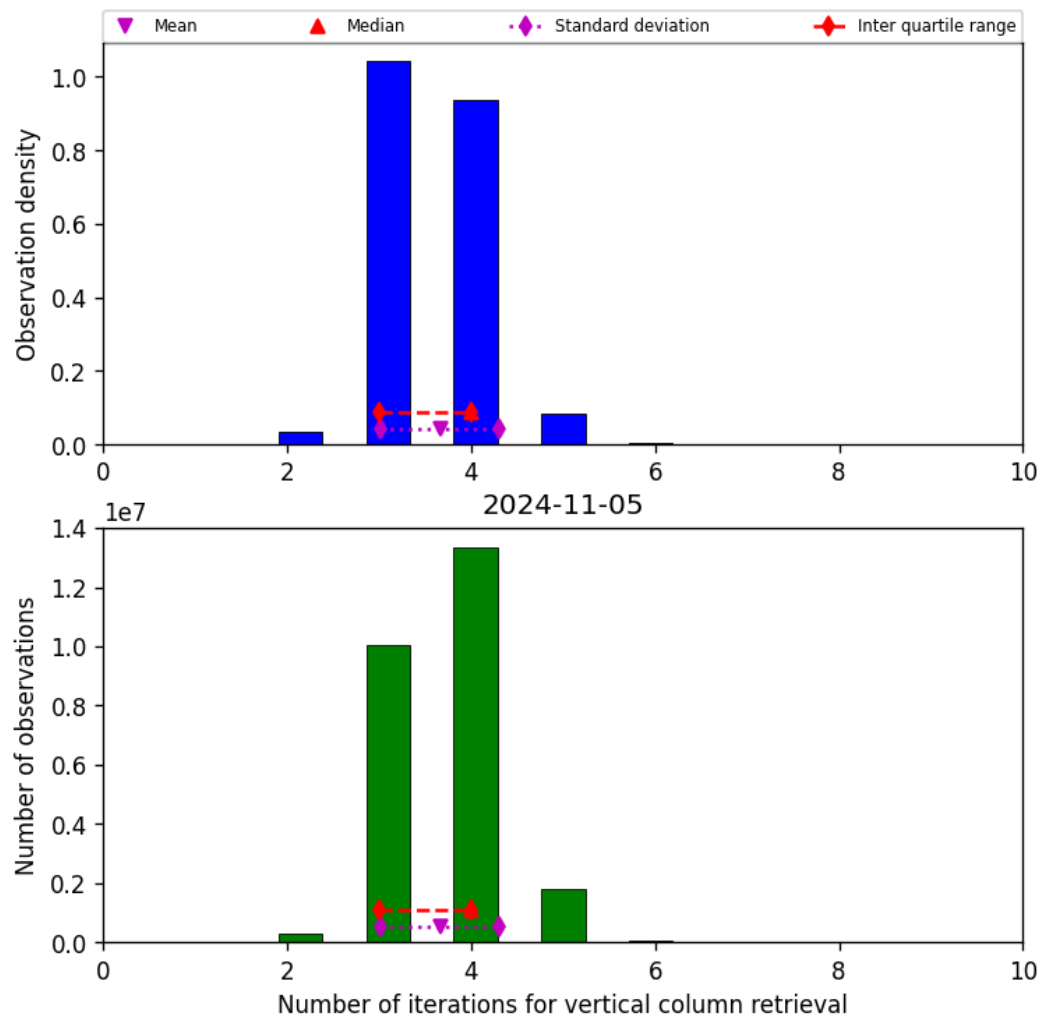
Figure 26: Histogram of “Number of iterations for vertical column retrieval” for 2024-11-04 to 2024-11-06
