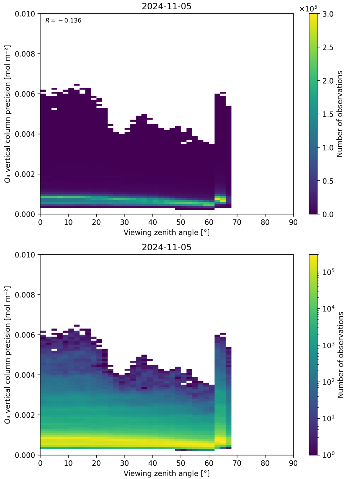
Figure 53: Scatter density plot of “Viewing zenith angle” against “O 3 vertical column precision” for 2024-11-04 to 2024-11-06.
