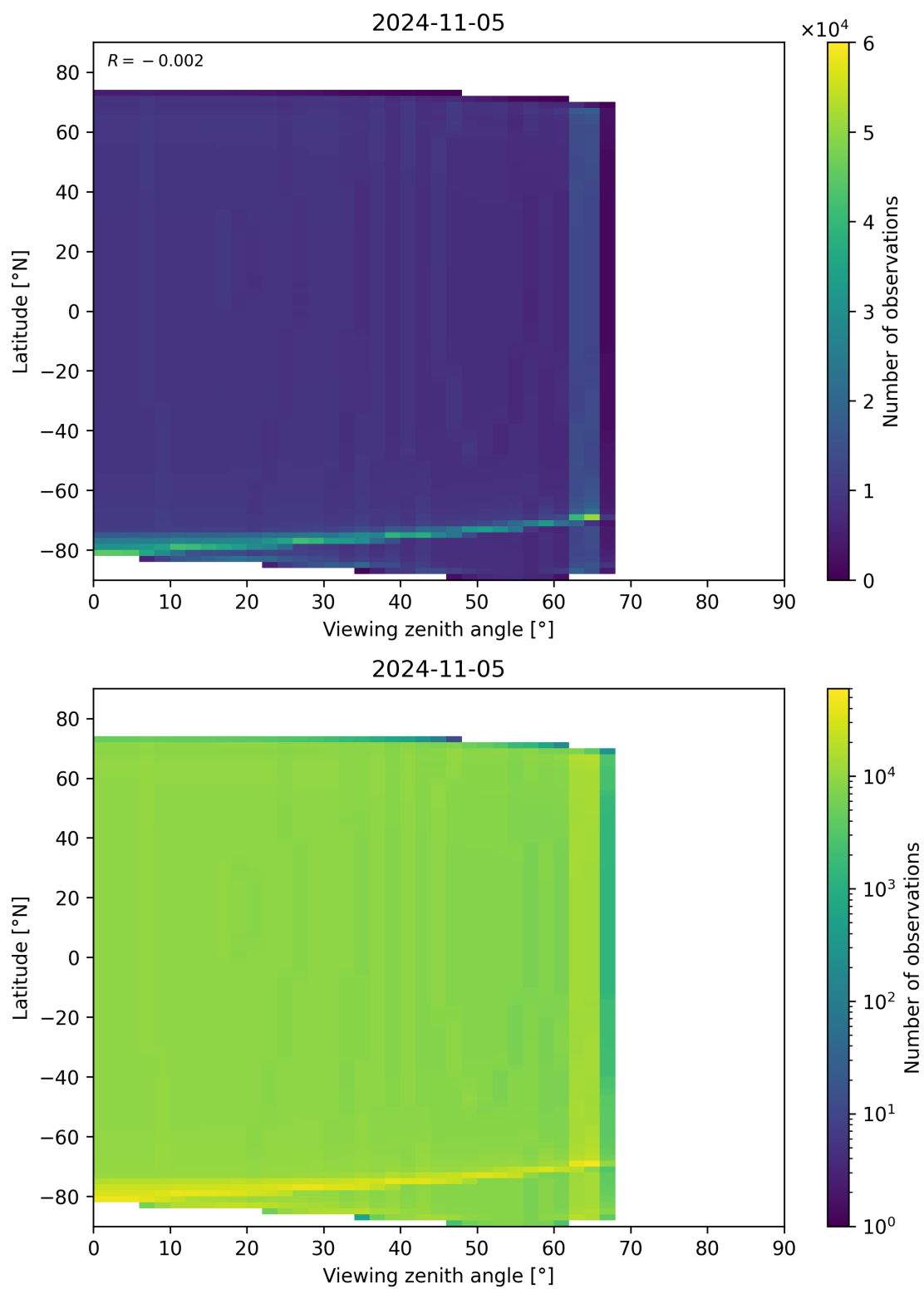
Figure 49: Scatter density plot of “Viewing zenith angle” against “Latitude” for 2024-11-04 to 2024-11-06.
