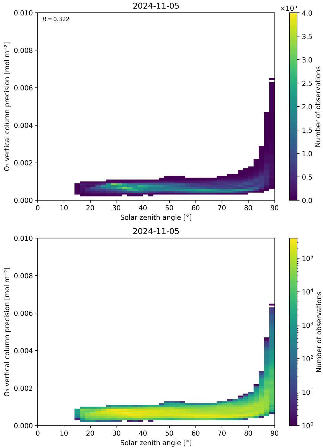
Figure 48: Scatter density plot of “Solar zenith angle” against “O 3 vertical column precision” for 2024-11-04 to 2024-11-06.
