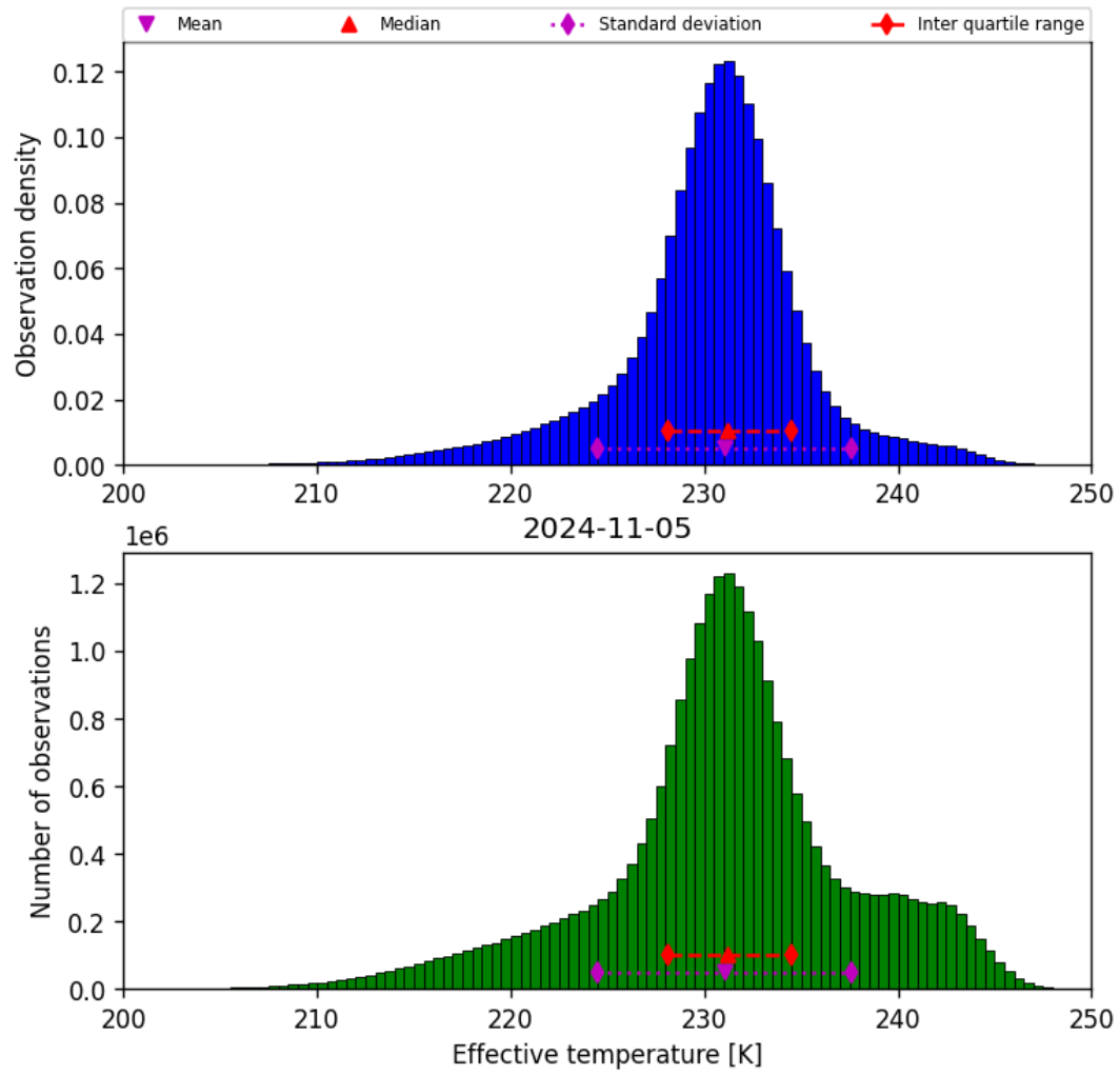
Figure 24: Histogram of “Effective temperature” for 2024-11-04 to 2024-11-06
