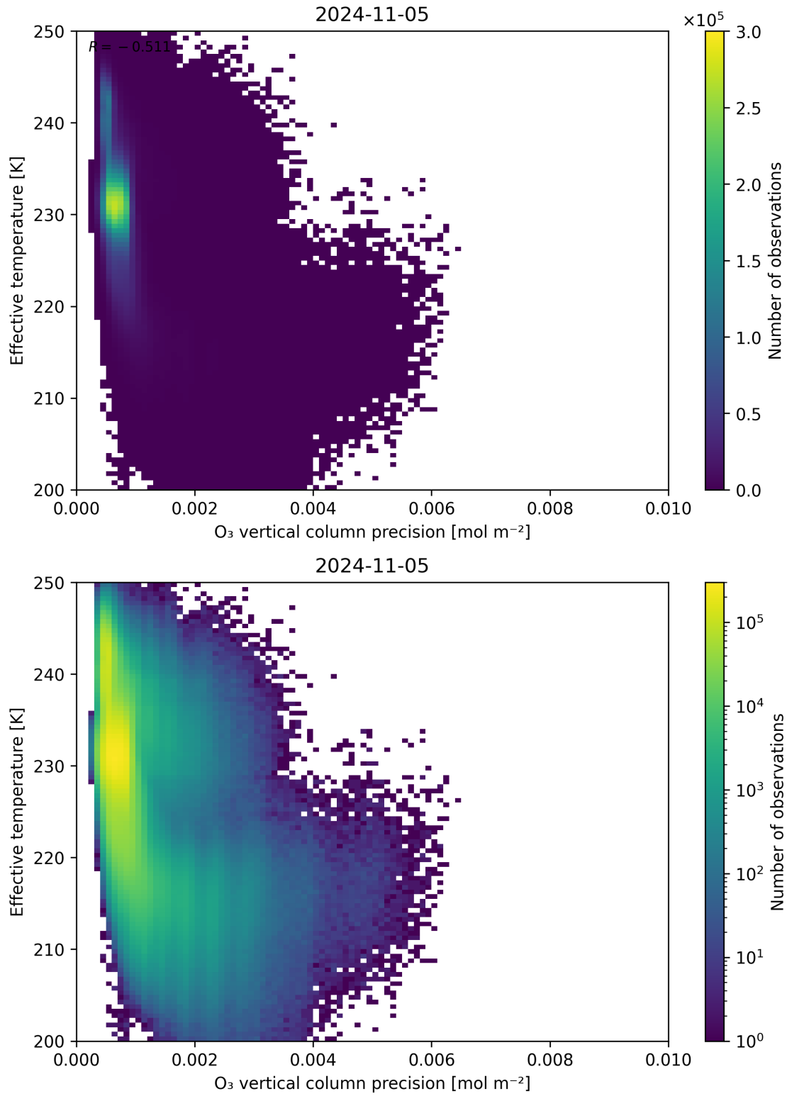
Figure 42: Scatter density plot of “O 3 vertical column precision” against “Effective temperature” for 2024-11-04 to 2024-11-06.
