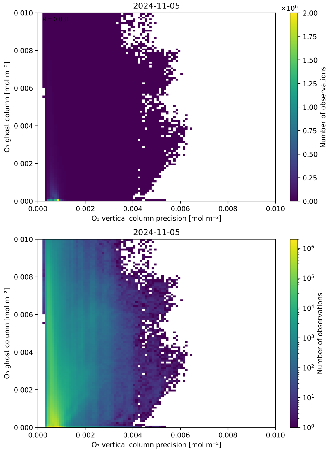
Figure 43: Scatter density plot of “O 3 vertical column precision” against “O 3 ghost column” for 2024-11-04 to 2024-11-06.
