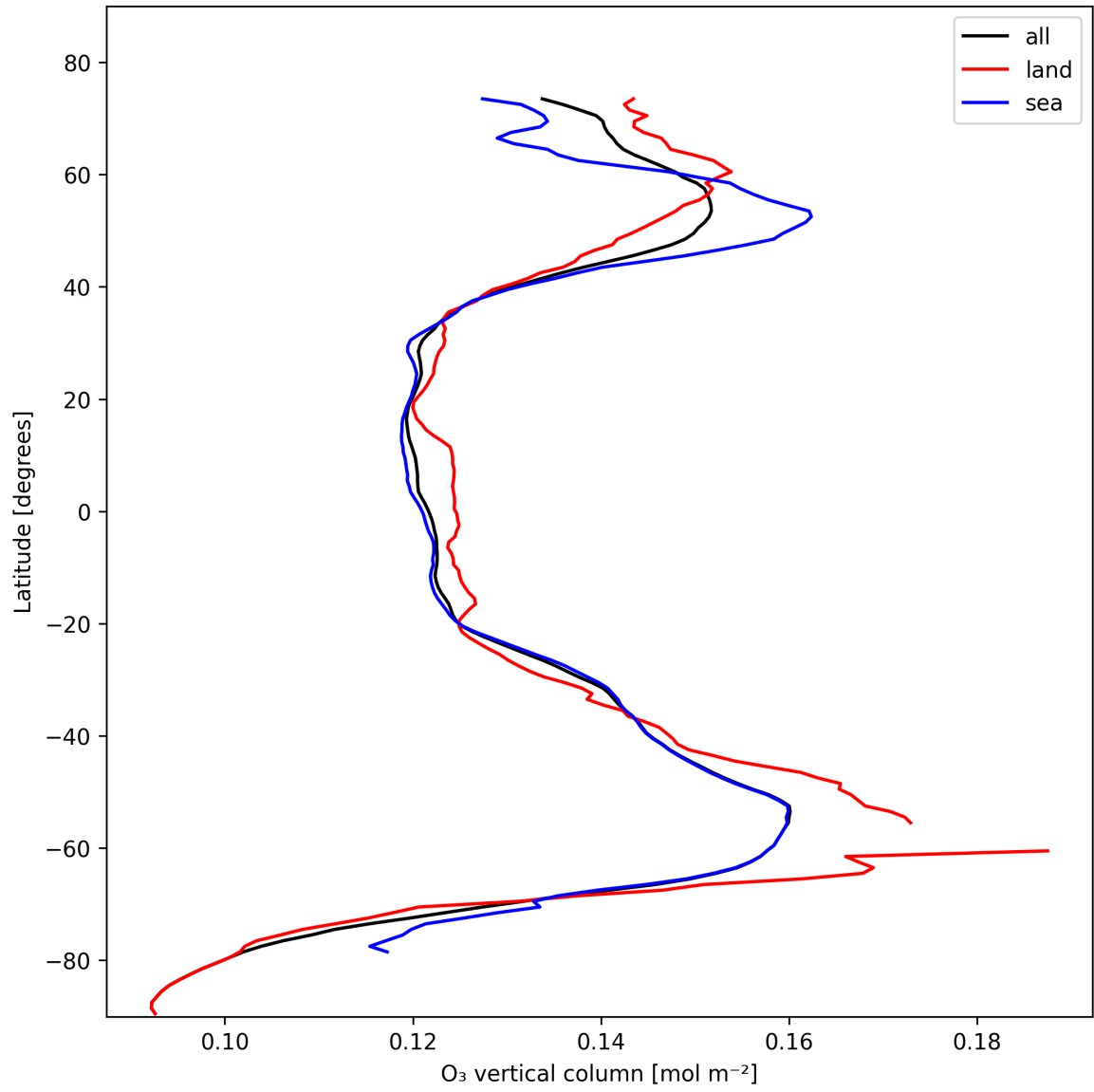
Figure 14: Zonal average of “O 3 vertical column” for 2024-11-04 to 2024-11-06.
