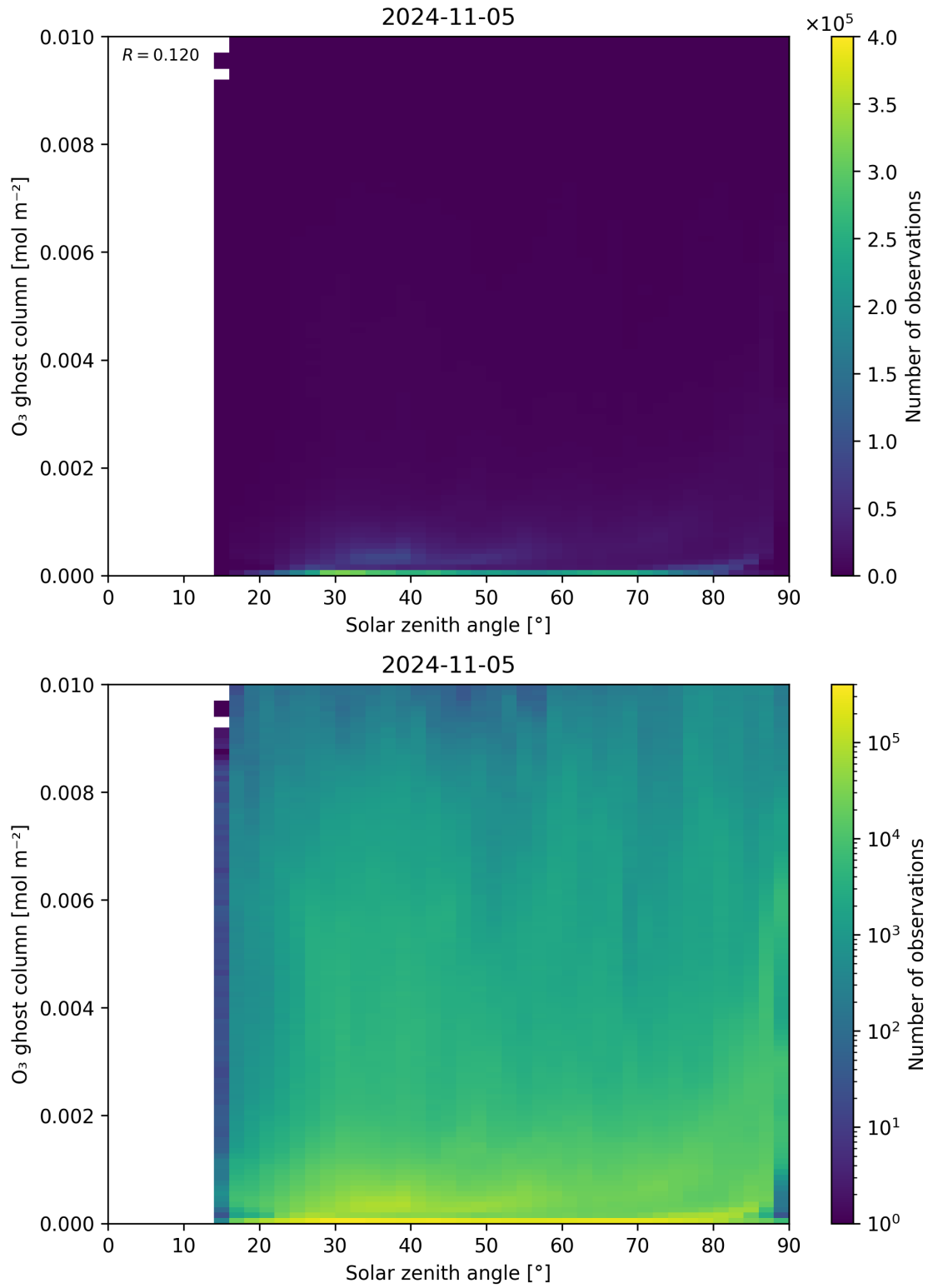
Figure 46: Scatter density plot of “Solar zenith angle” against “O 3 ghost column” for 2024-11-04 to 2024-11-06.
