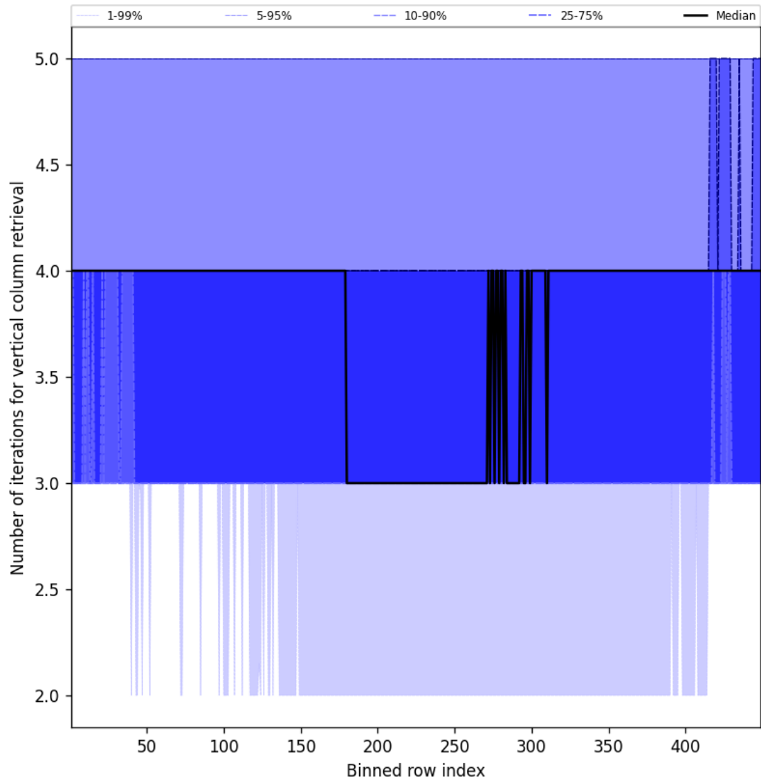
Figure 33: Along track statistics of “Number of iterations for vertical column retrieval” for 2024-11-04 to 2024-11-06
