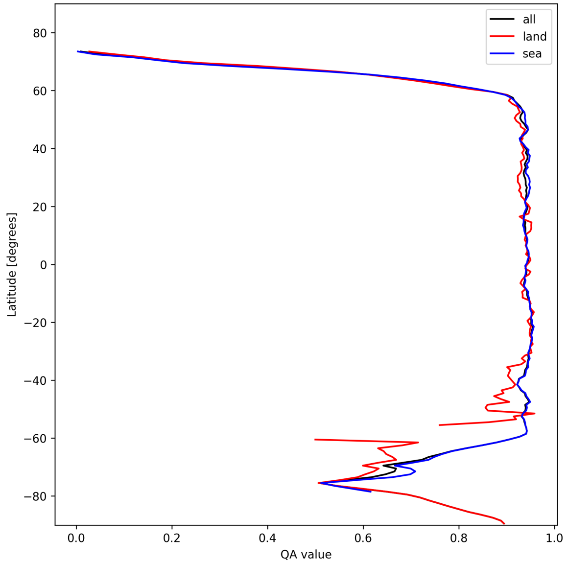
Figure 13: Zonal average of “QA value” for 2024-11-04 to 2024-11-06.
