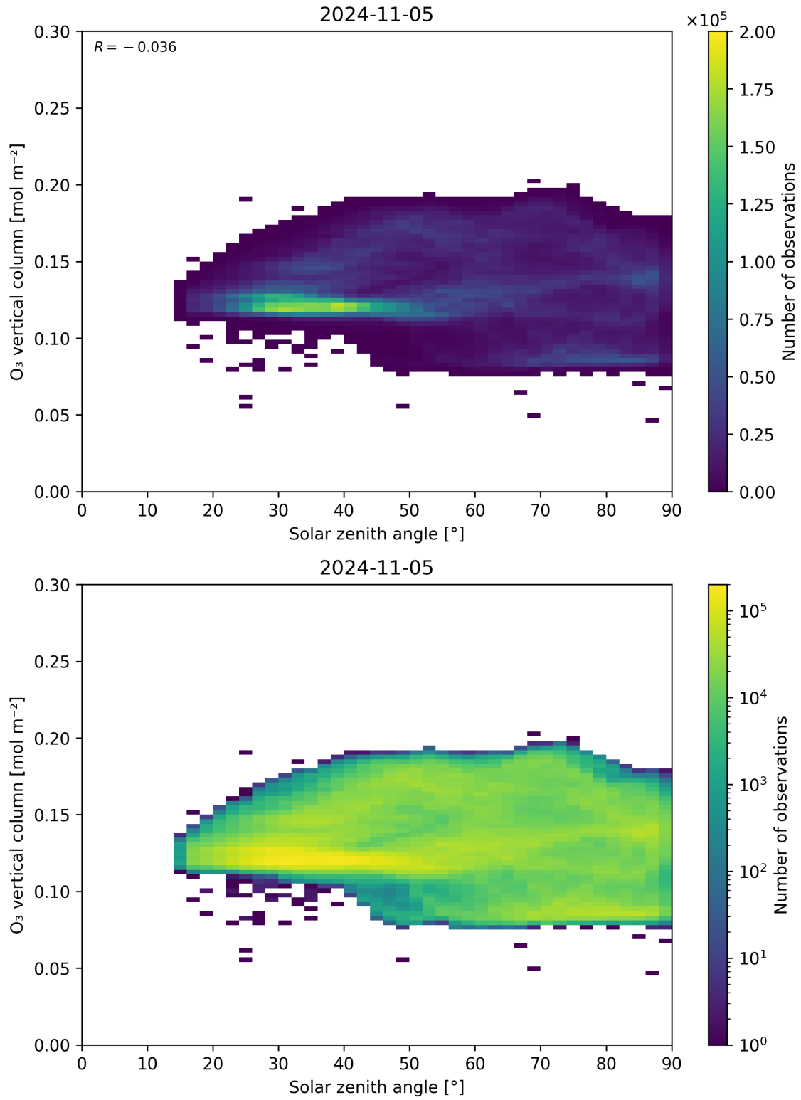
Figure 47: Scatter density plot of “Solar zenith angle” against “O 3 vertical column” for 2024-11-04 to 2024-11-06.
