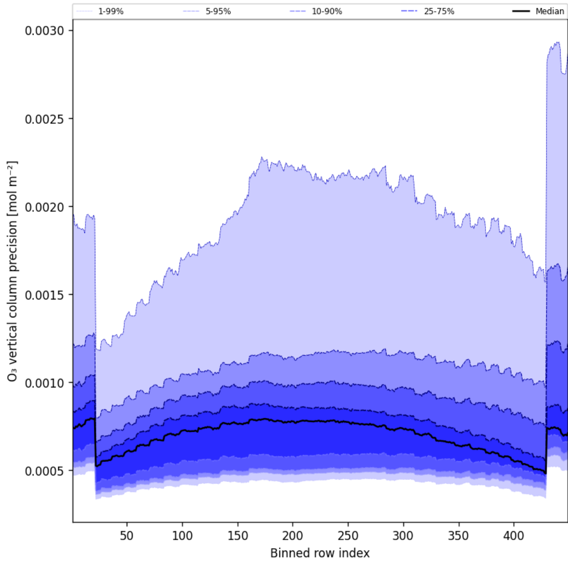
Figure 29: Along track statistics of “O 3 vertical column precision” for 2024-11-04 to 2024-11-06
