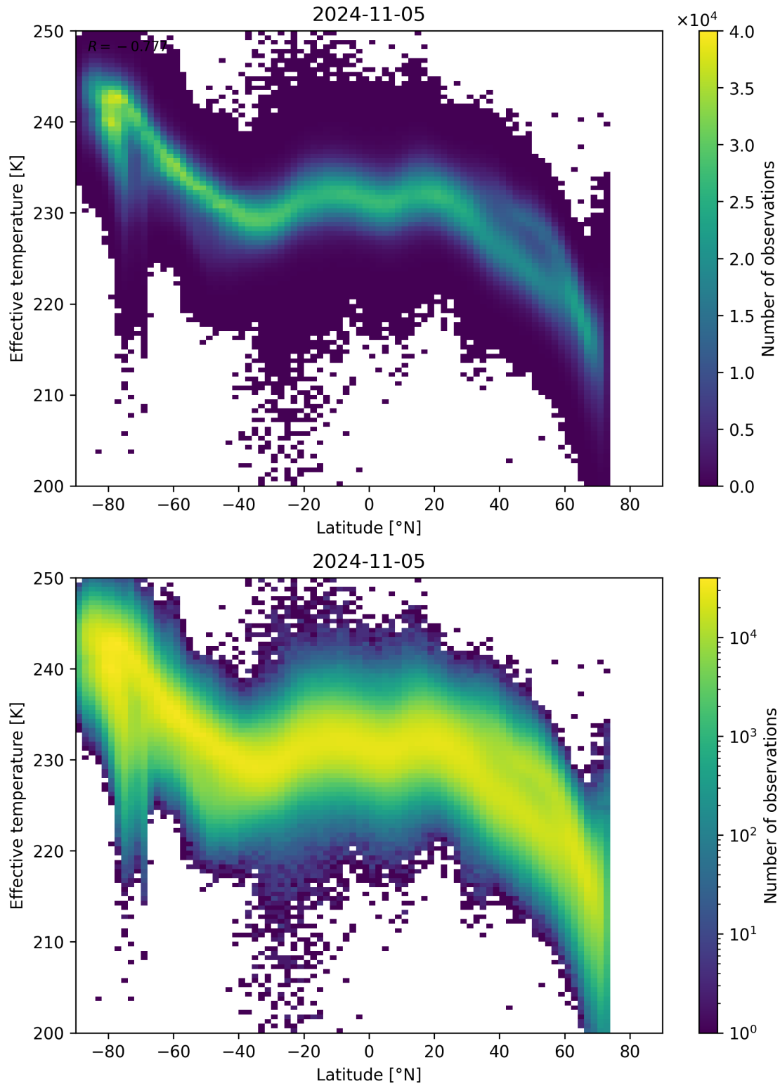
Figure 34: Scatter density plot of “Latitude” against “Effective temperature” for 2024-11-04 to 2024-11-06.
