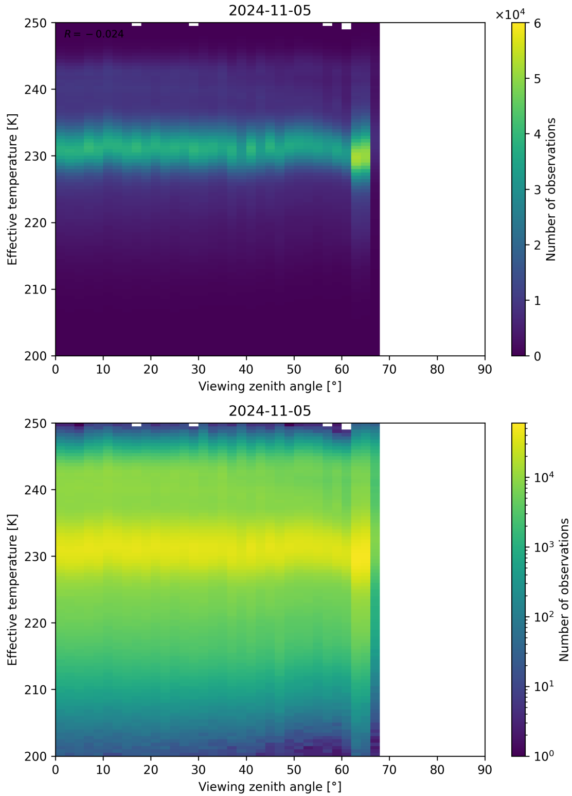
Figure 50: Scatter density plot of “Viewing zenith angle” against “Effective temperature” for 2024-11-04 to 2024-11-06.
