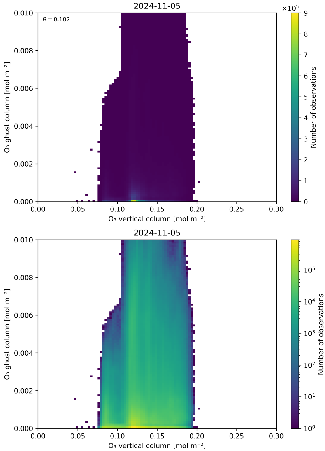
Figure 40: Scatter density plot of “O 3 vertical column” against “O 3 ghost column” for 2024-11-04 to 2024-11-06.
