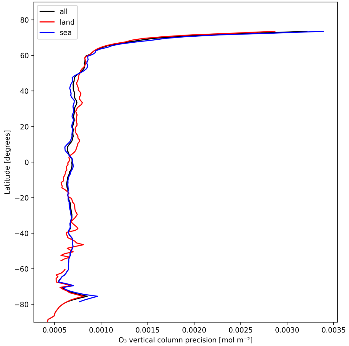
Figure 15: Zonal average of “O 3 vertical column precision” for 2024-11-04 to 2024-11-06.
