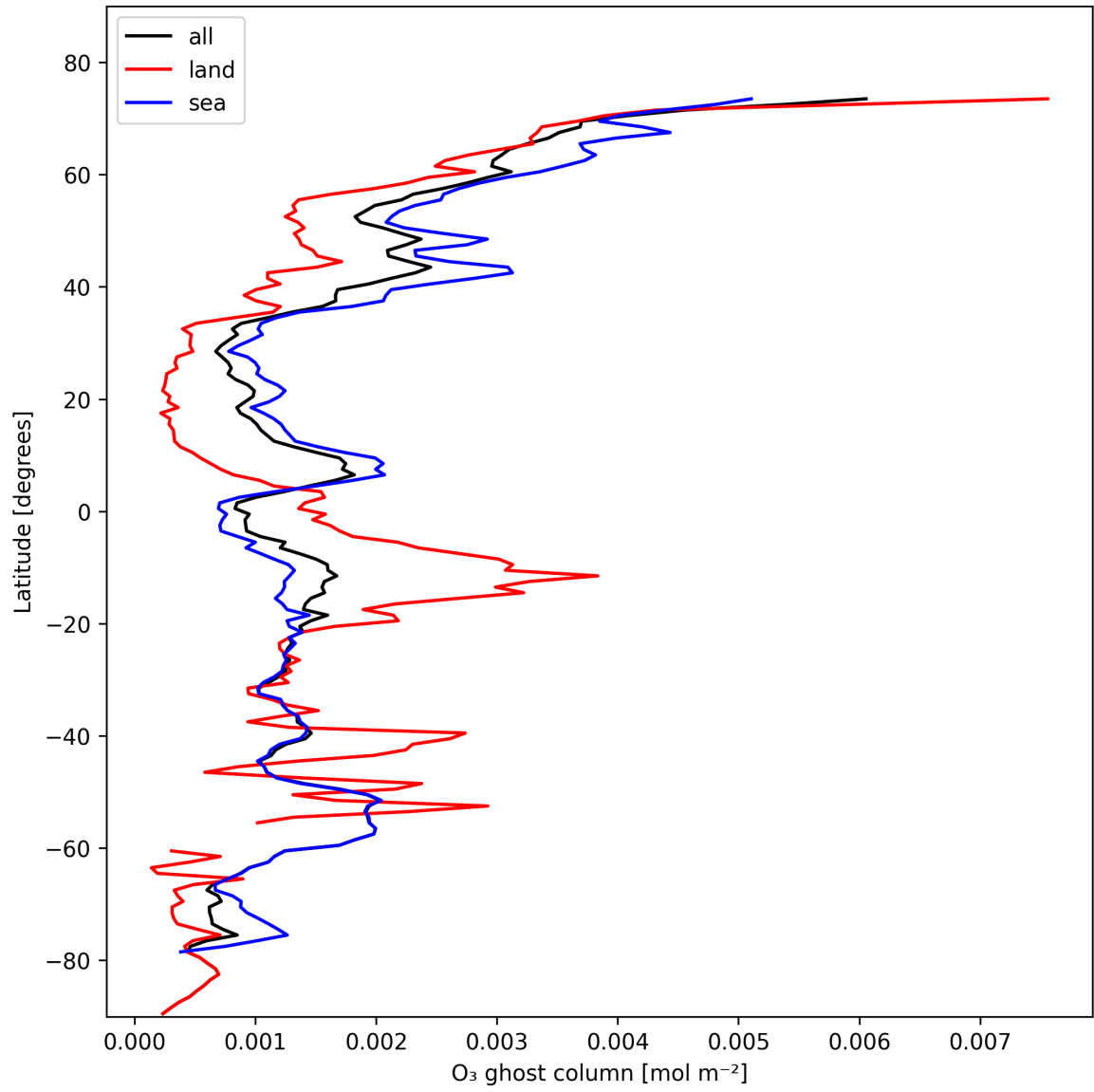
Figure 18: Zonal average of "O 3 ghost column" for 2024-11-04 to 2024-11-06.
