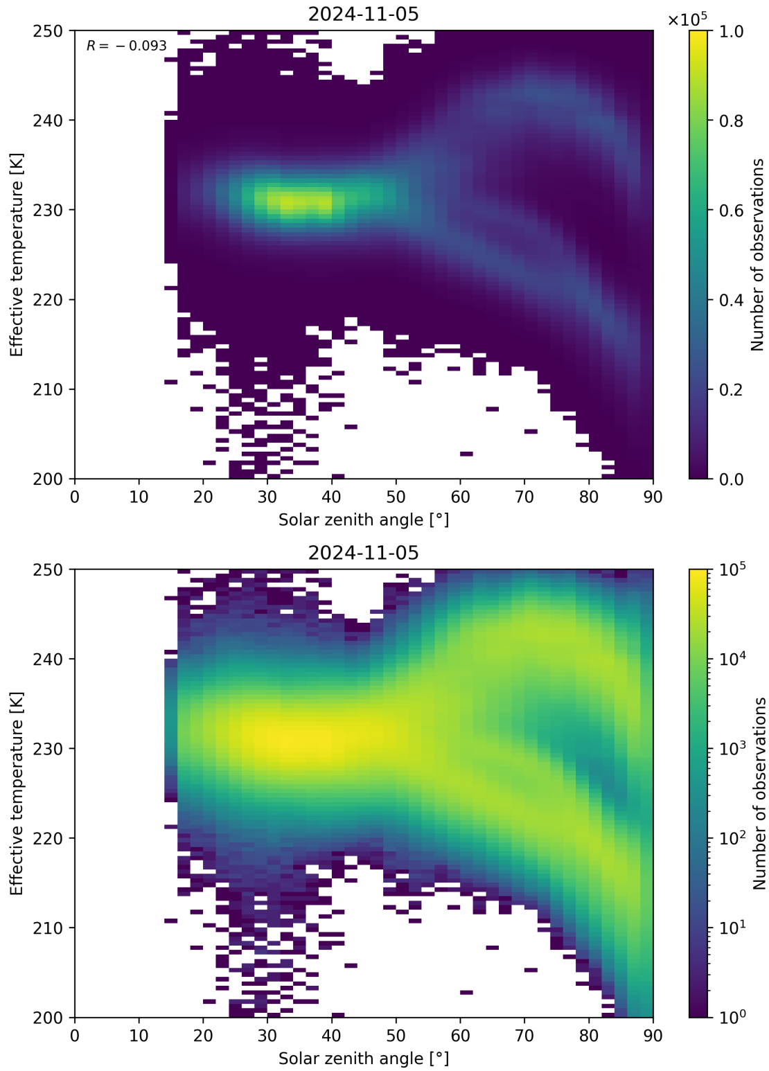
Figure 45: Scatter density plot of “Solar zenith angle” against “Effective temperature” for 2024-11-04 to 2024-11-06.
