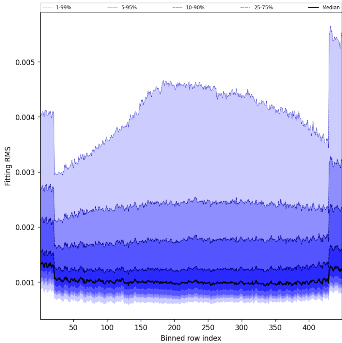
Figure 30: Along track statistics of “Fitting RMS” for 2024-11-04 to 2024-11-06
