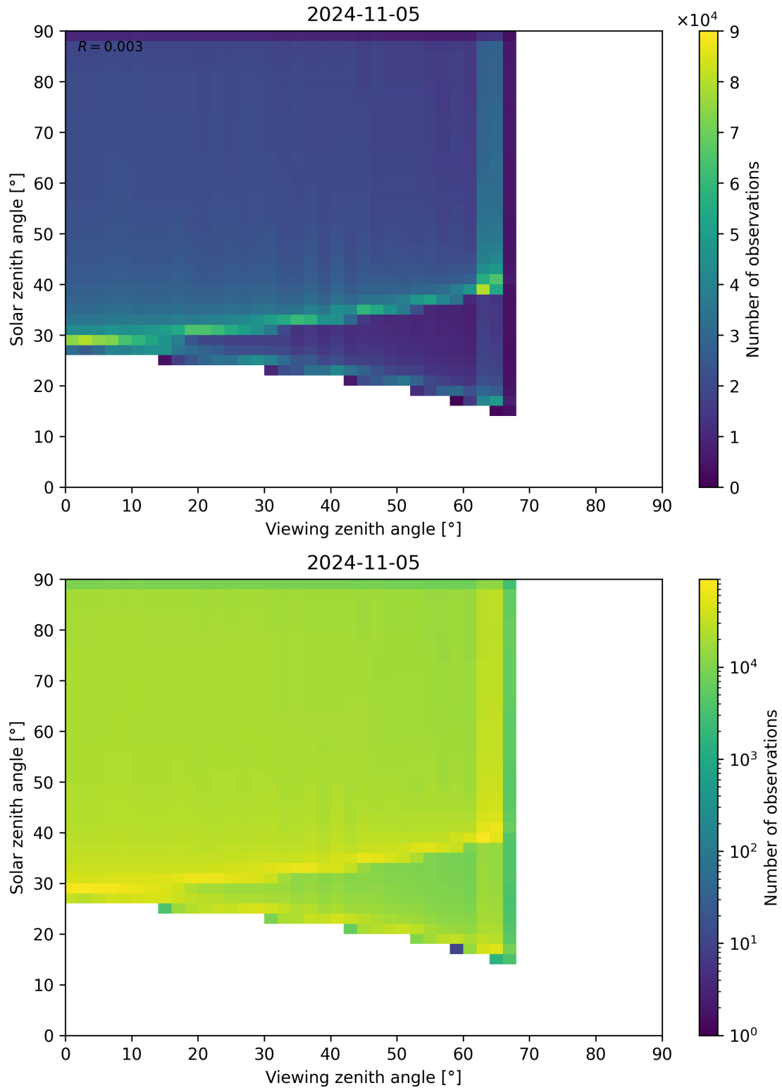
Figure 54: Scatter density plot of “Viewing zenith angle” against “Solar zenith angle” for 2024-11-04 to 2024-11-06.
