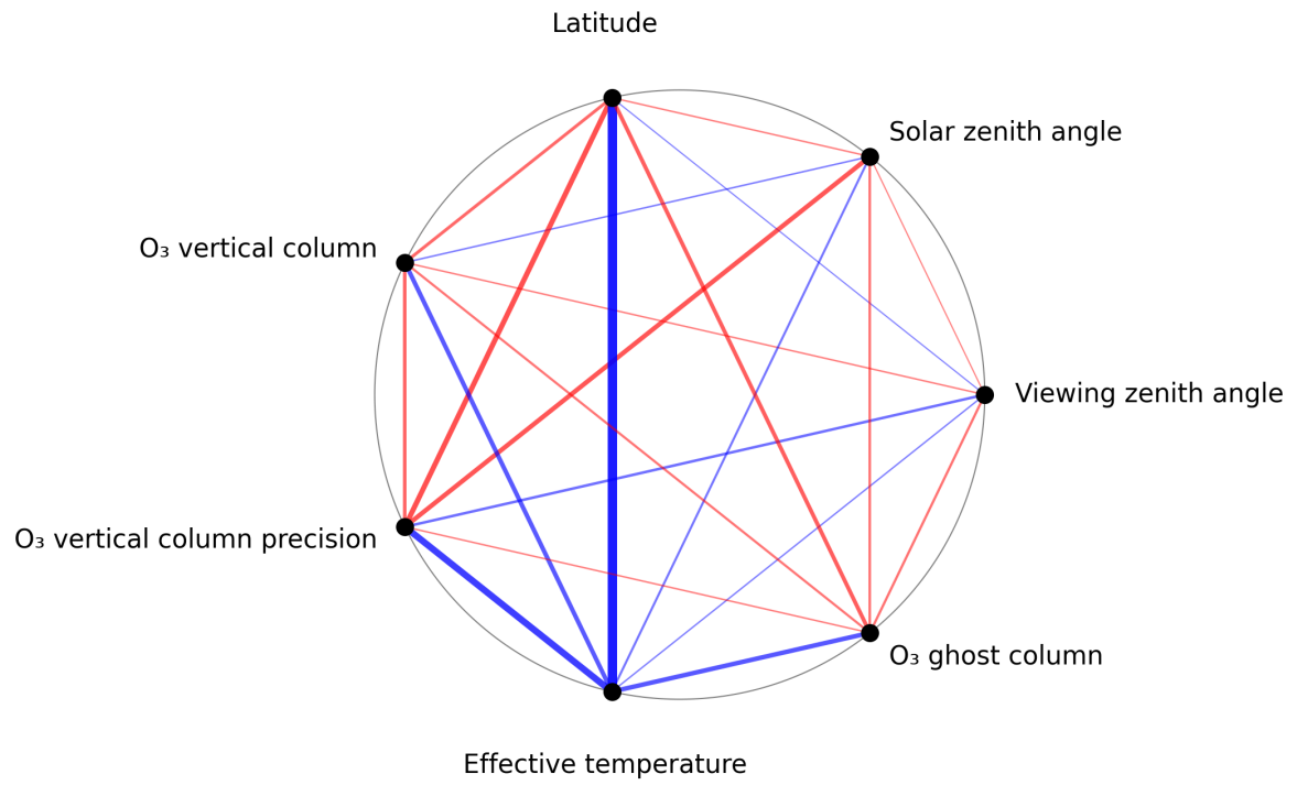
Figure 1: Map of correlation graph for 2024-11-04 to 2024-11-06.
