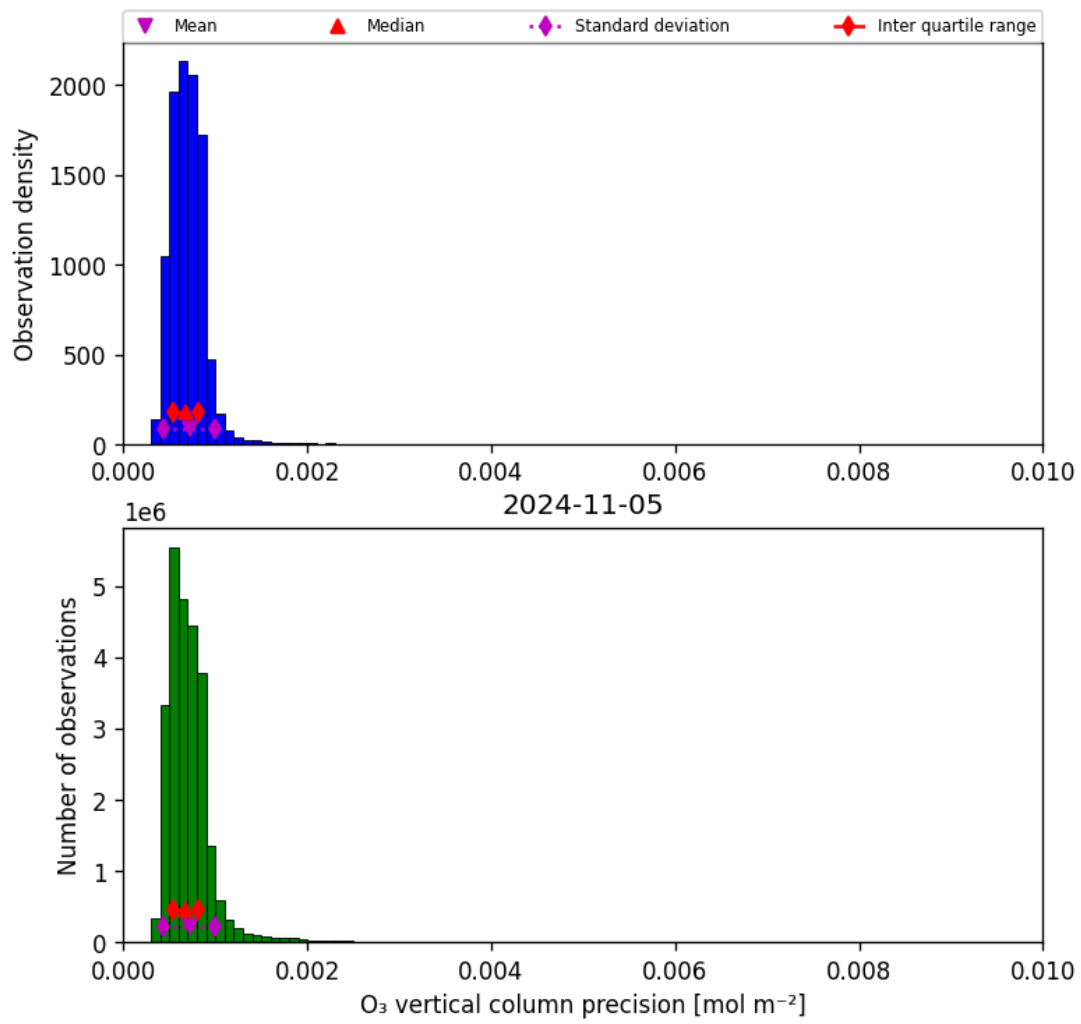
Figure 22: Histogram of “O 3 vertical column precision” for 2024-11-04 to 2024-11-06
