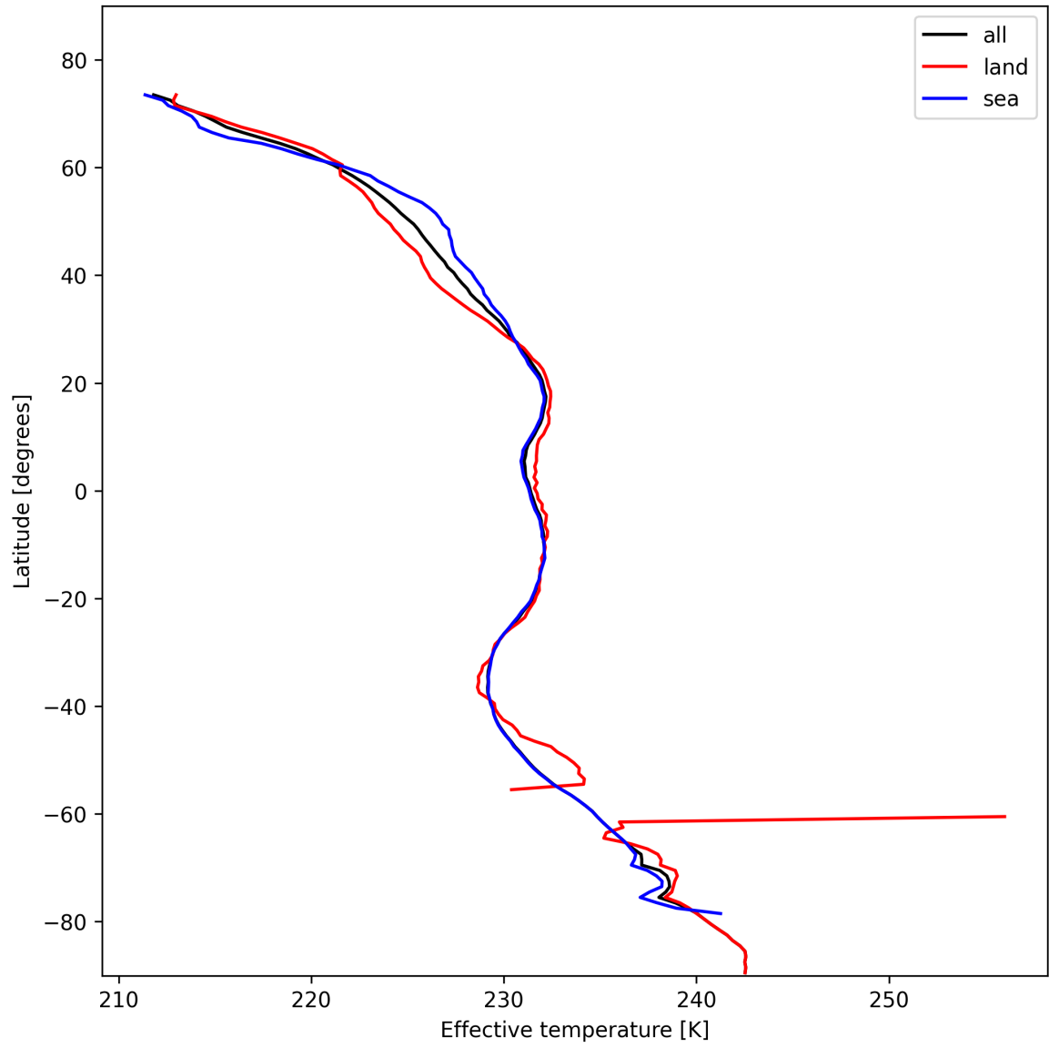
Figure 17: Zonal average of "Effective temperature" for 2024-11-04 to 2024-11-06.
