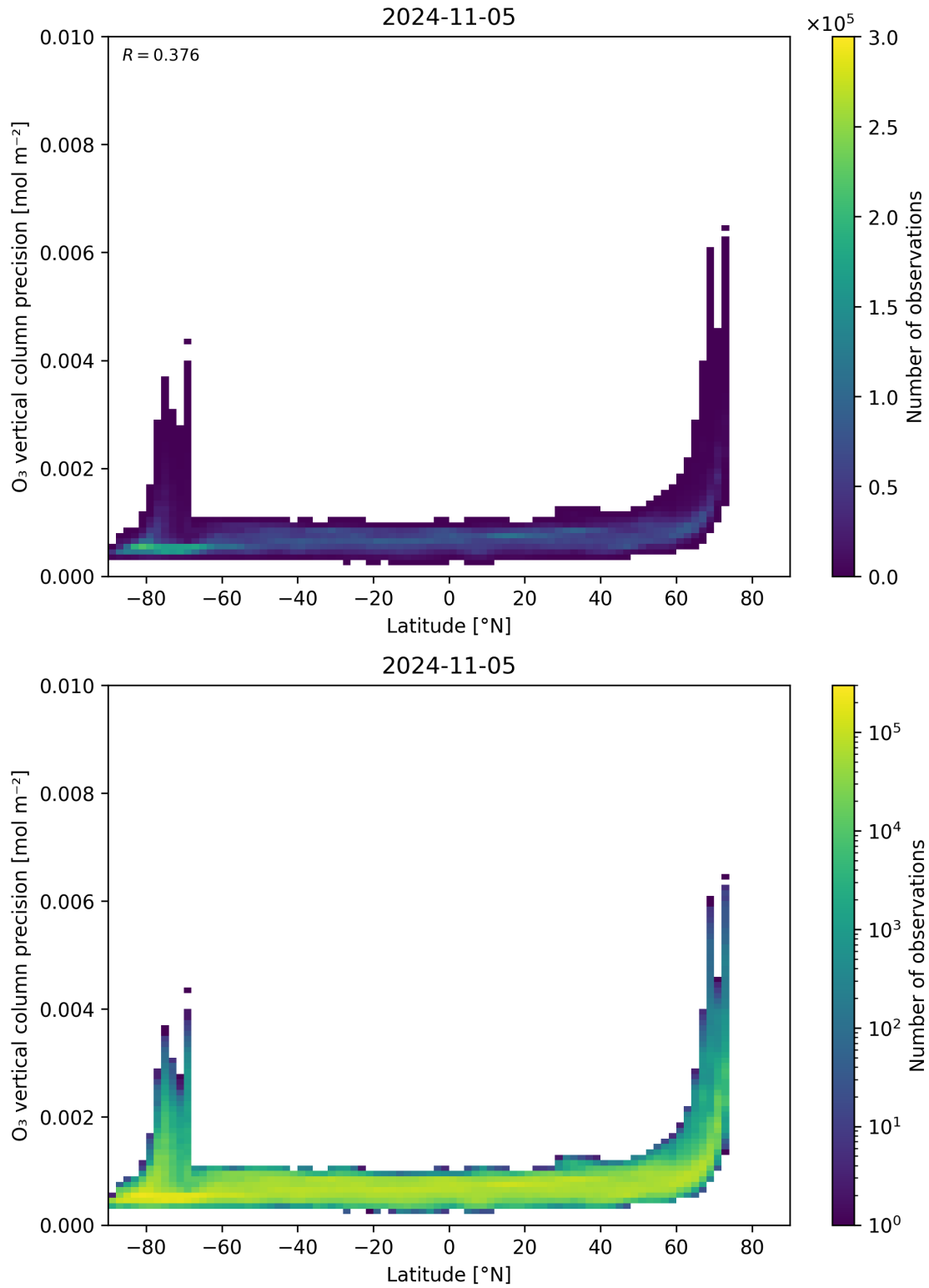
Figure 37: Scatter density plot of “Latitude” against “O 3 vertical column precision” for 2024-11-04 to 2024-11-06.
