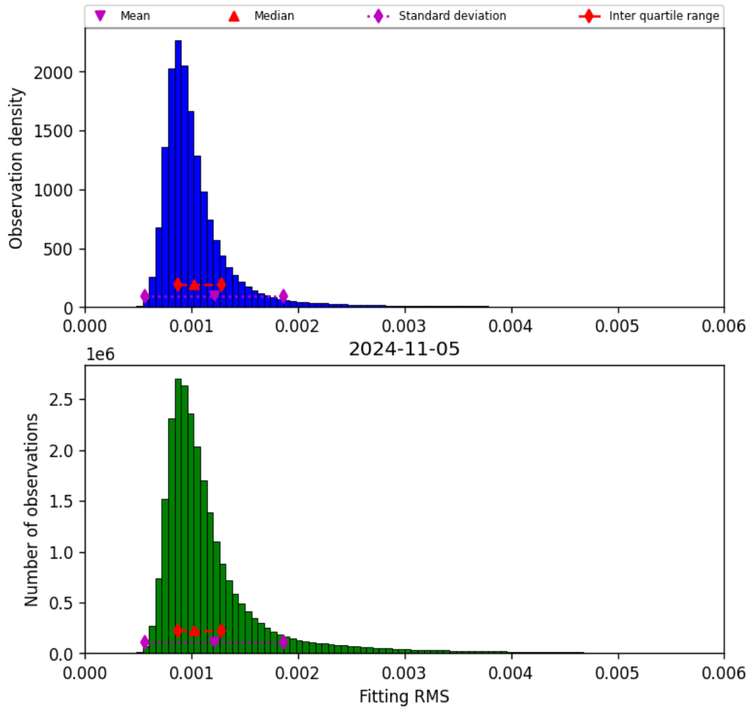
Figure 23: Histogram of “Fitting RMS” for 2024-11-04 to 2024-11-06
