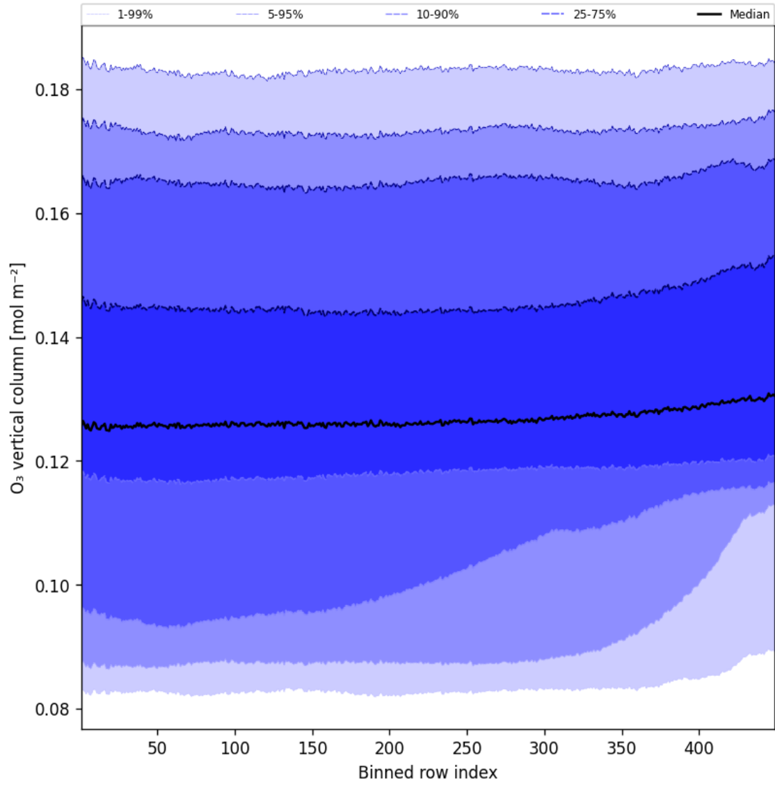
Figure 28: Along track statistics of “O 3 vertical column” for 2024-11-04 to 2024-11-06
