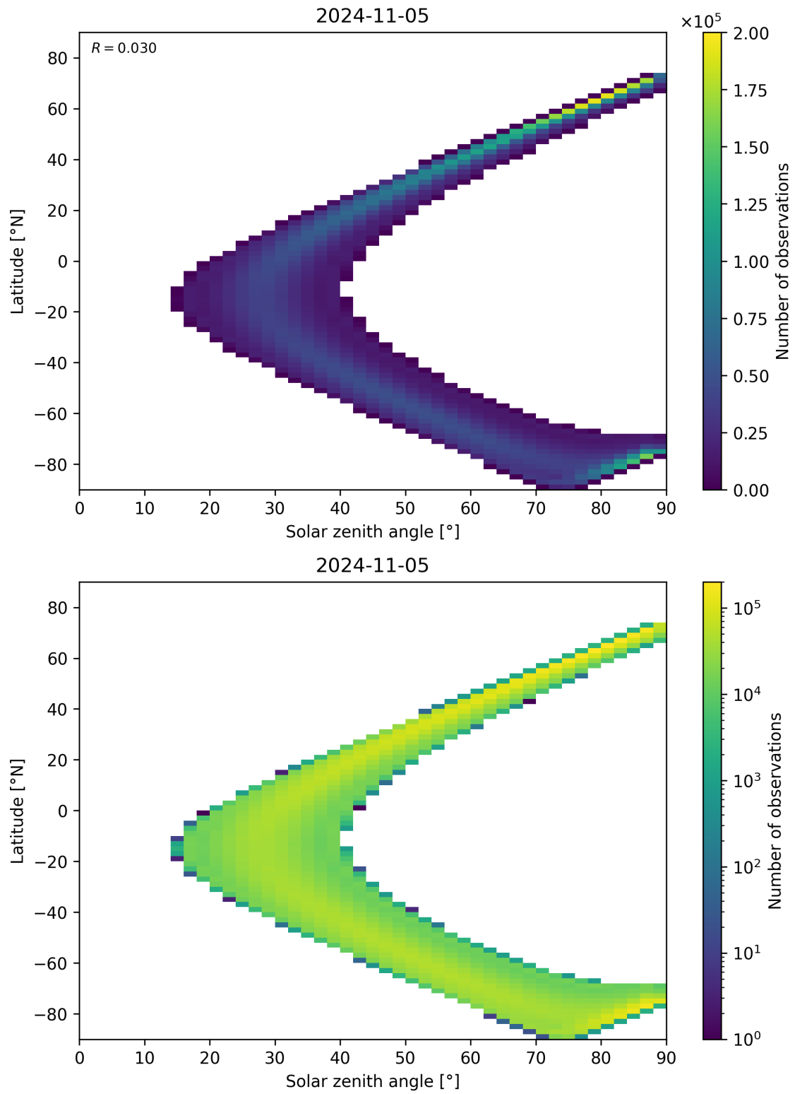
Figure 44: Scatter density plot of “Solar zenith angle” against “Latitude” for 2024-11-04 to 2024-11-06.
