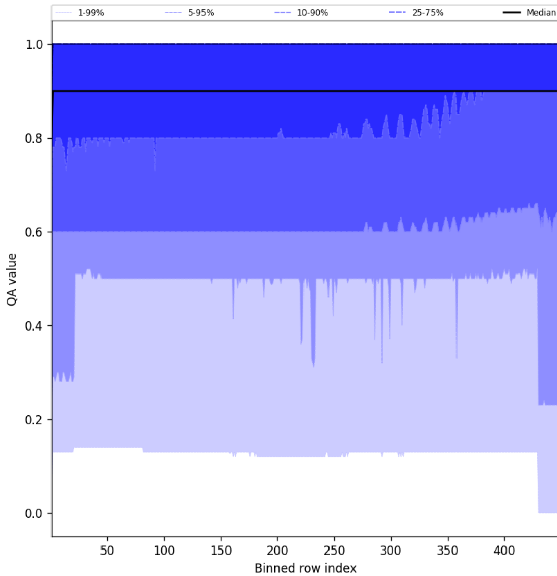
Figure 27: Along track statistics of “QA value” for 2024-11-04 to 2024-11-06
