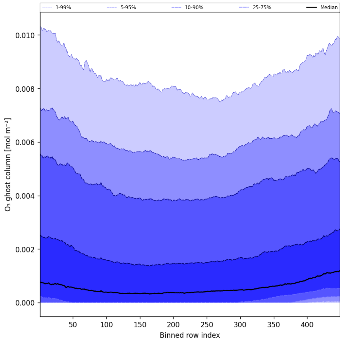
Figure 32: Along track statistics of “O 3 ghost column” for 2024-11-04 to 2024-11-06
