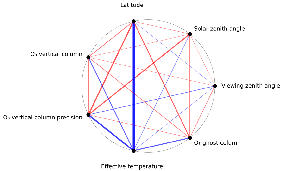
Figure 1: Map of correlation graph for 2024-11-05 to 2024-11-07.
