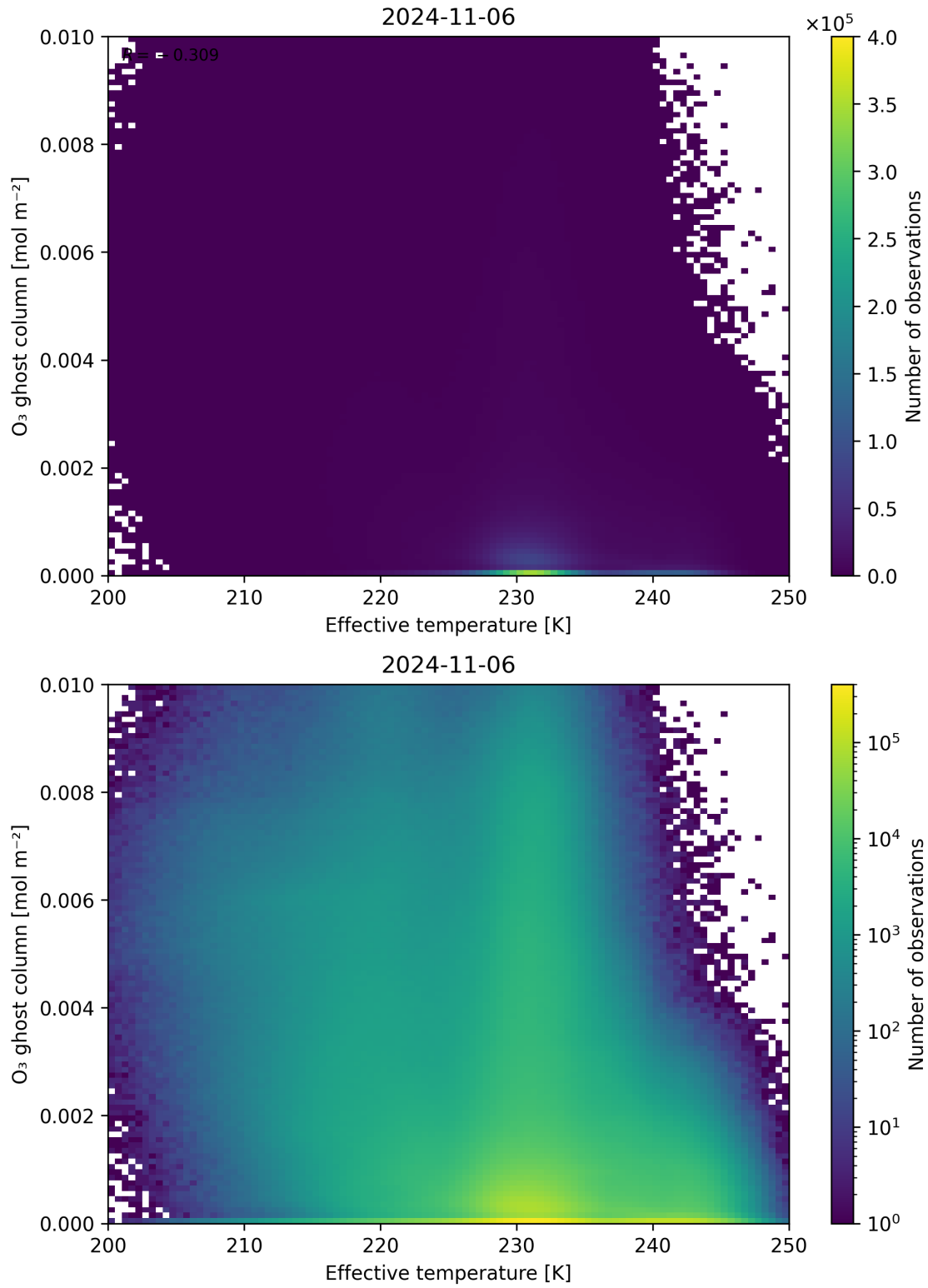
Figure 38: Scatter density plot of “Effective temperature” against “O 3 ghost column” for 2024-11-05 to 2024-11-07.
