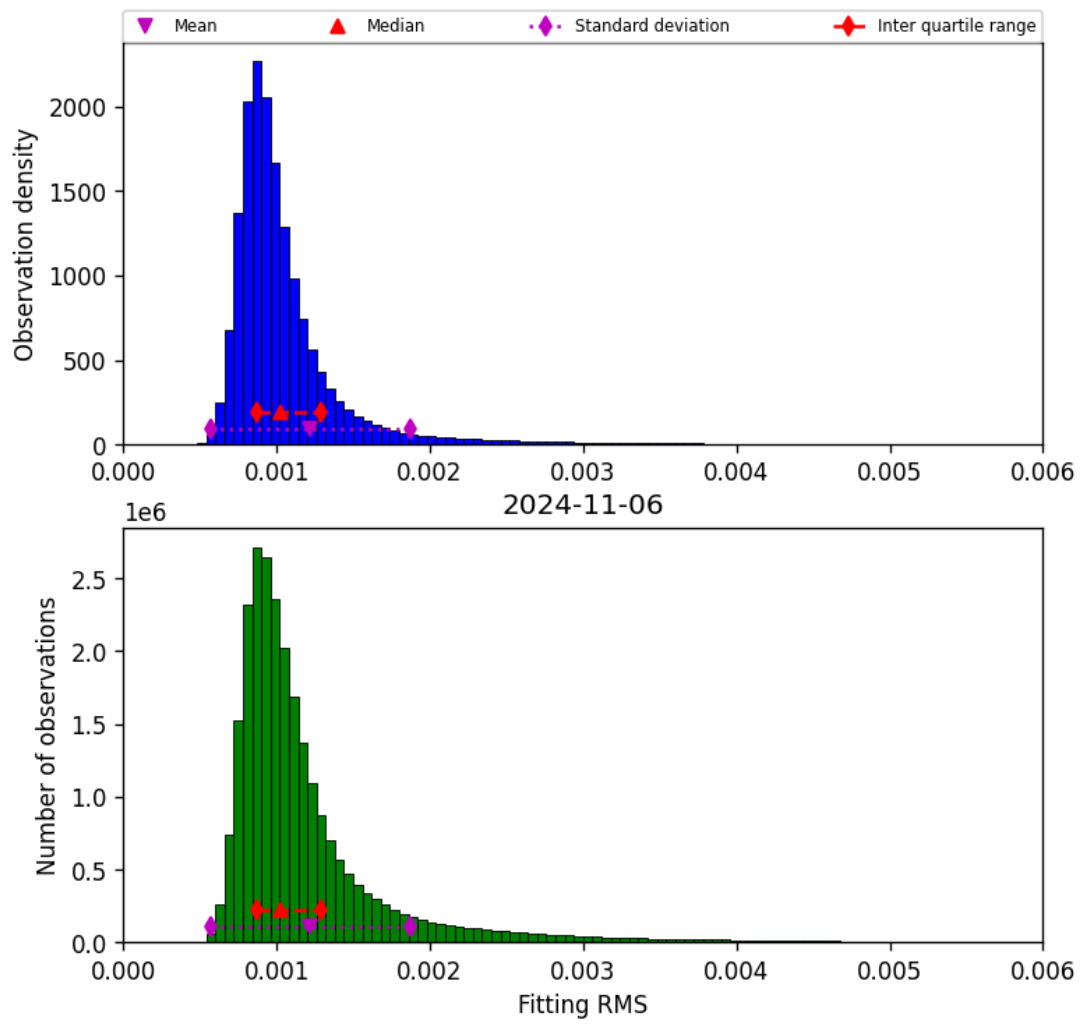
Figure 23: Histogram of “Fitting RMS” for 2024-11-05 to 2024-11-07
