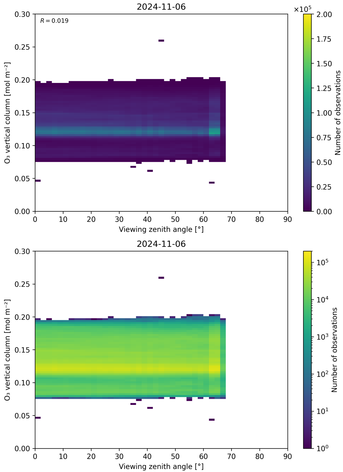
Figure 52: Scatter density plot of “Viewing zenith angle” against “O 3 vertical column” for 2024-11-05 to 2024-11-07.
