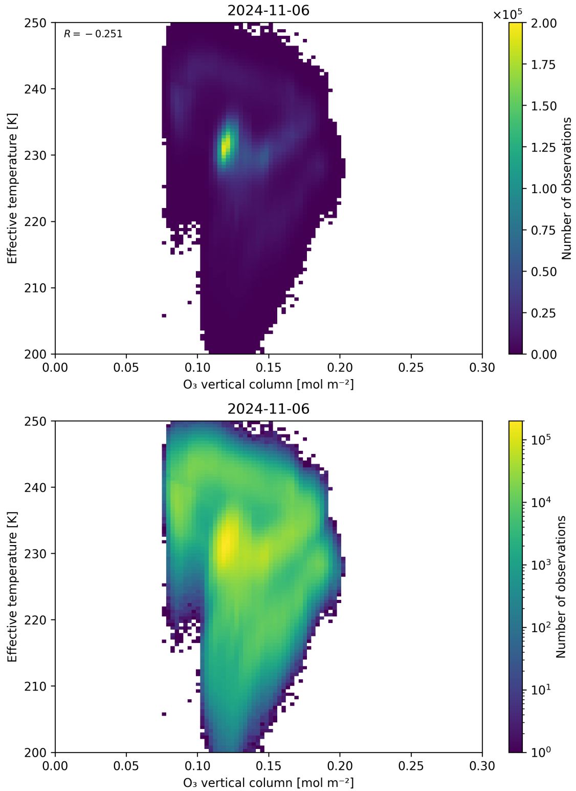
Figure 39: Scatter density plot of “O 3 vertical column” against “Effective temperature” for 2024-11-05 to 2024-11-07.
