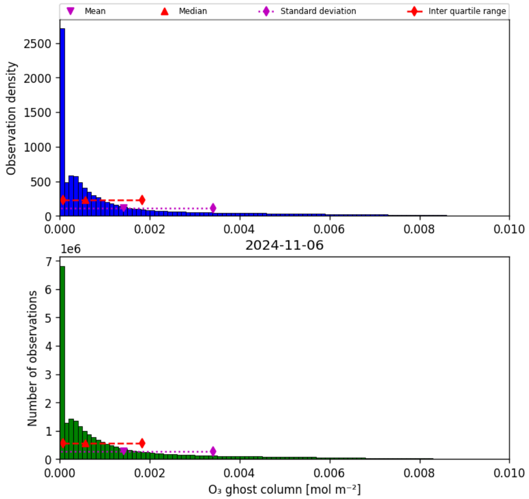
Figure 25: Histogram of “O 3 ghost column” for 2024-11-05 to 2024-11-07
