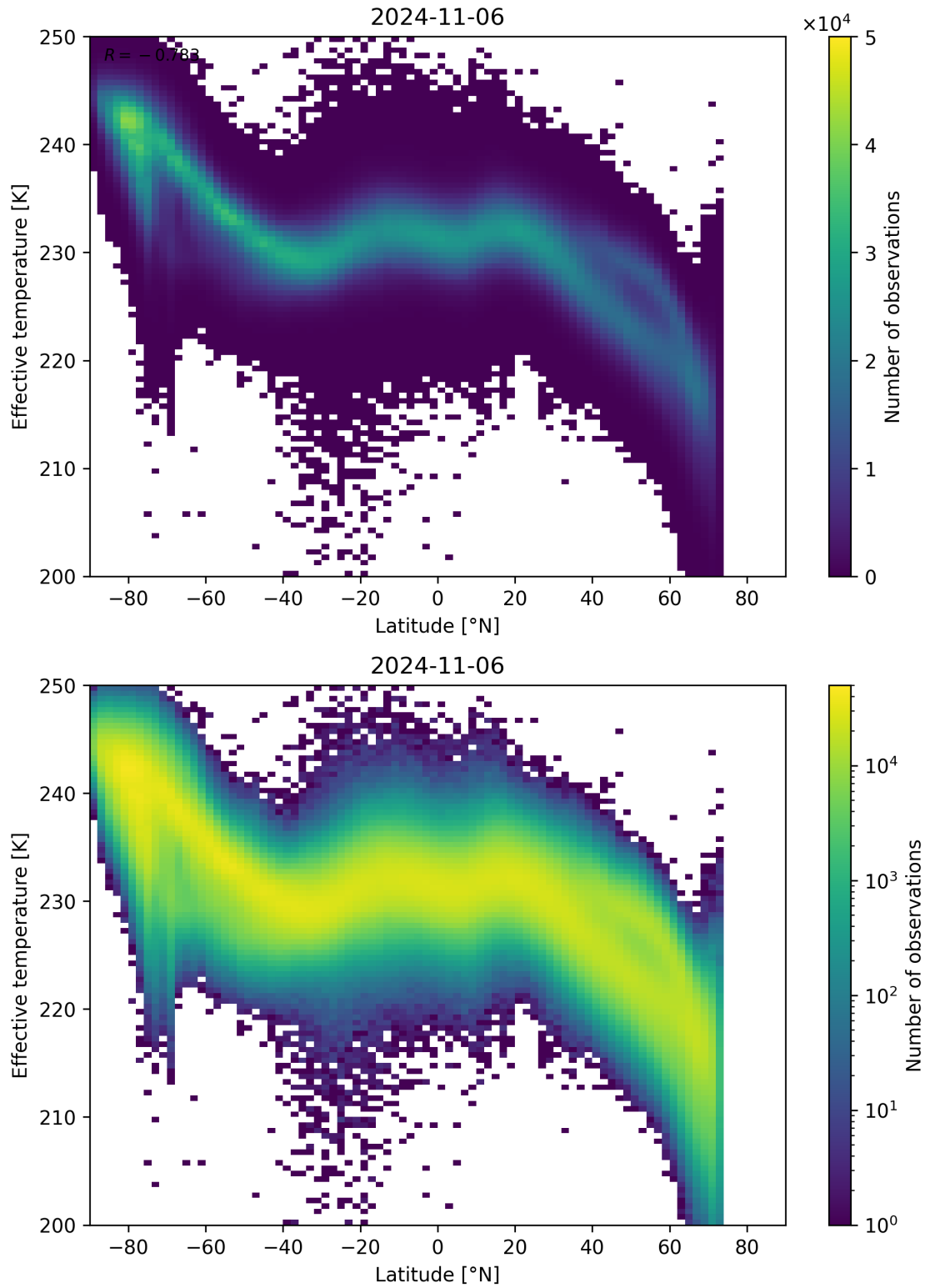
Figure 34: Scatter density plot of “Latitude” against “Effective temperature” for 2024-11-05 to 2024-11-07.
