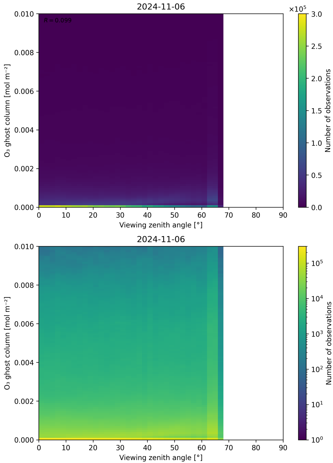
Figure 51: Scatter density plot of “Viewing zenith angle” against “O 3 ghost column” for 2024-11-05 to 2024-11-07.
