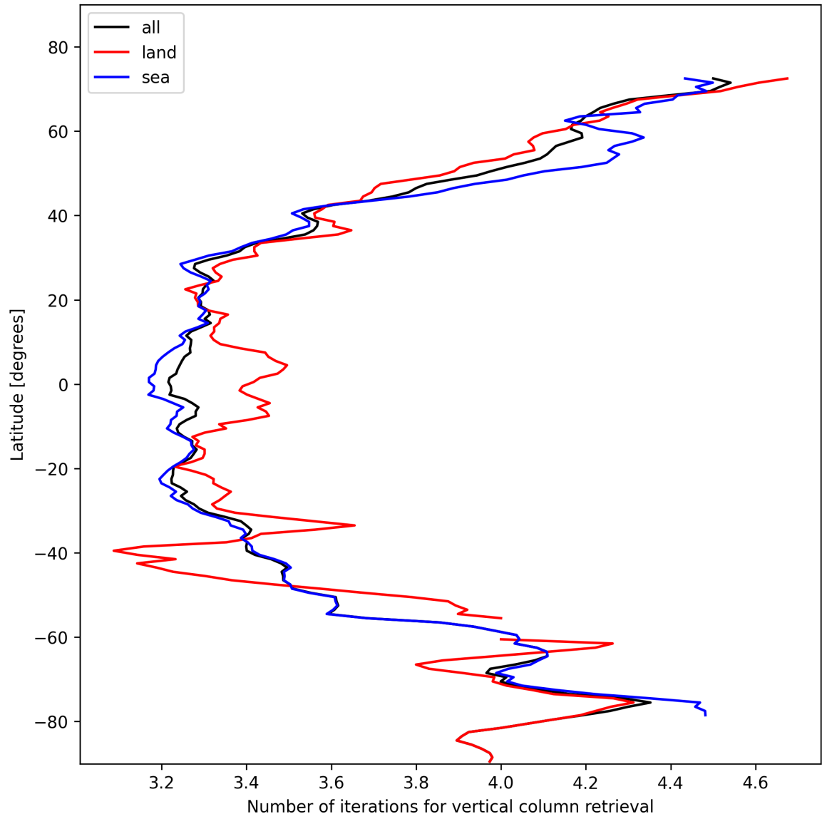
Figure 19: Zonal average of “Number of iterations for vertical column retrieval” for 2024-11-05 to 2024-11-07.
