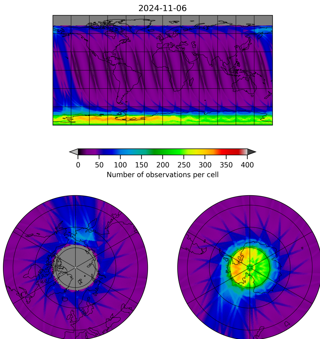
Figure 12: Map of the number of observations for 2024-11-05 to 2024-11-07
