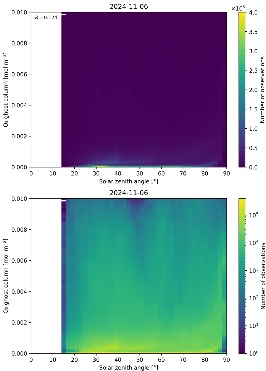
Figure 46: Scatter density plot of “Solar zenith angle” against “O 3 ghost column” for 2024-11-05 to 2024-11-07.
