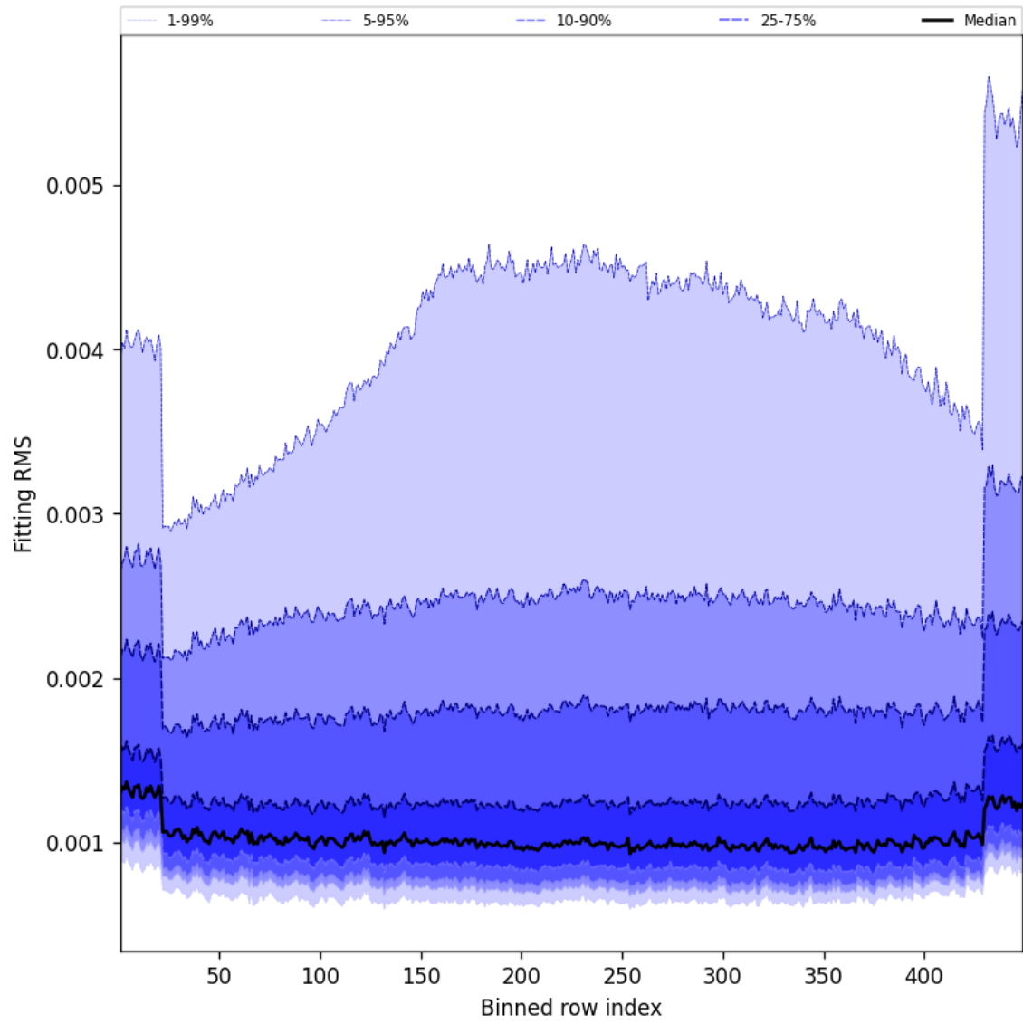
Figure 30: Along track statistics of “Fitting RMS” for 2024-11-05 to 2024-11-07
