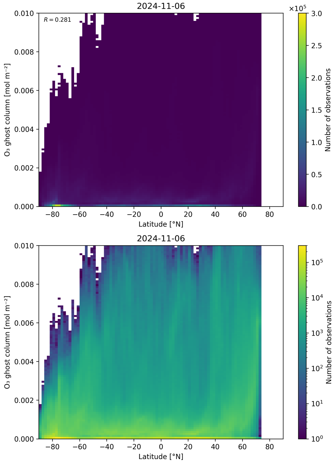
Figure 35: Scatter density plot of “Latitude” against “O 3 ghost column” for 2024-11-05 to 2024-11-07.
