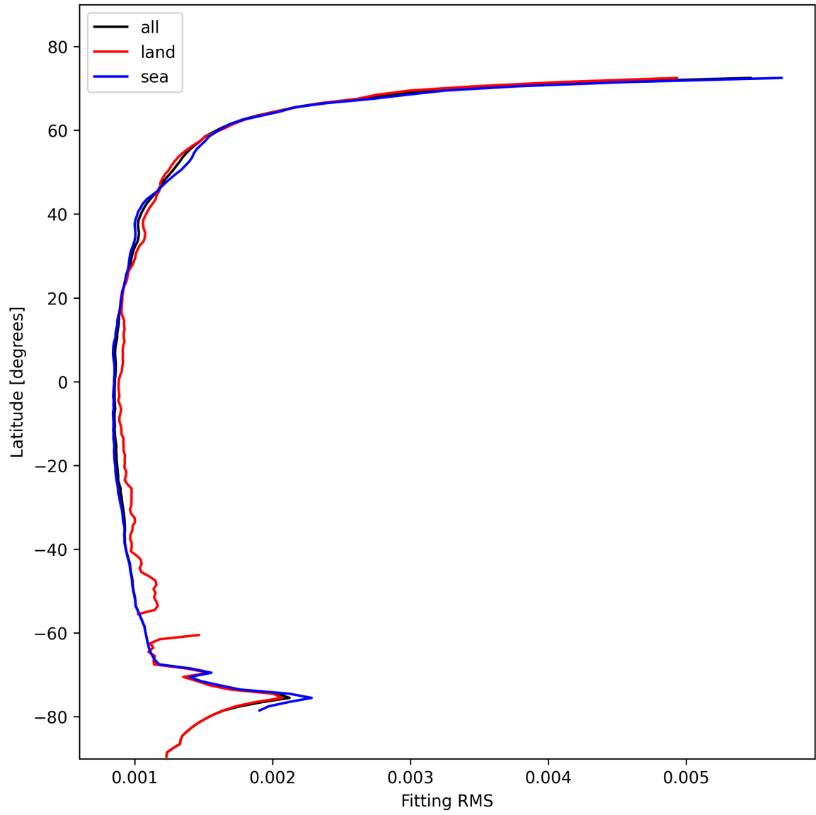
Figure 16: Zonal average of “Fitting RMS” for 2024-11-05 to 2024-11-07.
