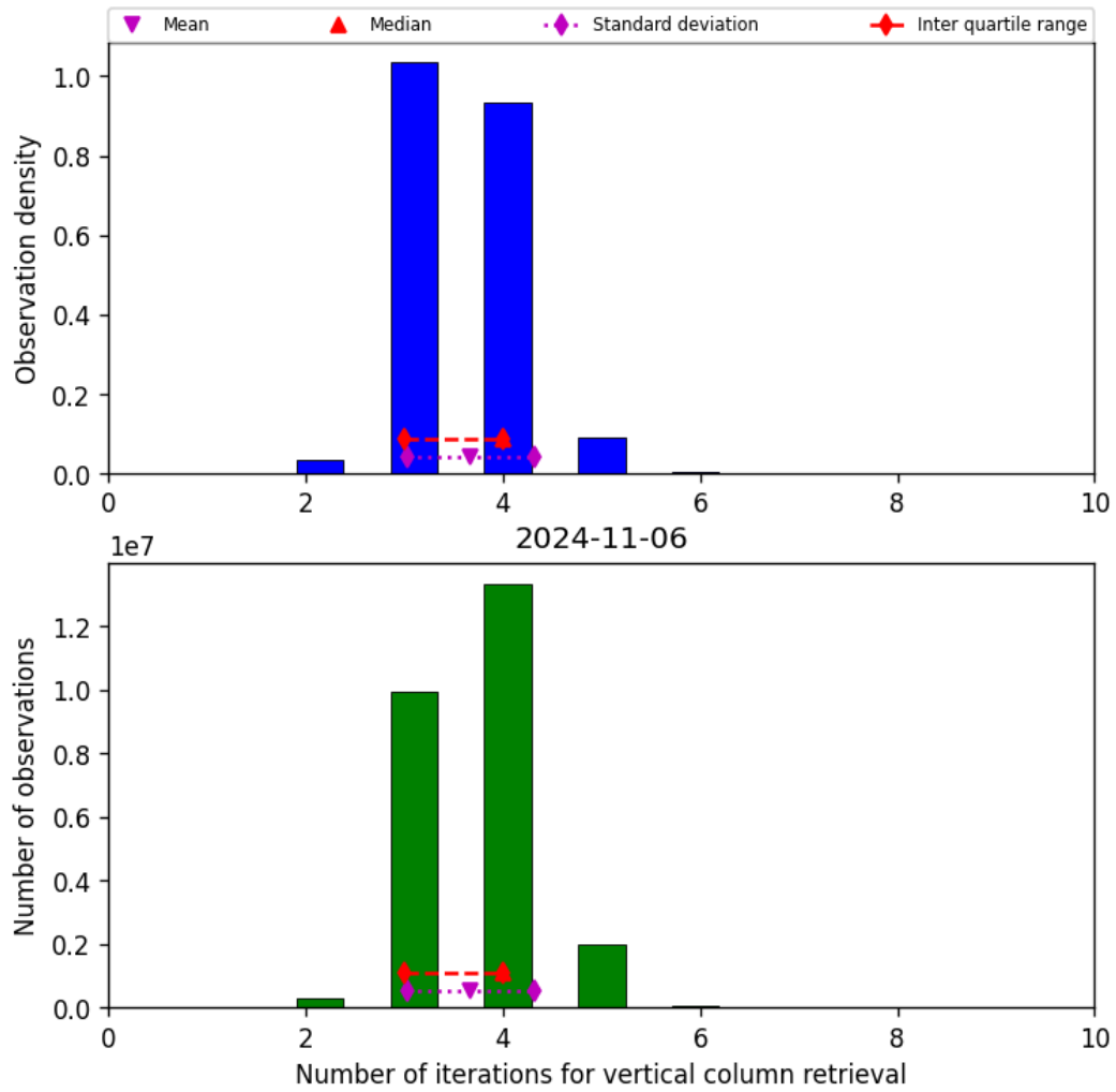
Figure 26: Histogram of “Number of iterations for vertical column retrieval” for 2024-11-05 to 2024-11-07
