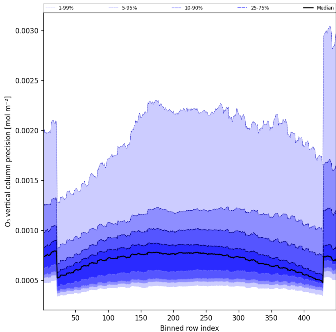
Figure 29: Along track statistics of “O 3 vertical column precision” for 2024-11-05 to 2024-11-07
