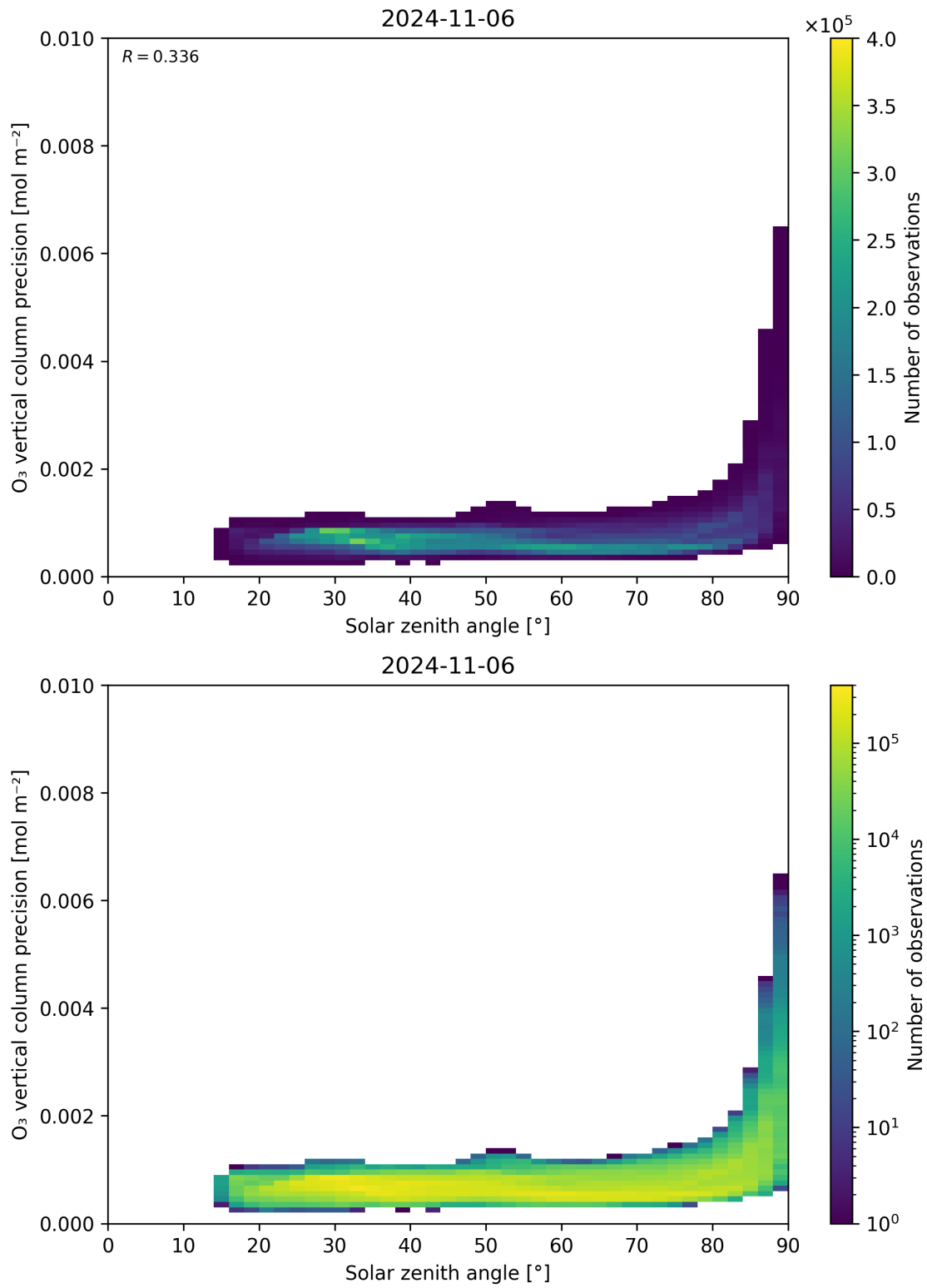
Figure 48: Scatter density plot of “Solar zenith angle” against “O 3 vertical column precision” for 2024-11-05 to 2024-11-07.
