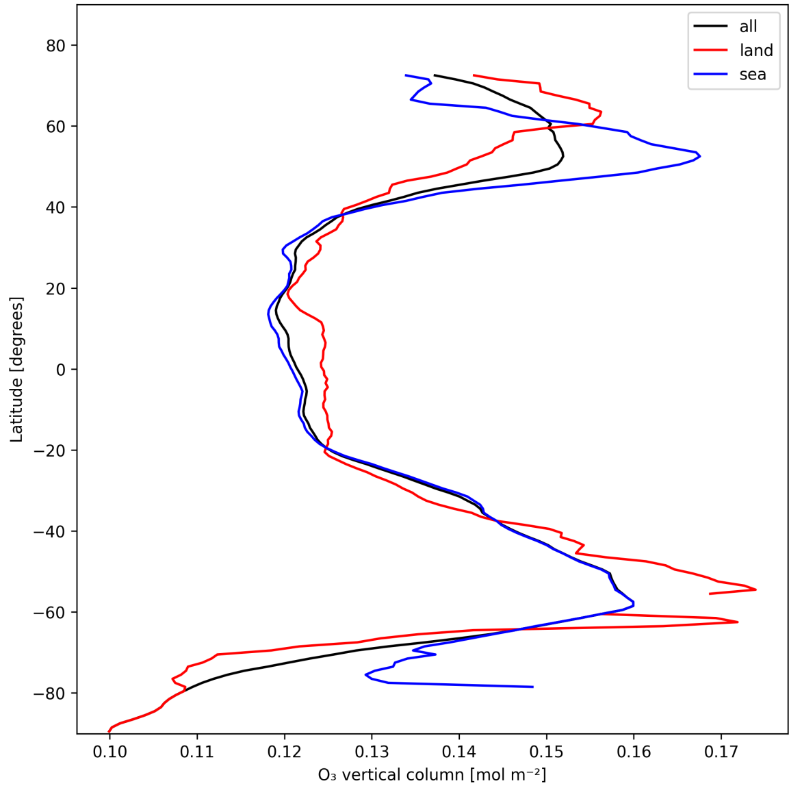
Figure 14: Zonal average of “O 3 vertical column” for 2024-11-05 to 2024-11-07.
