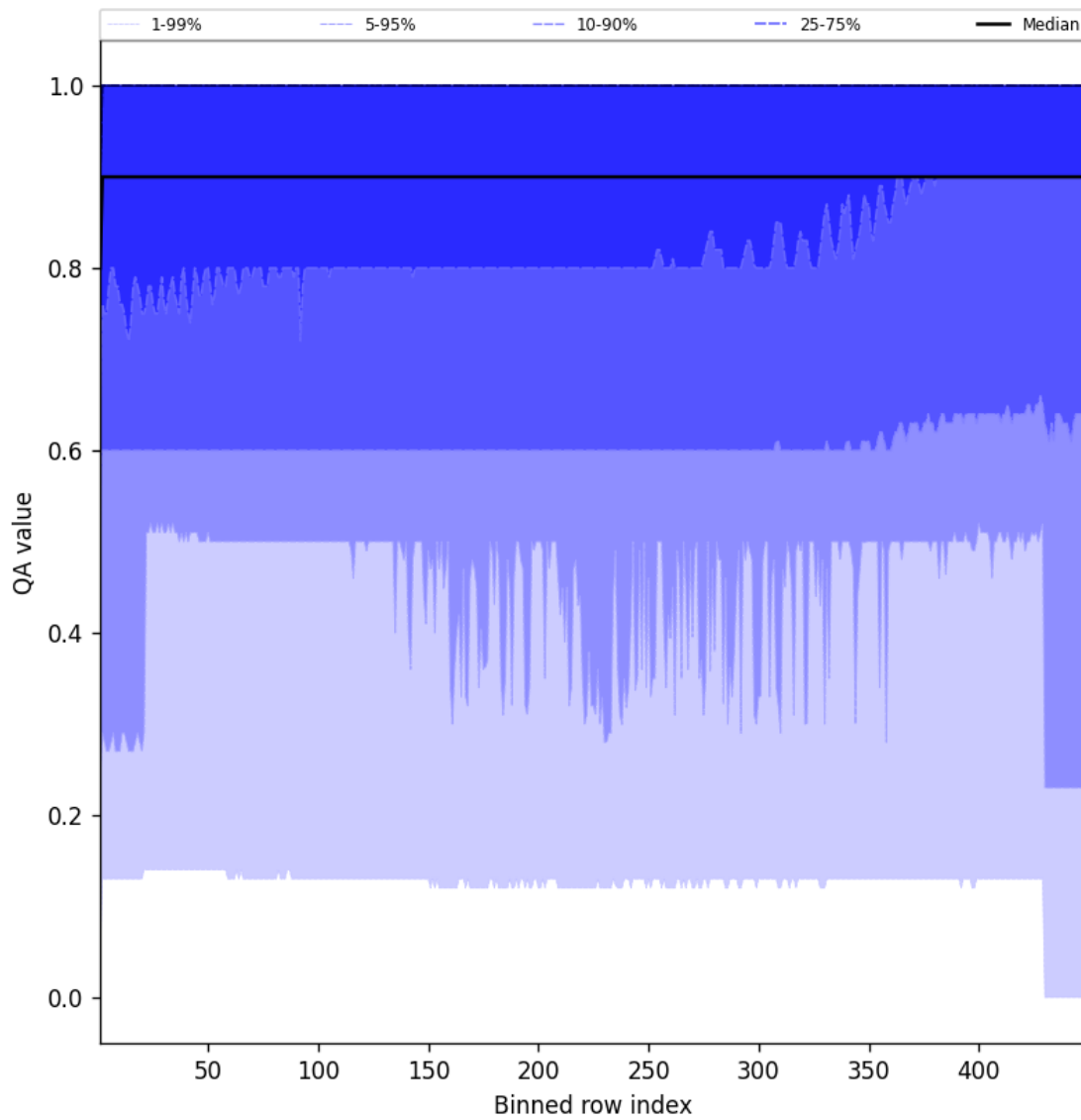
Figure 27: Along track statistics of “QA value” for 2024-11-05 to 2024-11-07
