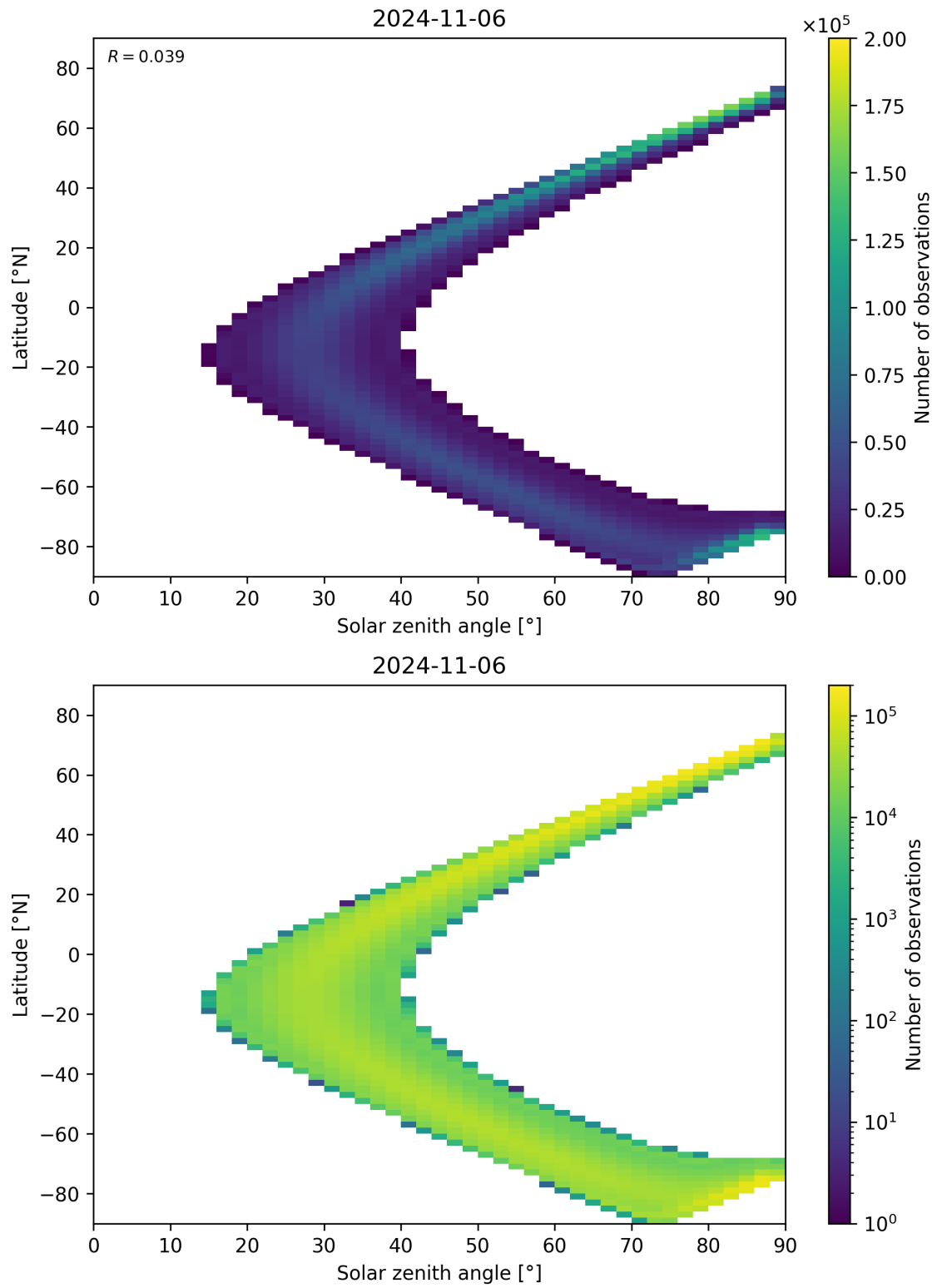
Figure 44: Scatter density plot of “Solar zenith angle” against “Latitude” for 2024-11-05 to 2024-11-07.
