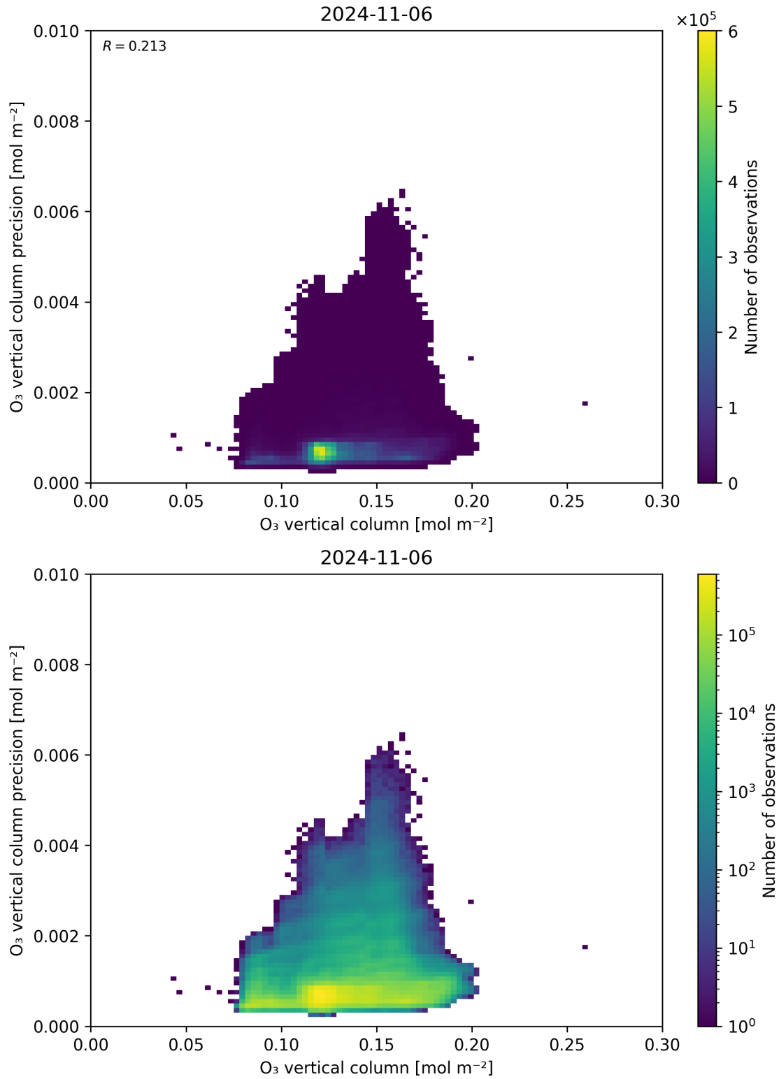
Figure 41: Scatter density plot of “O 3 vertical column” against “O 3 vertical column precision” for 2024-11-05 to 2024-11-07.
