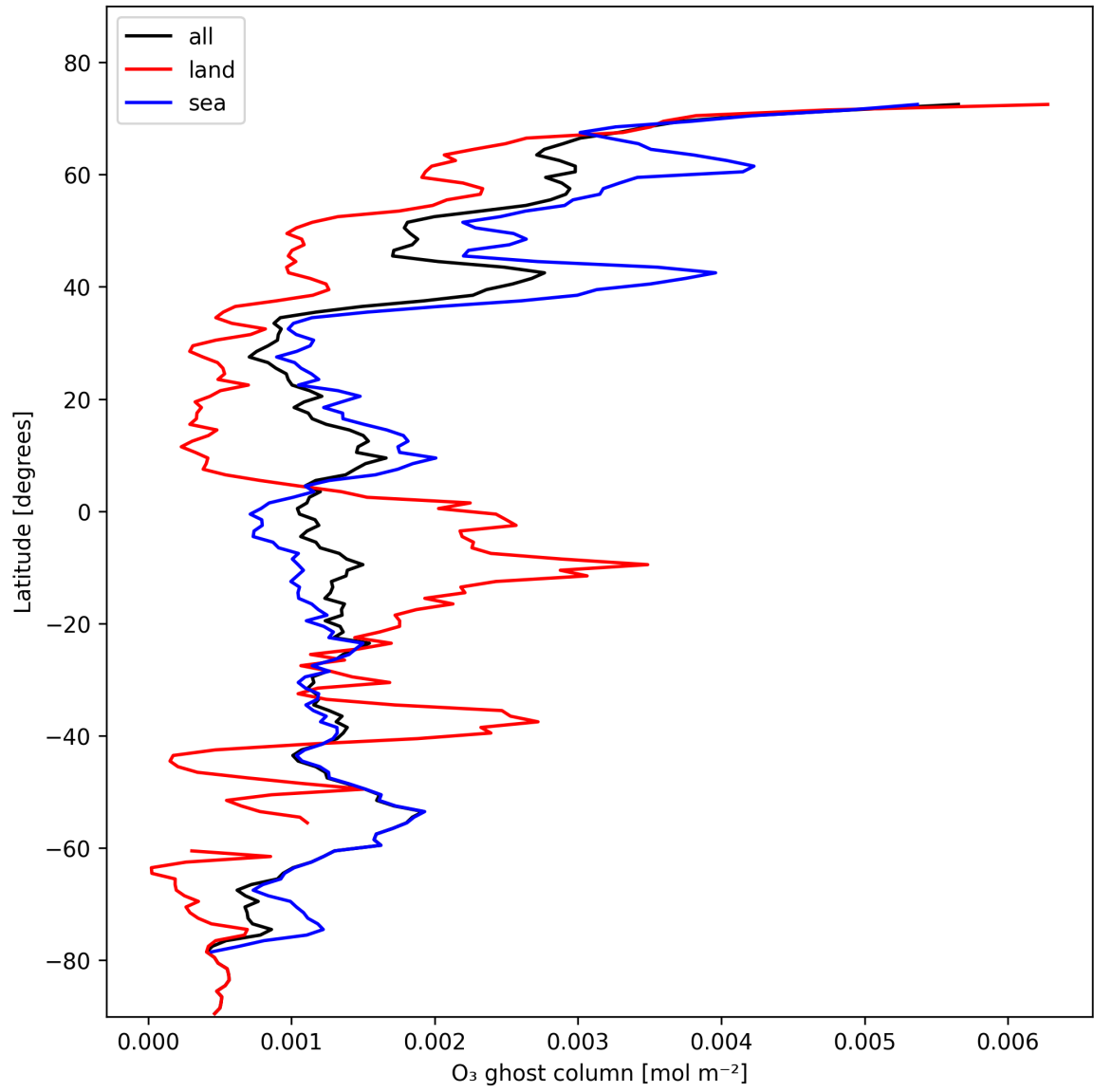
Figure 18: Zonal average of "O 3 ghost column" for 2024-11-05 to 2024-11-07.
