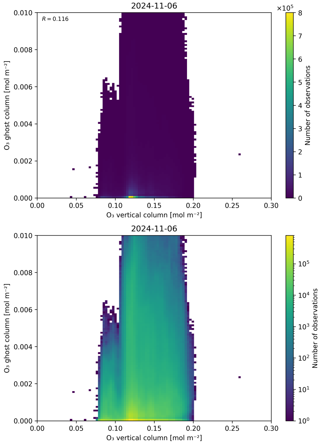
Figure 40: Scatter density plot of “O 3 vertical column” against “O 3 ghost column” for 2024-11-05 to 2024-11-07.
