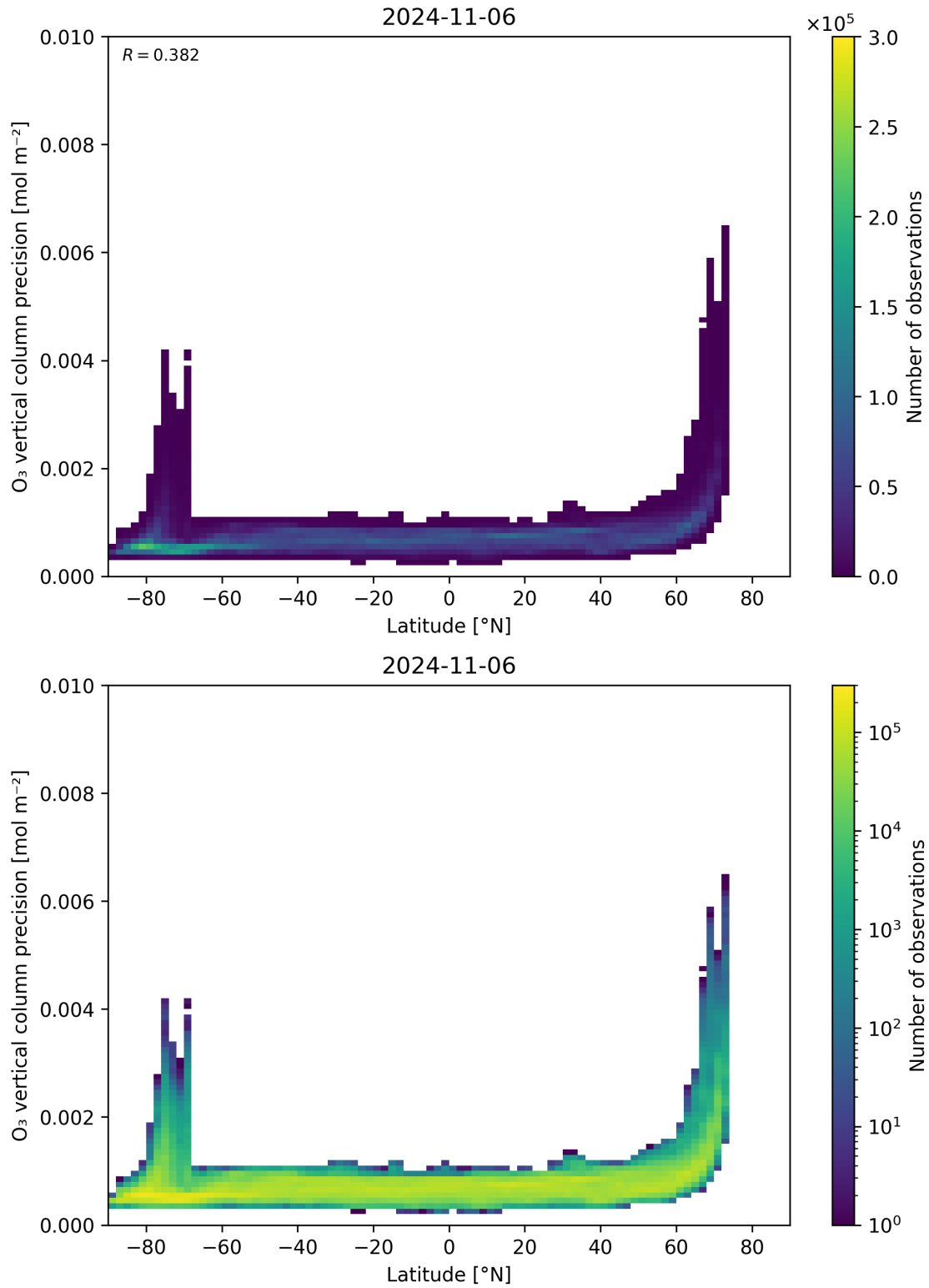
Figure 37: Scatter density plot of “Latitude” against “O 3 vertical column precision” for 2024-11-05 to 2024-11-07.
