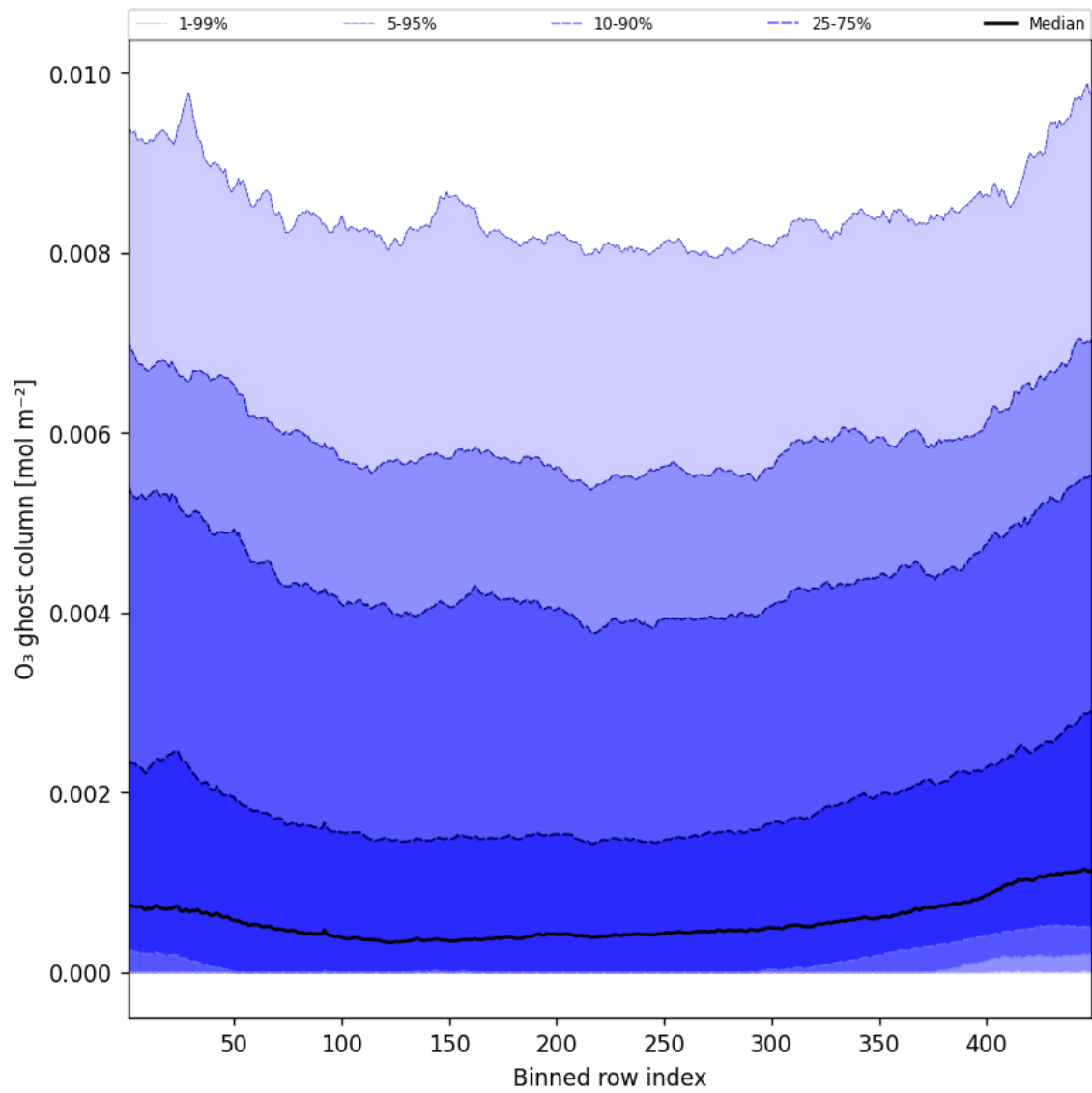
Figure 32: Along track statistics of “O 3 ghost column” for 2024-11-05 to 2024-11-07
