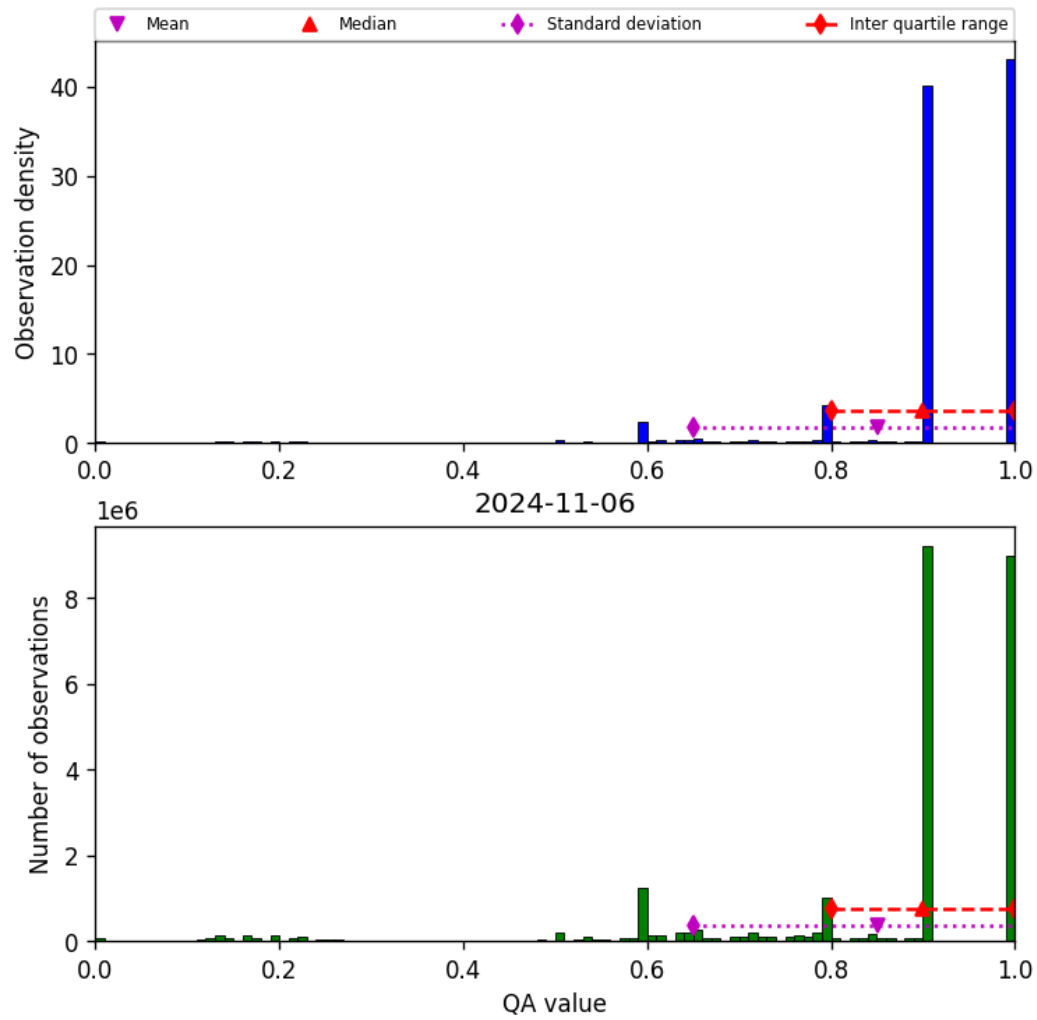
Figure 20: Histogram of “QA value” for 2024-11-05 to 2024-11-07
