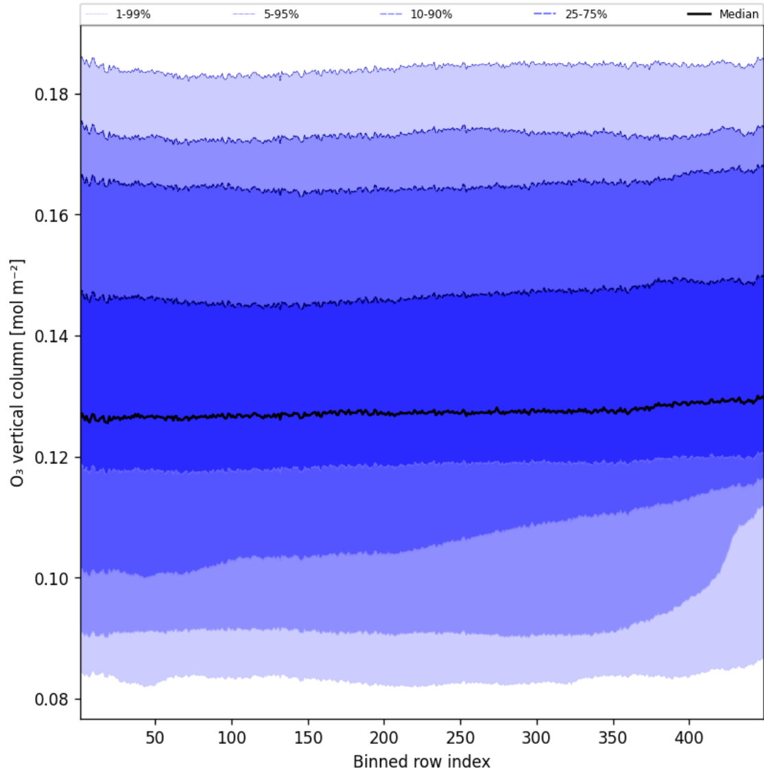
Figure 28: Along track statistics of “O 3 vertical column” for 2024-11-05 to 2024-11-07
