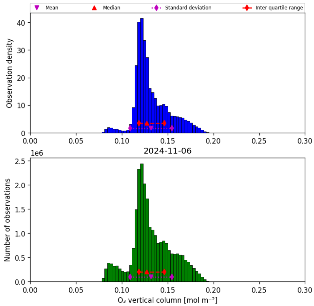
Figure 21: Histogram of “O 3 vertical column” for 2024-11-05 to 2024-11-07
