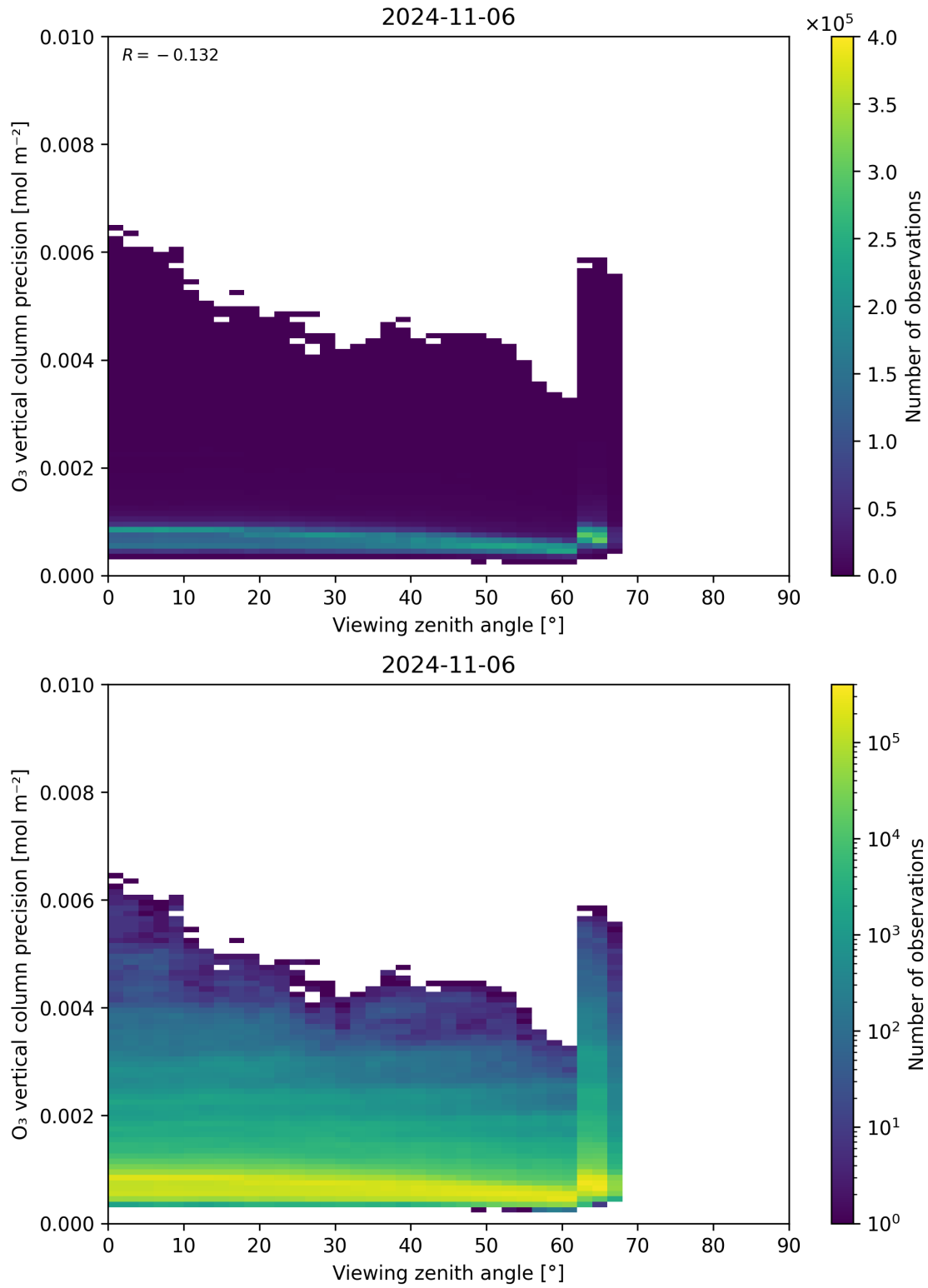
Figure 53: Scatter density plot of “Viewing zenith angle” against “O 3 vertical column precision” for 2024-11-05 to 2024-11-07.
