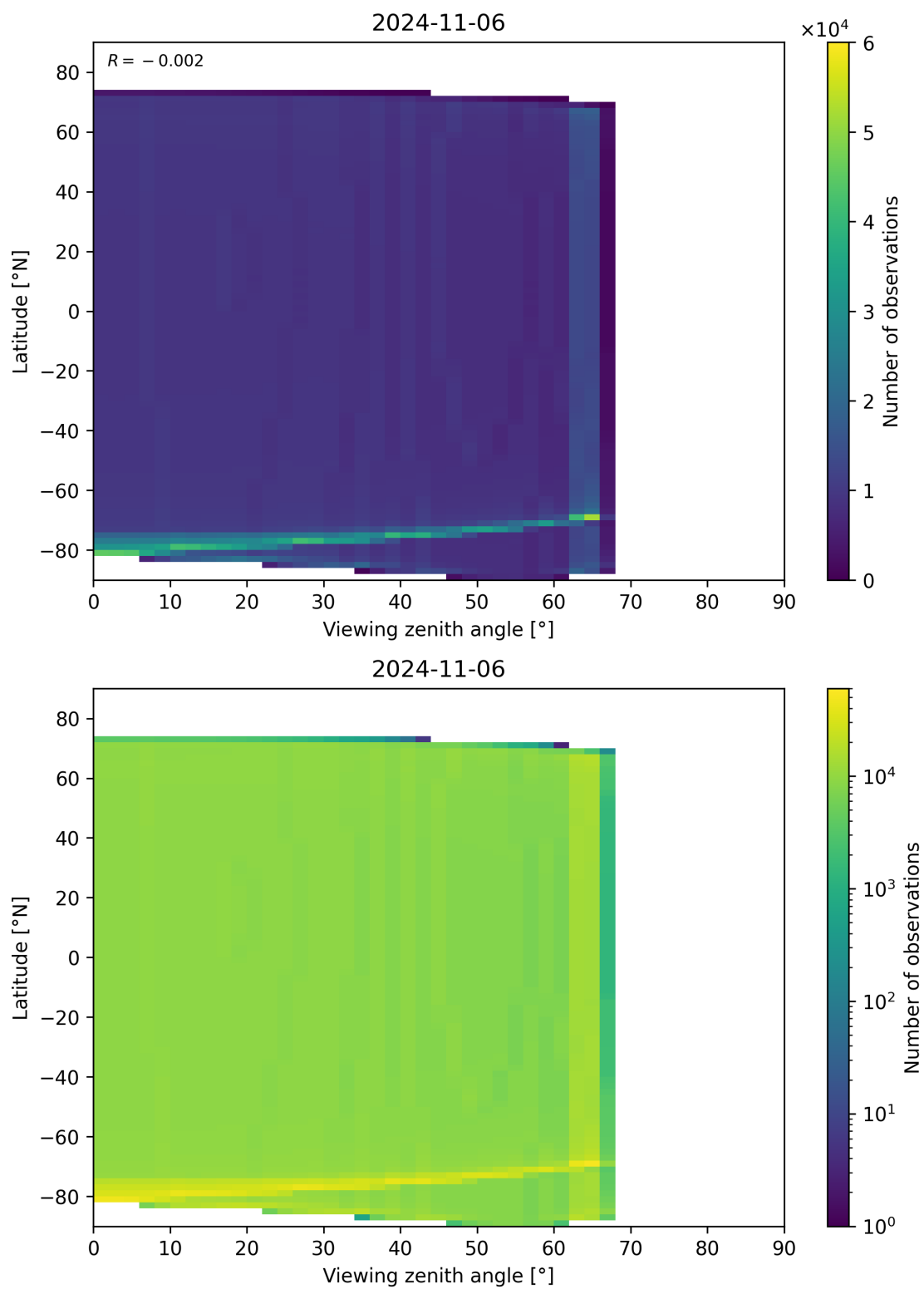
Figure 49: Scatter density plot of “Viewing zenith angle” against “Latitude” for 2024-11-05 to 2024-11-07.
