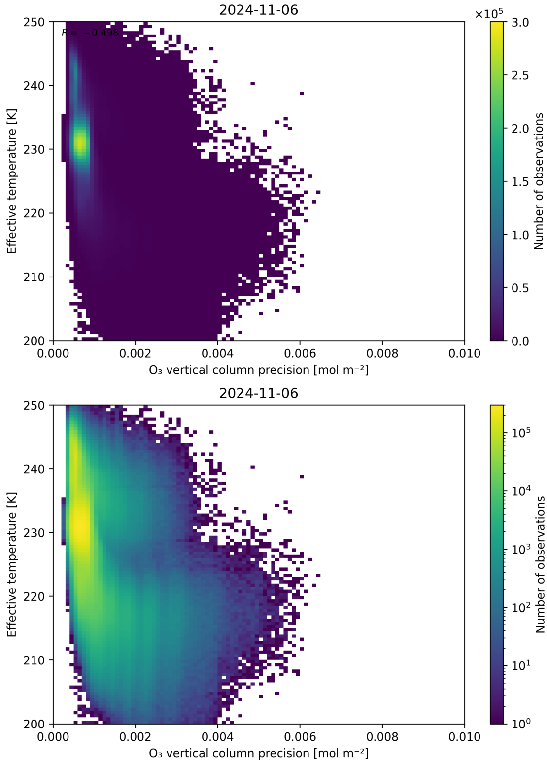
Figure 42: Scatter density plot of “O 3 vertical column precision” against “Effective temperature” for 2024-11-05 to 2024-11-07.
