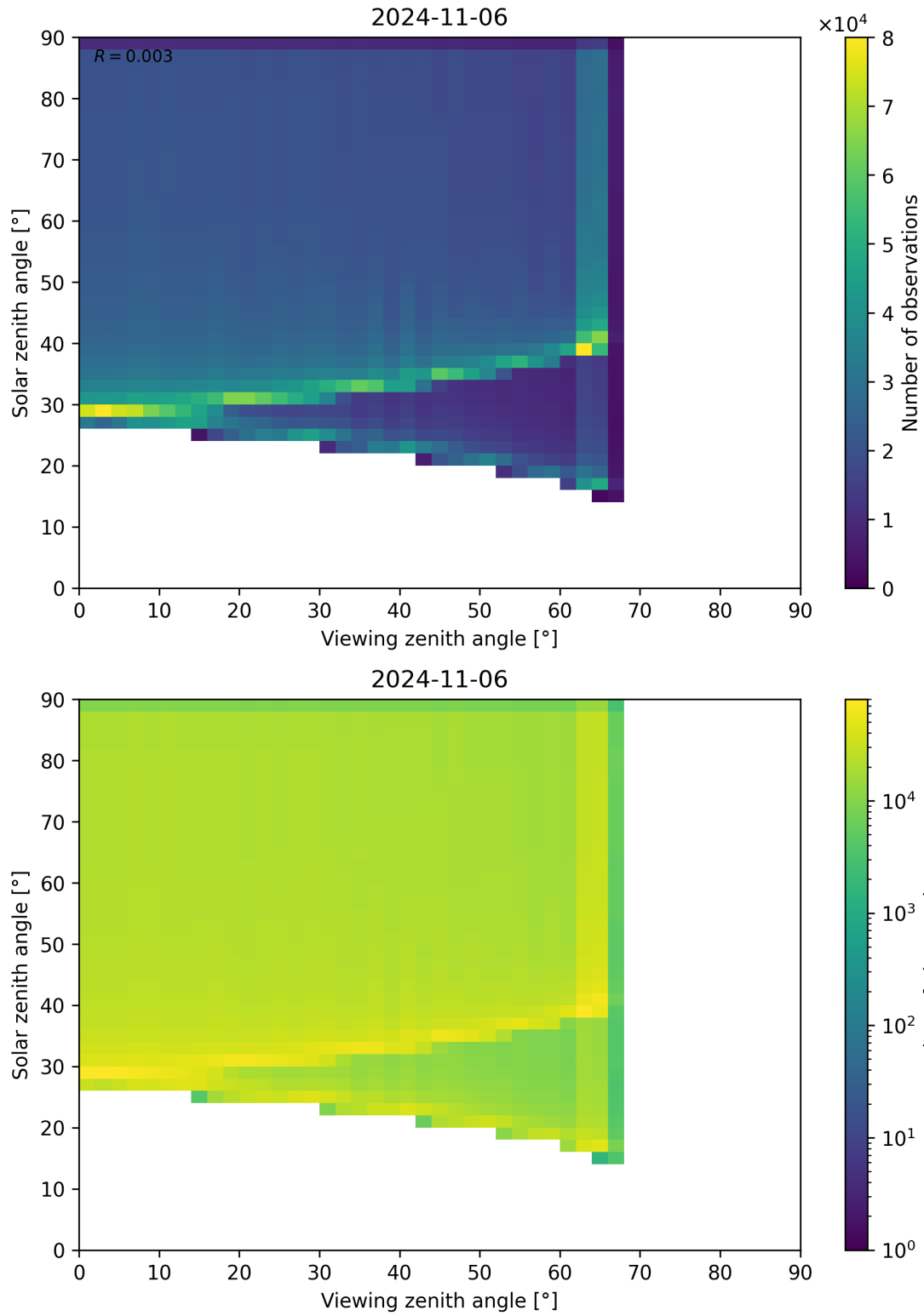
Figure 54: Scatter density plot of “Viewing zenith angle” against “Solar zenith angle” for 2024-11-05 to 2024-11-07.
