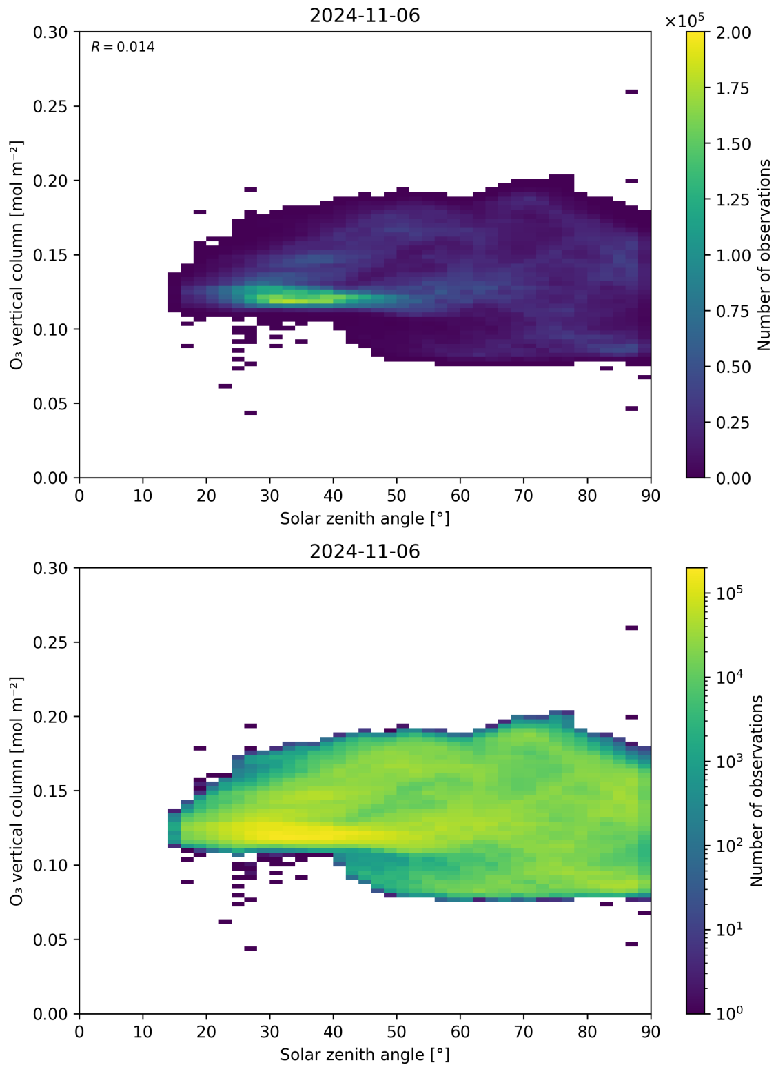
Figure 47: Scatter density plot of “Solar zenith angle” against “O 3 vertical column” for 2024-11-05 to 2024-11-07.
