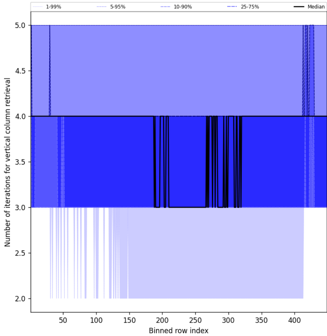
Figure 33: Along track statistics of “Number of iterations for vertical column retrieval” for 2024-11-05 to 2024-11-07
