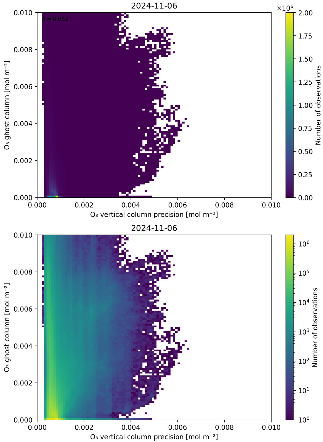
Figure 43: Scatter density plot of “O 3 vertical column precision” against “O 3 ghost column” for 2024-11-05 to 2024-11-07.
