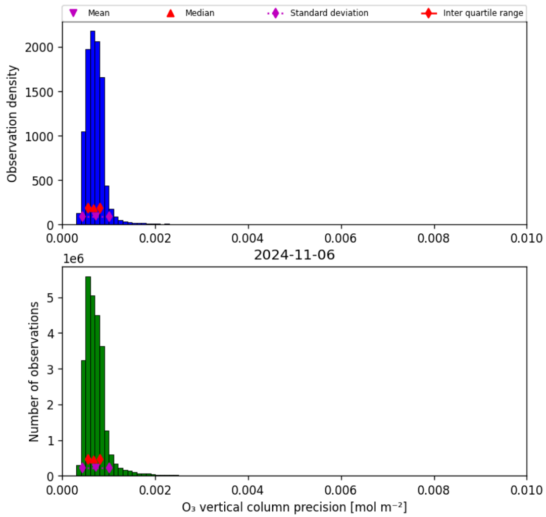
Figure 22: Histogram of “O 3 vertical column precision” for 2024-11-05 to 2024-11-07
