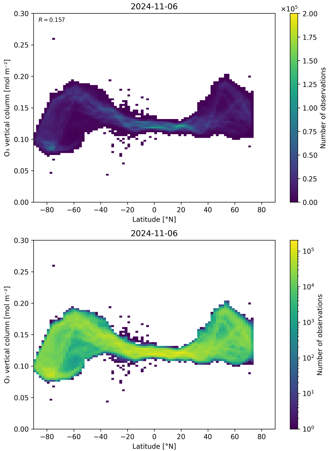
Figure 36: Scatter density plot of “Latitude” against “O 3 vertical column” for 2024-11-05 to 2024-11-07.
