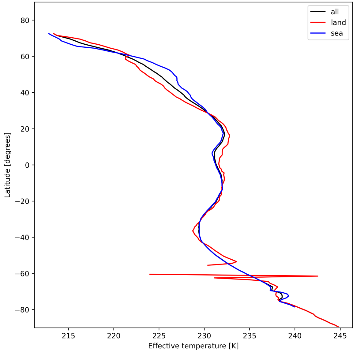
Figure 17: Zonal average of “Effective temperature” for 2024-11-05 to 2024-11-07.
