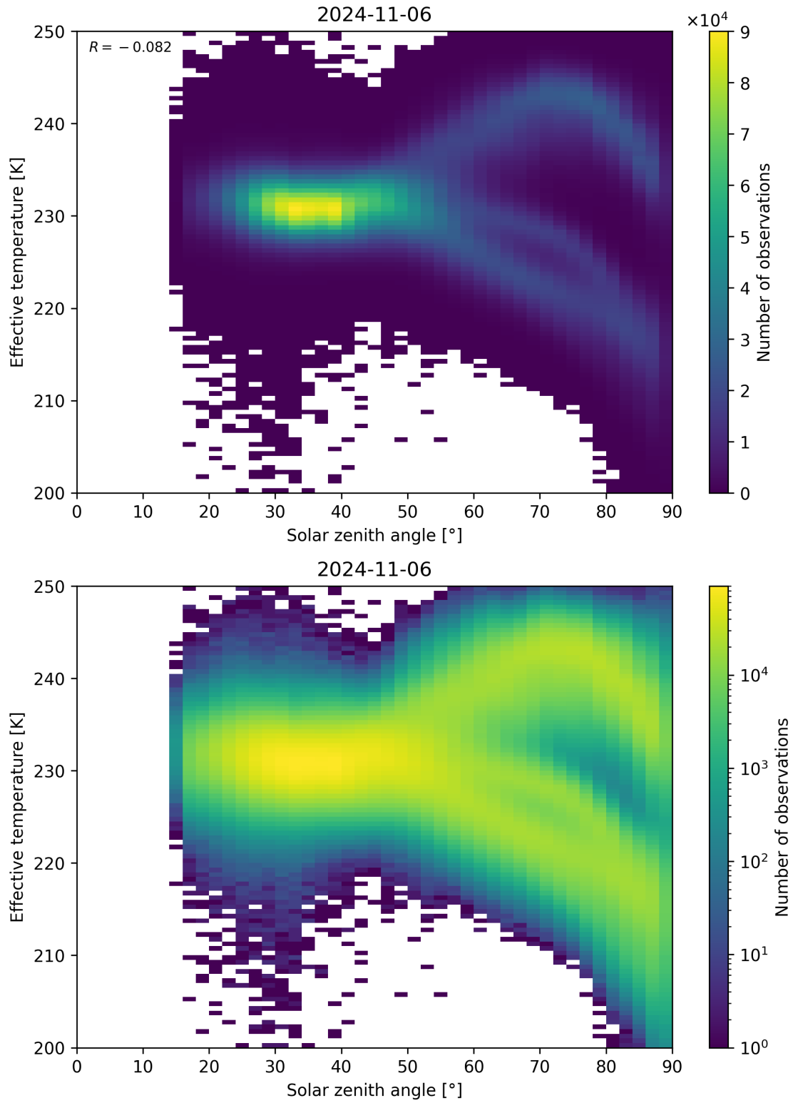
Figure 45: Scatter density plot of “Solar zenith angle” against “Effective temperature” for 2024-11-05 to 2024-11-07.
