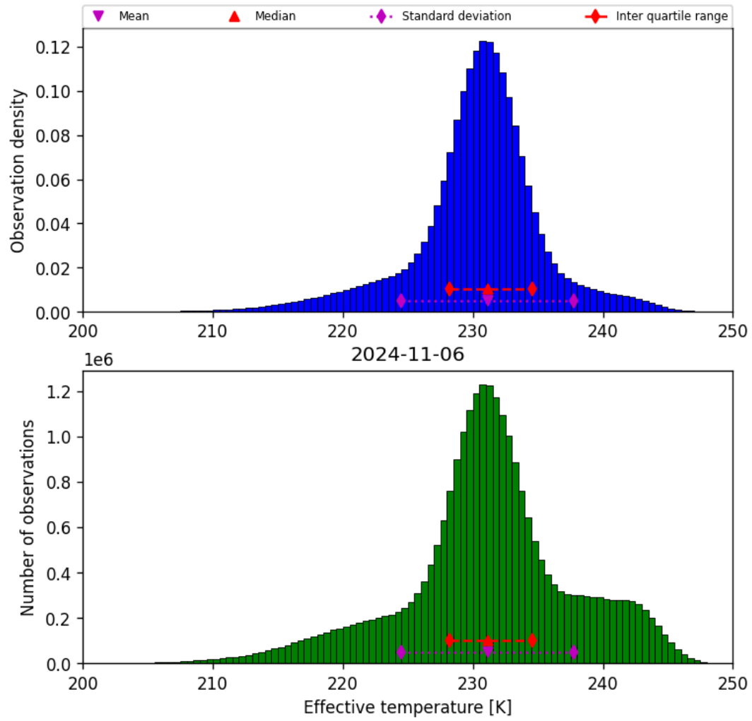
Figure 24: Histogram of “Effective temperature” for 2024-11-05 to 2024-11-07
