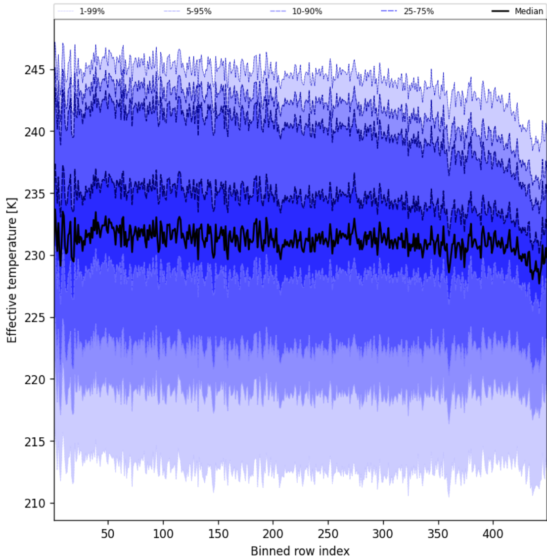
Figure 31: Along track statistics of “Effective temperature” for 2024-11-05 to 2024-11-07
