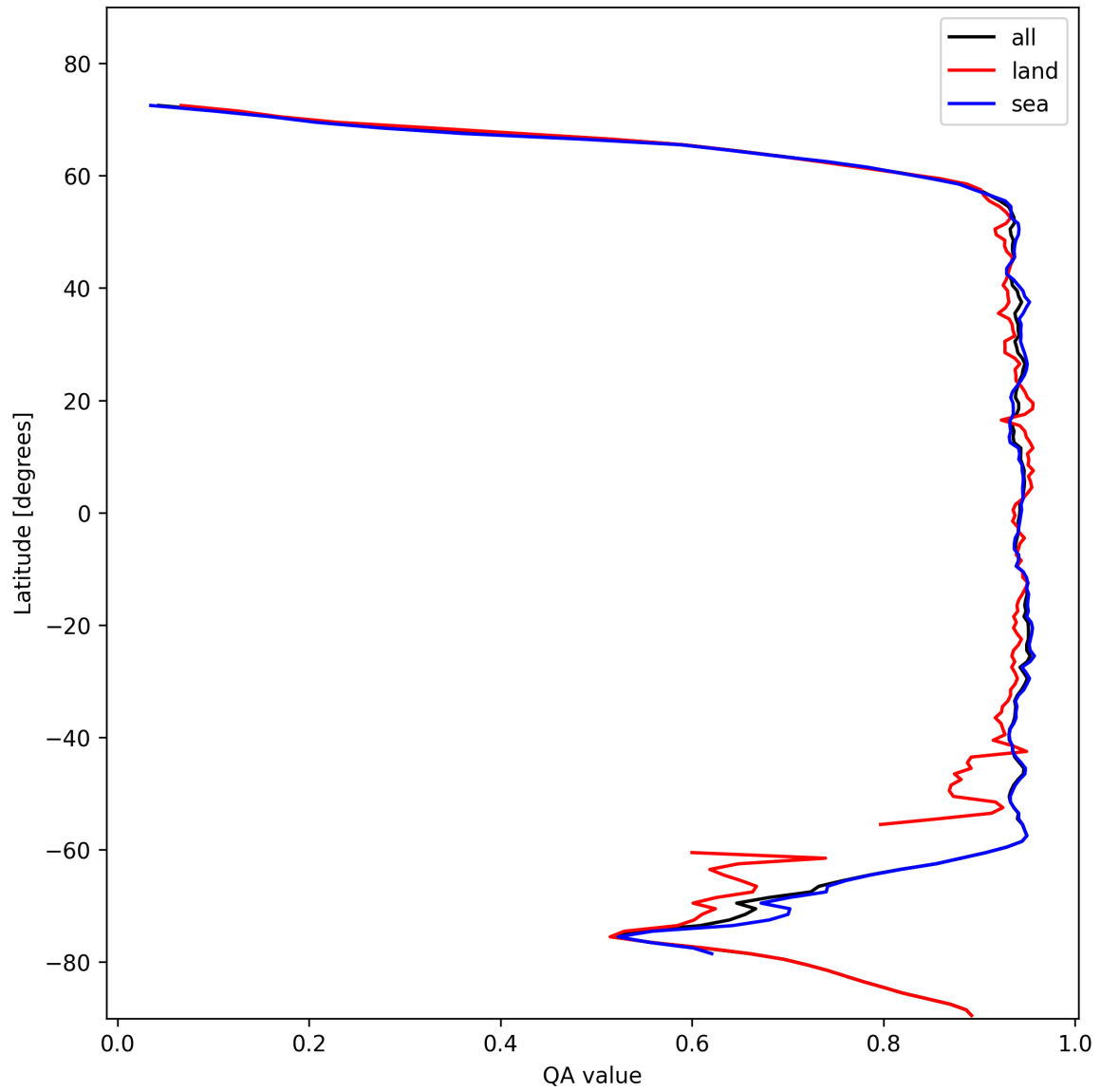
Figure 13: Zonal average of “QA value” for 2024-11-05 to 2024-11-07.
