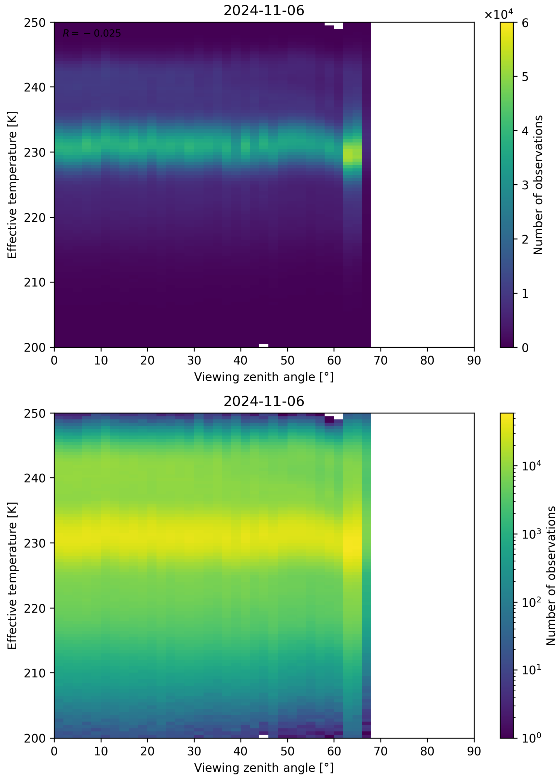
Figure 50: Scatter density plot of “Viewing zenith angle” against “Effective temperature” for 2024-11-05 to 2024-11-07.
