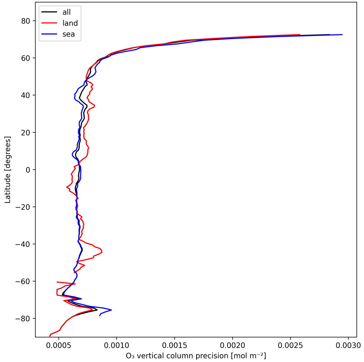
Figure 15: Zonal average of “O 3 vertical column precision” for 2024-11-05 to 2024-11-07.
