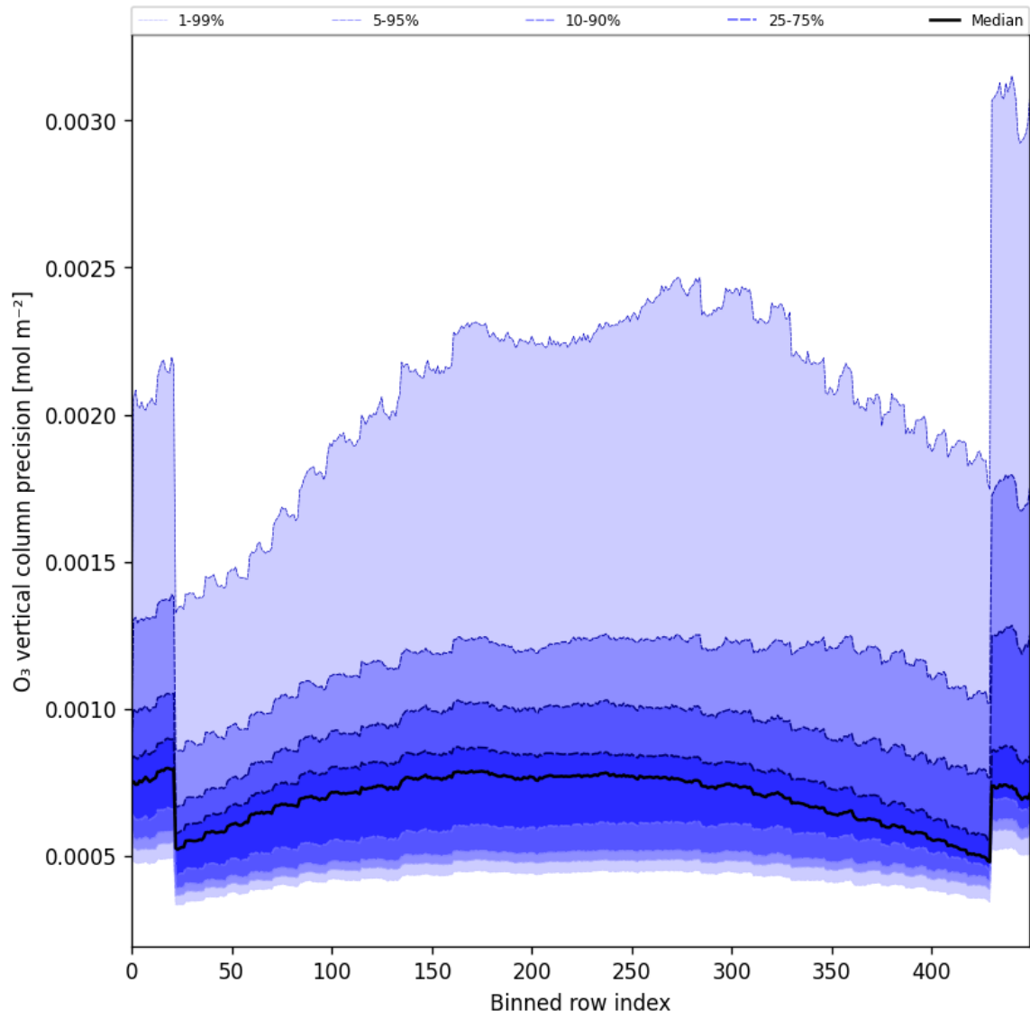
Figure 29: Along track statistics of “O 3 vertical column precision” for 2024-11-07 to 2024-11-09
