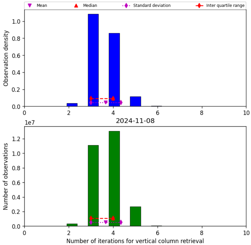
Figure 26: Histogram of “Number of iterations for vertical column retrieval” for 2024-11-07 to 2024-11-09
