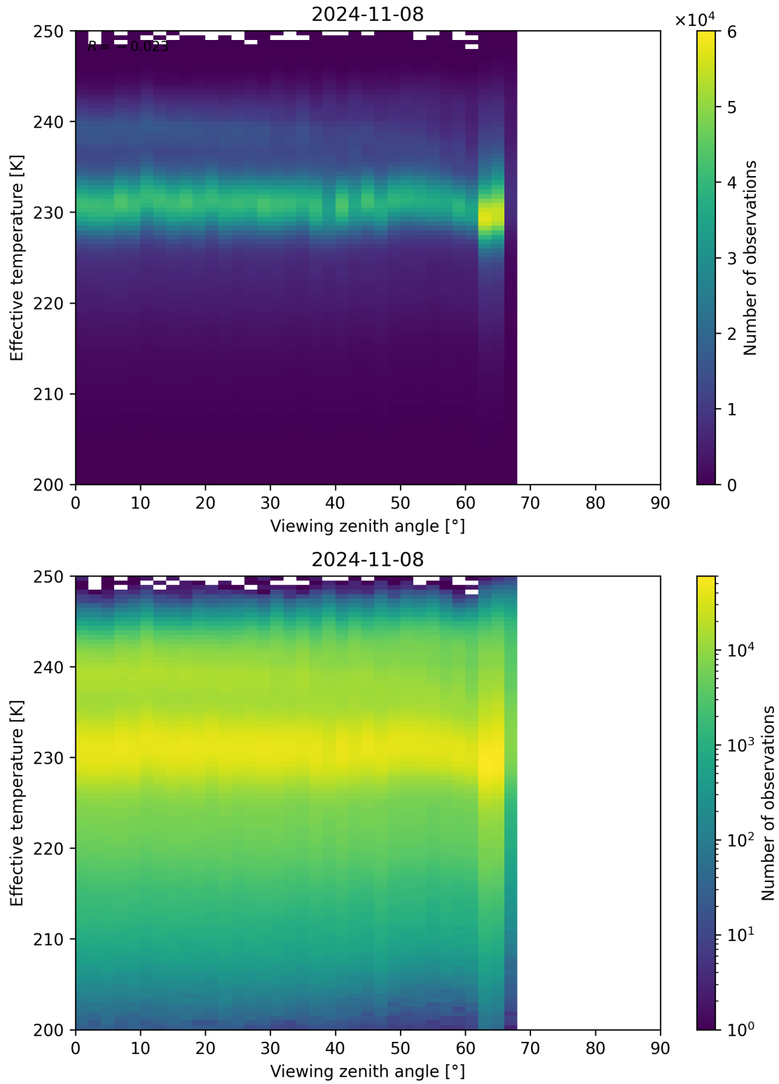
Figure 50: Scatter density plot of “Viewing zenith angle” against “Effective temperature” for 2024-11-07 to 2024-11-09.
