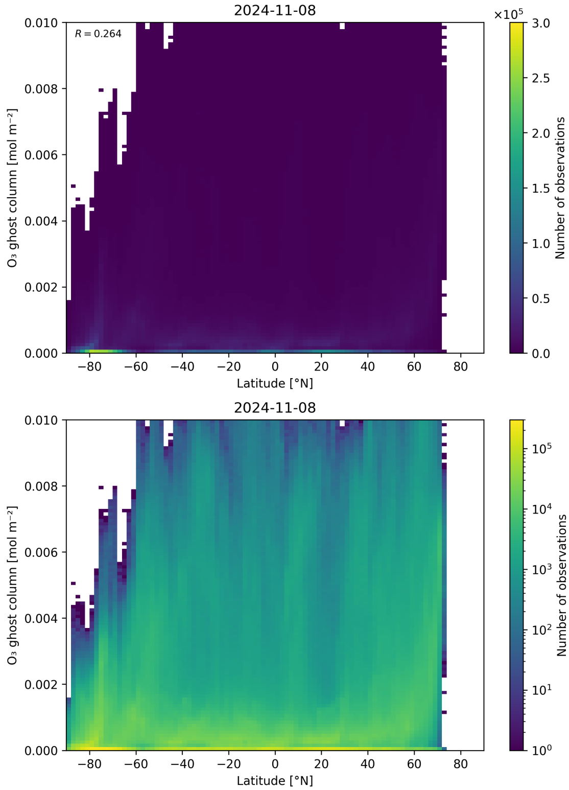
Figure 35: Scatter density plot of “Latitude” against “O 3 ghost column” for 2024-11-07 to 2024-11-09.
