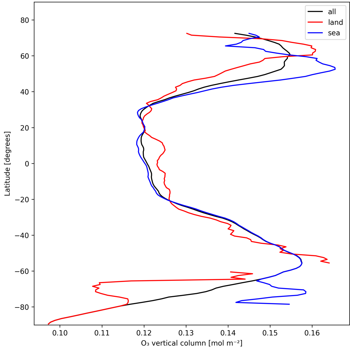
Figure 14: Zonal average of “O 3 vertical column” for 2024-11-07 to 2024-11-09.
