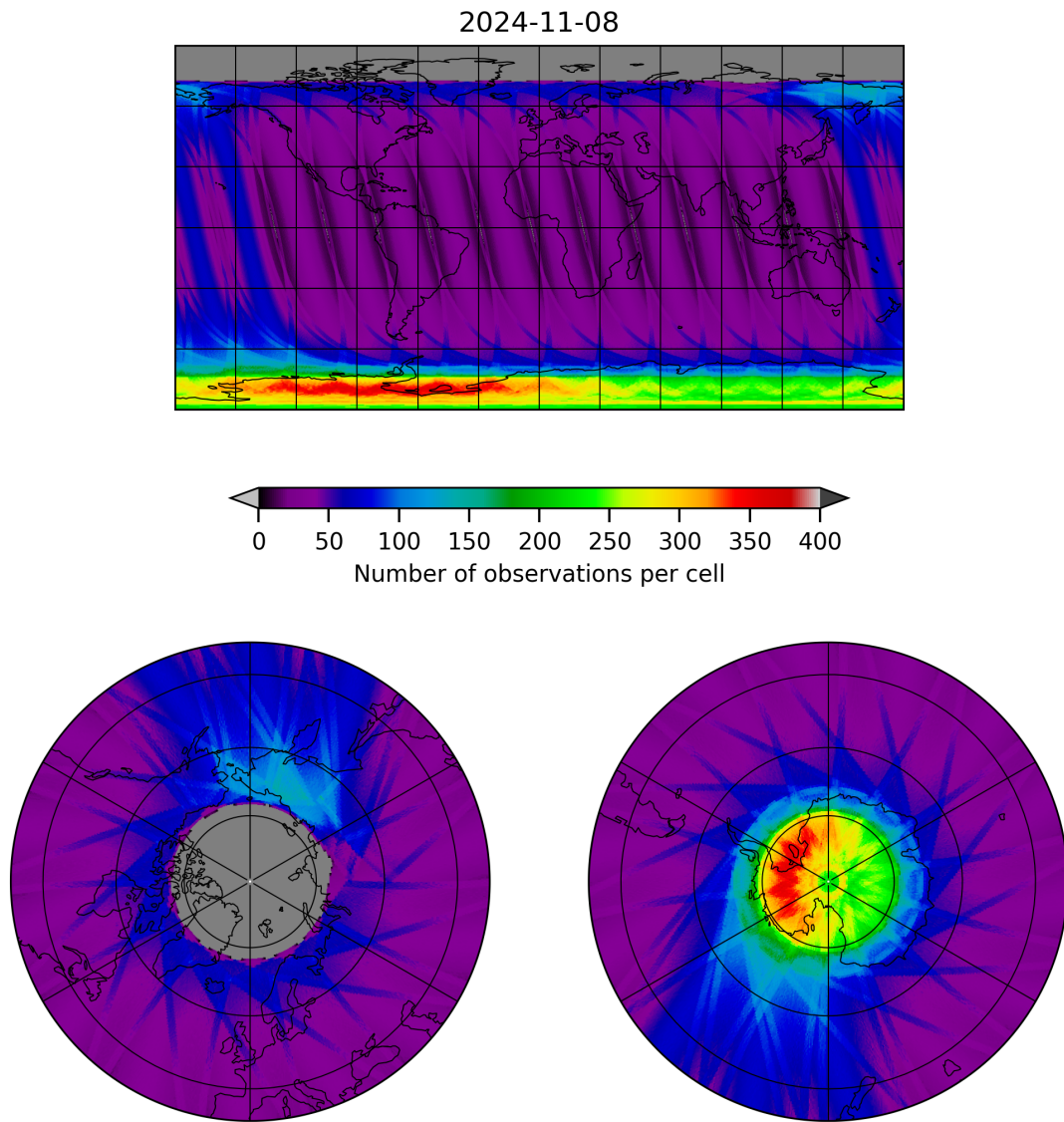
Figure 12: Map of the number of observations for 2024-11-07 to 2024-11-09
