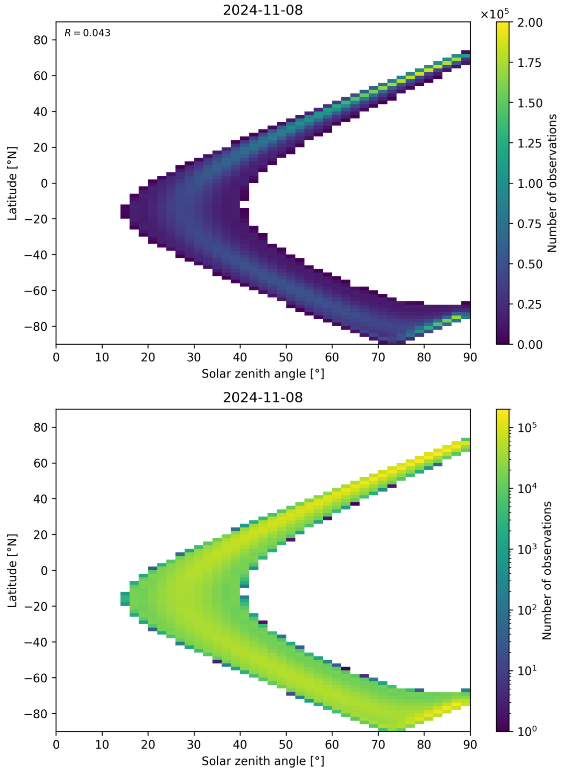
Figure 44: Scatter density plot of “Solar zenith angle” against “Latitude” for 2024-11-07 to 2024-11-09.
