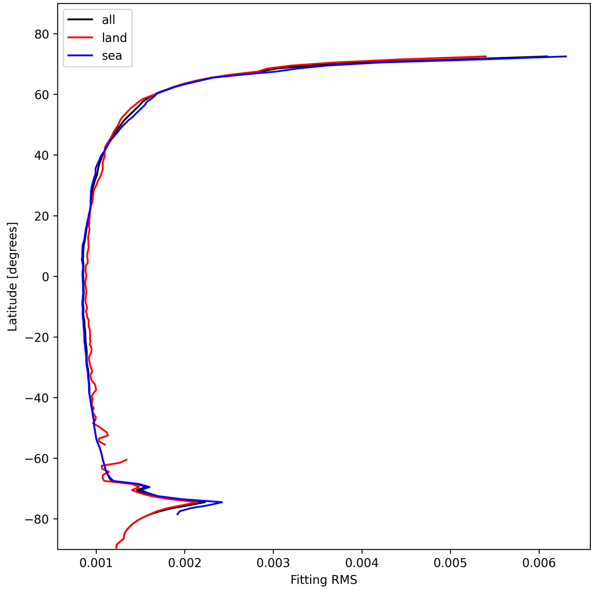
Figure 16: Zonal average of “Fitting RMS” for 2024-11-07 to 2024-11-09.
