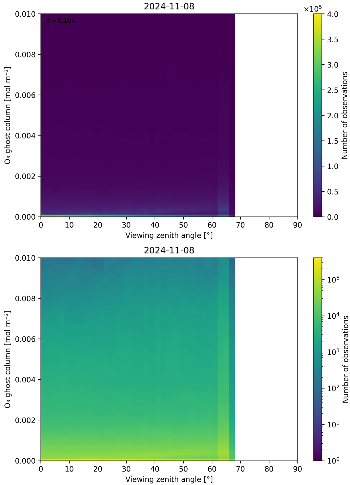
Figure 51: Scatter density plot of “Viewing zenith angle” against “O 3 ghost column” for 2024-11-07 to 2024-11-09.
