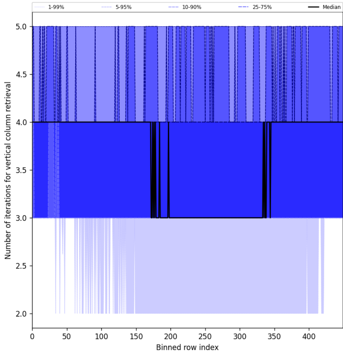
Figure 33: Along track statistics of “Number of iterations for vertical column retrieval” for 2024-11-07 to 2024-11-09
