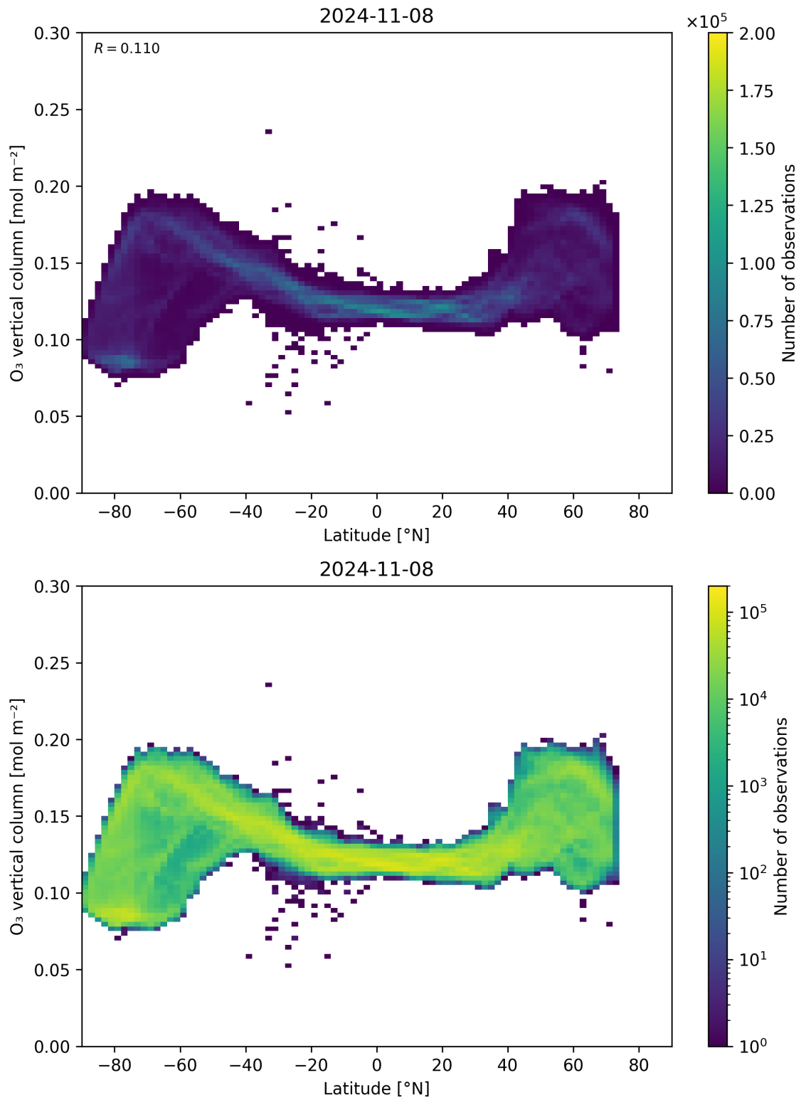
Figure 36: Scatter density plot of “Latitude” against “O 3 vertical column” for 2024-11-07 to 2024-11-09.
