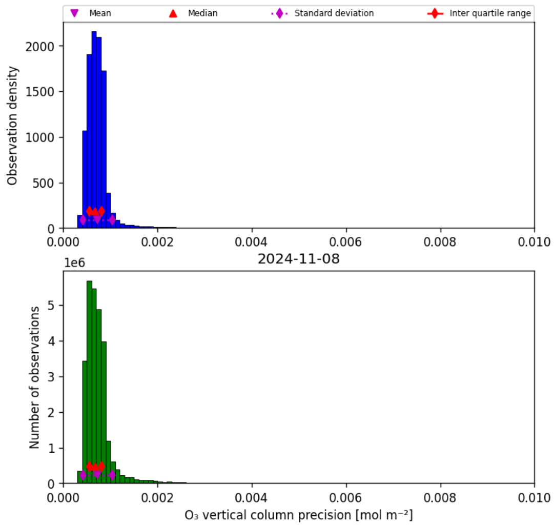
Figure 22: Histogram of “O 3 vertical column precision” for 2024-11-07 to 2024-11-09
