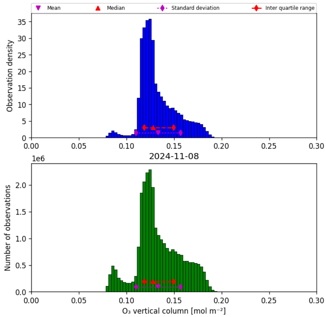
Figure 21: Histogram of “O 3 vertical column” for 2024-11-07 to 2024-11-09
