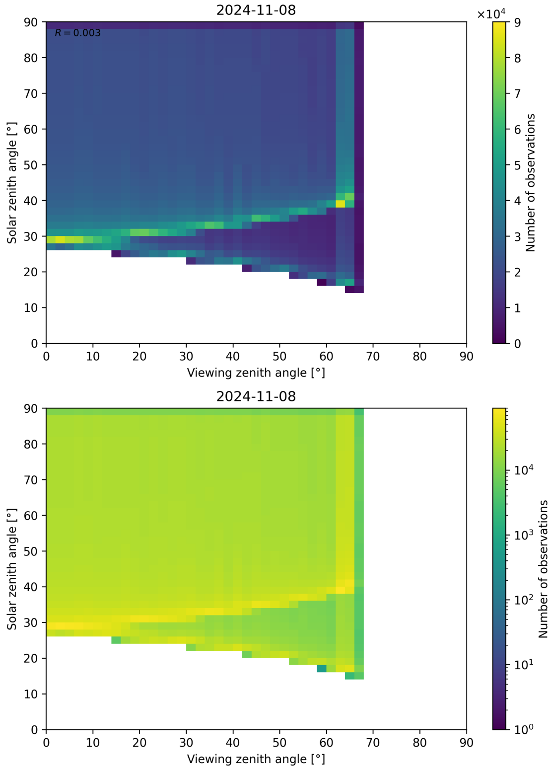
Figure 54: Scatter density plot of “Viewing zenith angle” against “Solar zenith angle” for 2024-11-07 to 2024-11-09.
