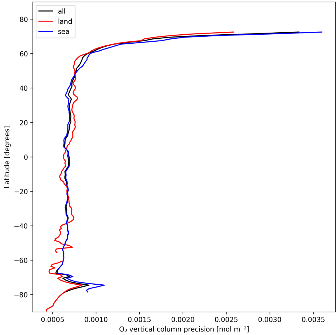
Figure 15: Zonal average of “O 3 vertical column precision” for 2024-11-07 to 2024-11-09.
