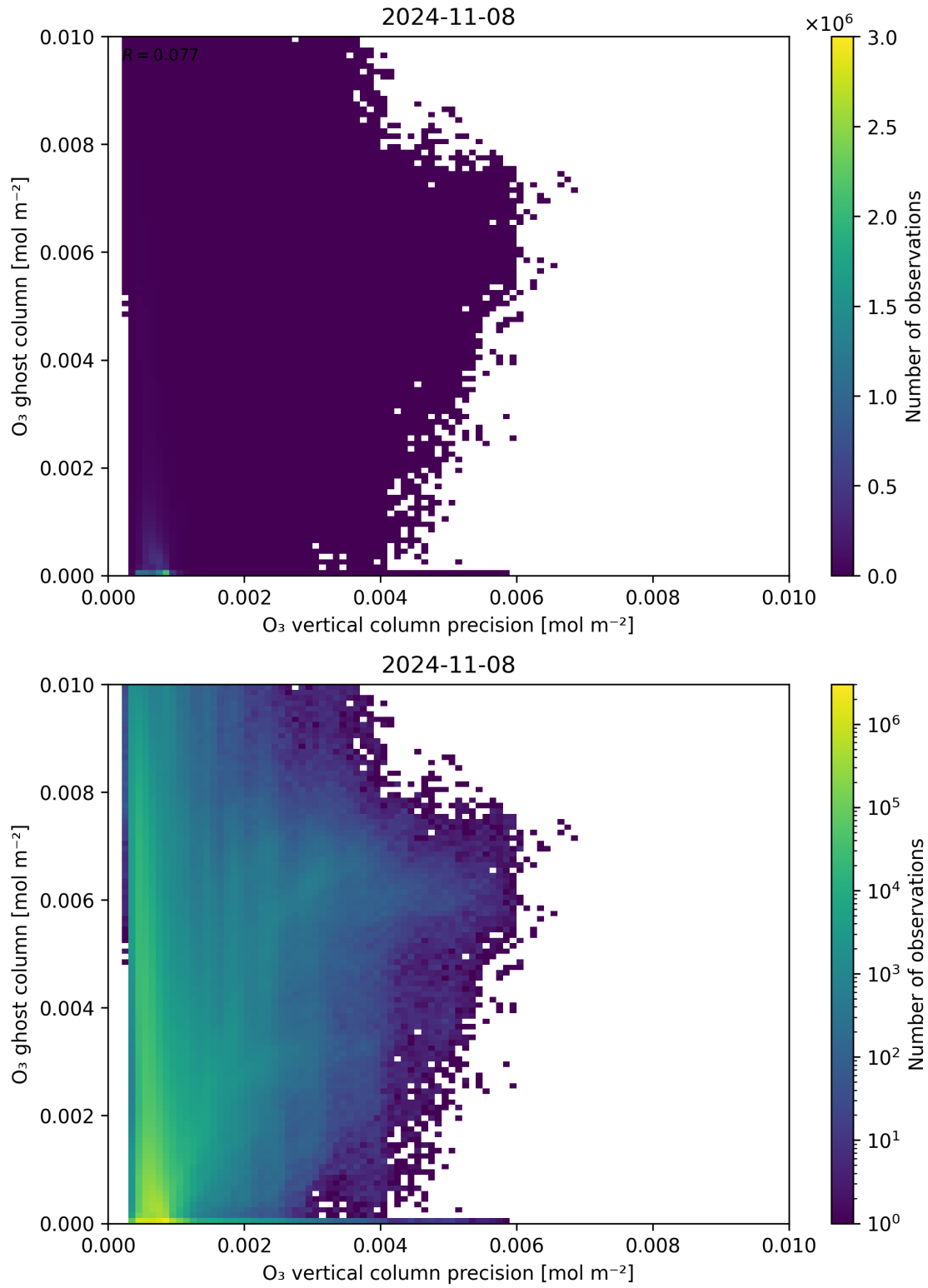
Figure 43: Scatter density plot of “O 3 vertical column precision” against “O 3 ghost column” for 2024-11-07 to 2024-11-09.
