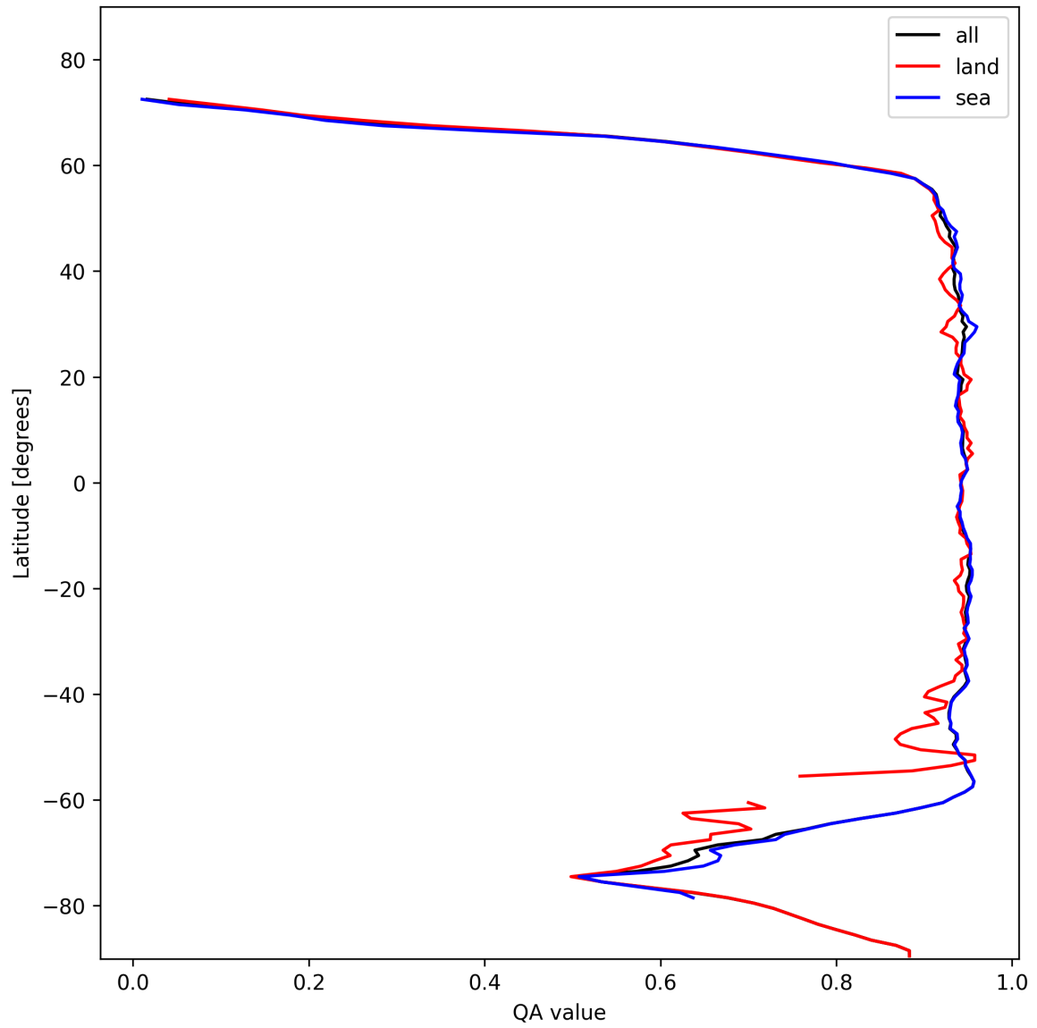
Figure 13: Zonal average of “QA value” for 2024-11-07 to 2024-11-09.
