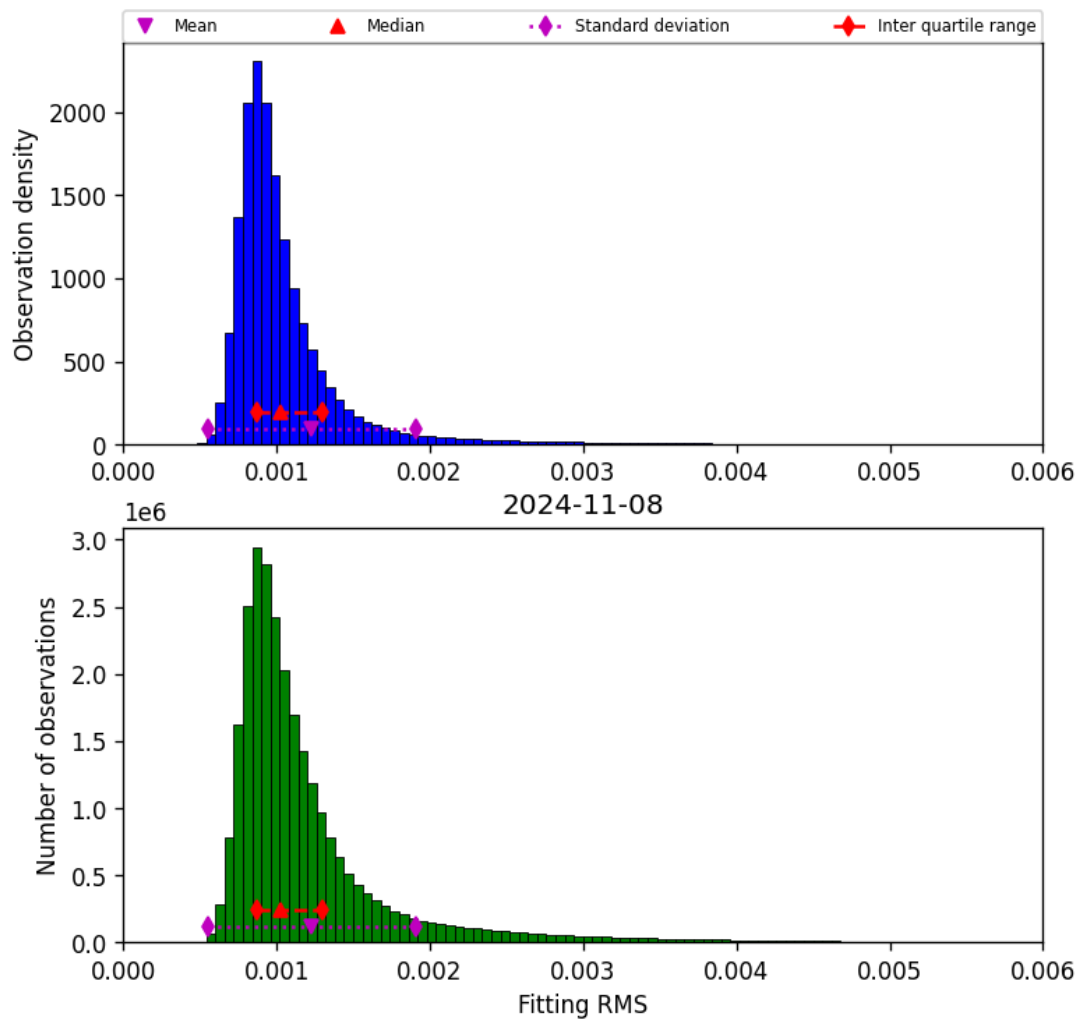
Figure 23: Histogram of “Fitting RMS” for 2024-11-07 to 2024-11-09
