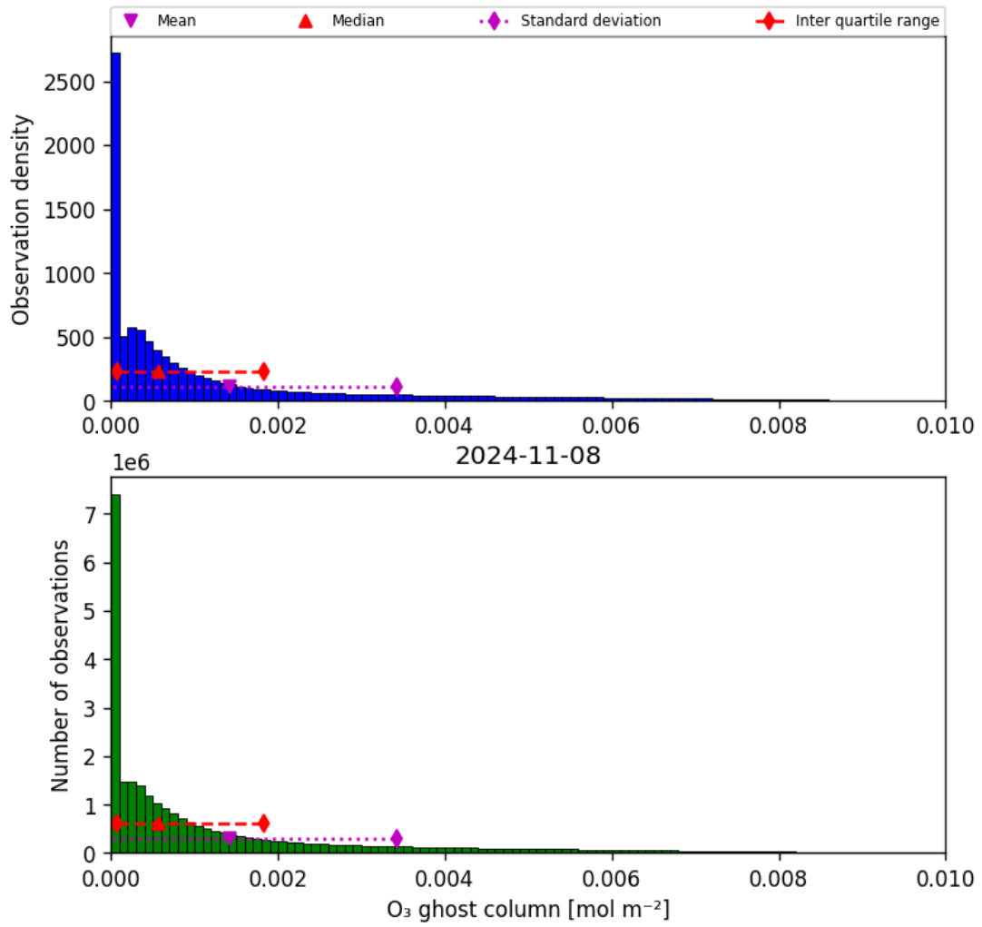
Figure 25: Histogram of “O 3 ghost column” for 2024-11-07 to 2024-11-09
