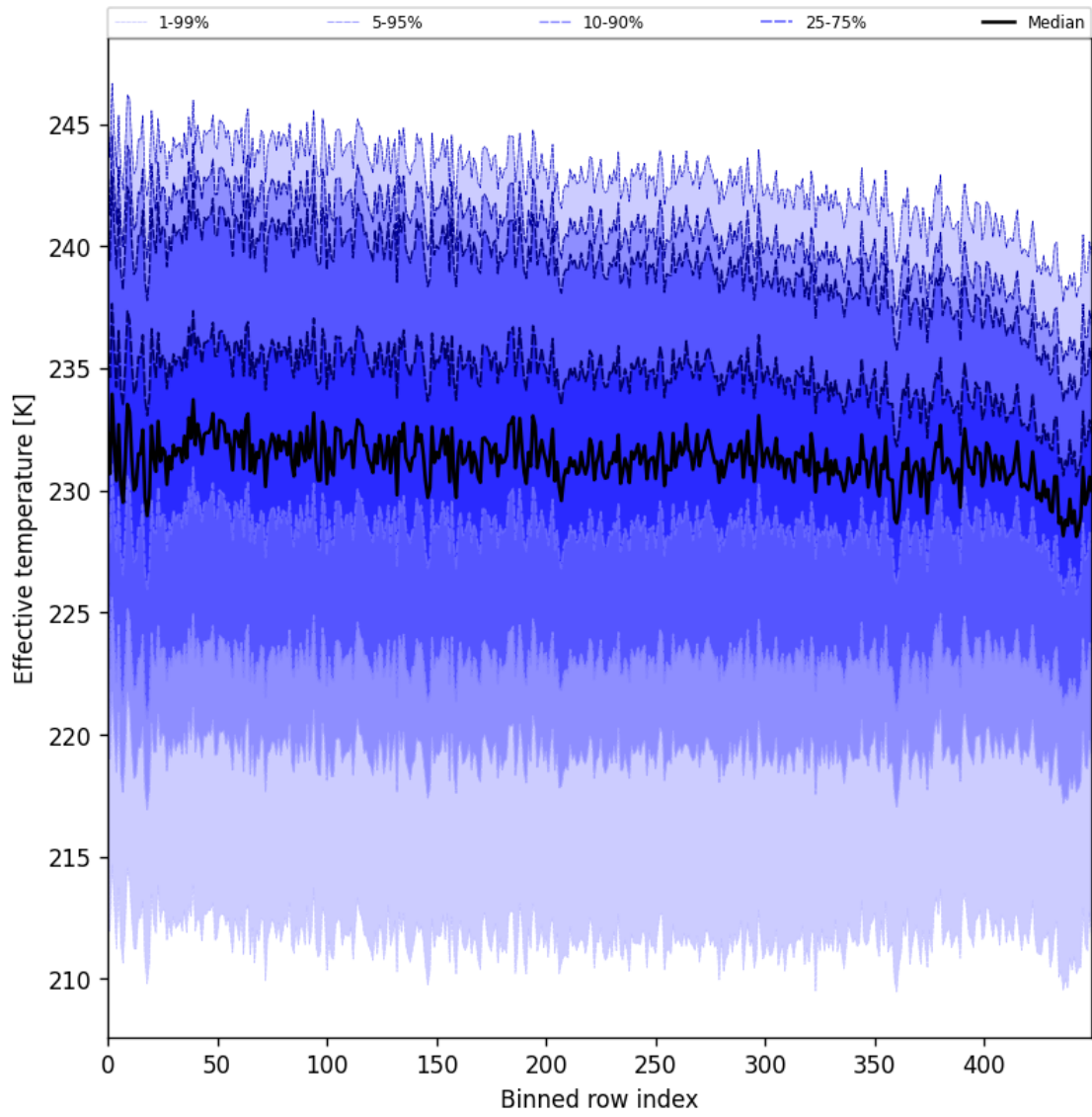
Figure 31: Along track statistics of “Effective temperature” for 2024-11-07 to 2024-11-09
