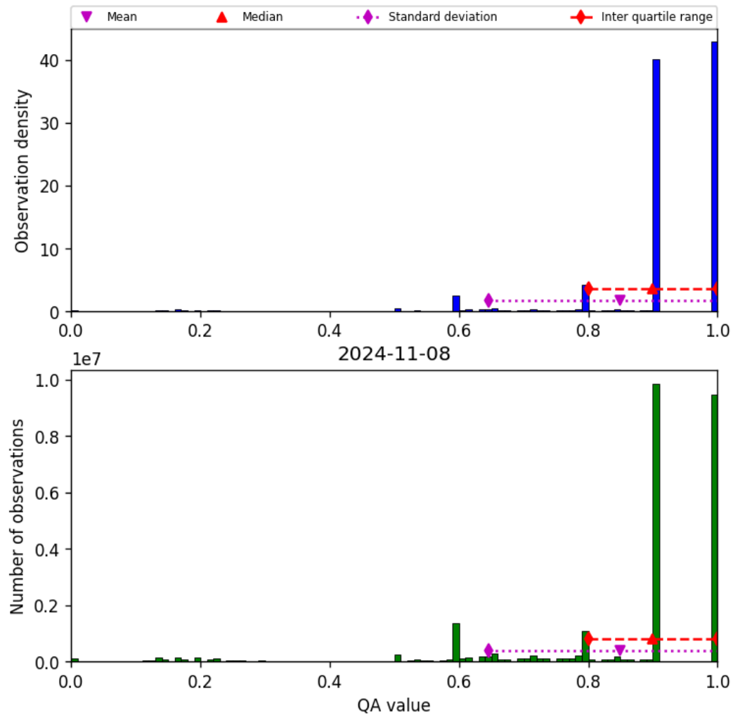
Figure 20: Histogram of “QA value” for 2024-11-07 to 2024-11-09
