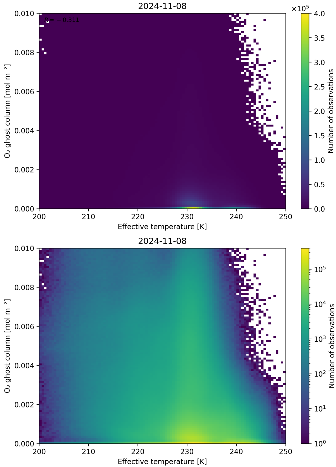
Figure 38: Scatter density plot of “Effective temperature” against “O 3 ghost column” for 2024-11-07 to 2024-11-09.
