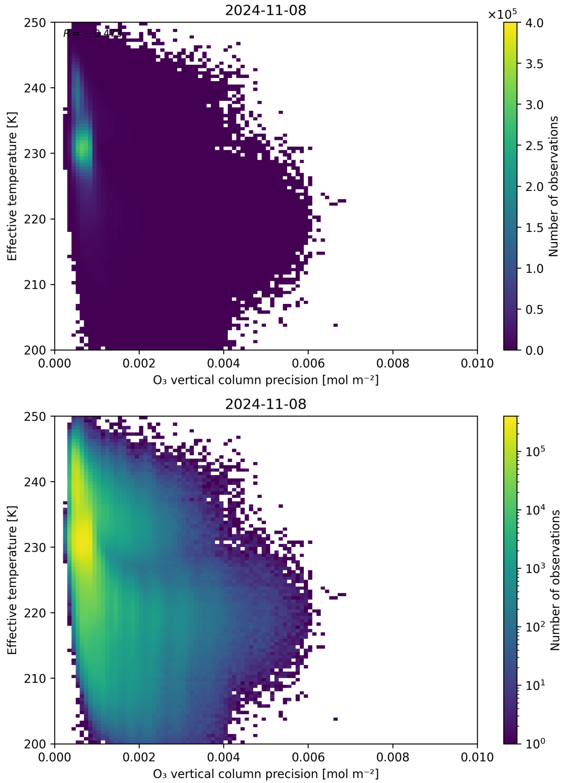
Figure 42: Scatter density plot of “O 3 vertical column precision” against “Effective temperature” for 2024-11-07 to 2024-11-09.
