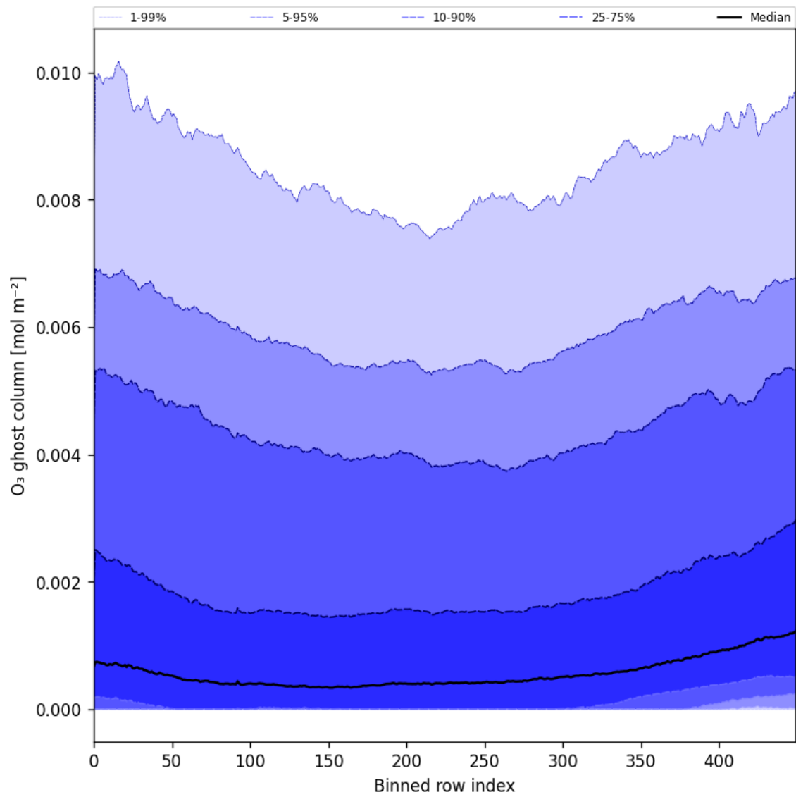
Figure 32: Along track statistics of “O 3 ghost column” for 2024-11-07 to 2024-11-09
