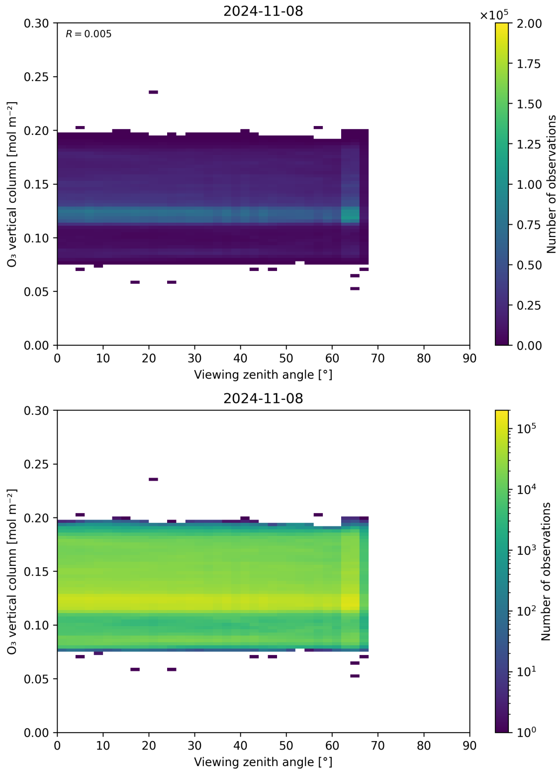
Figure 52: Scatter density plot of “Viewing zenith angle” against “O 3 vertical column” for 2024-11-07 to 2024-11-09.
