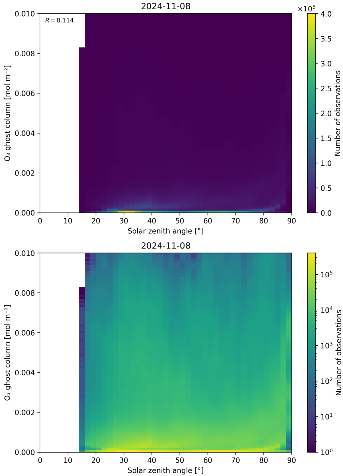
Figure 46: Scatter density plot of “Solar zenith angle” against “O 3 ghost column” for 2024-11-07 to 2024-11-09.
