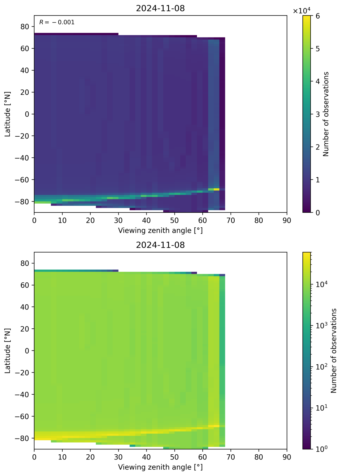
Figure 49: Scatter density plot of “Viewing zenith angle” against “Latitude” for 2024-11-07 to 2024-11-09.
