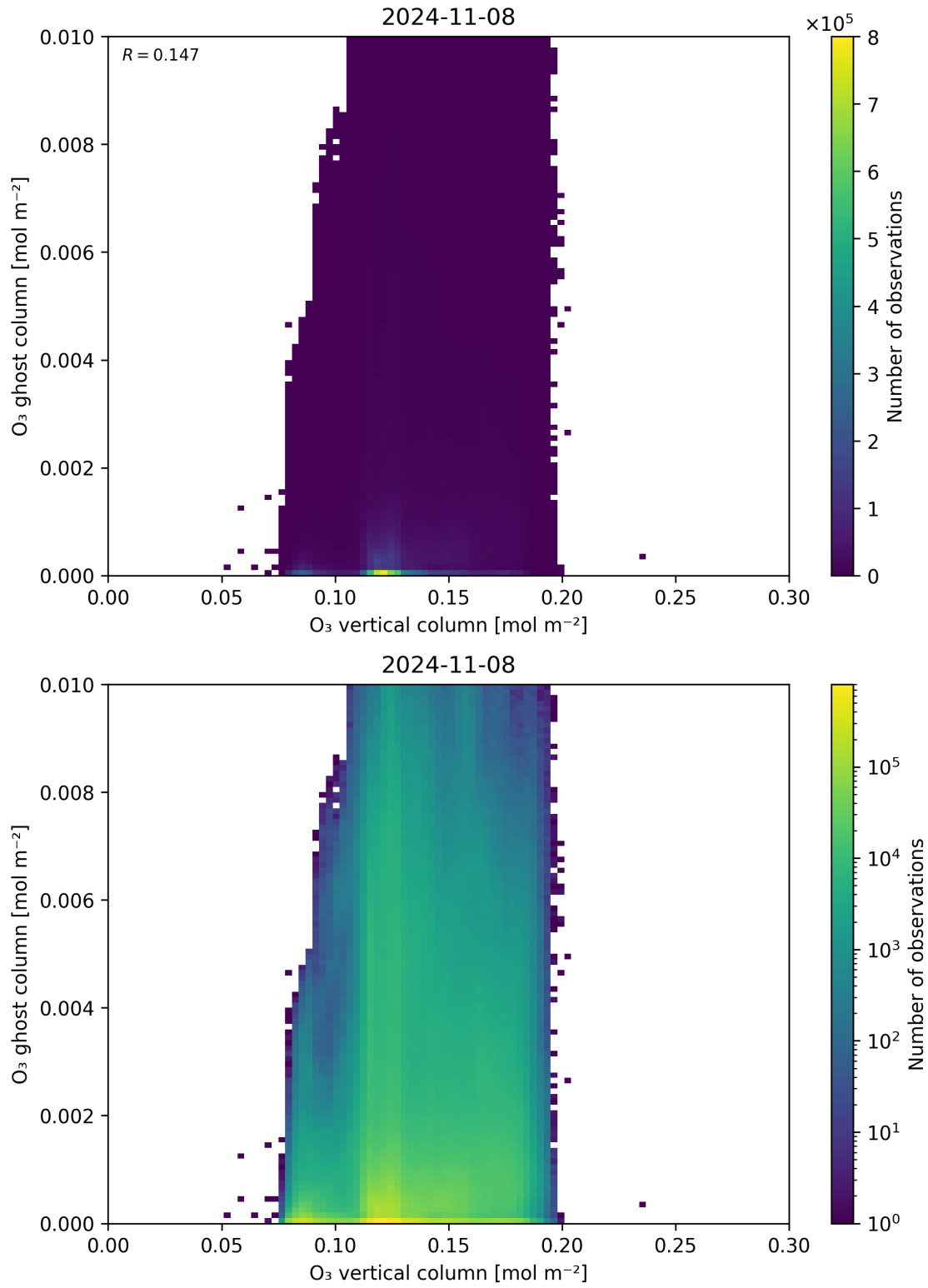
Figure 40: Scatter density plot of “O 3 vertical column” against “O 3 ghost column” for 2024-11-07 to 2024-11-09.
