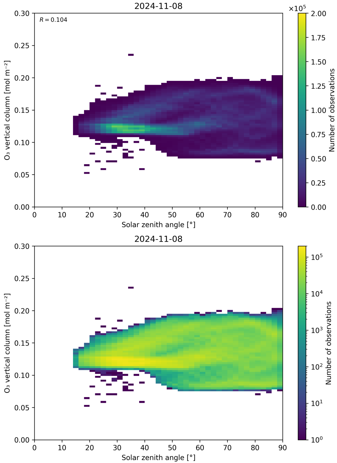
Figure 47: Scatter density plot of “Solar zenith angle” against “O 3 vertical column” for 2024-11-07 to 2024-11-09.
