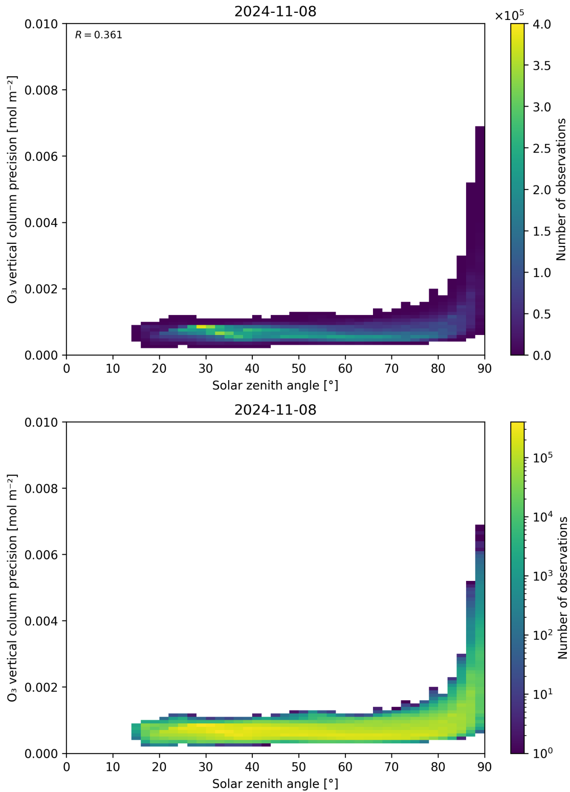
Figure 48: Scatter density plot of “Solar zenith angle” against “O 3 vertical column precision” for 2024-11-07 to 2024-11-09.
