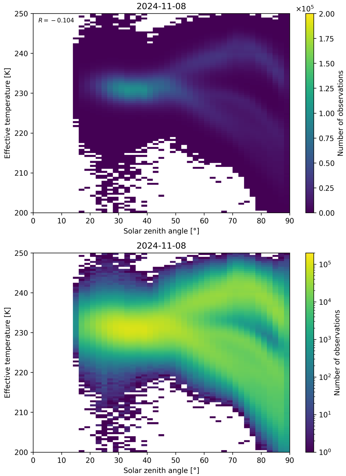
Figure 45: Scatter density plot of “Solar zenith angle” against “Effective temperature” for 2024-11-07 to 2024-11-09.
