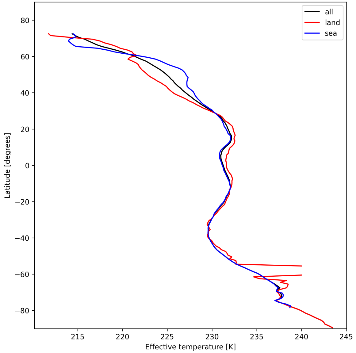
Figure 17: Zonal average of “Effective temperature” for 2024-11-07 to 2024-11-09.
