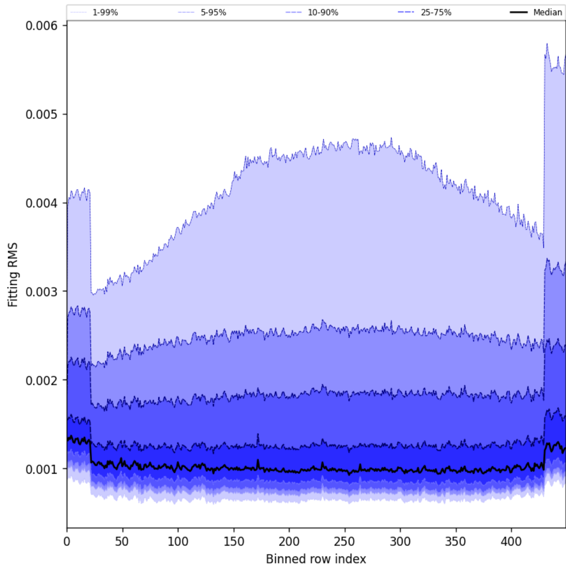
Figure 30: Along track statistics of “Fitting RMS” for 2024-11-07 to 2024-11-09
