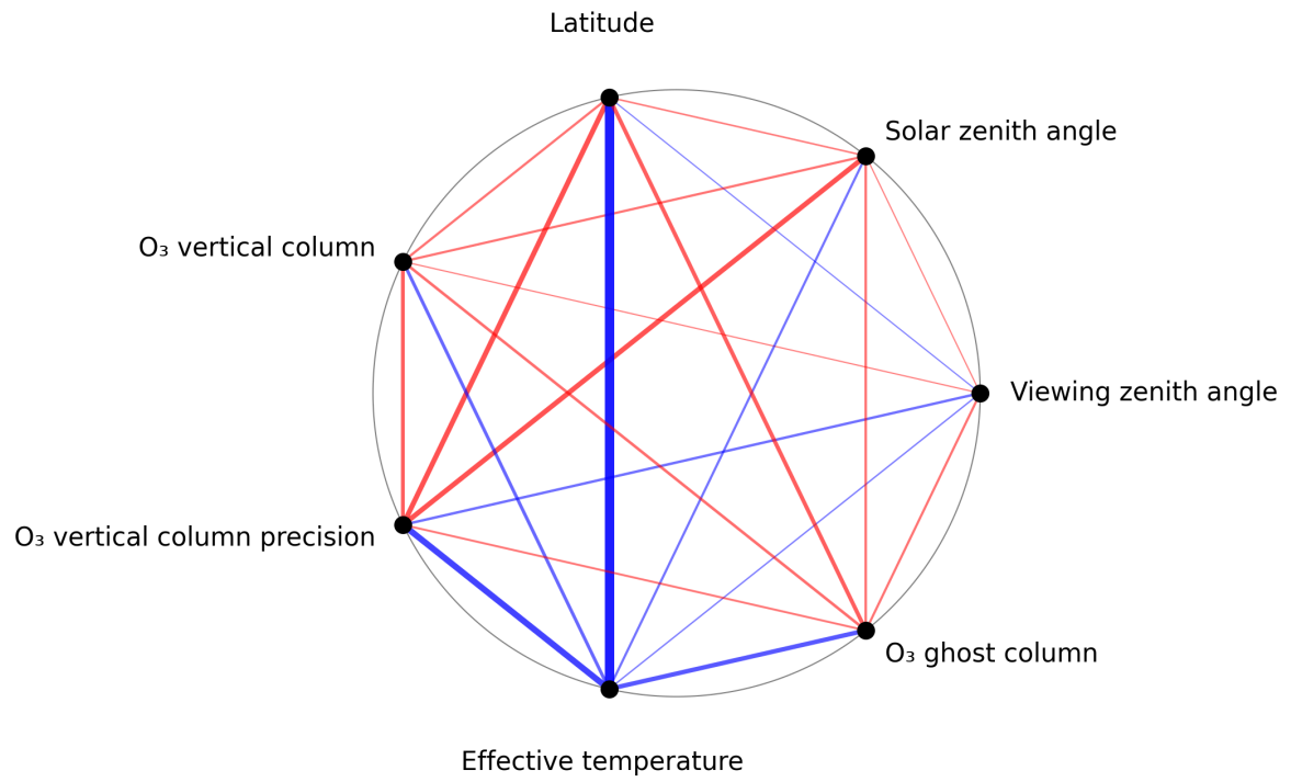
Figure 1: Map of correlation graph for 2024-11-07 to 2024-11-09.
