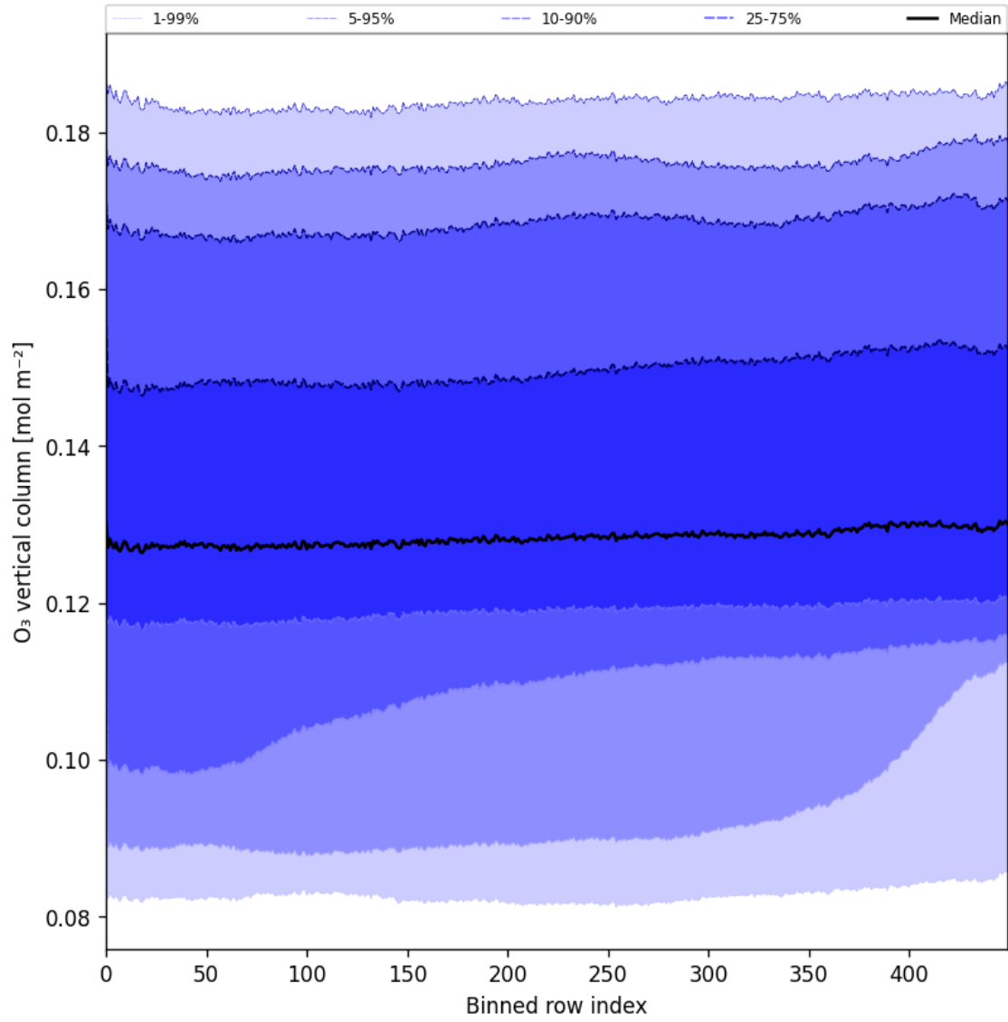
Figure 28: Along track statistics of “O 3 vertical column” for 2024-11-07 to 2024-11-09
