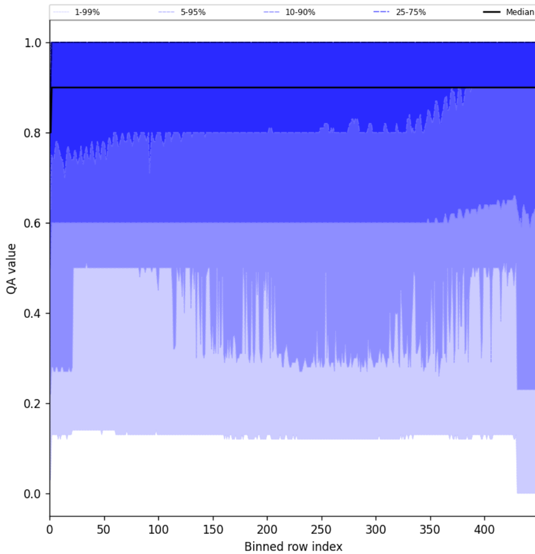
Figure 27: Along track statistics of “QA value” for 2024-11-07 to 2024-11-09
