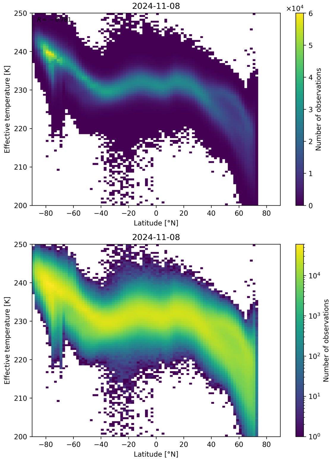
Figure 34: Scatter density plot of “Latitude” against “Effective temperature” for 2024-11-07 to 2024-11-09.
