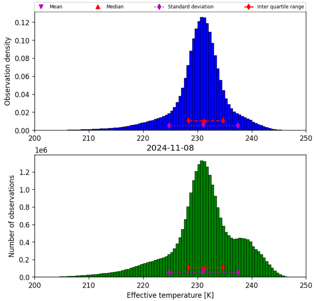
Figure 24: Histogram of “Effective temperature” for 2024-11-07 to 2024-11-09
