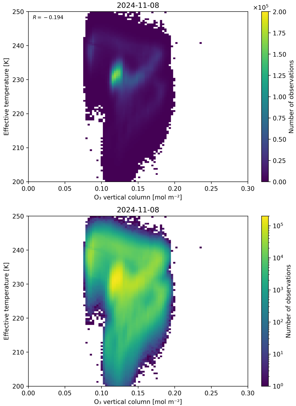
Figure 39: Scatter density plot of “O 3 vertical column” against “Effective temperature” for 2024-11-07 to 2024-11-09.
