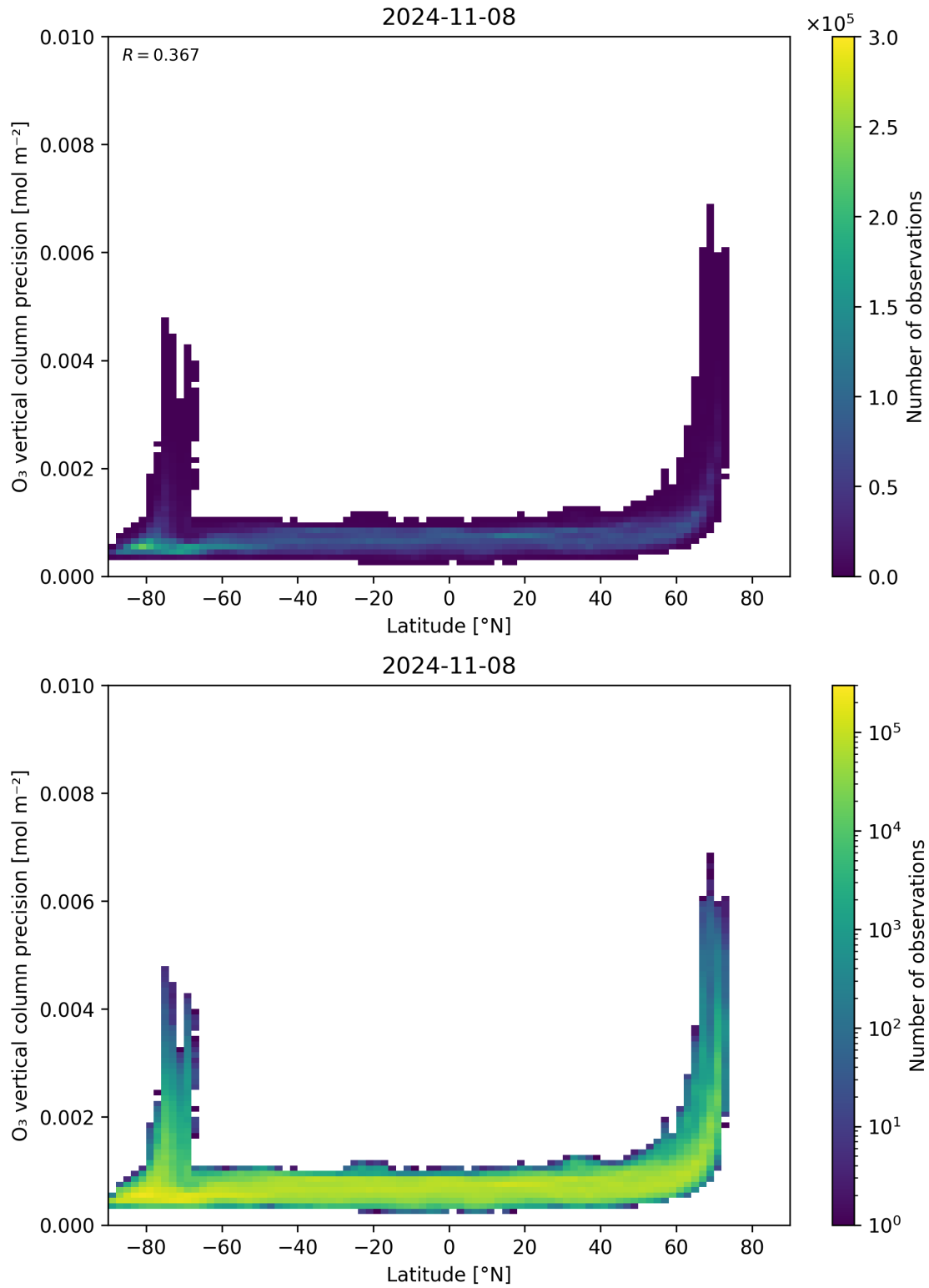
Figure 37: Scatter density plot of “Latitude” against “O 3 vertical column precision” for 2024-11-07 to 2024-11-09.
