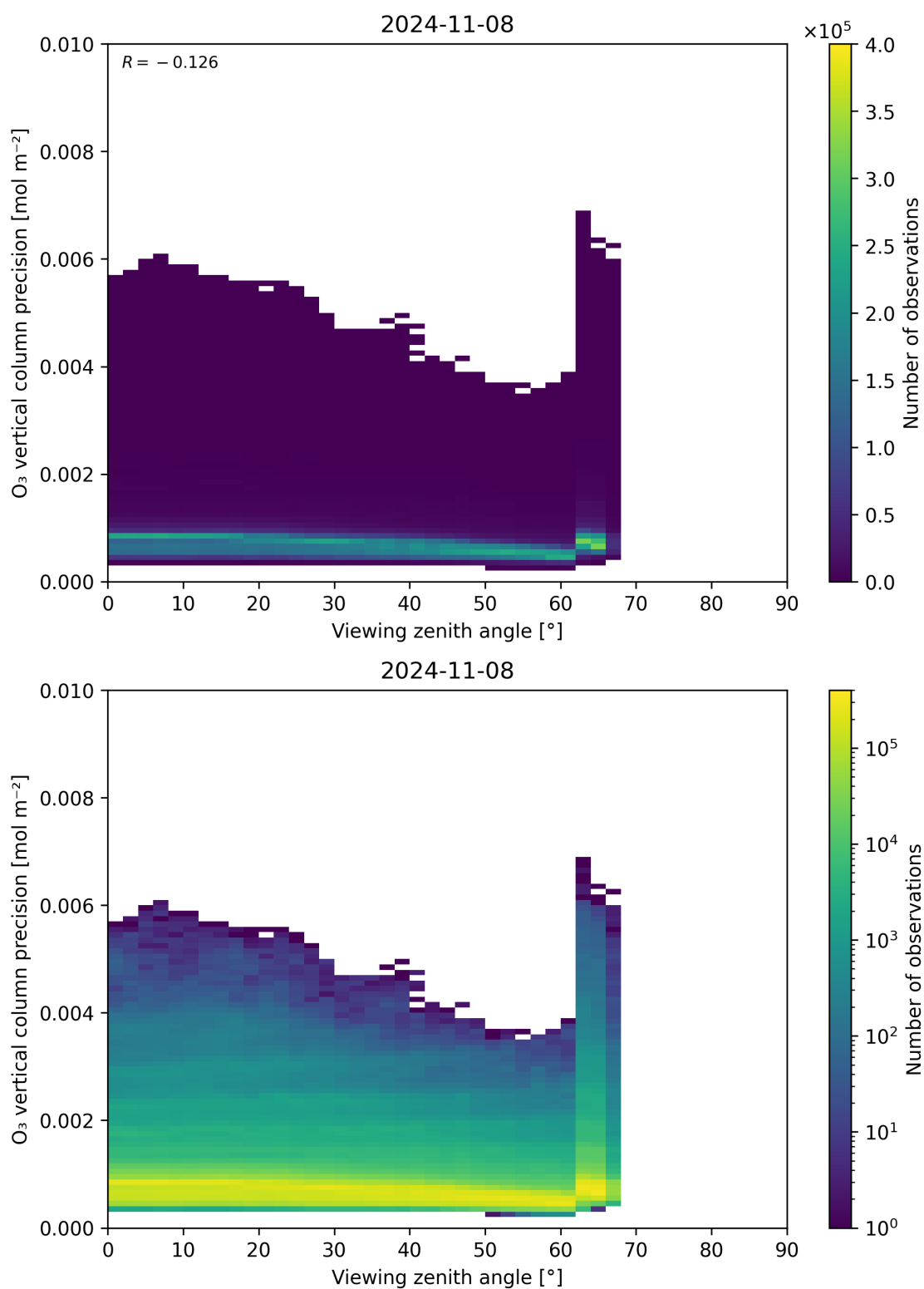
Figure 53: Scatter density plot of “Viewing zenith angle” against “O 3 vertical column precision” for 2024-11-07 to 2024-11-09.
