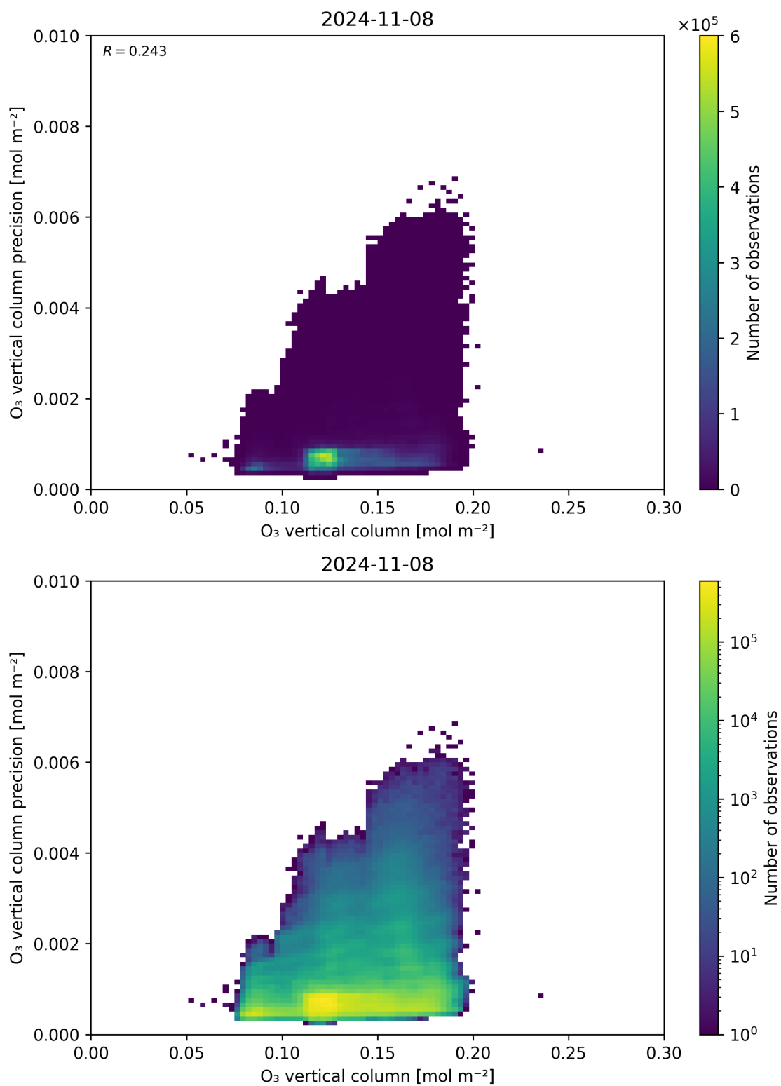
Figure 41: Scatter density plot of “O 3 vertical column” against “O 3 vertical column precision” for 2024-11-07 to 2024-11-09.
