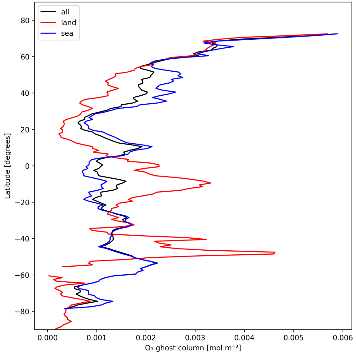
Figure 18: Zonal average of “O 3 ghost column” for 2024-11-07 to 2024-11-09.
