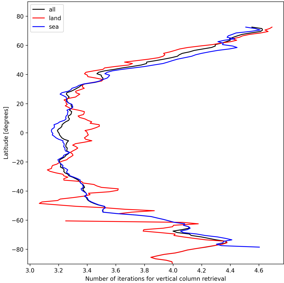
Figure 19: Zonal average of “Number of iterations for vertical column retrieval” for 2024-11-07 to 2024-11-09.
