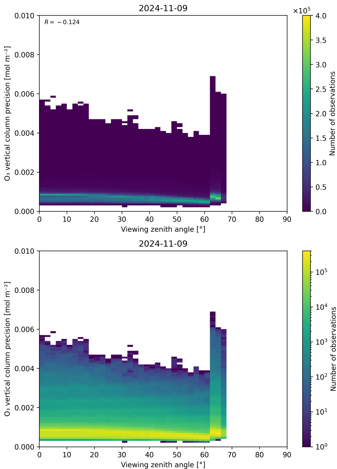
Figure 53: Scatter density plot of “Viewing zenith angle” against “O 3 vertical column precision” for 2024-11-09 to 2024-11-10.
