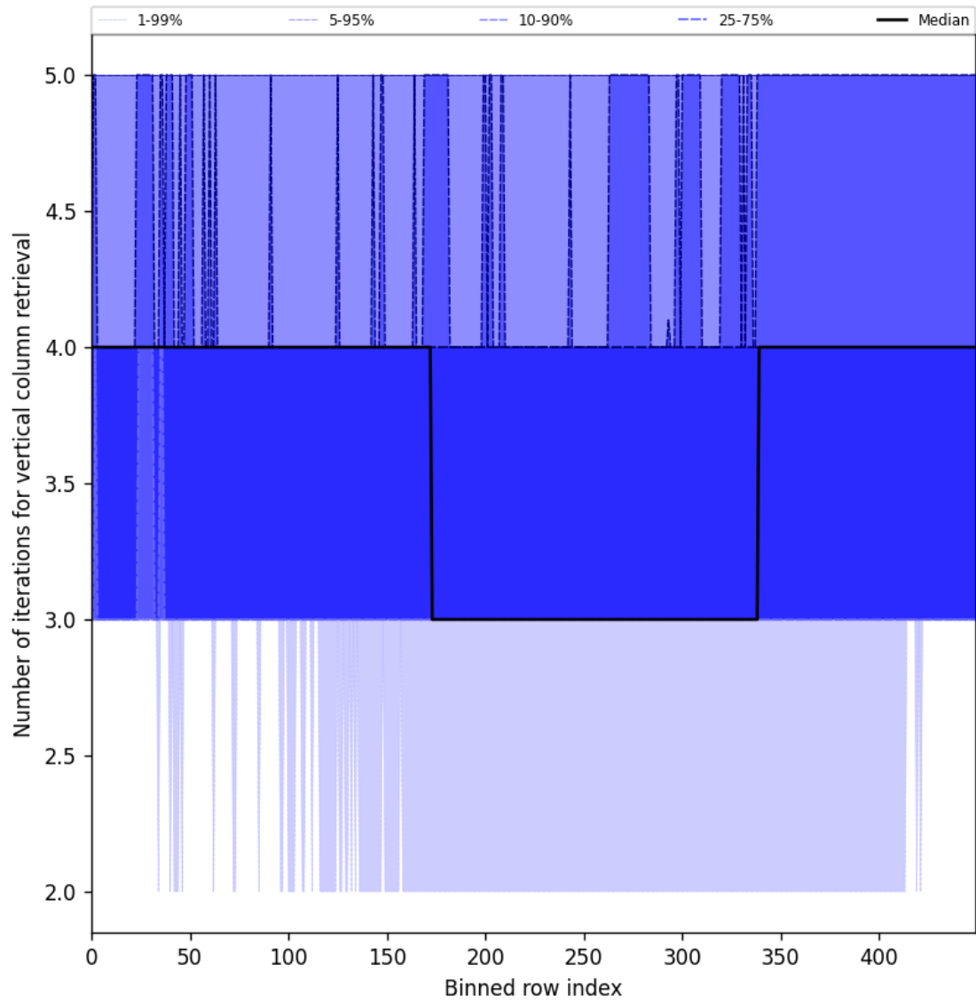
Figure 33: Along track statistics of “Number of iterations for vertical column retrieval” for 2024-11-09 to 2024-11-10
