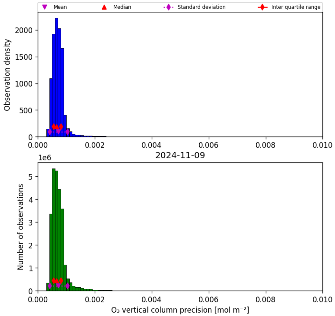
Figure 22: Histogram of “O 3 vertical column precision” for 2024-11-09 to 2024-11-10
