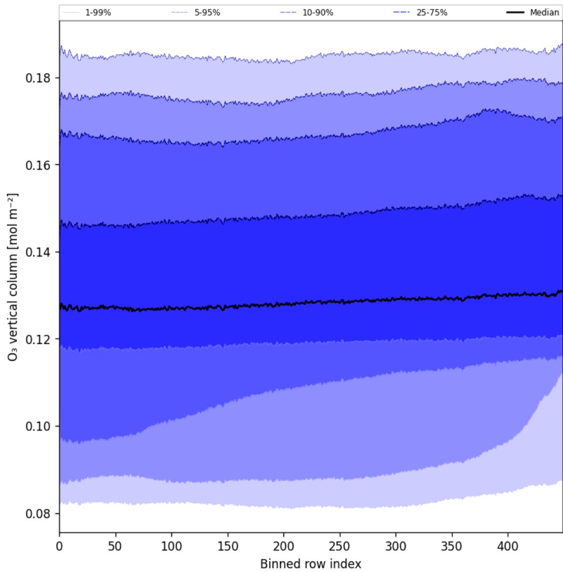
Figure 28: Along track statistics of “ O_3 vertical column” for 2024-11-09 to 2024-11-10
