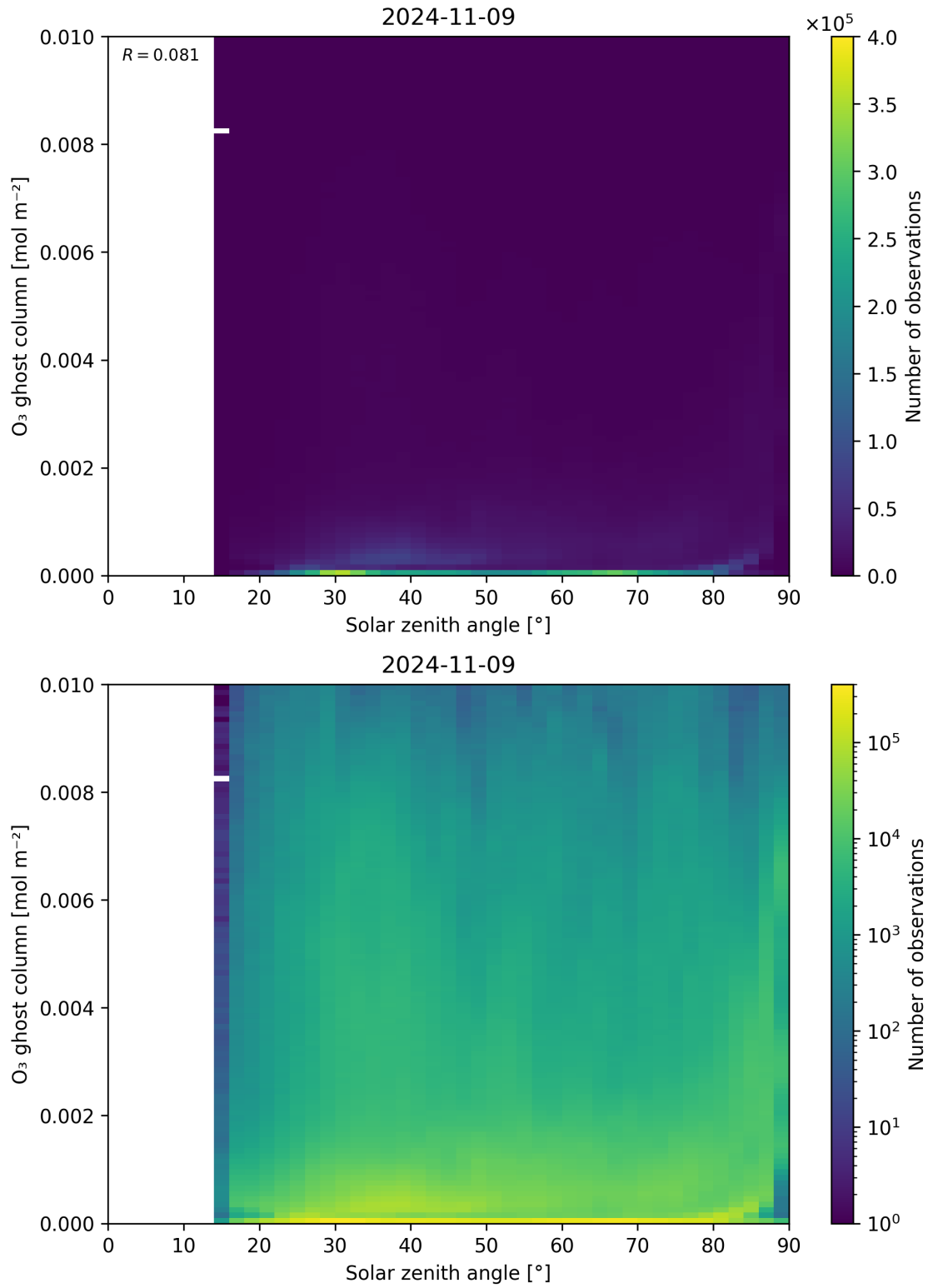
Figure 46: Scatter density plot of “Solar zenith angle” against “O 3 ghost column” for 2024-11-09 to 2024-11-10.
