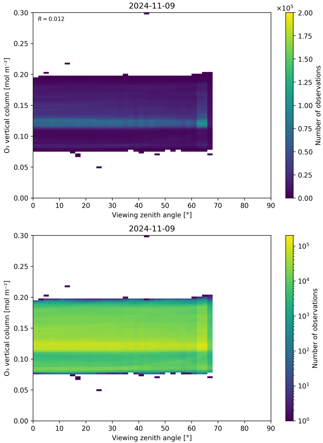
Figure 52: Scatter density plot of “Viewing zenith angle” against “O 3 vertical column” for 2024-11-09 to 2024-11-10.
