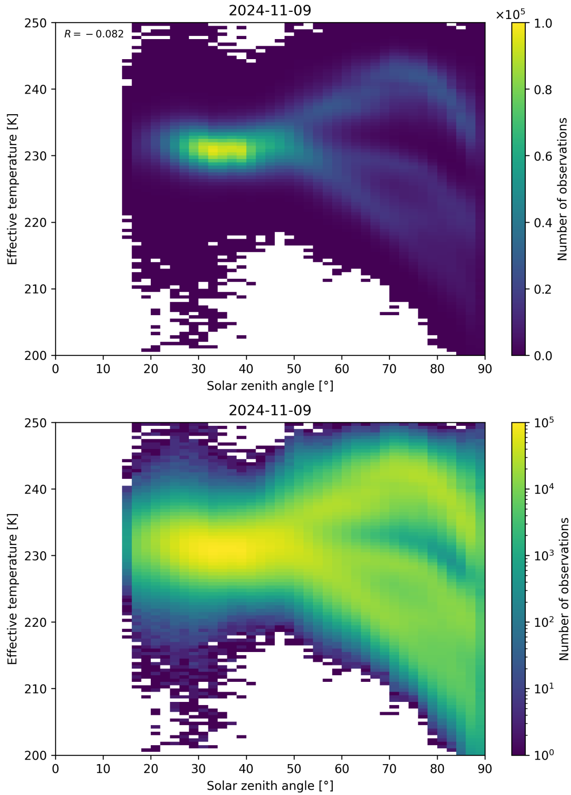
Figure 45: Scatter density plot of “Solar zenith angle” against “Effective temperature” for 2024-11-09 to 2024-11-10.
