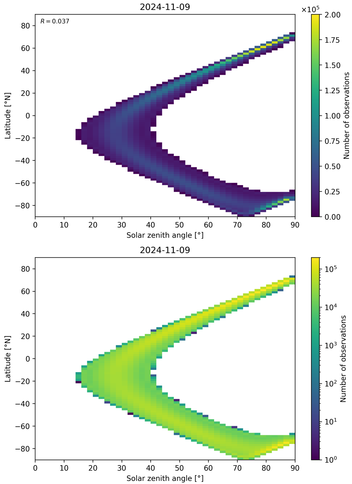
Figure 44: Scatter density plot of “Solar zenith angle” against “Latitude” for 2024-11-09 to 2024-11-10.
