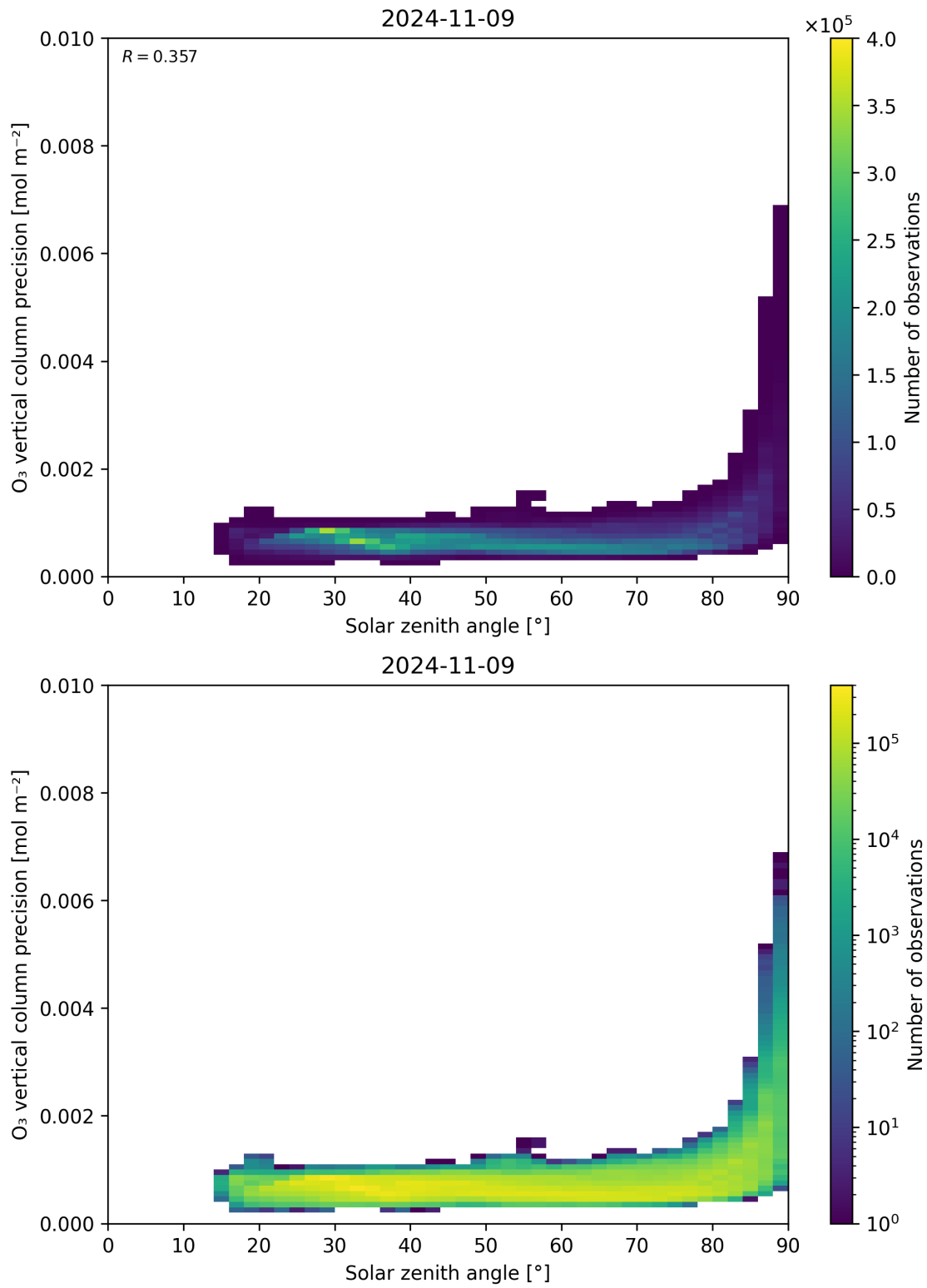
Figure 48: Scatter density plot of “Solar zenith angle” against “O 3 vertical column precision” for 2024-11-09 to 2024-11-10.
