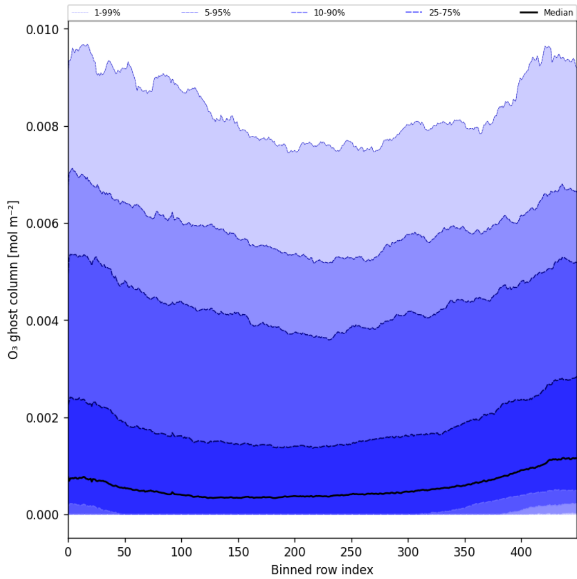
Figure 32: Along track statistics of “O 3 ghost column” for 2024-11-09 to 2024-11-10
