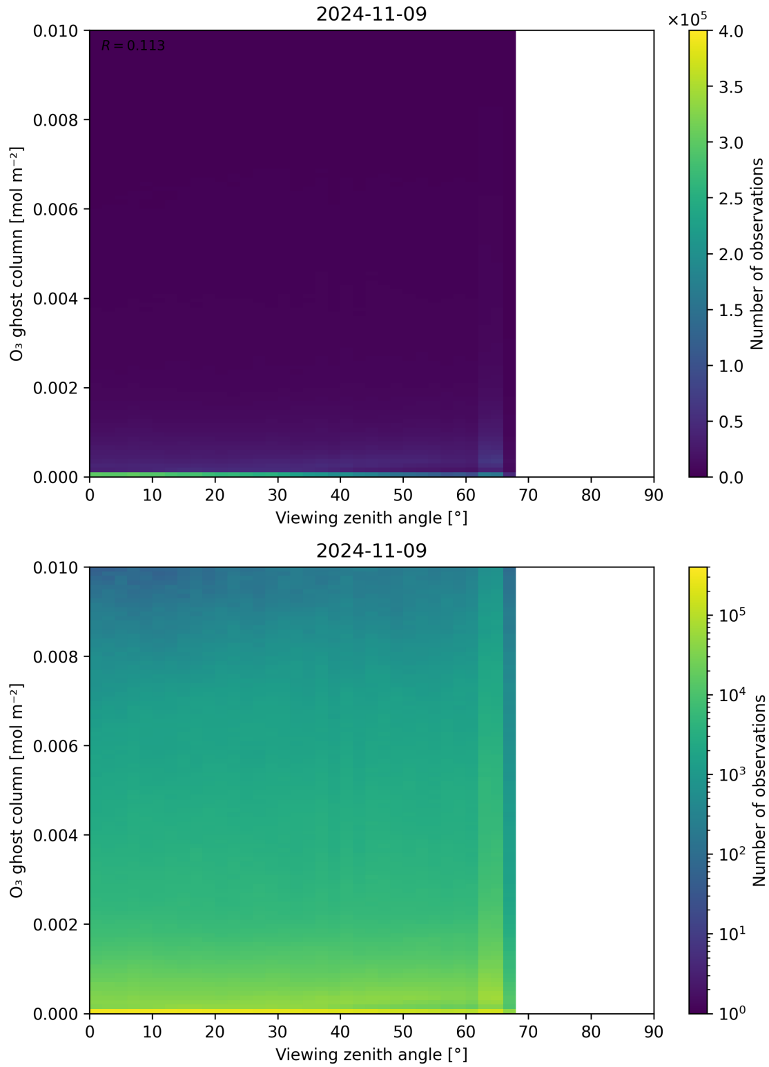
Figure 51: Scatter density plot of “Viewing zenith angle” against “O 3 ghost column” for 2024-11-09 to 2024-11-10.
