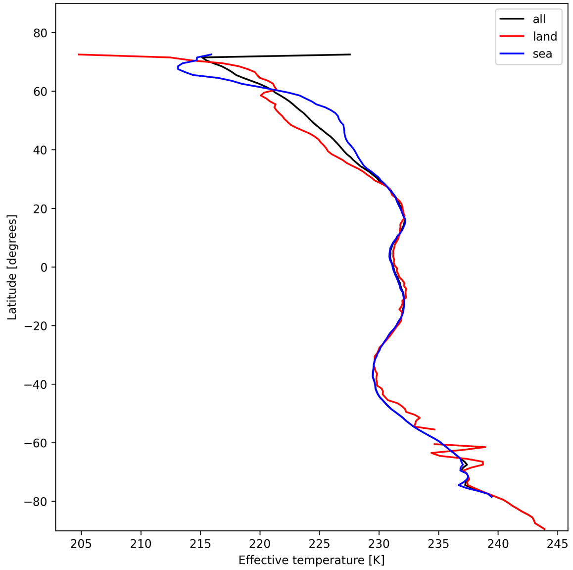
Figure 17: Zonal average of “Effective temperature” for 2024-11-09 to 2024-11-10.
