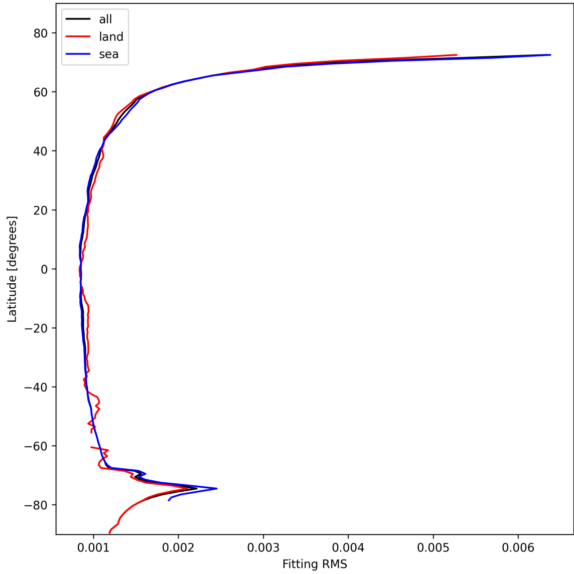
Figure 16: Zonal average of “Fitting RMS” for 2024-11-09 to 2024-11-10.
