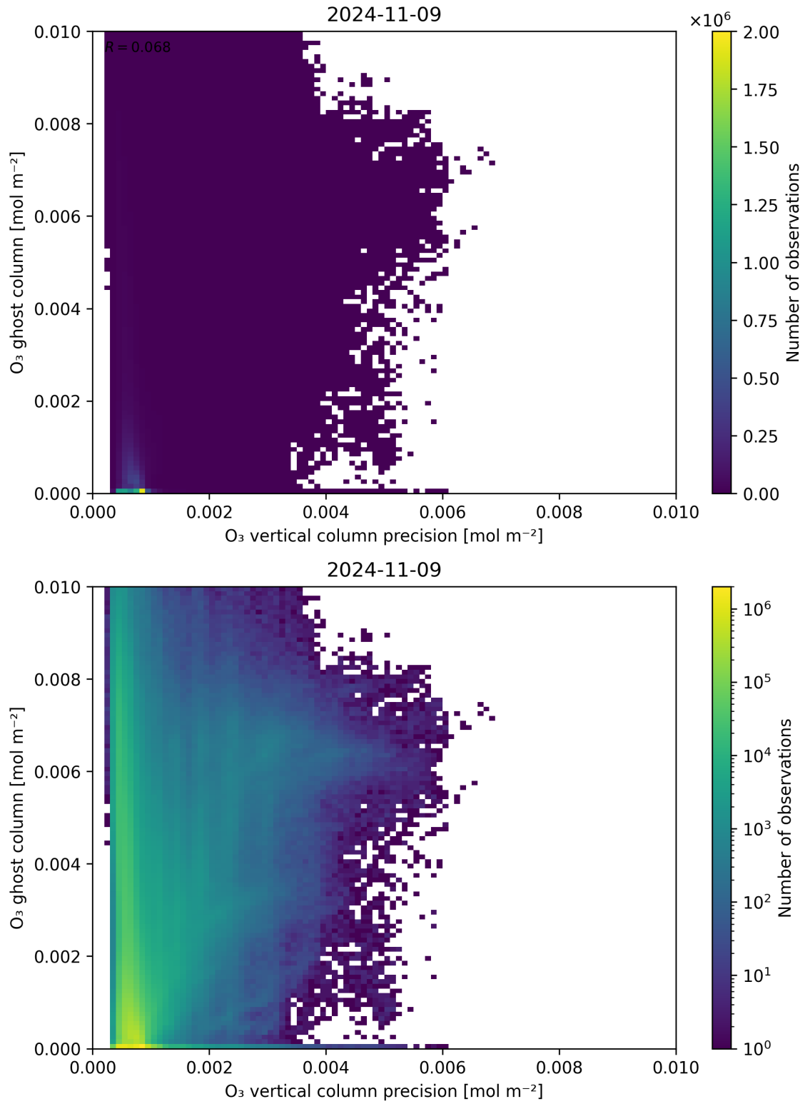
Figure 43: Scatter density plot of “ \text{O}_3 vertical column precision” against “ \text{O}_3 ghost column” for 2024-11-09 to 2024-11-10.
