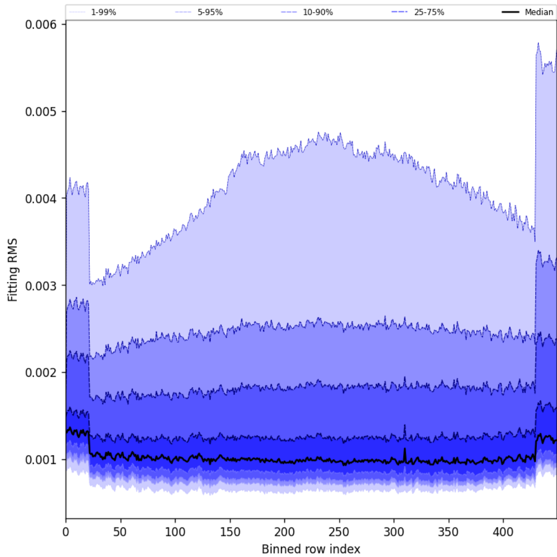
Figure 30: Along track statistics of “Fitting RMS” for 2024-11-09 to 2024-11-10
