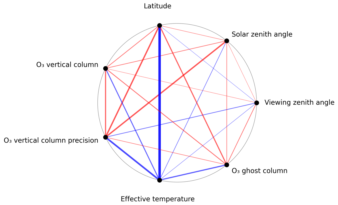
Figure 1: Map of correlation graph for 2024-11-09 to 2024-11-10.
