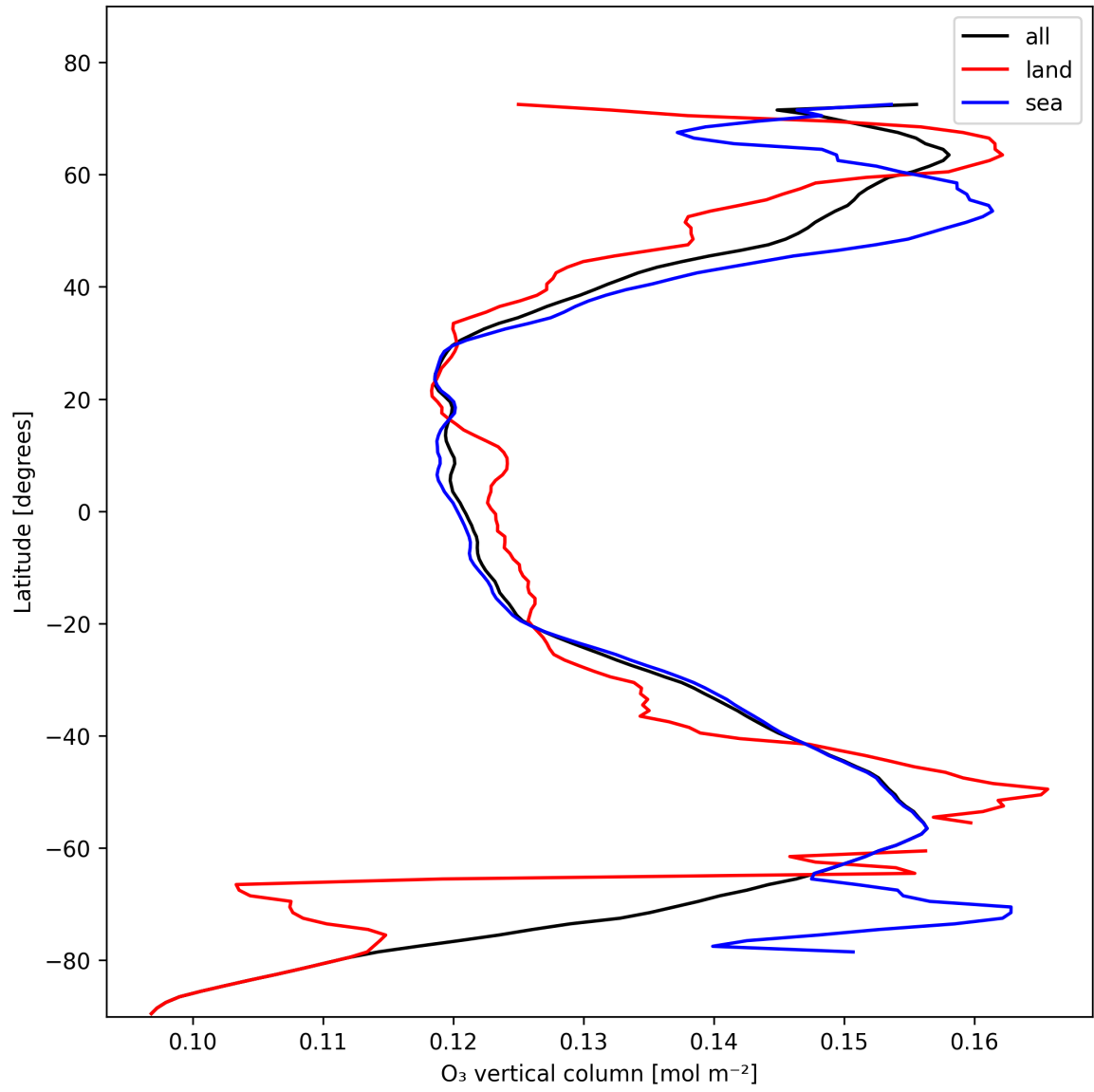
Figure 14: Zonal average of “O 3 vertical column” for 2024-11-09 to 2024-11-10.
