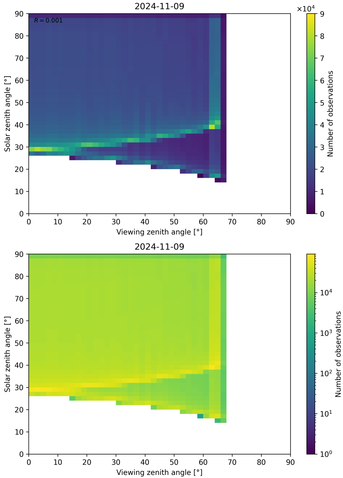
Figure 54: Scatter density plot of “Viewing zenith angle” against “Solar zenith angle” for 2024-11-09 to 2024-11-10.
