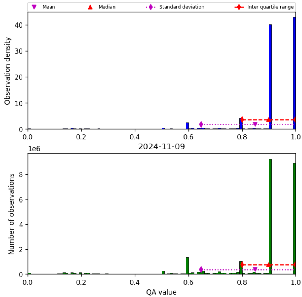
Figure 20: Histogram of “QA value” for 2024-11-09 to 2024-11-10
