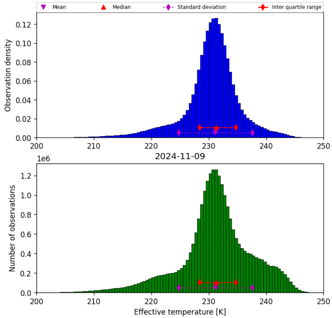
Figure 24: Histogram of “Effective temperature” for 2024-11-09 to 2024-11-10
