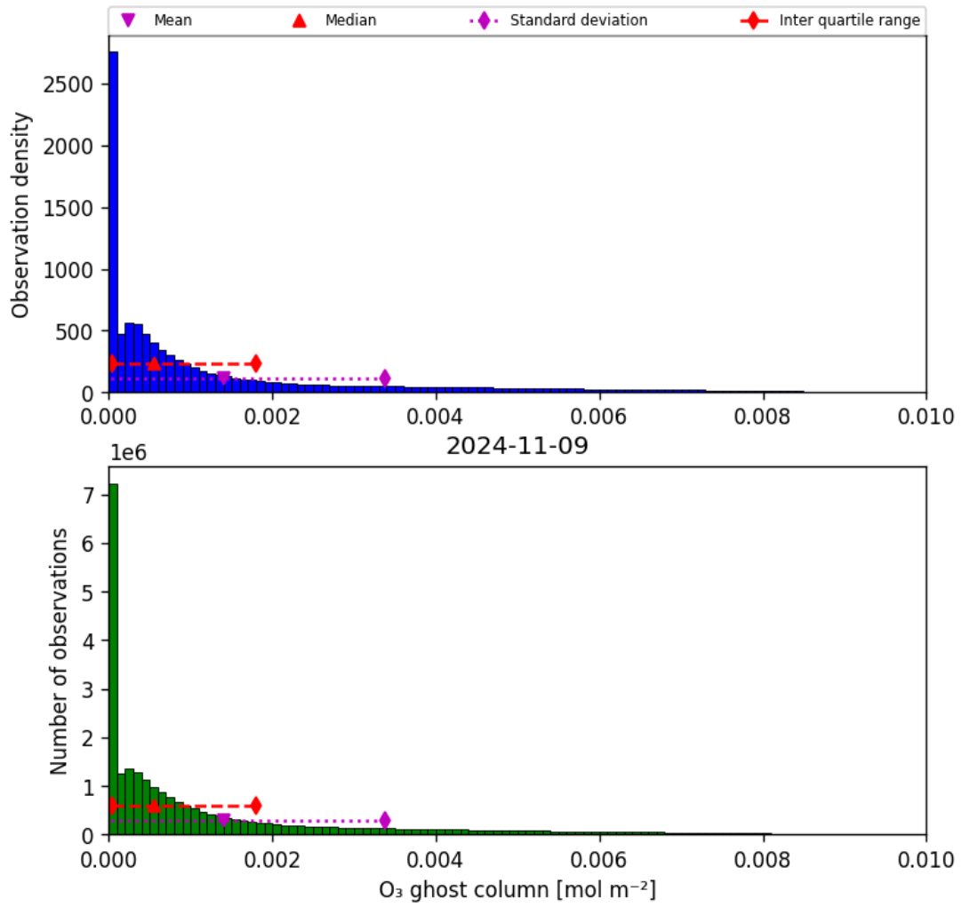
Figure 25: Histogram of “O 3 ghost column” for 2024-11-09 to 2024-11-10
