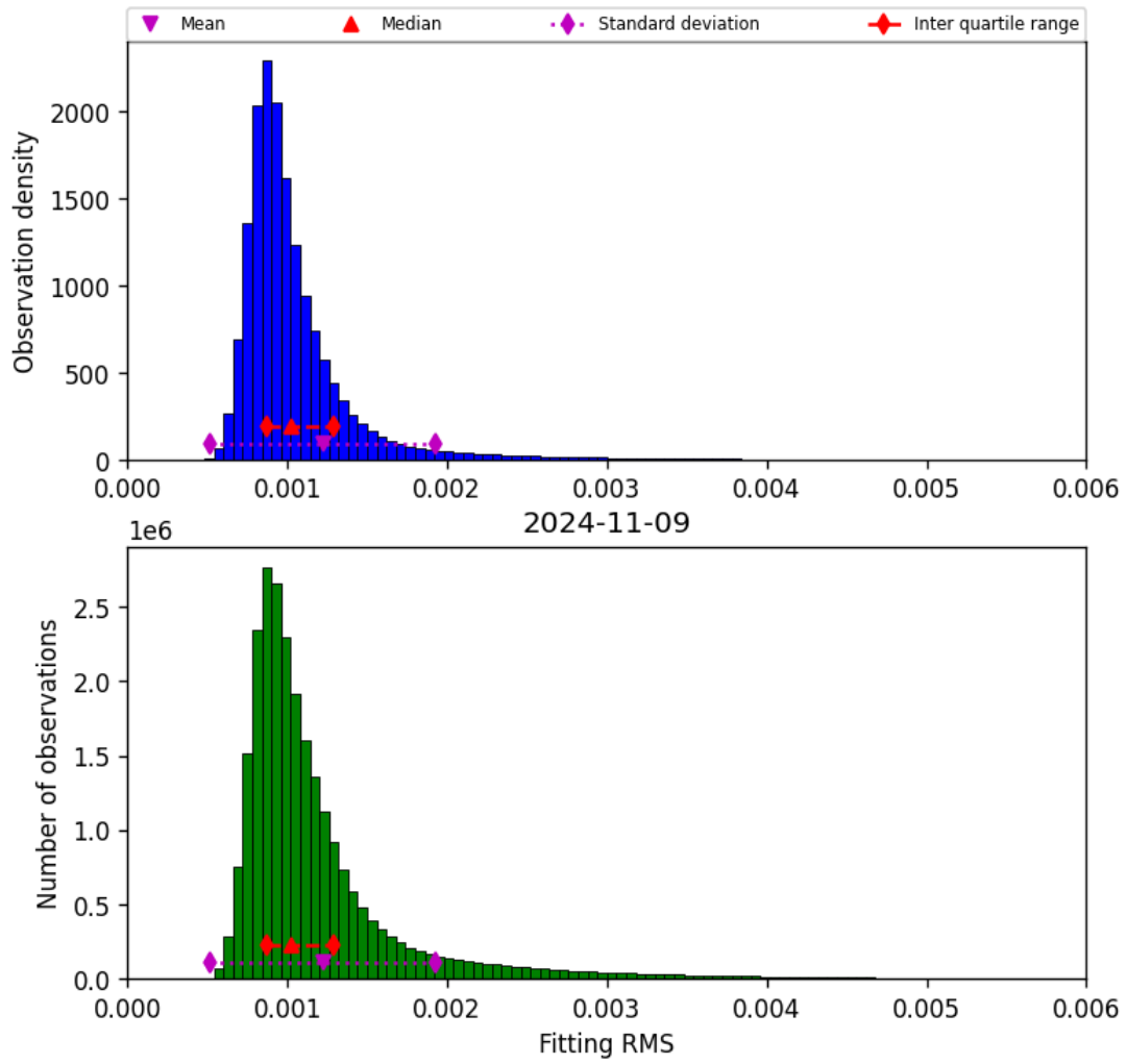
Figure 23: Histogram of “Fitting RMS” for 2024-11-09 to 2024-11-10
