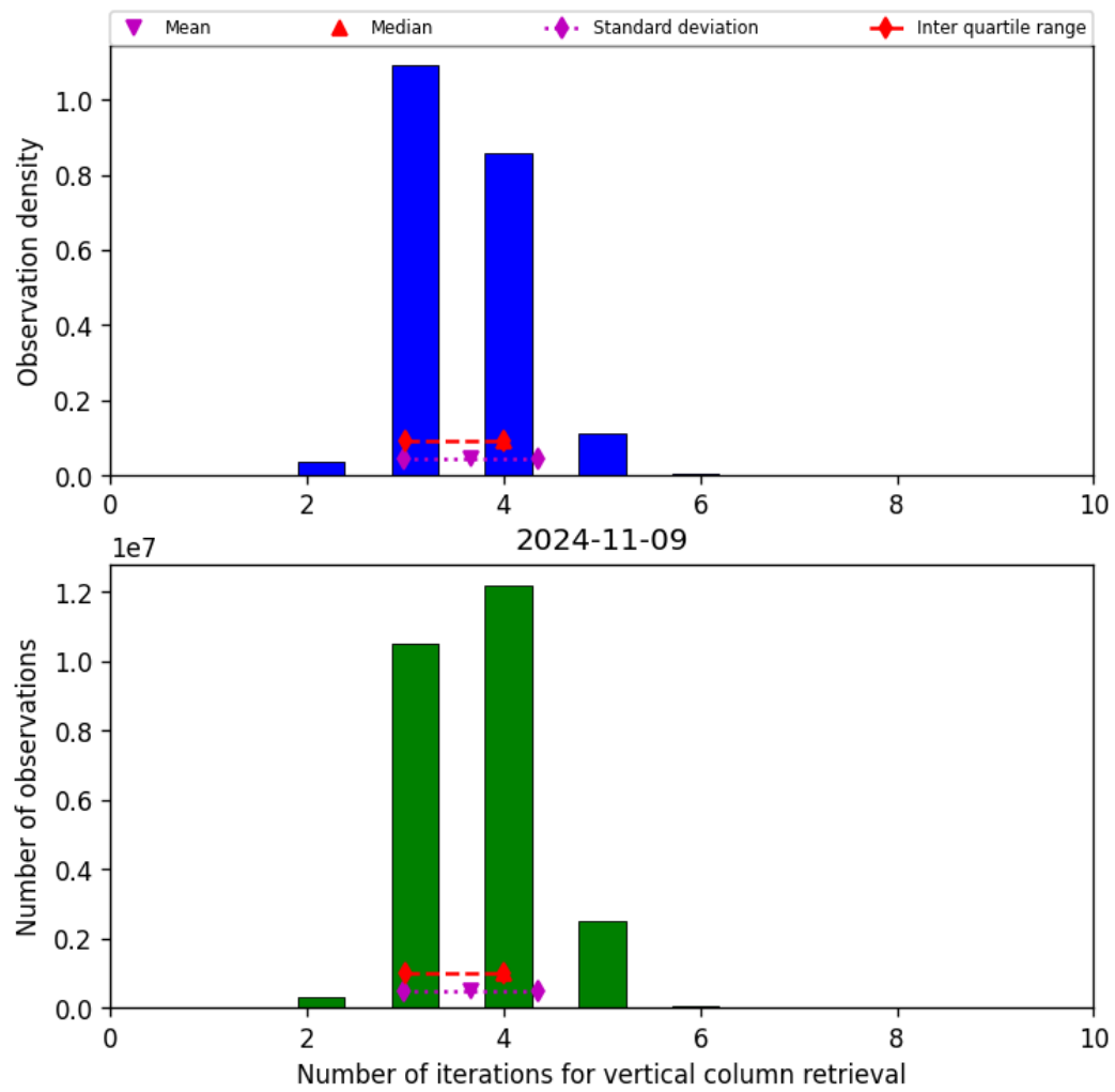
Figure 26: Histogram of “Number of iterations for vertical column retrieval” for 2024-11-09 to 2024-11-10
