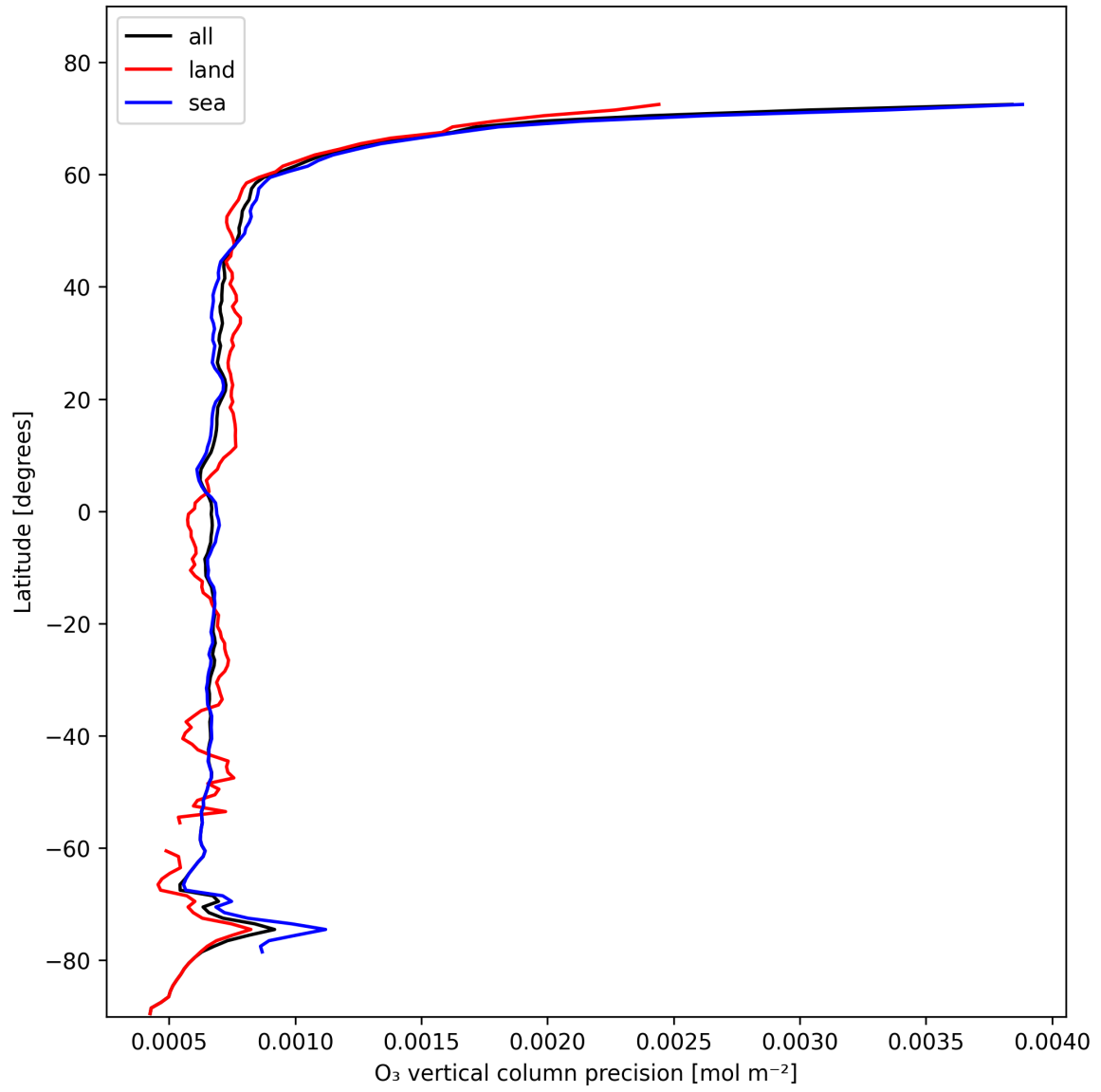
Figure 15: Zonal average of “O 3 vertical column precision” for 2024-11-09 to 2024-11-10.
