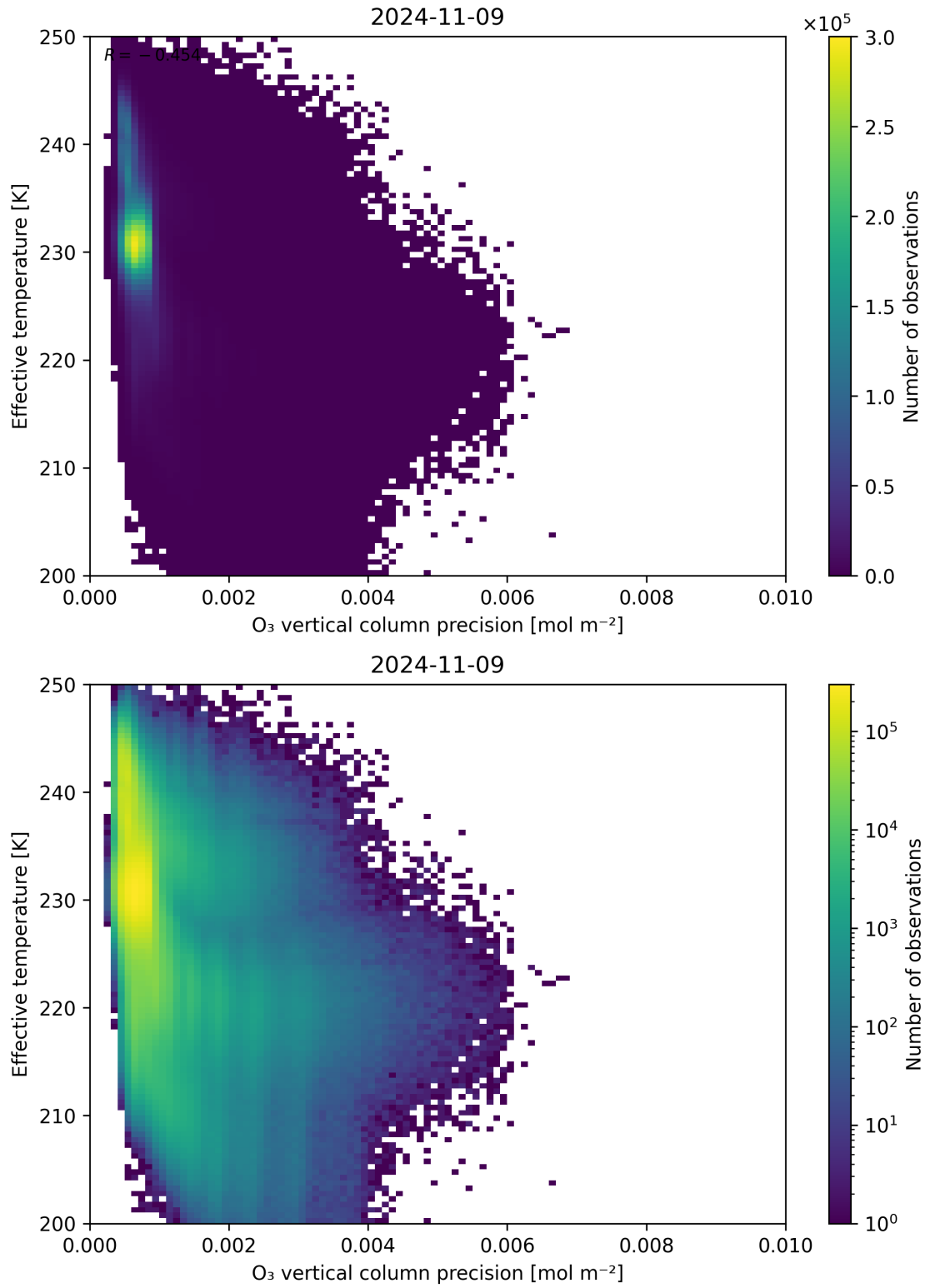
Figure 42: Scatter density plot of “O 3 vertical column precision” against “Effective temperature” for 2024-11-09 to 2024-11-10.
