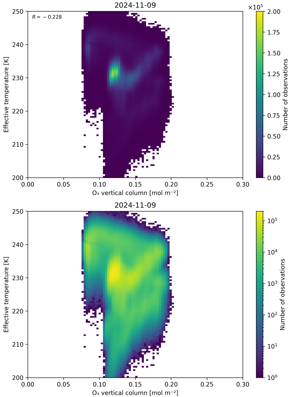
Figure 39: Scatter density plot of “O 3 vertical column” against “Effective temperature” for 2024-11-09 to 2024-11-10.
