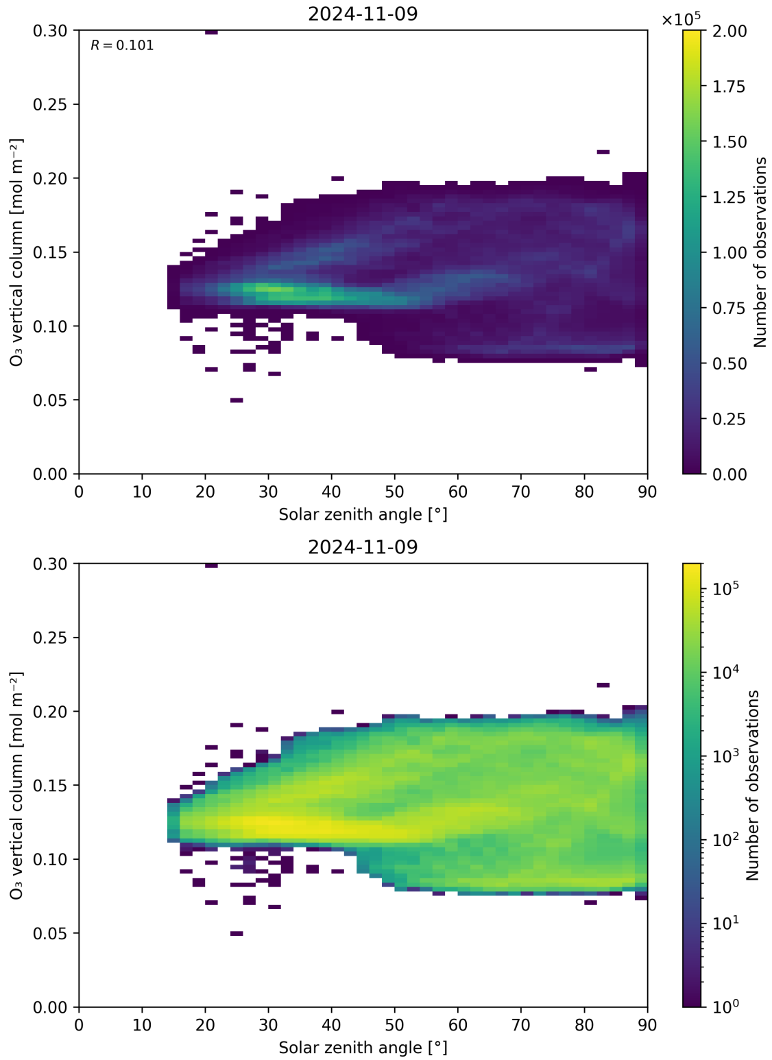
Figure 47: Scatter density plot of “Solar zenith angle” against “O 3 vertical column” for 2024-11-09 to 2024-11-10.
