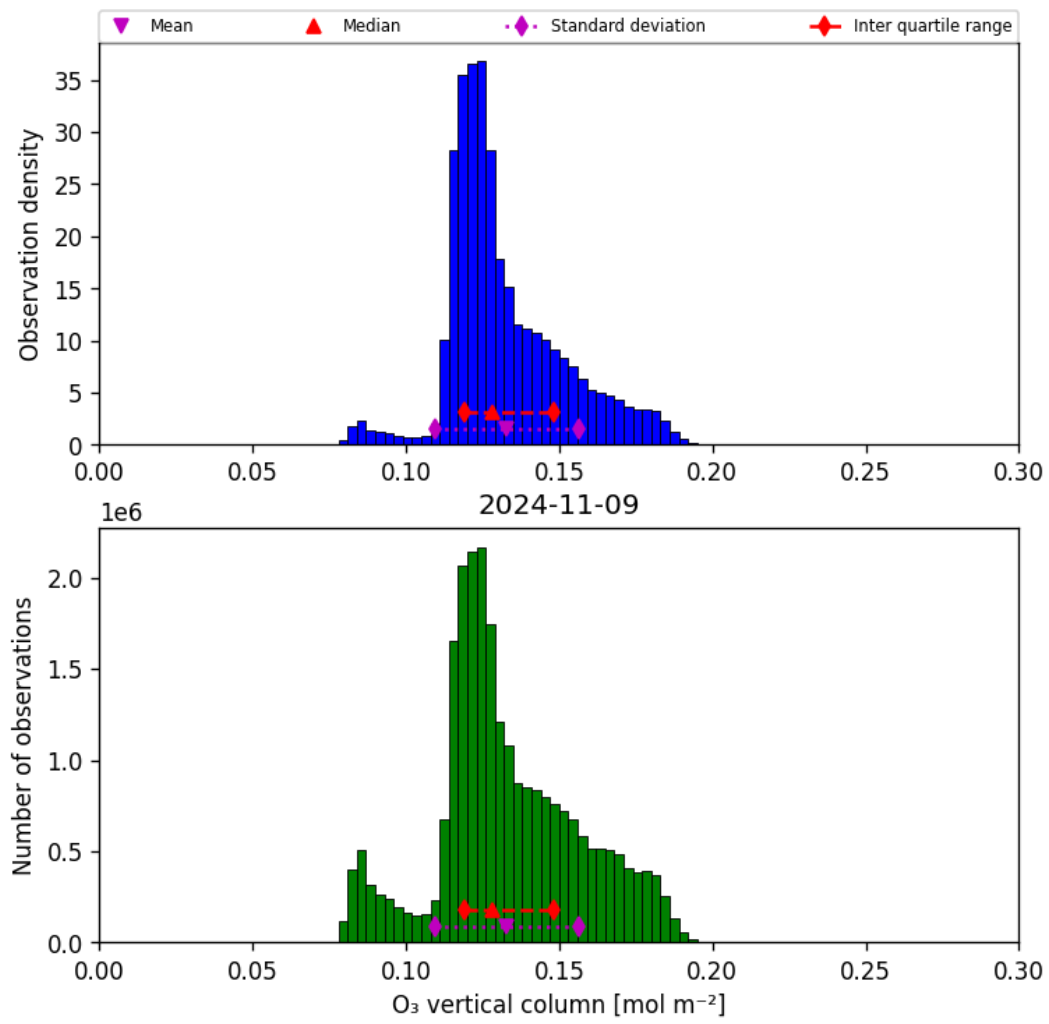
Figure 21: Histogram of “O 3 vertical column” for 2024-11-09 to 2024-11-10
