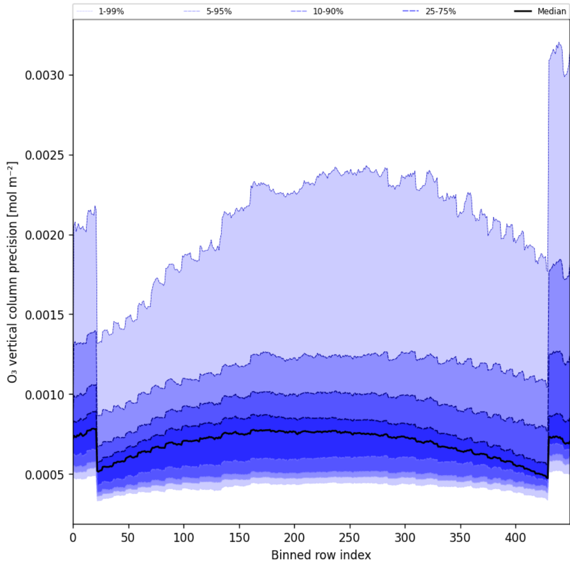
Figure 29: Along track statistics of “O 3 vertical column precision” for 2024-11-09 to 2024-11-10
