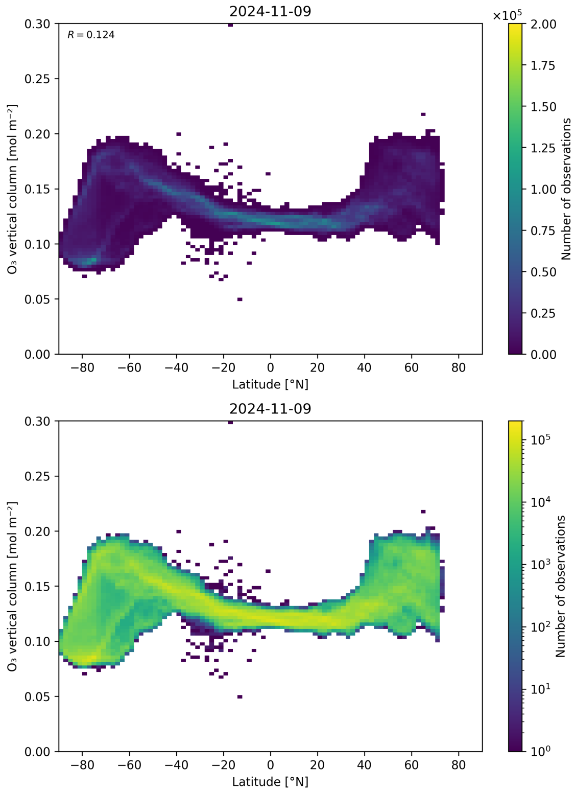
Figure 36: Scatter density plot of “Latitude” against “O 3 vertical column” for 2024-11-09 to 2024-11-10.
