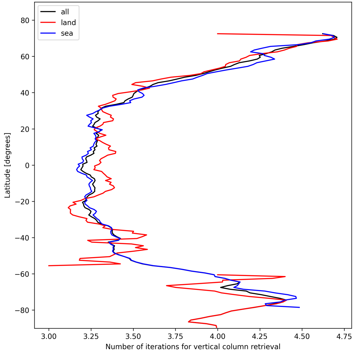
Figure 19: Zonal average of “Number of iterations for vertical column retrieval” for 2024-11-09 to 2024-11-10.
