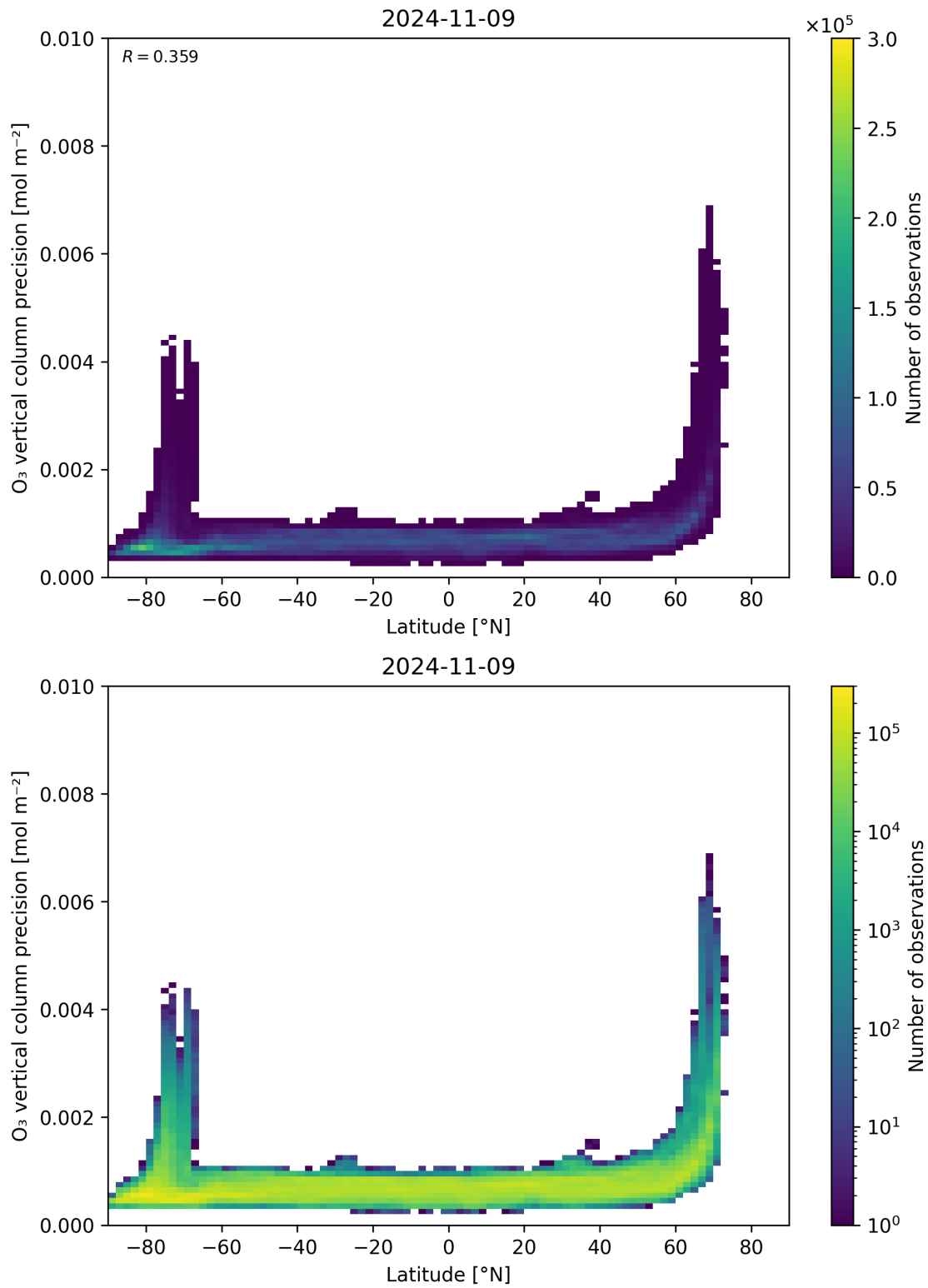
Figure 37: Scatter density plot of “Latitude” against “O 3 vertical column precision” for 2024-11-09 to 2024-11-10.
