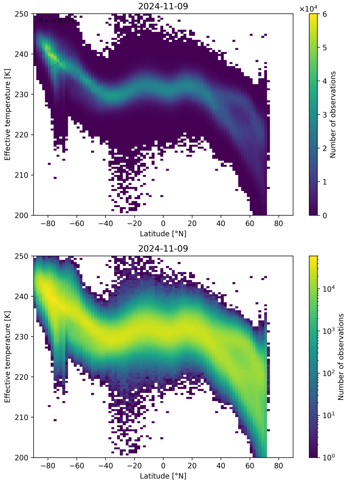
Figure 34: Scatter density plot of “Latitude” against “Effective temperature” for 2024-11-09 to 2024-11-10.
