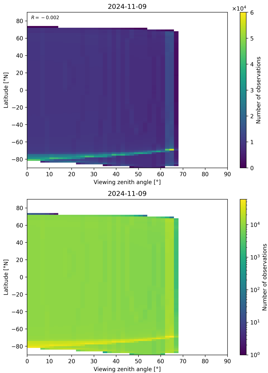
Figure 49: Scatter density plot of “Viewing zenith angle” against “Latitude” for 2024-11-09 to 2024-11-10.
