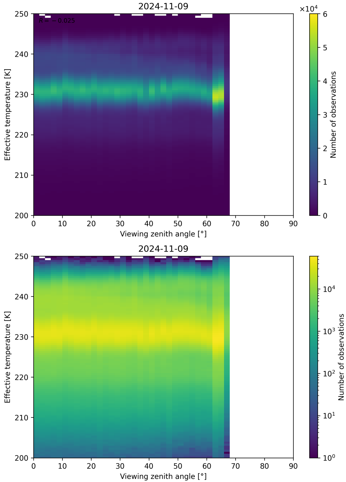
Figure 50: Scatter density plot of “Viewing zenith angle” against “Effective temperature” for 2024-11-09 to 2024-11-10.
