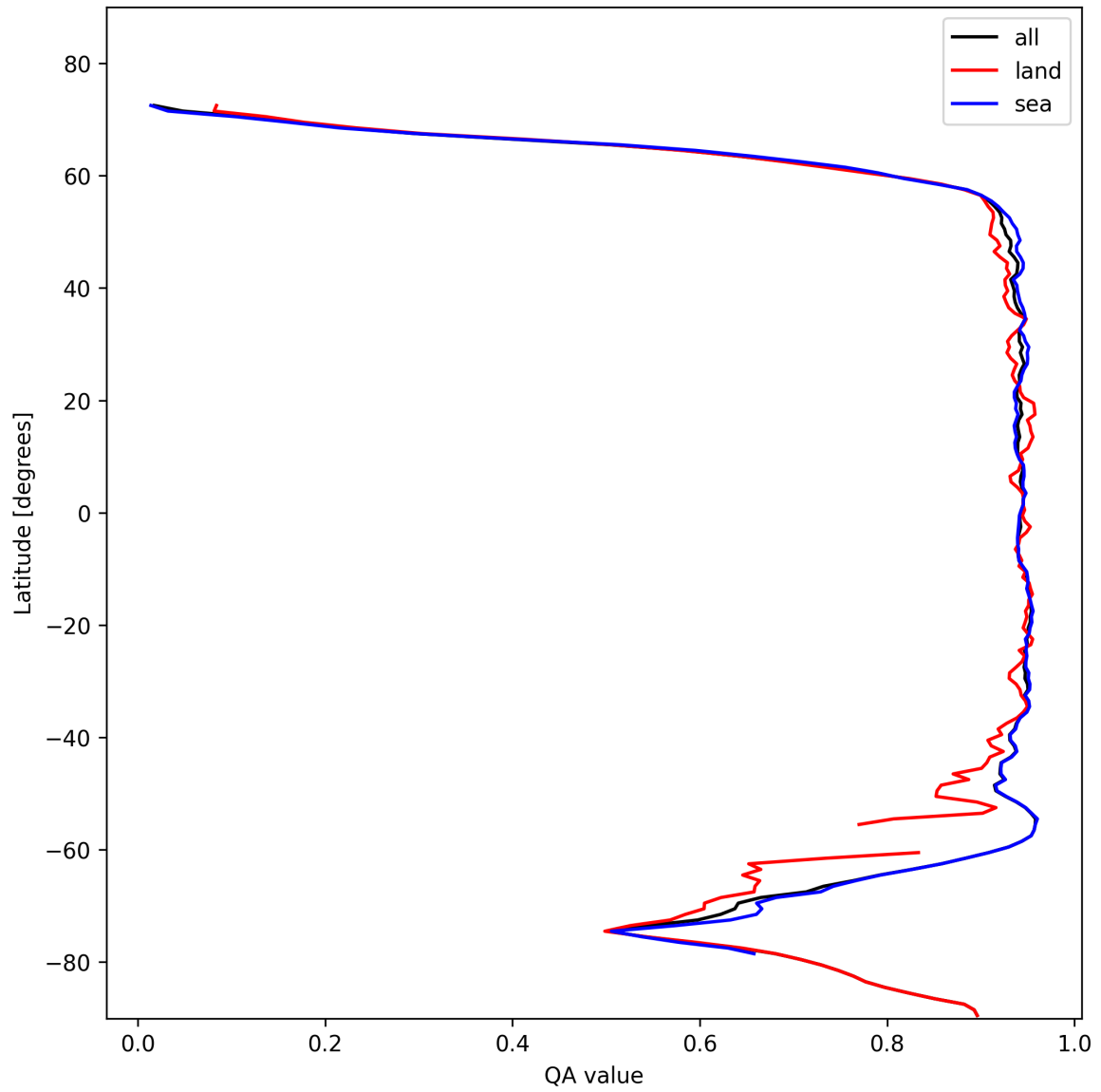
Figure 13: Zonal average of “QA value” for 2024-11-09 to 2024-11-10.
