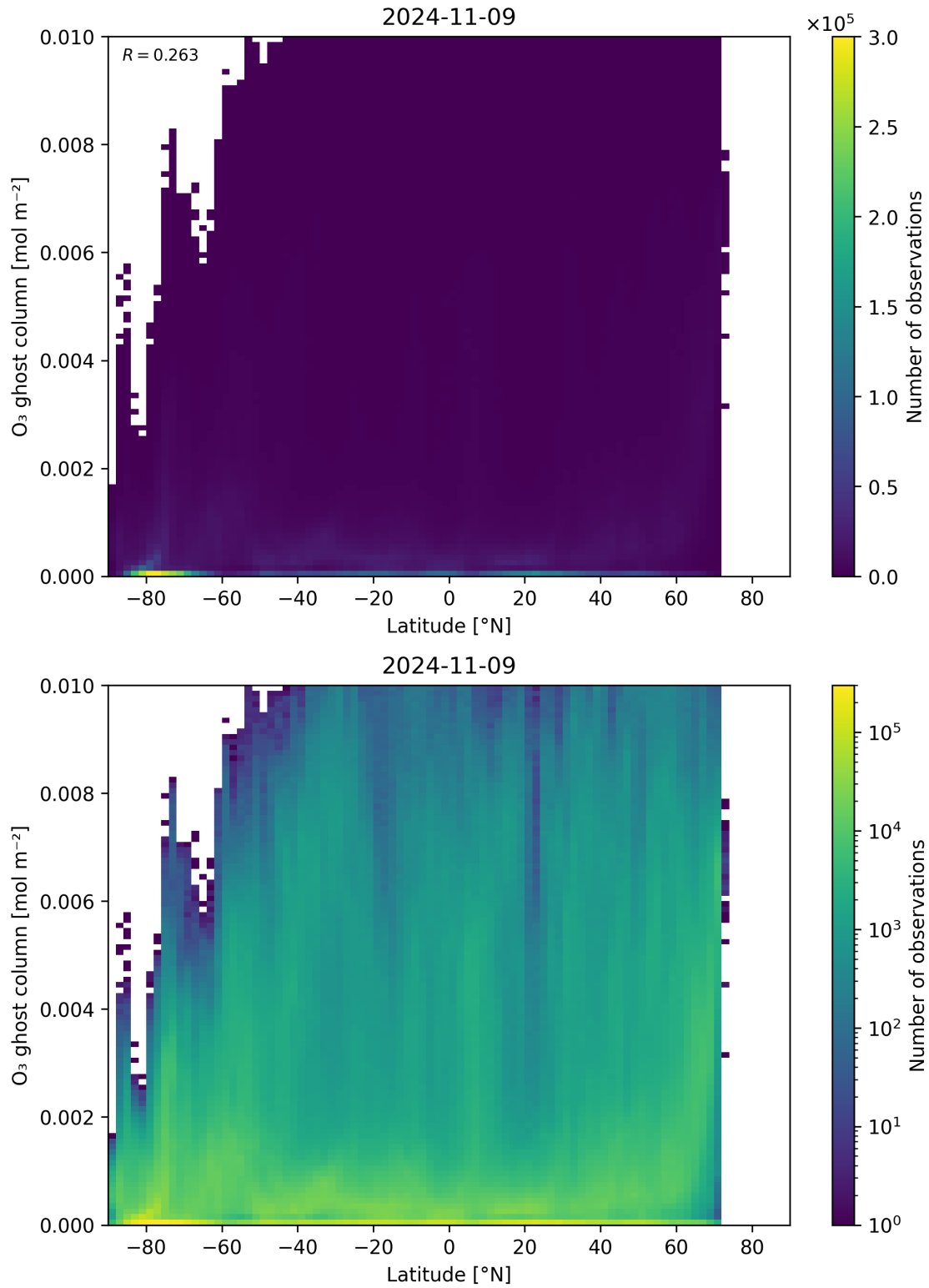
Figure 35: Scatter density plot of “Latitude” against “O 3 ghost column” for 2024-11-09 to 2024-11-10.
