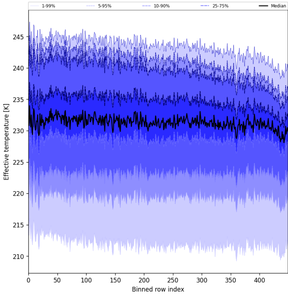
Figure 31: Along track statistics of “Effective temperature” for 2024-11-09 to 2024-11-10
