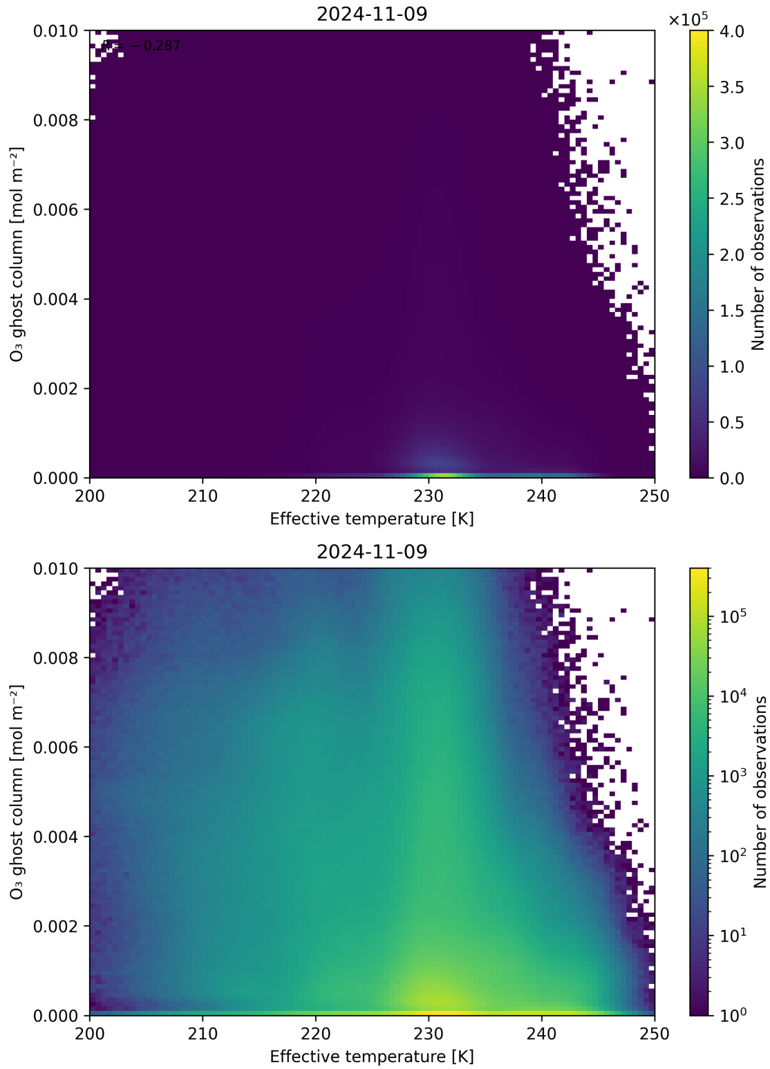
Figure 38: Scatter density plot of “Effective temperature” against “O 3 ghost column” for 2024-11-09 to 2024-11-10.
