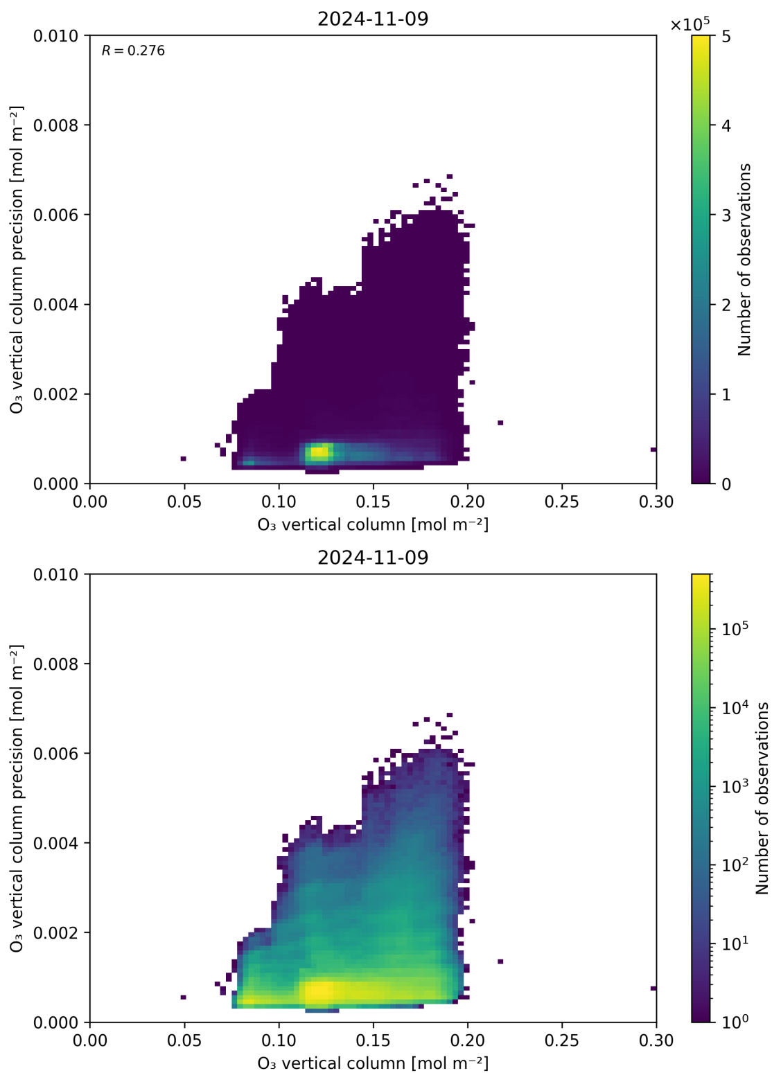
Figure 41: Scatter density plot of “O 3 vertical column” against “O 3 vertical column precision” for 2024-11-09 to 2024-11-10.
