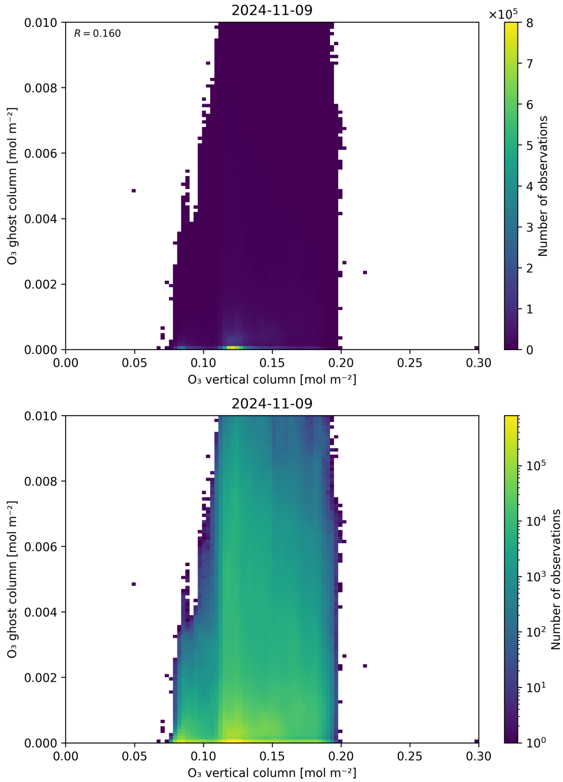
Figure 40: Scatter density plot of “O 3 vertical column” against “O 3 ghost column” for 2024-11-09 to 2024-11-10.
