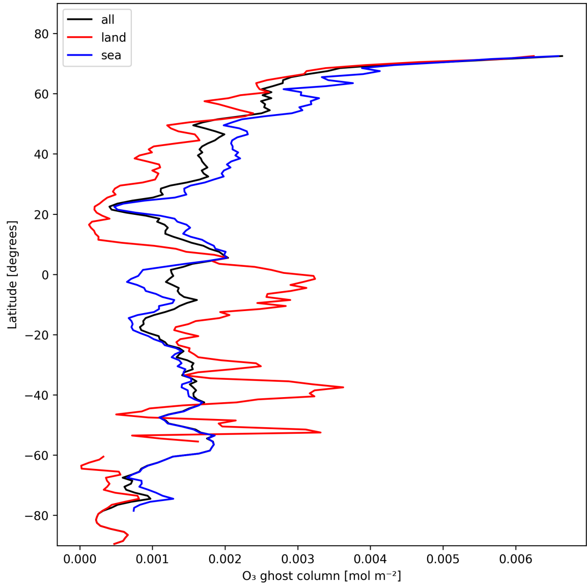
Figure 18: Zonal average of "O 3 ghost column" for 2024-11-09 to 2024-11-10.
