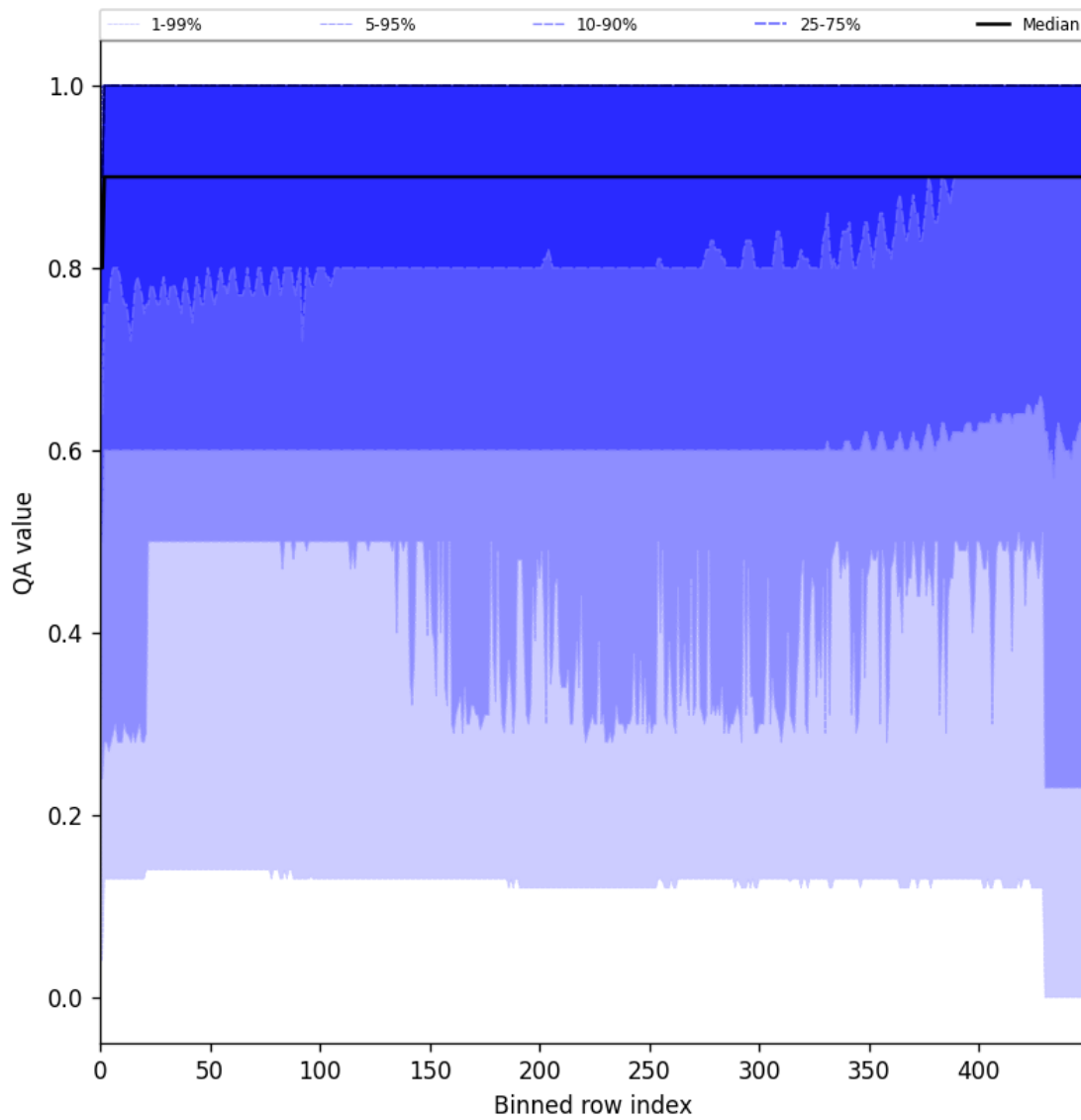
Figure 27: Along track statistics of “QA value” for 2024-11-09 to 2024-11-10
