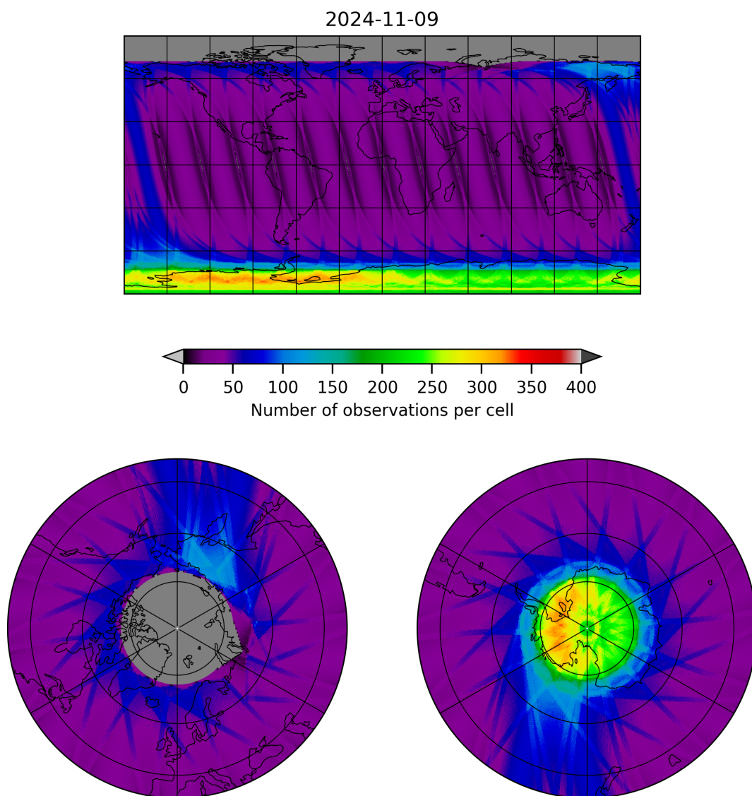
Figure 12: Map of the number of observations for 2024-11-09 to 2024-11-10
