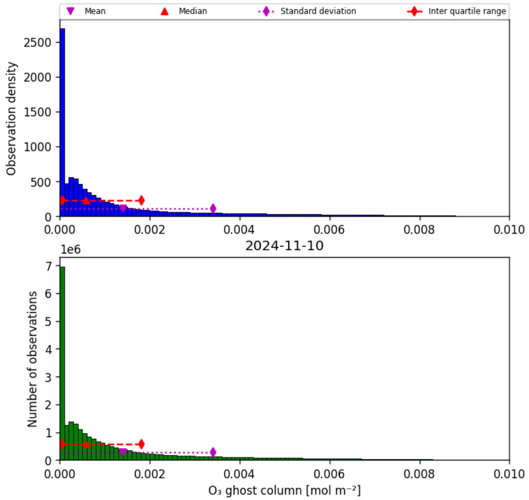
Figure 25: Histogram of “O 3 ghost column” for 2024-11-09 to 2024-11-11
