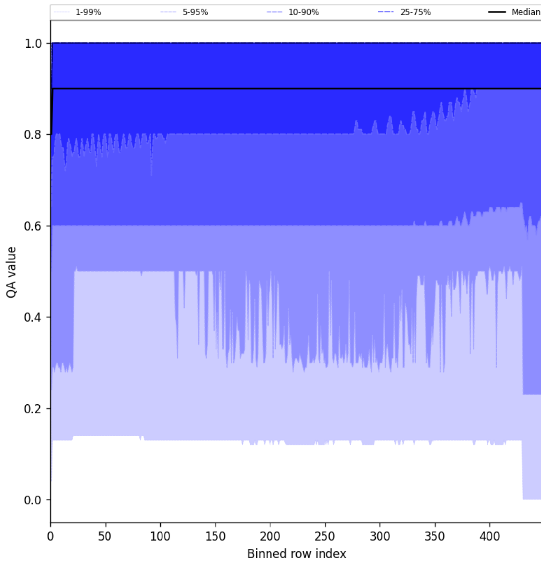
Figure 27: Along track statistics of “QA value” for 2024-11-09 to 2024-11-11
