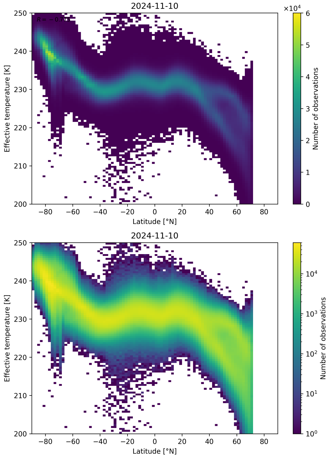
Figure 34: Scatter density plot of “Latitude” against “Effective temperature” for 2024-11-09 to 2024-11-11.
