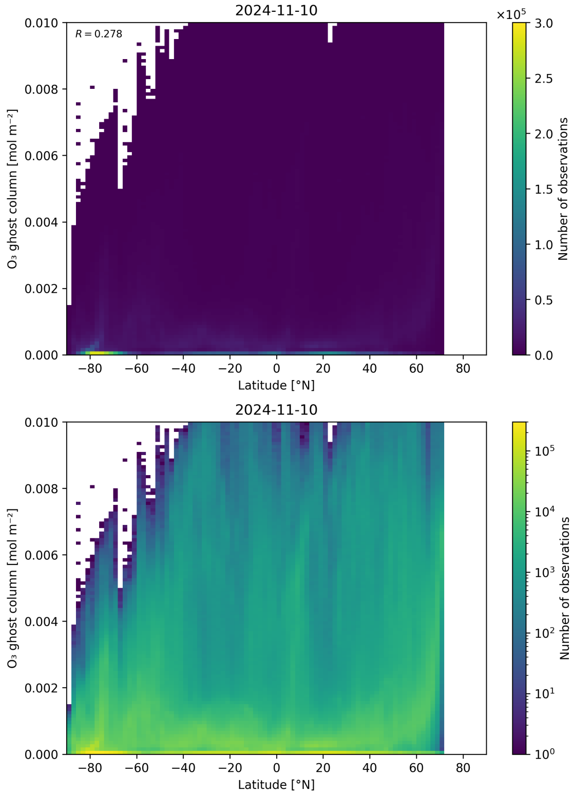
Figure 35: Scatter density plot of “Latitude” against “O 3 ghost column” for 2024-11-09 to 2024-11-11.
