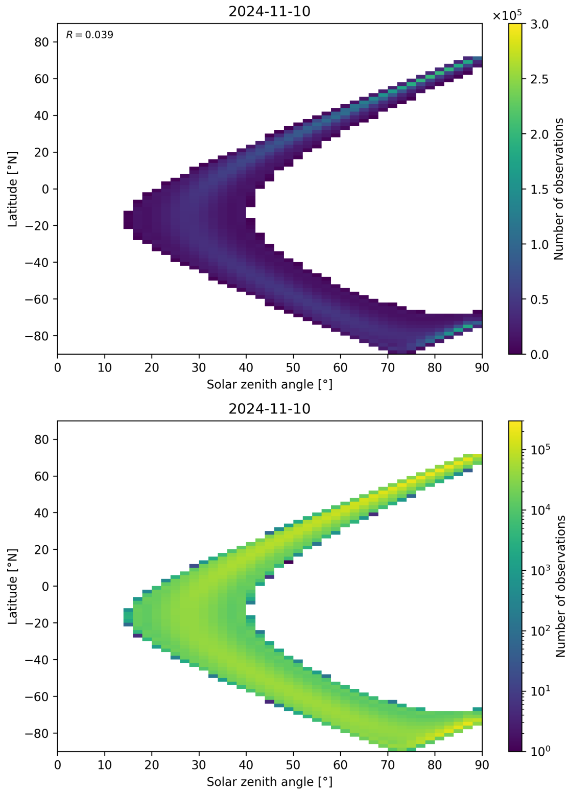
Figure 44: Scatter density plot of “Solar zenith angle” against “Latitude” for 2024-11-09 to 2024-11-11.
