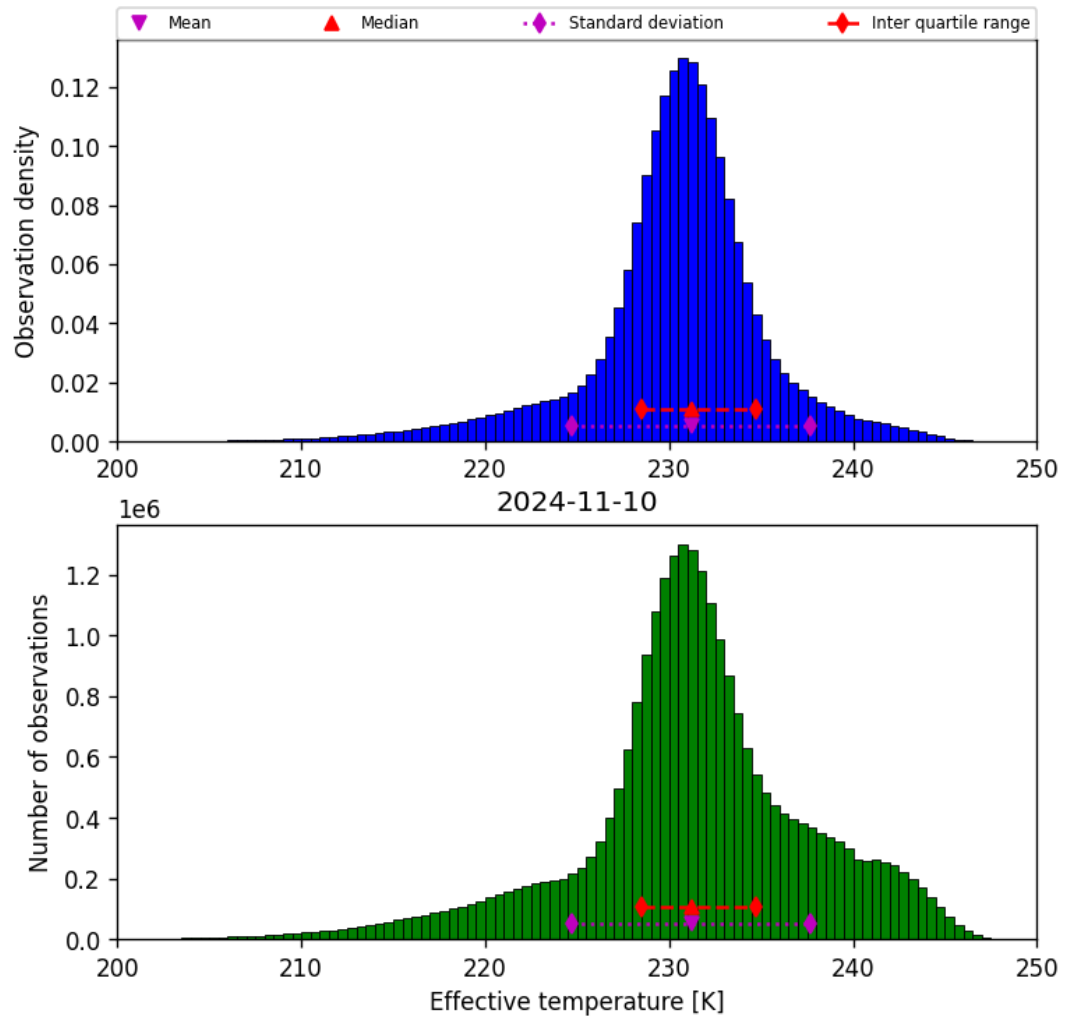
Figure 24: Histogram of “Effective temperature” for 2024-11-09 to 2024-11-11
