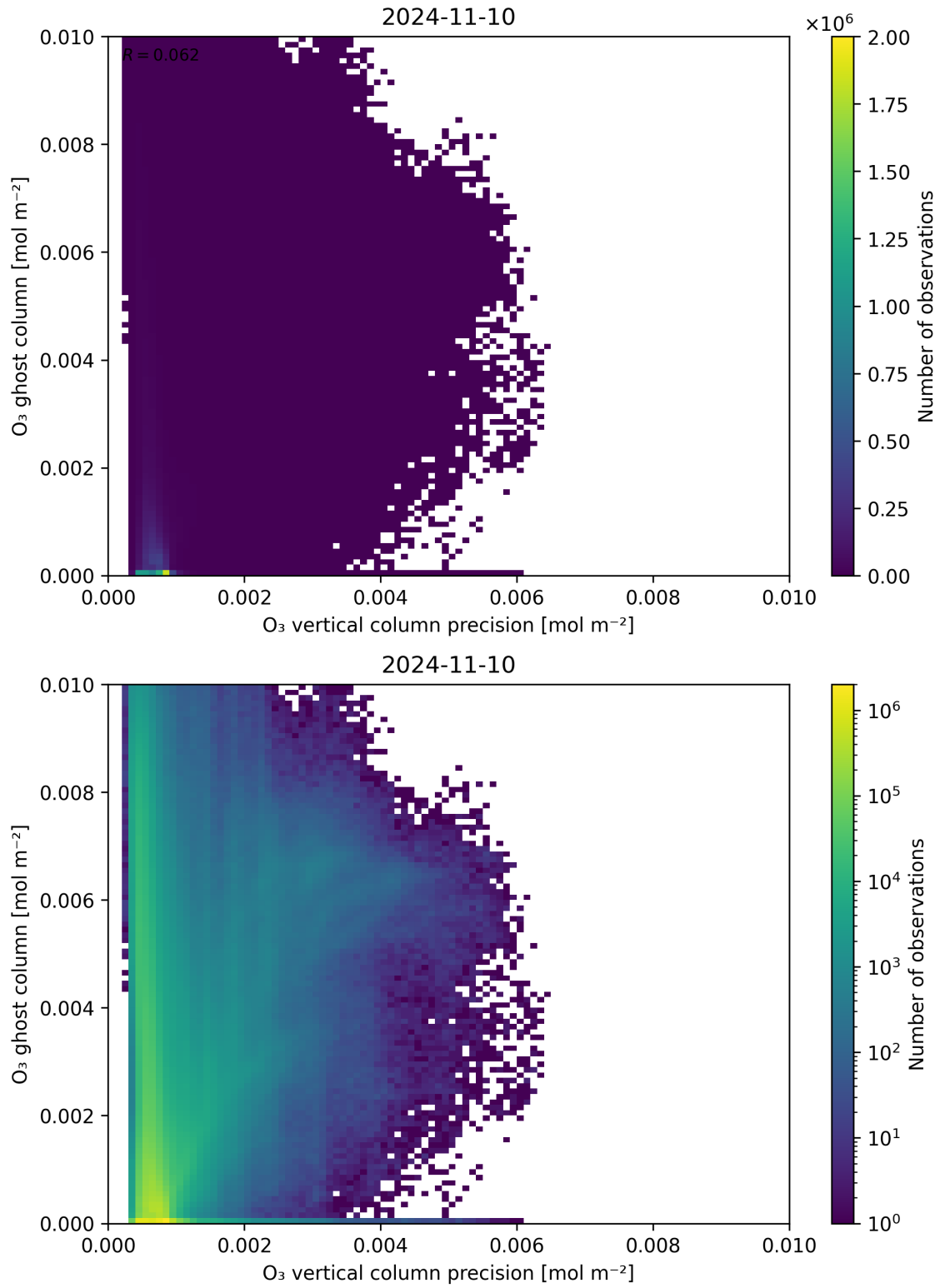
Figure 43: Scatter density plot of “O 3 vertical column precision” against “O 3 ghost column” for 2024-11-09 to 2024-11-11.
