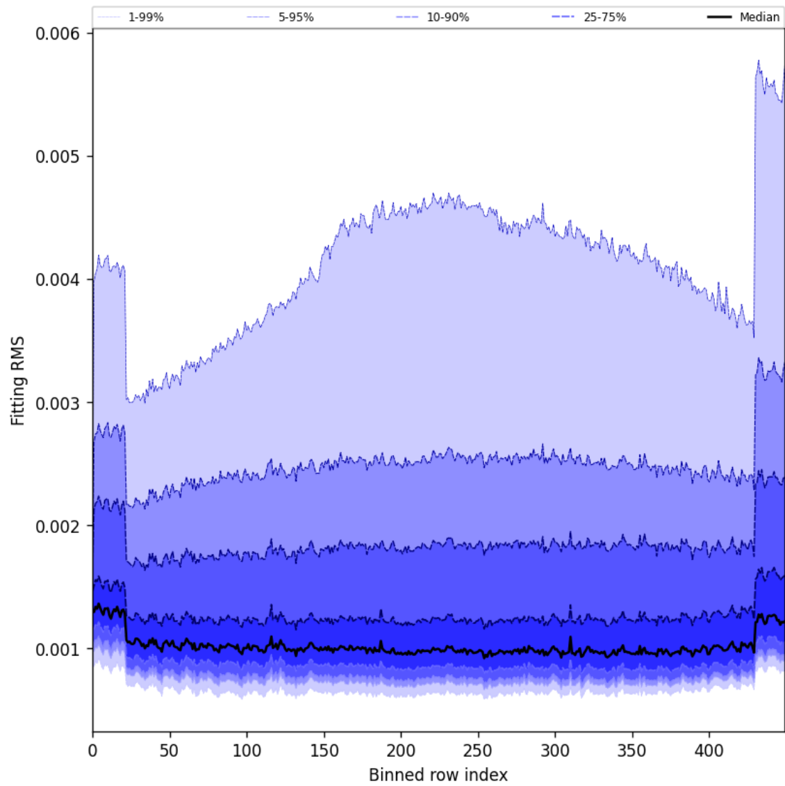
Figure 30: Along track statistics of “Fitting RMS” for 2024-11-09 to 2024-11-11
