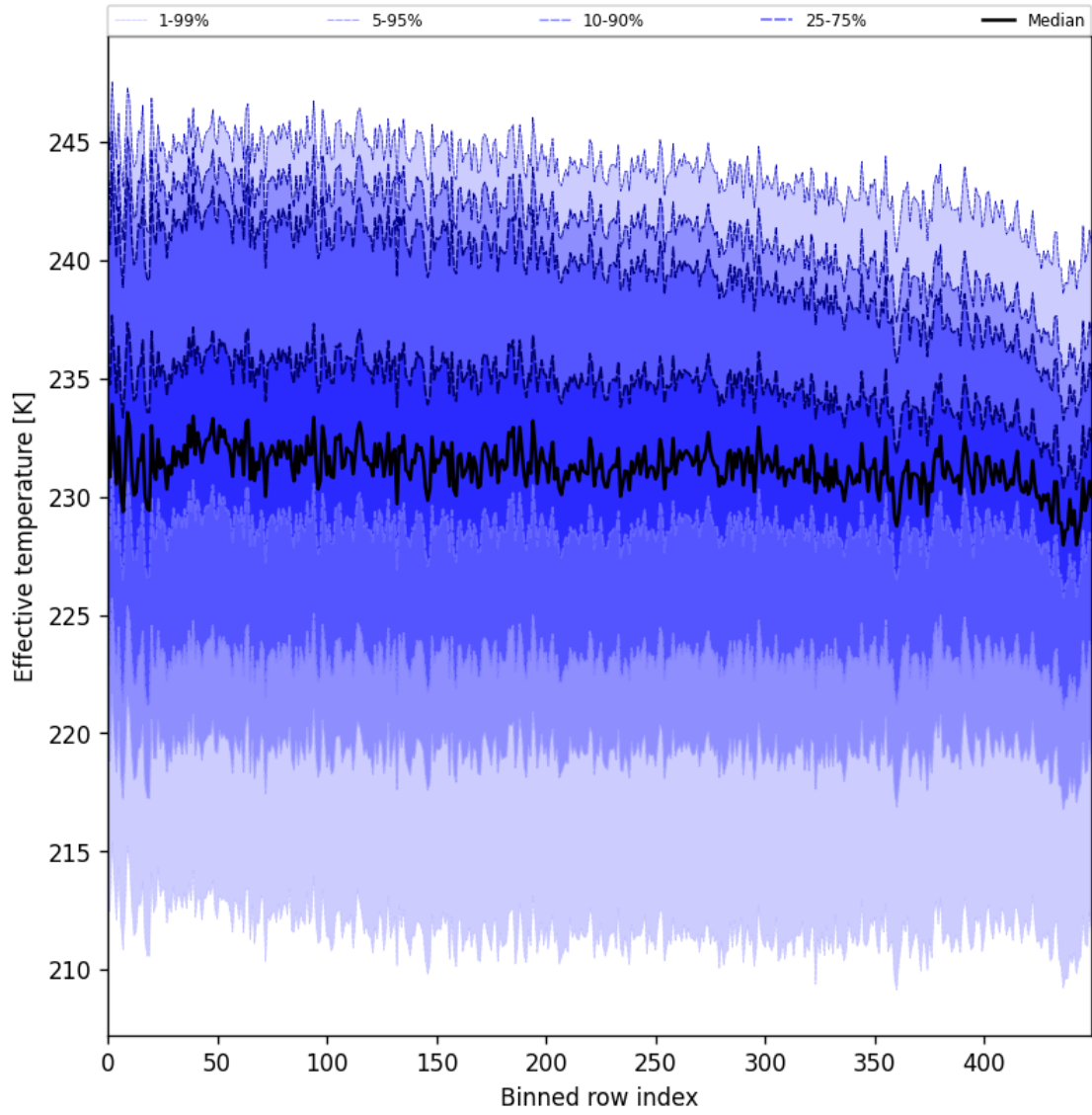
Figure 31: Along track statistics of “Effective temperature” for 2024-11-09 to 2024-11-11
