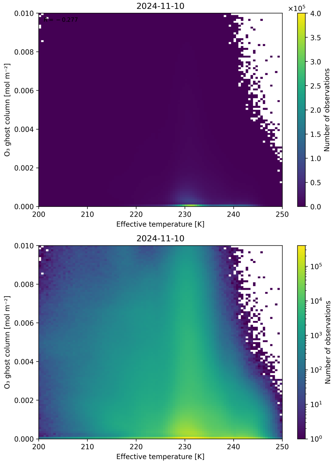
Figure 38: Scatter density plot of “Effective temperature” against “O 3 ghost column” for 2024-11-09 to 2024-11-11.
