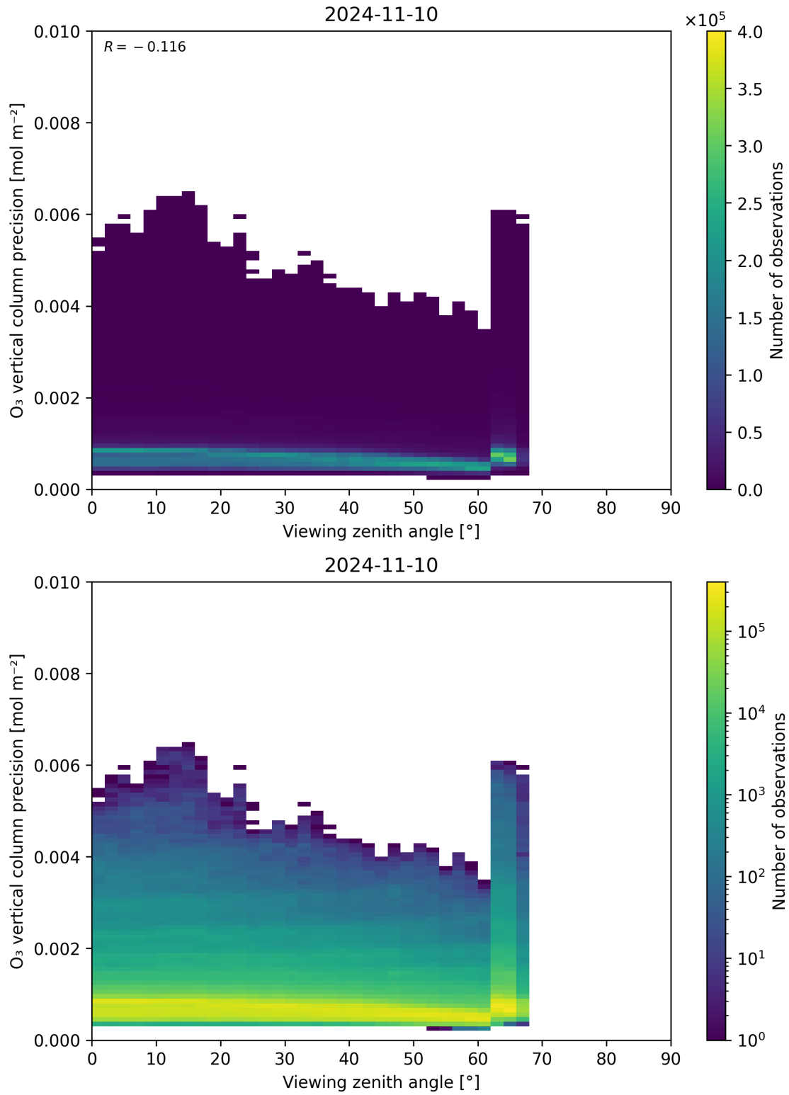
Figure 53: Scatter density plot of “Viewing zenith angle” against “O 3 vertical column precision” for 2024-11-09 to 2024-11-11.
