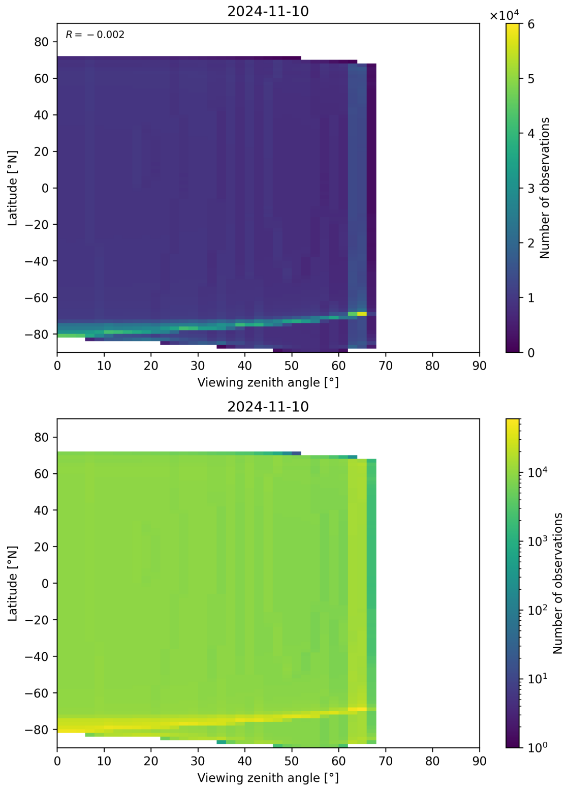
Figure 49: Scatter density plot of “Viewing zenith angle” against “Latitude” for 2024-11-09 to 2024-11-11.
