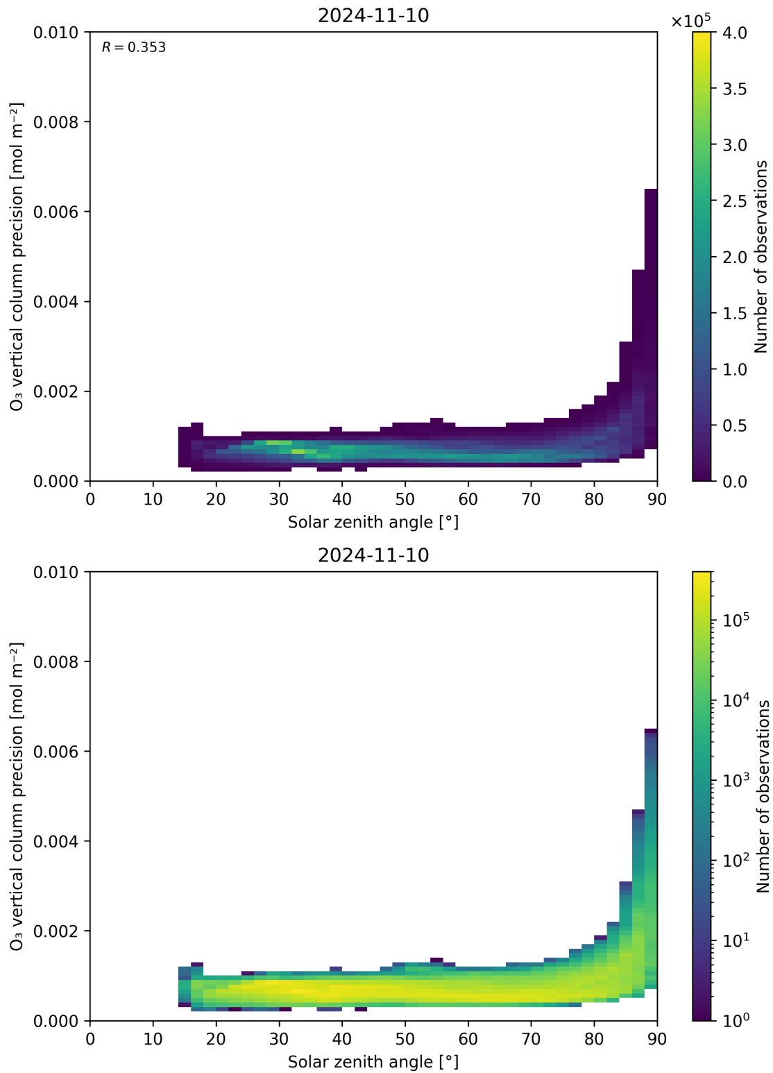
Figure 48: Scatter density plot of “Solar zenith angle” against “O 3 vertical column precision” for 2024-11-09 to 2024-11-11.
