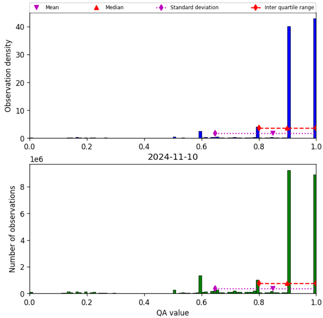
Figure 20: Histogram of “QA value” for 2024-11-09 to 2024-11-11
