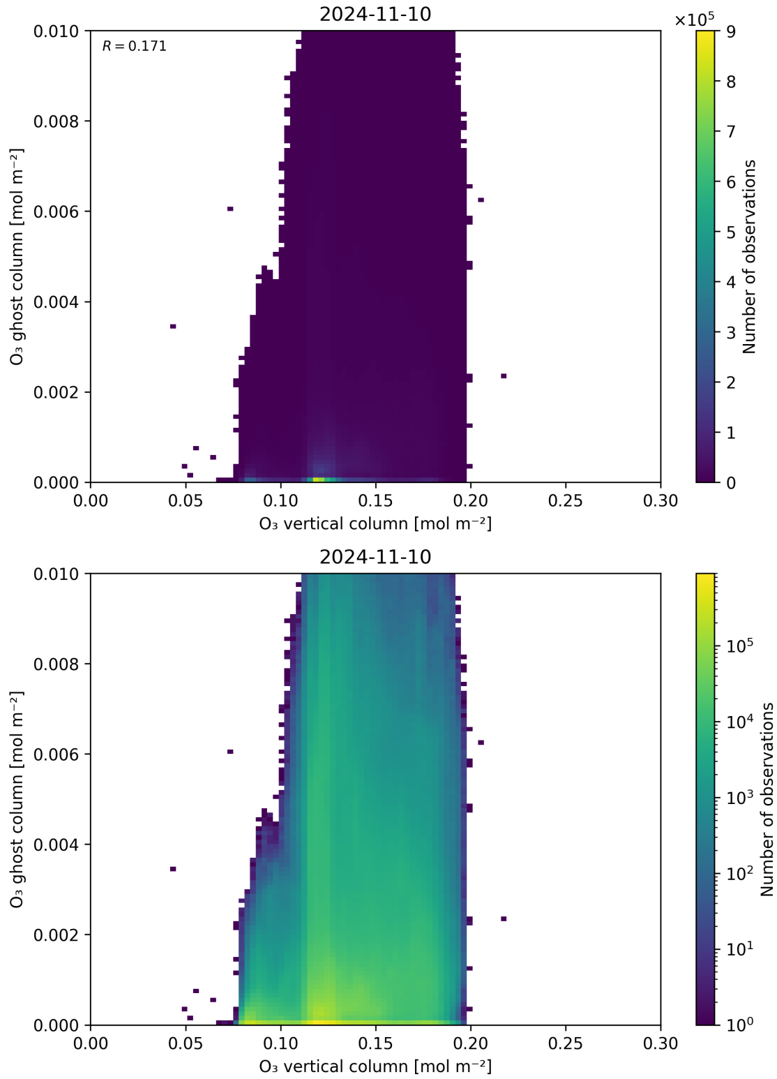
Figure 40: Scatter density plot of “O 3 vertical column” against “O 3 ghost column” for 2024-11-09 to 2024-11-11.
