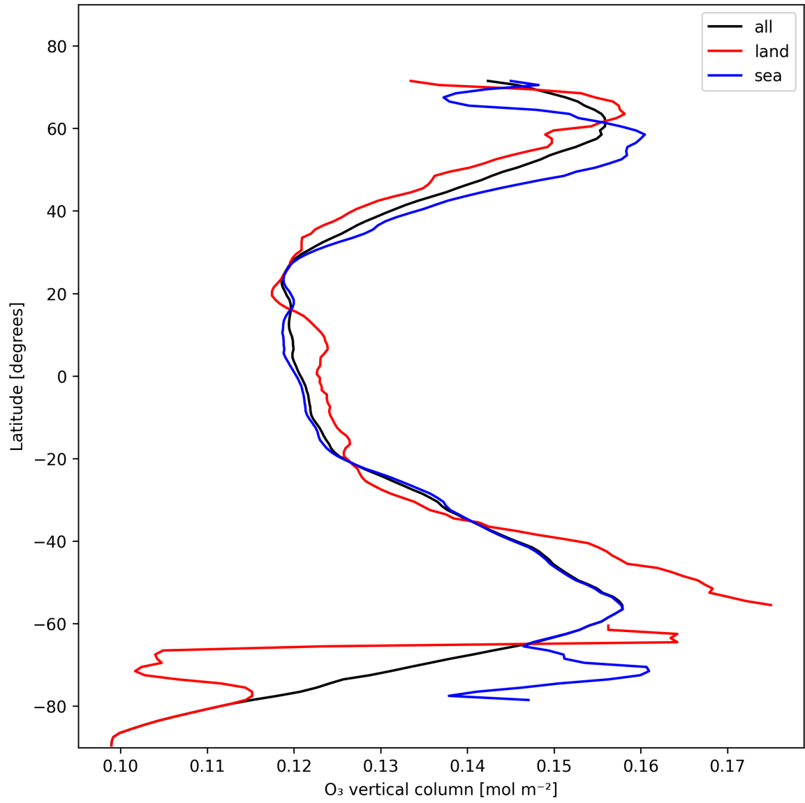
Figure 14: Zonal average of “O 3 vertical column” for 2024-11-09 to 2024-11-11.
