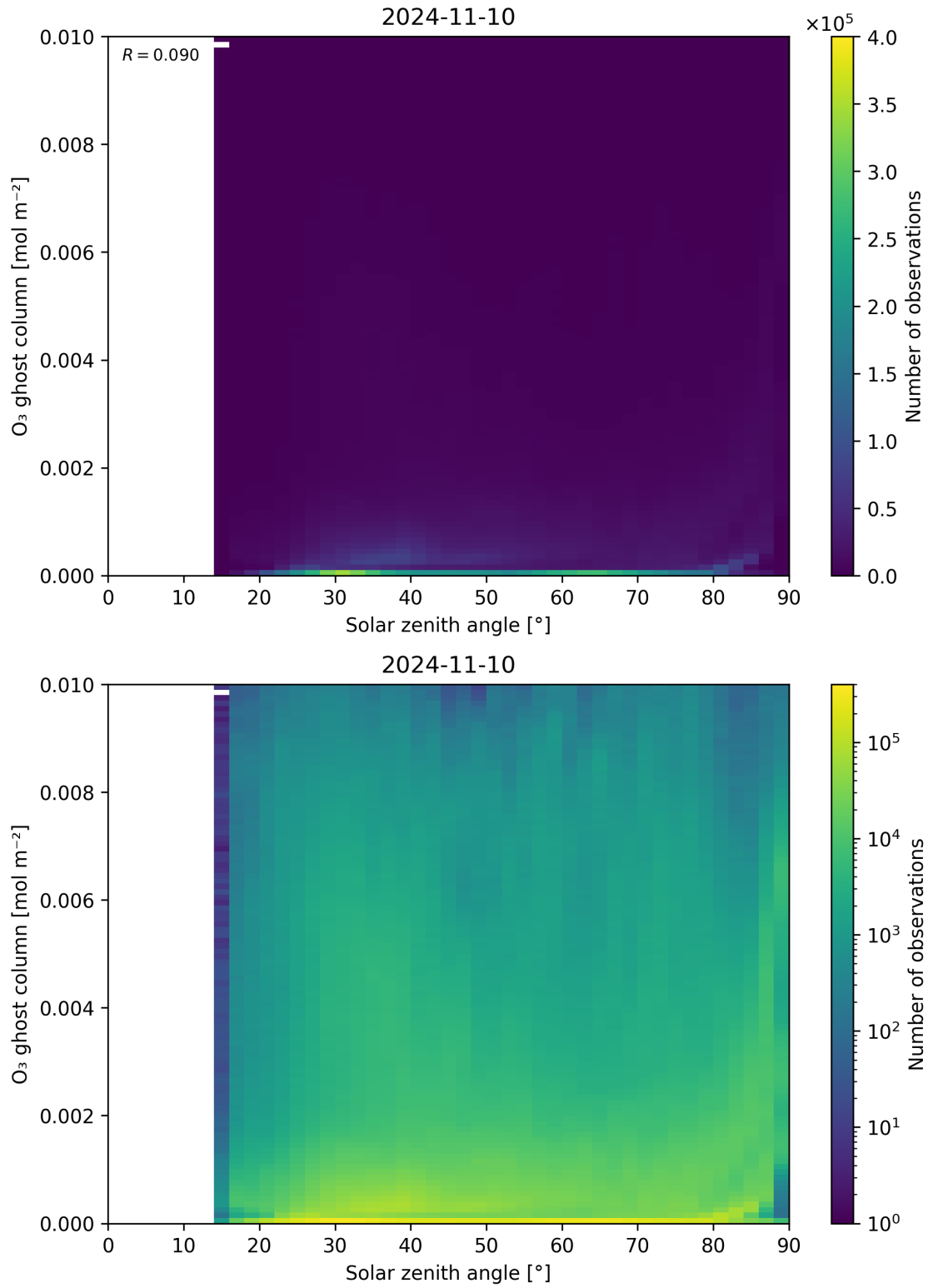
Figure 46: Scatter density plot of “Solar zenith angle” against “O 3 ghost column” for 2024-11-09 to 2024-11-11.
