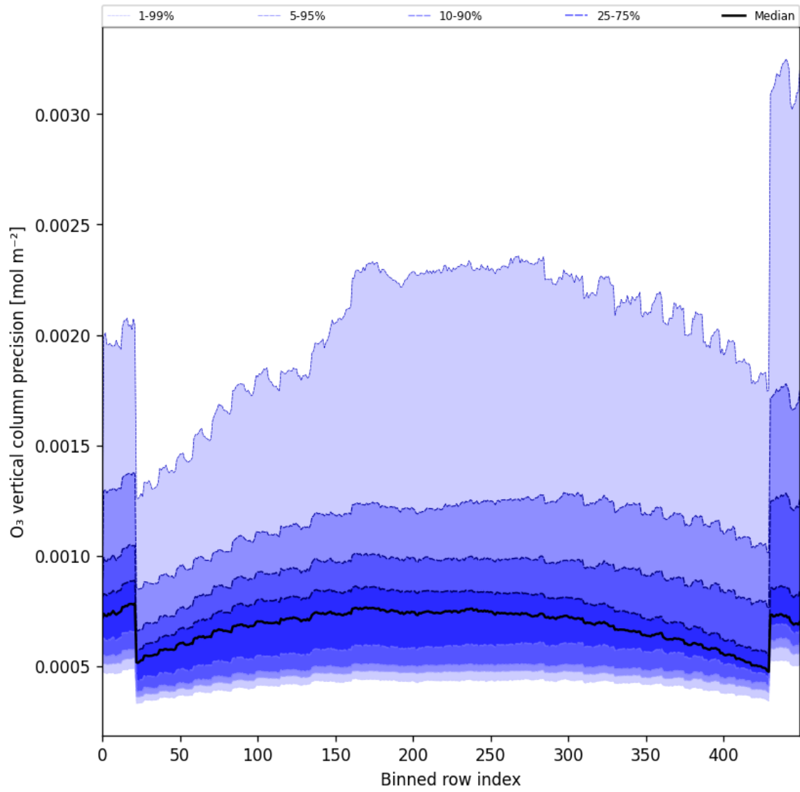
Figure 29: Along track statistics of “O 3 vertical column precision” for 2024-11-09 to 2024-11-11
