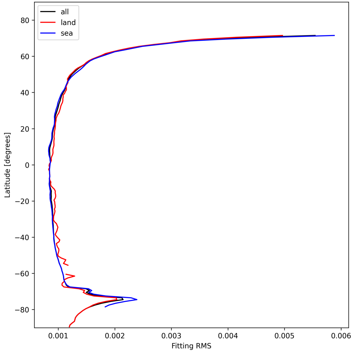
Figure 16: Zonal average of “Fitting RMS” for 2024-11-09 to 2024-11-11.
