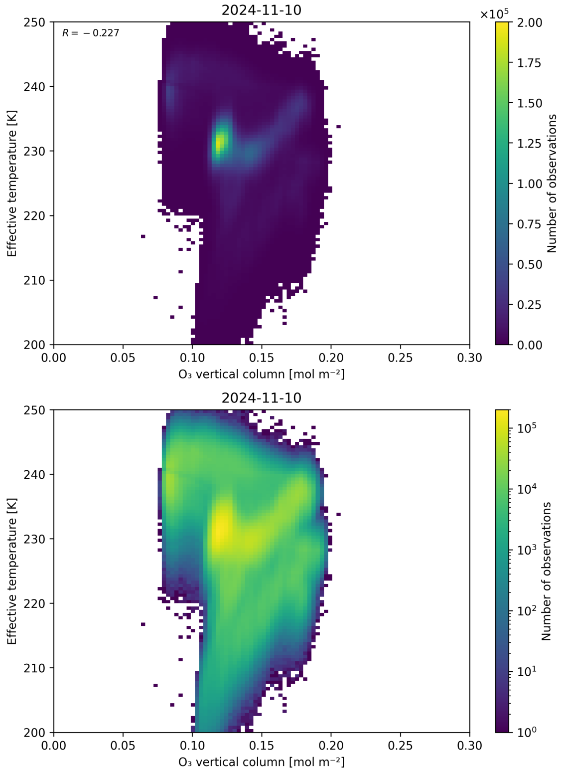
Figure 39: Scatter density plot of “O 3 vertical column” against “Effective temperature” for 2024-11-09 to 2024-11-11.
