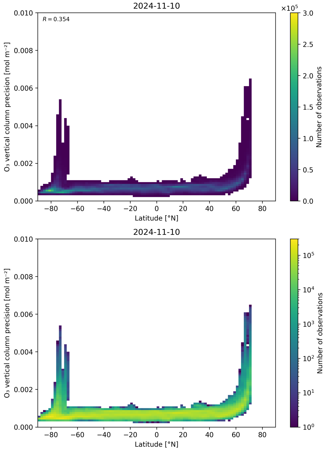
Figure 37: Scatter density plot of “Latitude” against “O 3 vertical column precision” for 2024-11-09 to 2024-11-11.
