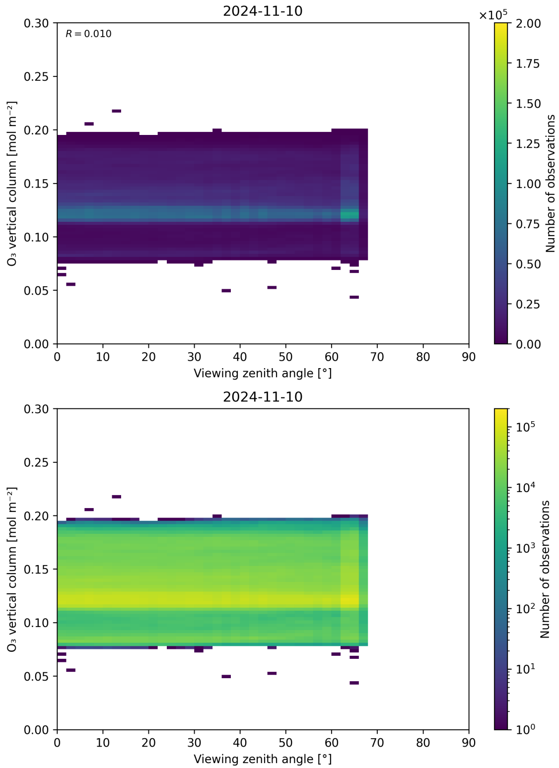
Figure 52: Scatter density plot of “Viewing zenith angle” against “O 3 vertical column” for 2024-11-09 to 2024-11-11.
