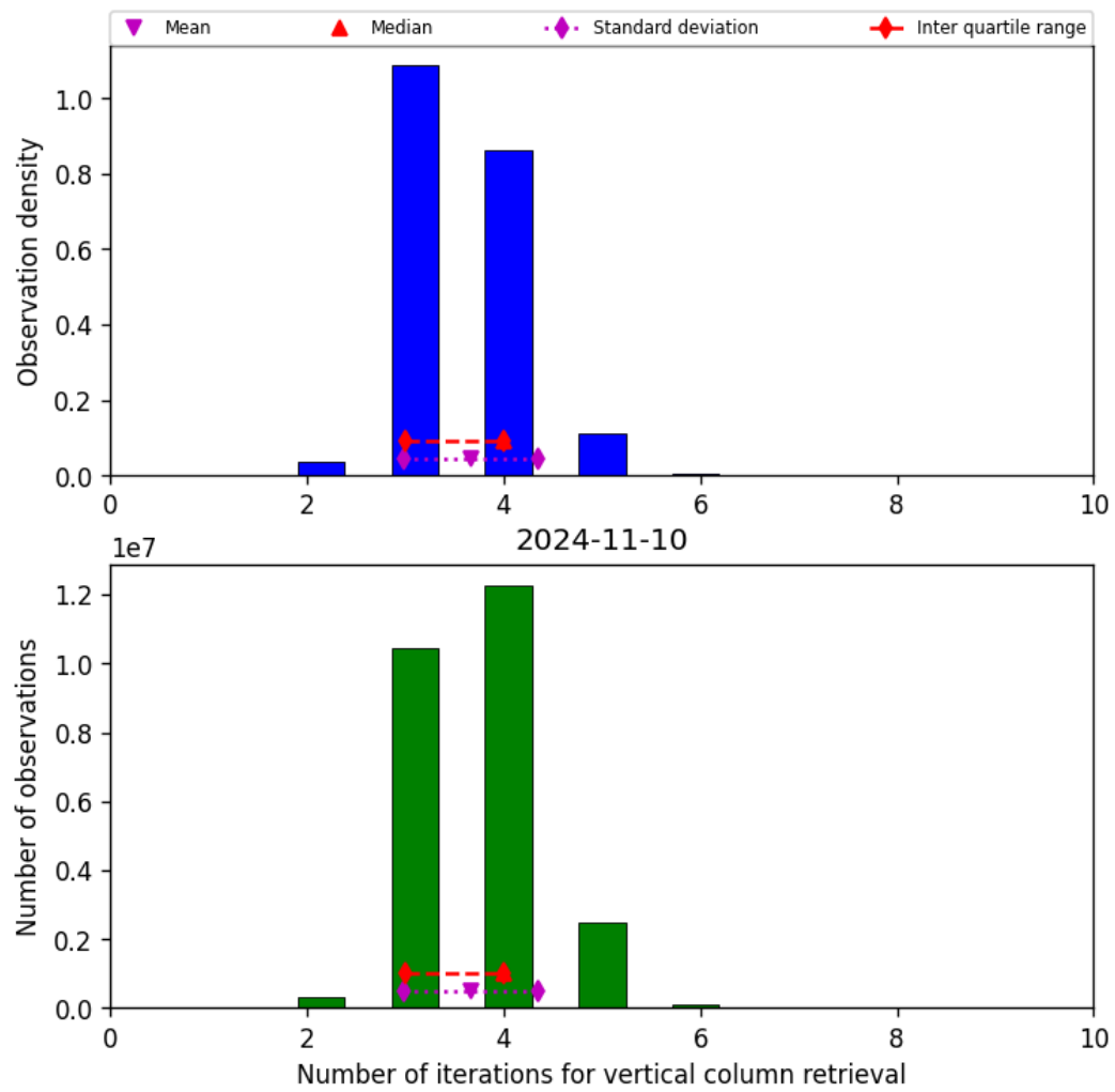
Figure 26: Histogram of “Number of iterations for vertical column retrieval” for 2024-11-09 to 2024-11-11
