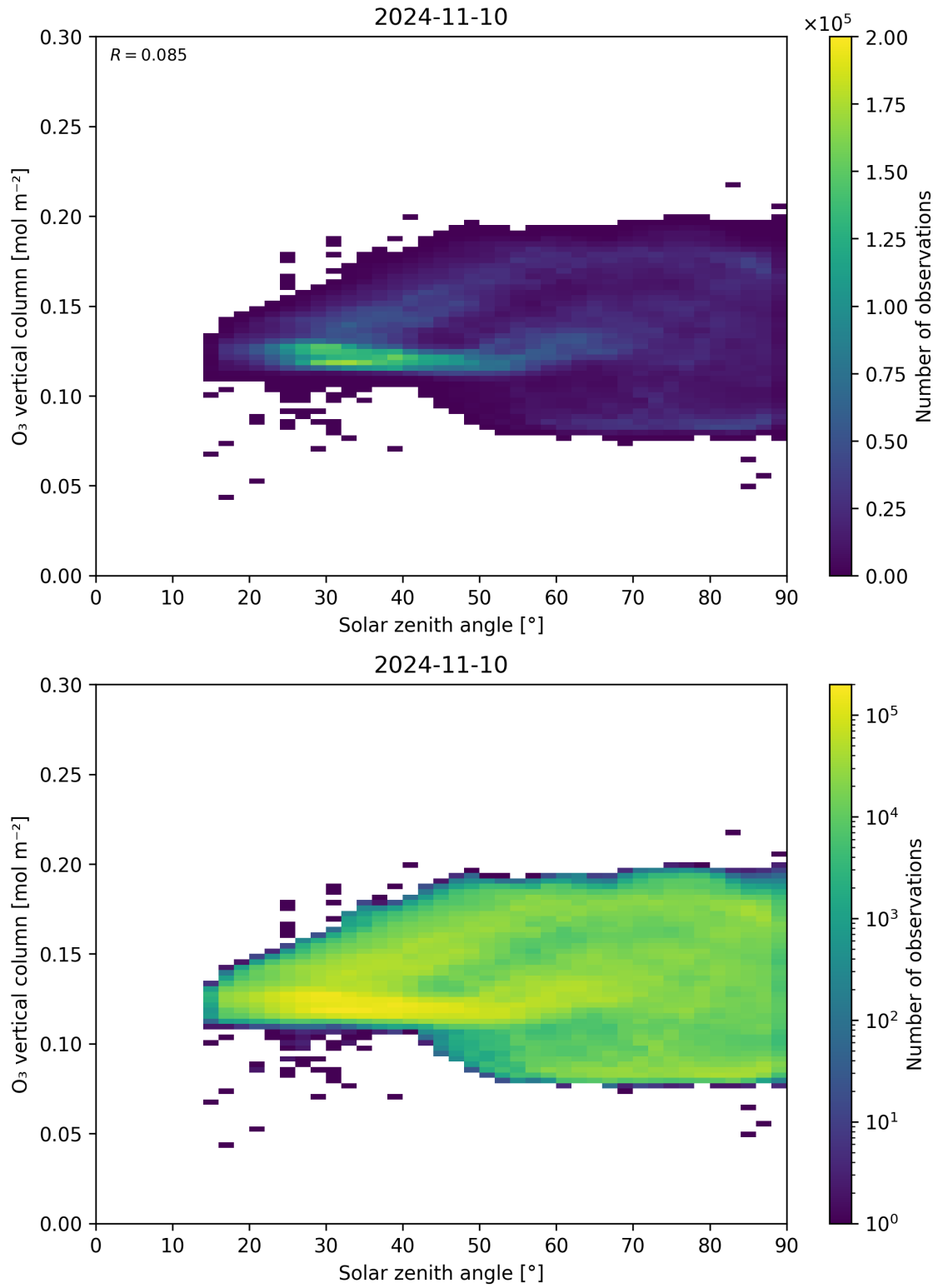
Figure 47: Scatter density plot of “Solar zenith angle” against “O 3 vertical column” for 2024-11-09 to 2024-11-11.
