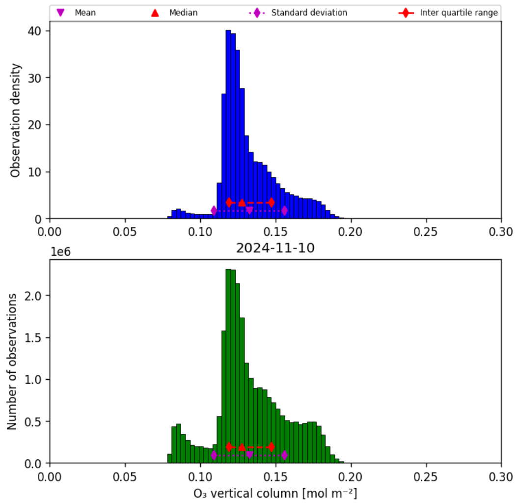
Figure 21: Histogram of “O 3 vertical column” for 2024-11-09 to 2024-11-11
