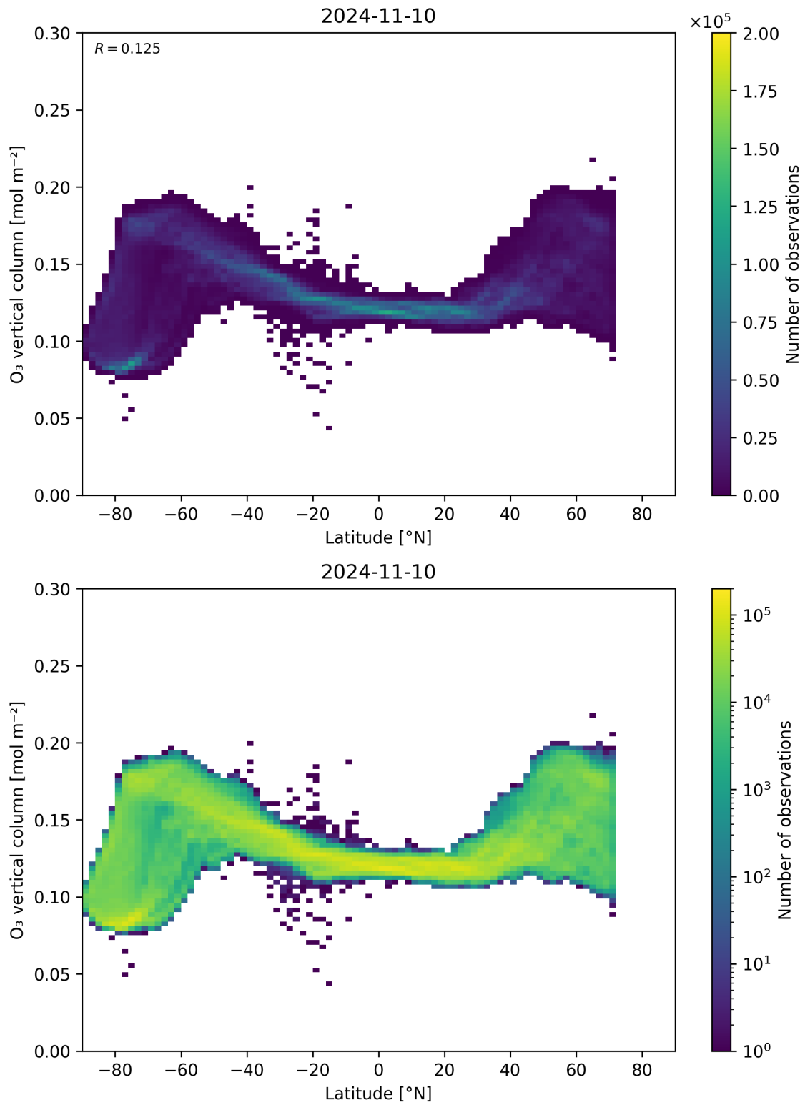
Figure 36: Scatter density plot of “Latitude” against “O 3 vertical column” for 2024-11-09 to 2024-11-11.
