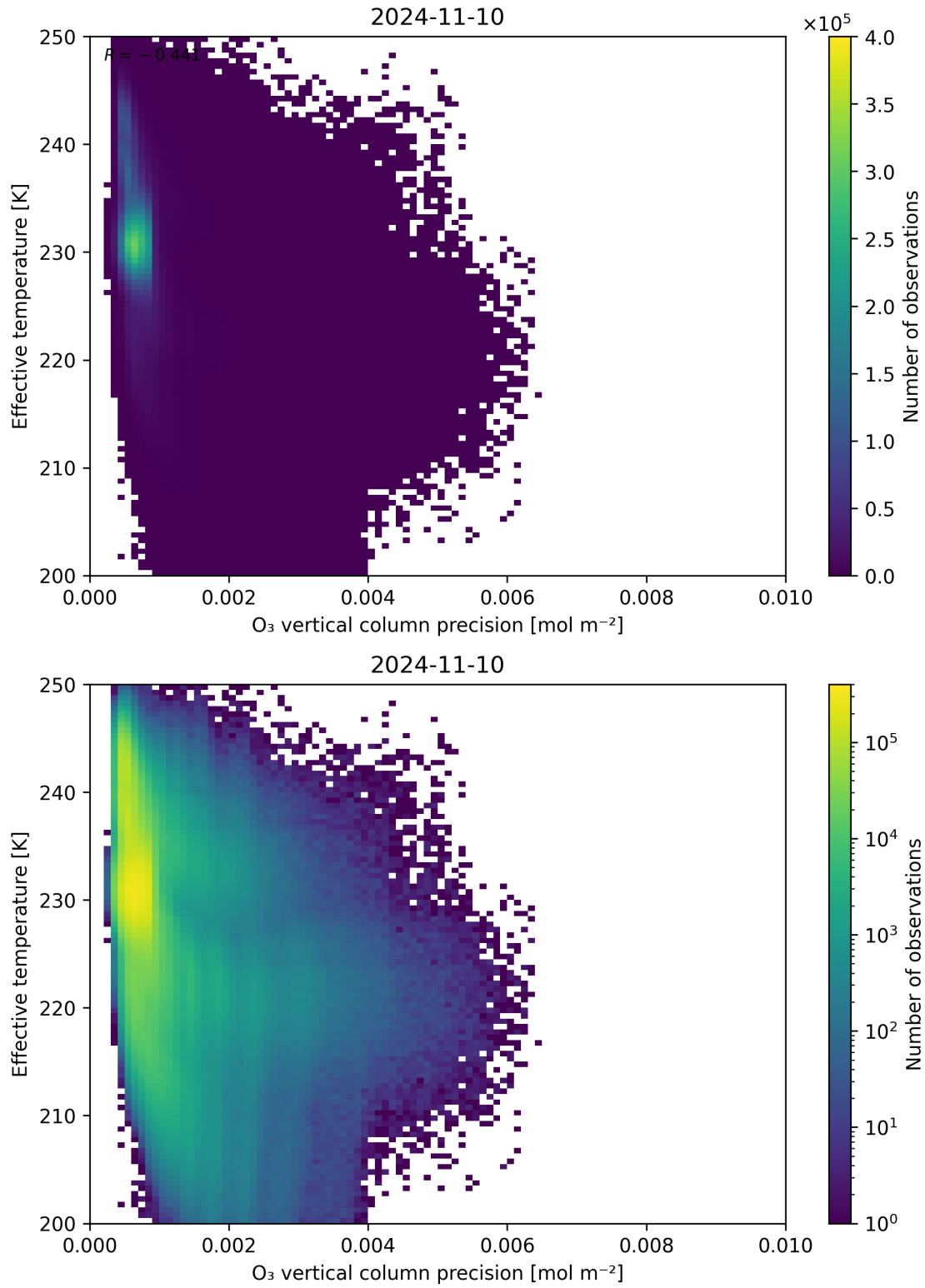
Figure 42: Scatter density plot of “O 3 vertical column precision” against “Effective temperature” for 2024-11-09 to 2024-11-11.
