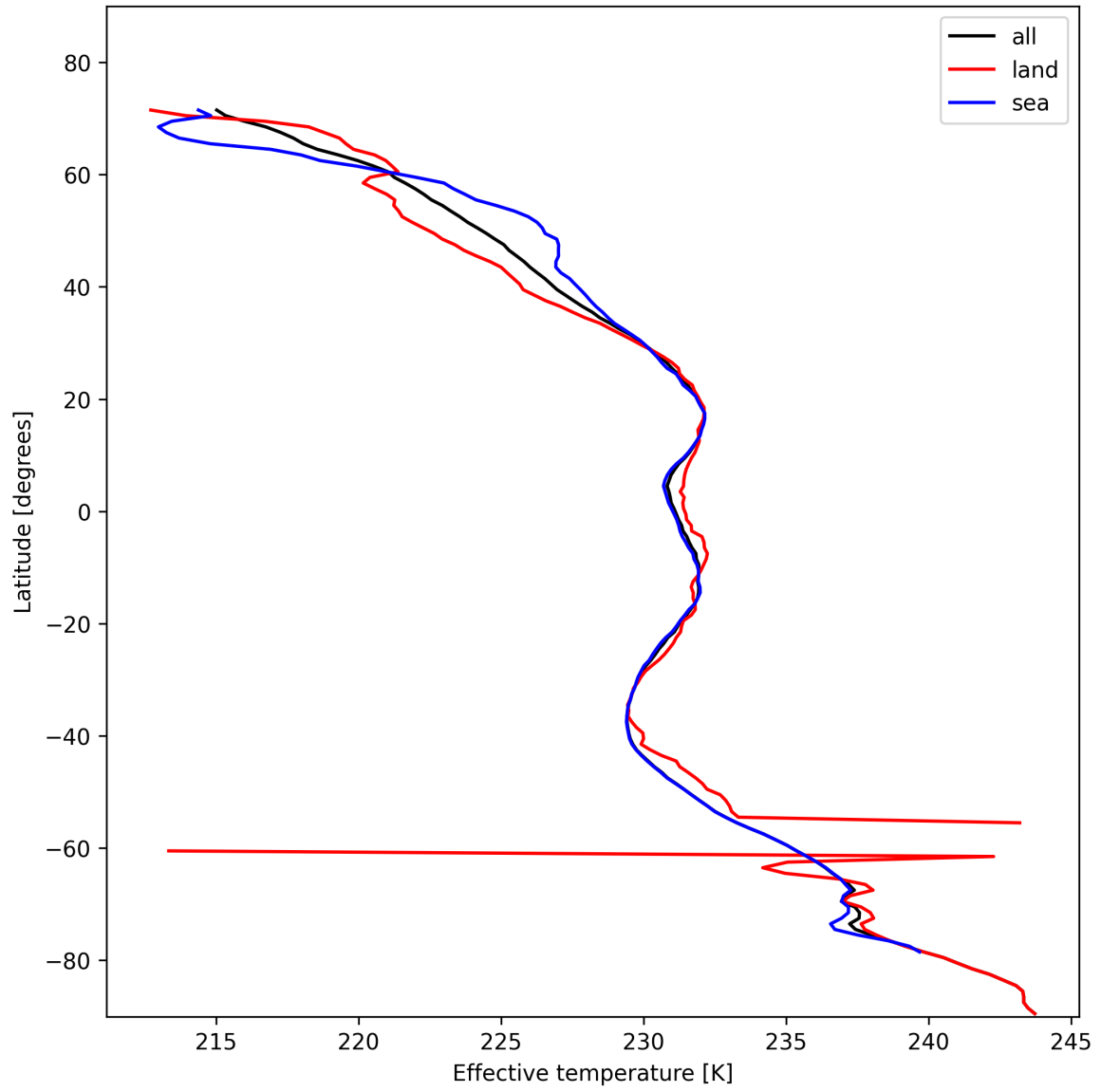
Figure 17: Zonal average of “Effective temperature” for 2024-11-09 to 2024-11-11.
