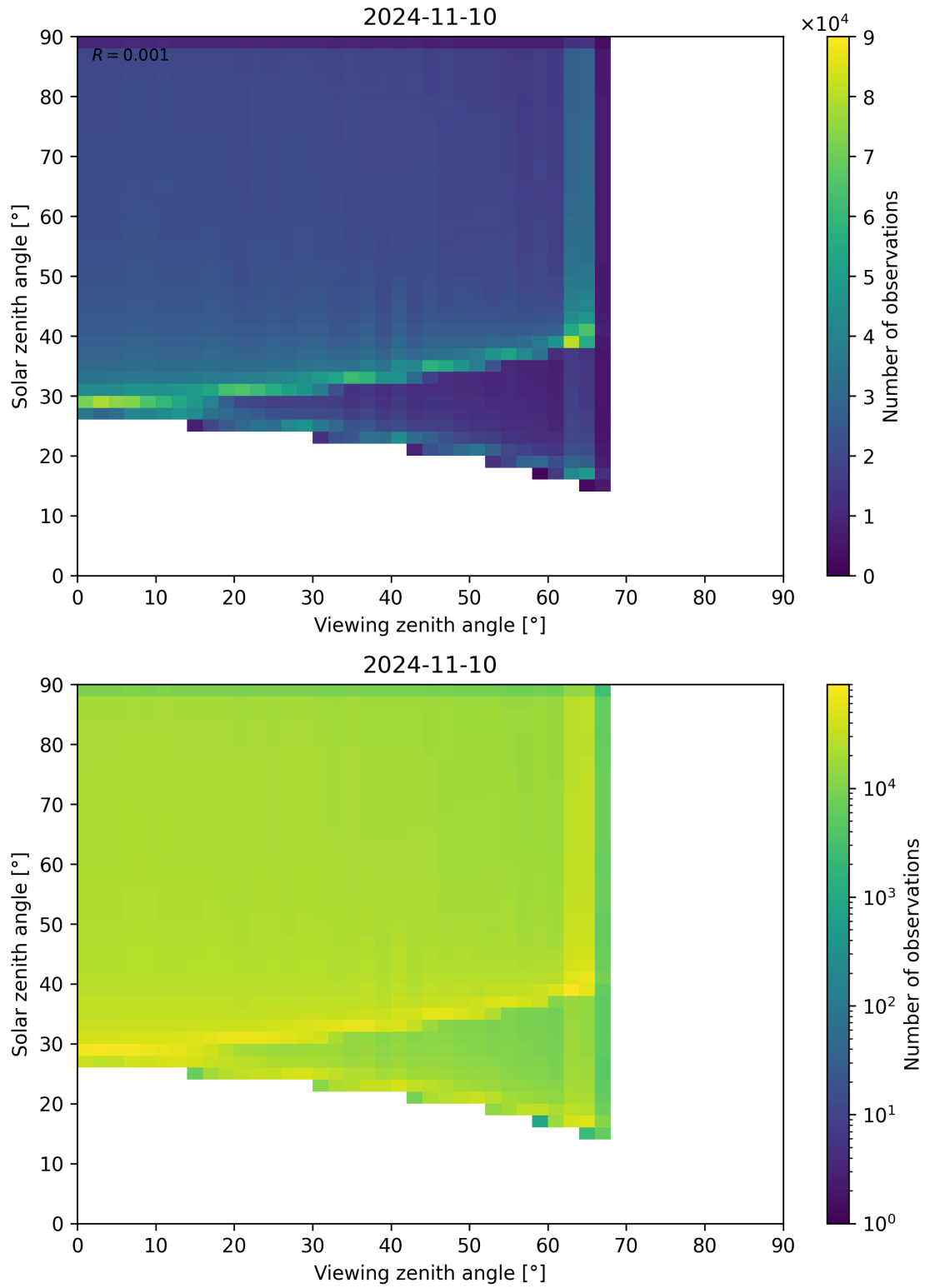
Figure 54: Scatter density plot of “Viewing zenith angle” against “Solar zenith angle” for 2024-11-09 to 2024-11-11.
