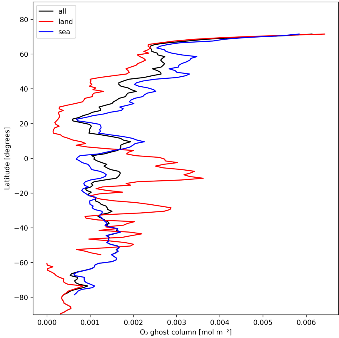
Figure 18: Zonal average of "O 3 ghost column" for 2024-11-09 to 2024-11-11.
