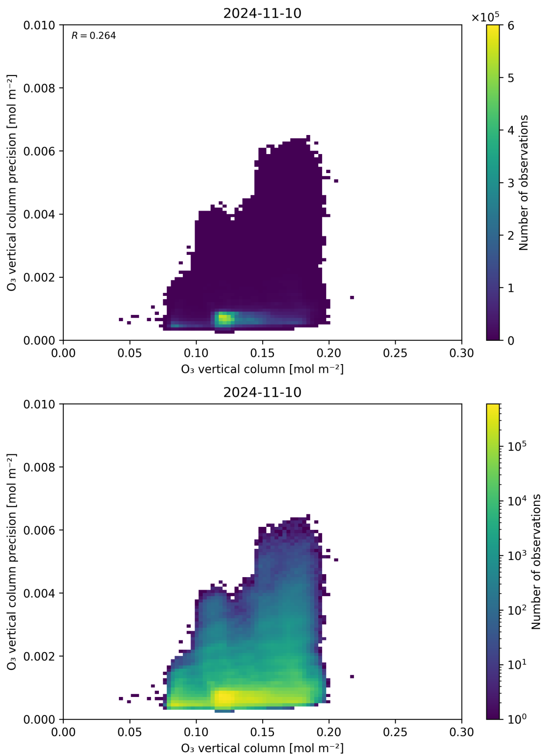
Figure 41: Scatter density plot of “O 3 vertical column” against “O 3 vertical column precision” for 2024-11-09 to 2024-11-11.
