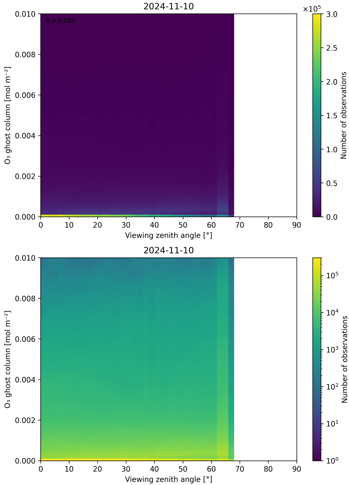
Figure 51: Scatter density plot of “Viewing zenith angle” against “O 3 ghost column” for 2024-11-09 to 2024-11-11.
