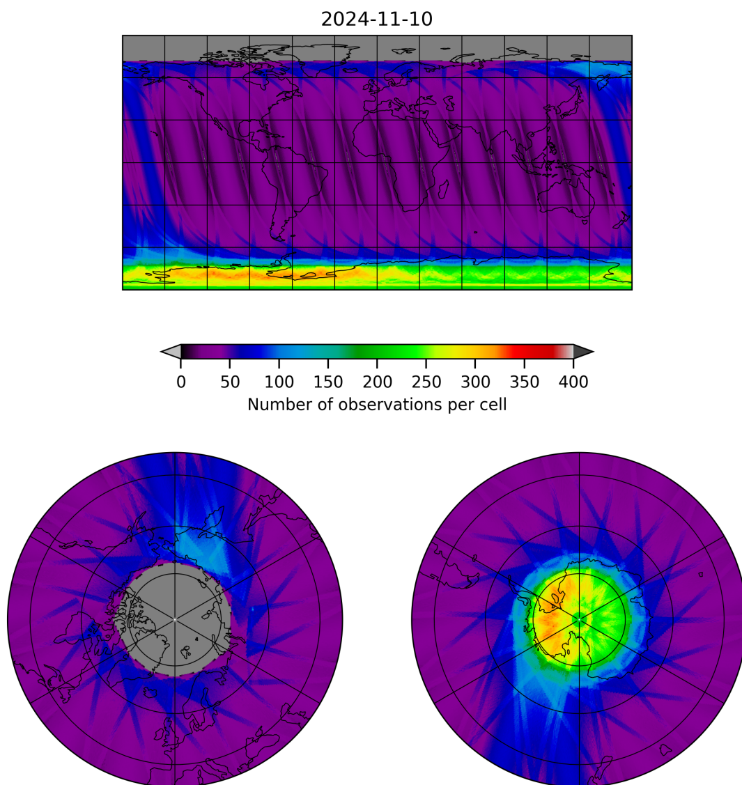
Figure 12: Map of the number of observations for 2024-11-09 to 2024-11-11
