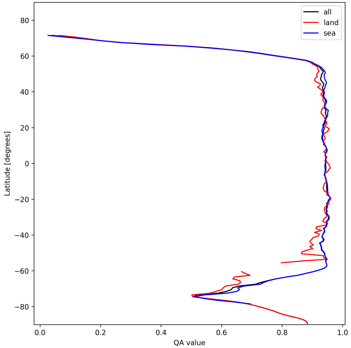
Figure 13: Zonal average of “QA value” for 2024-11-09 to 2024-11-11.
