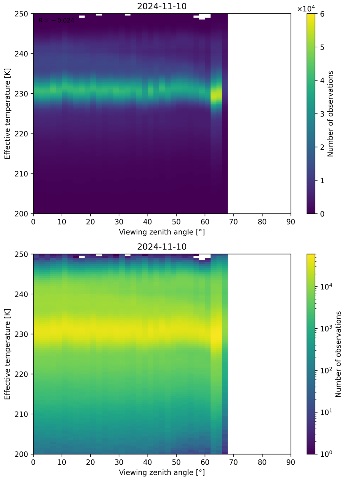
Figure 50: Scatter density plot of “Viewing zenith angle” against “Effective temperature” for 2024-11-09 to 2024-11-11.
