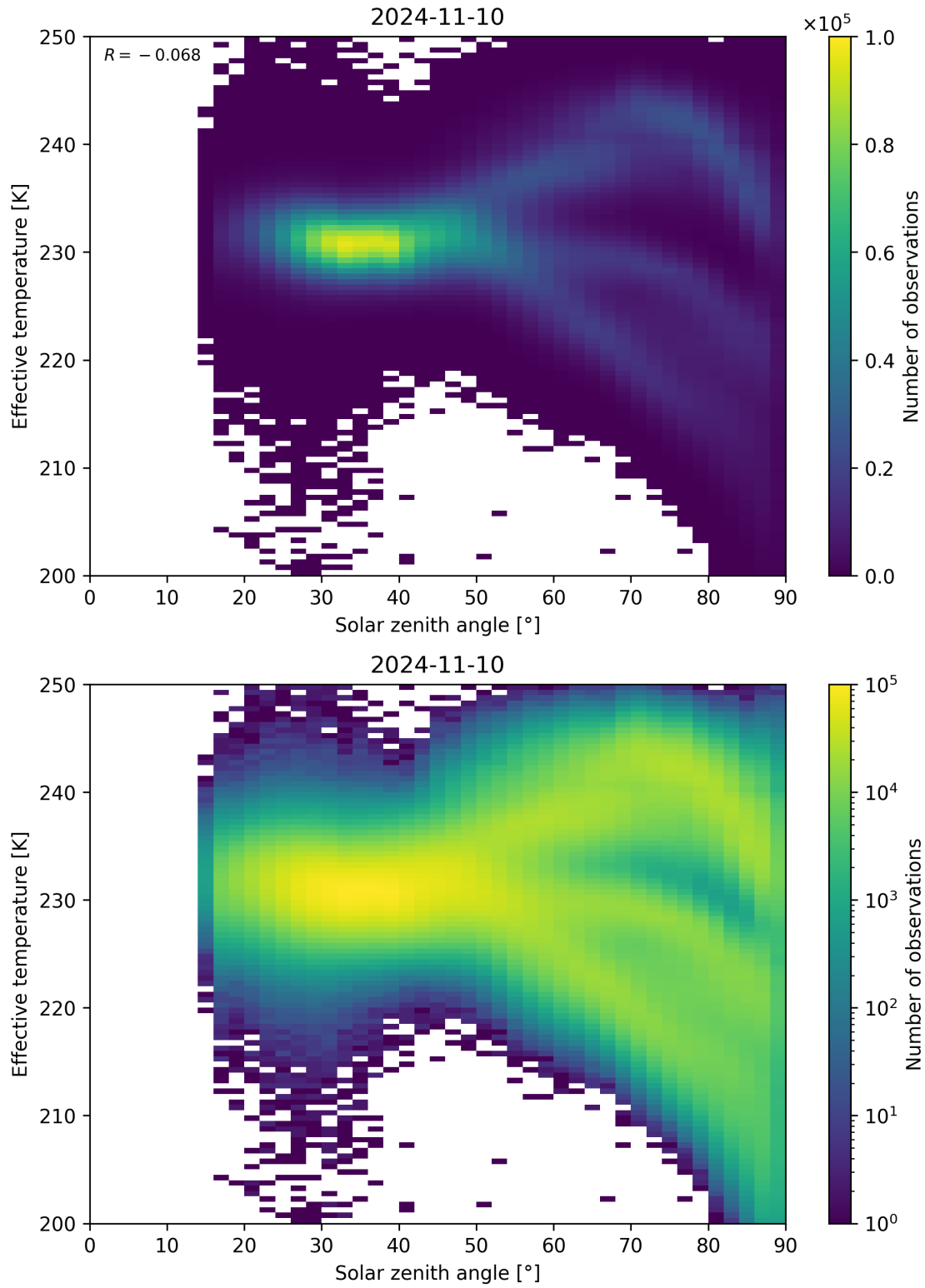
Figure 45: Scatter density plot of “Solar zenith angle” against “Effective temperature” for 2024-11-09 to 2024-11-11.
