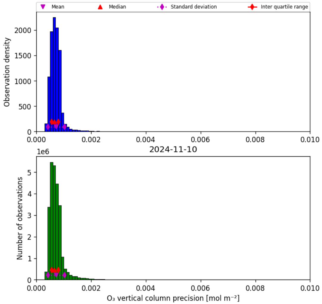
Figure 22: Histogram of “O 3 vertical column precision” for 2024-11-09 to 2024-11-11
