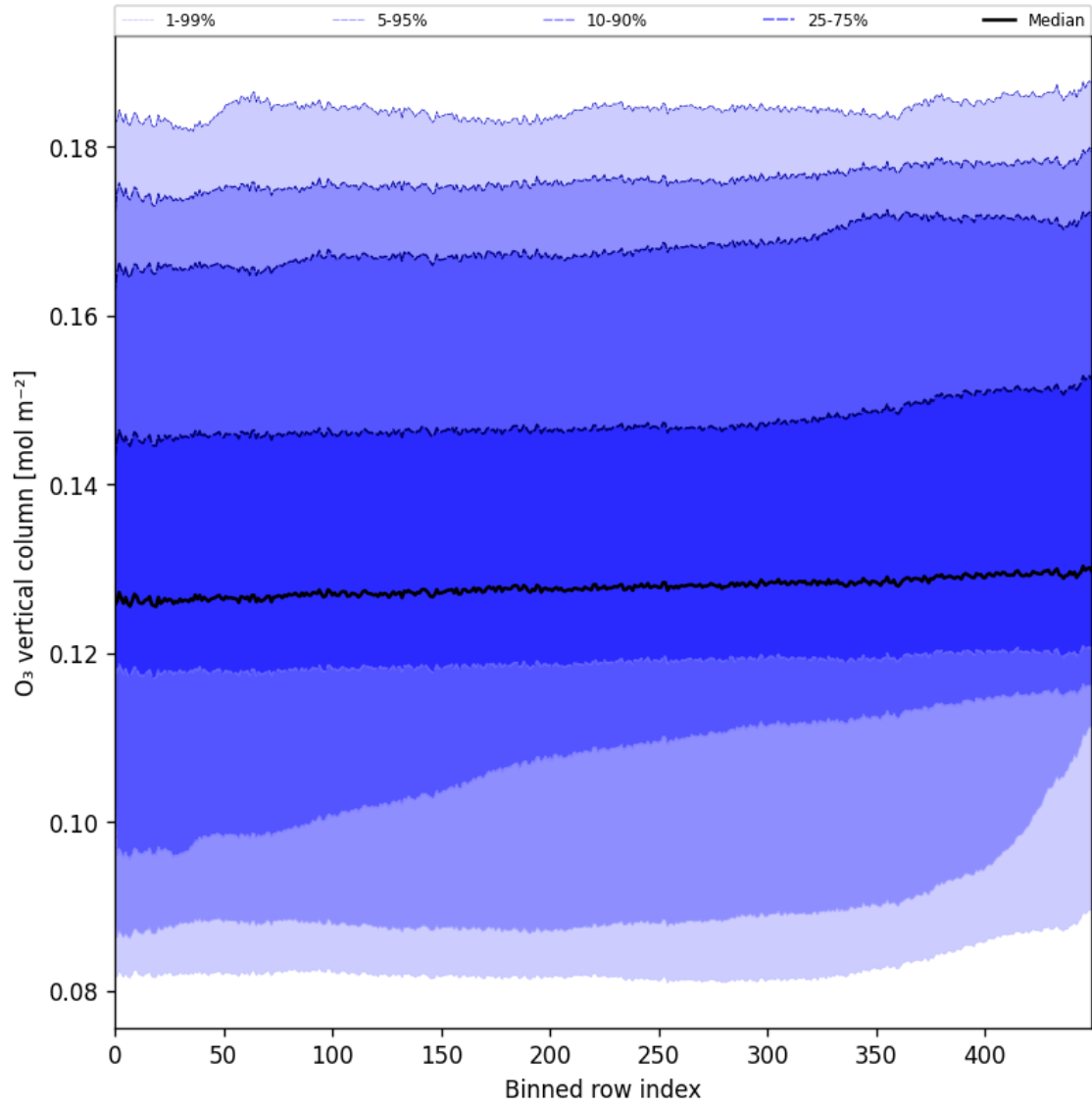
Figure 28: Along track statistics of “O 3 vertical column” for 2024-11-09 to 2024-11-11
