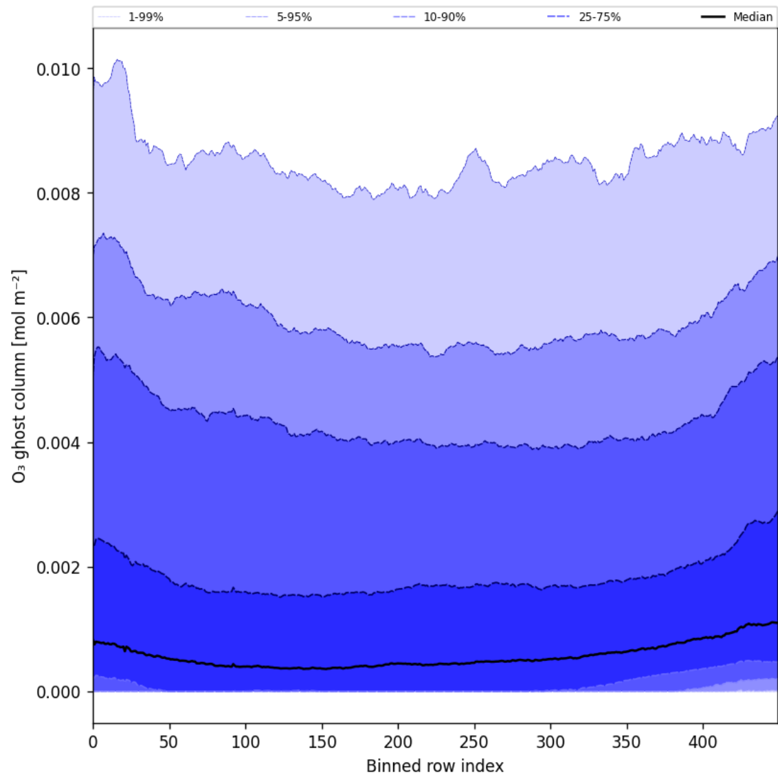
Figure 32: Along track statistics of “O 3 ghost column” for 2024-11-09 to 2024-11-11
