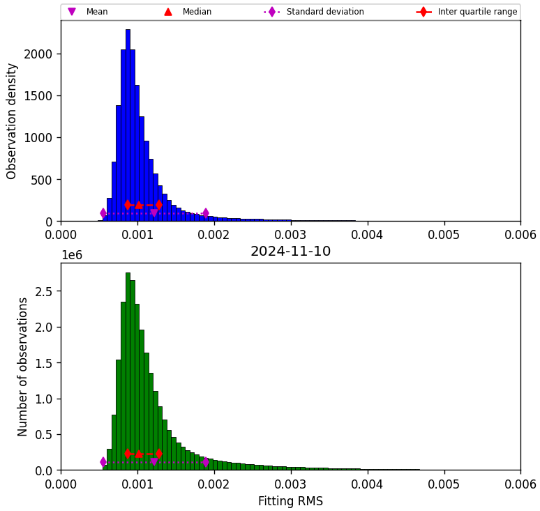
Figure 23: Histogram of “Fitting RMS” for 2024-11-09 to 2024-11-11
