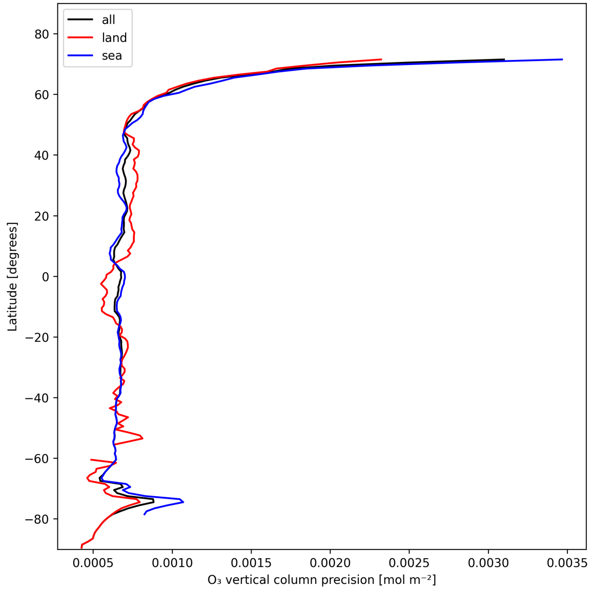
Figure 15: Zonal average of “O 3 vertical column precision” for 2024-11-09 to 2024-11-11.
