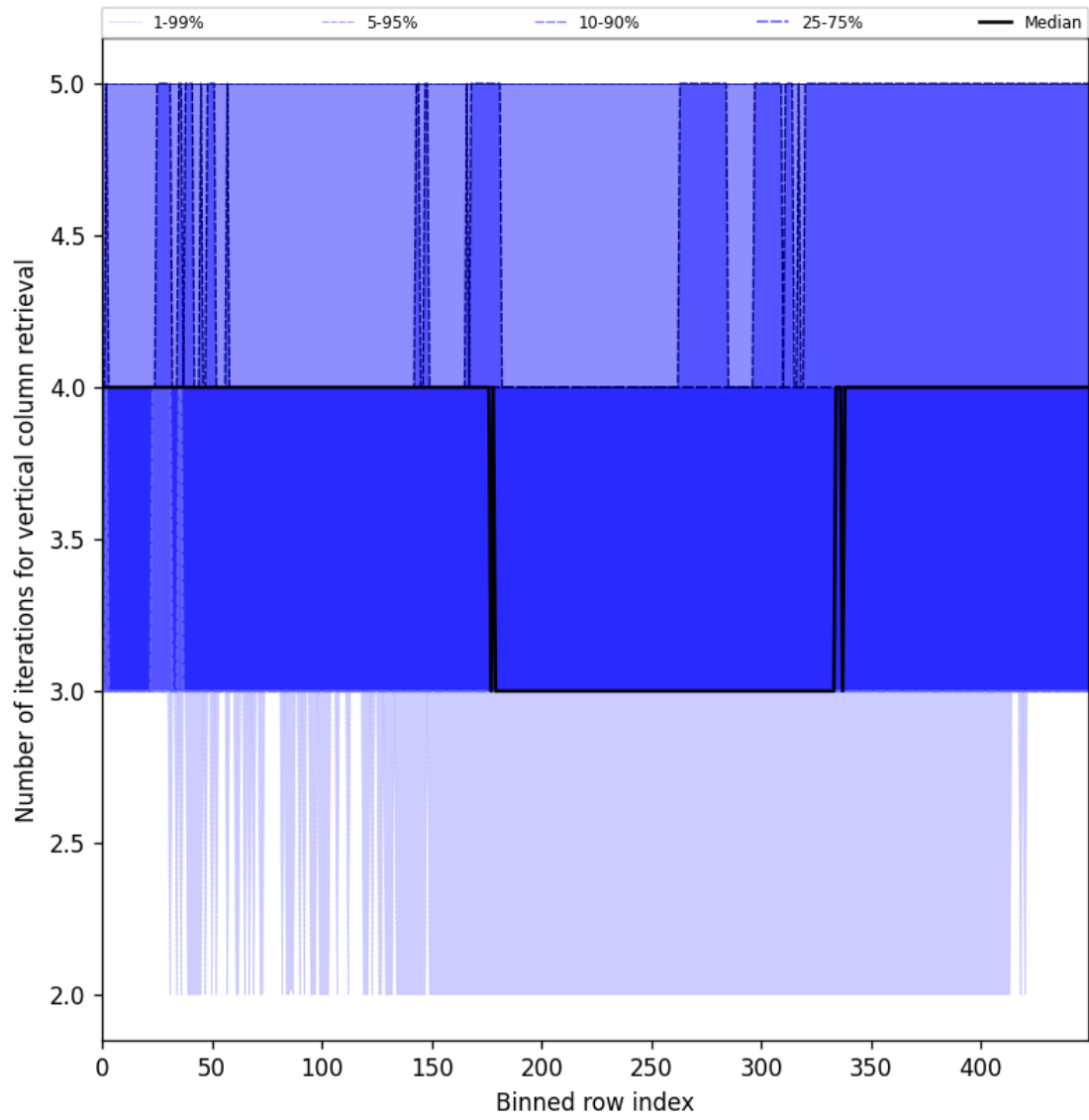
Figure 33: Along track statistics of “Number of iterations for vertical column retrieval” for 2024-11-09 to 2024-11-11
