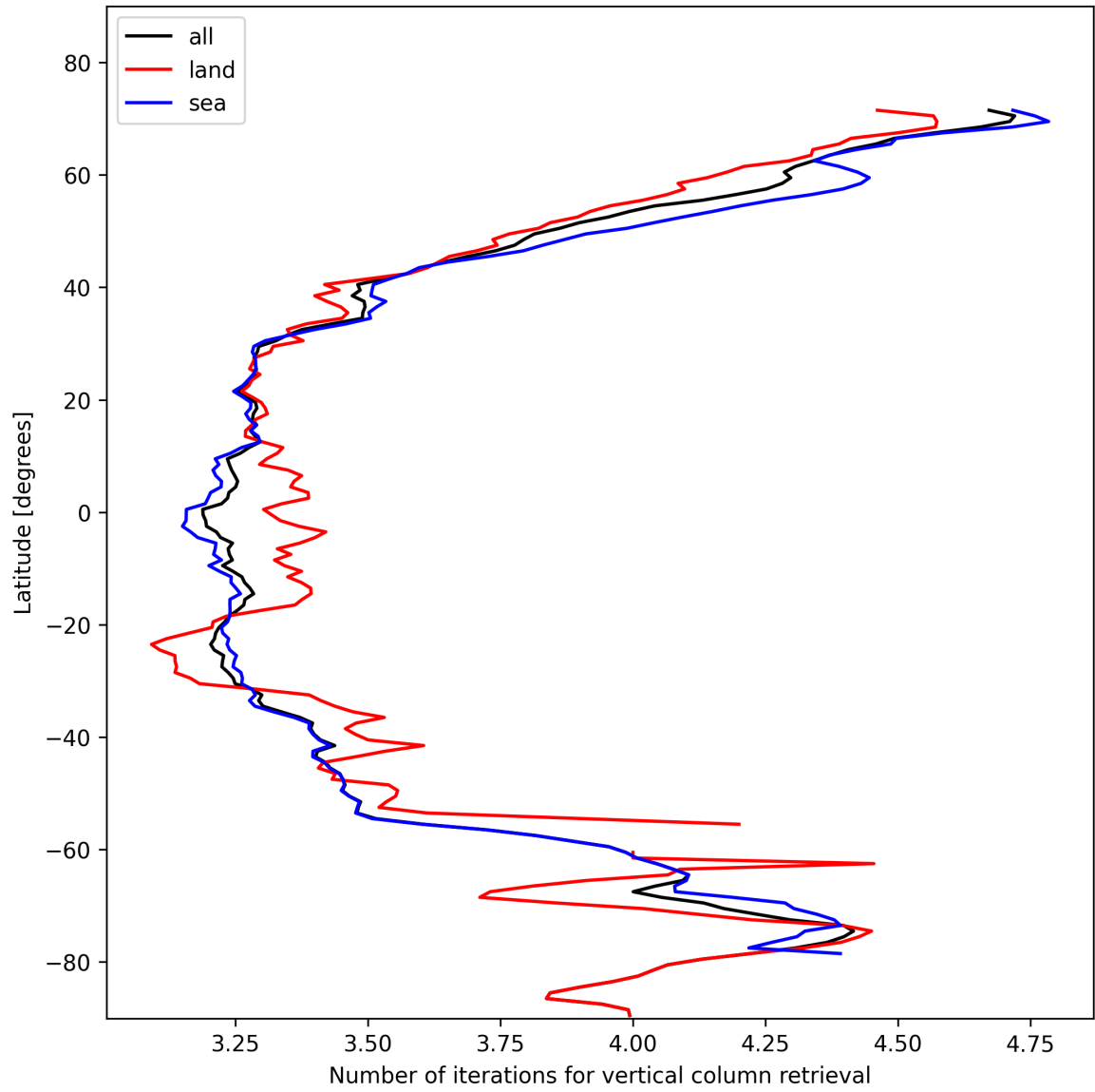
Figure 19: Zonal average of “Number of iterations for vertical column retrieval” for 2024-11-09 to 2024-11-11.
