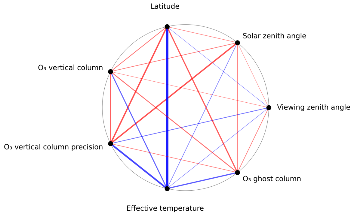
Figure 1: Map of correlation graph for 2024-11-09 to 2024-11-11.
