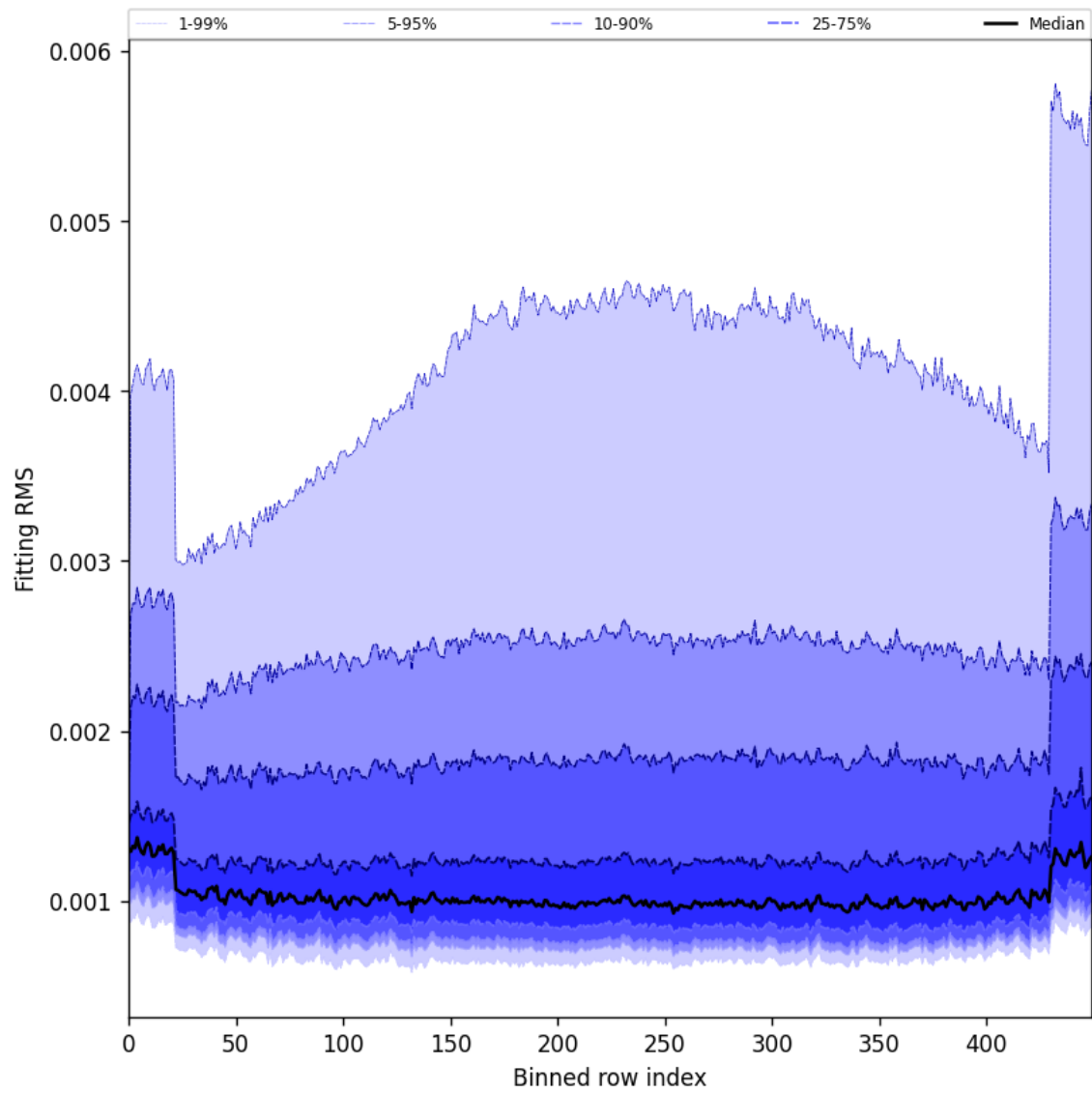
Figure 30: Along track statistics of “Fitting RMS” for 2024-11-11 to 2024-11-13
