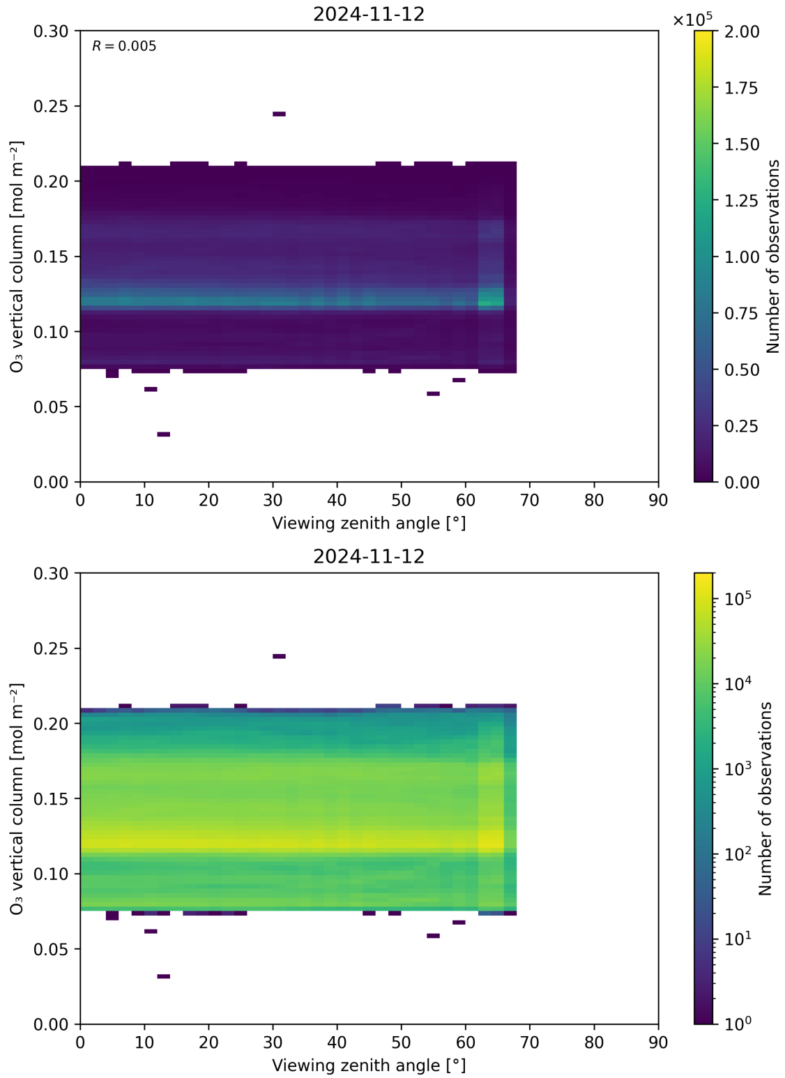
Figure 52: Scatter density plot of “Viewing zenith angle” against “O 3 vertical column” for 2024-11-11 to 2024-11-13.
