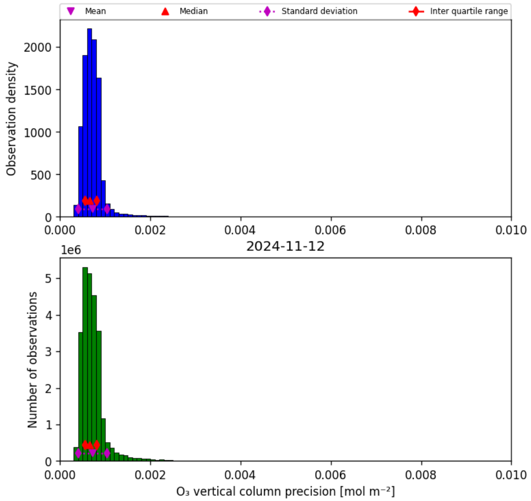
Figure 22: Histogram of “O 3 vertical column precision” for 2024-11-11 to 2024-11-13
