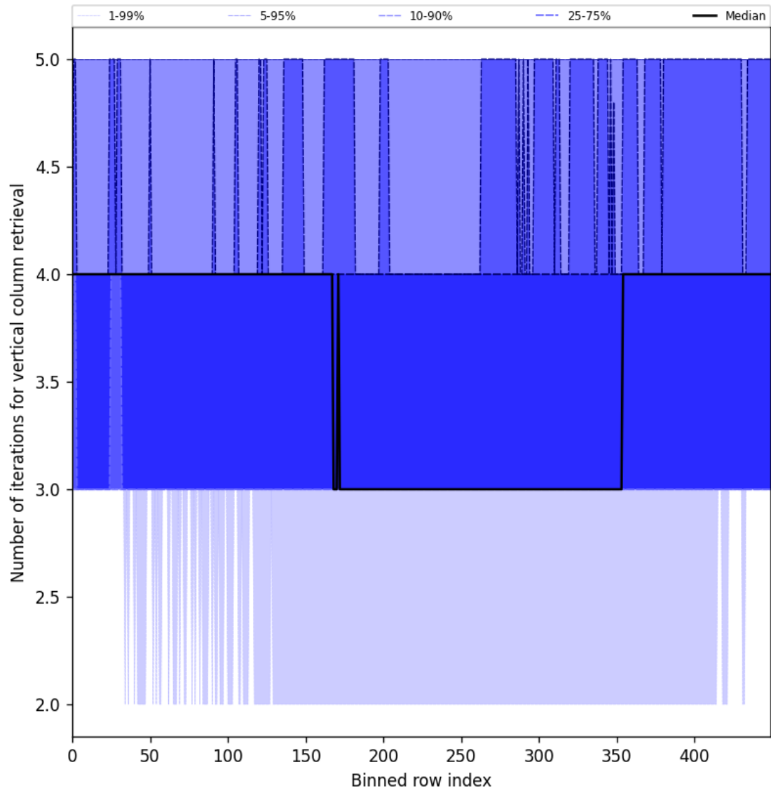
Figure 33: Along track statistics of “Number of iterations for vertical column retrieval” for 2024-11-11 to 2024-11-13
