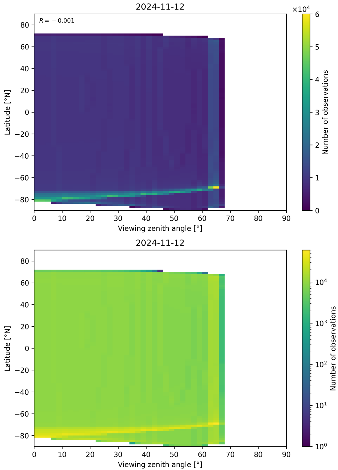
Figure 49: Scatter density plot of “Viewing zenith angle” against “Latitude” for 2024-11-11 to 2024-11-13.
