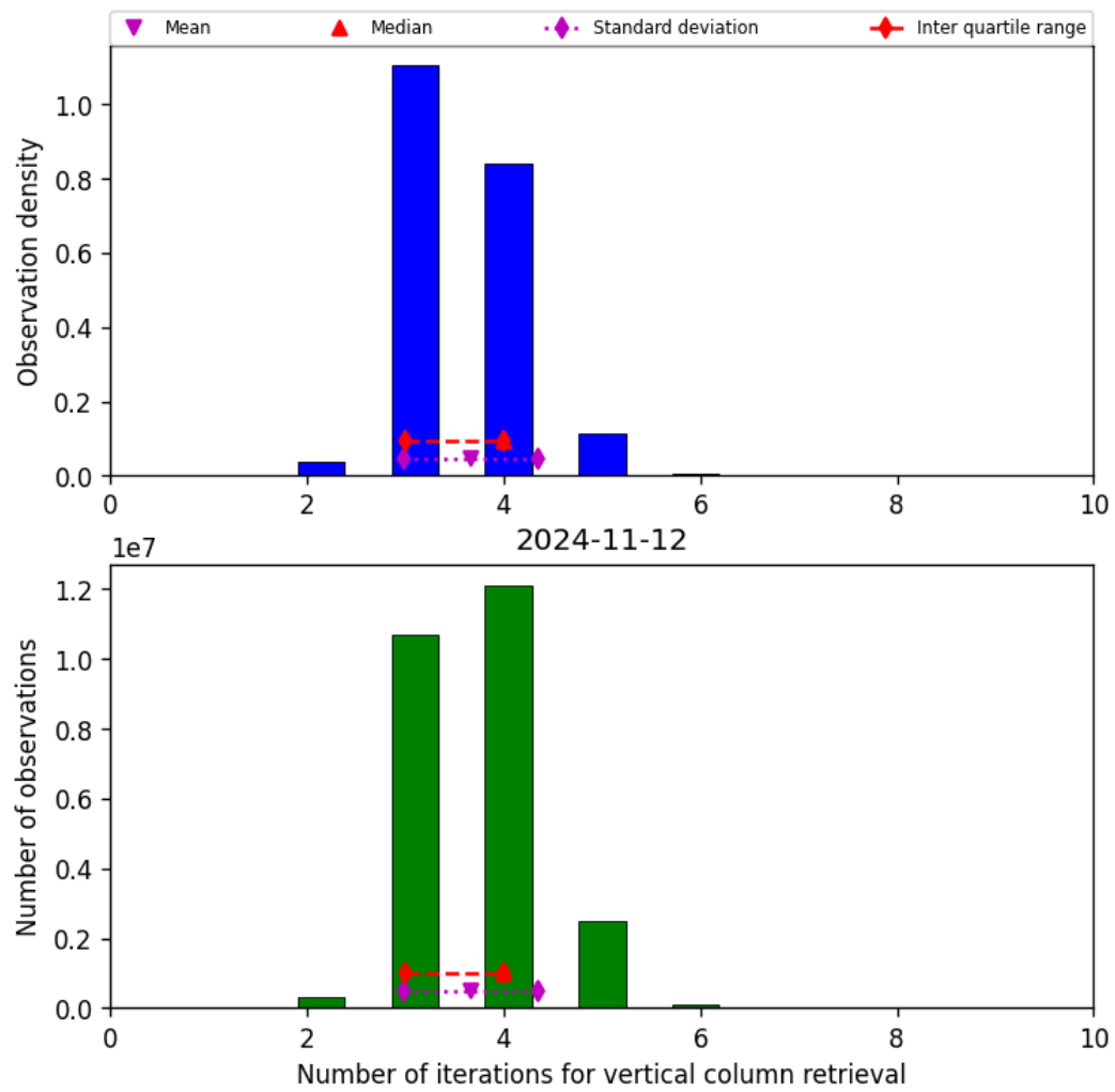
Figure 26: Histogram of “Number of iterations for vertical column retrieval” for 2024-11-11 to 2024-11-13
