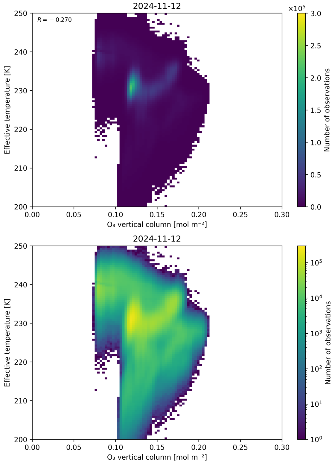
Figure 39: Scatter density plot of “O 3 vertical column” against “Effective temperature” for 2024-11-11 to 2024-11-13.
