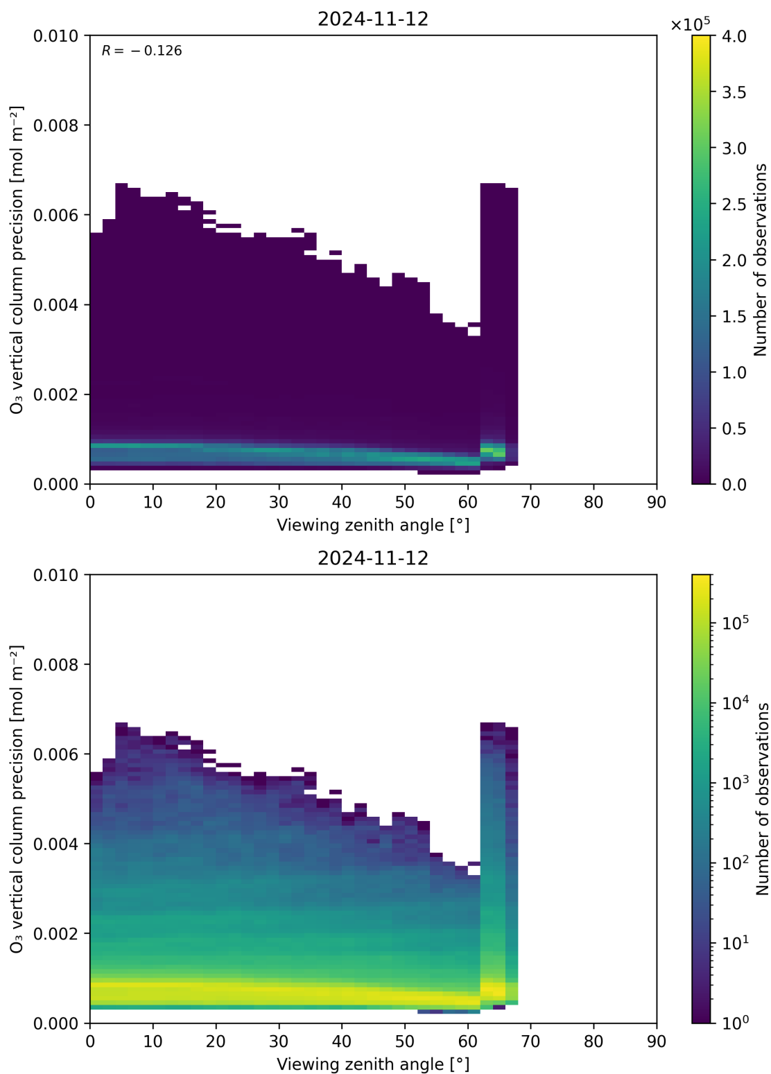
Figure 53: Scatter density plot of “Viewing zenith angle” against “O 3 vertical column precision” for 2024-11-11 to 2024-11-13.
