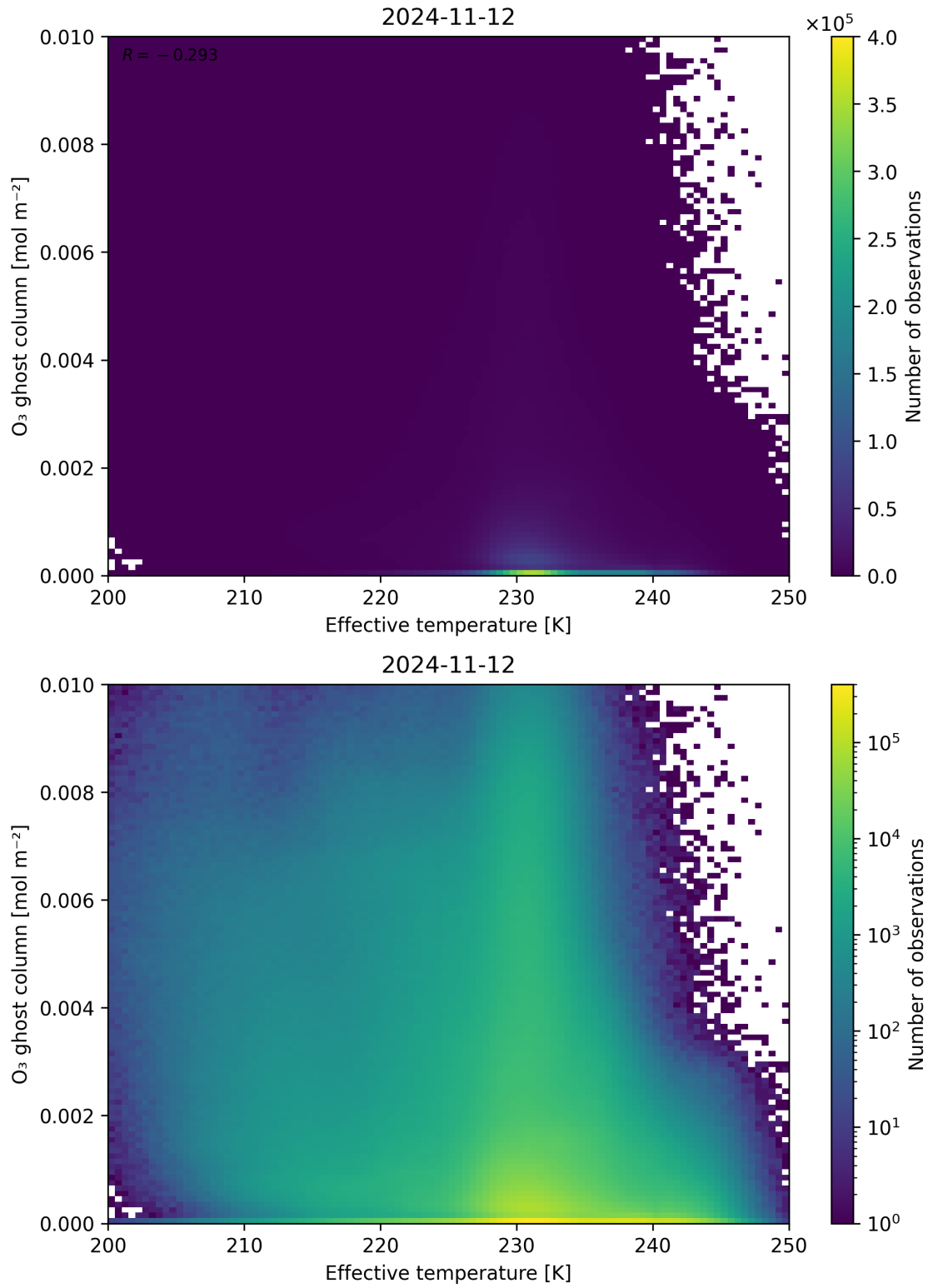
Figure 38: Scatter density plot of “Effective temperature” against “O 3 ghost column” for 2024-11-11 to 2024-11-13.
