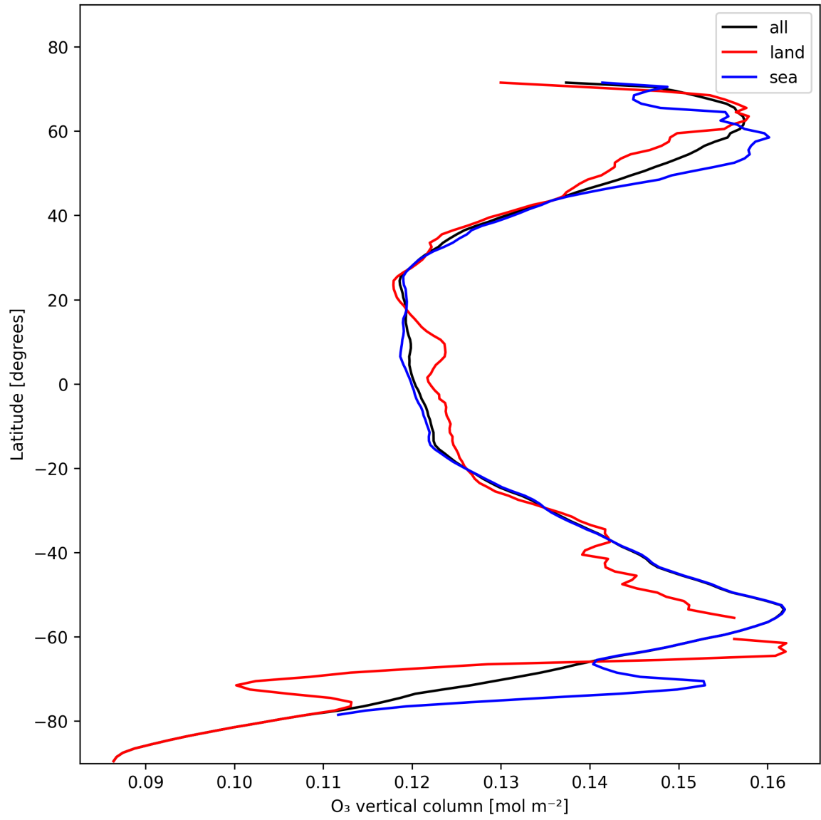
Figure 14: Zonal average of “O 3 vertical column” for 2024-11-11 to 2024-11-13.
