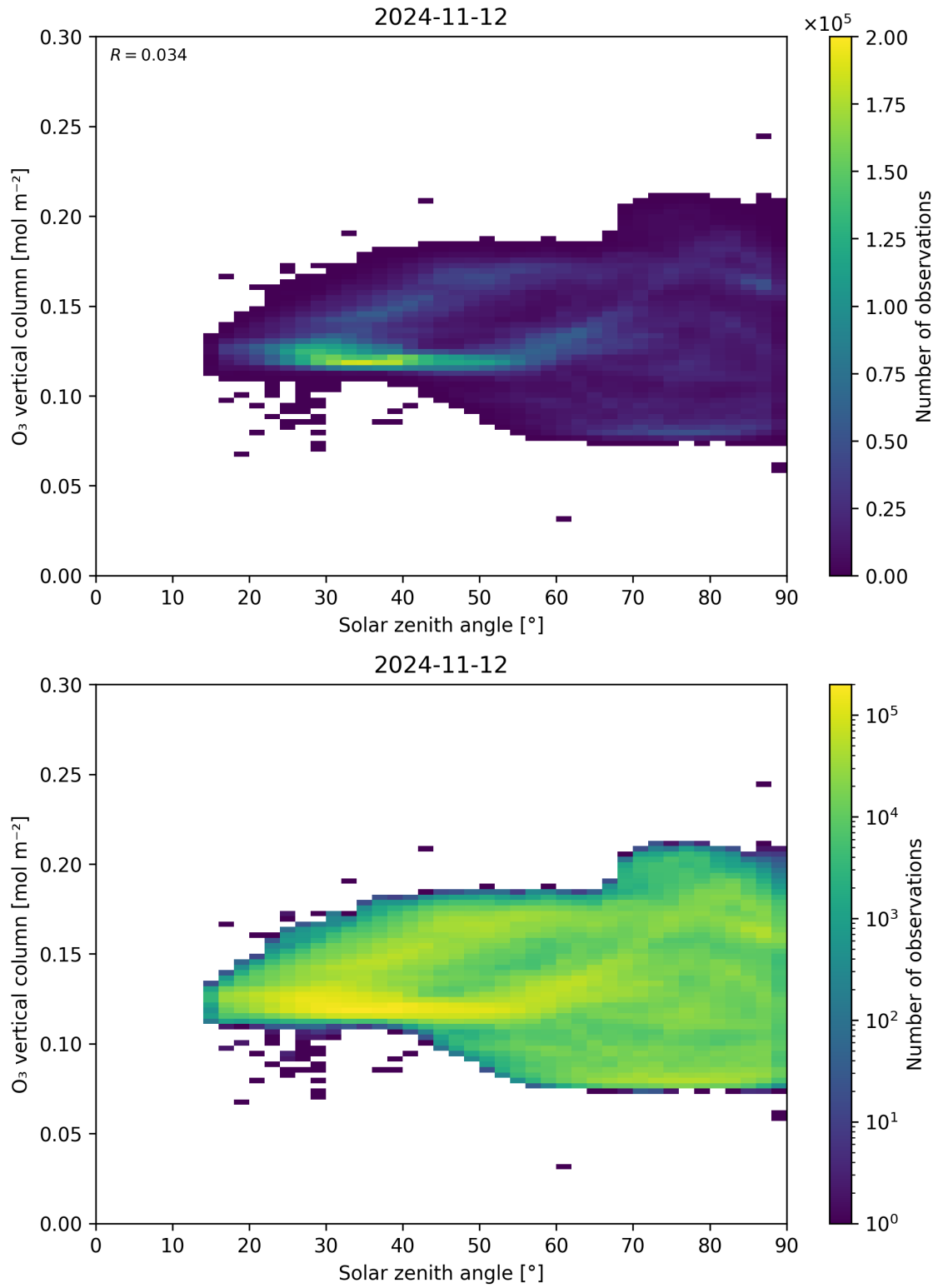
Figure 47: Scatter density plot of “Solar zenith angle” against “O 3 vertical column” for 2024-11-11 to 2024-11-13.
