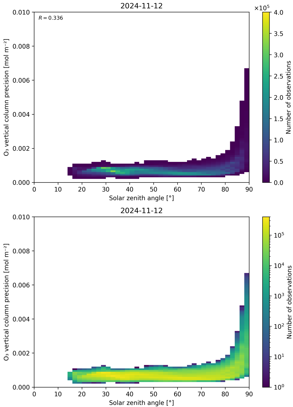
Figure 48: Scatter density plot of “Solar zenith angle” against “O 3 vertical column precision” for 2024-11-11 to 2024-11-13.
