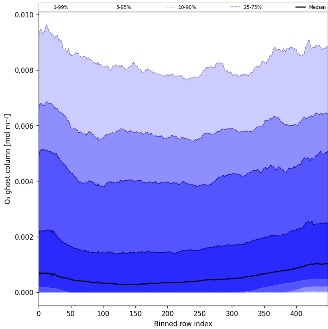
Figure 32: Along track statistics of “O 3 ghost column” for 2024-11-11 to 2024-11-13
