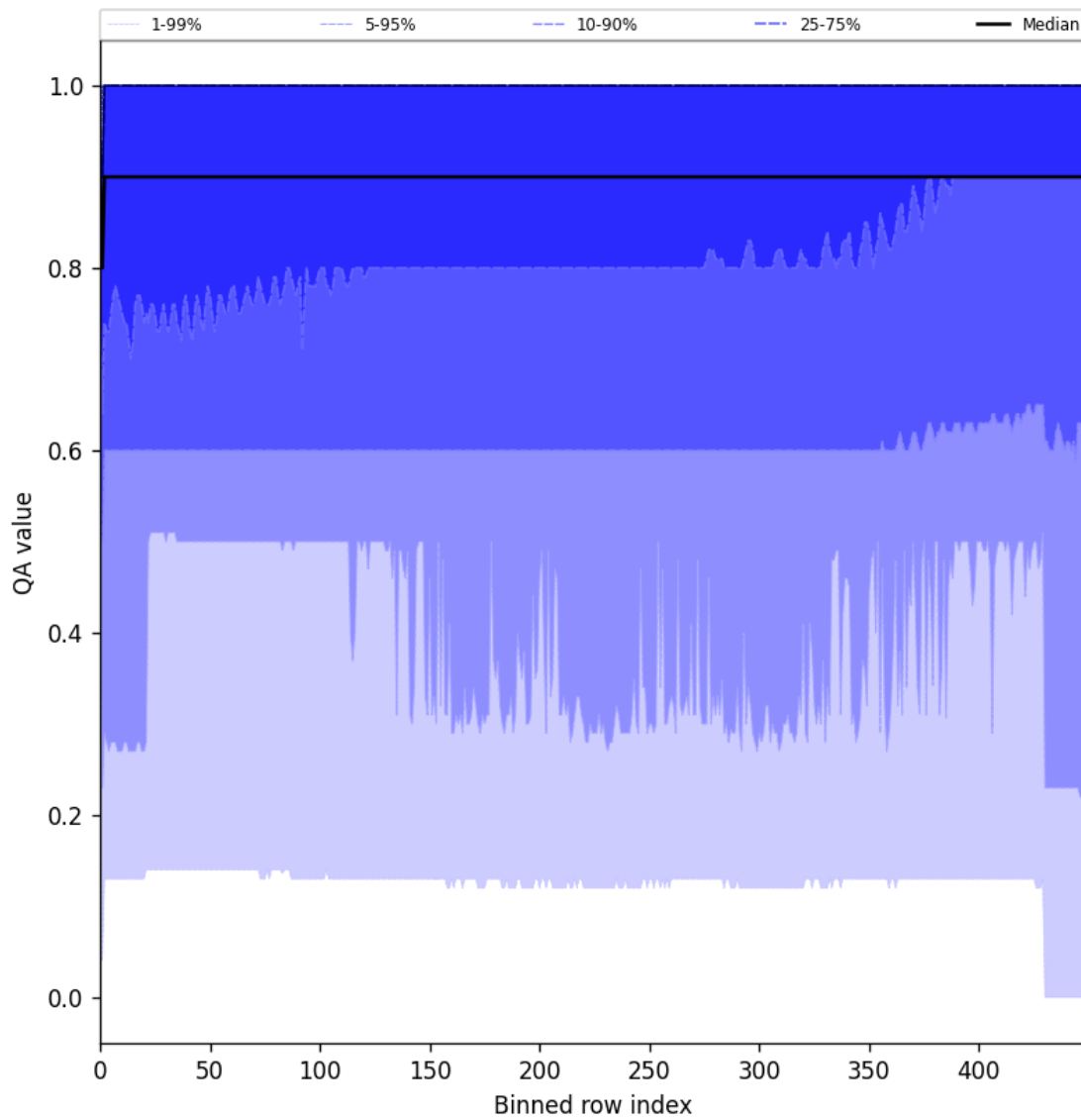
Figure 27: Along track statistics of “QA value” for 2024-11-11 to 2024-11-13
