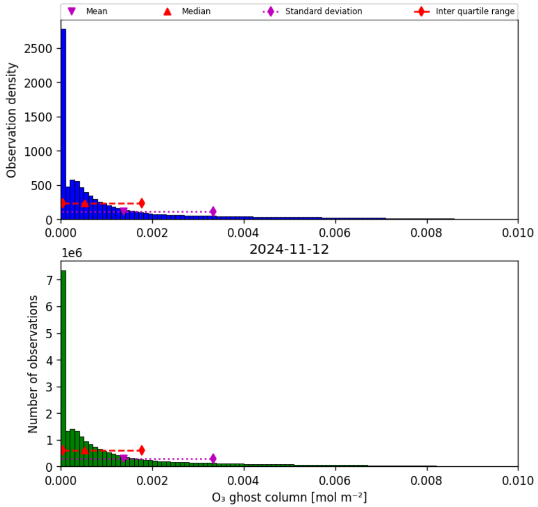
Figure 25: Histogram of "O 3 ghost column" for 2024-11-11 to 2024-11-13
