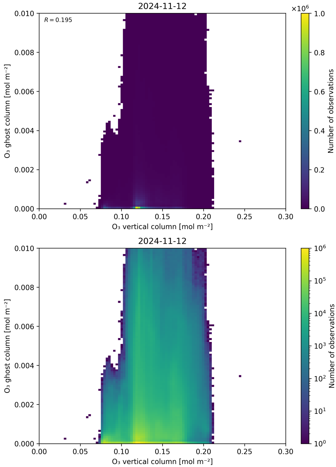
Figure 40: Scatter density plot of “O 3 vertical column” against “O 3 ghost column” for 2024-11-11 to 2024-11-13.
