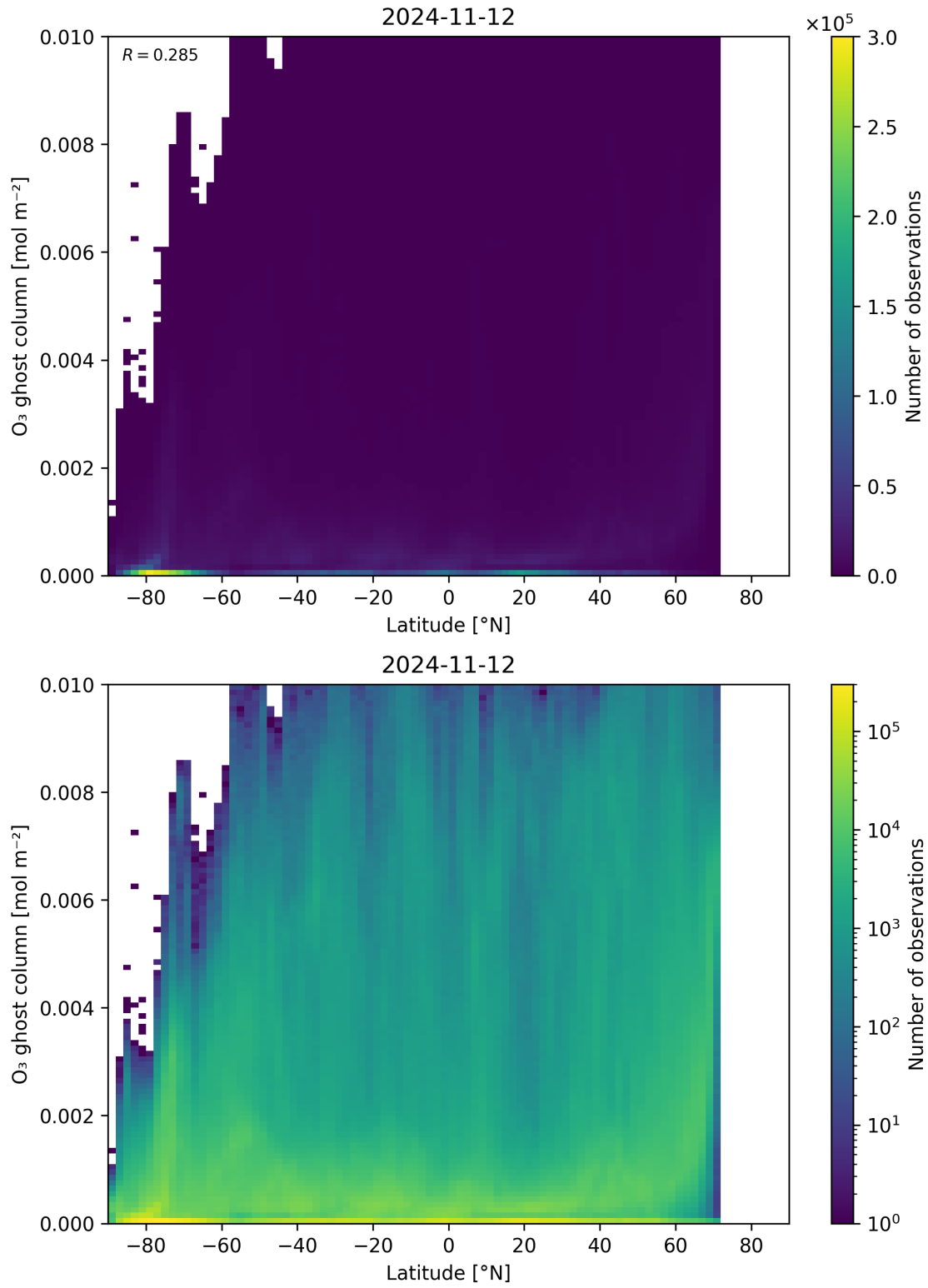
Figure 35: Scatter density plot of “Latitude” against “O 3 ghost column” for 2024-11-11 to 2024-11-13.
