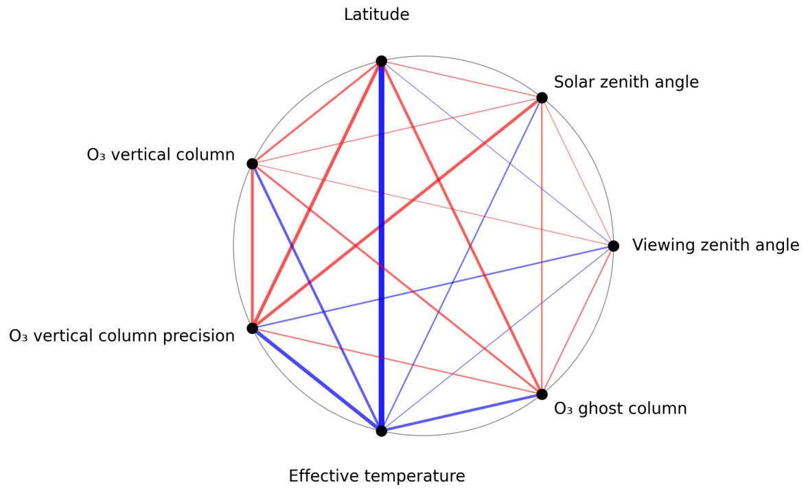
Figure 1: Map of correlation graph for 2024-11-11 to 2024-11-13.
