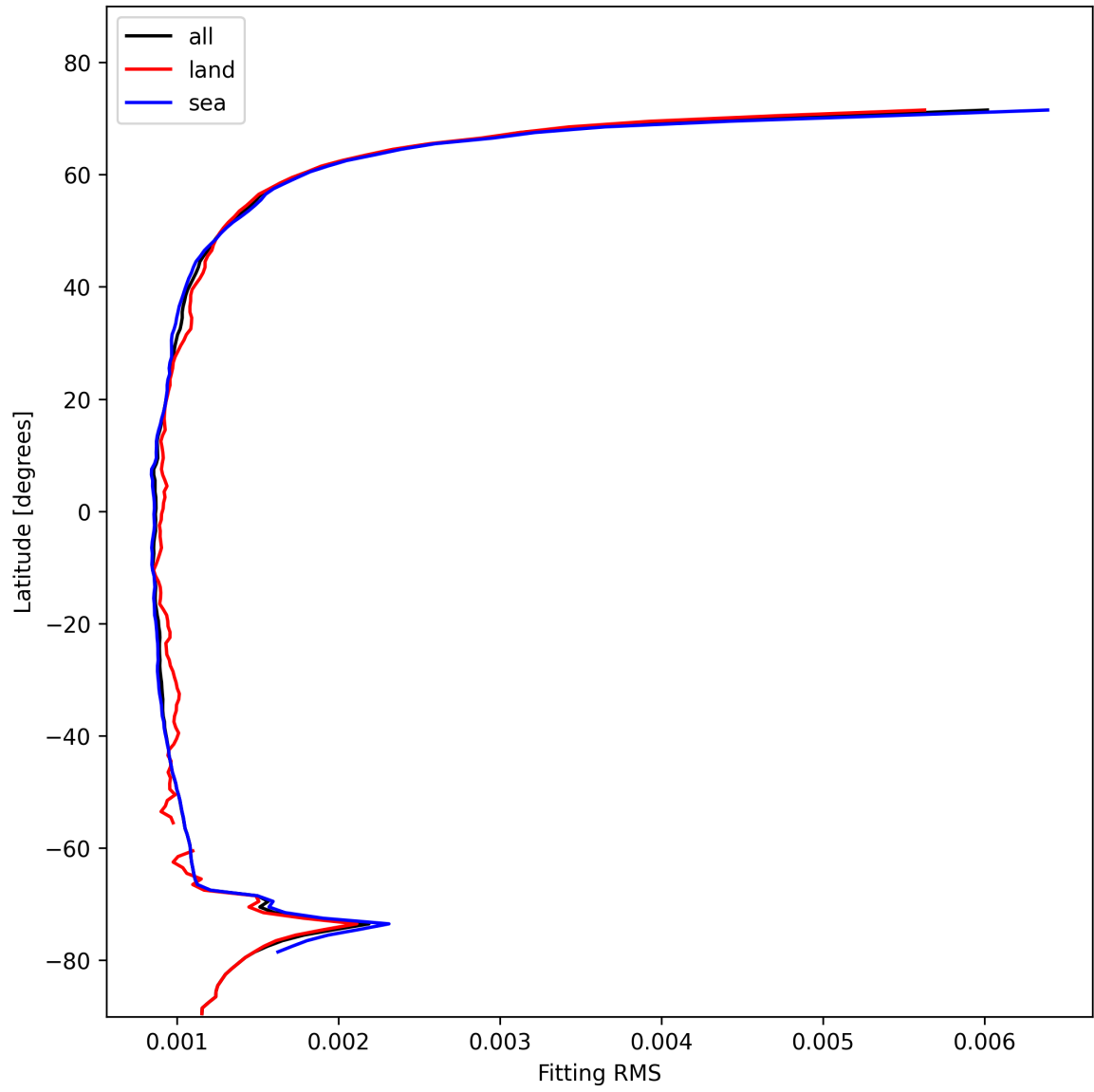
Figure 16: Zonal average of “Fitting RMS” for 2024-11-11 to 2024-11-13.
