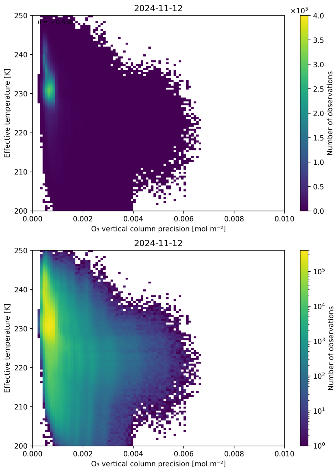
Figure 42: Scatter density plot of “O 3 vertical column precision” against “Effective temperature” for 2024-11-11 to 2024-11-13.
