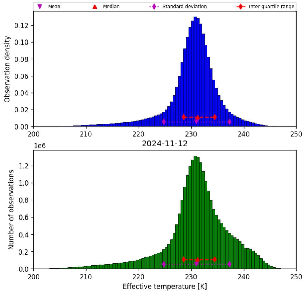
Figure 24: Histogram of “Effective temperature” for 2024-11-11 to 2024-11-13
