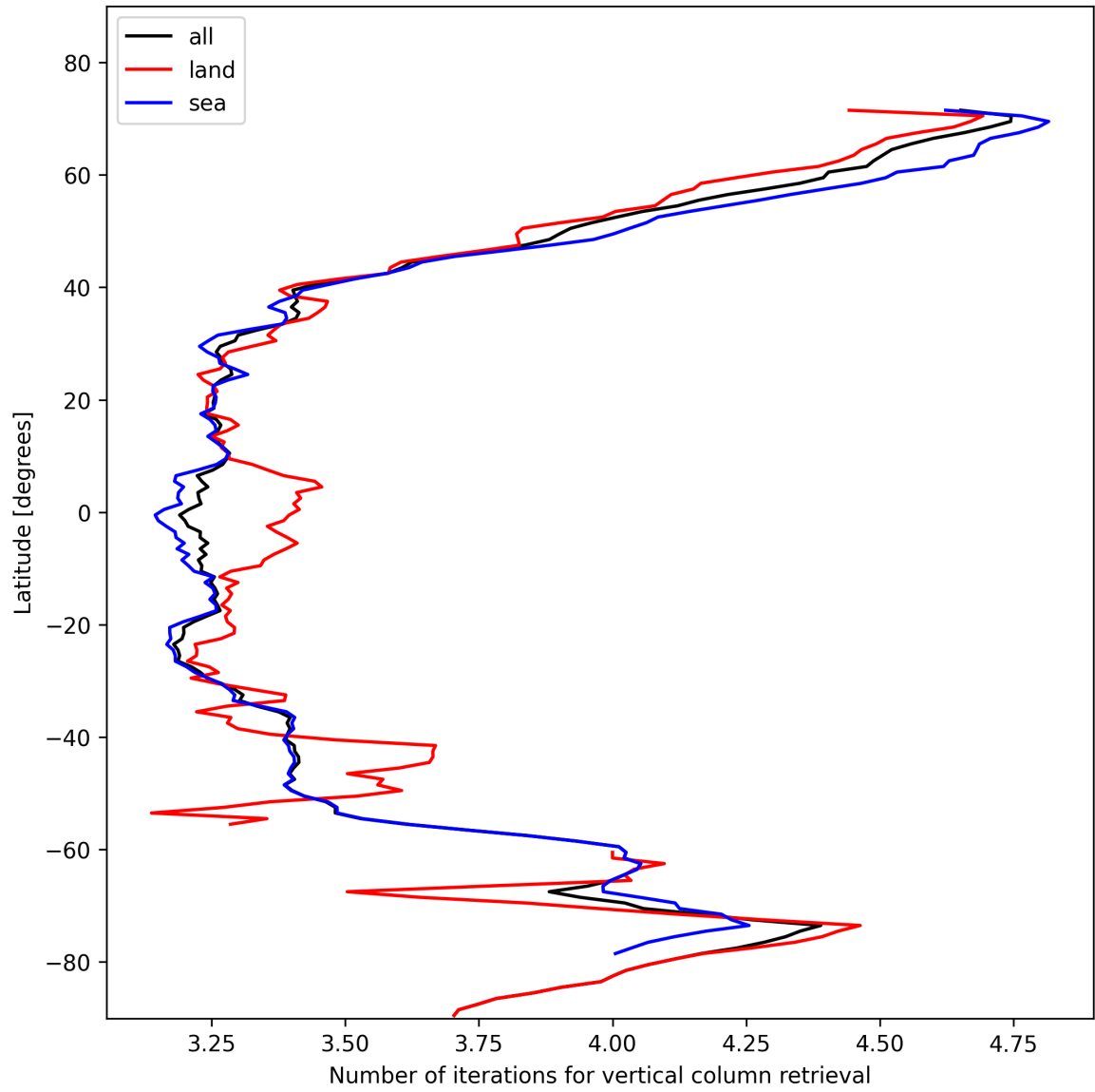
Figure 19: Zonal average of “Number of iterations for vertical column retrieval” for 2024-11-11 to 2024-11-13.
