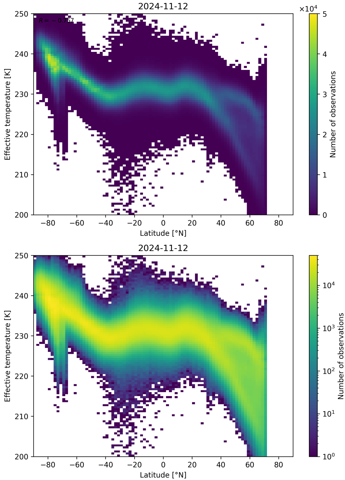
Figure 34: Scatter density plot of “Latitude” against “Effective temperature” for 2024-11-11 to 2024-11-13.
