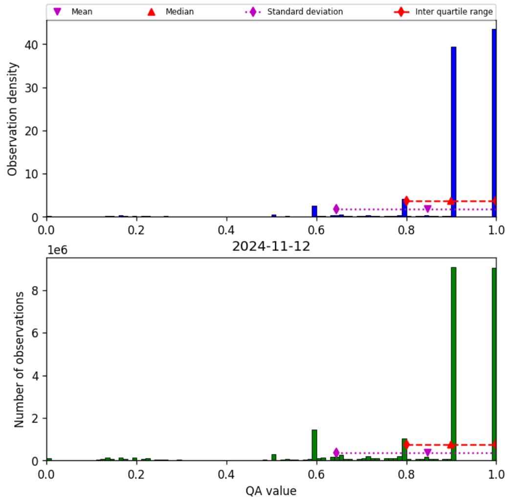
Figure 20: Histogram of “QA value” for 2024-11-11 to 2024-11-13
