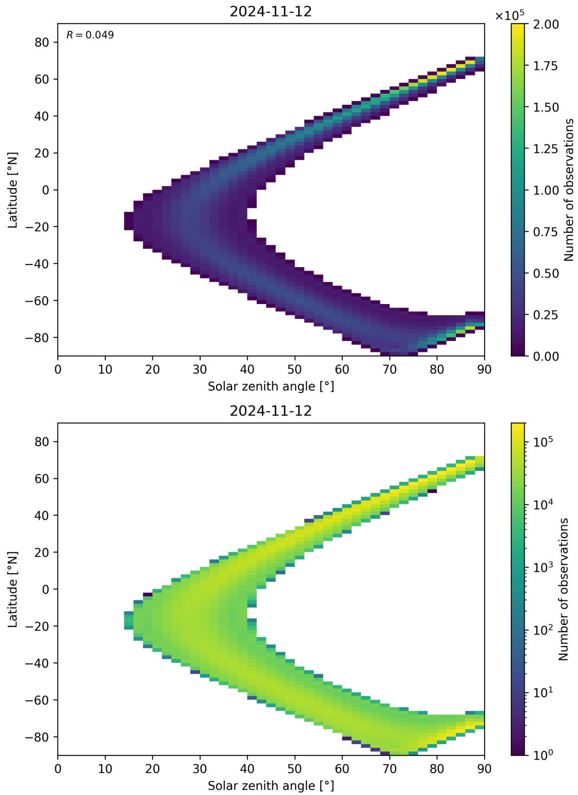
Figure 44: Scatter density plot of “Solar zenith angle” against “Latitude” for 2024-11-11 to 2024-11-13.
