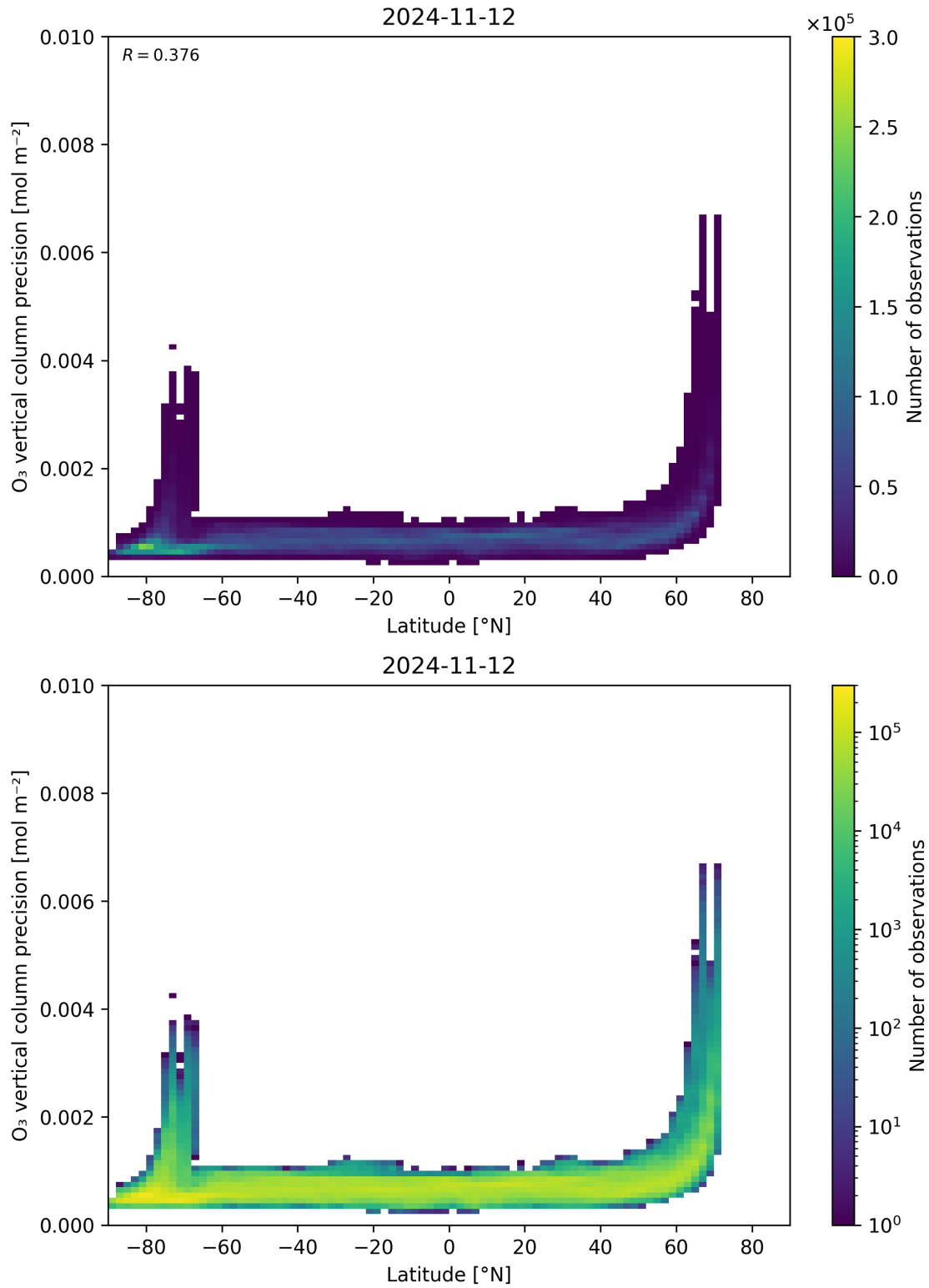
Figure 37: Scatter density plot of “Latitude” against “O 3 vertical column precision” for 2024-11-11 to 2024-11-13.
