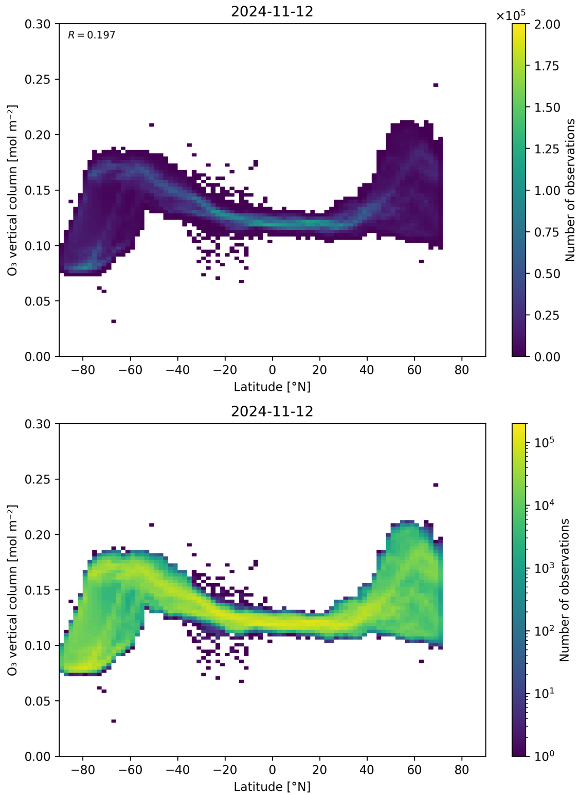
Figure 36: Scatter density plot of “Latitude” against “O 3 vertical column” for 2024-11-11 to 2024-11-13.
