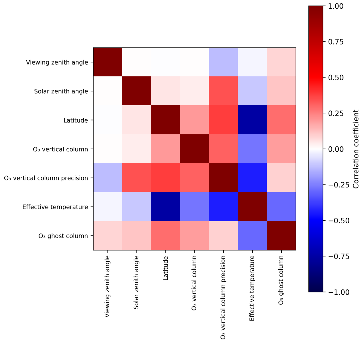
Figure 2: Map of correlation matrix for 2024-11-11 to 2024-11-13.
