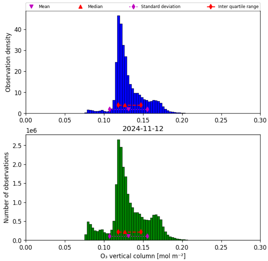
Figure 21: Histogram of “O 3 vertical column” for 2024-11-11 to 2024-11-13
