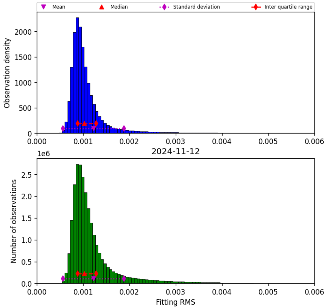
Figure 23: Histogram of “Fitting RMS” for 2024-11-11 to 2024-11-13
