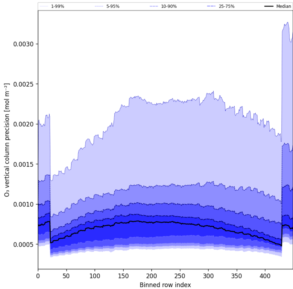
Figure 29: Along track statistics of “O 3 vertical column precision” for 2024-11-11 to 2024-11-13
