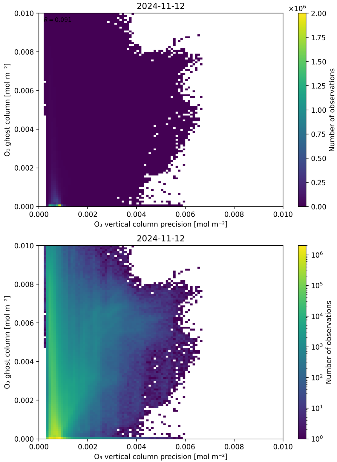
Figure 43: Scatter density plot of “O 3 vertical column precision” against “O 3 ghost column” for 2024-11-11 to 2024-11-13.
