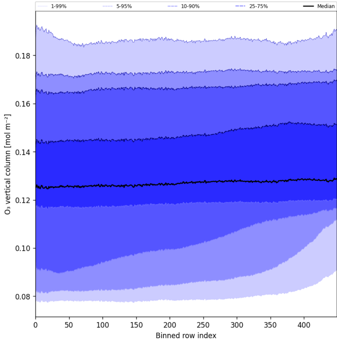
Figure 28: Along track statistics of “O 3 vertical column” for 2024-11-11 to 2024-11-13
