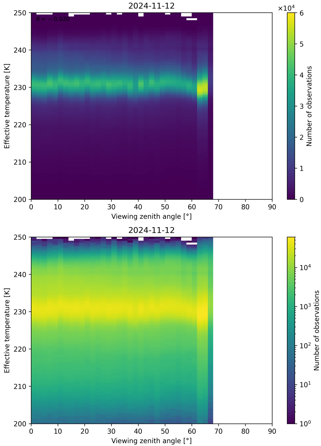
Figure 50: Scatter density plot of “Viewing zenith angle” against “Effective temperature” for 2024-11-11 to 2024-11-13.
