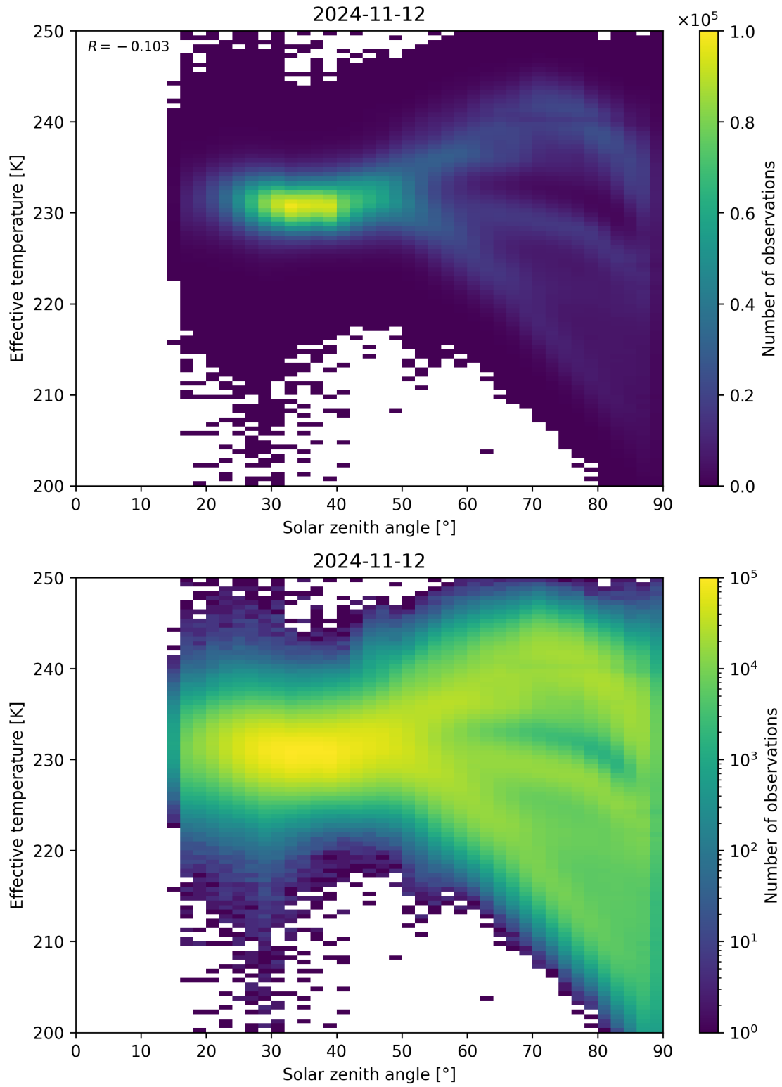
Figure 45: Scatter density plot of “Solar zenith angle” against “Effective temperature” for 2024-11-11 to 2024-11-13.
