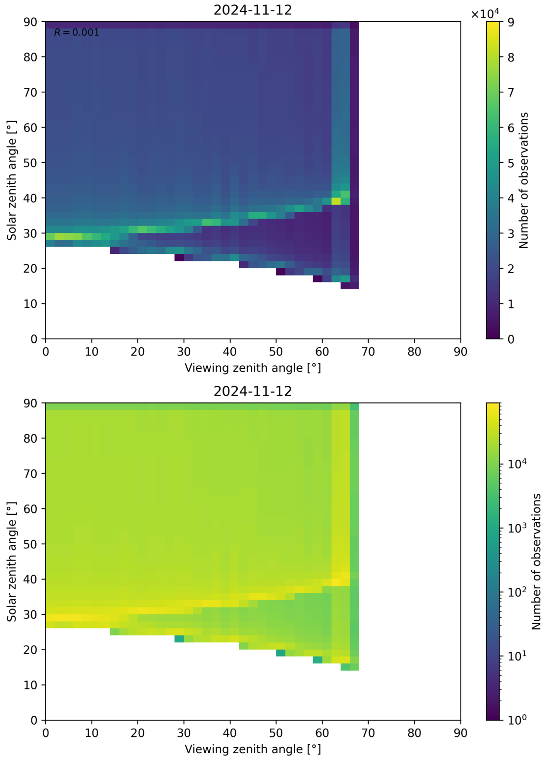
Figure 54: Scatter density plot of “Viewing zenith angle” against “Solar zenith angle” for 2024-11-11 to 2024-11-13.
