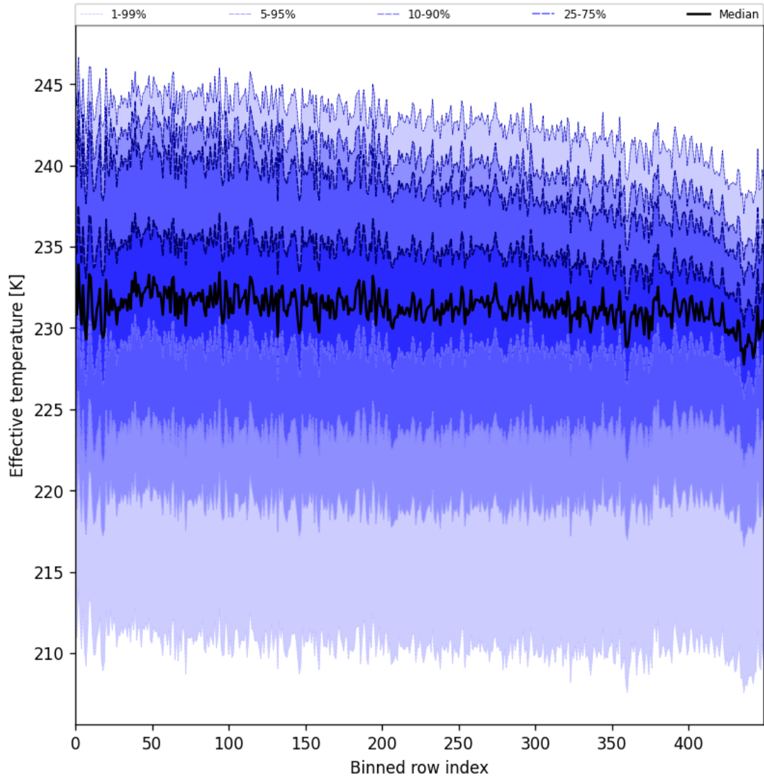
Figure 31: Along track statistics of “Effective temperature” for 2024-11-11 to 2024-11-13
