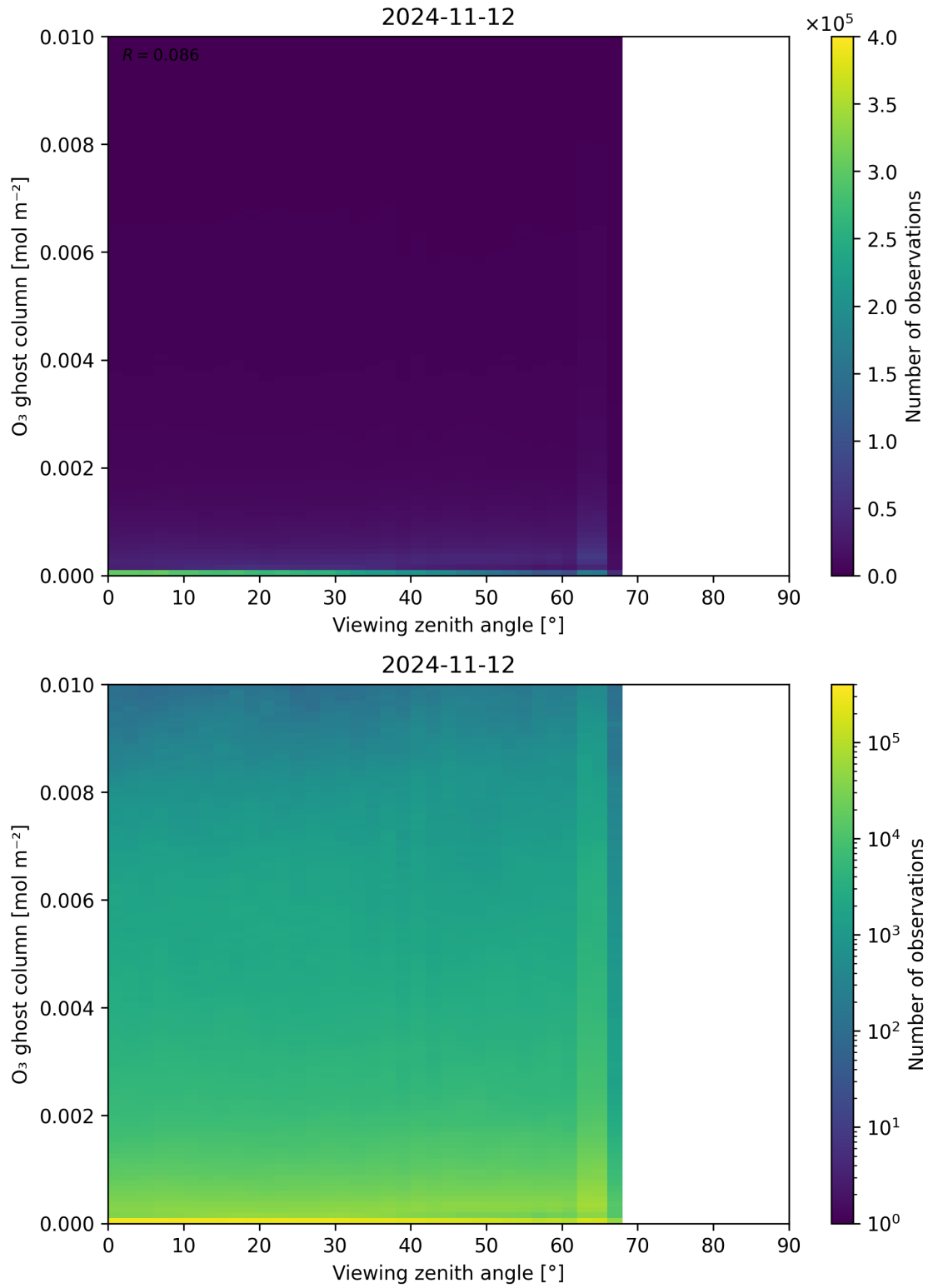
Figure 51: Scatter density plot of “Viewing zenith angle” against “O 3 ghost column” for 2024-11-11 to 2024-11-13.
