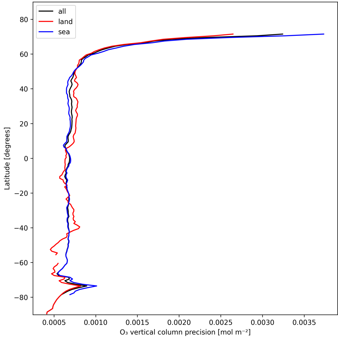
Figure 15: Zonal average of “O 3 vertical column precision” for 2024-11-11 to 2024-11-13.
