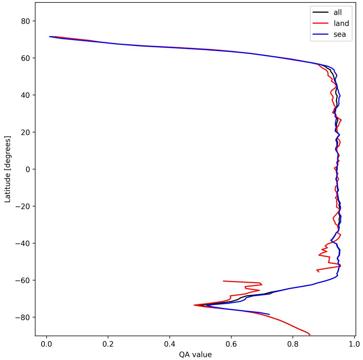
Figure 13: Zonal average of “QA value” for 2024-11-11 to 2024-11-13.
