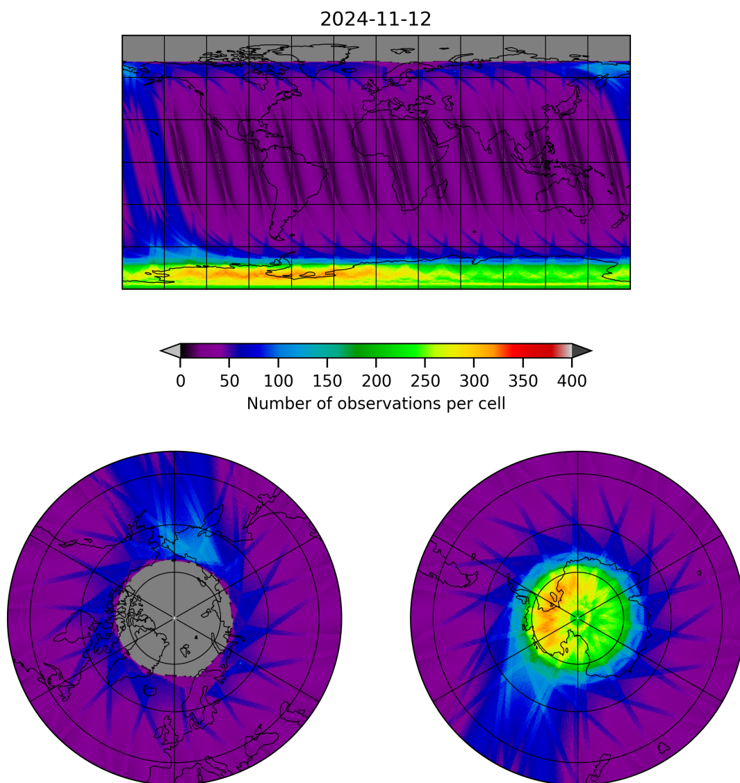
Figure 12: Map of the number of observations for 2024-11-11 to 2024-11-13
