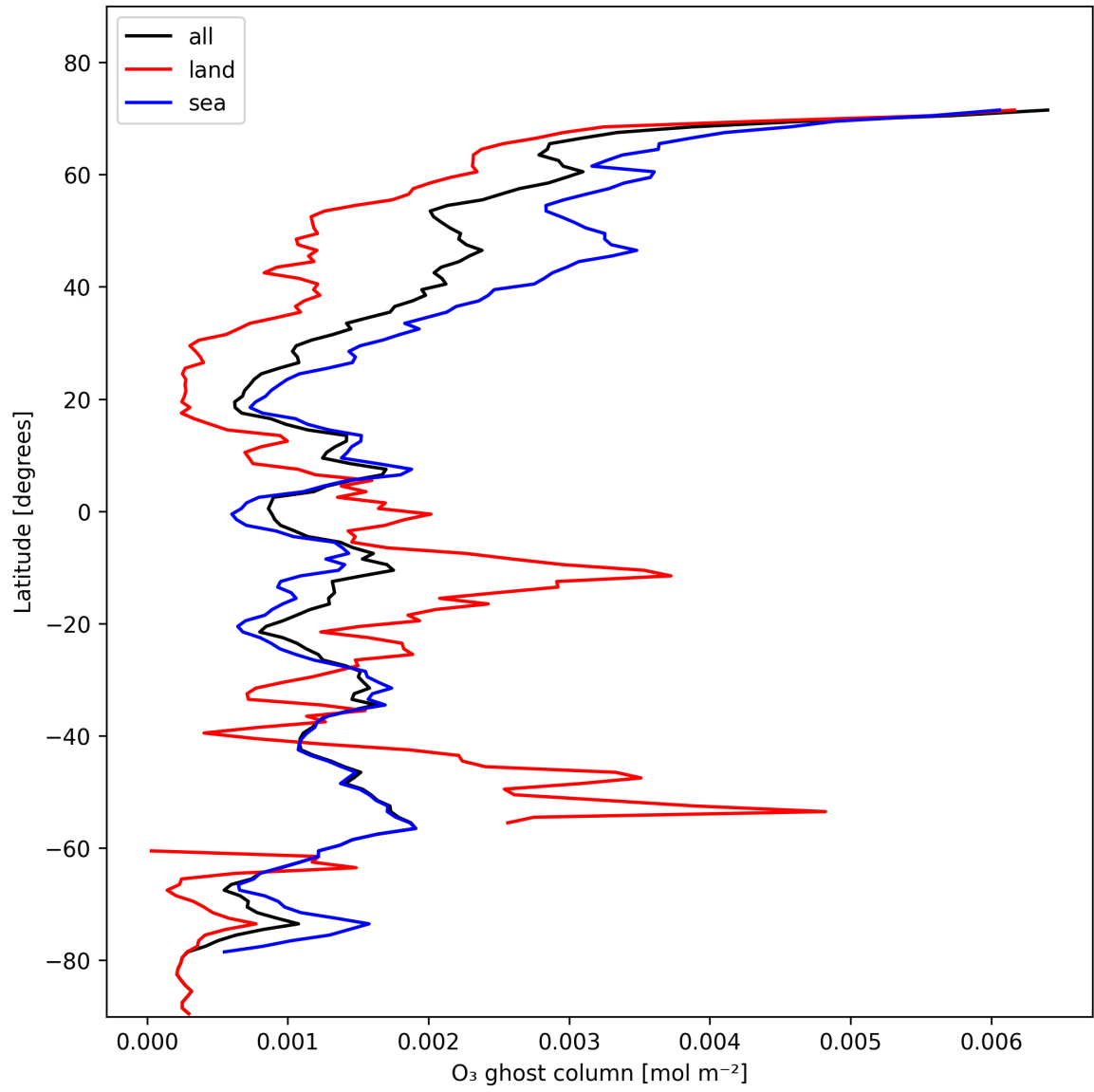
Figure 18: Zonal average of “O 3 ghost column” for 2024-11-11 to 2024-11-13.
