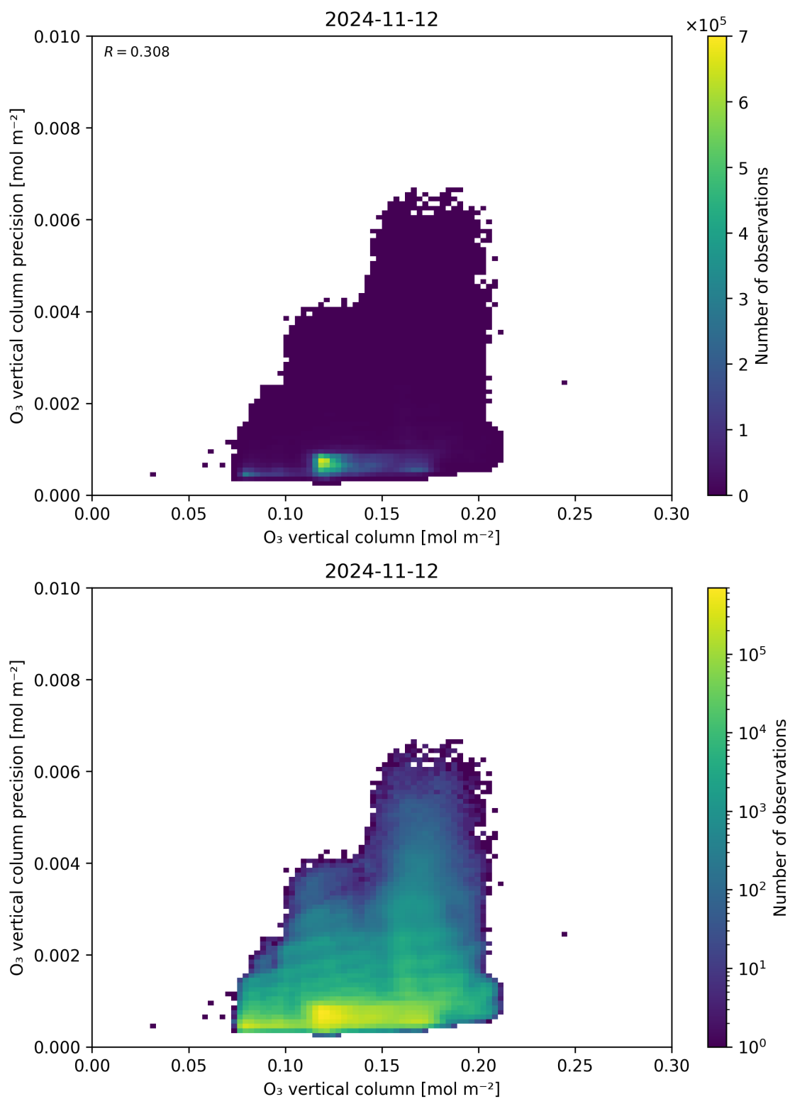
Figure 41: Scatter density plot of “O 3 vertical column” against “O 3 vertical column precision” for 2024-11-11 to 2024-11-13.
