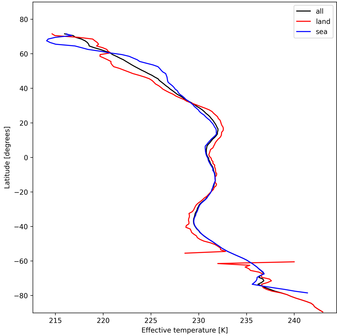
Figure 17: Zonal average of "Effective temperature" for 2024-11-11 to 2024-11-13.
