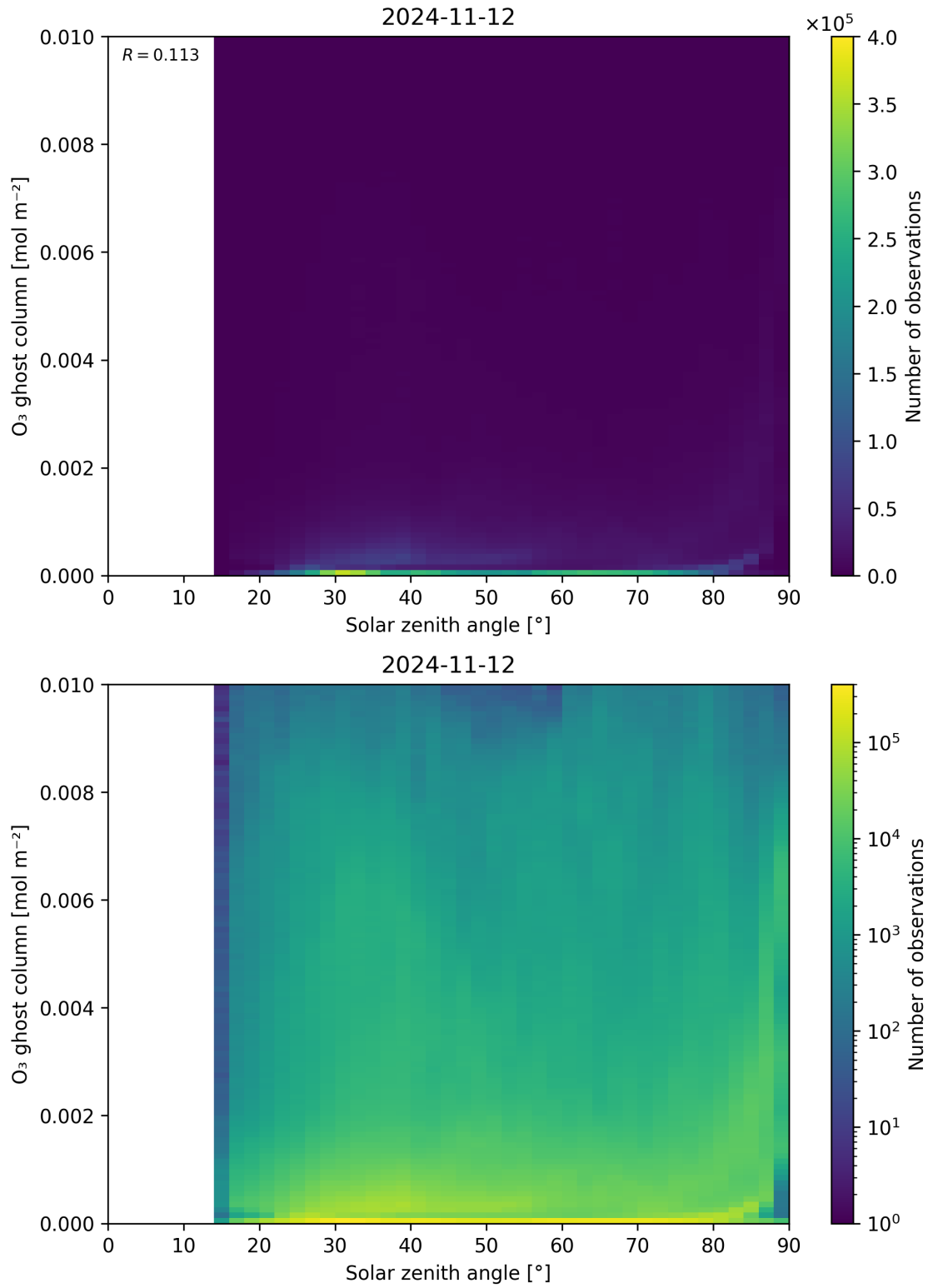
Figure 46: Scatter density plot of “Solar zenith angle” against “O 3 ghost column” for 2024-11-11 to 2024-11-13.
