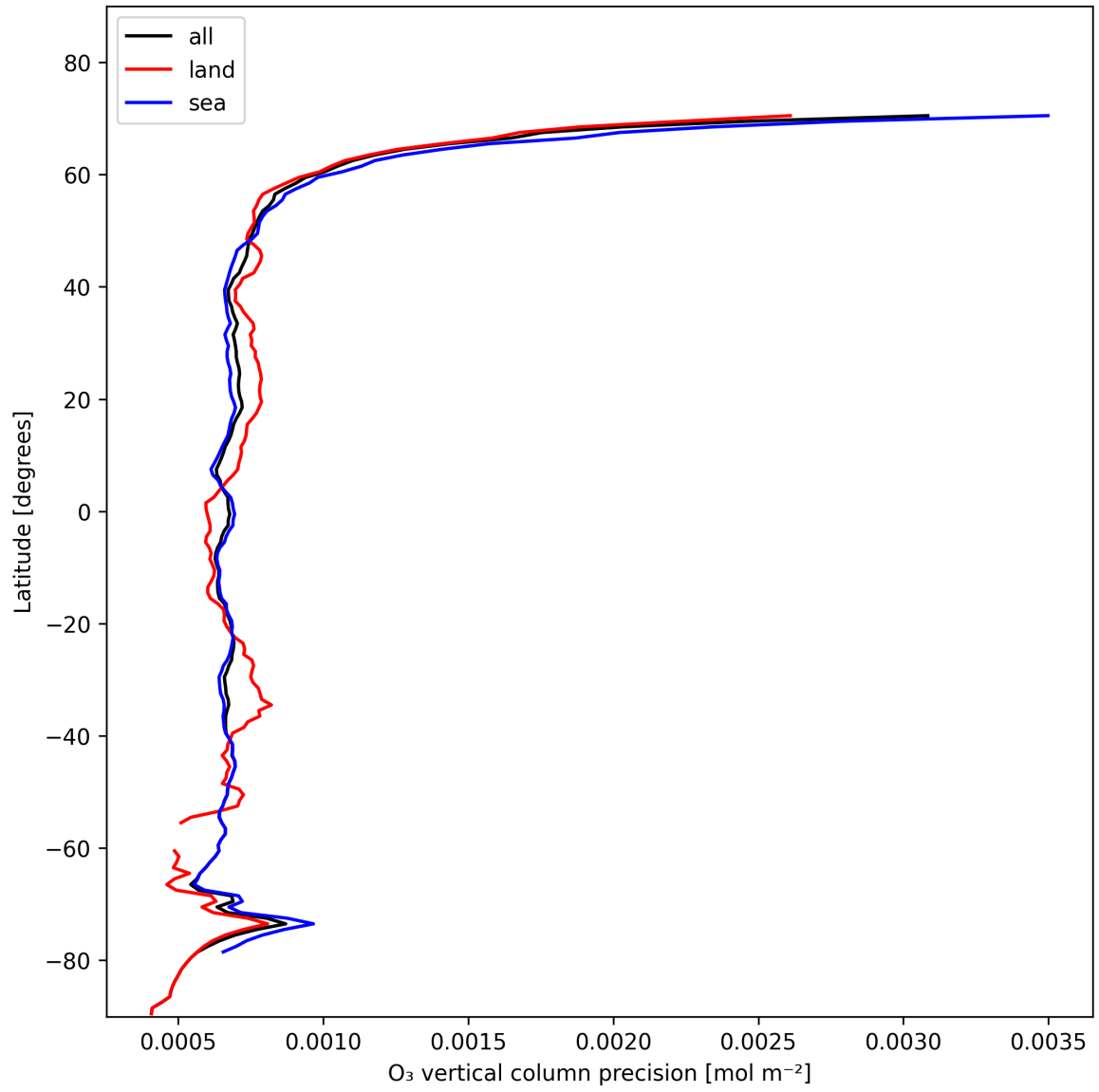
Figure 15: Zonal average of “O 3 vertical column precision” for 2024-11-12 to 2024-11-14.
