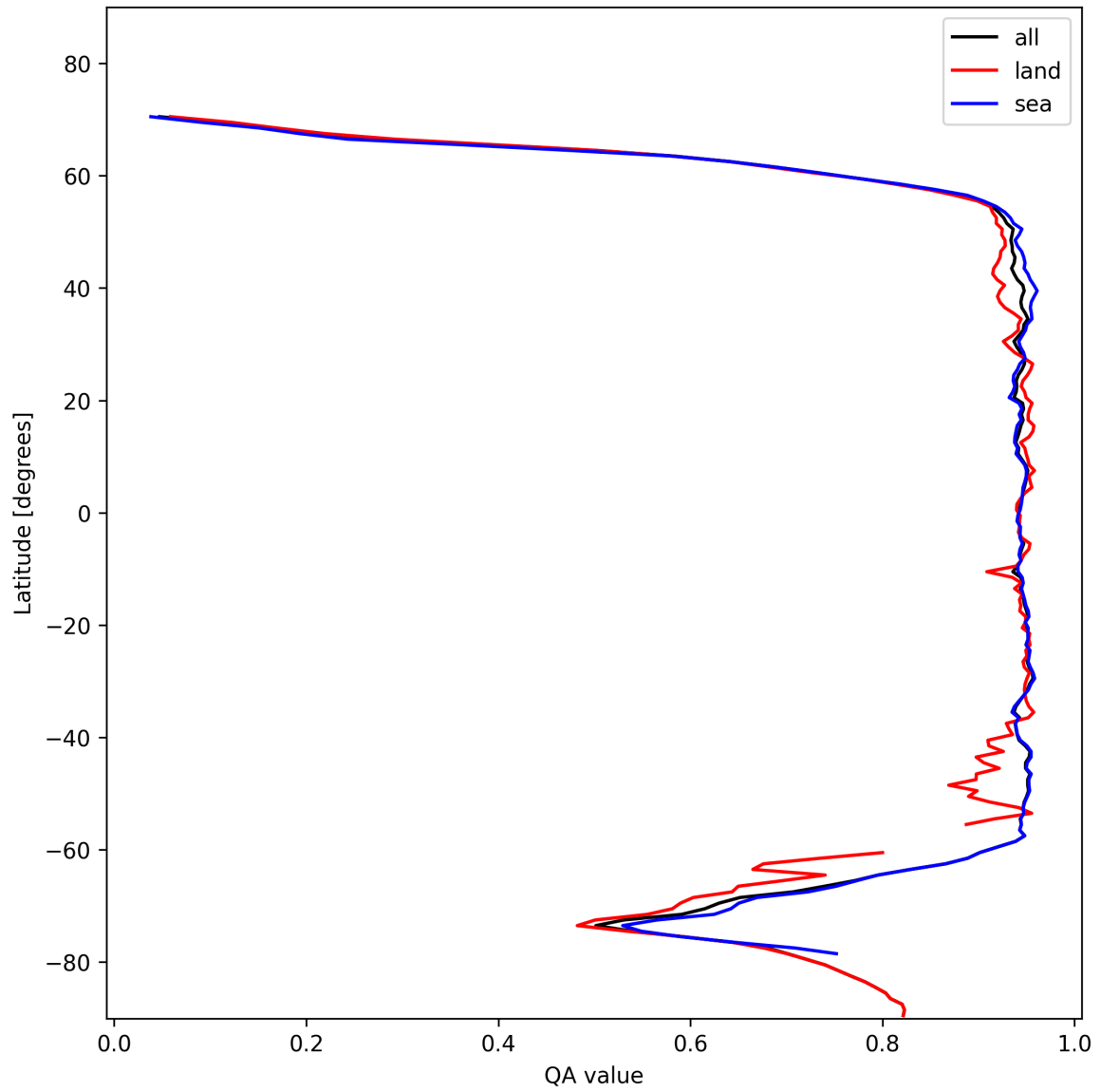
Figure 13: Zonal average of “QA value” for 2024-11-12 to 2024-11-14.
