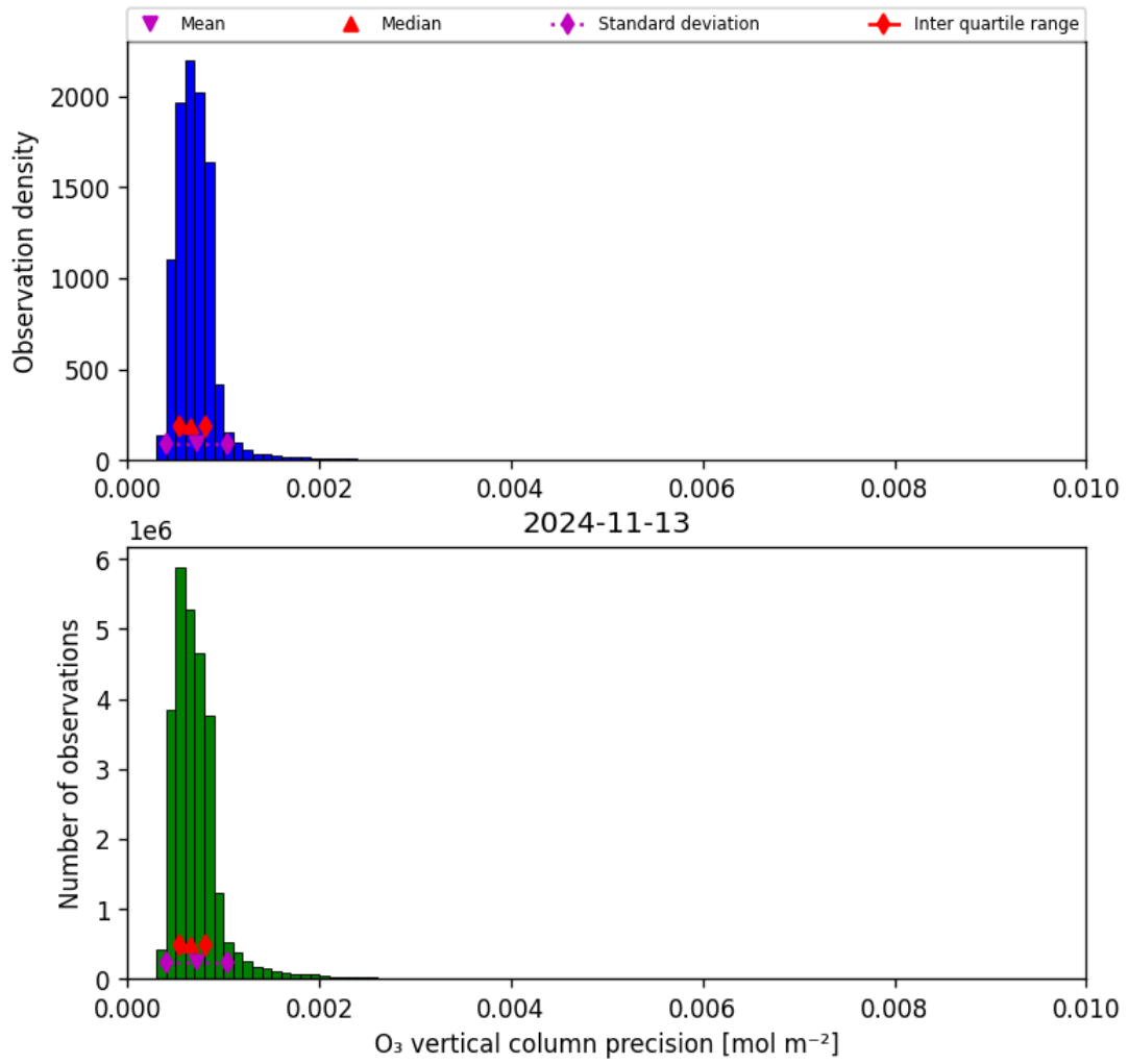
Figure 22: Histogram of “O 3 vertical column precision” for 2024-11-12 to 2024-11-14
