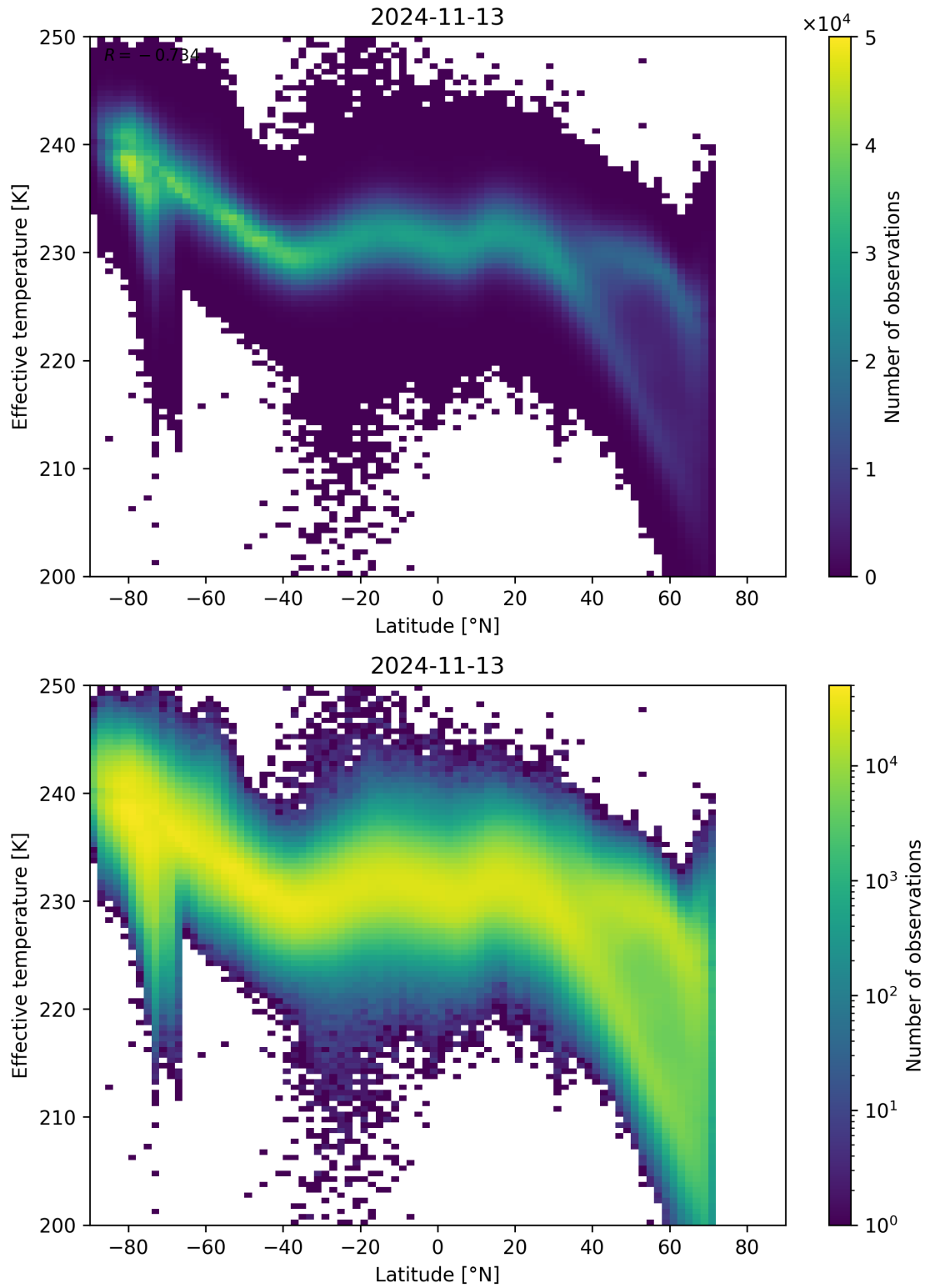
Figure 34: Scatter density plot of “Latitude” against “Effective temperature” for 2024-11-12 to 2024-11-14.
