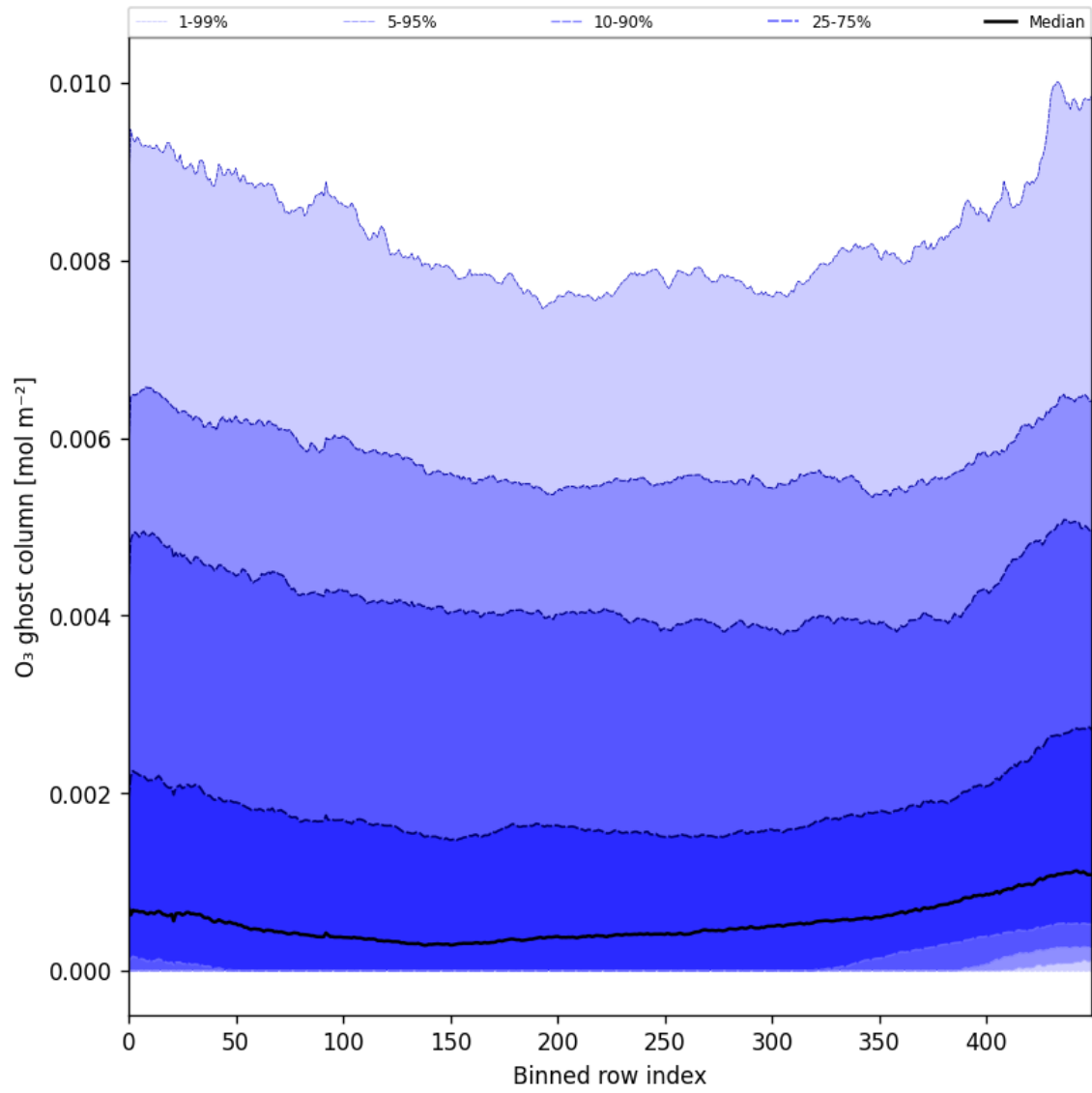
Figure 32: Along track statistics of “O 3 ghost column” for 2024-11-12 to 2024-11-14
