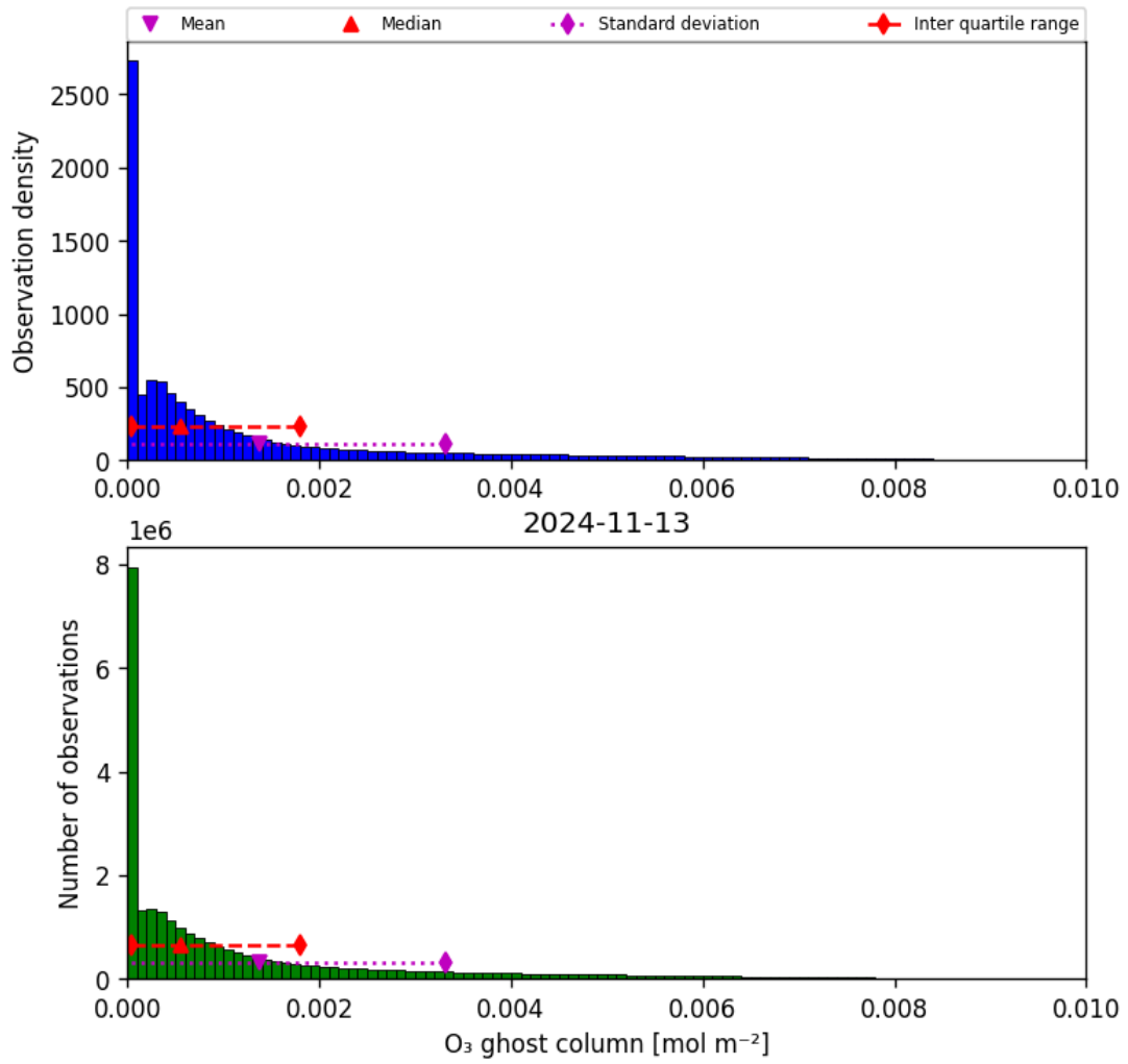
Figure 25: Histogram of “O 3 ghost column” for 2024-11-12 to 2024-11-14
