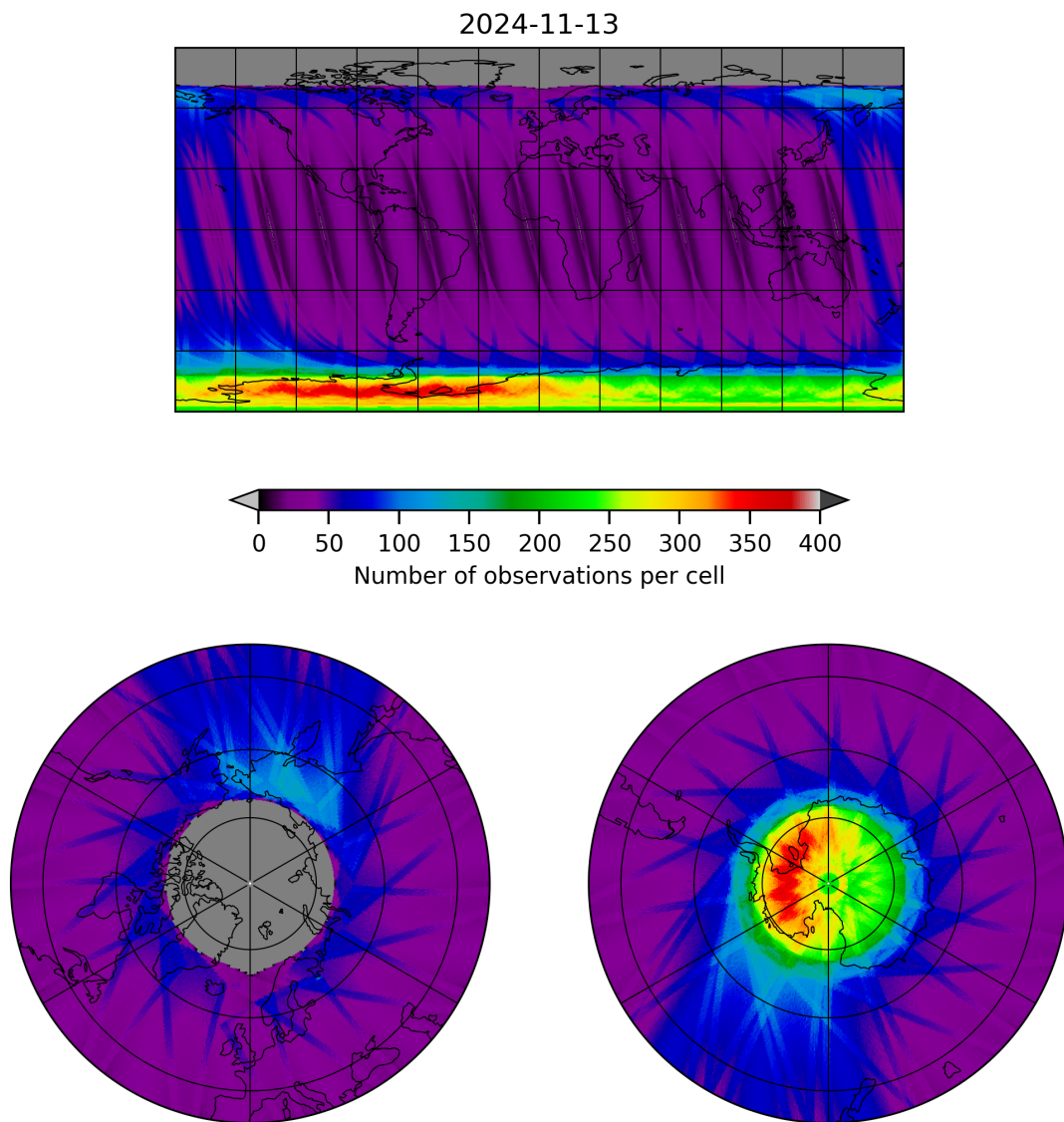
Figure 12: Map of the number of observations for 2024-11-12 to 2024-11-14
