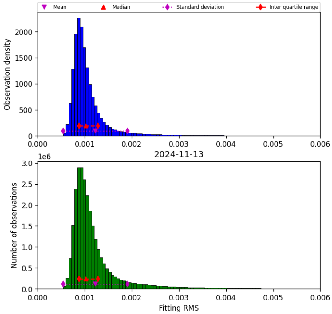
Figure 23: Histogram of “Fitting RMS” for 2024-11-12 to 2024-11-14
