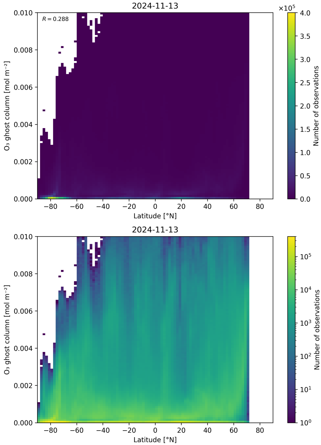
Figure 35: Scatter density plot of “Latitude” against “O 3 ghost column” for 2024-11-12 to 2024-11-14.
