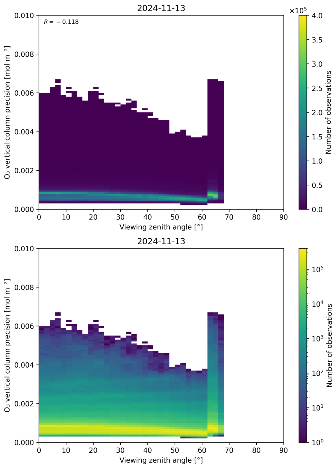
Figure 53: Scatter density plot of “Viewing zenith angle” against “O 3 vertical column precision” for 2024-11-12 to 2024-11-14.
