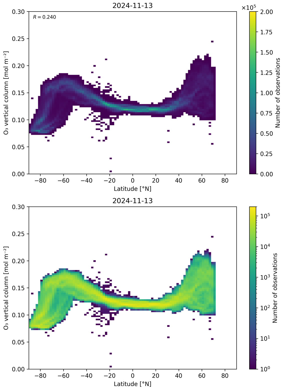
Figure 36: Scatter density plot of “Latitude” against “O 3 vertical column” for 2024-11-12 to 2024-11-14.
