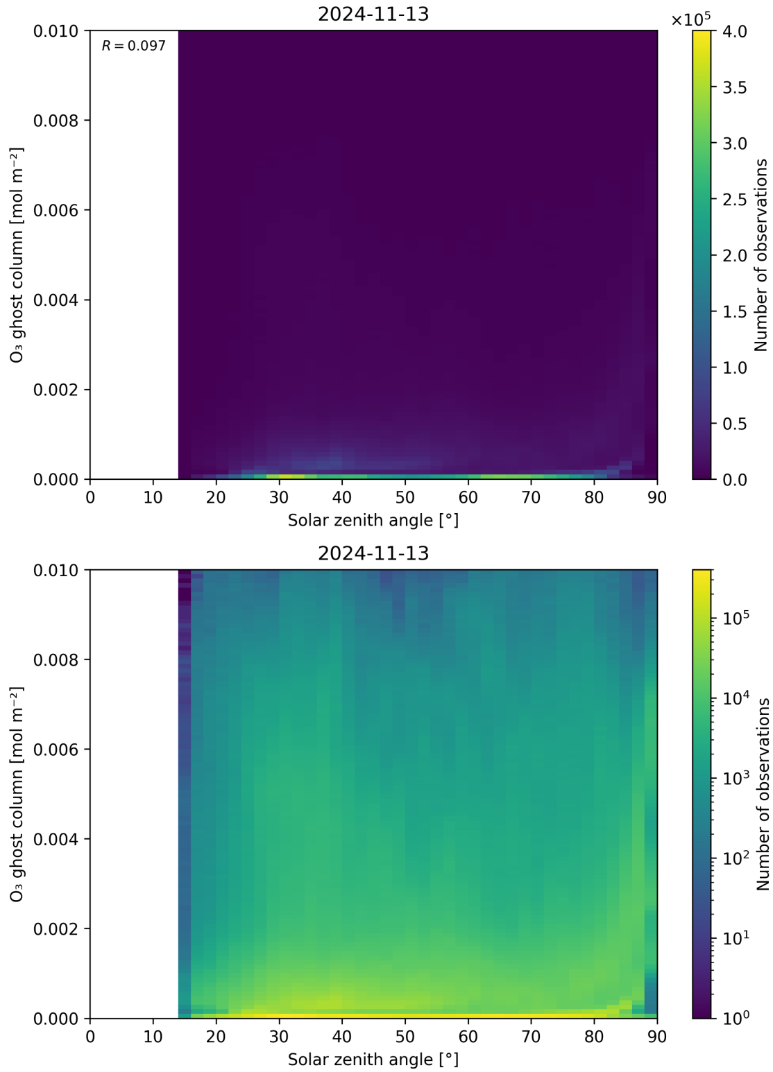
Figure 46: Scatter density plot of “Solar zenith angle” against “O 3 ghost column” for 2024-11-12 to 2024-11-14.
