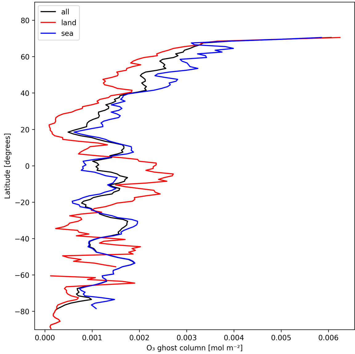
Figure 18: Zonal average of "O 3 ghost column" for 2024-11-12 to 2024-11-14.
