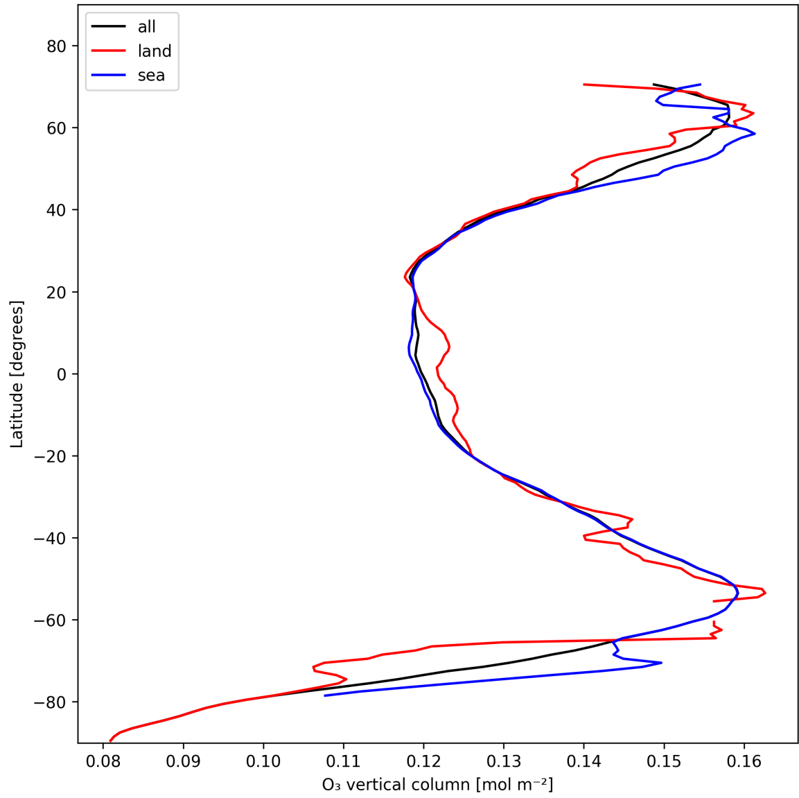
Figure 14: Zonal average of “O 3 vertical column” for 2024-11-12 to 2024-11-14.
