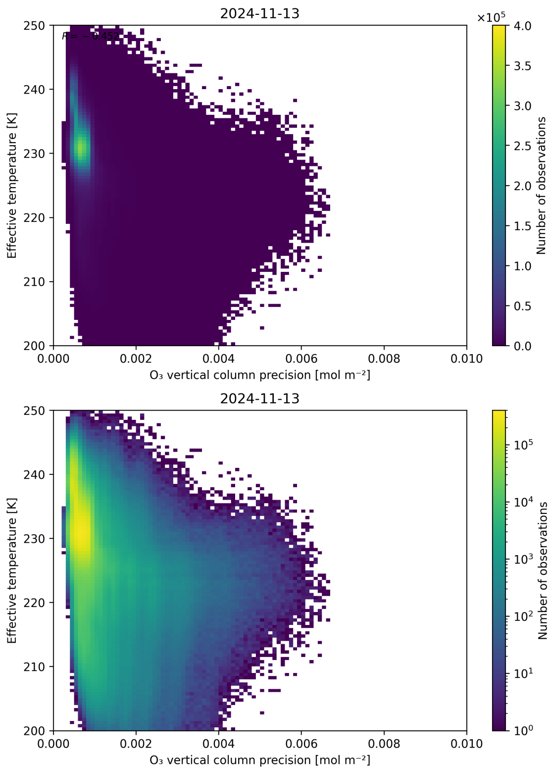
Figure 42: Scatter density plot of “O 3 vertical column precision” against “Effective temperature” for 2024-11-12 to 2024-11-14.
