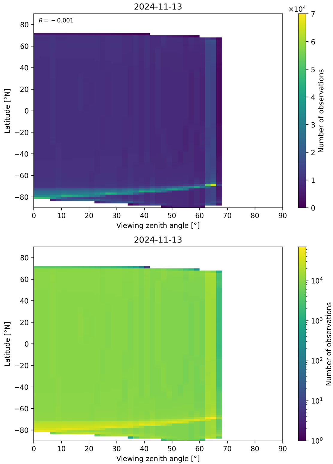
Figure 49: Scatter density plot of “Viewing zenith angle” against “Latitude” for 2024-11-12 to 2024-11-14.
