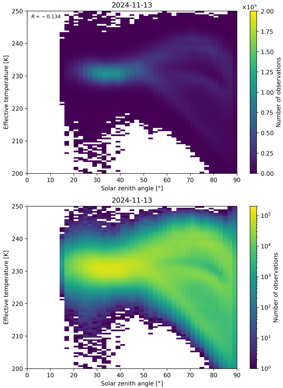
Figure 45: Scatter density plot of “Solar zenith angle” against “Effective temperature” for 2024-11-12 to 2024-11-14.
