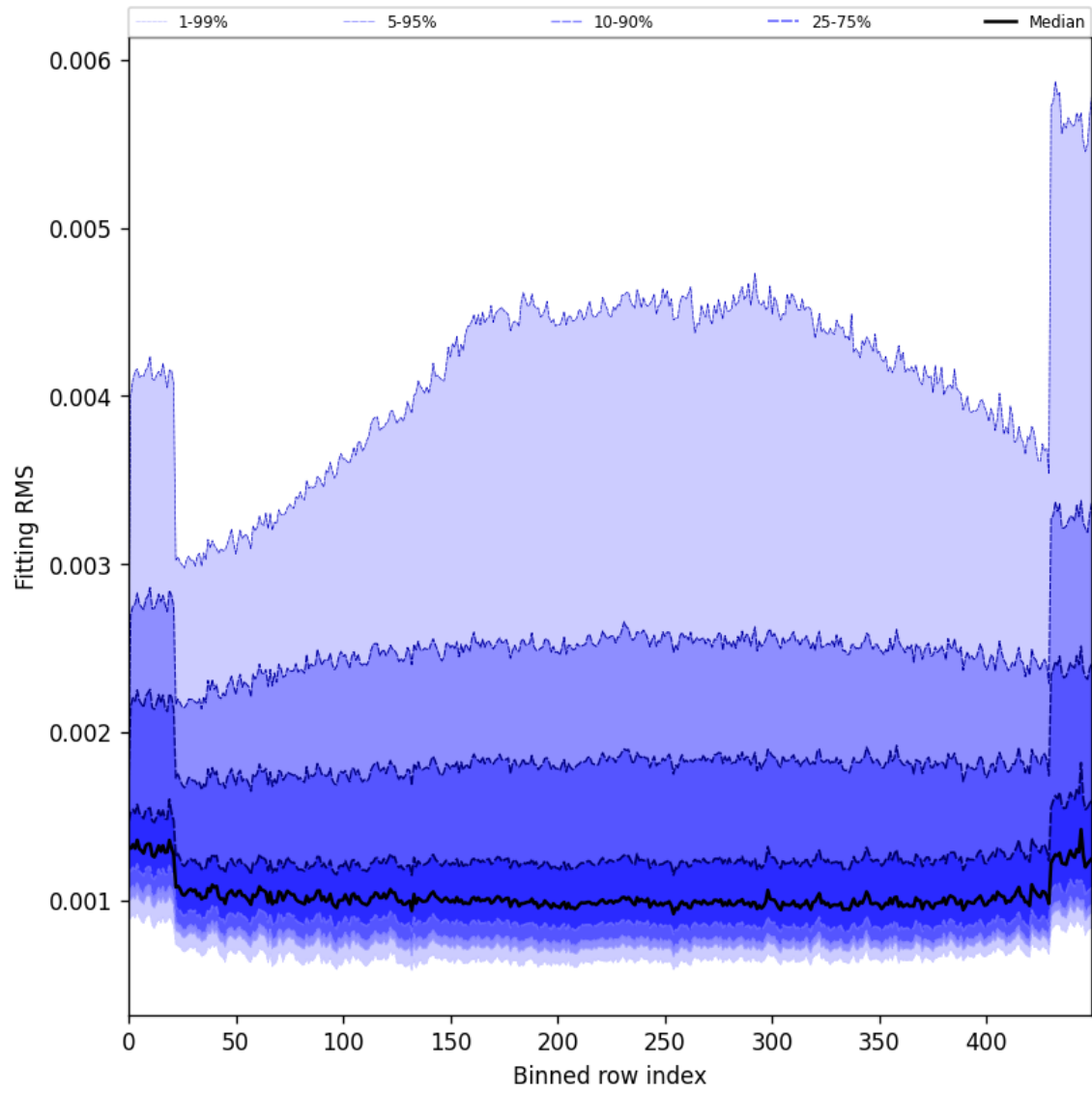
Figure 30: Along track statistics of “Fitting RMS” for 2024-11-12 to 2024-11-14
