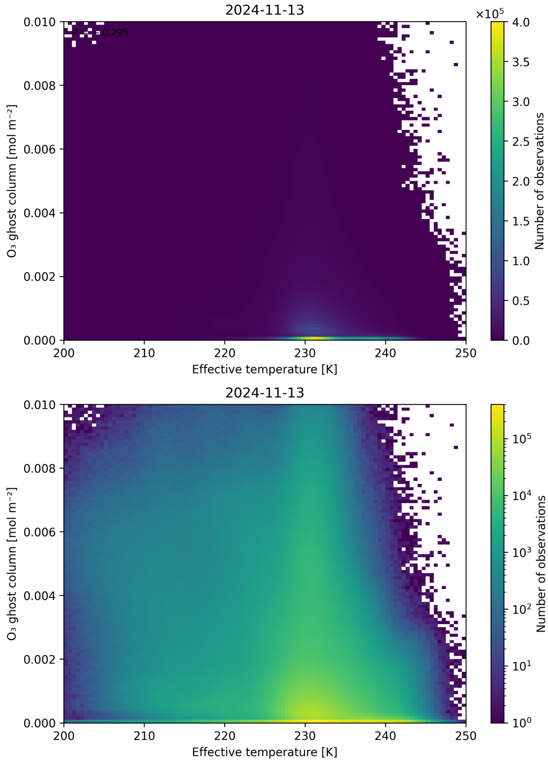
Figure 38: Scatter density plot of “Effective temperature” against “O 3 ghost column” for 2024-11-12 to 2024-11-14.
