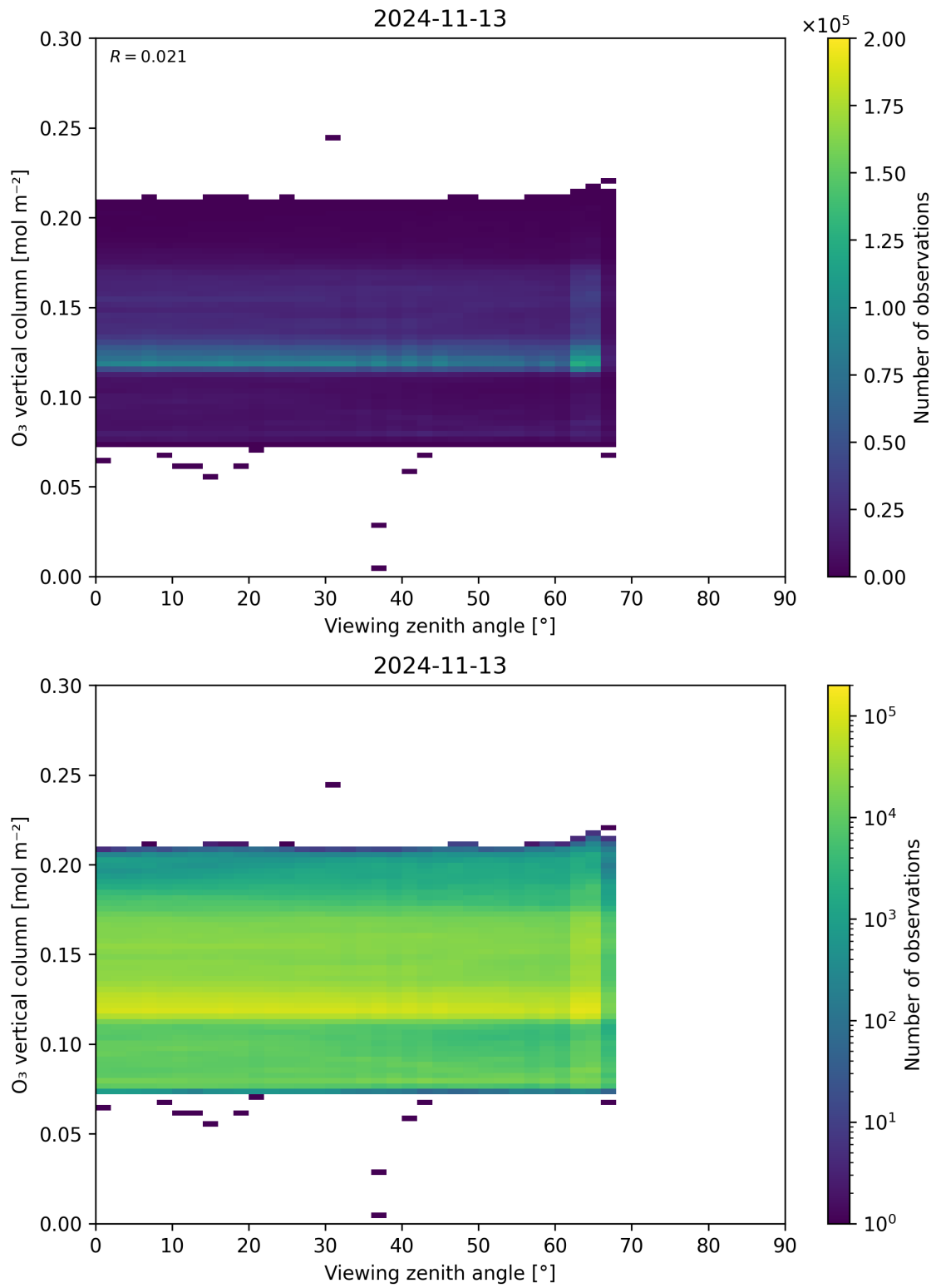
Figure 52: Scatter density plot of “Viewing zenith angle” against “O 3 vertical column” for 2024-11-12 to 2024-11-14.
