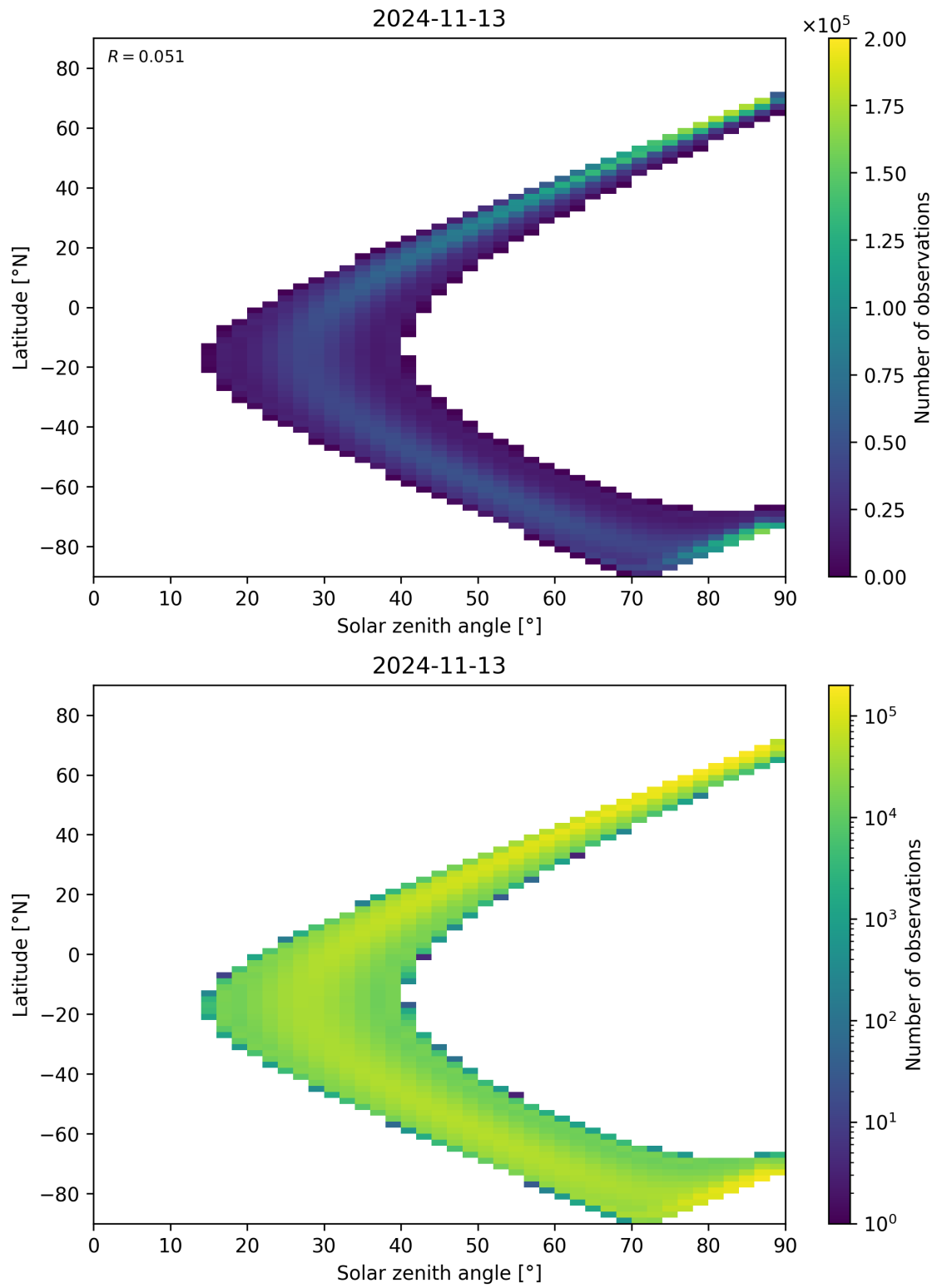
Figure 44: Scatter density plot of “Solar zenith angle” against “Latitude” for 2024-11-12 to 2024-11-14.
