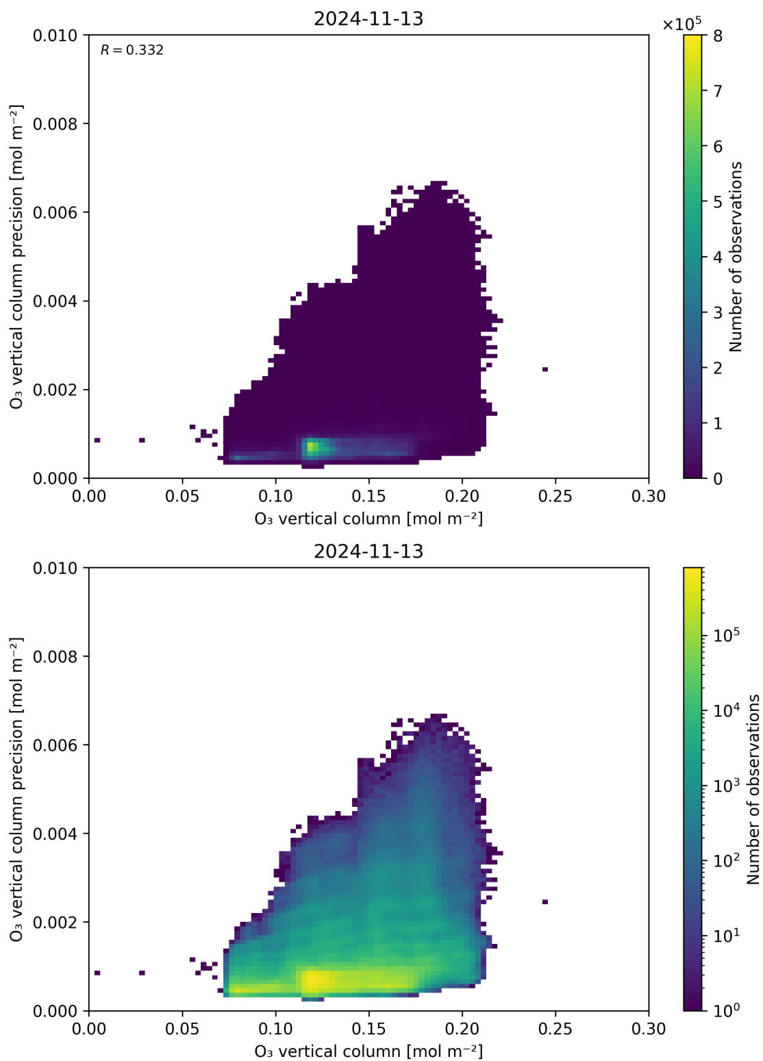
Figure 41: Scatter density plot of “O 3 vertical column” against “O 3 vertical column precision” for 2024-11-12 to 2024-11-14.
