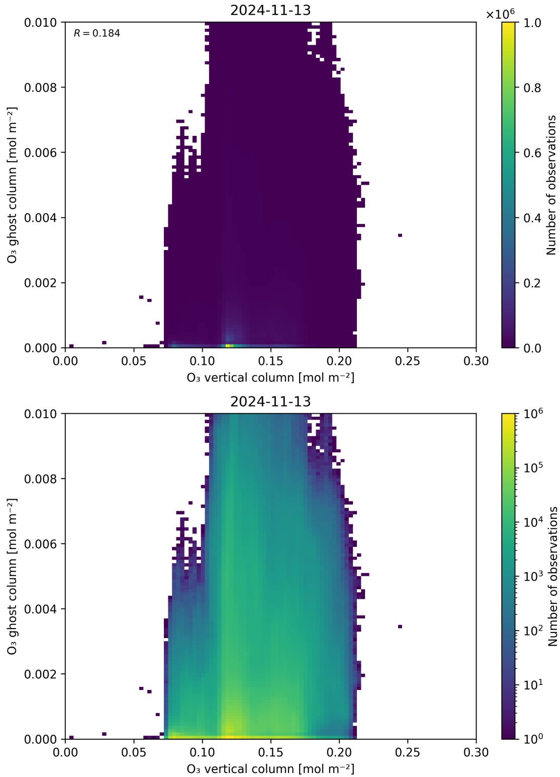
Figure 40: Scatter density plot of “O 3 vertical column” against “O 3 ghost column” for 2024-11-12 to 2024-11-14.
