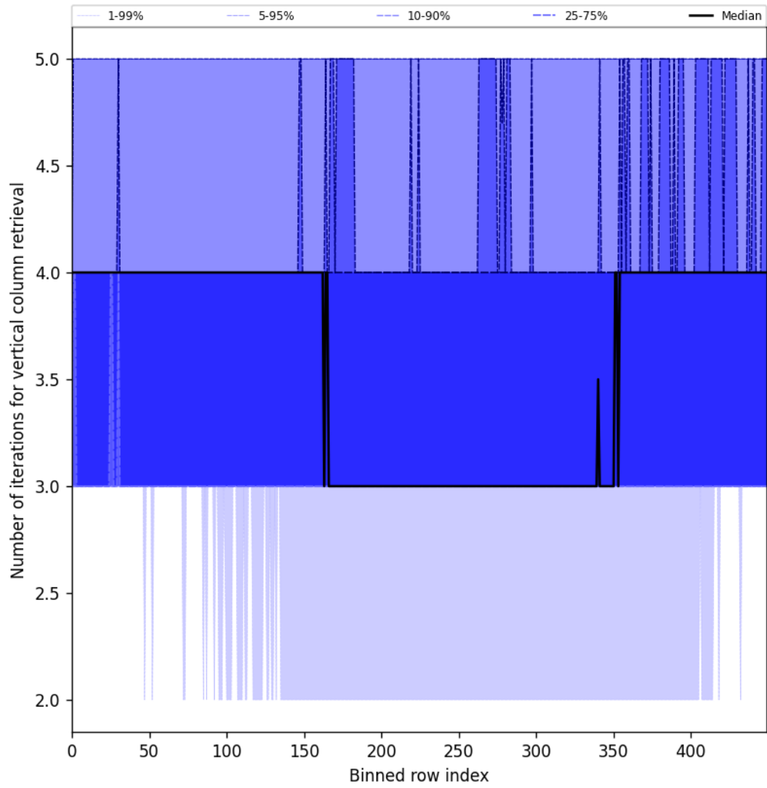
Figure 33: Along track statistics of “Number of iterations for vertical column retrieval” for 2024-11-12 to 2024-11-14
