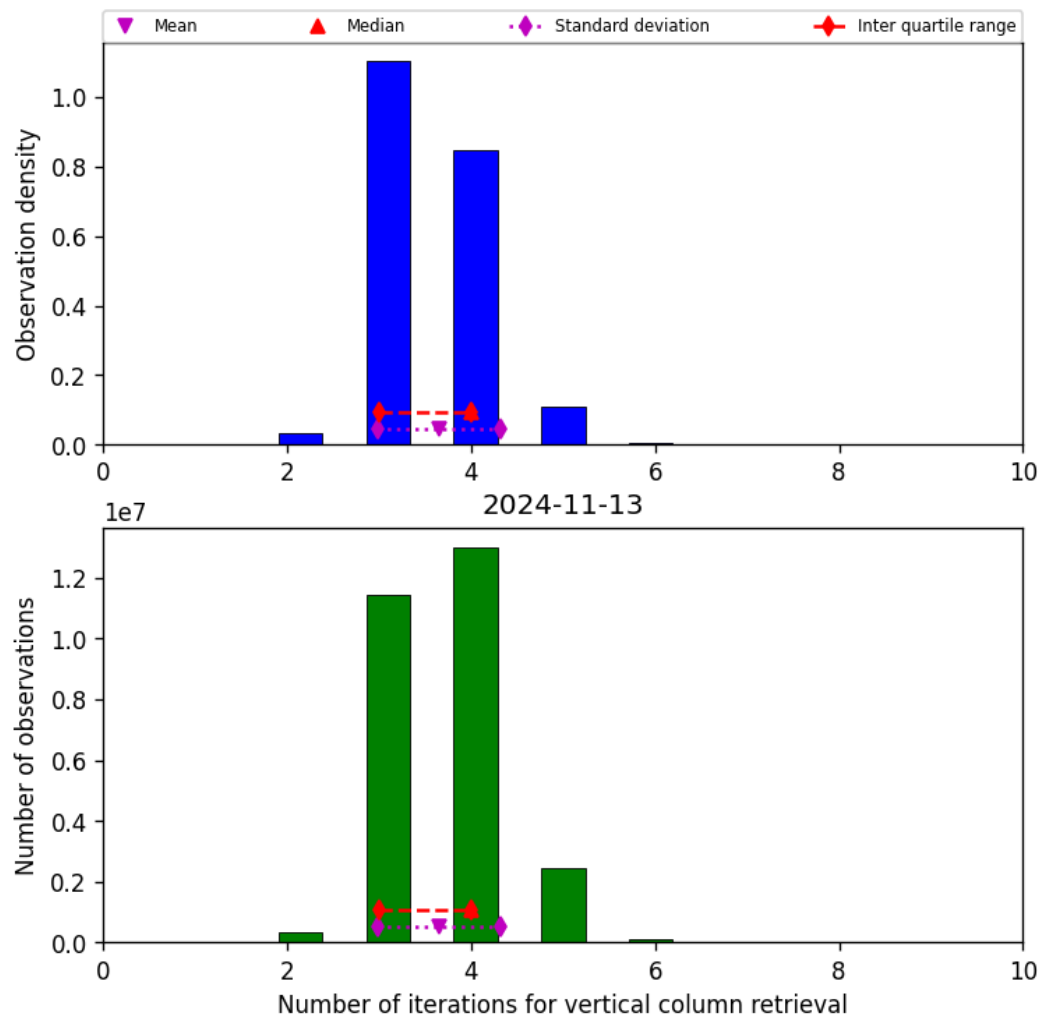
Figure 26: Histogram of “Number of iterations for vertical column retrieval” for 2024-11-12 to 2024-11-14
