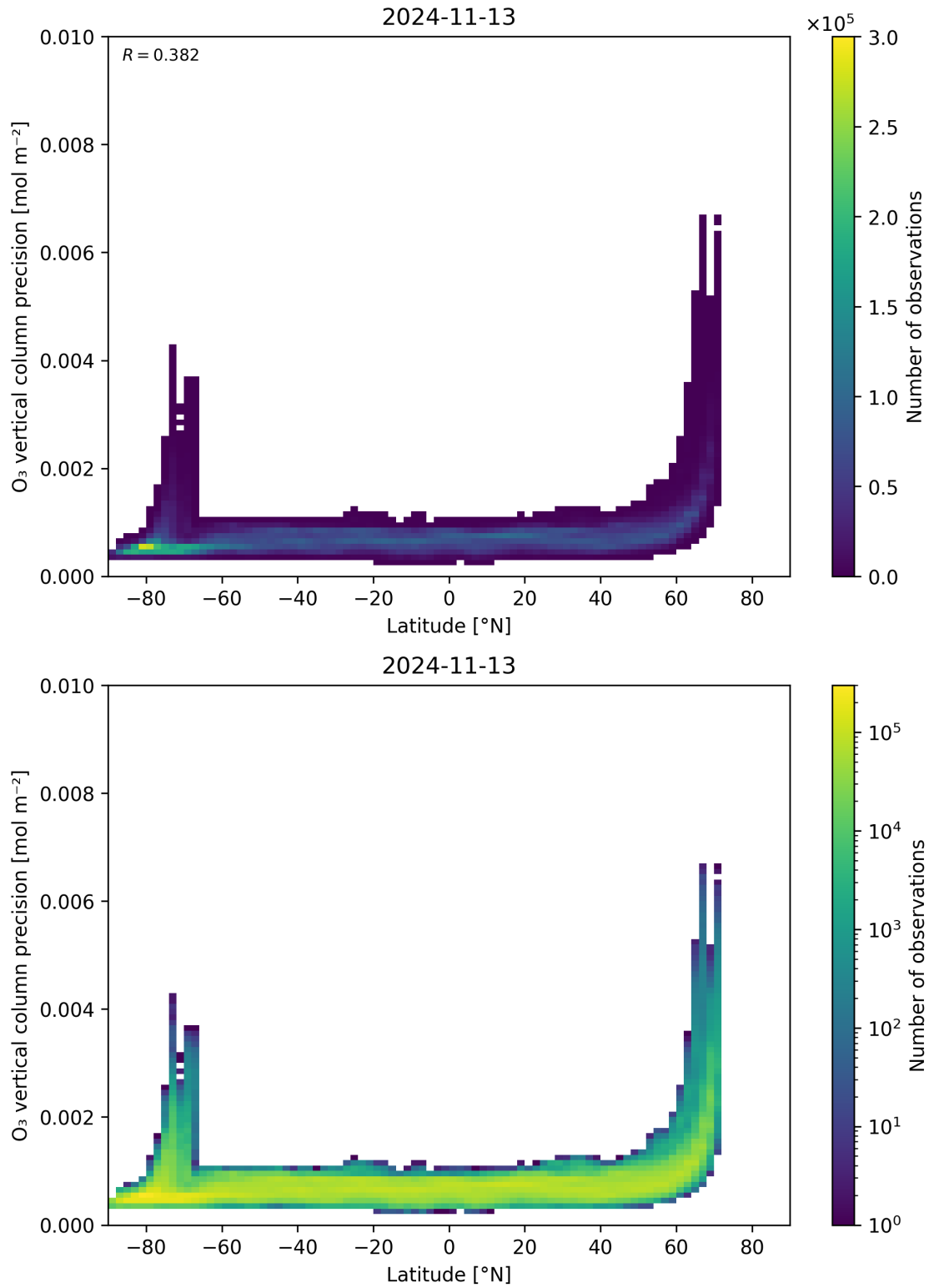
Figure 37: Scatter density plot of “Latitude” against “O 3 vertical column precision” for 2024-11-12 to 2024-11-14.
