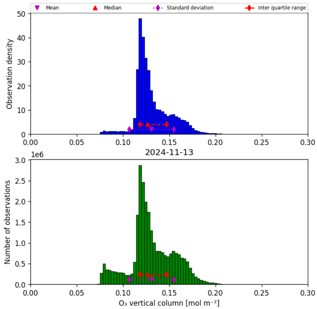
Figure 21: Histogram of “O 3 vertical column” for 2024-11-12 to 2024-11-14
