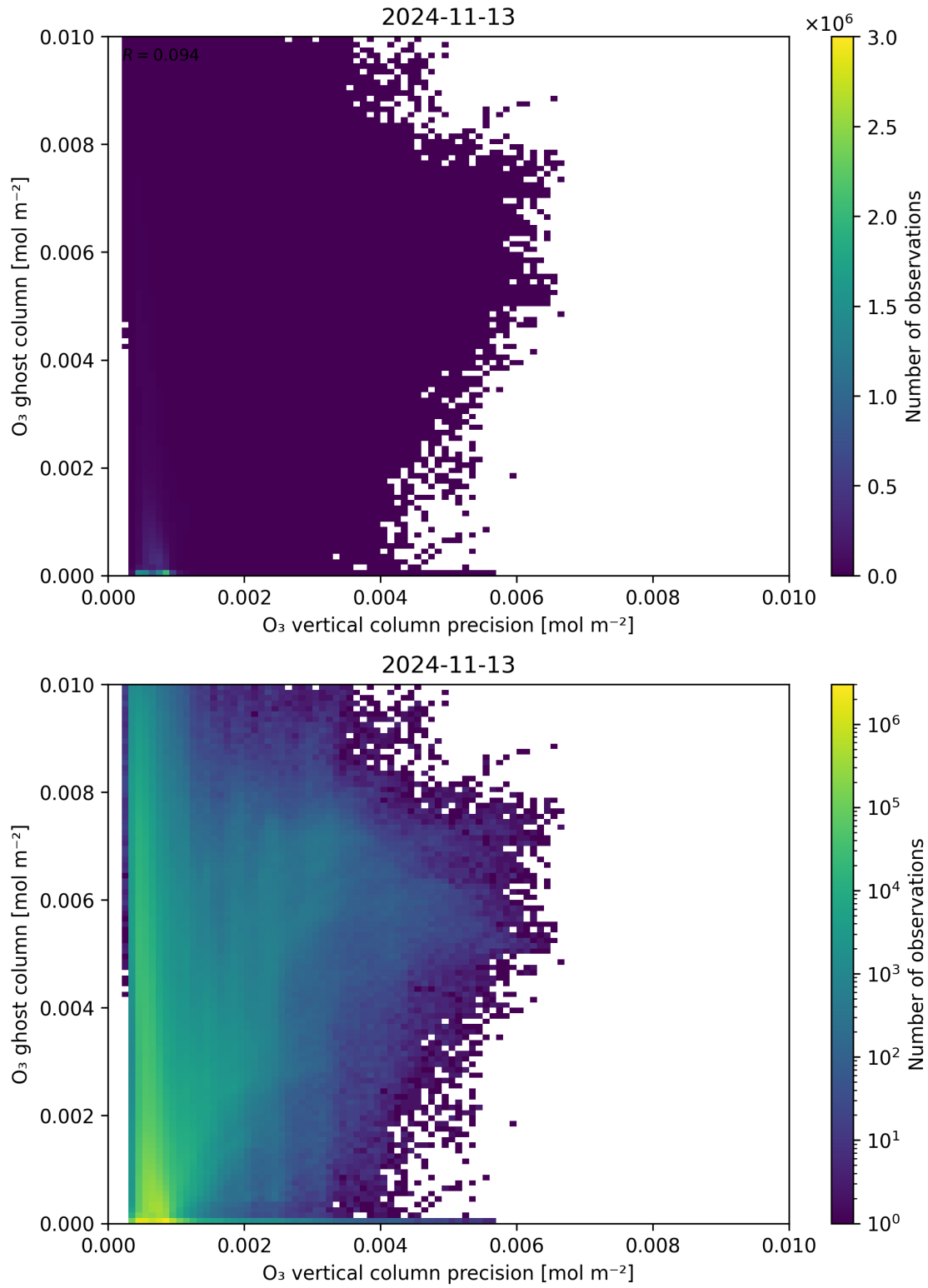
Figure 43: Scatter density plot of “ \text{O}_3 vertical column precision” against “ \text{O}_3 ghost column” for 2024-11-12 to 2024-11-14.
