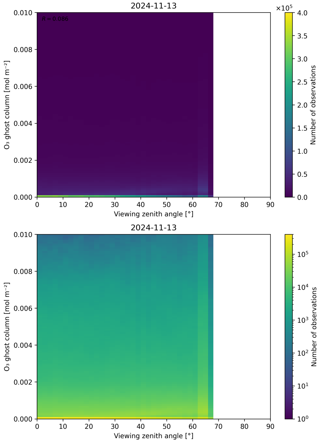
Figure 51: Scatter density plot of “Viewing zenith angle” against “O 3 ghost column” for 2024-11-12 to 2024-11-14.
