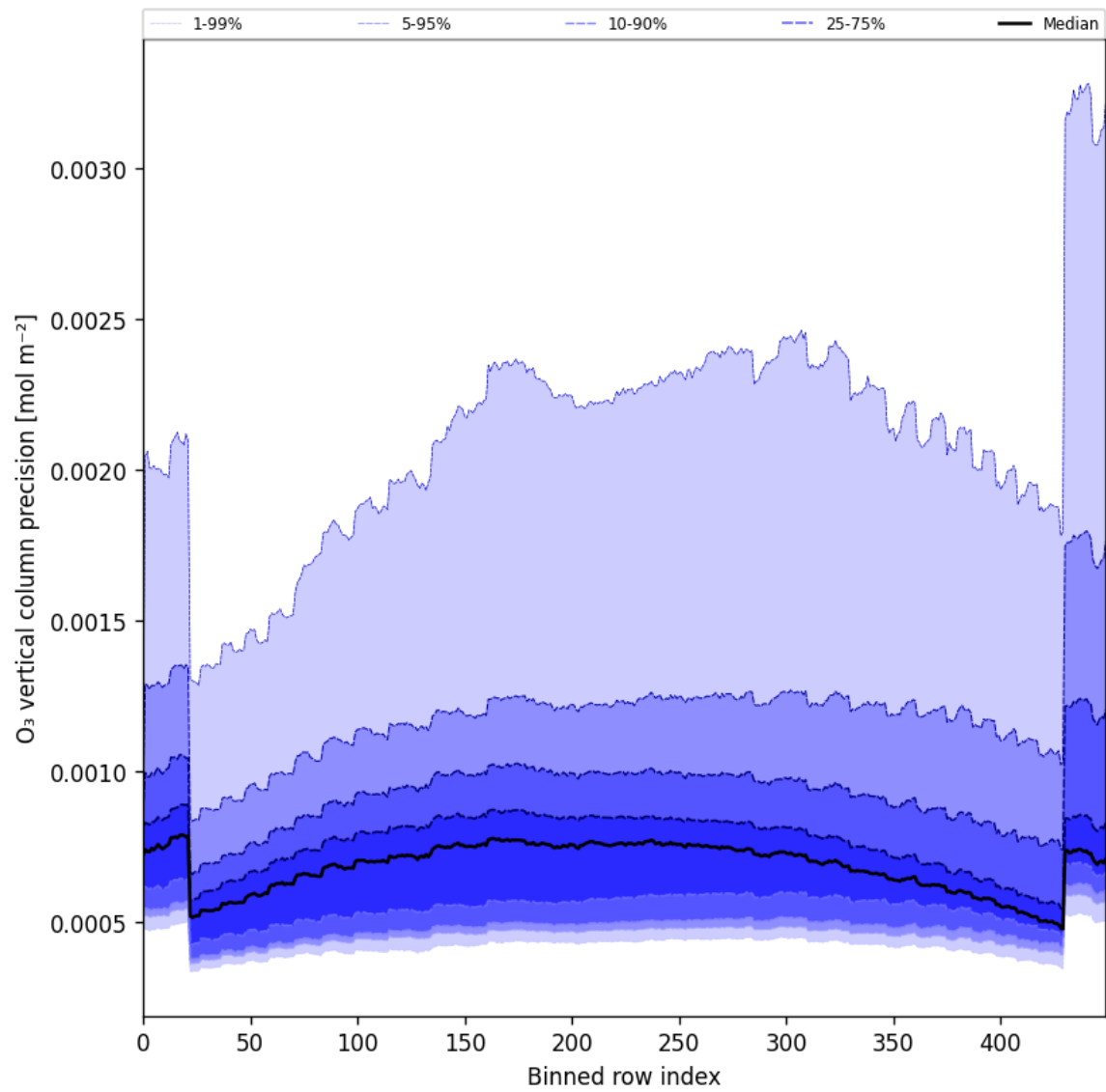
Figure 29: Along track statistics of “O 3 vertical column precision” for 2024-11-12 to 2024-11-14
