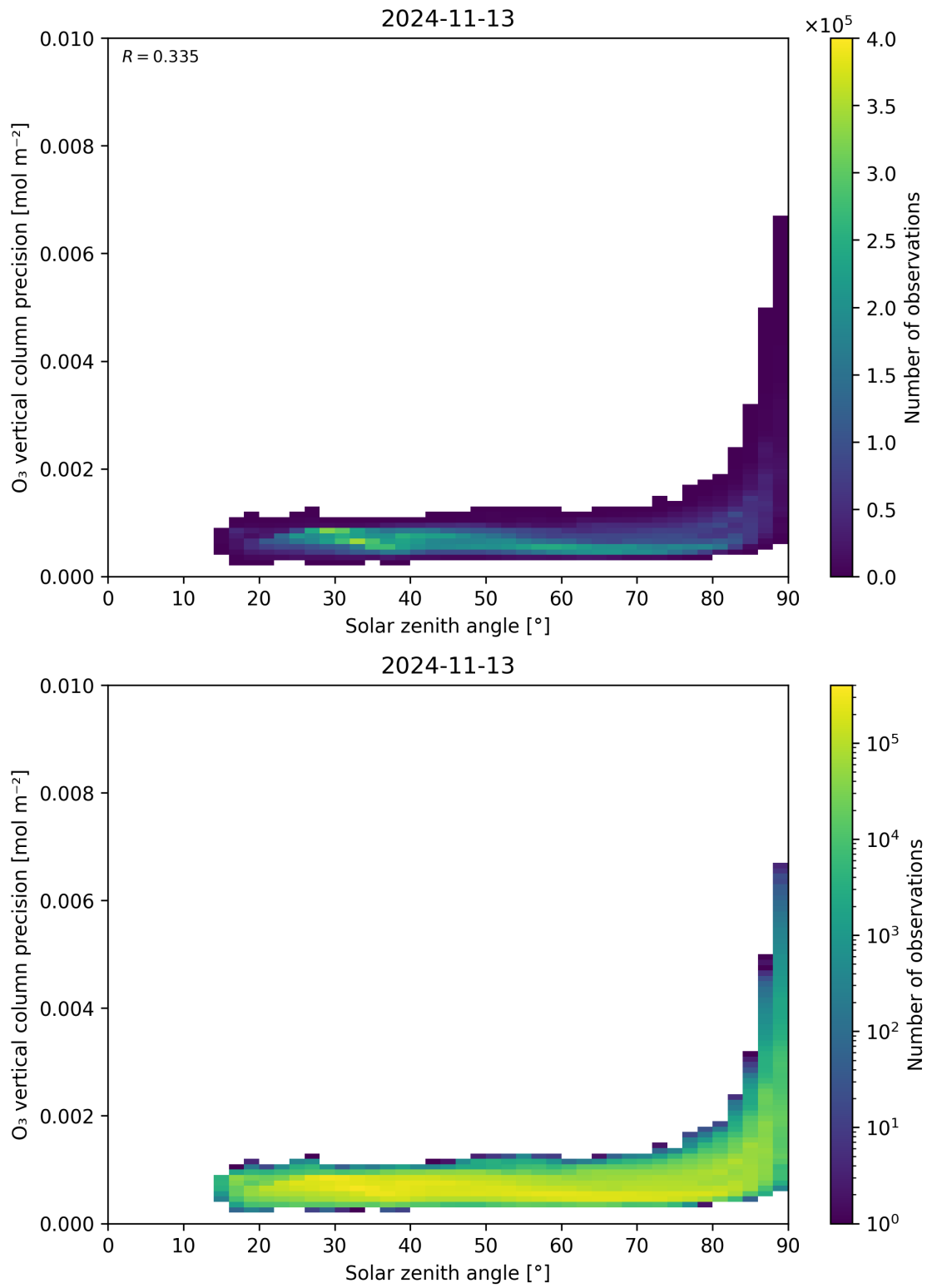
Figure 48: Scatter density plot of “Solar zenith angle” against “O 3 vertical column precision” for 2024-11-12 to 2024-11-14.
