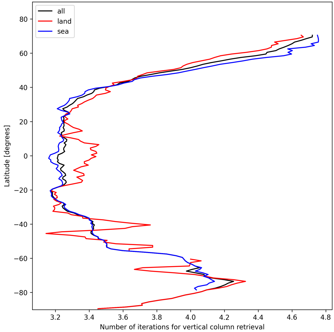
Figure 19: Zonal average of “Number of iterations for vertical column retrieval” for 2024-11-12 to 2024-11-14.
