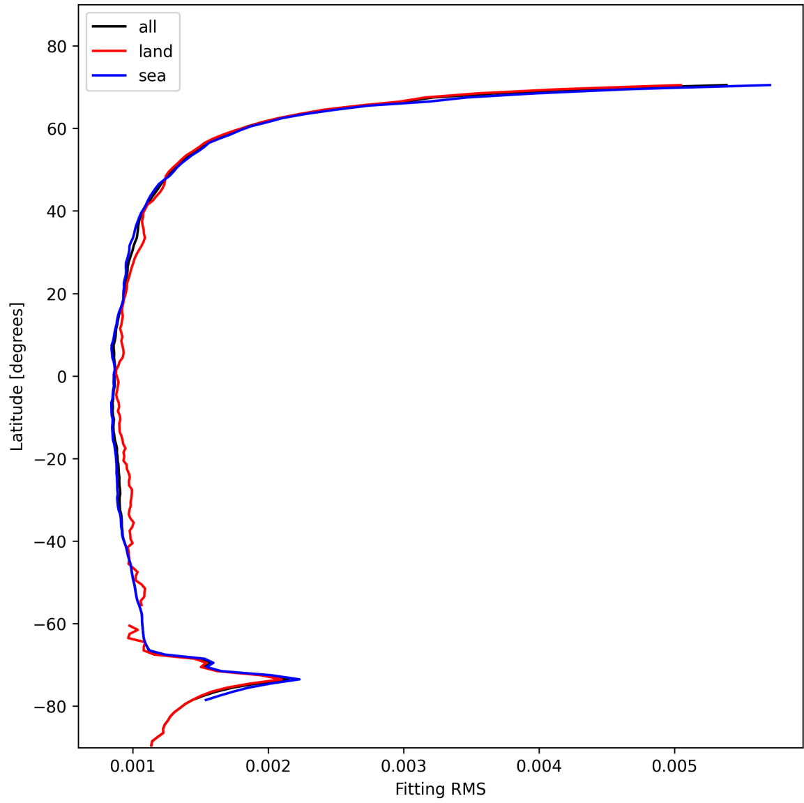
Figure 16: Zonal average of “Fitting RMS” for 2024-11-12 to 2024-11-14.
