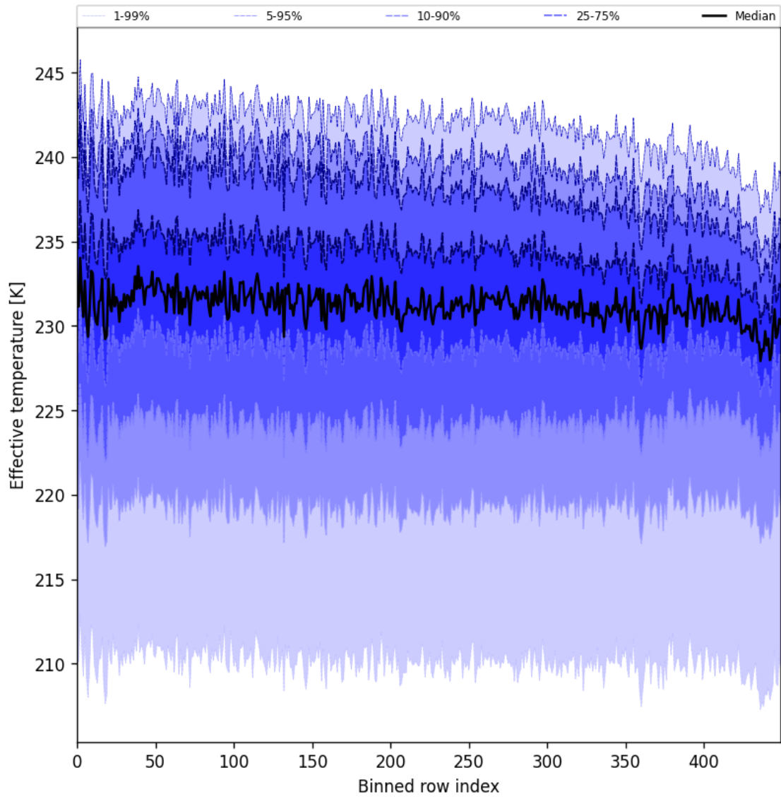
Figure 31: Along track statistics of “Effective temperature” for 2024-11-12 to 2024-11-14
