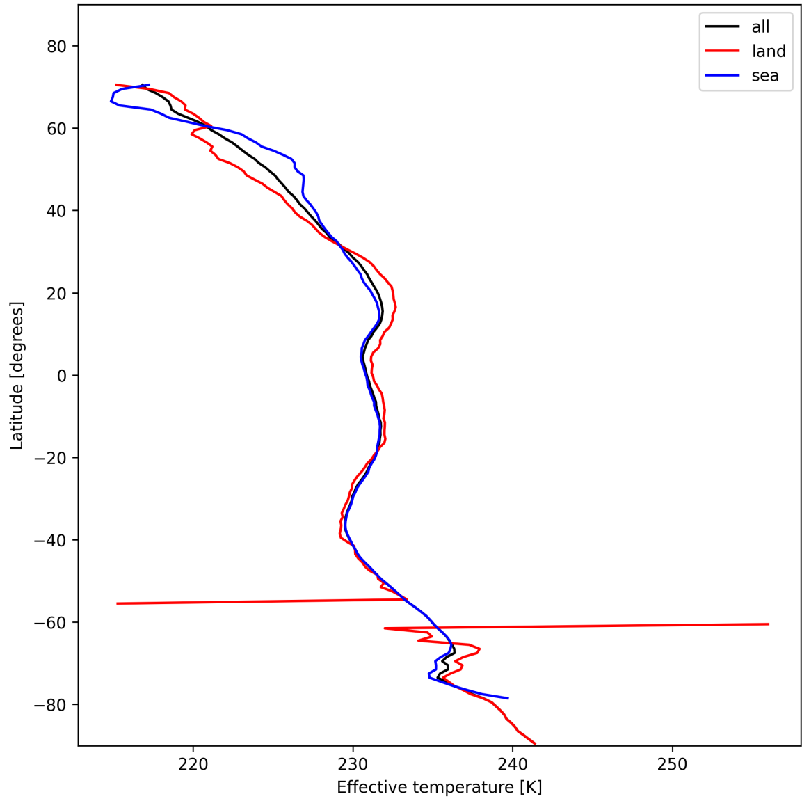
Figure 17: Zonal average of “Effective temperature” for 2024-11-12 to 2024-11-14.
