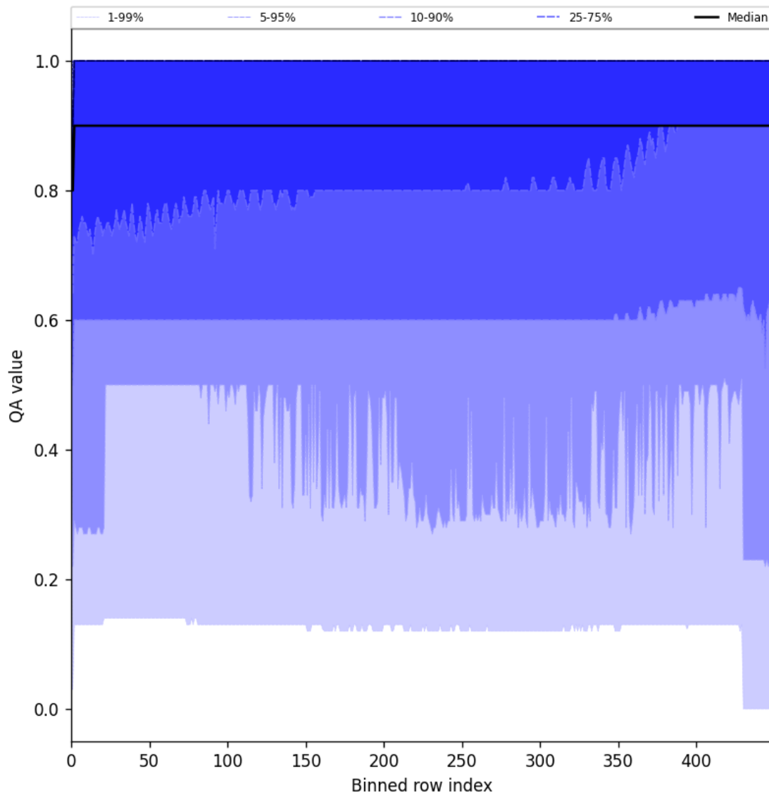
Figure 27: Along track statistics of “QA value” for 2024-11-12 to 2024-11-14
