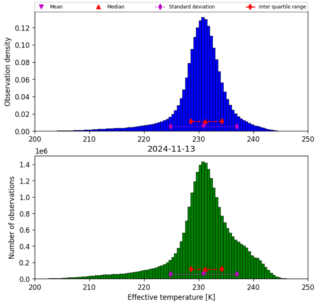
Figure 24: Histogram of “Effective temperature” for 2024-11-12 to 2024-11-14
