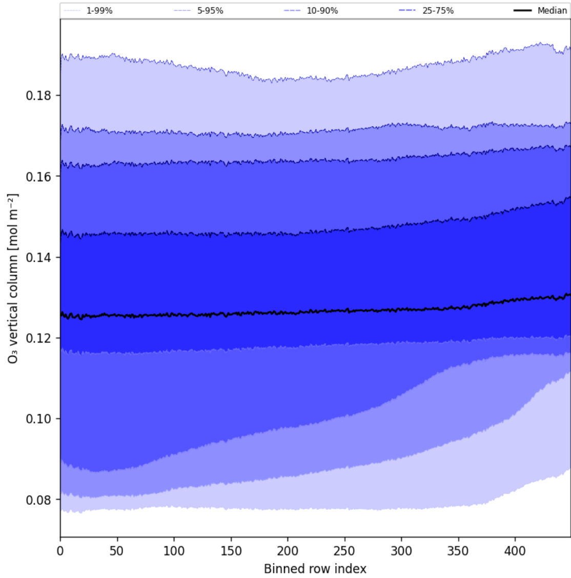
Figure 28: Along track statistics of “O 3 vertical column” for 2024-11-12 to 2024-11-14
