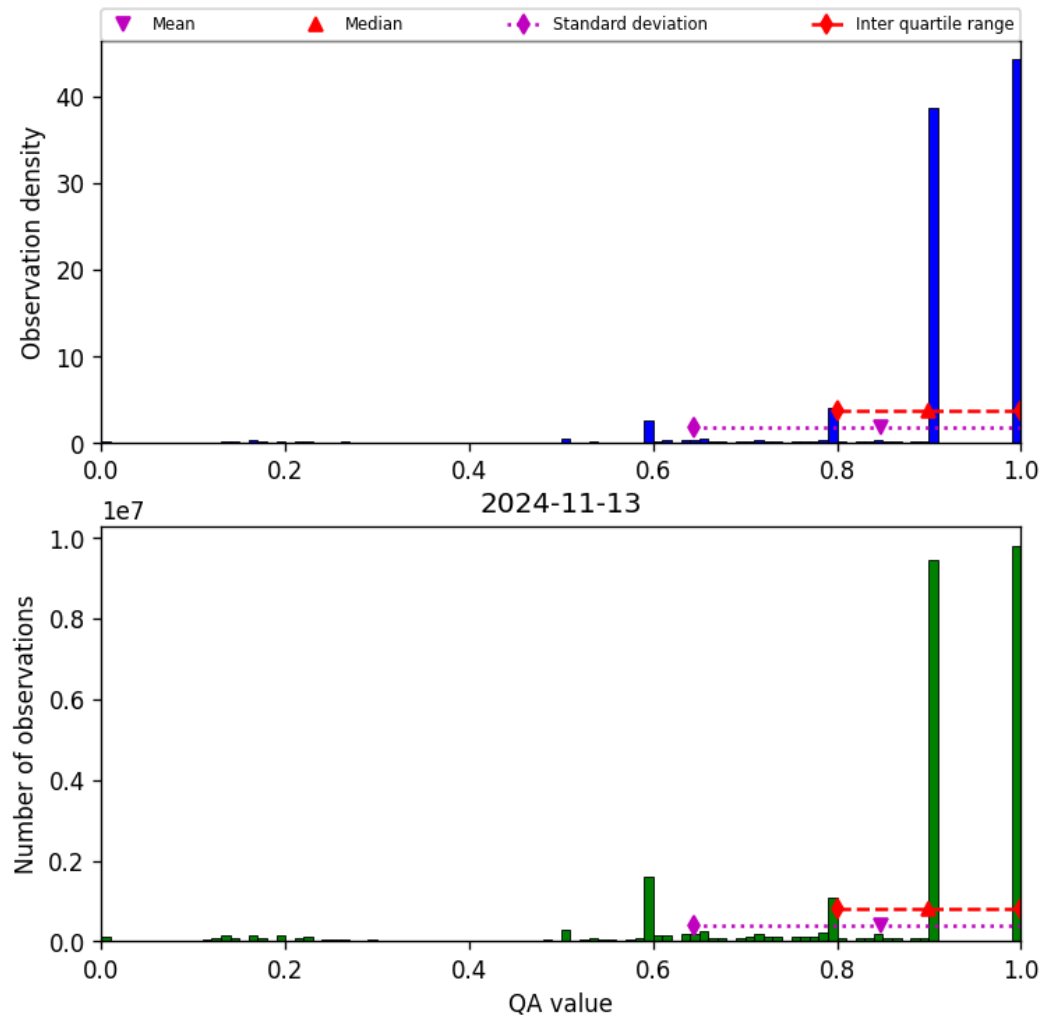
Figure 20: Histogram of “QA value” for 2024-11-12 to 2024-11-14
