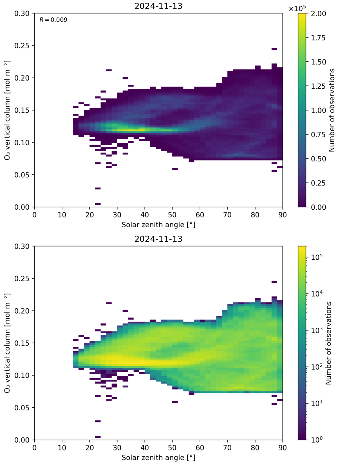
Figure 47: Scatter density plot of “Solar zenith angle” against “O 3 vertical column” for 2024-11-12 to 2024-11-14.
