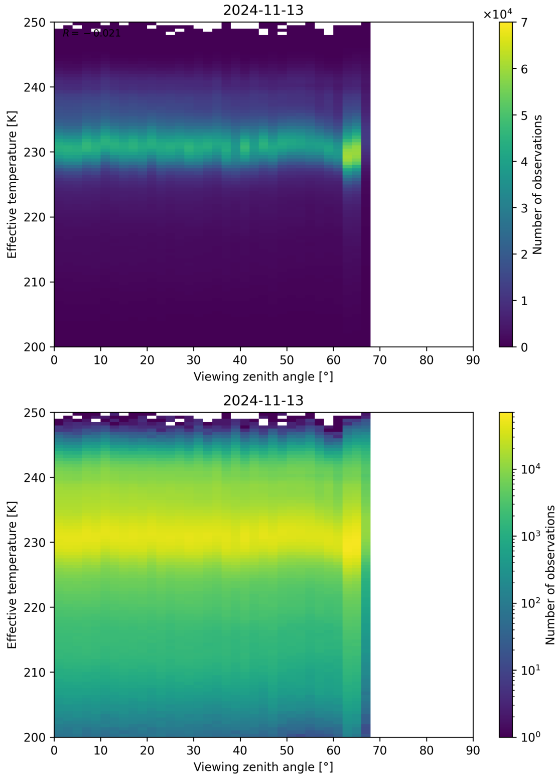
Figure 50: Scatter density plot of “Viewing zenith angle” against “Effective temperature” for 2024-11-12 to 2024-11-14.
