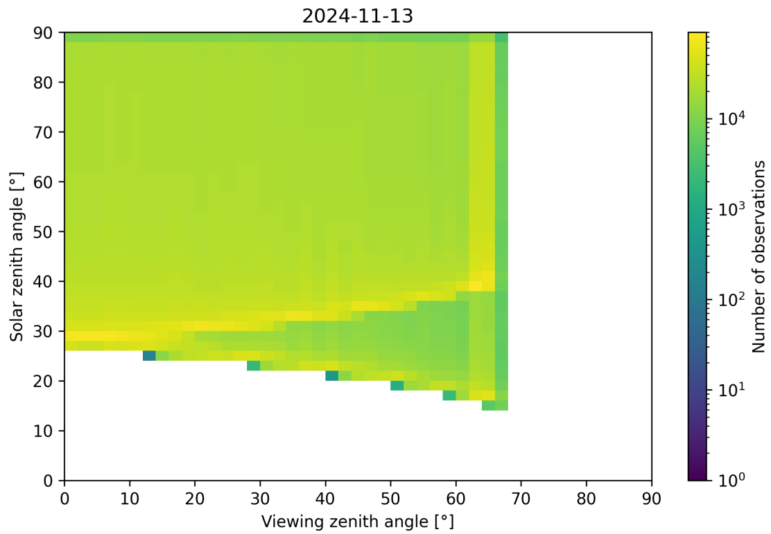
Figure 54: Scatter density plot of “Viewing zenith angle” against “Solar zenith angle” for 2024-11-12 to 2024-11-14.
