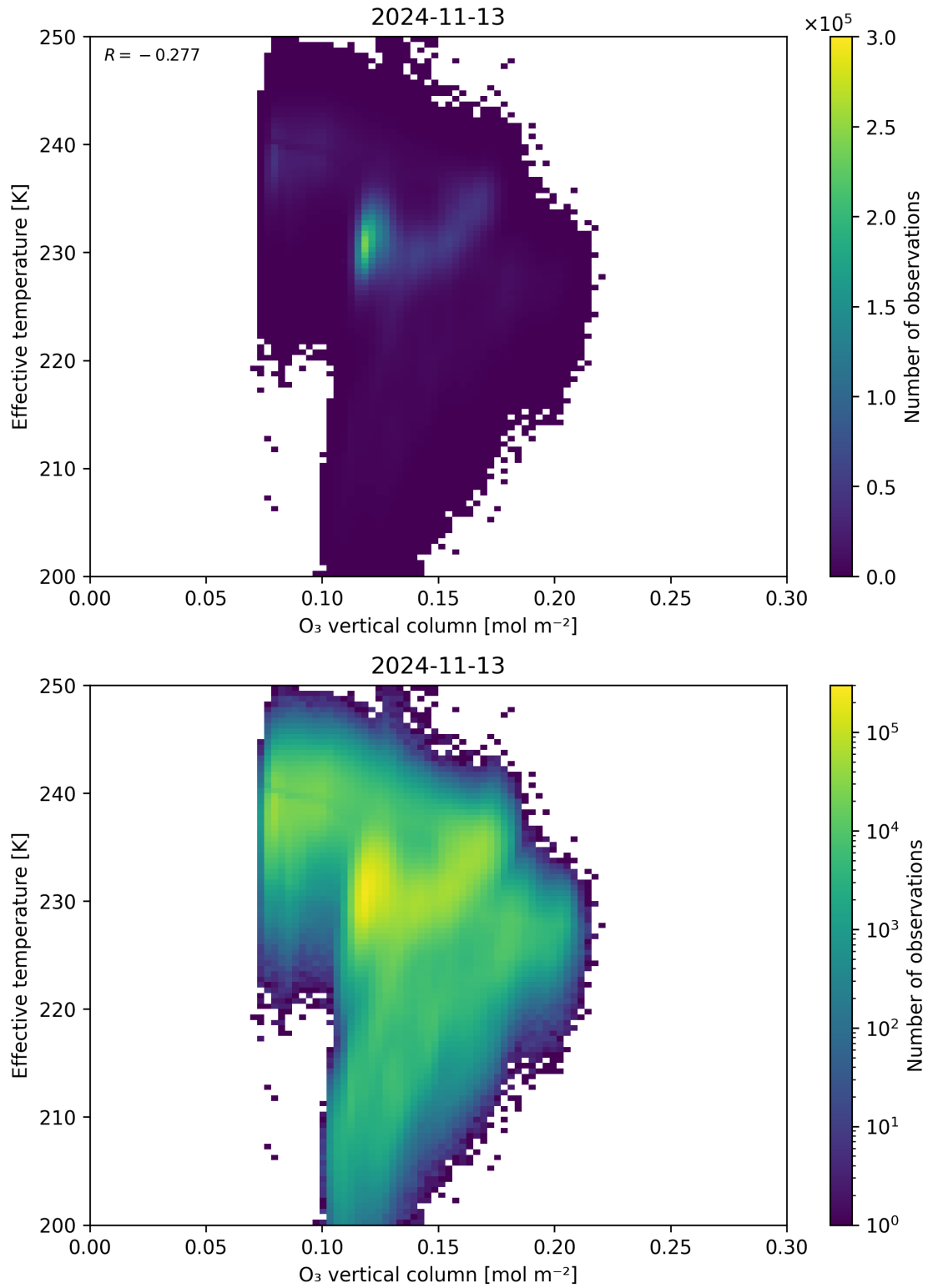
Figure 39: Scatter density plot of “O 3 vertical column” against “Effective temperature” for 2024-11-12 to 2024-11-14.
