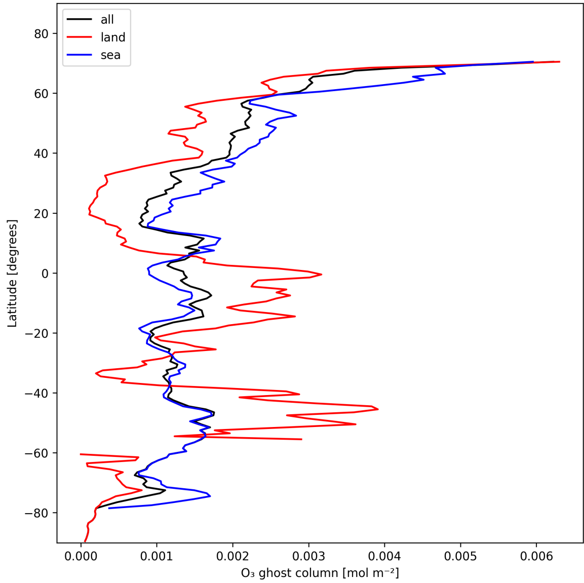
Figure 18: Zonal average of "O 3 ghost column" for 2024-11-14 to 2024-11-15.
