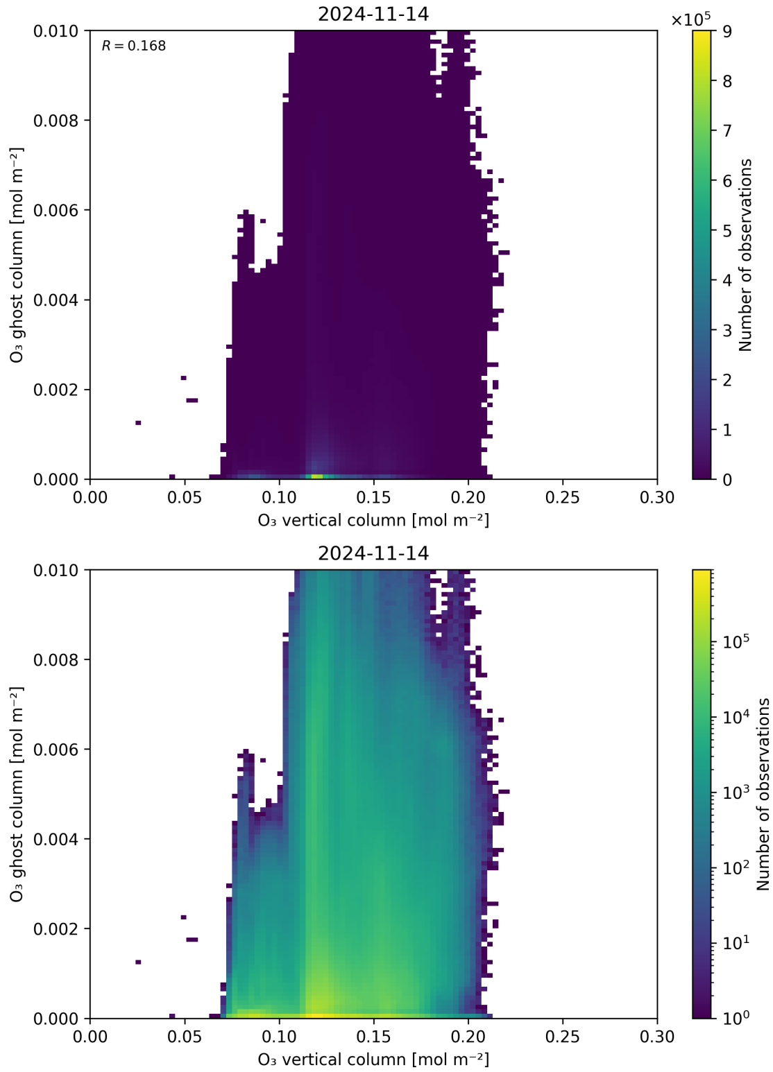
Figure 40: Scatter density plot of “O 3 vertical column” against “O 3 ghost column” for 2024-11-14 to 2024-11-15.
