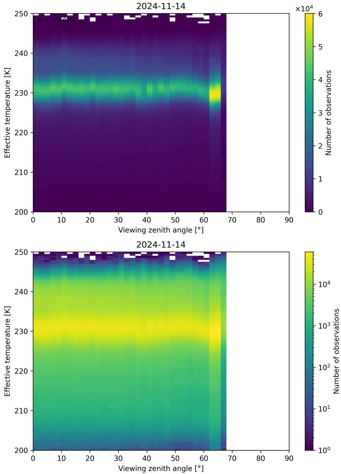
Figure 50: Scatter density plot of “Viewing zenith angle” against “Effective temperature” for 2024-11-14 to 2024-11-15.
