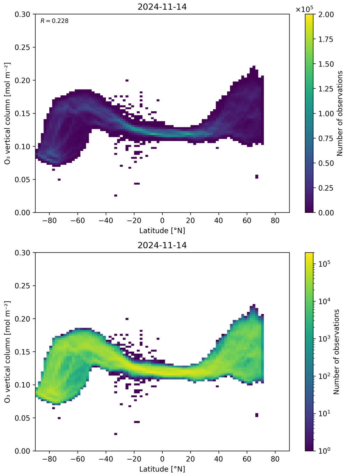
Figure 36: Scatter density plot of “Latitude” against “O 3 vertical column” for 2024-11-14 to 2024-11-15.
