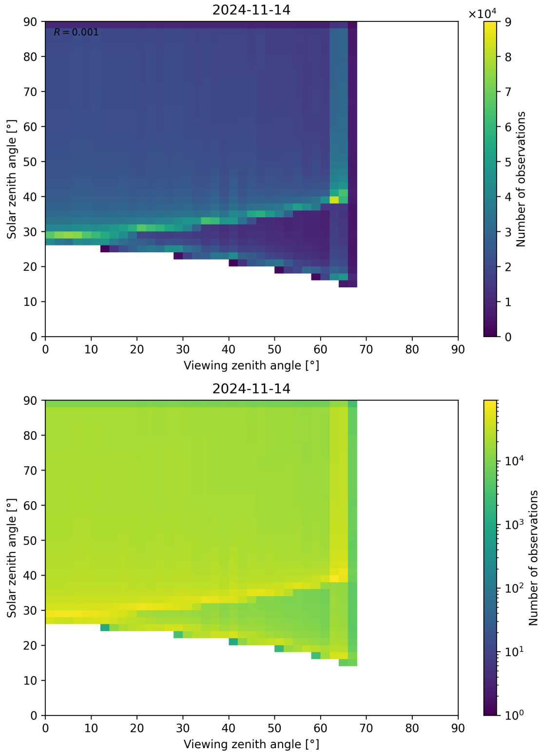
Figure 54: Scatter density plot of “Viewing zenith angle” against “Solar zenith angle” for 2024-11-14 to 2024-11-15.
