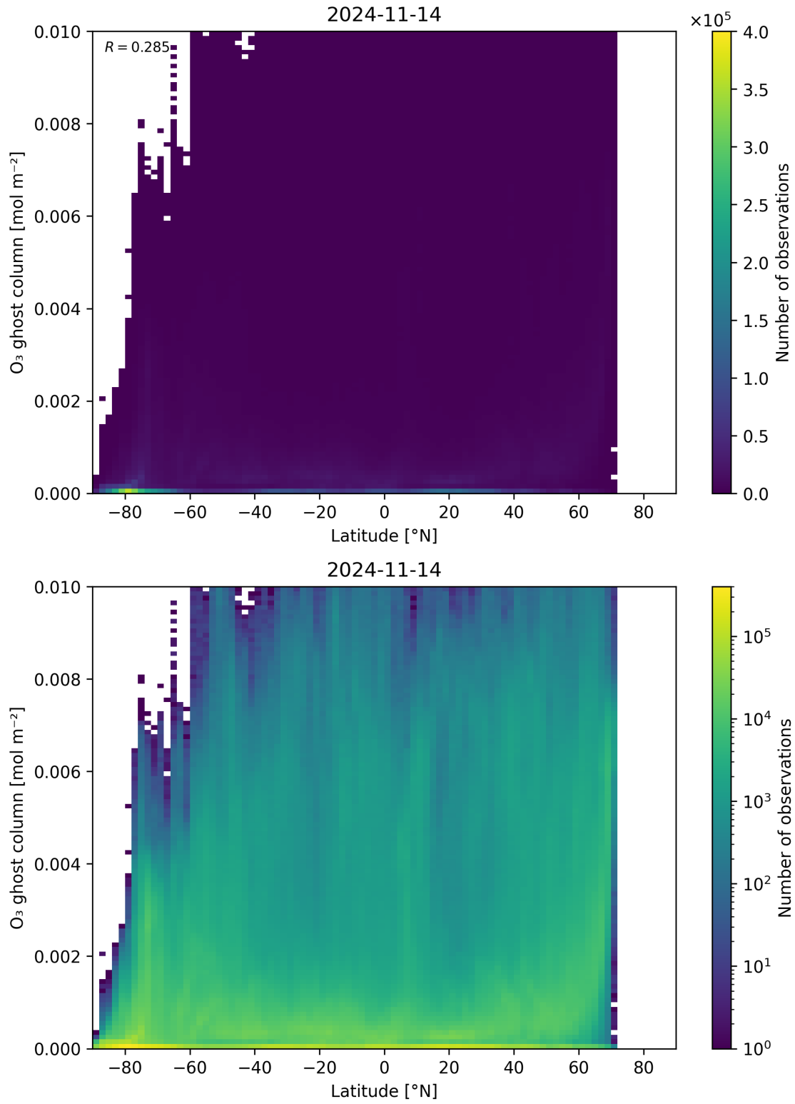
Figure 35: Scatter density plot of “Latitude” against “O 3 ghost column” for 2024-11-14 to 2024-11-15.
