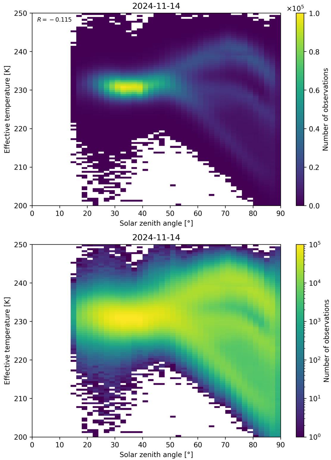
Figure 45: Scatter density plot of “Solar zenith angle” against “Effective temperature” for 2024-11-14 to 2024-11-15.
