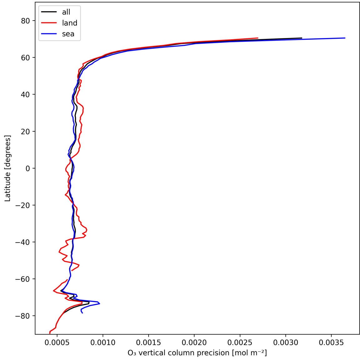
Figure 15: Zonal average of “O 3 vertical column precision” for 2024-11-14 to 2024-11-15.
