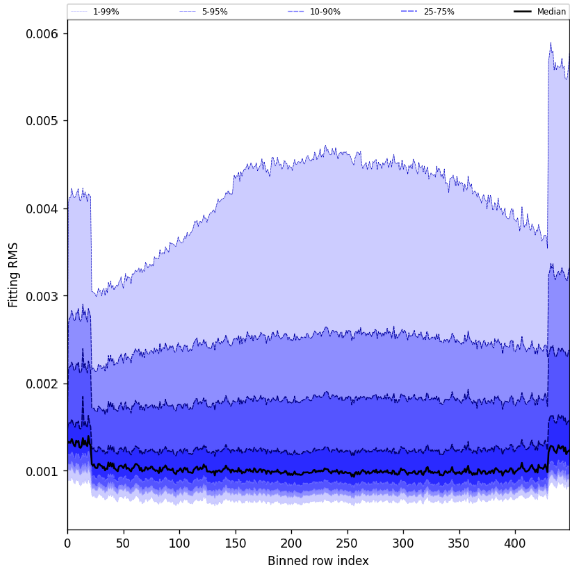
Figure 30: Along track statistics of “Fitting RMS” for 2024-11-14 to 2024-11-15
