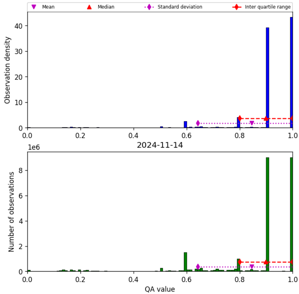
Figure 20: Histogram of “QA value” for 2024-11-14 to 2024-11-15
