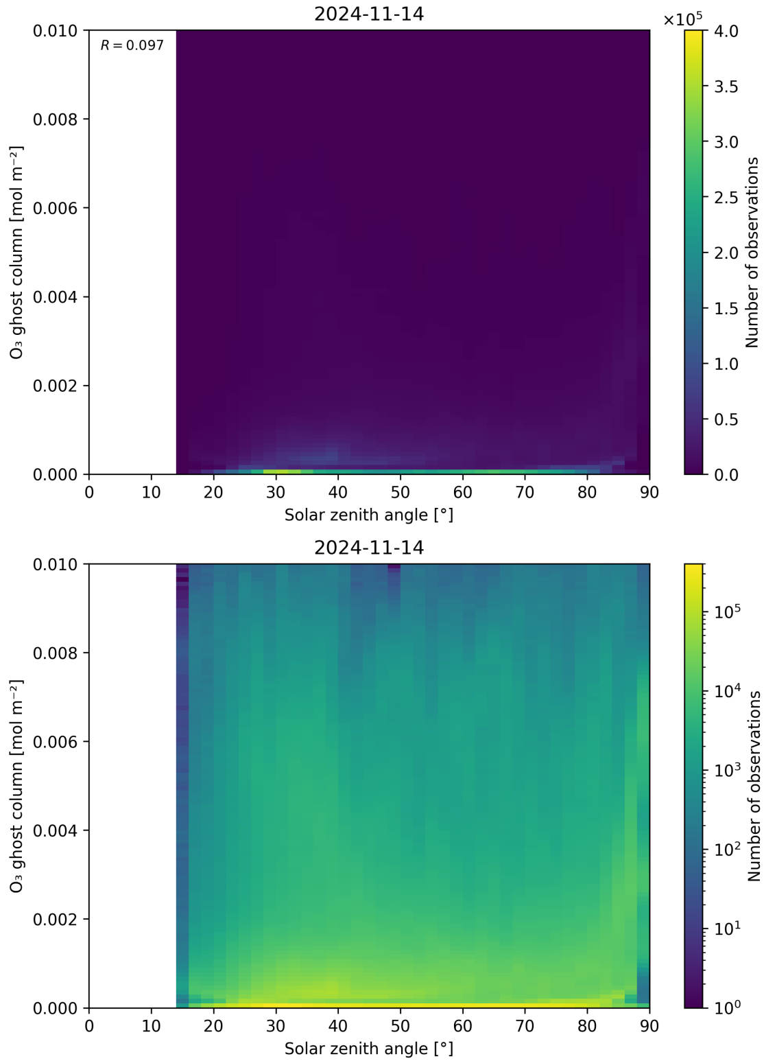
Figure 46: Scatter density plot of “Solar zenith angle” against “O 3 ghost column” for 2024-11-14 to 2024-11-15.
