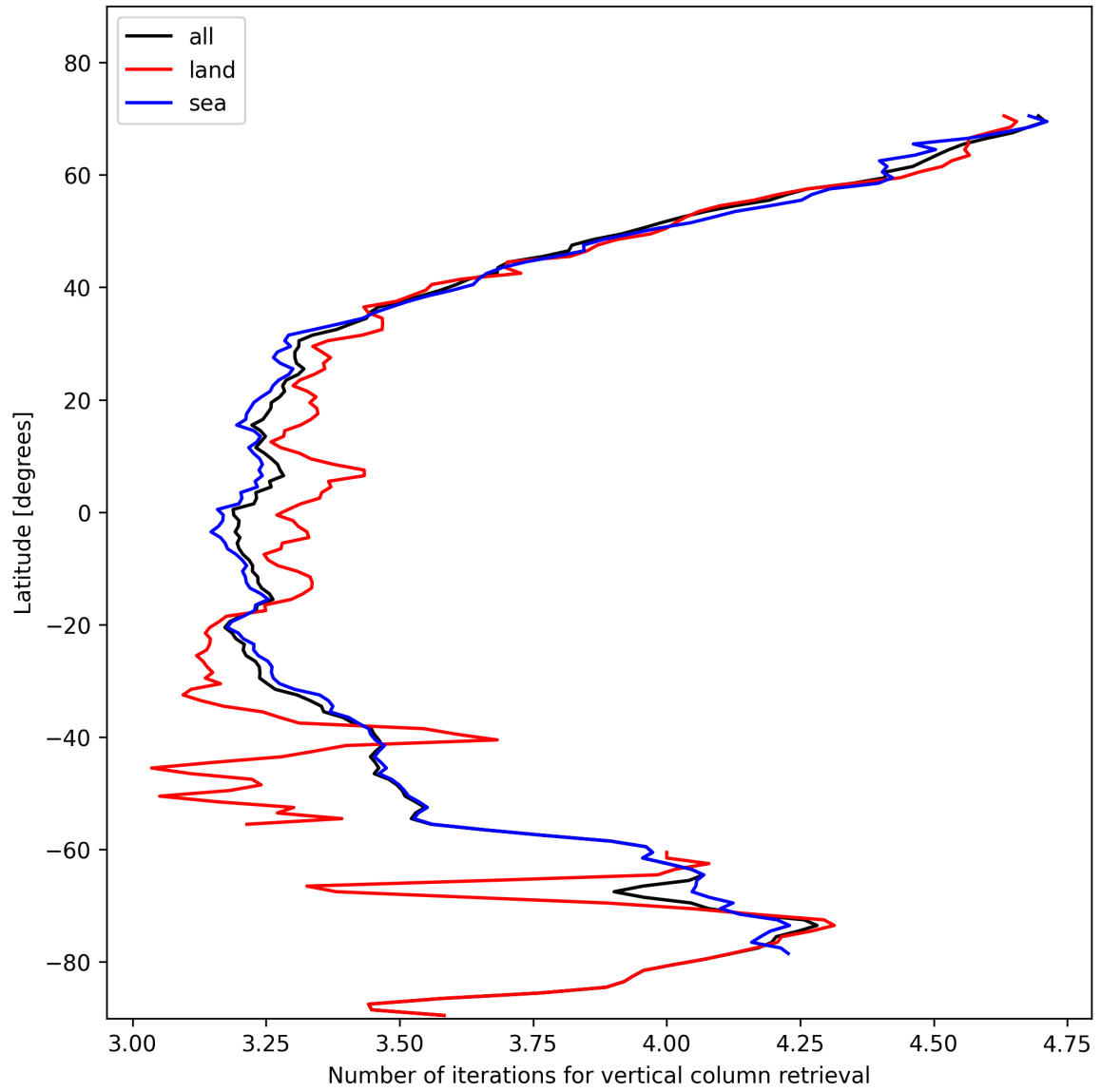
Figure 19: Zonal average of “Number of iterations for vertical column retrieval” for 2024-11-14 to 2024-11-15.
