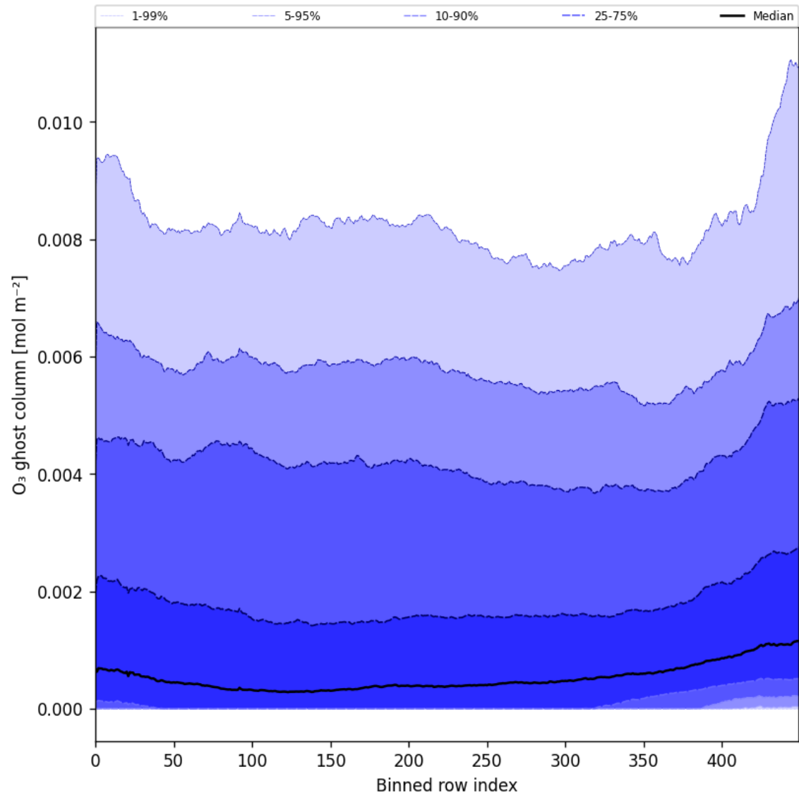
Figure 32: Along track statistics of “O 3 ghost column” for 2024-11-14 to 2024-11-15
