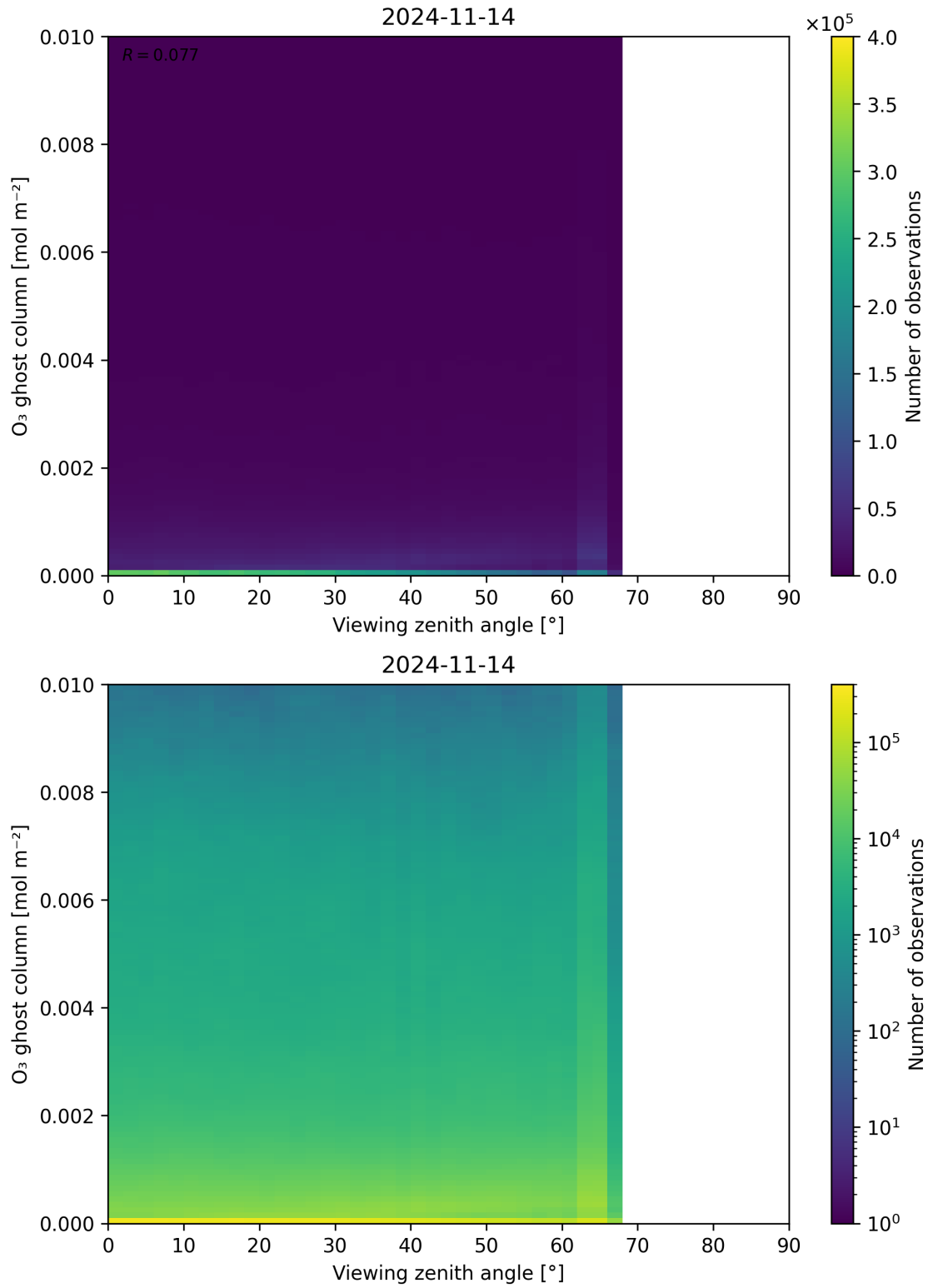
Figure 51: Scatter density plot of “Viewing zenith angle” against “O 3 ghost column” for 2024-11-14 to 2024-11-15.
