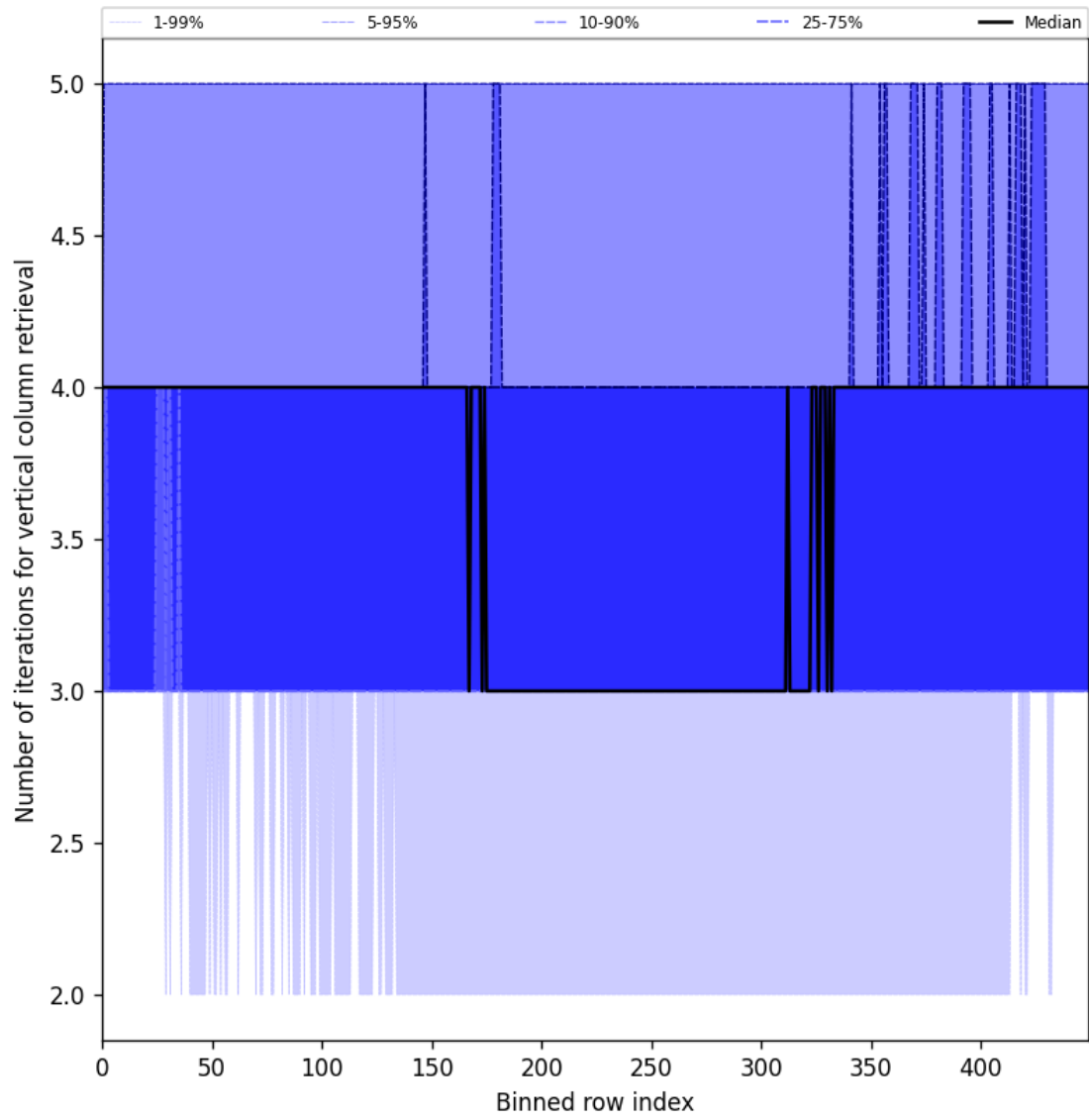
Figure 33: Along track statistics of “Number of iterations for vertical column retrieval” for 2024-11-14 to 2024-11-15
