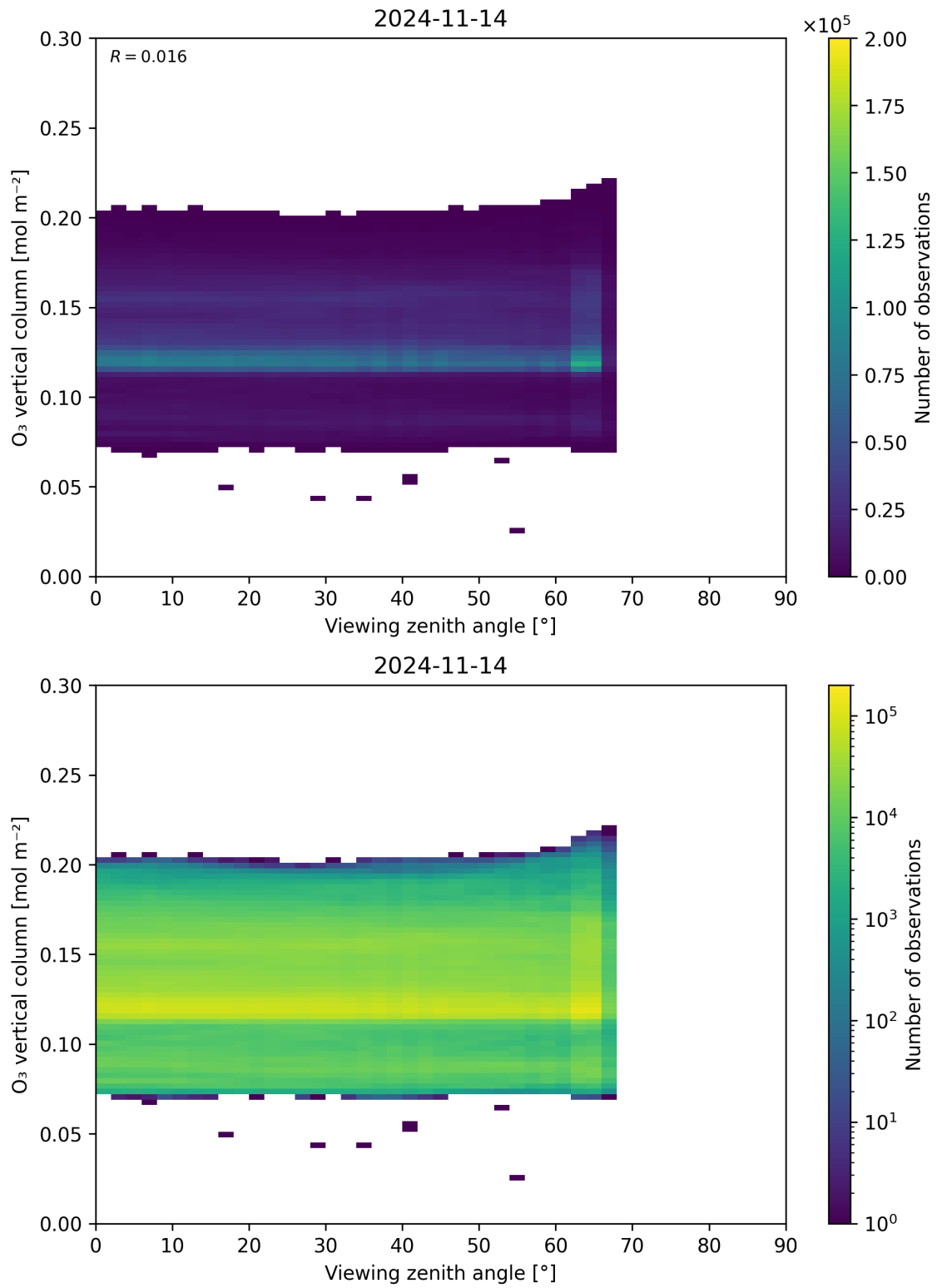
Figure 52: Scatter density plot of “Viewing zenith angle” against “O 3 vertical column” for 2024-11-14 to 2024-11-15.
