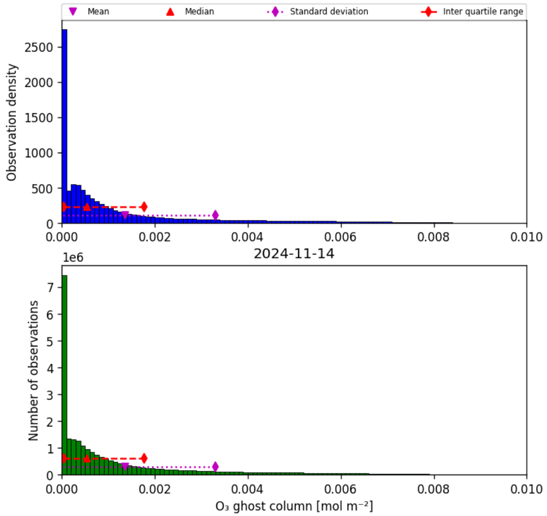
Figure 25: Histogram of “O 3 ghost column” for 2024-11-14 to 2024-11-15
