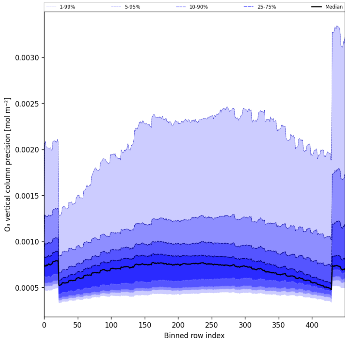
Figure 29: Along track statistics of “O 3 vertical column precision” for 2024-11-14 to 2024-11-15
