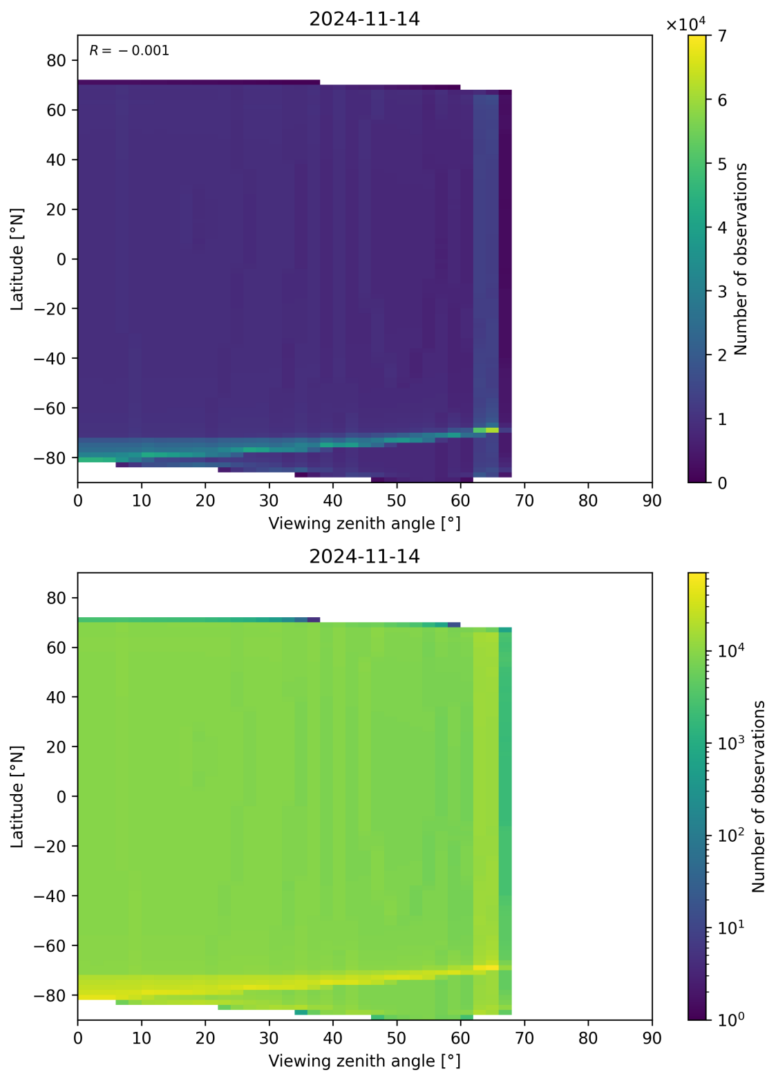
Figure 49: Scatter density plot of “Viewing zenith angle” against “Latitude” for 2024-11-14 to 2024-11-15.
