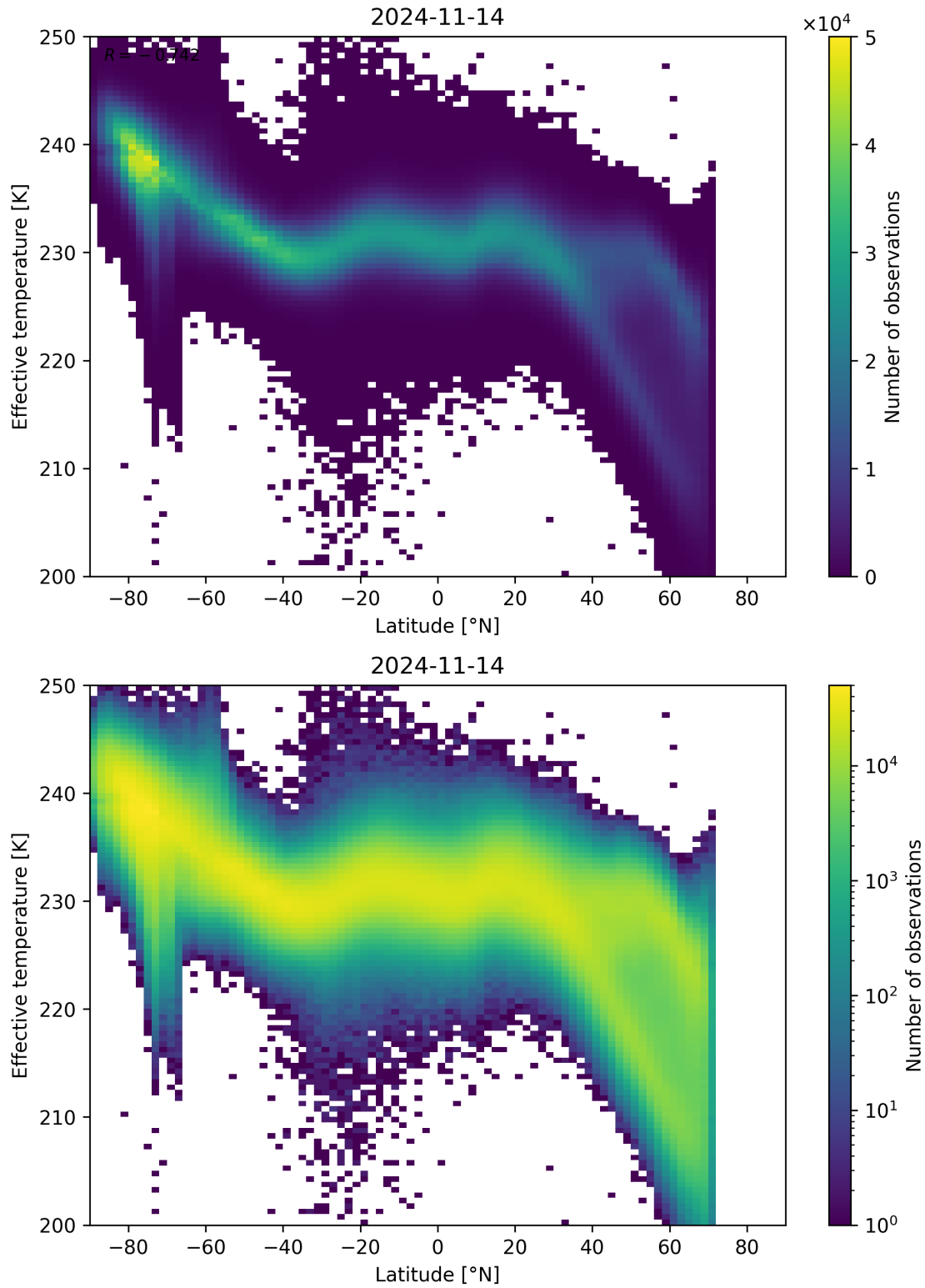
Figure 34: Scatter density plot of “Latitude” against “Effective temperature” for 2024-11-14 to 2024-11-15.
