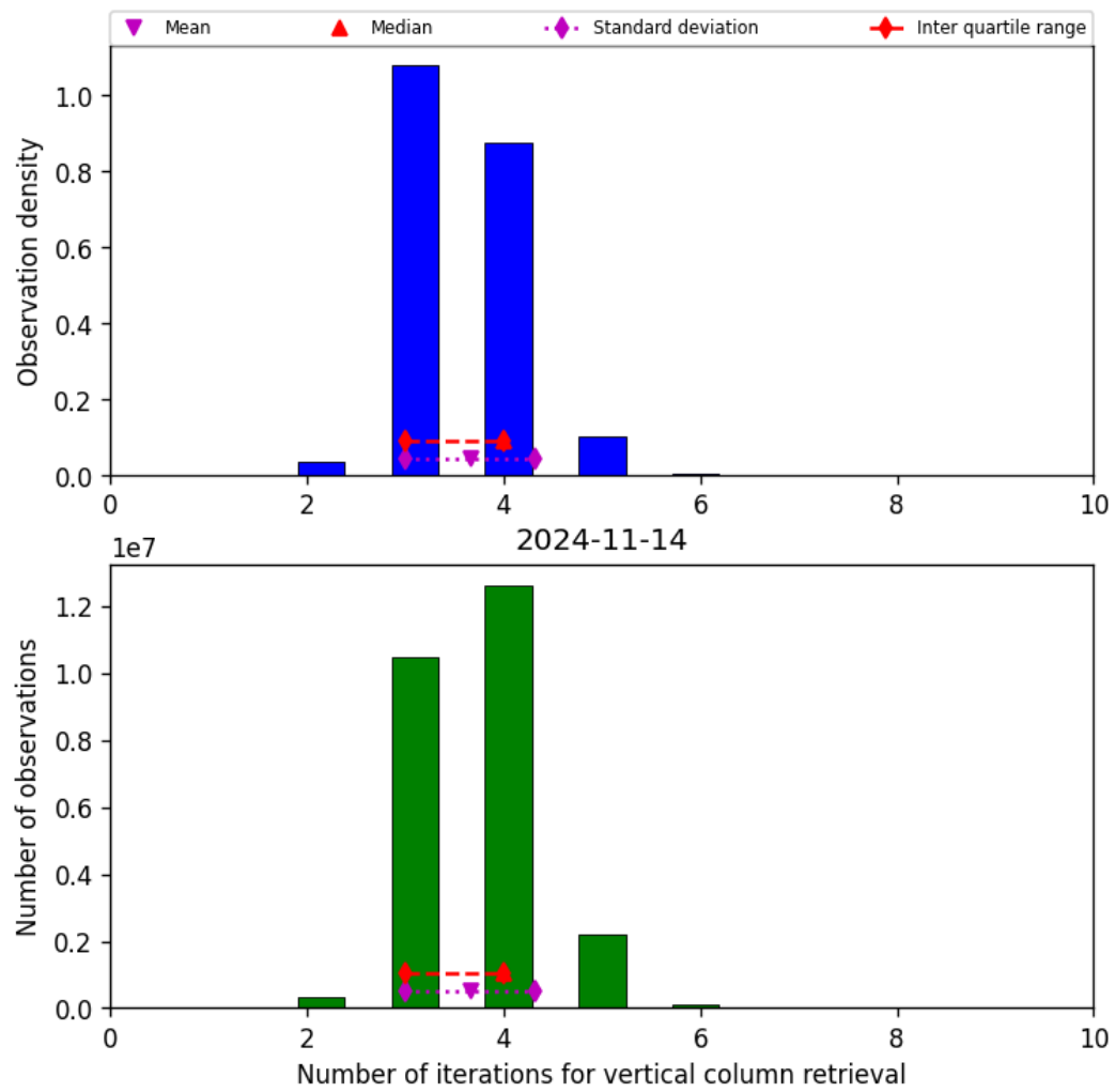
Figure 26: Histogram of “Number of iterations for vertical column retrieval” for 2024-11-14 to 2024-11-15
