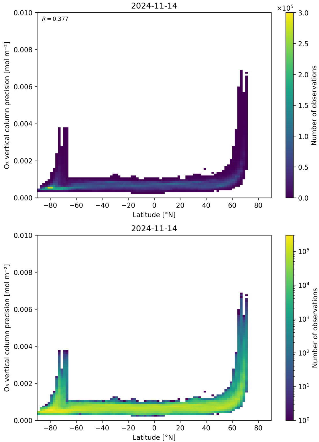
Figure 37: Scatter density plot of “Latitude” against “O 3 vertical column precision” for 2024-11-14 to 2024-11-15.
