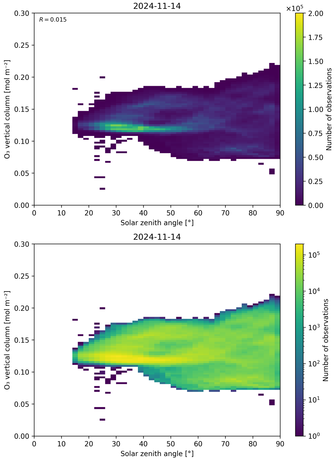
Figure 47: Scatter density plot of “Solar zenith angle” against “O 3 vertical column” for 2024-11-14 to 2024-11-15.
