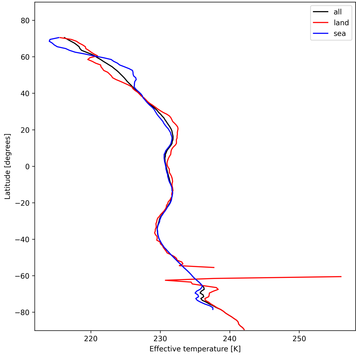
Figure 17: Zonal average of “Effective temperature” for 2024-11-14 to 2024-11-15.
