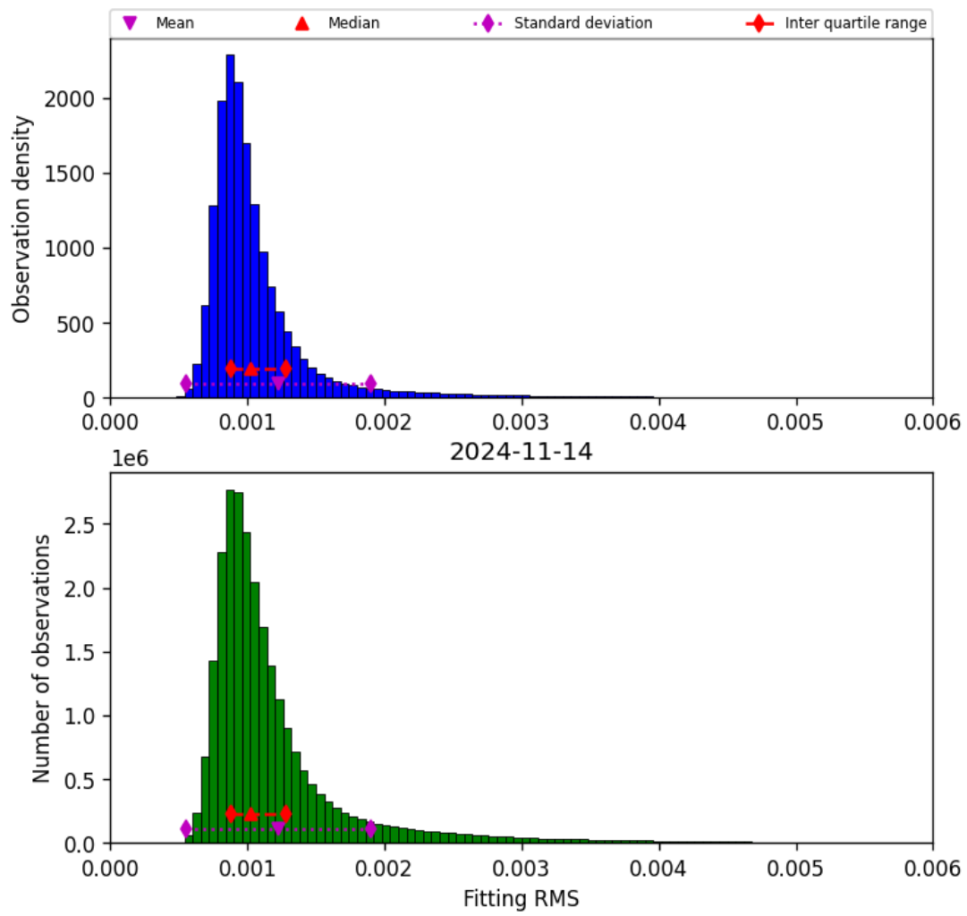
Figure 23: Histogram of “Fitting RMS” for 2024-11-14 to 2024-11-15
