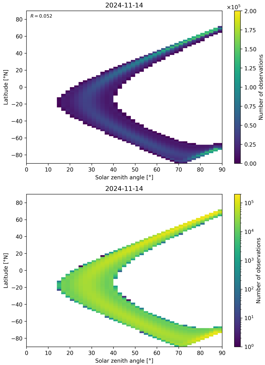
Figure 44: Scatter density plot of “Solar zenith angle” against “Latitude” for 2024-11-14 to 2024-11-15.
