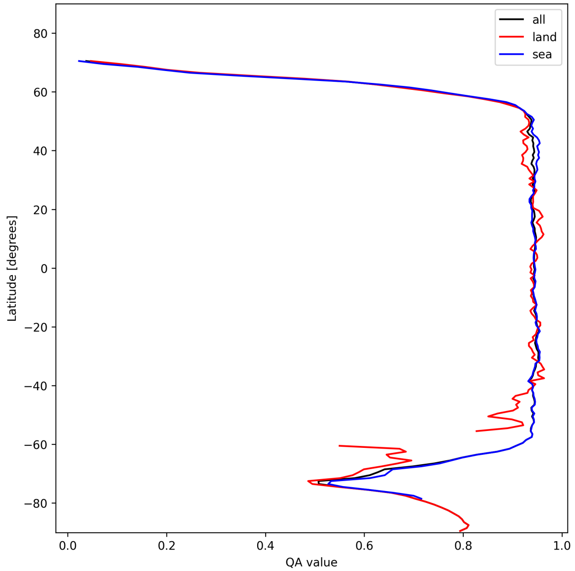
Figure 13: Zonal average of “QA value” for 2024-11-14 to 2024-11-15.
