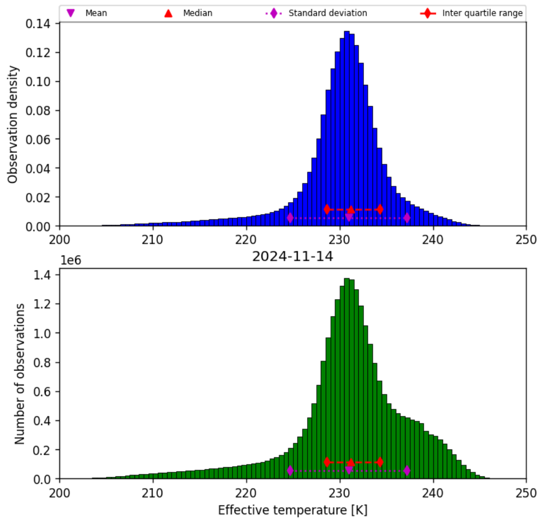
Figure 24: Histogram of “Effective temperature” for 2024-11-14 to 2024-11-15
