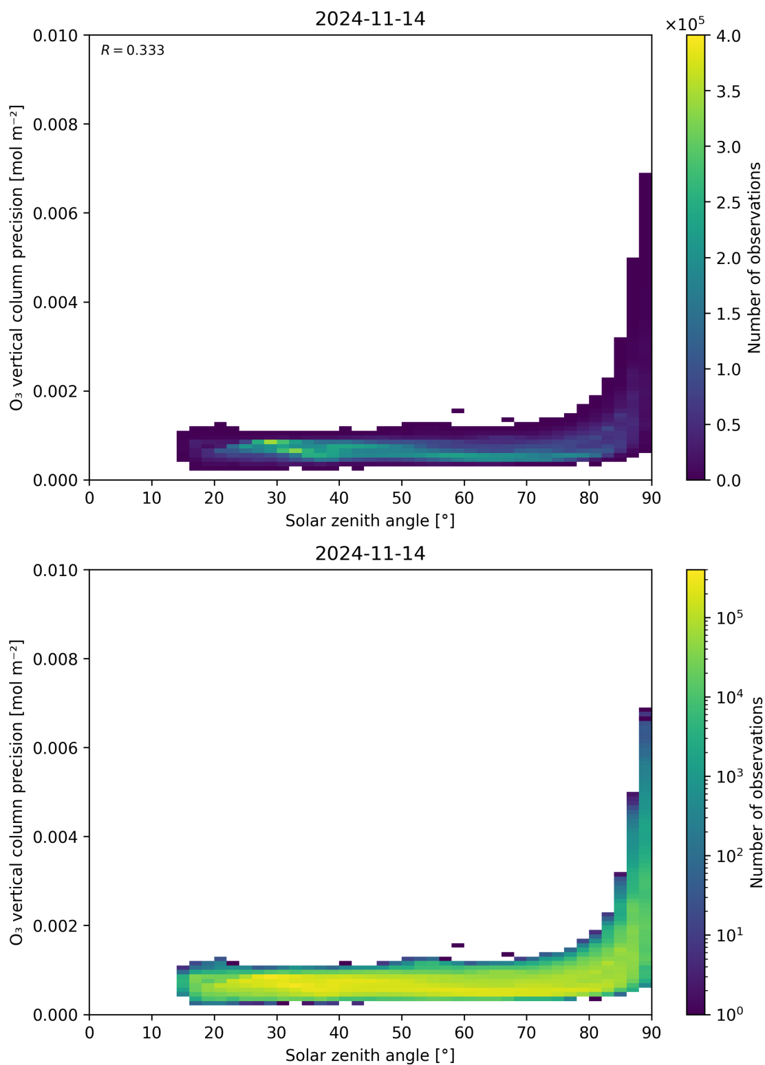
Figure 48: Scatter density plot of “Solar zenith angle” against “O 3 vertical column precision” for 2024-11-14 to 2024-11-15.
