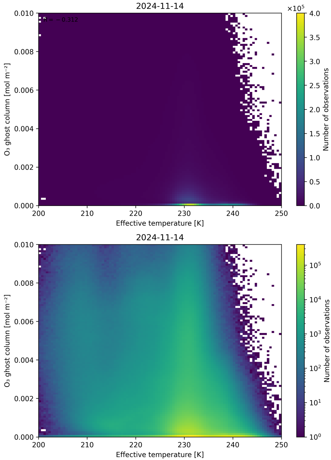
Figure 38: Scatter density plot of “Effective temperature” against “O 3 ghost column” for 2024-11-14 to 2024-11-15.
