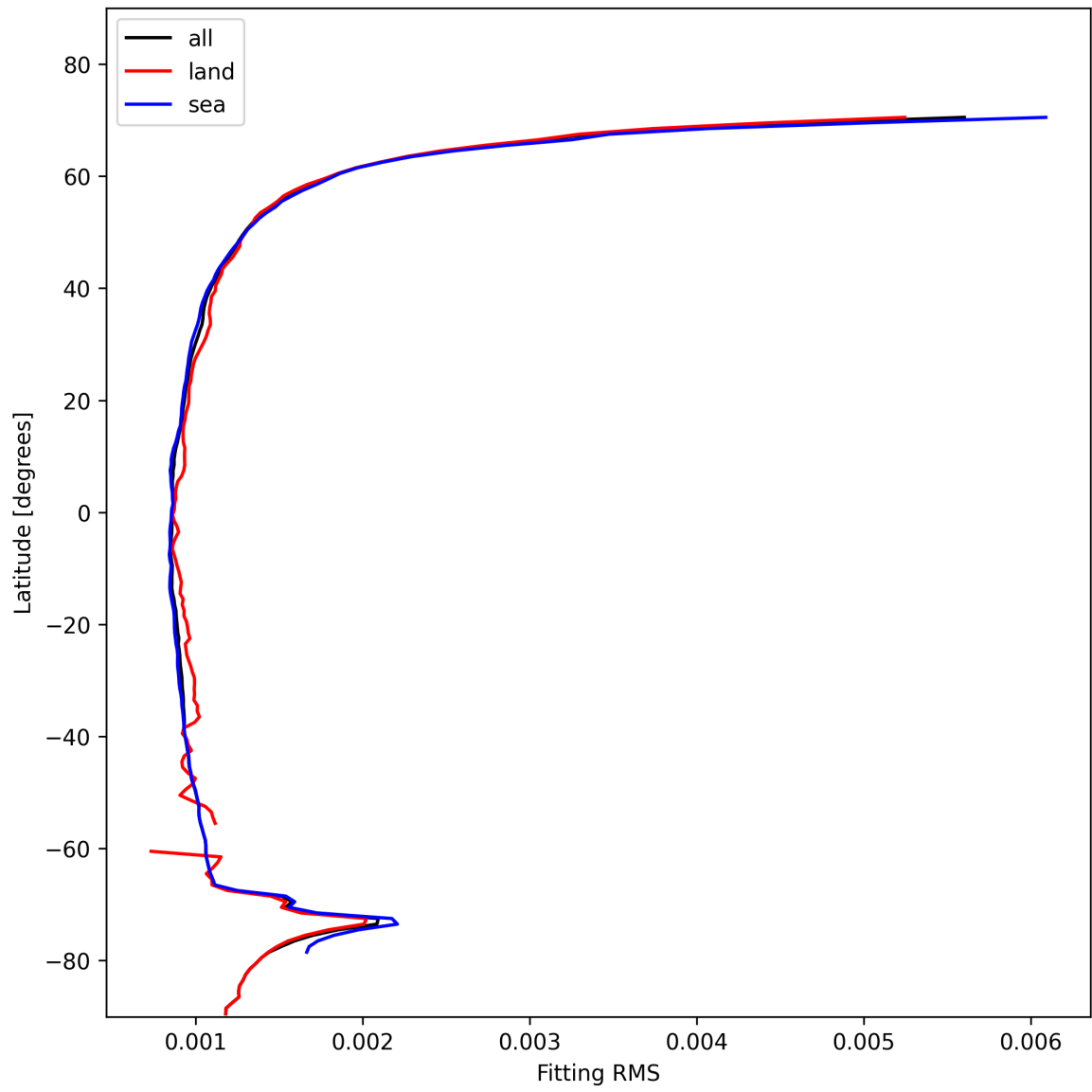
Figure 16: Zonal average of “Fitting RMS” for 2024-11-14 to 2024-11-15.
