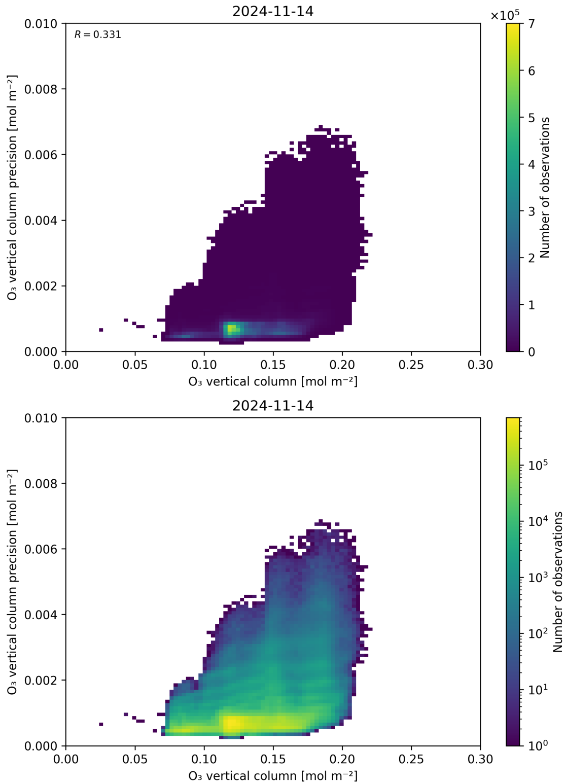
Figure 41: Scatter density plot of “O 3 vertical column” against “O 3 vertical column precision” for 2024-11-14 to 2024-11-15.
