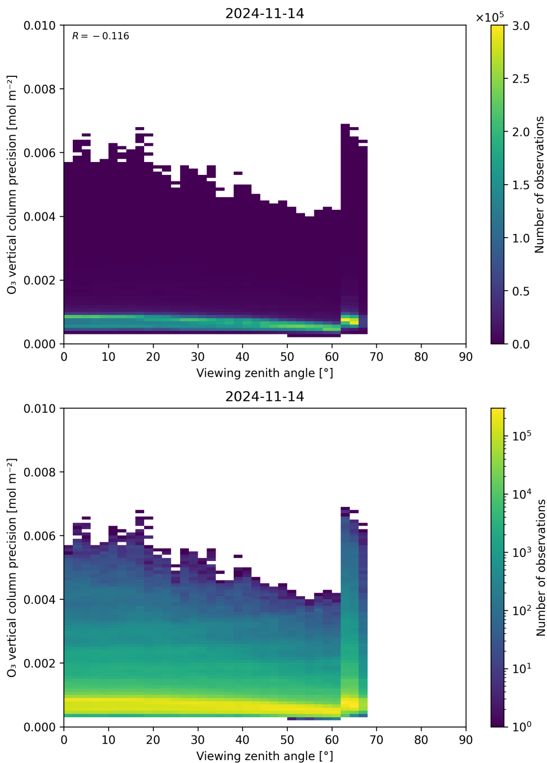
Figure 53: Scatter density plot of “Viewing zenith angle” against “O 3 vertical column precision” for 2024-11-14 to 2024-11-15.
