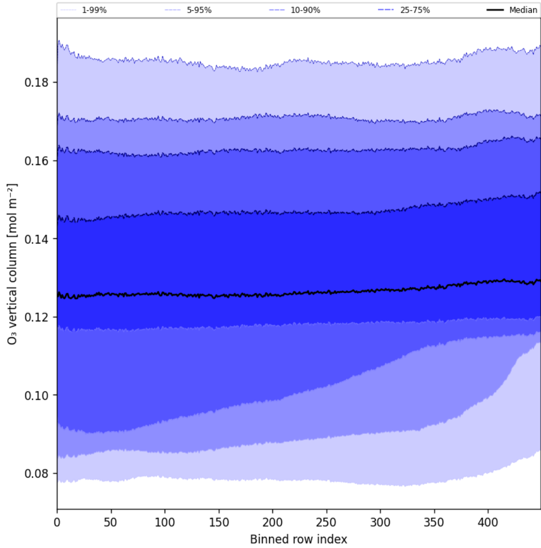
Figure 28: Along track statistics of “O 3 vertical column” for 2024-11-14 to 2024-11-15
