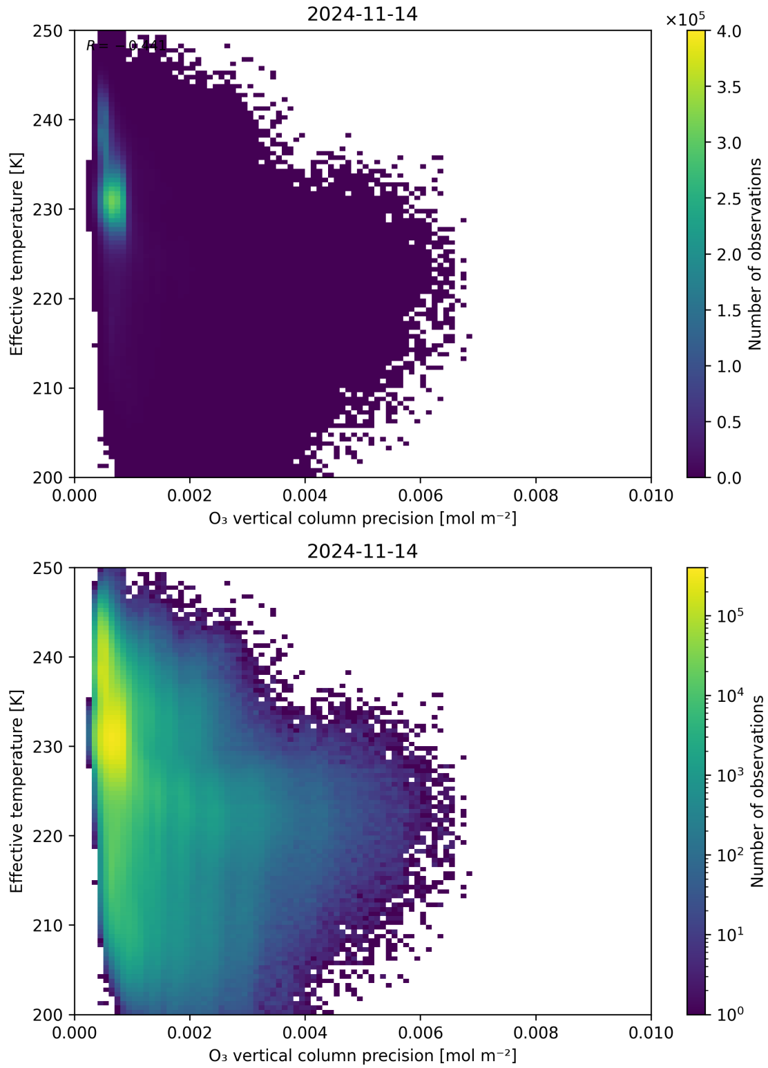
Figure 42: Scatter density plot of “ O_3 vertical column precision” against “Effective temperature” for 2024-11-14 to 2024-11-15.
