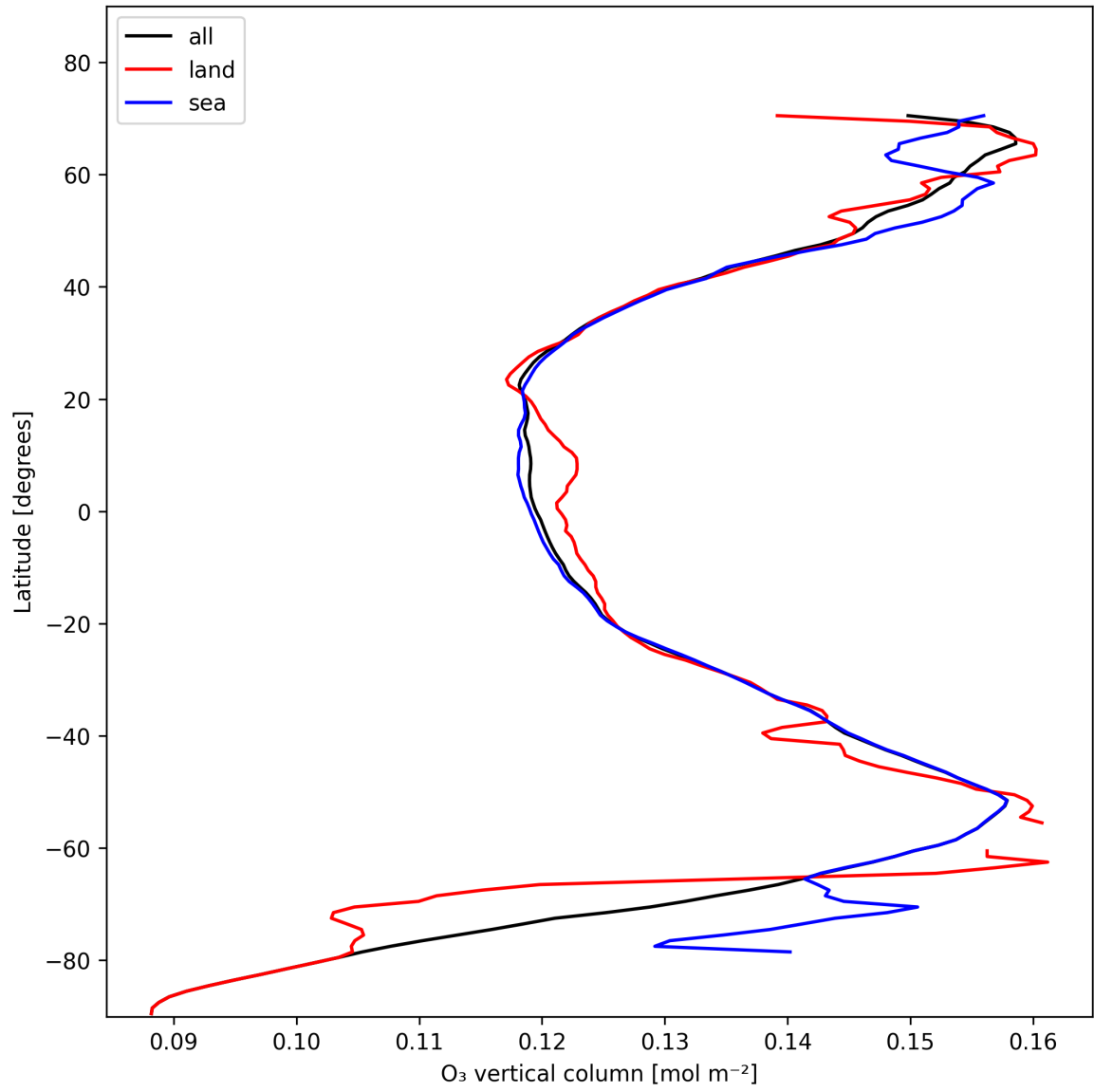
Figure 14: Zonal average of “O 3 vertical column” for 2024-11-14 to 2024-11-15.
