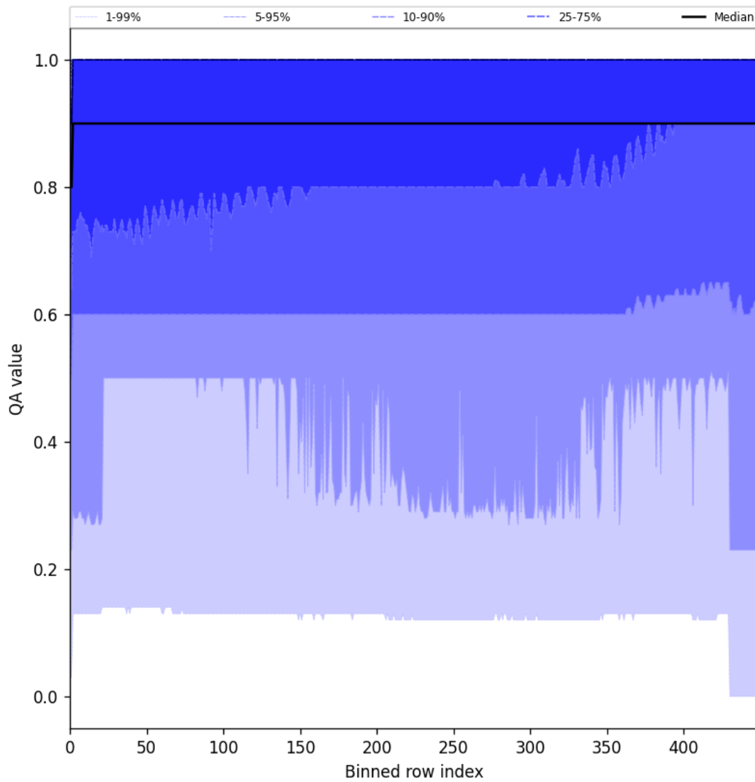
Figure 27: Along track statistics of “QA value” for 2024-11-14 to 2024-11-15
