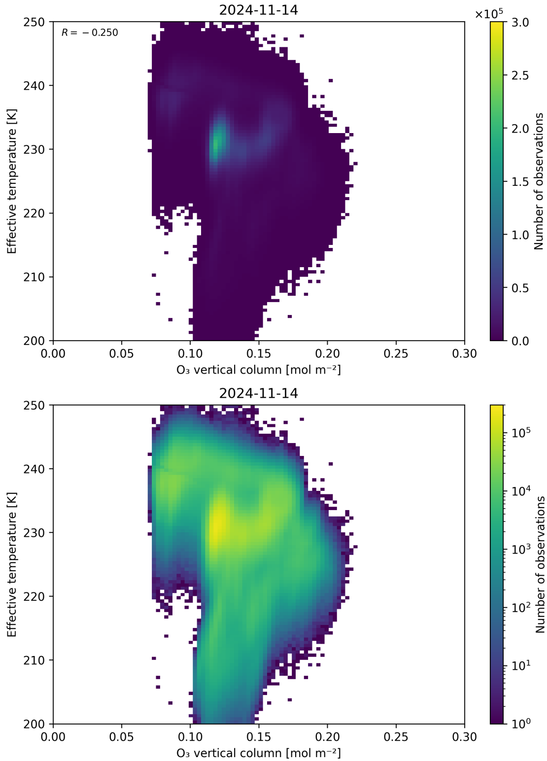
Figure 39: Scatter density plot of “O 3 vertical column” against “Effective temperature” for 2024-11-14 to 2024-11-15.
