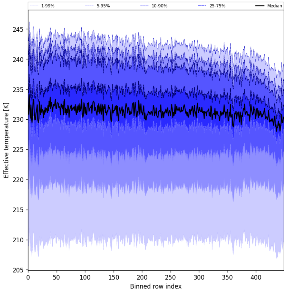
Figure 31: Along track statistics of “Effective temperature” for 2024-11-14 to 2024-11-15
