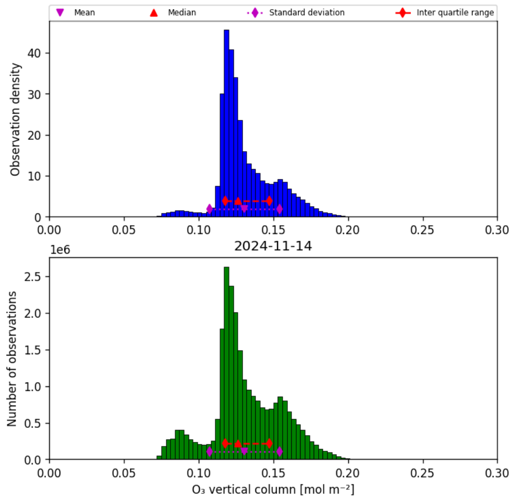
Figure 21: Histogram of “O 3 vertical column” for 2024-11-14 to 2024-11-15
