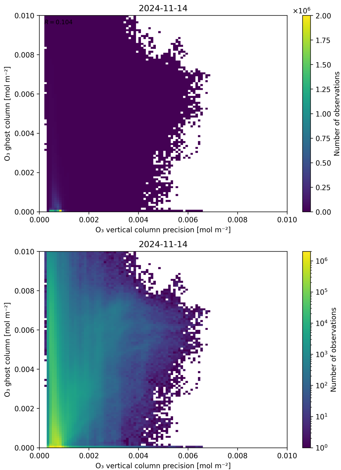
Figure 43: Scatter density plot of “ \text{O}_3 vertical column precision” against “ \text{O}_3 ghost column” for 2024-11-14 to 2024-11-15.
