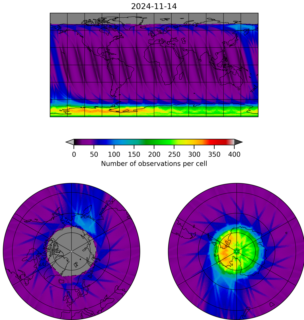
Figure 12: Map of the number of observations for 2024-11-14 to 2024-11-15
