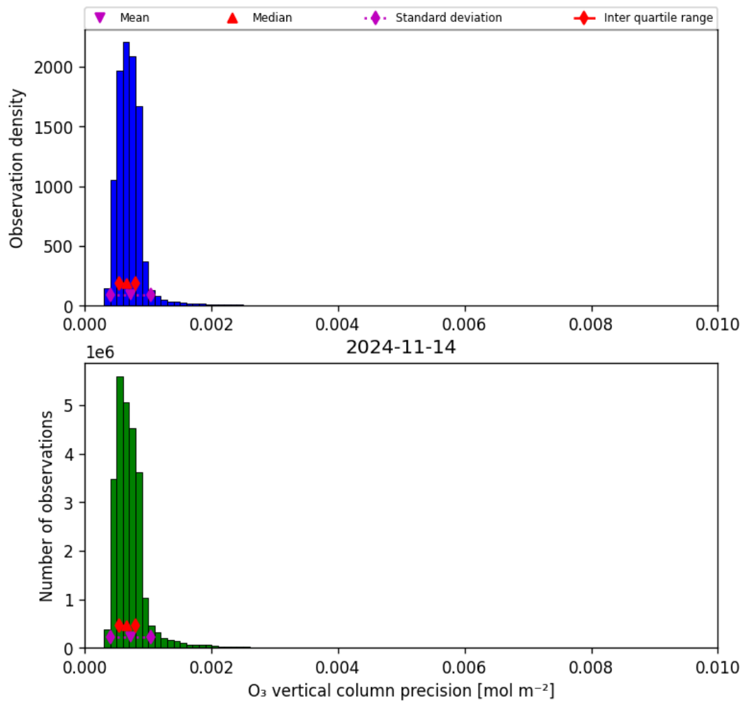
Figure 22: Histogram of “O 3 vertical column precision” for 2024-11-14 to 2024-11-15
