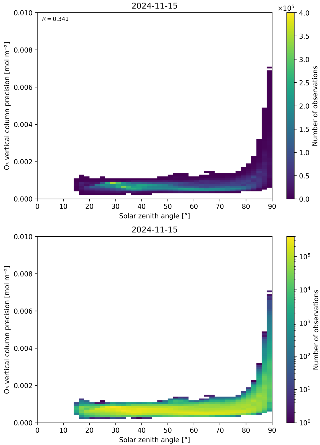
Figure 48: Scatter density plot of “Solar zenith angle” against “O 3 vertical column precision” for 2024-11-14 to 2024-11-16.
