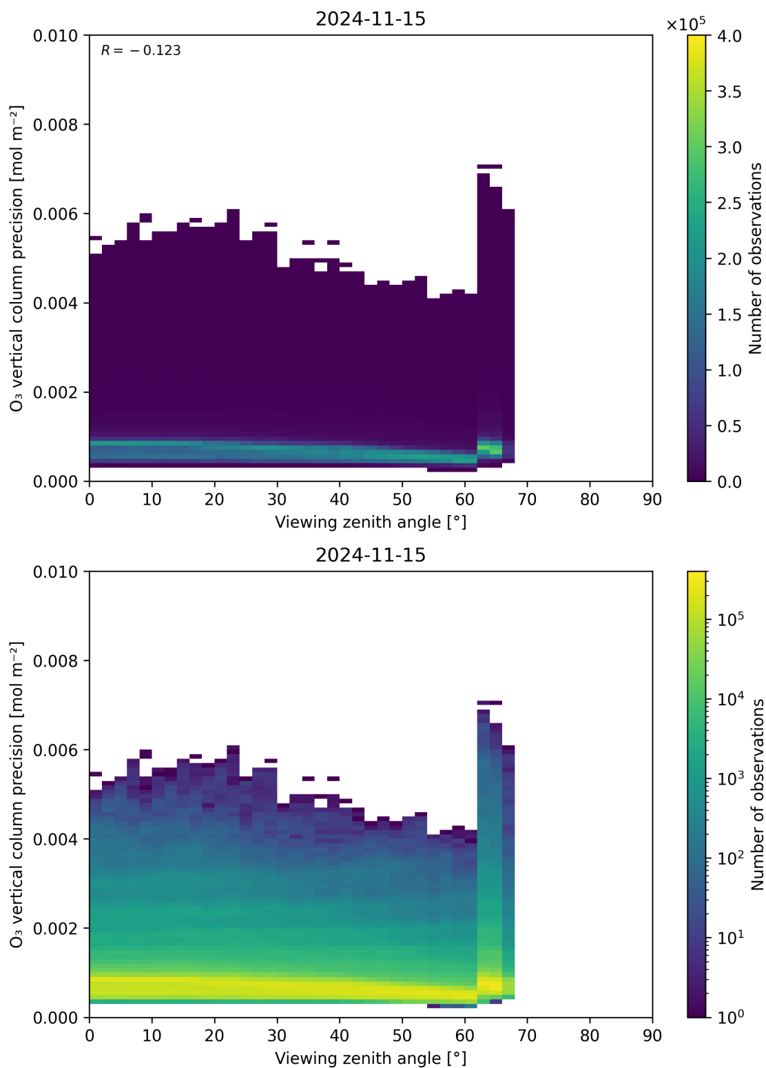
Figure 53: Scatter density plot of “Viewing zenith angle” against “O 3 vertical column precision” for 2024-11-14 to 2024-11-16.
