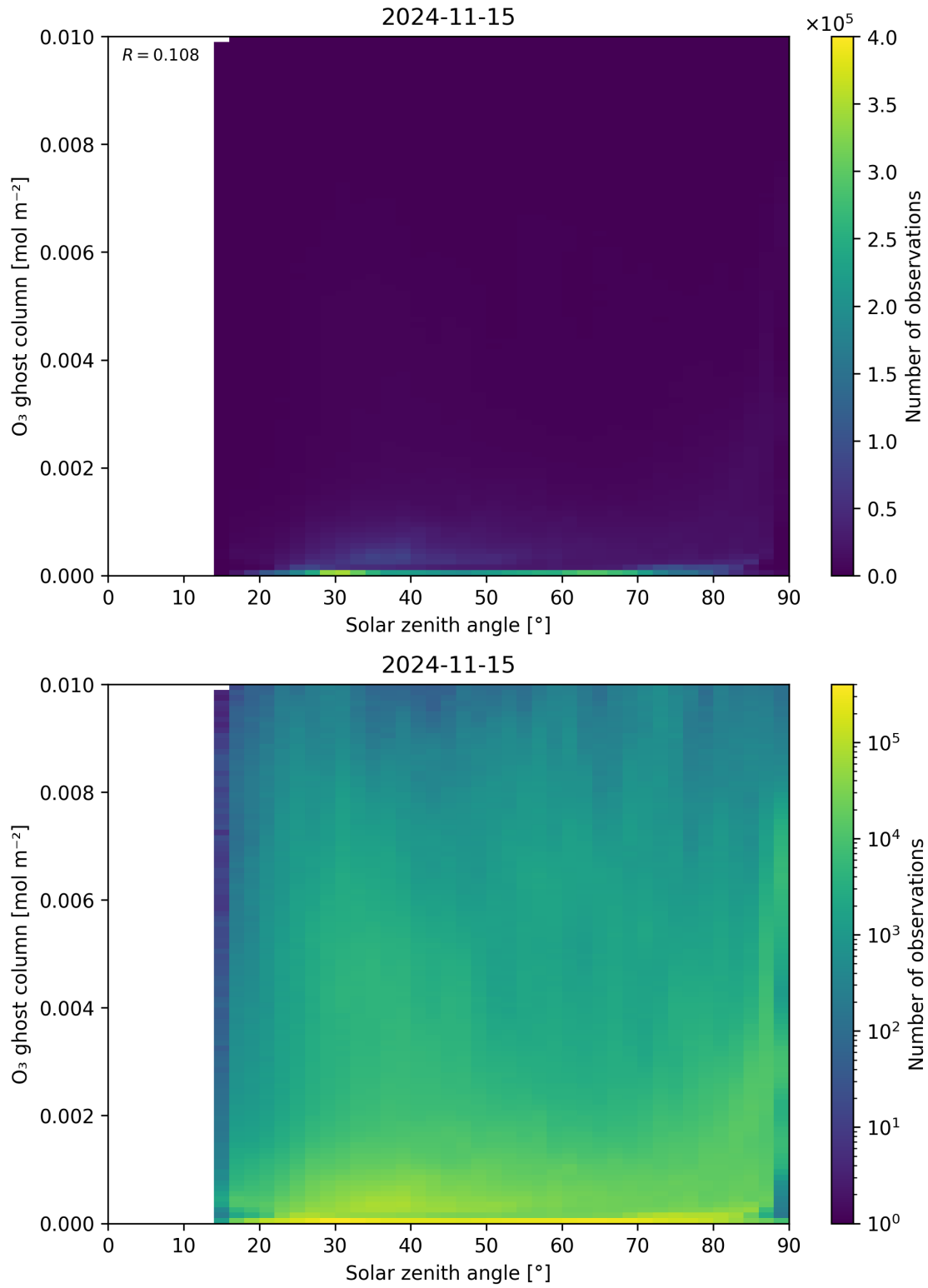
Figure 46: Scatter density plot of “Solar zenith angle” against “O 3 ghost column” for 2024-11-14 to 2024-11-16.
