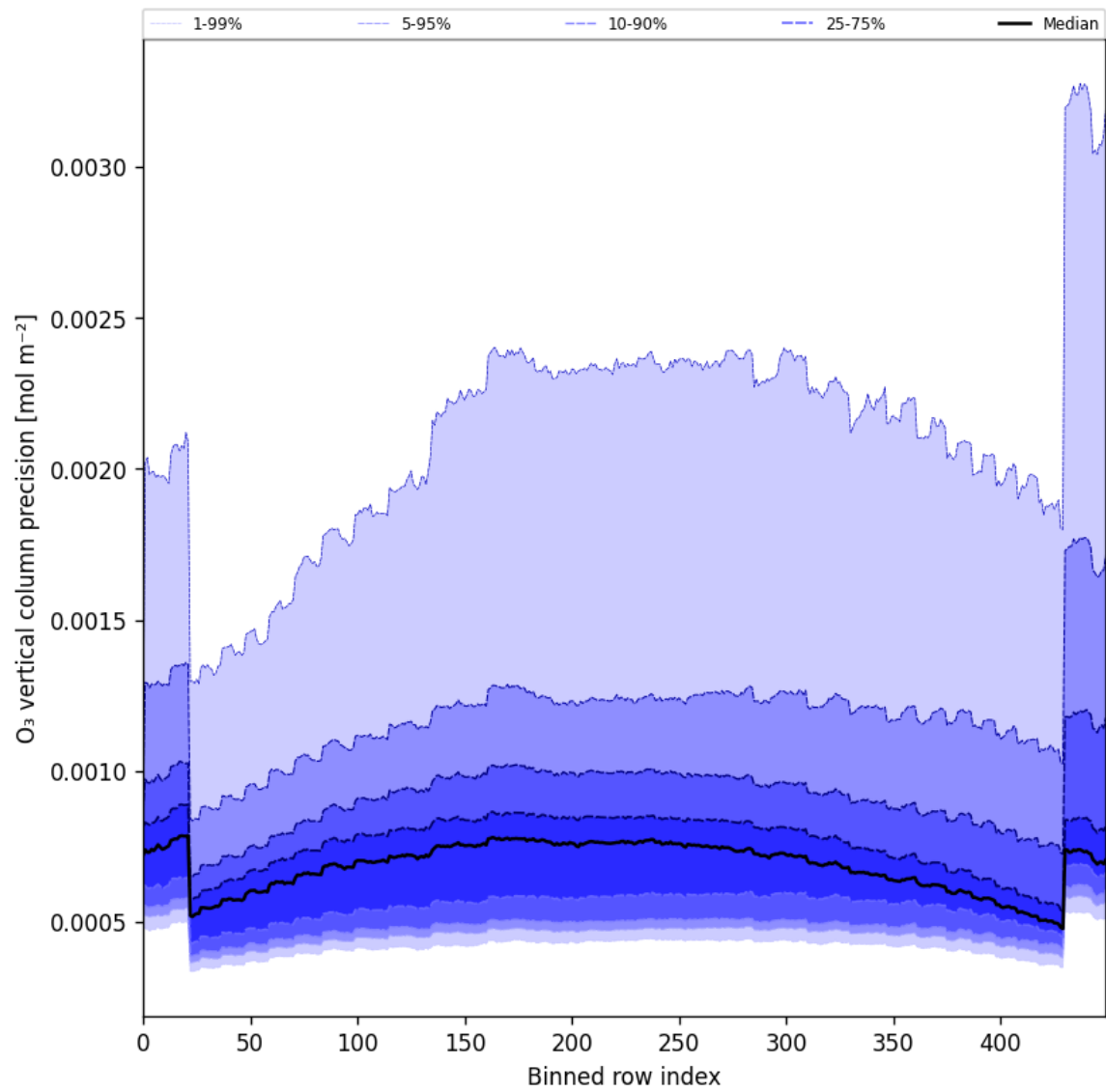
Figure 29: Along track statistics of “O 3 vertical column precision” for 2024-11-14 to 2024-11-16
