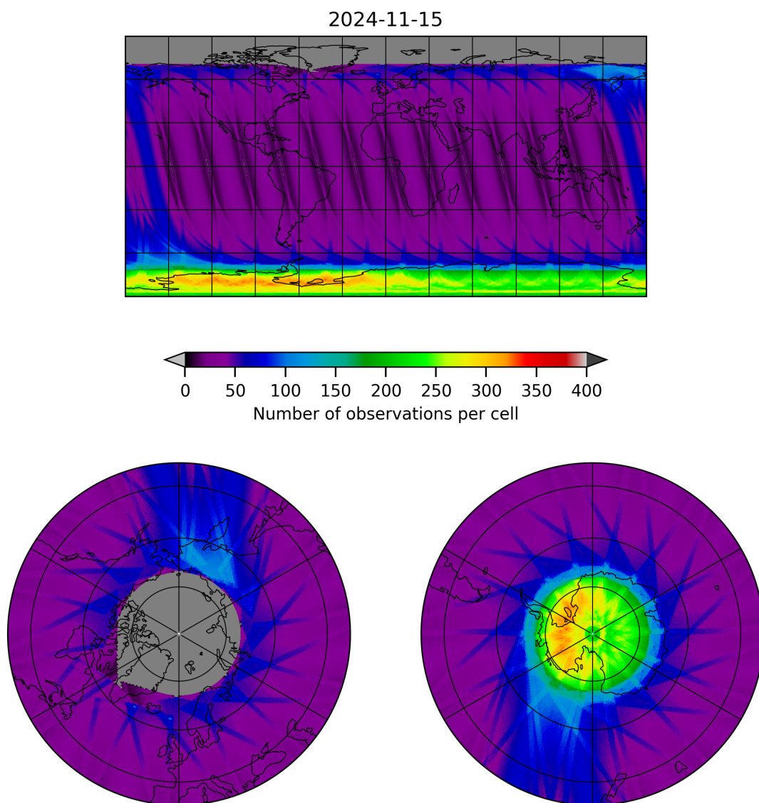
Figure 12: Map of the number of observations for 2024-11-14 to 2024-11-16
