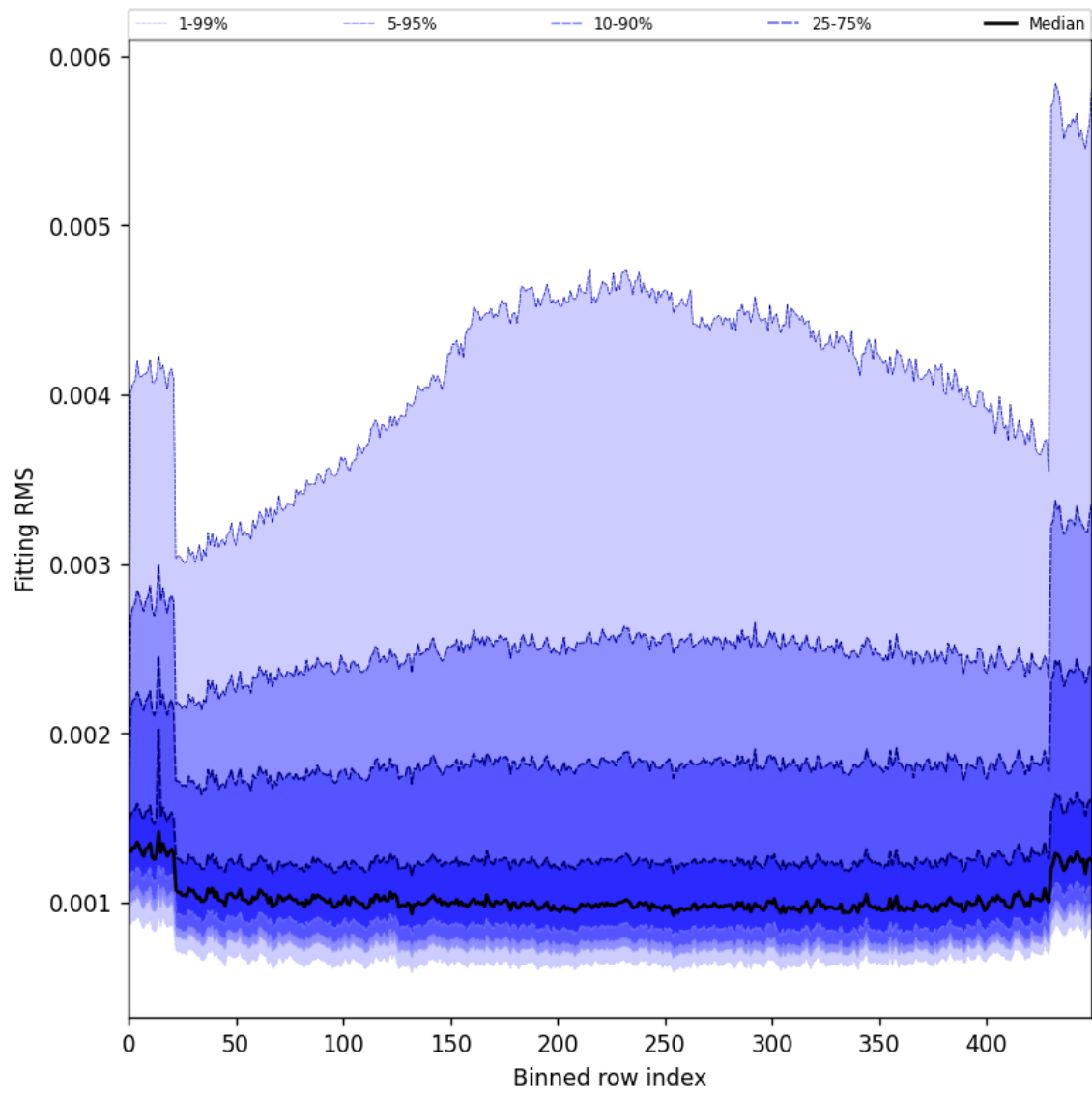
Figure 30: Along track statistics of “Fitting RMS” for 2024-11-14 to 2024-11-16
