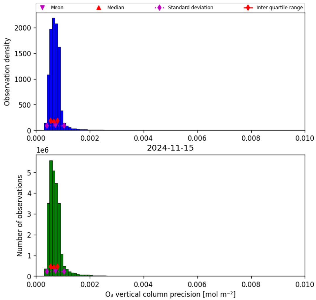
Figure 22: Histogram of “O 3 vertical column precision” for 2024-11-14 to 2024-11-16
