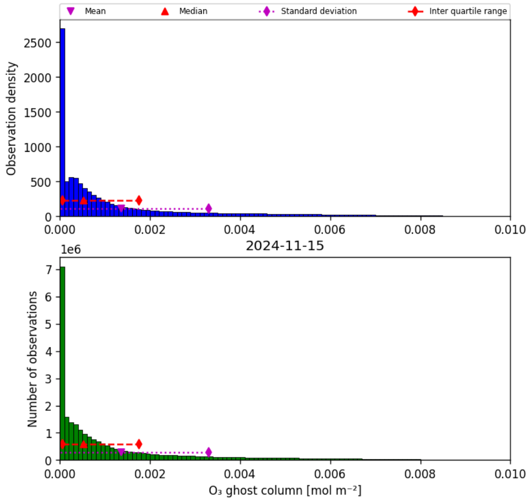
Figure 25: Histogram of "O 3 ghost column" for 2024-11-14 to 2024-11-16
