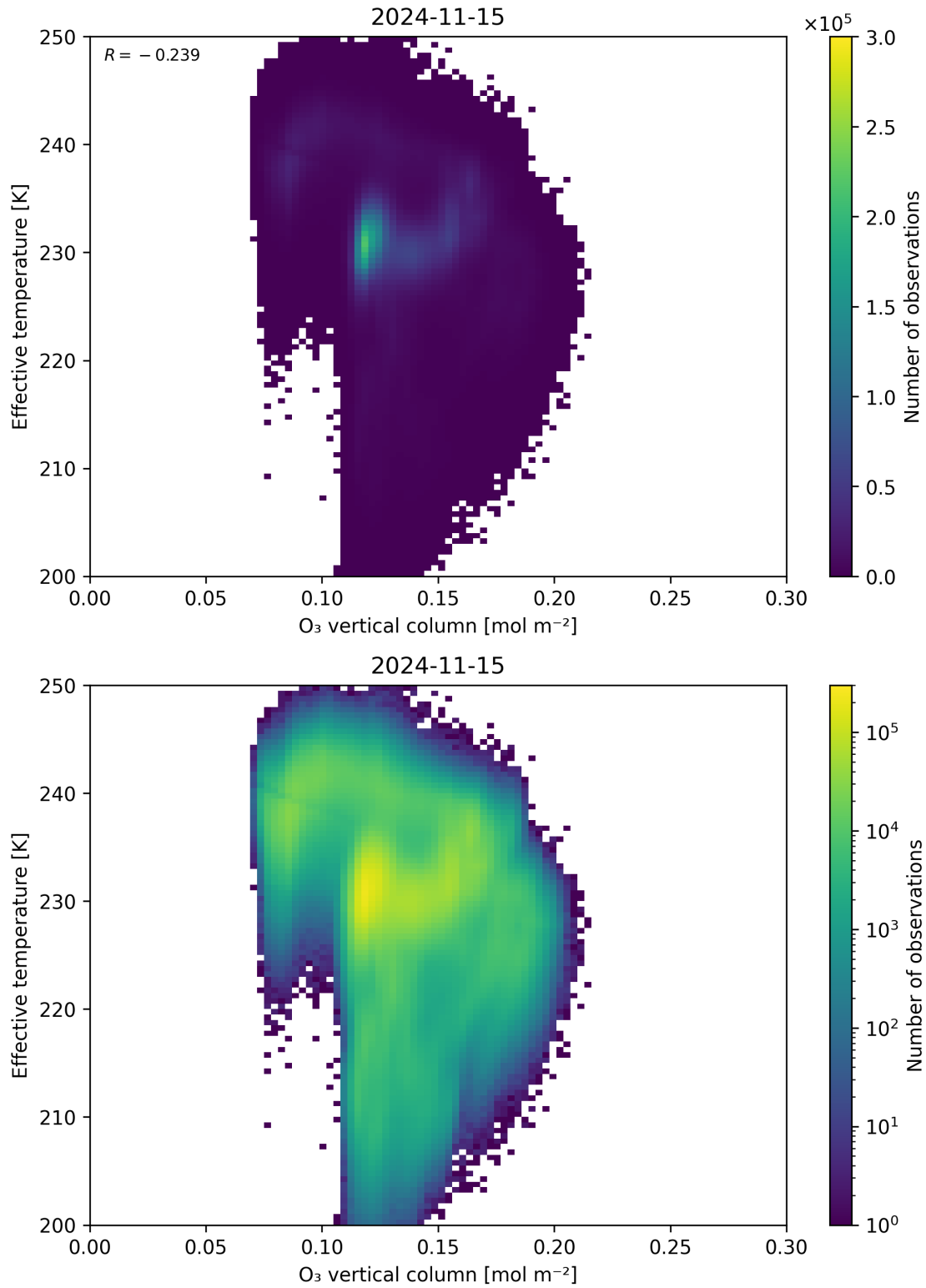
Figure 39: Scatter density plot of “O 3 vertical column” against “Effective temperature” for 2024-11-14 to 2024-11-16.
