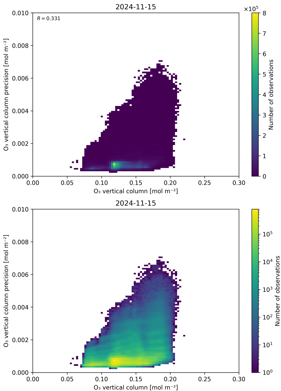
Figure 41: Scatter density plot of “O 3 vertical column” against “O 3 vertical column precision” for 2024-11-14 to 2024-11-16.
