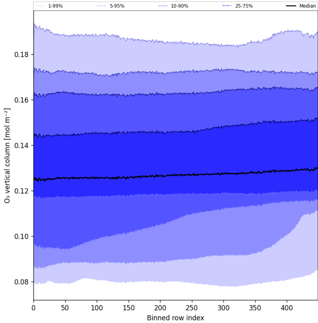
Figure 28: Along track statistics of “O 3 vertical column” for 2024-11-14 to 2024-11-16
