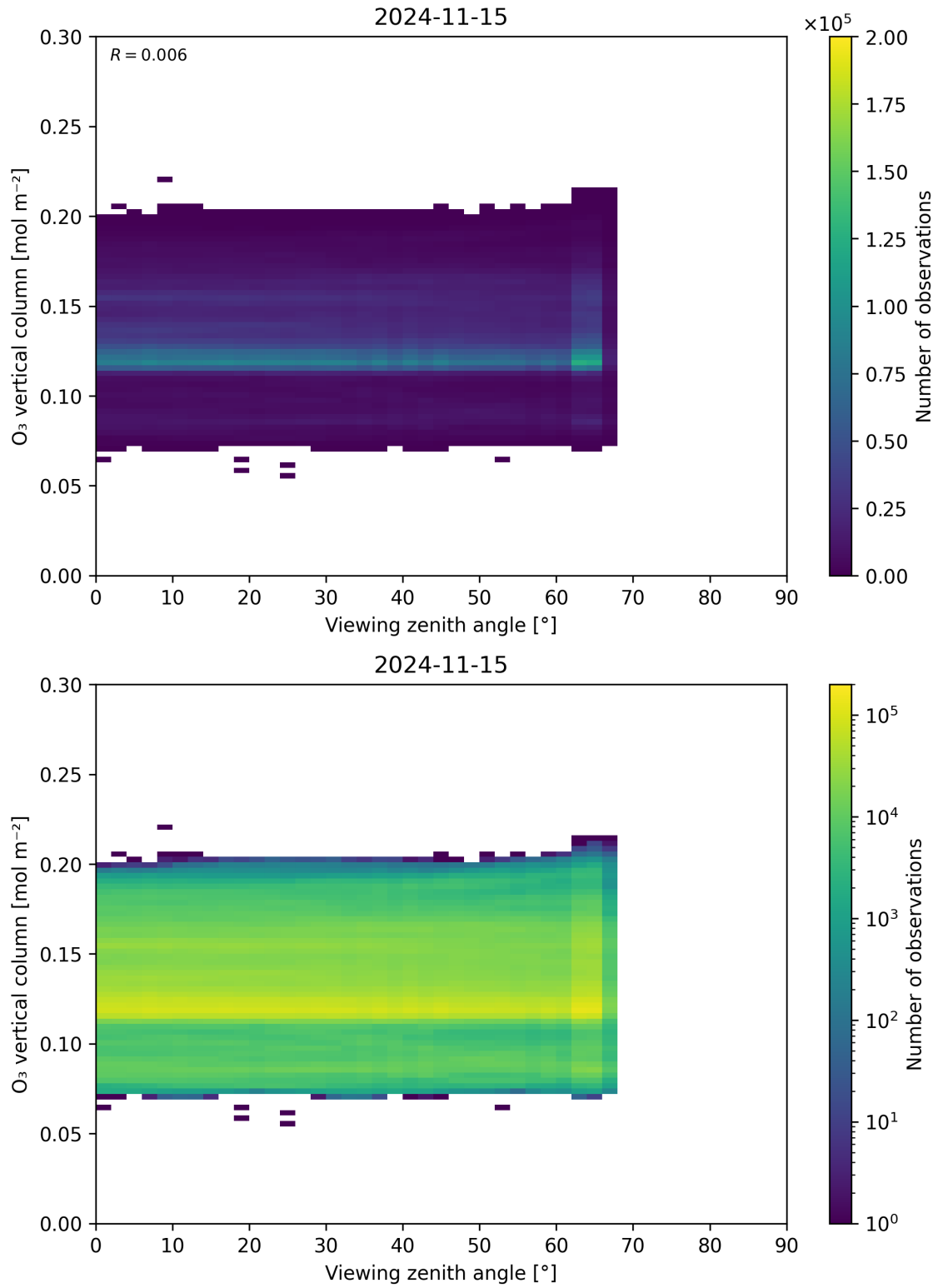
Figure 52: Scatter density plot of “Viewing zenith angle” against “O 3 vertical column” for 2024-11-14 to 2024-11-16.
