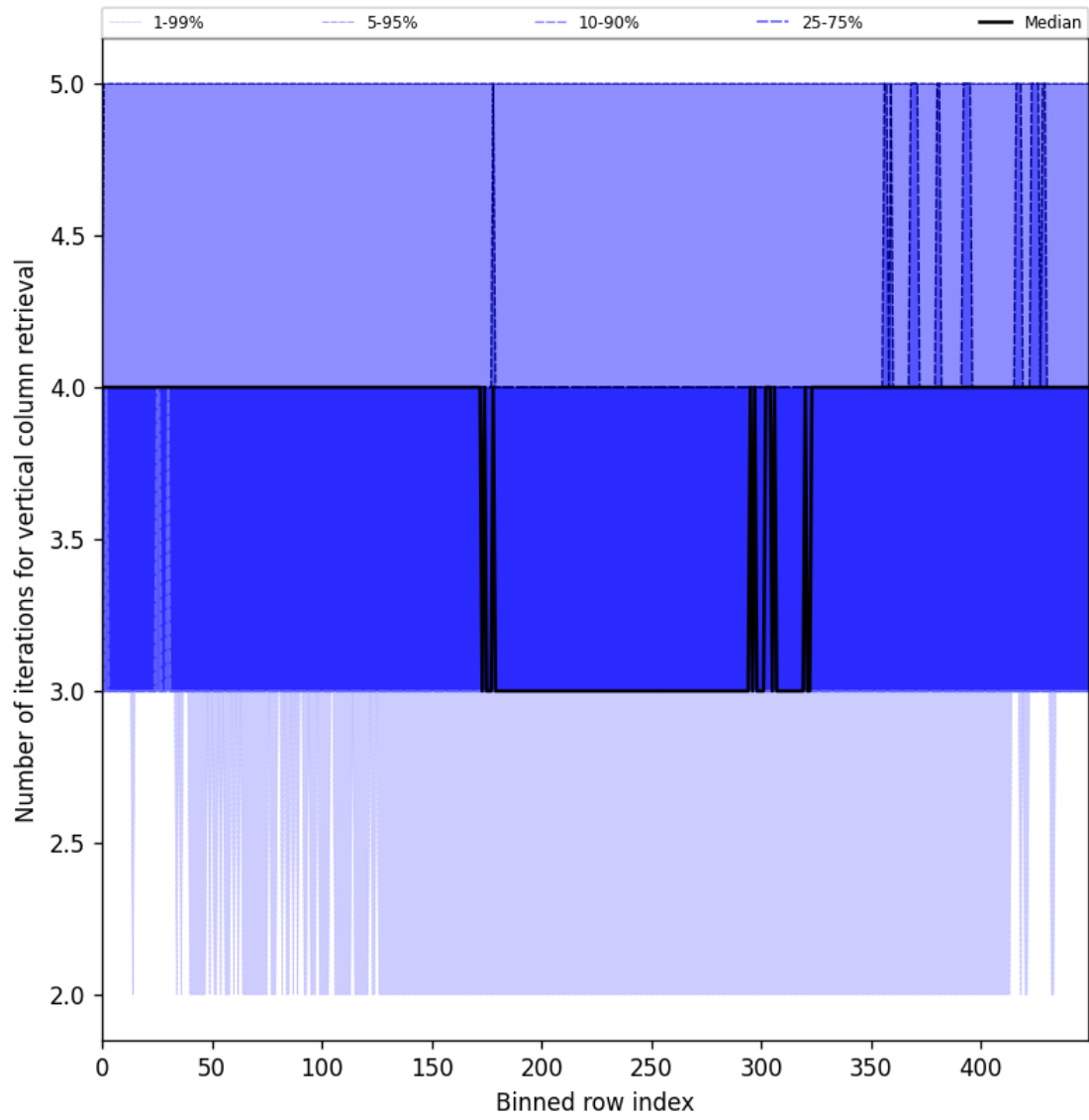
Figure 33: Along track statistics of “Number of iterations for vertical column retrieval” for 2024-11-14 to 2024-11-16
