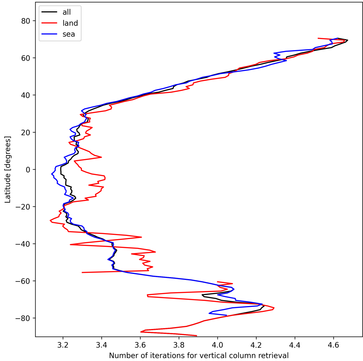
Figure 19: Zonal average of “Number of iterations for vertical column retrieval” for 2024-11-14 to 2024-11-16.
