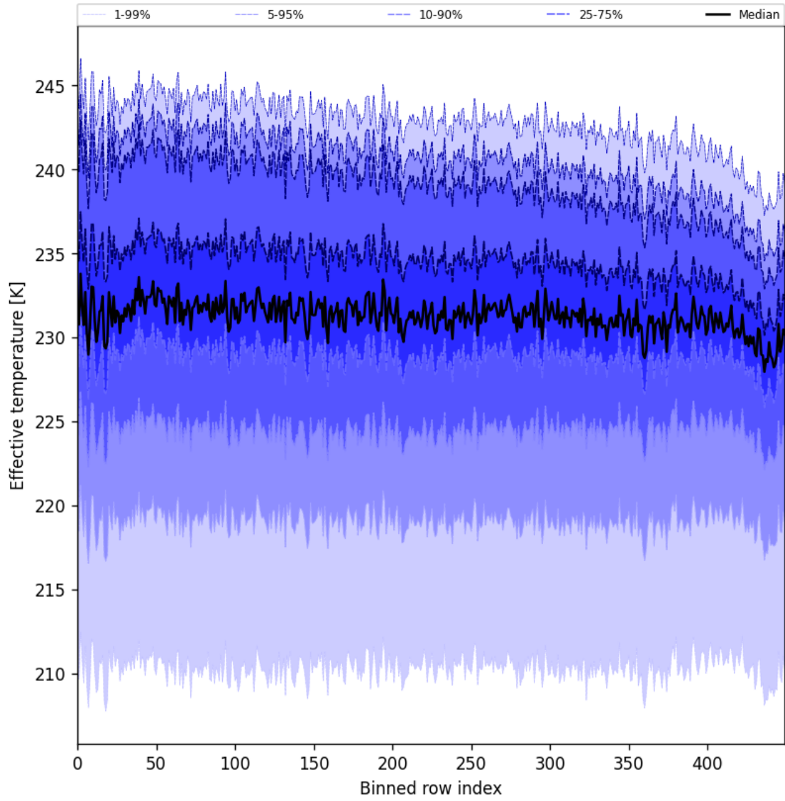
Figure 31: Along track statistics of “Effective temperature” for 2024-11-14 to 2024-11-16
