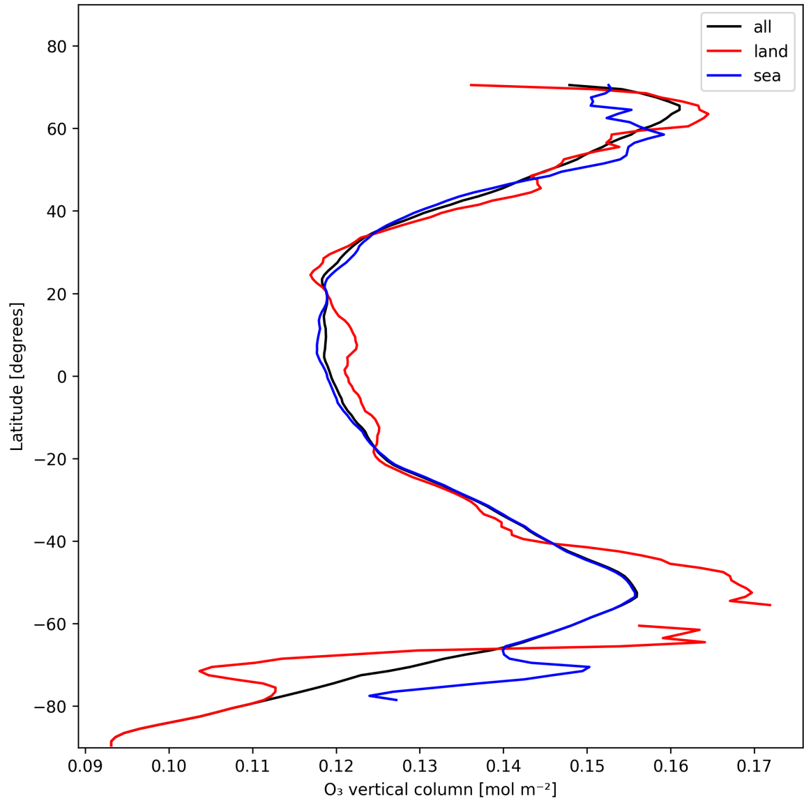
Figure 14: Zonal average of “O 3 vertical column” for 2024-11-14 to 2024-11-16.
