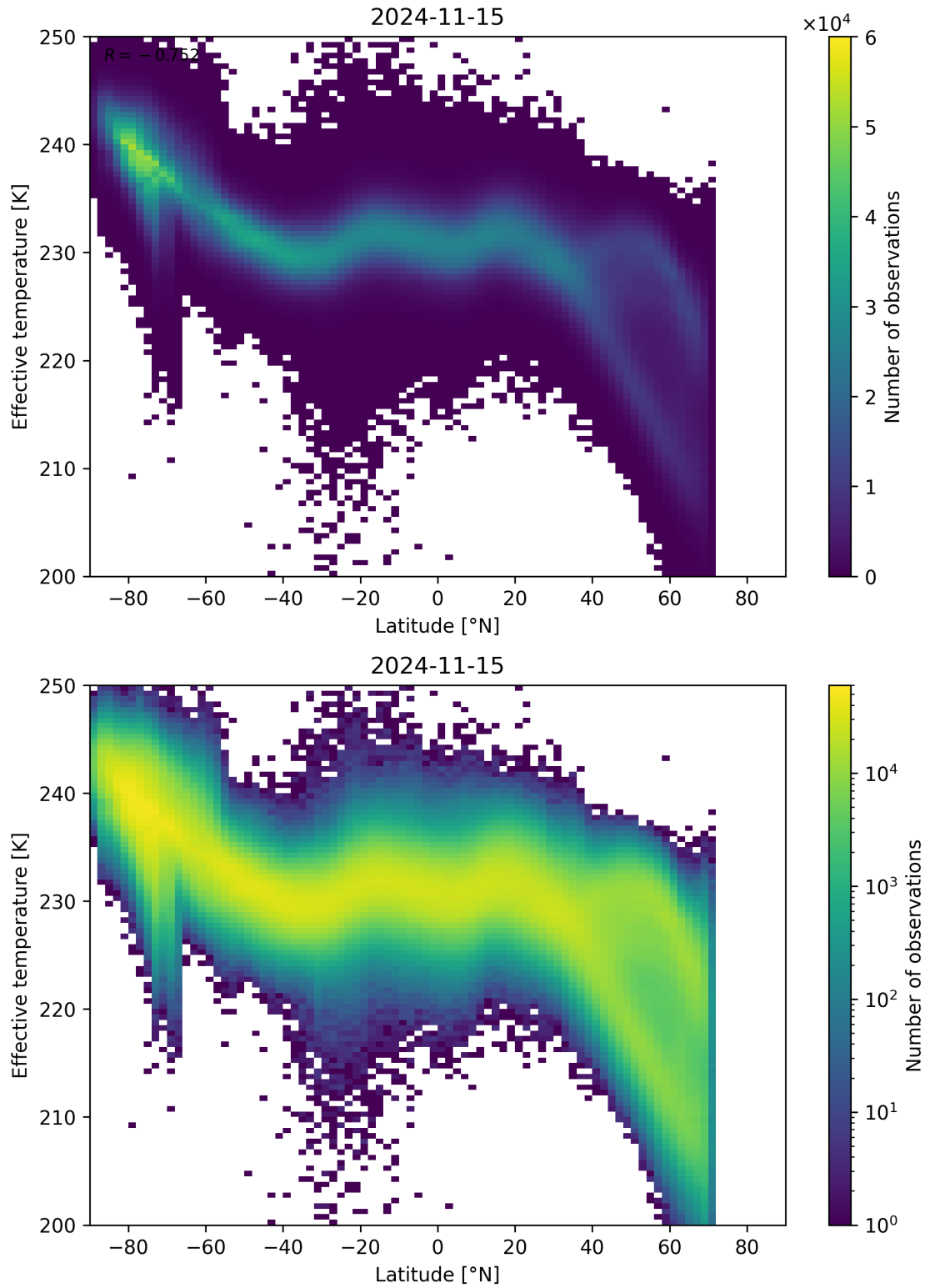
Figure 34: Scatter density plot of “Latitude” against “Effective temperature” for 2024-11-14 to 2024-11-16.
