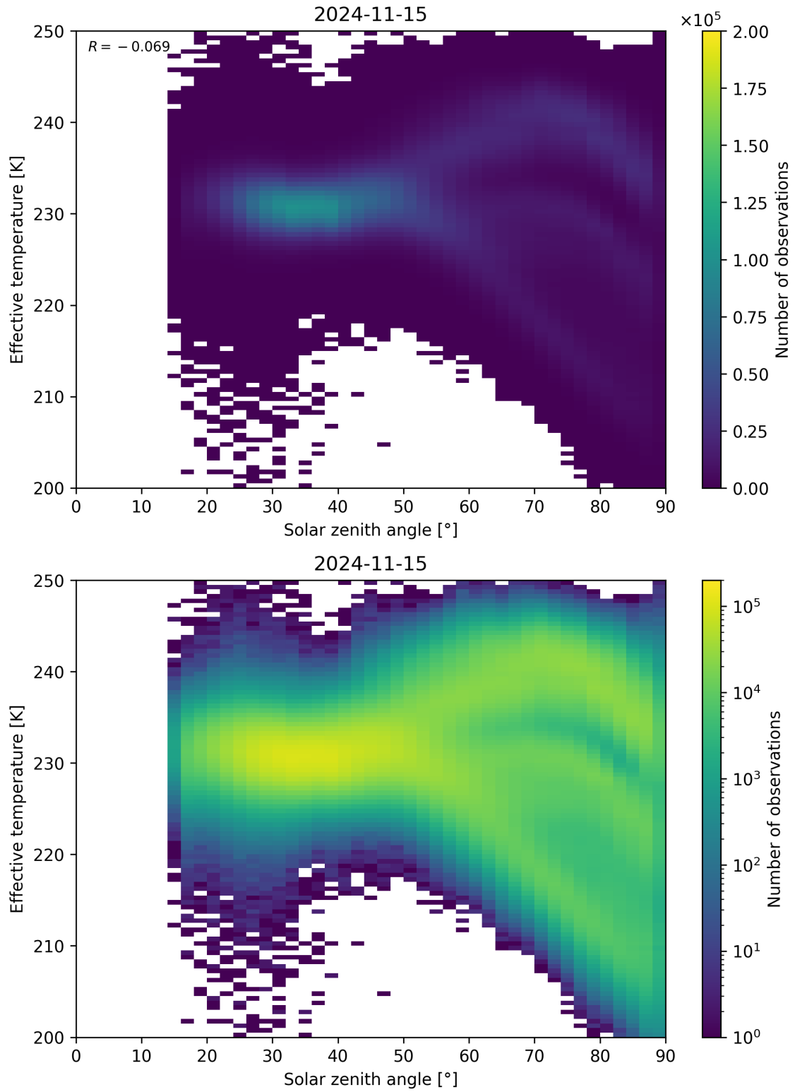
Figure 45: Scatter density plot of “Solar zenith angle” against “Effective temperature” for 2024-11-14 to 2024-11-16.
