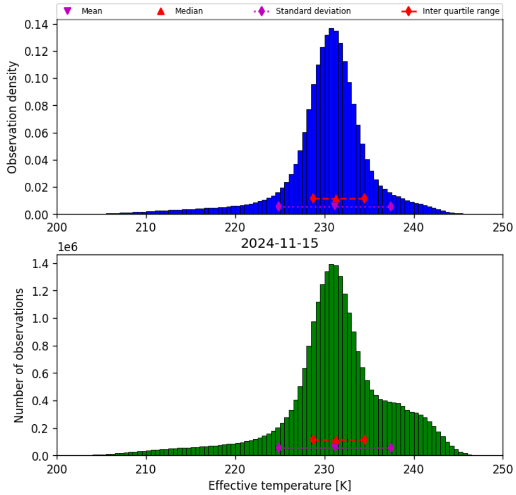
Figure 24: Histogram of “Effective temperature” for 2024-11-14 to 2024-11-16
