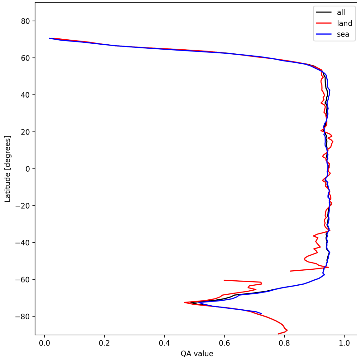
Figure 13: Zonal average of “QA value” for 2024-11-14 to 2024-11-16.
