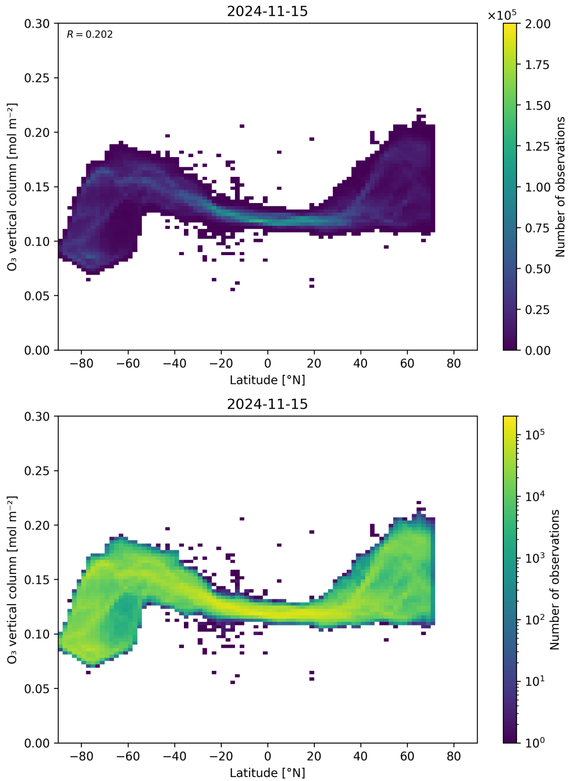
Figure 36: Scatter density plot of “Latitude” against “O 3 vertical column” for 2024-11-14 to 2024-11-16.
