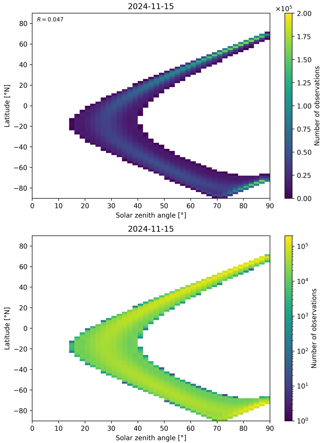
Figure 44: Scatter density plot of “Solar zenith angle” against “Latitude” for 2024-11-14 to 2024-11-16.
