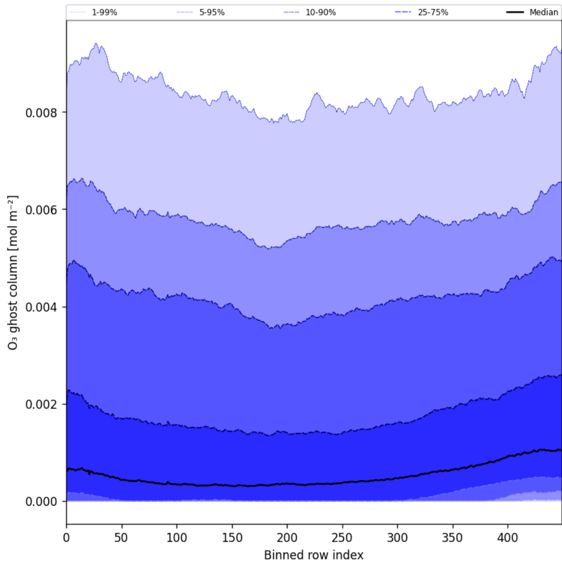
Figure 32: Along track statistics of “O 3 ghost column” for 2024-11-14 to 2024-11-16
