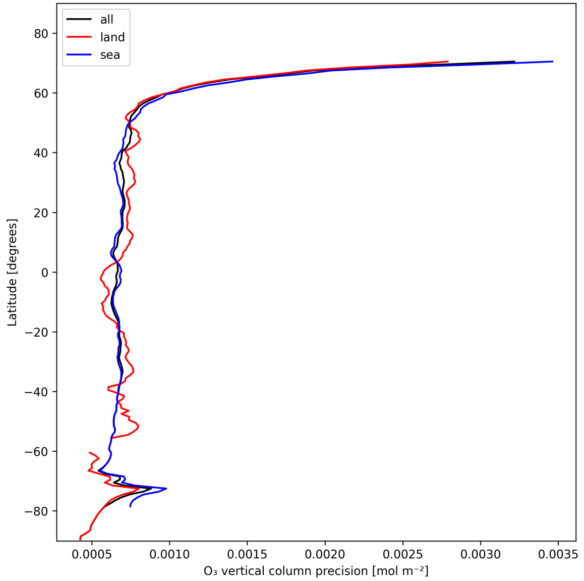
Figure 15: Zonal average of “O 3 vertical column precision” for 2024-11-14 to 2024-11-16.
