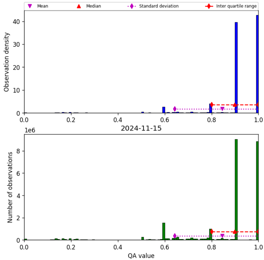
Figure 20: Histogram of “QA value” for 2024-11-14 to 2024-11-16
