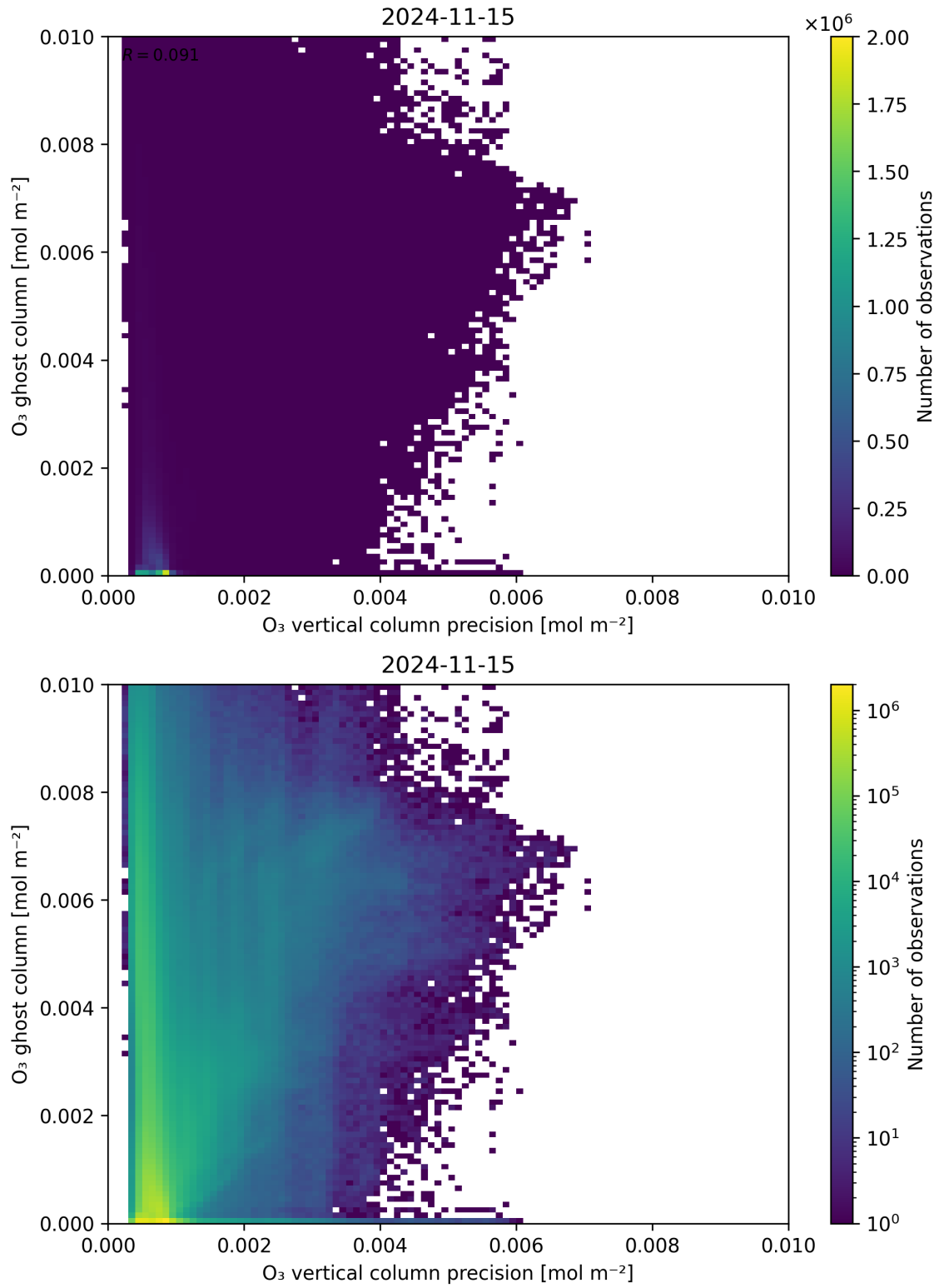
Figure 43: Scatter density plot of “ \text{O}_3 vertical column precision” against “ \text{O}_3 ghost column” for 2024-11-14 to 2024-11-16.
