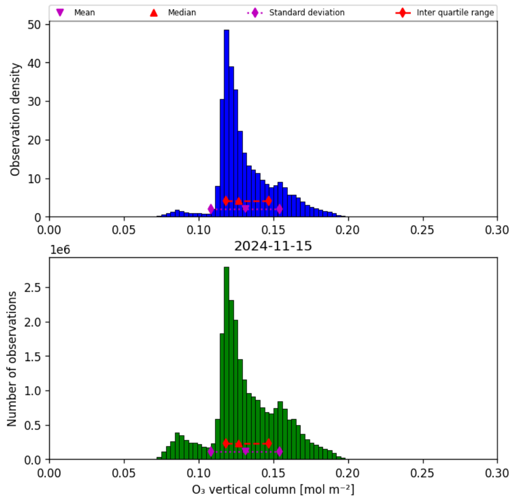
Figure 21: Histogram of “O 3 vertical column” for 2024-11-14 to 2024-11-16
