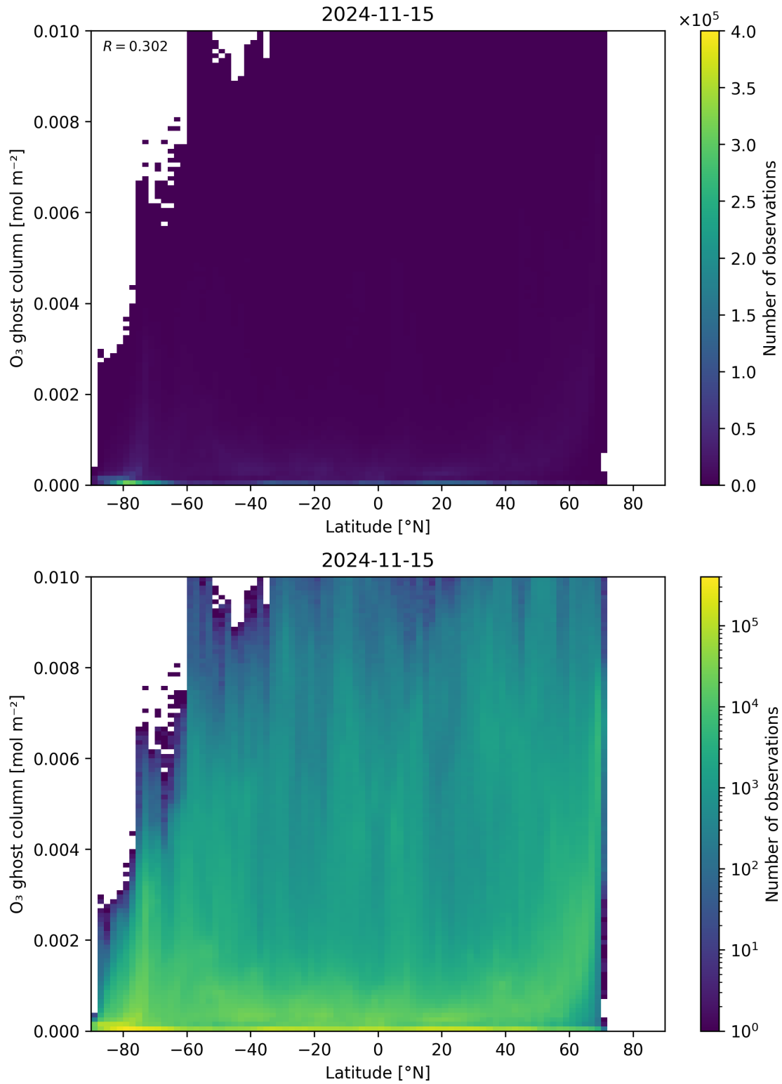
Figure 35: Scatter density plot of “Latitude” against “O 3 ghost column” for 2024-11-14 to 2024-11-16.
