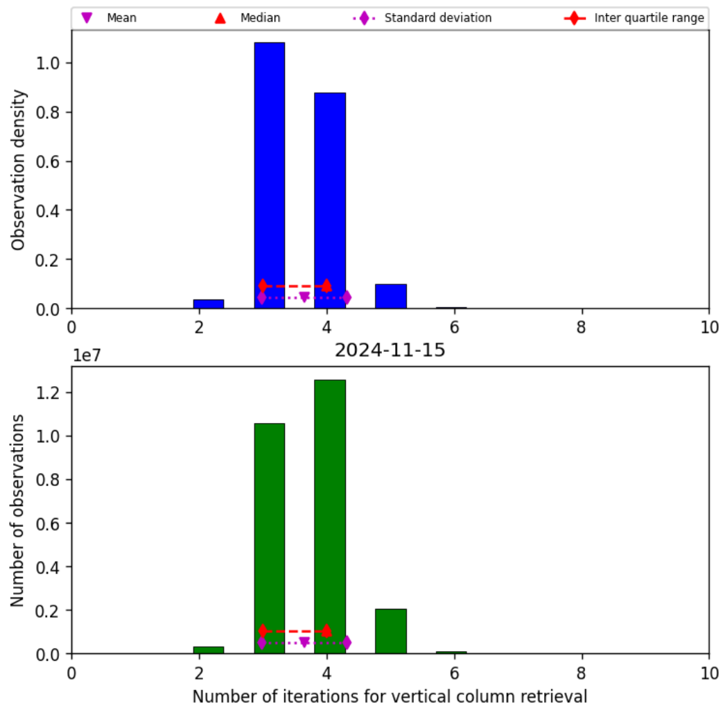
Figure 26: Histogram of “Number of iterations for vertical column retrieval” for 2024-11-14 to 2024-11-16
