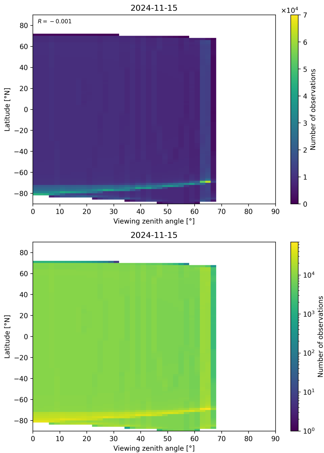
Figure 49: Scatter density plot of “Viewing zenith angle” against “Latitude” for 2024-11-14 to 2024-11-16.
