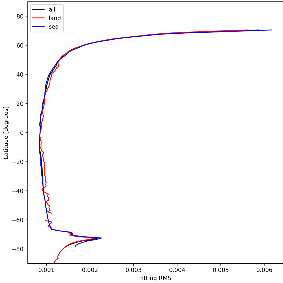
Figure 16: Zonal average of “Fitting RMS” for 2024-11-14 to 2024-11-16.
