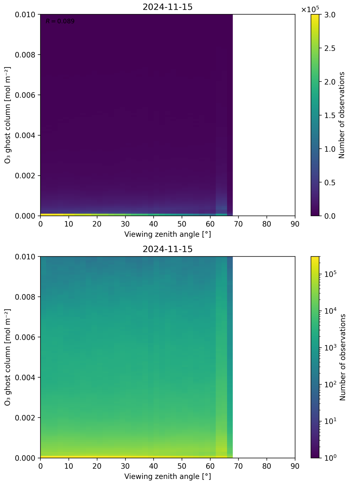
Figure 51: Scatter density plot of “Viewing zenith angle” against “O 3 ghost column” for 2024-11-14 to 2024-11-16.
