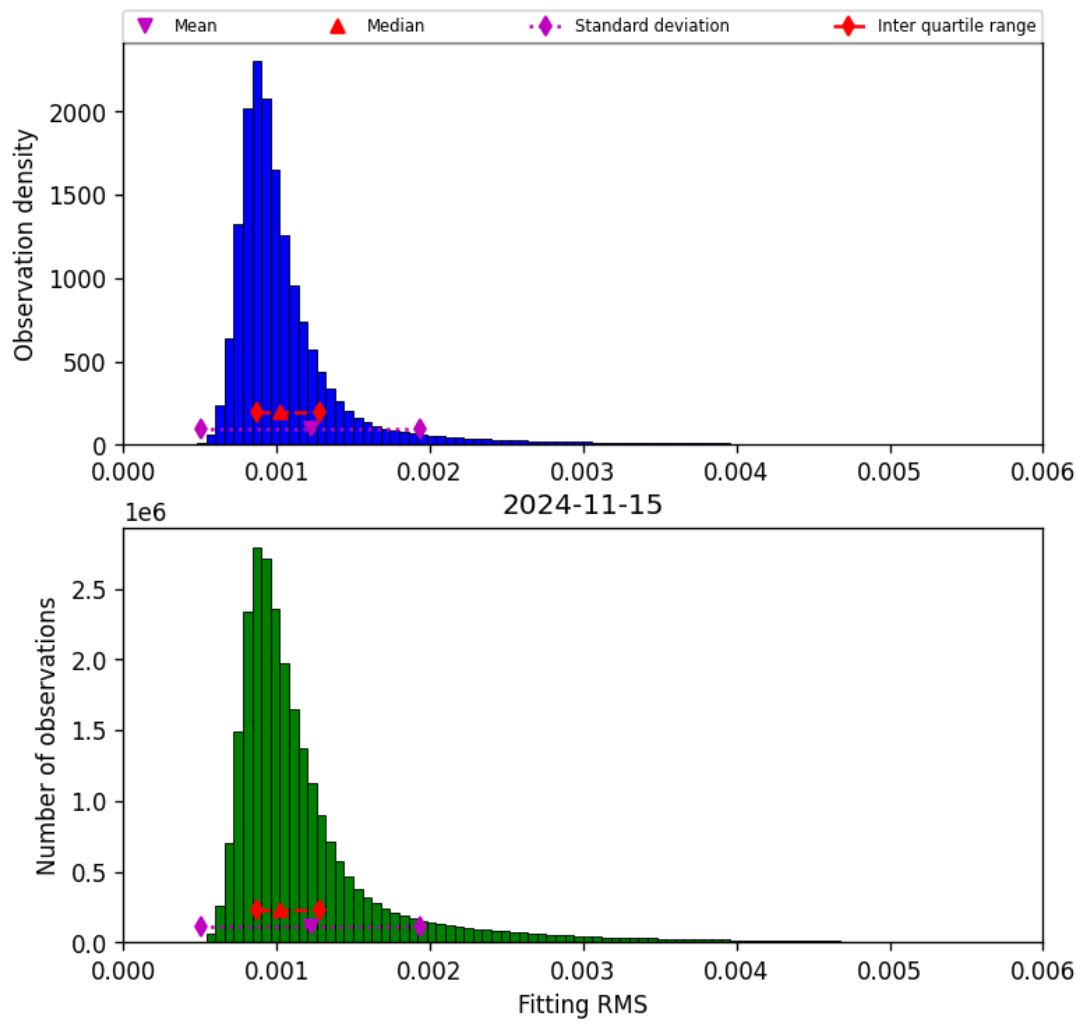
Figure 23: Histogram of “Fitting RMS” for 2024-11-14 to 2024-11-16
