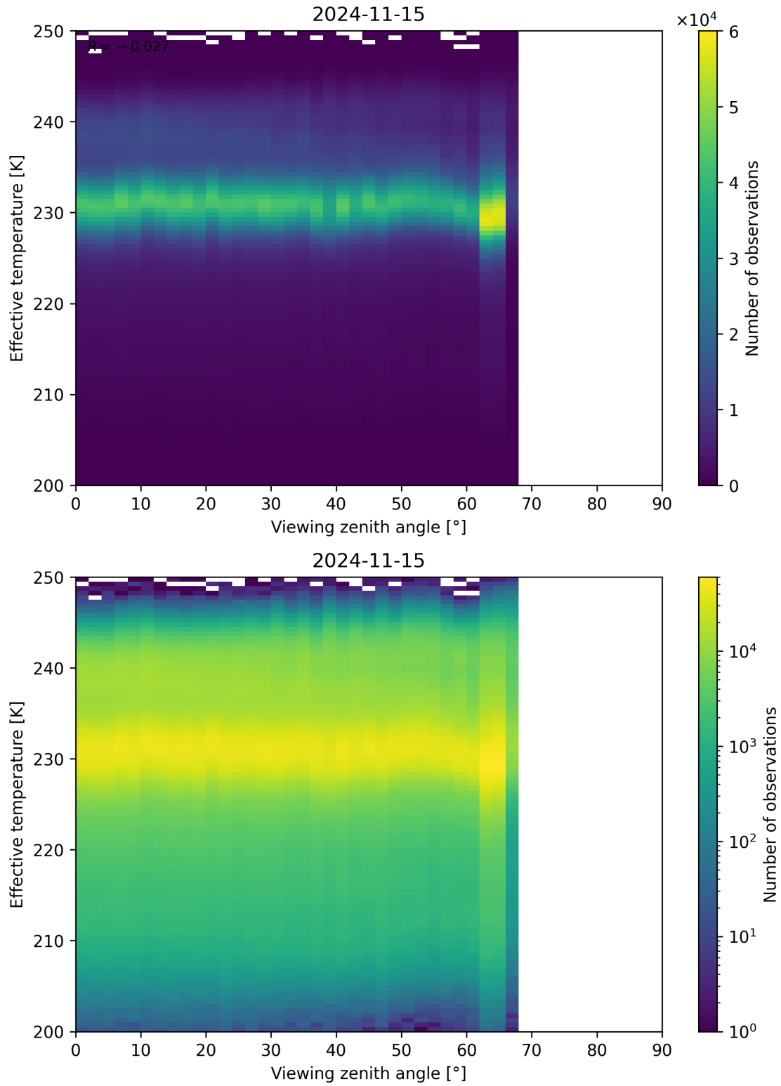
Figure 50: Scatter density plot of “Viewing zenith angle” against “Effective temperature” for 2024-11-14 to 2024-11-16.
