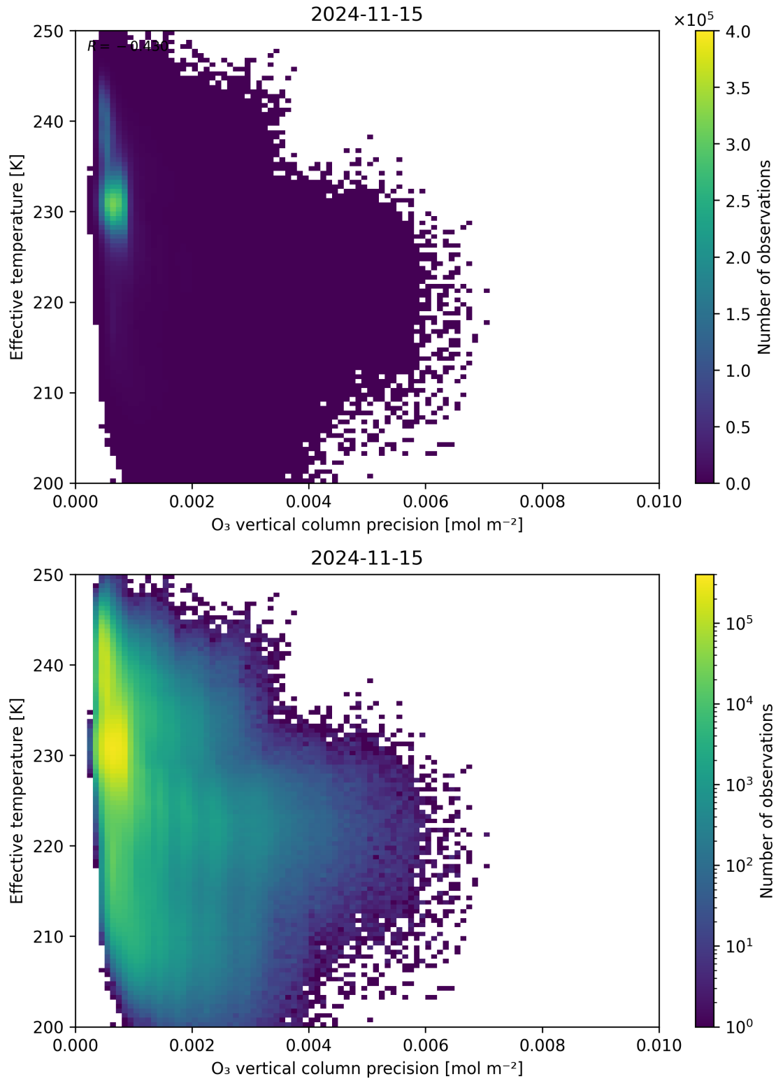
Figure 42: Scatter density plot of “O 3 vertical column precision” against “Effective temperature” for 2024-11-14 to 2024-11-16.
