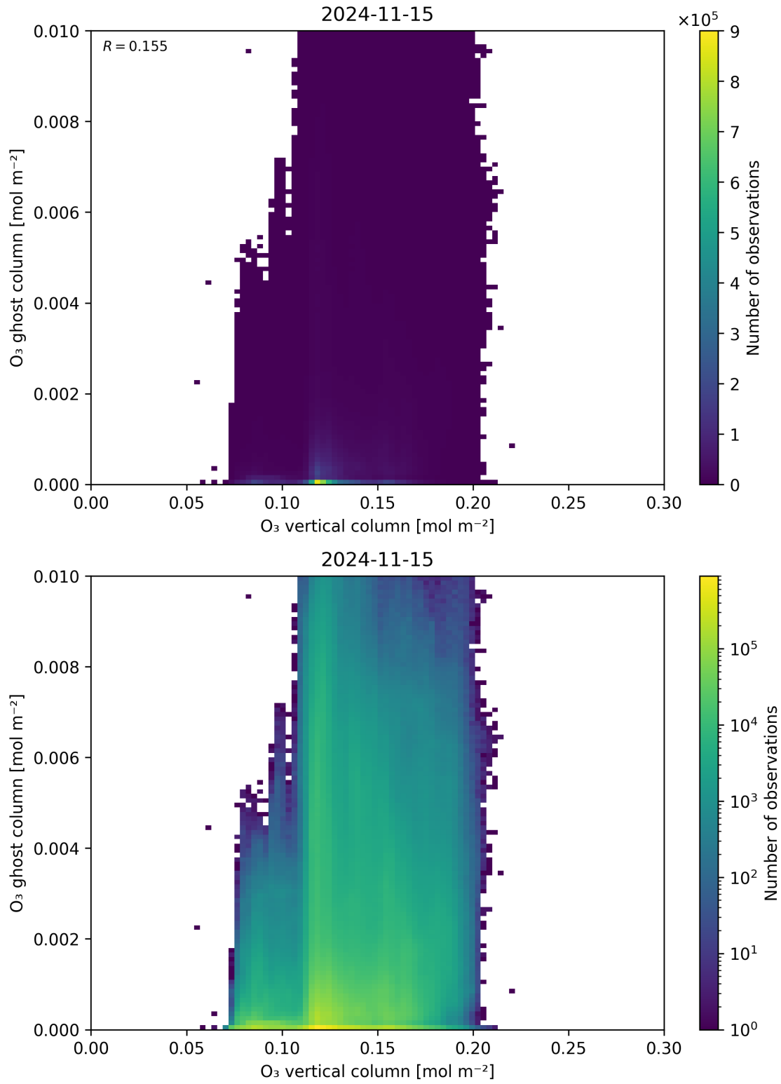
Figure 40: Scatter density plot of “O 3 vertical column” against “O 3 ghost column” for 2024-11-14 to 2024-11-16.
