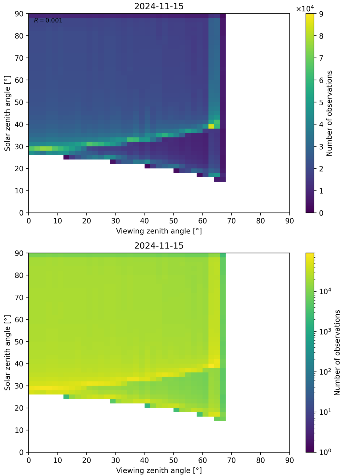
Figure 54: Scatter density plot of “Viewing zenith angle” against “Solar zenith angle” for 2024-11-14 to 2024-11-16.
