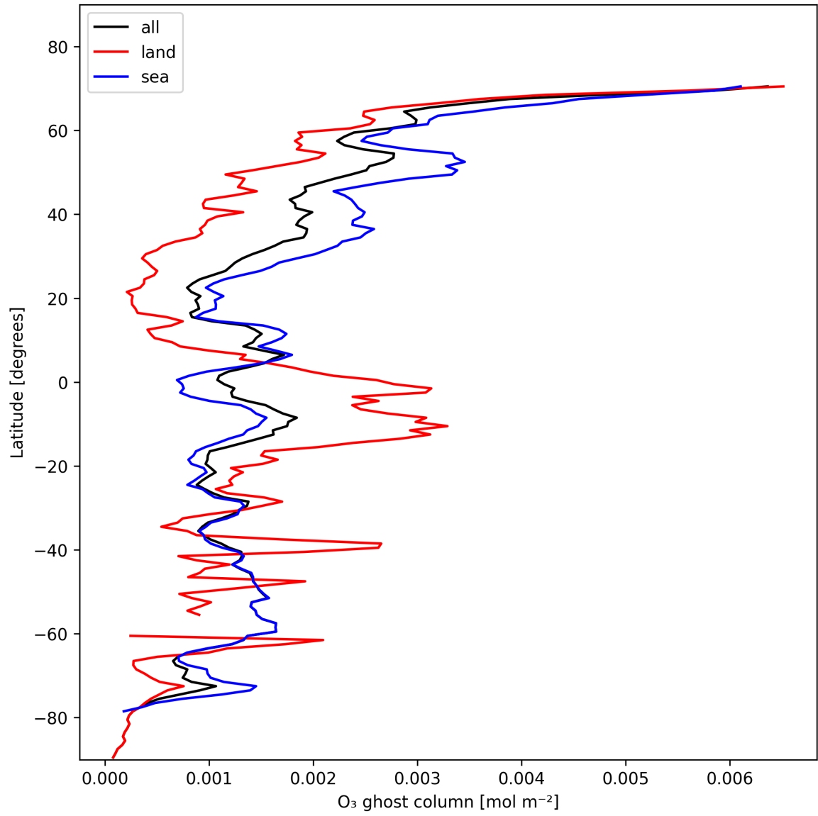
Figure 18: Zonal average of "O 3 ghost column" for 2024-11-14 to 2024-11-16.
