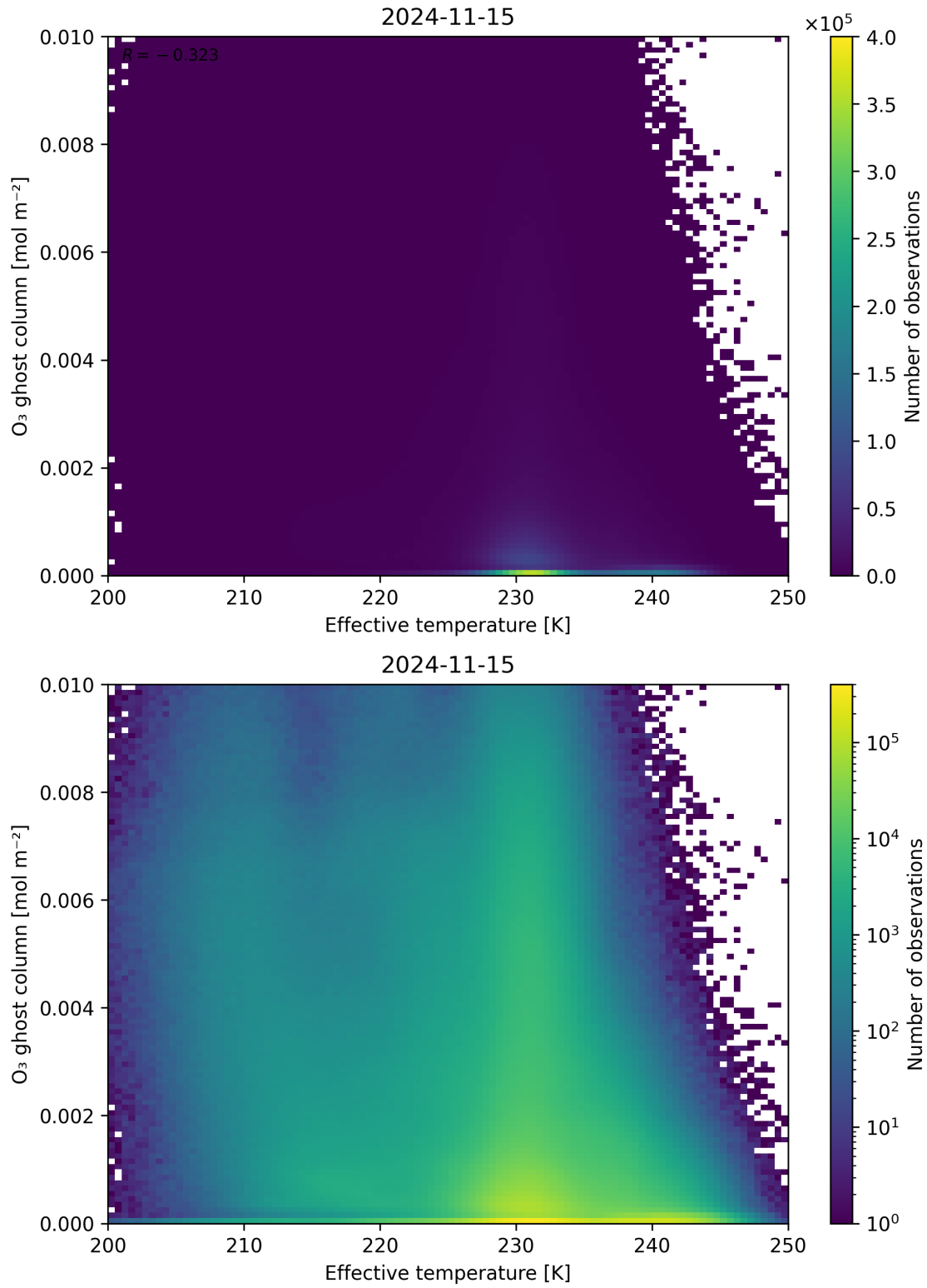
Figure 38: Scatter density plot of “Effective temperature” against “O 3 ghost column” for 2024-11-14 to 2024-11-16.
