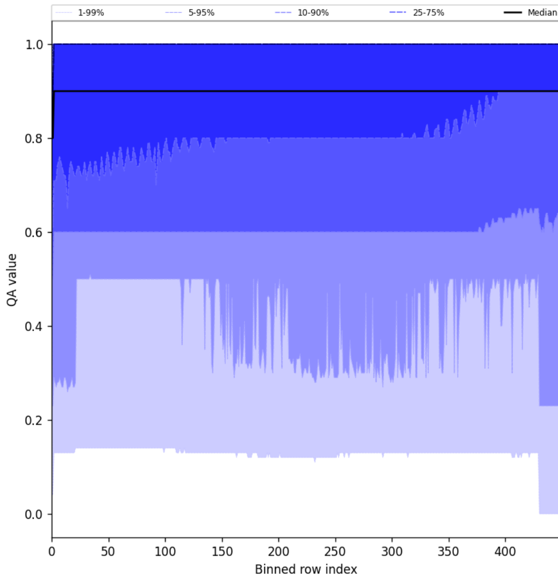
Figure 27: Along track statistics of “QA value” for 2024-11-14 to 2024-11-16
