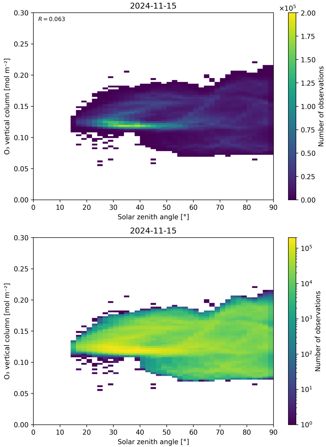
Figure 47: Scatter density plot of “Solar zenith angle” against “O 3 vertical column” for 2024-11-14 to 2024-11-16.
