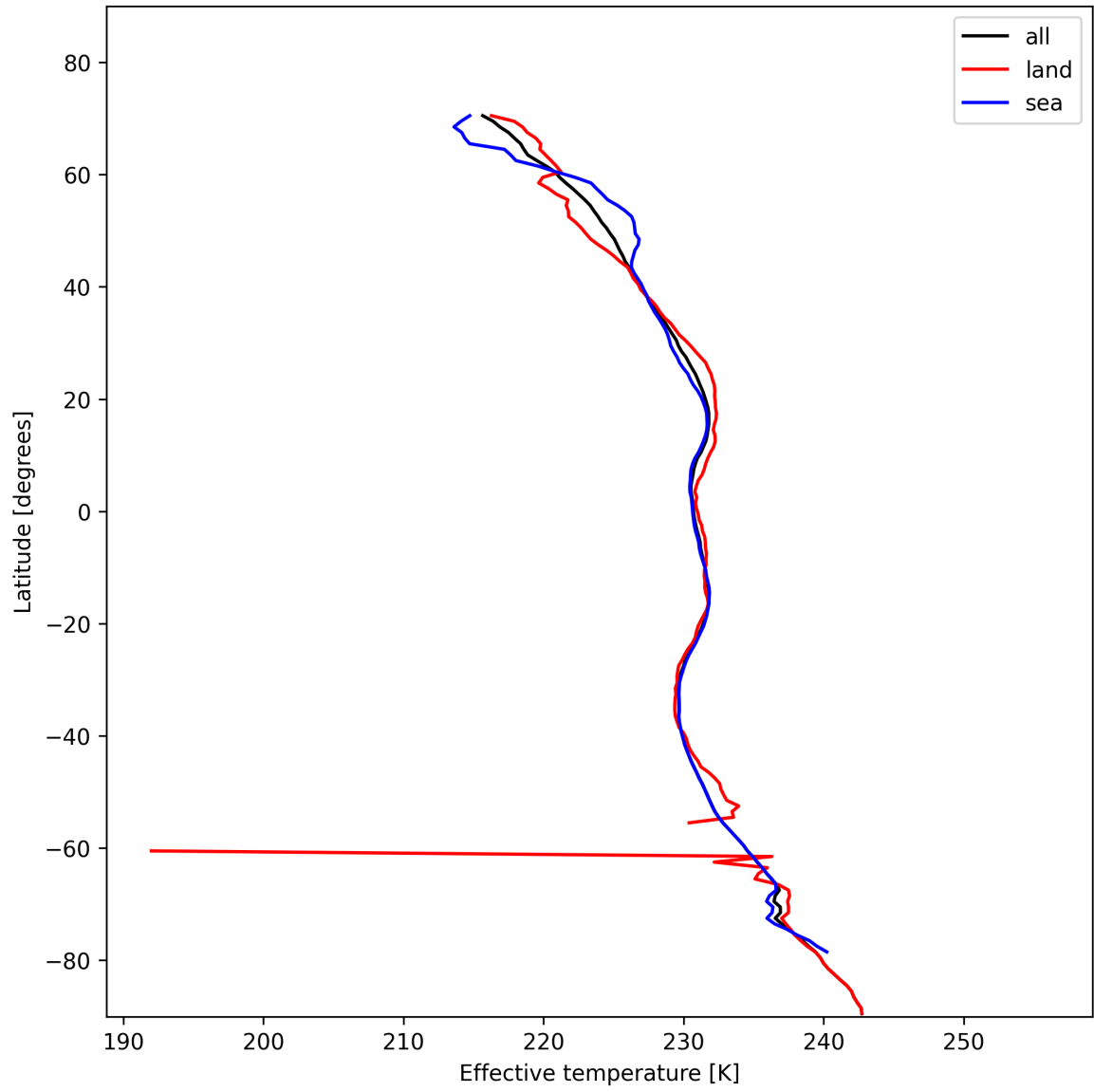
Figure 17: Zonal average of "Effective temperature" for 2024-11-14 to 2024-11-16.
