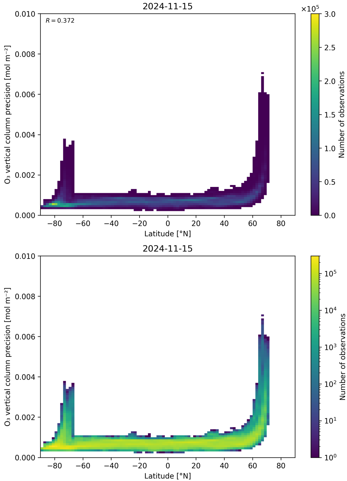
Figure 37: Scatter density plot of “Latitude” against “O 3 vertical column precision” for 2024-11-14 to 2024-11-16.
