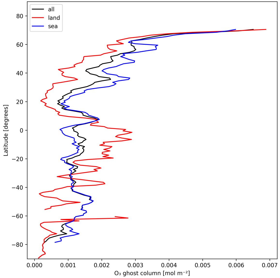
Figure 18: Zonal average of "O 3 ghost column" for 2024-11-15 to 2024-11-17.
