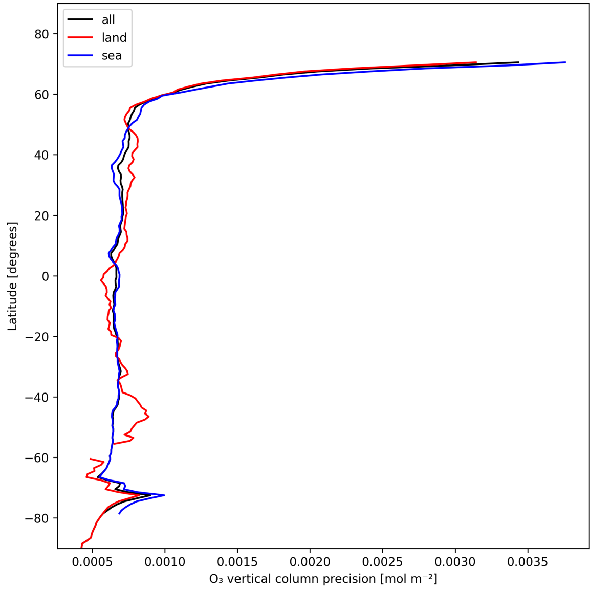
Figure 15: Zonal average of “O 3 vertical column precision” for 2024-11-15 to 2024-11-17.
