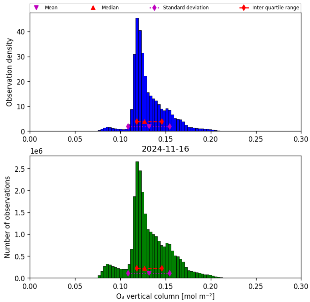
Figure 21: Histogram of “O 3 vertical column” for 2024-11-15 to 2024-11-17
