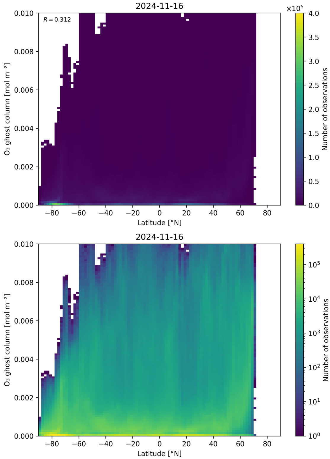
Figure 35: Scatter density plot of “Latitude” against “O 3 ghost column” for 2024-11-15 to 2024-11-17.
