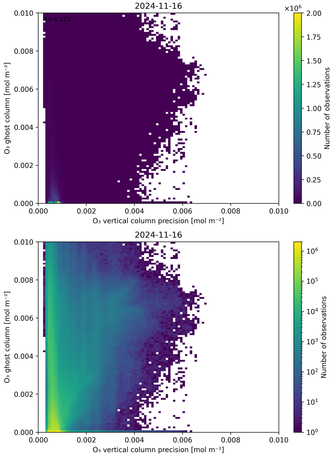
Figure 43: Scatter density plot of “ \text{O}_3 vertical column precision” against “ \text{O}_3 ghost column” for 2024-11-15 to 2024-11-17.
