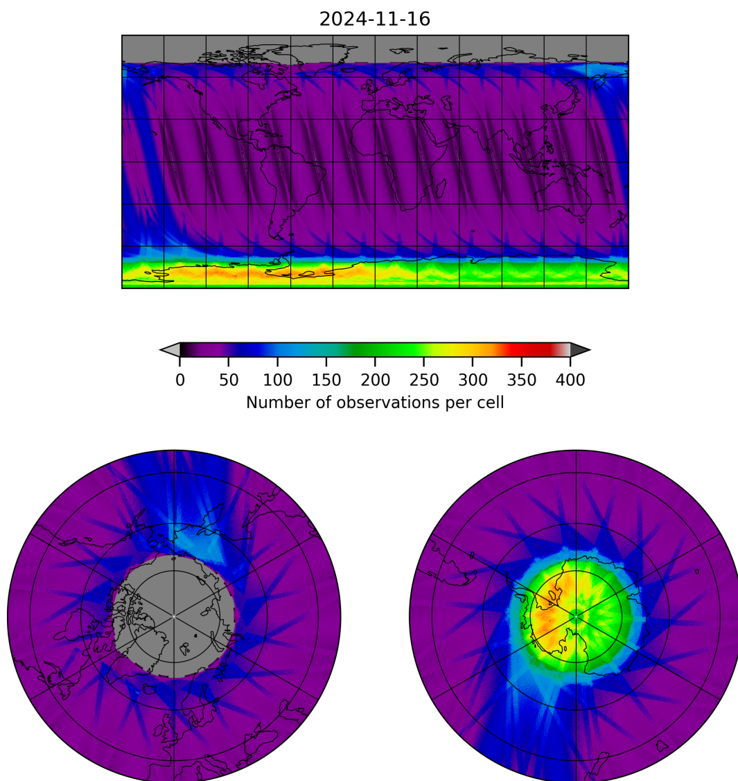
Figure 12: Map of the number of observations for 2024-11-15 to 2024-11-17
