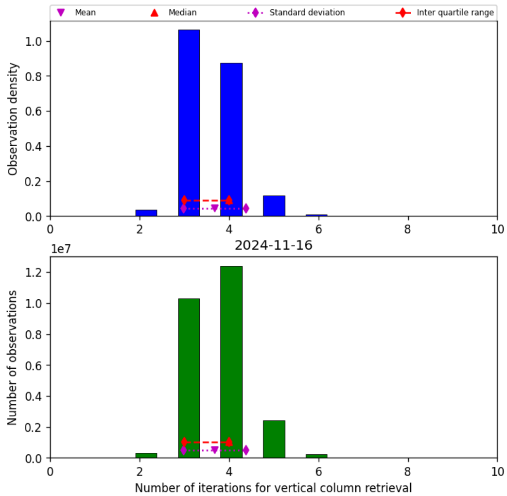
Figure 26: Histogram of “Number of iterations for vertical column retrieval” for 2024-11-15 to 2024-11-17
