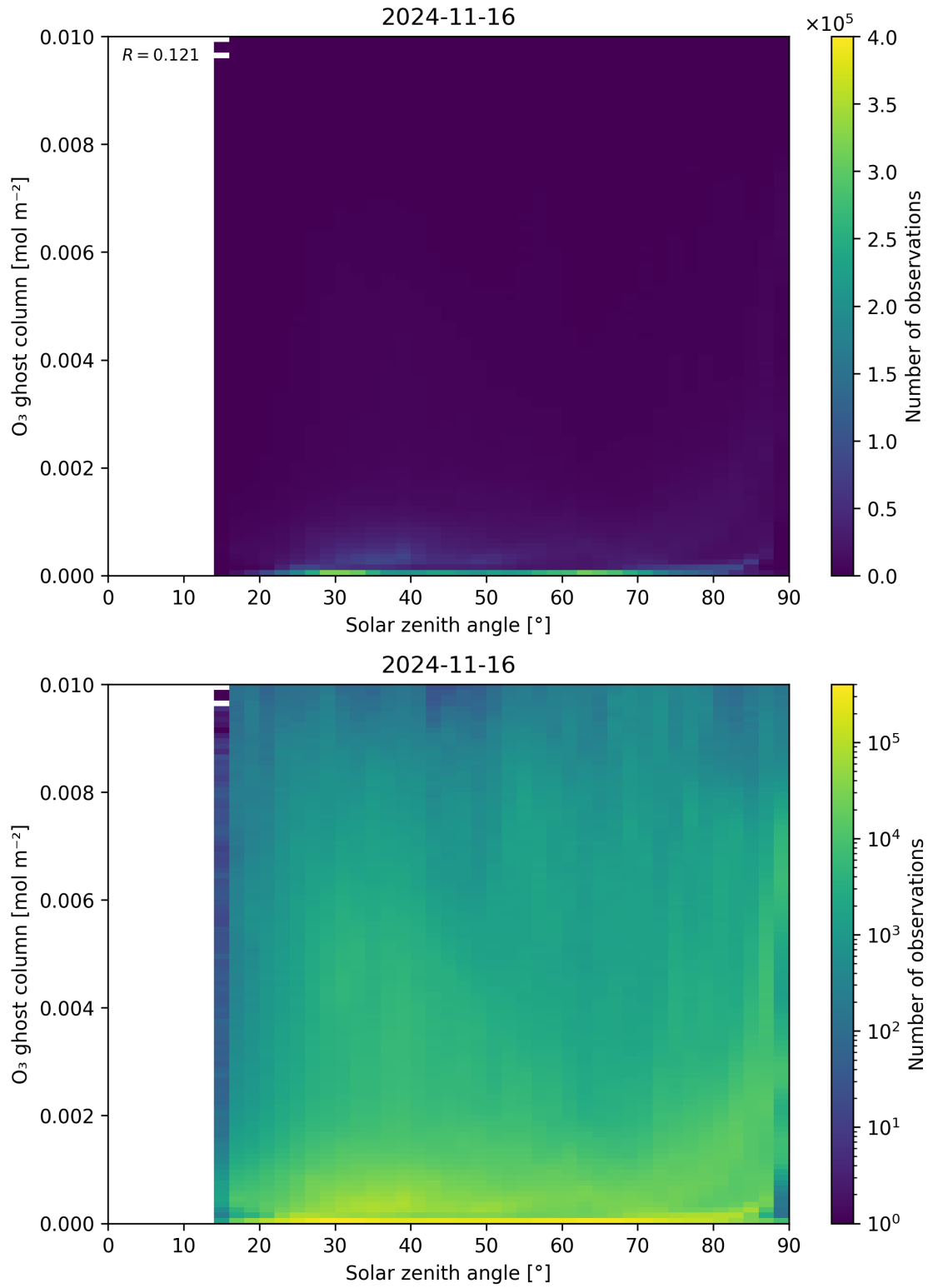
Figure 46: Scatter density plot of “Solar zenith angle” against “O 3 ghost column” for 2024-11-15 to 2024-11-17.
