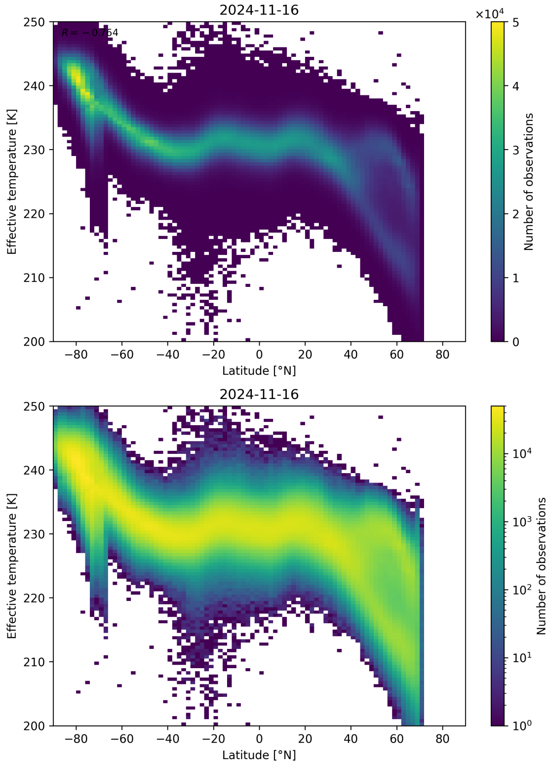
Figure 34: Scatter density plot of “Latitude” against “Effective temperature” for 2024-11-15 to 2024-11-17.
