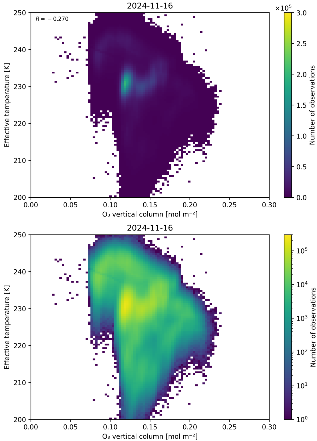
Figure 39: Scatter density plot of “O 3 vertical column” against “Effective temperature” for 2024-11-15 to 2024-11-17.
