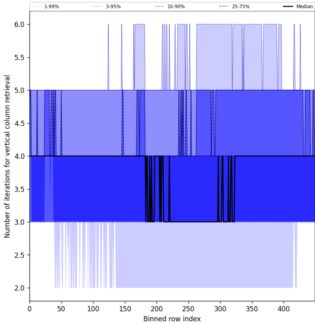
Figure 33: Along track statistics of “Number of iterations for vertical column retrieval” for 2024-11-15 to 2024-11-17
