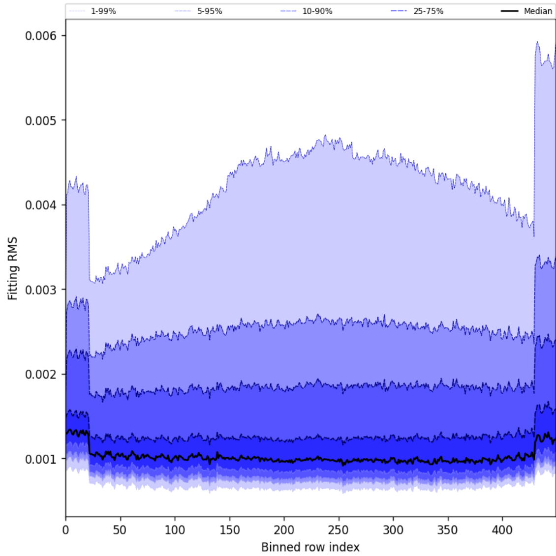
Figure 30: Along track statistics of “Fitting RMS” for 2024-11-15 to 2024-11-17
