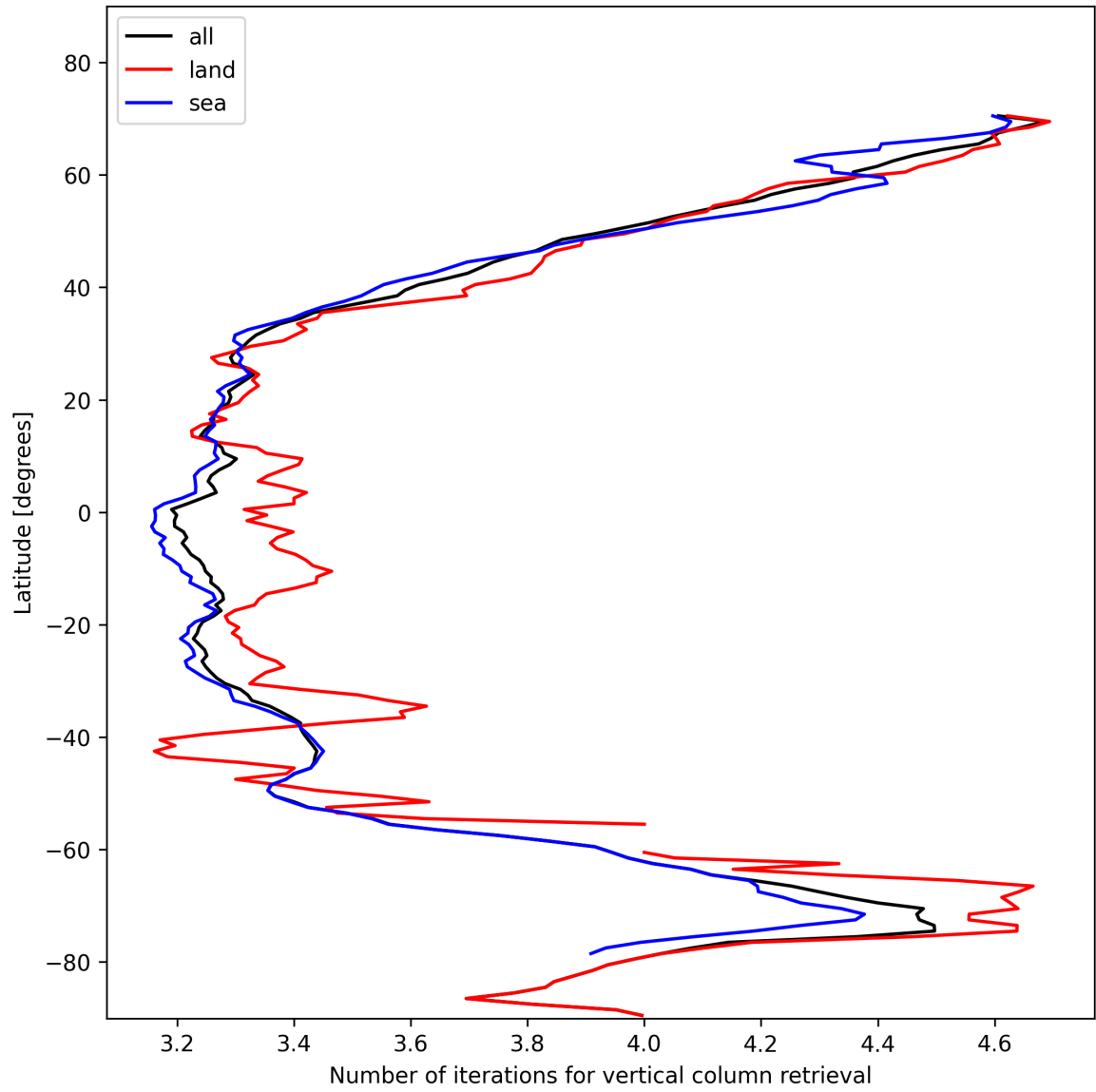
Figure 19: Zonal average of “Number of iterations for vertical column retrieval” for 2024-11-15 to 2024-11-17.
