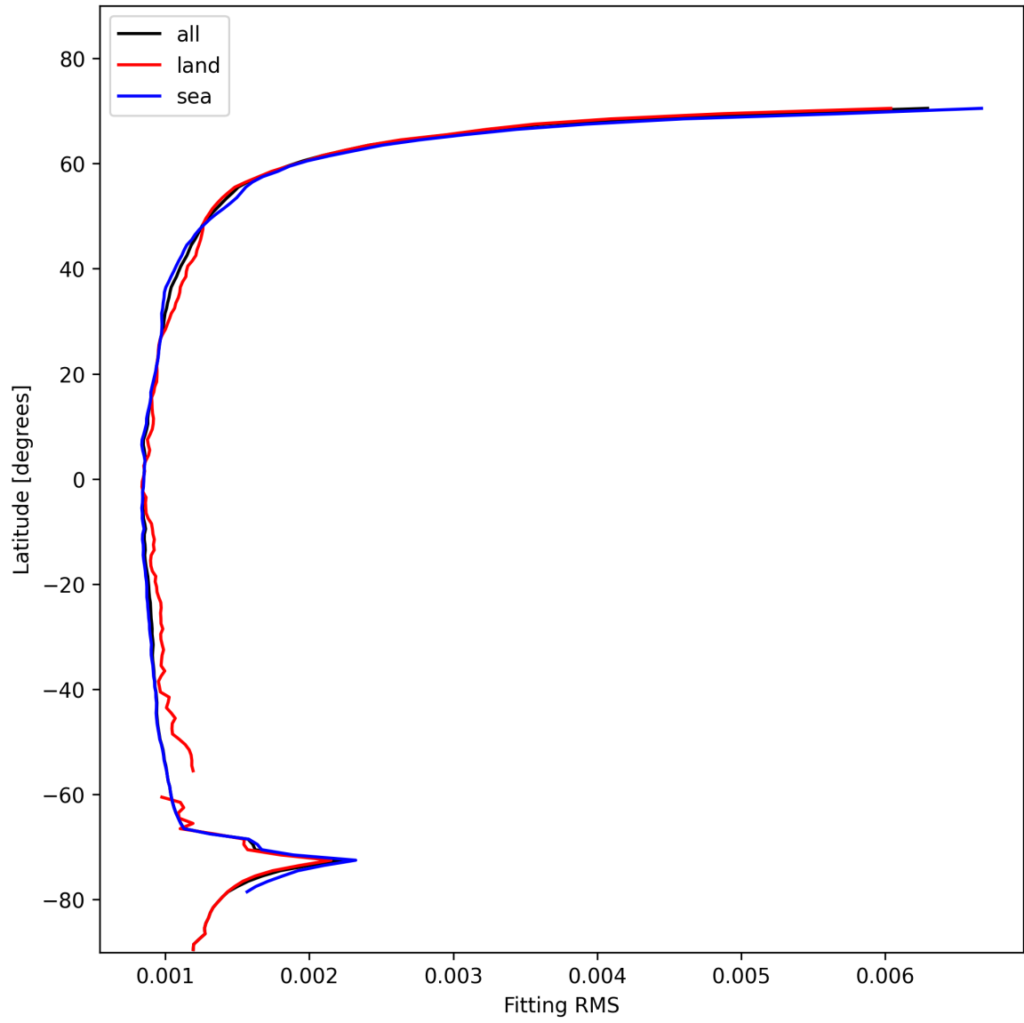
Figure 16: Zonal average of “Fitting RMS” for 2024-11-15 to 2024-11-17.
