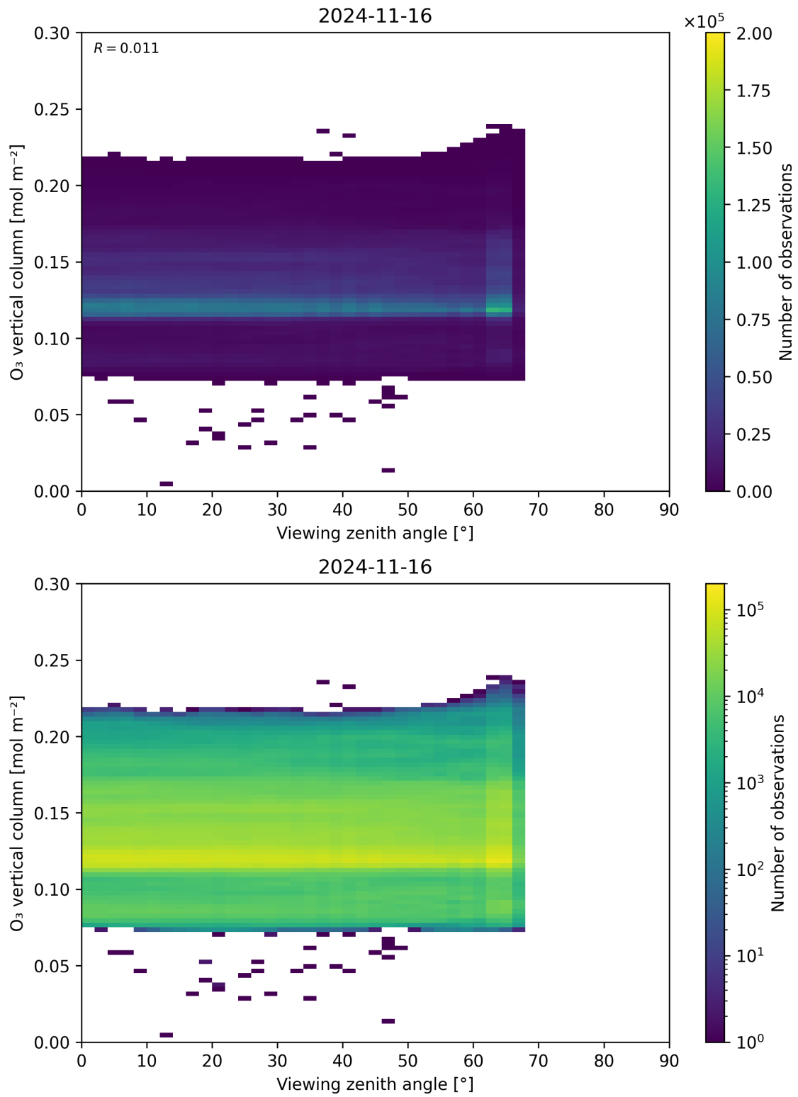
Figure 52: Scatter density plot of “Viewing zenith angle” against “O 3 vertical column” for 2024-11-15 to 2024-11-17.
