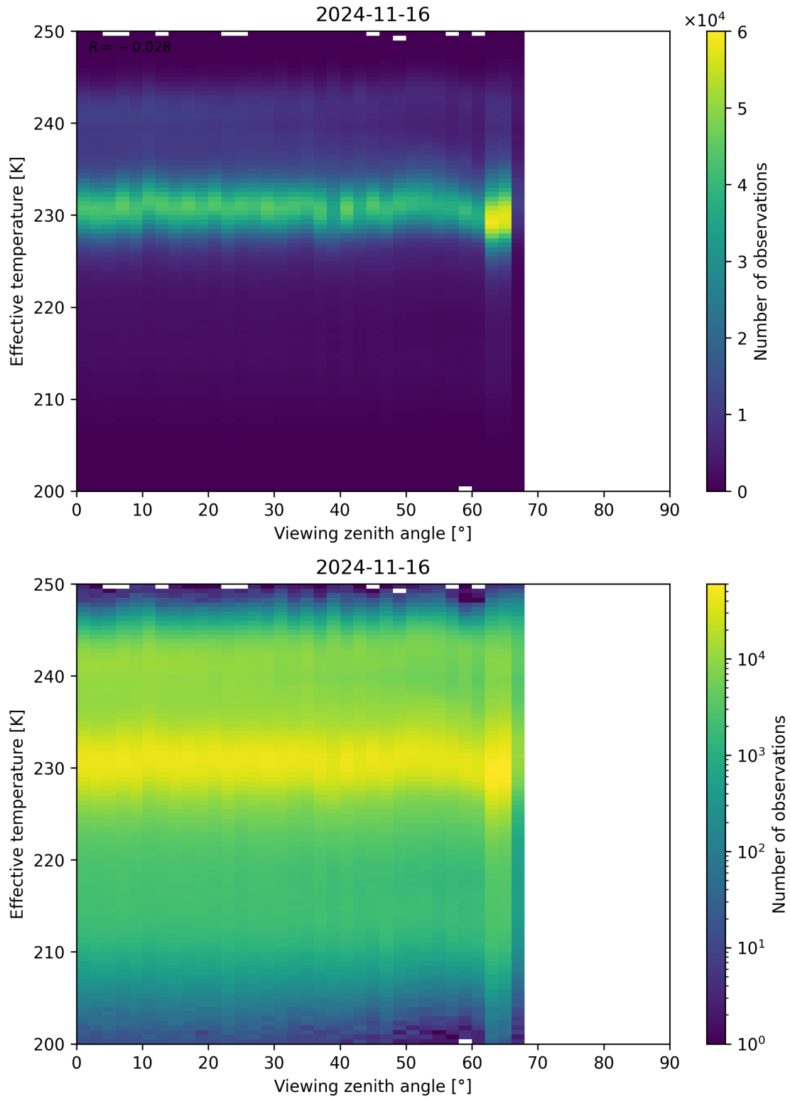
Figure 50: Scatter density plot of “Viewing zenith angle” against “Effective temperature” for 2024-11-15 to 2024-11-17.
