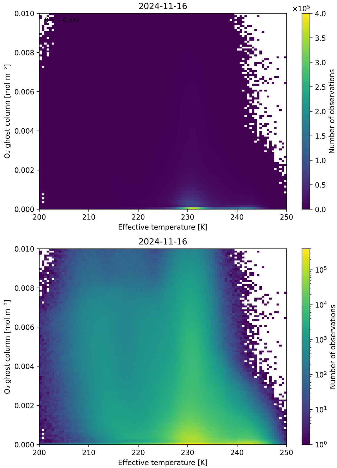
Figure 38: Scatter density plot of “Effective temperature” against “O 3 ghost column” for 2024-11-15 to 2024-11-17.
