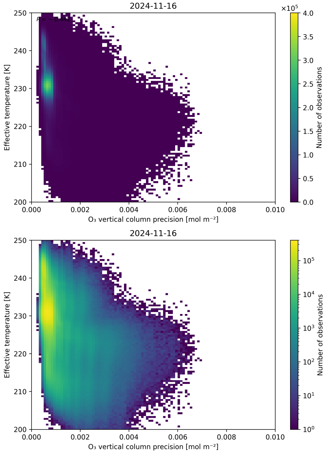
Figure 42: Scatter density plot of “O 3 vertical column precision” against “Effective temperature” for 2024-11-15 to 2024-11-17.
