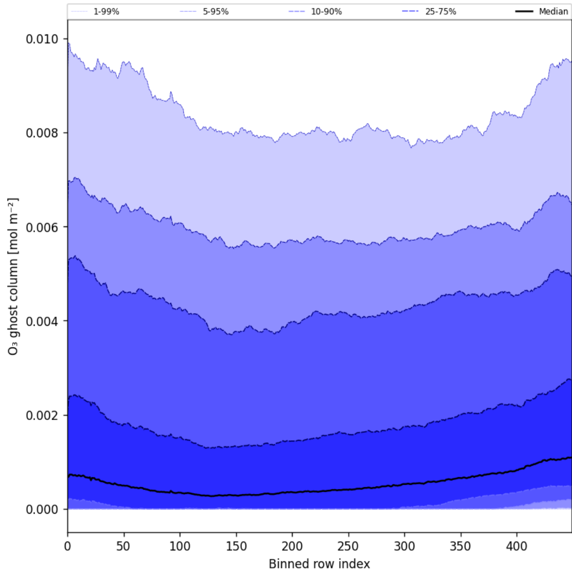
Figure 32: Along track statistics of “O 3 ghost column” for 2024-11-15 to 2024-11-17
