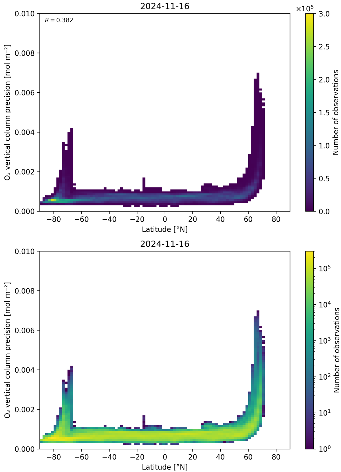
Figure 37: Scatter density plot of “Latitude” against “O 3 vertical column precision” for 2024-11-15 to 2024-11-17.
