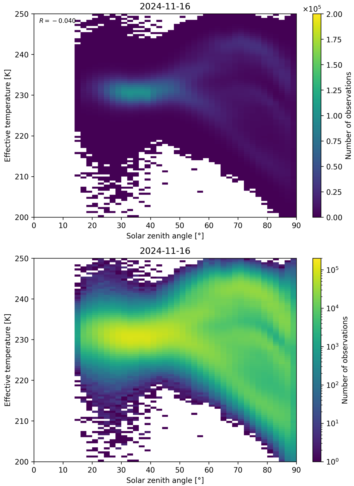
Figure 45: Scatter density plot of “Solar zenith angle” against “Effective temperature” for 2024-11-15 to 2024-11-17.
