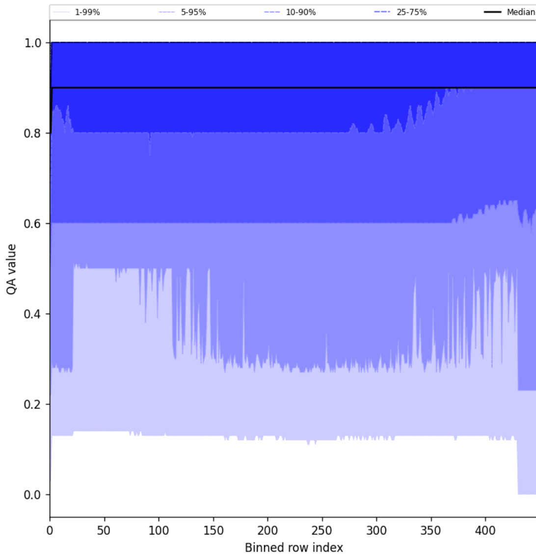
Figure 27: Along track statistics of “QA value” for 2024-11-15 to 2024-11-17
