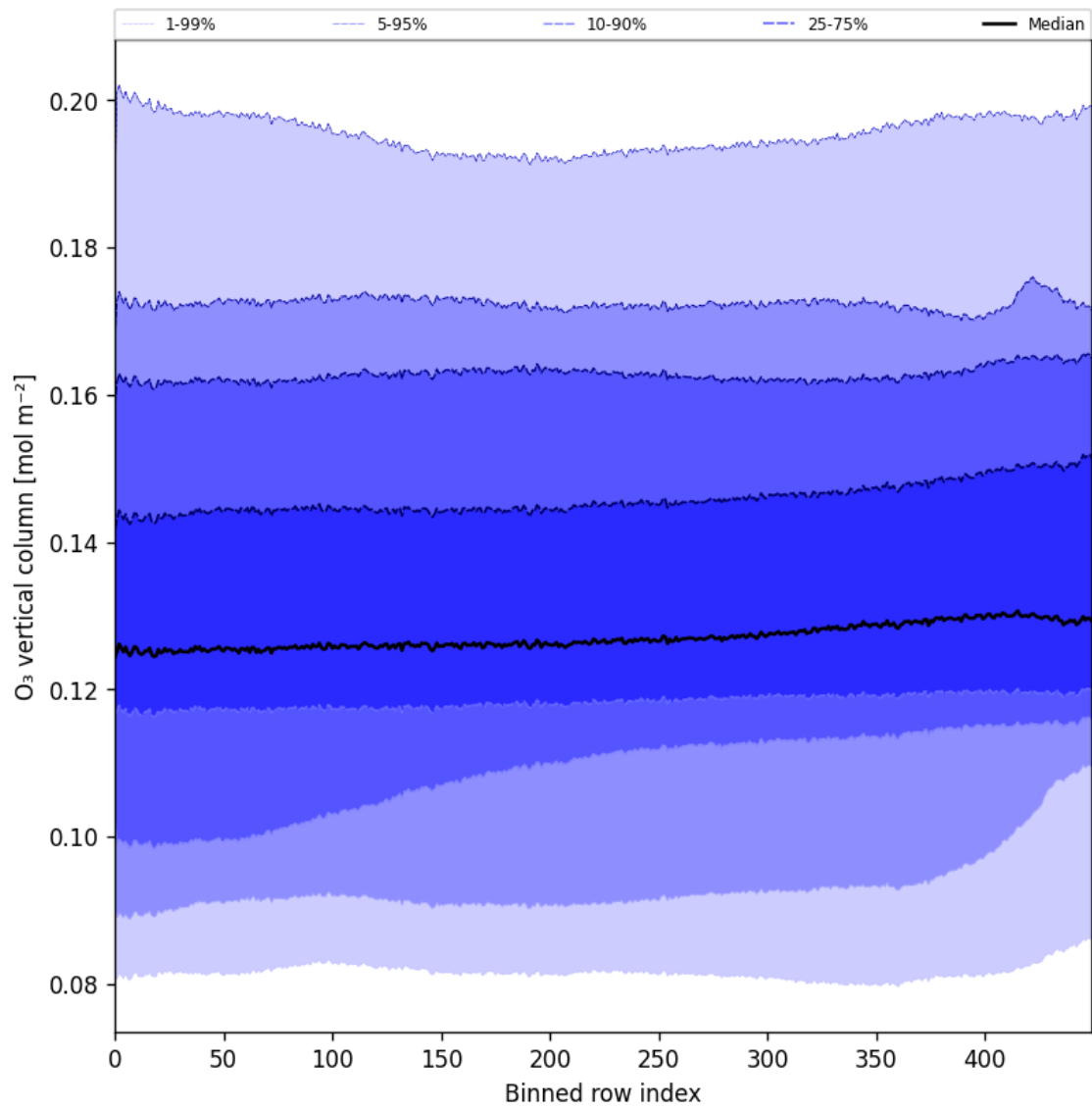
Figure 28: Along track statistics of “O 3 vertical column” for 2024-11-15 to 2024-11-17
