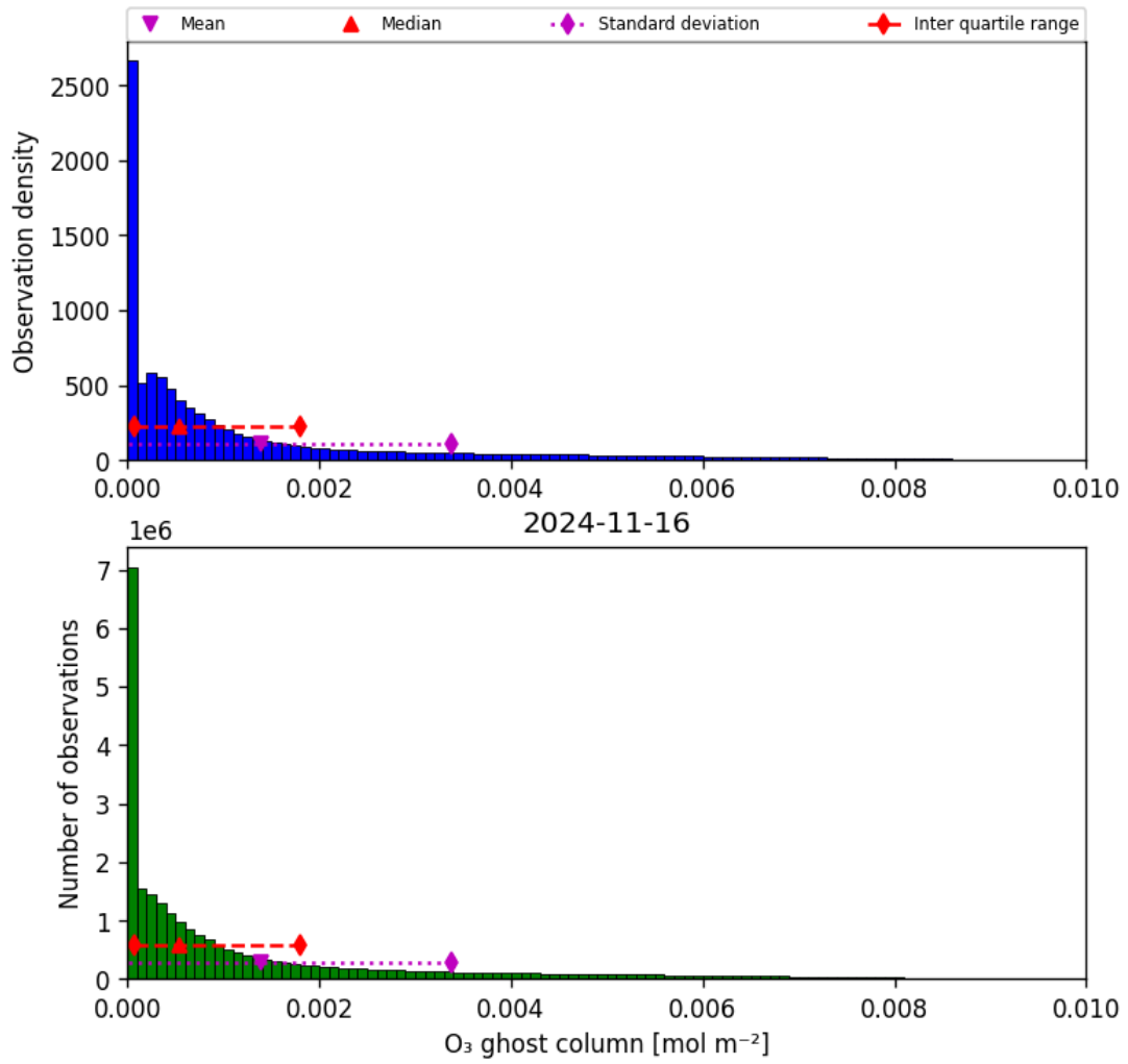
Figure 25: Histogram of “O 3 ghost column” for 2024-11-15 to 2024-11-17
