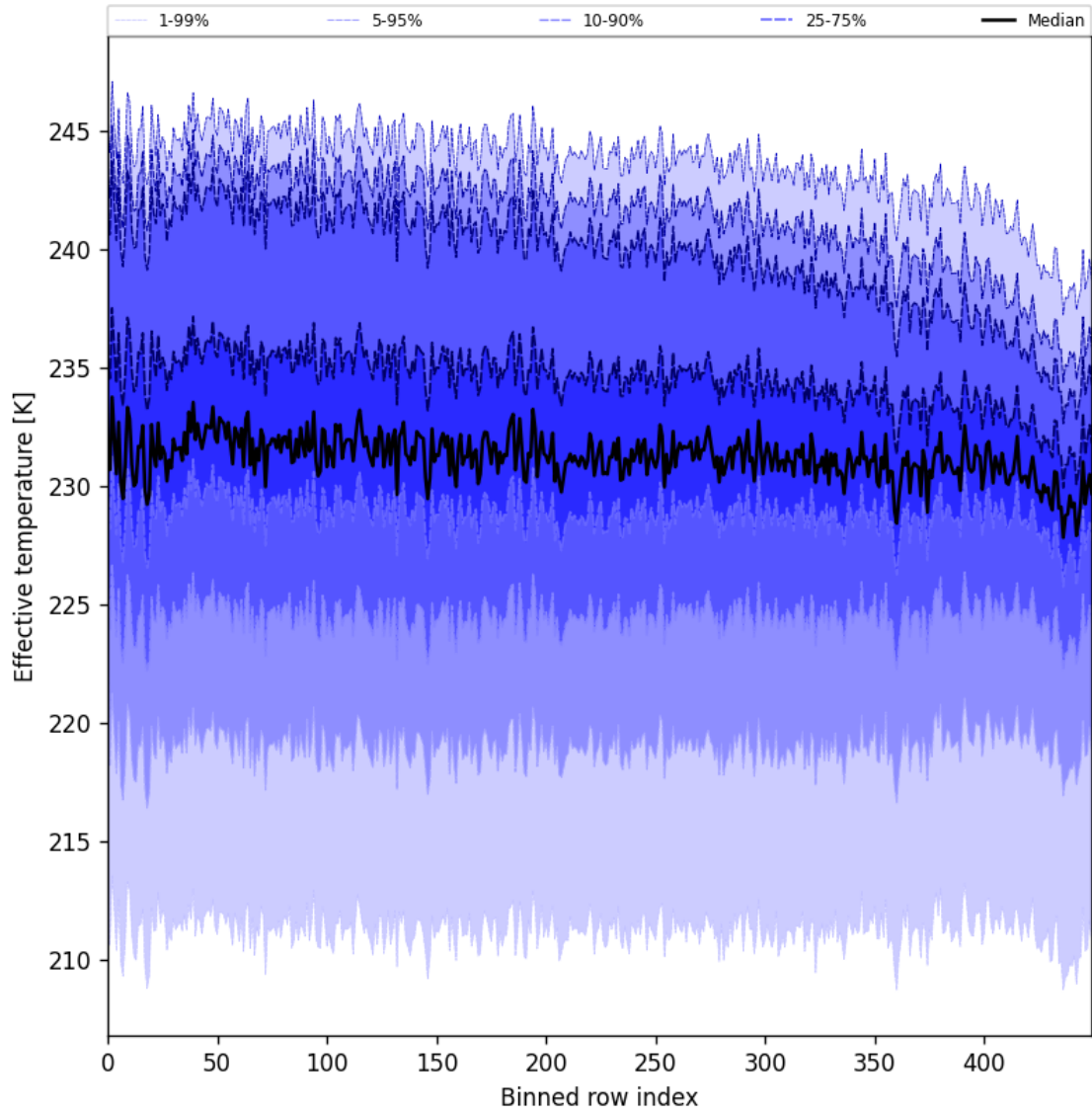
Figure 31: Along track statistics of “Effective temperature” for 2024-11-15 to 2024-11-17
