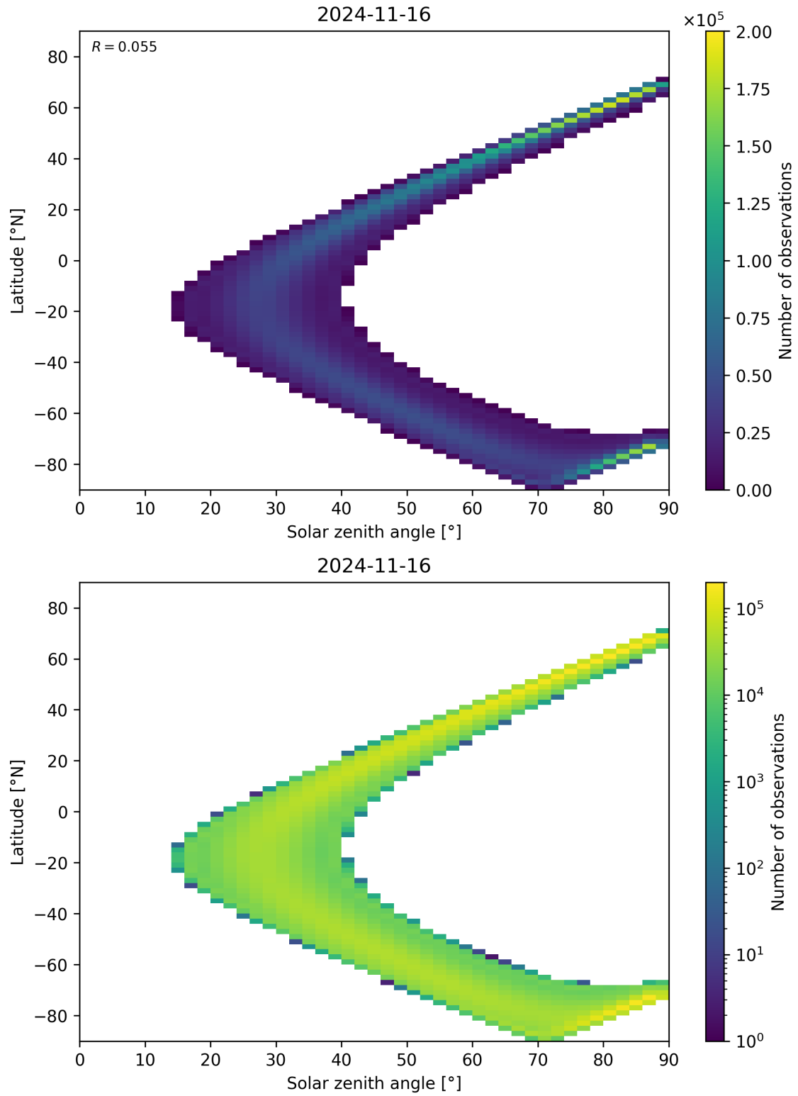
Figure 44: Scatter density plot of “Solar zenith angle” against “Latitude” for 2024-11-15 to 2024-11-17.
