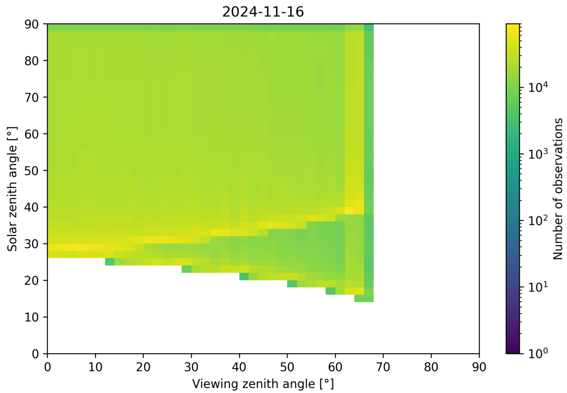
Figure 54: Scatter density plot of “Viewing zenith angle” against “Solar zenith angle” for 2024-11-15 to 2024-11-17.
