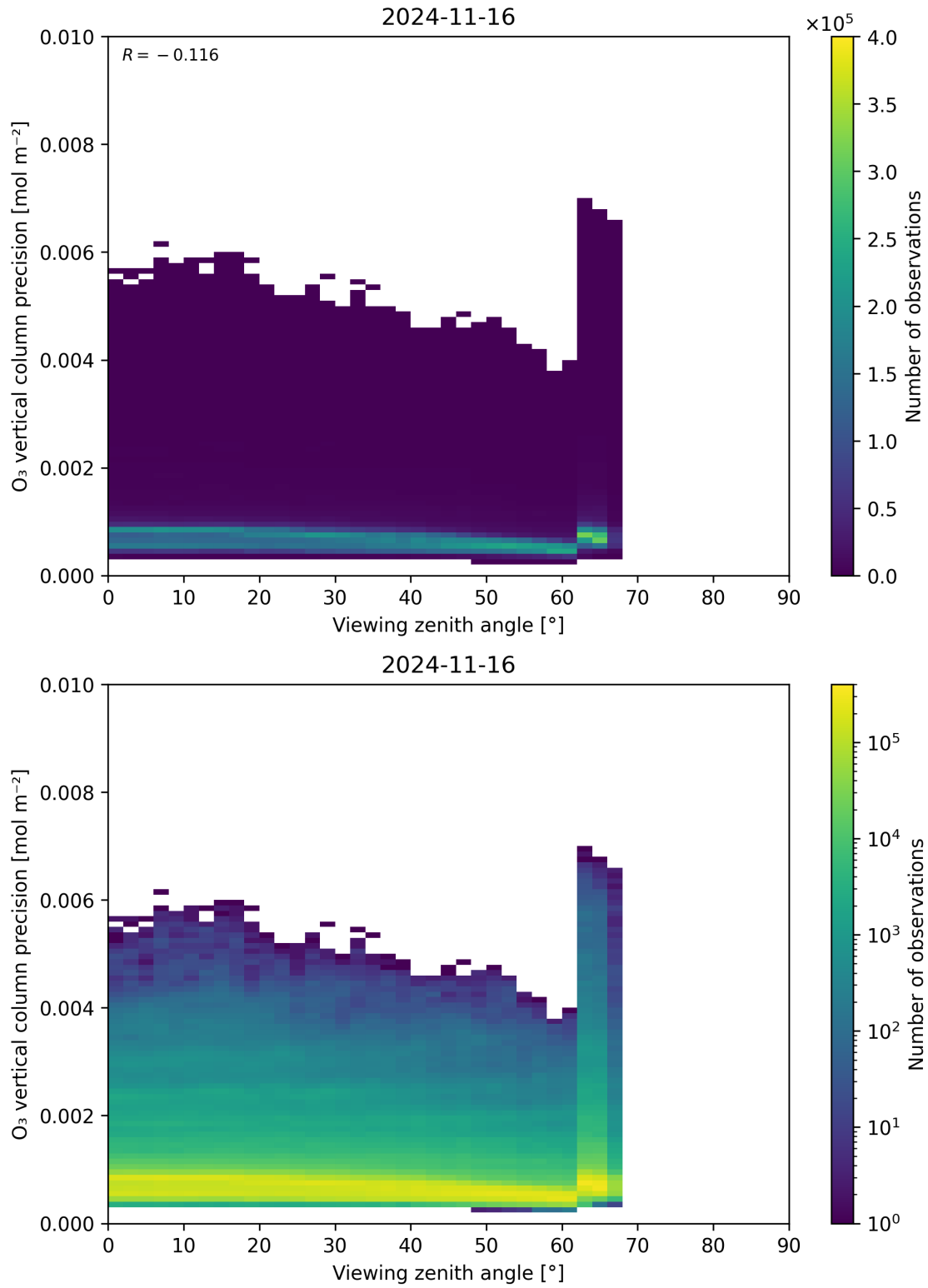
Figure 53: Scatter density plot of “Viewing zenith angle” against “O 3 vertical column precision” for 2024-11-15 to 2024-11-17.
