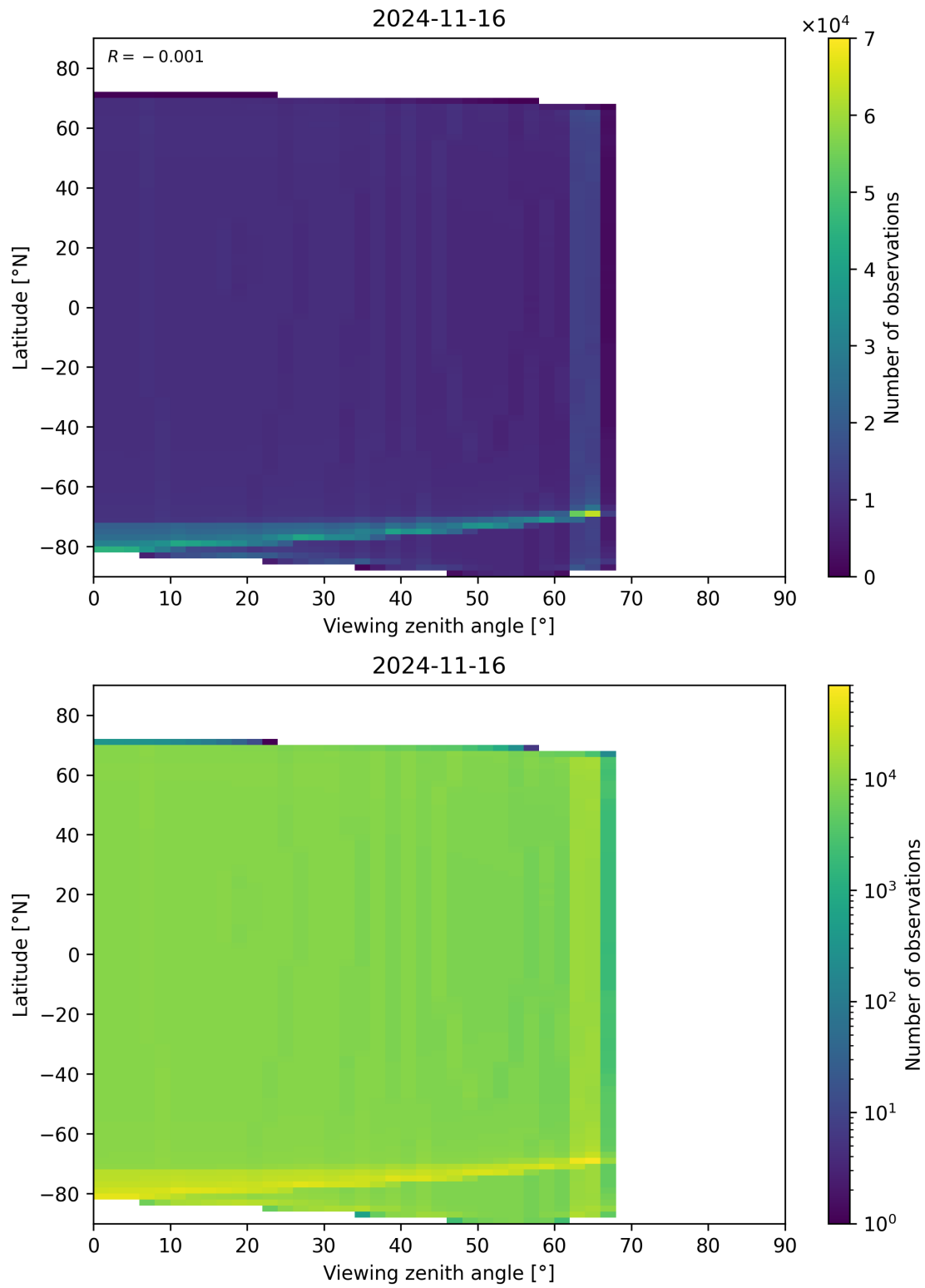
Figure 49: Scatter density plot of “Viewing zenith angle” against “Latitude” for 2024-11-15 to 2024-11-17.
