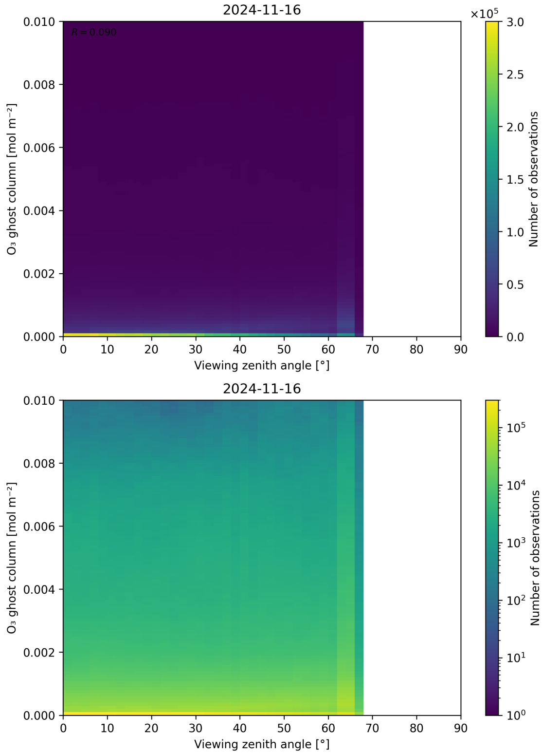
Figure 51: Scatter density plot of “Viewing zenith angle” against “O 3 ghost column” for 2024-11-15 to 2024-11-17.
