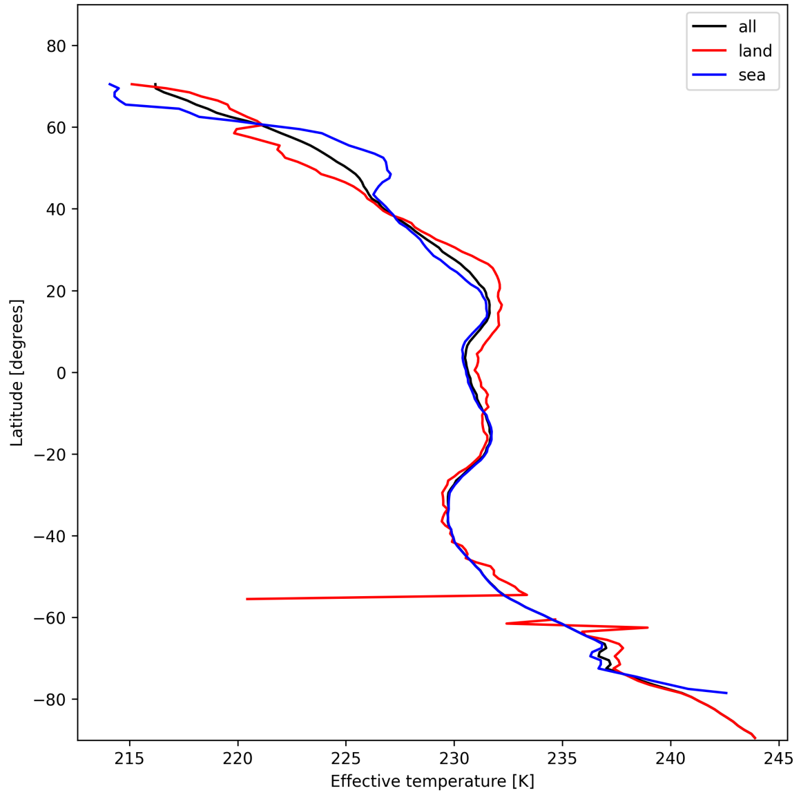
Figure 17: Zonal average of “Effective temperature” for 2024-11-15 to 2024-11-17.
