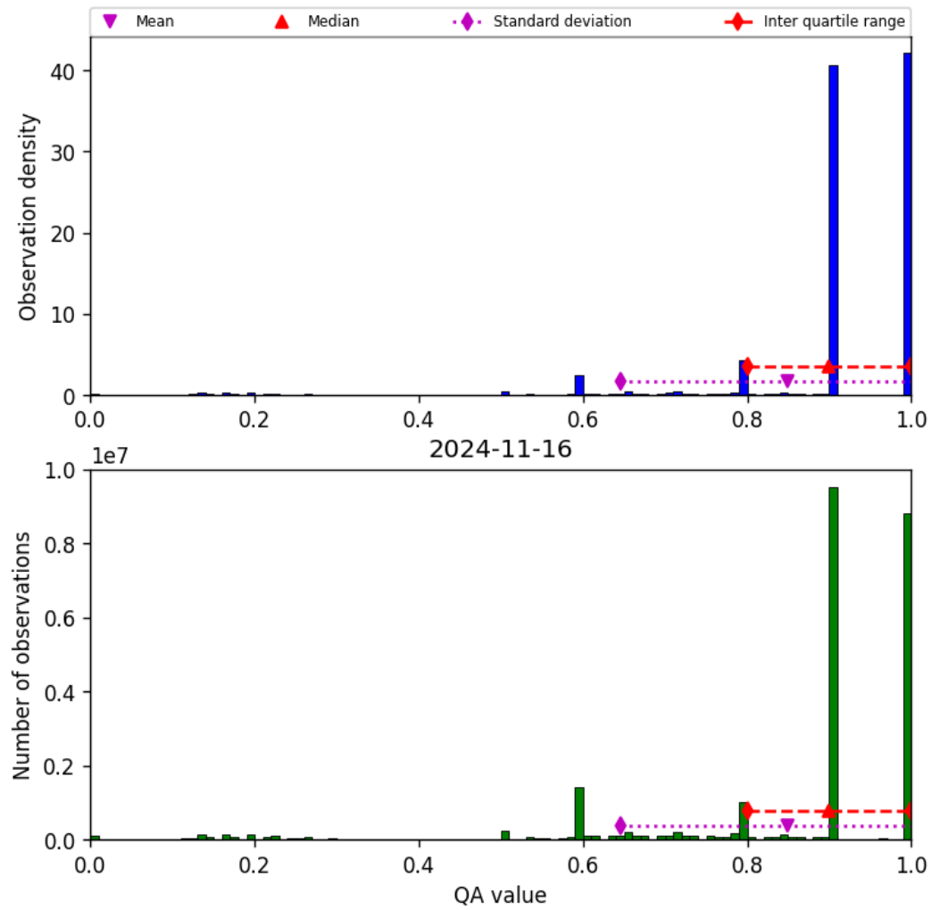
Figure 20: Histogram of “QA value” for 2024-11-15 to 2024-11-17
