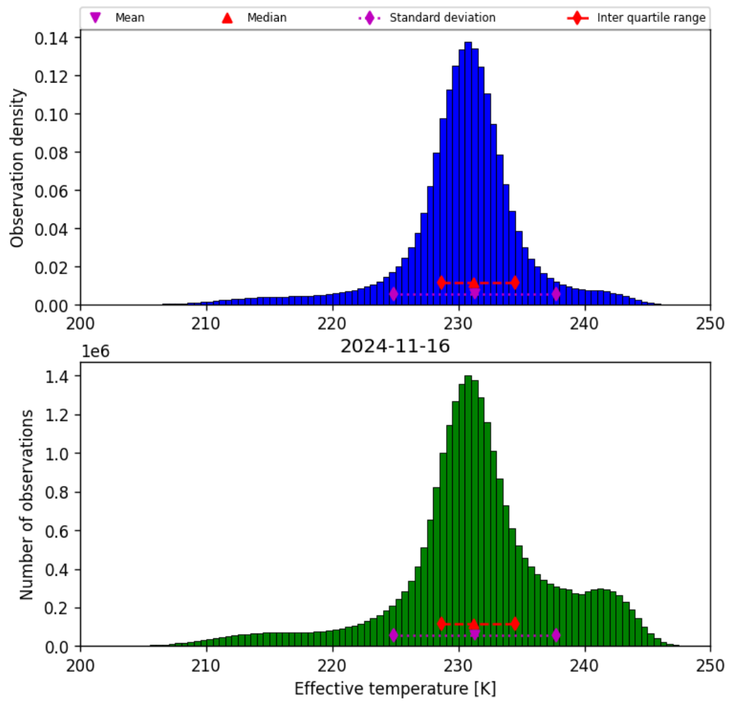
Figure 24: Histogram of “Effective temperature” for 2024-11-15 to 2024-11-17
