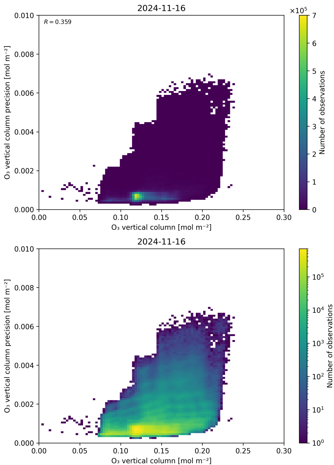
Figure 41: Scatter density plot of “O 3 vertical column” against “O 3 vertical column precision” for 2024-11-15 to 2024-11-17.
