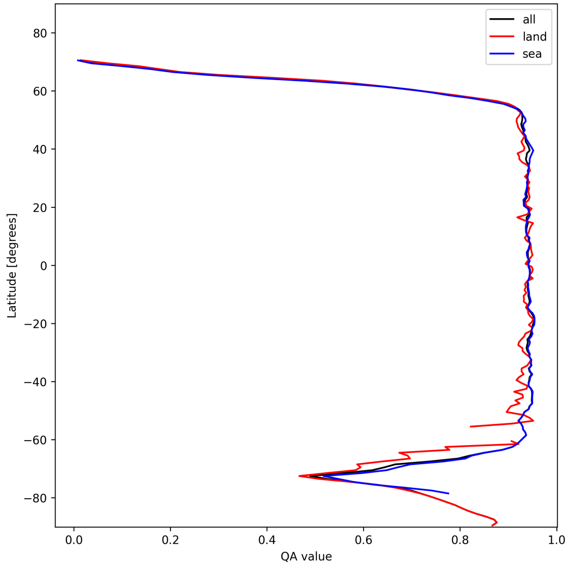
Figure 13: Zonal average of “QA value” for 2024-11-15 to 2024-11-17.
