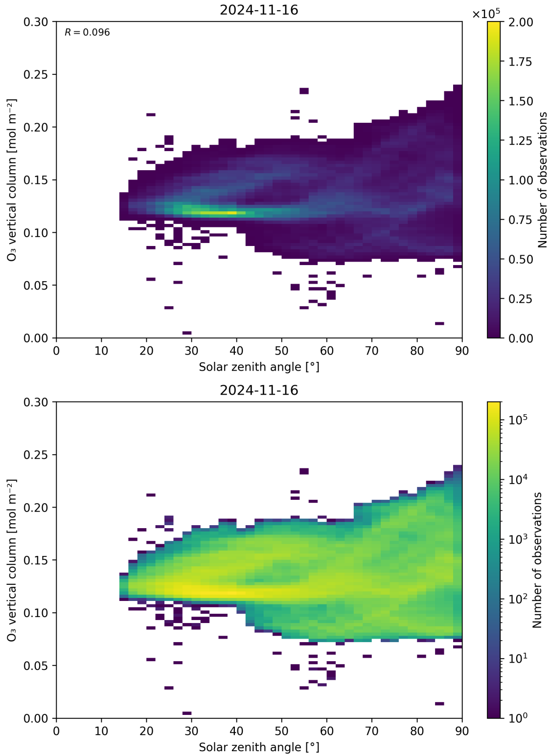
Figure 47: Scatter density plot of “Solar zenith angle” against “O 3 vertical column” for 2024-11-15 to 2024-11-17.
