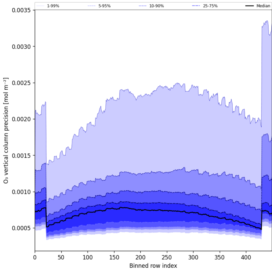
Figure 29: Along track statistics of “O 3 vertical column precision” for 2024-11-15 to 2024-11-17
