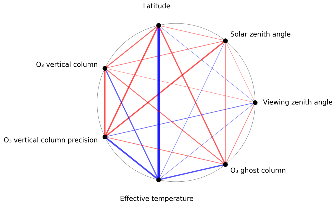
Figure 1: Map of correlation graph for 2024-11-15 to 2024-11-17.
