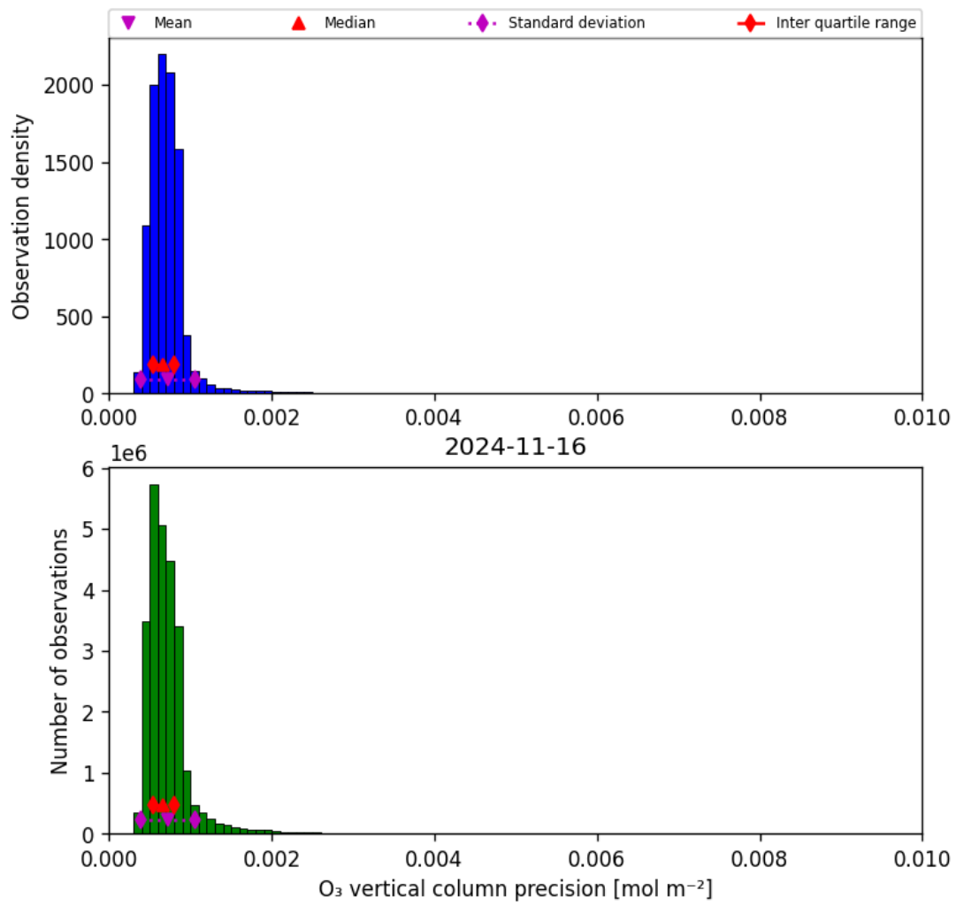
Figure 22: Histogram of “O 3 vertical column precision” for 2024-11-15 to 2024-11-17
