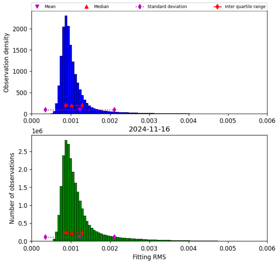
Figure 23: Histogram of “Fitting RMS” for 2024-11-15 to 2024-11-17
