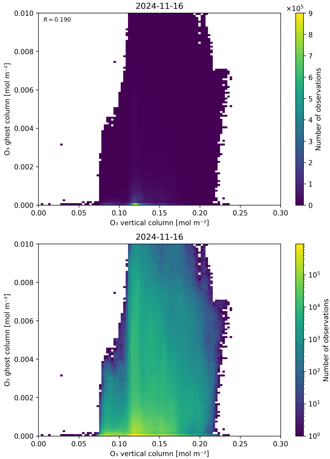
Figure 40: Scatter density plot of “O 3 vertical column” against “O 3 ghost column” for 2024-11-15 to 2024-11-17.
