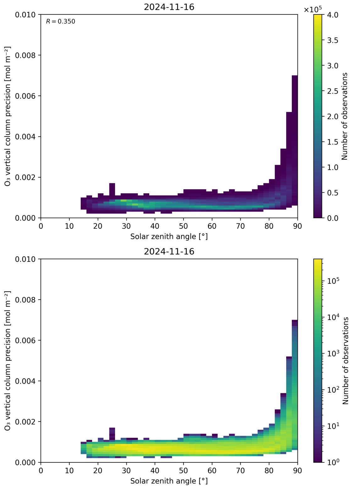
Figure 48: Scatter density plot of “Solar zenith angle” against “O 3 vertical column precision” for 2024-11-15 to 2024-11-17.
