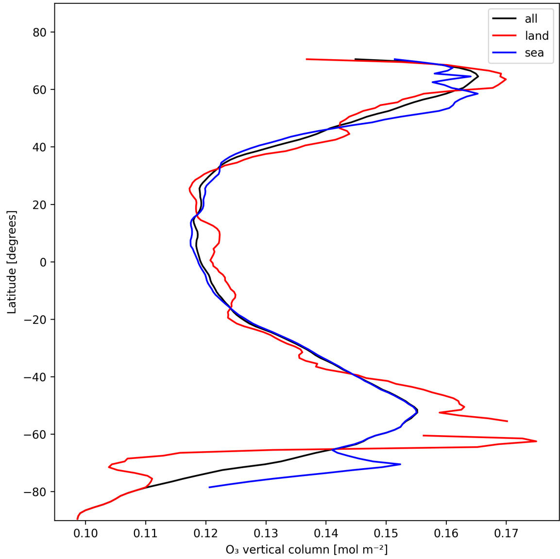
Figure 14: Zonal average of “O 3 vertical column” for 2024-11-15 to 2024-11-17.
