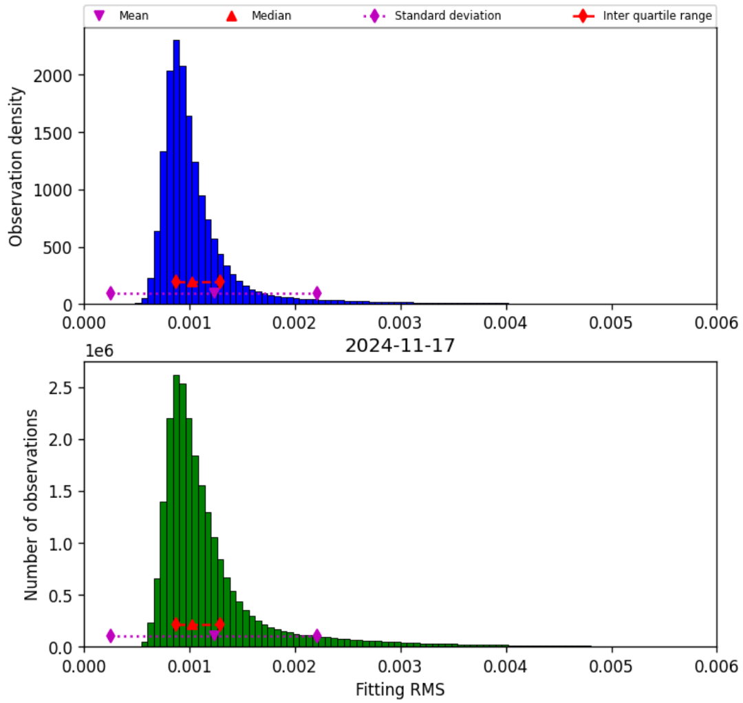
Figure 23: Histogram of “Fitting RMS” for 2024-11-17 to 2024-11-18
