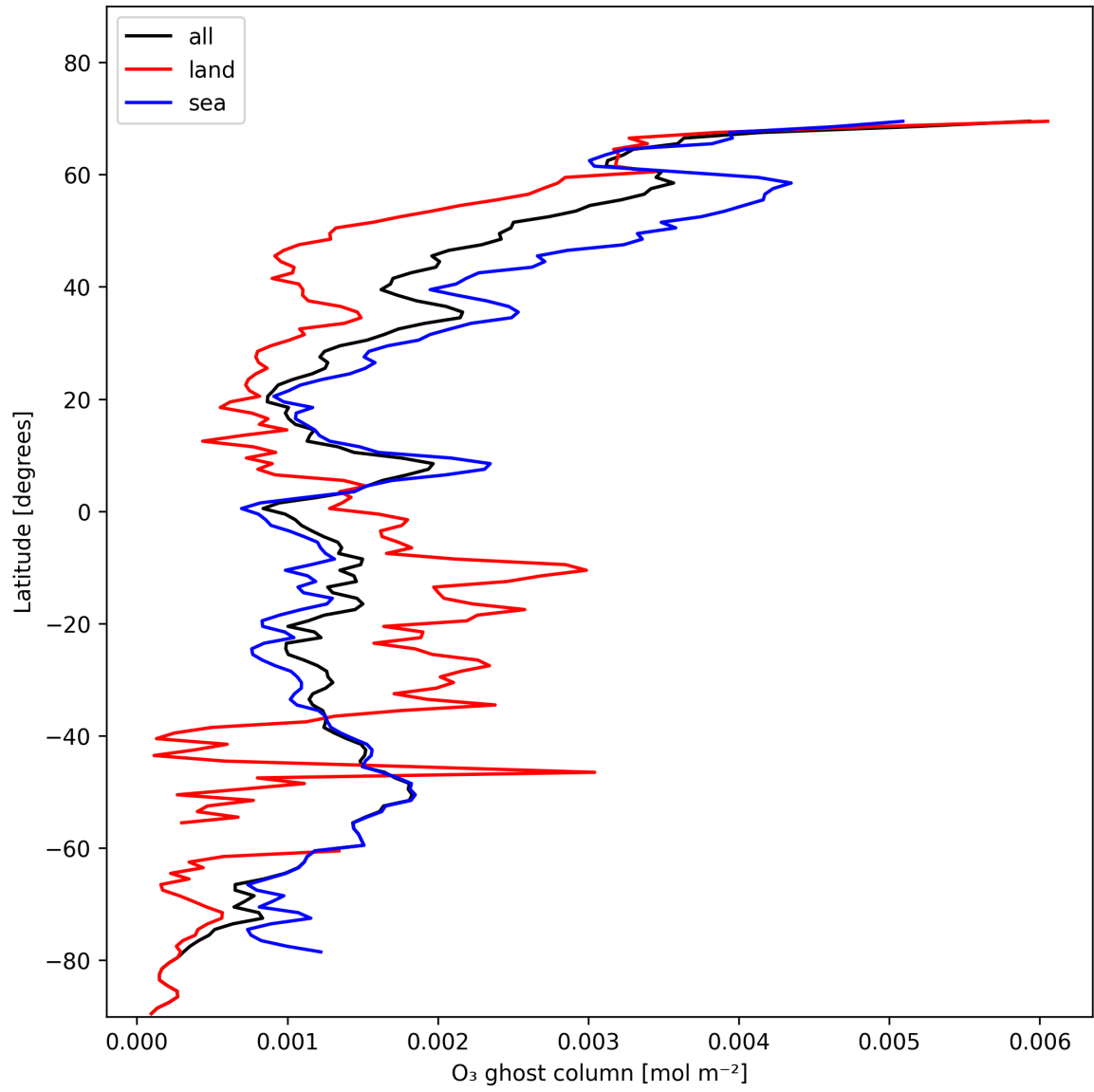
Figure 18: Zonal average of "O 3 ghost column" for 2024-11-17 to 2024-11-18.
