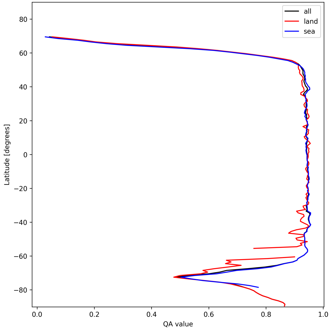
Figure 13: Zonal average of “QA value” for 2024-11-17 to 2024-11-18.
