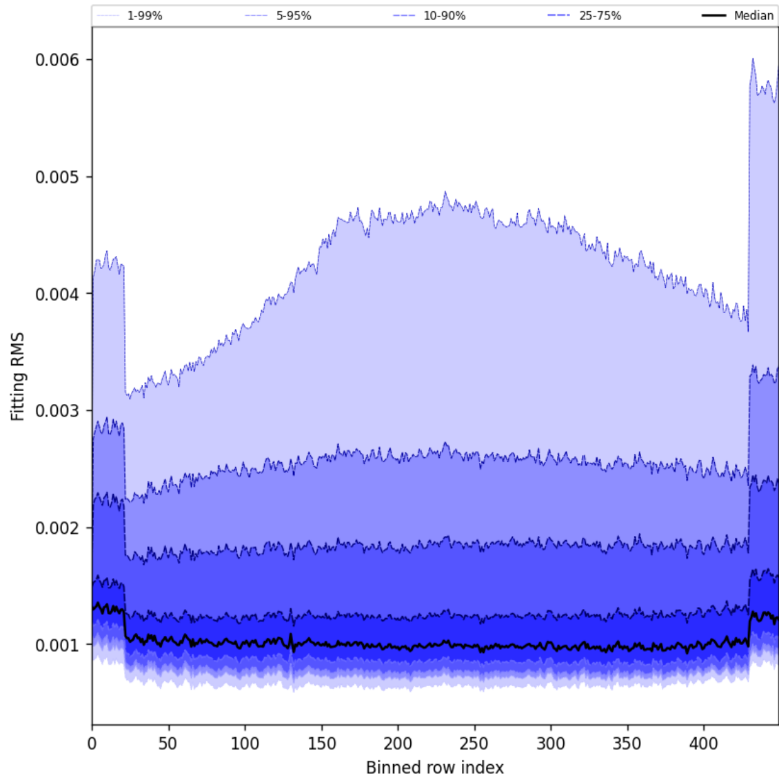
Figure 30: Along track statistics of “Fitting RMS” for 2024-11-17 to 2024-11-18
