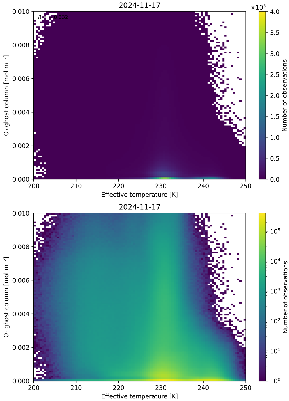
Figure 38: Scatter density plot of “Effective temperature” against “O 3 ghost column” for 2024-11-17 to 2024-11-18.
