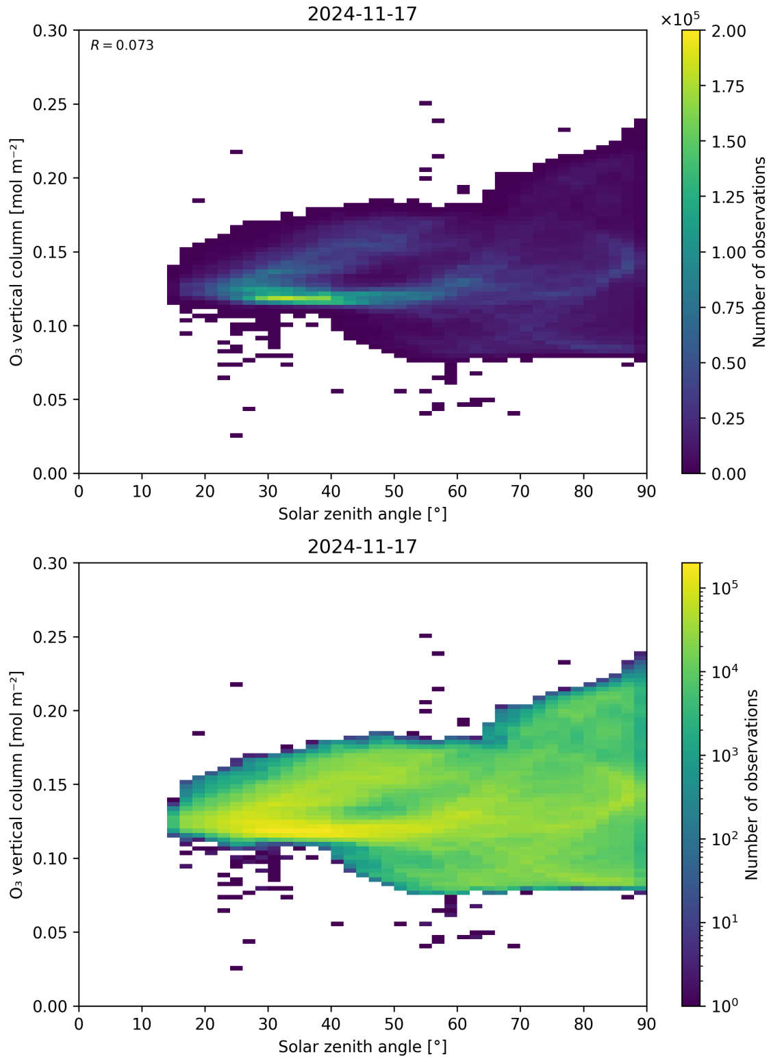
Figure 47: Scatter density plot of “Solar zenith angle” against “O 3 vertical column” for 2024-11-17 to 2024-11-18.
