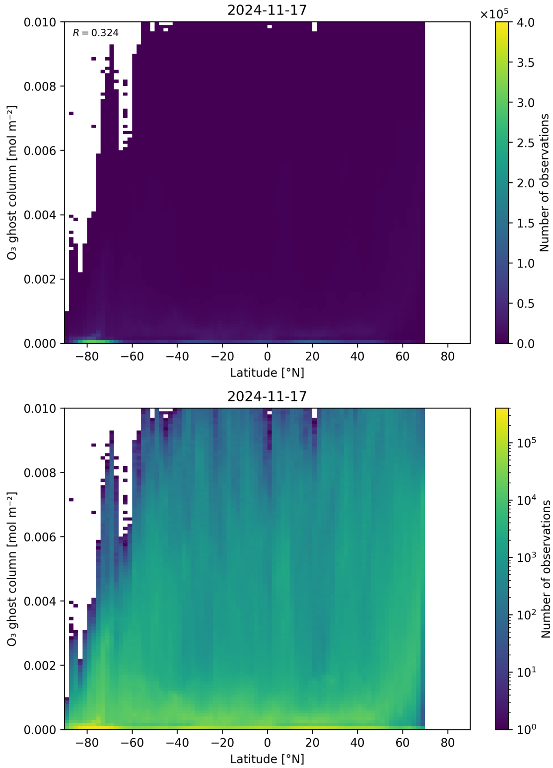
Figure 35: Scatter density plot of “Latitude” against “O 3 ghost column” for 2024-11-17 to 2024-11-18.
