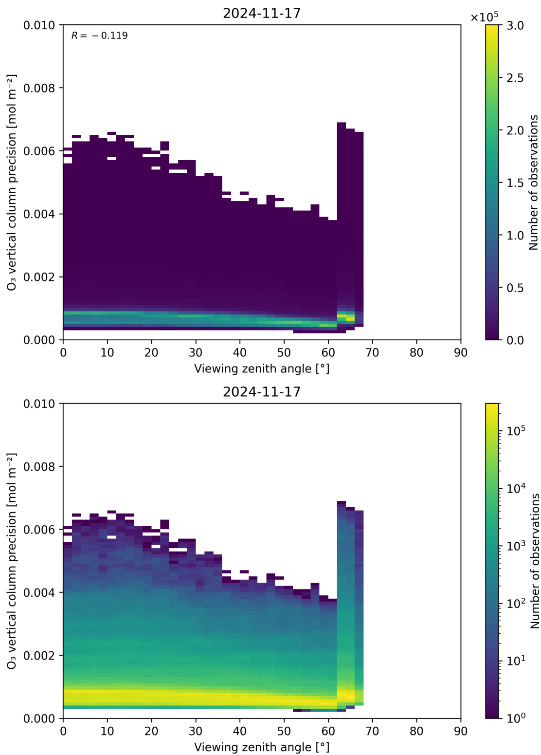
Figure 53: Scatter density plot of “Viewing zenith angle” against “O 3 vertical column precision” for 2024-11-17 to 2024-11-18.
