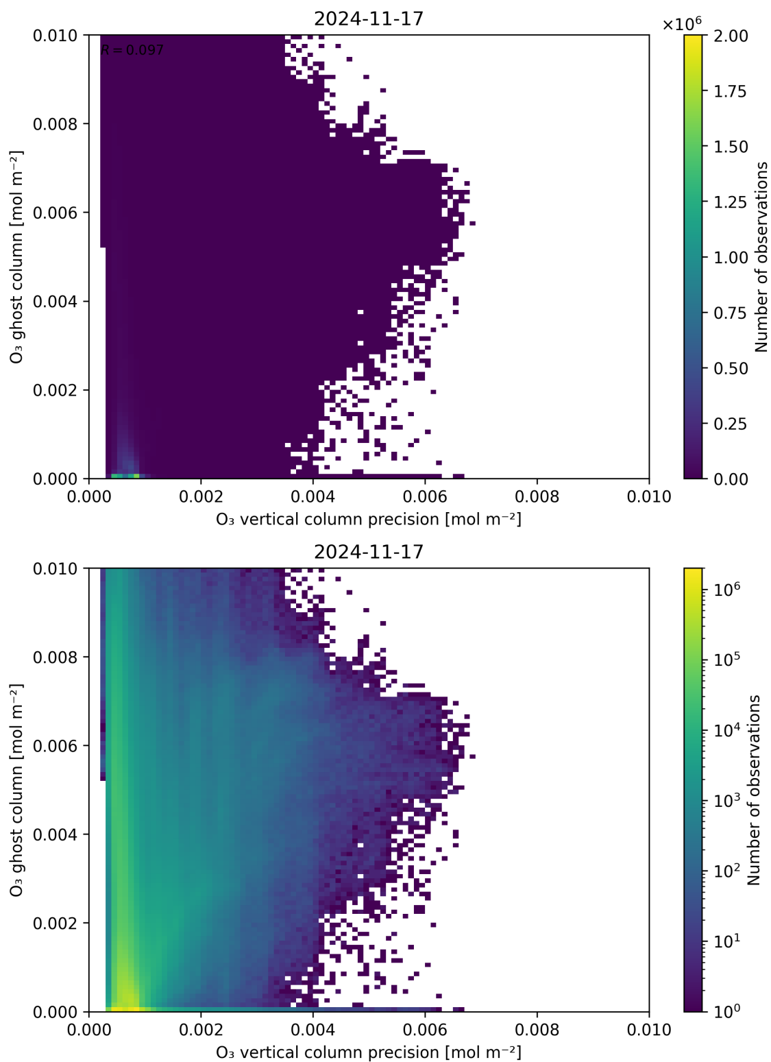
Figure 43: Scatter density plot of “O 3 vertical column precision” against “O 3 ghost column” for 2024-11-17 to 2024-11-18.
