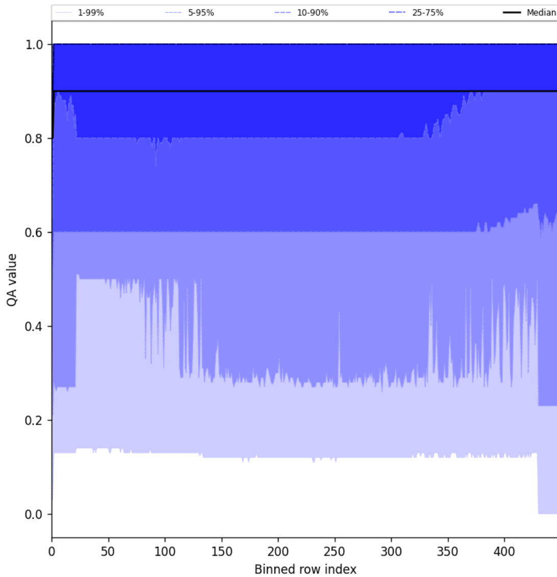
Figure 27: Along track statistics of “QA value” for 2024-11-17 to 2024-11-18
