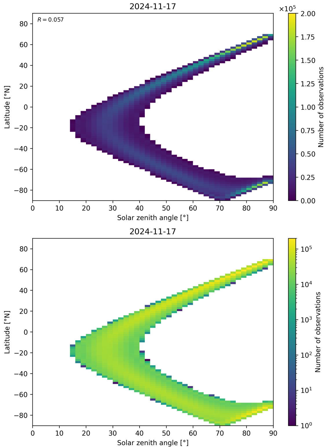
Figure 44: Scatter density plot of “Solar zenith angle” against “Latitude” for 2024-11-17 to 2024-11-18.
