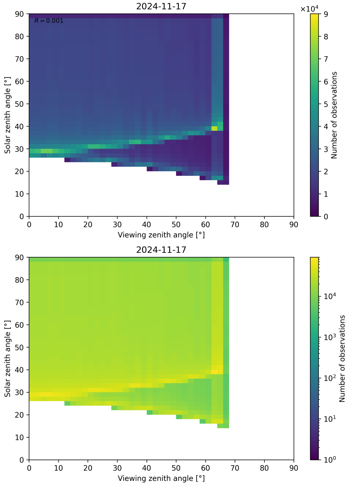
Figure 54: Scatter density plot of “Viewing zenith angle” against “Solar zenith angle” for 2024-11-17 to 2024-11-18.
