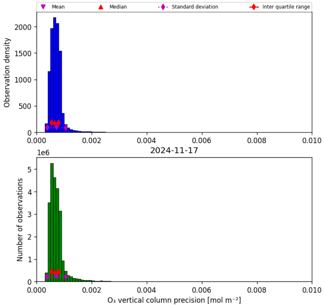
Figure 22: Histogram of “O 3 vertical column precision” for 2024-11-17 to 2024-11-18
