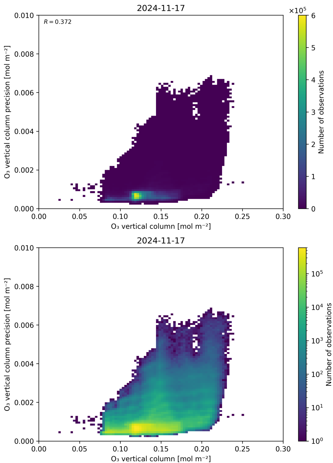
Figure 41: Scatter density plot of “O 3 vertical column” against “O 3 vertical column precision” for 2024-11-17 to 2024-11-18.
