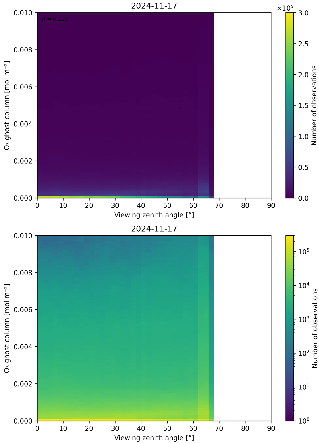
Figure 51: Scatter density plot of “Viewing zenith angle” against “O 3 ghost column” for 2024-11-17 to 2024-11-18.
