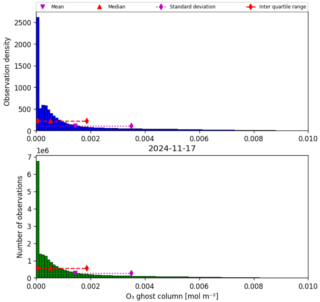
Figure 25: Histogram of “O 3 ghost column” for 2024-11-17 to 2024-11-18
