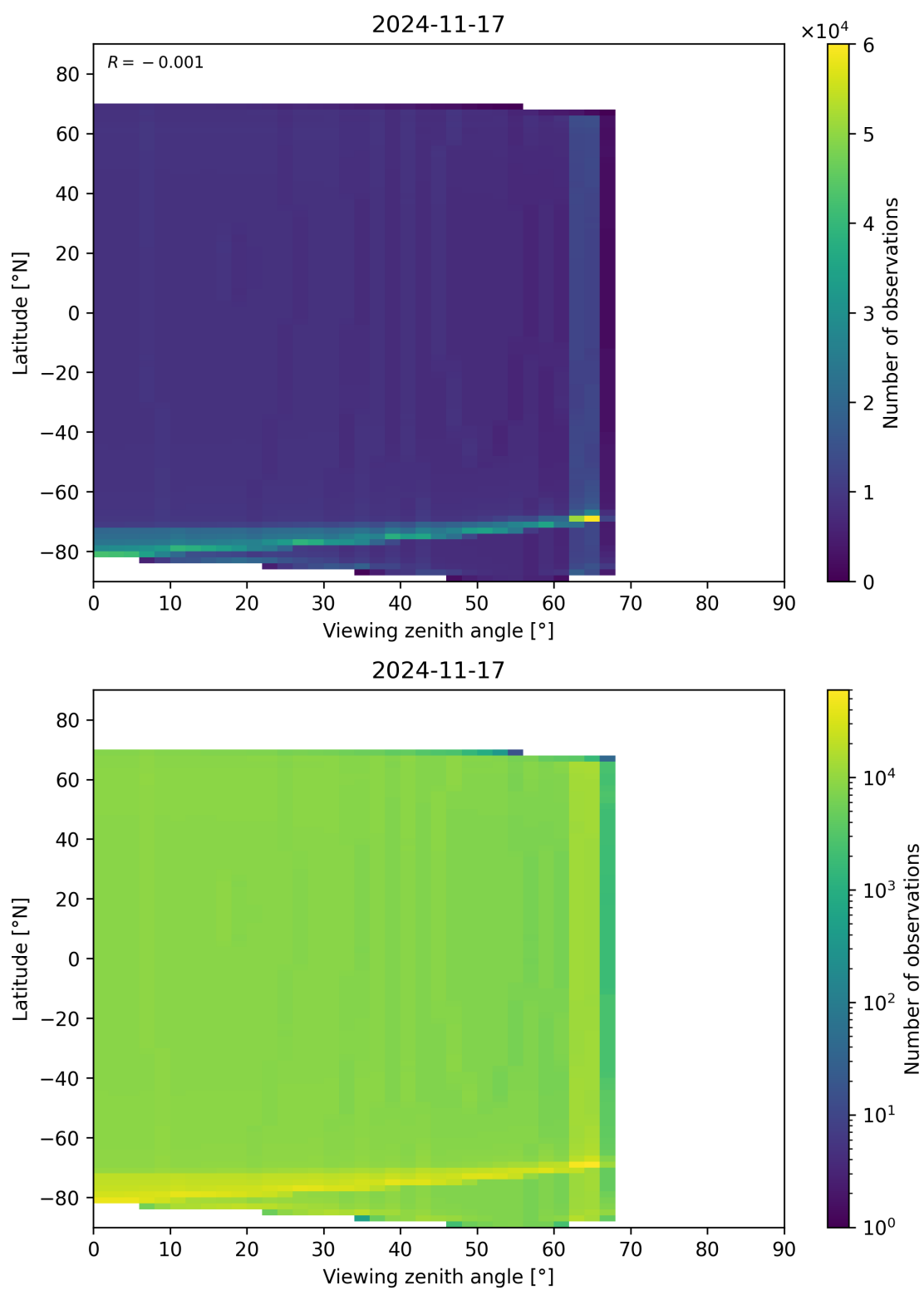
Figure 49: Scatter density plot of “Viewing zenith angle” against “Latitude” for 2024-11-17 to 2024-11-18.
