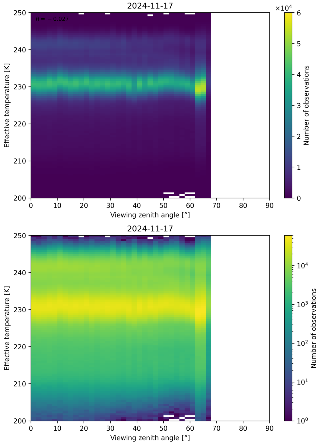
Figure 50: Scatter density plot of “Viewing zenith angle” against “Effective temperature” for 2024-11-17 to 2024-11-18.
