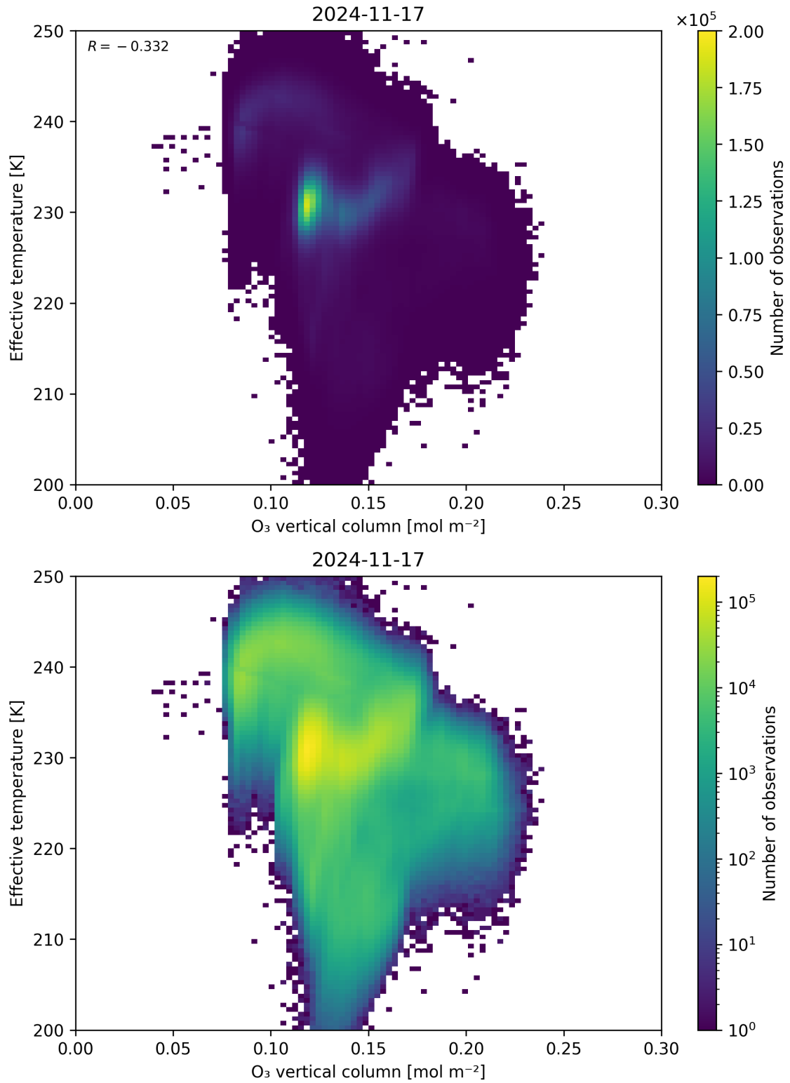
Figure 39: Scatter density plot of “O 3 vertical column” against “Effective temperature” for 2024-11-17 to 2024-11-18.
