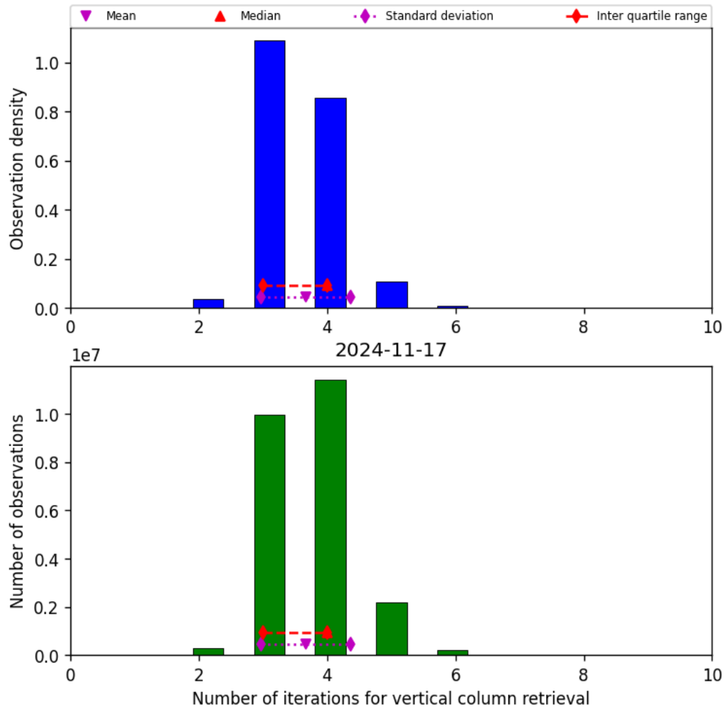
Figure 26: Histogram of “Number of iterations for vertical column retrieval” for 2024-11-17 to 2024-11-18
