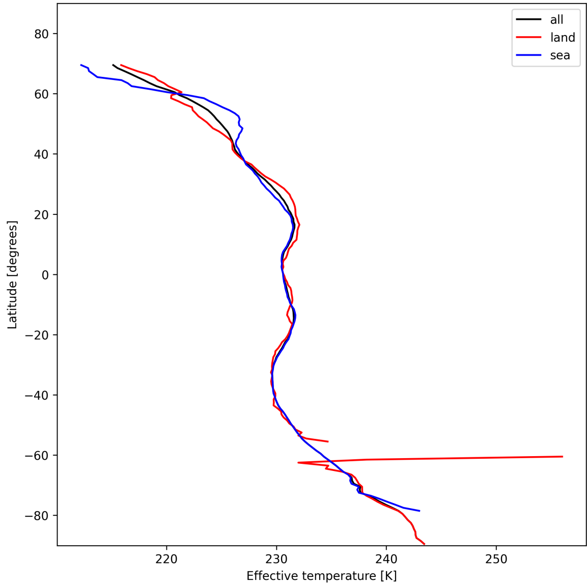
Figure 17: Zonal average of “Effective temperature” for 2024-11-17 to 2024-11-18.
