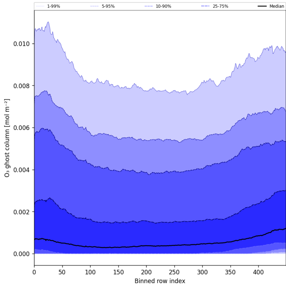
Figure 32: Along track statistics of “O 3 ghost column” for 2024-11-17 to 2024-11-18
