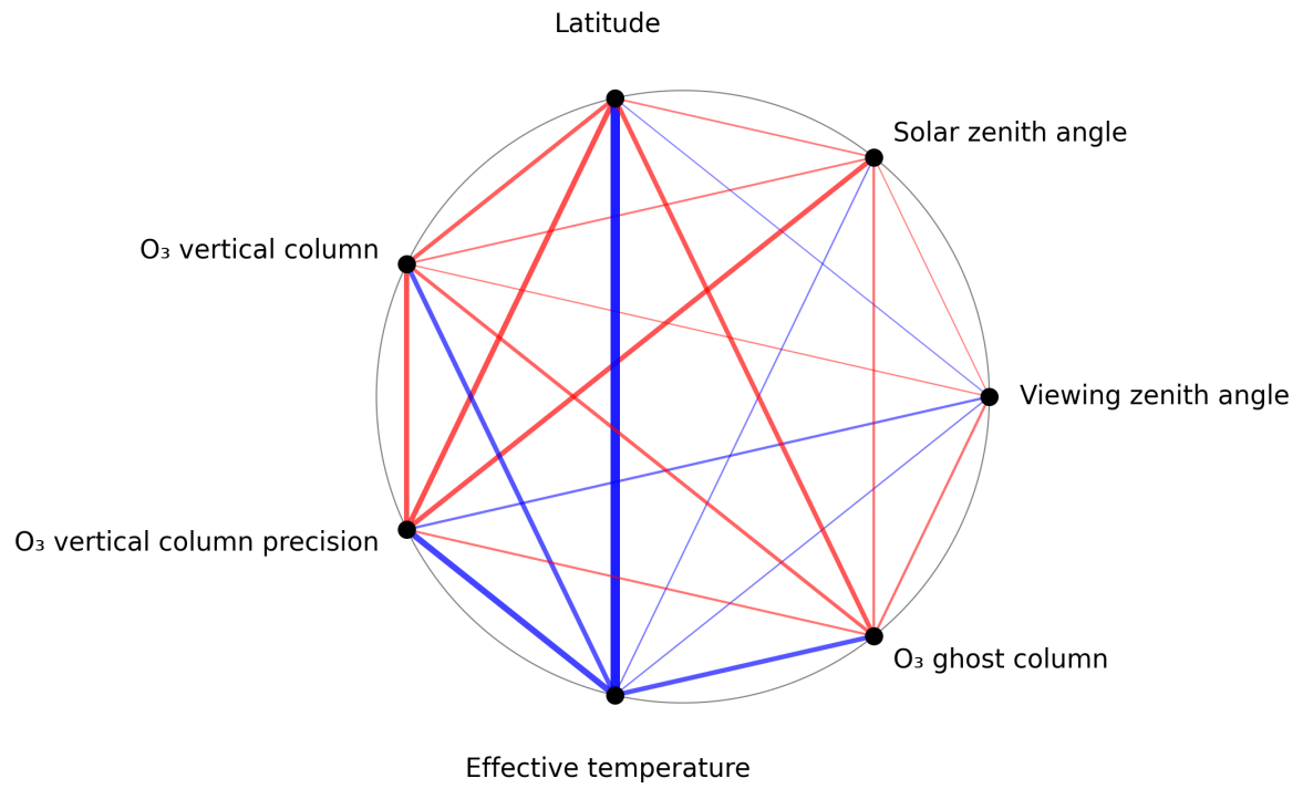
Figure 1: Map of correlation graph for 2024-11-17 to 2024-11-18.
