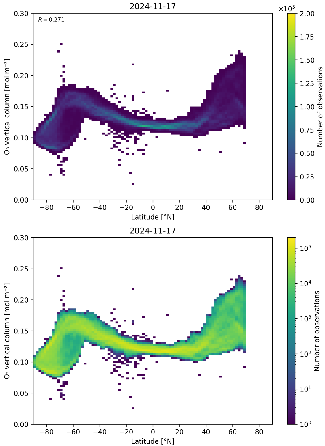
Figure 36: Scatter density plot of “Latitude” against “O 3 vertical column” for 2024-11-17 to 2024-11-18.
