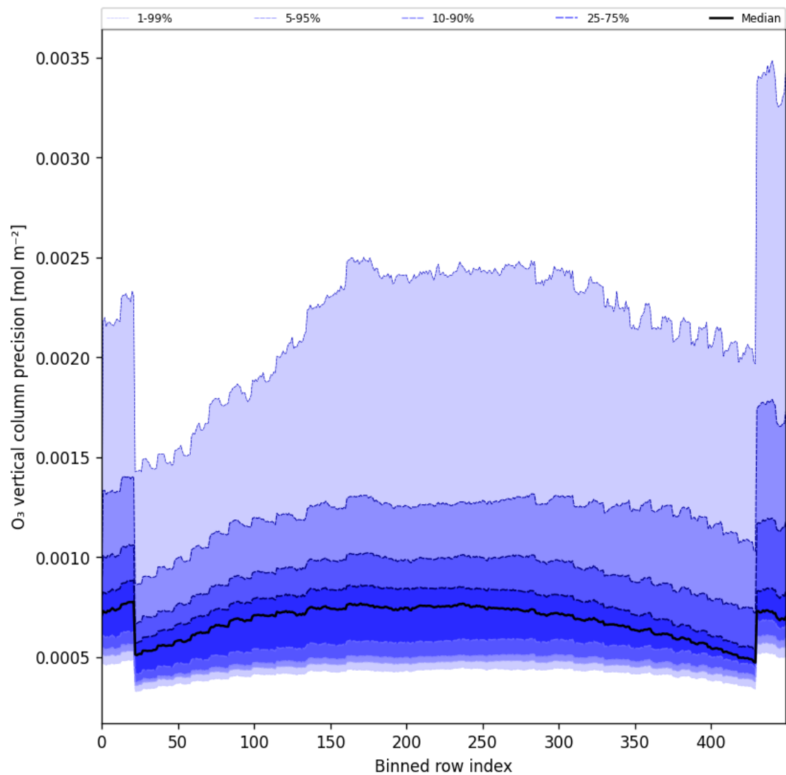
Figure 29: Along track statistics of “O 3 vertical column precision” for 2024-11-17 to 2024-11-18
