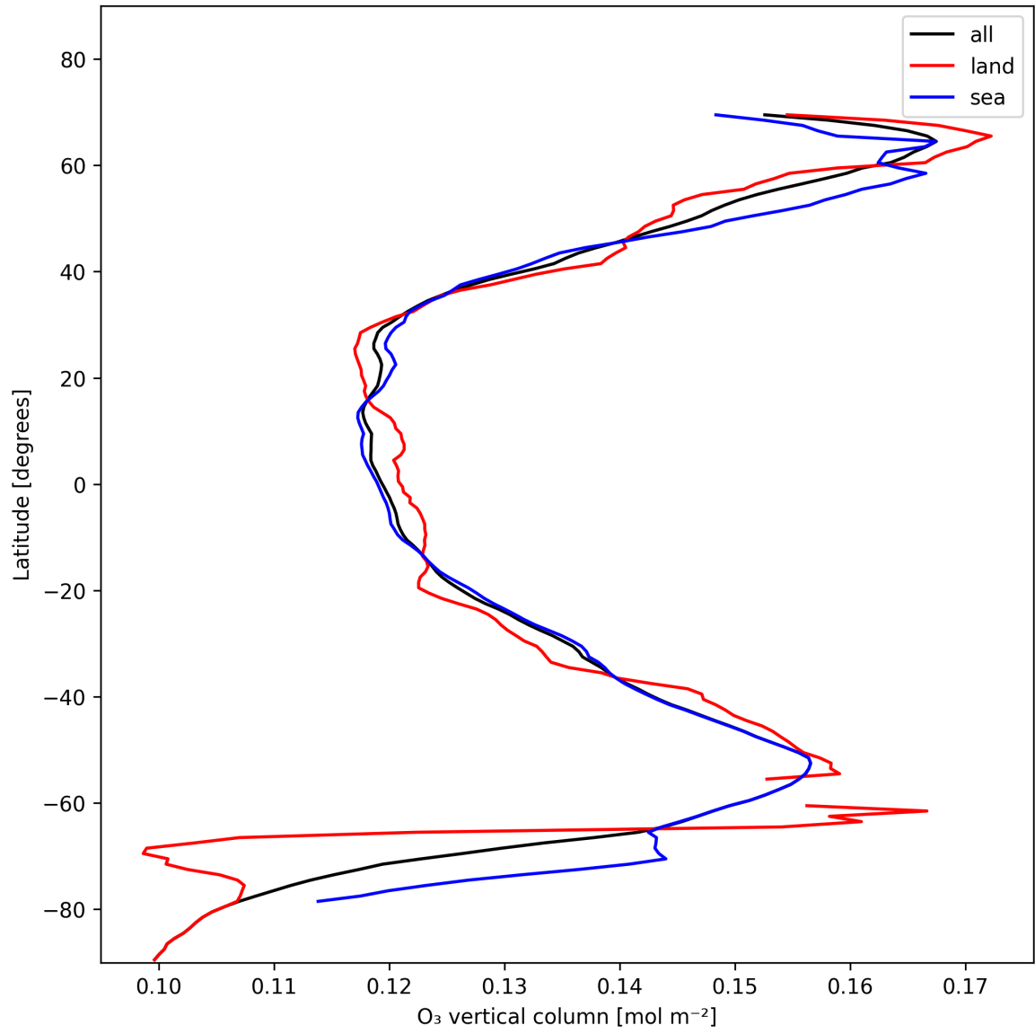
Figure 14: Zonal average of “O 3 vertical column” for 2024-11-17 to 2024-11-18.
