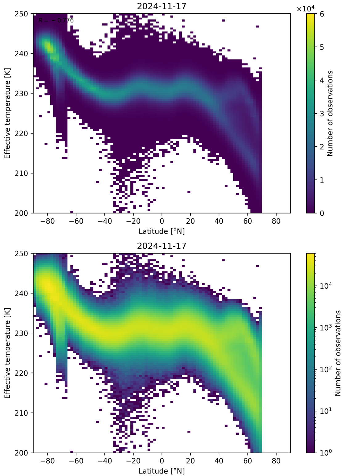
Figure 34: Scatter density plot of “Latitude” against “Effective temperature” for 2024-11-17 to 2024-11-18.
