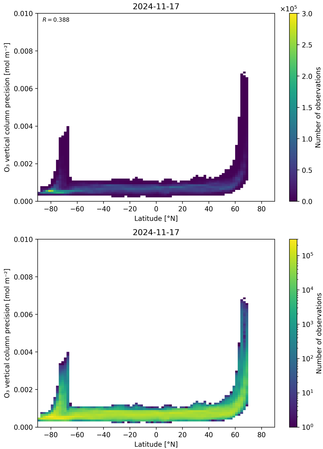
Figure 37: Scatter density plot of “Latitude” against “O 3 vertical column precision” for 2024-11-17 to 2024-11-18.
