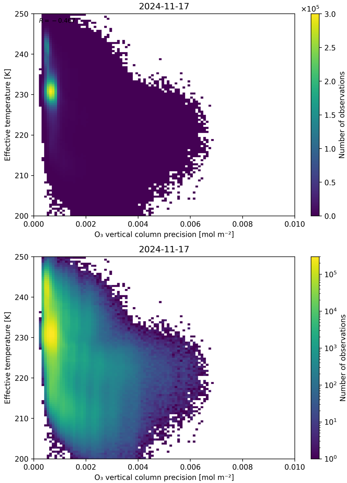
Figure 42: Scatter density plot of “O 3 vertical column precision” against “Effective temperature” for 2024-11-17 to 2024-11-18.
