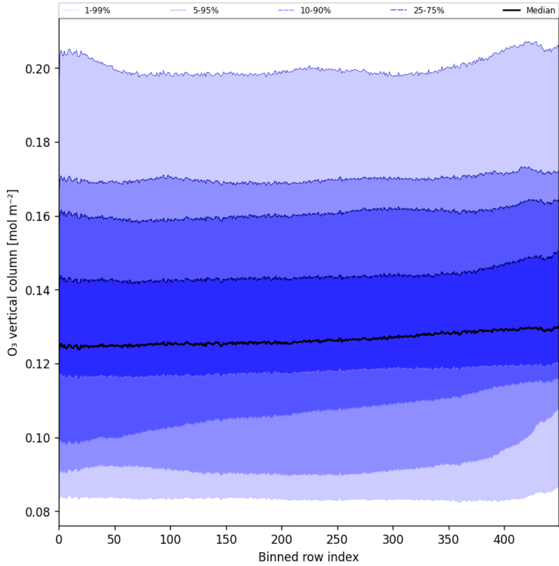
Figure 28: Along track statistics of “O 3 vertical column” for 2024-11-17 to 2024-11-18
