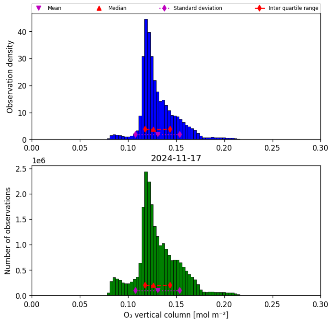
Figure 21: Histogram of “O 3 vertical column” for 2024-11-17 to 2024-11-18
