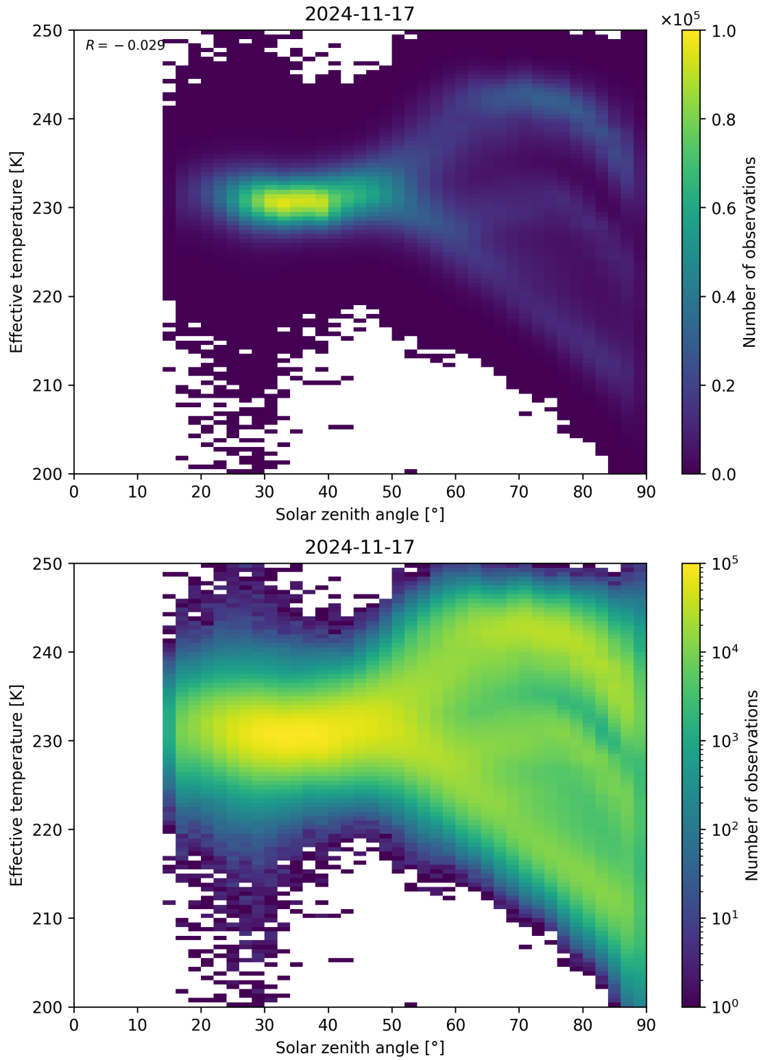
Figure 45: Scatter density plot of “Solar zenith angle” against “Effective temperature” for 2024-11-17 to 2024-11-18.
