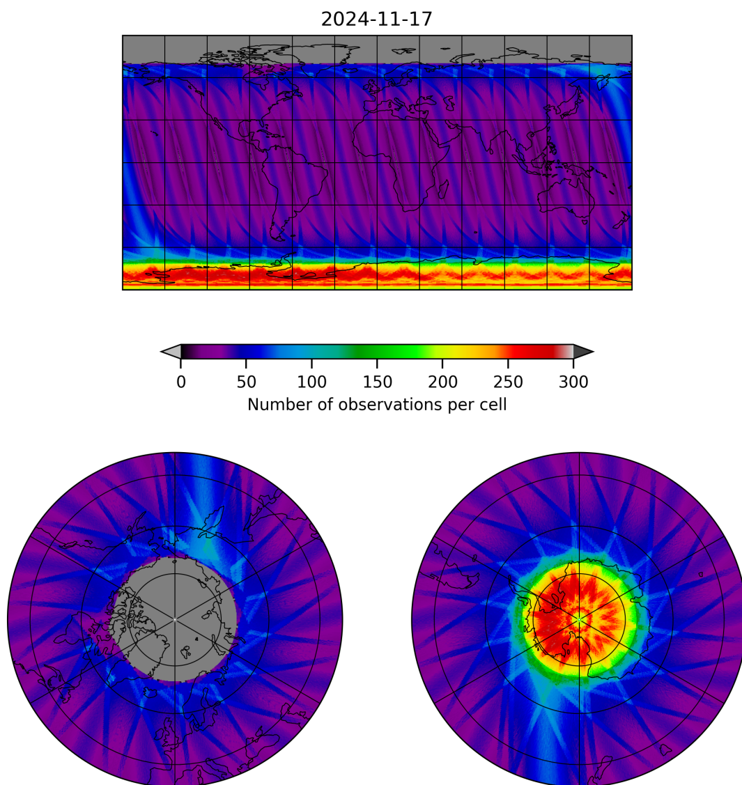
Figure 12: Map of the number of observations for 2024-11-17 to 2024-11-18
