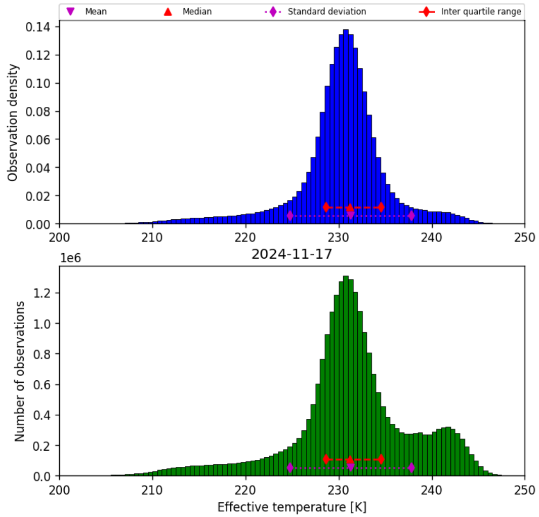
Figure 24: Histogram of “Effective temperature” for 2024-11-17 to 2024-11-18
