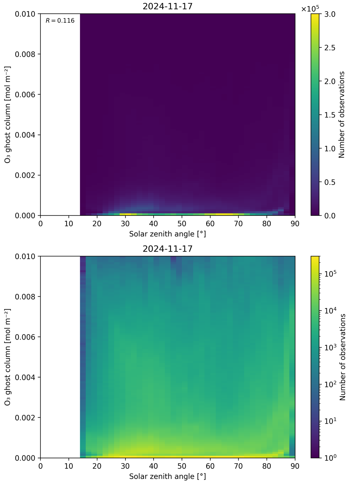
Figure 46: Scatter density plot of “Solar zenith angle” against “O 3 ghost column” for 2024-11-17 to 2024-11-18.
