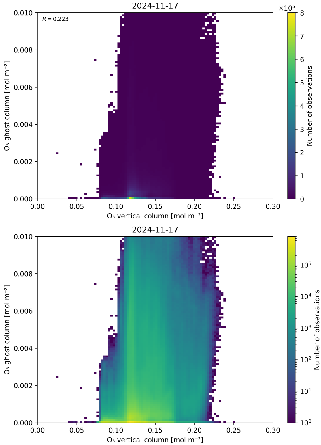
Figure 40: Scatter density plot of “O 3 vertical column” against “O 3 ghost column” for 2024-11-17 to 2024-11-18.
