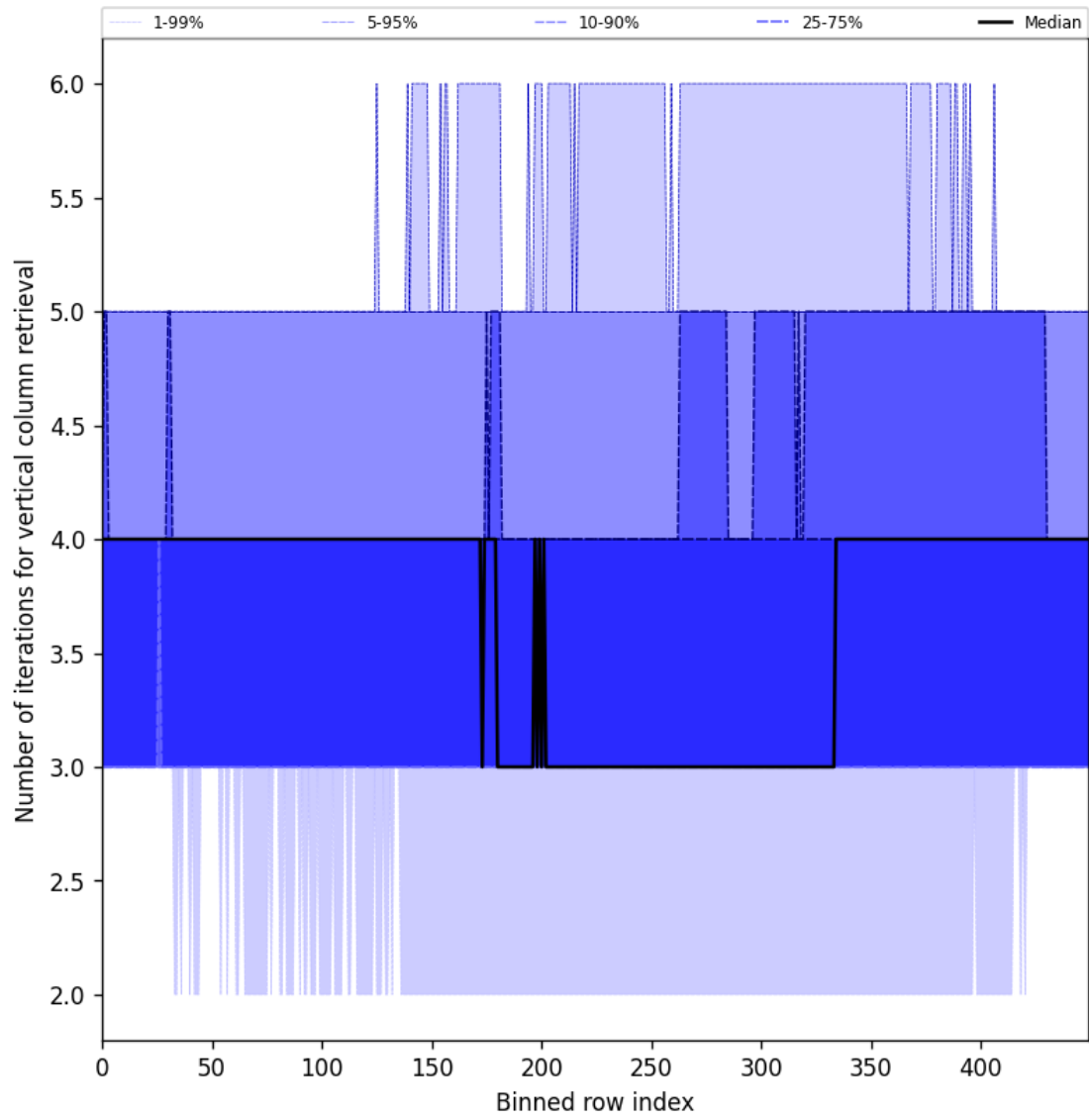
Figure 33: Along track statistics of “Number of iterations for vertical column retrieval” for 2024-11-17 to 2024-11-18
