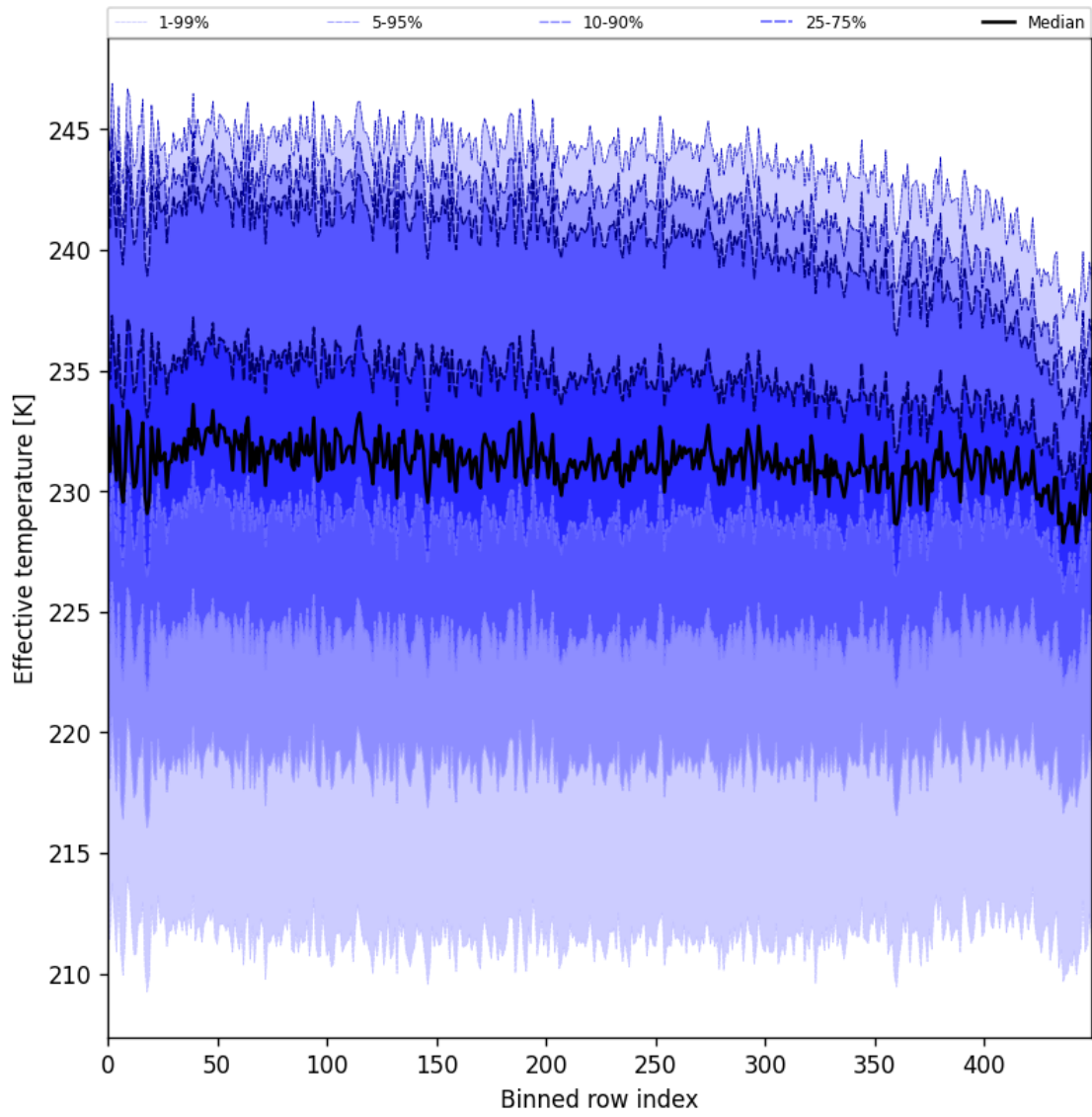
Figure 31: Along track statistics of “Effective temperature” for 2024-11-17 to 2024-11-18
