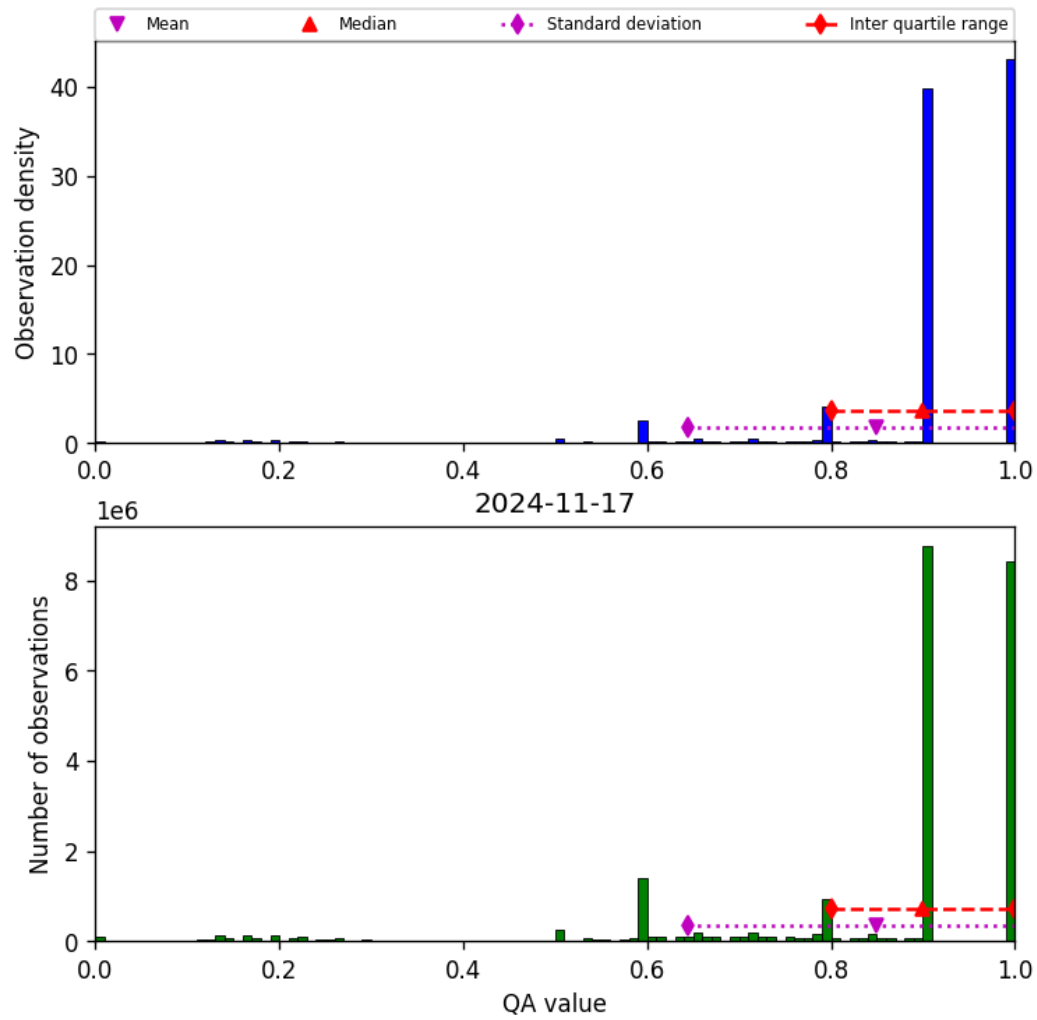
Figure 20: Histogram of “QA value” for 2024-11-17 to 2024-11-18
