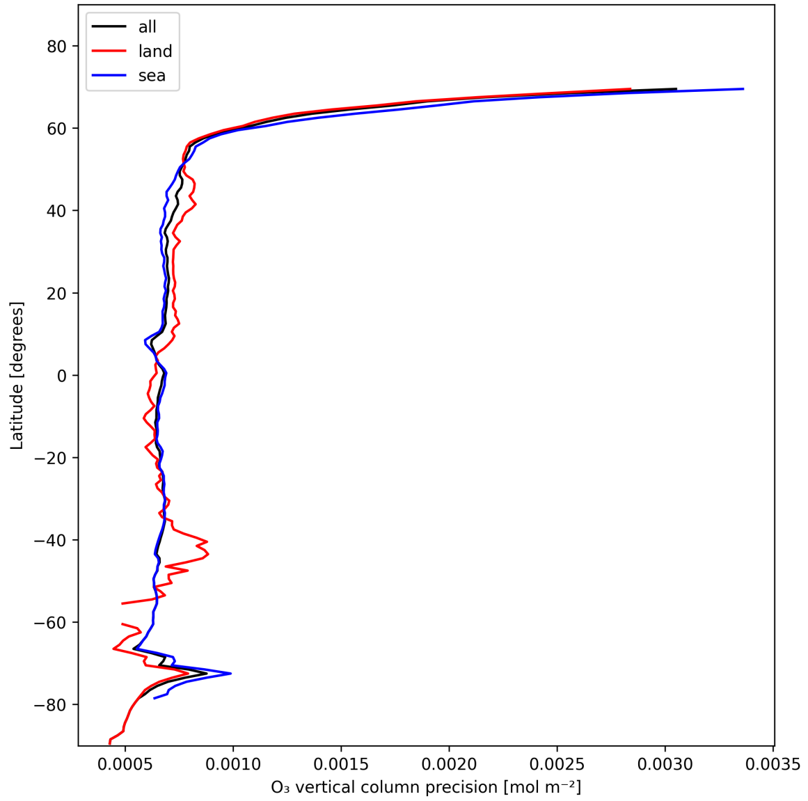
Figure 15: Zonal average of “O 3 vertical column precision” for 2024-11-17 to 2024-11-18.
