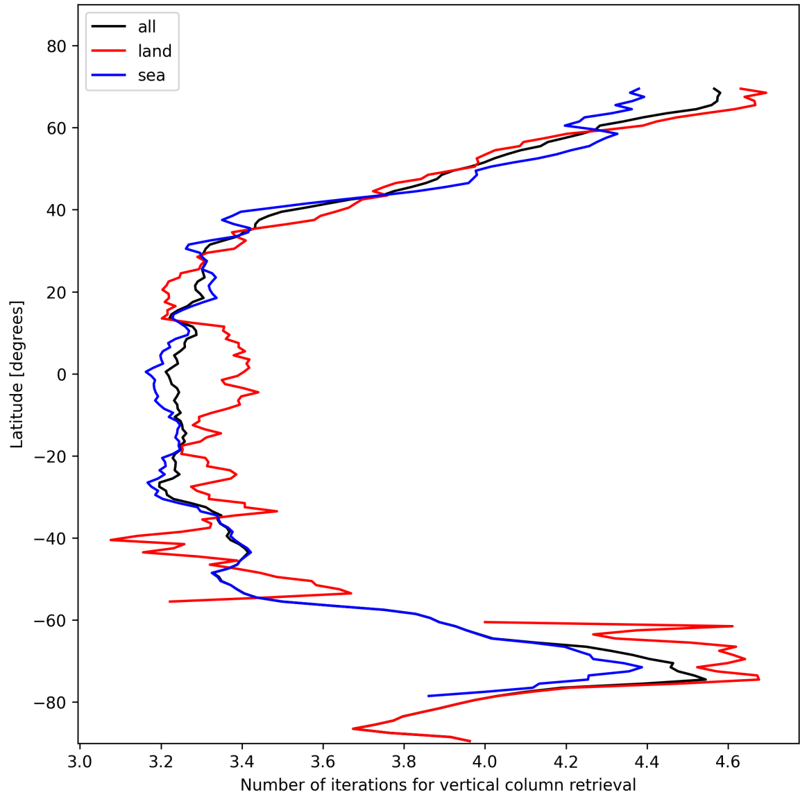
Figure 19: Zonal average of “Number of iterations for vertical column retrieval” for 2024-11-17 to 2024-11-18.
