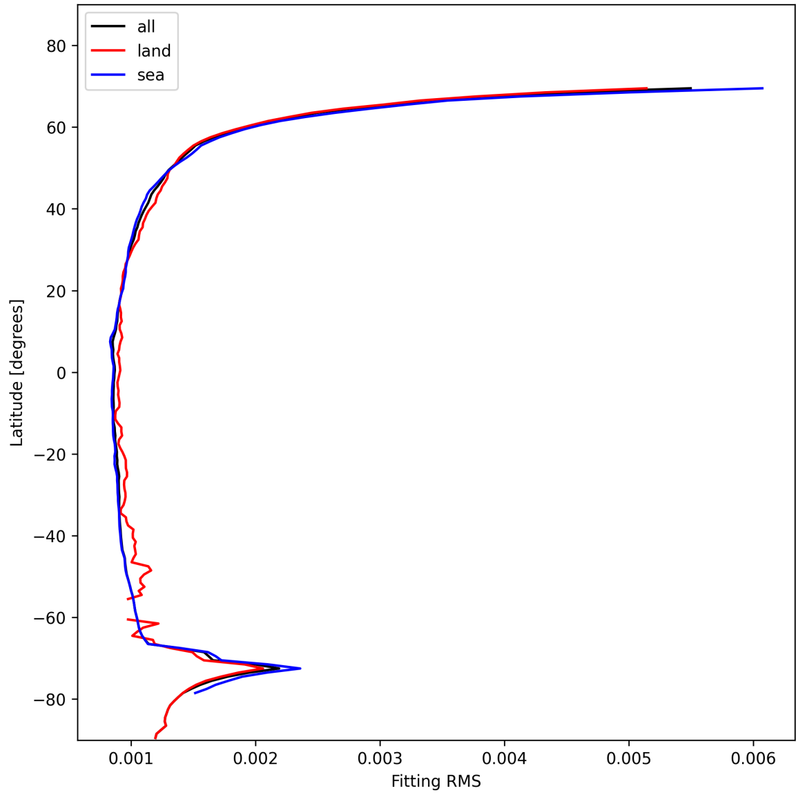
Figure 16: Zonal average of “Fitting RMS” for 2024-11-17 to 2024-11-18.
