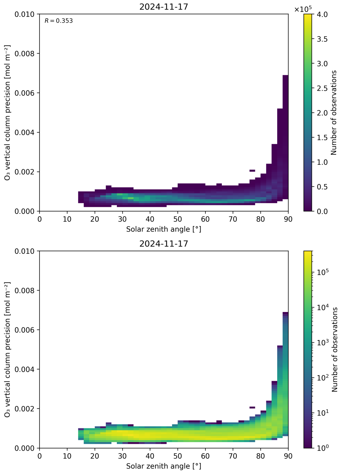
Figure 48: Scatter density plot of “Solar zenith angle” against “O 3 vertical column precision” for 2024-11-17 to 2024-11-18.
