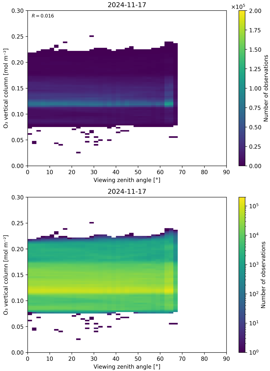
Figure 52: Scatter density plot of “Viewing zenith angle” against “O 3 vertical column” for 2024-11-17 to 2024-11-18.
