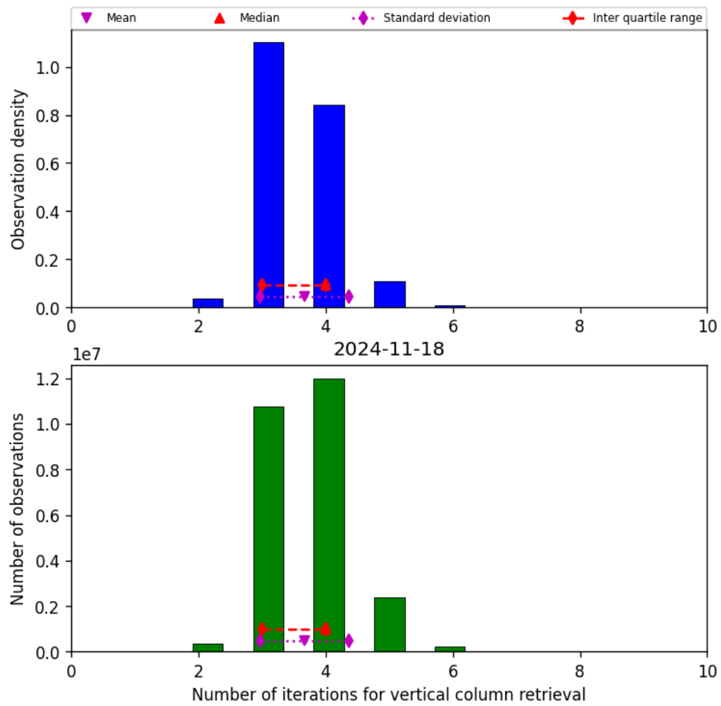
Figure 26: Histogram of “Number of iterations for vertical column retrieval” for 2024-11-17 to 2024-11-19
