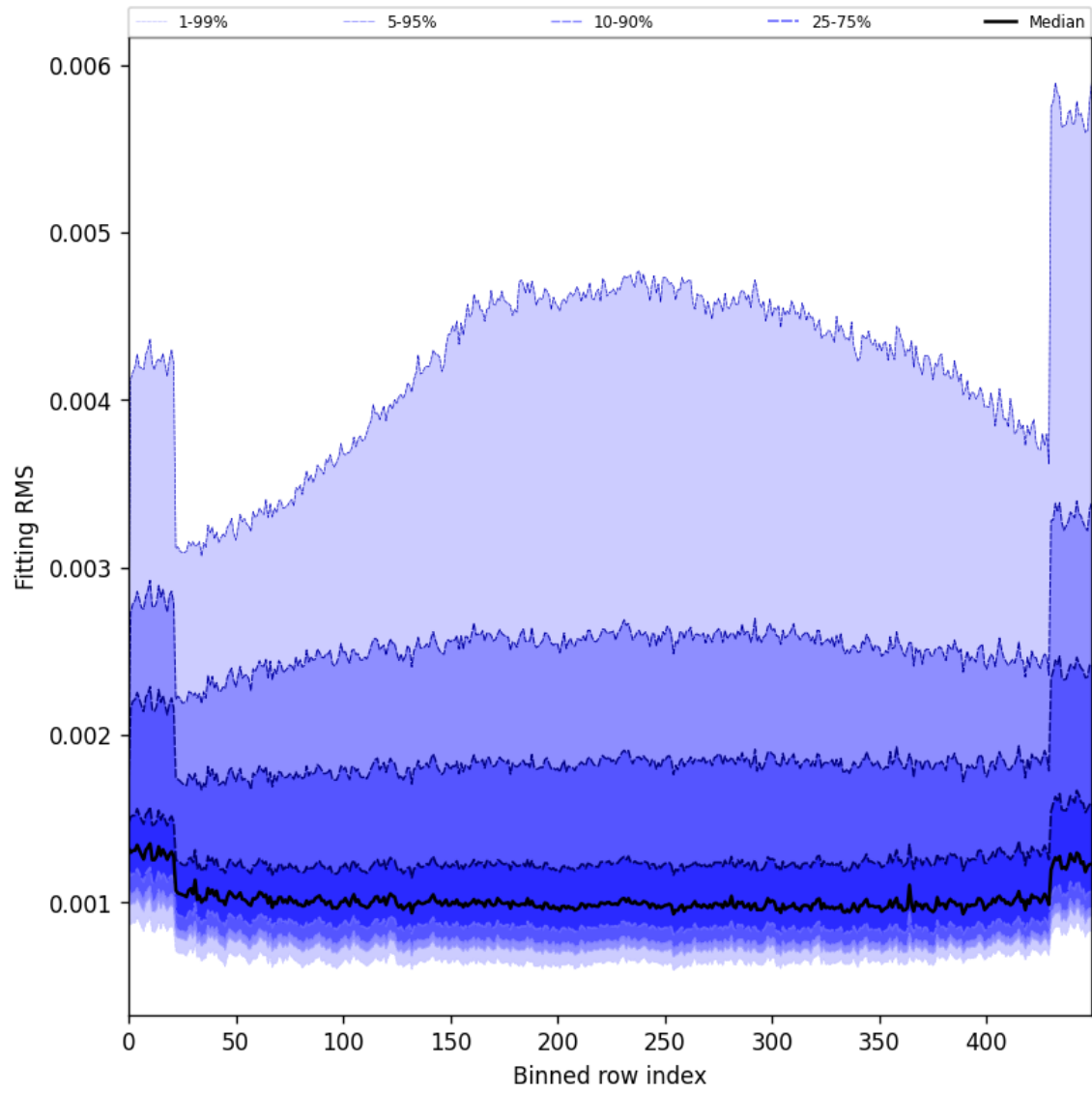
Figure 30: Along track statistics of “Fitting RMS” for 2024-11-17 to 2024-11-19
