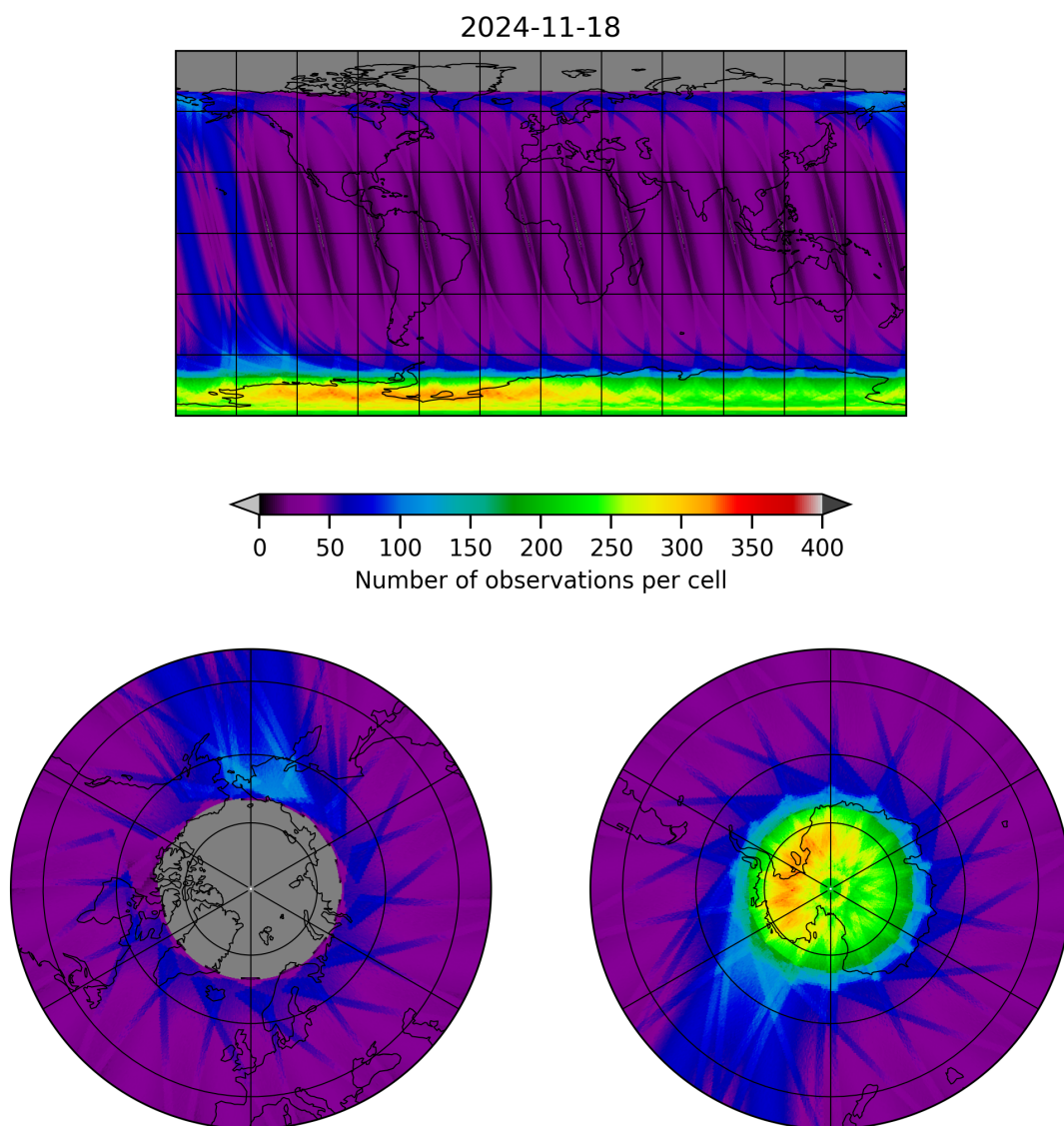
Figure 12: Map of the number of observations for 2024-11-17 to 2024-11-19
