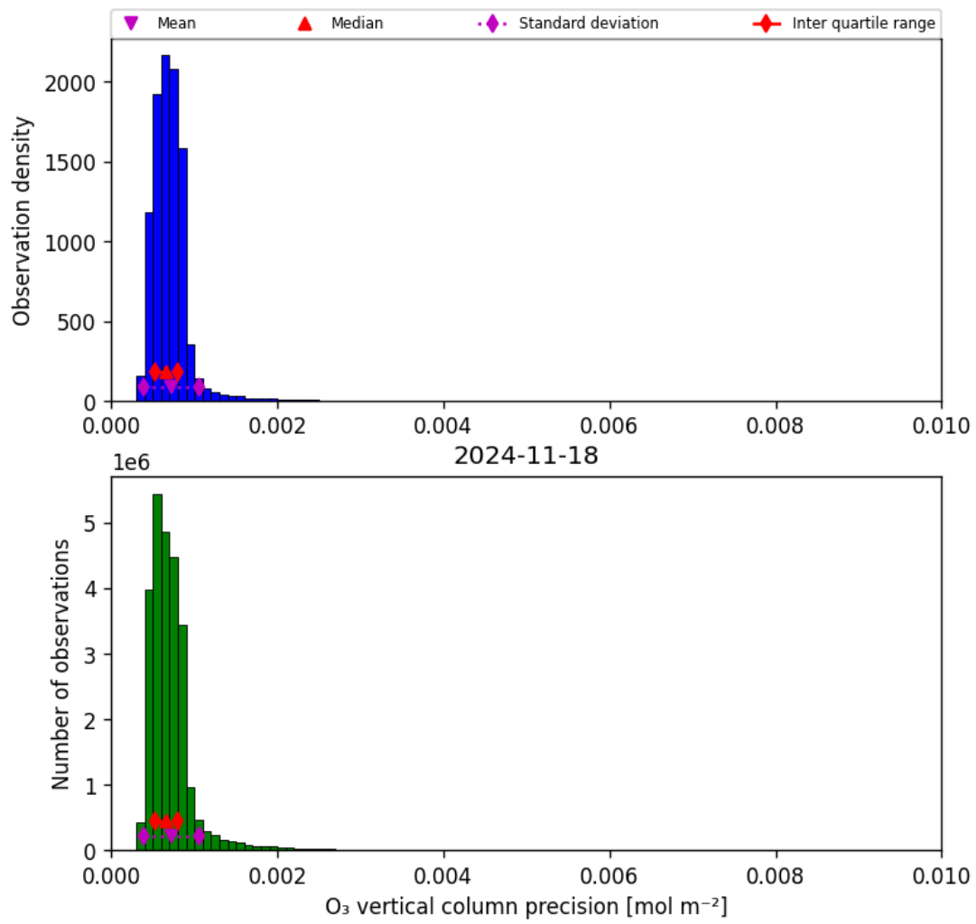
Figure 22: Histogram of “O 3 vertical column precision” for 2024-11-17 to 2024-11-19
