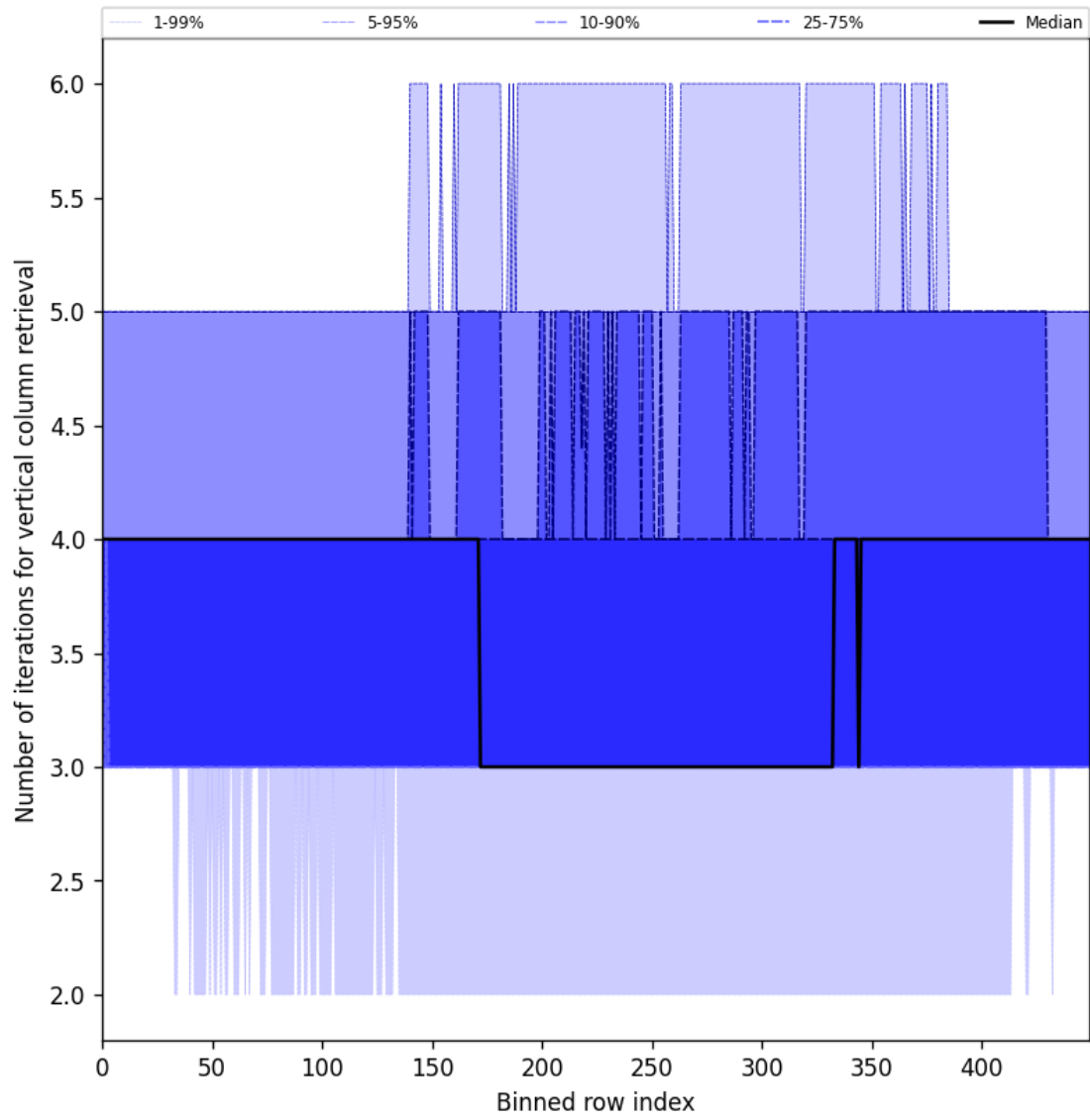
Figure 33: Along track statistics of “Number of iterations for vertical column retrieval” for 2024-11-17 to 2024-11-19
