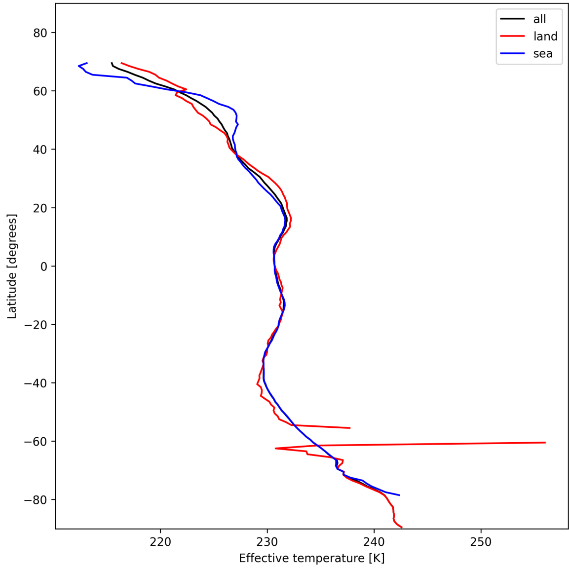
Figure 17: Zonal average of “Effective temperature” for 2024-11-17 to 2024-11-19.
