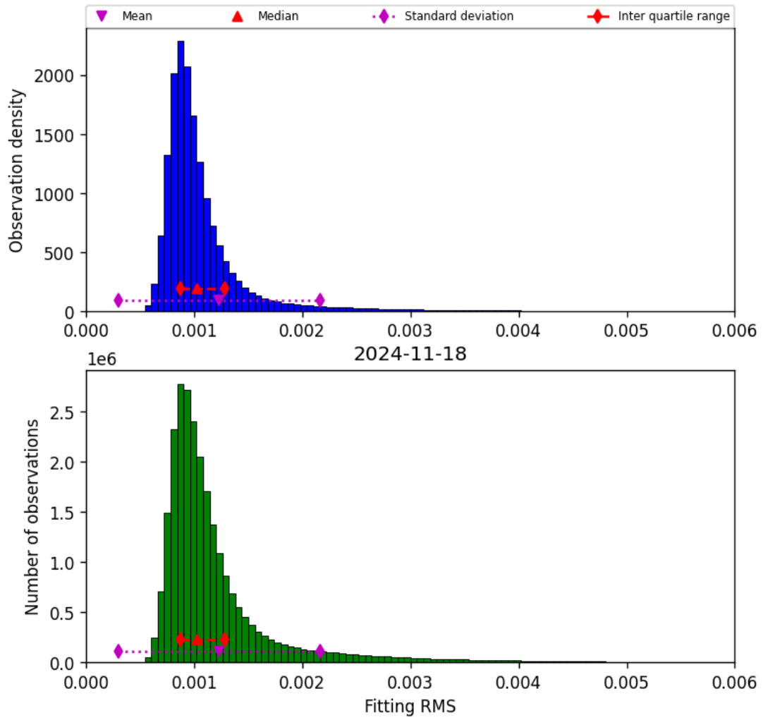
Figure 23: Histogram of “Fitting RMS” for 2024-11-17 to 2024-11-19
