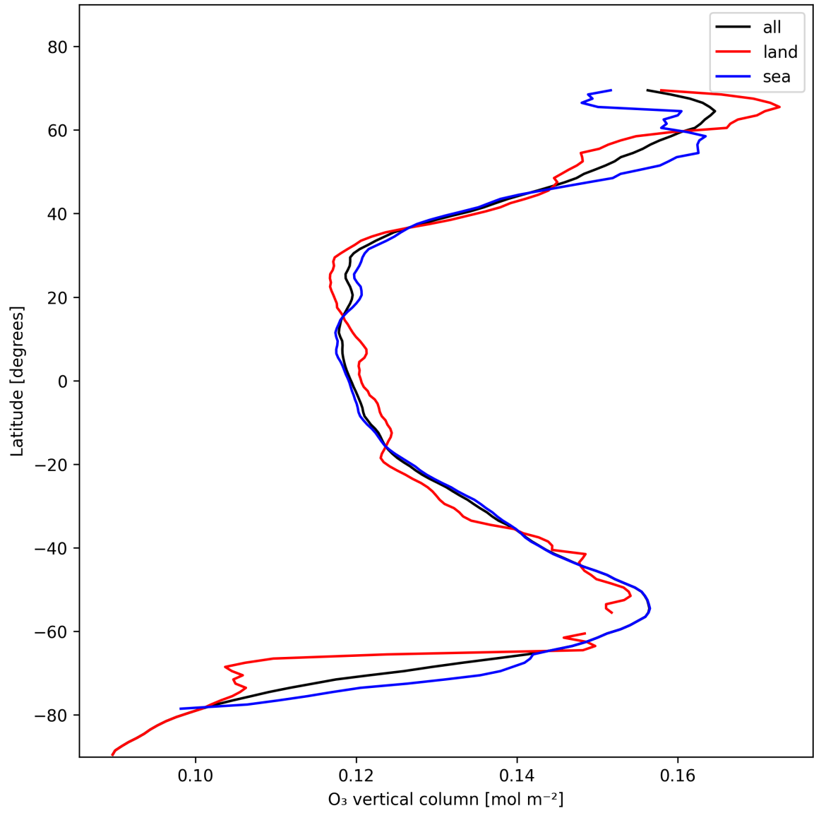
Figure 14: Zonal average of “O 3 vertical column” for 2024-11-17 to 2024-11-19.
