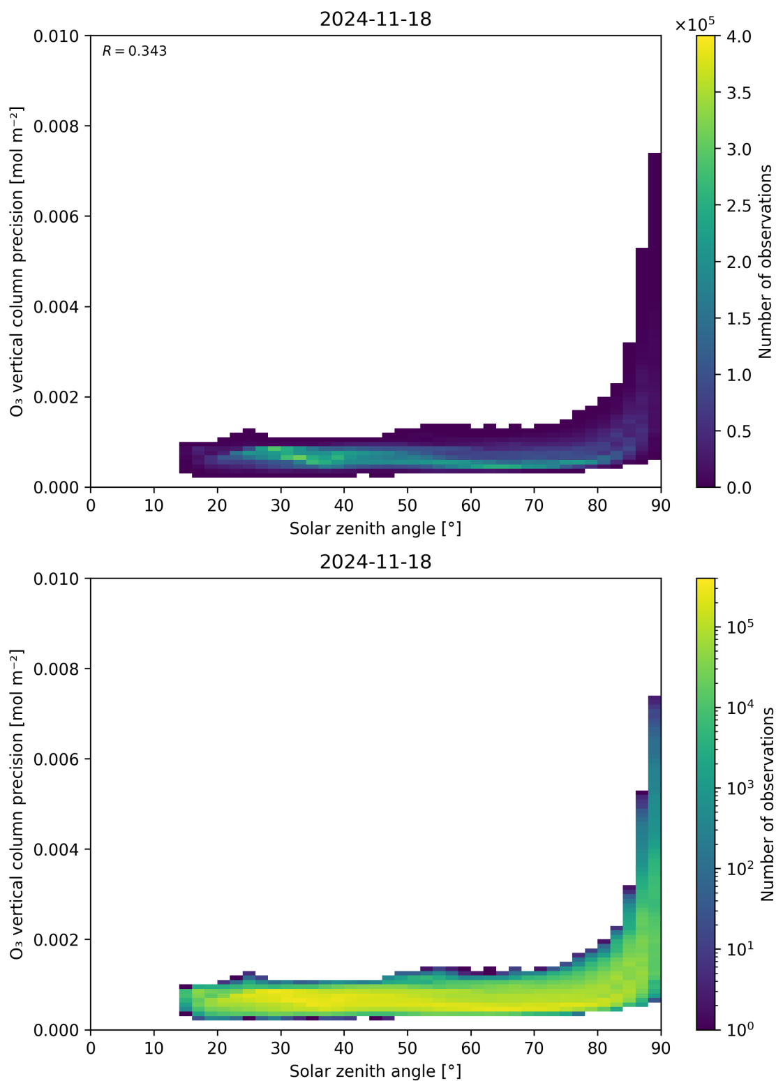
Figure 48: Scatter density plot of “Solar zenith angle” against “O 3 vertical column precision” for 2024-11-17 to 2024-11-19.
