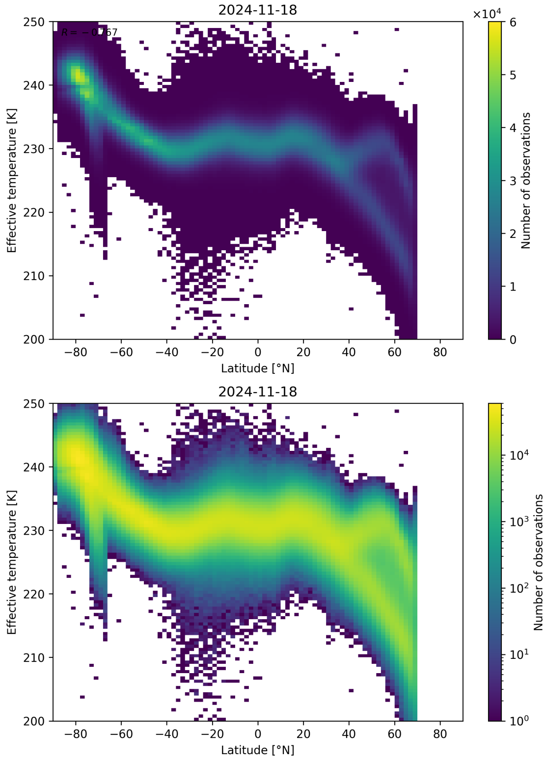
Figure 34: Scatter density plot of “Latitude” against “Effective temperature” for 2024-11-17 to 2024-11-19.
