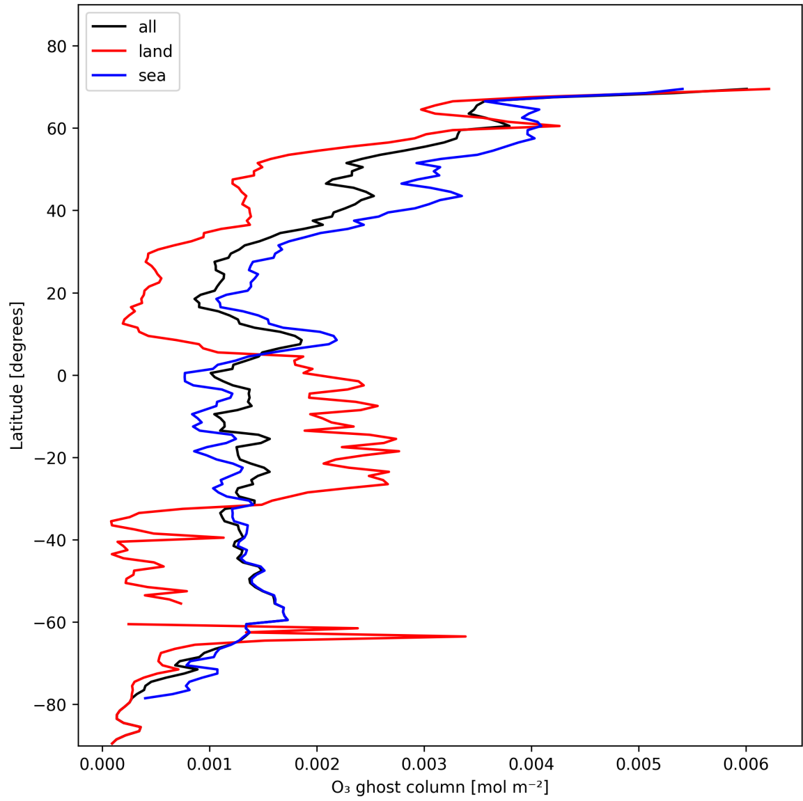
Figure 18: Zonal average of “O 3 ghost column” for 2024-11-17 to 2024-11-19.
