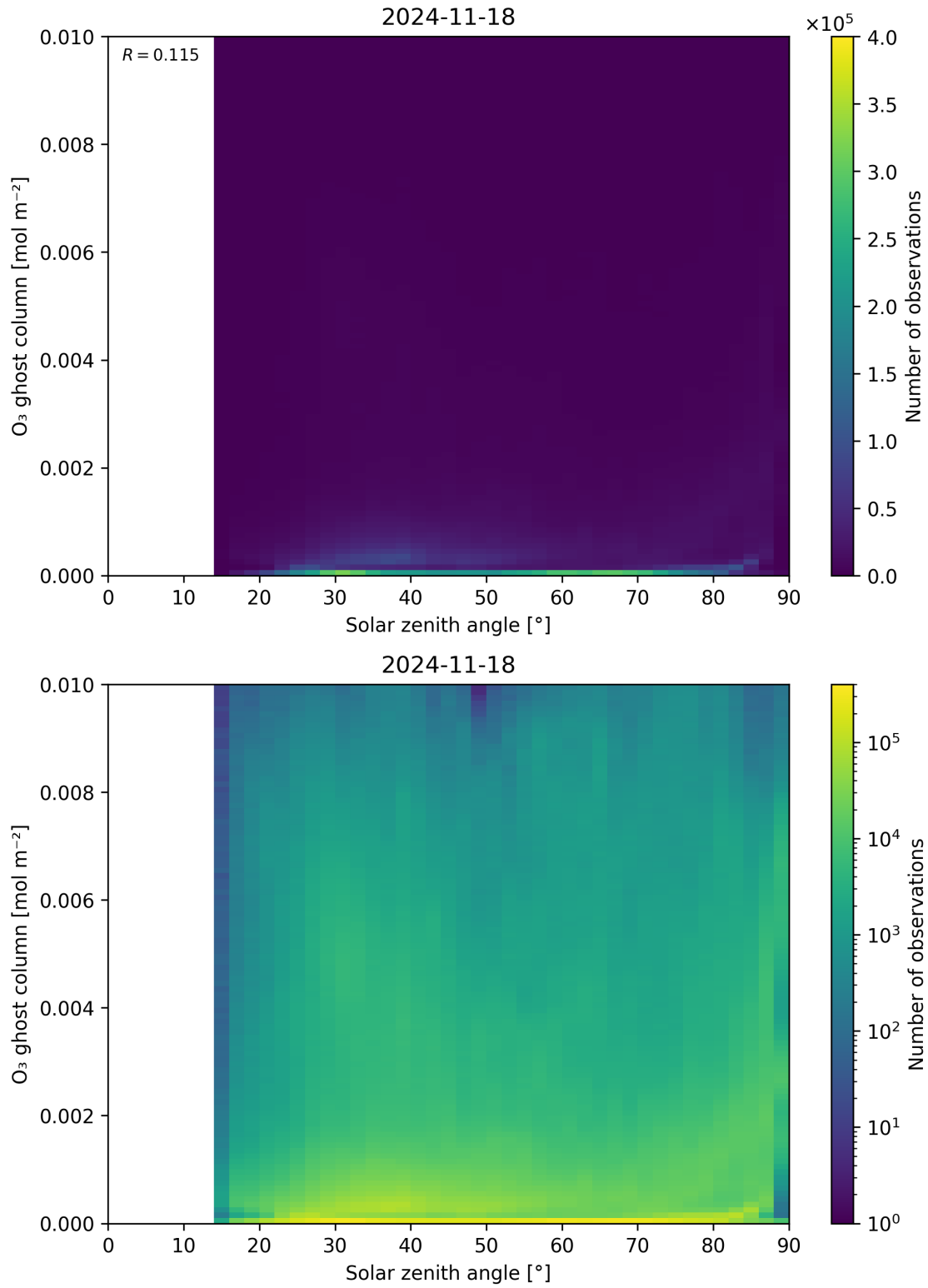
Figure 46: Scatter density plot of “Solar zenith angle” against “O 3 ghost column” for 2024-11-17 to 2024-11-19.
