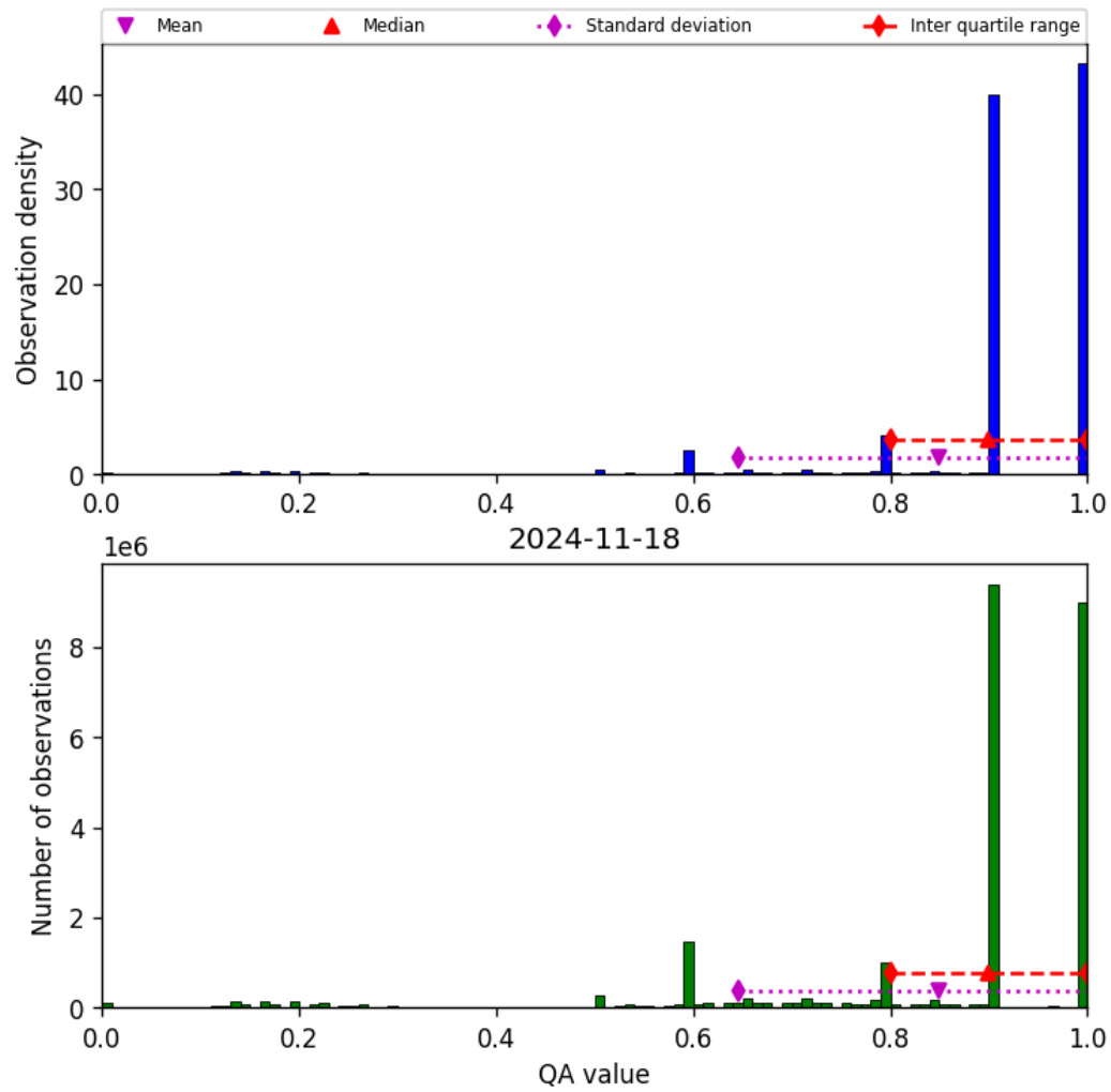
Figure 20: Histogram of “QA value” for 2024-11-17 to 2024-11-19
