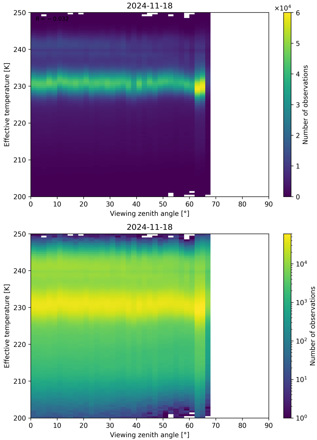
Figure 50: Scatter density plot of “Viewing zenith angle” against “Effective temperature” for 2024-11-17 to 2024-11-19.
