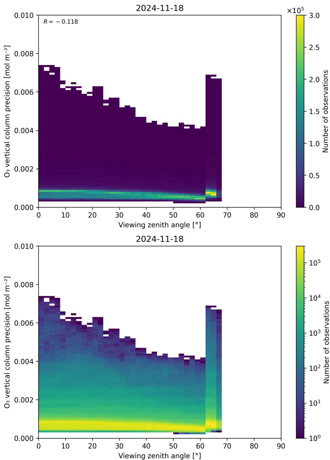
Figure 53: Scatter density plot of “Viewing zenith angle” against “O 3 vertical column precision” for 2024-11-17 to 2024-11-19.
