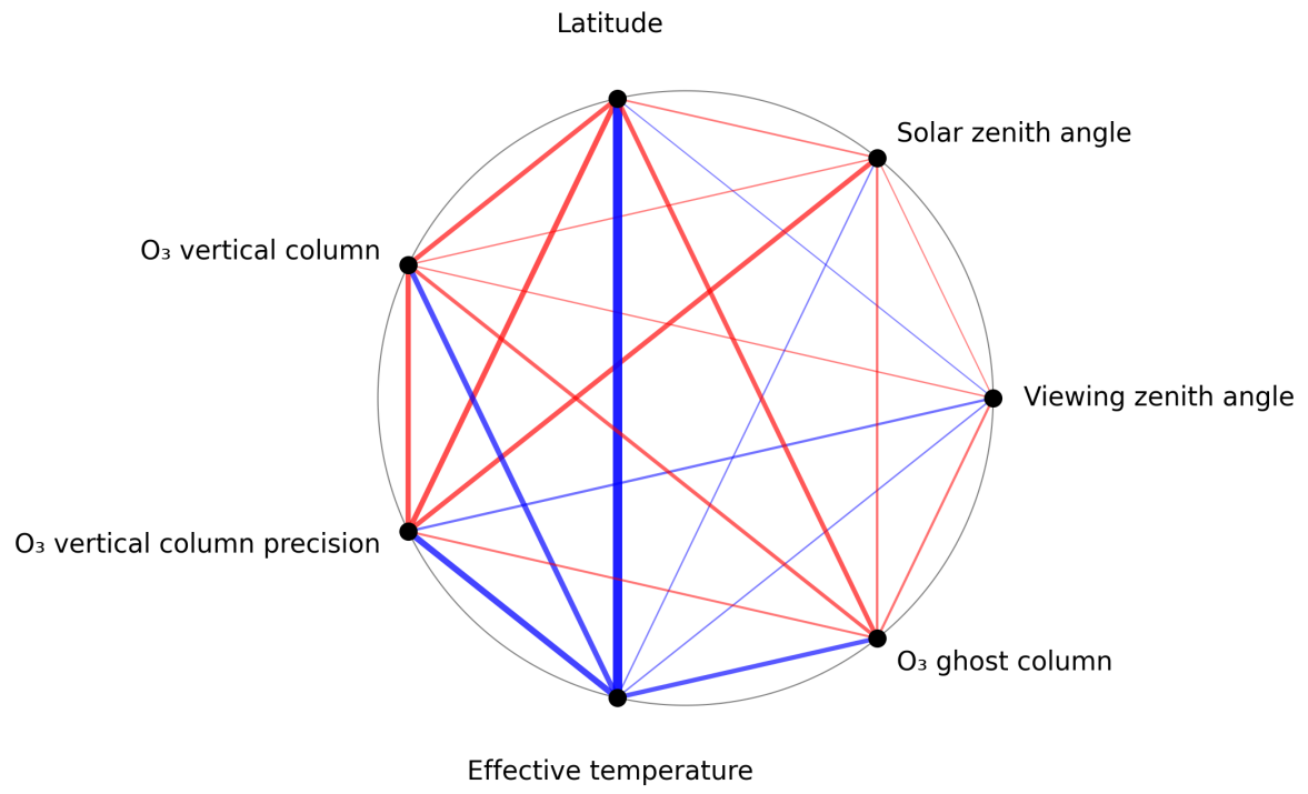
Figure 1: Map of correlation graph for 2024-11-17 to 2024-11-19.
