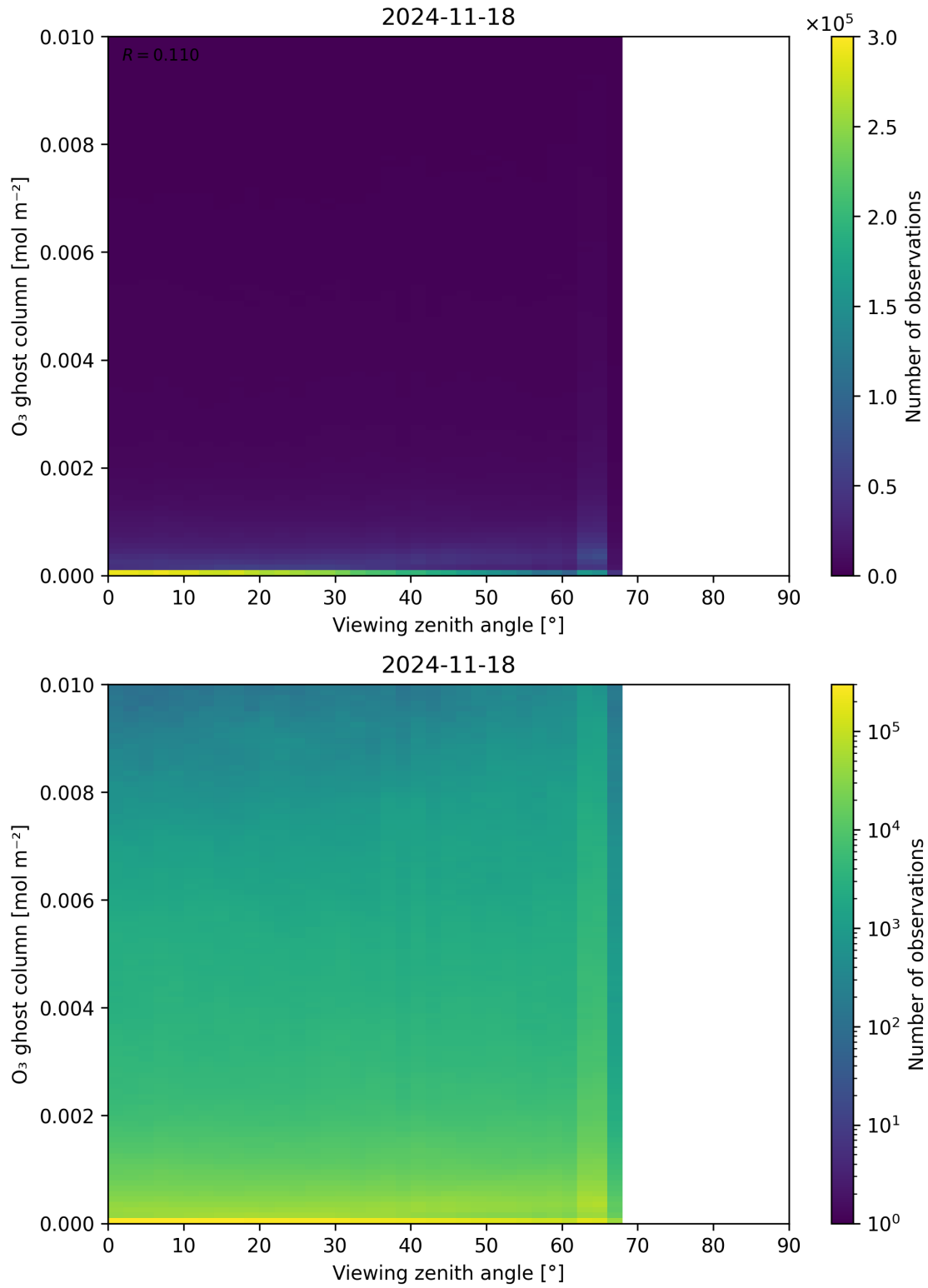
Figure 51: Scatter density plot of “Viewing zenith angle” against “O 3 ghost column” for 2024-11-17 to 2024-11-19.
