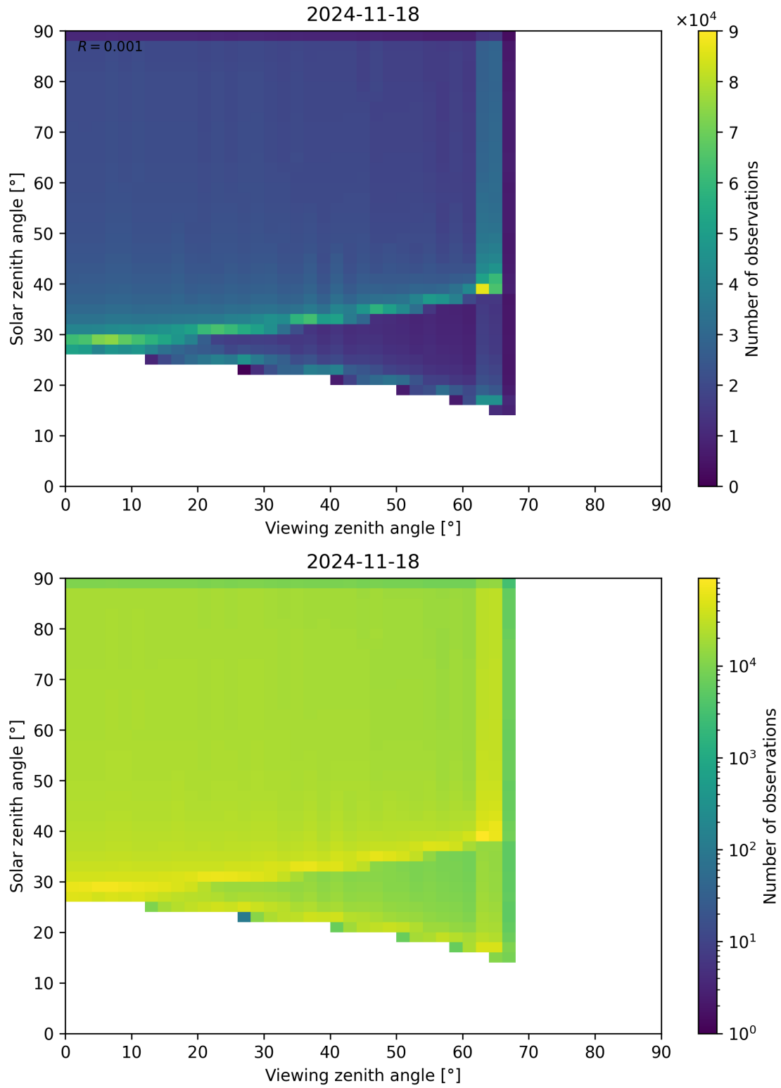
Figure 54: Scatter density plot of “Viewing zenith angle” against “Solar zenith angle” for 2024-11-17 to 2024-11-19.
