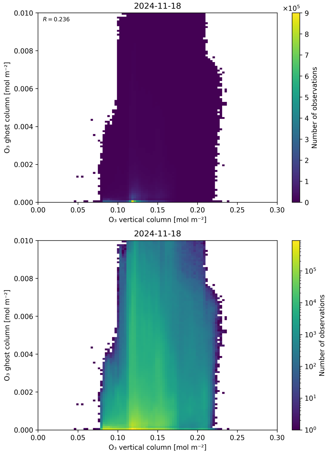
Figure 40: Scatter density plot of “O 3 vertical column” against “O 3 ghost column” for 2024-11-17 to 2024-11-19.
