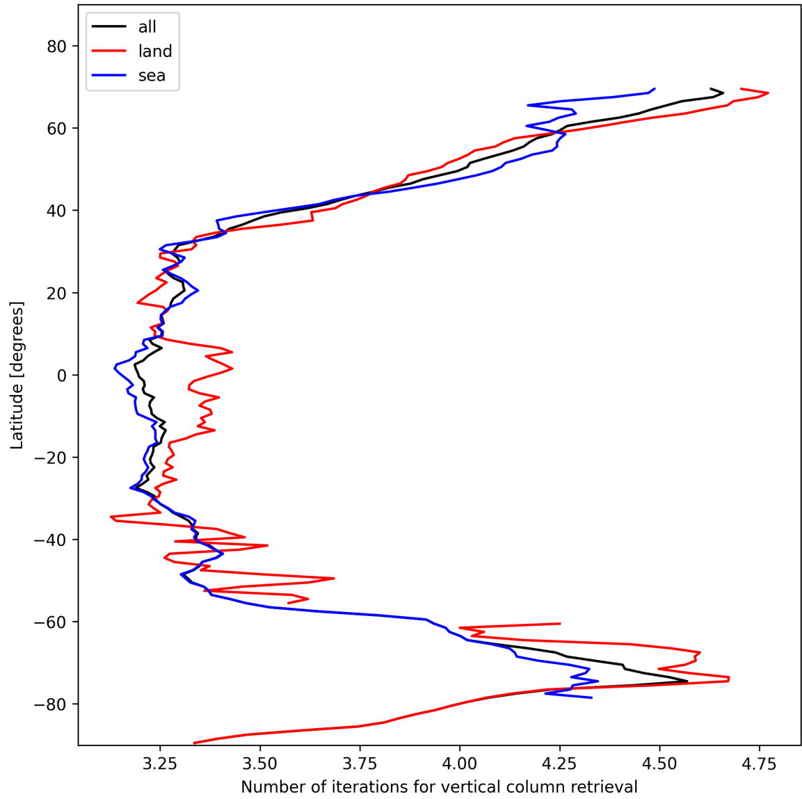
Figure 19: Zonal average of “Number of iterations for vertical column retrieval” for 2024-11-17 to 2024-11-19.
