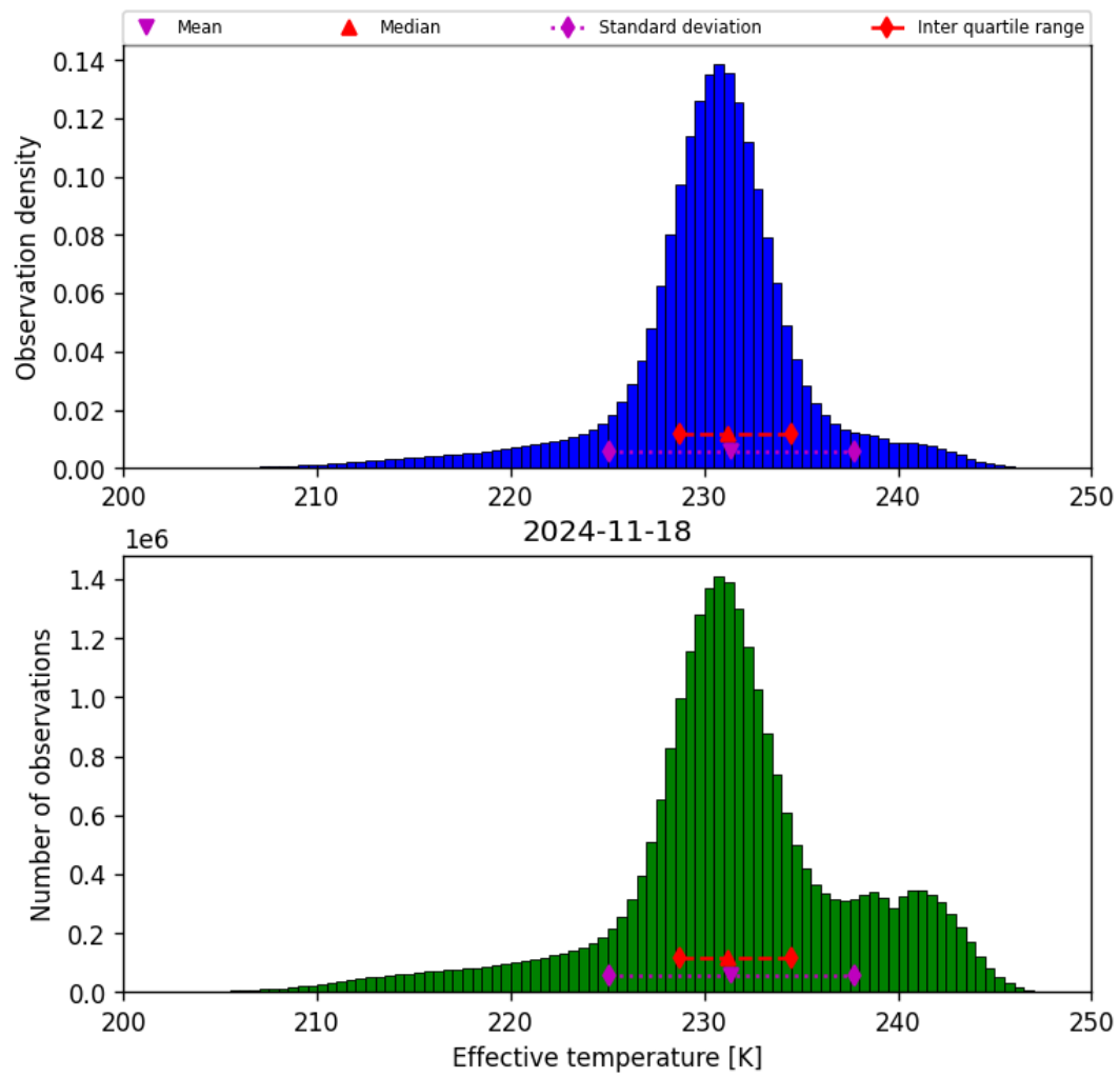
Figure 24: Histogram of “Effective temperature” for 2024-11-17 to 2024-11-19
