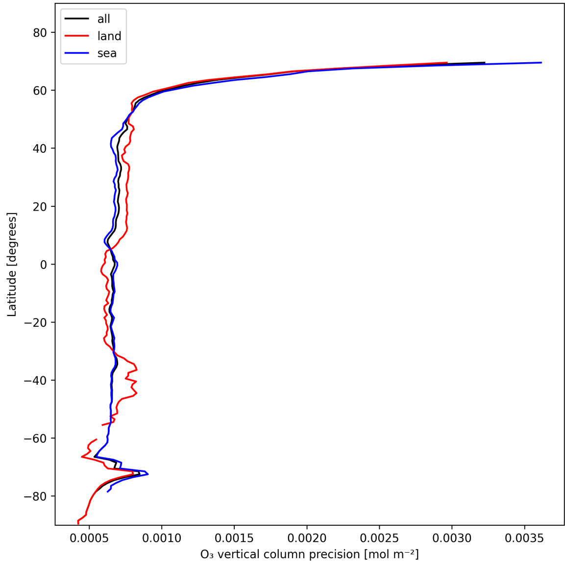
Figure 15: Zonal average of “O 3 vertical column precision” for 2024-11-17 to 2024-11-19.
