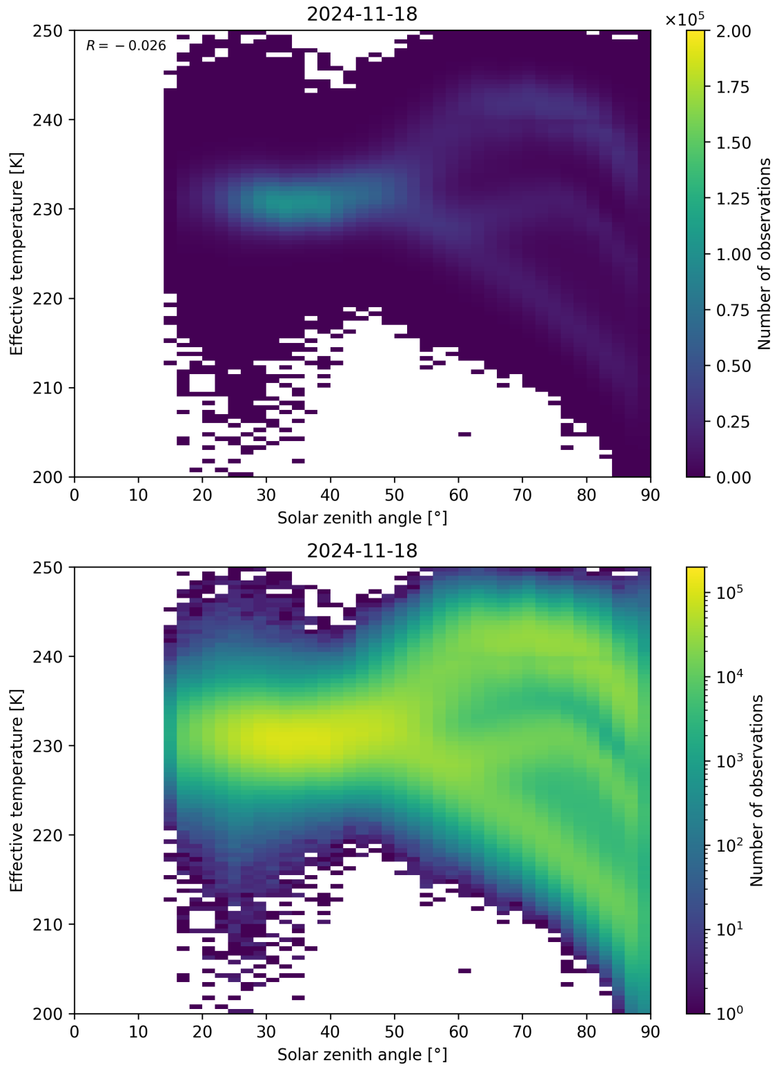
Figure 45: Scatter density plot of “Solar zenith angle” against “Effective temperature” for 2024-11-17 to 2024-11-19.
