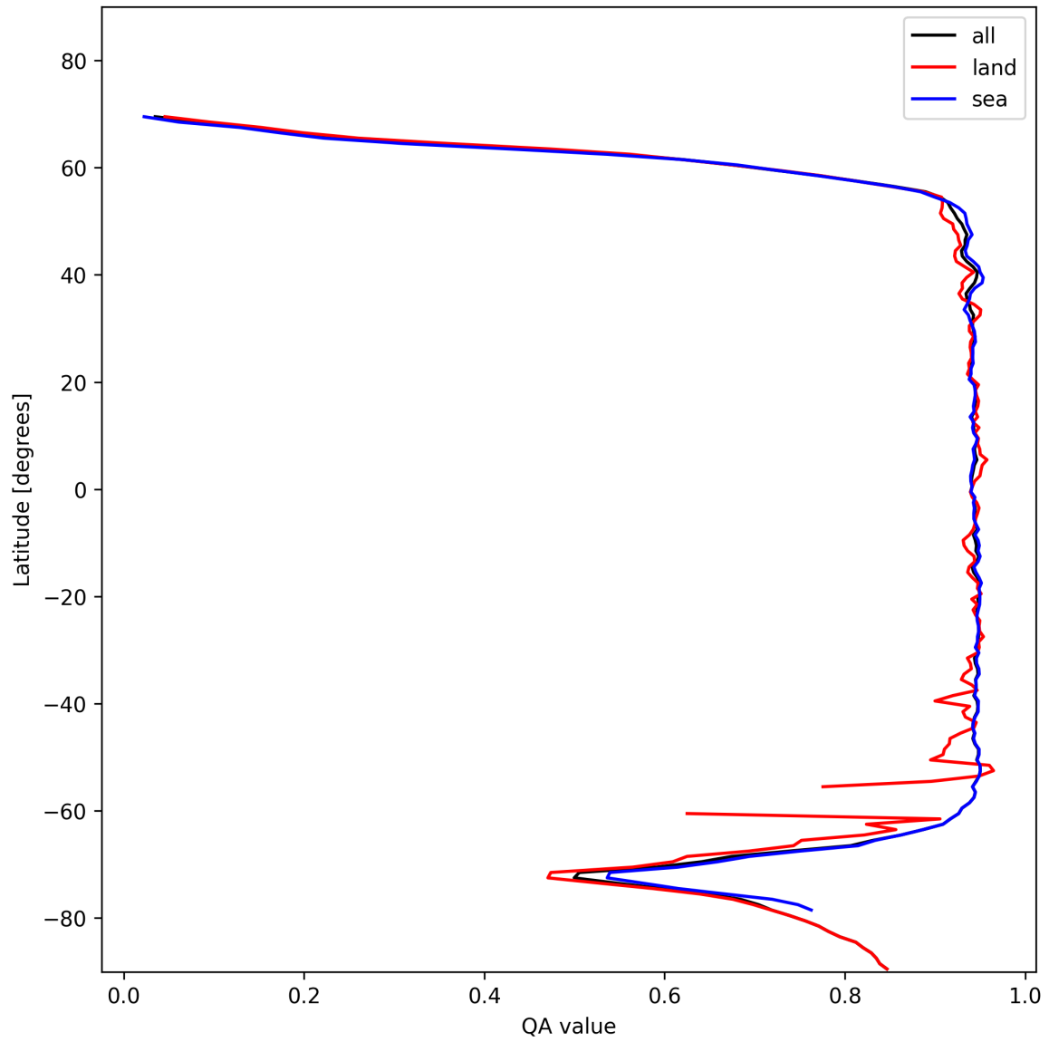
Figure 13: Zonal average of “QA value” for 2024-11-17 to 2024-11-19.
