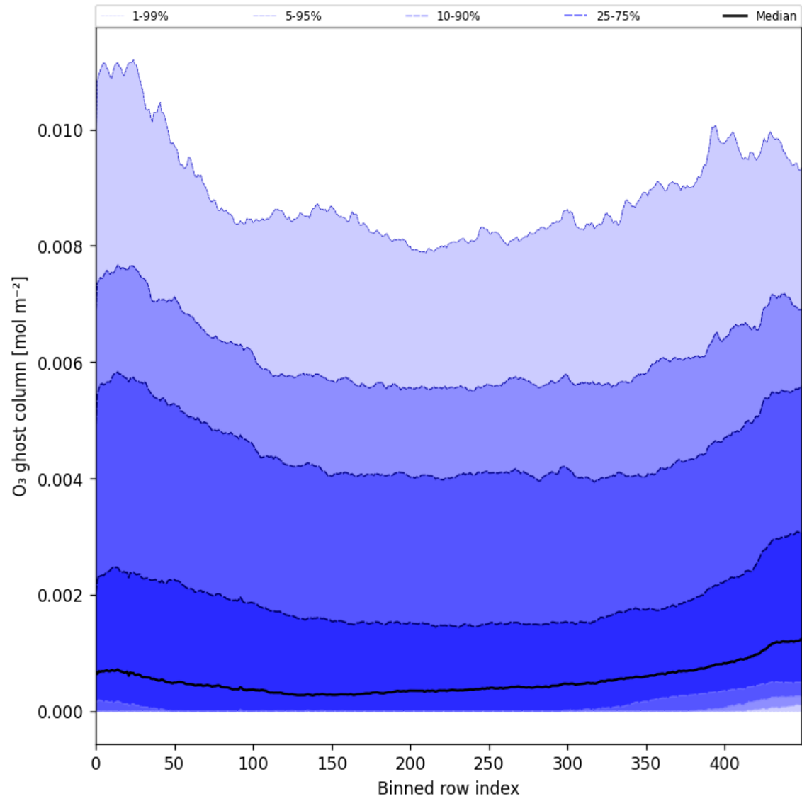
Figure 32: Along track statistics of “O 3 ghost column” for 2024-11-17 to 2024-11-19
