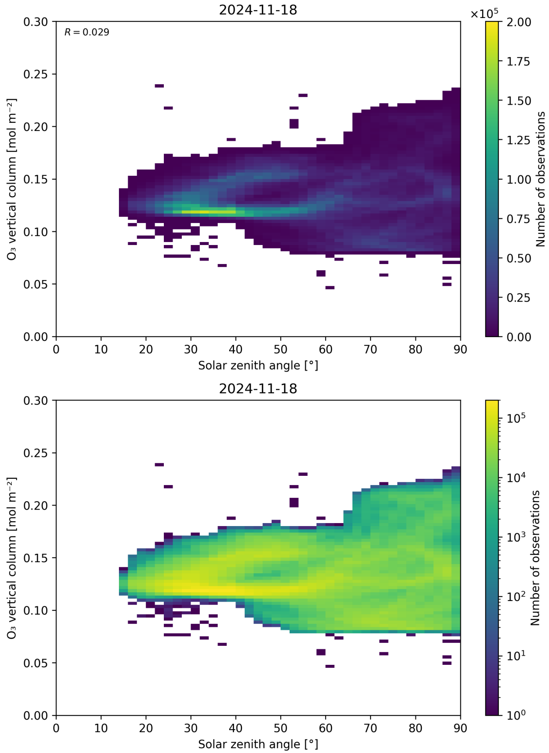
Figure 47: Scatter density plot of “Solar zenith angle” against “O 3 vertical column” for 2024-11-17 to 2024-11-19.
