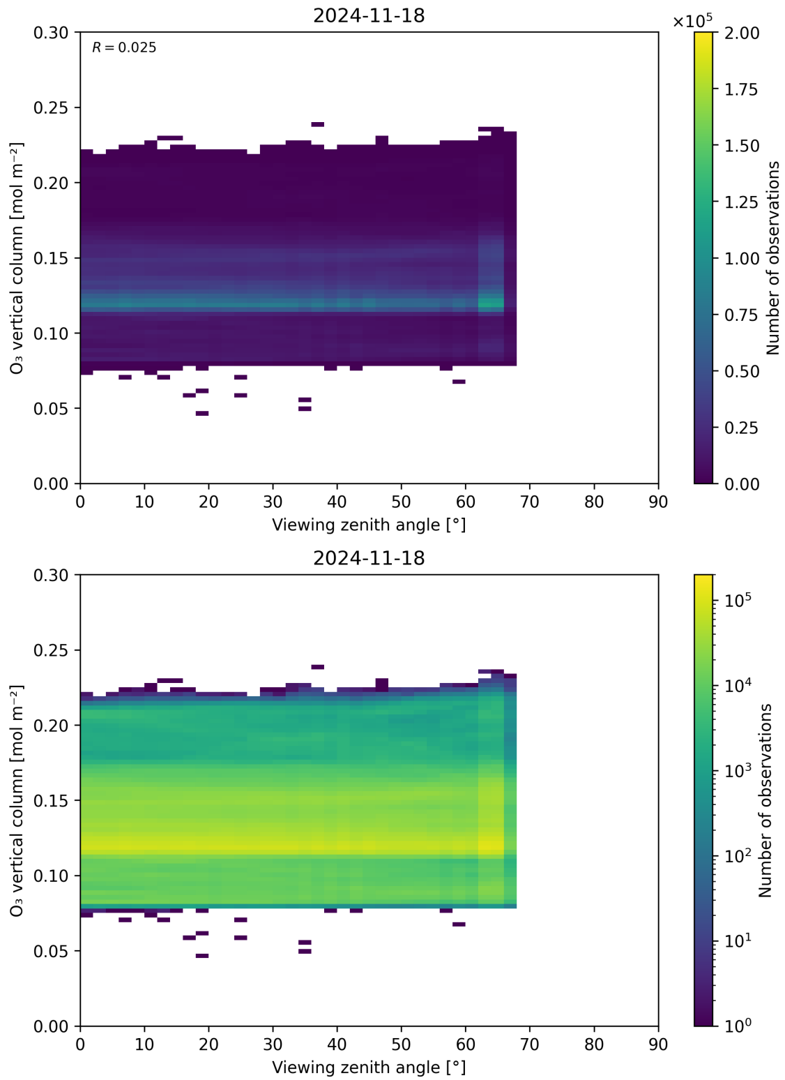
Figure 52: Scatter density plot of “Viewing zenith angle” against “O 3 vertical column” for 2024-11-17 to 2024-11-19.
