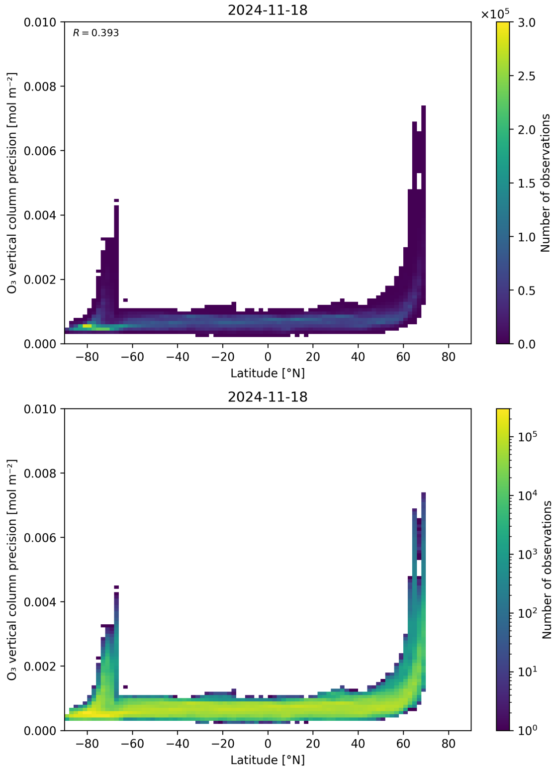
Figure 37: Scatter density plot of “Latitude” against “O 3 vertical column precision” for 2024-11-17 to 2024-11-19.
