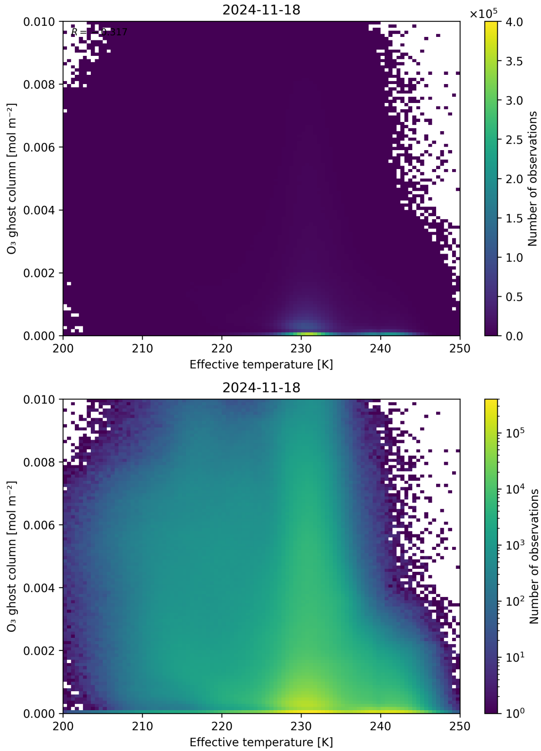
Figure 38: Scatter density plot of “Effective temperature” against “O 3 ghost column” for 2024-11-17 to 2024-11-19.
