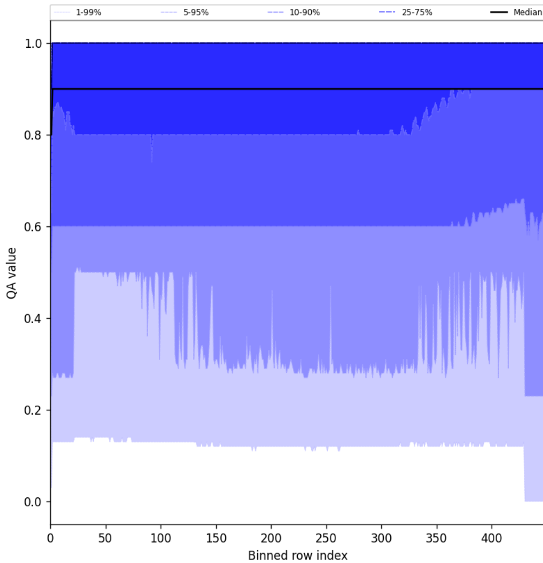
Figure 27: Along track statistics of “QA value” for 2024-11-17 to 2024-11-19
