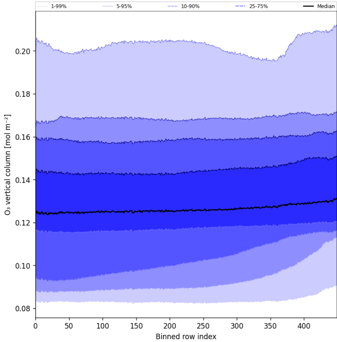
Figure 28: Along track statistics of "O 3 vertical column" for 2024-11-17 to 2024-11-19
