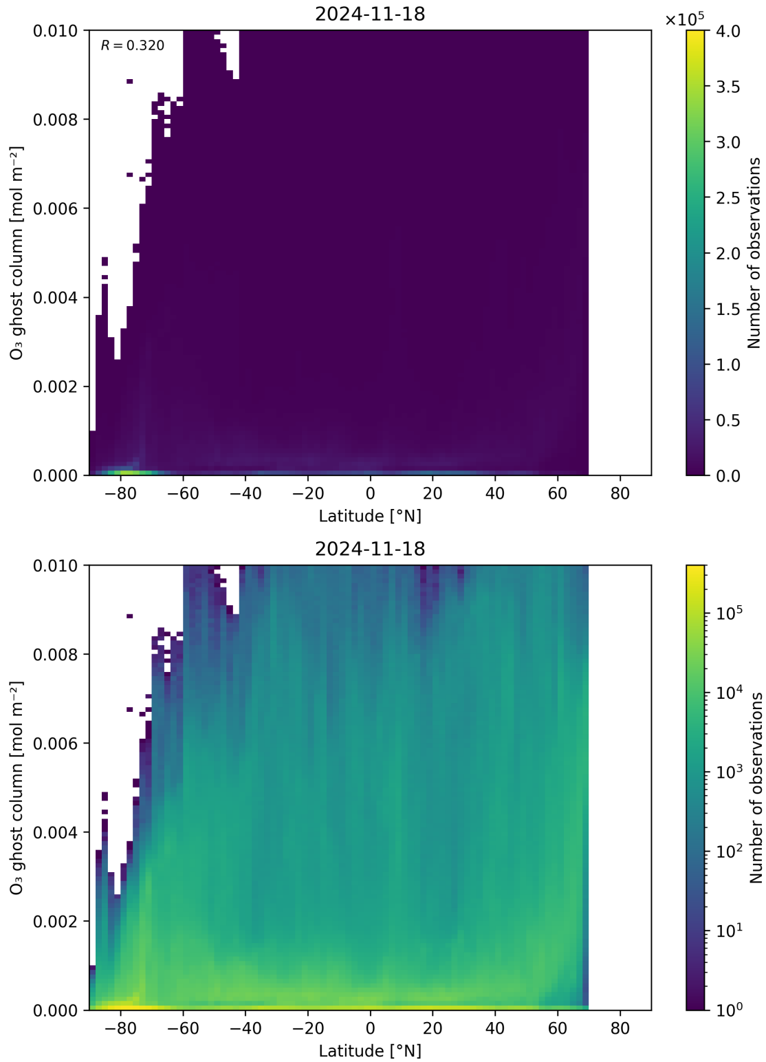
Figure 35: Scatter density plot of “Latitude” against “O 3 ghost column” for 2024-11-17 to 2024-11-19.
