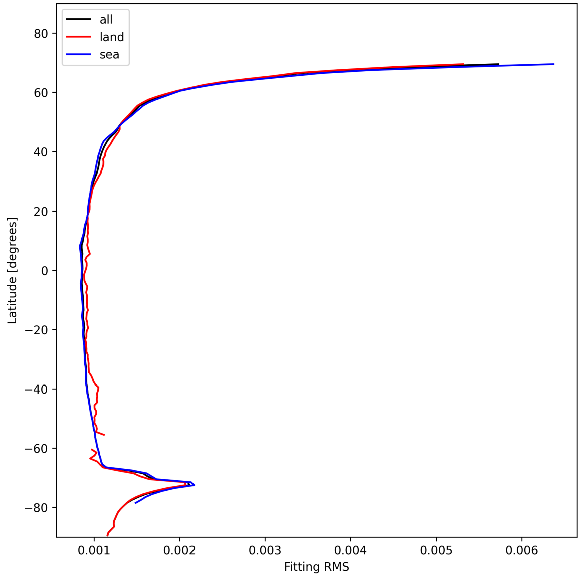
Figure 16: Zonal average of “Fitting RMS” for 2024-11-17 to 2024-11-19.
