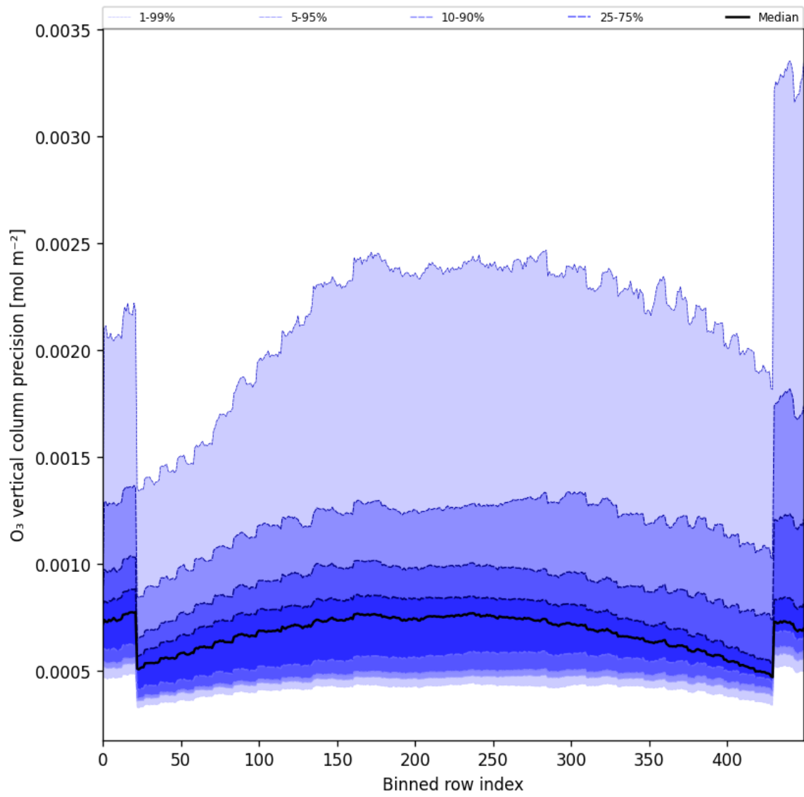
Figure 29: Along track statistics of “O 3 vertical column precision” for 2024-11-17 to 2024-11-19
