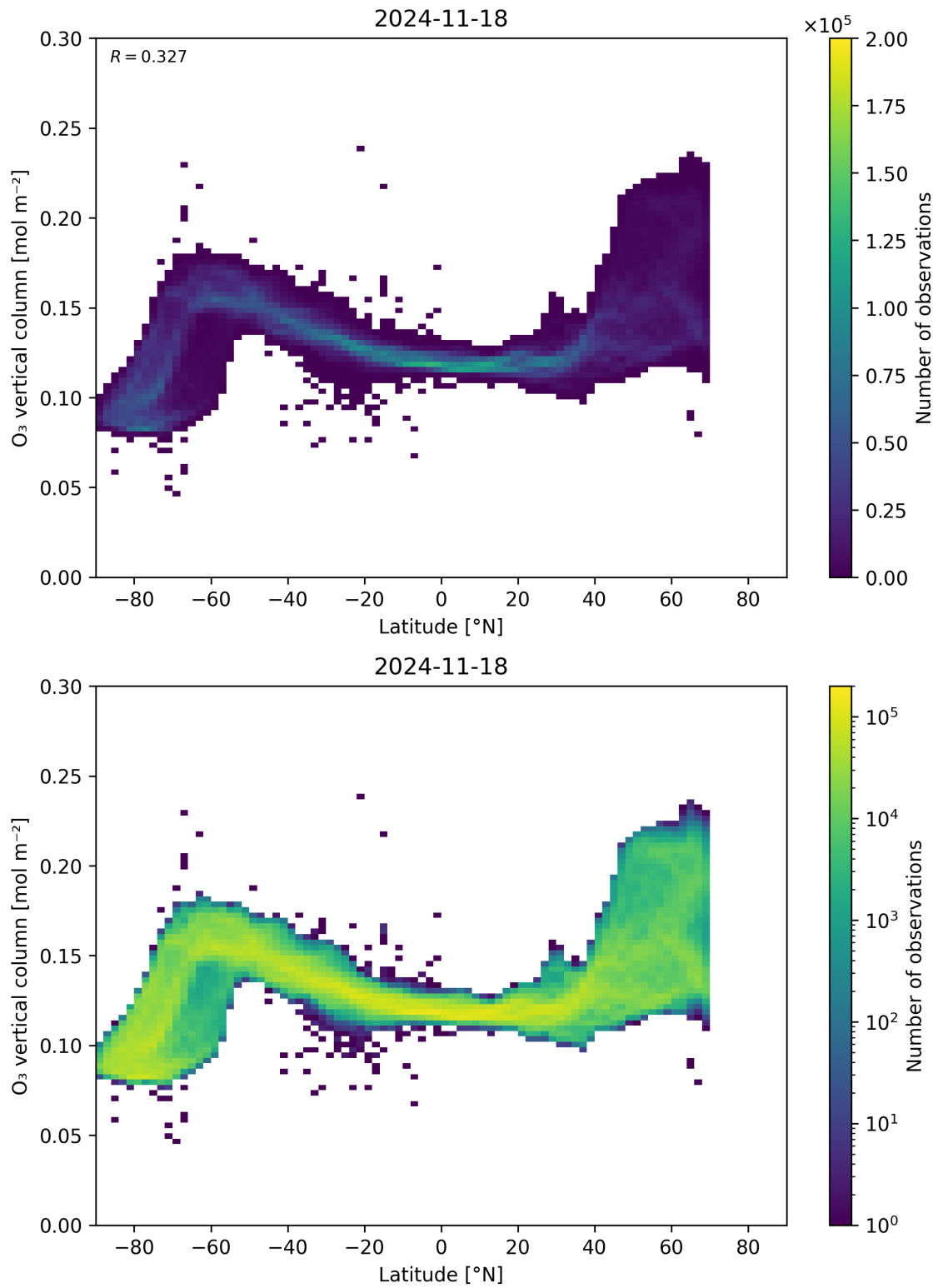
Figure 36: Scatter density plot of “Latitude” against “O 3 vertical column” for 2024-11-17 to 2024-11-19.
