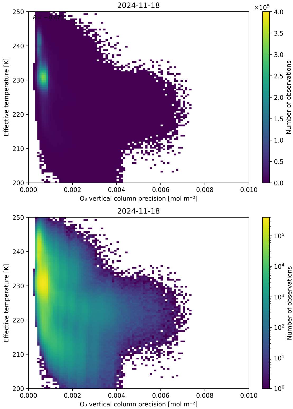
Figure 42: Scatter density plot of “O 3 vertical column precision” against “Effective temperature” for 2024-11-17 to 2024-11-19.
