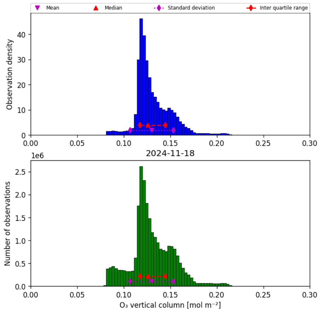
Figure 21: Histogram of “O 3 vertical column” for 2024-11-17 to 2024-11-19
