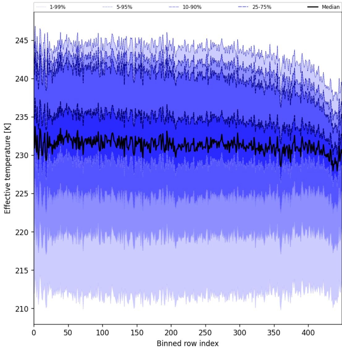
Figure 31: Along track statistics of “Effective temperature” for 2024-11-17 to 2024-11-19
