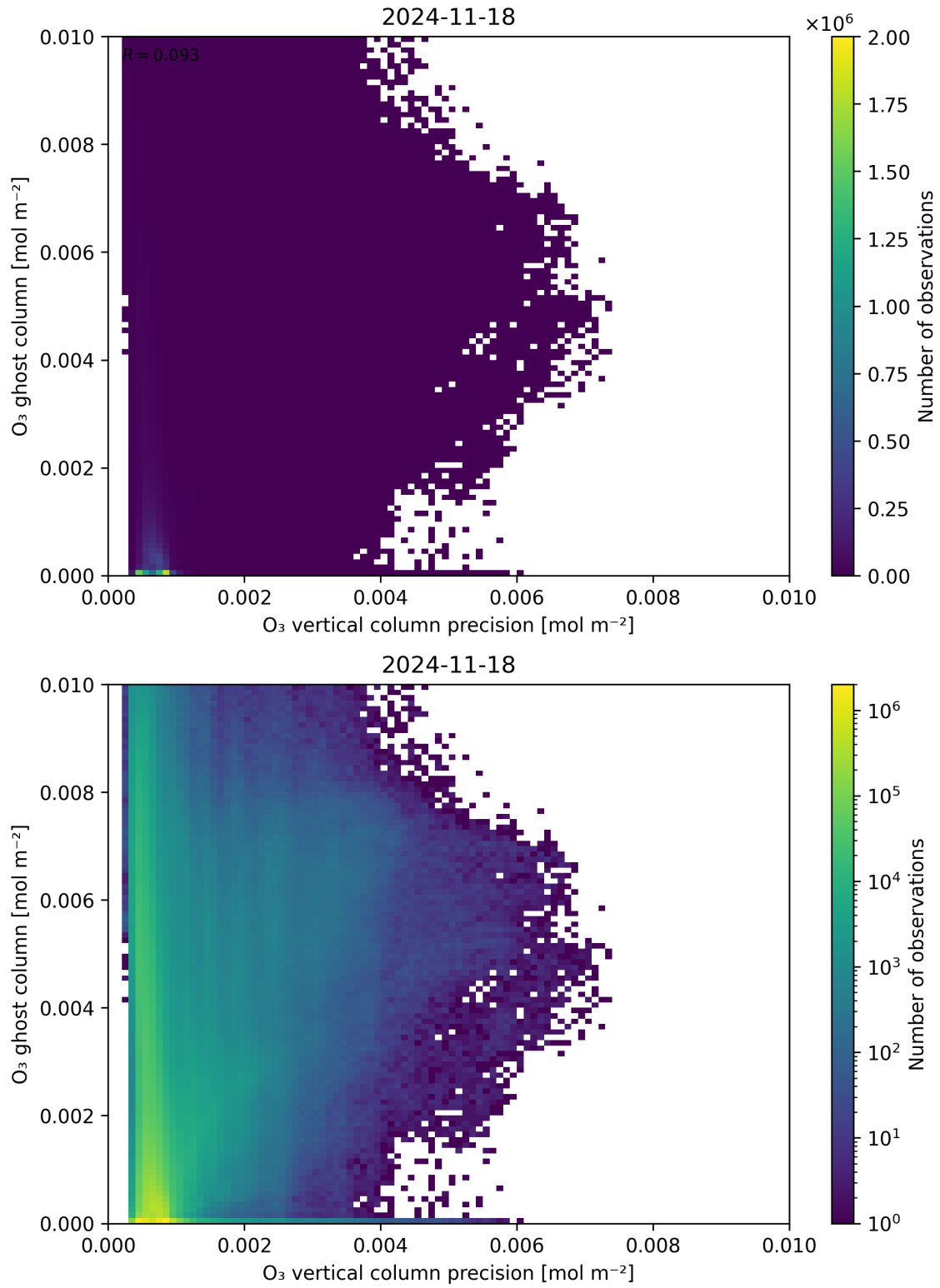
Figure 43: Scatter density plot of “ \text{O}_3 vertical column precision” against “ \text{O}_3 ghost column” for 2024-11-17 to 2024-11-19.
