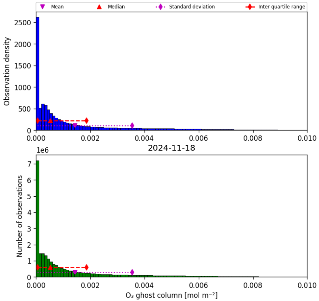
Figure 25: Histogram of “O 3 ghost column” for 2024-11-17 to 2024-11-19
