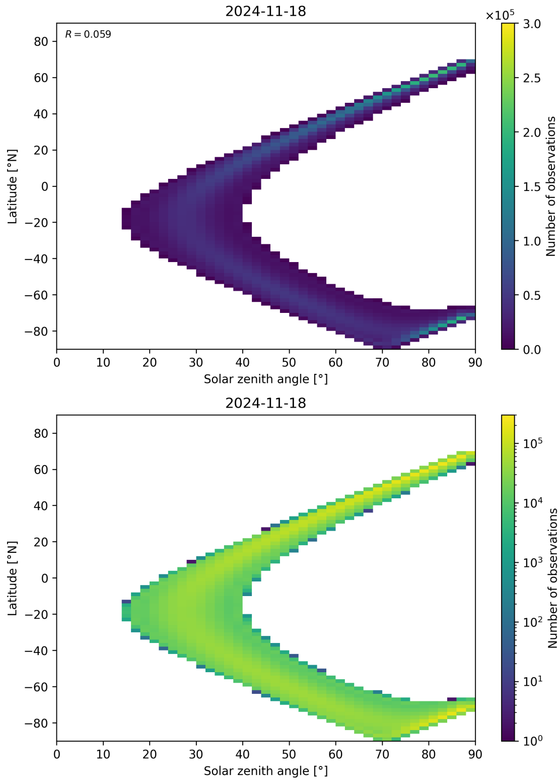
Figure 44: Scatter density plot of “Solar zenith angle” against “Latitude” for 2024-11-17 to 2024-11-19.
