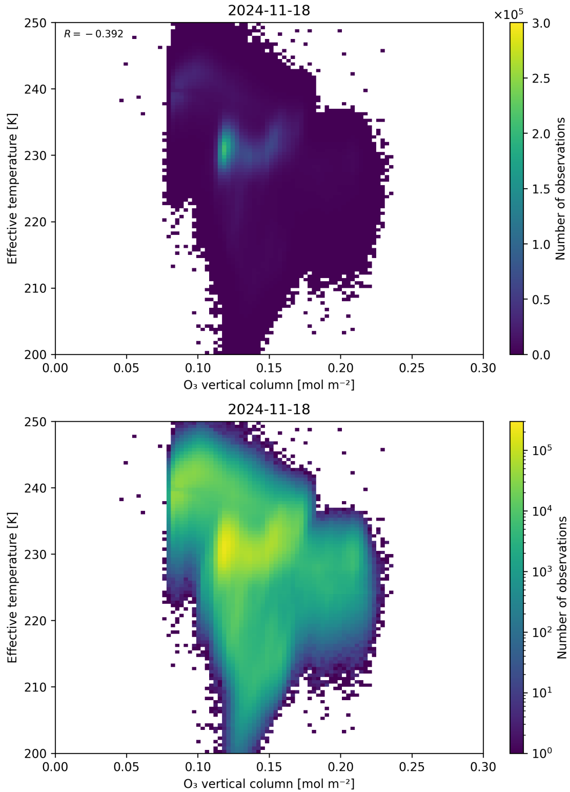
Figure 39: Scatter density plot of “O 3 vertical column” against “Effective temperature” for 2024-11-17 to 2024-11-19.
