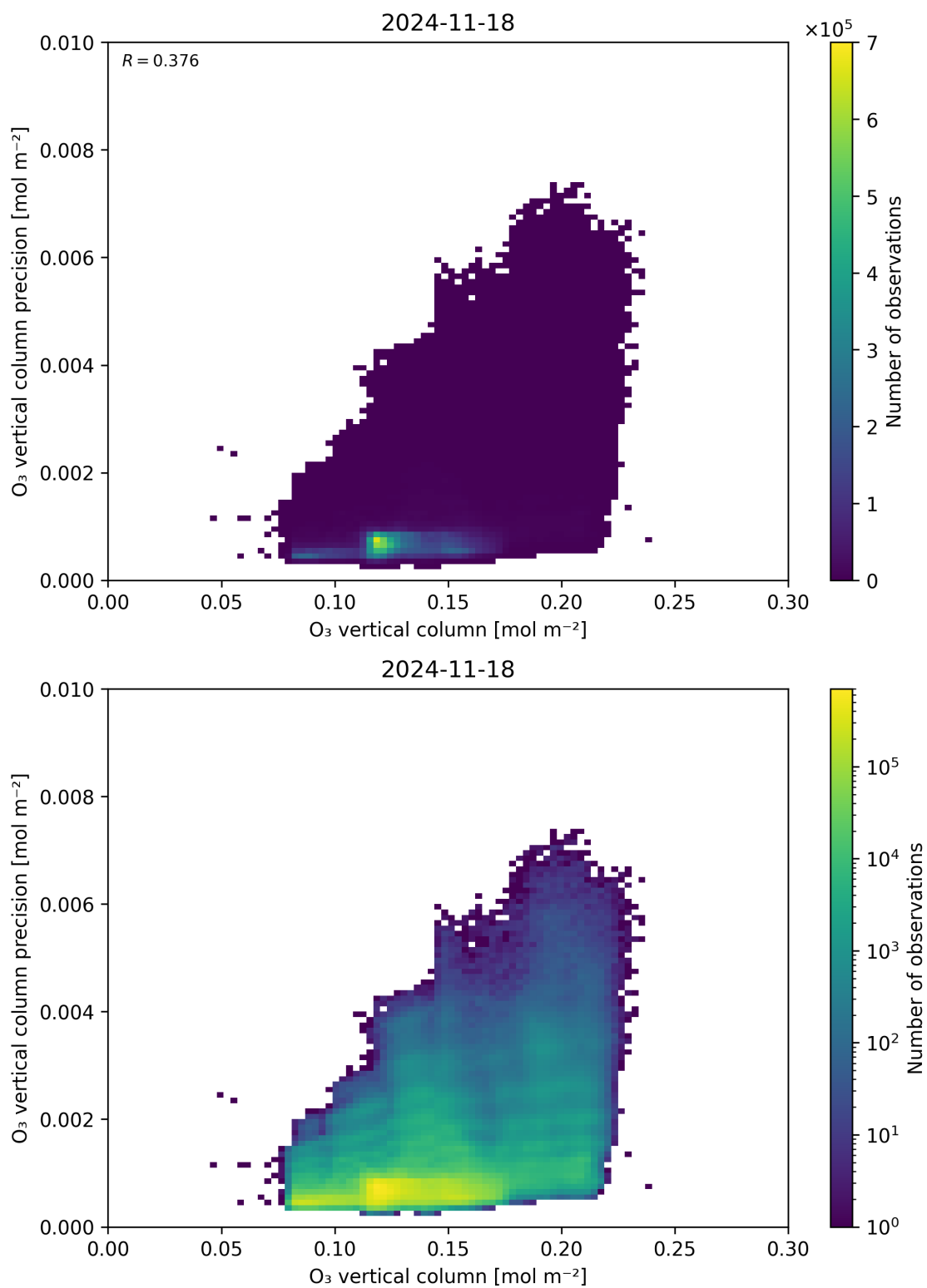
Figure 41: Scatter density plot of “O 3 vertical column” against “O 3 vertical column precision” for 2024-11-17 to 2024-11-19.
