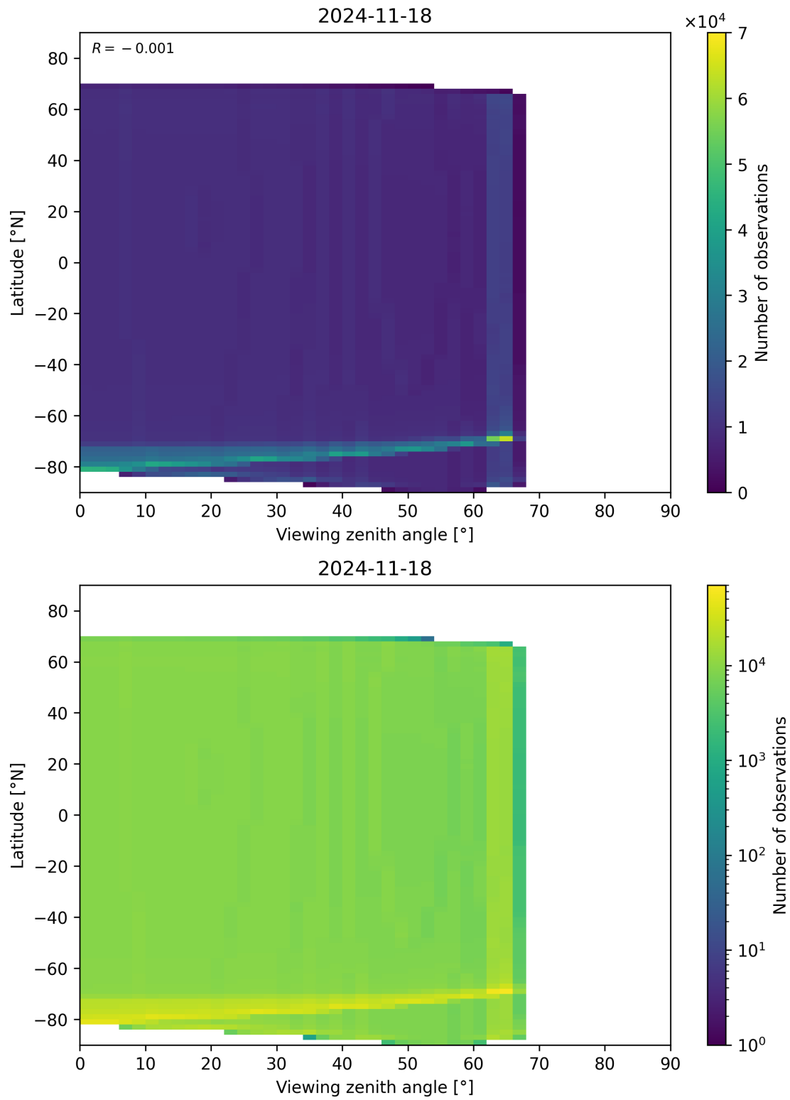
Figure 49: Scatter density plot of “Viewing zenith angle” against “Latitude” for 2024-11-17 to 2024-11-19.
