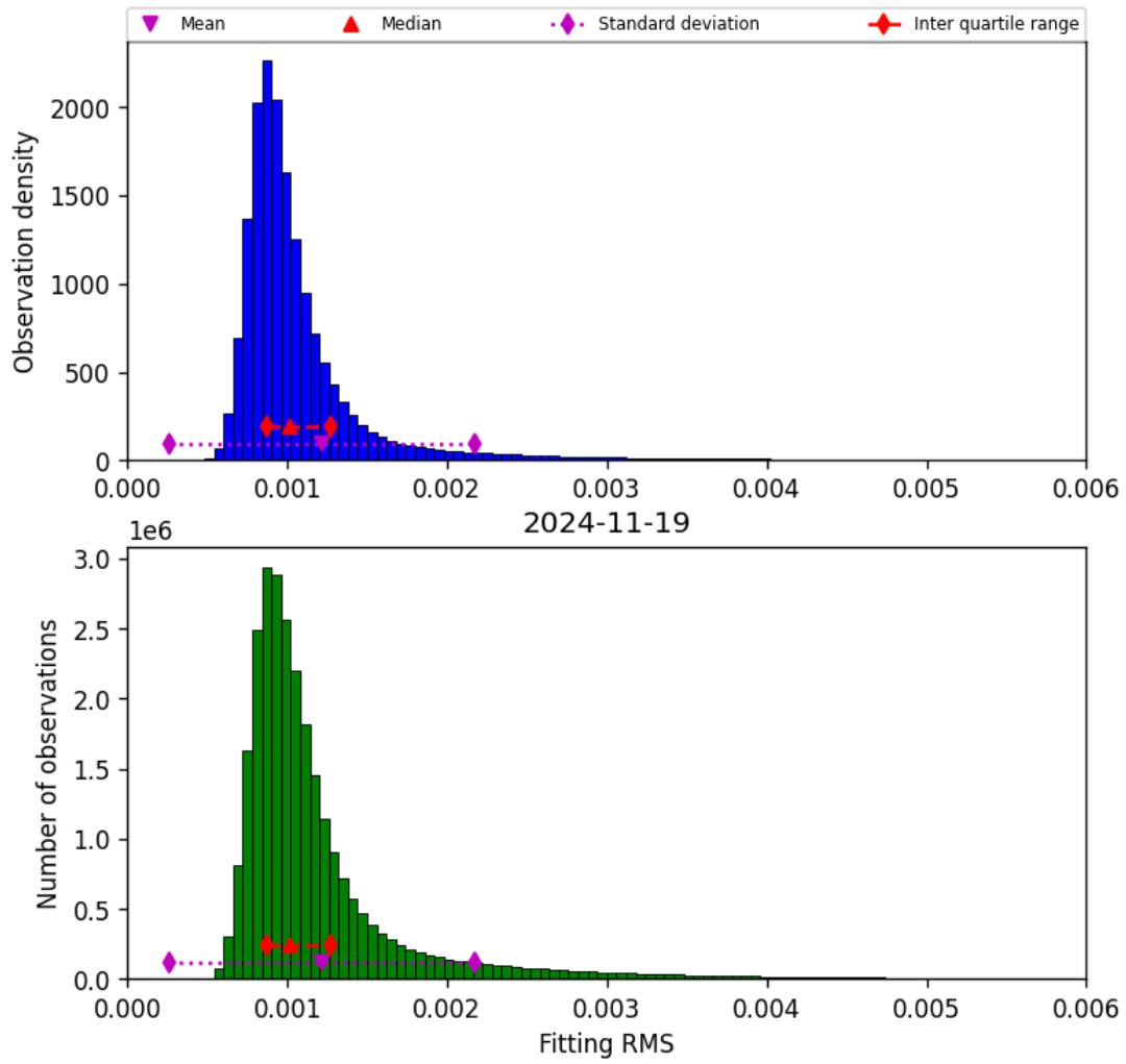
Figure 23: Histogram of “Fitting RMS” for 2024-11-18 to 2024-11-20
