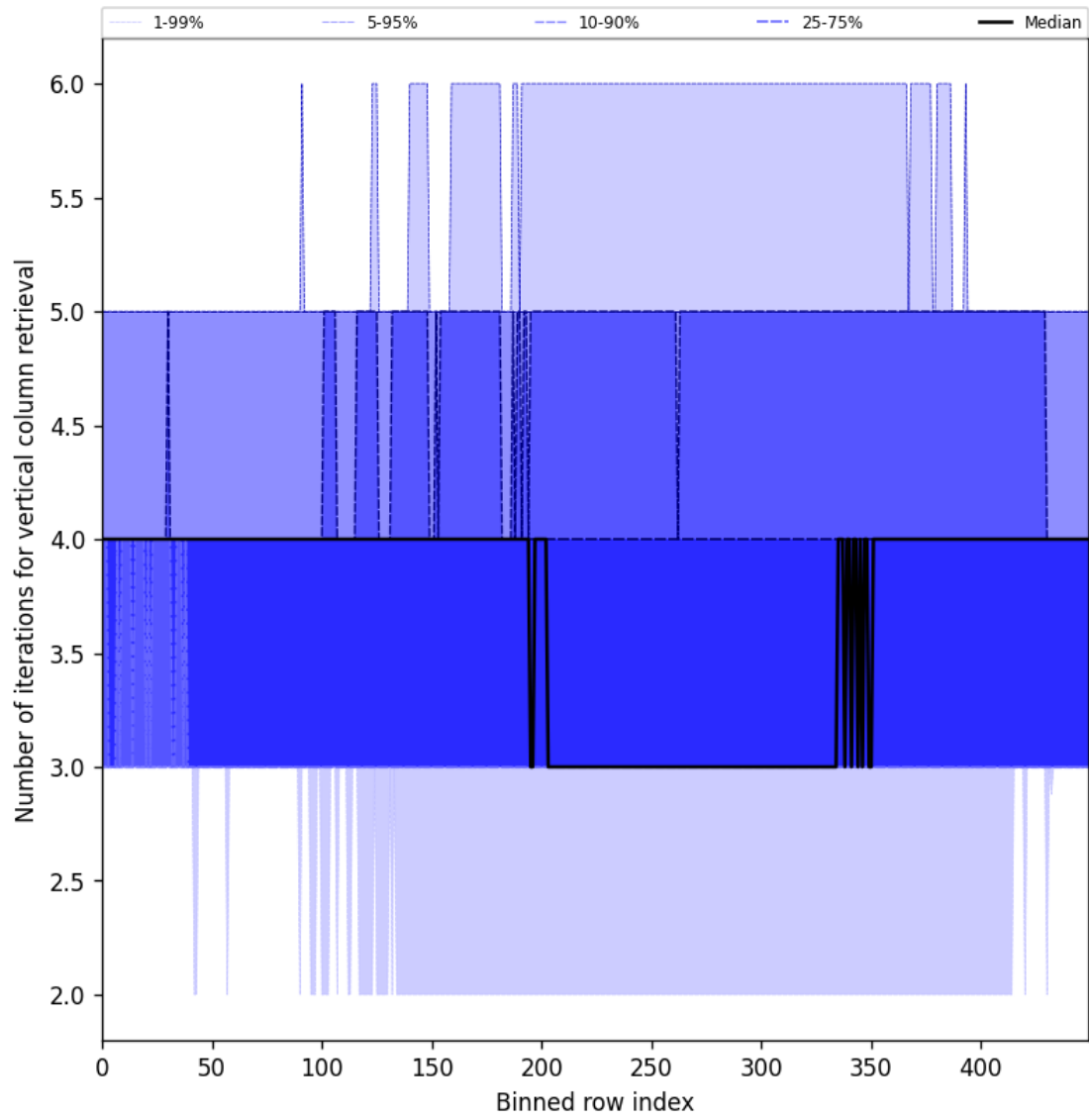
Figure 33: Along track statistics of “Number of iterations for vertical column retrieval” for 2024-11-18 to 2024-11-20
