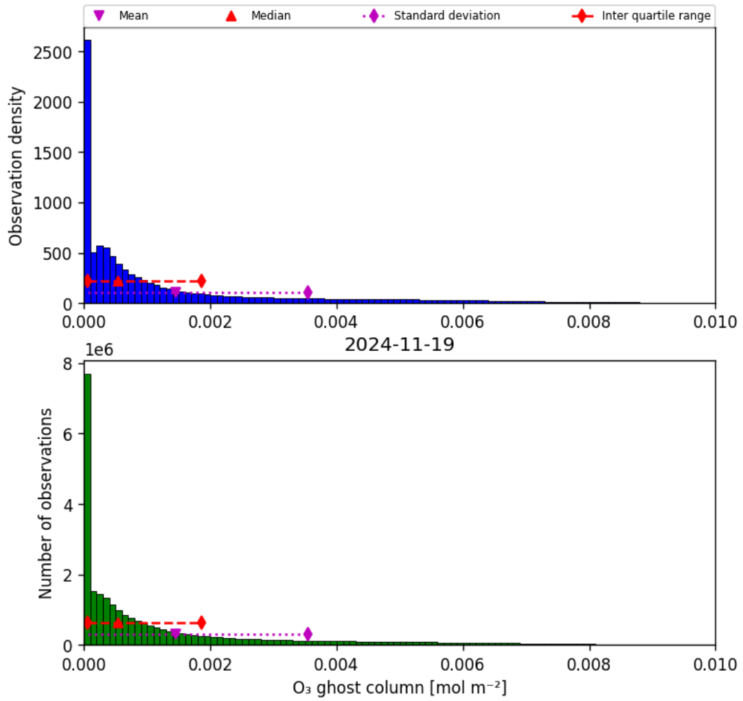
Figure 25: Histogram of “O 3 ghost column” for 2024-11-18 to 2024-11-20
