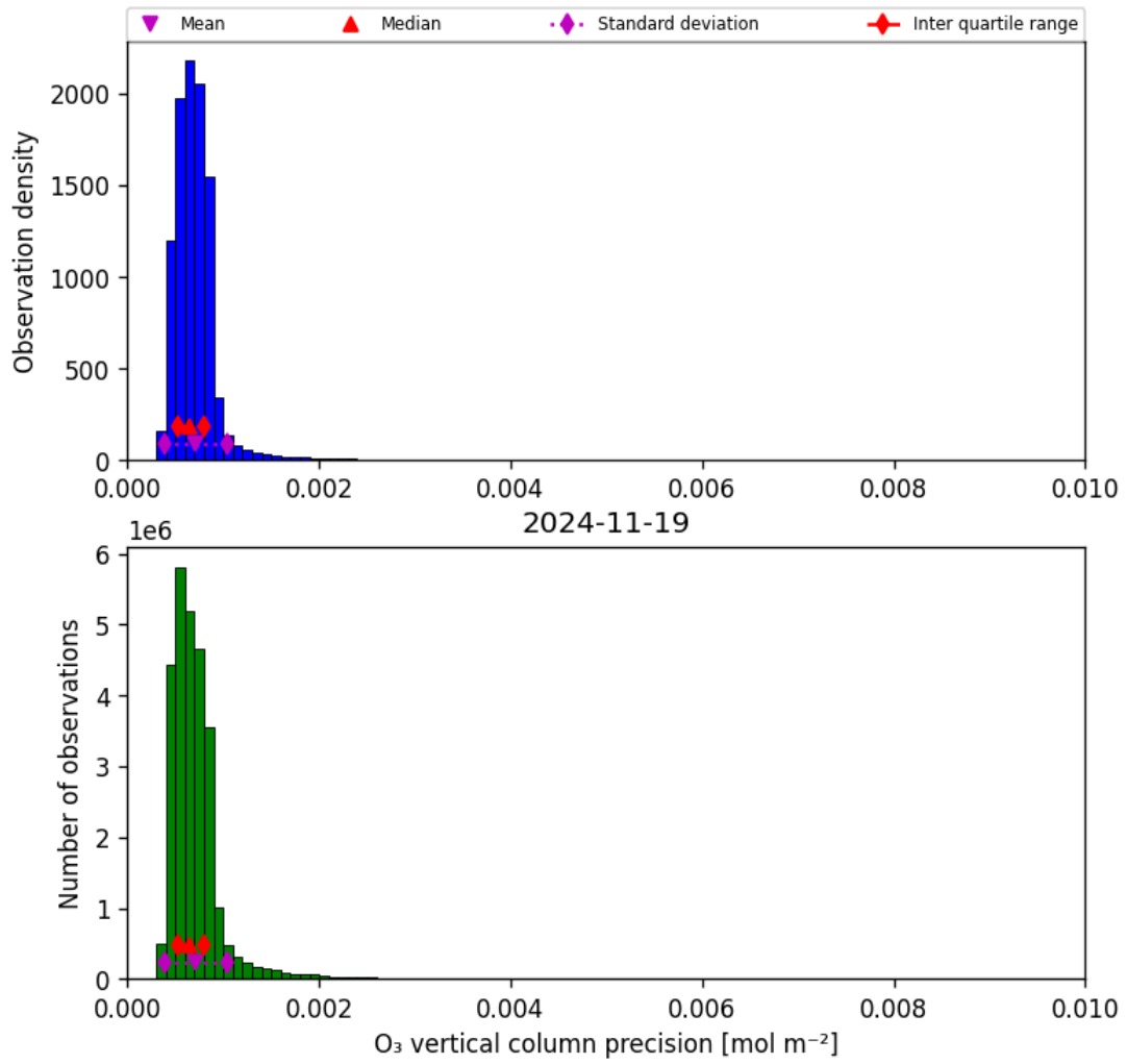
Figure 22: Histogram of “O 3 vertical column precision” for 2024-11-18 to 2024-11-20
