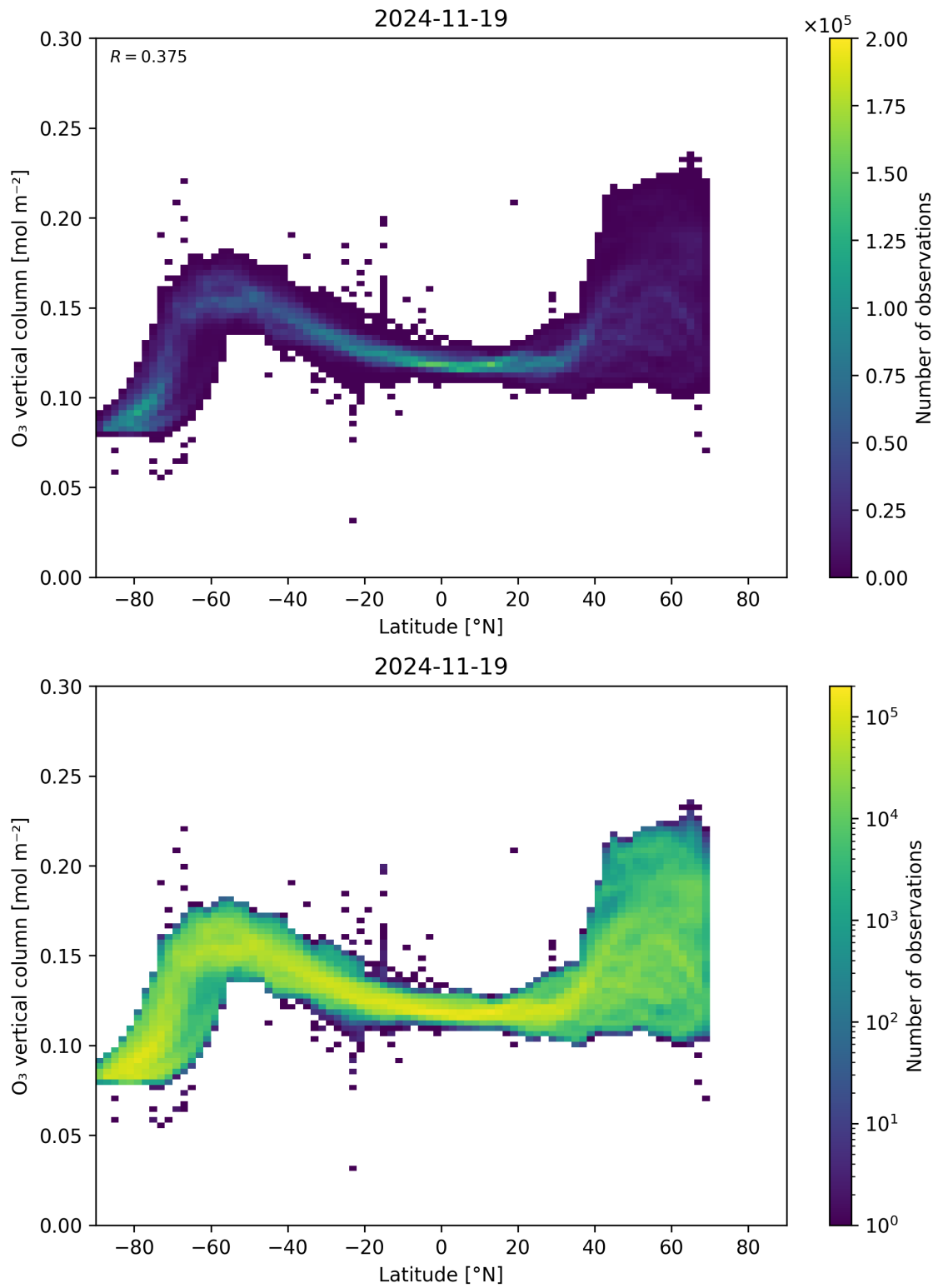
Figure 36: Scatter density plot of “Latitude” against “O 3 vertical column” for 2024-11-18 to 2024-11-20.
