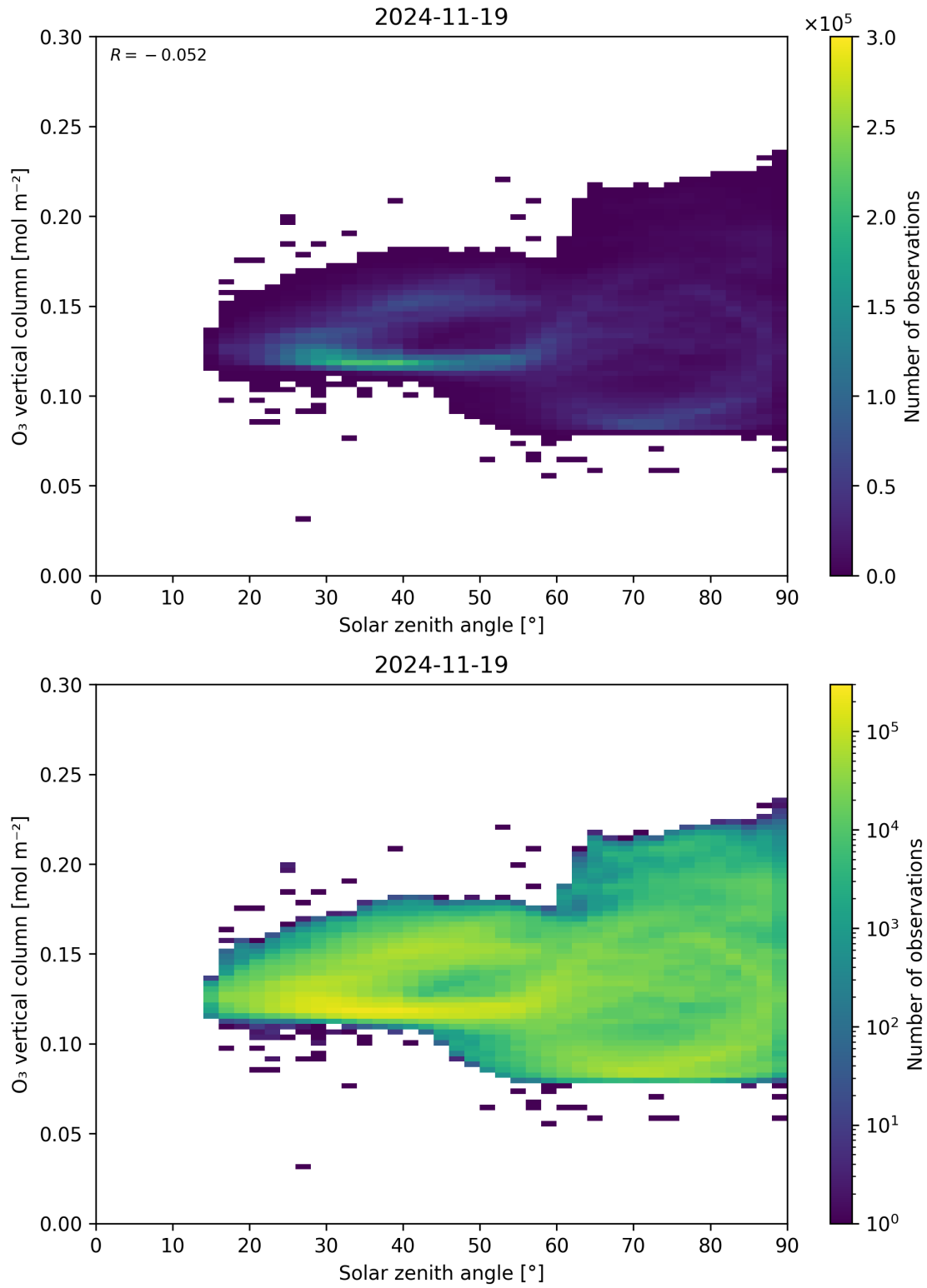
Figure 47: Scatter density plot of “Solar zenith angle” against “O 3 vertical column” for 2024-11-18 to 2024-11-20.
