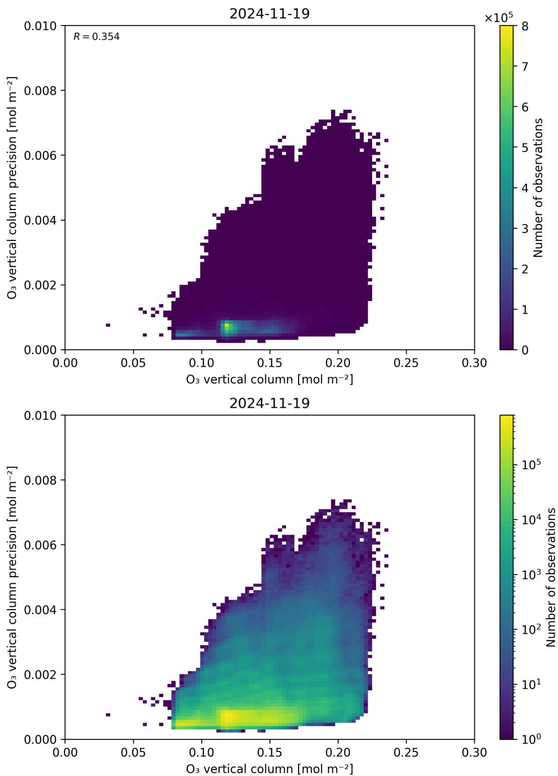
Figure 41: Scatter density plot of “O 3 vertical column” against “O 3 vertical column precision” for 2024-11-18 to 2024-11-20.
