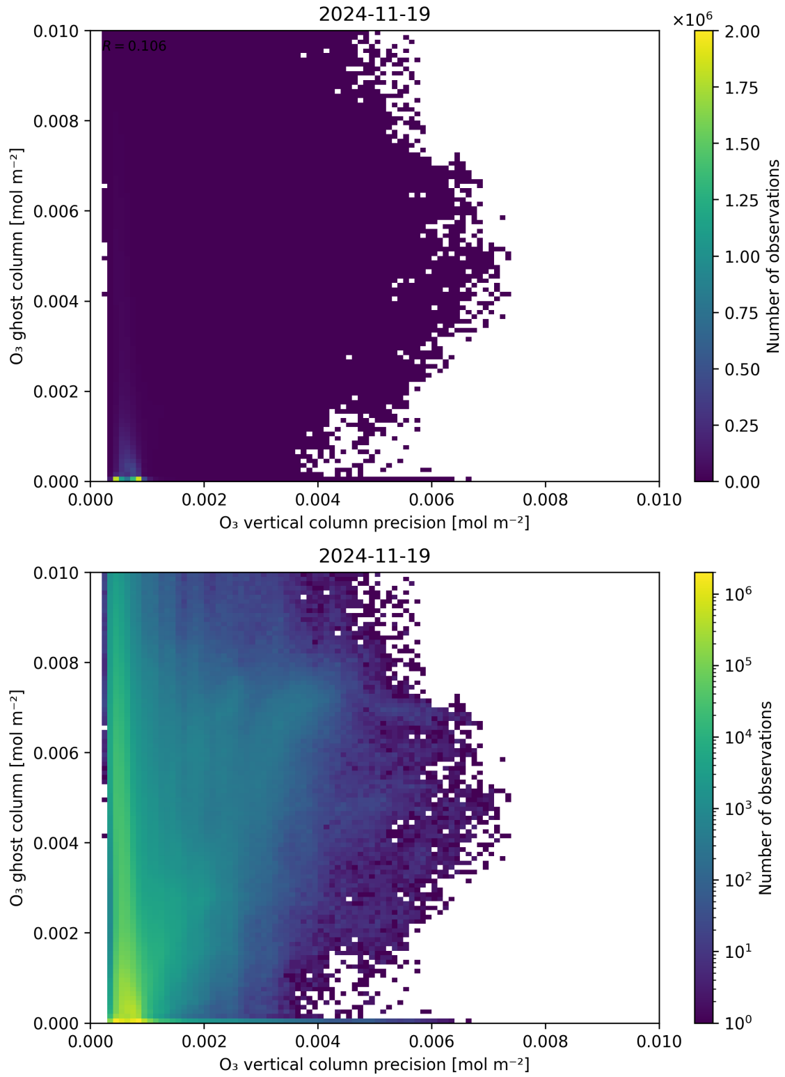
Figure 43: Scatter density plot of “ \text{O}_3 vertical column precision” against “ \text{O}_3 ghost column” for 2024-11-18 to 2024-11-20.
