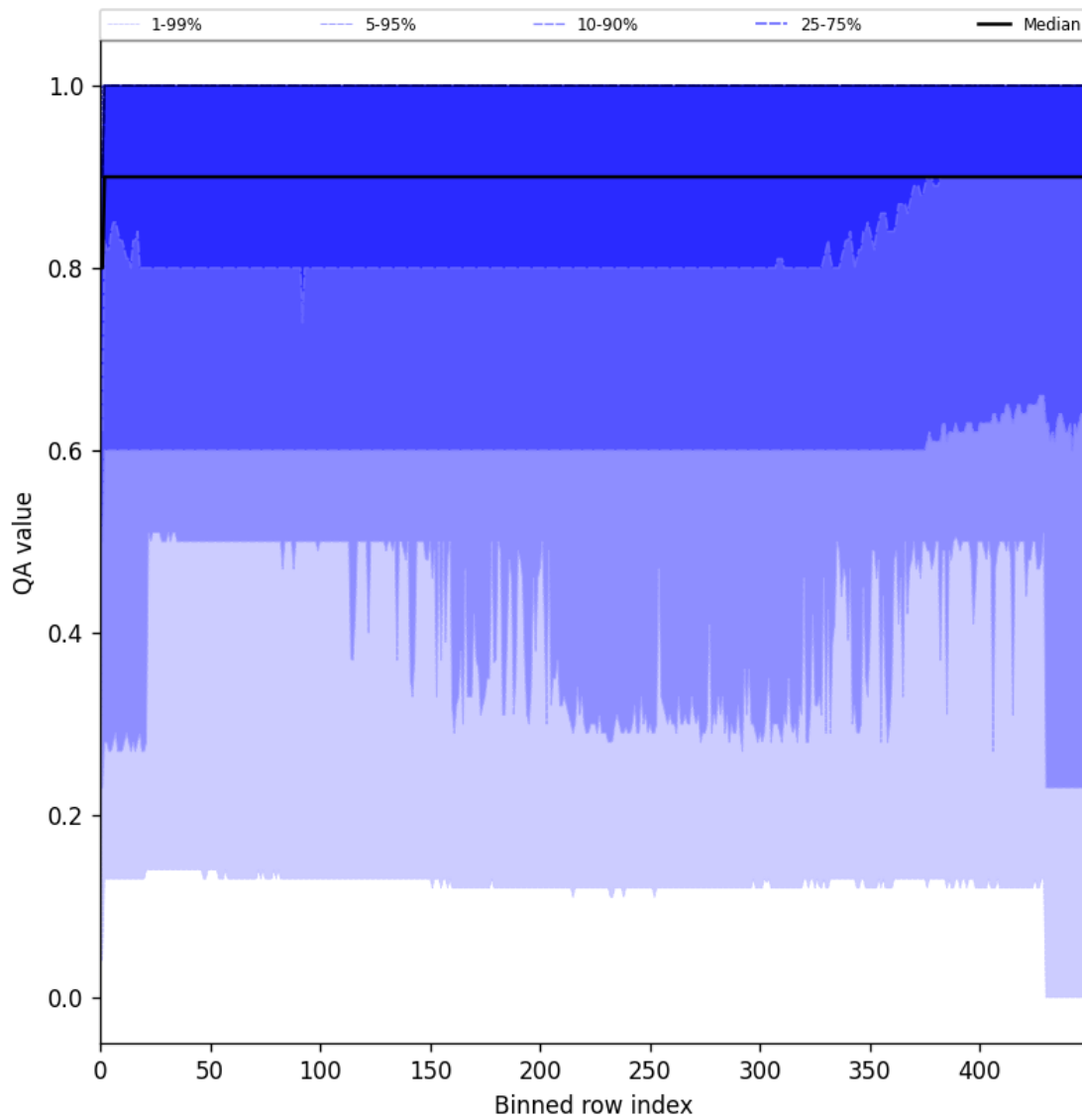
Figure 27: Along track statistics of “QA value” for 2024-11-18 to 2024-11-20
