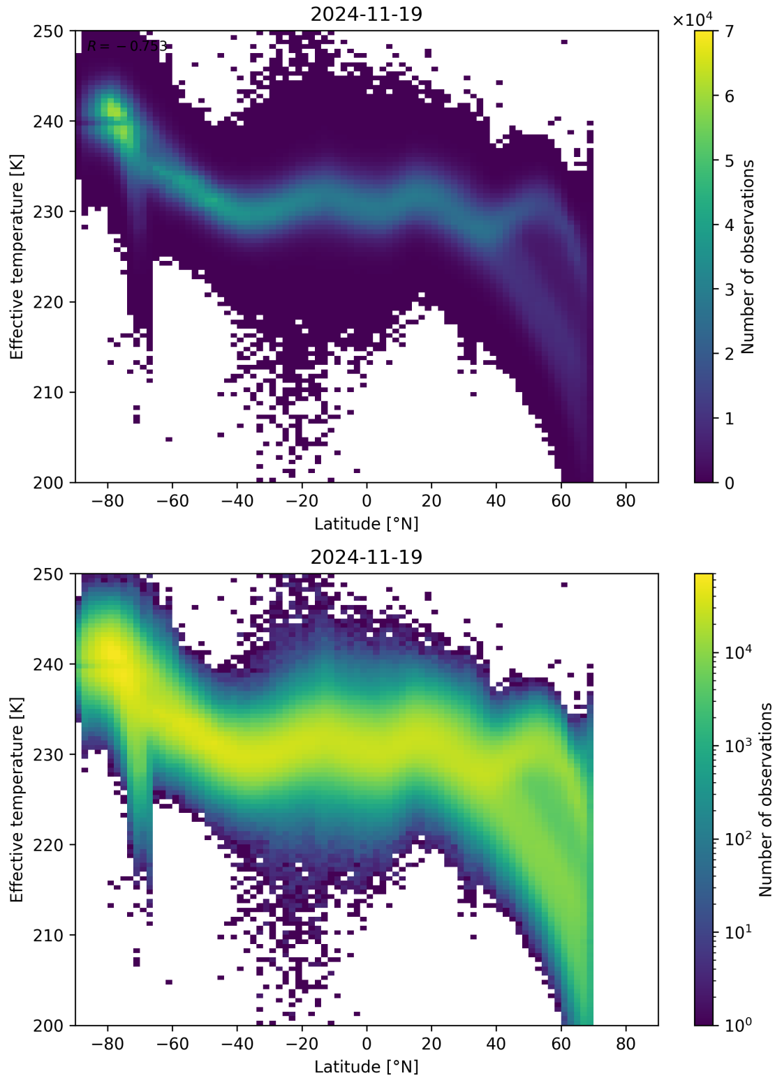
Figure 34: Scatter density plot of “Latitude” against “Effective temperature” for 2024-11-18 to 2024-11-20.
