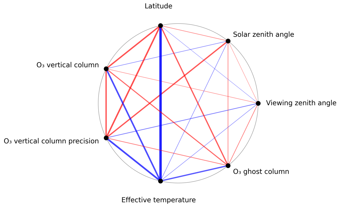
Figure 1: Map of correlation graph for 2024-11-18 to 2024-11-20.
