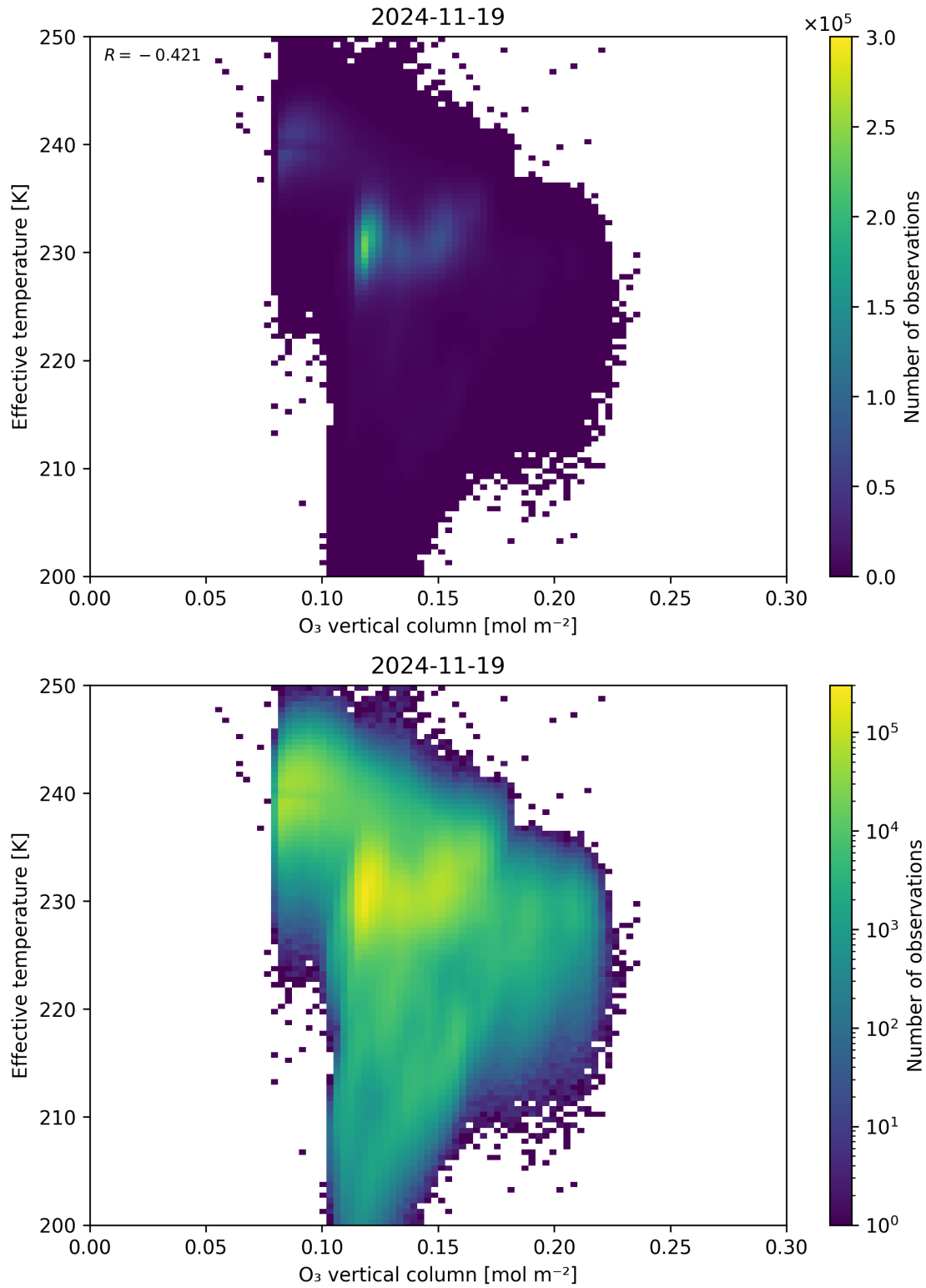
Figure 39: Scatter density plot of “O 3 vertical column” against “Effective temperature” for 2024-11-18 to 2024-11-20.
