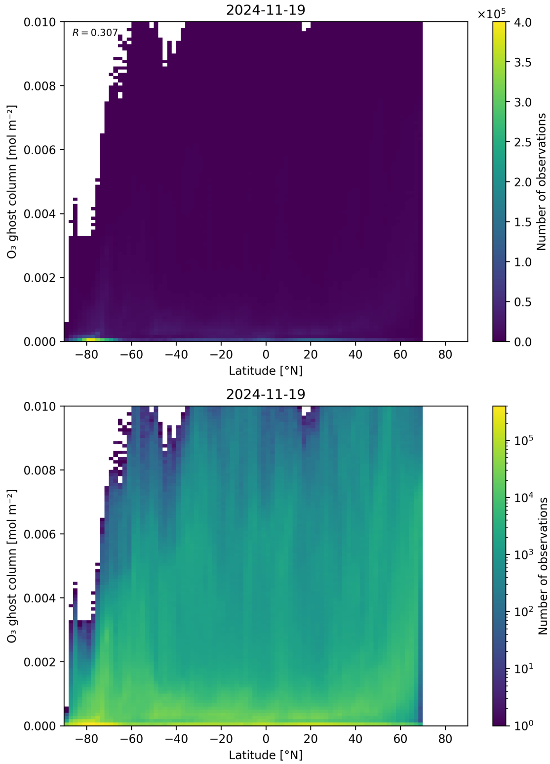
Figure 35: Scatter density plot of “Latitude” against “O 3 ghost column” for 2024-11-18 to 2024-11-20.
