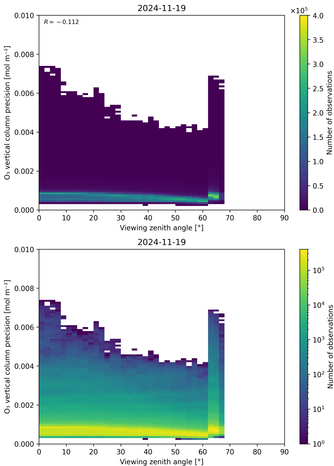
Figure 53: Scatter density plot of “Viewing zenith angle” against “O 3 vertical column precision” for 2024-11-18 to 2024-11-20.
