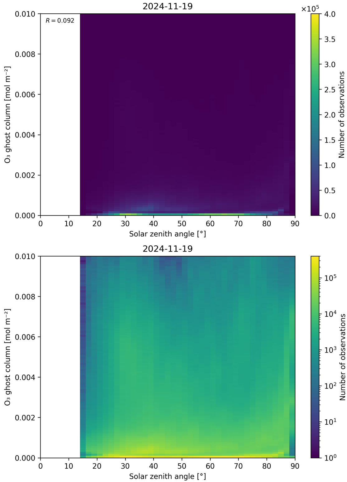
Figure 46: Scatter density plot of “Solar zenith angle” against “O 3 ghost column” for 2024-11-18 to 2024-11-20.
