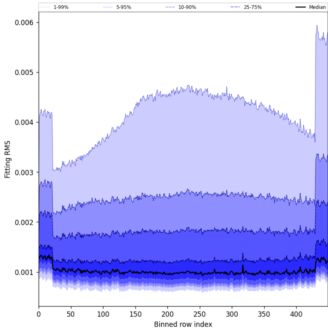
Figure 30: Along track statistics of “Fitting RMS” for 2024-11-18 to 2024-11-20
