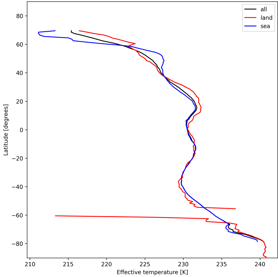
Figure 17: Zonal average of “Effective temperature” for 2024-11-18 to 2024-11-20.
