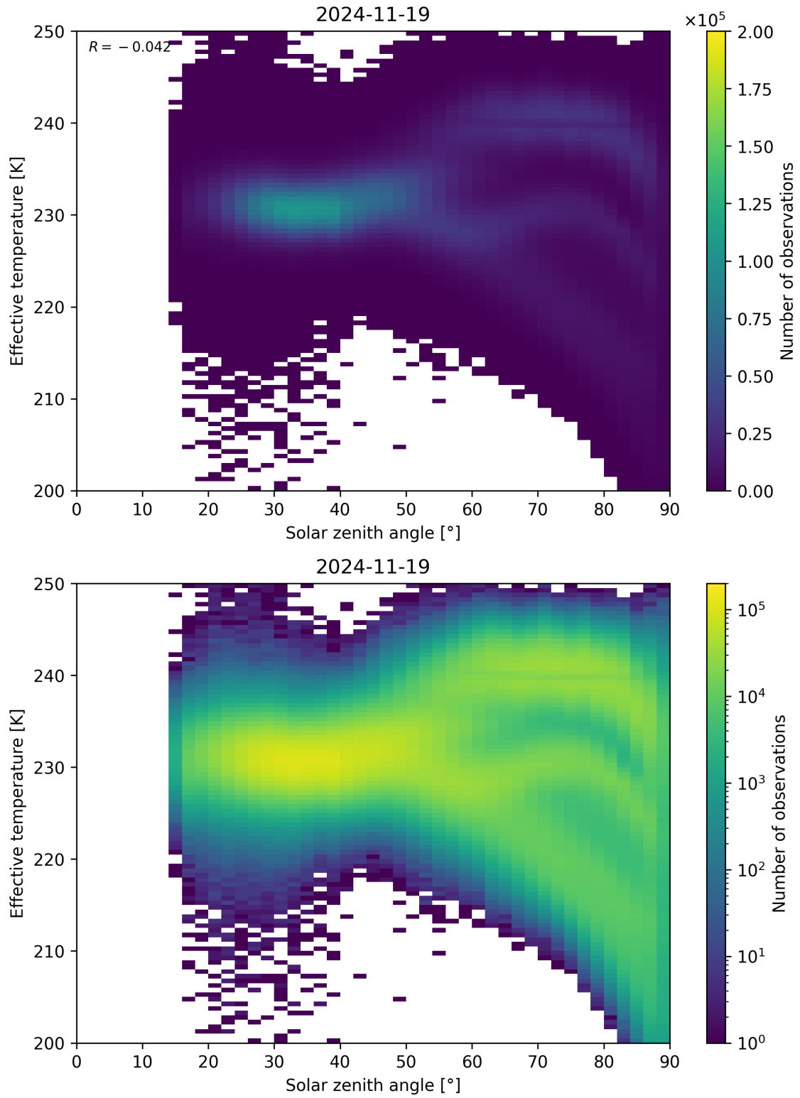
Figure 45: Scatter density plot of “Solar zenith angle” against “Effective temperature” for 2024-11-18 to 2024-11-20.
