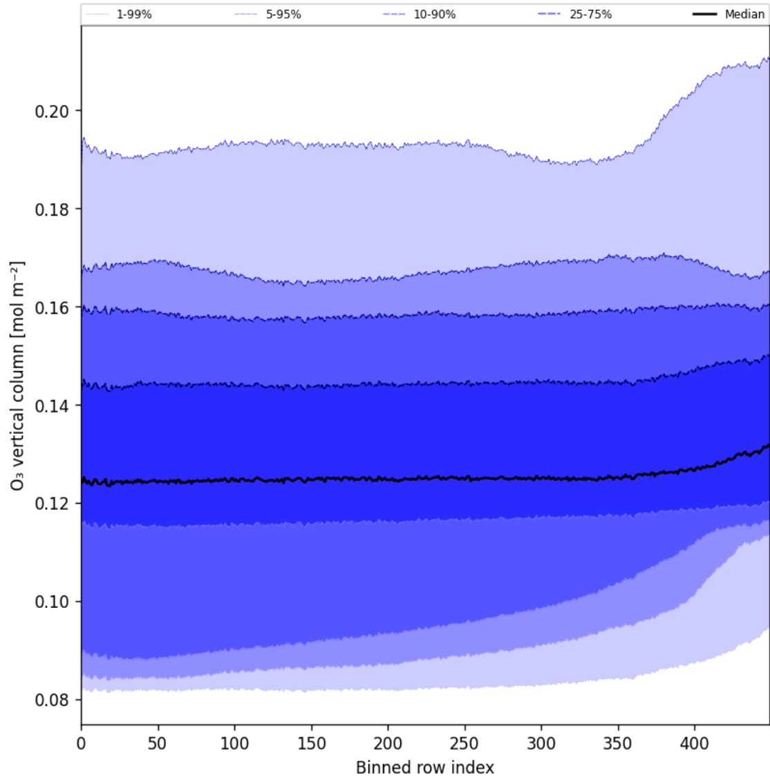
Figure 28: Along track statistics of “O 3 vertical column” for 2024-11-18 to 2024-11-20
