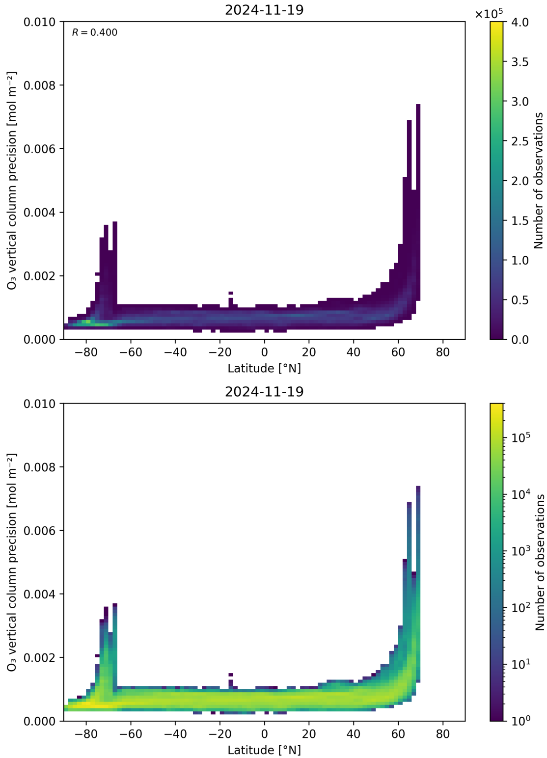
Figure 37: Scatter density plot of “Latitude” against “O 3 vertical column precision” for 2024-11-18 to 2024-11-20.
