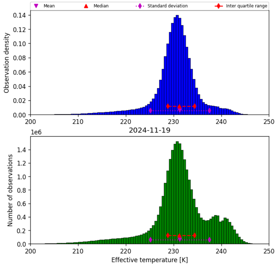
Figure 24: Histogram of “Effective temperature” for 2024-11-18 to 2024-11-20
