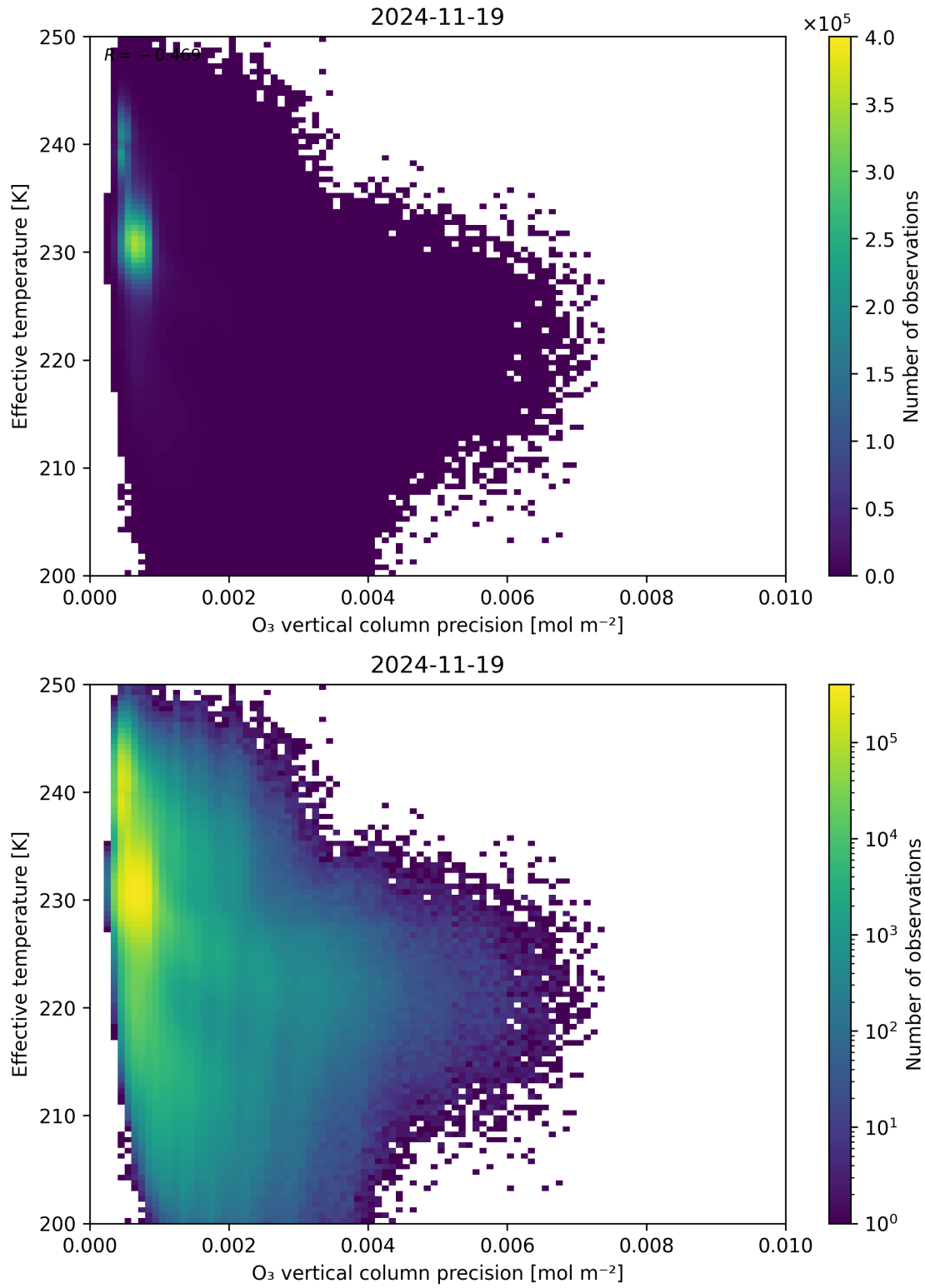
Figure 42: Scatter density plot of “O 3 vertical column precision” against “Effective temperature” for 2024-11-18 to 2024-11-20.
