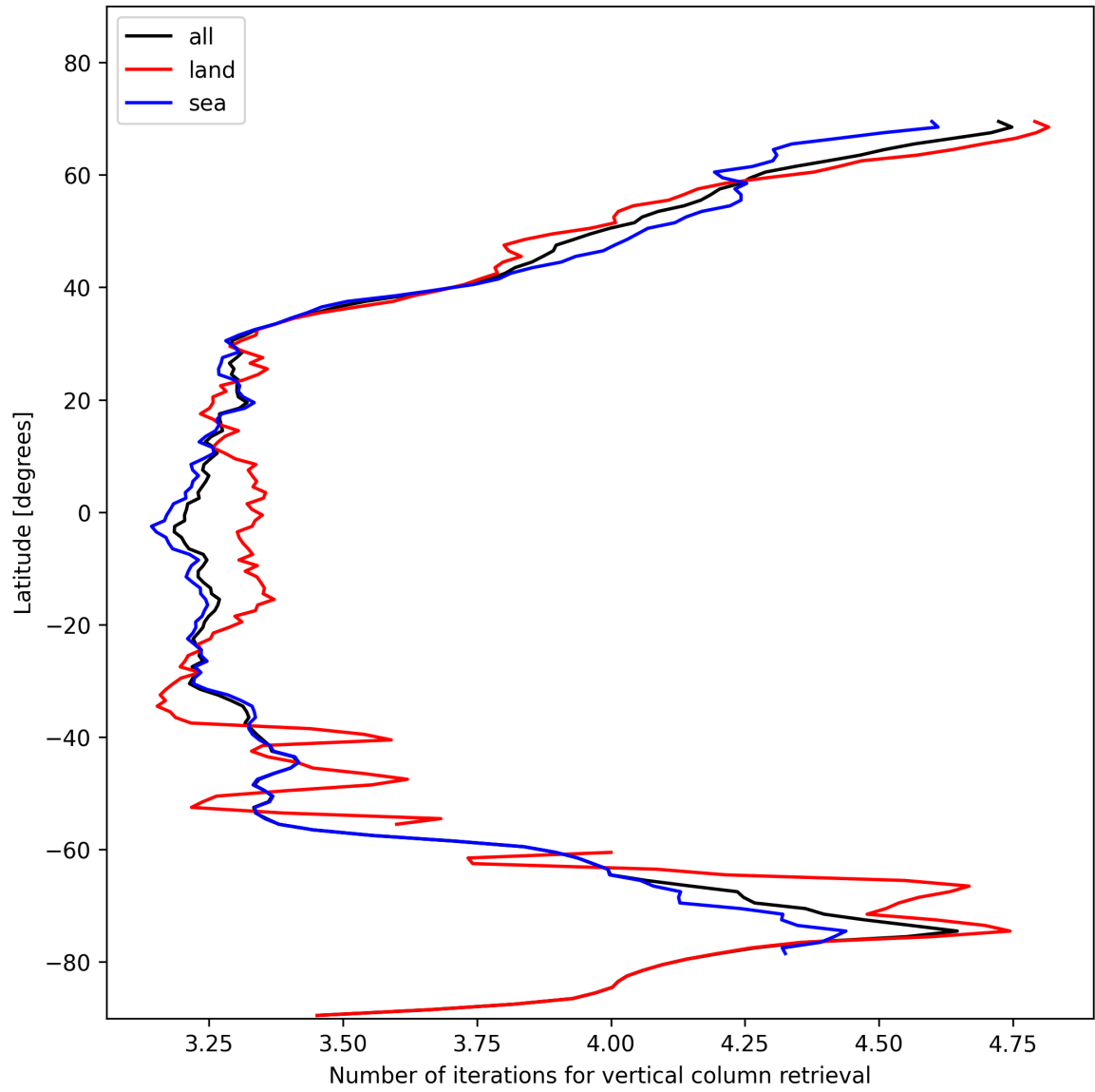
Figure 19: Zonal average of “Number of iterations for vertical column retrieval” for 2024-11-18 to 2024-11-20.
