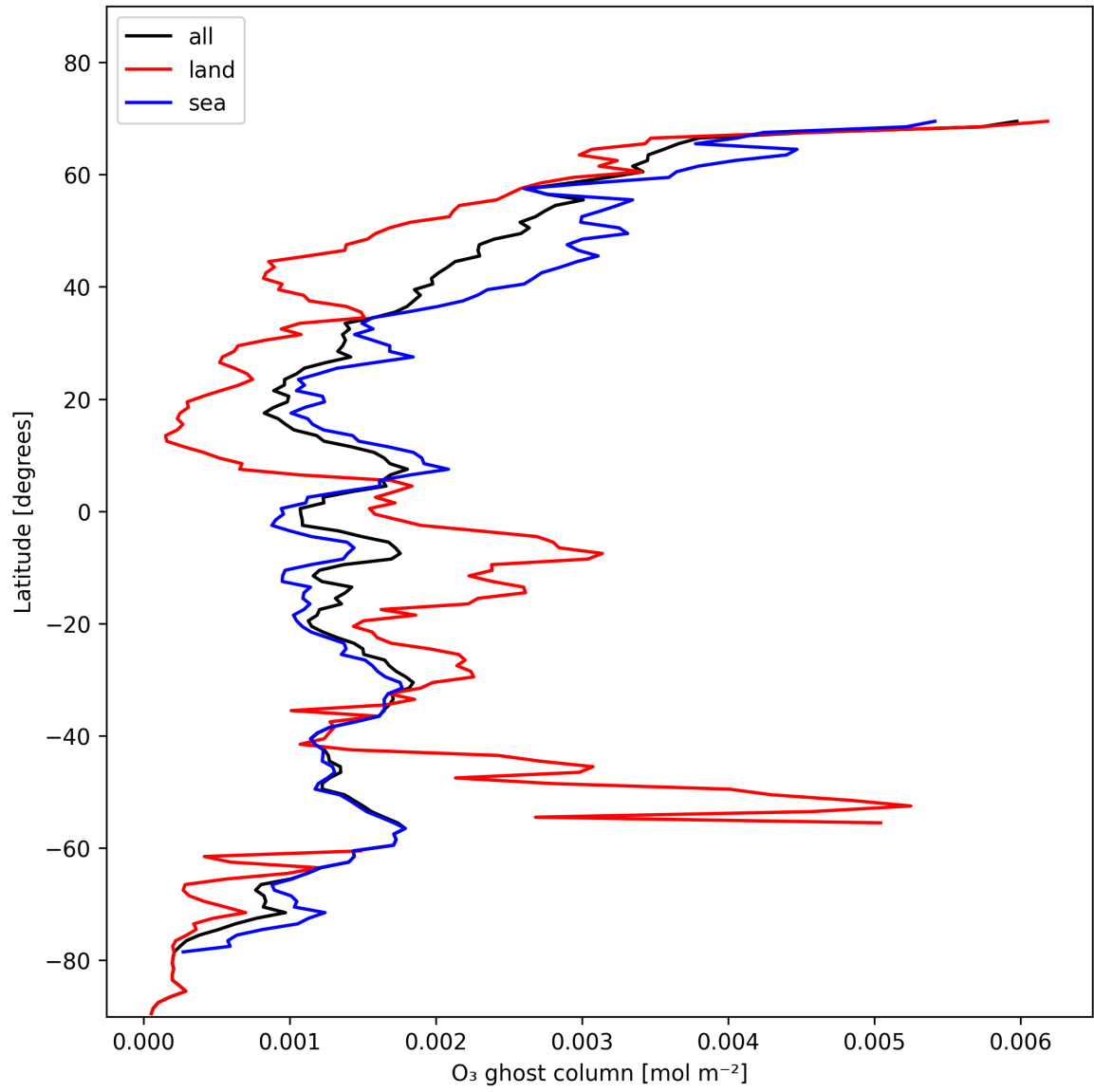
Figure 18: Zonal average of "O 3 ghost column" for 2024-11-18 to 2024-11-20.
