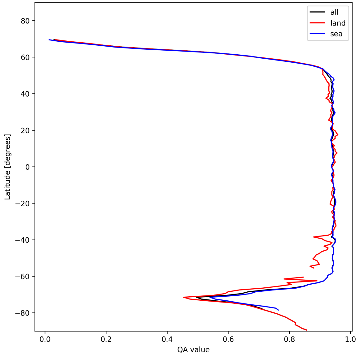
Figure 13: Zonal average of “QA value” for 2024-11-18 to 2024-11-20.
