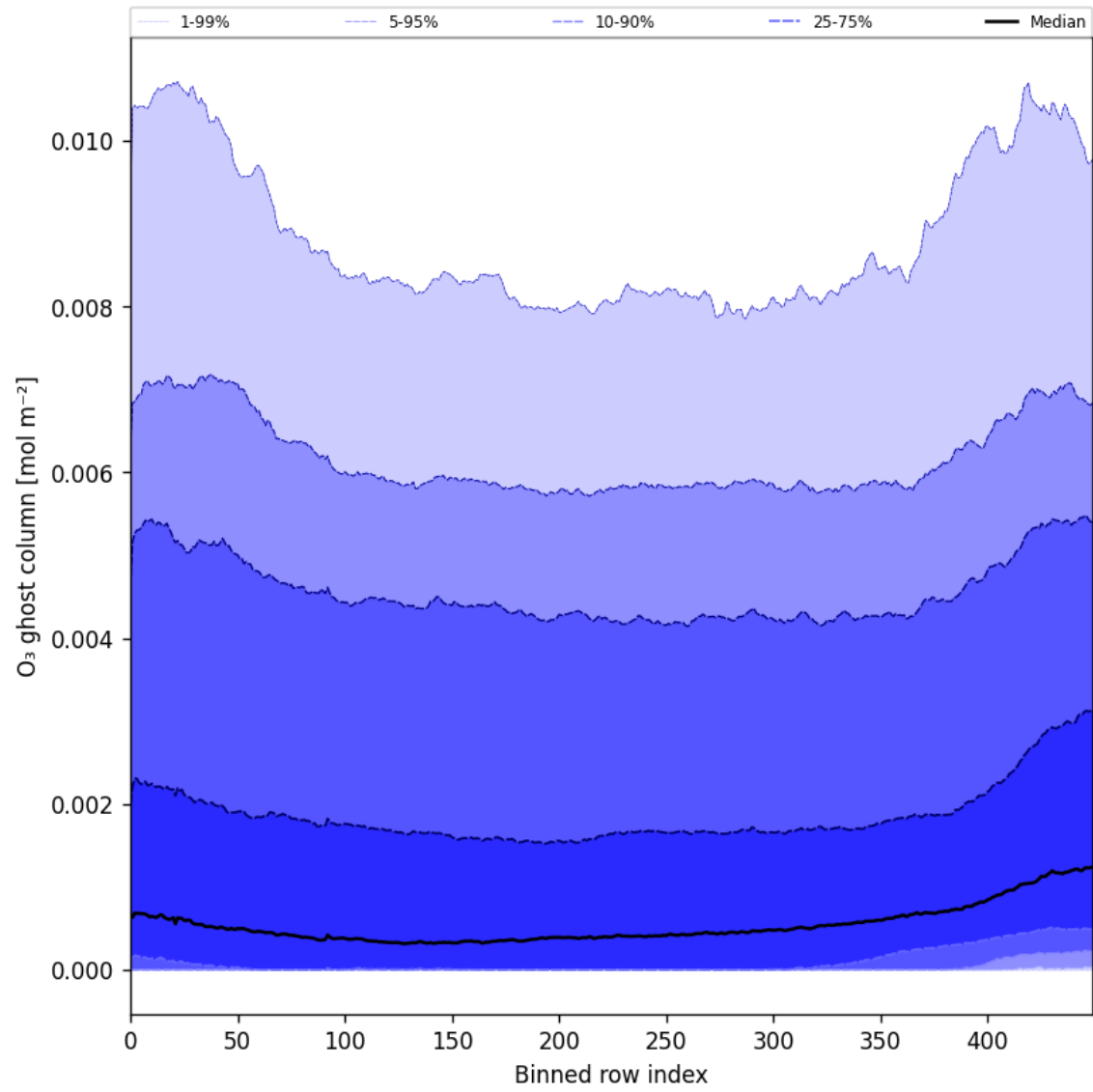
Figure 32: Along track statistics of “O 3 ghost column” for 2024-11-18 to 2024-11-20
