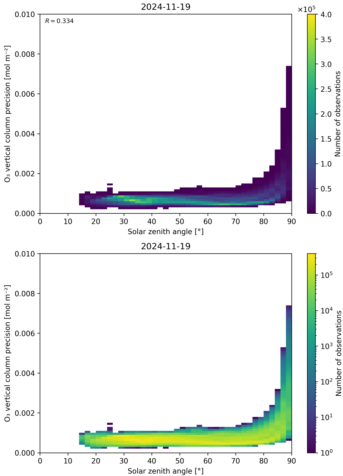
Figure 48: Scatter density plot of “Solar zenith angle” against “O 3 vertical column precision” for 2024-11-18 to 2024-11-20.
