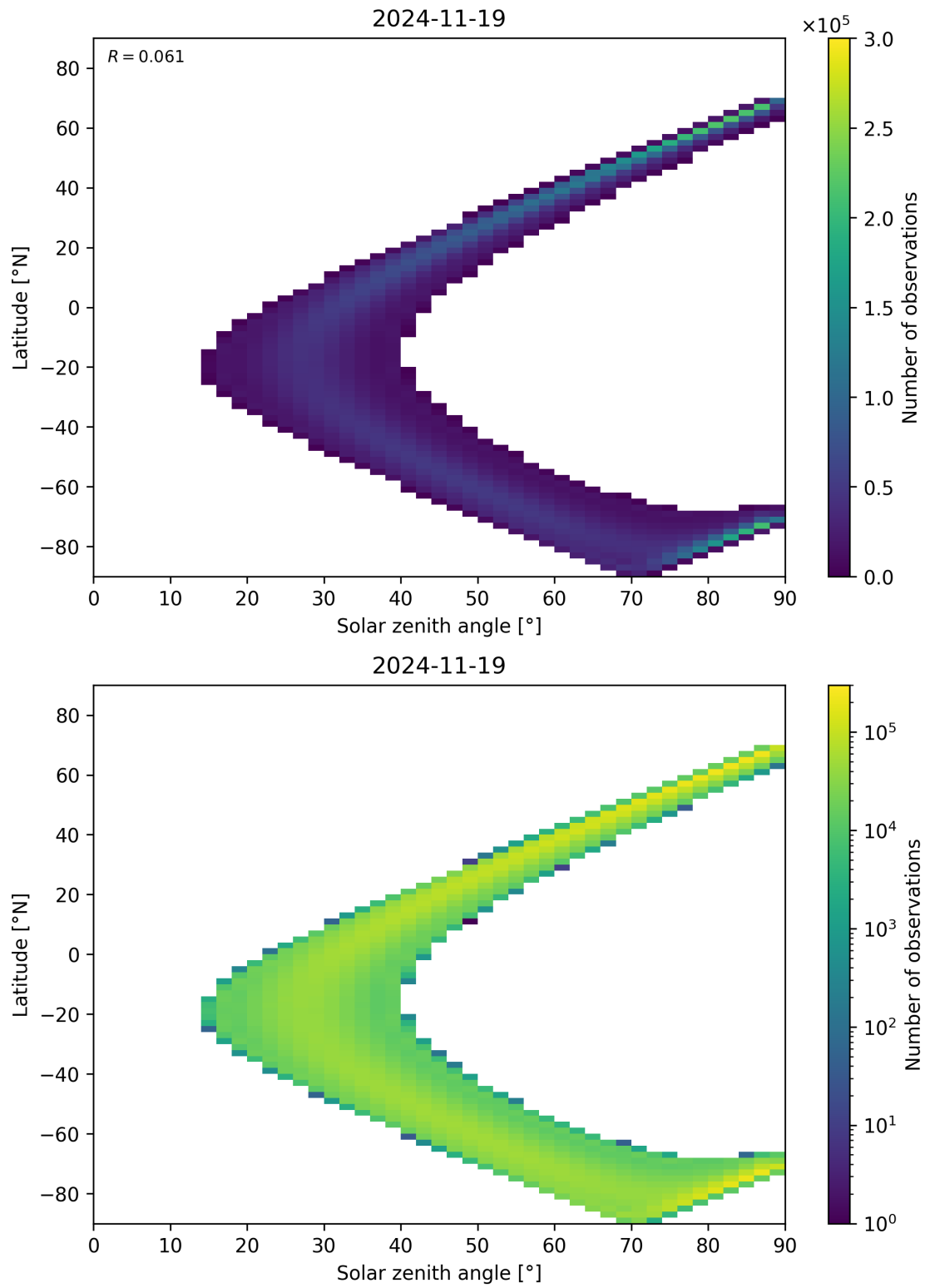
Figure 44: Scatter density plot of “Solar zenith angle” against “Latitude” for 2024-11-18 to 2024-11-20.
