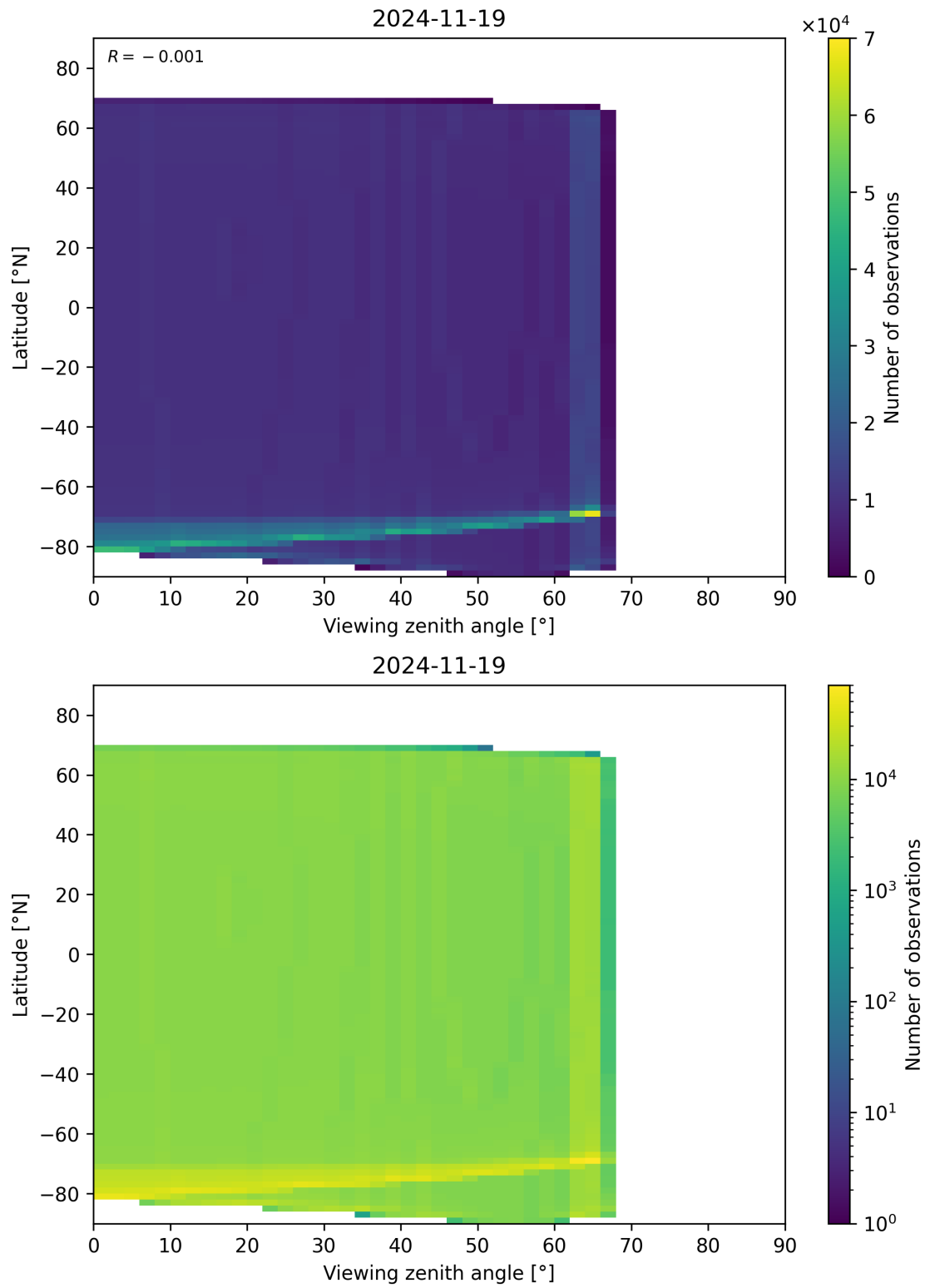
Figure 49: Scatter density plot of “Viewing zenith angle” against “Latitude” for 2024-11-18 to 2024-11-20.
