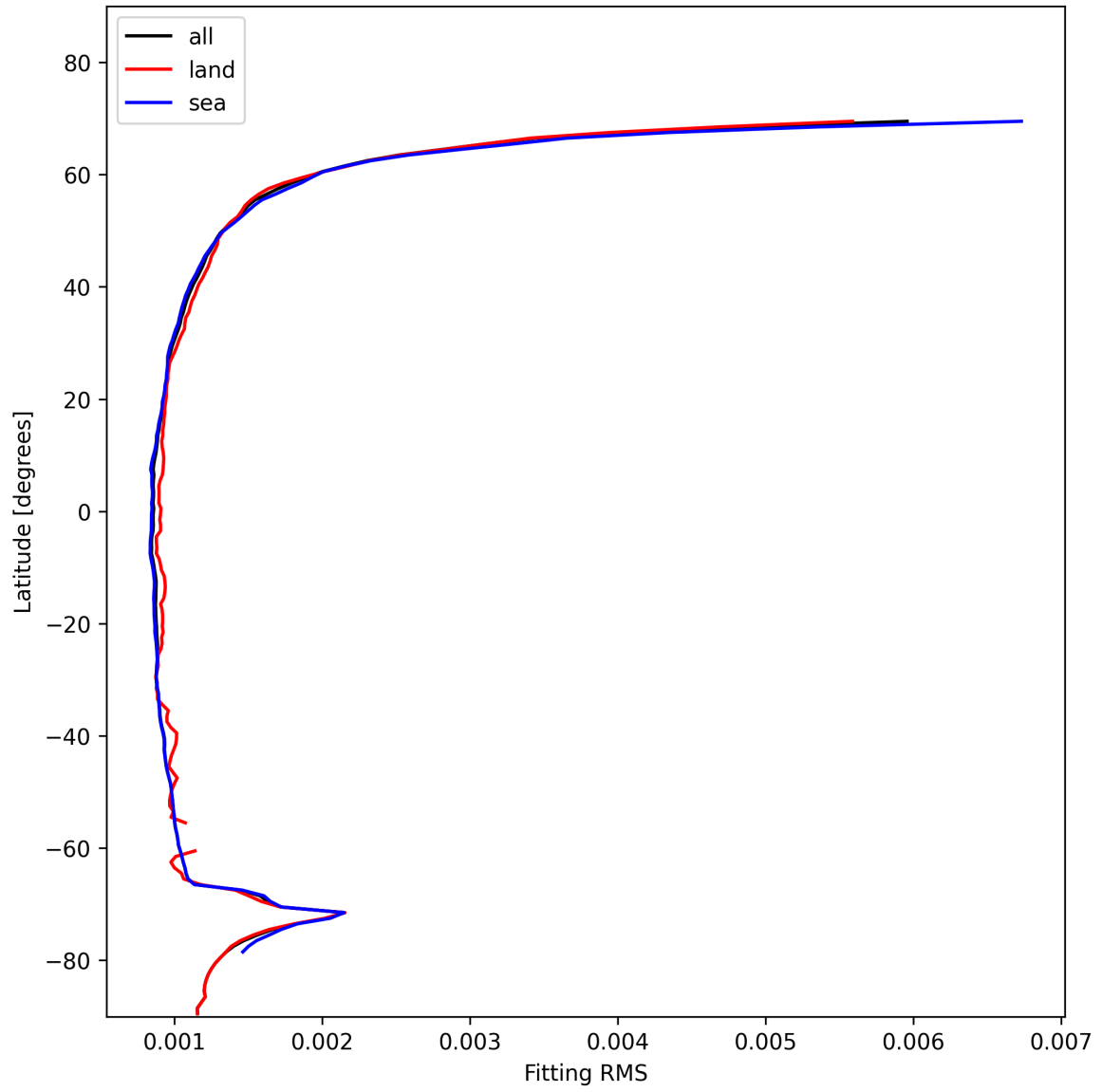
Figure 16: Zonal average of “Fitting RMS” for 2024-11-18 to 2024-11-20.
