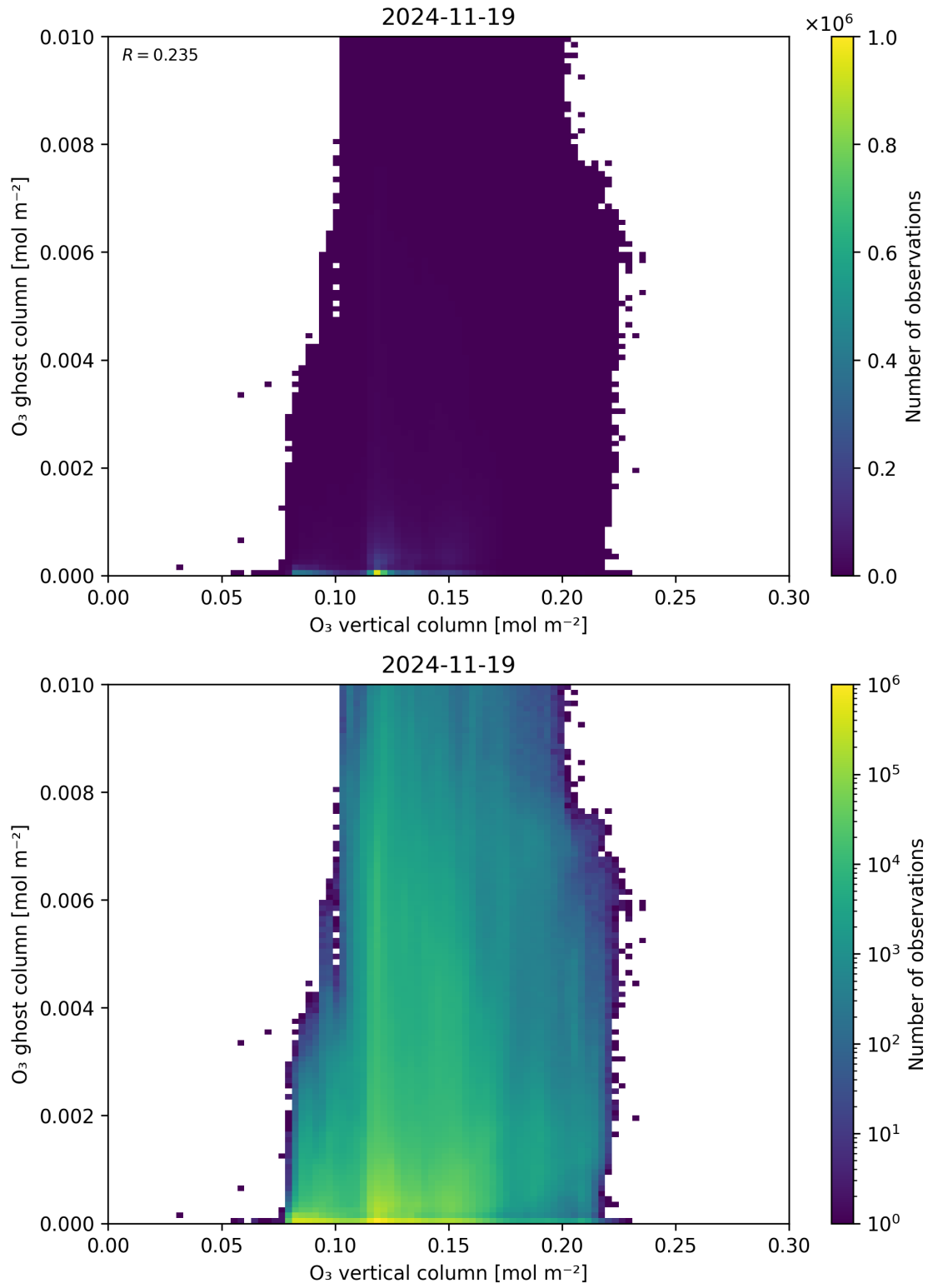
Figure 40: Scatter density plot of “O 3 vertical column” against “O 3 ghost column” for 2024-11-18 to 2024-11-20.
