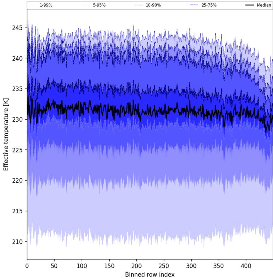
Figure 31: Along track statistics of “Effective temperature” for 2024-11-18 to 2024-11-20
