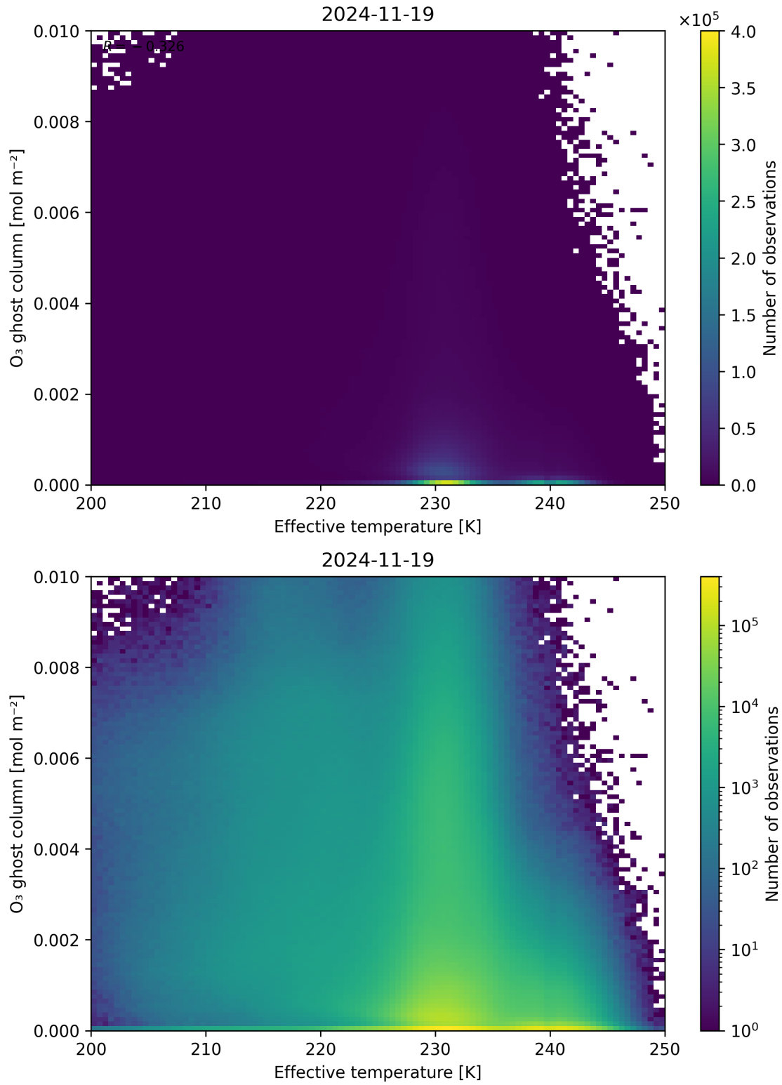
Figure 38: Scatter density plot of “Effective temperature” against “O 3 ghost column” for 2024-11-18 to 2024-11-20.
