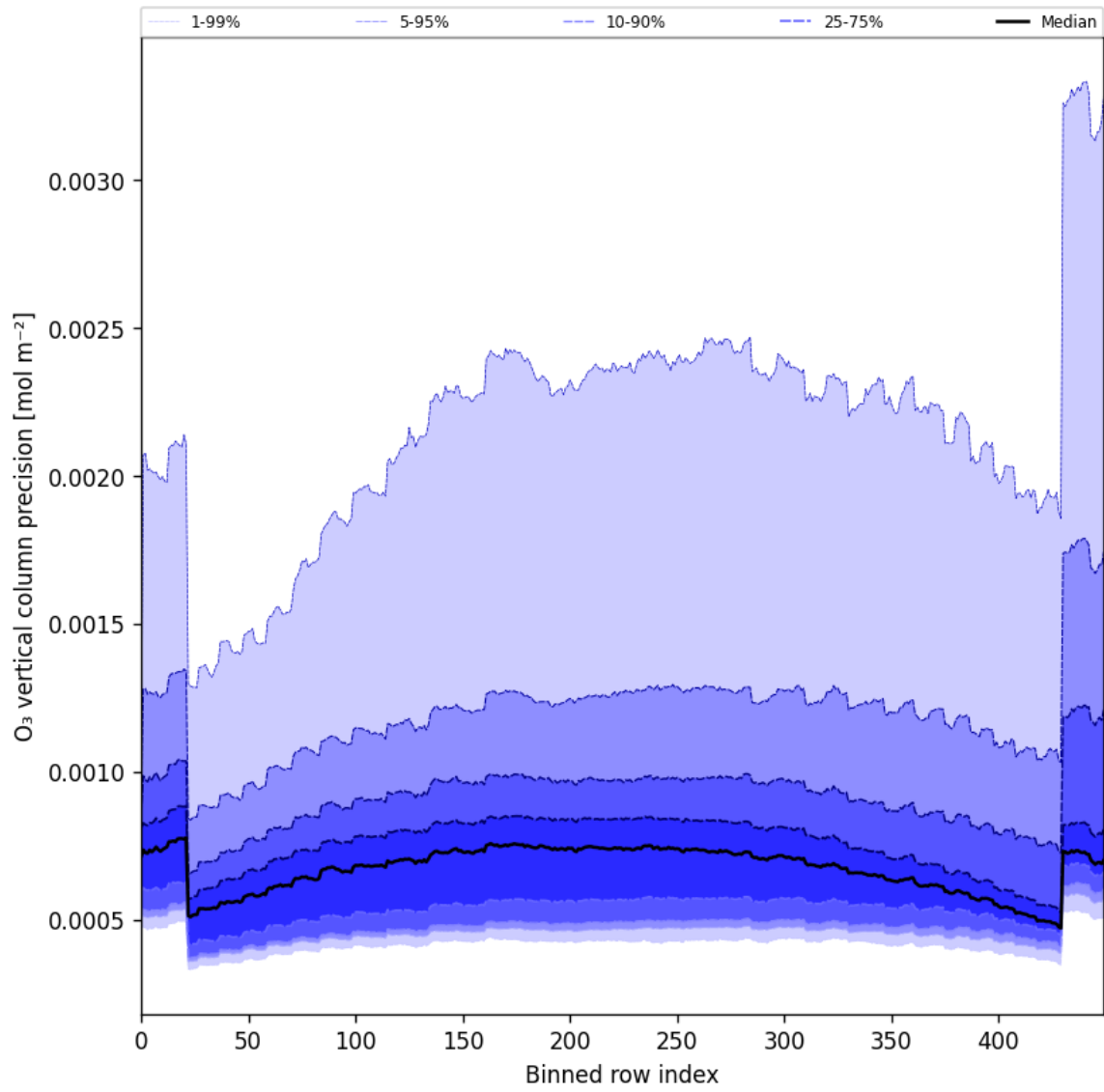
Figure 29: Along track statistics of “O 3 vertical column precision” for 2024-11-18 to 2024-11-20
