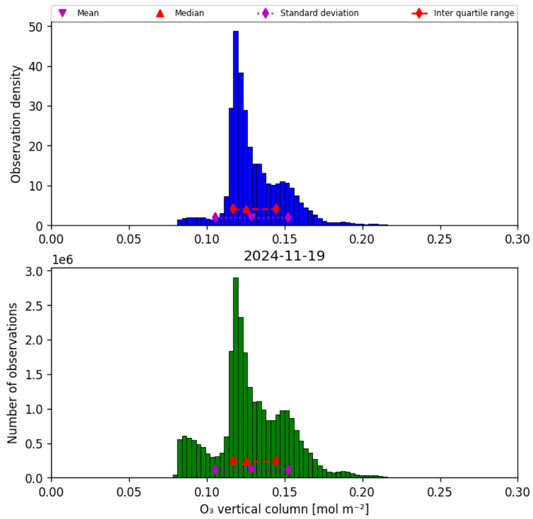
Figure 21: Histogram of “O 3 vertical column” for 2024-11-18 to 2024-11-20
