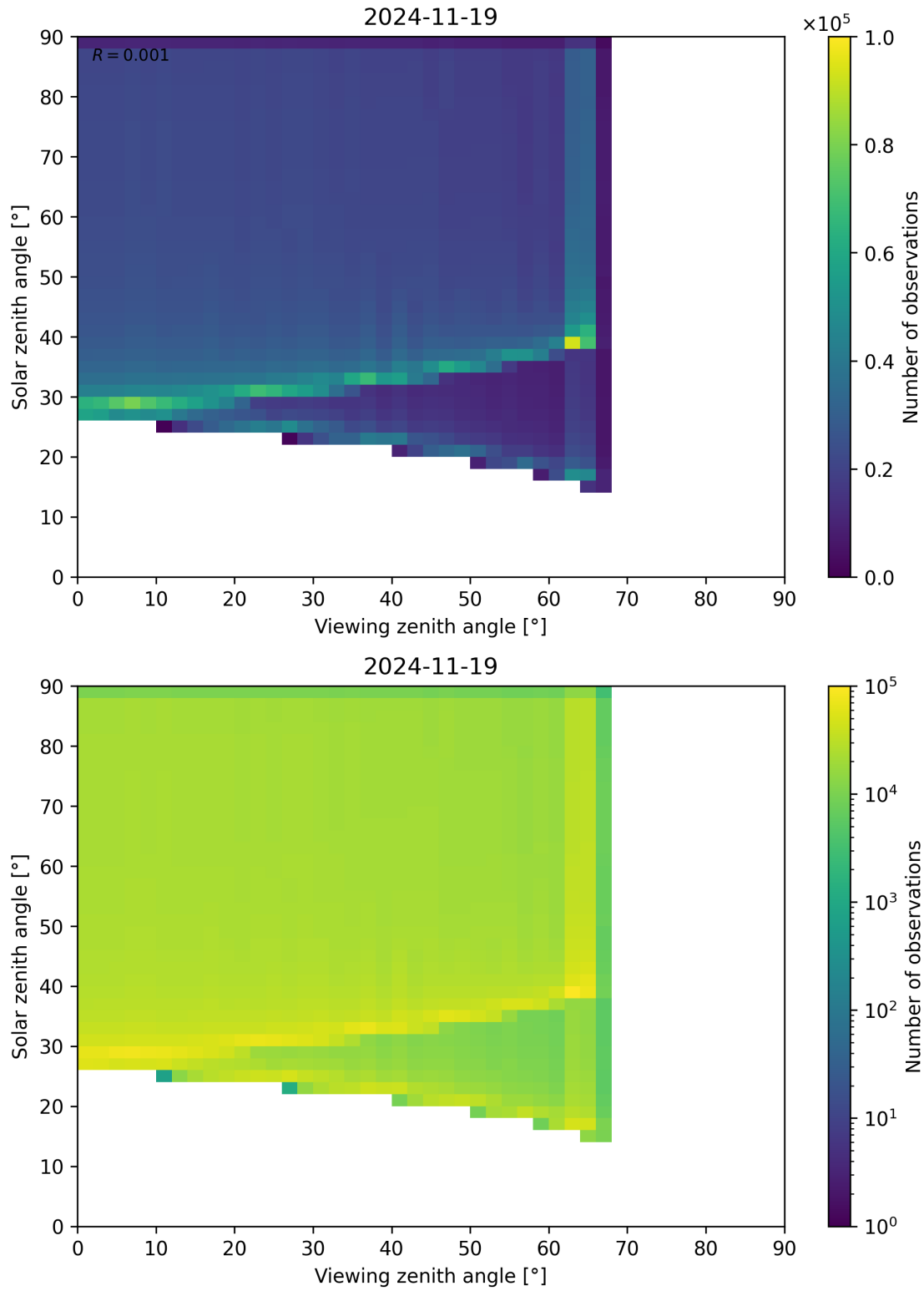
Figure 54: Scatter density plot of “Viewing zenith angle” against “Solar zenith angle” for 2024-11-18 to 2024-11-20.
