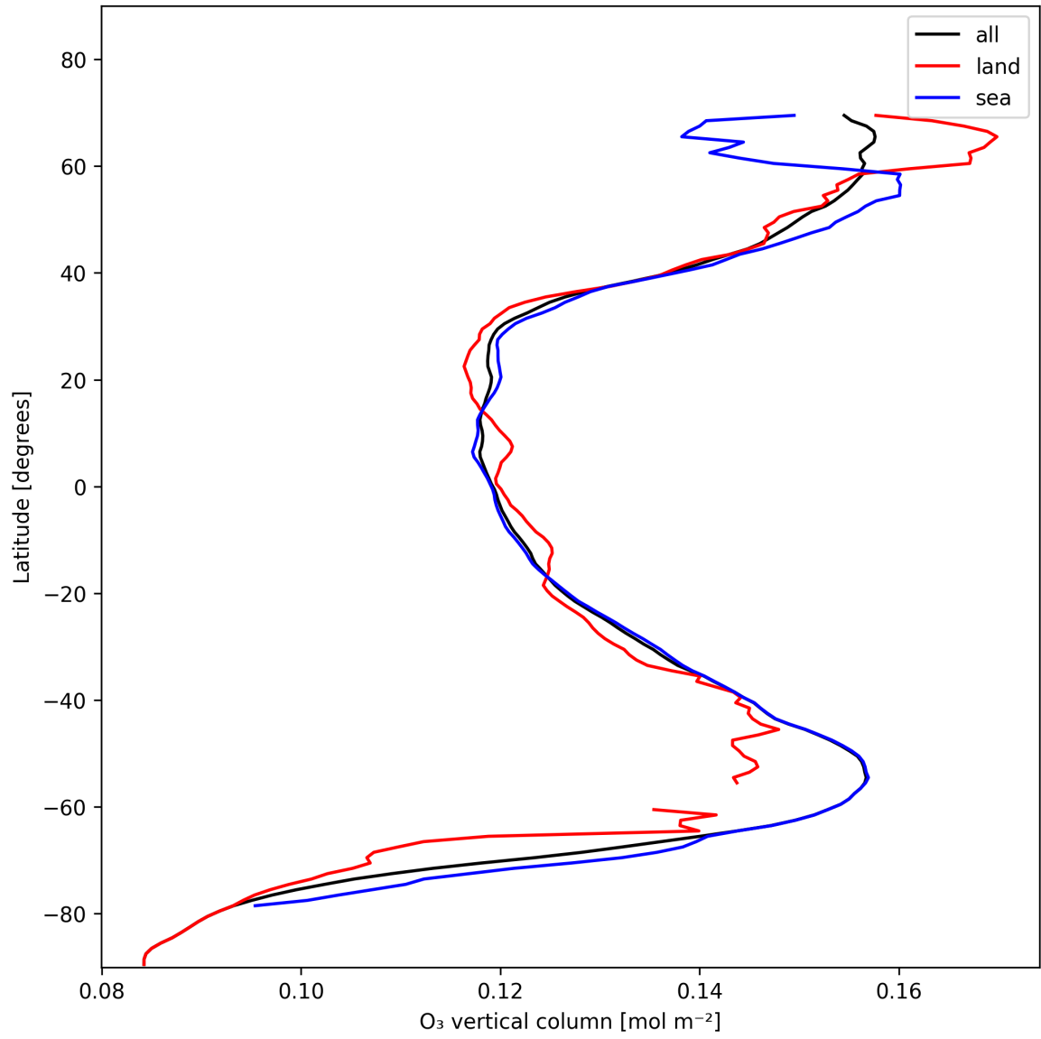
Figure 14: Zonal average of “O 3 vertical column” for 2024-11-18 to 2024-11-20.
