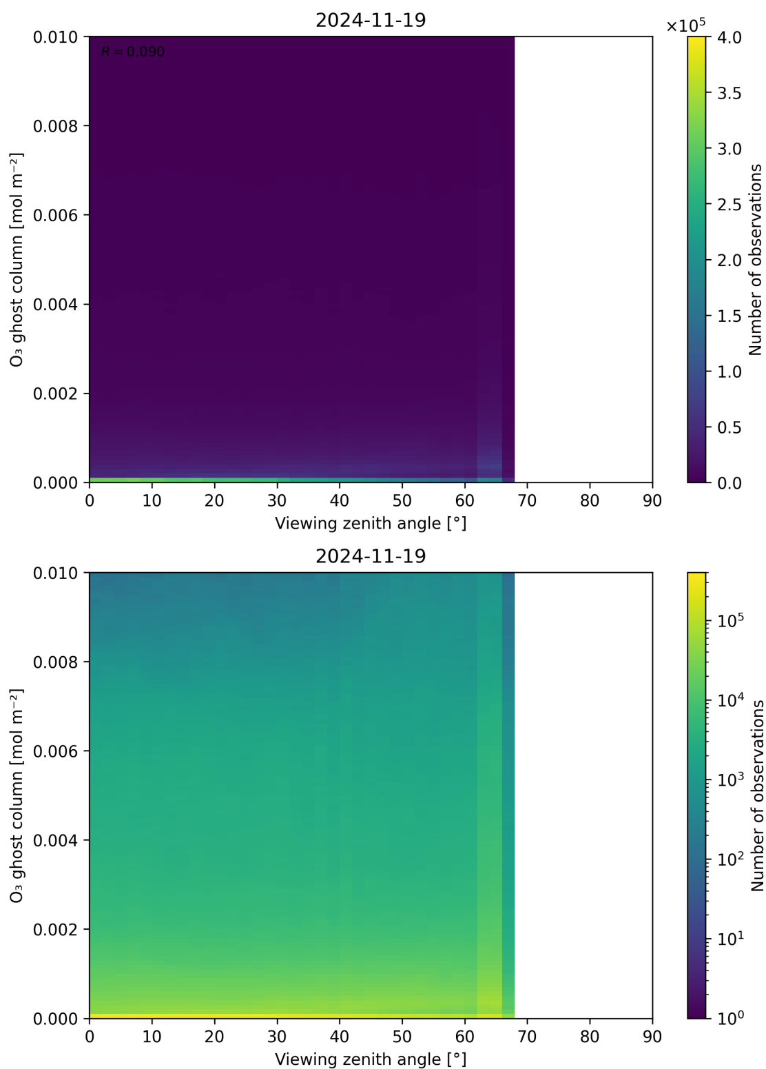
Figure 51: Scatter density plot of “Viewing zenith angle” against “O 3 ghost column” for 2024-11-18 to 2024-11-20.
