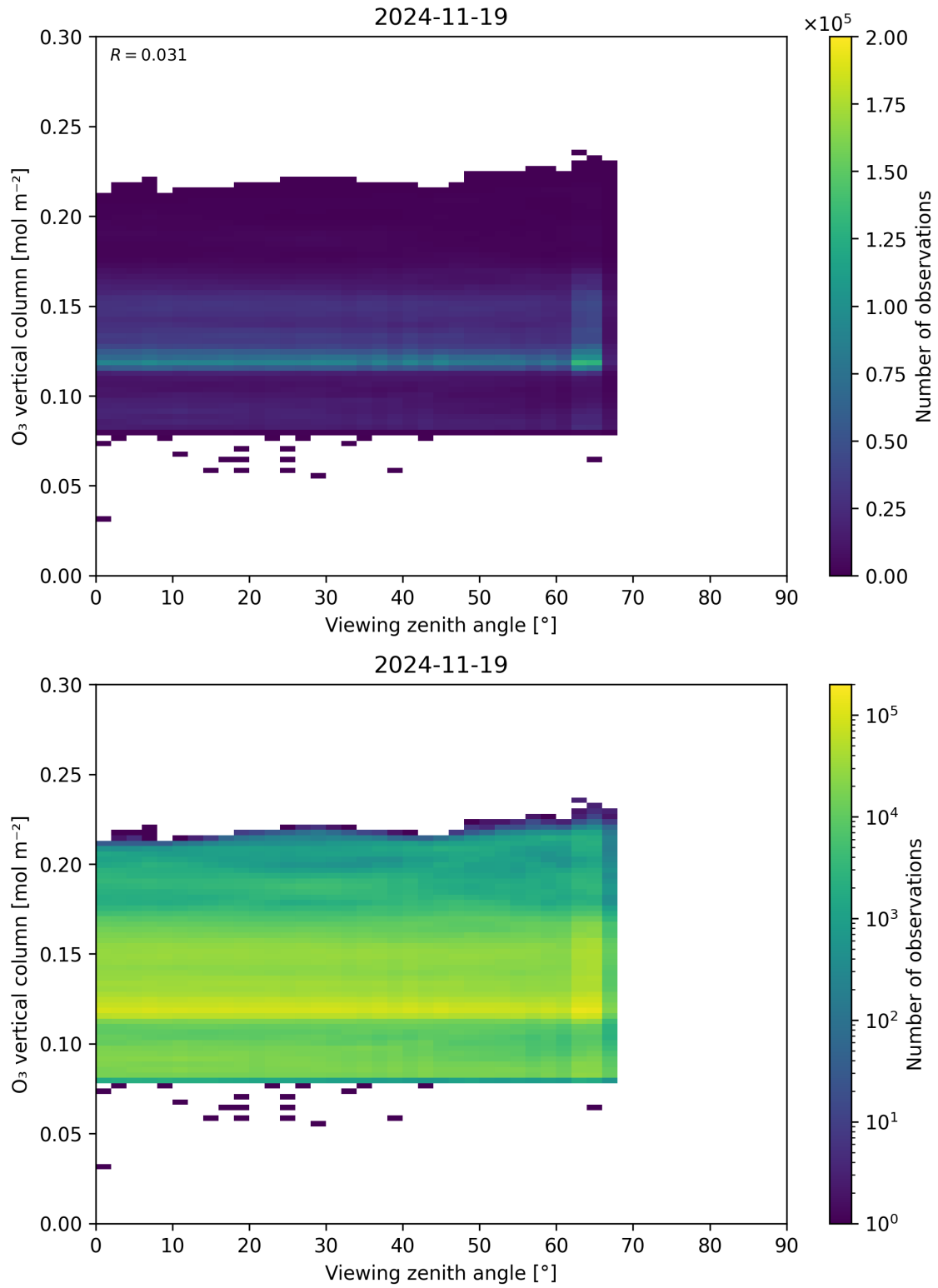
Figure 52: Scatter density plot of “Viewing zenith angle” against “O 3 vertical column” for 2024-11-18 to 2024-11-20.
