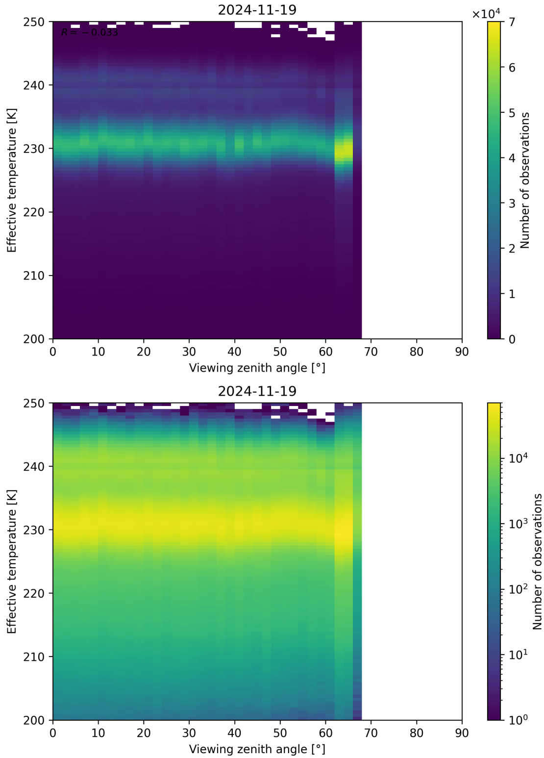
Figure 50: Scatter density plot of “Viewing zenith angle” against “Effective temperature” for 2024-11-18 to 2024-11-20.
