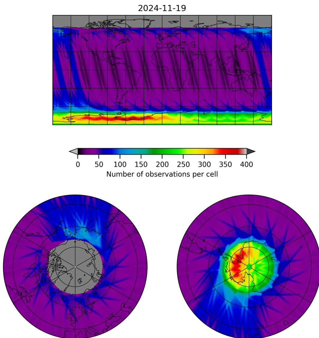
Figure 12: Map of the number of observations for 2024-11-18 to 2024-11-20
