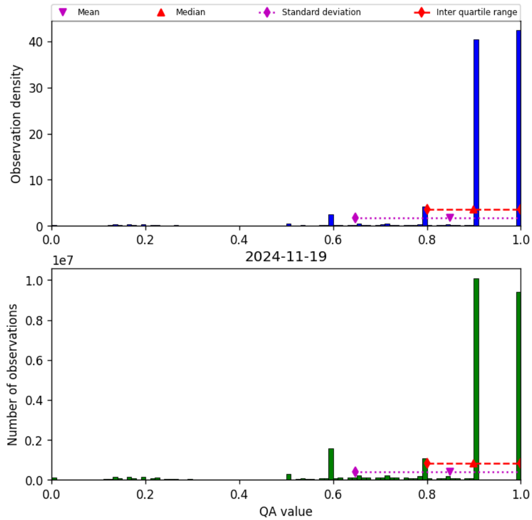
Figure 20: Histogram of “QA value” for 2024-11-18 to 2024-11-20
