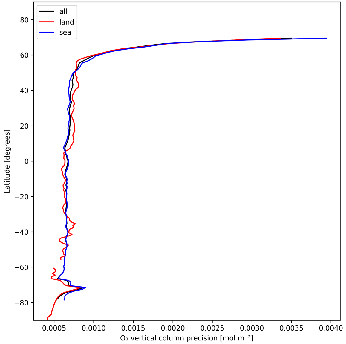
Figure 15: Zonal average of “O 3 vertical column precision” for 2024-11-18 to 2024-11-20.
