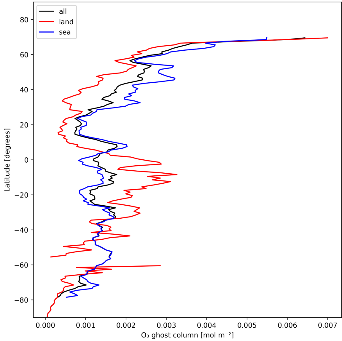
Figure 18: Zonal average of "O 3 ghost column" for 2024-11-20 to 2024-11-21.
