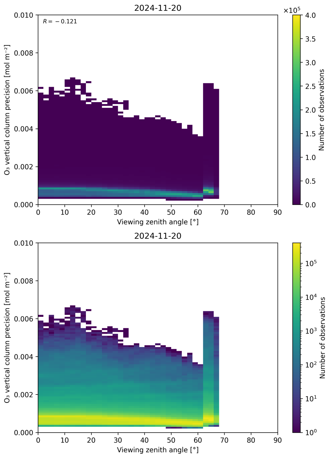
Figure 53: Scatter density plot of “Viewing zenith angle” against “O 3 vertical column precision” for 2024-11-20 to 2024-11-21.
