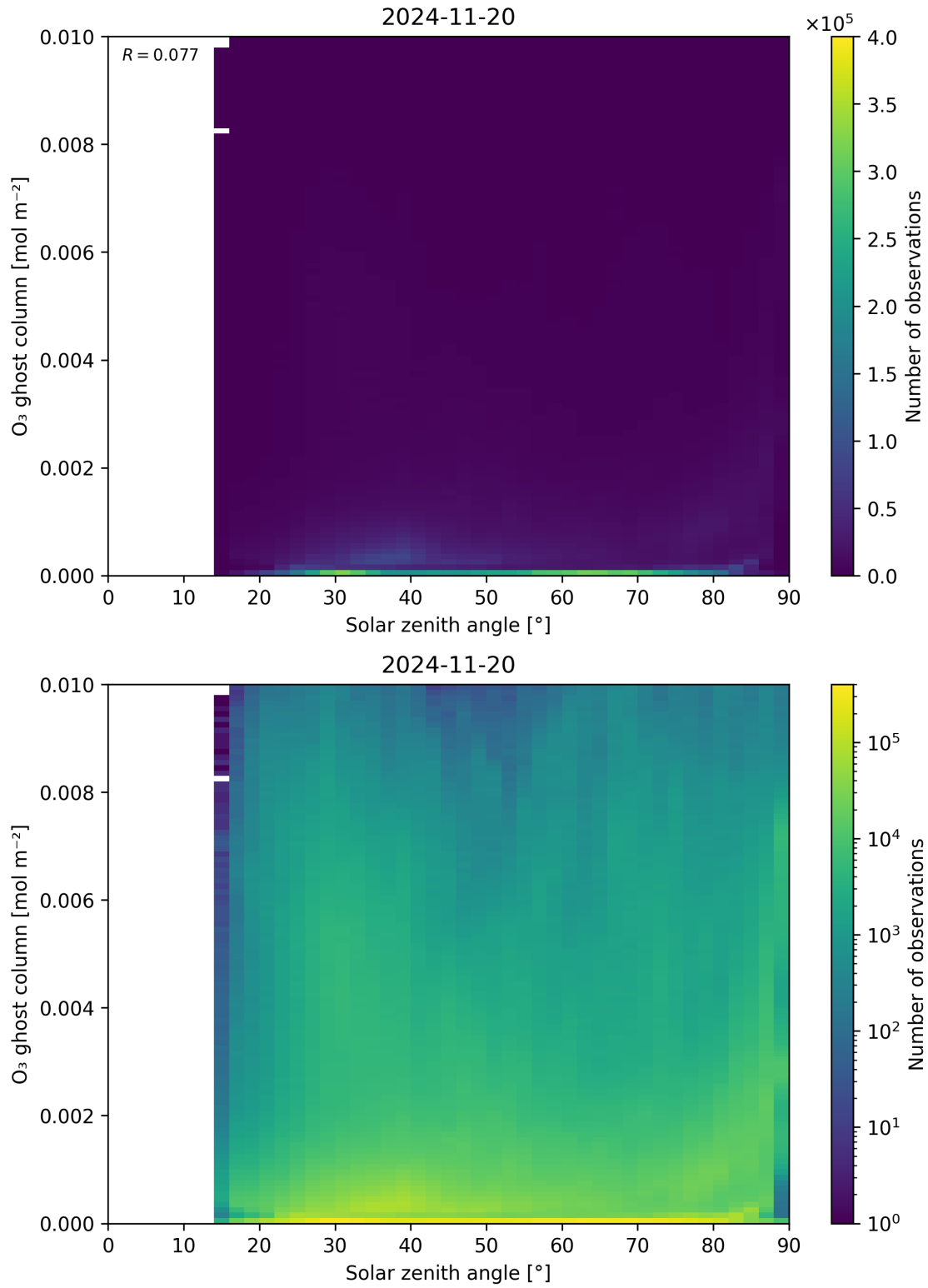
Figure 46: Scatter density plot of “Solar zenith angle” against “O 3 ghost column” for 2024-11-20 to 2024-11-21.
