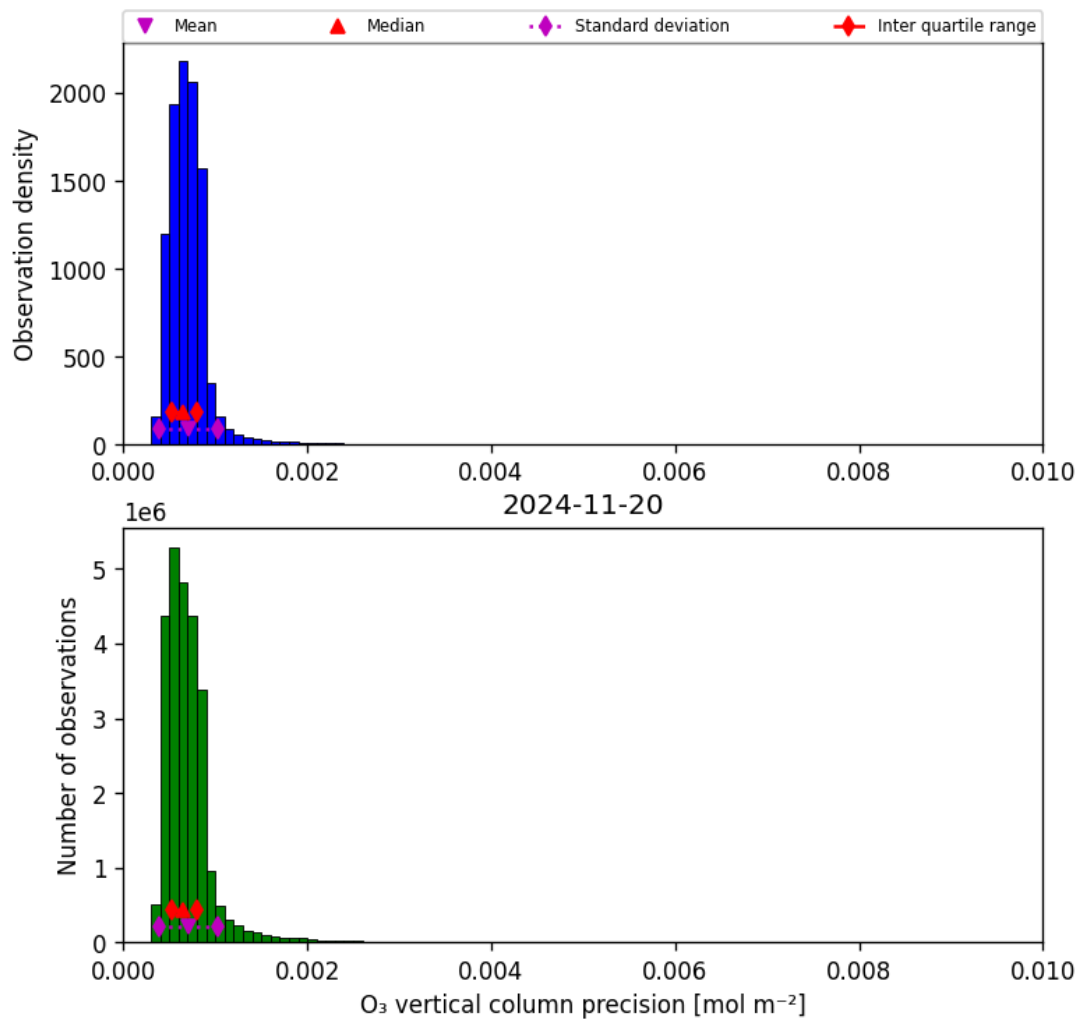
Figure 22: Histogram of “O 3 vertical column precision” for 2024-11-20 to 2024-11-21
