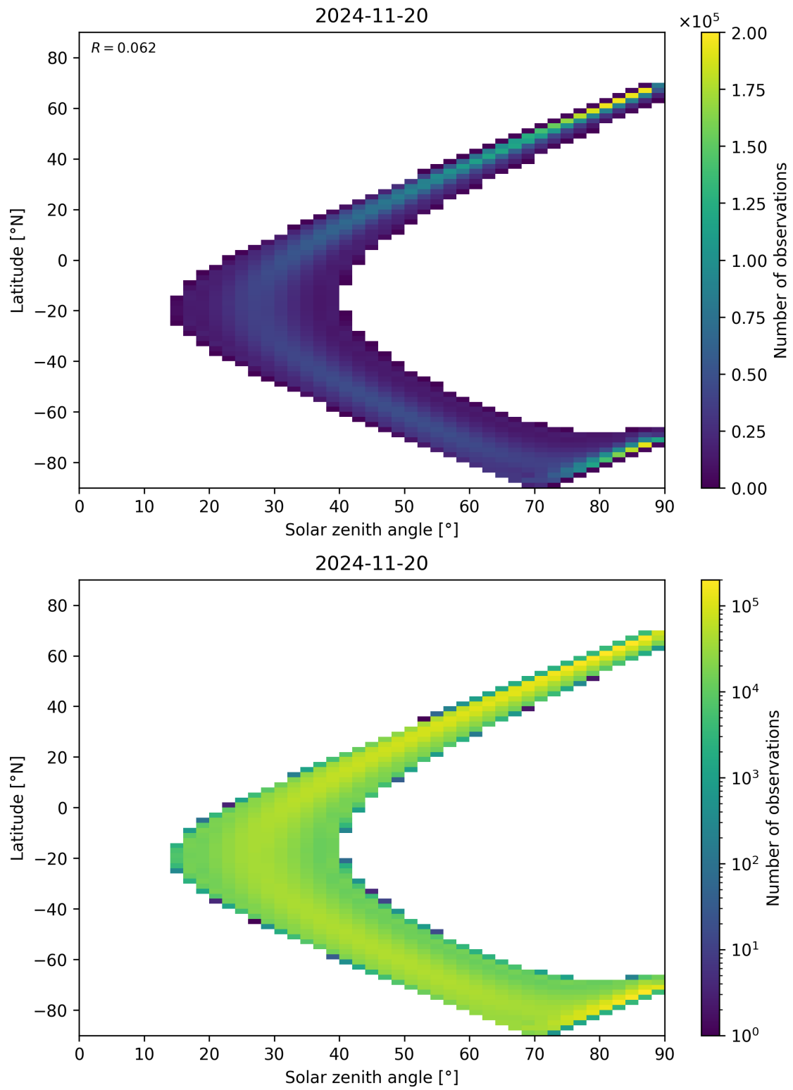
Figure 44: Scatter density plot of “Solar zenith angle” against “Latitude” for 2024-11-20 to 2024-11-21.
