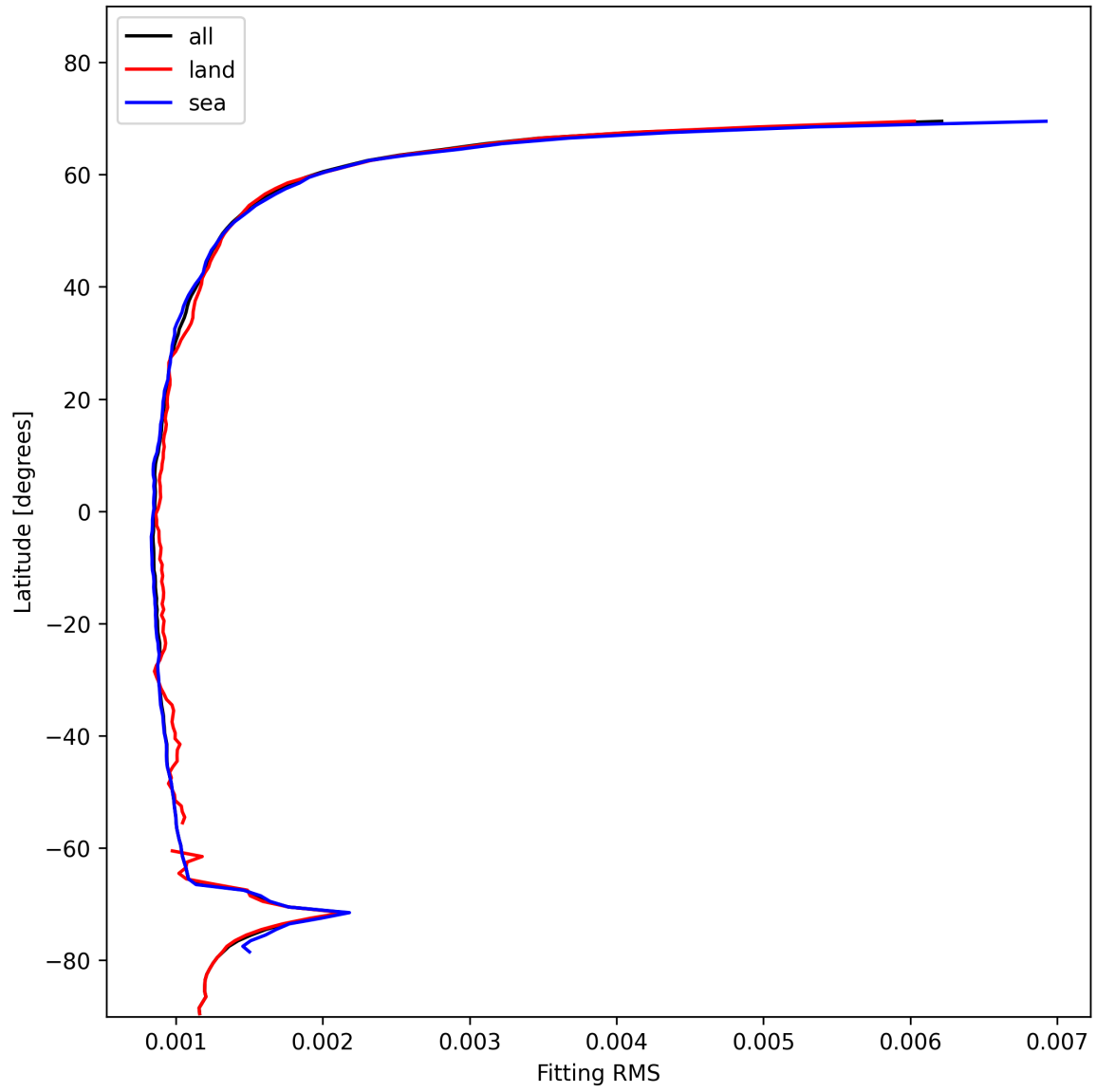
Figure 16: Zonal average of “Fitting RMS” for 2024-11-20 to 2024-11-21.
