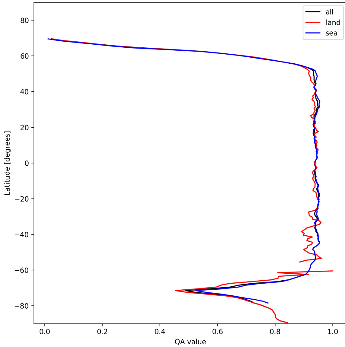
Figure 13: Zonal average of “QA value” for 2024-11-20 to 2024-11-21.
