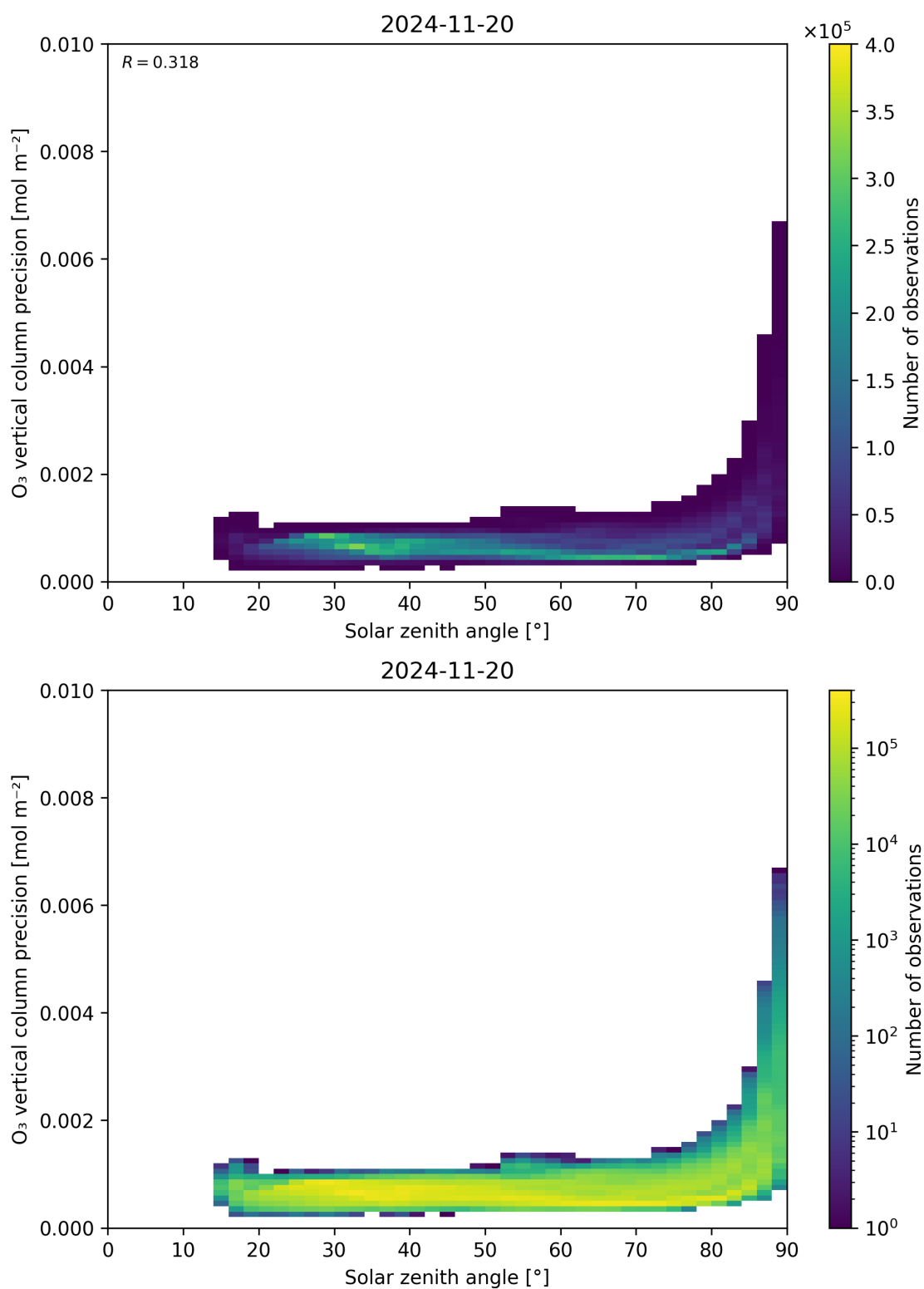
Figure 48: Scatter density plot of “Solar zenith angle” against “O 3 vertical column precision” for 2024-11-20 to 2024-11-21.
