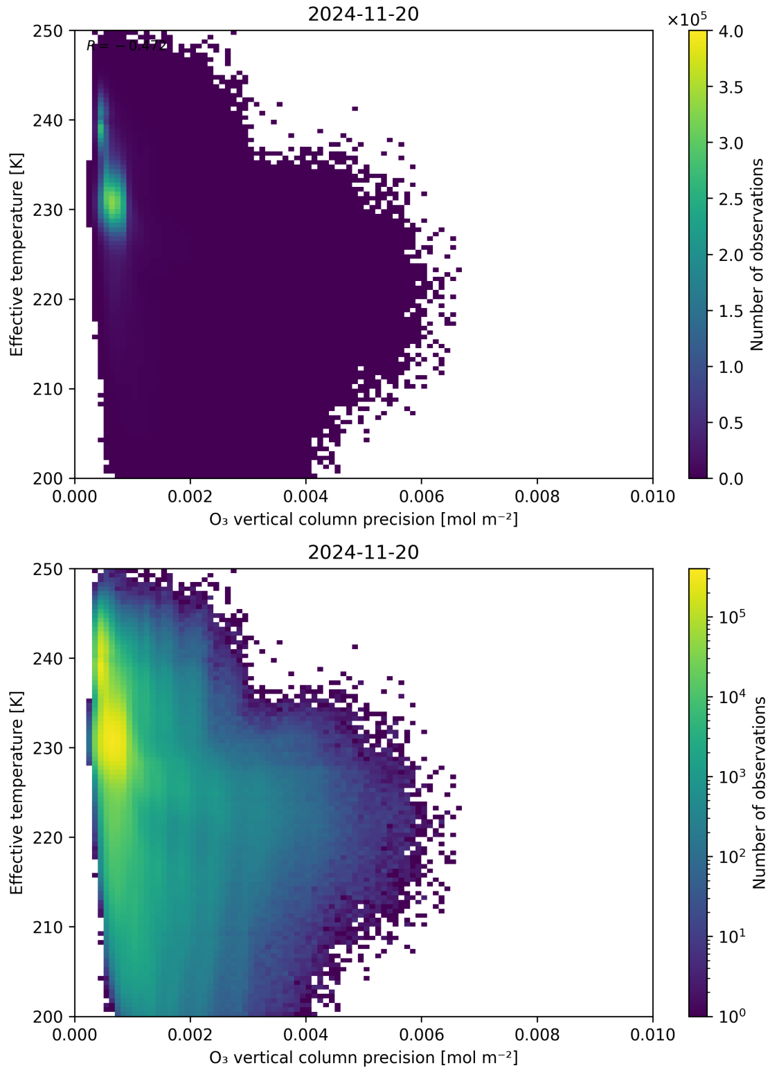
Figure 42: Scatter density plot of “O 3 vertical column precision” against “Effective temperature” for 2024-11-20 to 2024-11-21.
