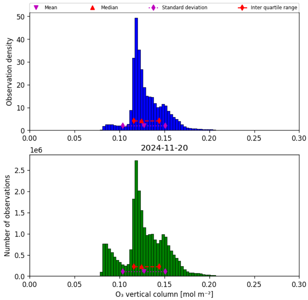
Figure 21: Histogram of “O 3 vertical column” for 2024-11-20 to 2024-11-21
