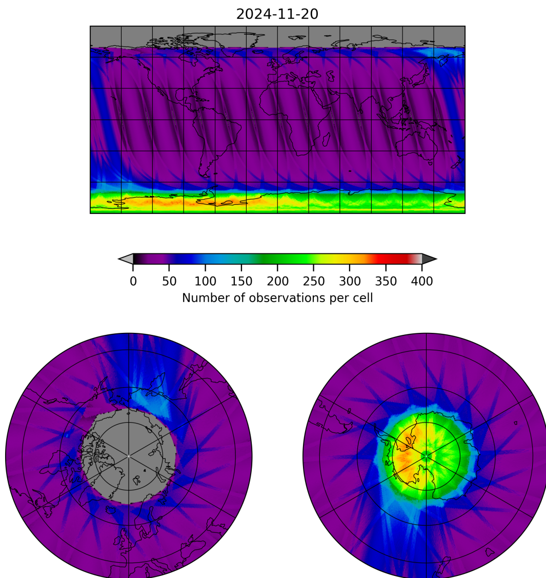
Figure 12: Map of the number of observations for 2024-11-20 to 2024-11-21
