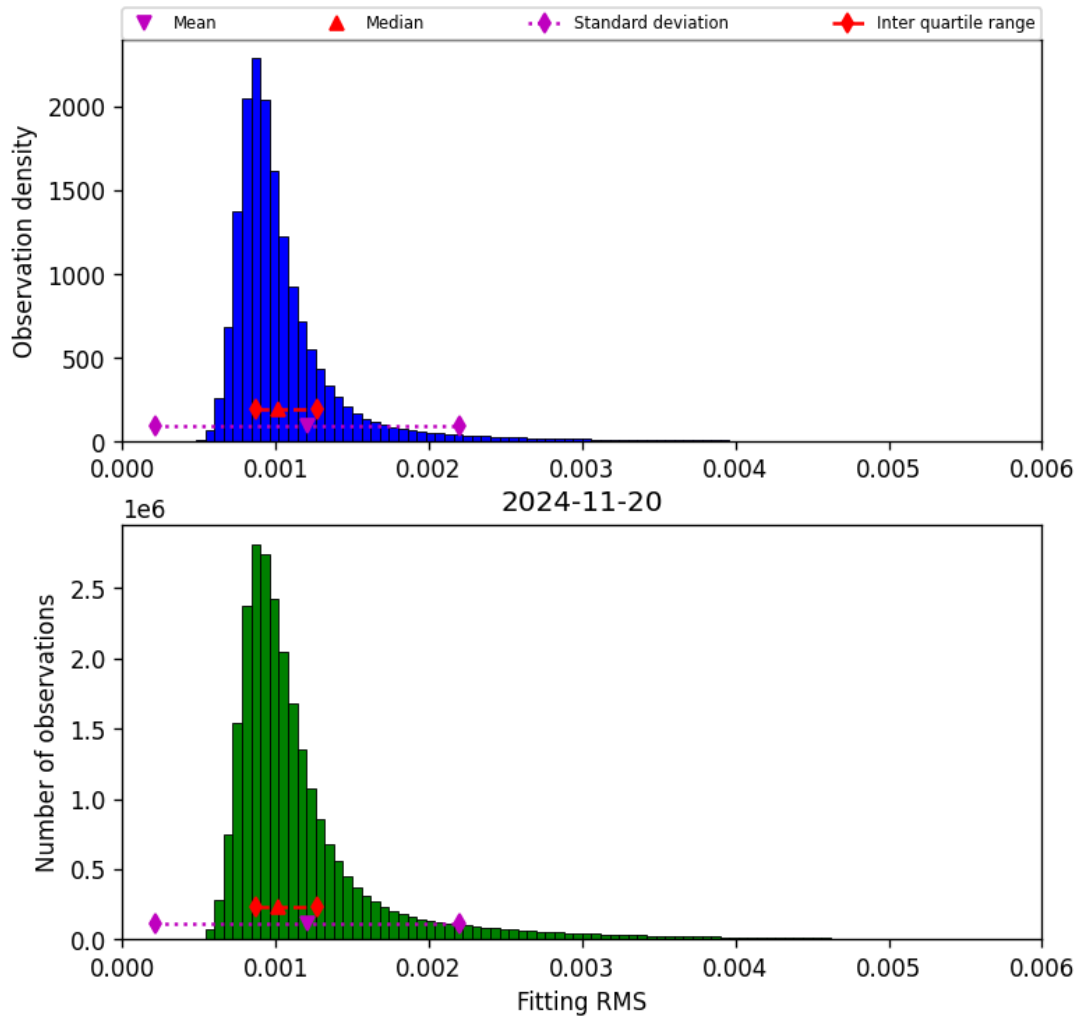
Figure 23: Histogram of “Fitting RMS” for 2024-11-20 to 2024-11-21
