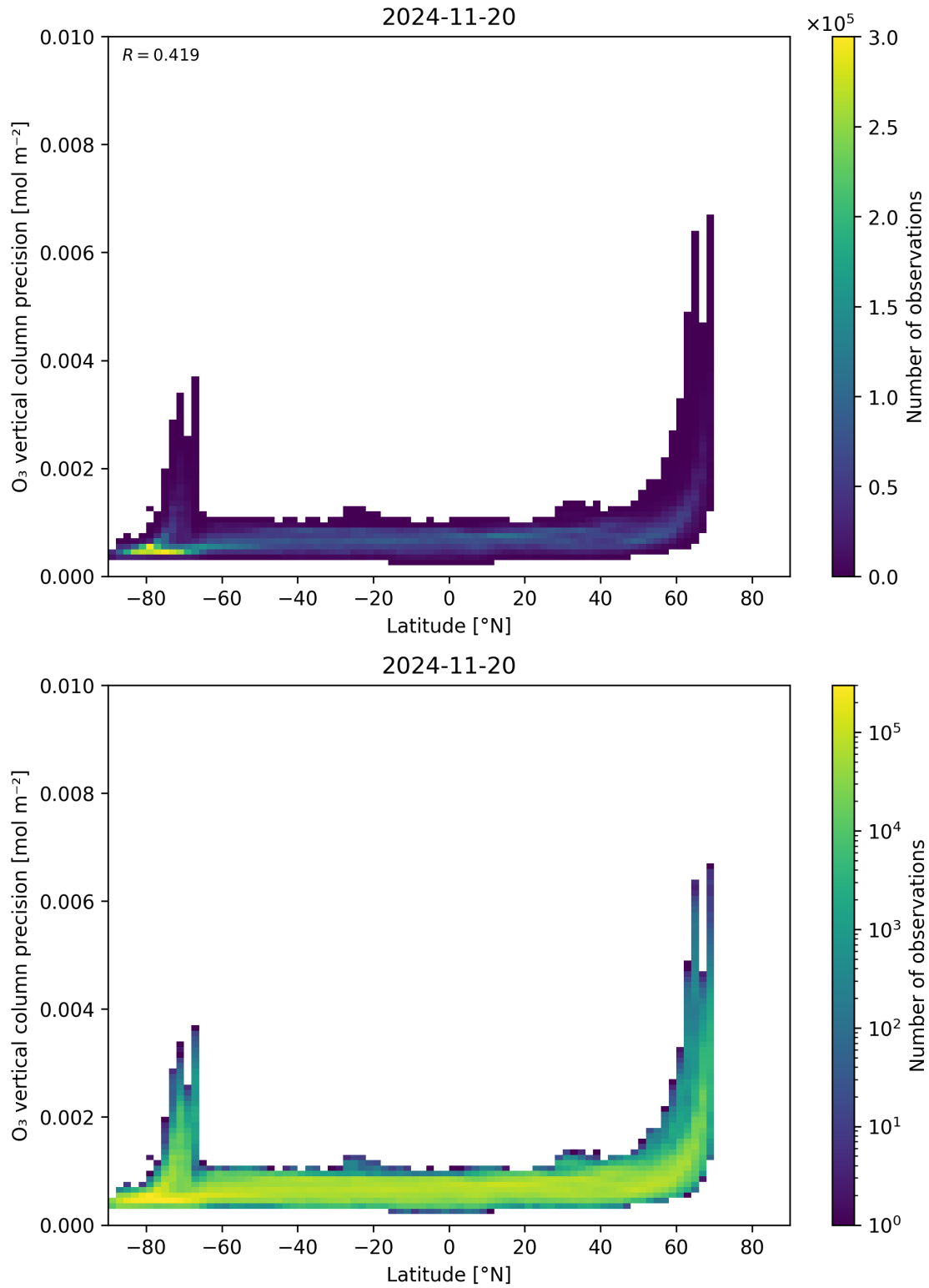
Figure 37: Scatter density plot of “Latitude” against “O 3 vertical column precision” for 2024-11-20 to 2024-11-21.
