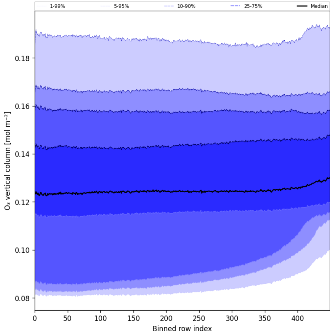
Figure 28: Along track statistics of “O 3 vertical column” for 2024-11-20 to 2024-11-21
