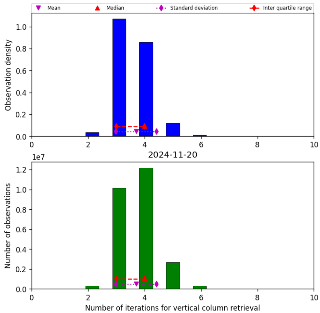
Figure 26: Histogram of “Number of iterations for vertical column retrieval” for 2024-11-20 to 2024-11-21
