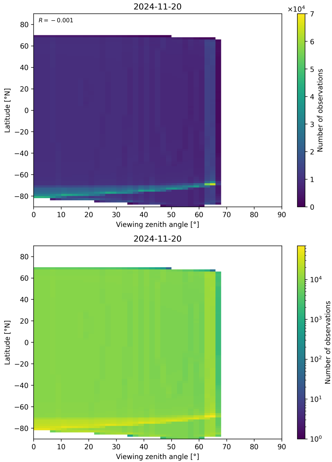
Figure 49: Scatter density plot of “Viewing zenith angle” against “Latitude” for 2024-11-20 to 2024-11-21.
