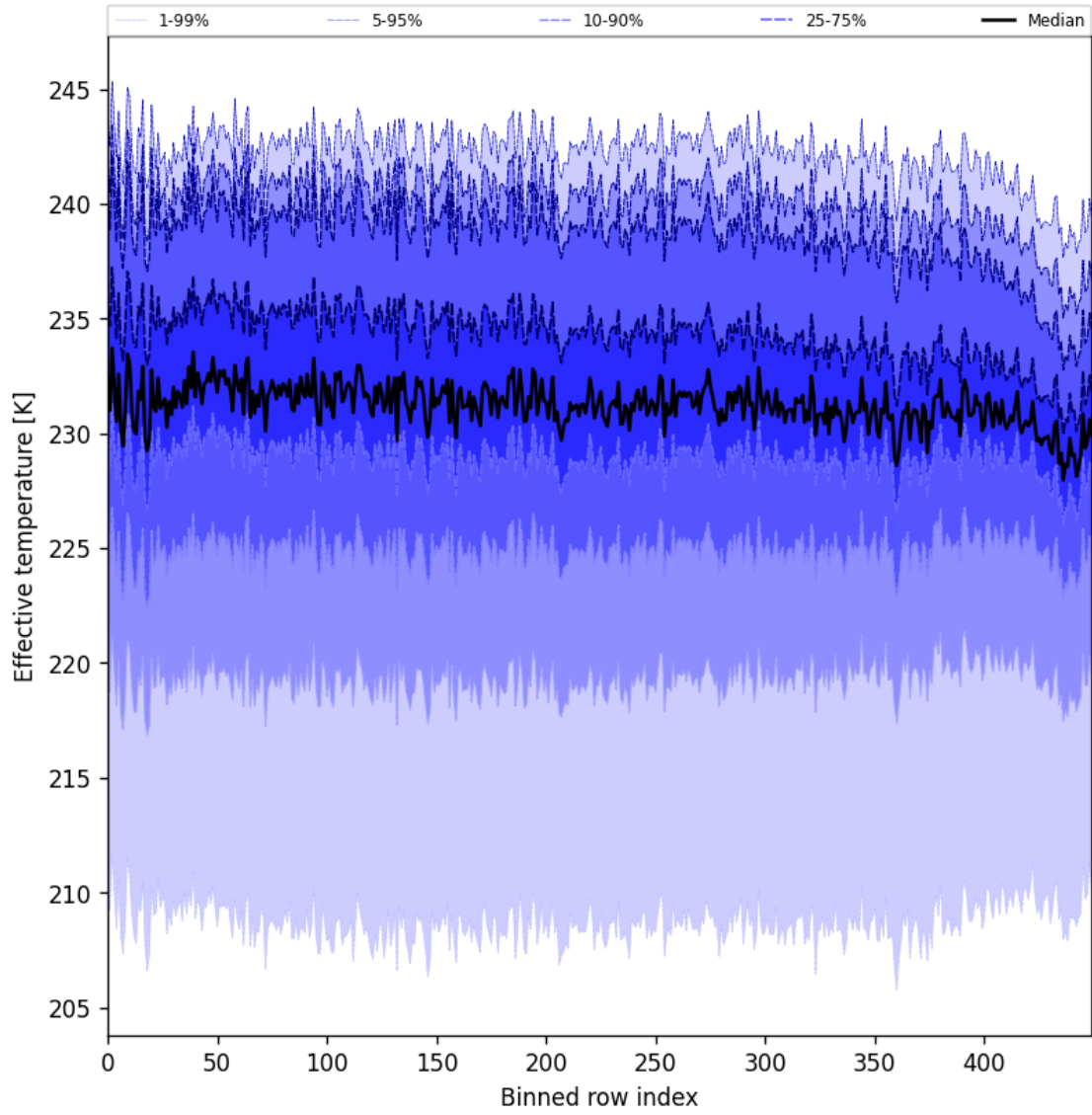
Figure 31: Along track statistics of “Effective temperature” for 2024-11-20 to 2024-11-21
