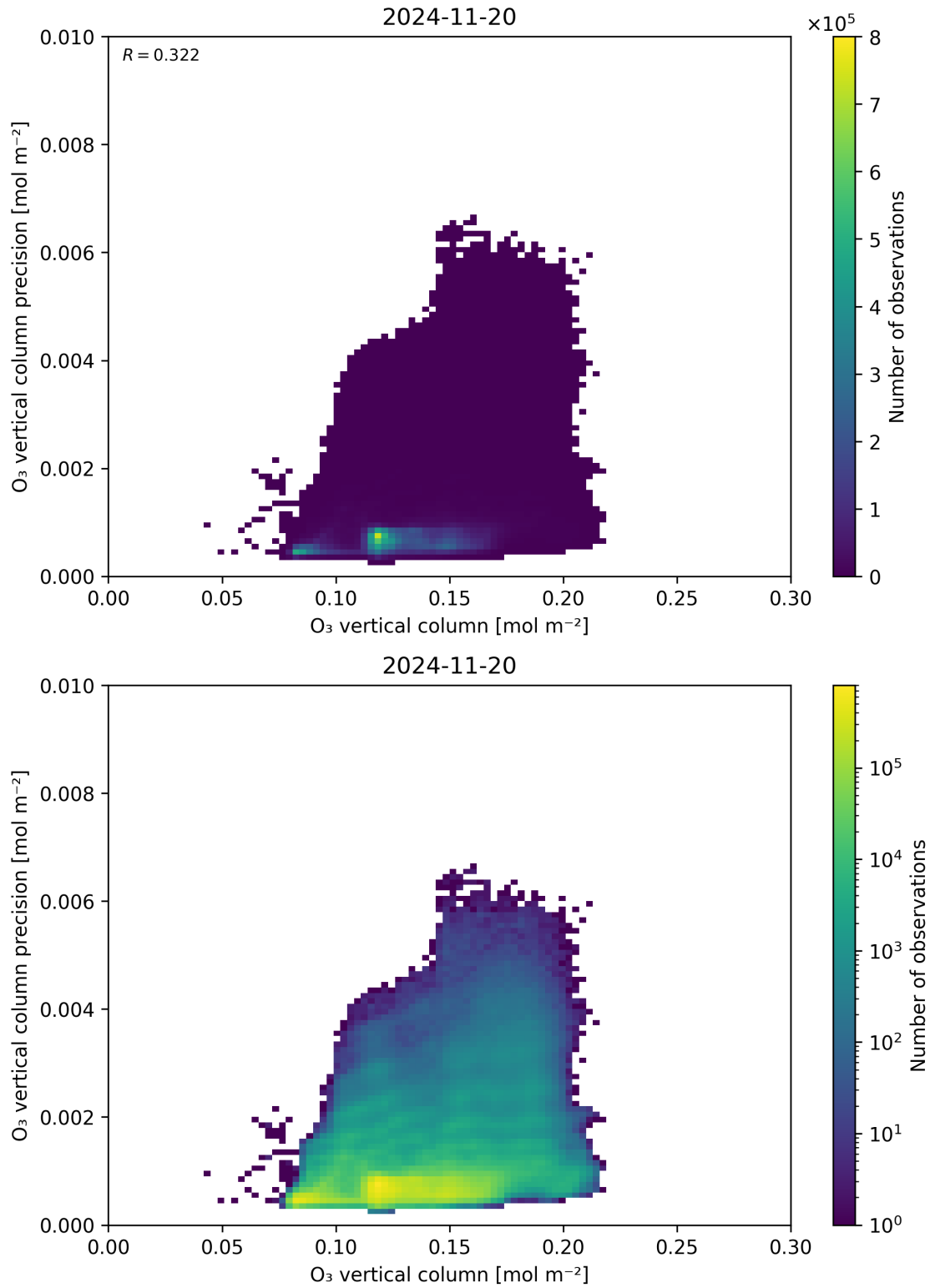
Figure 41: Scatter density plot of “O 3 vertical column” against “O 3 vertical column precision” for 2024-11-20 to 2024-11-21.
