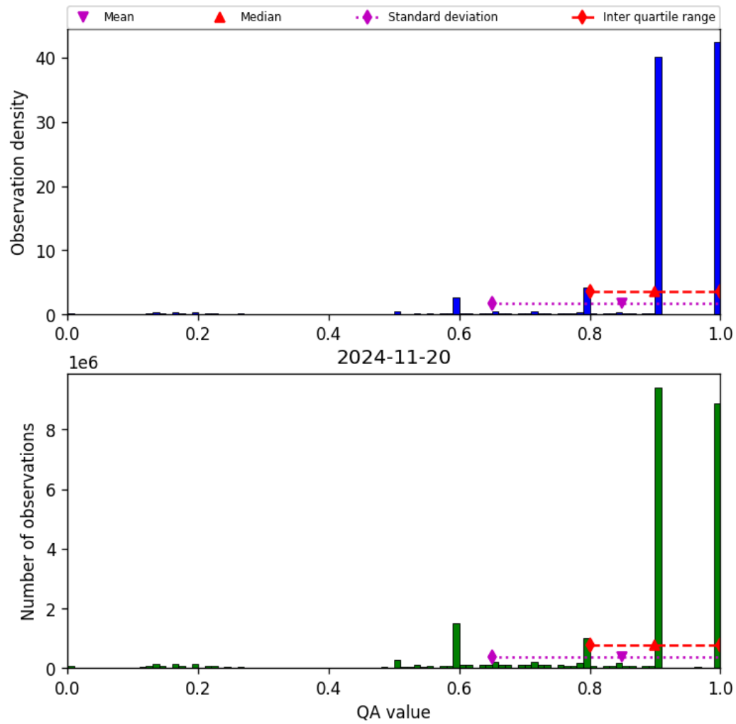
Figure 20: Histogram of “QA value” for 2024-11-20 to 2024-11-21
