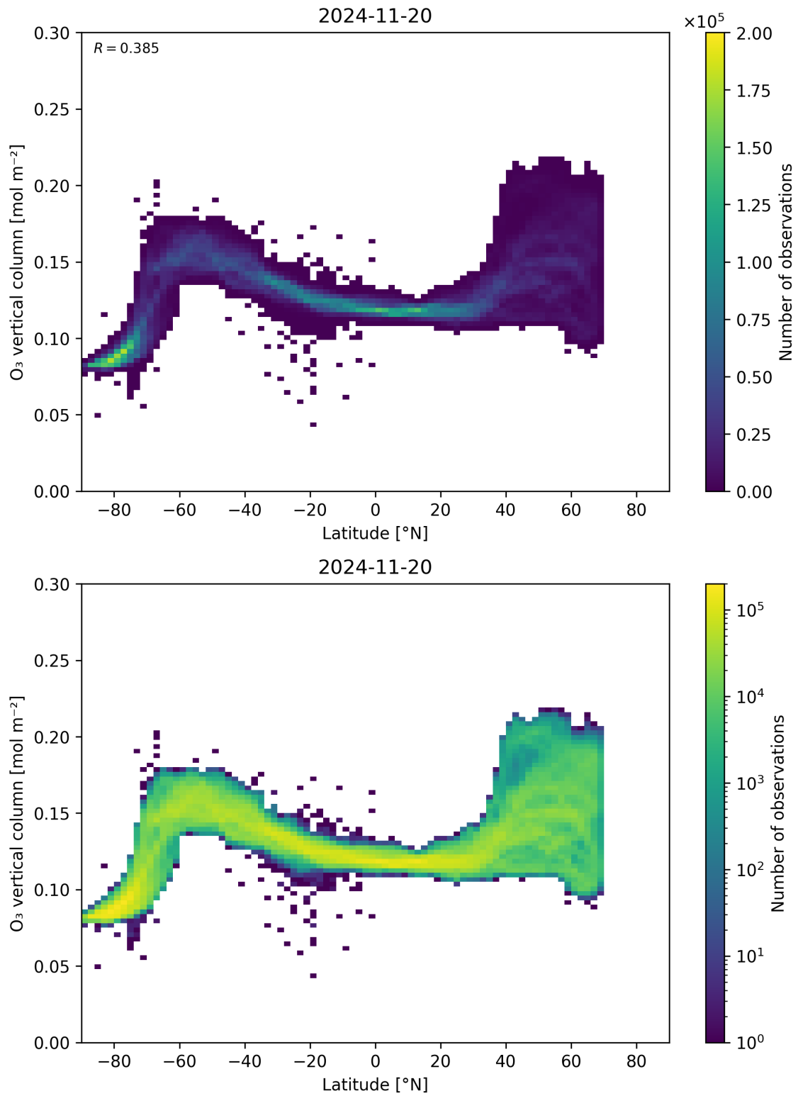
Figure 36: Scatter density plot of “Latitude” against “O 3 vertical column” for 2024-11-20 to 2024-11-21.
