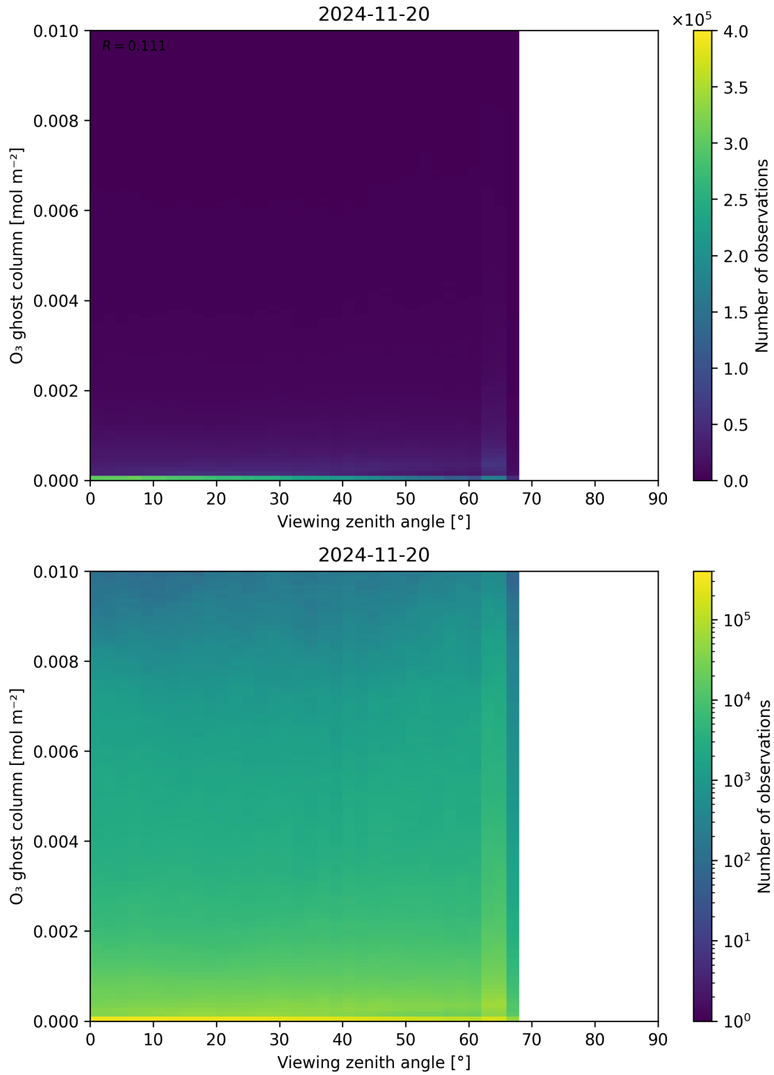
Figure 51: Scatter density plot of “Viewing zenith angle” against “O 3 ghost column” for 2024-11-20 to 2024-11-21.
