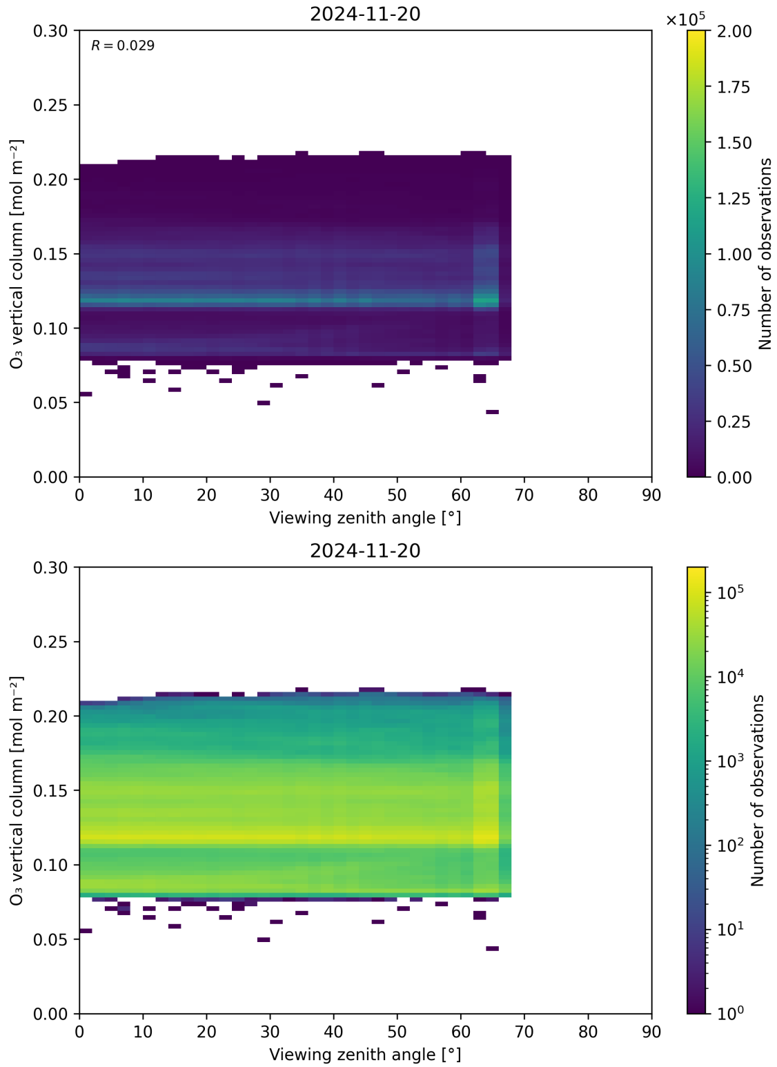
Figure 52: Scatter density plot of “Viewing zenith angle” against “O 3 vertical column” for 2024-11-20 to 2024-11-21.
