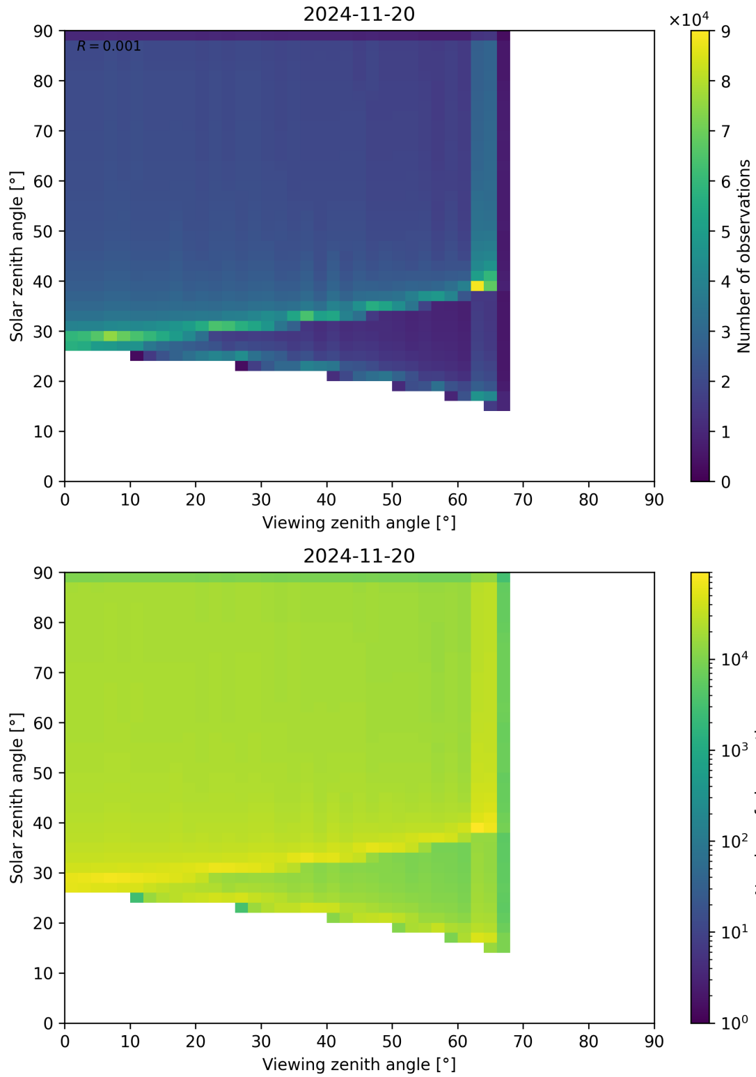
Figure 54: Scatter density plot of “Viewing zenith angle” against “Solar zenith angle” for 2024-11-20 to 2024-11-21.
