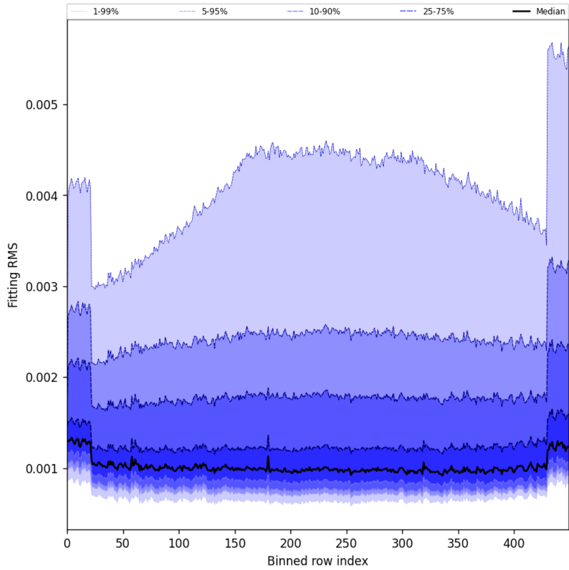
Figure 30: Along track statistics of “Fitting RMS” for 2024-11-20 to 2024-11-21
