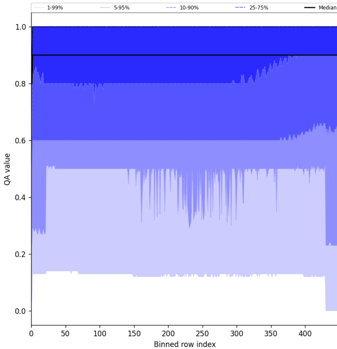
Figure 27: Along track statistics of “QA value” for 2024-11-20 to 2024-11-21
