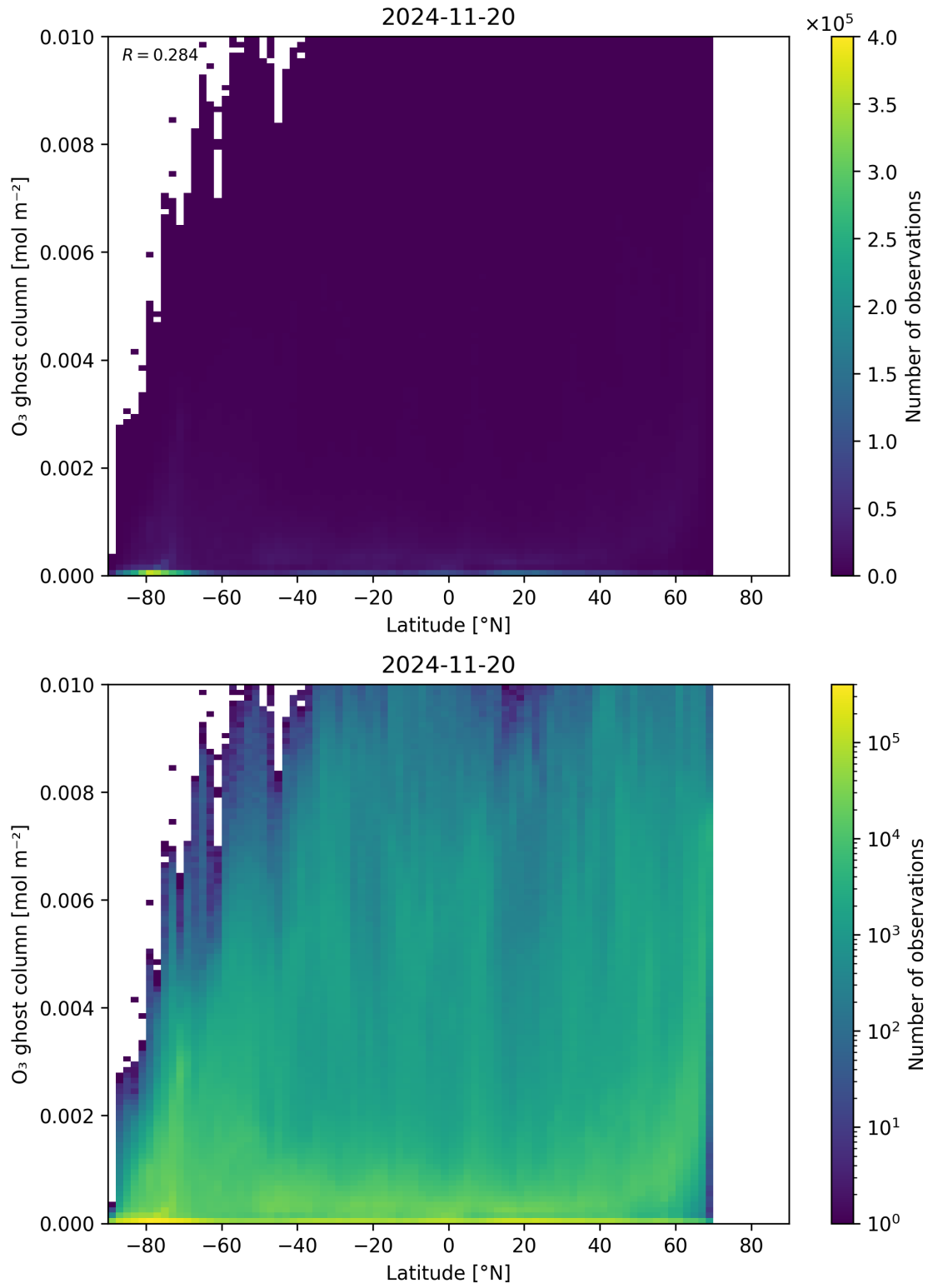
Figure 35: Scatter density plot of “Latitude” against “O 3 ghost column” for 2024-11-20 to 2024-11-21.
