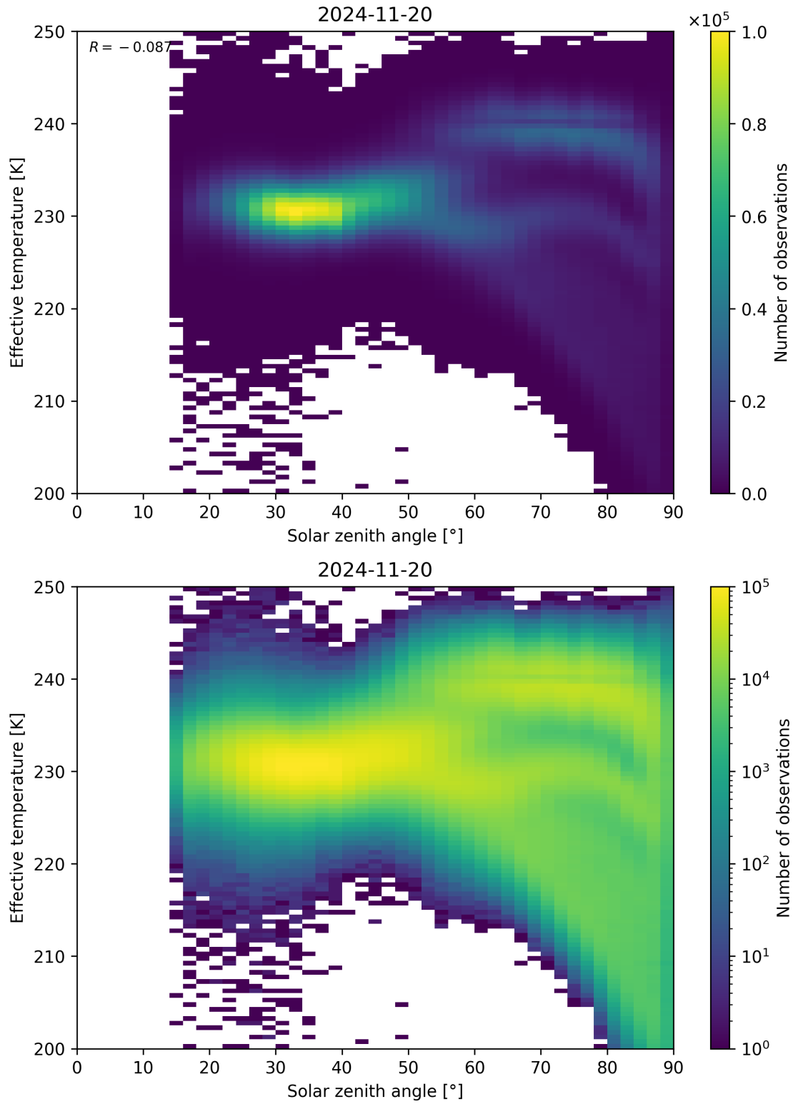
Figure 45: Scatter density plot of “Solar zenith angle” against “Effective temperature” for 2024-11-20 to 2024-11-21.
