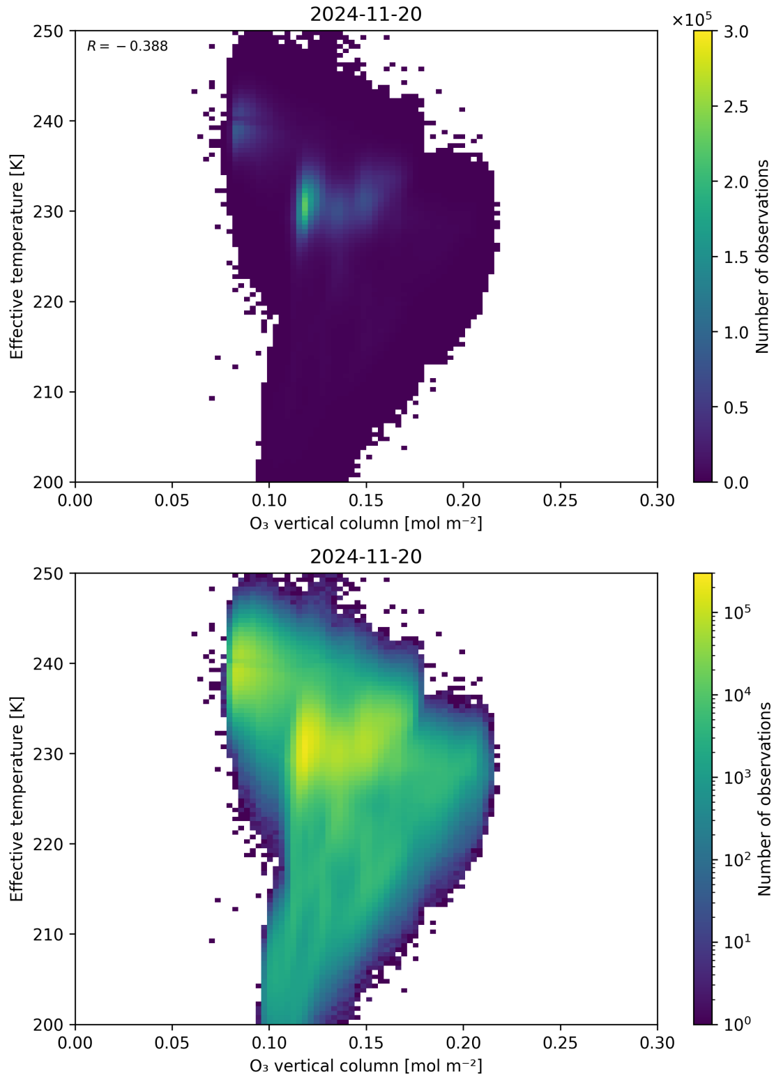
Figure 39: Scatter density plot of “O 3 vertical column” against “Effective temperature” for 2024-11-20 to 2024-11-21.
