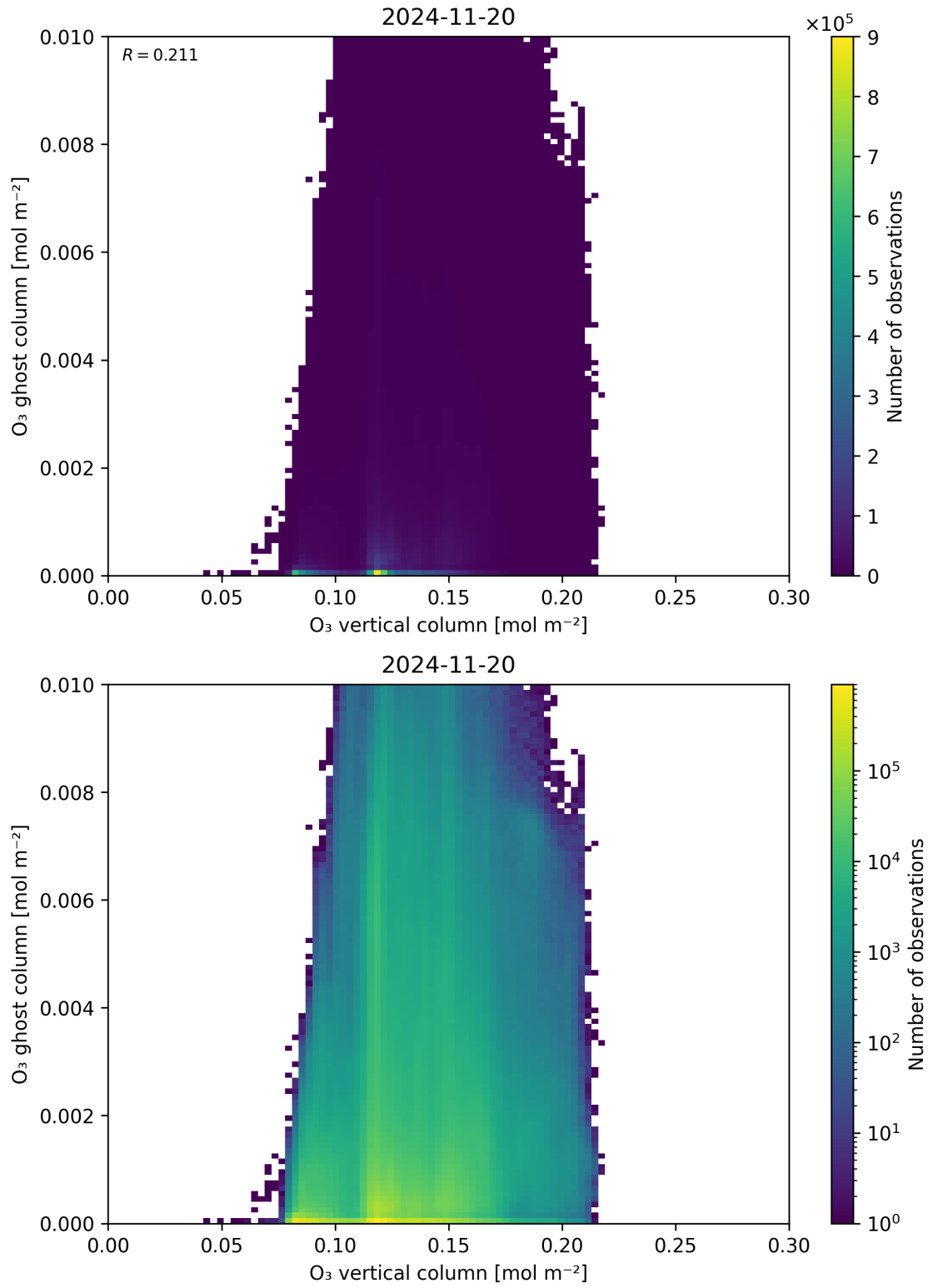
Figure 40: Scatter density plot of “O 3 vertical column” against “O 3 ghost column” for 2024-11-20 to 2024-11-21.
