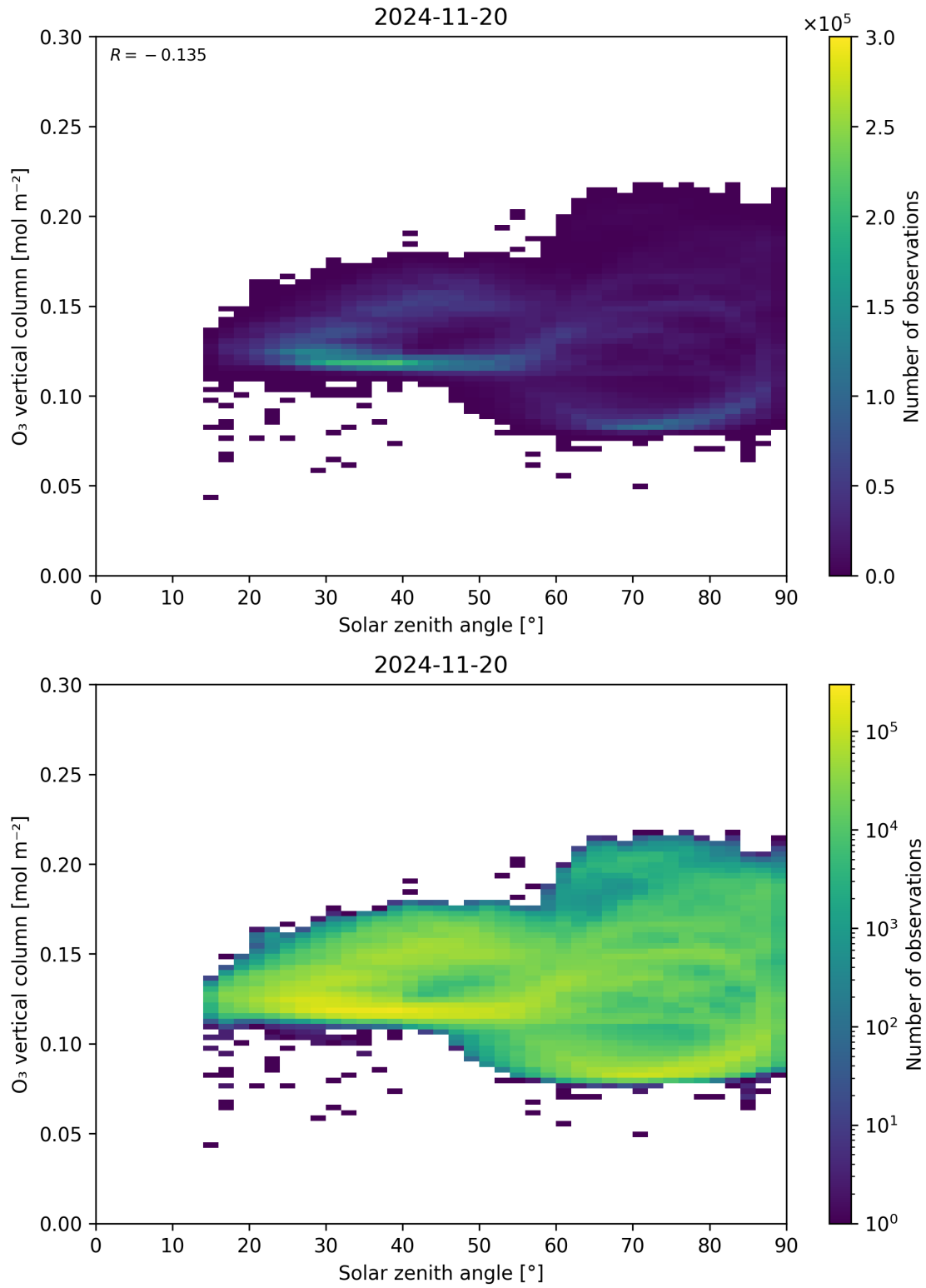
Figure 47: Scatter density plot of “Solar zenith angle” against “O 3 vertical column” for 2024-11-20 to 2024-11-21.
