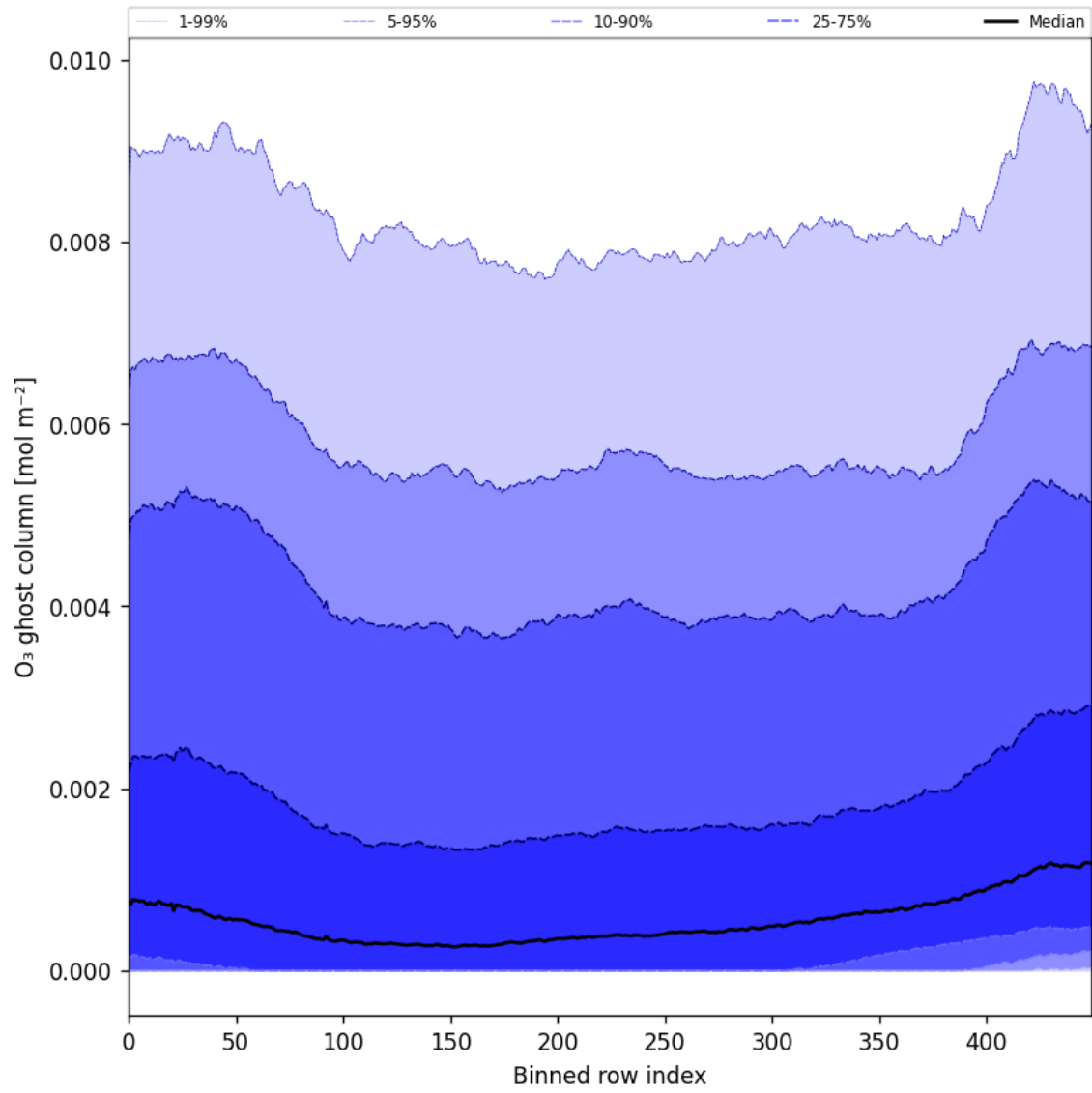
Figure 32: Along track statistics of “O 3 ghost column” for 2024-11-20 to 2024-11-21
