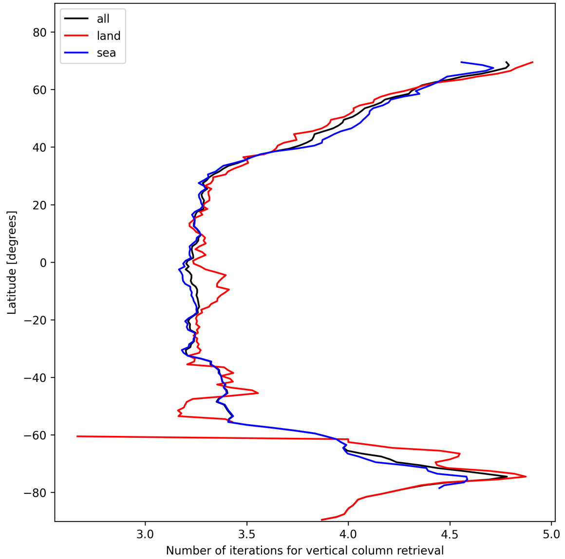
Figure 19: Zonal average of “Number of iterations for vertical column retrieval” for 2024-11-20 to 2024-11-21.
