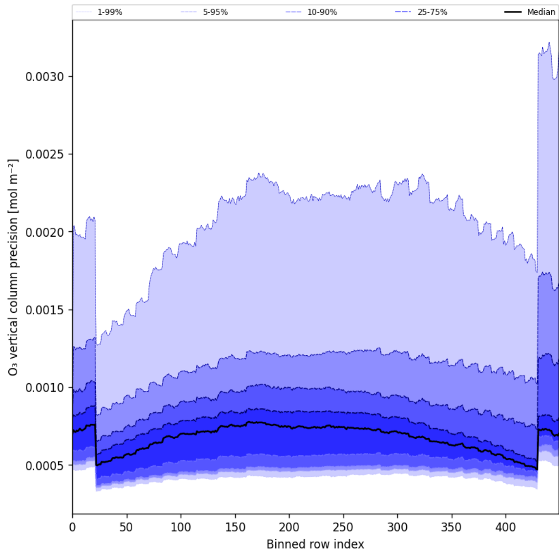
Figure 29: Along track statistics of “O 3 vertical column precision” for 2024-11-20 to 2024-11-21
