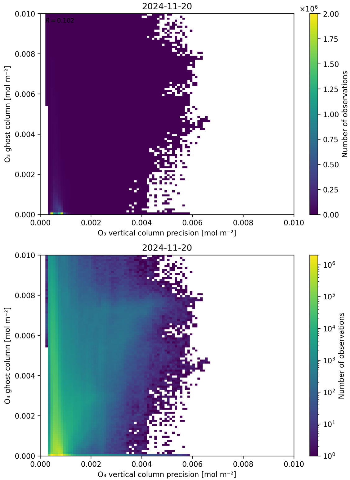
Figure 43: Scatter density plot of “ \text{O}_3 vertical column precision” against “ \text{O}_3 ghost column” for 2024-11-20 to 2024-11-21.
