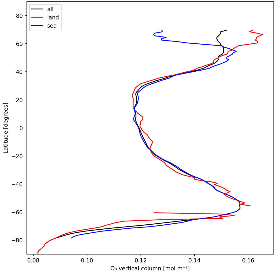
Figure 14: Zonal average of “O 3 vertical column” for 2024-11-20 to 2024-11-21.
