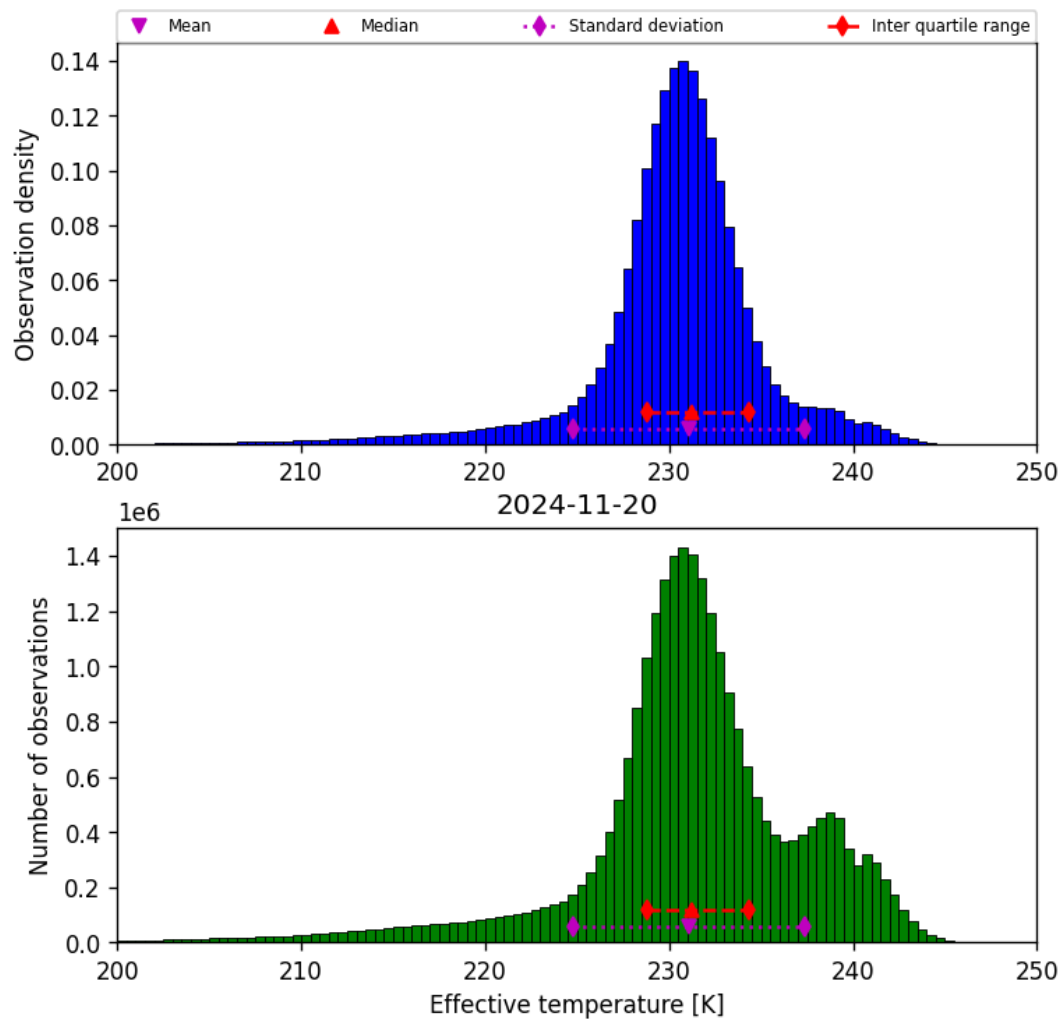
Figure 24: Histogram of “Effective temperature” for 2024-11-20 to 2024-11-21
