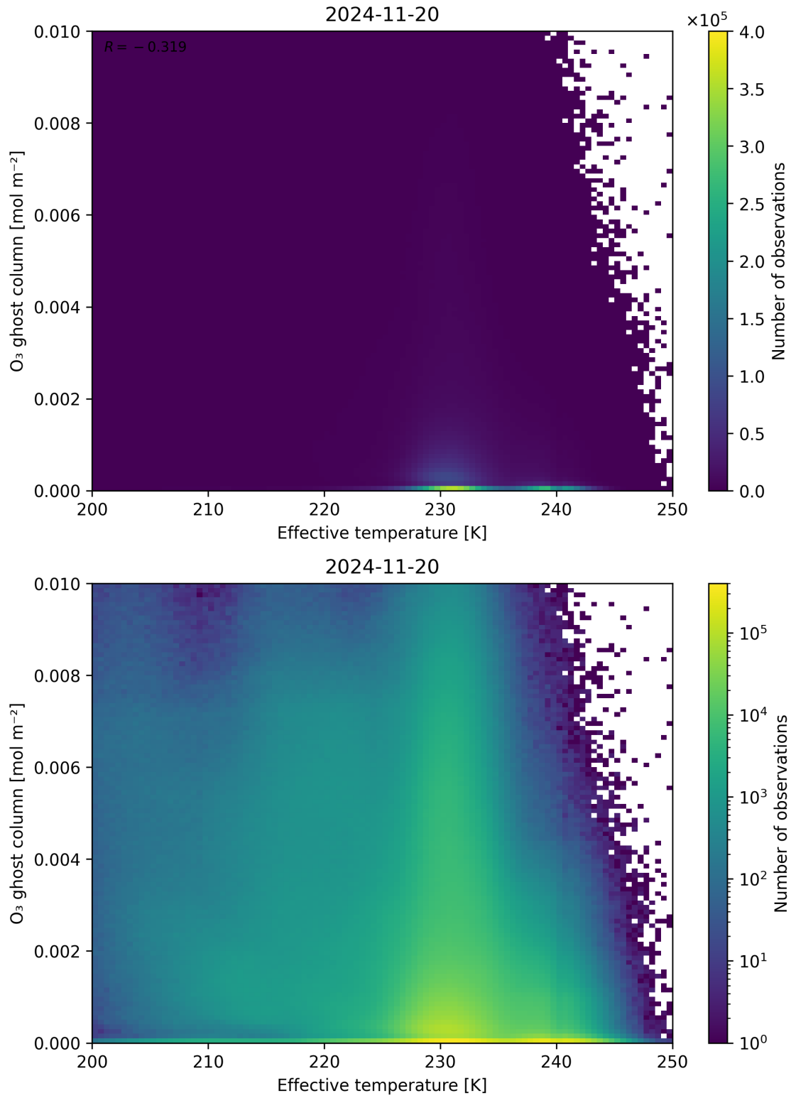
Figure 38: Scatter density plot of “Effective temperature” against “O 3 ghost column” for 2024-11-20 to 2024-11-21.
