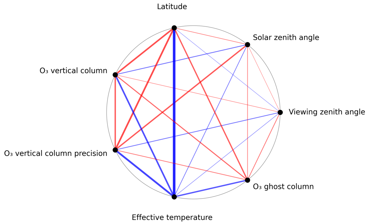
Figure 1: Map of correlation graph for 2024-11-20 to 2024-11-21.
