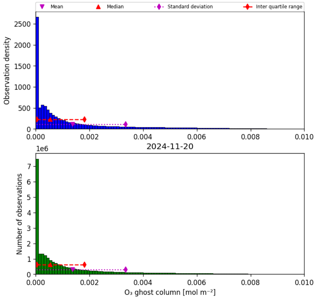
Figure 25: Histogram of “O 3 ghost column” for 2024-11-20 to 2024-11-21
