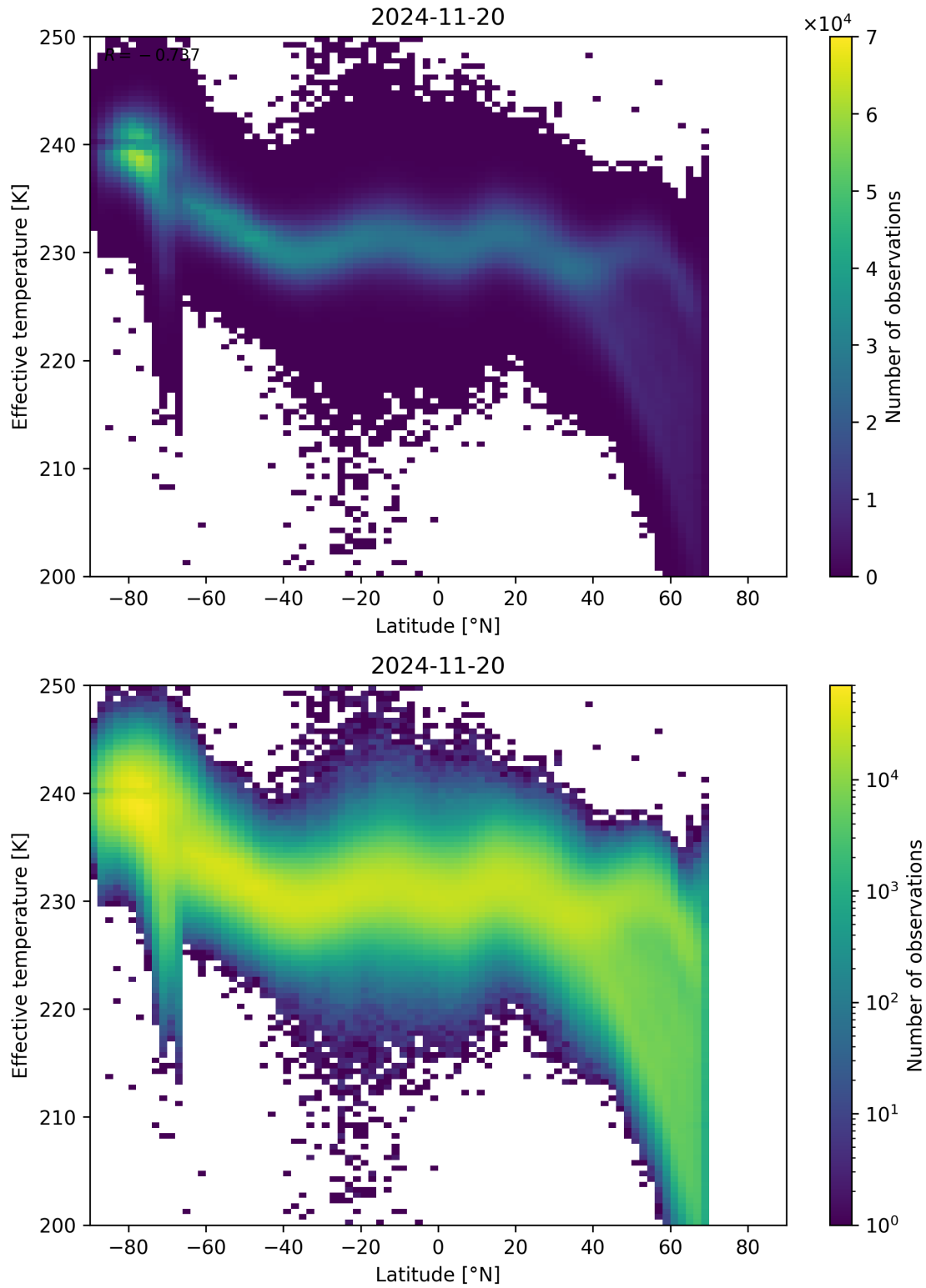
Figure 34: Scatter density plot of “Latitude” against “Effective temperature” for 2024-11-20 to 2024-11-21.
