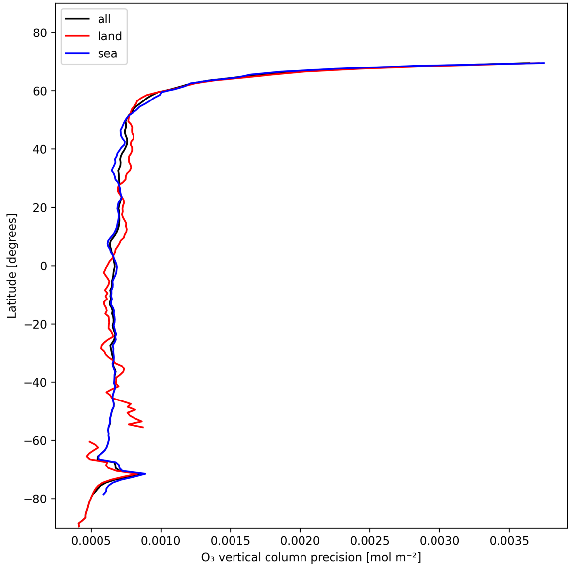
Figure 15: Zonal average of “O 3 vertical column precision” for 2024-11-20 to 2024-11-21.
