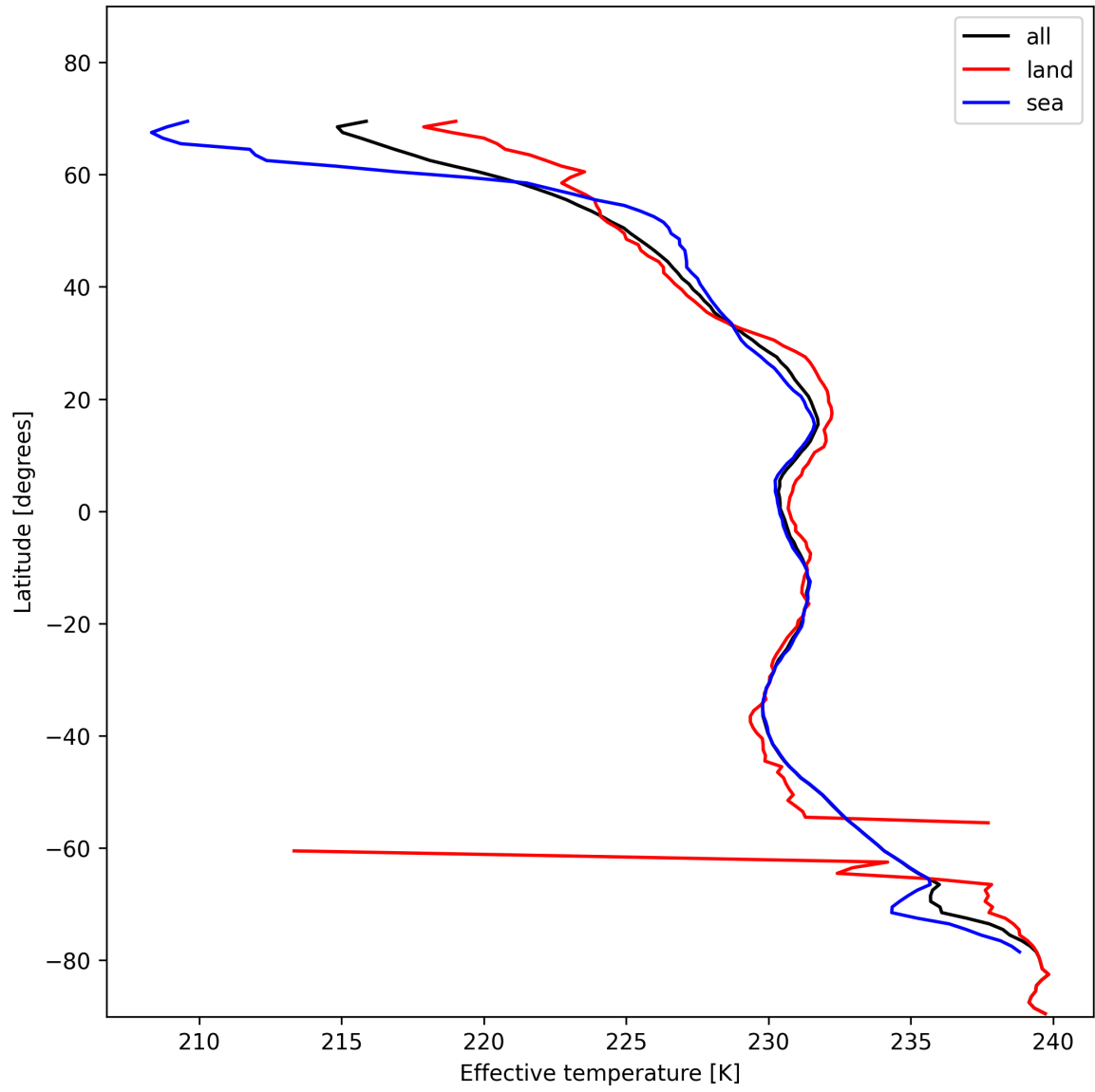
Figure 17: Zonal average of “Effective temperature” for 2024-11-20 to 2024-11-21.
