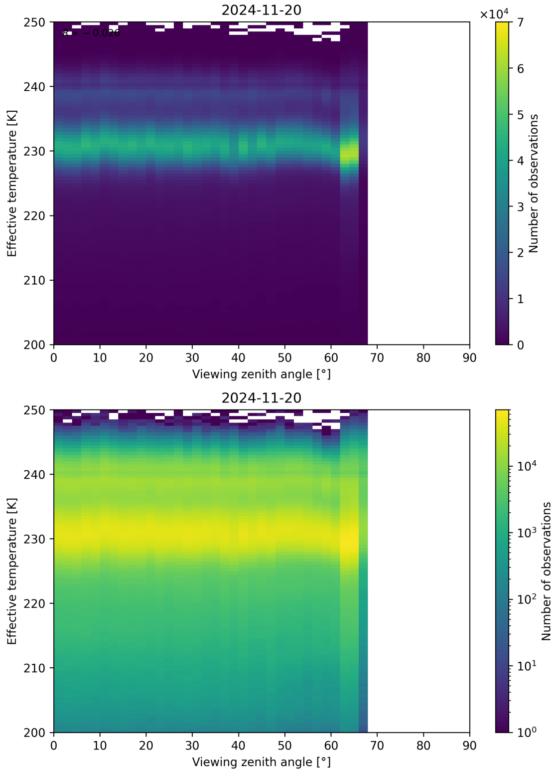
Figure 50: Scatter density plot of “Viewing zenith angle” against “Effective temperature” for 2024-11-20 to 2024-11-21.
