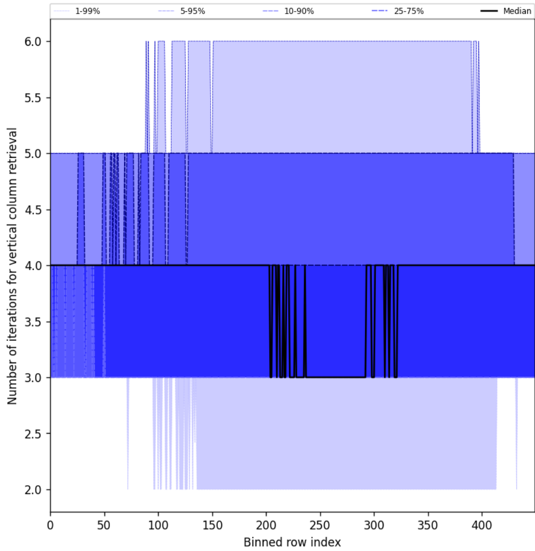
Figure 33: Along track statistics of “Number of iterations for vertical column retrieval” for 2024-11-20 to 2024-11-21
