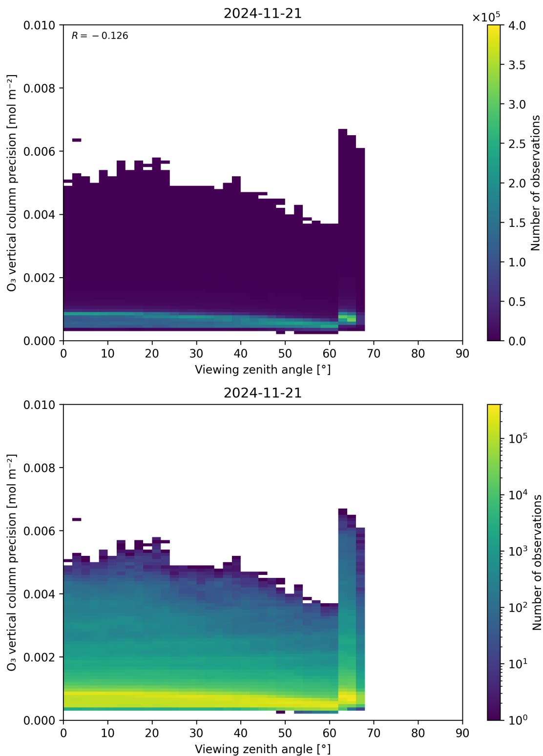
Figure 53: Scatter density plot of “Viewing zenith angle” against “O 3 vertical column precision” for 2024-11-20 to 2024-11-22.
