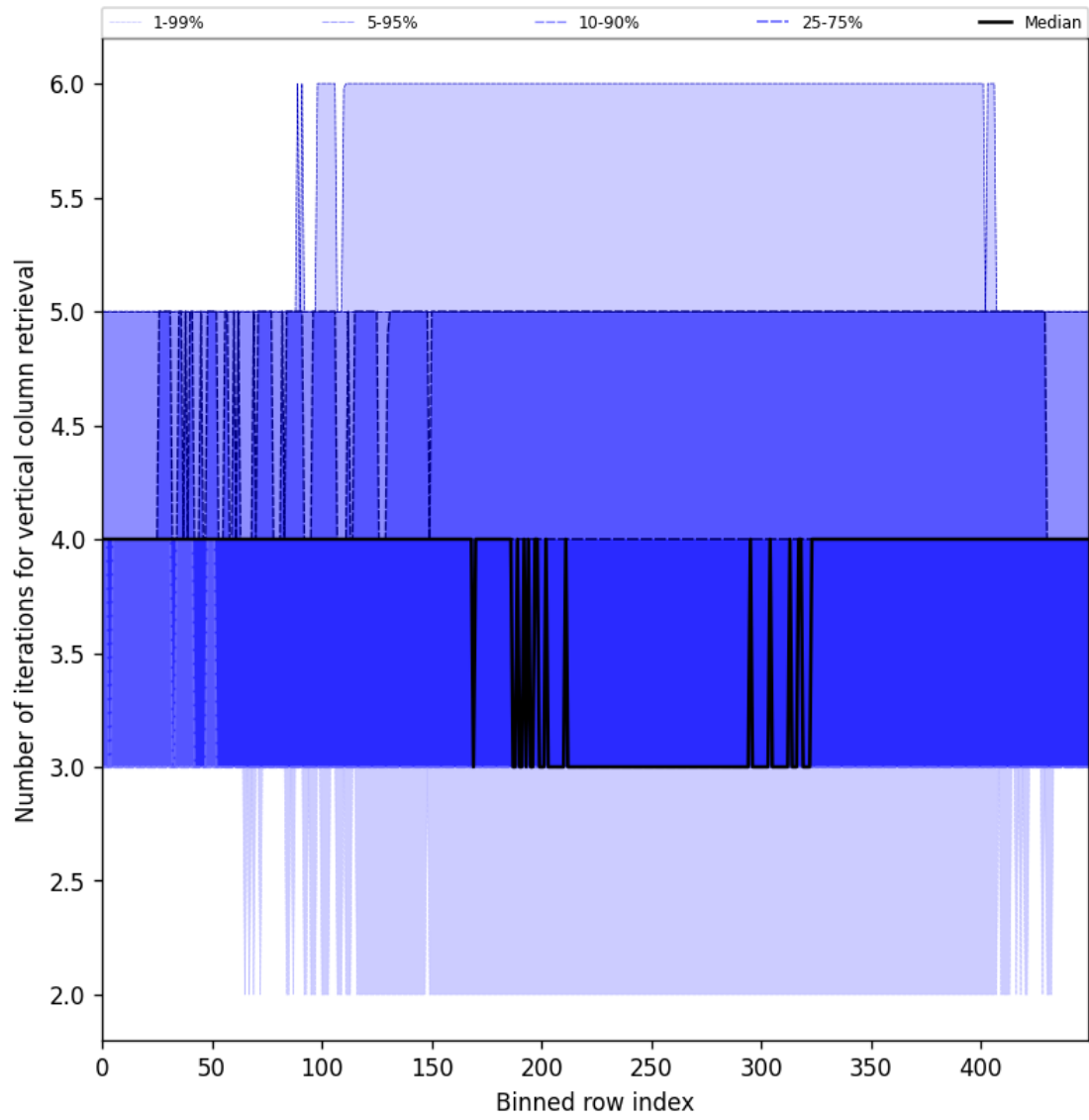
Figure 33: Along track statistics of “Number of iterations for vertical column retrieval” for 2024-11-20 to 2024-11-22
