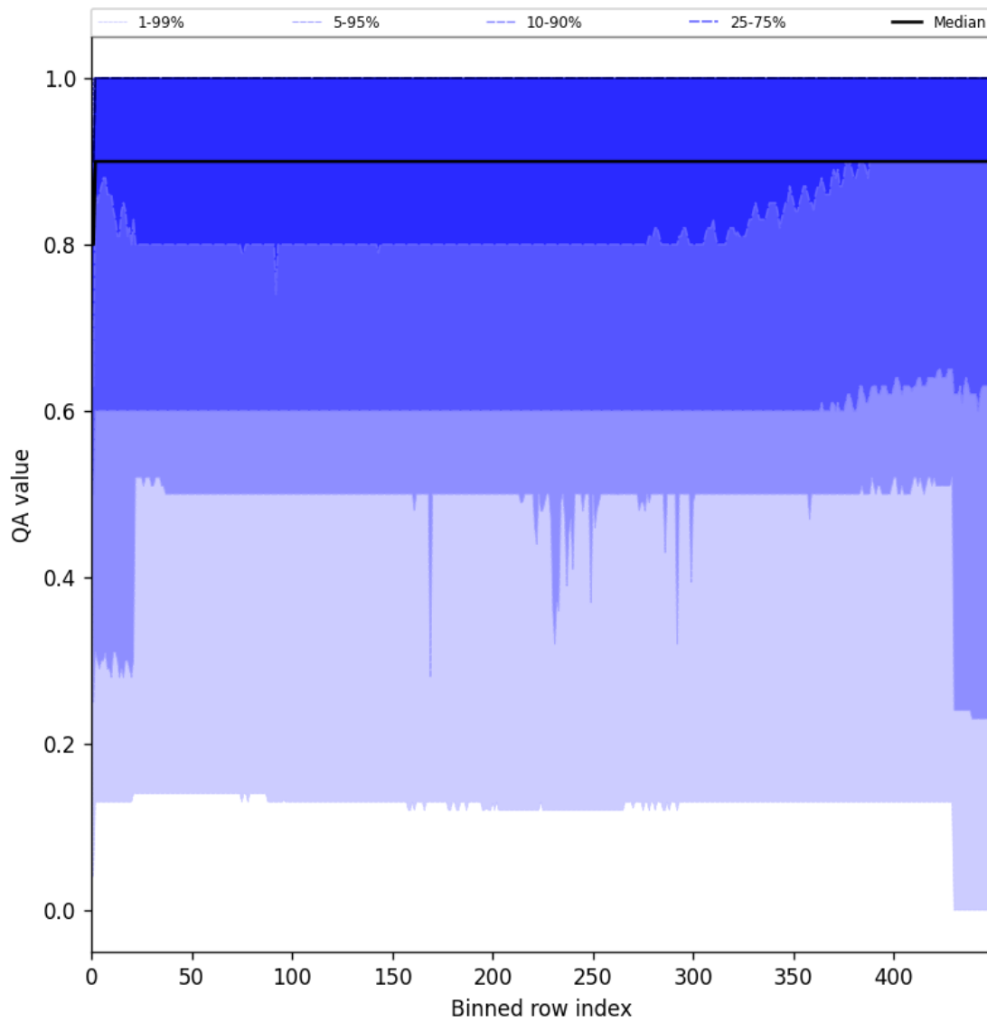
Figure 27: Along track statistics of “QA value” for 2024-11-20 to 2024-11-22
