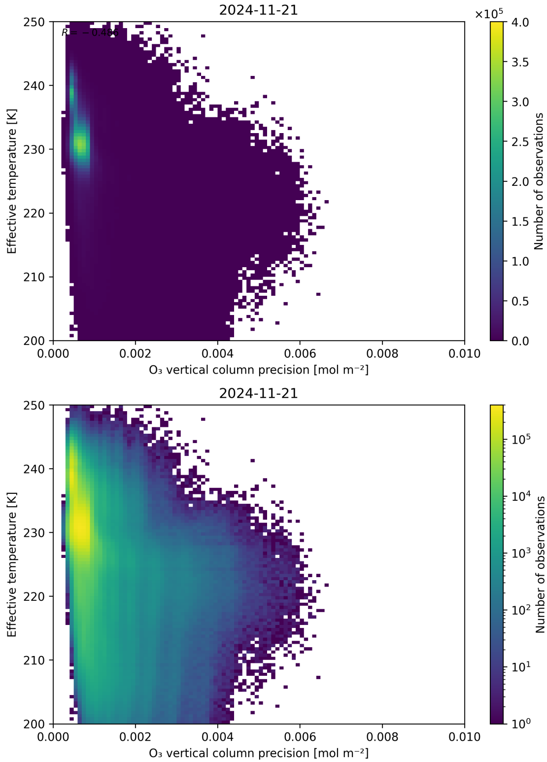
Figure 42: Scatter density plot of “O 3 vertical column precision” against “Effective temperature” for 2024-11-20 to 2024-11-22.
