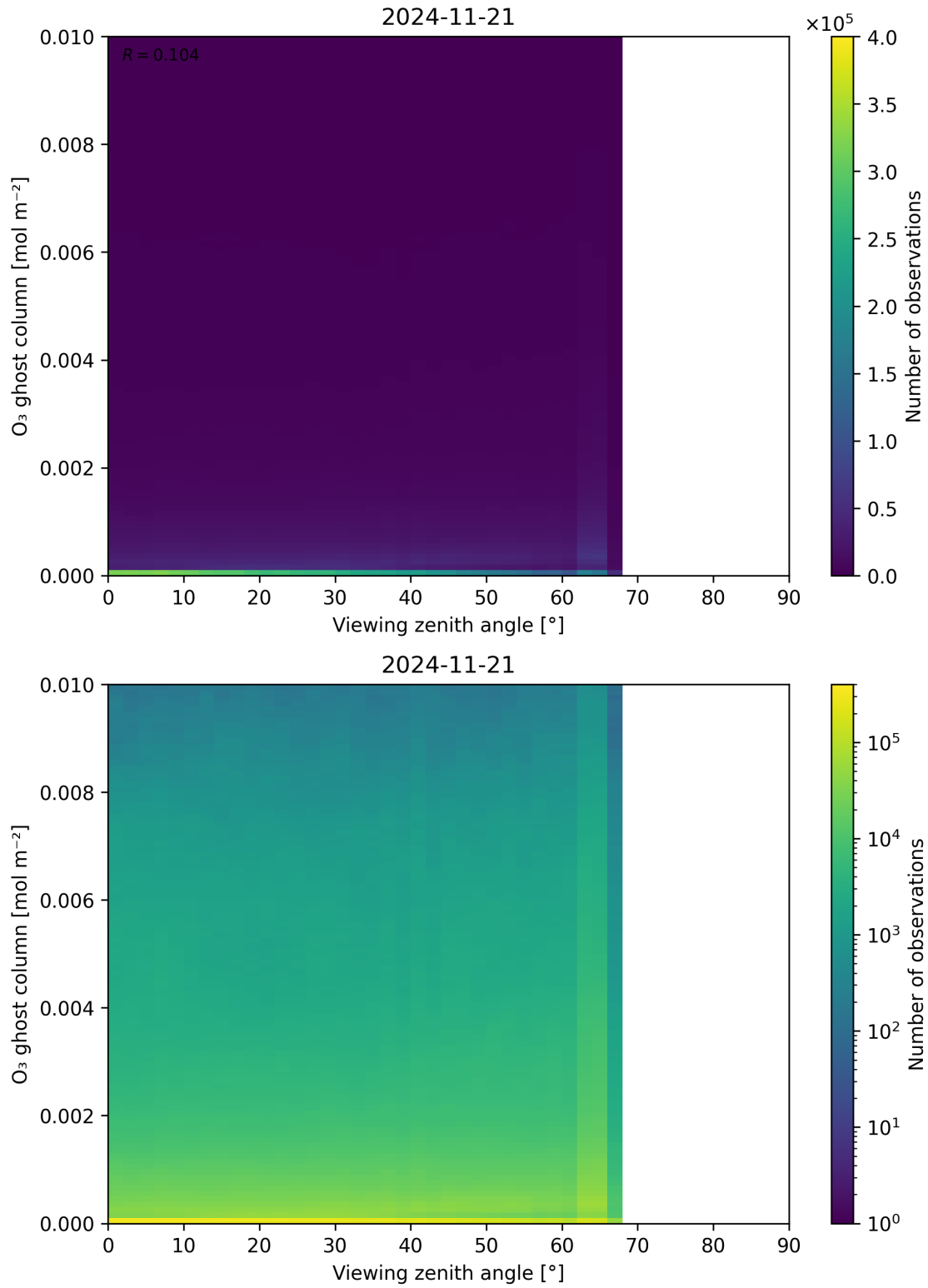
Figure 51: Scatter density plot of “Viewing zenith angle” against “O 3 ghost column” for 2024-11-20 to 2024-11-22.
