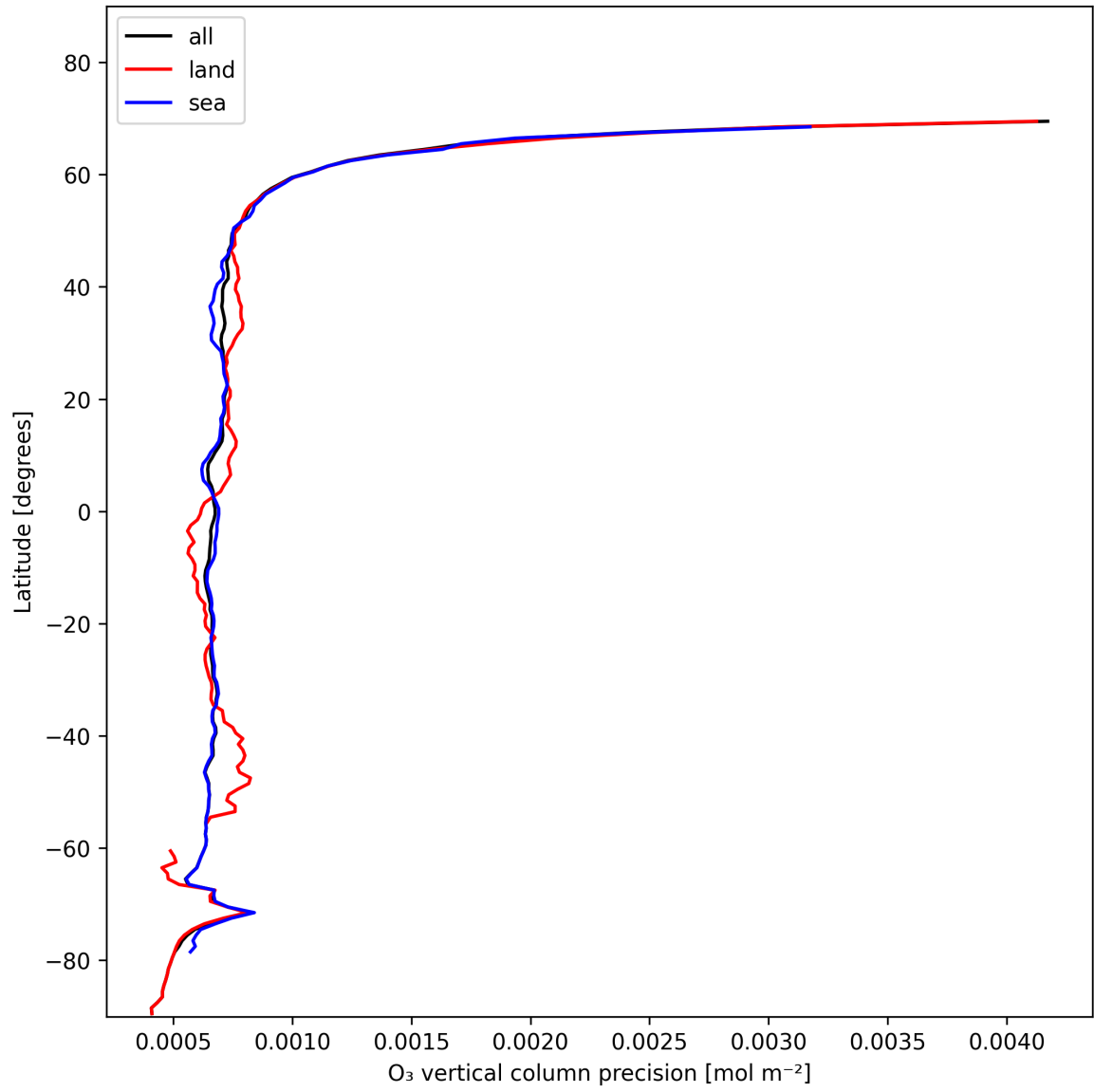
Figure 15: Zonal average of “O 3 vertical column precision” for 2024-11-20 to 2024-11-22.
