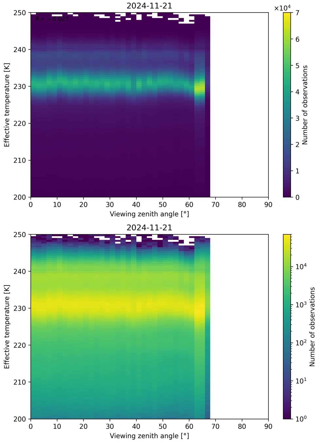
Figure 50: Scatter density plot of “Viewing zenith angle” against “Effective temperature” for 2024-11-20 to 2024-11-22.
