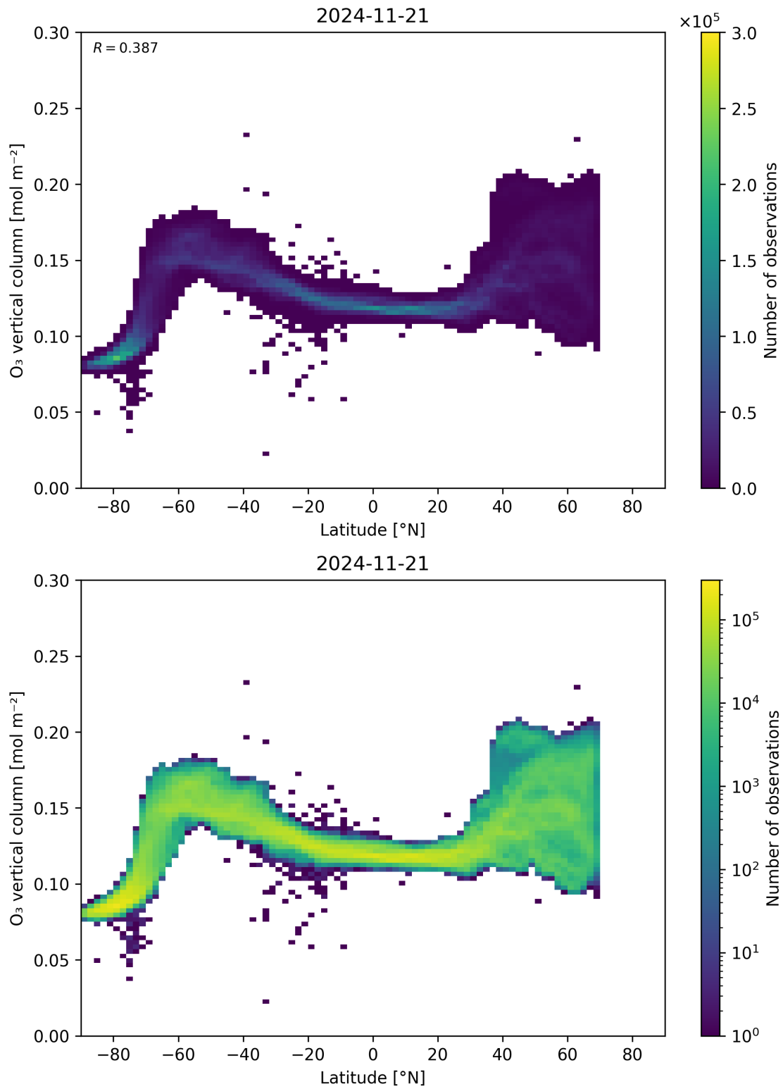
Figure 36: Scatter density plot of “Latitude” against “O 3 vertical column” for 2024-11-20 to 2024-11-22.
