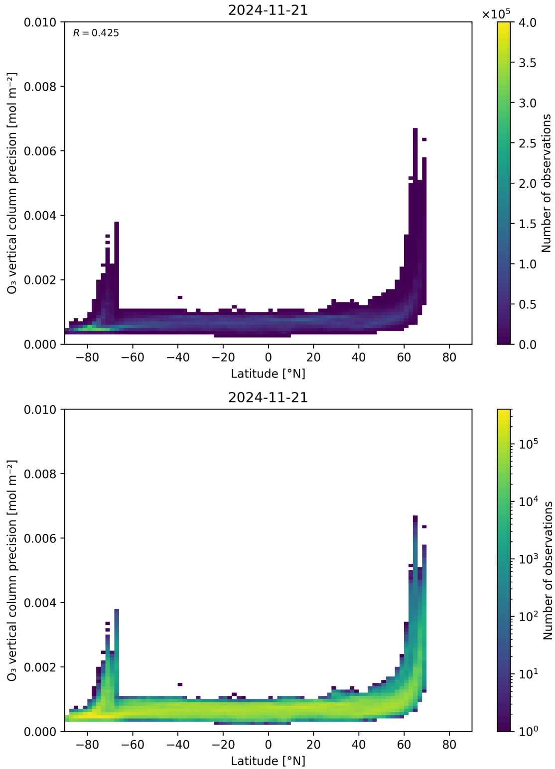
Figure 37: Scatter density plot of “Latitude” against “O 3 vertical column precision” for 2024-11-20 to 2024-11-22.
