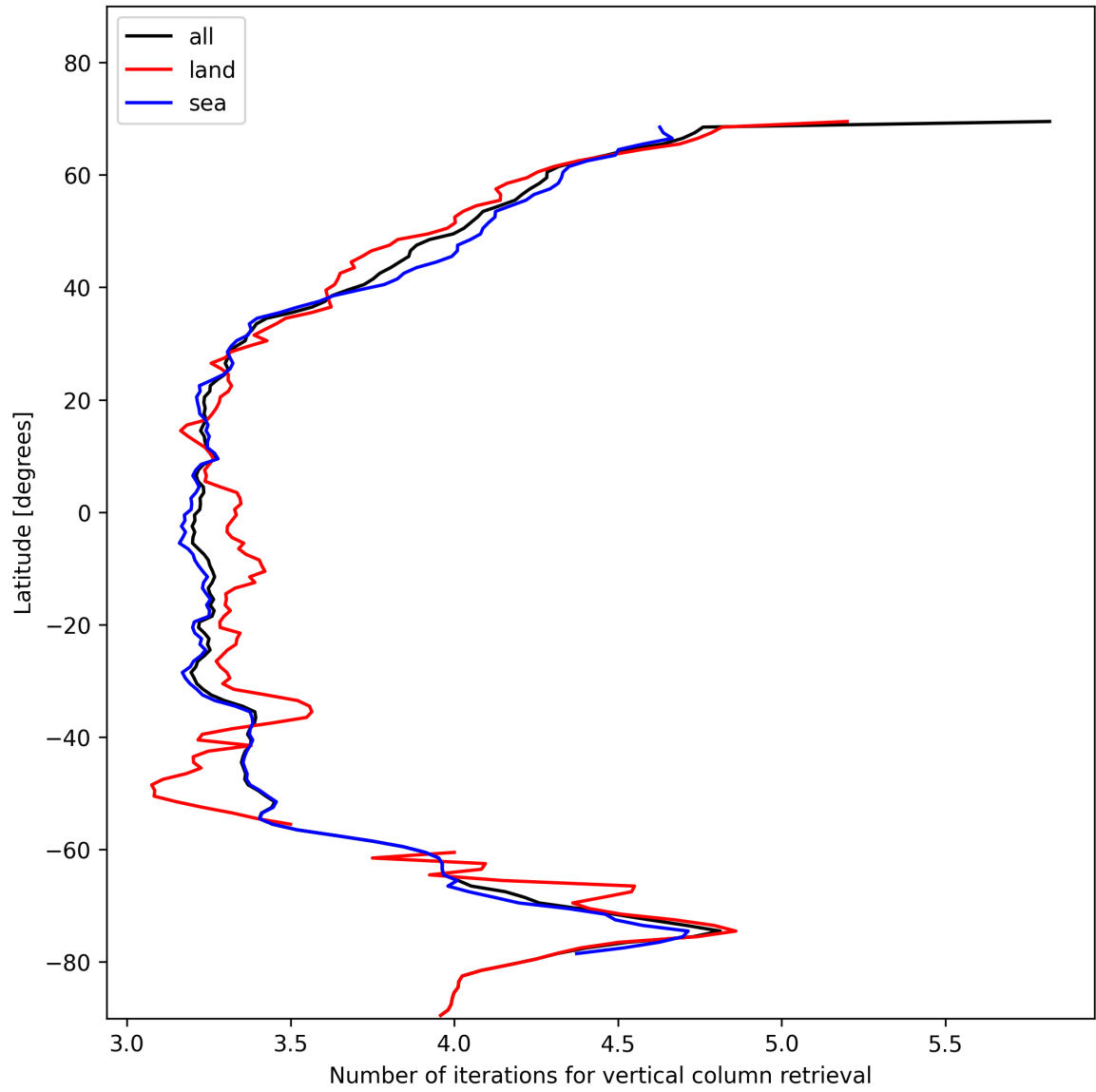
Figure 19: Zonal average of “Number of iterations for vertical column retrieval” for 2024-11-20 to 2024-11-22.
