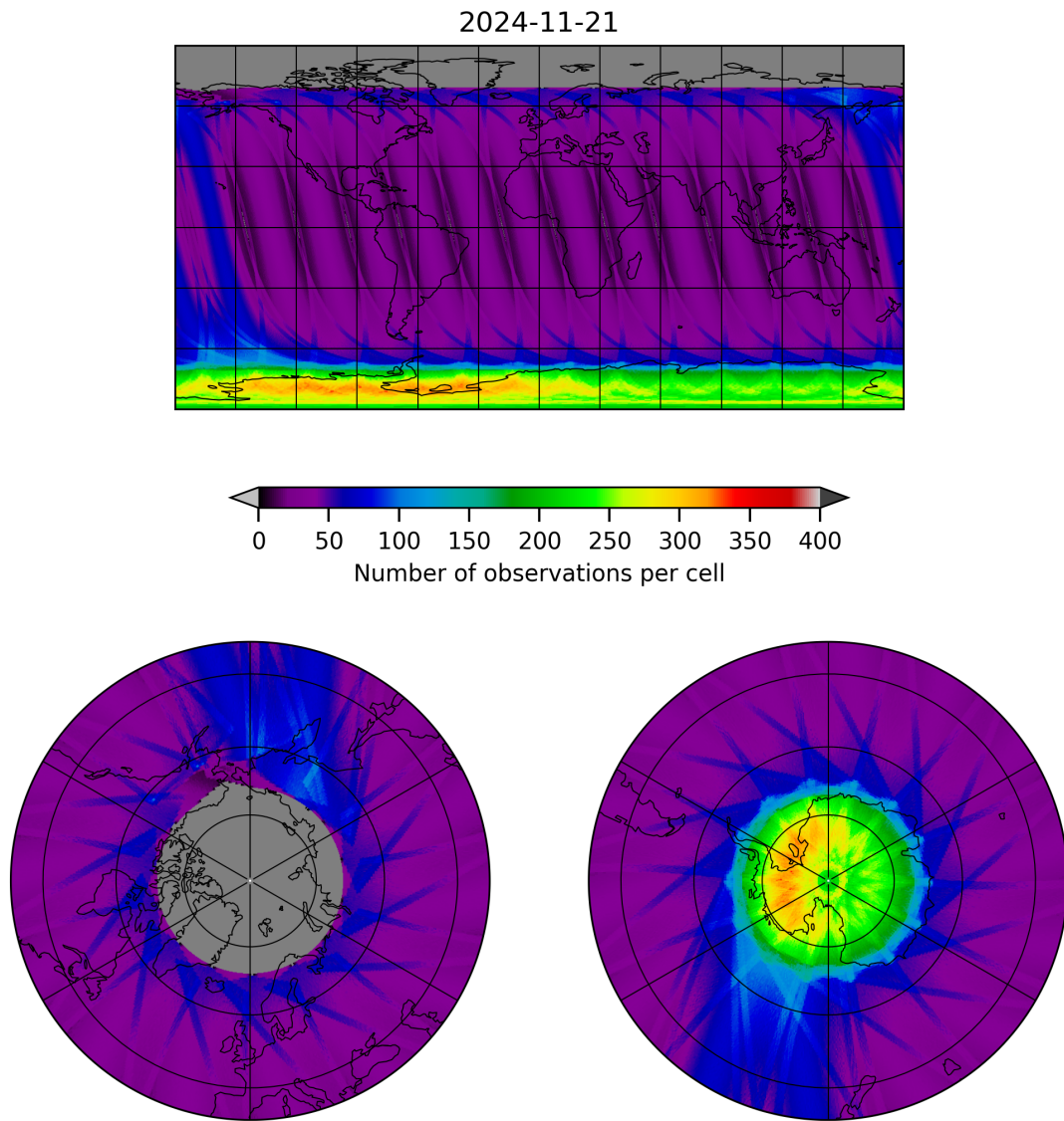
Figure 12: Map of the number of observations for 2024-11-20 to 2024-11-22
