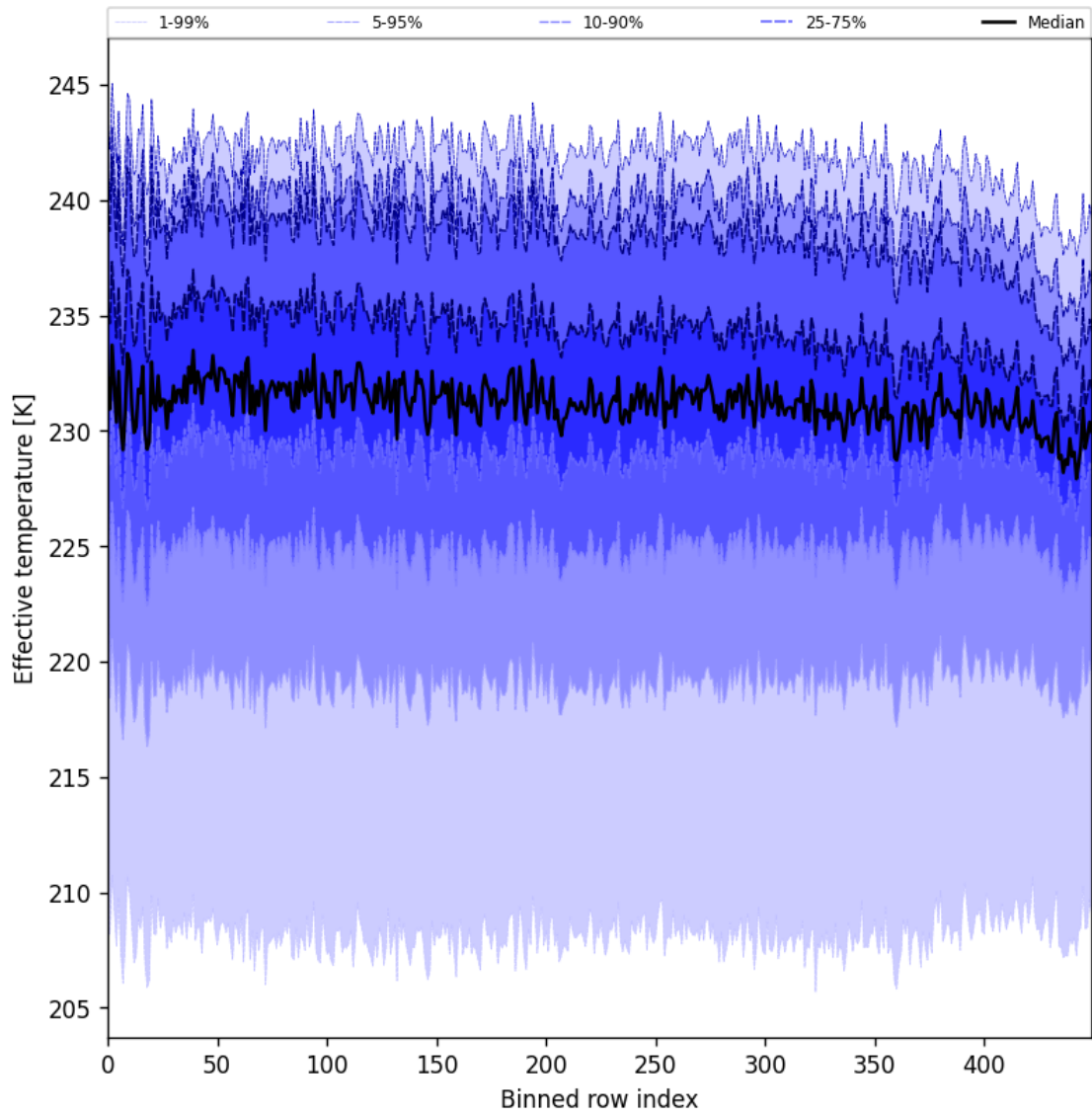
Figure 31: Along track statistics of “Effective temperature” for 2024-11-20 to 2024-11-22
