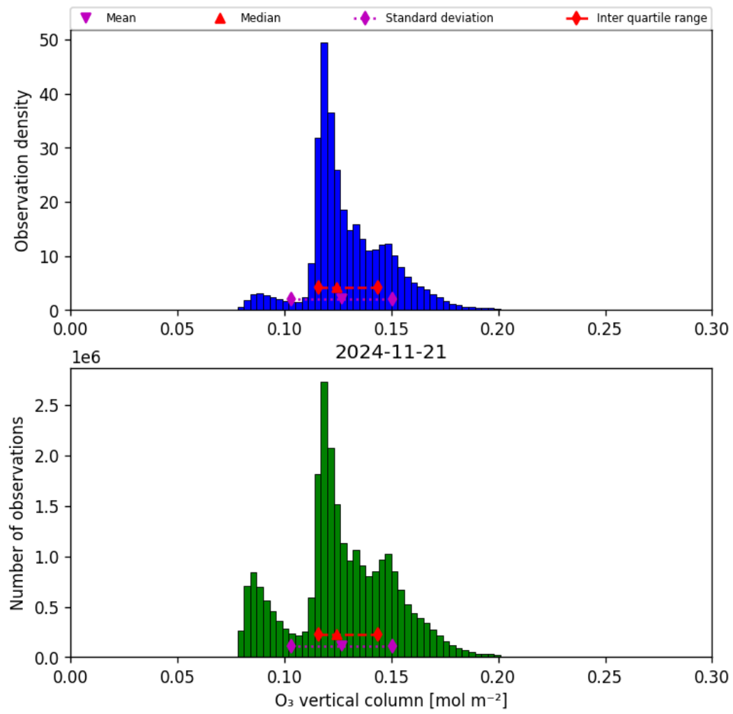
Figure 21: Histogram of “O 3 vertical column” for 2024-11-20 to 2024-11-22
