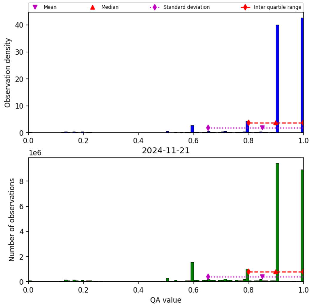
Figure 20: Histogram of “QA value” for 2024-11-20 to 2024-11-22
