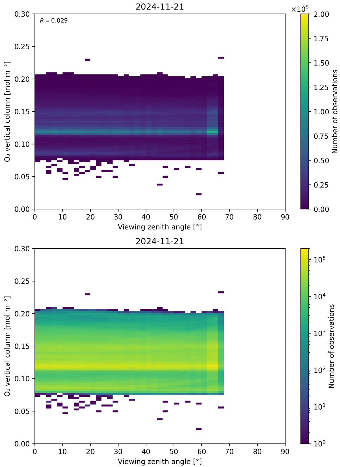
Figure 52: Scatter density plot of “Viewing zenith angle” against “O 3 vertical column” for 2024-11-20 to 2024-11-22.
