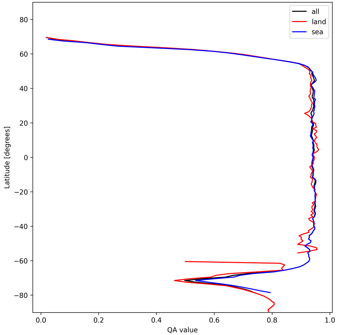
Figure 13: Zonal average of “QA value” for 2024-11-20 to 2024-11-22.
