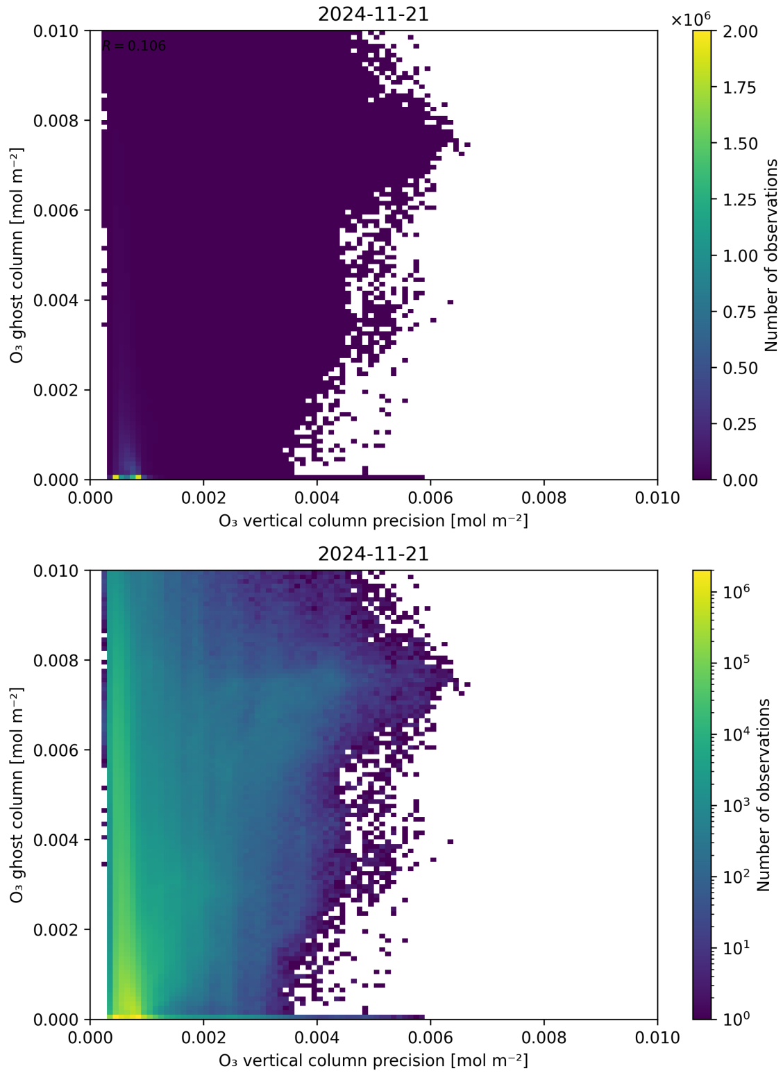
Figure 43: Scatter density plot of “ \text{O}_3 vertical column precision” against “ \text{O}_3 ghost column” for 2024-11-20 to 2024-11-22.
