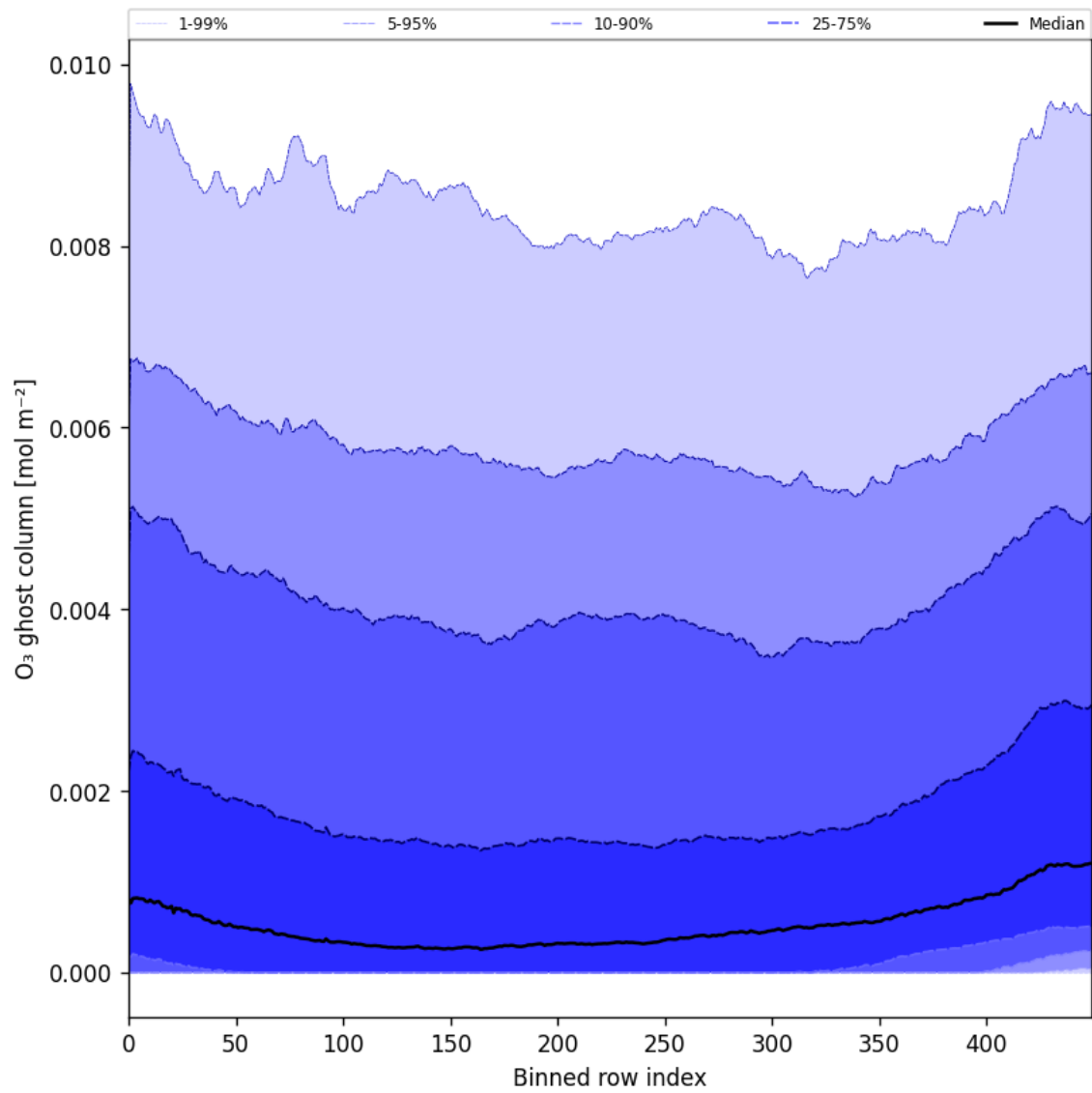
Figure 32: Along track statistics of "O 3 ghost column" for 2024-11-20 to 2024-11-22
