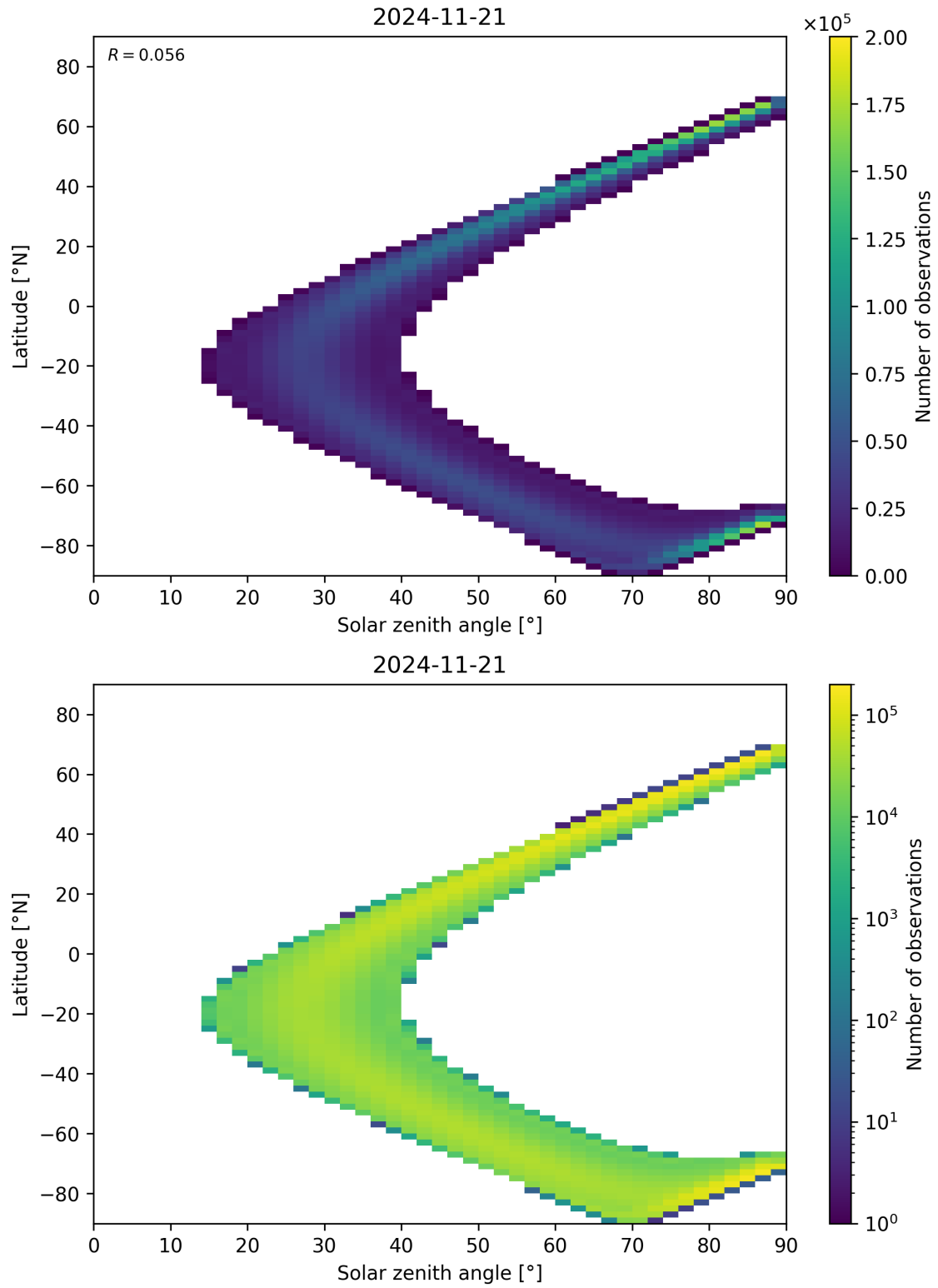
Figure 44: Scatter density plot of “Solar zenith angle” against “Latitude” for 2024-11-20 to 2024-11-22.
