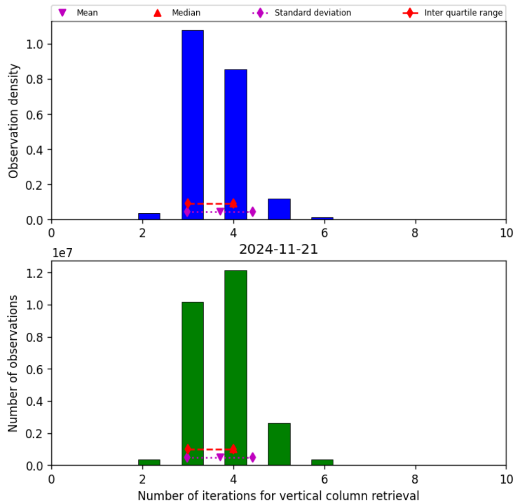
Figure 26: Histogram of “Number of iterations for vertical column retrieval” for 2024-11-20 to 2024-11-22
