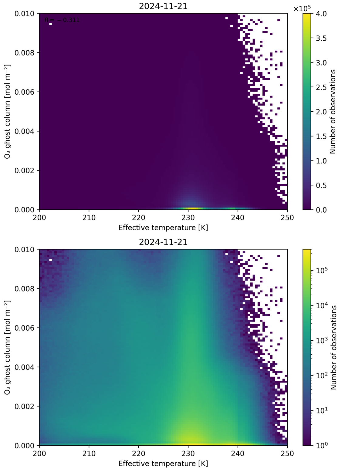
Figure 38: Scatter density plot of “Effective temperature” against “O 3 ghost column” for 2024-11-20 to 2024-11-22.
