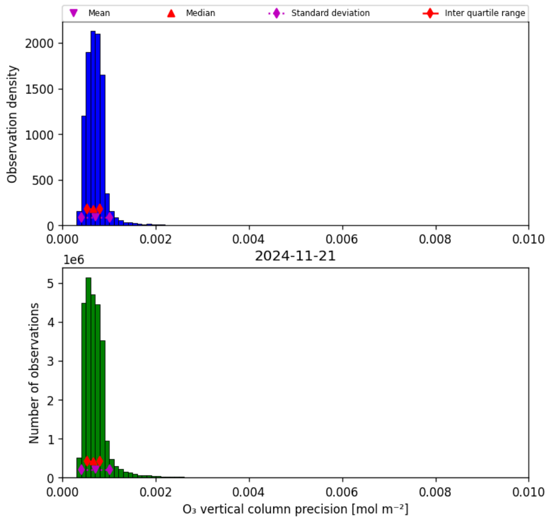
Figure 22: Histogram of “O 3 vertical column precision” for 2024-11-20 to 2024-11-22
