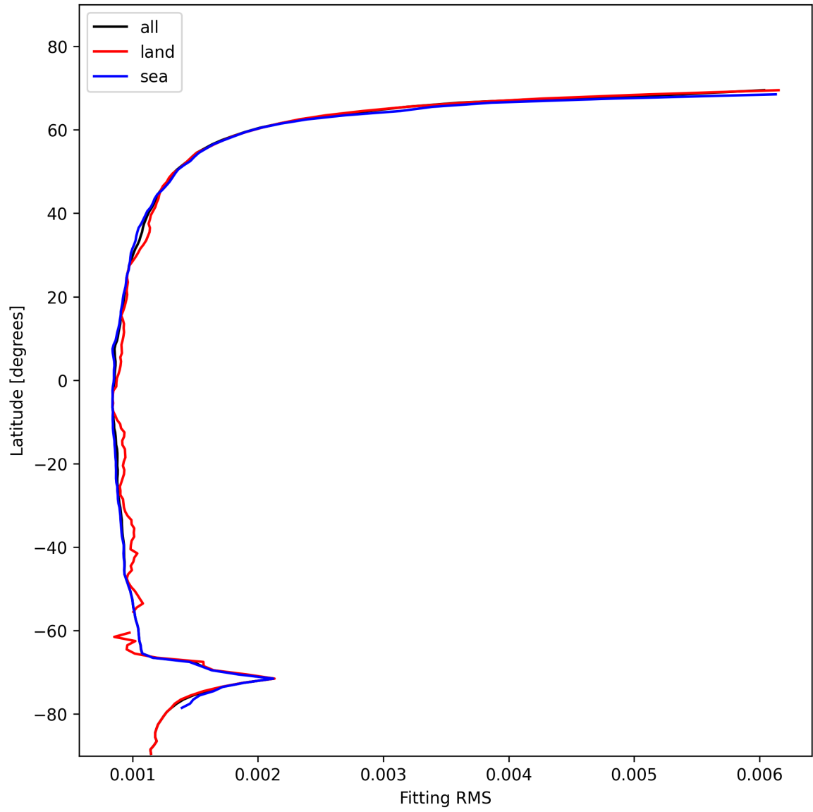
Figure 16: Zonal average of “Fitting RMS” for 2024-11-20 to 2024-11-22.
