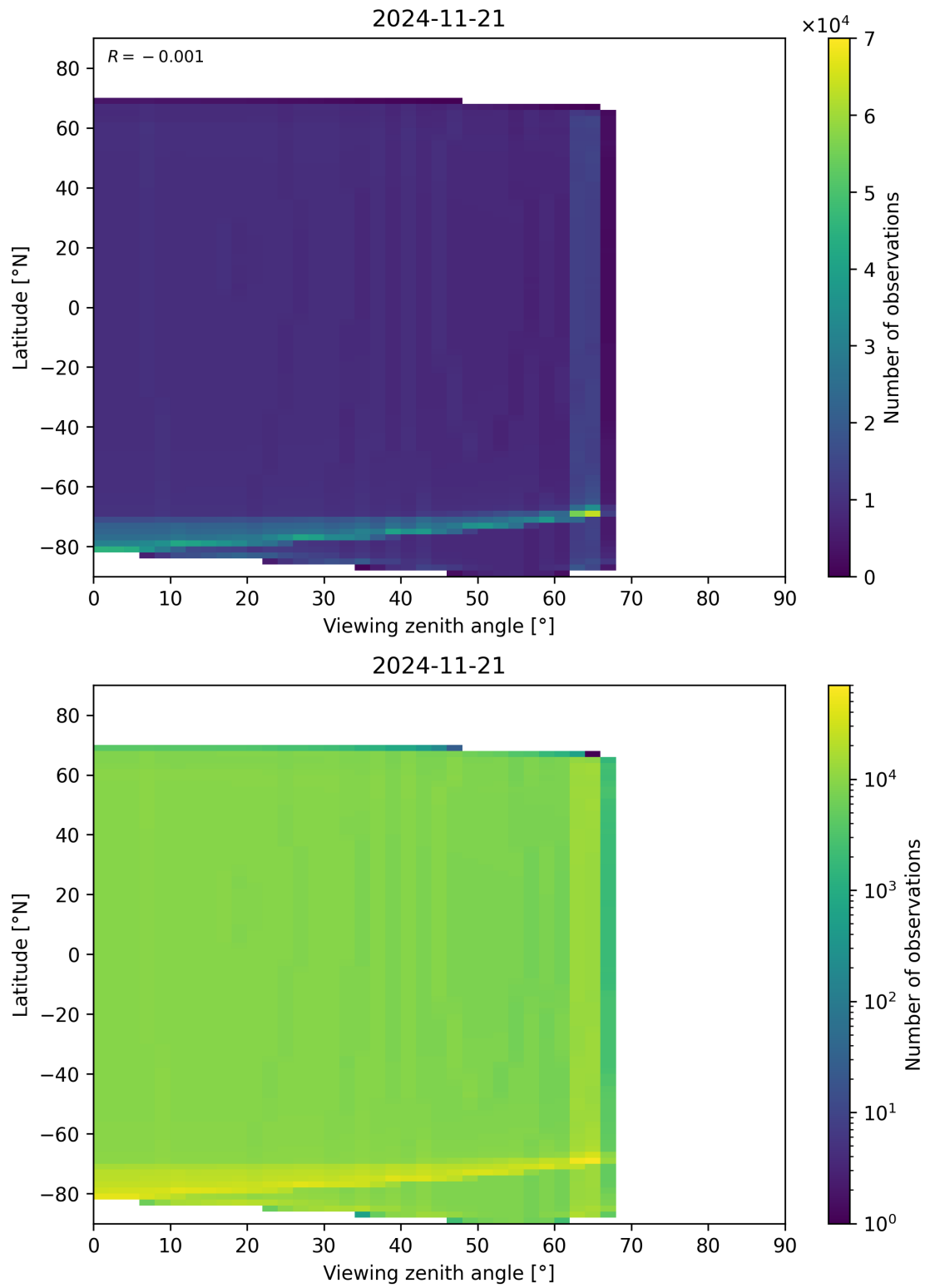
Figure 49: Scatter density plot of “Viewing zenith angle” against “Latitude” for 2024-11-20 to 2024-11-22.
