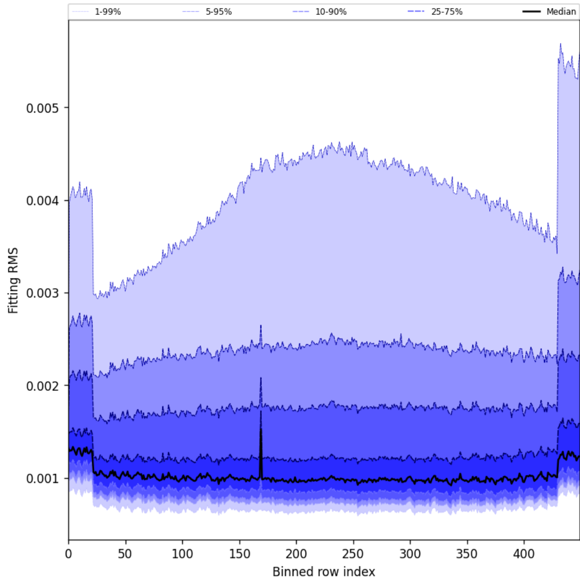
Figure 30: Along track statistics of “Fitting RMS” for 2024-11-20 to 2024-11-22
