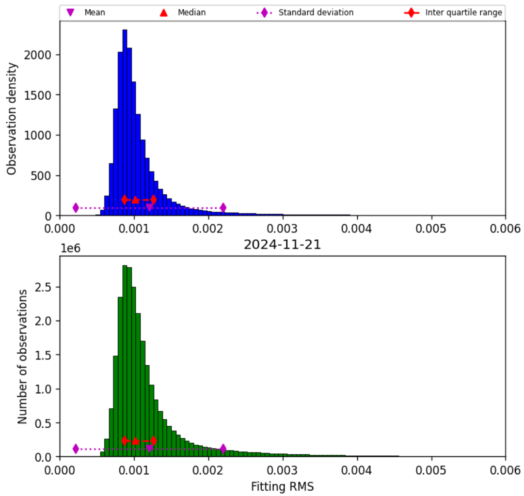
Figure 23: Histogram of “Fitting RMS” for 2024-11-20 to 2024-11-22
