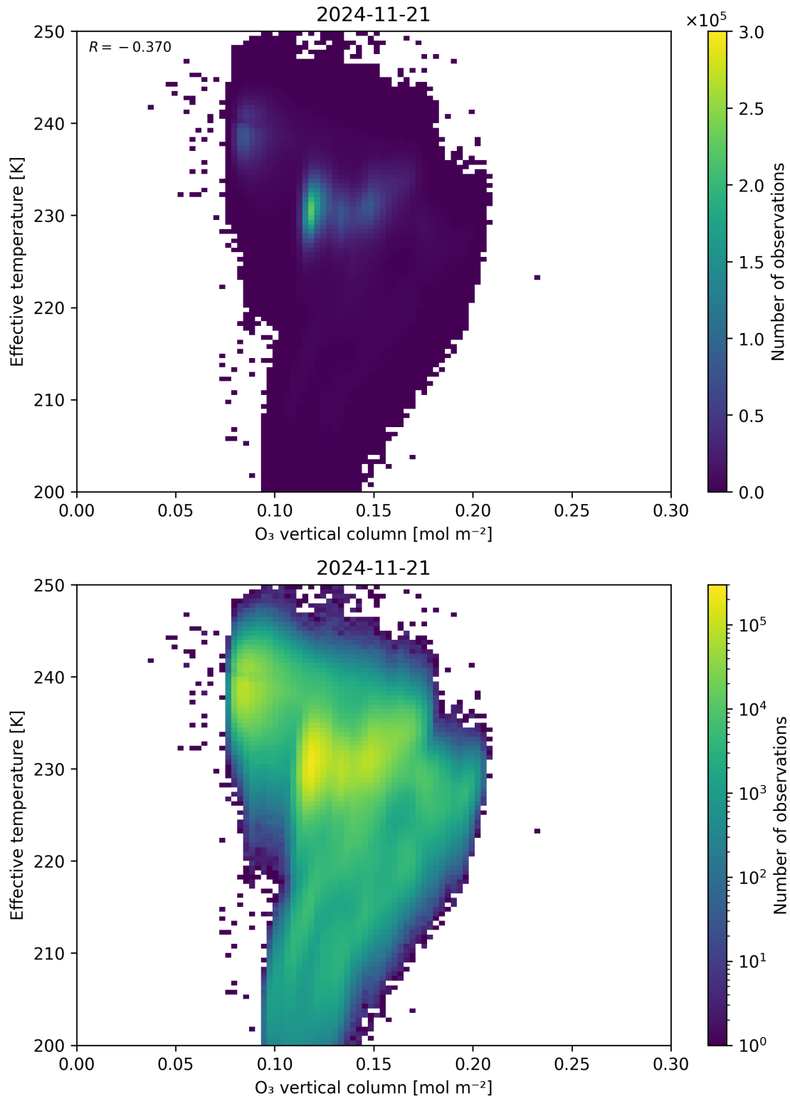
Figure 39: Scatter density plot of “O 3 vertical column” against “Effective temperature” for 2024-11-20 to 2024-11-22.
