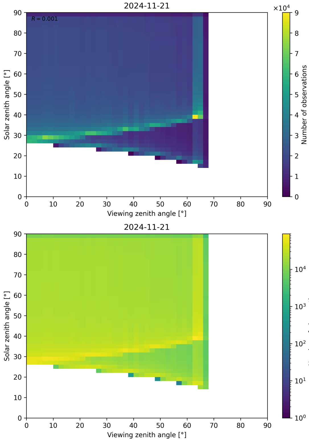
Figure 54: Scatter density plot of “Viewing zenith angle” against “Solar zenith angle” for 2024-11-20 to 2024-11-22.
