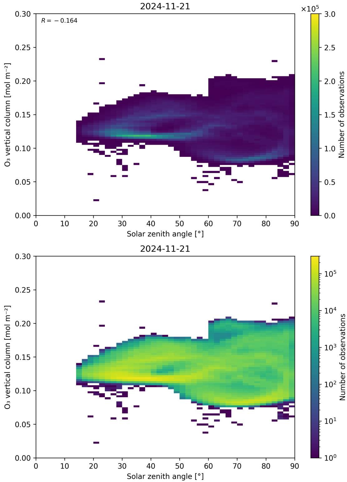
Figure 47: Scatter density plot of “Solar zenith angle” against “O 3 vertical column” for 2024-11-20 to 2024-11-22.
