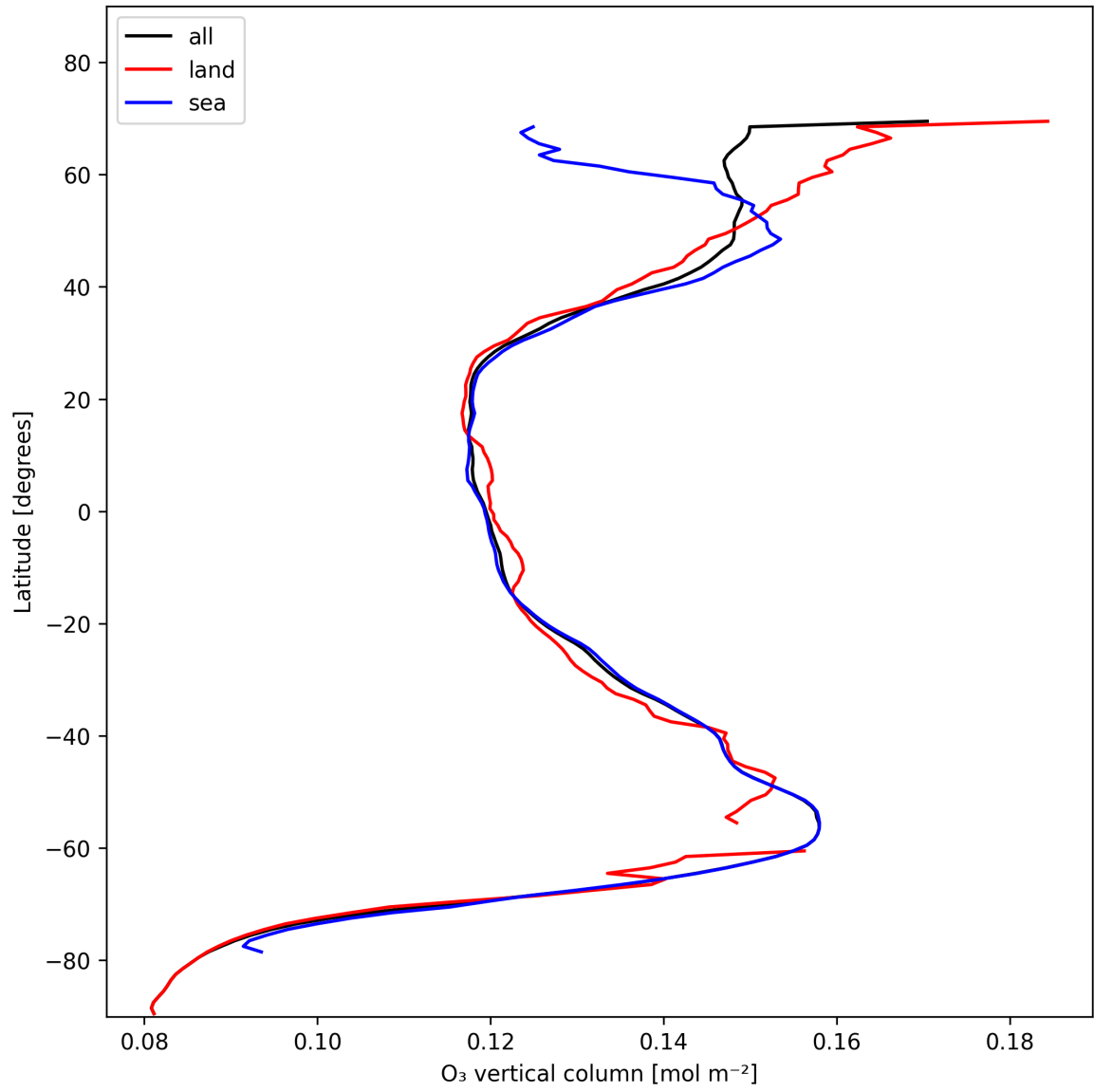
Figure 14: Zonal average of “O 3 vertical column” for 2024-11-20 to 2024-11-22.
