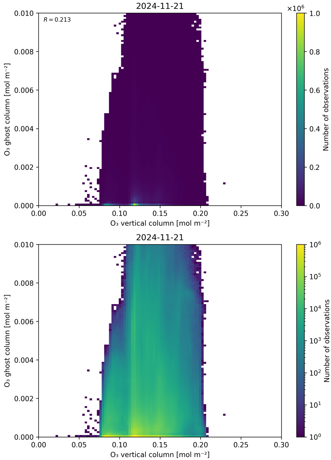
Figure 40: Scatter density plot of “O 3 vertical column” against “O 3 ghost column” for 2024-11-20 to 2024-11-22.
