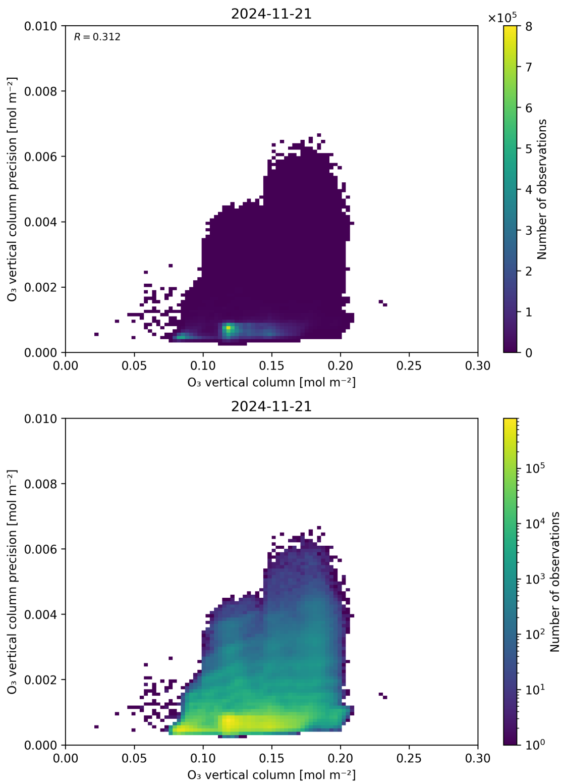
Figure 41: Scatter density plot of “O 3 vertical column” against “O 3 vertical column precision” for 2024-11-20 to 2024-11-22.
