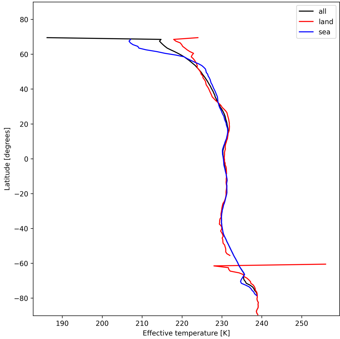
Figure 17: Zonal average of “Effective temperature” for 2024-11-20 to 2024-11-22.
