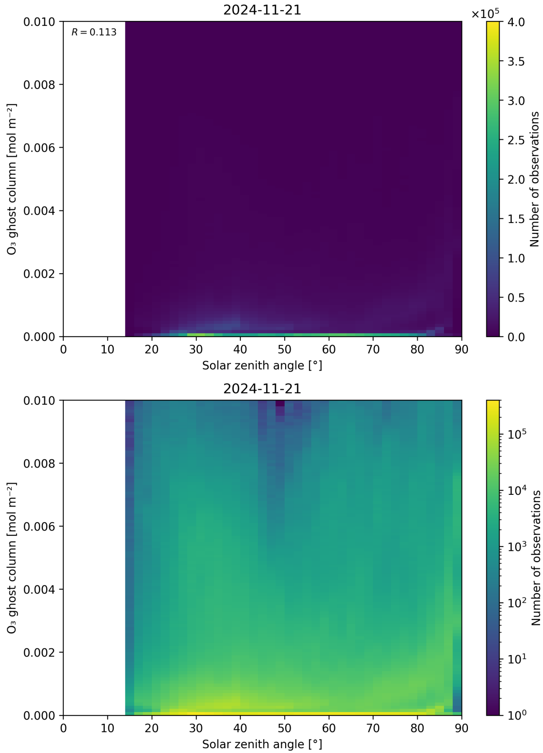
Figure 46: Scatter density plot of “Solar zenith angle” against “O 3 ghost column” for 2024-11-20 to 2024-11-22.
