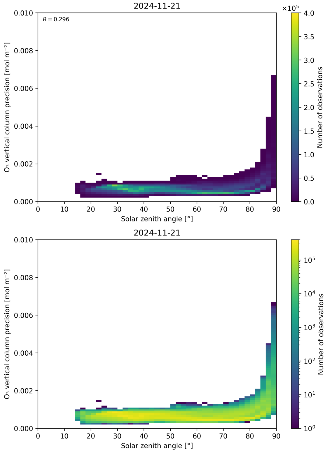
Figure 48: Scatter density plot of “Solar zenith angle” against “O 3 vertical column precision” for 2024-11-20 to 2024-11-22.
