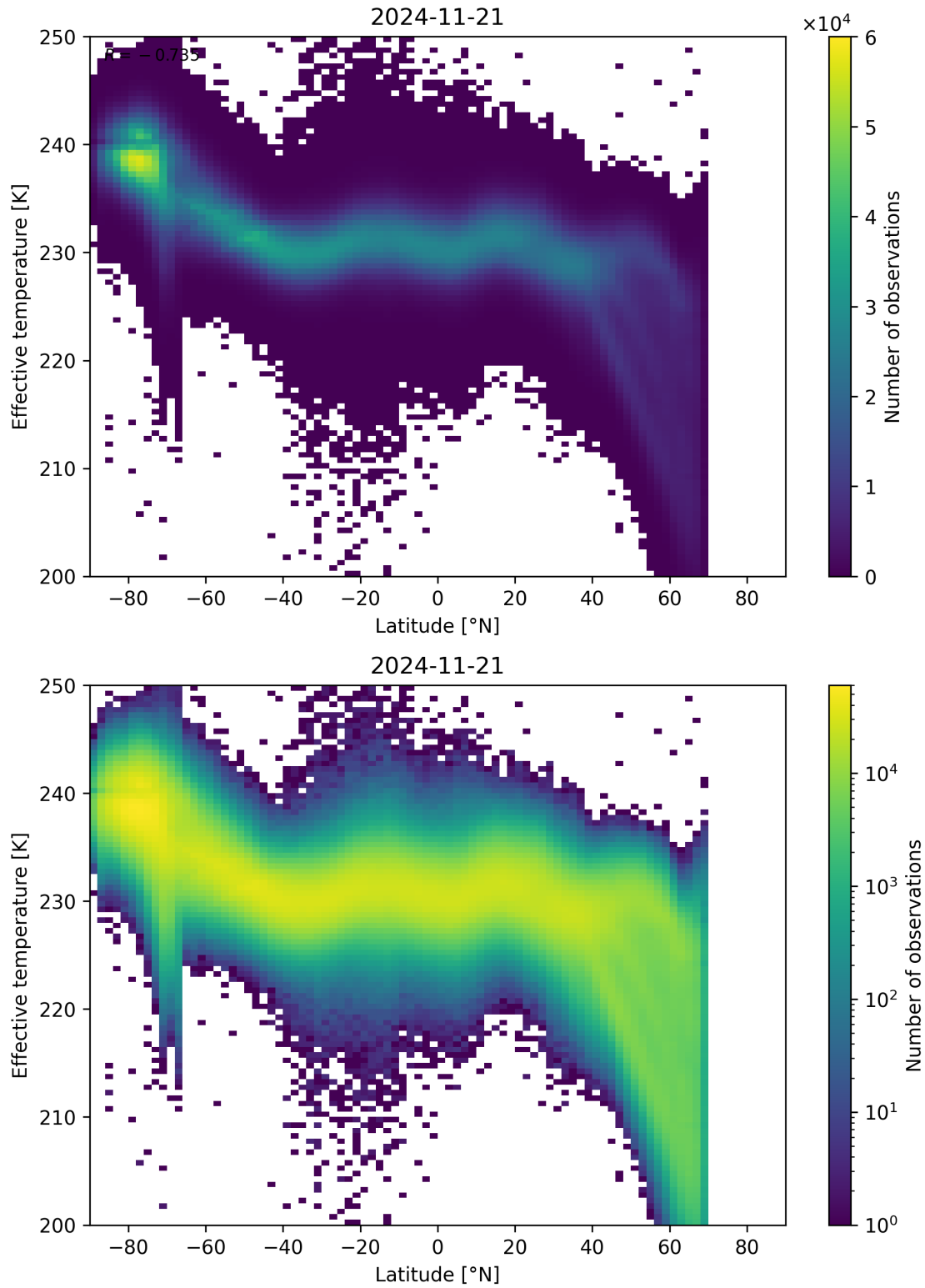
Figure 34: Scatter density plot of “Latitude” against “Effective temperature” for 2024-11-20 to 2024-11-22.
