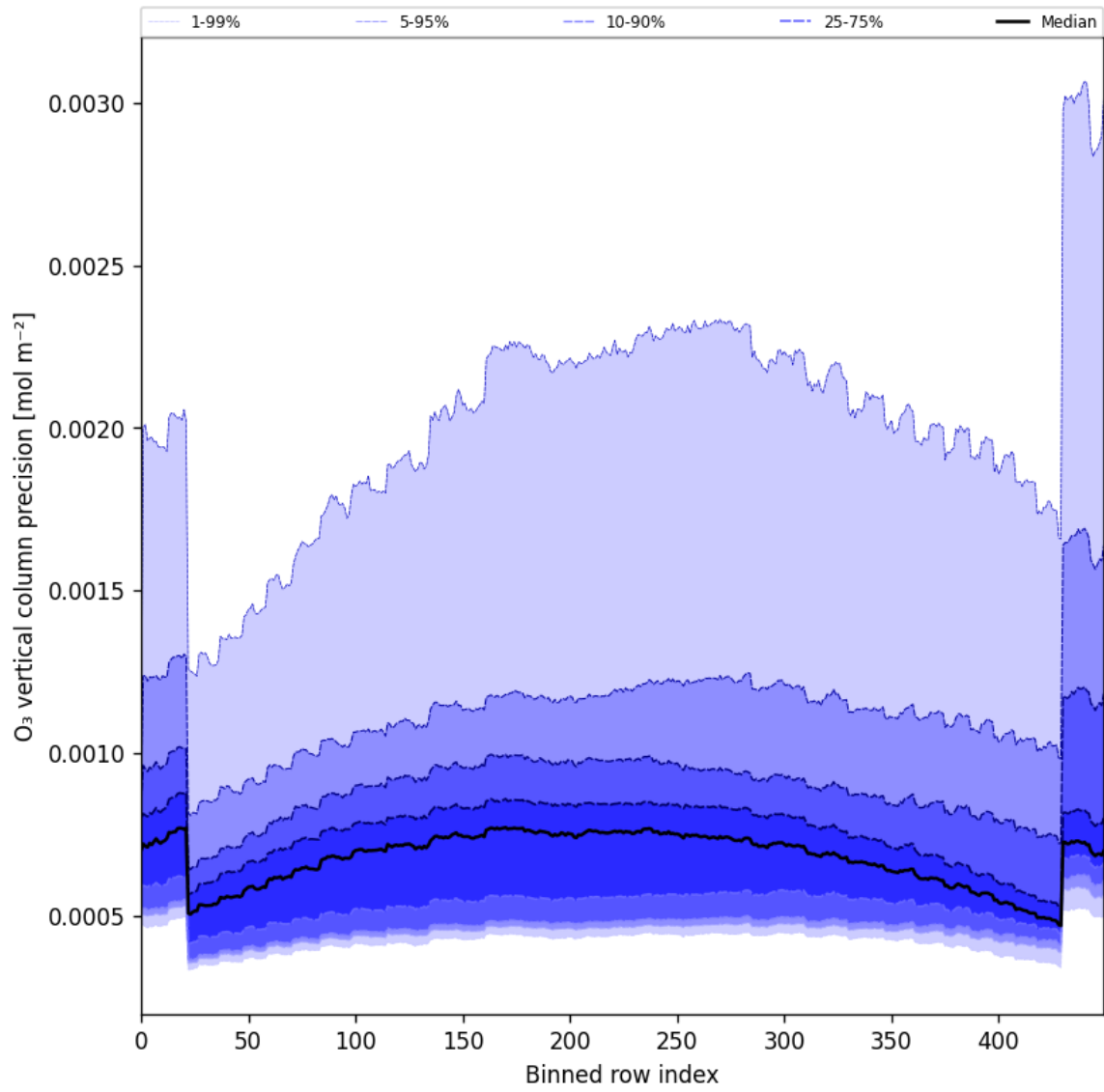
Figure 29: Along track statistics of “O 3 vertical column precision” for 2024-11-20 to 2024-11-22
