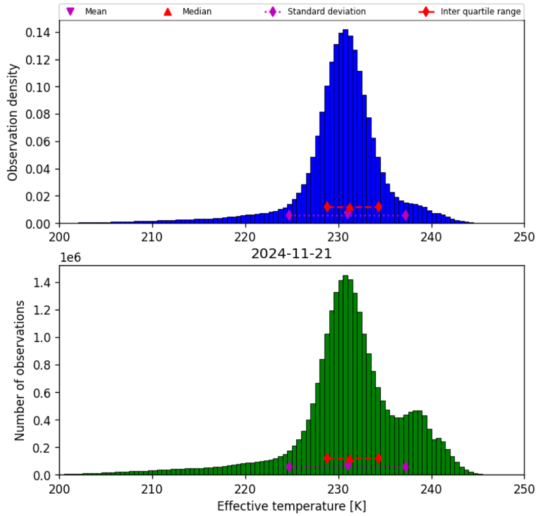
Figure 24: Histogram of “Effective temperature” for 2024-11-20 to 2024-11-22
