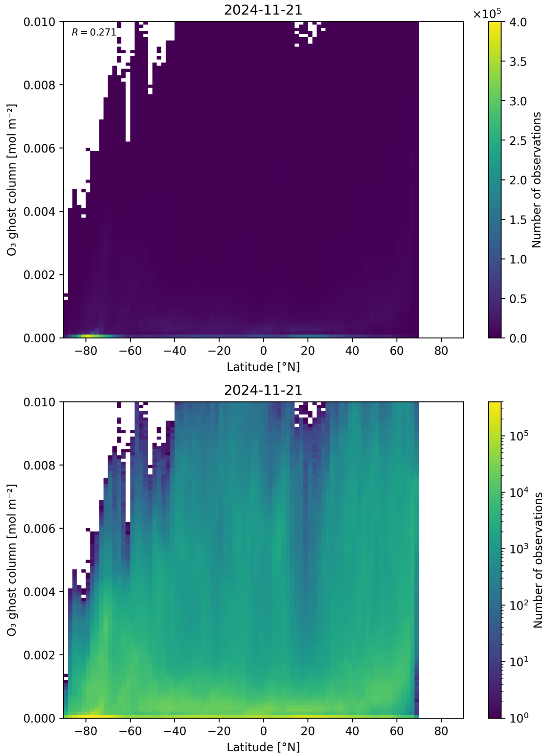
Figure 35: Scatter density plot of “Latitude” against “O 3 ghost column” for 2024-11-20 to 2024-11-22.
