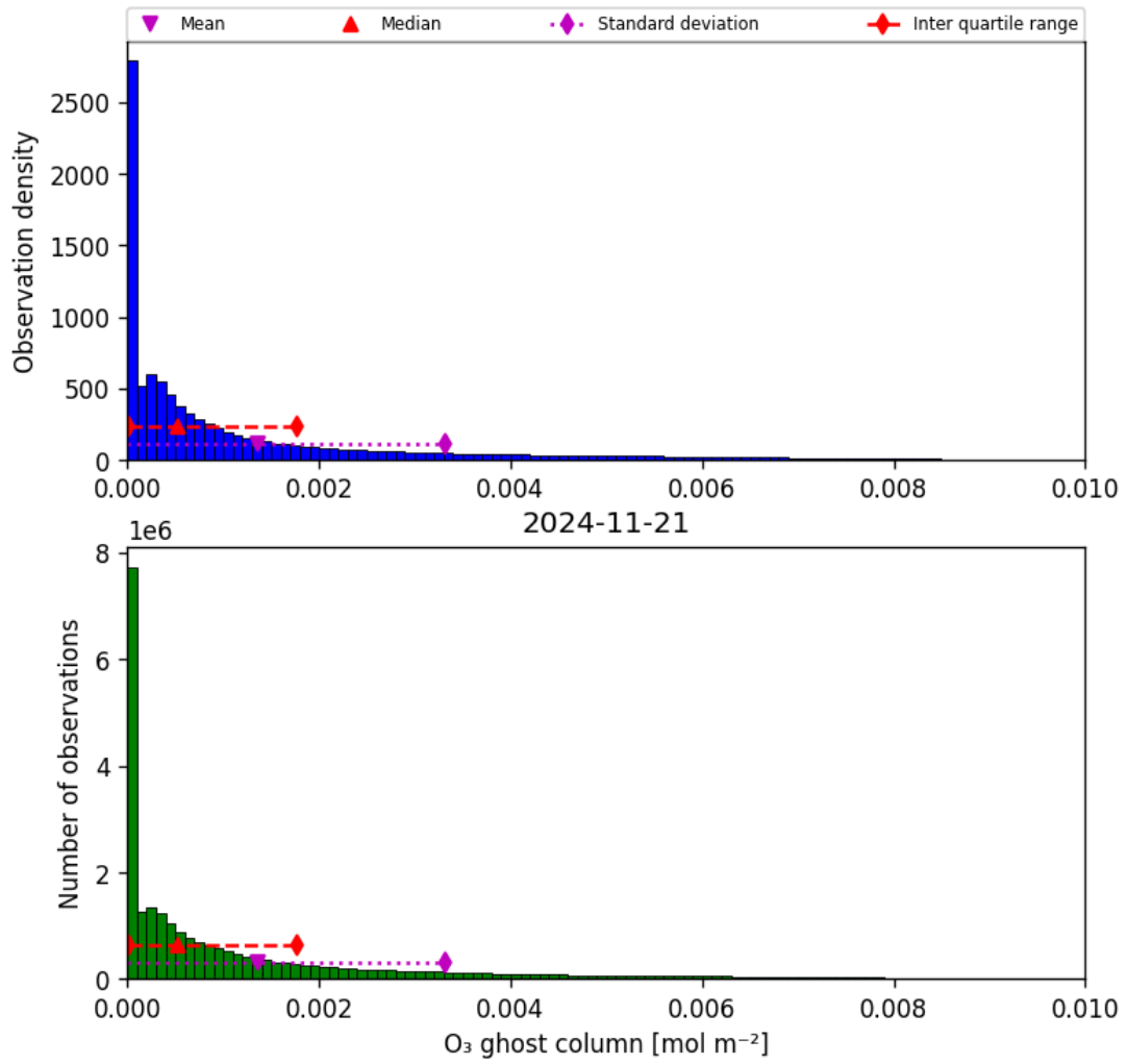
Figure 25: Histogram of "O 3 ghost column" for 2024-11-20 to 2024-11-22
