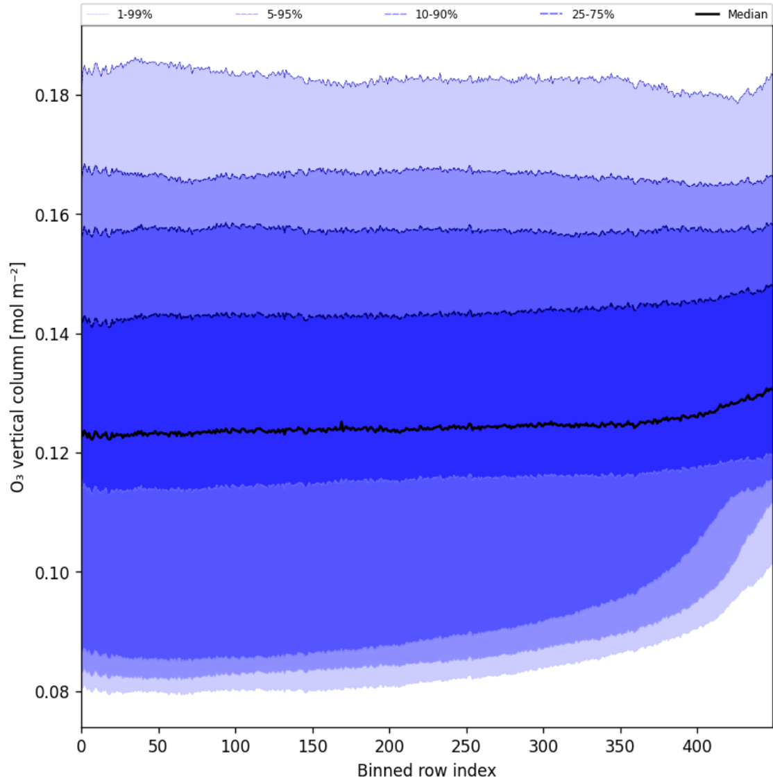
Figure 28: Along track statistics of “O 3 vertical column” for 2024-11-20 to 2024-11-22
