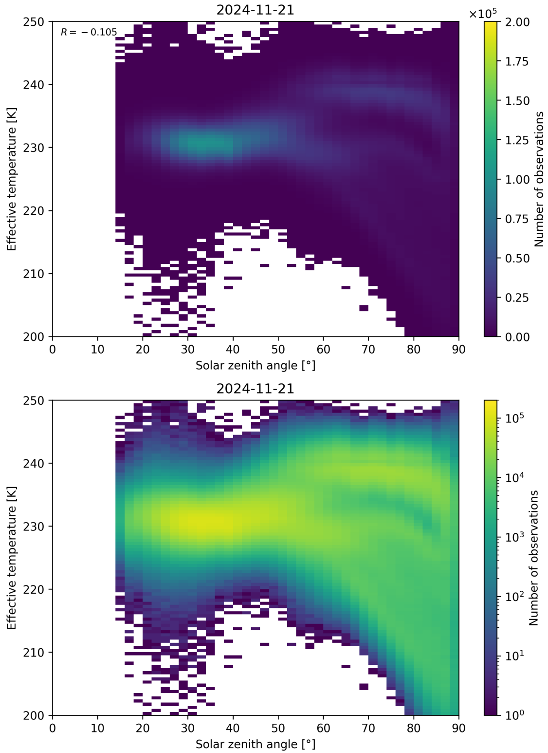
Figure 45: Scatter density plot of “Solar zenith angle” against “Effective temperature” for 2024-11-20 to 2024-11-22.
