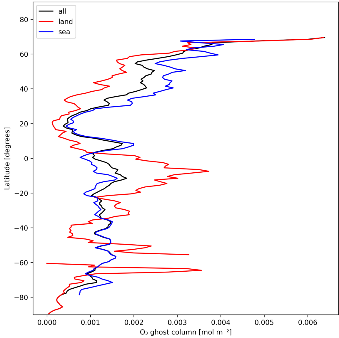
Figure 18: Zonal average of "O 3 ghost column" for 2024-11-20 to 2024-11-22.
