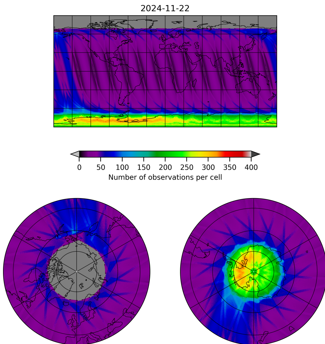
Figure 12: Map of the number of observations for 2024-11-21 to 2024-11-23
