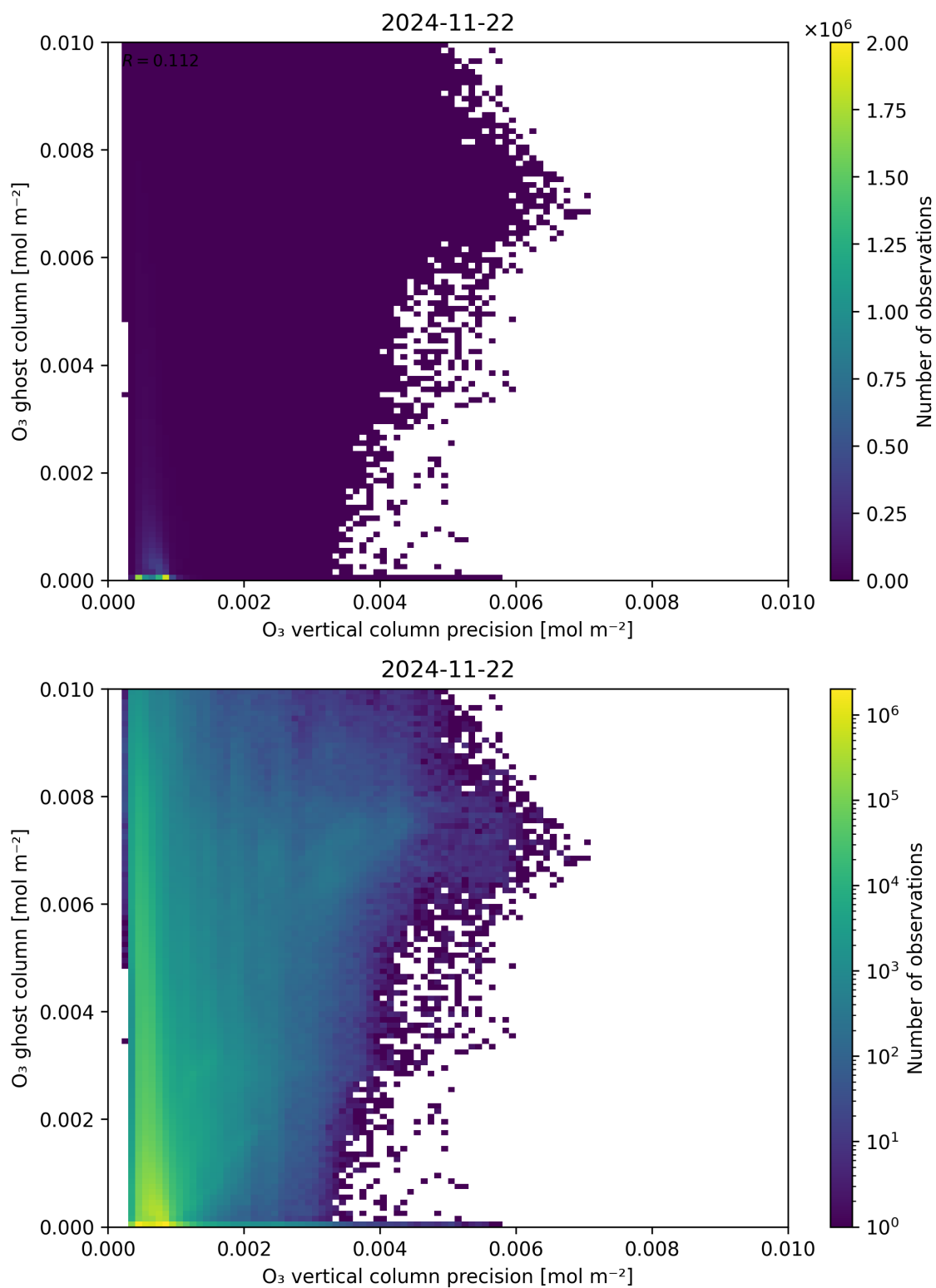
Figure 43: Scatter density plot of “O 3 vertical column precision” against “O 3 ghost column” for 2024-11-21 to 2024-11-23.
