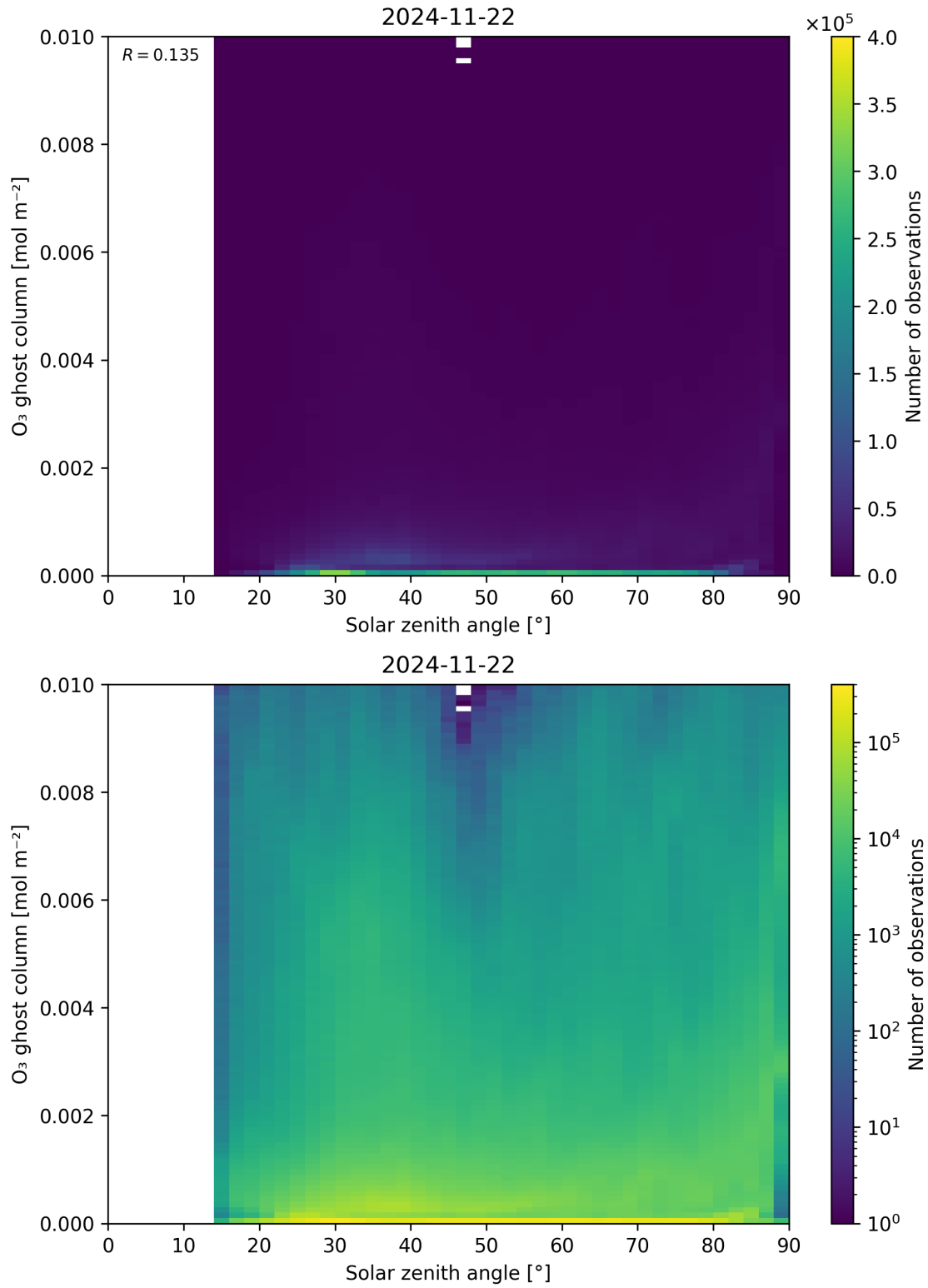
Figure 46: Scatter density plot of “Solar zenith angle” against “O 3 ghost column” for 2024-11-21 to 2024-11-23.
