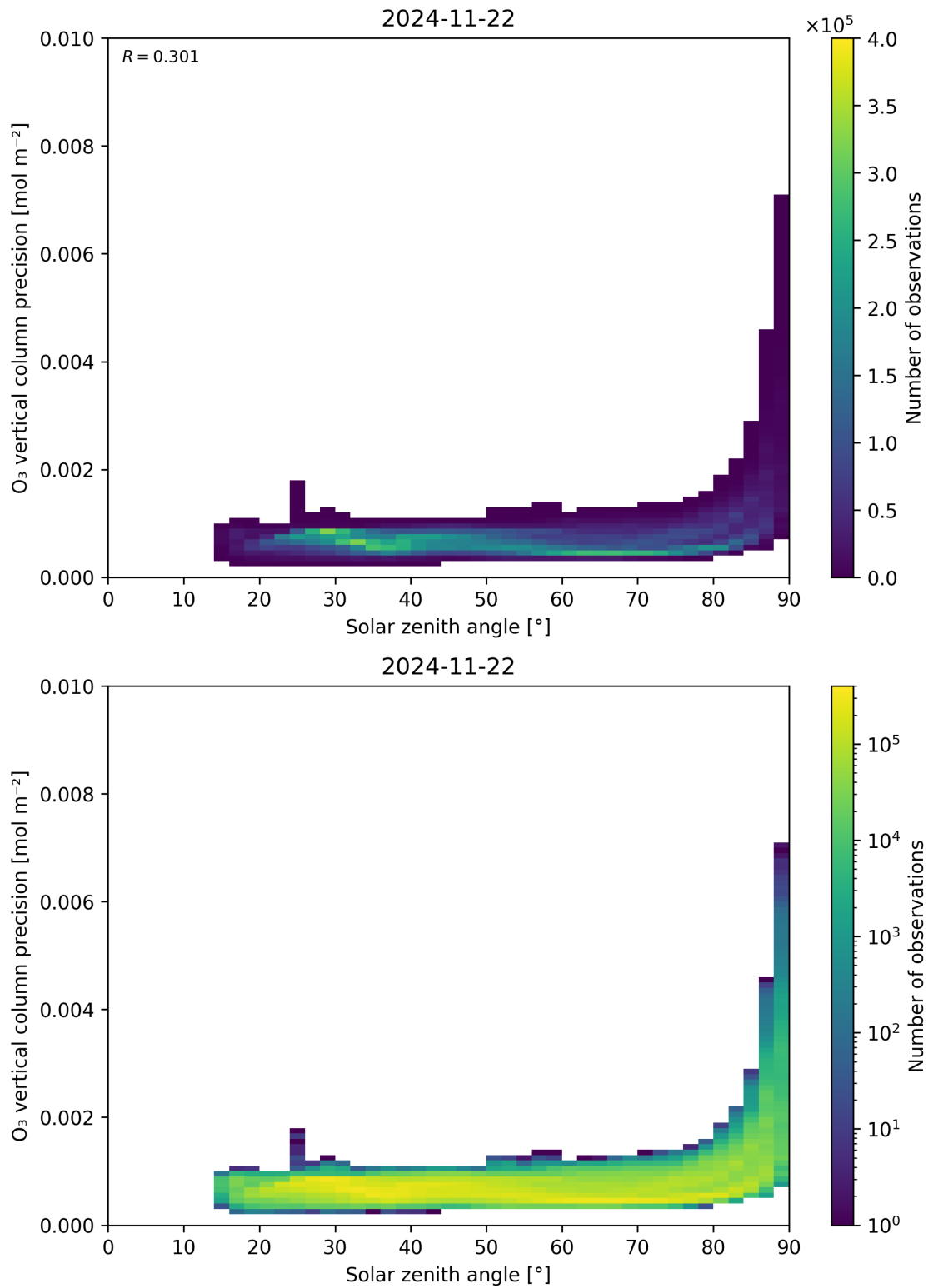
Figure 48: Scatter density plot of “Solar zenith angle” against “O 3 vertical column precision” for 2024-11-21 to 2024-11-23.
