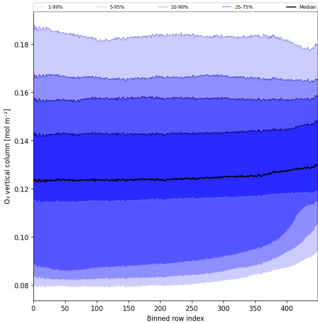
Figure 28: Along track statistics of “O 3 vertical column” for 2024-11-21 to 2024-11-23
