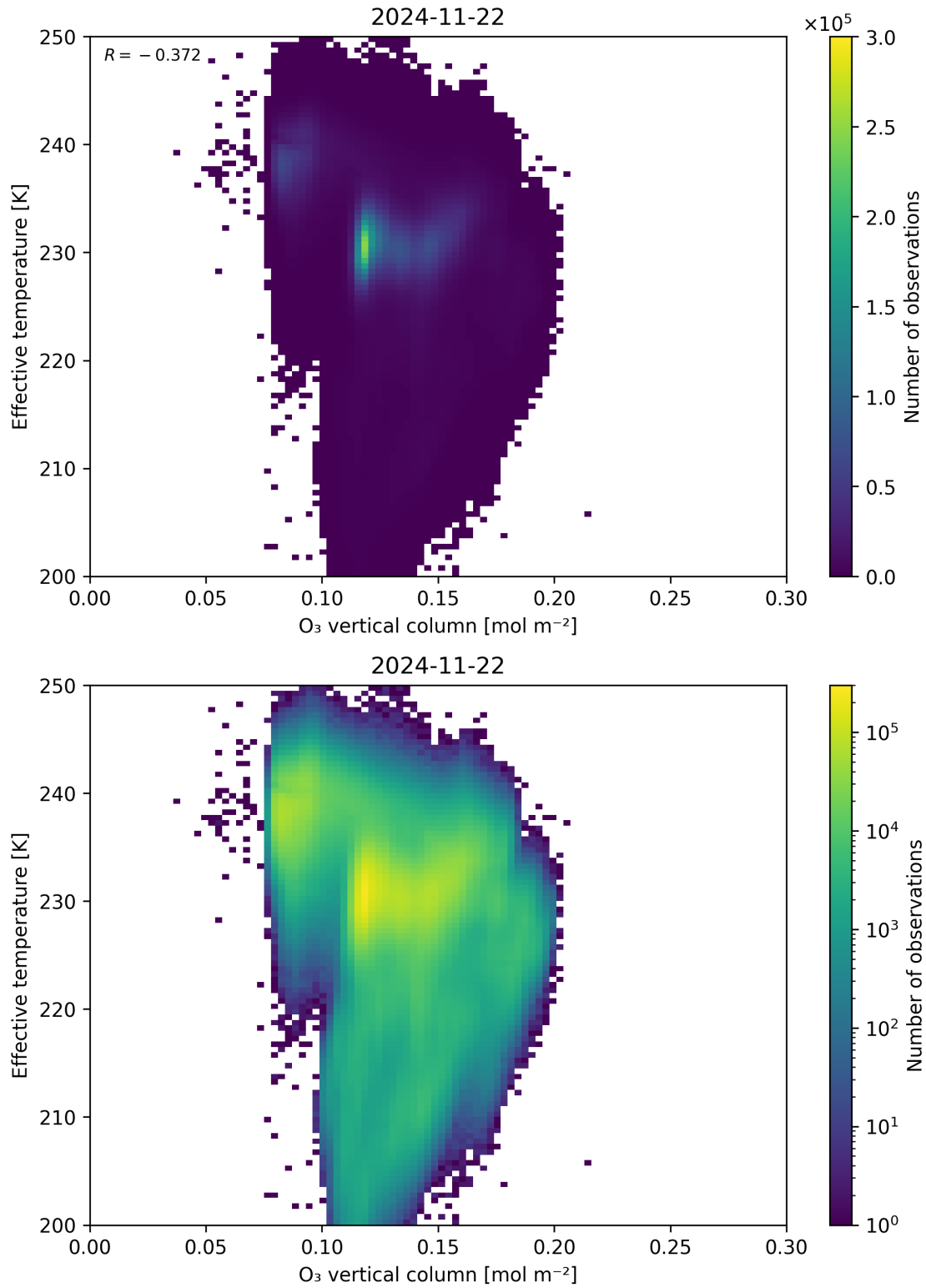
Figure 39: Scatter density plot of “O 3 vertical column” against “Effective temperature” for 2024-11-21 to 2024-11-23.
