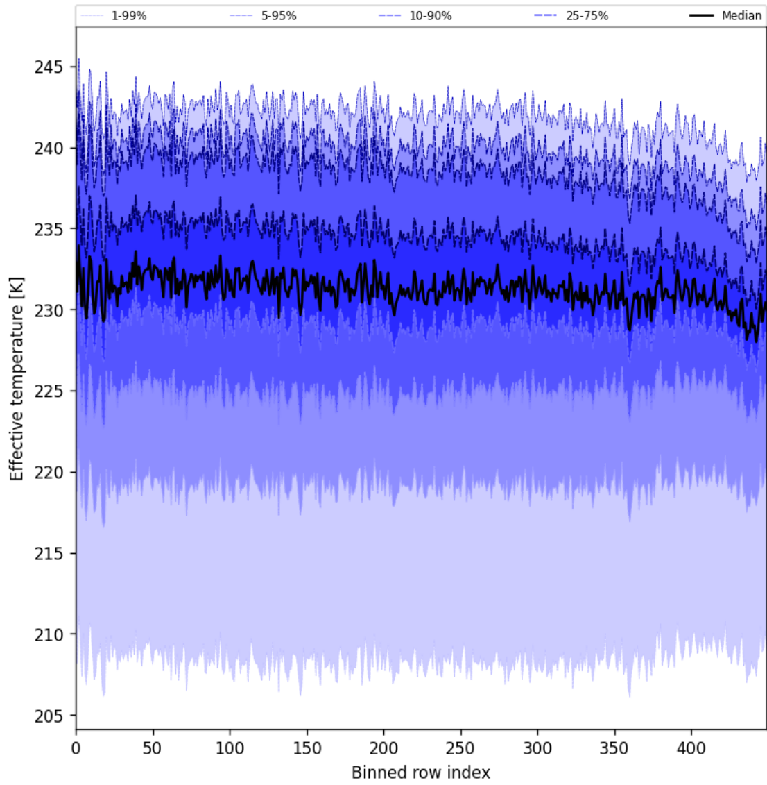
Figure 31: Along track statistics of “Effective temperature” for 2024-11-21 to 2024-11-23
