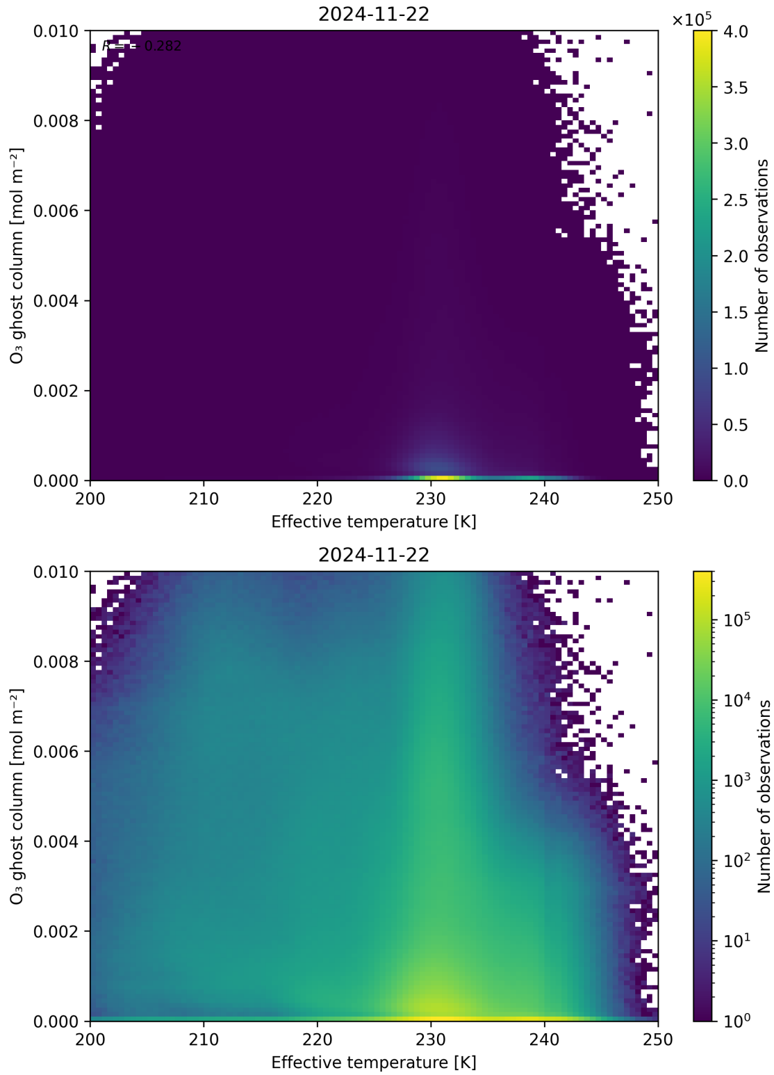
Figure 38: Scatter density plot of “Effective temperature” against “O 3 ghost column” for 2024-11-21 to 2024-11-23.
