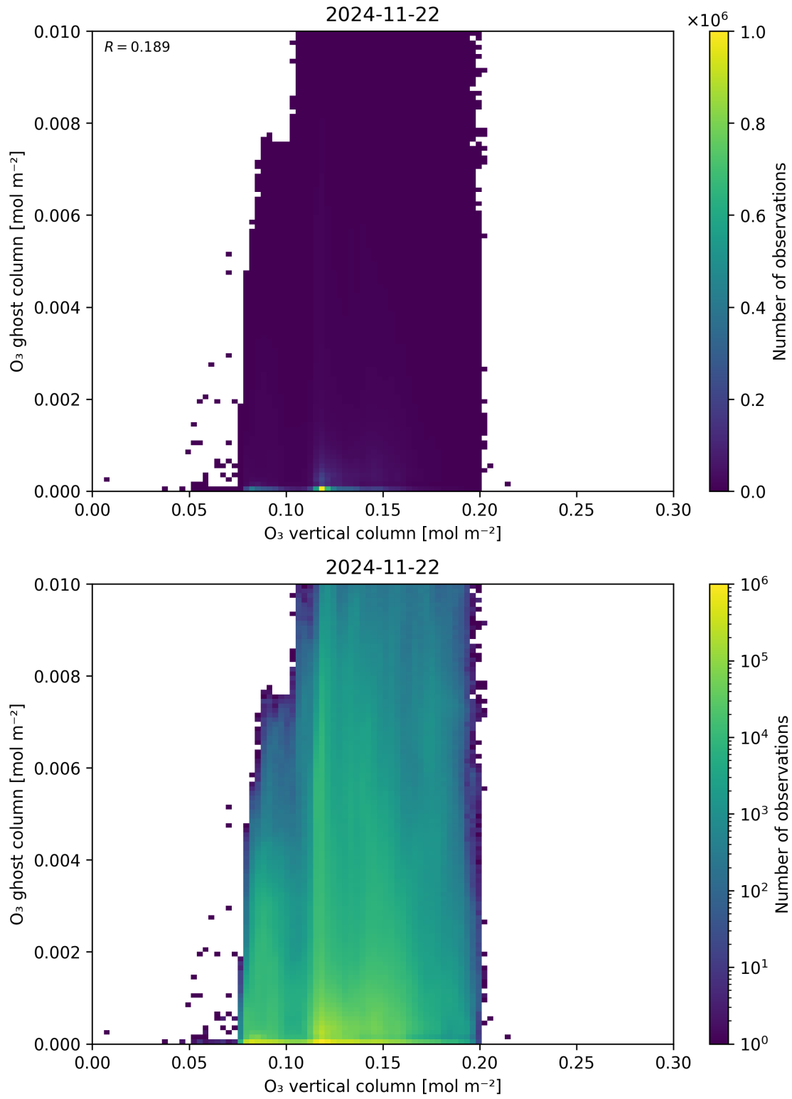
Figure 40: Scatter density plot of “O 3 vertical column” against “O 3 ghost column” for 2024-11-21 to 2024-11-23.
