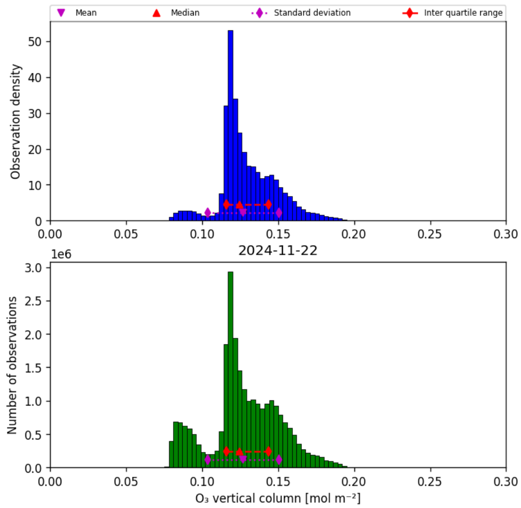
Figure 21: Histogram of “O 3 vertical column” for 2024-11-21 to 2024-11-23
