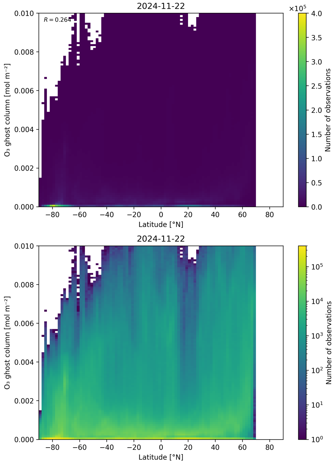
Figure 35: Scatter density plot of “Latitude” against “O 3 ghost column” for 2024-11-21 to 2024-11-23.
