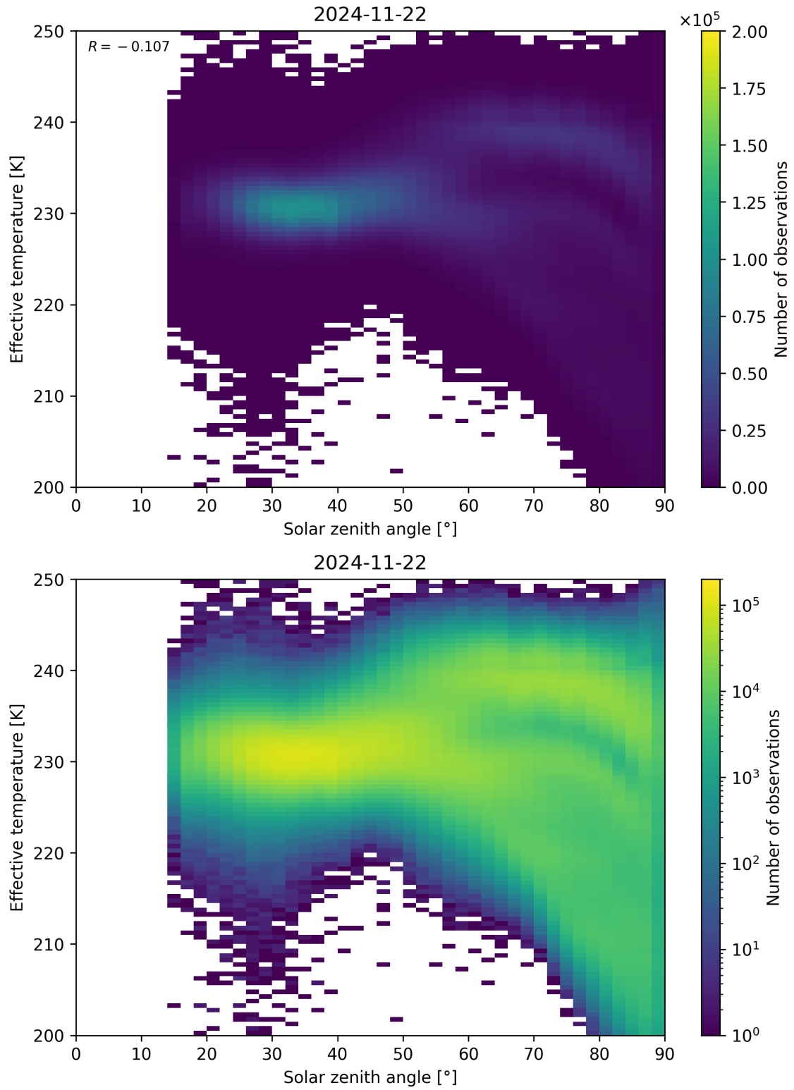
Figure 45: Scatter density plot of “Solar zenith angle” against “Effective temperature” for 2024-11-21 to 2024-11-23.
