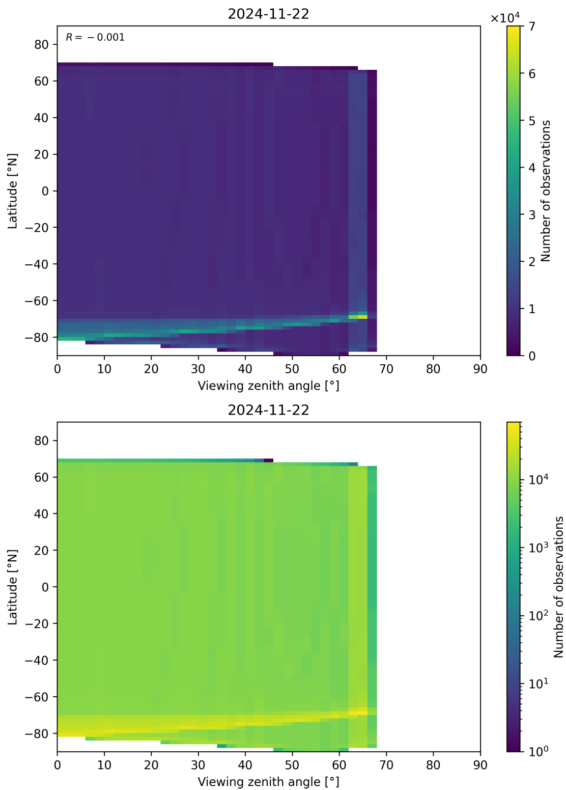
Figure 49: Scatter density plot of “Viewing zenith angle” against “Latitude” for 2024-11-21 to 2024-11-23.
