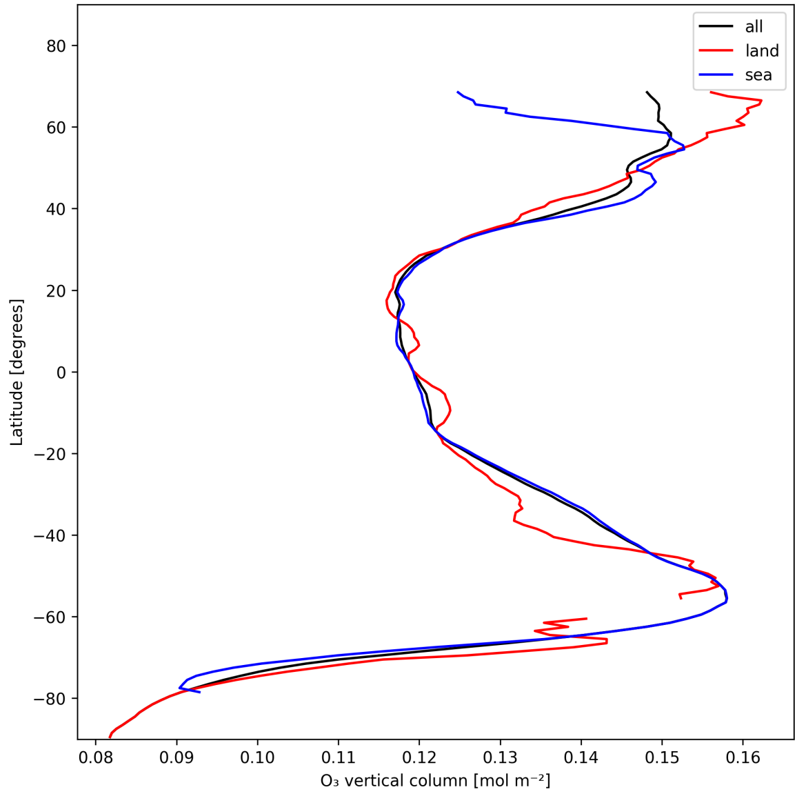
Figure 14: Zonal average of “O 3 vertical column” for 2024-11-21 to 2024-11-23.
