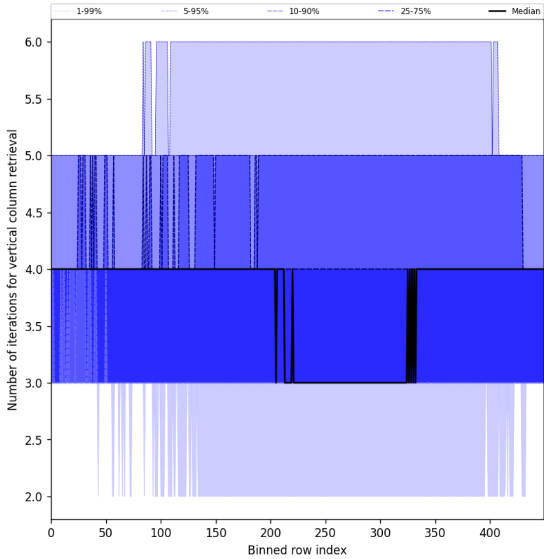
Figure 33: Along track statistics of “Number of iterations for vertical column retrieval” for 2024-11-21 to 2024-11-23
