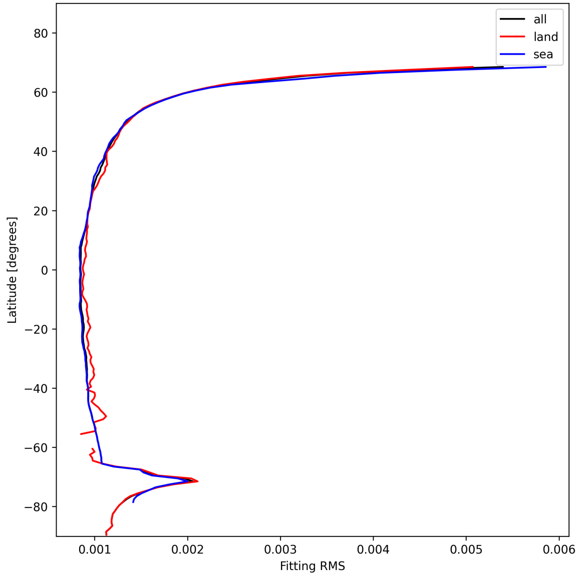
Figure 16: Zonal average of “Fitting RMS” for 2024-11-21 to 2024-11-23.
