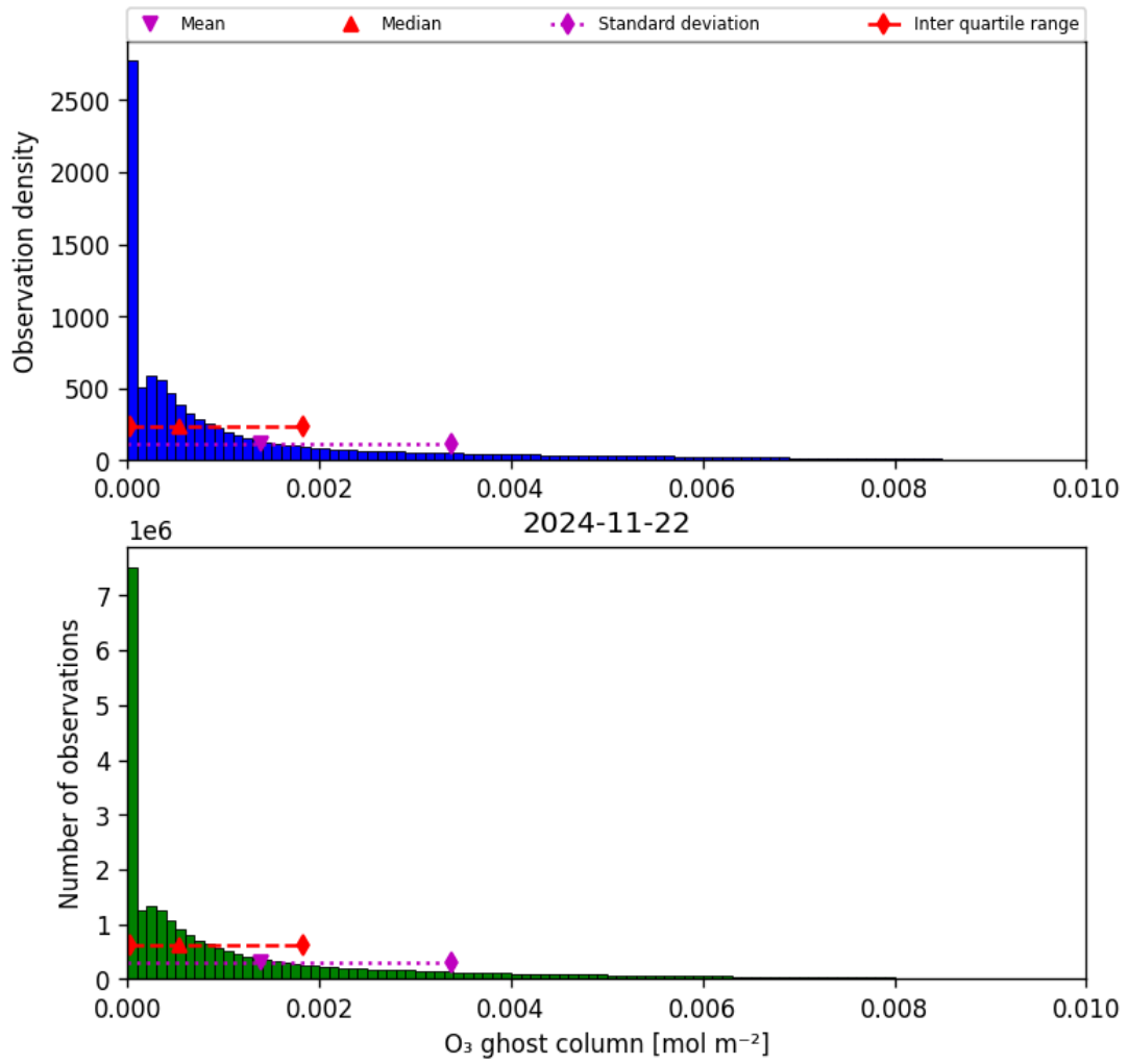
Figure 25: Histogram of "O 3 ghost column" for 2024-11-21 to 2024-11-23
