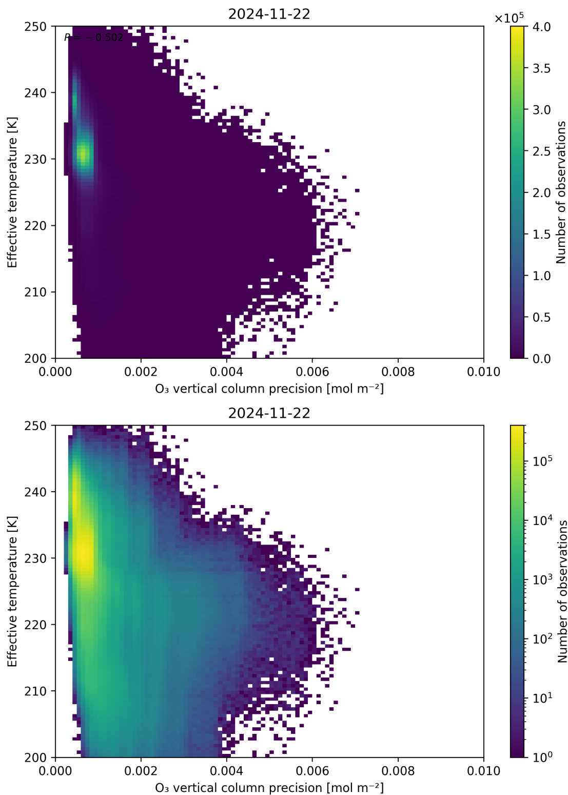
Figure 42: Scatter density plot of “O 3 vertical column precision” against “Effective temperature” for 2024-11-21 to 2024-11-23.
