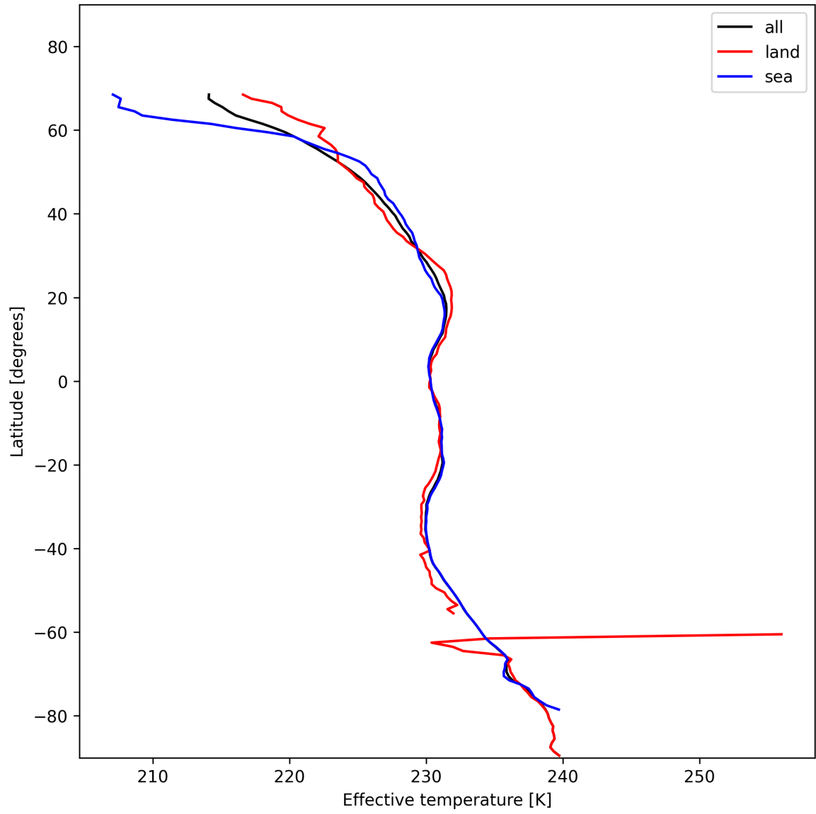
Figure 17: Zonal average of “Effective temperature” for 2024-11-21 to 2024-11-23.
