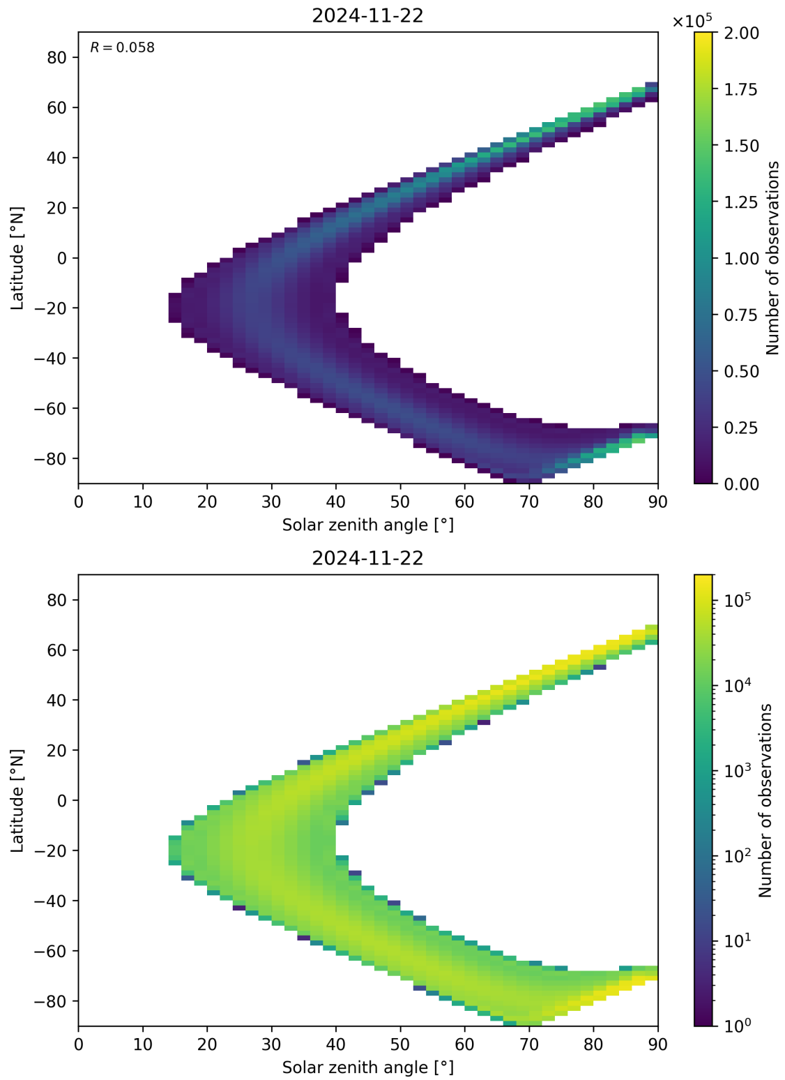
Figure 44: Scatter density plot of “Solar zenith angle” against “Latitude” for 2024-11-21 to 2024-11-23.
