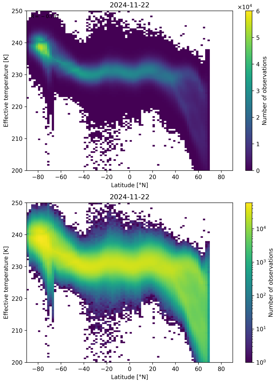
Figure 34: Scatter density plot of “Latitude” against “Effective temperature” for 2024-11-21 to 2024-11-23.
