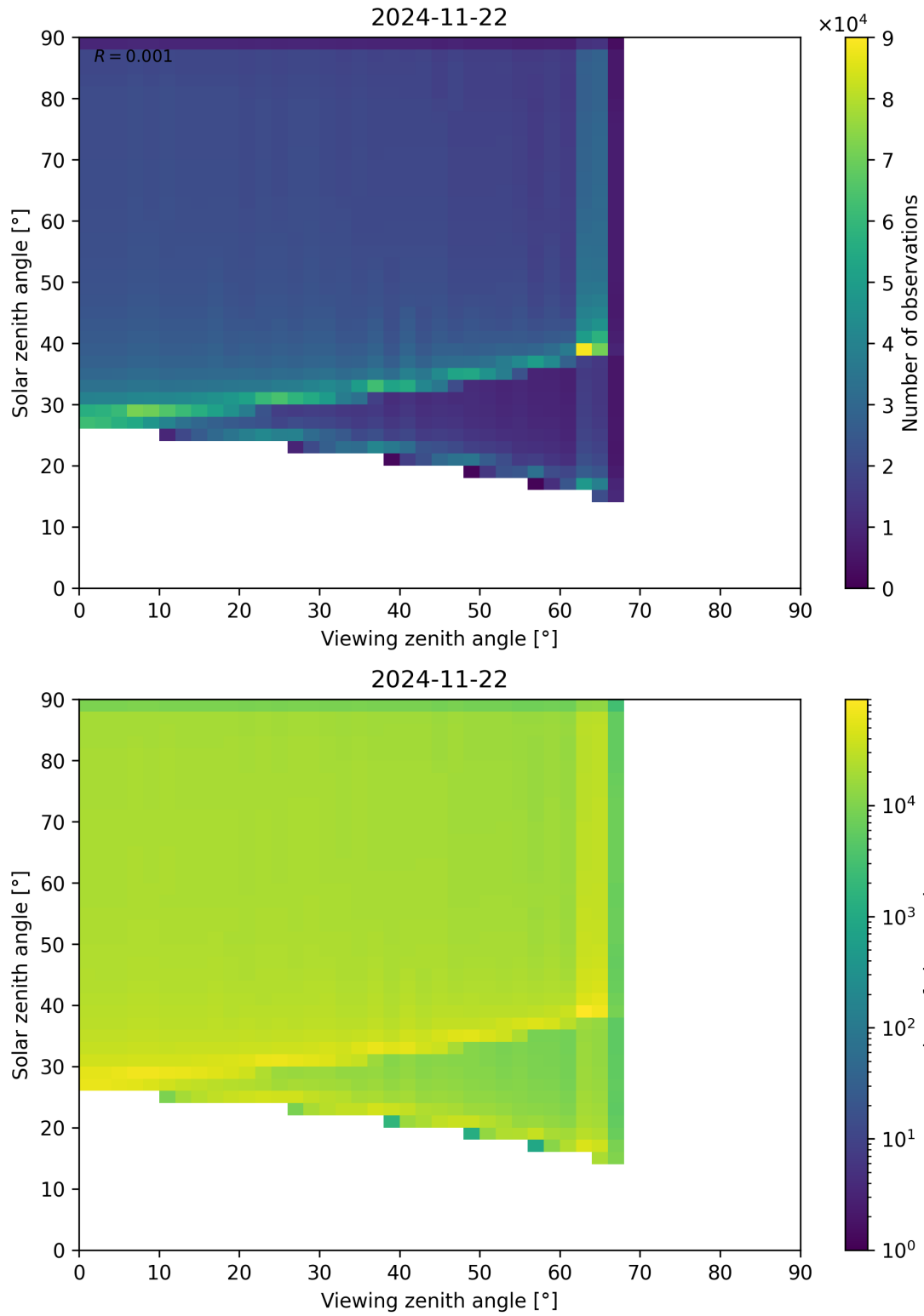
Figure 54: Scatter density plot of “Viewing zenith angle” against “Solar zenith angle” for 2024-11-21 to 2024-11-23.
