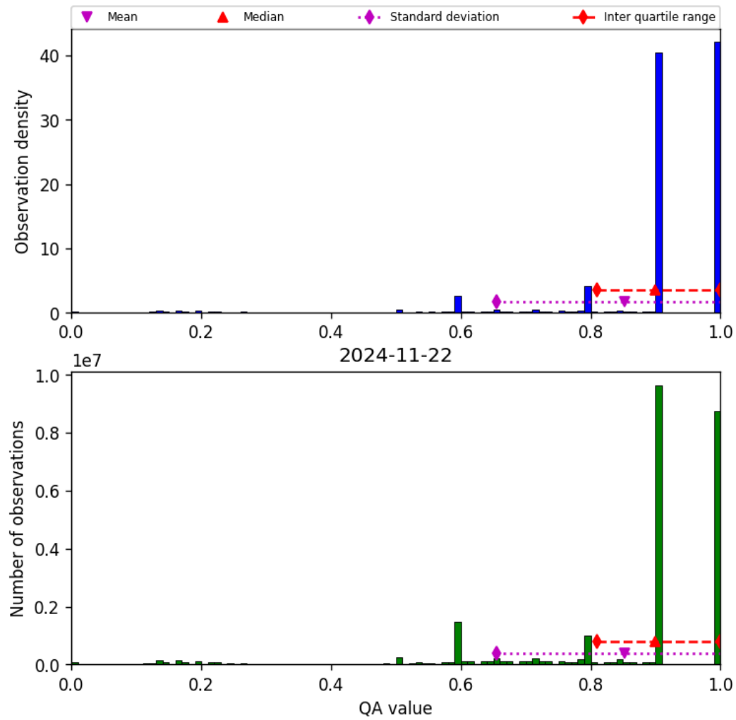
Figure 20: Histogram of “QA value” for 2024-11-21 to 2024-11-23
