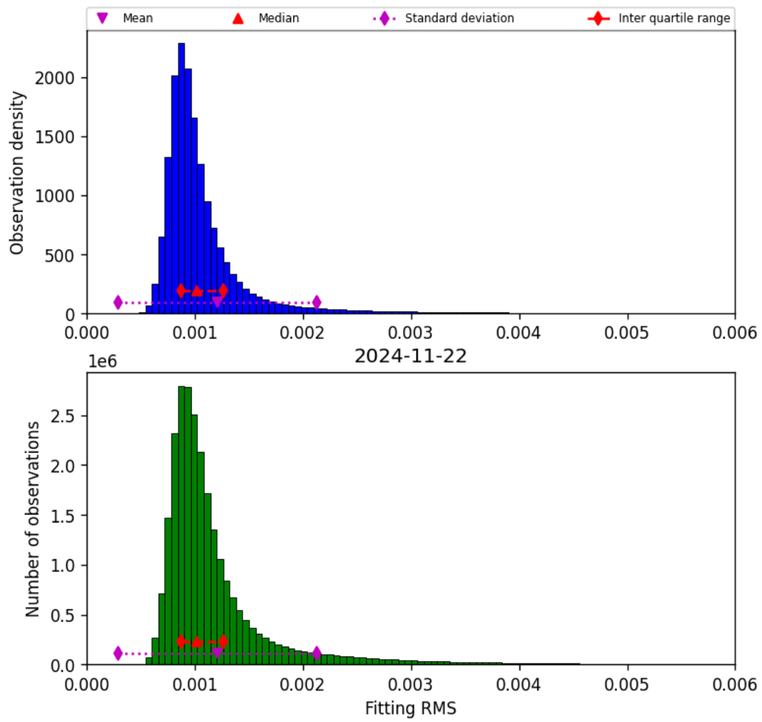
Figure 23: Histogram of “Fitting RMS” for 2024-11-21 to 2024-11-23
