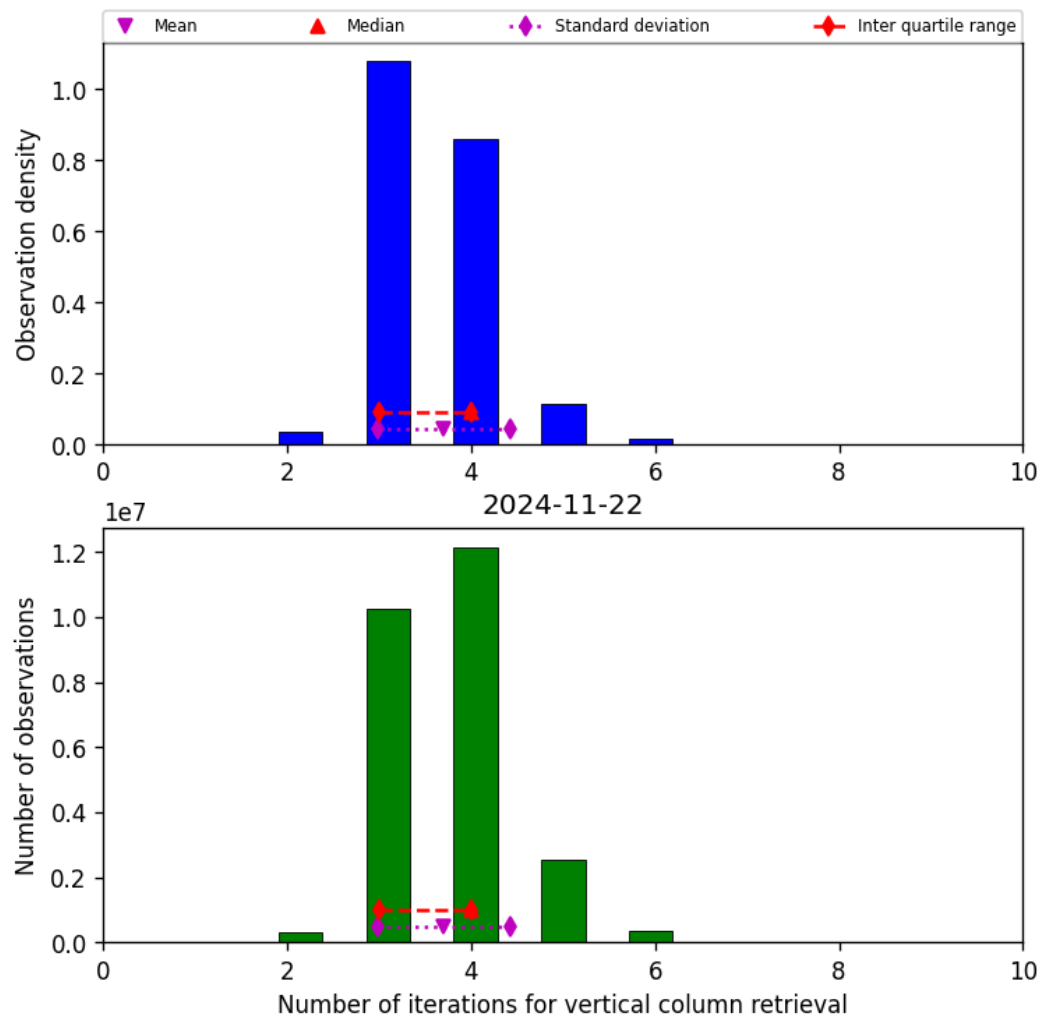
Figure 26: Histogram of “Number of iterations for vertical column retrieval” for 2024-11-21 to 2024-11-23
