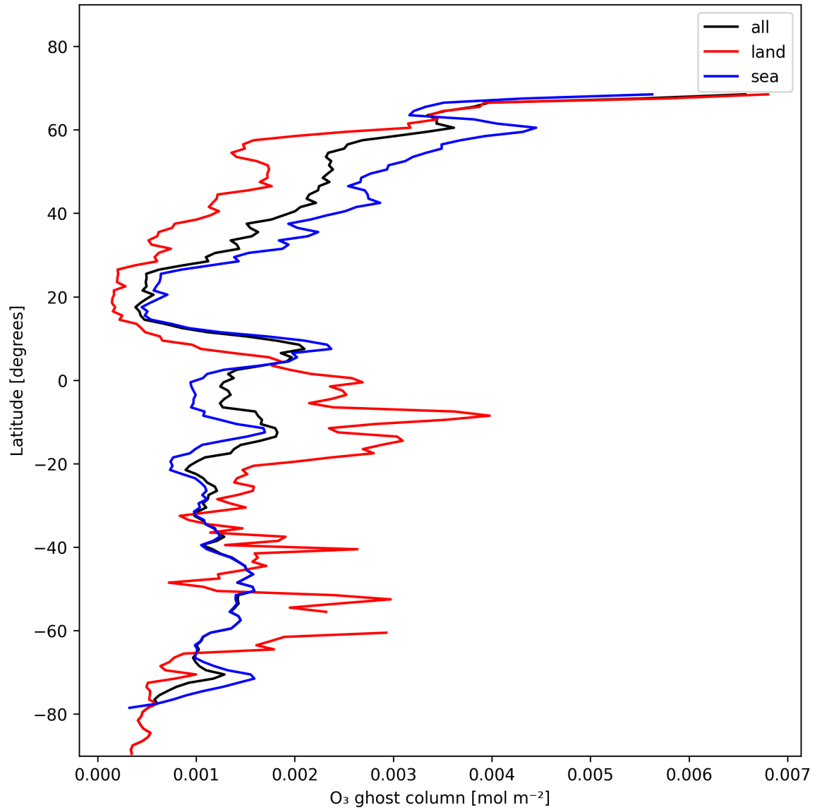
Figure 18: Zonal average of "O 3 ghost column" for 2024-11-21 to 2024-11-23.
