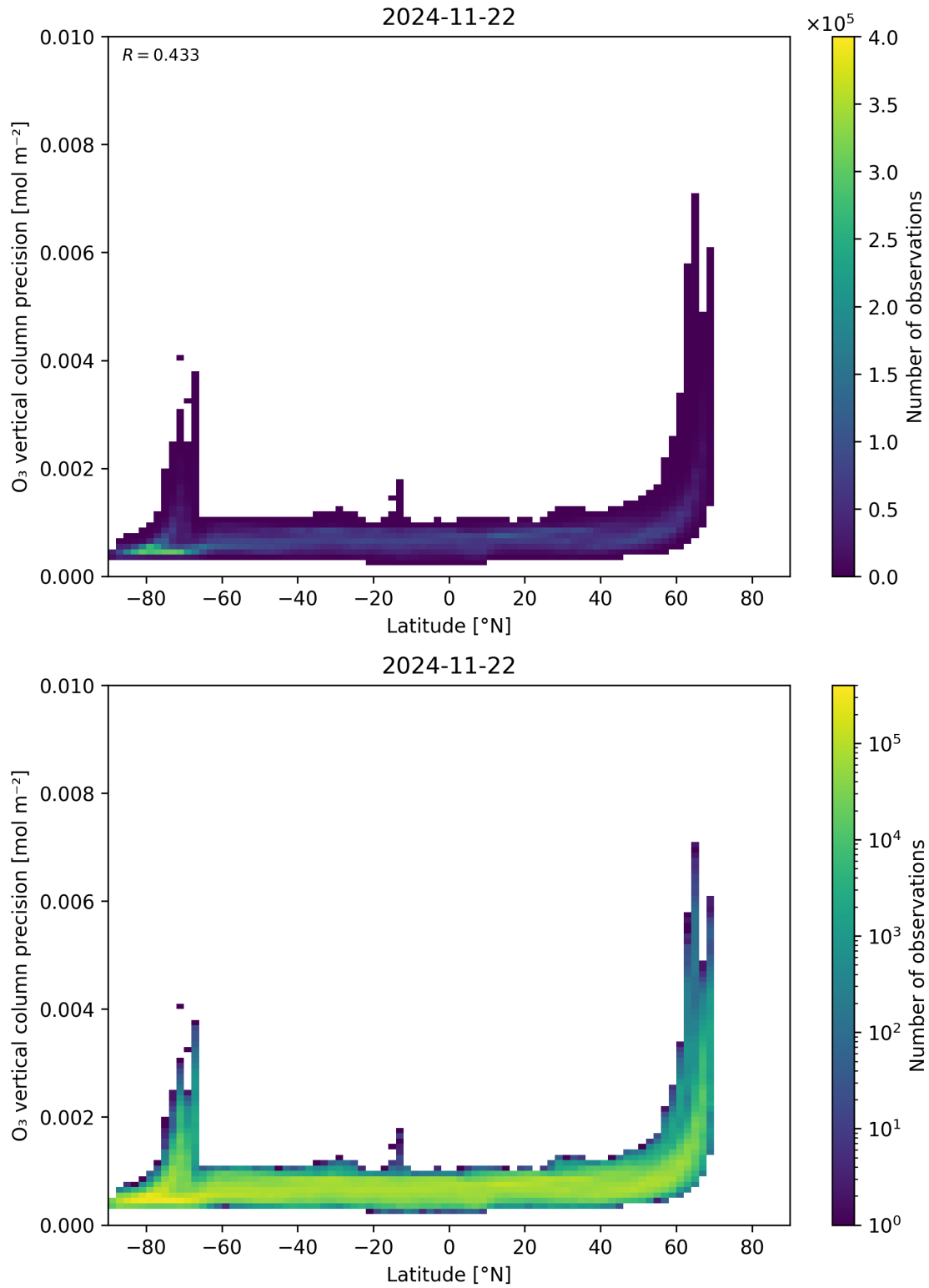
Figure 37: Scatter density plot of “Latitude” against “O 3 vertical column precision” for 2024-11-21 to 2024-11-23.
