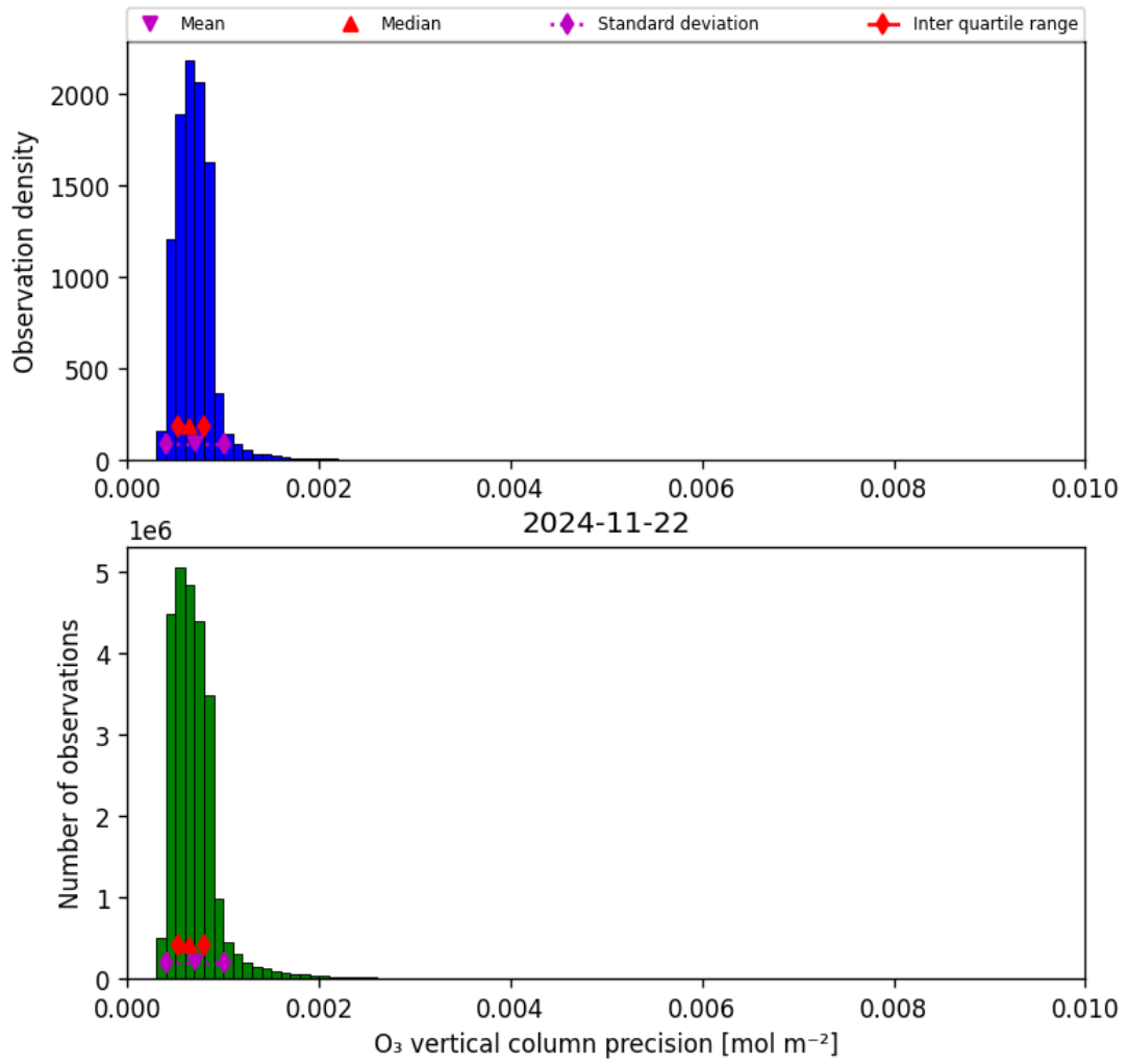
Figure 22: Histogram of "O 3 vertical column precision" for 2024-11-21 to 2024-11-23
