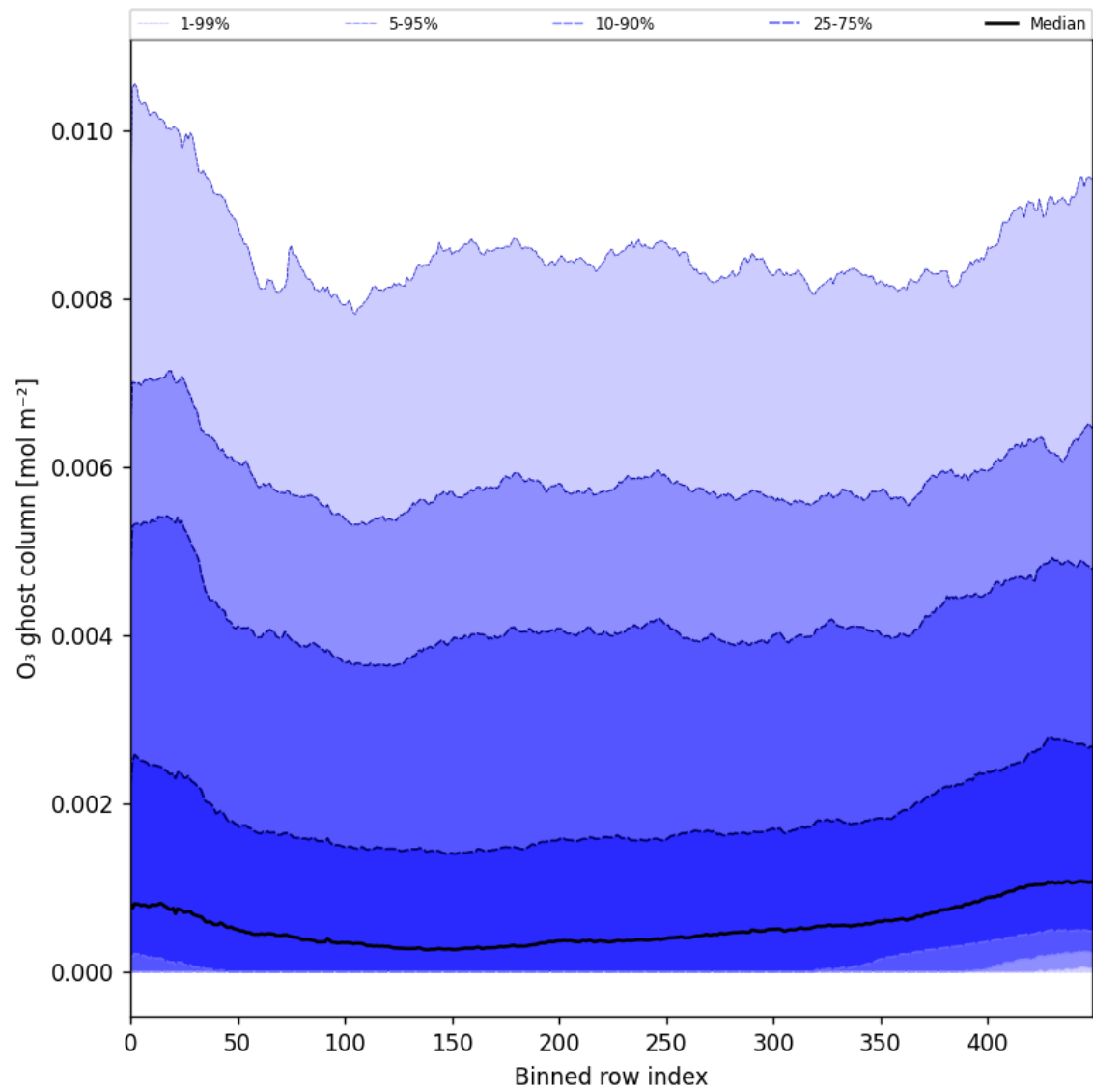
Figure 32: Along track statistics of “O 3 ghost column” for 2024-11-21 to 2024-11-23
