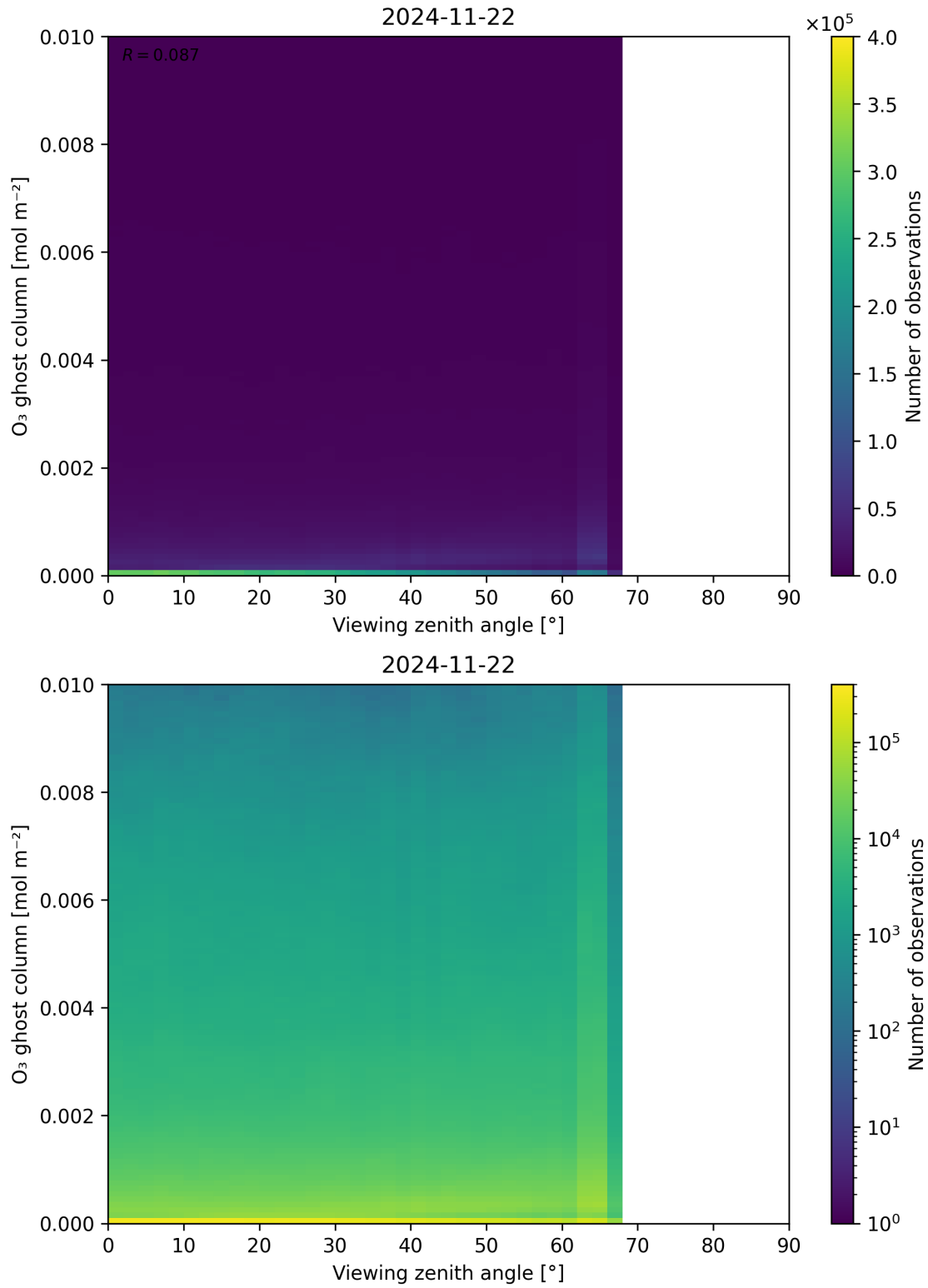
Figure 51: Scatter density plot of “Viewing zenith angle” against “O 3 ghost column” for 2024-11-21 to 2024-11-23.
