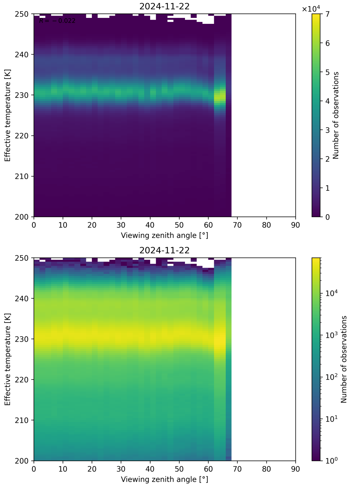
Figure 50: Scatter density plot of “Viewing zenith angle” against “Effective temperature” for 2024-11-21 to 2024-11-23.
