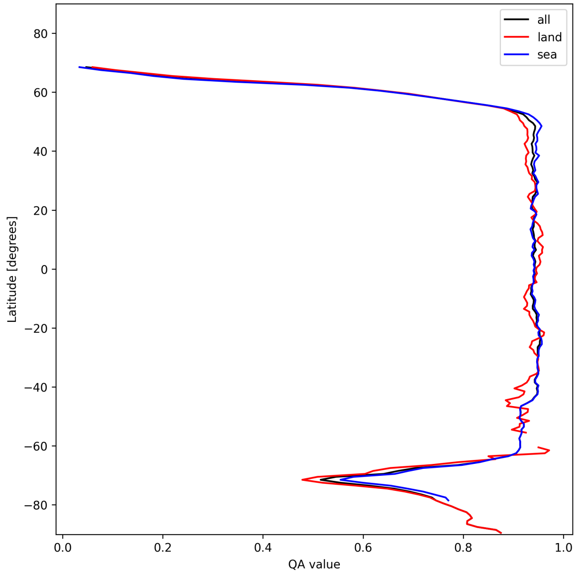
Figure 13: Zonal average of “QA value” for 2024-11-21 to 2024-11-23.
