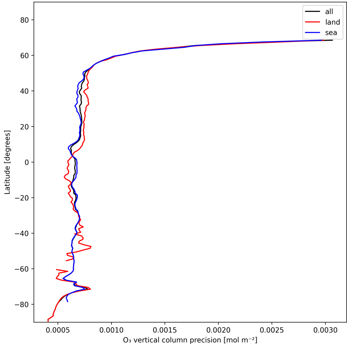
Figure 15: Zonal average of “O 3 vertical column precision” for 2024-11-21 to 2024-11-23.
