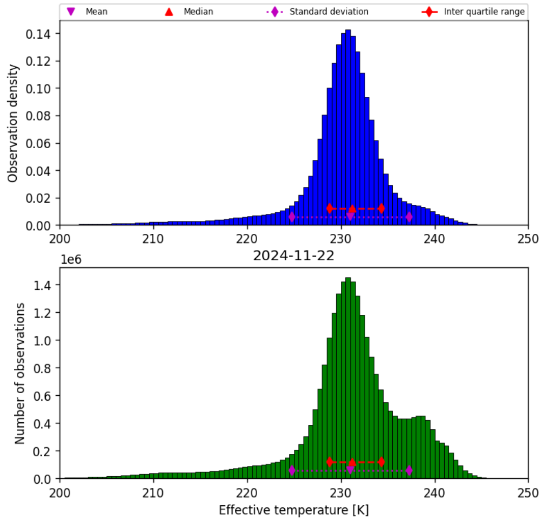
Figure 24: Histogram of “Effective temperature” for 2024-11-21 to 2024-11-23
