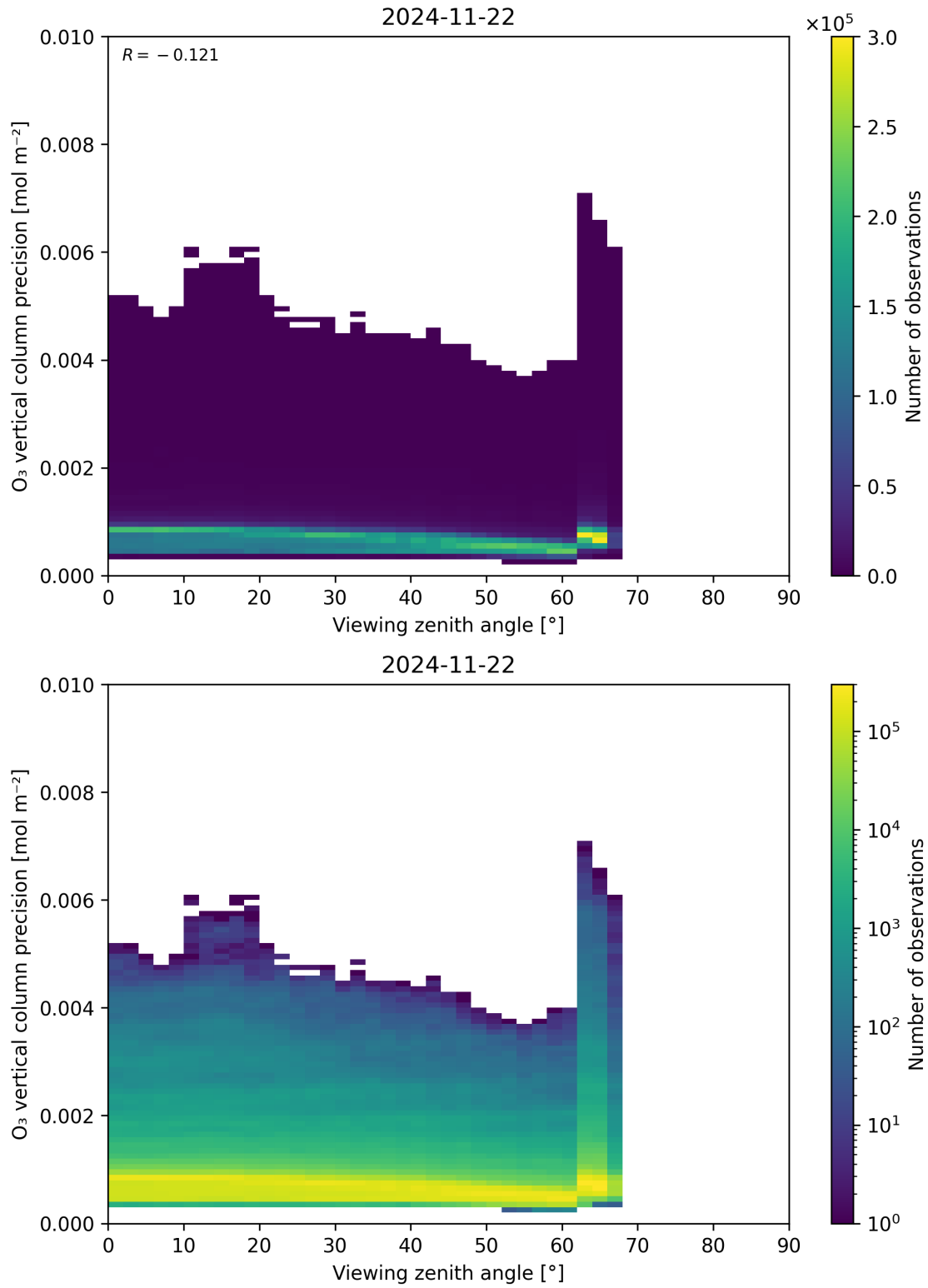
Figure 53: Scatter density plot of “Viewing zenith angle” against “O 3 vertical column precision” for 2024-11-21 to 2024-11-23.
