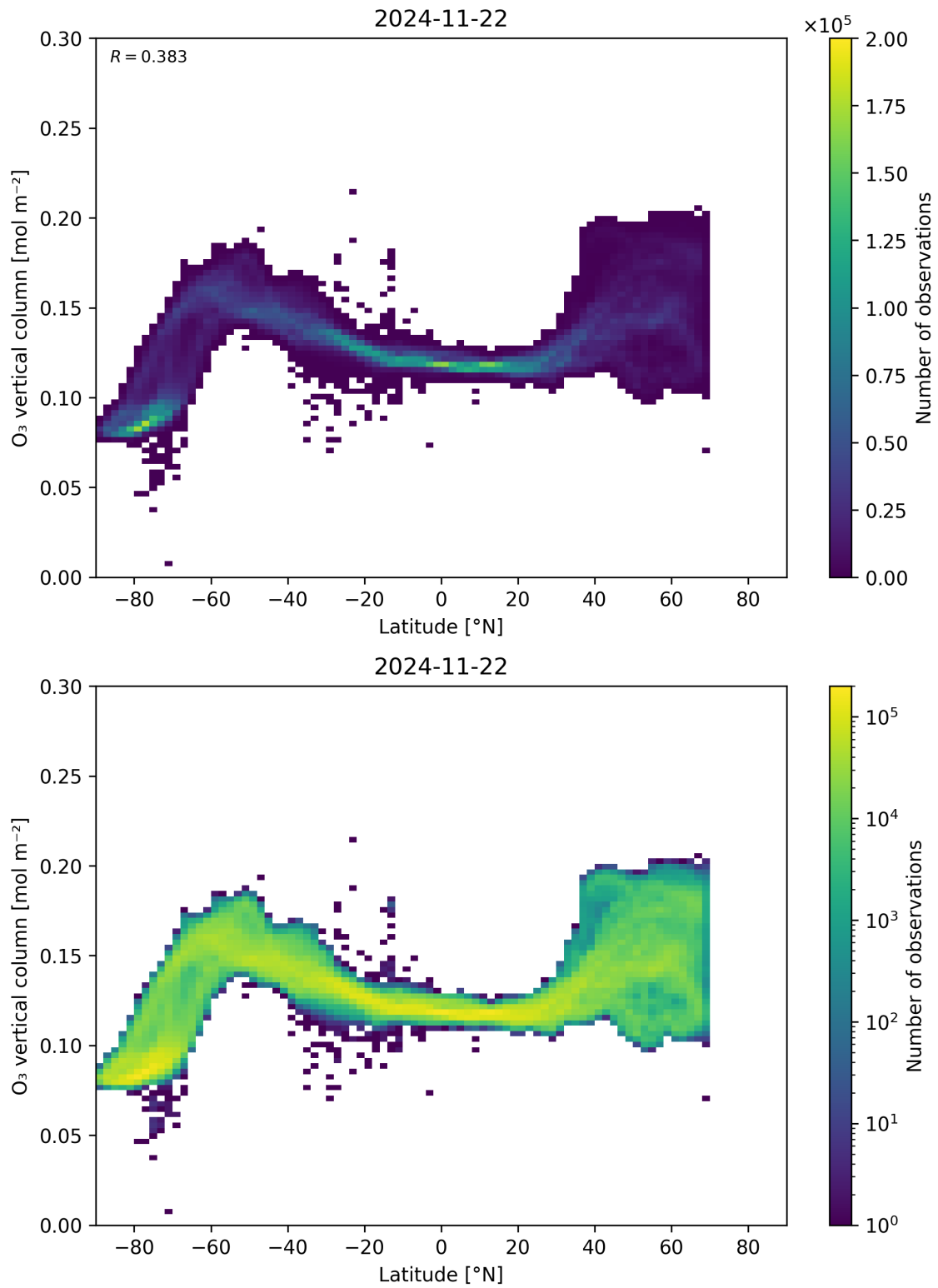
Figure 36: Scatter density plot of “Latitude” against “O 3 vertical column” for 2024-11-21 to 2024-11-23.
