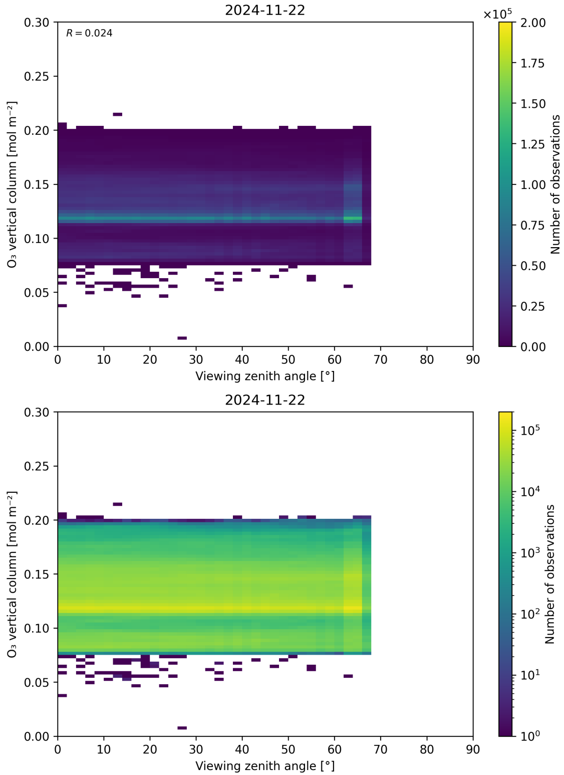
Figure 52: Scatter density plot of “Viewing zenith angle” against “O 3 vertical column” for 2024-11-21 to 2024-11-23.
