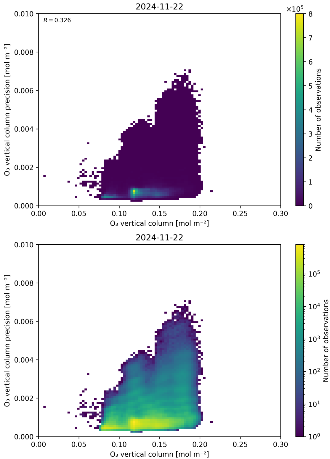
Figure 41: Scatter density plot of “O 3 vertical column” against “O 3 vertical column precision” for 2024-11-21 to 2024-11-23.
