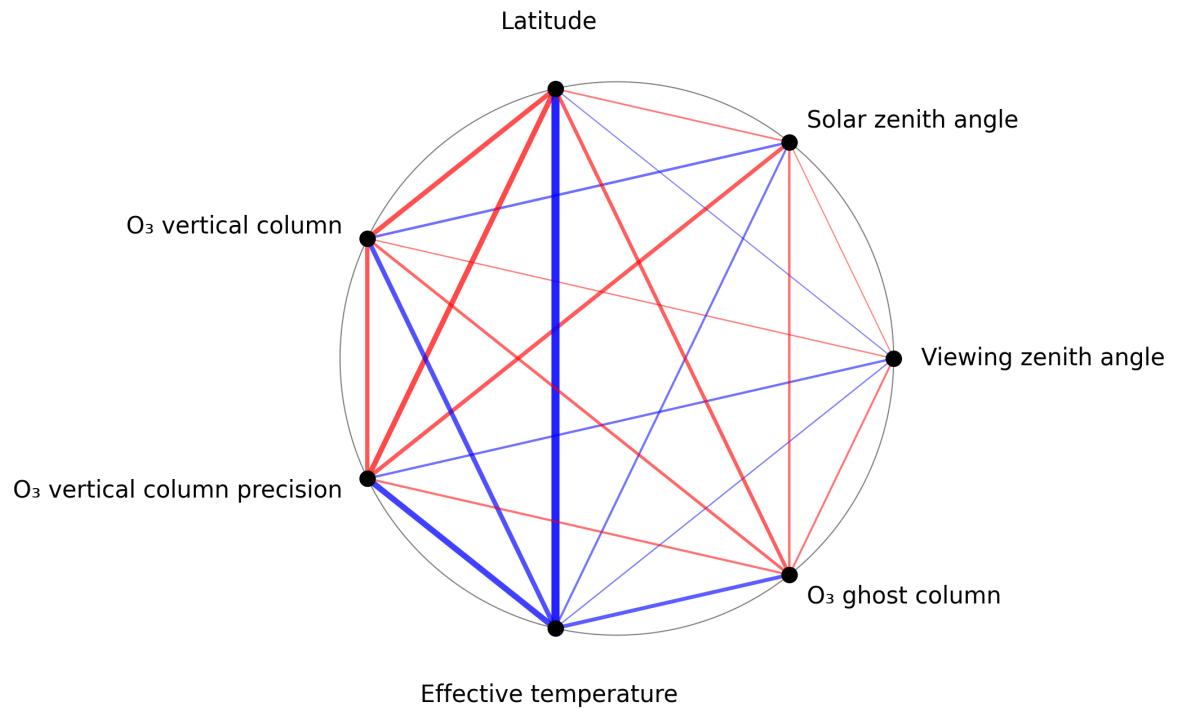
Figure 1: Map of correlation graph for 2024-11-21 to 2024-11-23.
