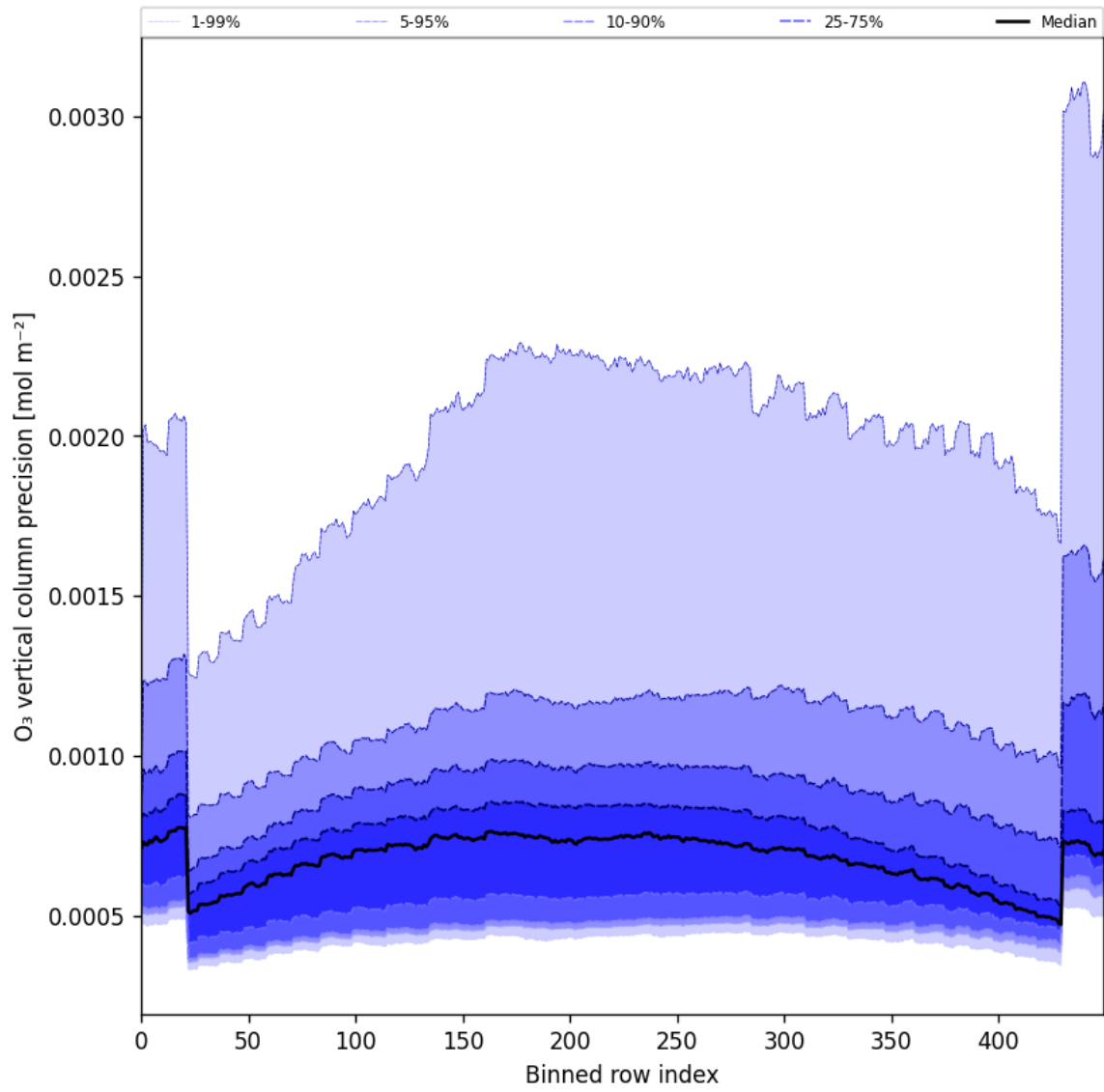
Figure 29: Along track statistics of “O 3 vertical column precision” for 2024-11-21 to 2024-11-23
