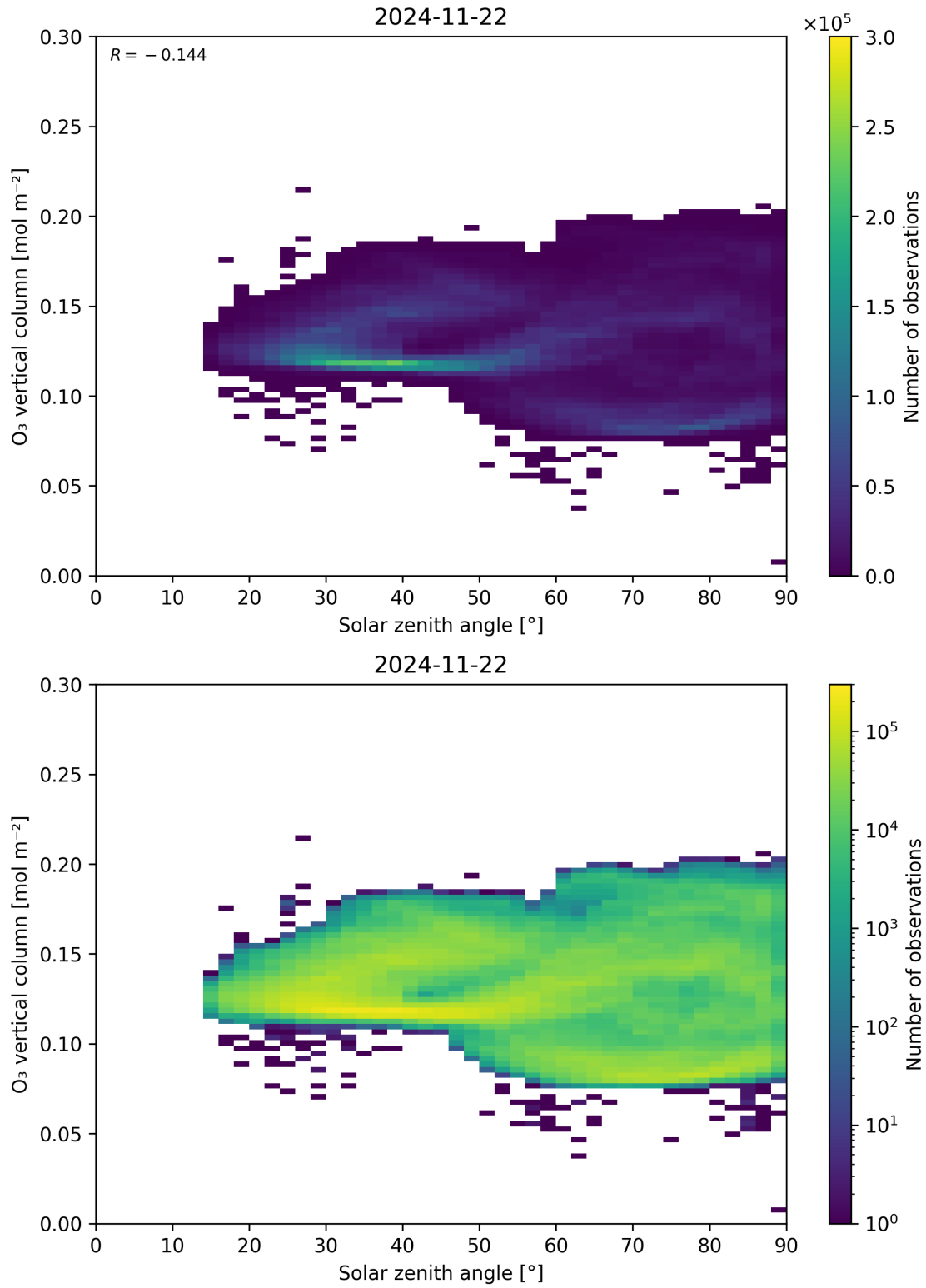
Figure 47: Scatter density plot of “Solar zenith angle” against “O 3 vertical column” for 2024-11-21 to 2024-11-23.
