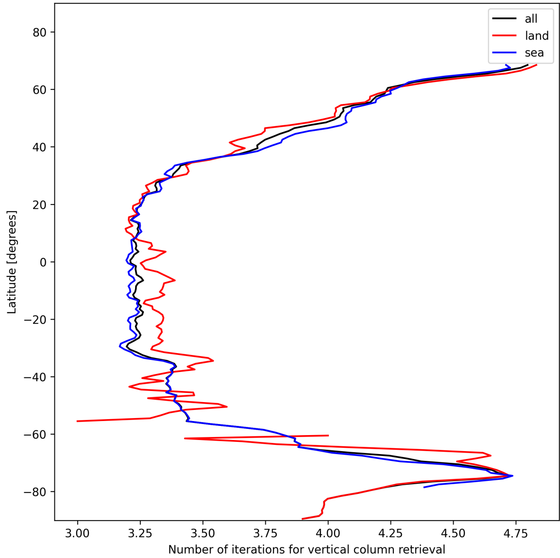
Figure 19: Zonal average of “Number of iterations for vertical column retrieval” for 2024-11-21 to 2024-11-23.
