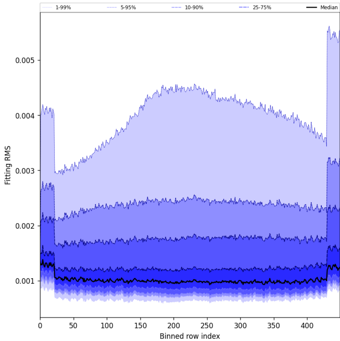
Figure 30: Along track statistics of “Fitting RMS” for 2024-11-21 to 2024-11-23
