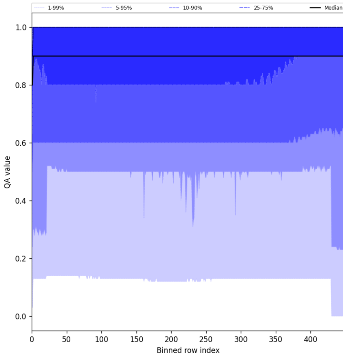
Figure 27: Along track statistics of “QA value” for 2024-11-21 to 2024-11-23
