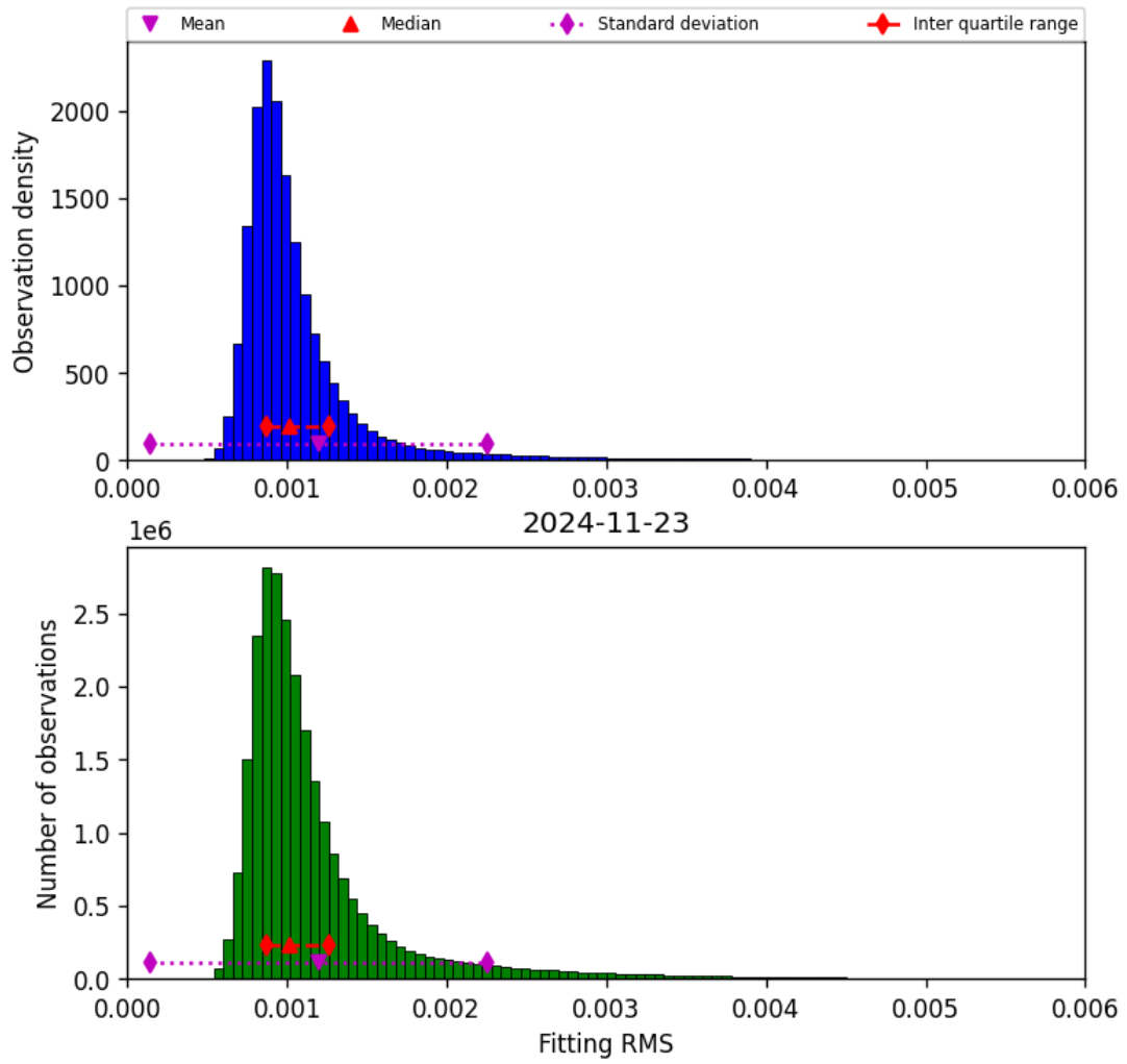
Figure 23: Histogram of “Fitting RMS” for 2024-11-22 to 2024-11-24
