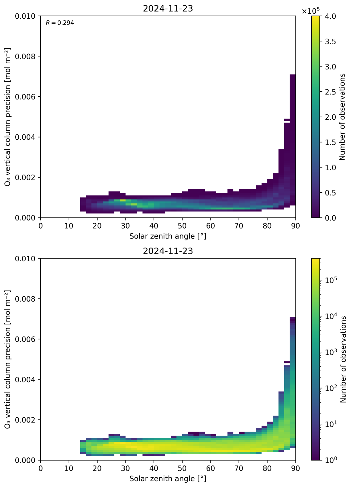
Figure 48: Scatter density plot of “Solar zenith angle” against “O 3 vertical column precision” for 2024-11-22 to 2024-11-24.
