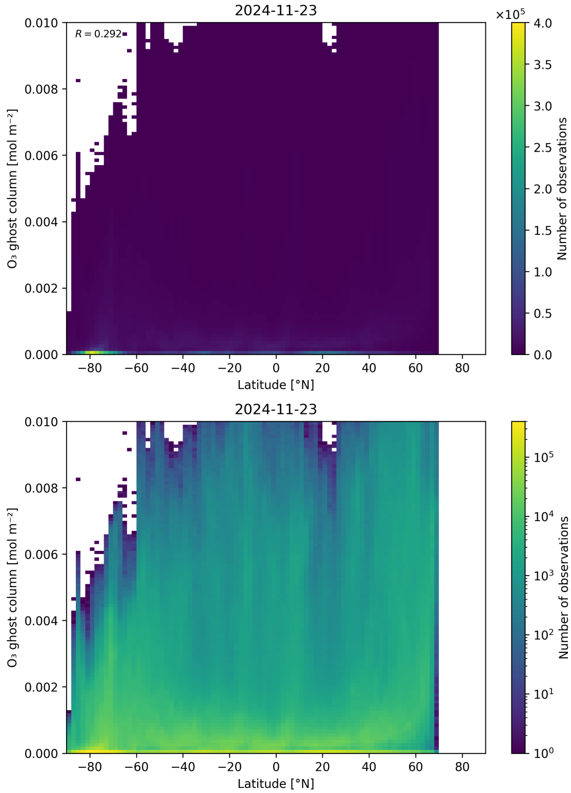
Figure 35: Scatter density plot of “Latitude” against “O 3 ghost column” for 2024-11-22 to 2024-11-24.
