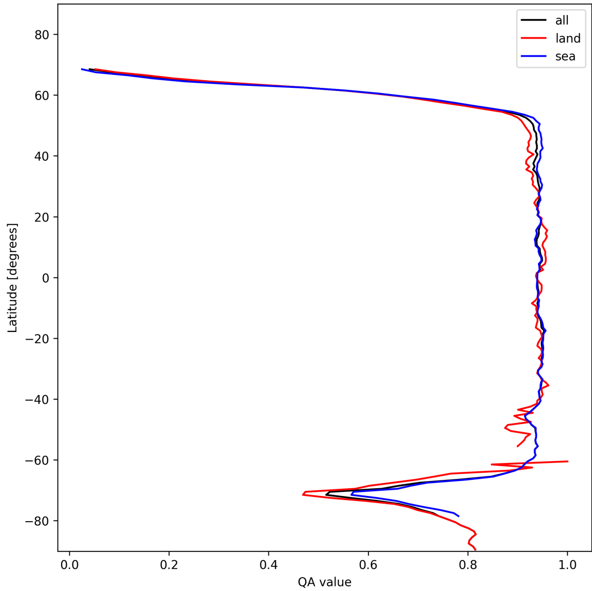
Figure 13: Zonal average of “QA value” for 2024-11-22 to 2024-11-24.
