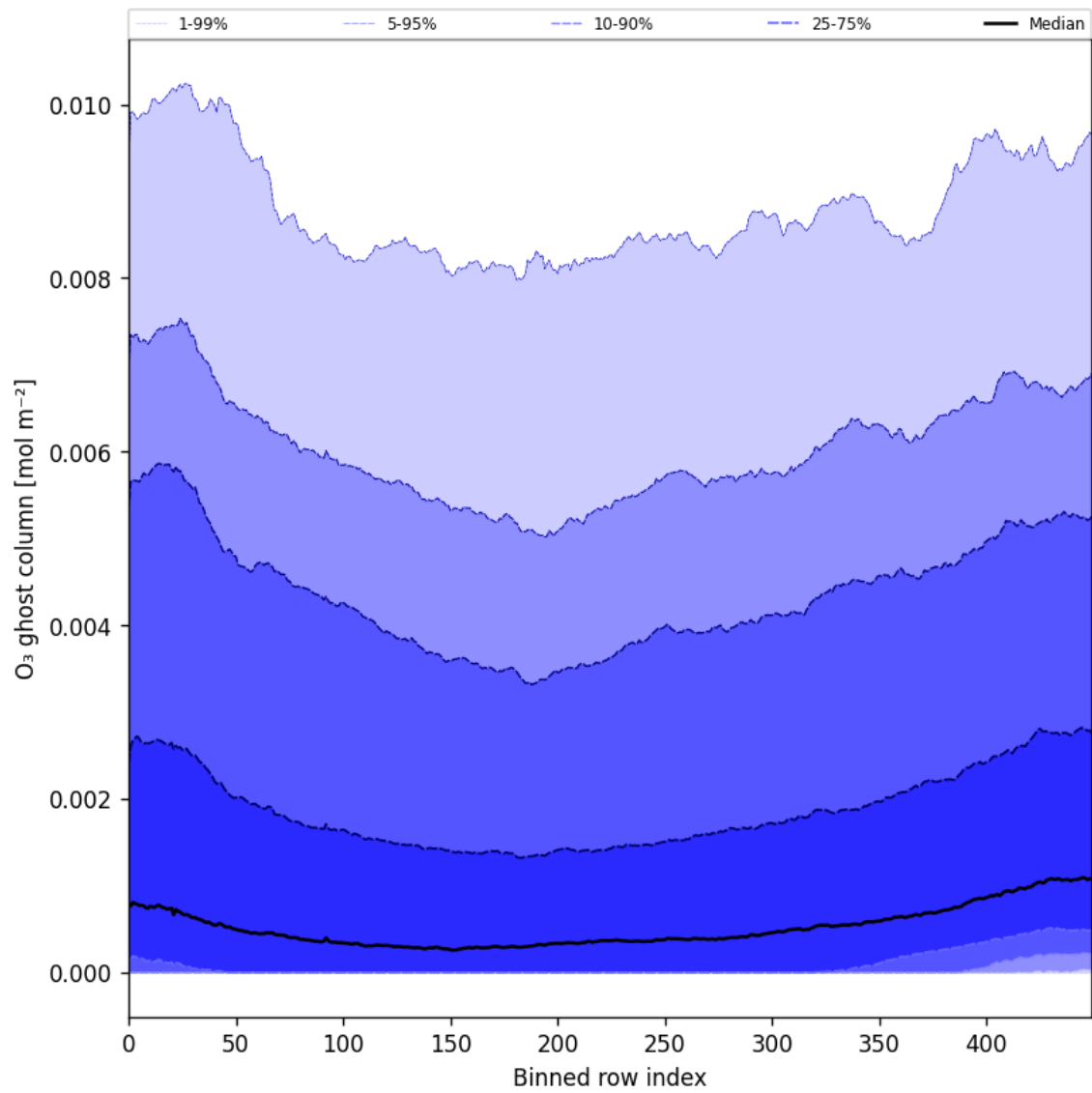
Figure 32: Along track statistics of “O 3 ghost column” for 2024-11-22 to 2024-11-24
