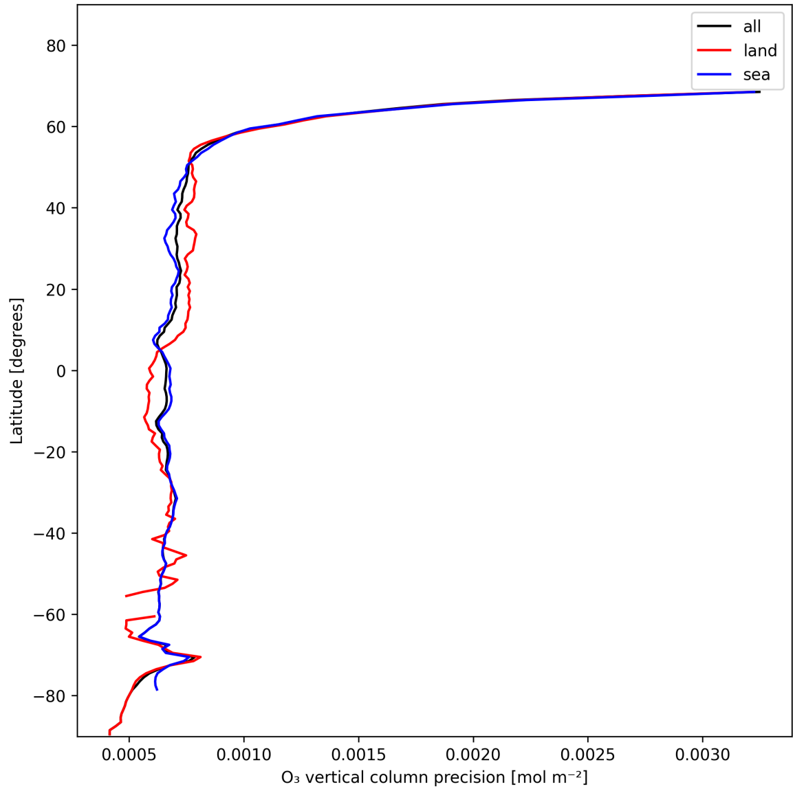
Figure 15: Zonal average of “O 3 vertical column precision” for 2024-11-22 to 2024-11-24.
