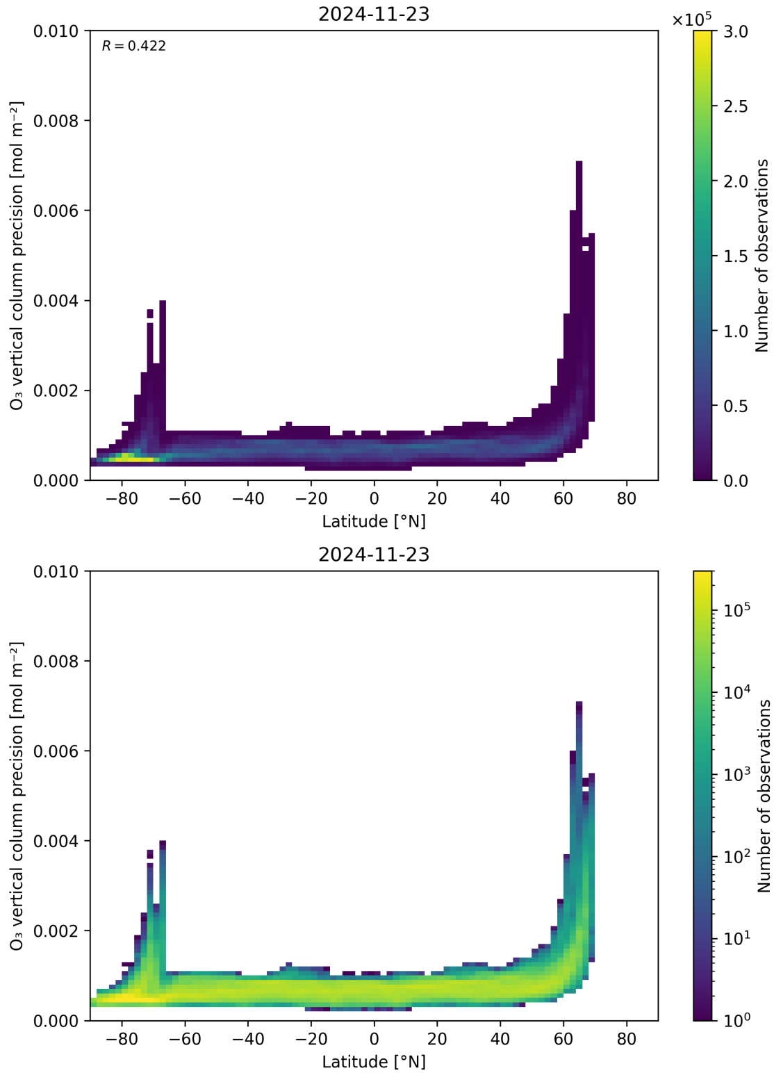
Figure 37: Scatter density plot of “Latitude” against “O 3 vertical column precision” for 2024-11-22 to 2024-11-24.
