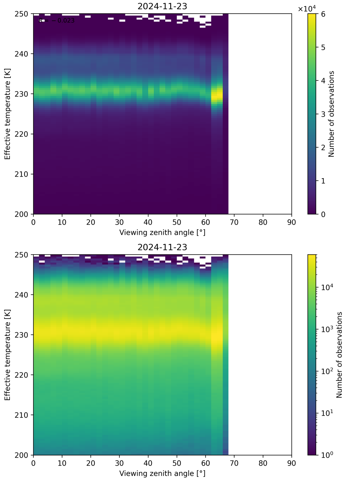
Figure 50: Scatter density plot of “Viewing zenith angle” against “Effective temperature” for 2024-11-22 to 2024-11-24.
