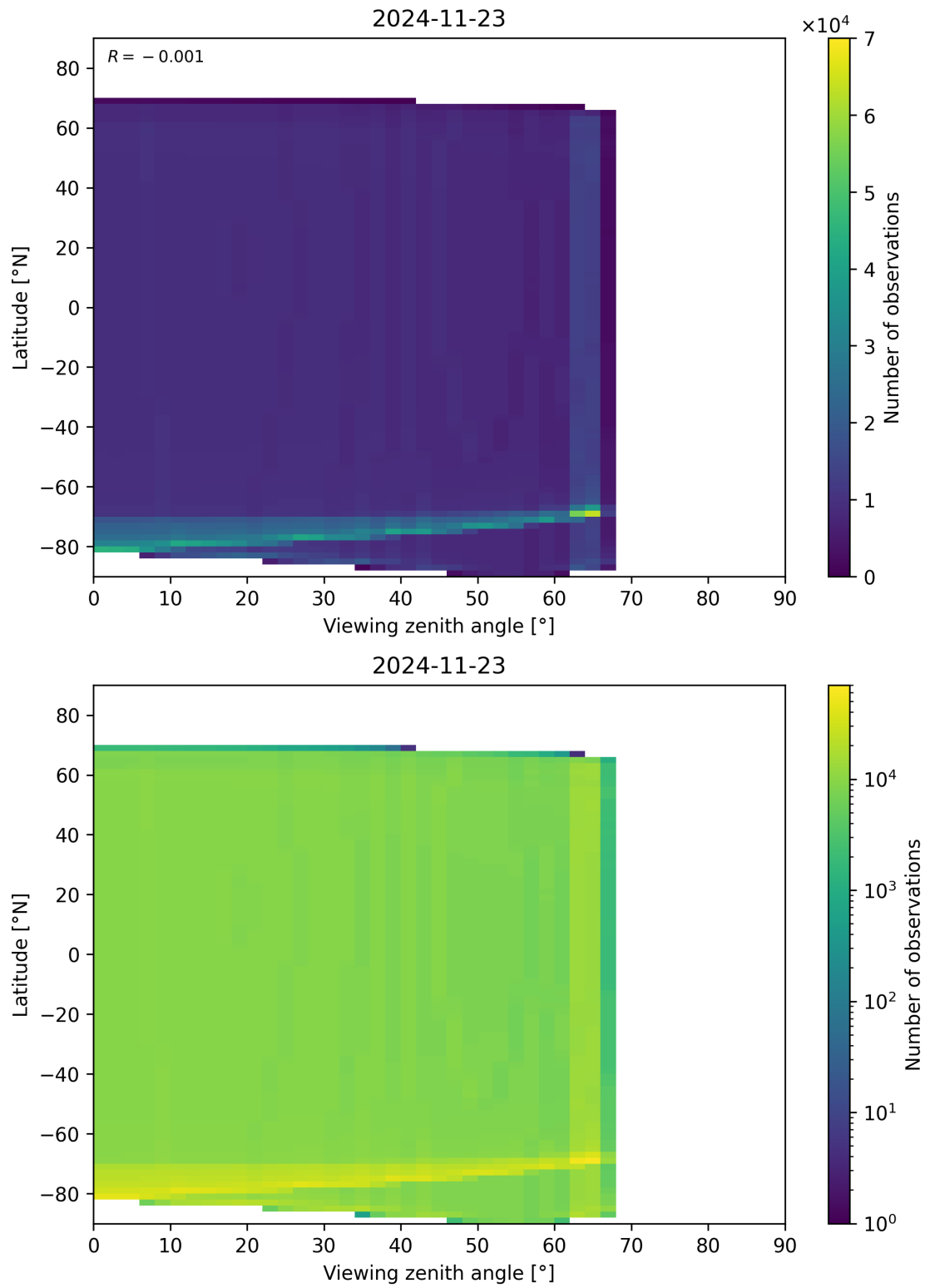
Figure 49: Scatter density plot of “Viewing zenith angle” against “Latitude” for 2024-11-22 to 2024-11-24.
