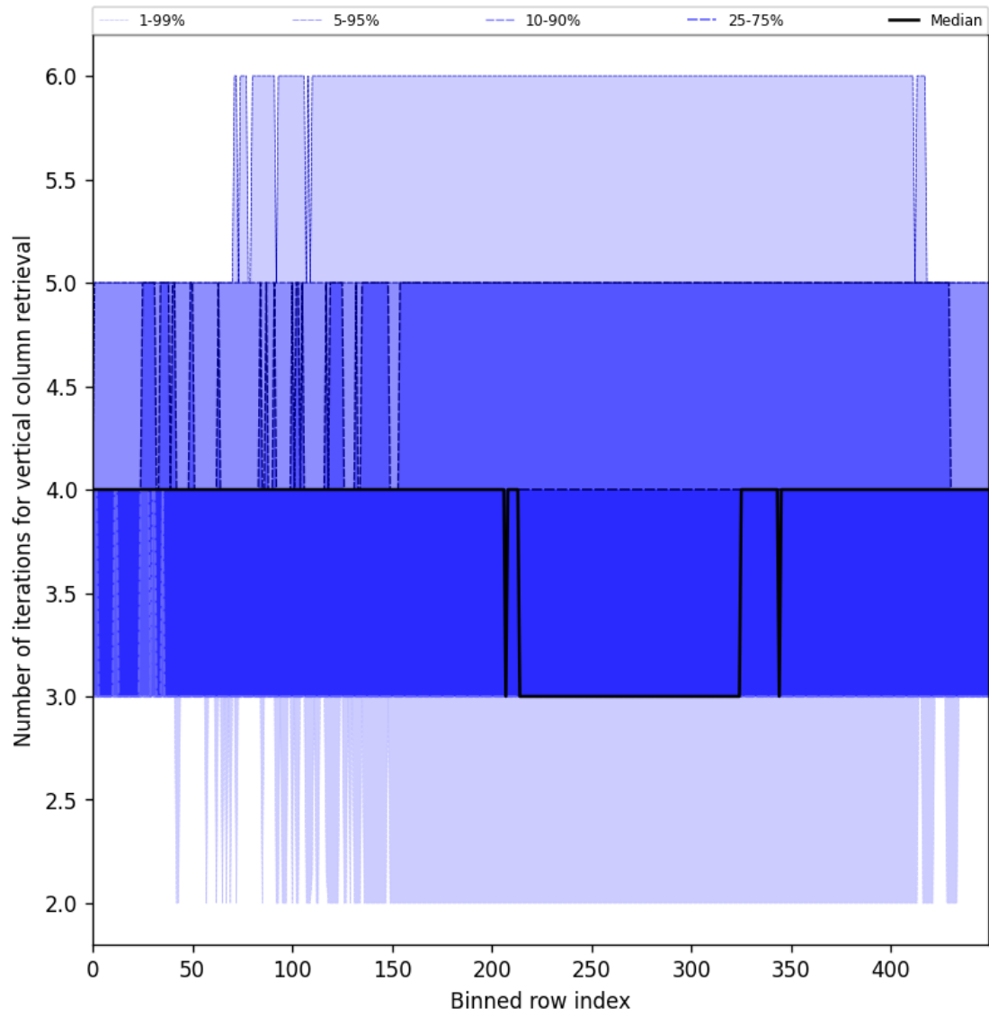
Figure 33: Along track statistics of “Number of iterations for vertical column retrieval” for 2024-11-22 to 2024-11-24
