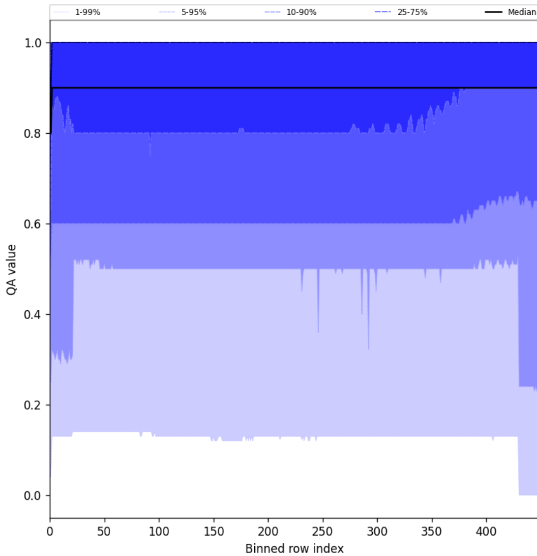
Figure 27: Along track statistics of “QA value” for 2024-11-22 to 2024-11-24
