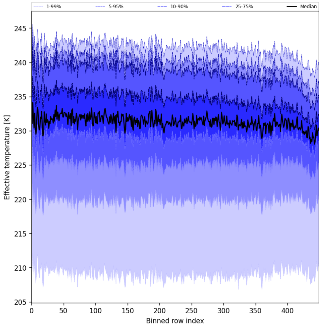
Figure 31: Along track statistics of “Effective temperature” for 2024-11-22 to 2024-11-24
