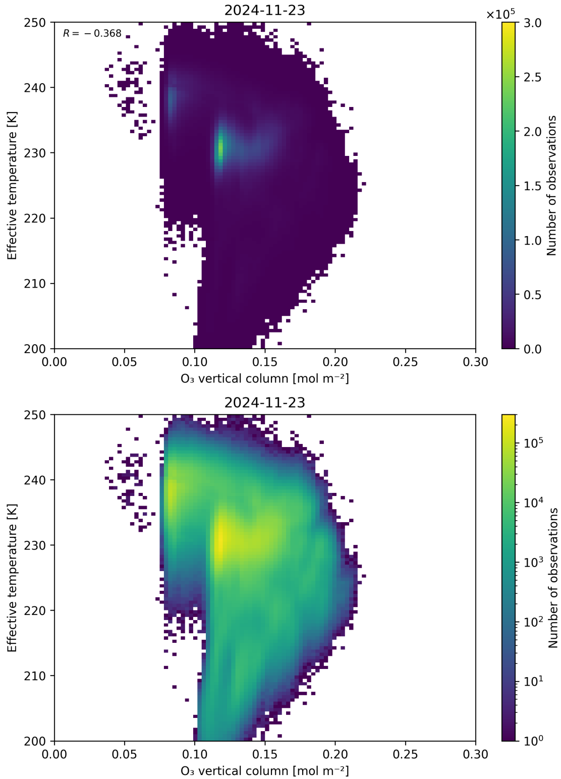
Figure 39: Scatter density plot of “O 3 vertical column” against “Effective temperature” for 2024-11-22 to 2024-11-24.
