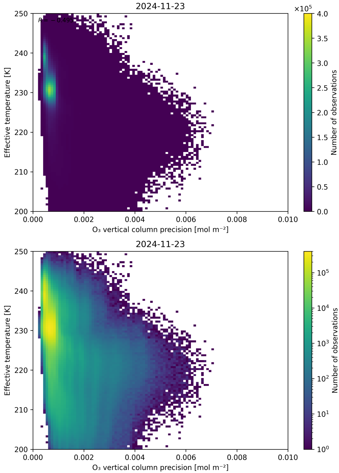
Figure 42: Scatter density plot of “O 3 vertical column precision” against “Effective temperature” for 2024-11-22 to 2024-11-24.
