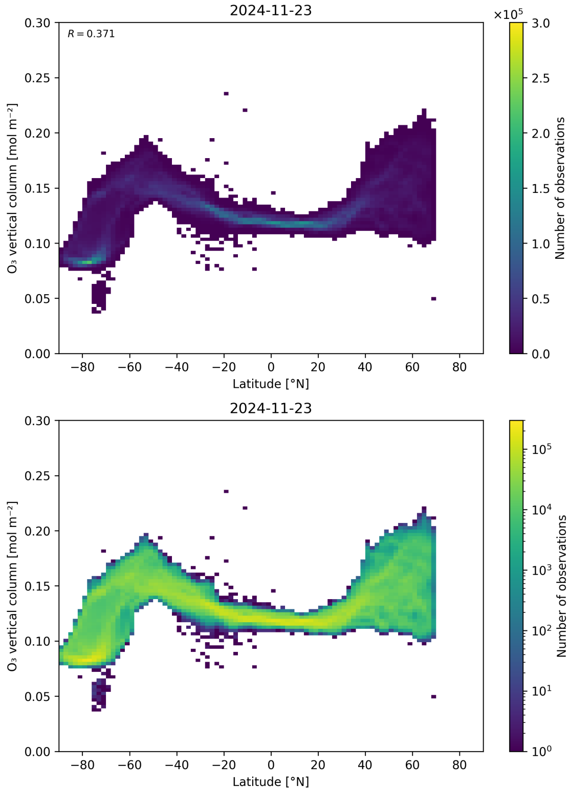
Figure 36: Scatter density plot of “Latitude” against “O 3 vertical column” for 2024-11-22 to 2024-11-24.
