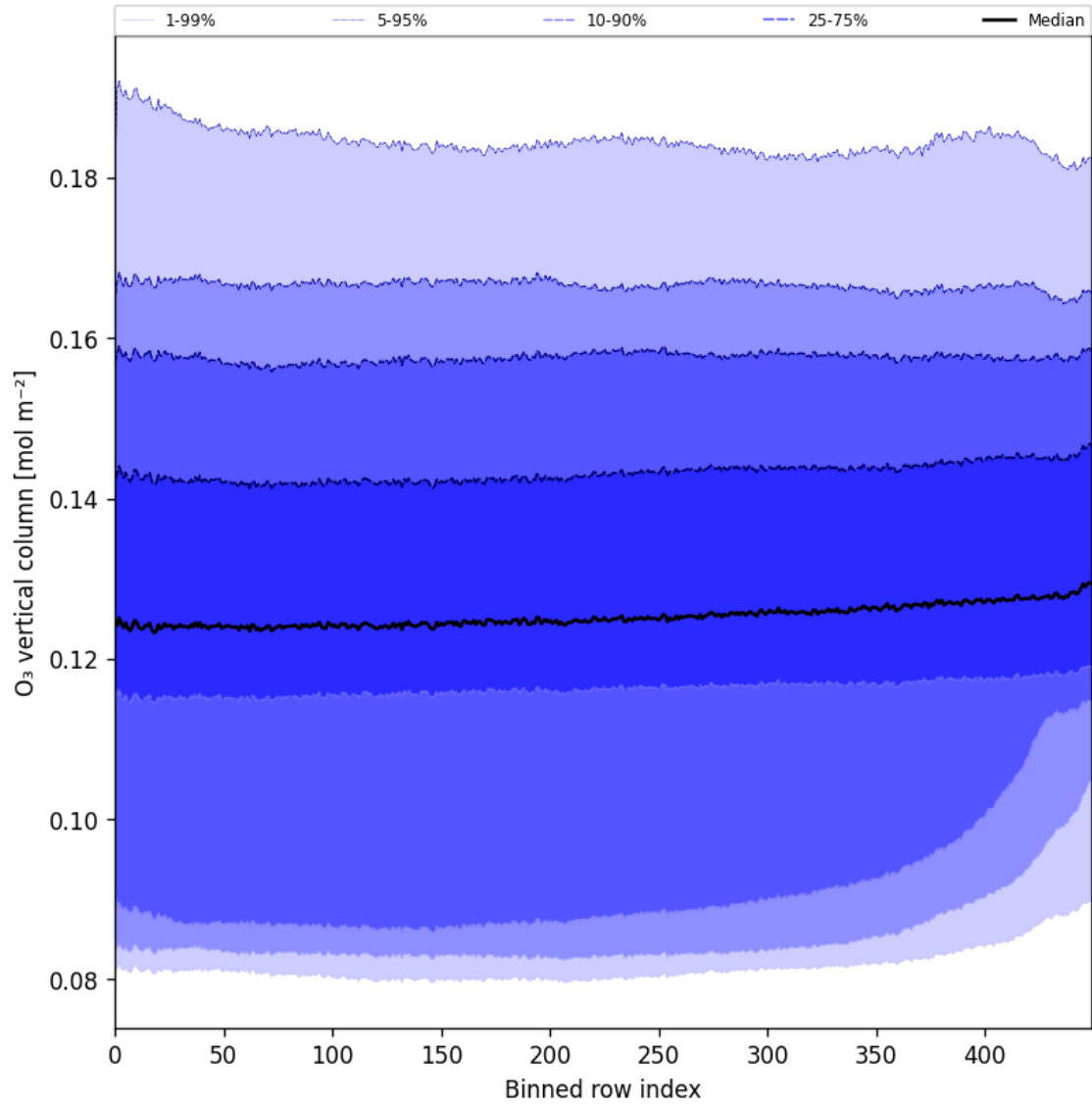
Figure 28: Along track statistics of “O 3 vertical column” for 2024-11-22 to 2024-11-24
