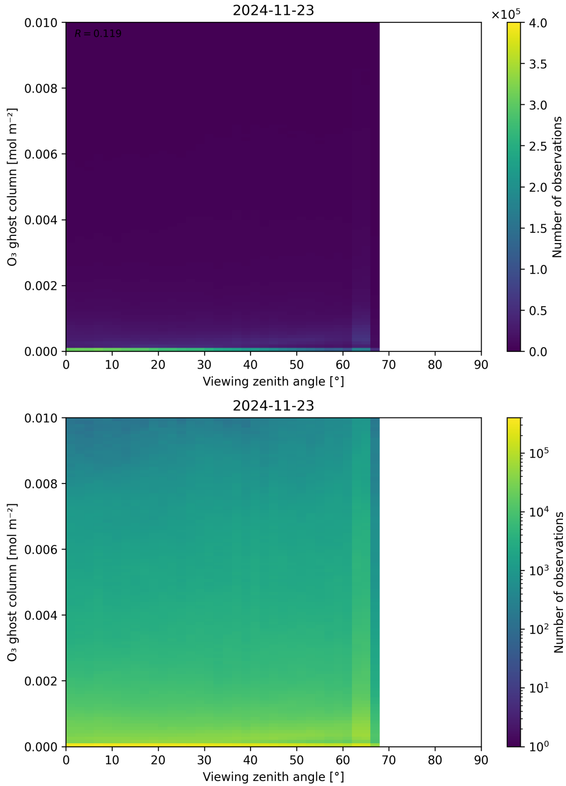
Figure 51: Scatter density plot of “Viewing zenith angle” against “O 3 ghost column” for 2024-11-22 to 2024-11-24.
