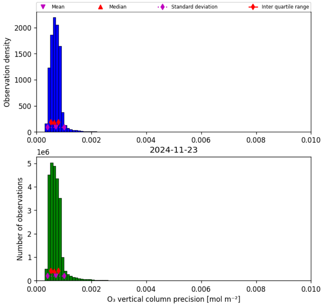
Figure 22: Histogram of "O 3 vertical column precision" for 2024-11-22 to 2024-11-24
