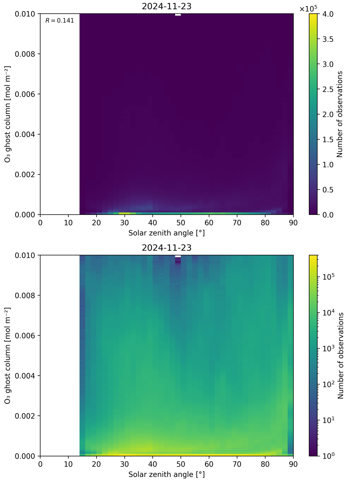
Figure 46: Scatter density plot of “Solar zenith angle” against “O 3 ghost column” for 2024-11-22 to 2024-11-24.
