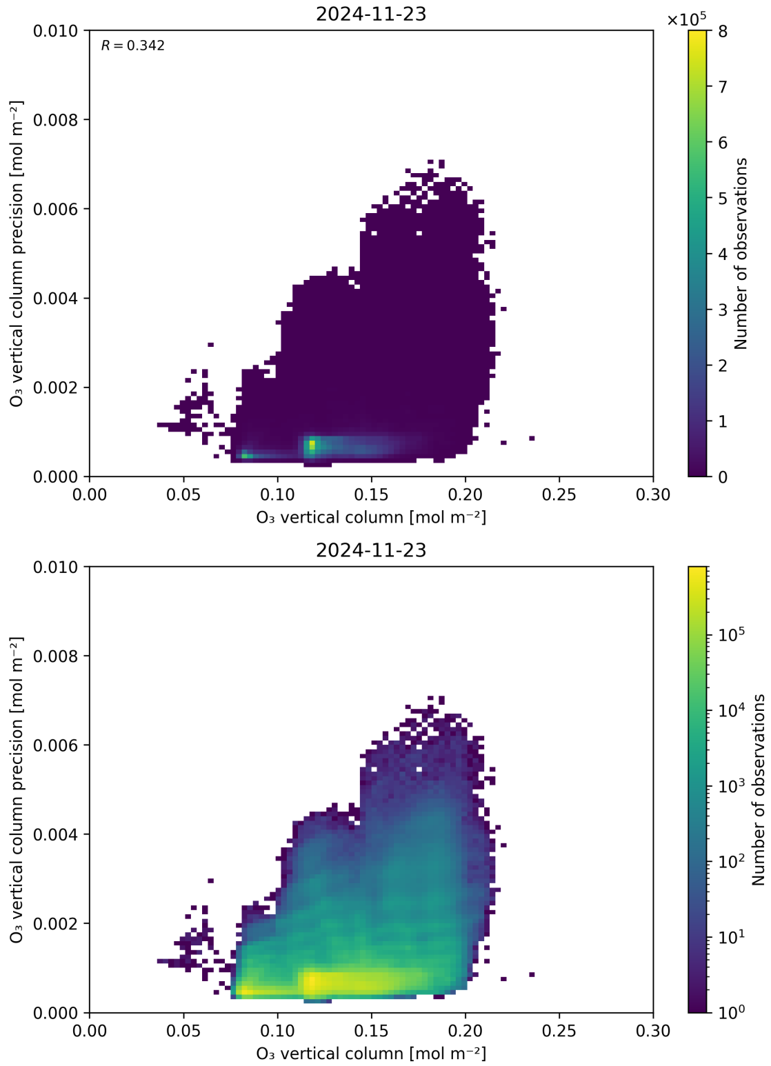
Figure 41: Scatter density plot of “O 3 vertical column” against “O 3 vertical column precision” for 2024-11-22 to 2024-11-24.
