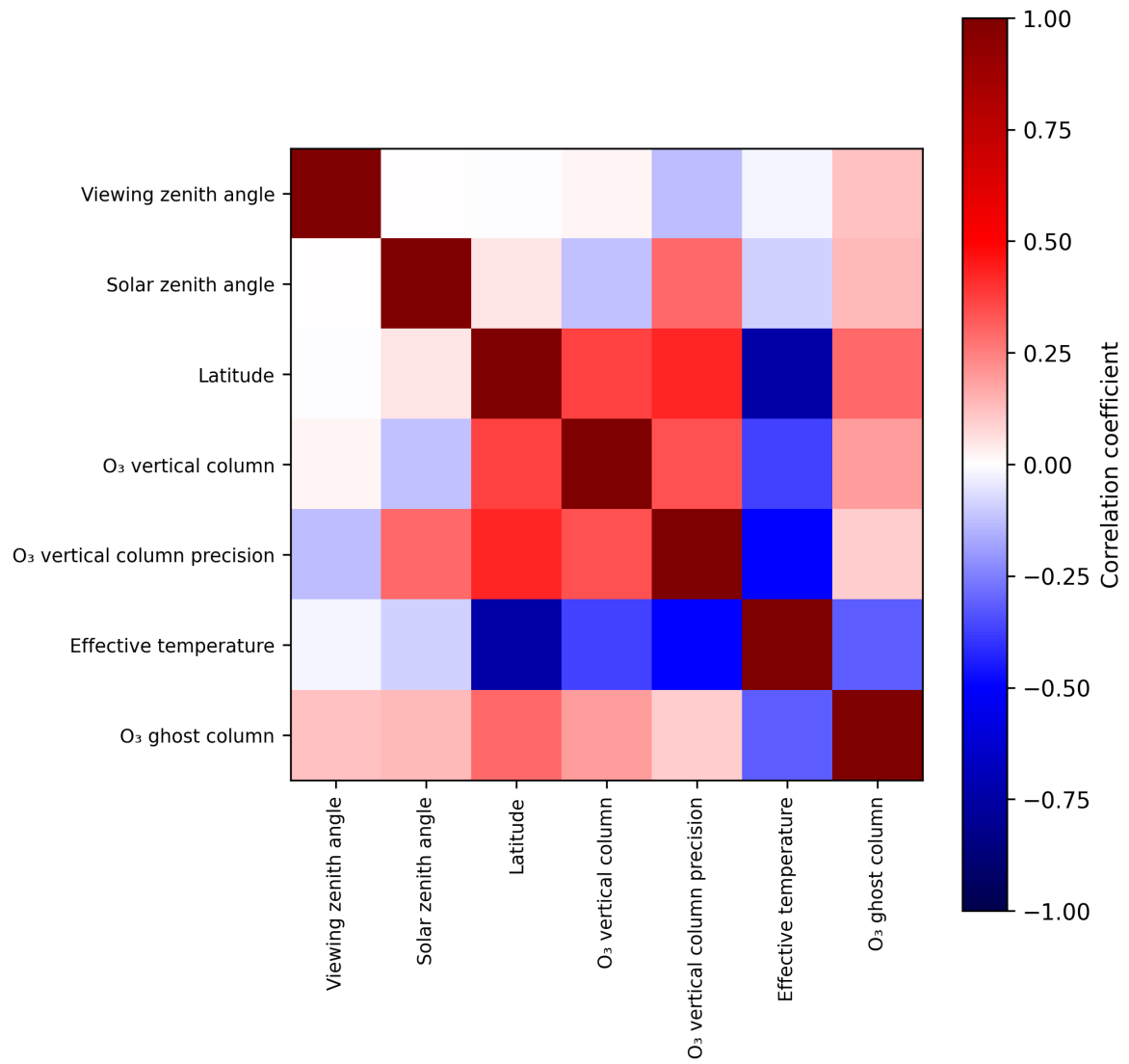
Figure 2: Map of correlation matrix for 2024-11-22 to 2024-11-24.
