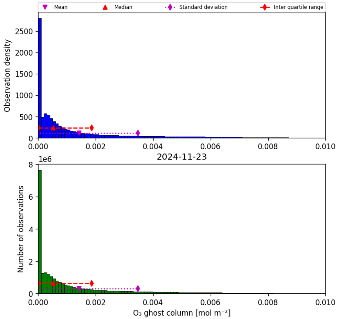
Figure 25: Histogram of "O 3 ghost column" for 2024-11-22 to 2024-11-24
