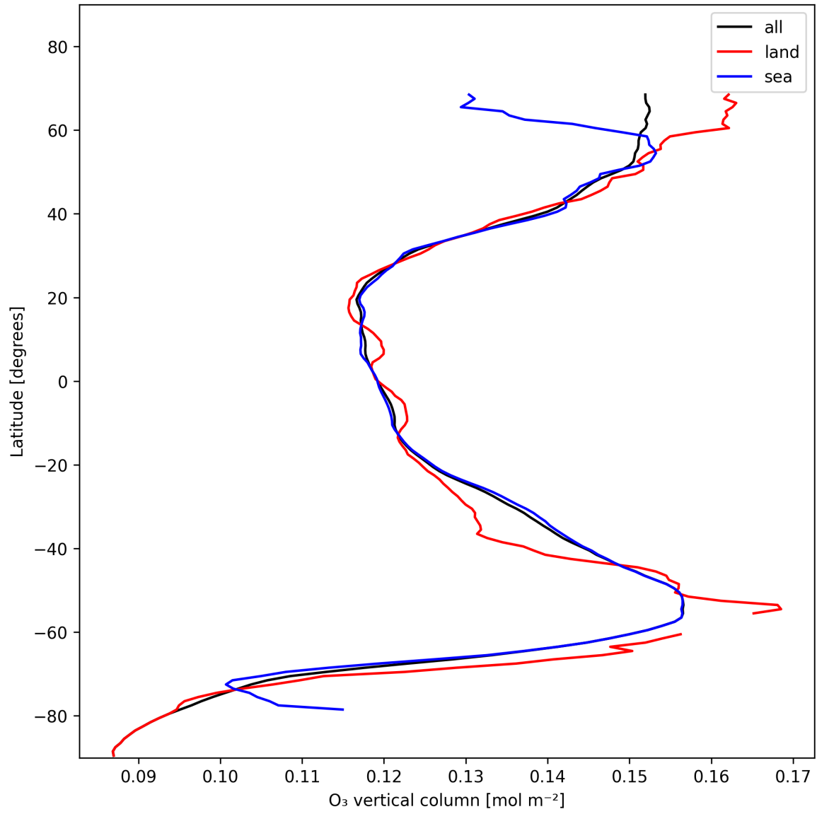
Figure 14: Zonal average of “O 3 vertical column” for 2024-11-22 to 2024-11-24.
