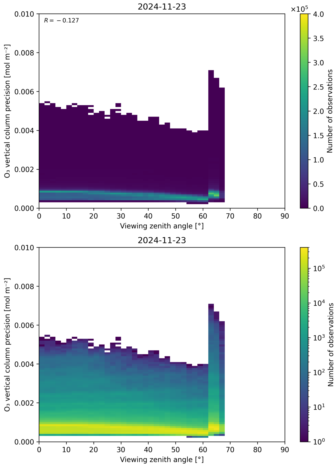
Figure 53: Scatter density plot of “Viewing zenith angle” against “O 3 vertical column precision” for 2024-11-22 to 2024-11-24.
