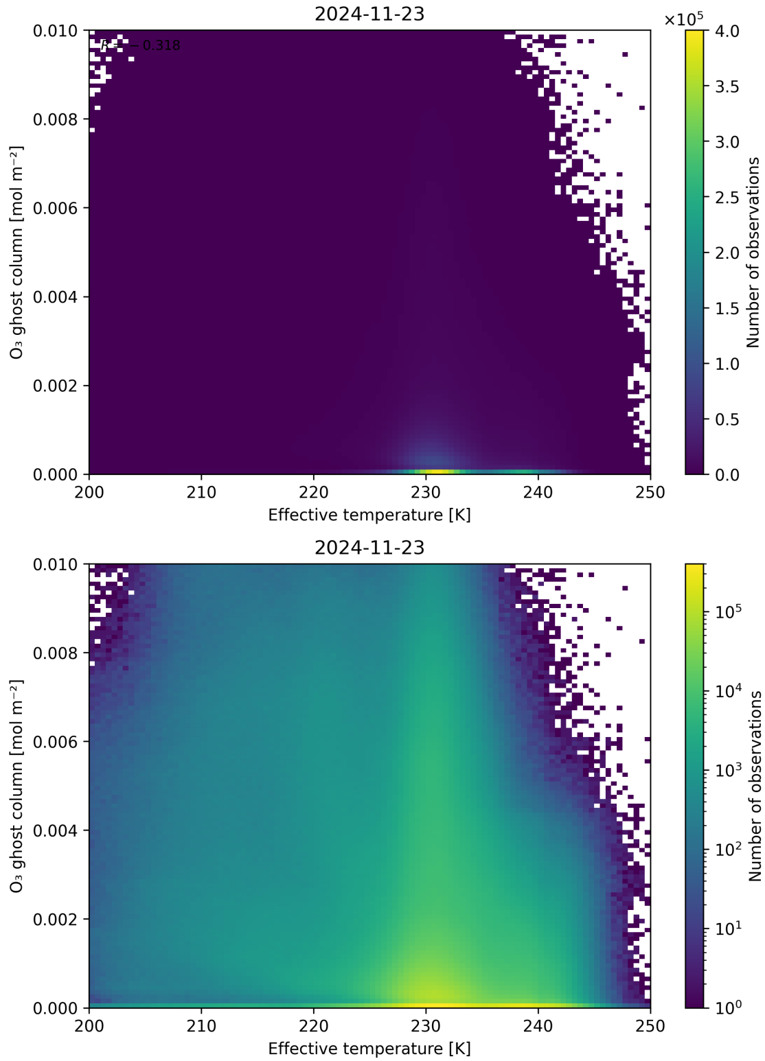
Figure 38: Scatter density plot of “Effective temperature” against “O 3 ghost column” for 2024-11-22 to 2024-11-24.
