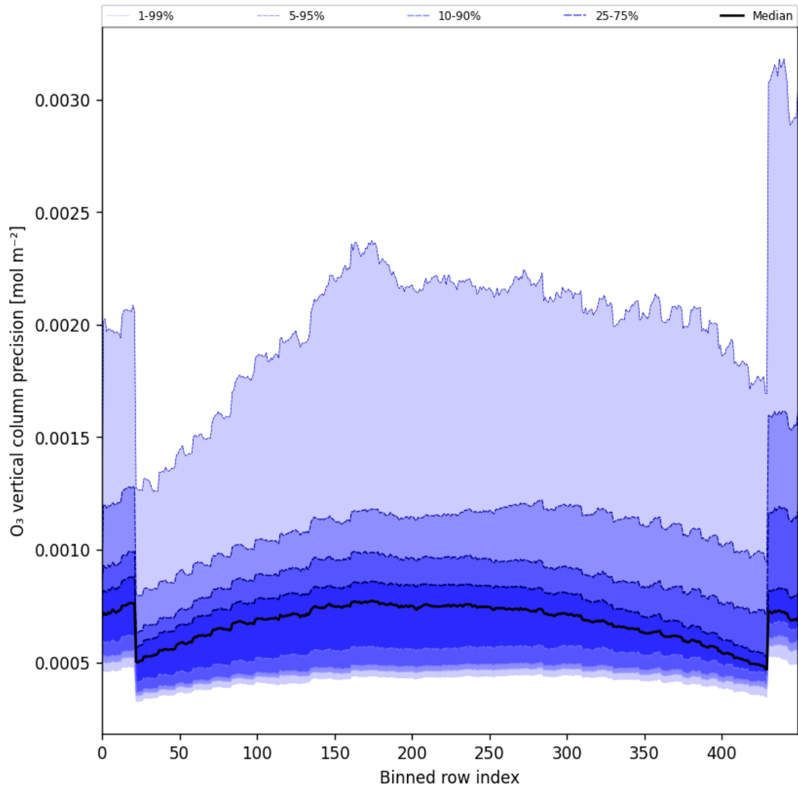
Figure 29: Along track statistics of “O 3 vertical column precision” for 2024-11-22 to 2024-11-24
