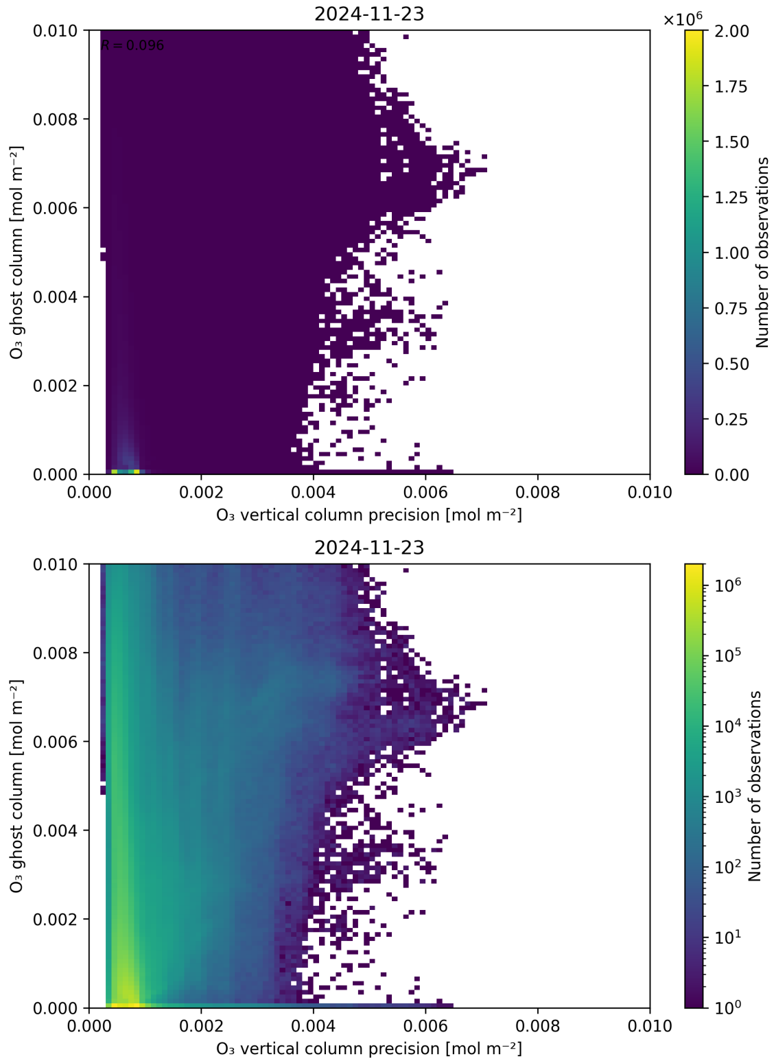
Figure 43: Scatter density plot of “ \text{O}_3 vertical column precision” against “ \text{O}_3 ghost column” for 2024-11-22 to 2024-11-24.
