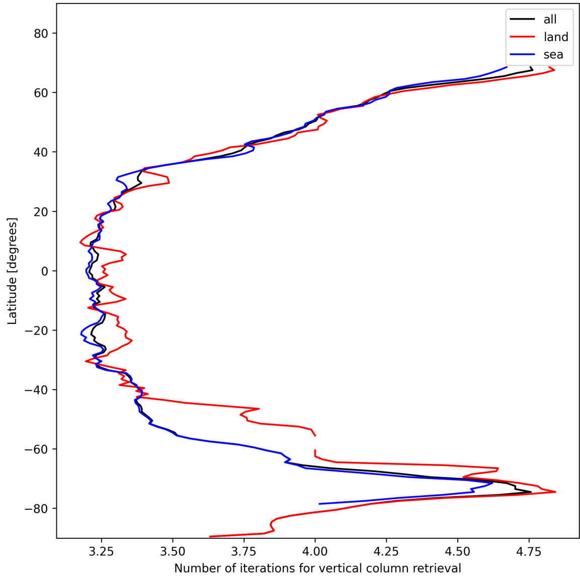
Figure 19: Zonal average of “Number of iterations for vertical column retrieval” for 2024-11-22 to 2024-11-24.
