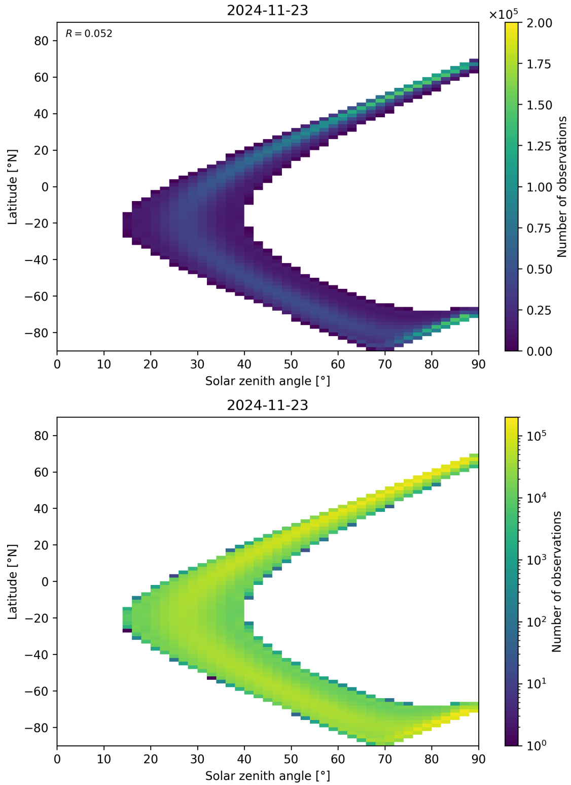
Figure 44: Scatter density plot of “Solar zenith angle” against “Latitude” for 2024-11-22 to 2024-11-24.
