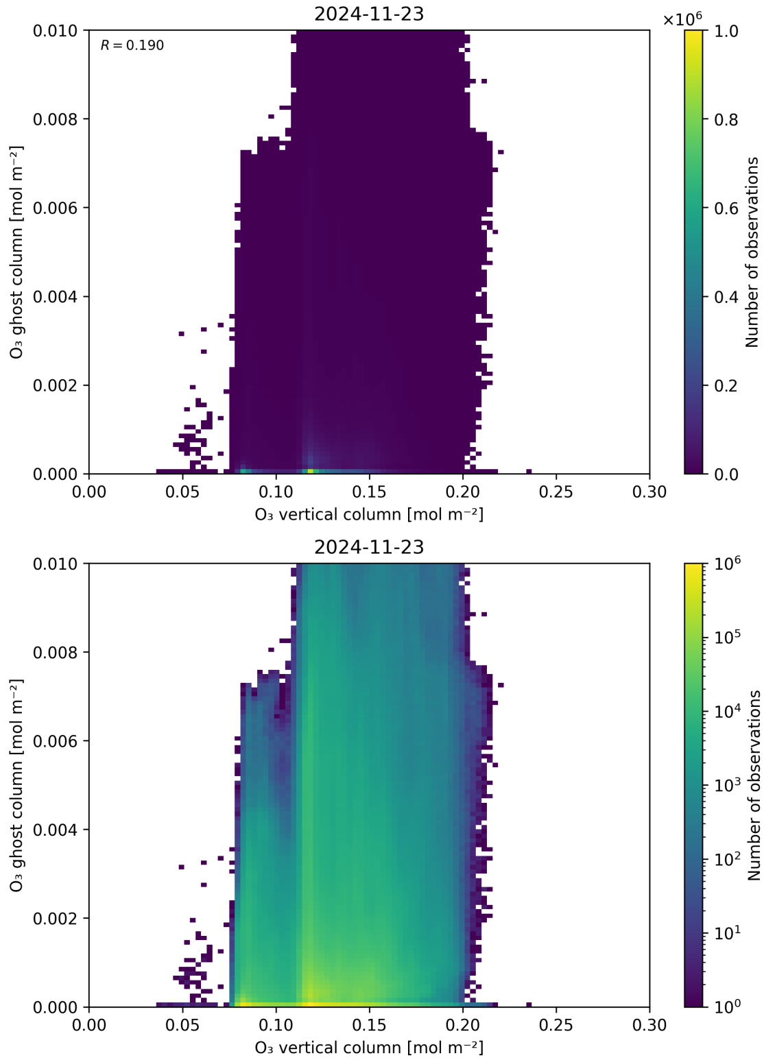
Figure 40: Scatter density plot of “O 3 vertical column” against “O 3 ghost column” for 2024-11-22 to 2024-11-24.
