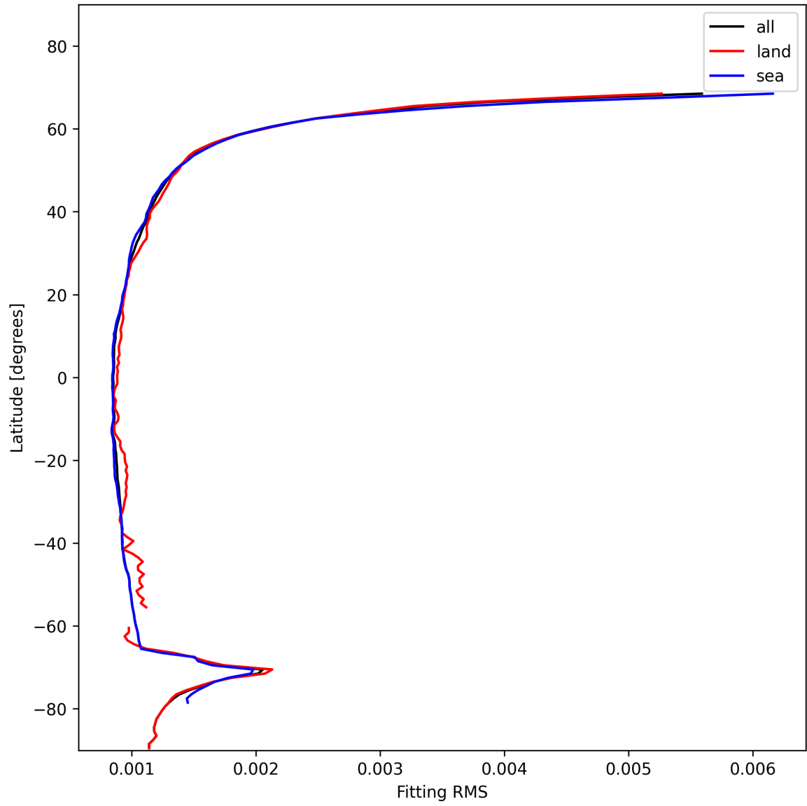
Figure 16: Zonal average of “Fitting RMS” for 2024-11-22 to 2024-11-24.
