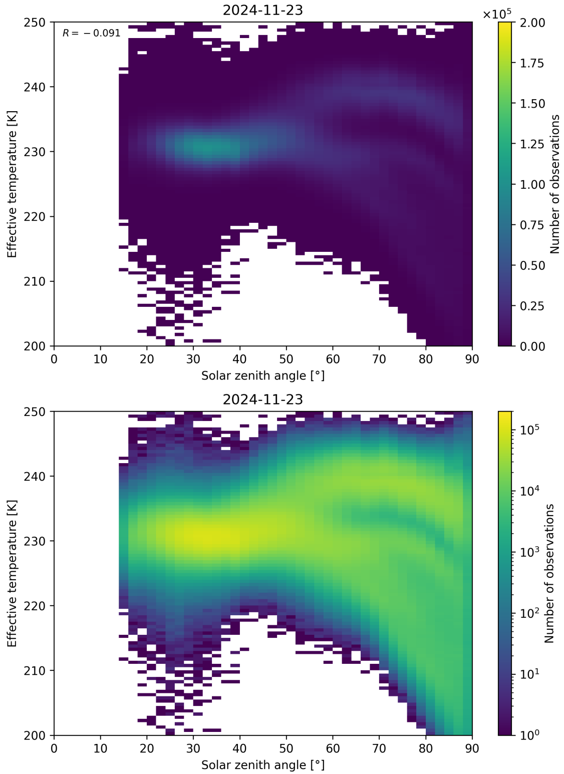
Figure 45: Scatter density plot of “Solar zenith angle” against “Effective temperature” for 2024-11-22 to 2024-11-24.
