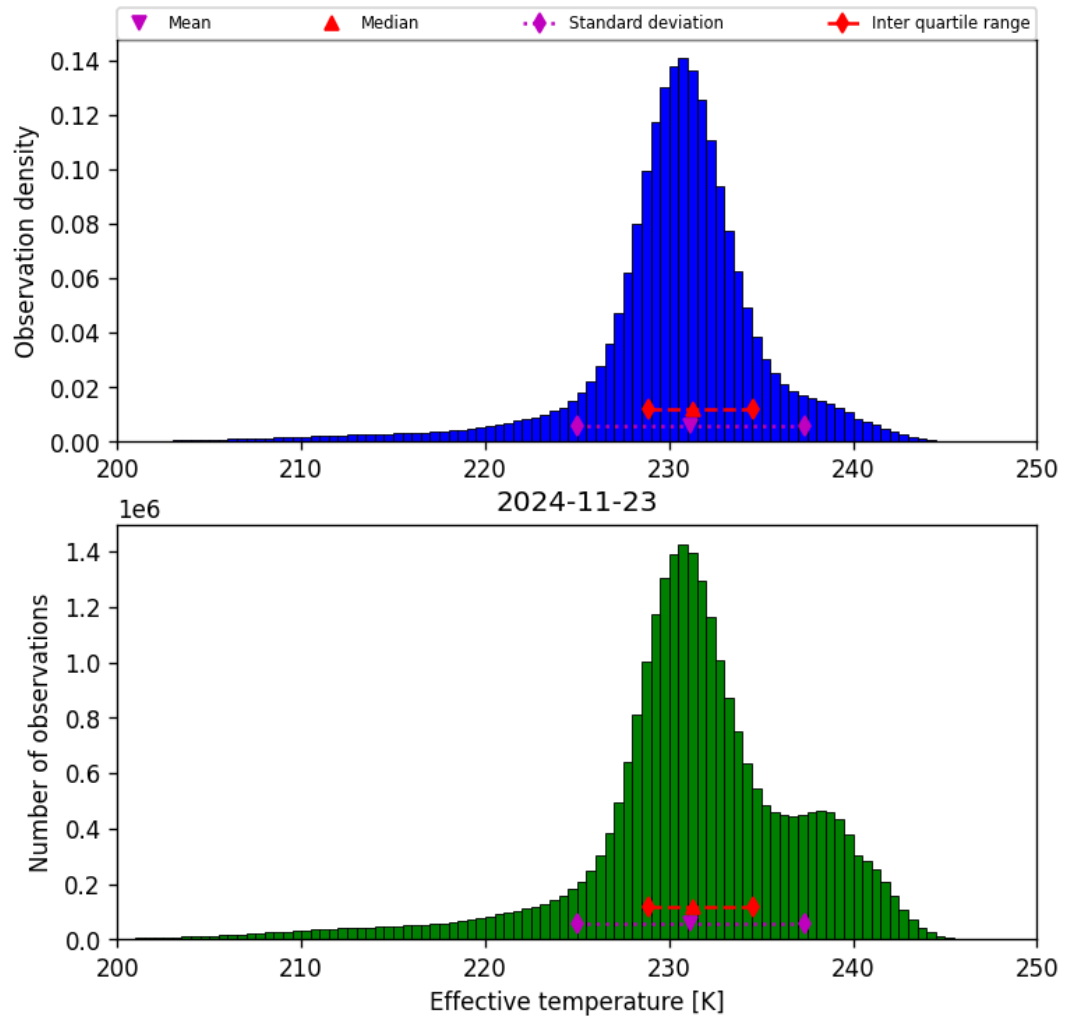
Figure 24: Histogram of “Effective temperature” for 2024-11-22 to 2024-11-24
