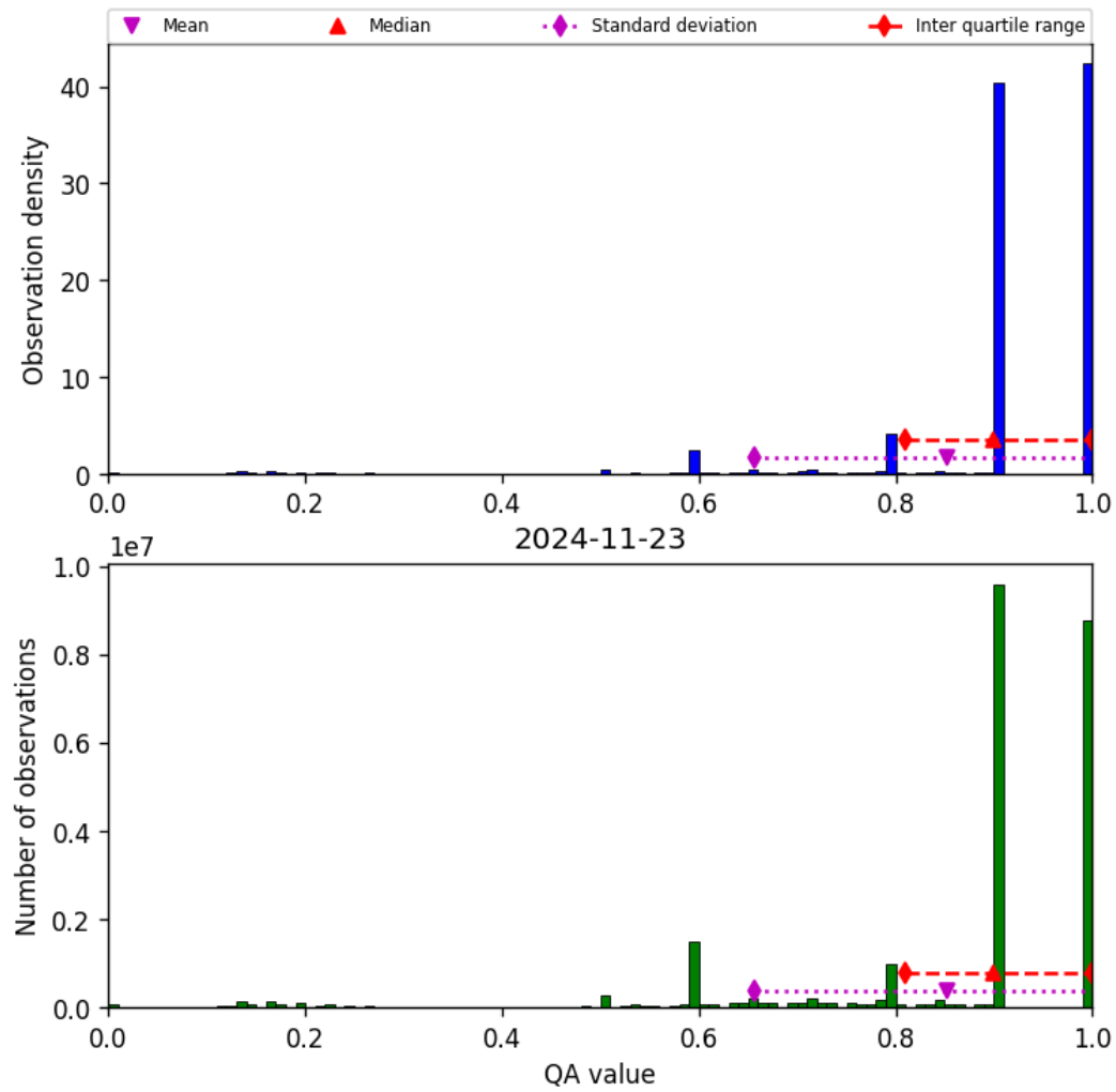
Figure 20: Histogram of “QA value” for 2024-11-22 to 2024-11-24
