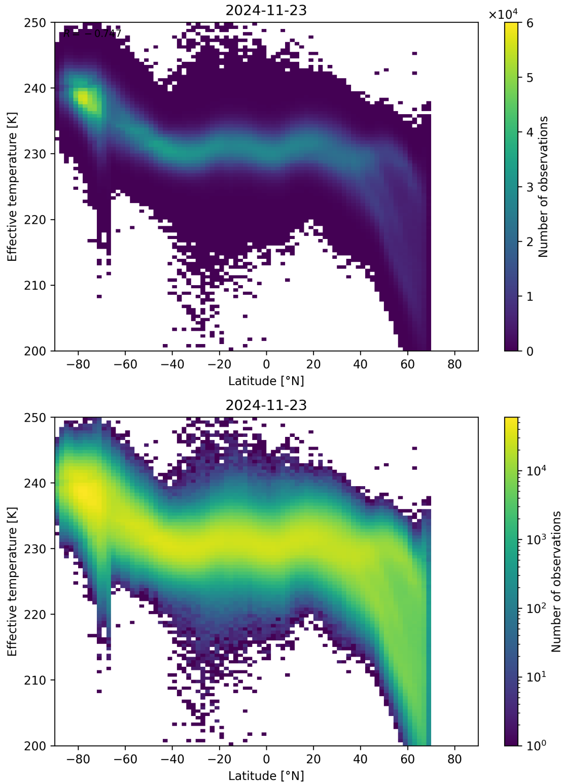
Figure 34: Scatter density plot of “Latitude” against “Effective temperature” for 2024-11-22 to 2024-11-24.
