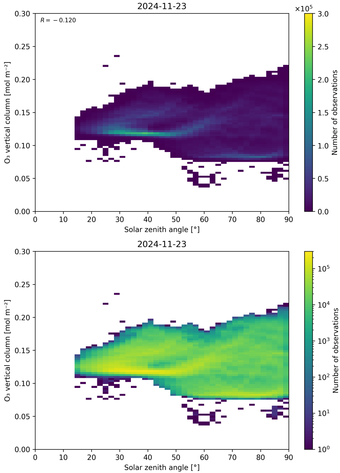
Figure 47: Scatter density plot of “Solar zenith angle” against “O 3 vertical column” for 2024-11-22 to 2024-11-24.
