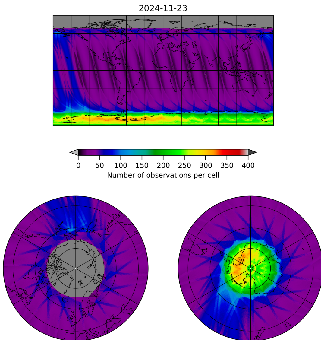
Figure 12: Map of the number of observations for 2024-11-22 to 2024-11-24
