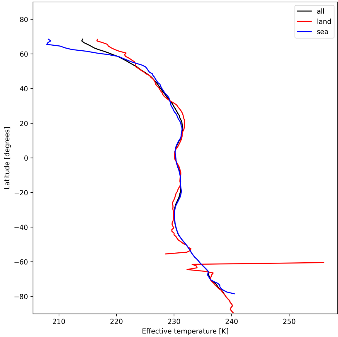
Figure 17: Zonal average of “Effective temperature” for 2024-11-22 to 2024-11-24.
