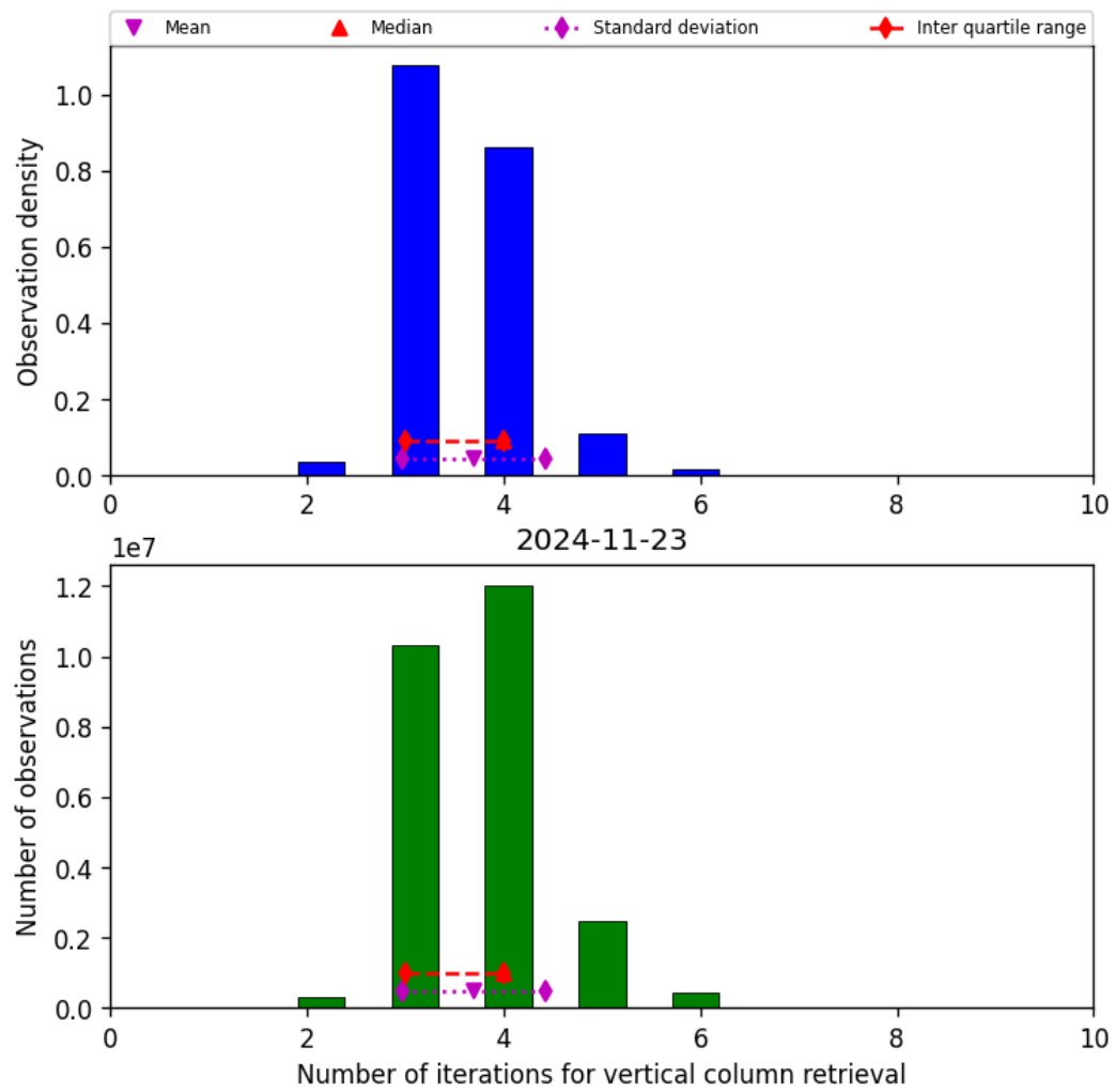
Figure 26: Histogram of "Number of iterations for vertical column retrieval" for 2024-11-22 to 2024-11-24
