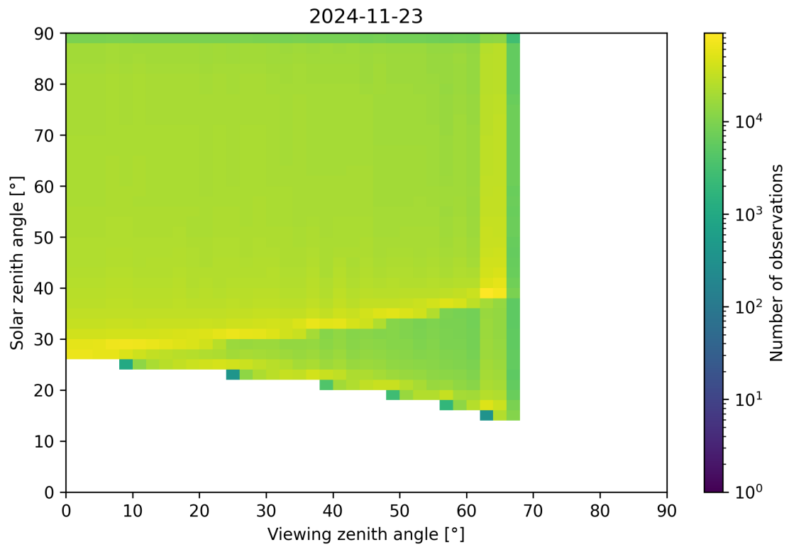
Figure 54: Scatter density plot of “Viewing zenith angle” against “Solar zenith angle” for 2024-11-22 to 2024-11-24.
