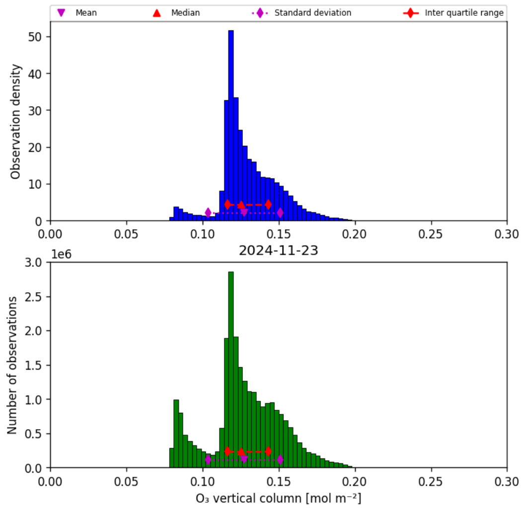
Figure 21: Histogram of “O 3 vertical column” for 2024-11-22 to 2024-11-24
