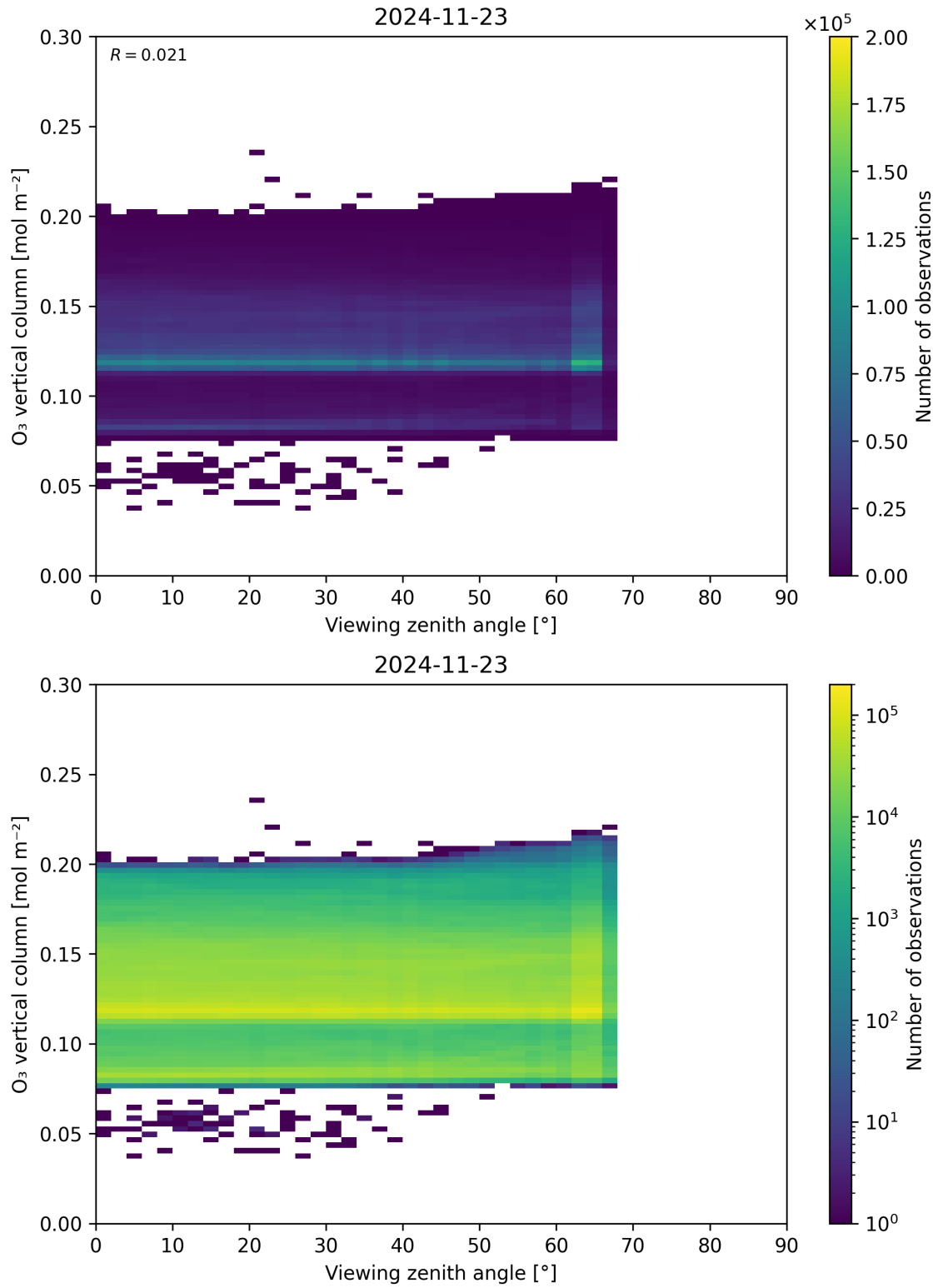
Figure 52: Scatter density plot of “Viewing zenith angle” against “O 3 vertical column” for 2024-11-22 to 2024-11-24.
