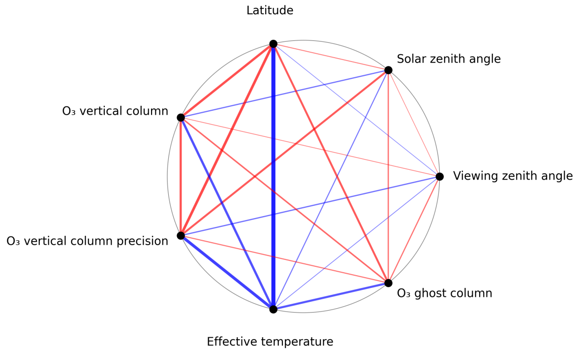
Figure 1: Map of correlation graph for 2024-11-22 to 2024-11-24.
