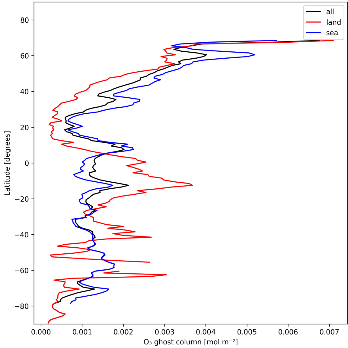
Figure 18: Zonal average of "O 3 ghost column" for 2024-11-22 to 2024-11-24.
