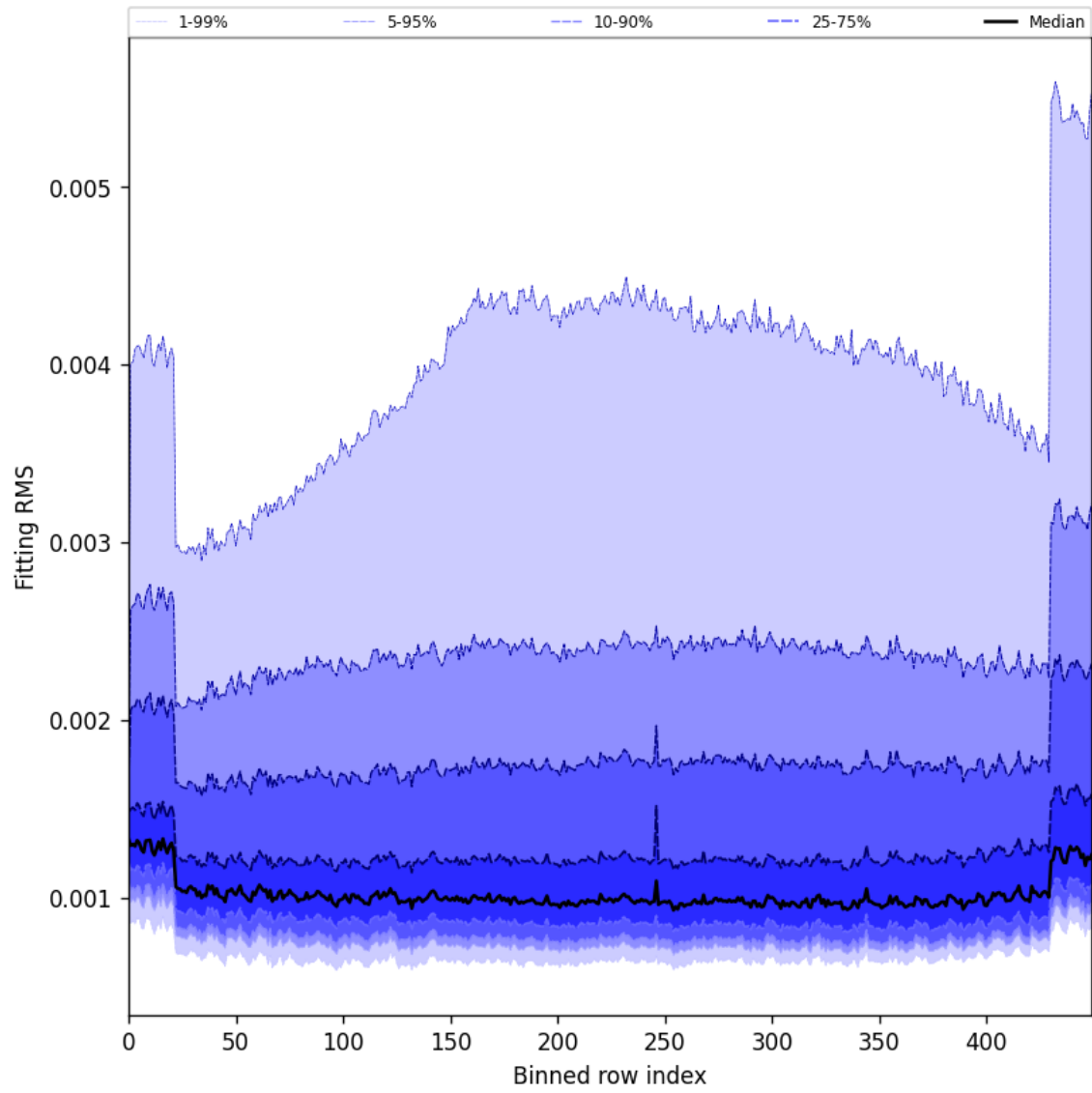
Figure 30: Along track statistics of “Fitting RMS” for 2024-11-22 to 2024-11-24
