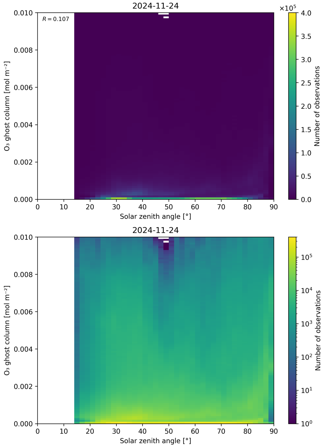
Figure 46: Scatter density plot of “Solar zenith angle” against “O 3 ghost column” for 2024-11-23 to 2024-11-25.
