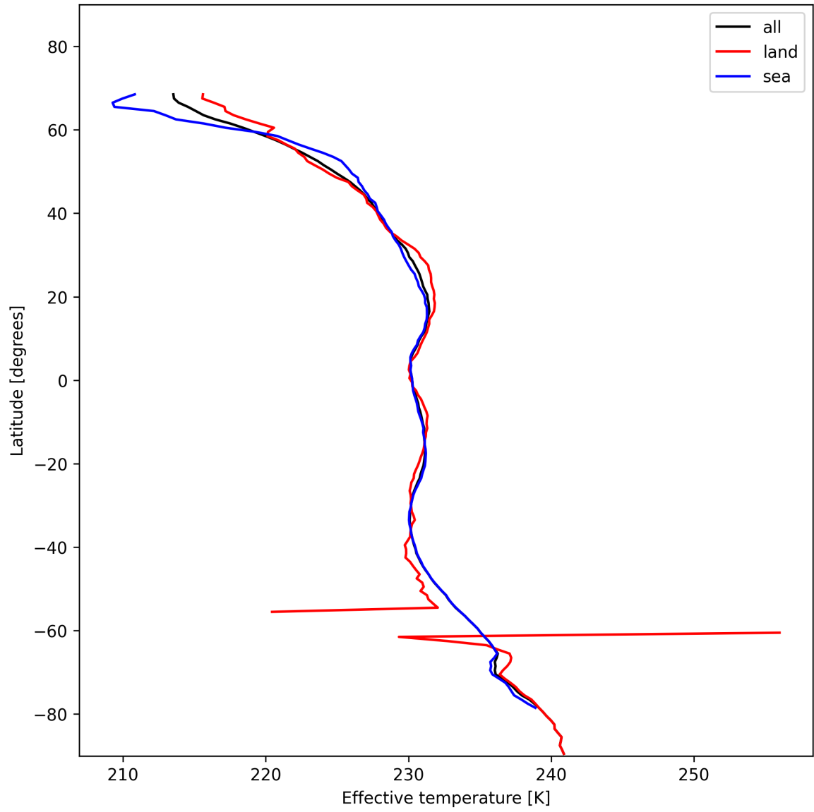
Figure 17: Zonal average of “Effective temperature” for 2024-11-23 to 2024-11-25.
