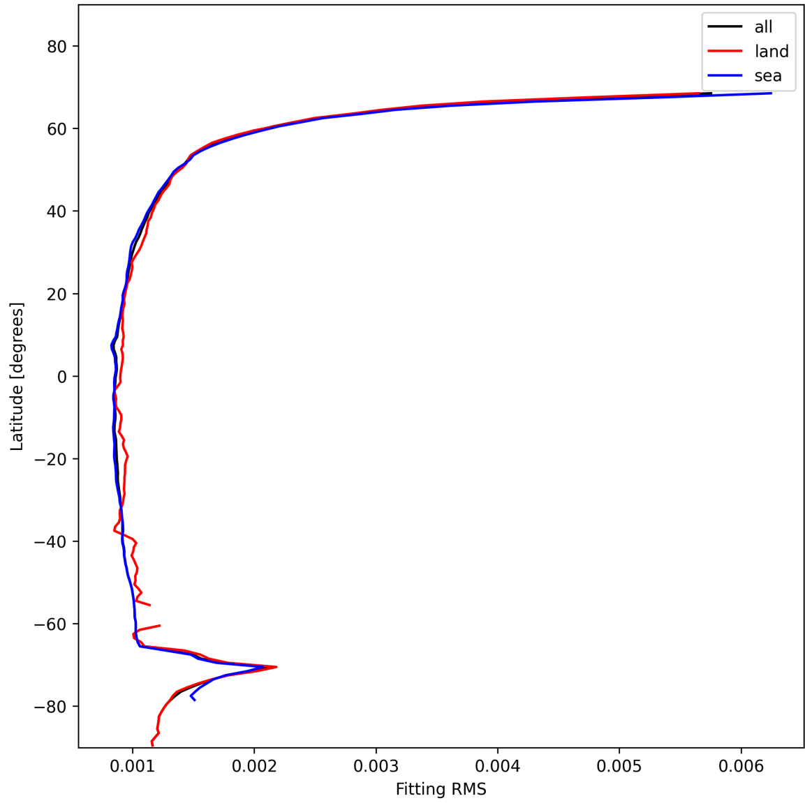
Figure 16: Zonal average of “Fitting RMS” for 2024-11-23 to 2024-11-25.
