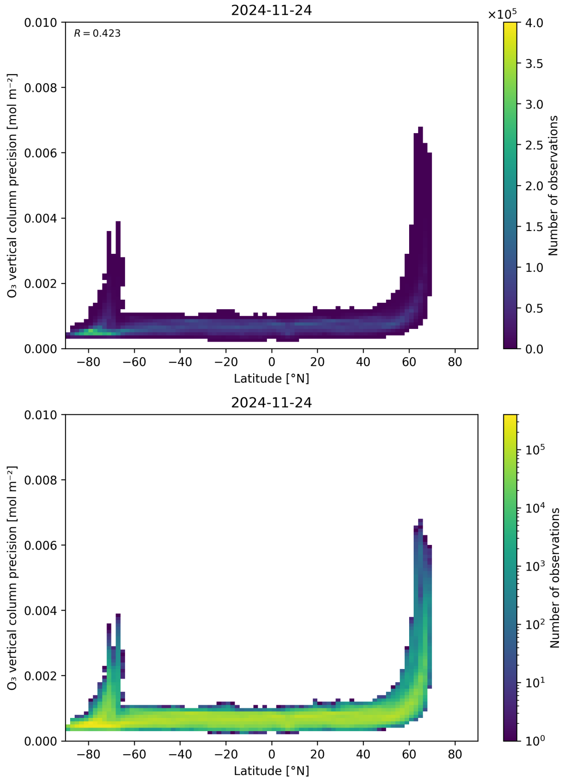
Figure 37: Scatter density plot of “Latitude” against “O 3 vertical column precision” for 2024-11-23 to 2024-11-25.
