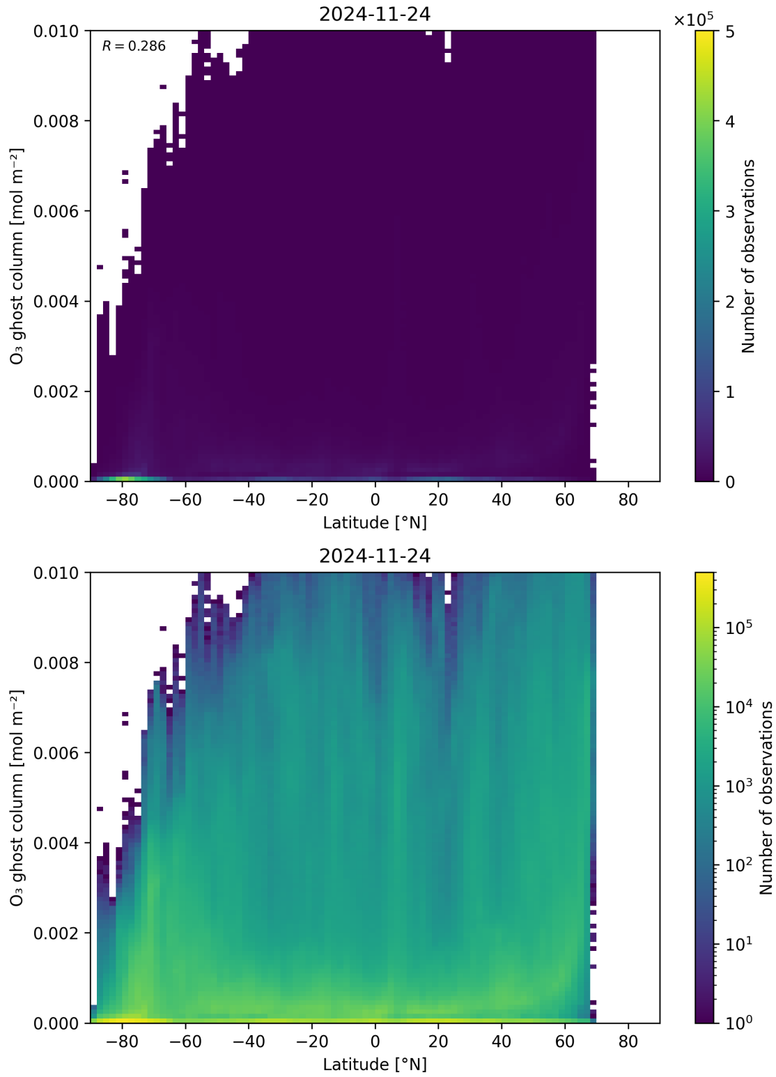
Figure 35: Scatter density plot of “Latitude” against “O 3 ghost column” for 2024-11-23 to 2024-11-25.
