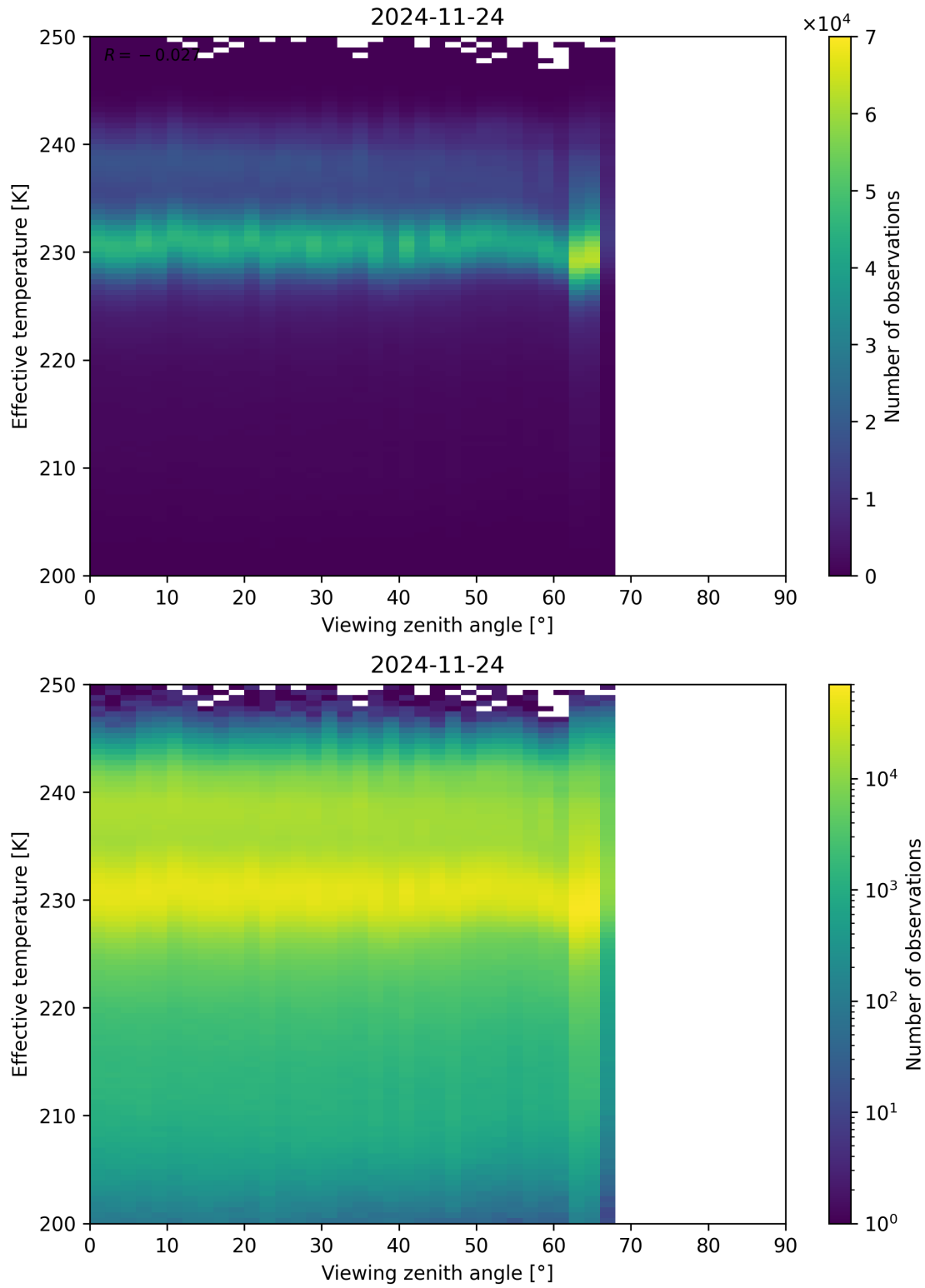
Figure 50: Scatter density plot of “Viewing zenith angle” against “Effective temperature” for 2024-11-23 to 2024-11-25.
