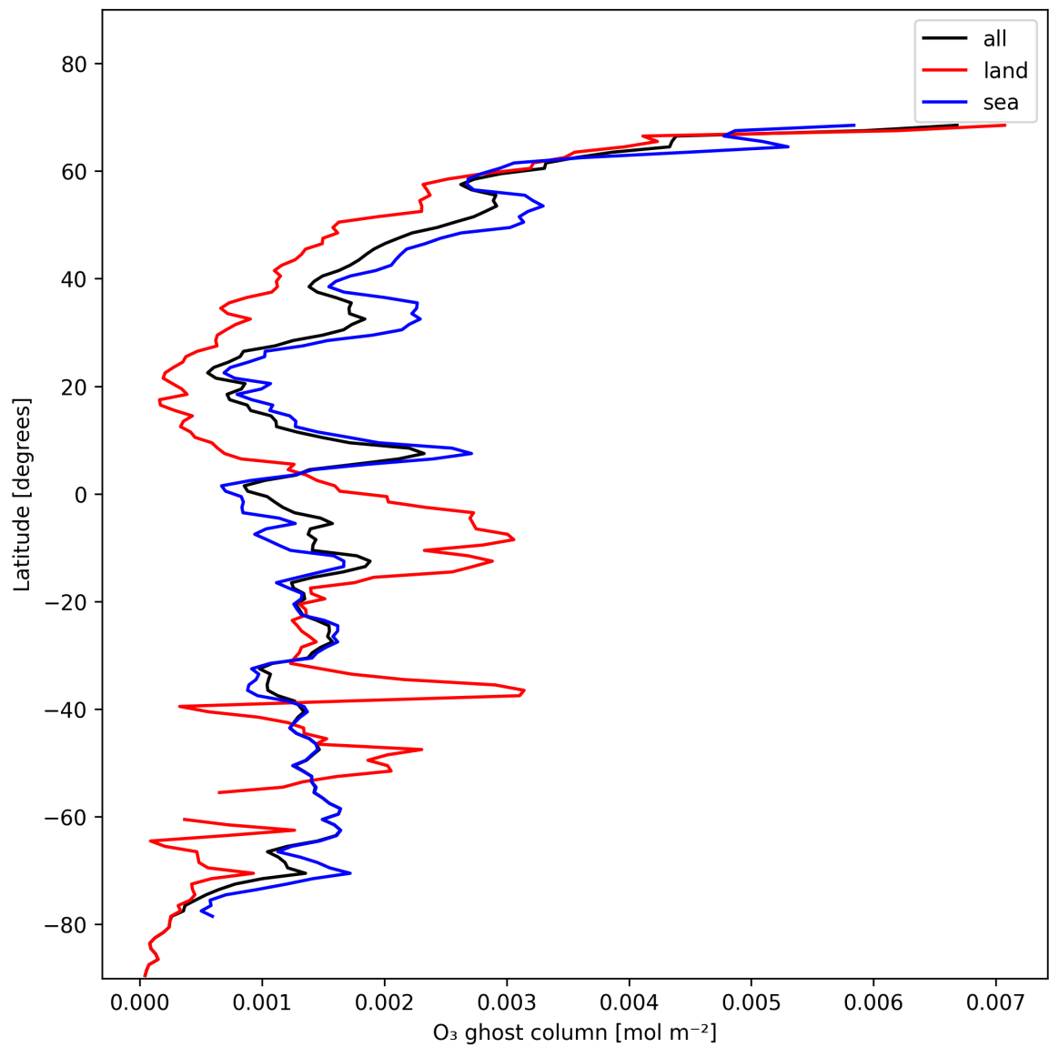
Figure 18: Zonal average of “O 3 ghost column” for 2024-11-23 to 2024-11-25.
