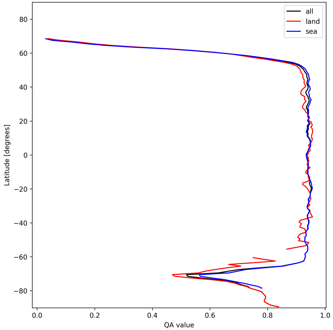
Figure 13: Zonal average of “QA value” for 2024-11-23 to 2024-11-25.
