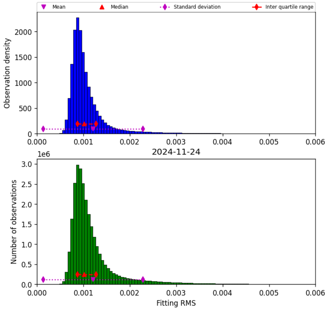
Figure 23: Histogram of “Fitting RMS” for 2024-11-23 to 2024-11-25
