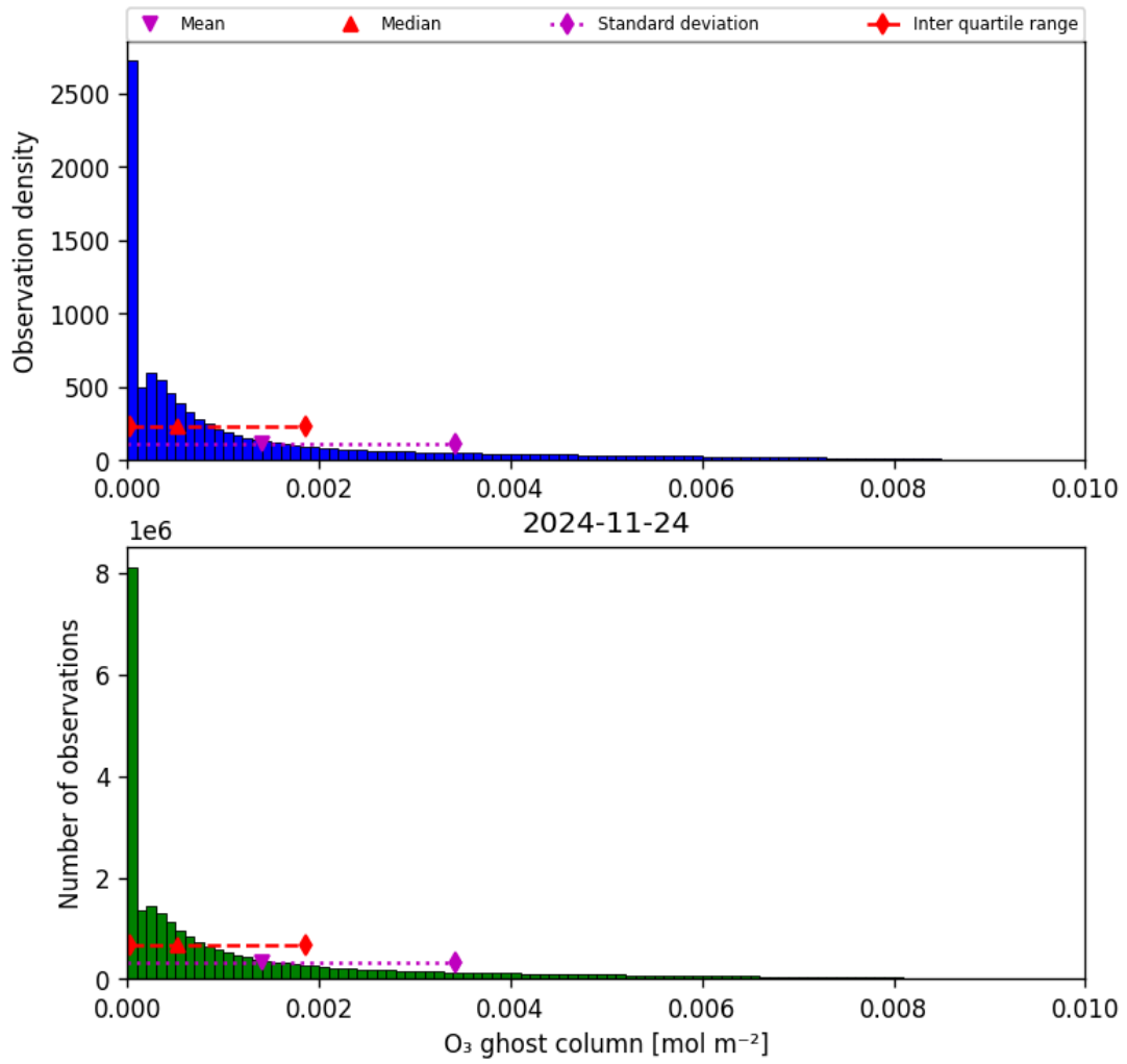
Figure 25: Histogram of “O 3 ghost column” for 2024-11-23 to 2024-11-25
