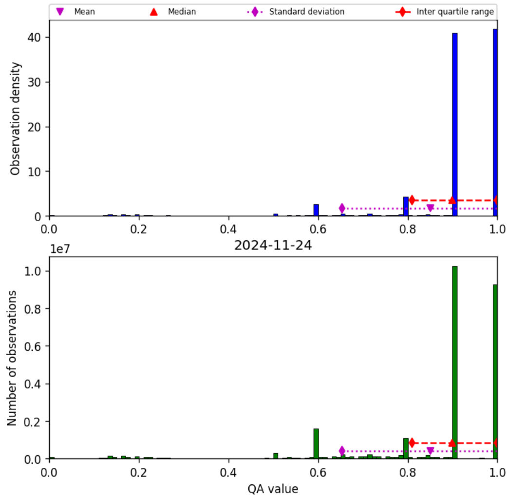
Figure 20: Histogram of “QA value” for 2024-11-23 to 2024-11-25
