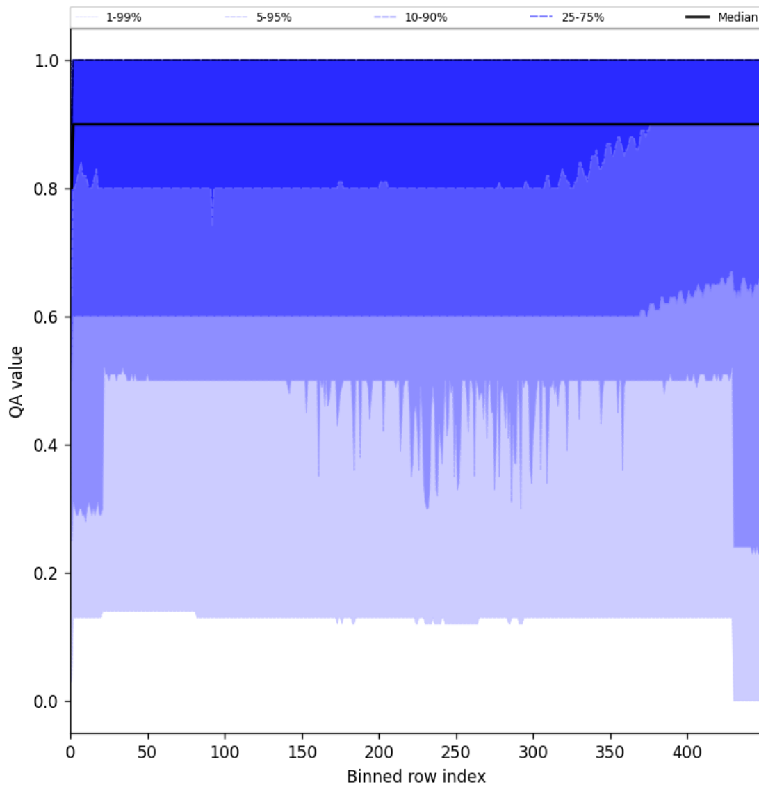
Figure 27: Along track statistics of “QA value” for 2024-11-23 to 2024-11-25
