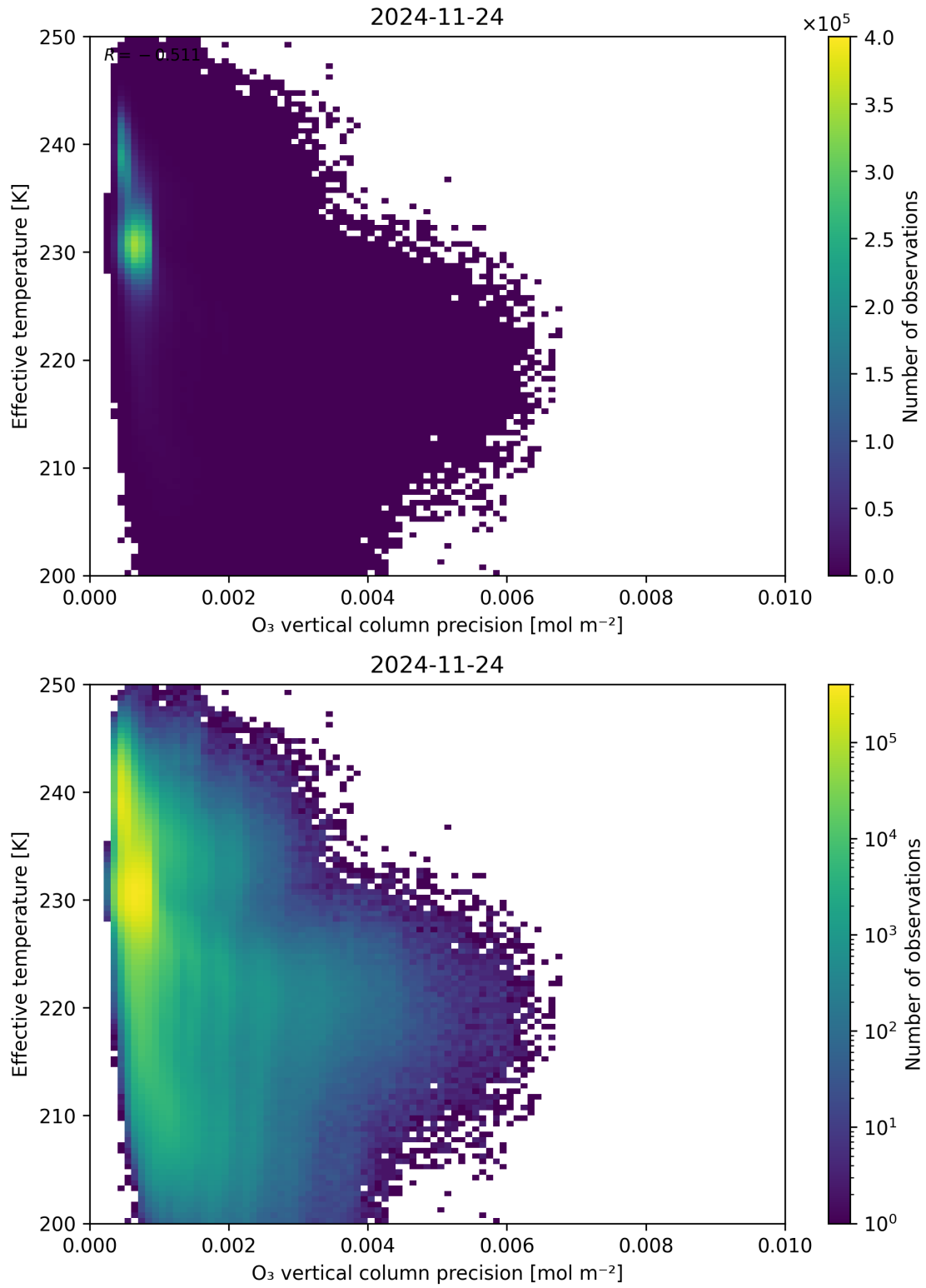
Figure 42: Scatter density plot of “O 3 vertical column precision” against “Effective temperature” for 2024-11-23 to 2024-11-25.
