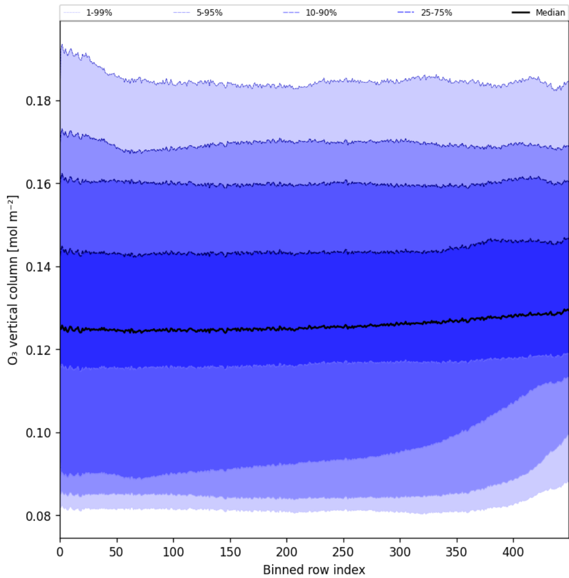
Figure 28: Along track statistics of “O 3 vertical column” for 2024-11-23 to 2024-11-25
