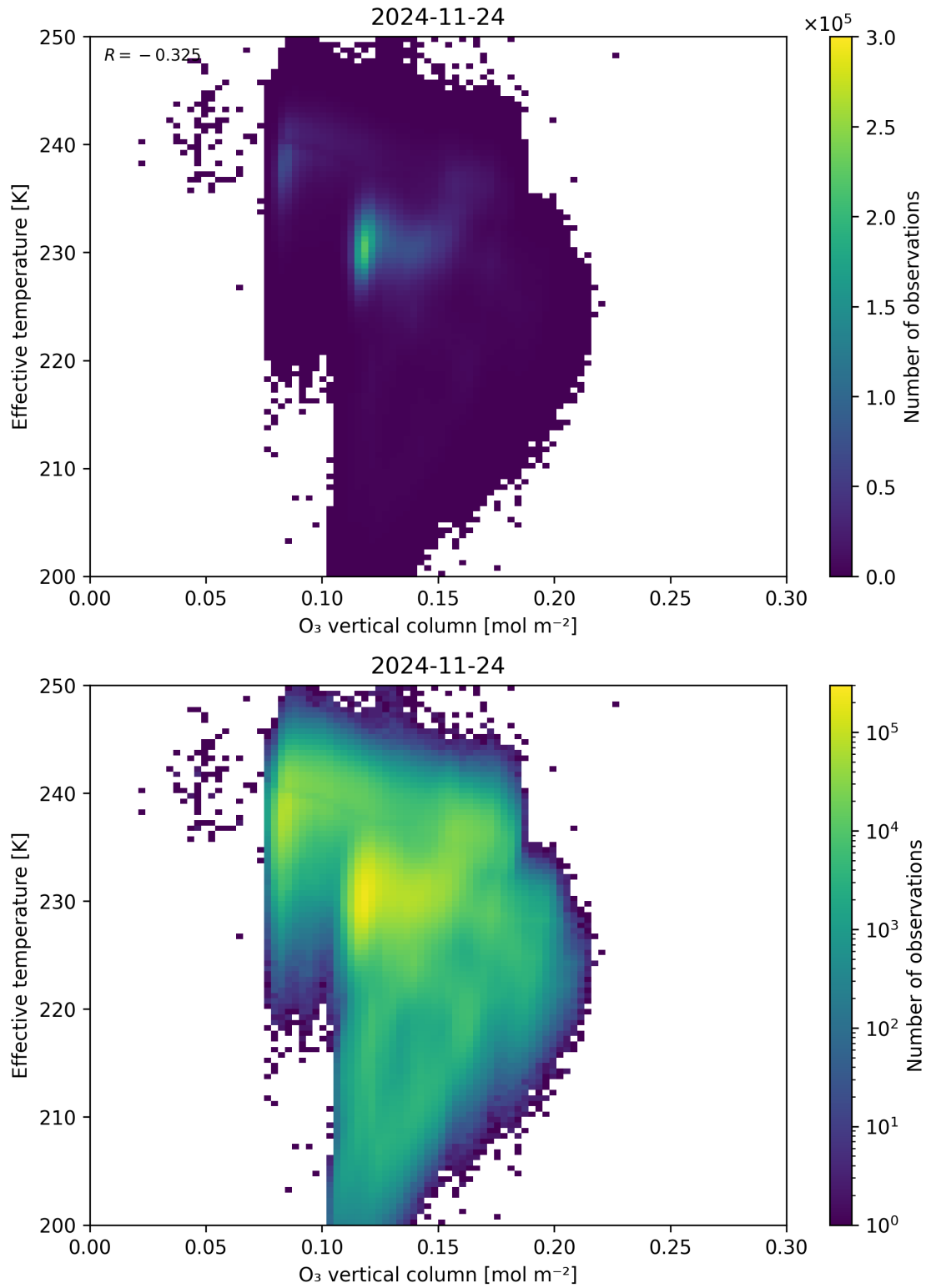
Figure 39: Scatter density plot of “O 3 vertical column” against “Effective temperature” for 2024-11-23 to 2024-11-25.
