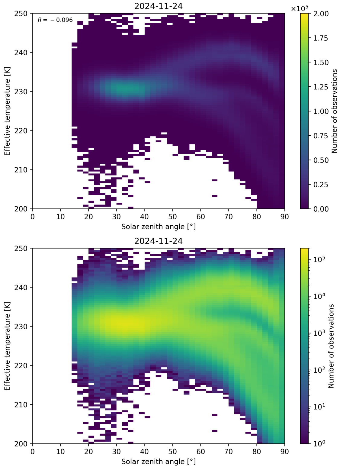
Figure 45: Scatter density plot of “Solar zenith angle” against “Effective temperature” for 2024-11-23 to 2024-11-25.
