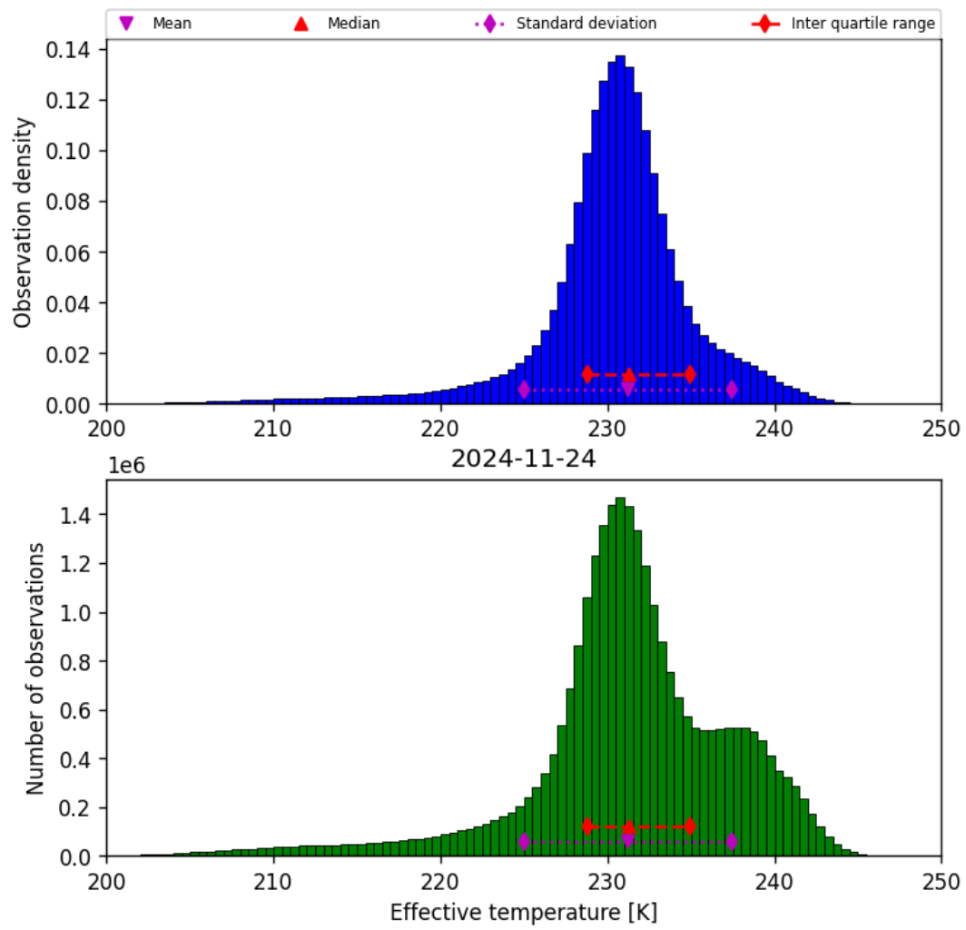
Figure 24: Histogram of “Effective temperature” for 2024-11-23 to 2024-11-25
