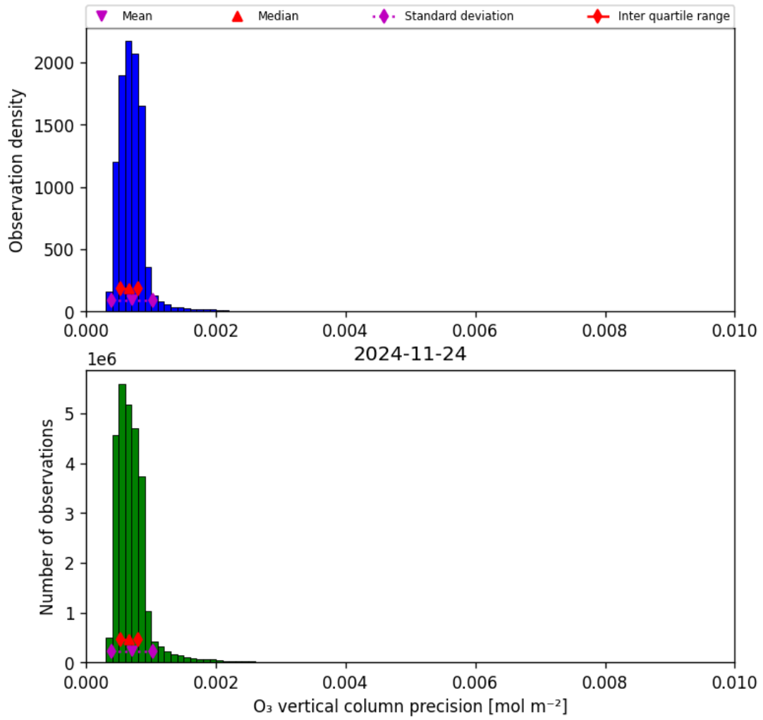
Figure 22: Histogram of “O 3 vertical column precision” for 2024-11-23 to 2024-11-25
