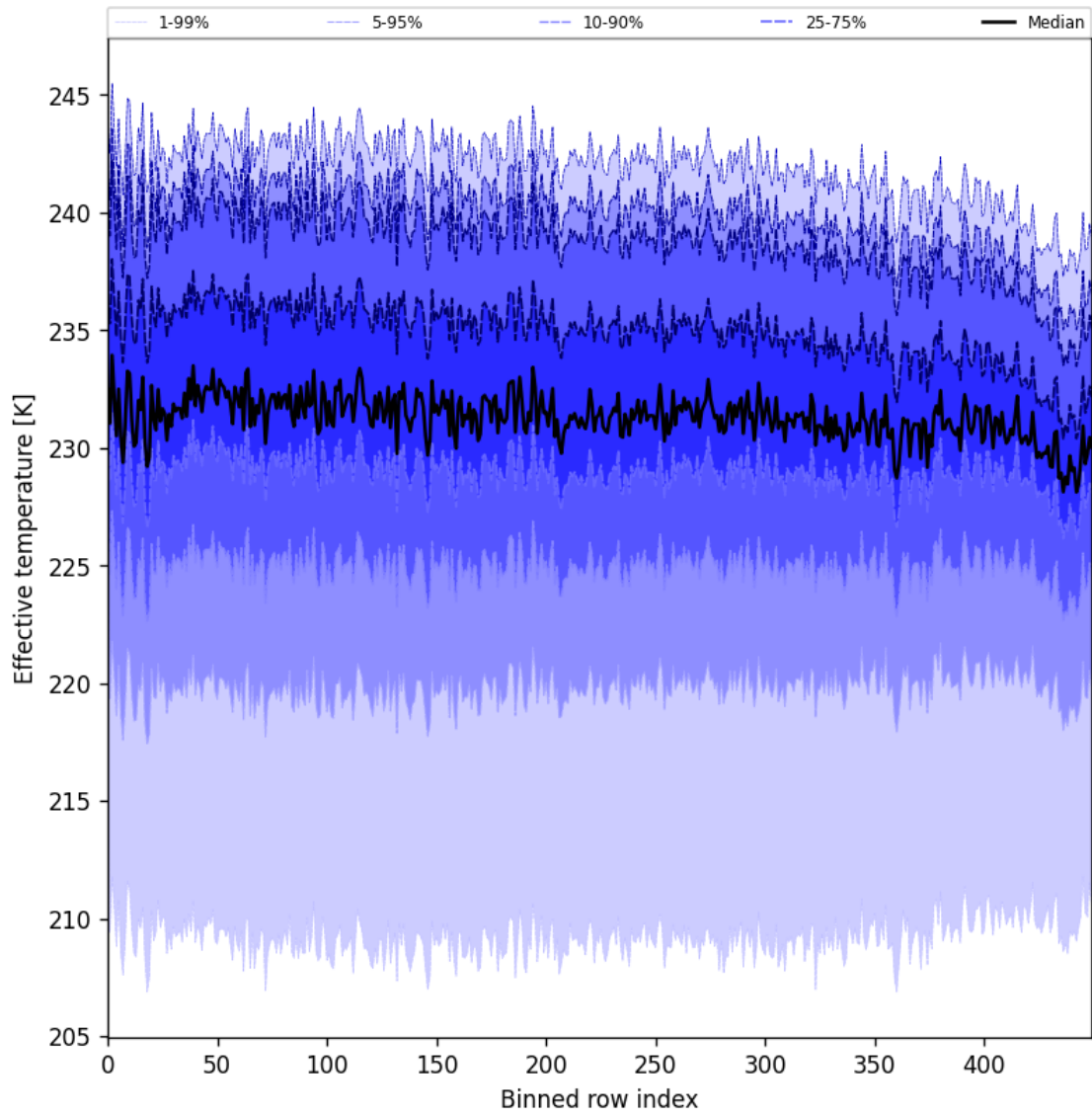
Figure 31: Along track statistics of “Effective temperature” for 2024-11-23 to 2024-11-25
