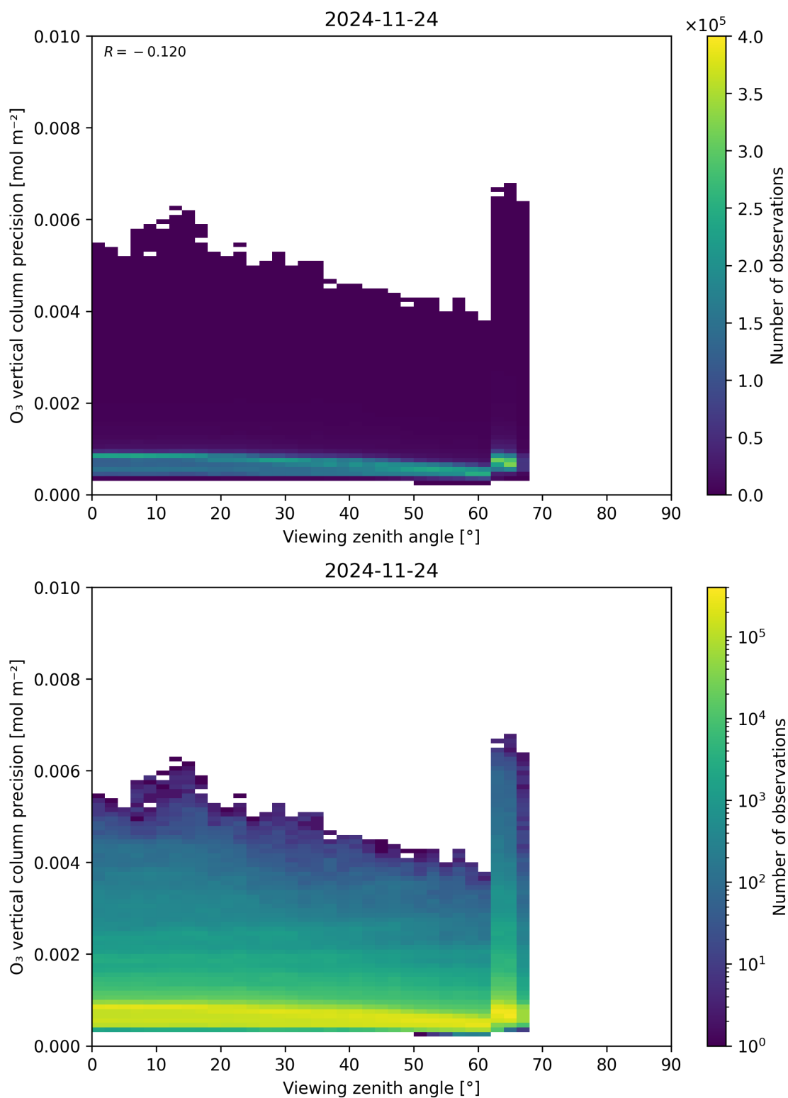
Figure 53: Scatter density plot of “Viewing zenith angle” against “O 3 vertical column precision” for 2024-11-23 to 2024-11-25.
