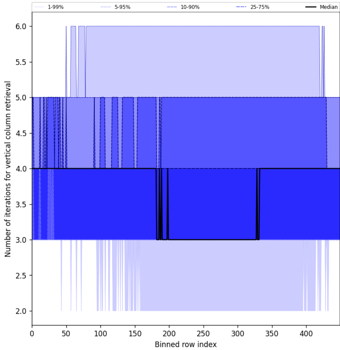
Figure 33: Along track statistics of “Number of iterations for vertical column retrieval” for 2024-11-23 to 2024-11-25
