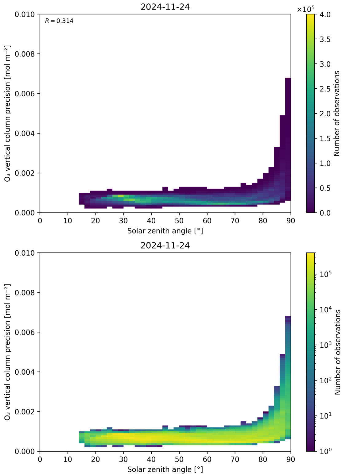
Figure 48: Scatter density plot of “Solar zenith angle” against “O 3 vertical column precision” for 2024-11-23 to 2024-11-25.
