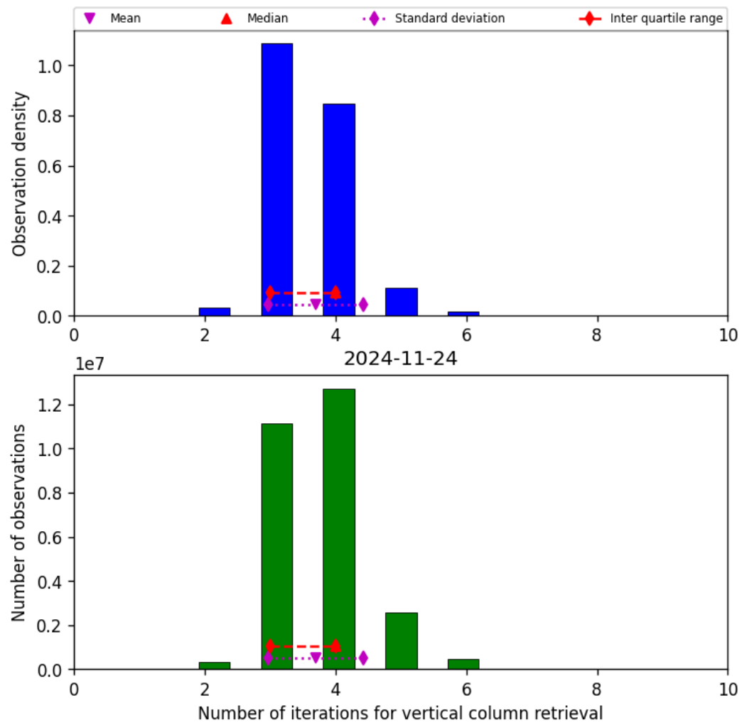
Figure 26: Histogram of “Number of iterations for vertical column retrieval” for 2024-11-23 to 2024-11-25
