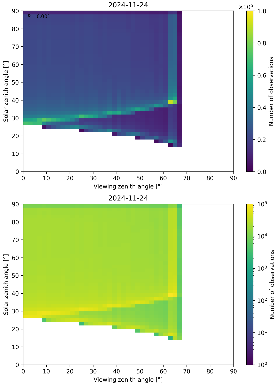
Figure 54: Scatter density plot of “Viewing zenith angle” against “Solar zenith angle” for 2024-11-23 to 2024-11-25.
