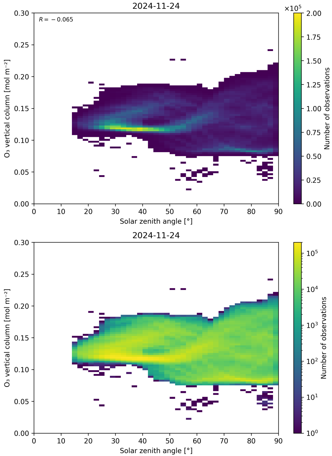
Figure 47: Scatter density plot of “Solar zenith angle” against “O 3 vertical column” for 2024-11-23 to 2024-11-25.
