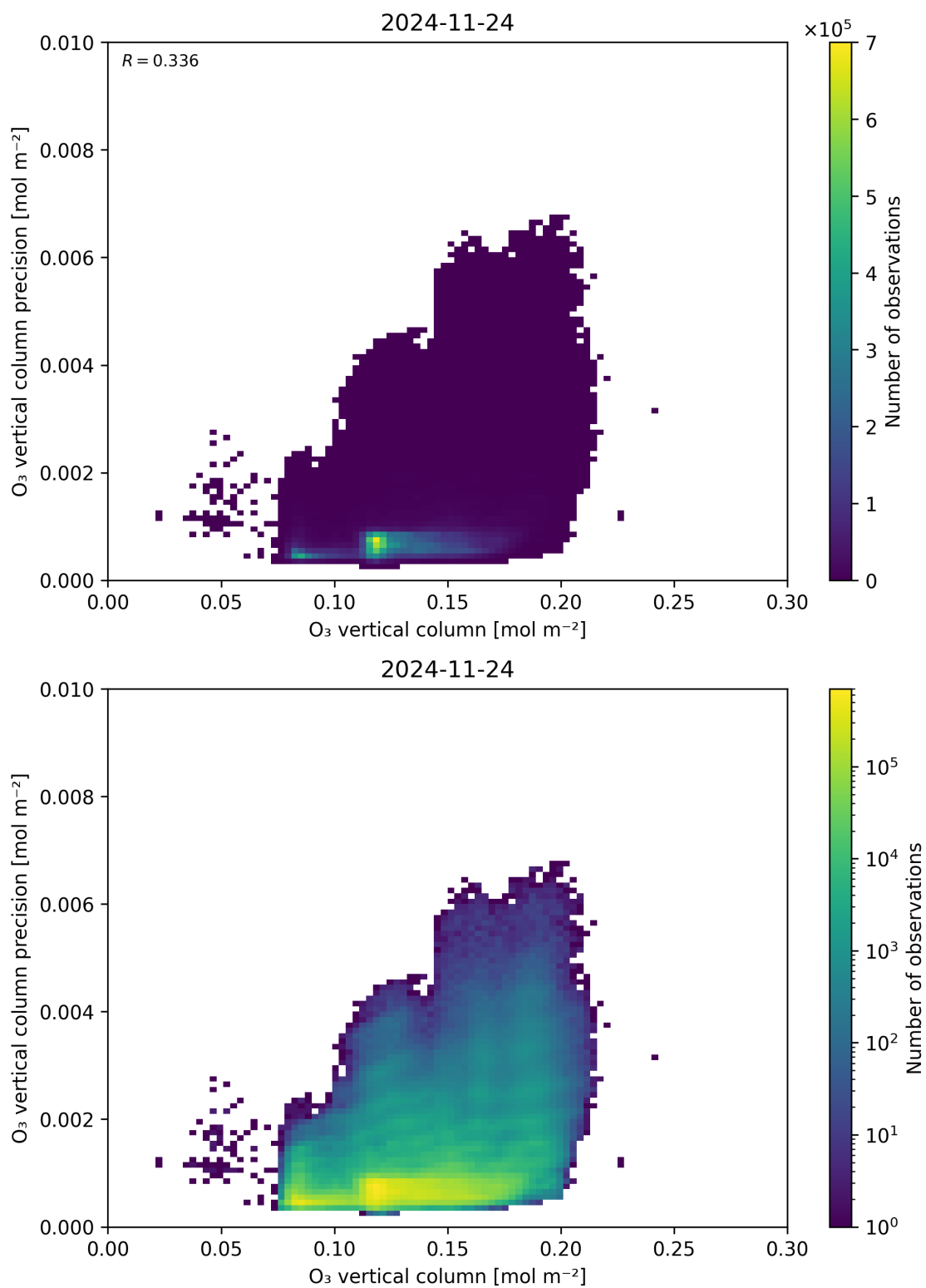
Figure 41: Scatter density plot of “O 3 vertical column” against “O 3 vertical column precision” for 2024-11-23 to 2024-11-25.
