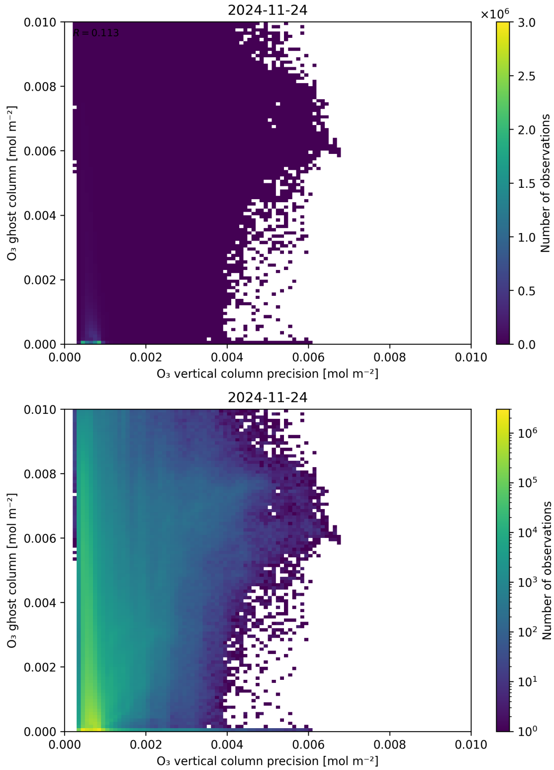
Figure 43: Scatter density plot of “O 3 vertical column precision” against “O 3 ghost column” for 2024-11-23 to 2024-11-25.
