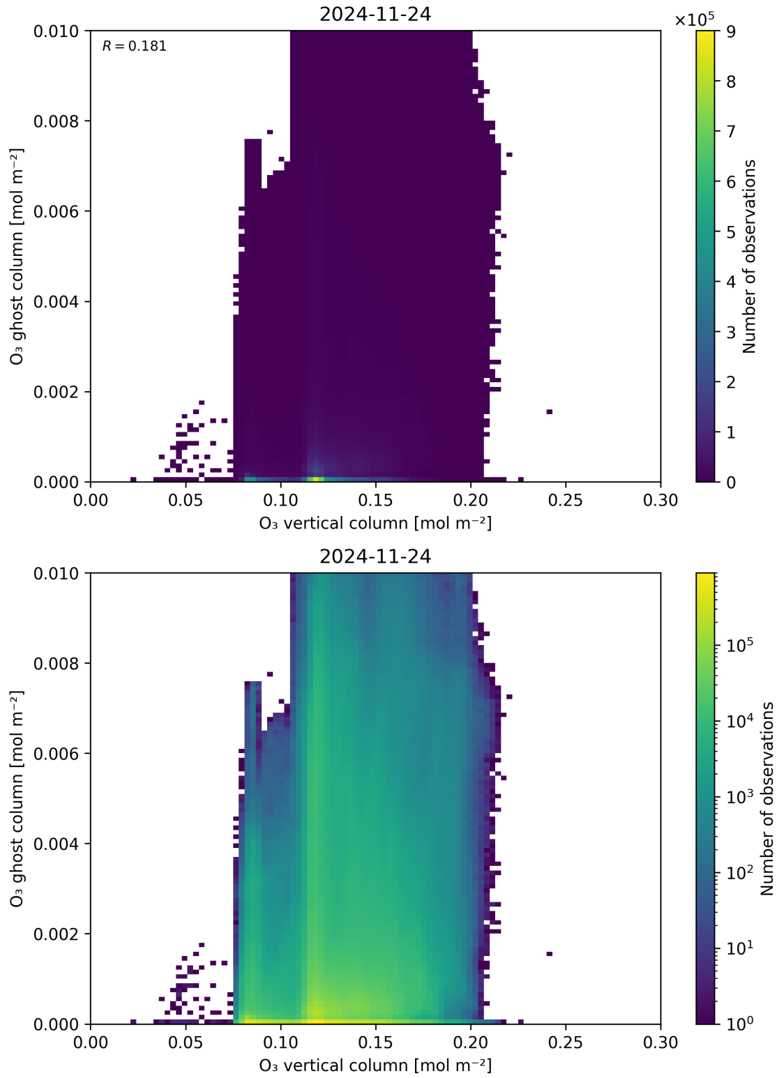
Figure 40: Scatter density plot of “O 3 vertical column” against “O 3 ghost column” for 2024-11-23 to 2024-11-25.
