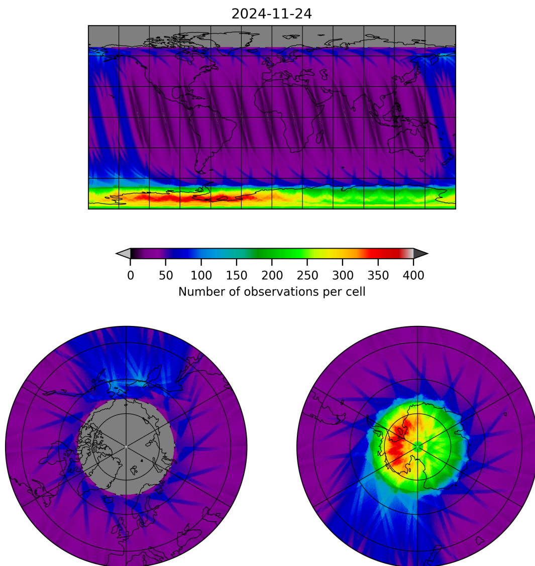
Figure 12: Map of the number of observations for 2024-11-23 to 2024-11-25
