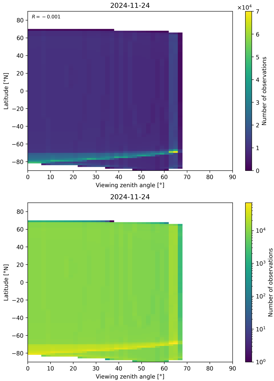
Figure 49: Scatter density plot of “Viewing zenith angle” against “Latitude” for 2024-11-23 to 2024-11-25.
