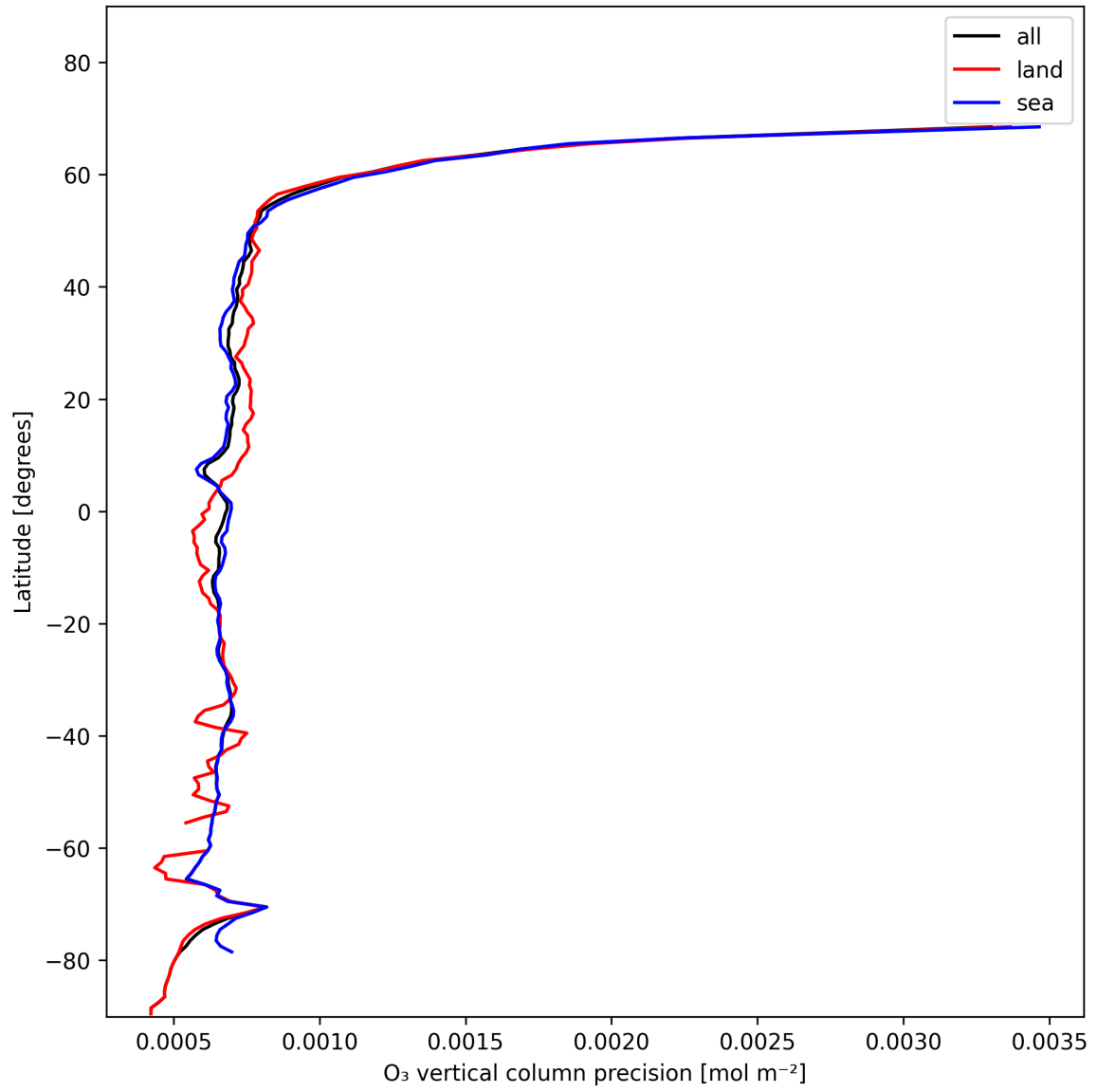
Figure 15: Zonal average of “O 3 vertical column precision” for 2024-11-23 to 2024-11-25.
