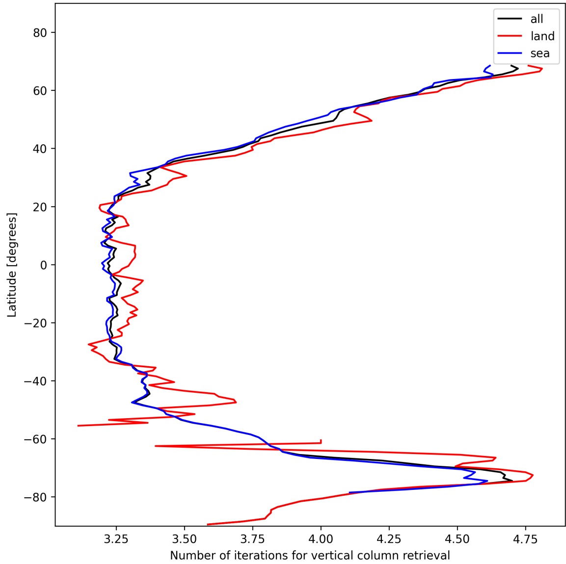
Figure 19: Zonal average of “Number of iterations for vertical column retrieval” for 2024-11-23 to 2024-11-25.
