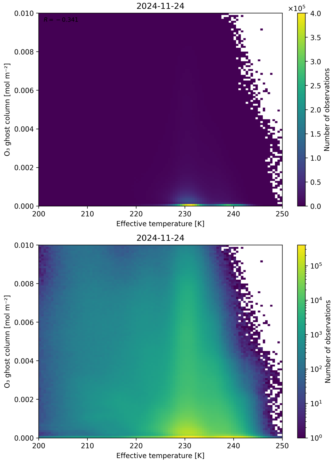
Figure 38: Scatter density plot of “Effective temperature” against “O 3 ghost column” for 2024-11-23 to 2024-11-25.
