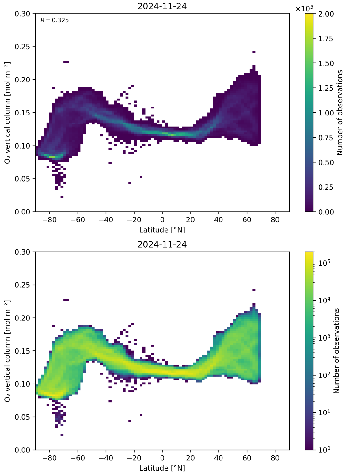
Figure 36: Scatter density plot of “Latitude” against “O 3 vertical column” for 2024-11-23 to 2024-11-25.
