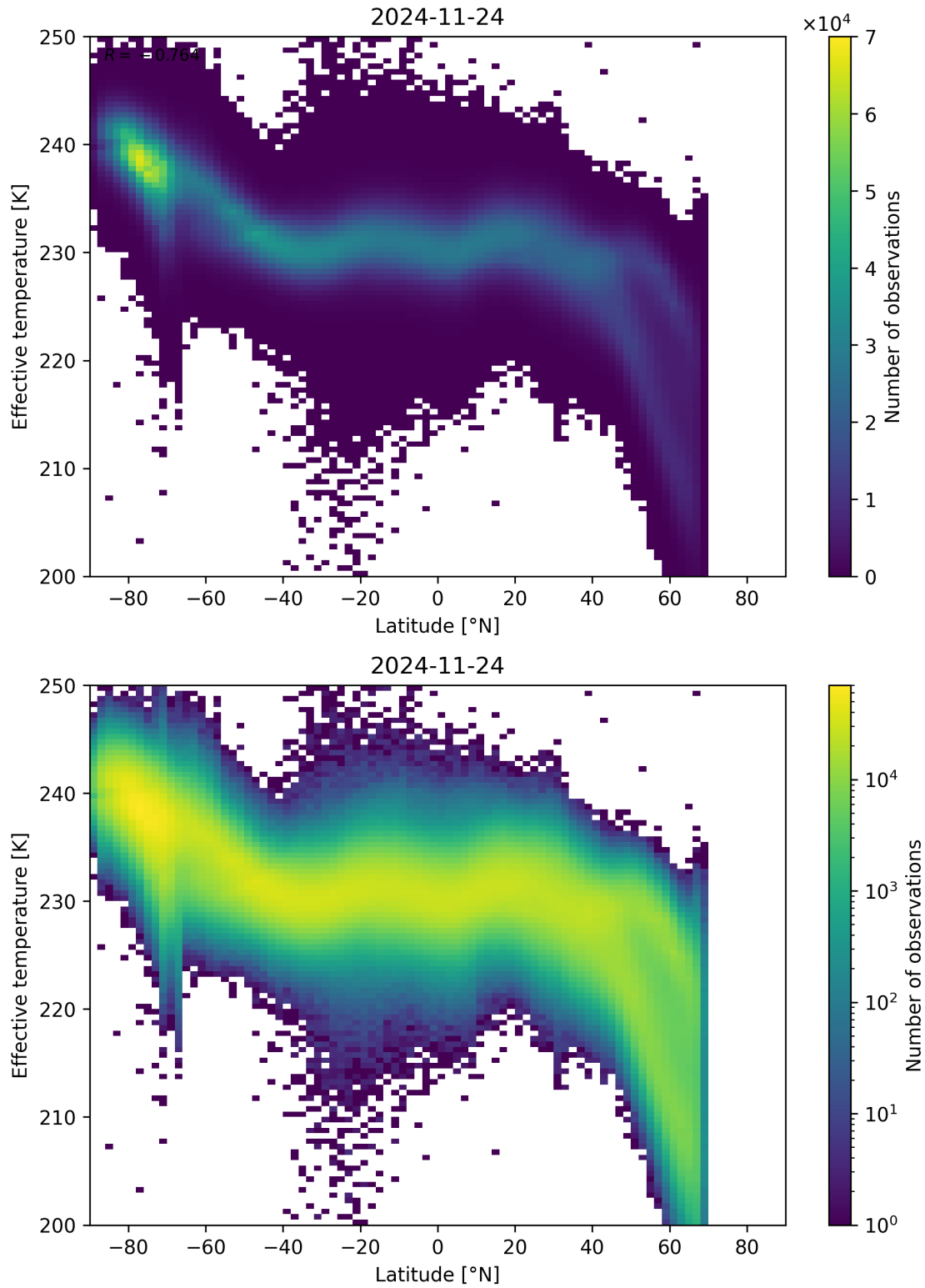
Figure 34: Scatter density plot of “Latitude” against “Effective temperature” for 2024-11-23 to 2024-11-25.
