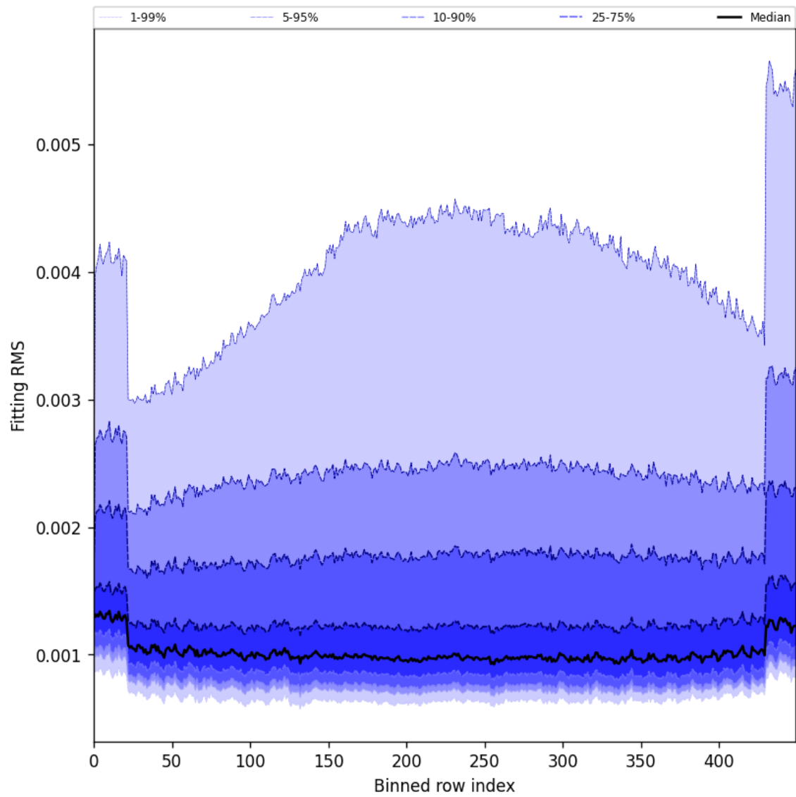
Figure 30: Along track statistics of “Fitting RMS” for 2024-11-23 to 2024-11-25
