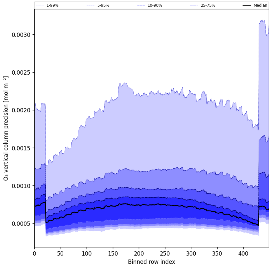
Figure 29: Along track statistics of “O 3 vertical column precision” for 2024-11-23 to 2024-11-25
