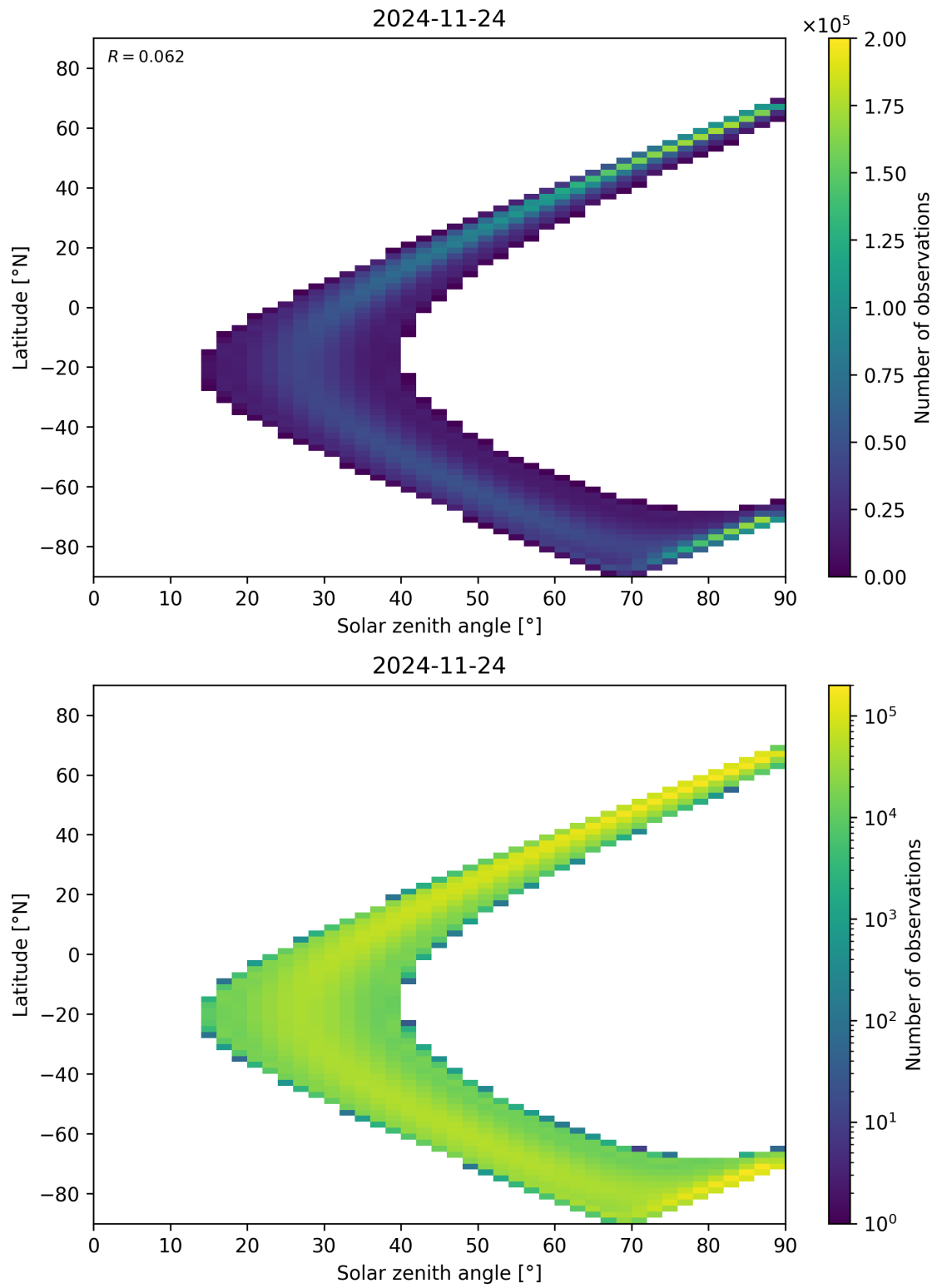
Figure 44: Scatter density plot of “Solar zenith angle” against “Latitude” for 2024-11-23 to 2024-11-25.
