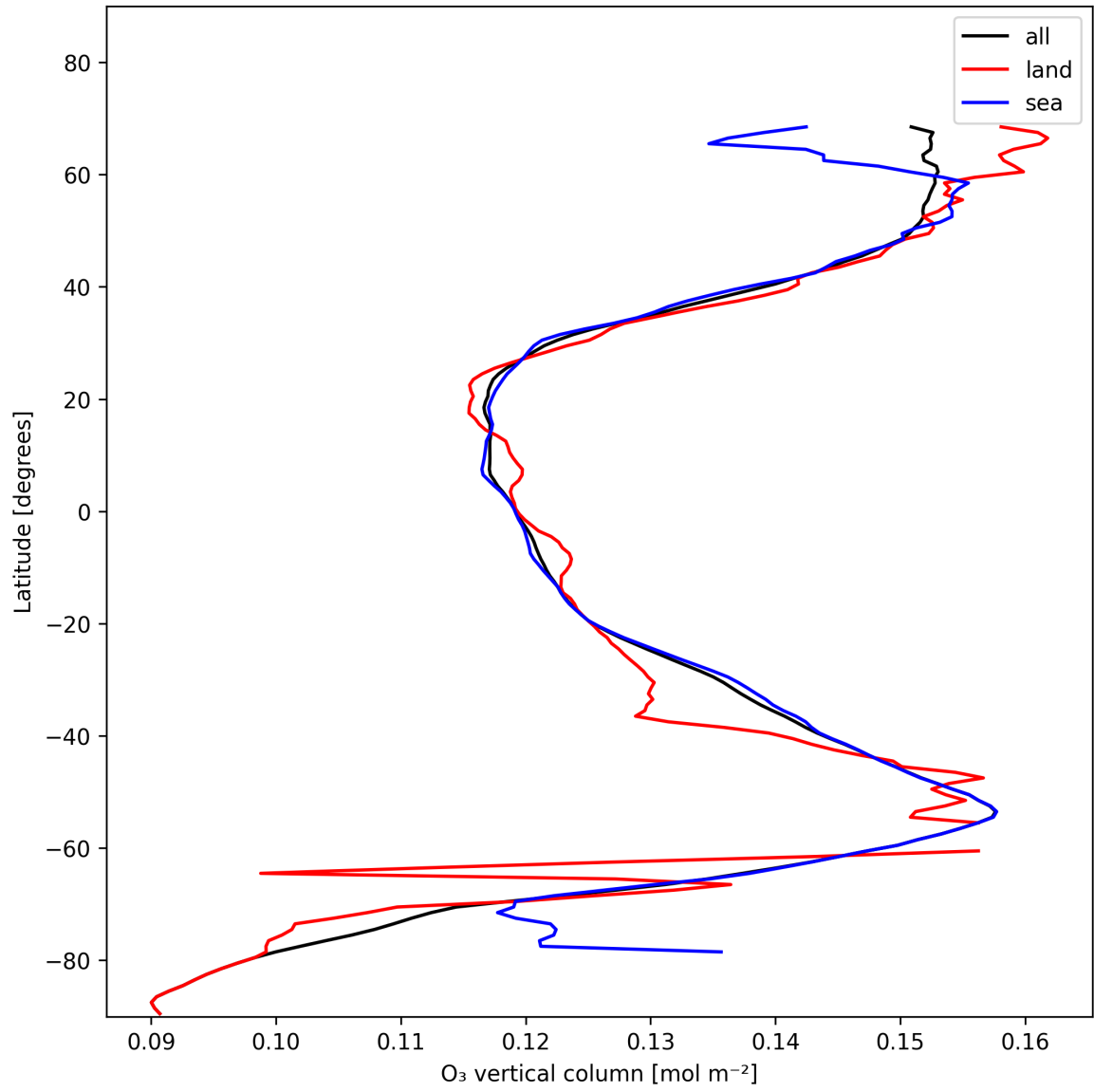
Figure 14: Zonal average of “O 3 vertical column” for 2024-11-23 to 2024-11-25.
