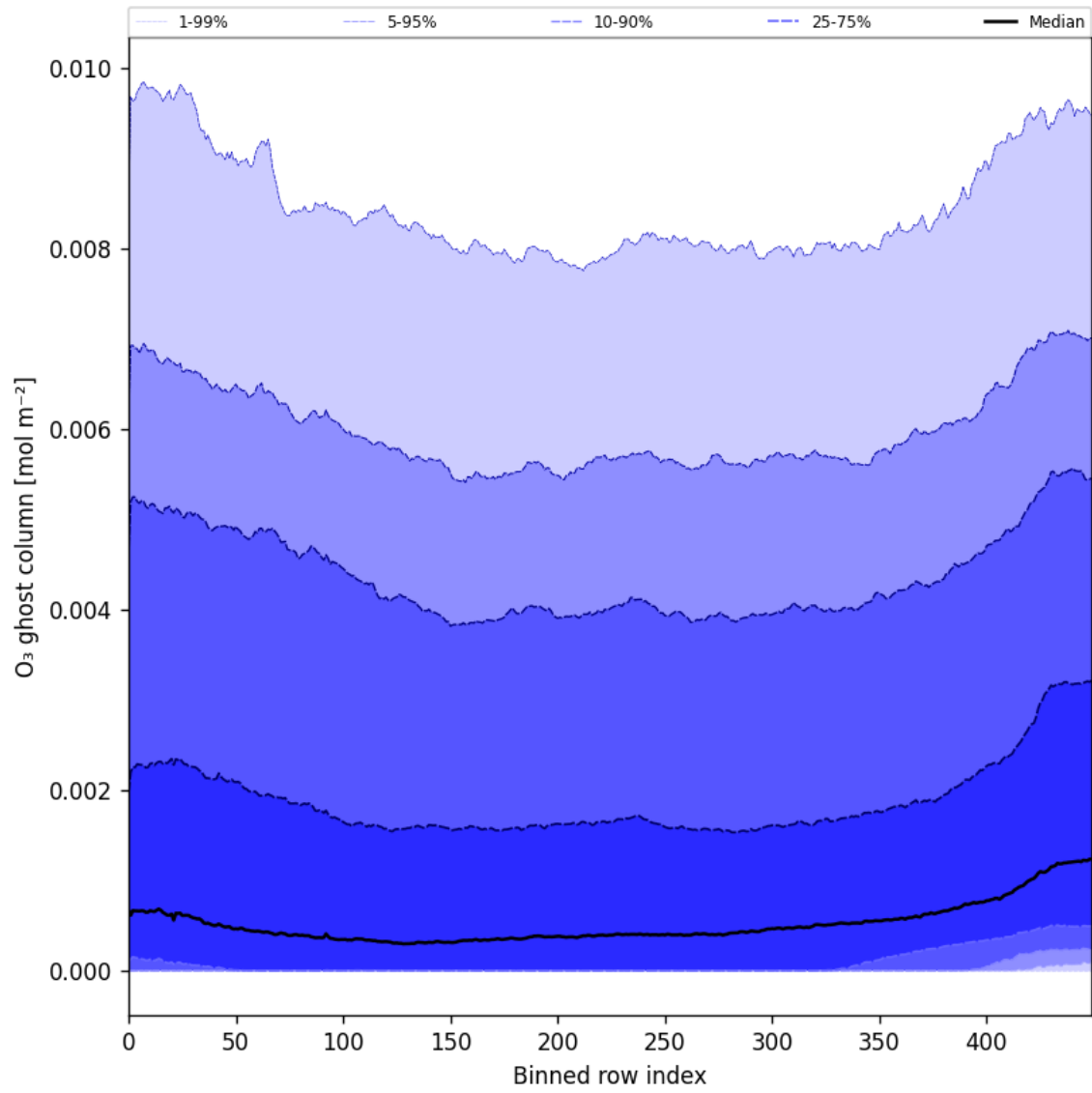
Figure 32: Along track statistics of “O 3 ghost column” for 2024-11-23 to 2024-11-25
