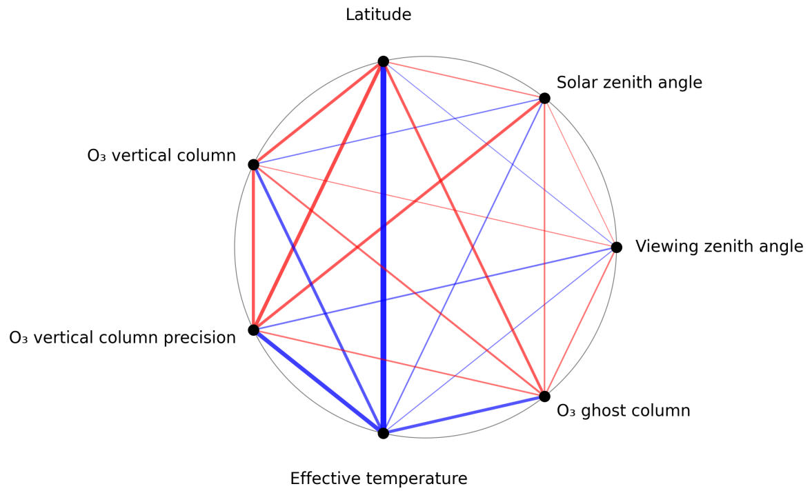
Figure 1: Map of correlation graph for 2024-11-23 to 2024-11-25.
