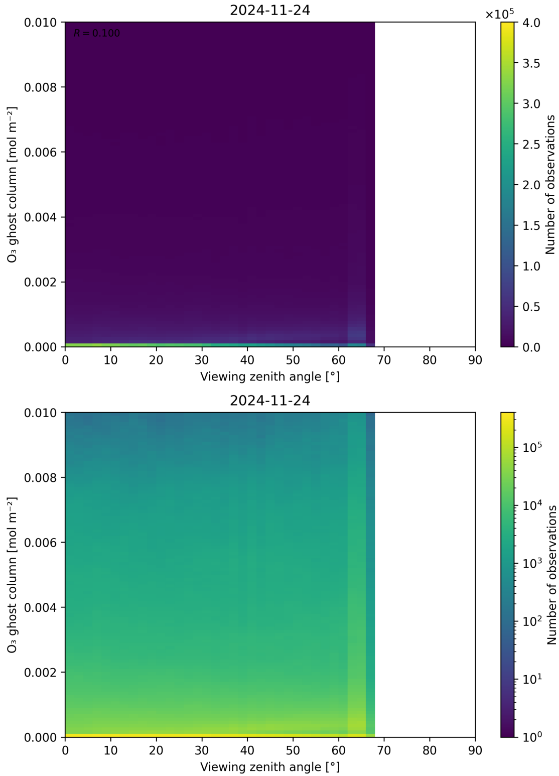
Figure 51: Scatter density plot of “Viewing zenith angle” against “O 3 ghost column” for 2024-11-23 to 2024-11-25.
