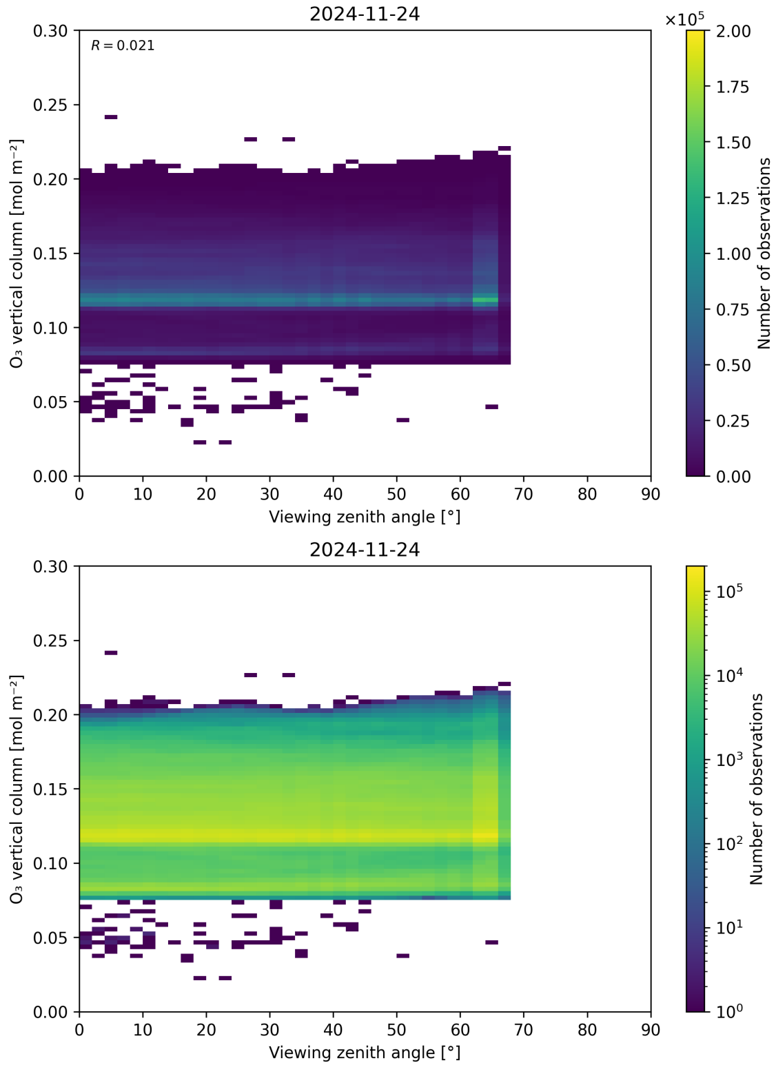
Figure 52: Scatter density plot of “Viewing zenith angle” against “O 3 vertical column” for 2024-11-23 to 2024-11-25.
