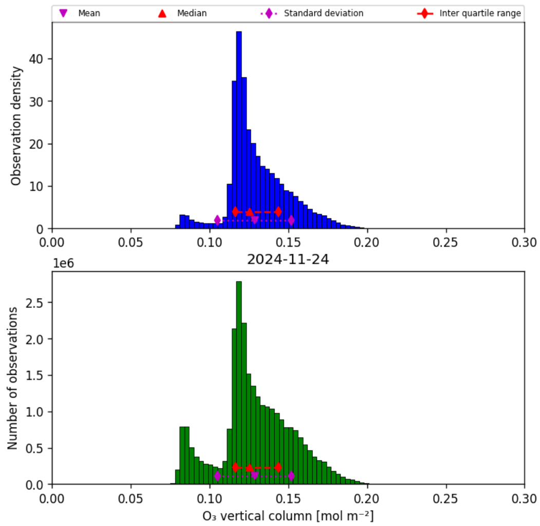
Figure 21: Histogram of “O 3 vertical column” for 2024-11-23 to 2024-11-25
