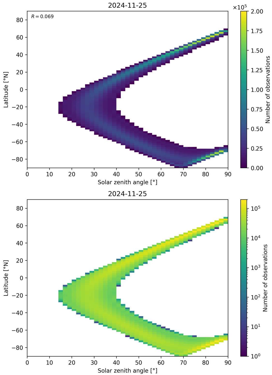
Figure 44: Scatter density plot of “Solar zenith angle” against “Latitude” for 2024-11-25 to 2024-11-26.
