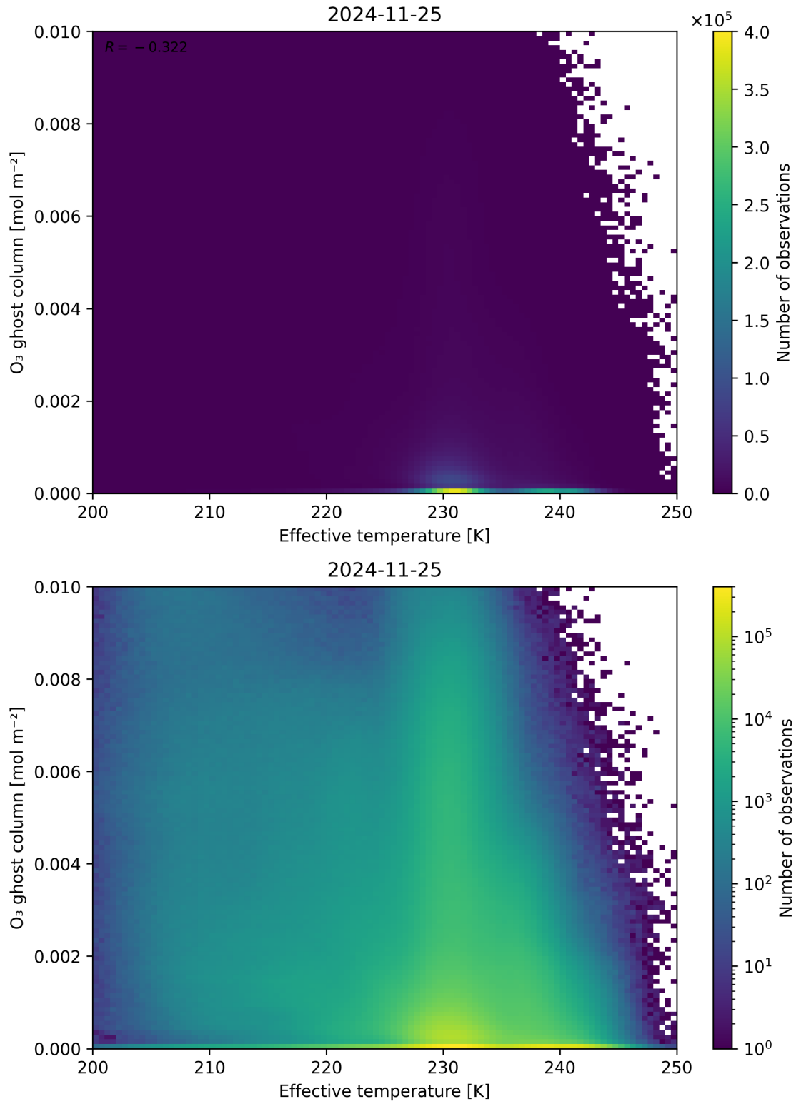
Figure 38: Scatter density plot of “Effective temperature” against “O 3 ghost column” for 2024-11-25 to 2024-11-26.
