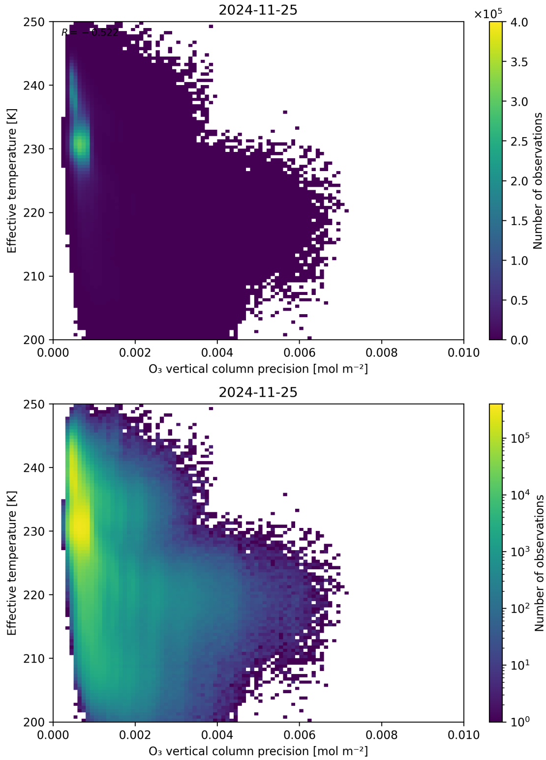
Figure 42: Scatter density plot of “O 3 vertical column precision” against “Effective temperature” for 2024-11-25 to 2024-11-26.
