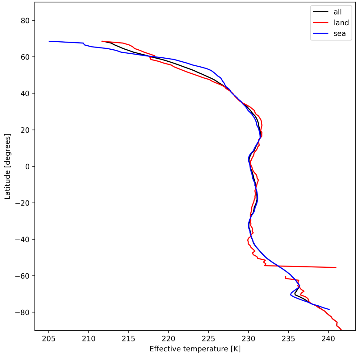
Figure 17: Zonal average of “Effective temperature” for 2024-11-25 to 2024-11-26.
