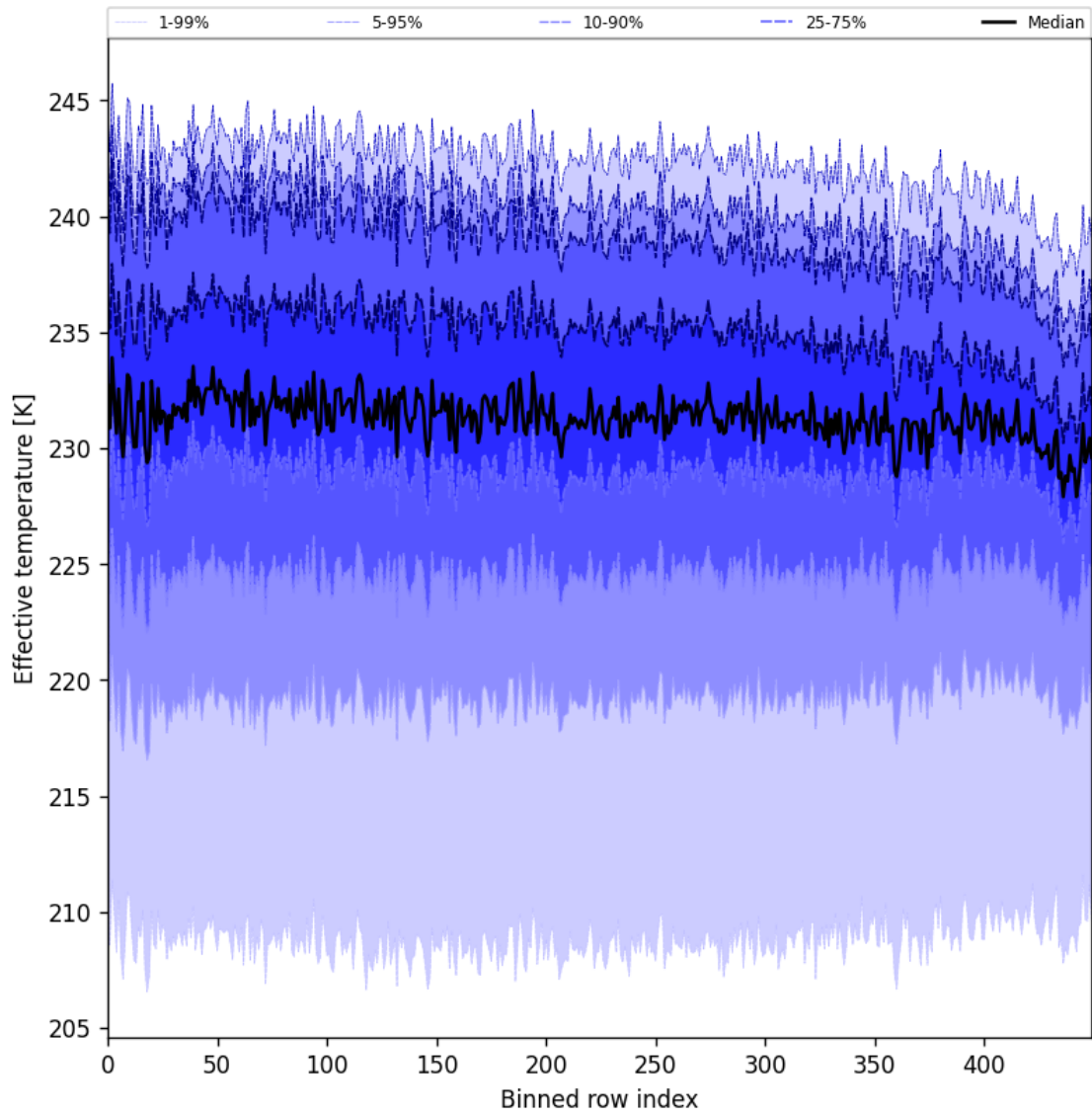
Figure 31: Along track statistics of “Effective temperature” for 2024-11-25 to 2024-11-26
