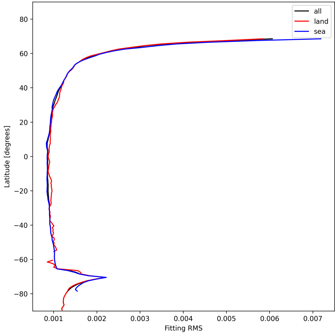
Figure 16: Zonal average of “Fitting RMS” for 2024-11-25 to 2024-11-26.
