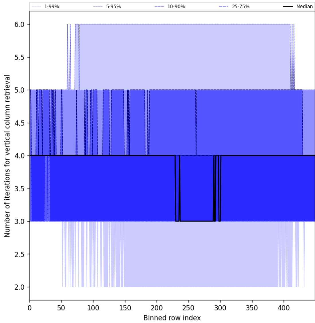
Figure 33: Along track statistics of “Number of iterations for vertical column retrieval” for 2024-11-25 to 2024-11-26
