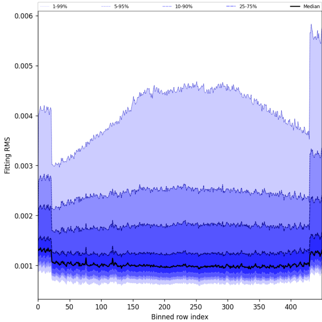
Figure 30: Along track statistics of “Fitting RMS” for 2024-11-25 to 2024-11-26
