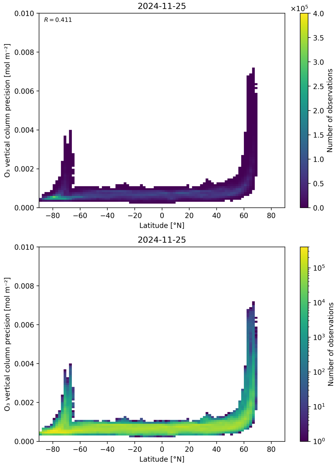
Figure 37: Scatter density plot of “Latitude” against “O 3 vertical column precision” for 2024-11-25 to 2024-11-26.
