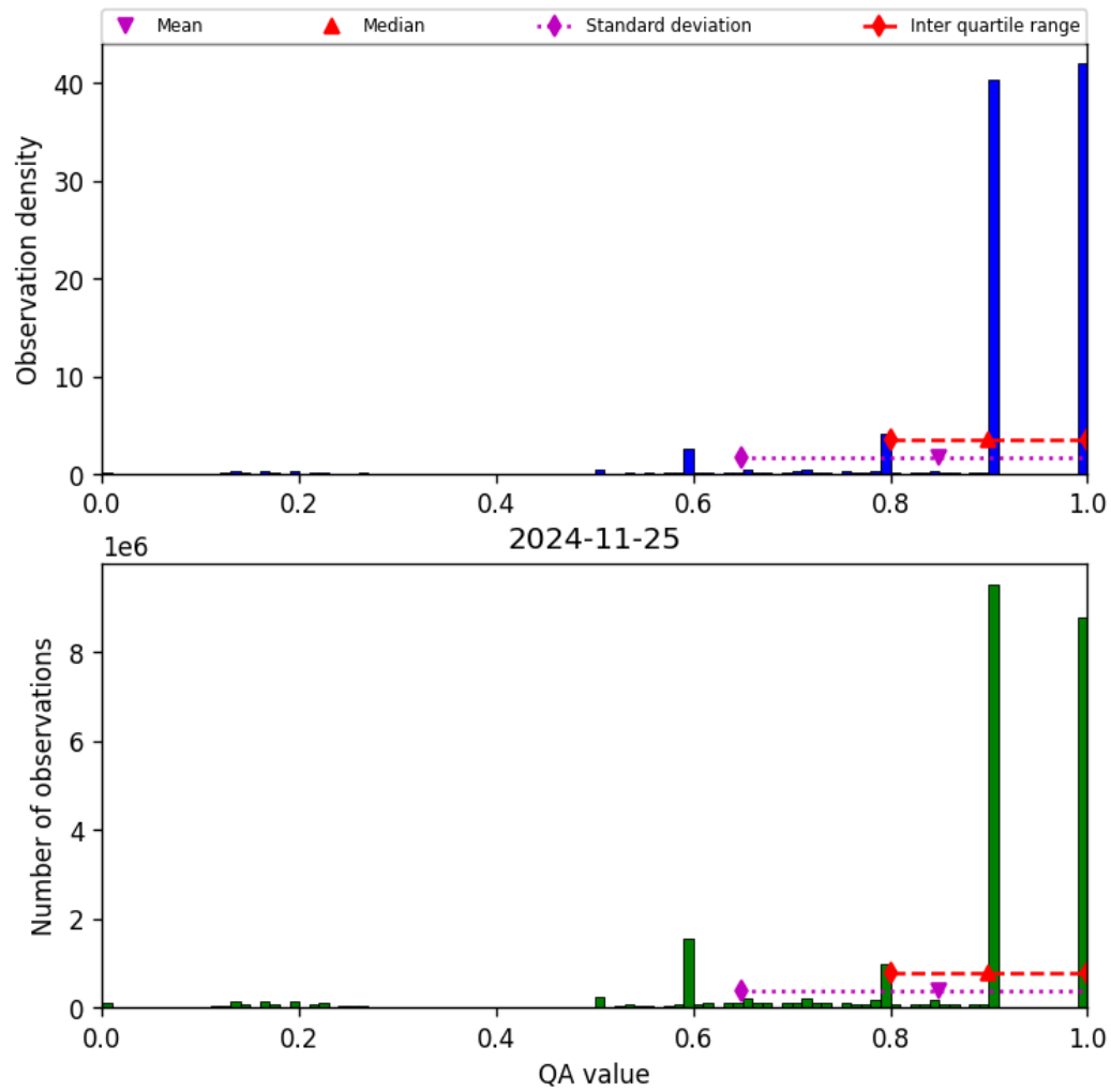
Figure 20: Histogram of “QA value” for 2024-11-25 to 2024-11-26
