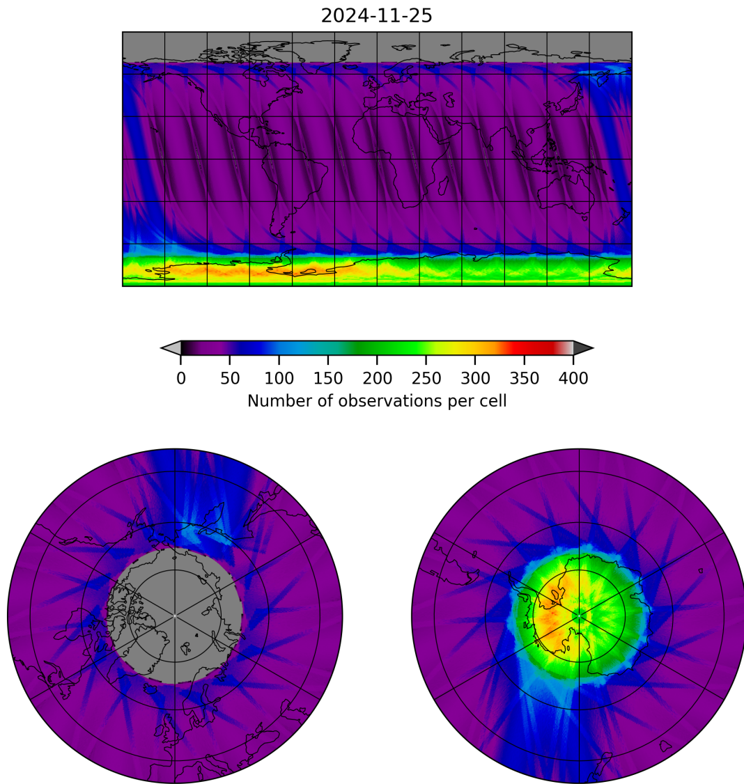
Figure 12: Map of the number of observations for 2024-11-25 to 2024-11-26
