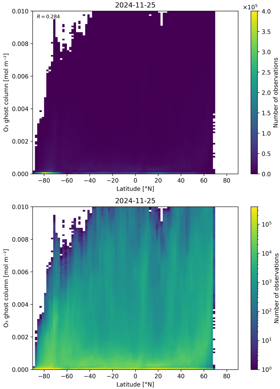
Figure 35: Scatter density plot of “Latitude” against “O 3 ghost column” for 2024-11-25 to 2024-11-26.
