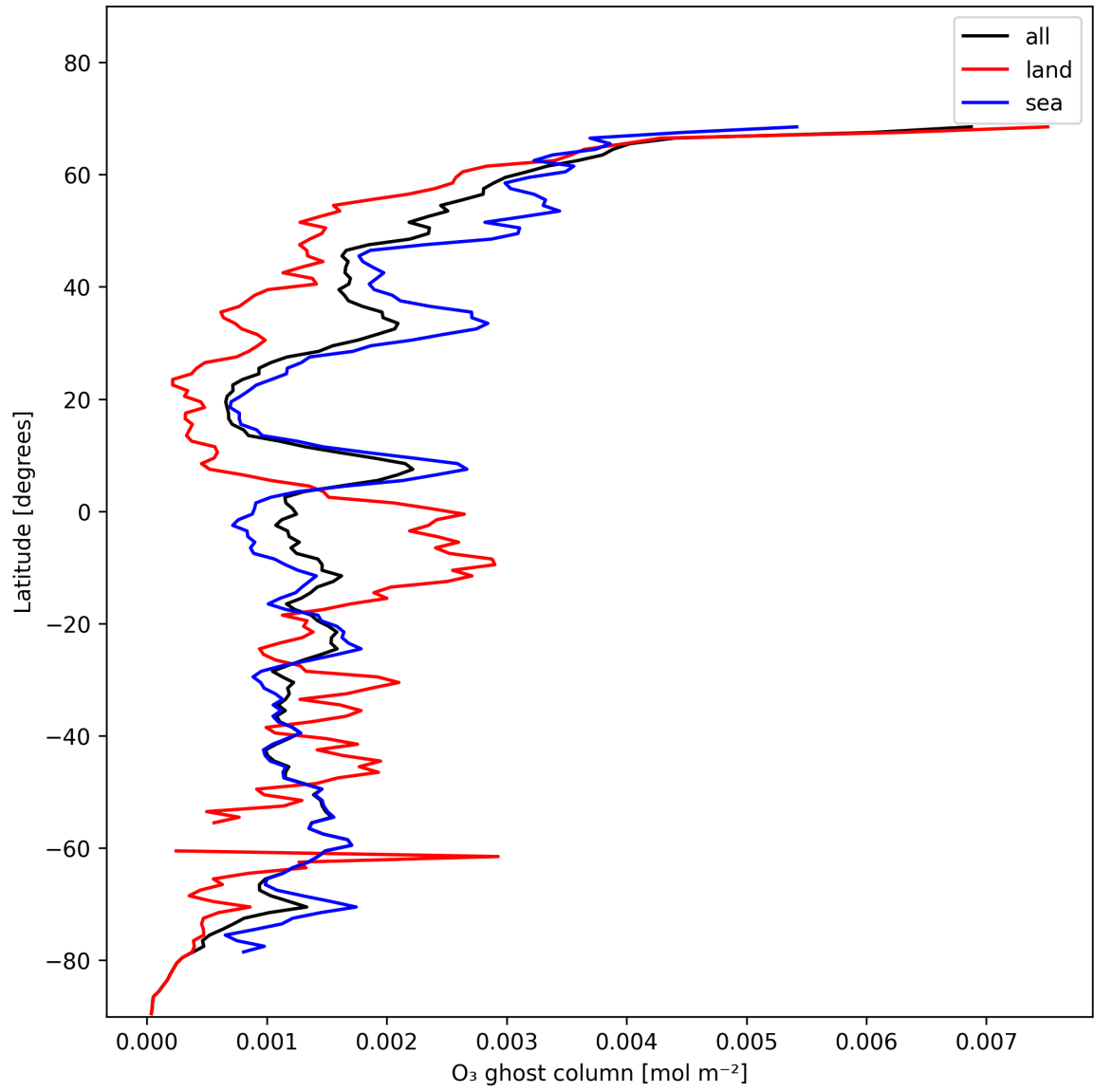
Figure 18: Zonal average of "O 3 ghost column" for 2024-11-25 to 2024-11-26.
