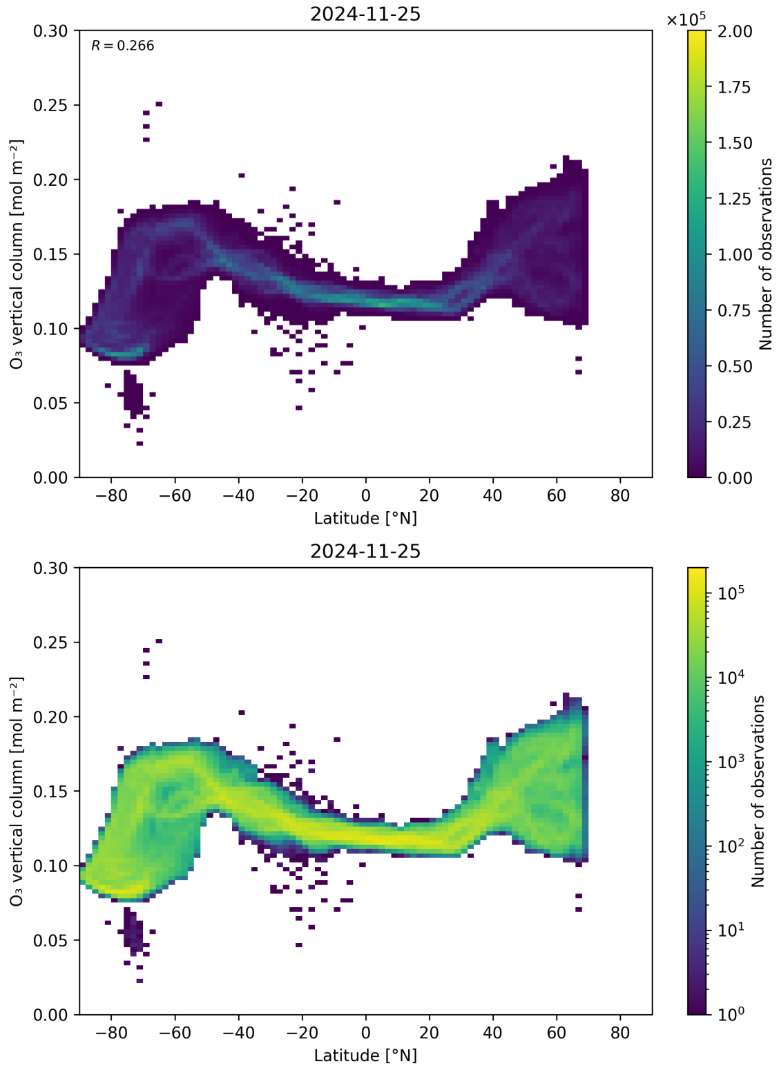
Figure 36: Scatter density plot of “Latitude” against “O 3 vertical column” for 2024-11-25 to 2024-11-26.
