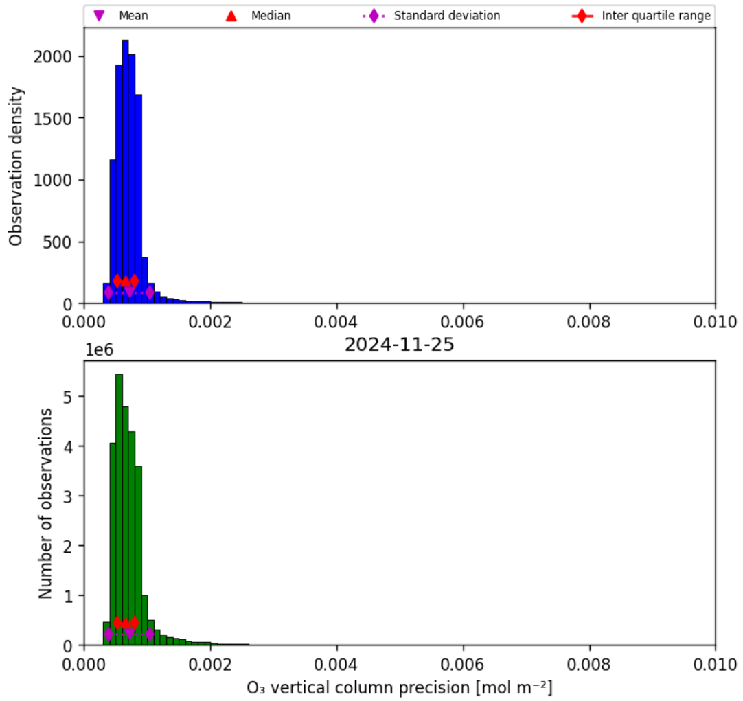
Figure 22: Histogram of “O 3 vertical column precision” for 2024-11-25 to 2024-11-26
