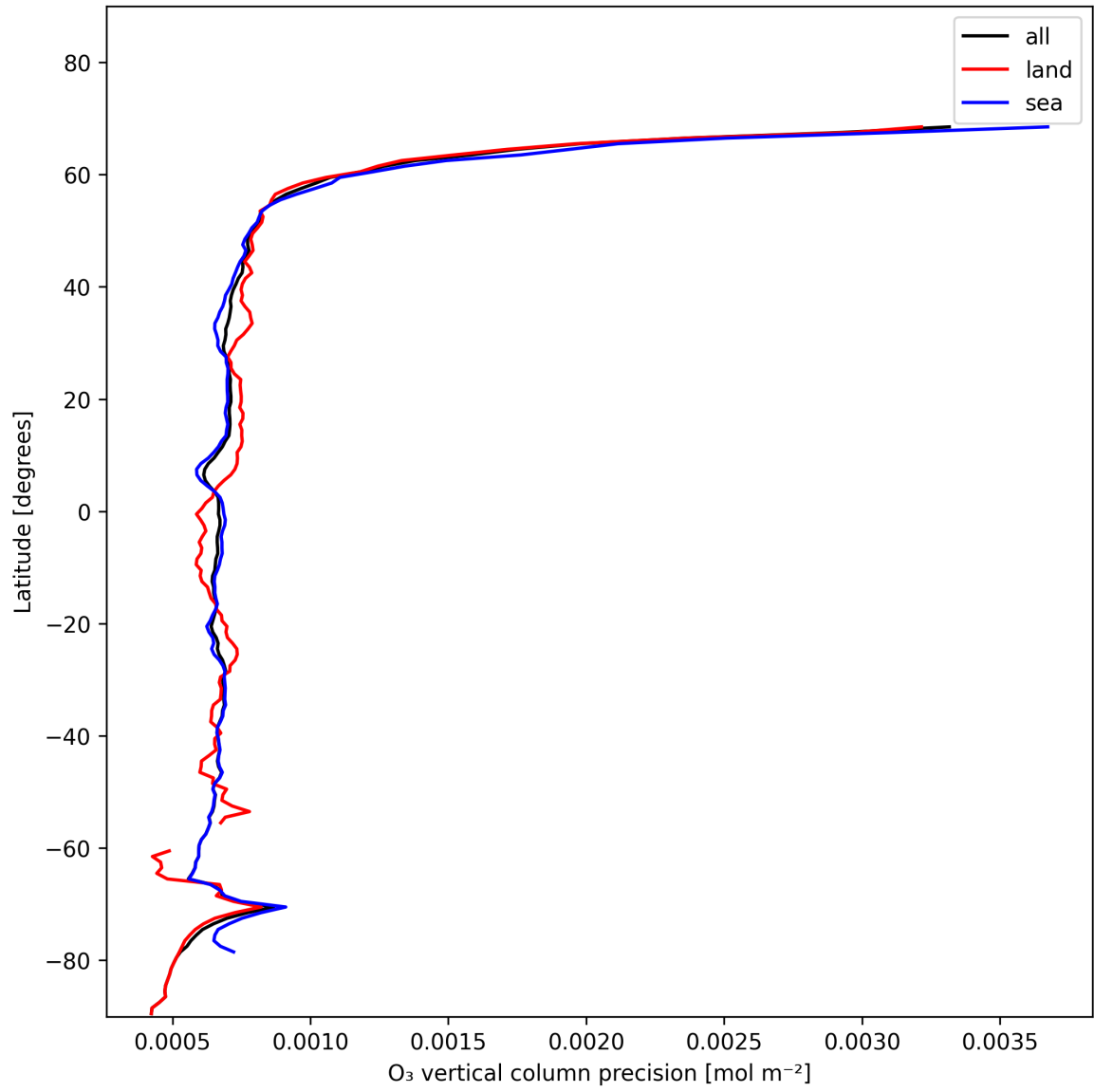
Figure 15: Zonal average of “O 3 vertical column precision” for 2024-11-25 to 2024-11-26.
