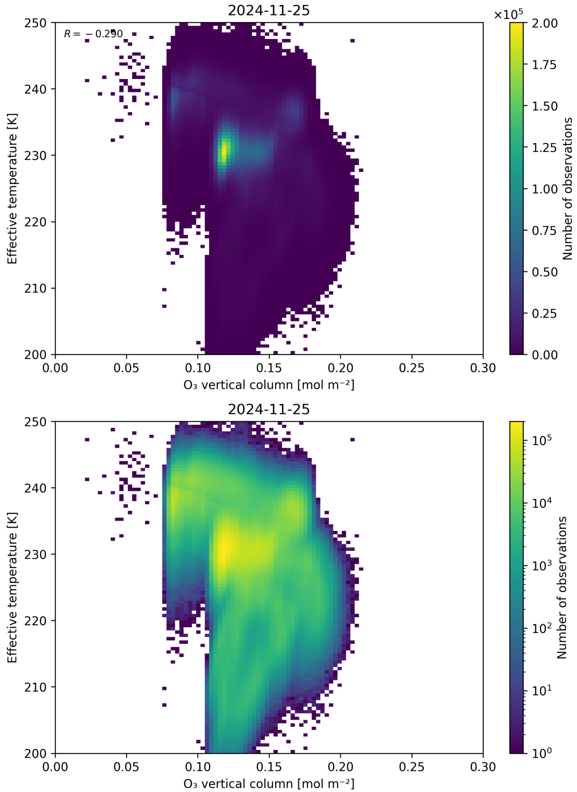
Figure 39: Scatter density plot of “O 3 vertical column” against “Effective temperature” for 2024-11-25 to 2024-11-26.
