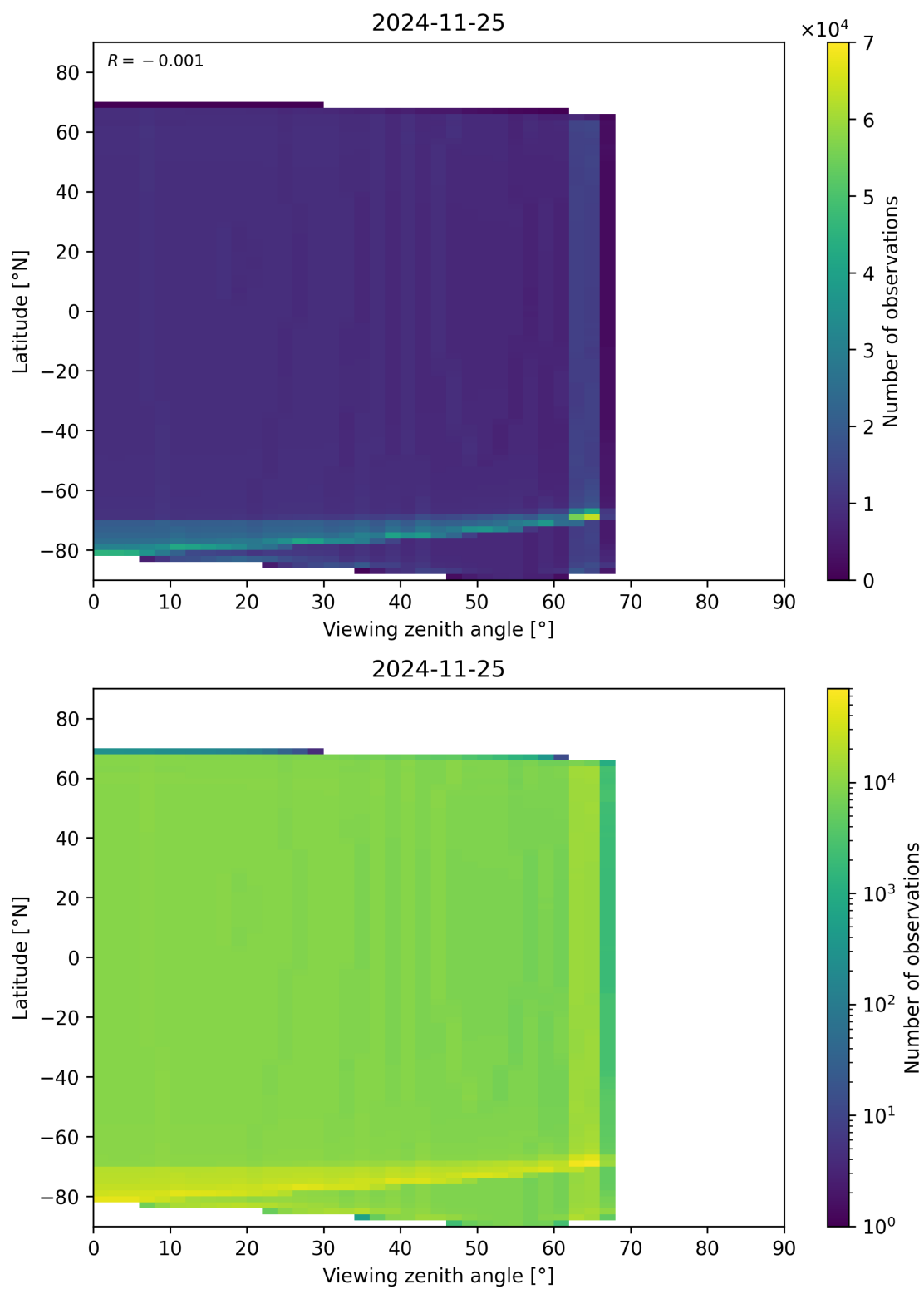
Figure 49: Scatter density plot of “Viewing zenith angle” against “Latitude” for 2024-11-25 to 2024-11-26.
