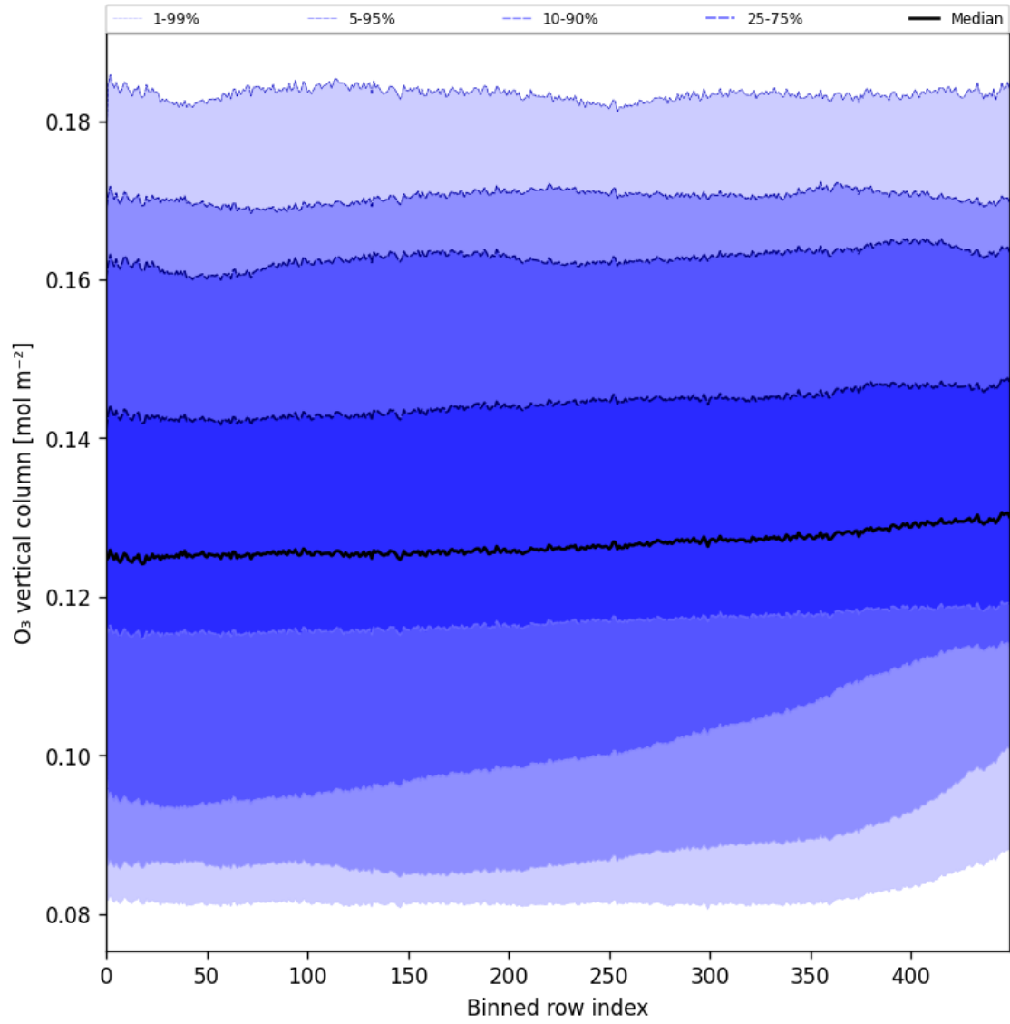
Figure 28: Along track statistics of “O 3 vertical column” for 2024-11-25 to 2024-11-26
