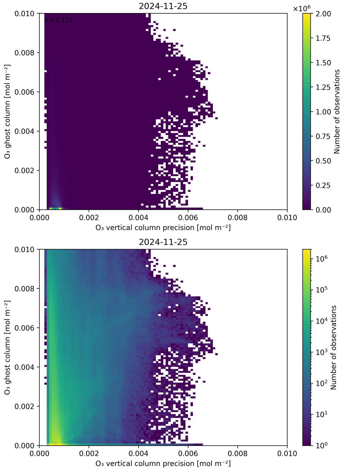
Figure 43: Scatter density plot of “ \text{O}_3 vertical column precision” against “ \text{O}_3 ghost column” for 2024-11-25 to 2024-11-26.
