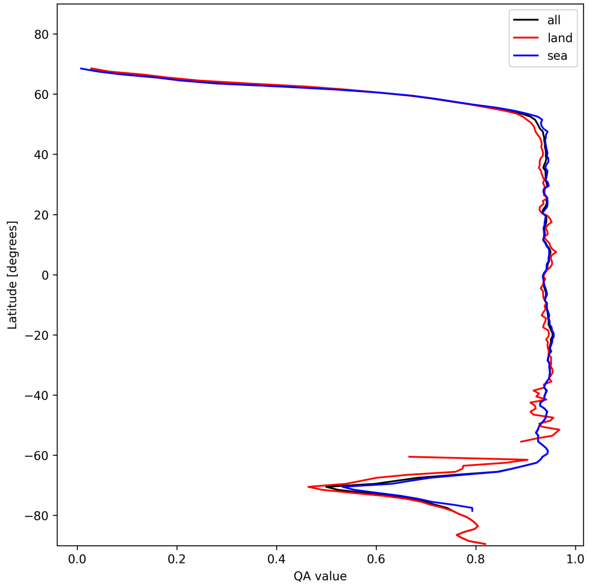
Figure 13: Zonal average of “QA value” for 2024-11-25 to 2024-11-26.
