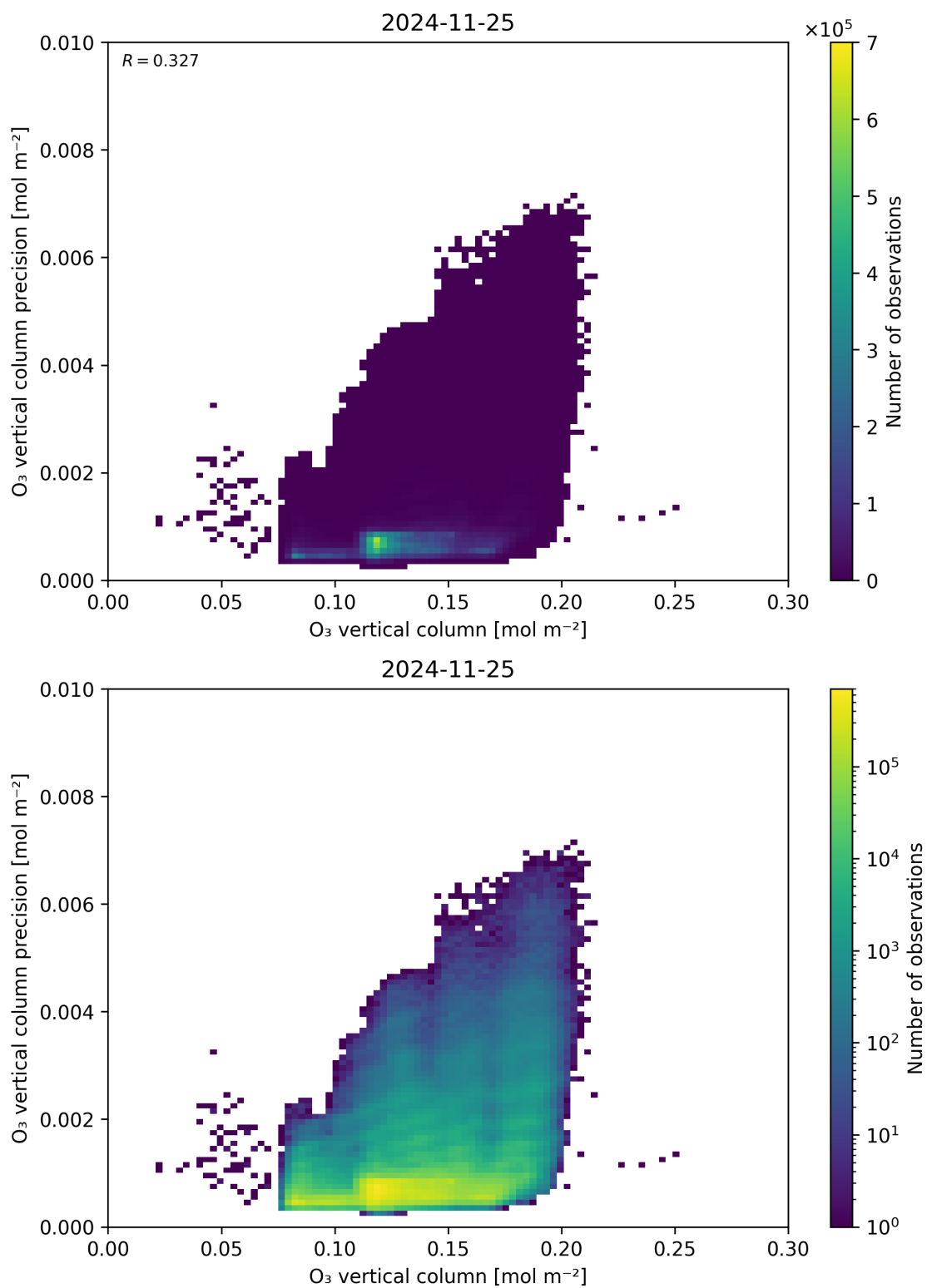
Figure 41: Scatter density plot of “O 3 vertical column” against “O 3 vertical column precision” for 2024-11-25 to 2024-11-26.
