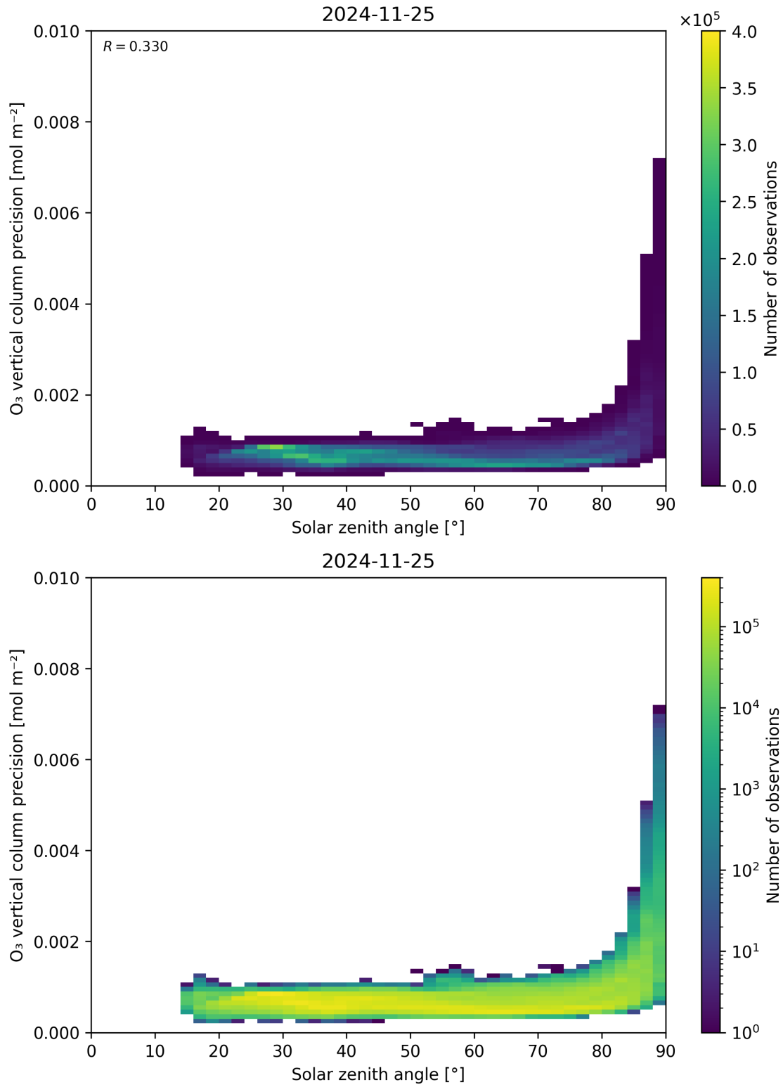
Figure 48: Scatter density plot of “Solar zenith angle” against “O 3 vertical column precision” for 2024-11-25 to 2024-11-26.
