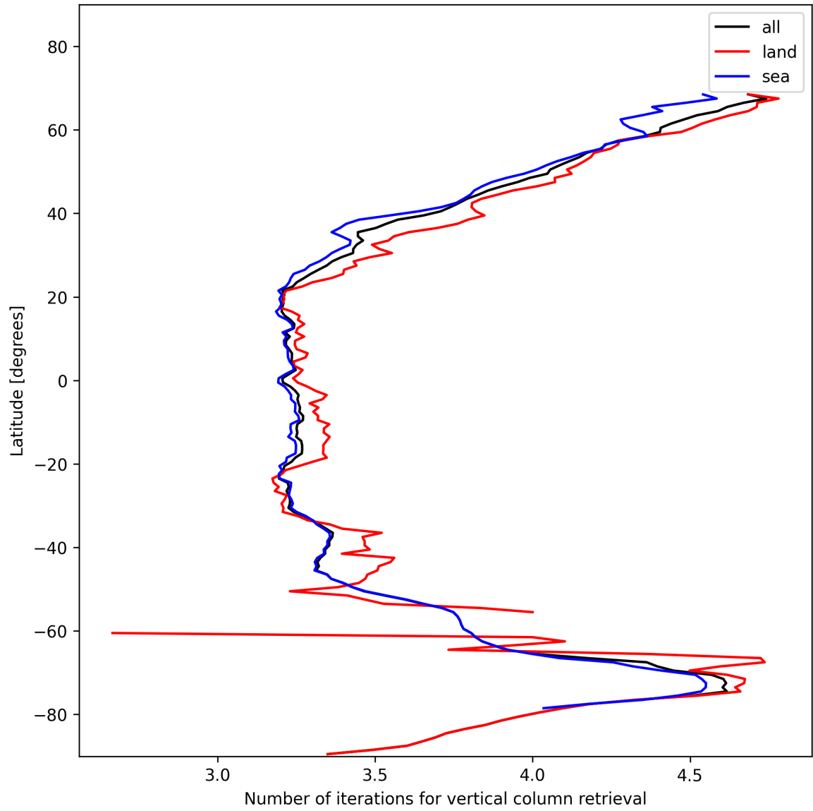
Figure 19: Zonal average of “Number of iterations for vertical column retrieval” for 2024-11-25 to 2024-11-26.
