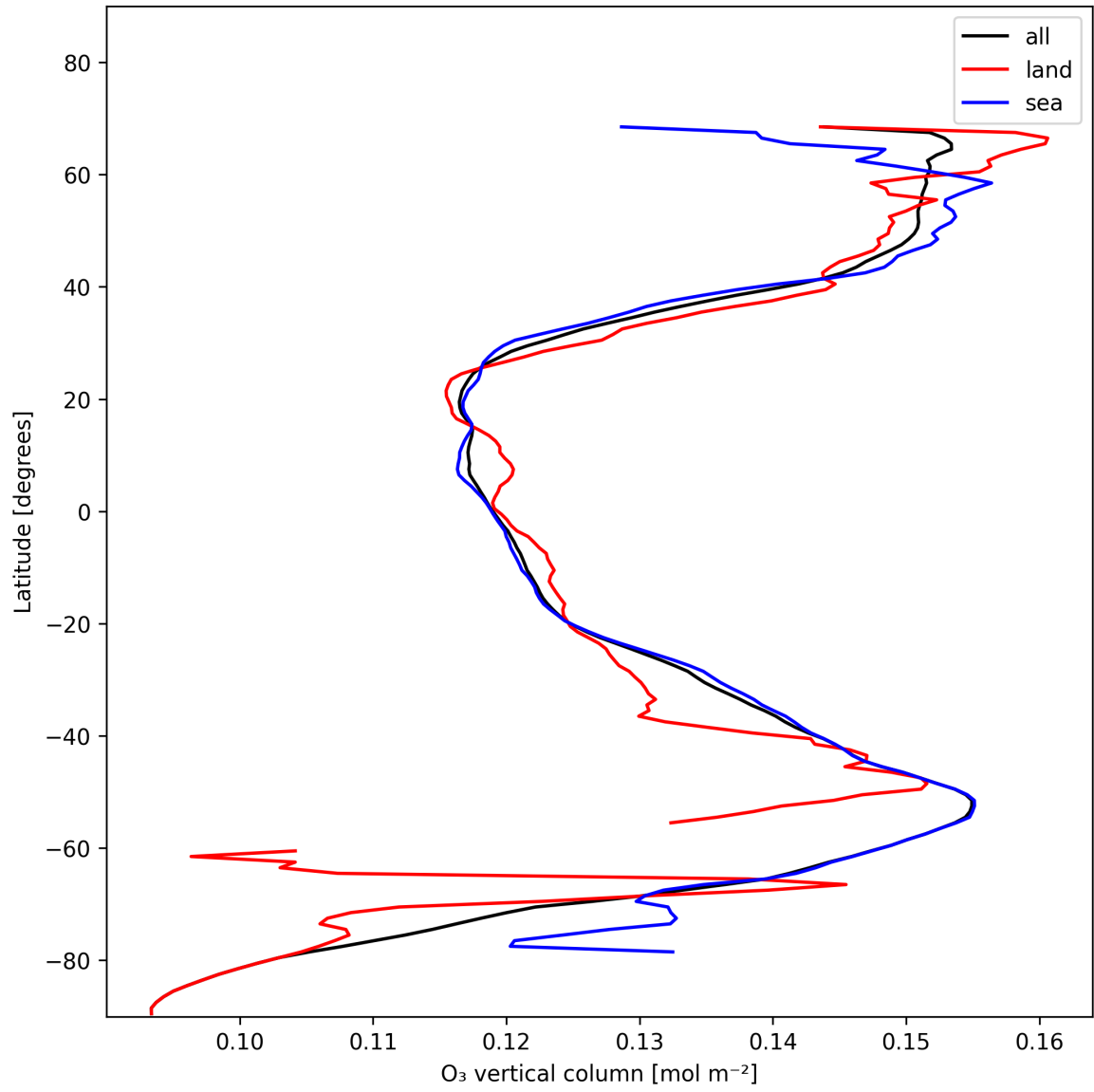
Figure 14: Zonal average of “O 3 vertical column” for 2024-11-25 to 2024-11-26.
