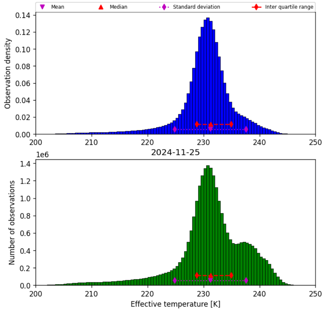
Figure 24: Histogram of “Effective temperature” for 2024-11-25 to 2024-11-26
