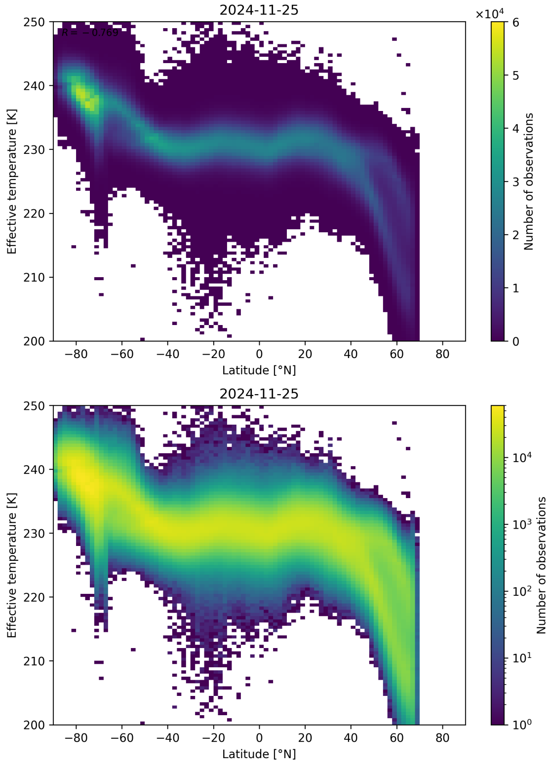
Figure 34: Scatter density plot of “Latitude” against “Effective temperature” for 2024-11-25 to 2024-11-26.
