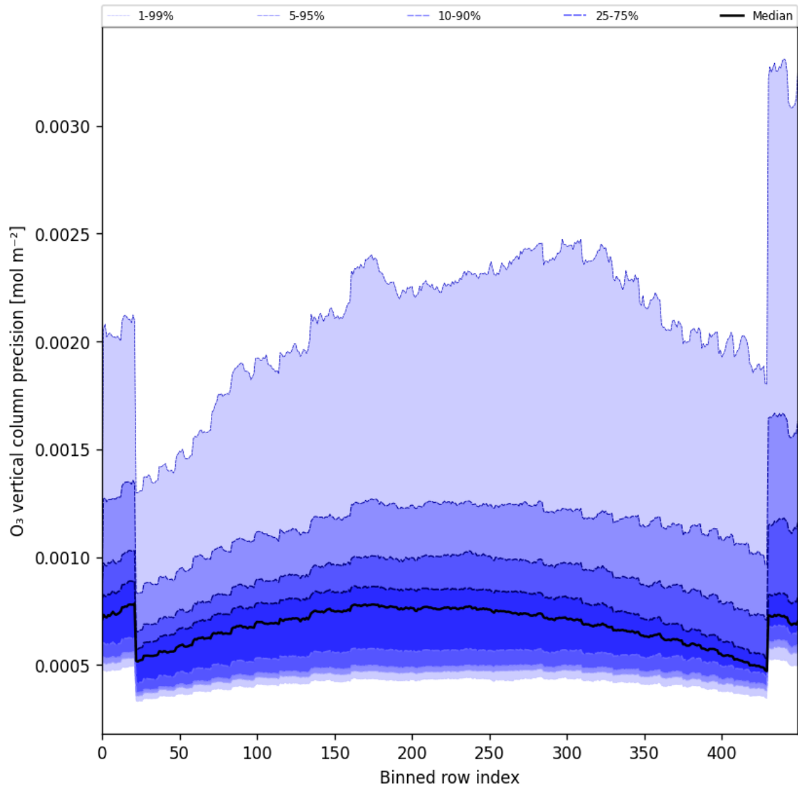
Figure 29: Along track statistics of “O 3 vertical column precision” for 2024-11-25 to 2024-11-26
