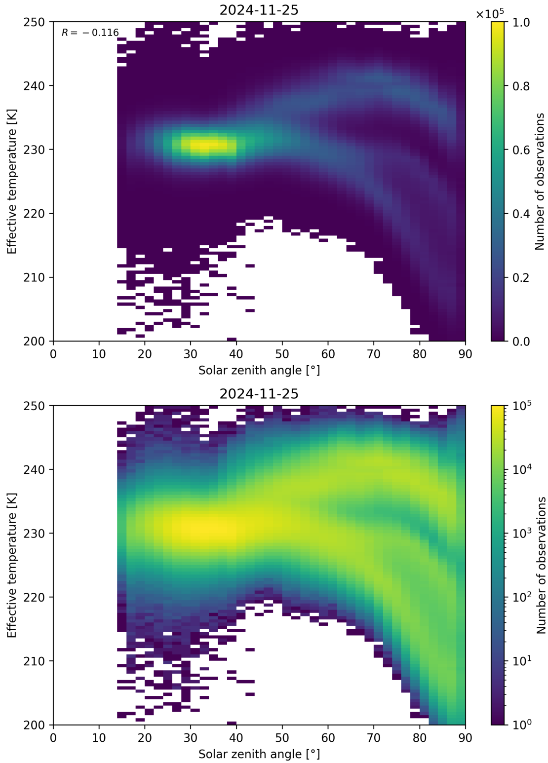
Figure 45: Scatter density plot of “Solar zenith angle” against “Effective temperature” for 2024-11-25 to 2024-11-26.
