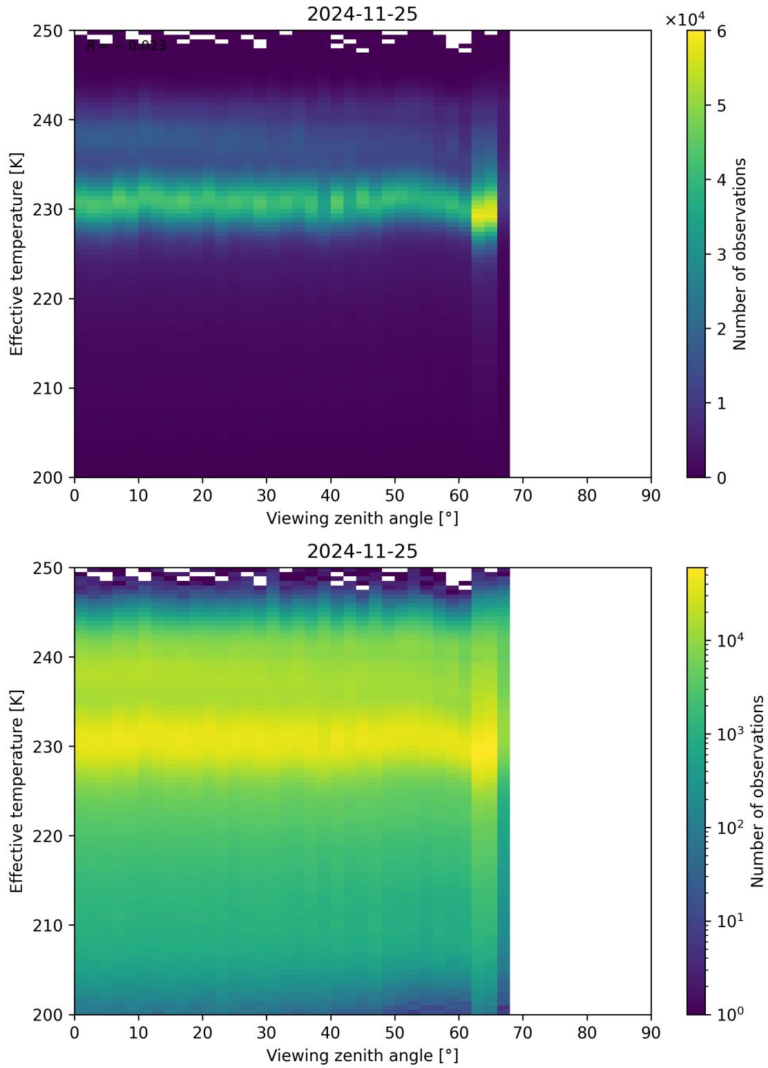
Figure 50: Scatter density plot of “Viewing zenith angle” against “Effective temperature” for 2024-11-25 to 2024-11-26.
