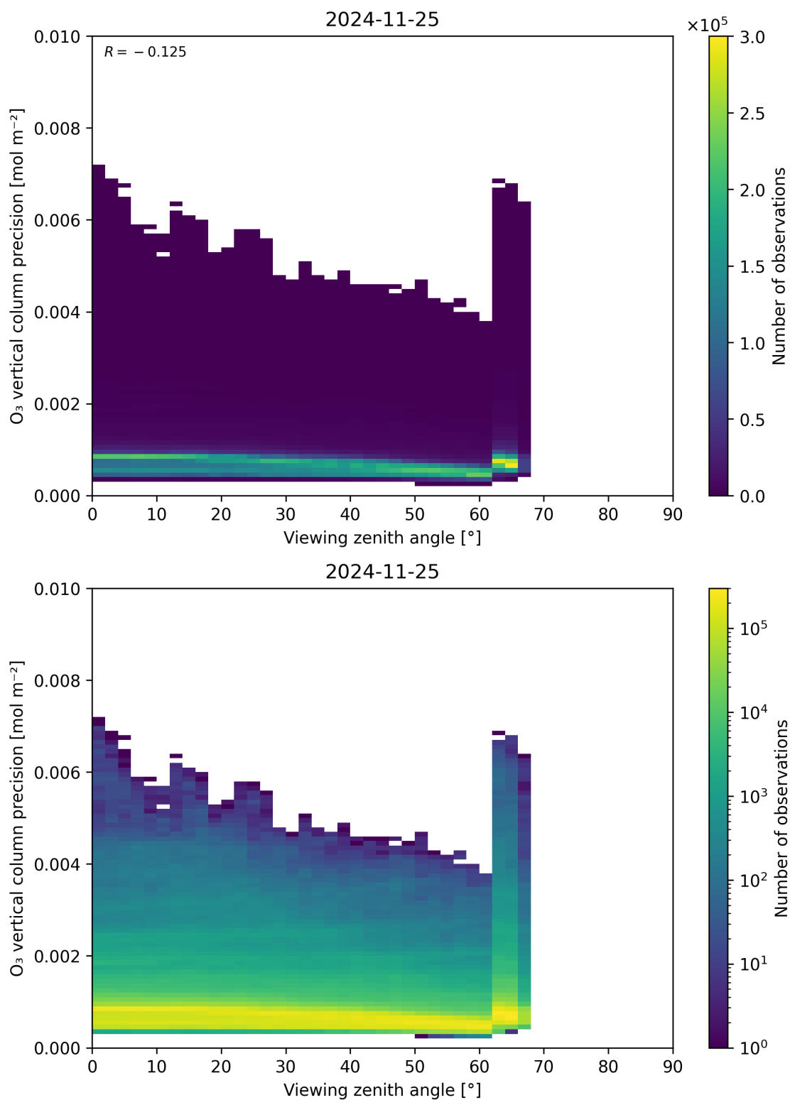
Figure 53: Scatter density plot of “Viewing zenith angle” against “O 3 vertical column precision” for 2024-11-25 to 2024-11-26.
