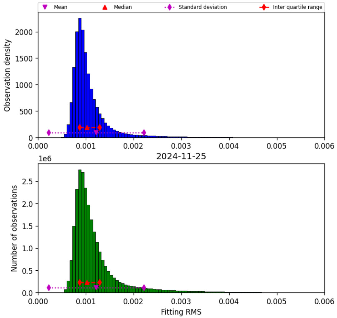
Figure 23: Histogram of “Fitting RMS” for 2024-11-25 to 2024-11-26
