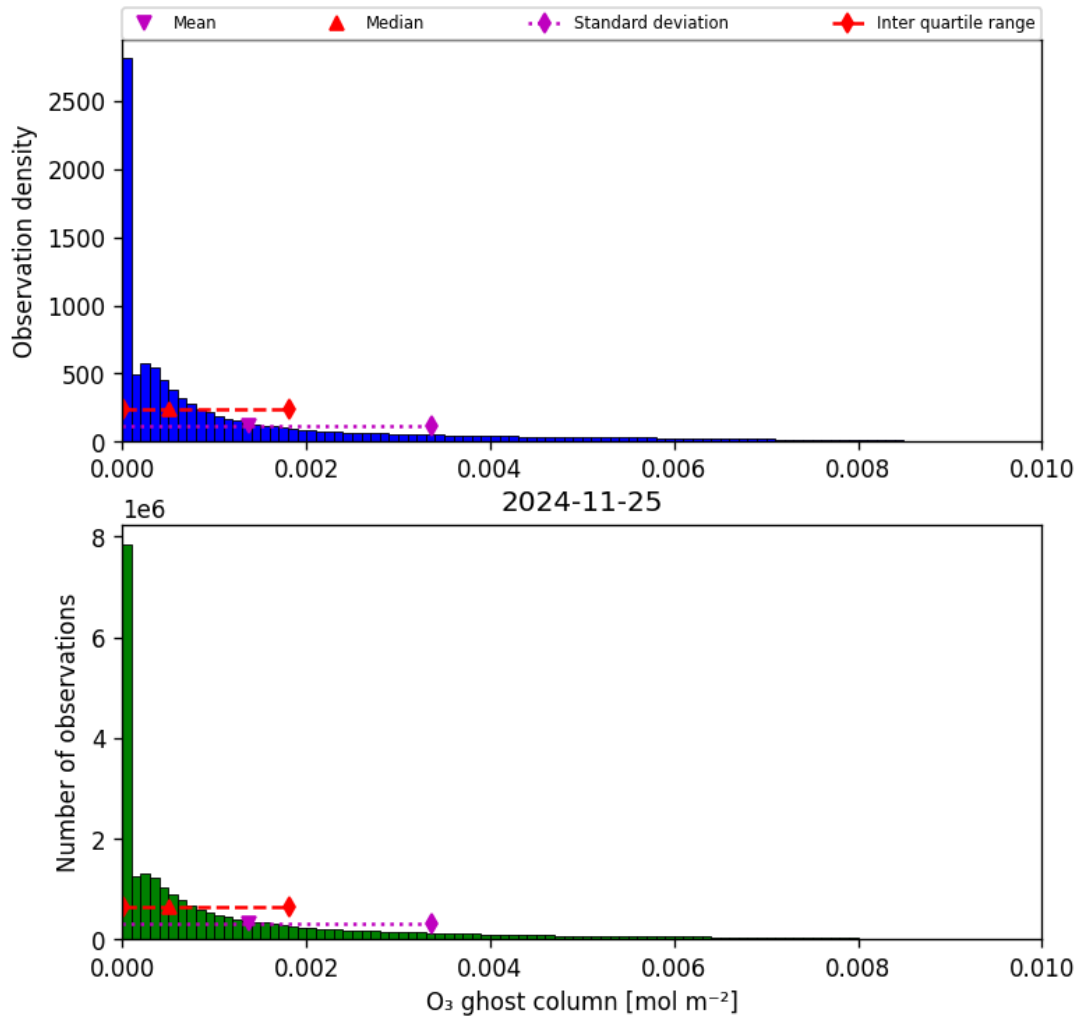
Figure 25: Histogram of “O 3 ghost column” for 2024-11-25 to 2024-11-26
