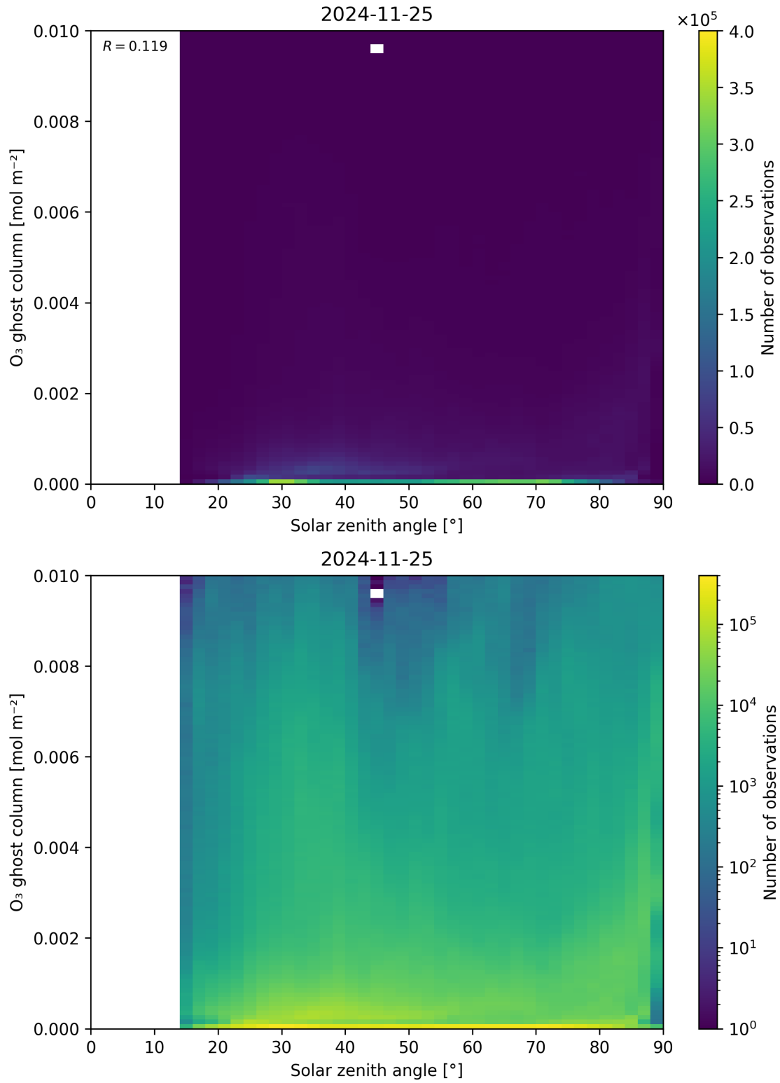
Figure 46: Scatter density plot of “Solar zenith angle” against “O 3 ghost column” for 2024-11-25 to 2024-11-26.
