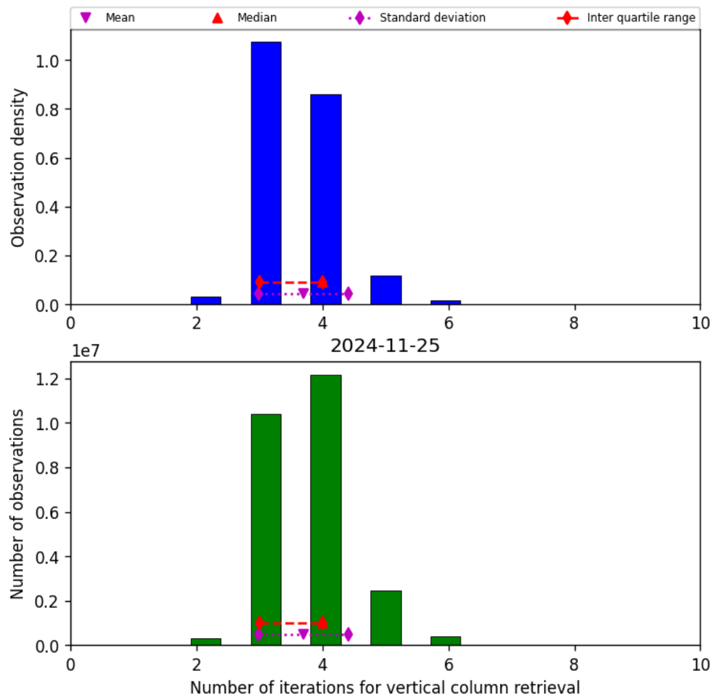
Figure 26: Histogram of “Number of iterations for vertical column retrieval” for 2024-11-25 to 2024-11-26
