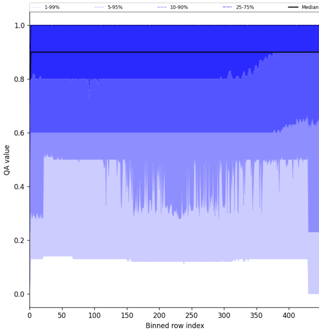
Figure 27: Along track statistics of “QA value” for 2024-11-25 to 2024-11-26
