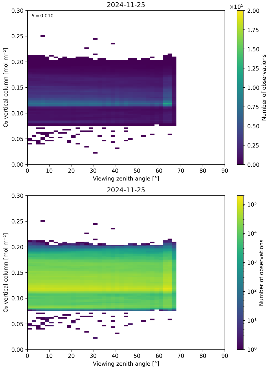
Figure 52: Scatter density plot of “Viewing zenith angle” against “O 3 vertical column” for 2024-11-25 to 2024-11-26.
