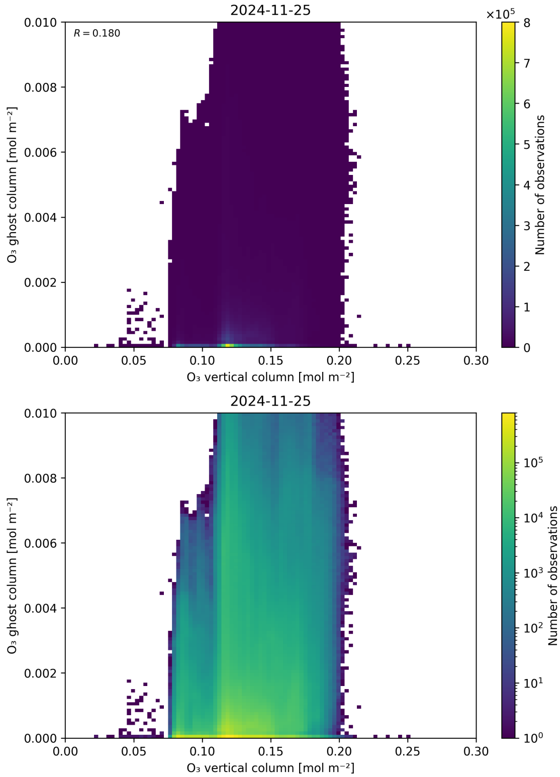
Figure 40: Scatter density plot of “O 3 vertical column” against “O 3 ghost column” for 2024-11-25 to 2024-11-26.
