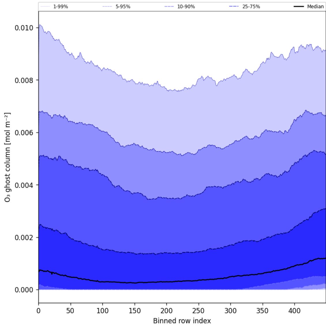
Figure 32: Along track statistics of “O 3 ghost column” for 2024-11-25 to 2024-11-26
