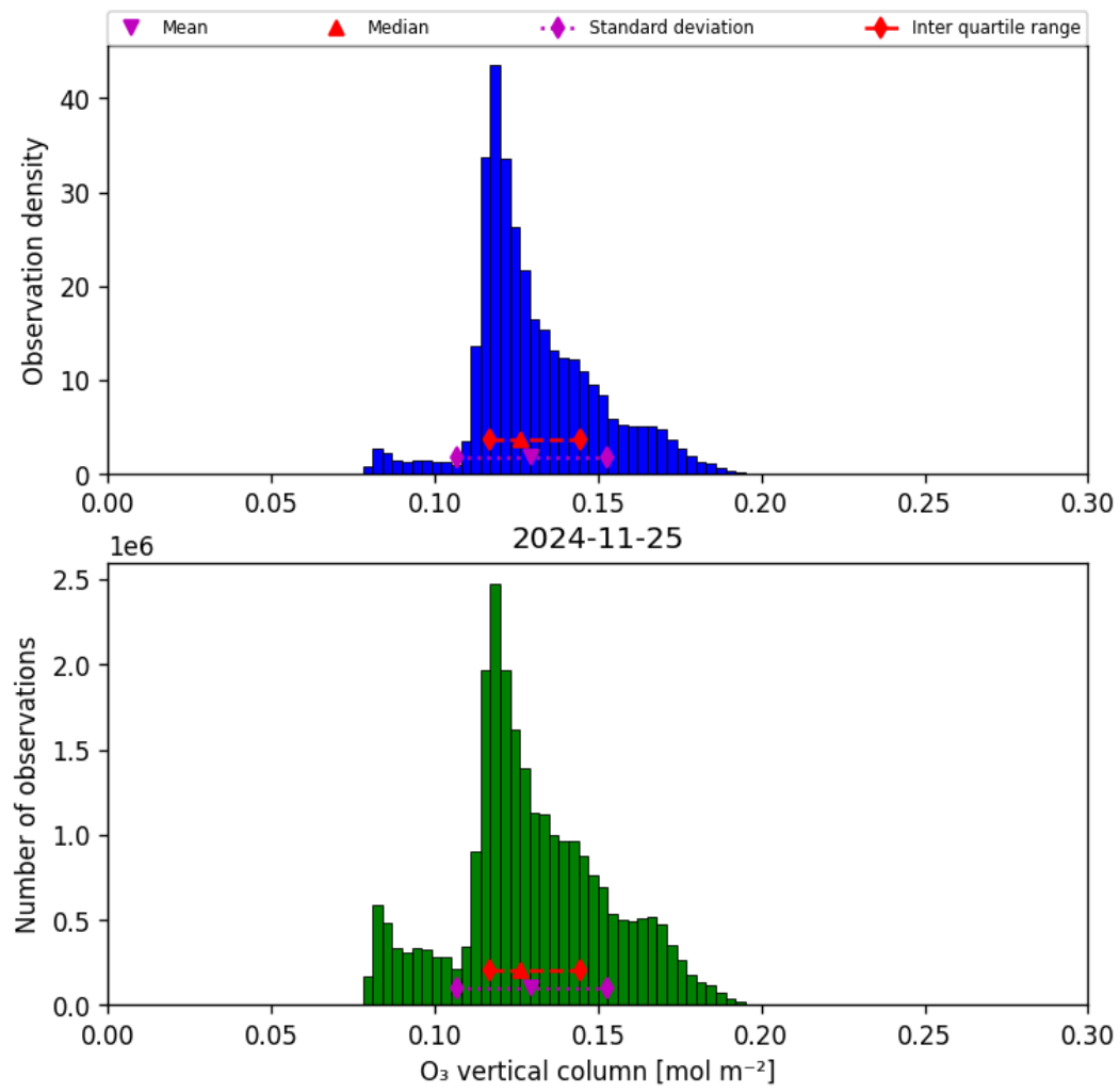
Figure 21: Histogram of “O 3 vertical column” for 2024-11-25 to 2024-11-26
