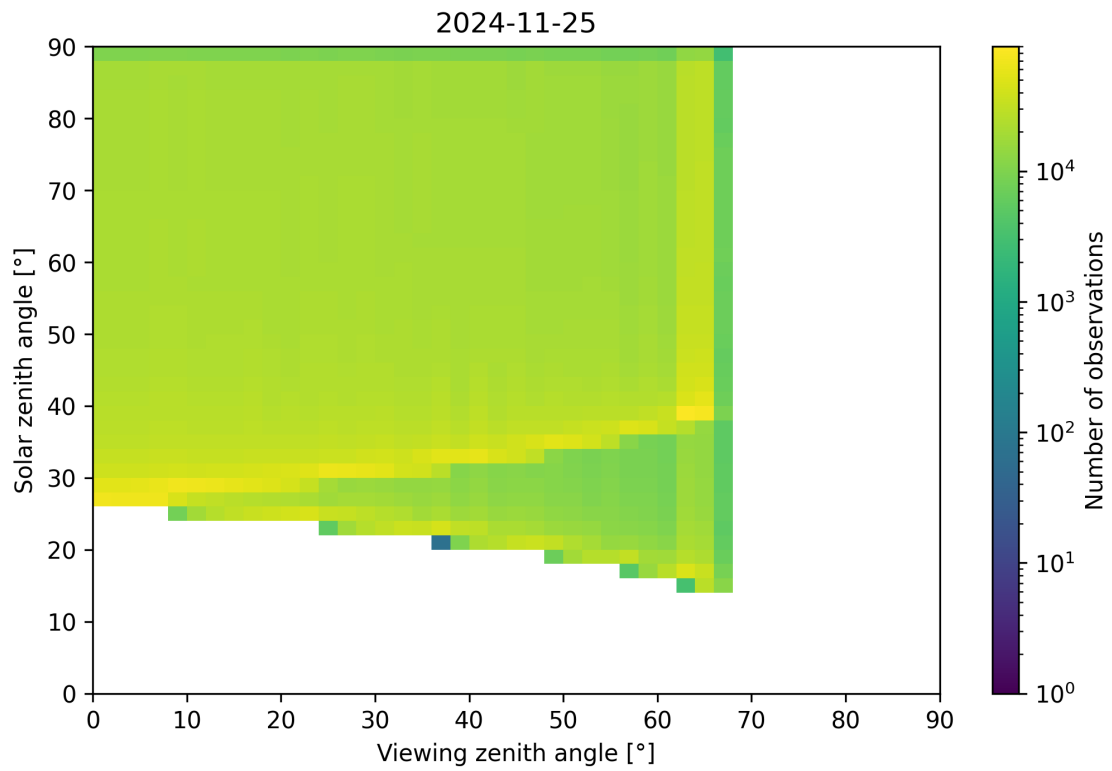
Figure 54: Scatter density plot of “Viewing zenith angle” against “Solar zenith angle” for 2024-11-25 to 2024-11-26.
