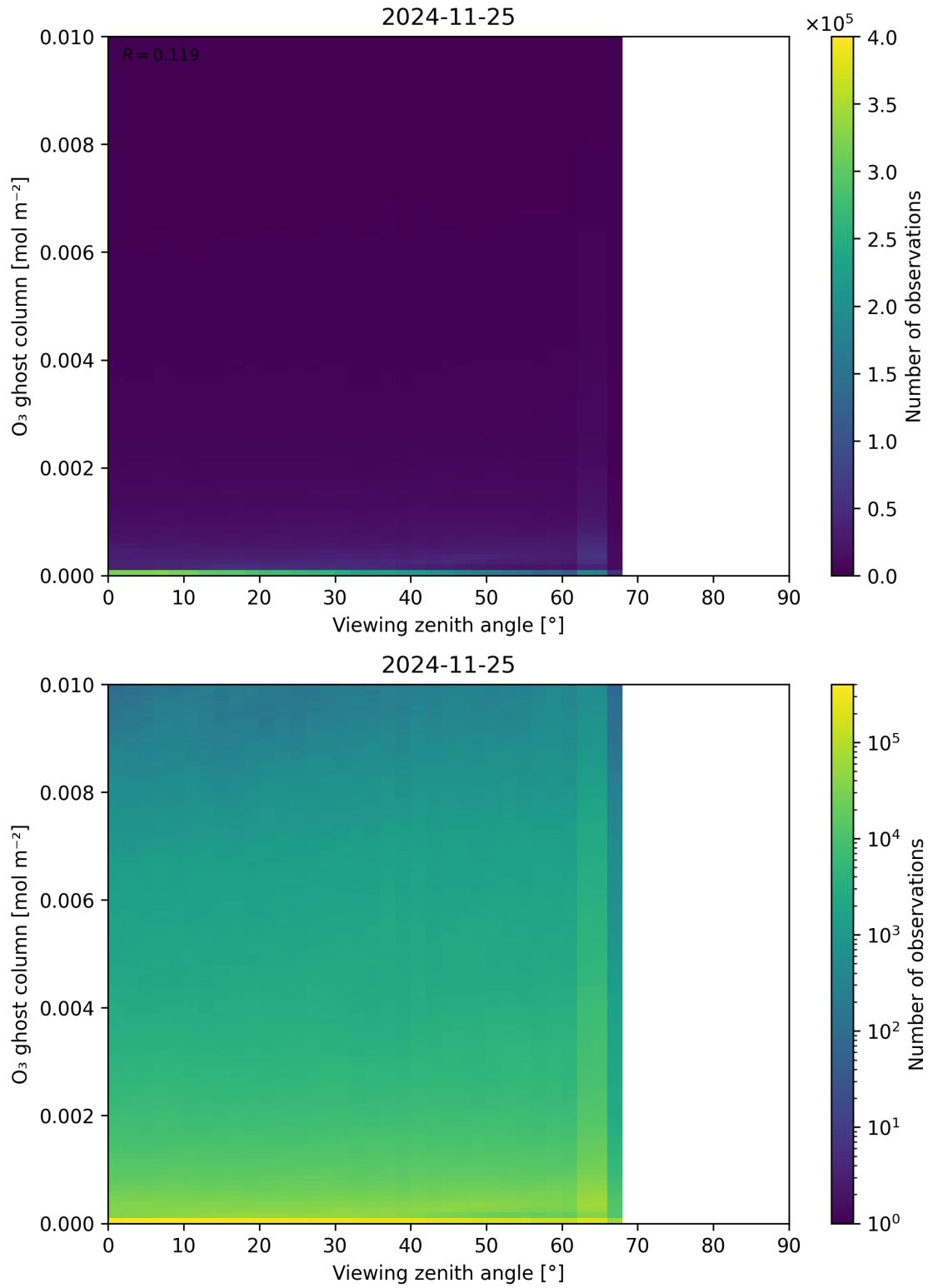
Figure 51: Scatter density plot of “Viewing zenith angle” against “O 3 ghost column” for 2024-11-25 to 2024-11-26.
