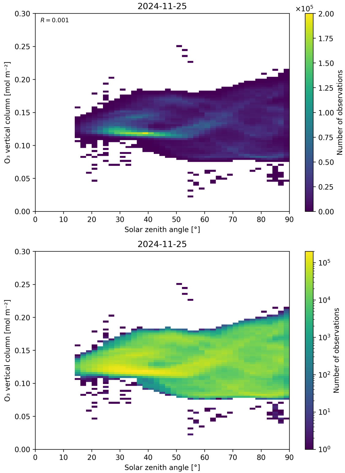
Figure 47: Scatter density plot of “Solar zenith angle” against “O 3 vertical column” for 2024-11-25 to 2024-11-26.
