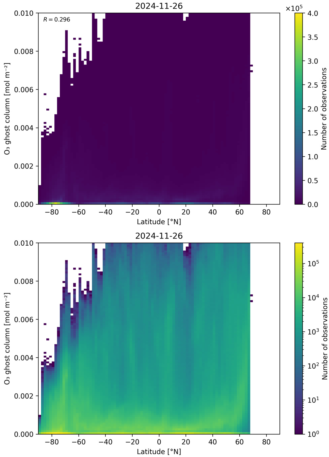
Figure 35: Scatter density plot of “Latitude” against “O 3 ghost column” for 2024-11-25 to 2024-11-27.
