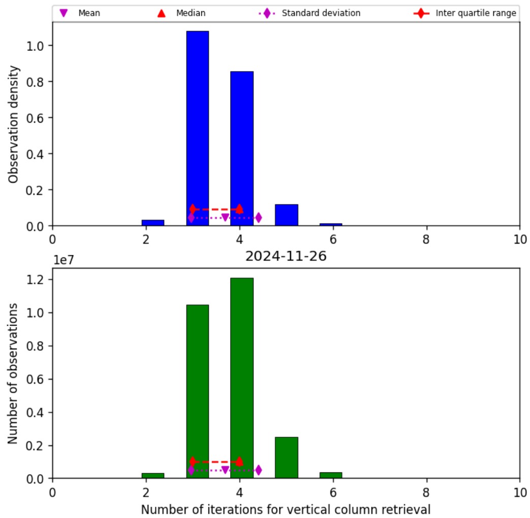
Figure 26: Histogram of “Number of iterations for vertical column retrieval” for 2024-11-25 to 2024-11-27
