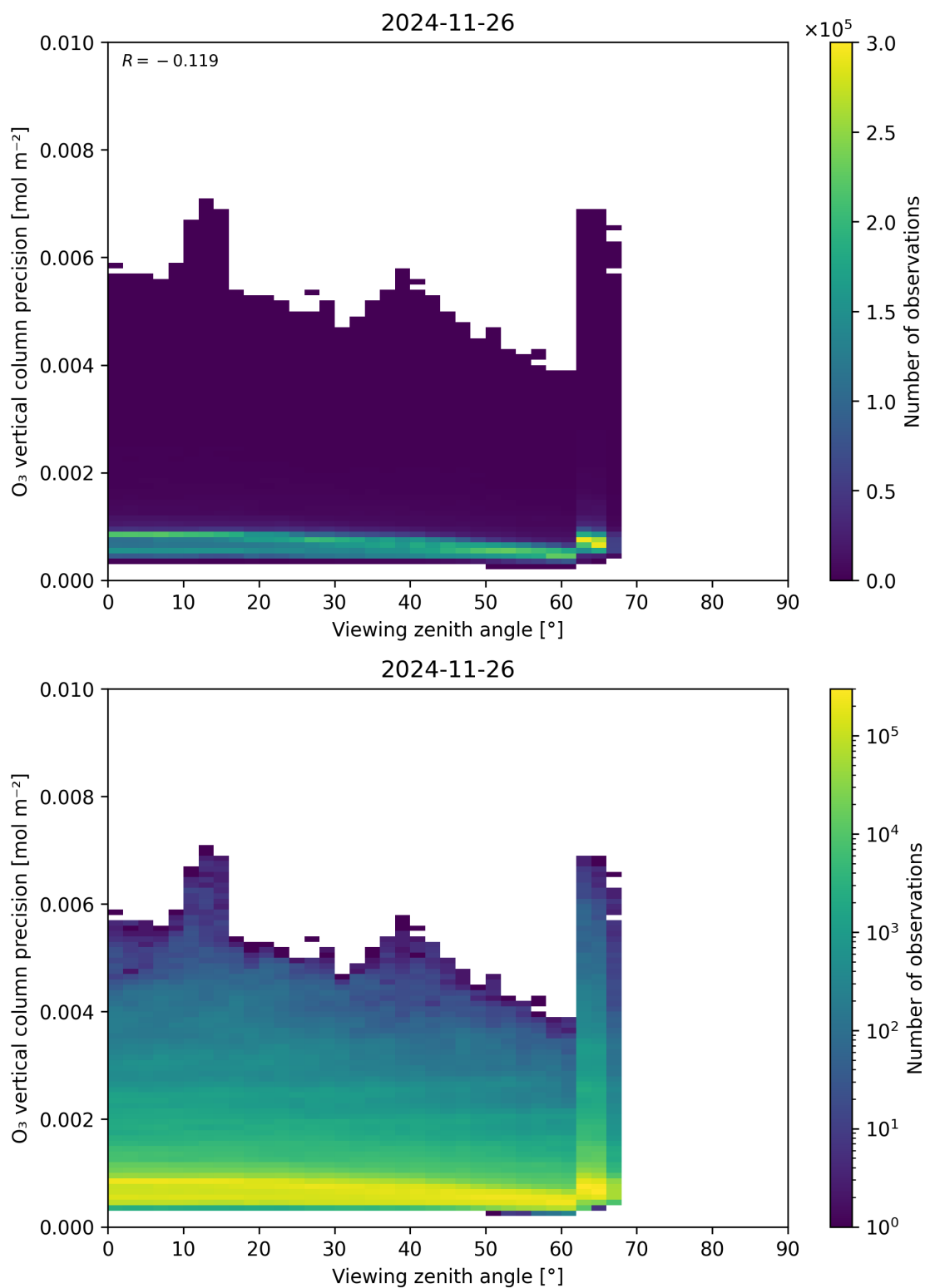
Figure 53: Scatter density plot of “Viewing zenith angle” against “O 3 vertical column precision” for 2024-11-25 to 2024-11-27.
