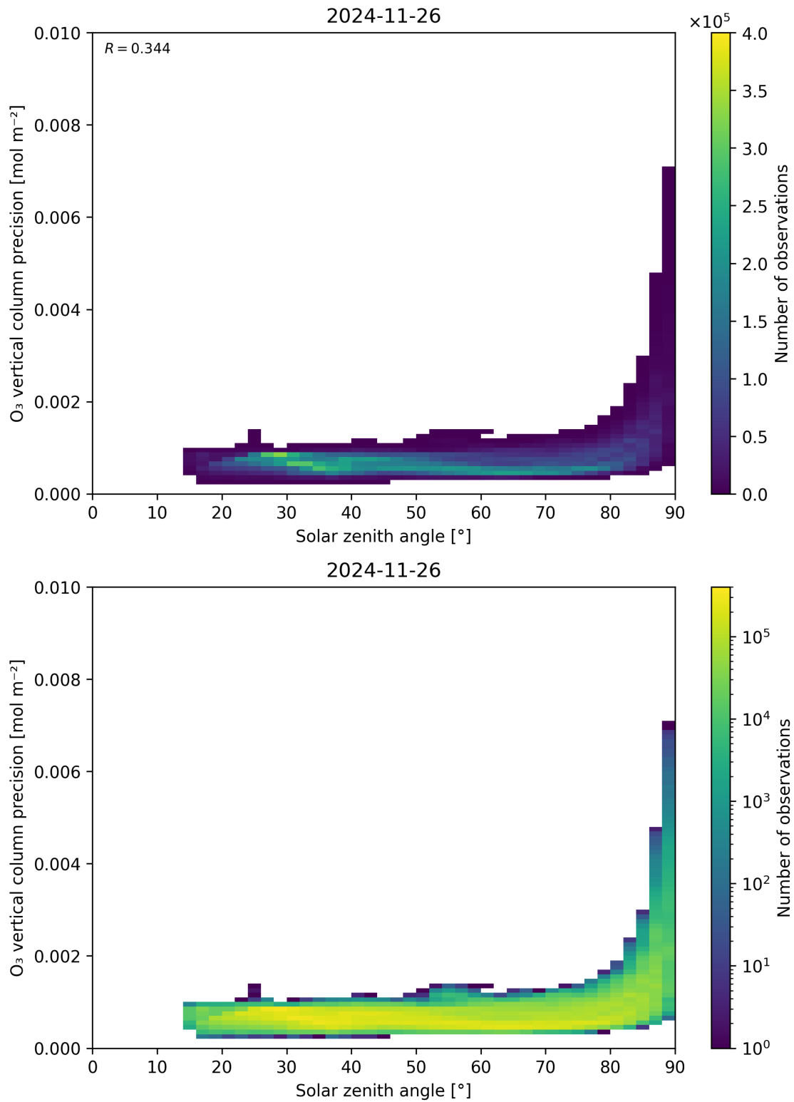
Figure 48: Scatter density plot of “Solar zenith angle” against “O 3 vertical column precision” for 2024-11-25 to 2024-11-27.
