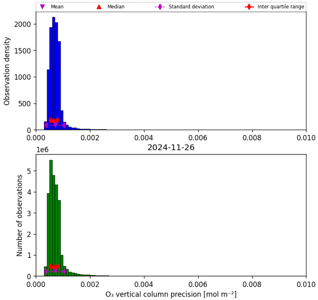
Figure 22: Histogram of “O 3 vertical column precision” for 2024-11-25 to 2024-11-27
