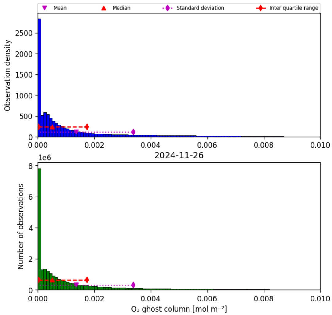
Figure 25: Histogram of “O 3 ghost column” for 2024-11-25 to 2024-11-27
