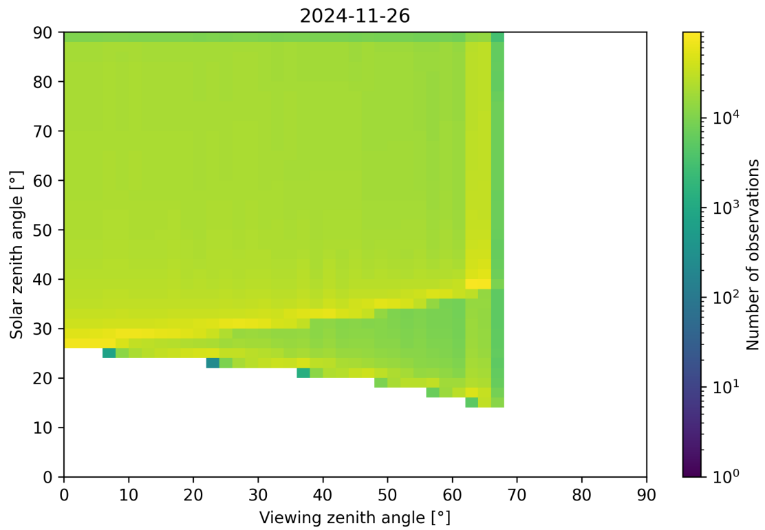
Figure 54: Scatter density plot of “Viewing zenith angle” against “Solar zenith angle” for 2024-11-25 to 2024-11-27.
