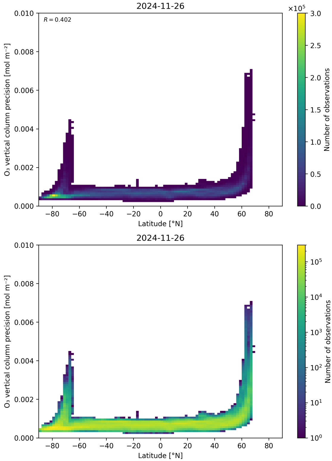
Figure 37: Scatter density plot of “Latitude” against “O 3 vertical column precision” for 2024-11-25 to 2024-11-27.
