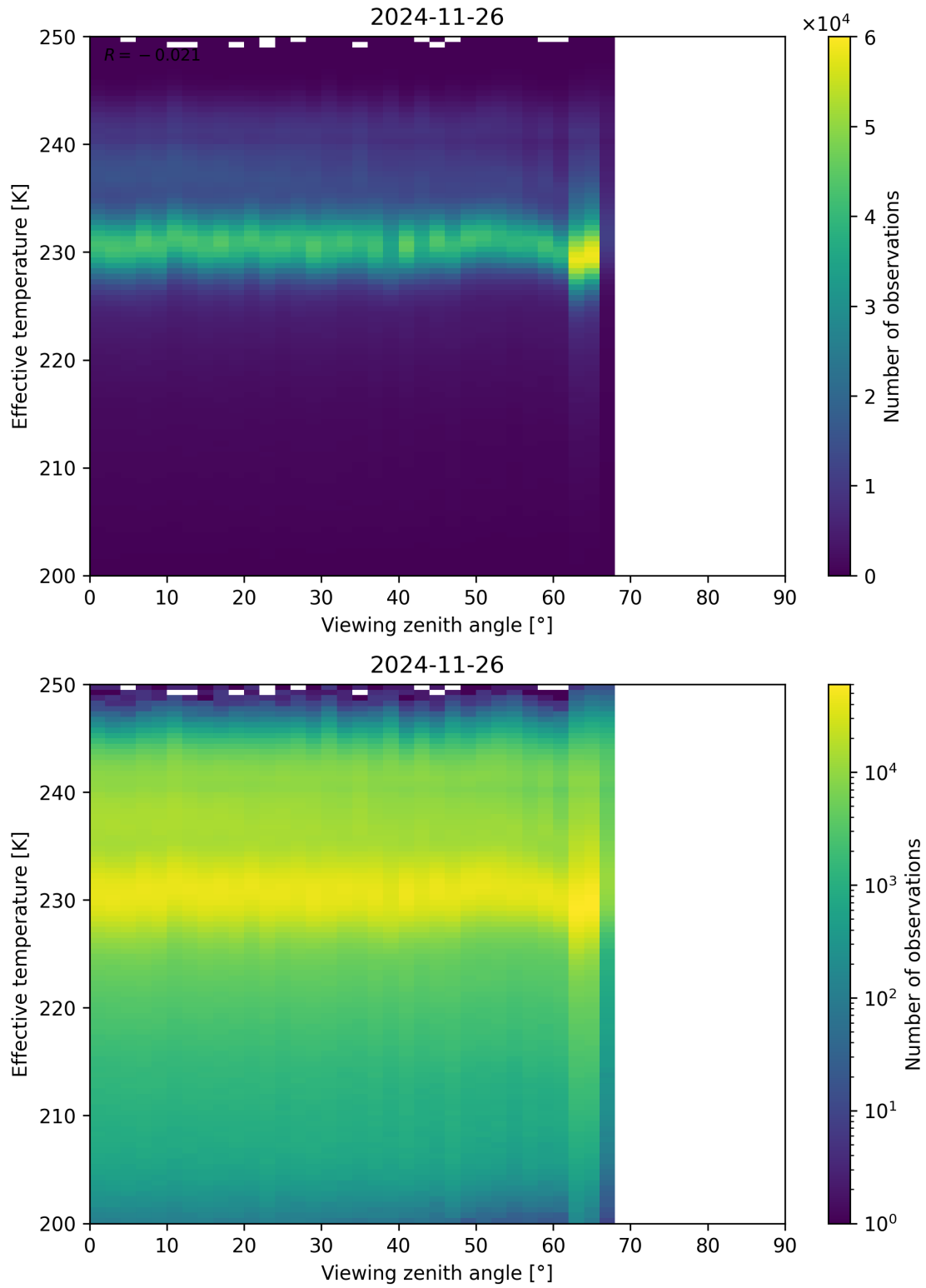
Figure 50: Scatter density plot of “Viewing zenith angle” against “Effective temperature” for 2024-11-25 to 2024-11-27.
