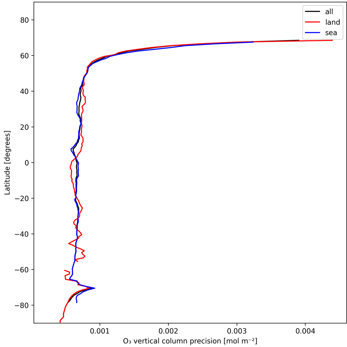
Figure 15: Zonal average of “O 3 vertical column precision” for 2024-11-25 to 2024-11-27.
