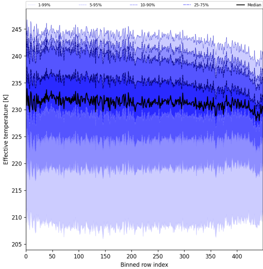
Figure 31: Along track statistics of “Effective temperature” for 2024-11-25 to 2024-11-27
