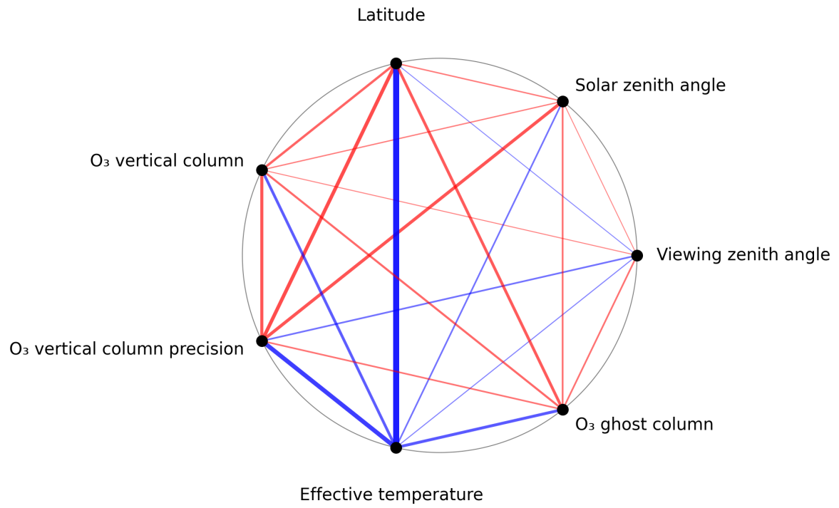
Figure 1: Map of correlation graph for 2024-11-25 to 2024-11-27.
