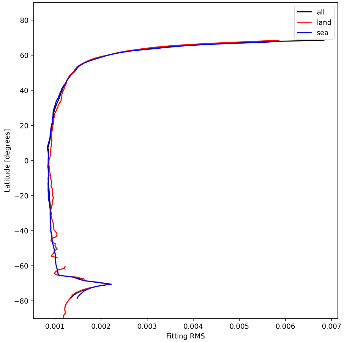
Figure 16: Zonal average of “Fitting RMS” for 2024-11-25 to 2024-11-27.
