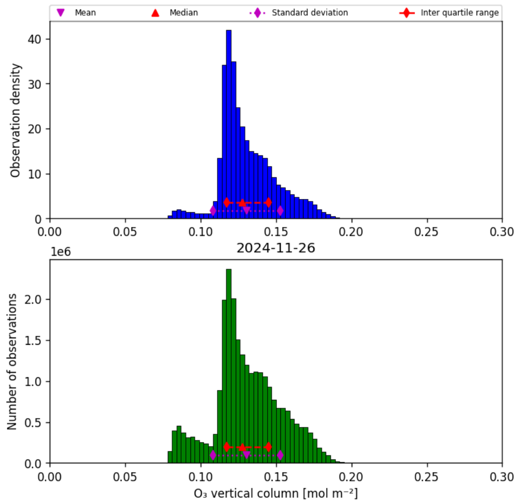
Figure 21: Histogram of “O 3 vertical column” for 2024-11-25 to 2024-11-27
