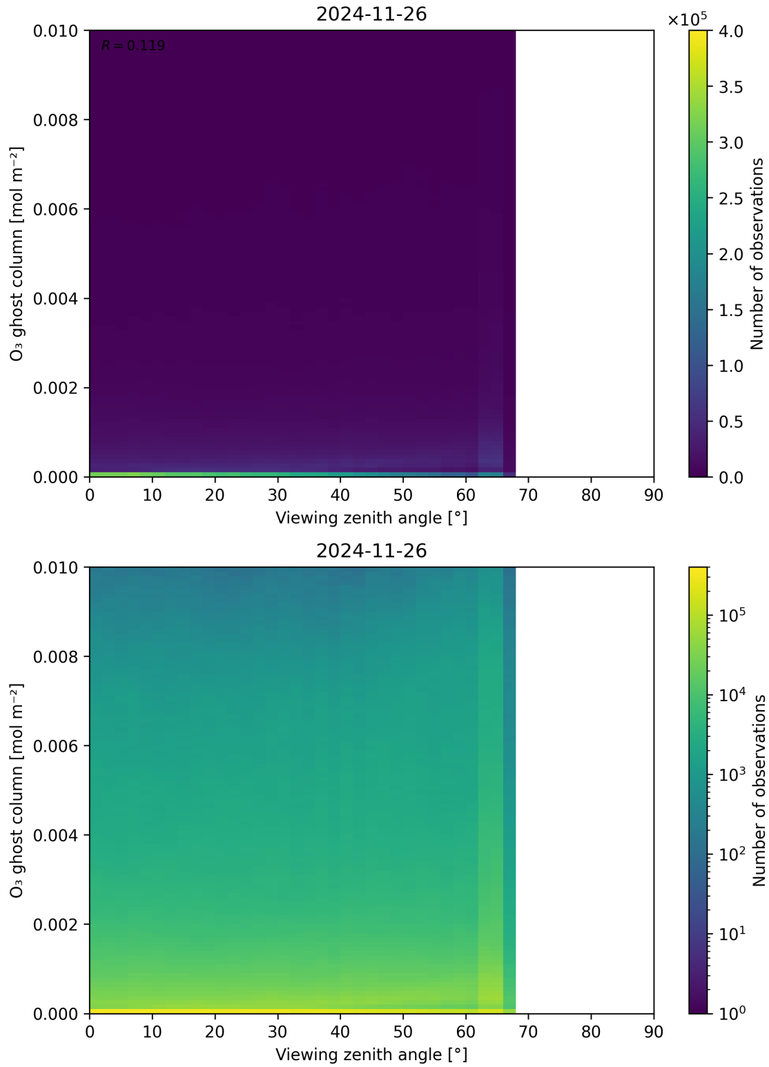
Figure 51: Scatter density plot of “Viewing zenith angle” against “O 3 ghost column” for 2024-11-25 to 2024-11-27.
