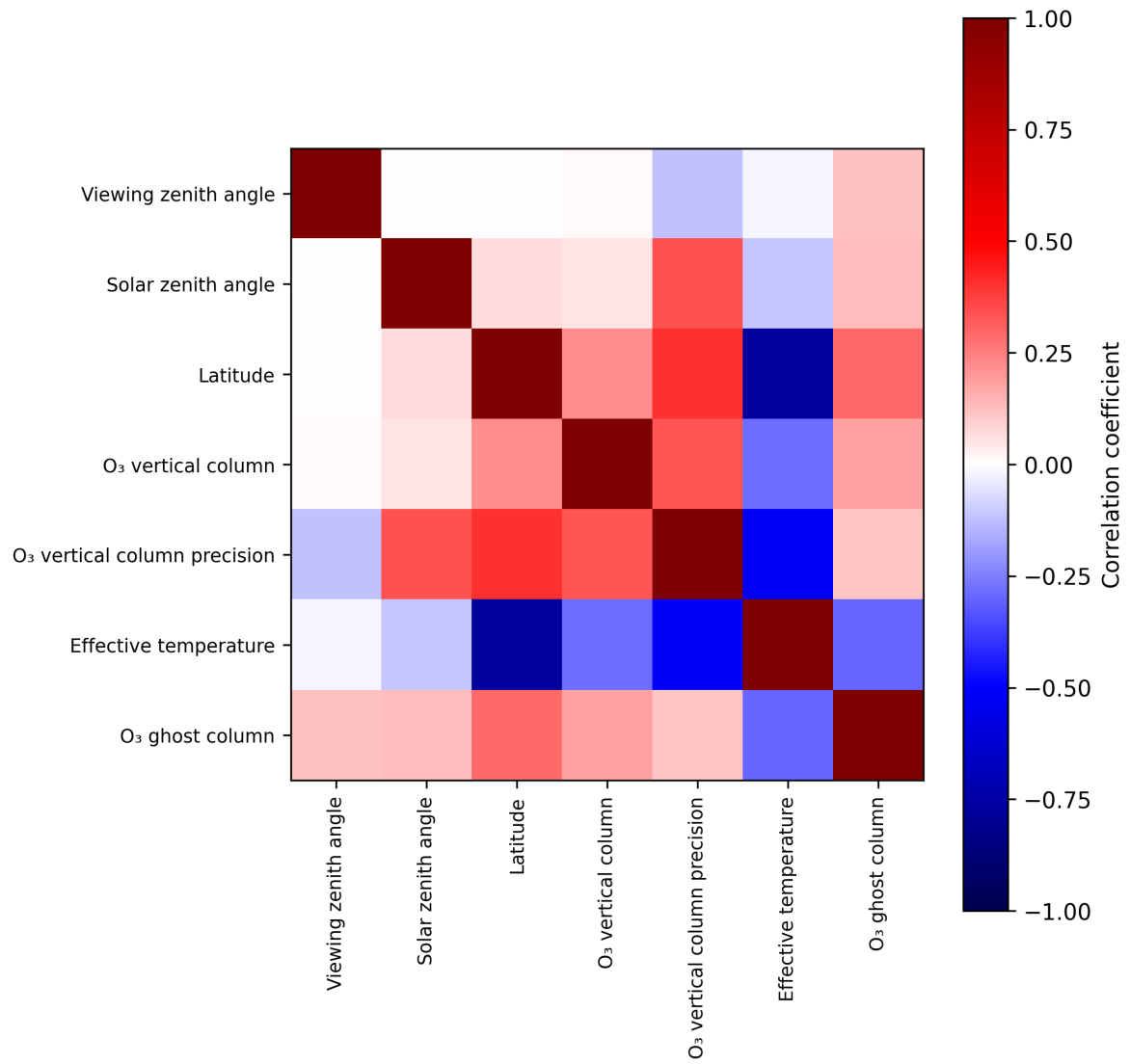
Figure 2: Map of correlation matrix for 2024-11-25 to 2024-11-27.
