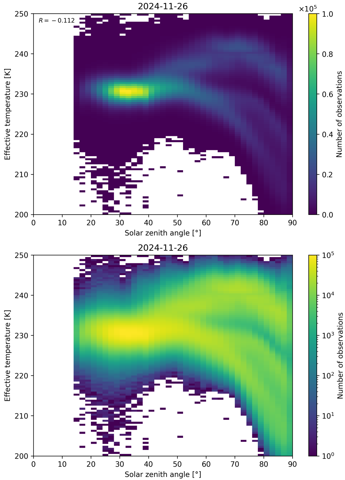
Figure 45: Scatter density plot of “Solar zenith angle” against “Effective temperature” for 2024-11-25 to 2024-11-27.
