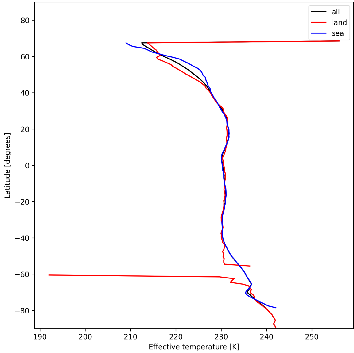
Figure 17: Zonal average of “Effective temperature” for 2024-11-25 to 2024-11-27.
