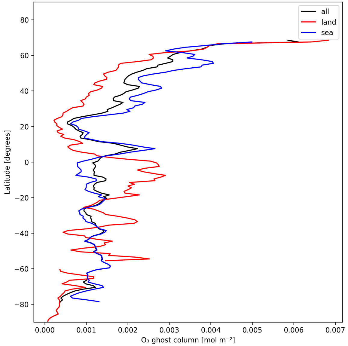
Figure 18: Zonal average of “O 3 ghost column” for 2024-11-25 to 2024-11-27.
