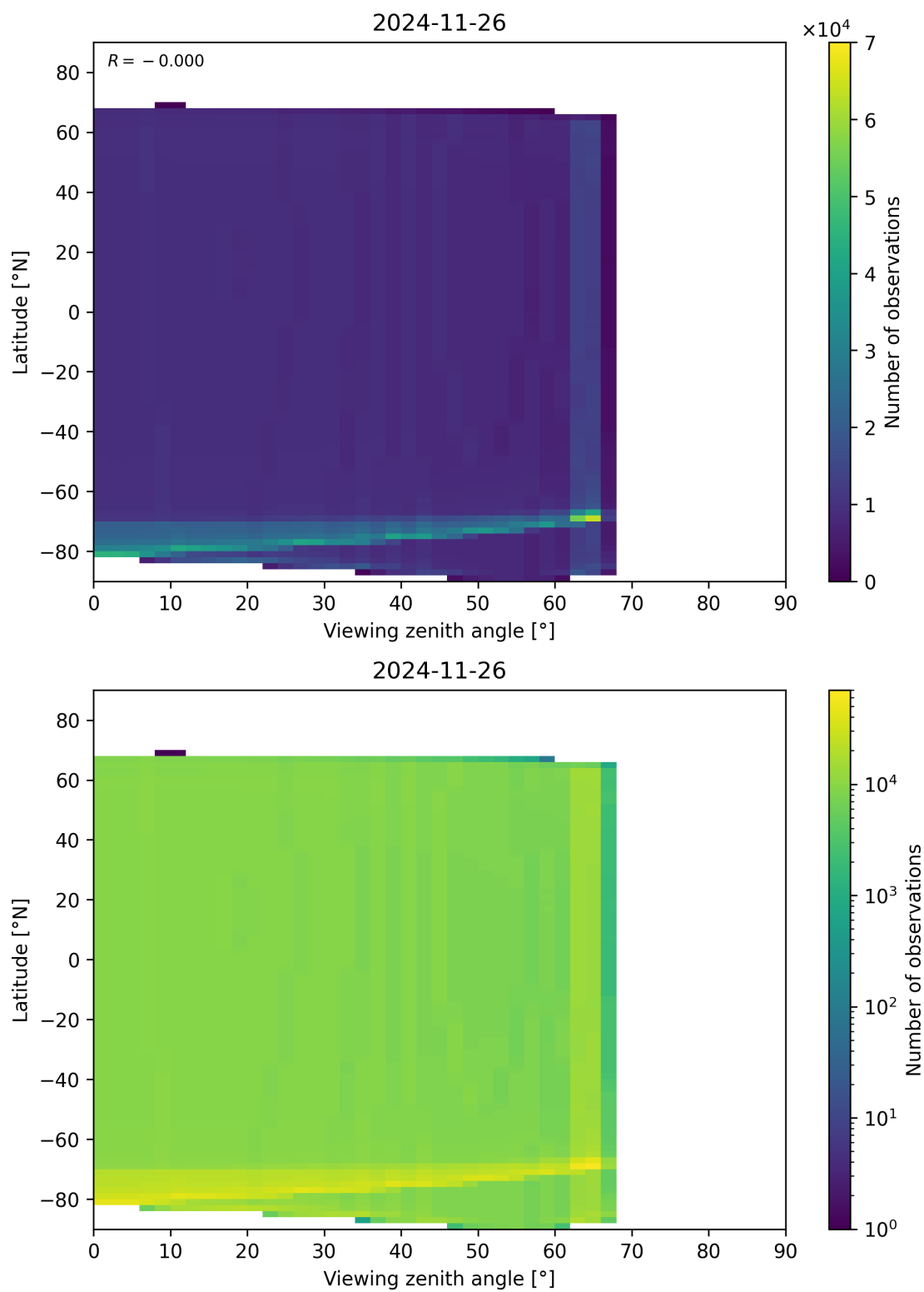
Figure 49: Scatter density plot of “Viewing zenith angle” against “Latitude” for 2024-11-25 to 2024-11-27.
