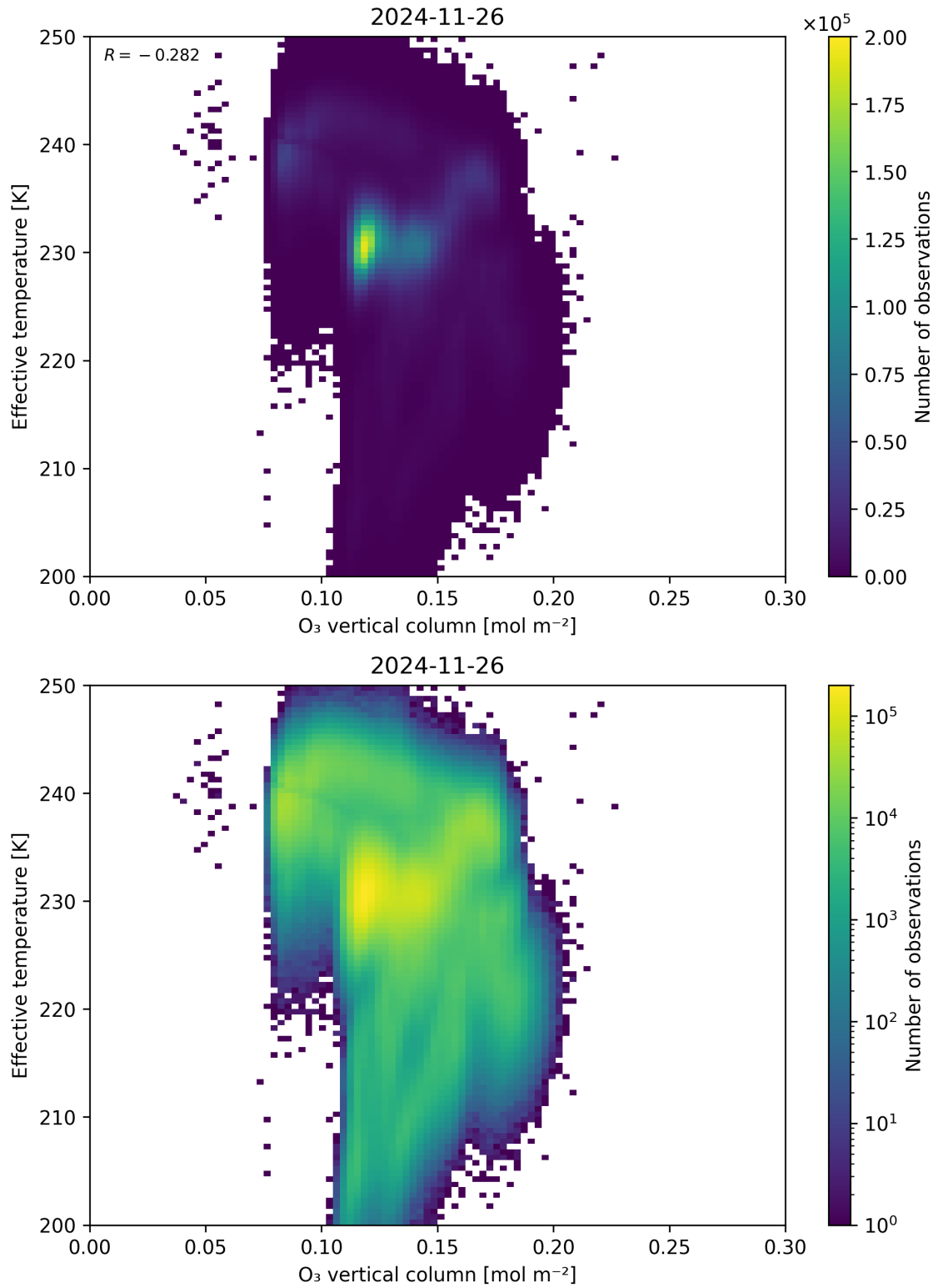
Figure 39: Scatter density plot of “O 3 vertical column” against “Effective temperature” for 2024-11-25 to 2024-11-27.
