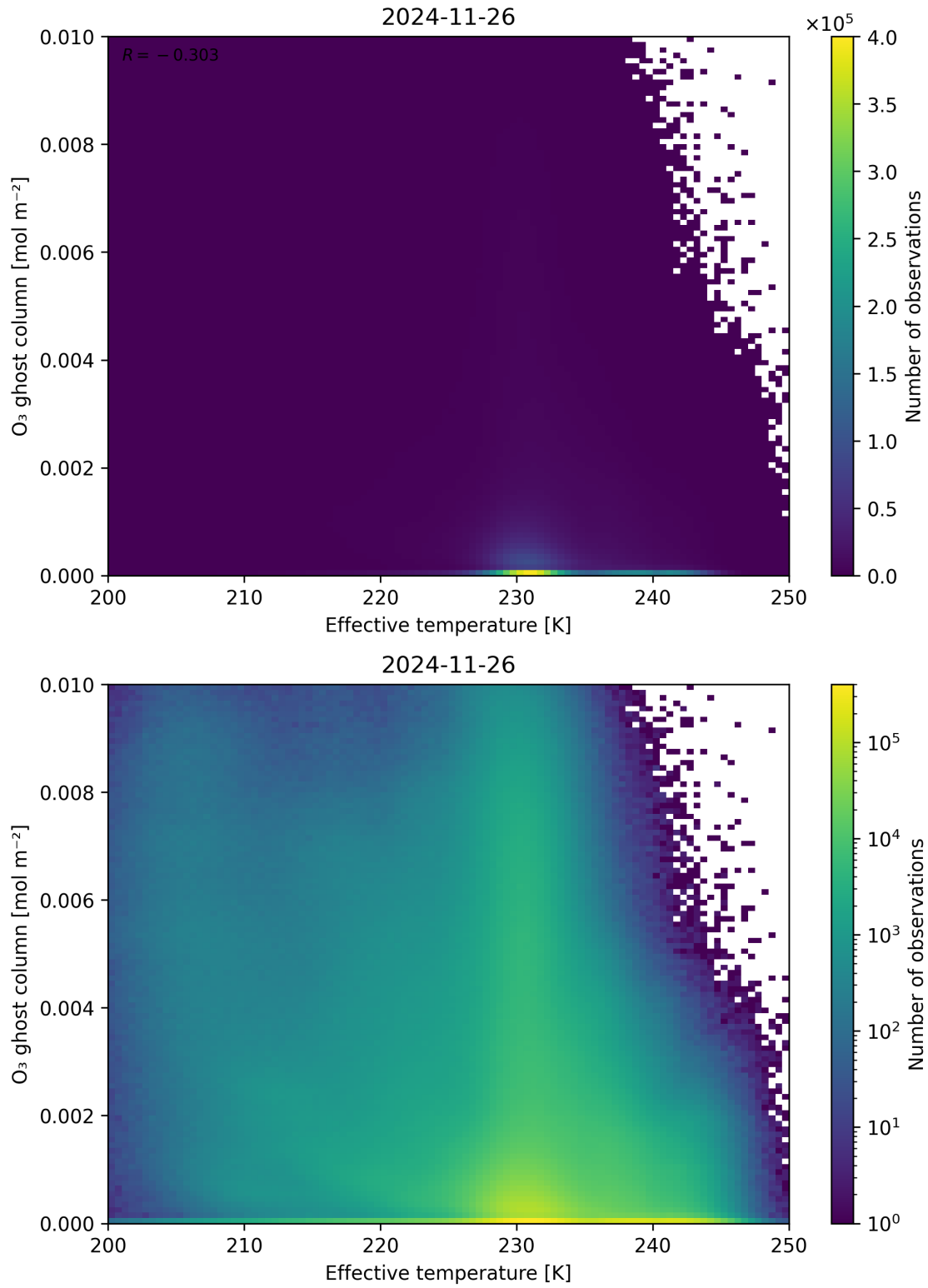
Figure 38: Scatter density plot of “Effective temperature” against “O 3 ghost column” for 2024-11-25 to 2024-11-27.
