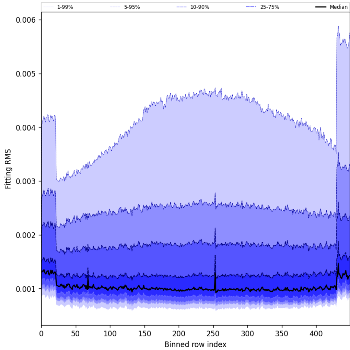
Figure 30: Along track statistics of “Fitting RMS” for 2024-11-25 to 2024-11-27
