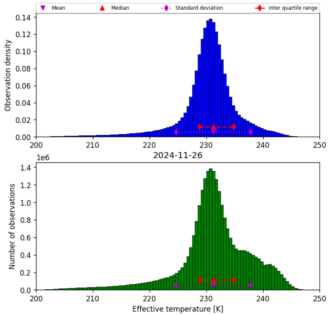
Figure 24: Histogram of “Effective temperature” for 2024-11-25 to 2024-11-27
