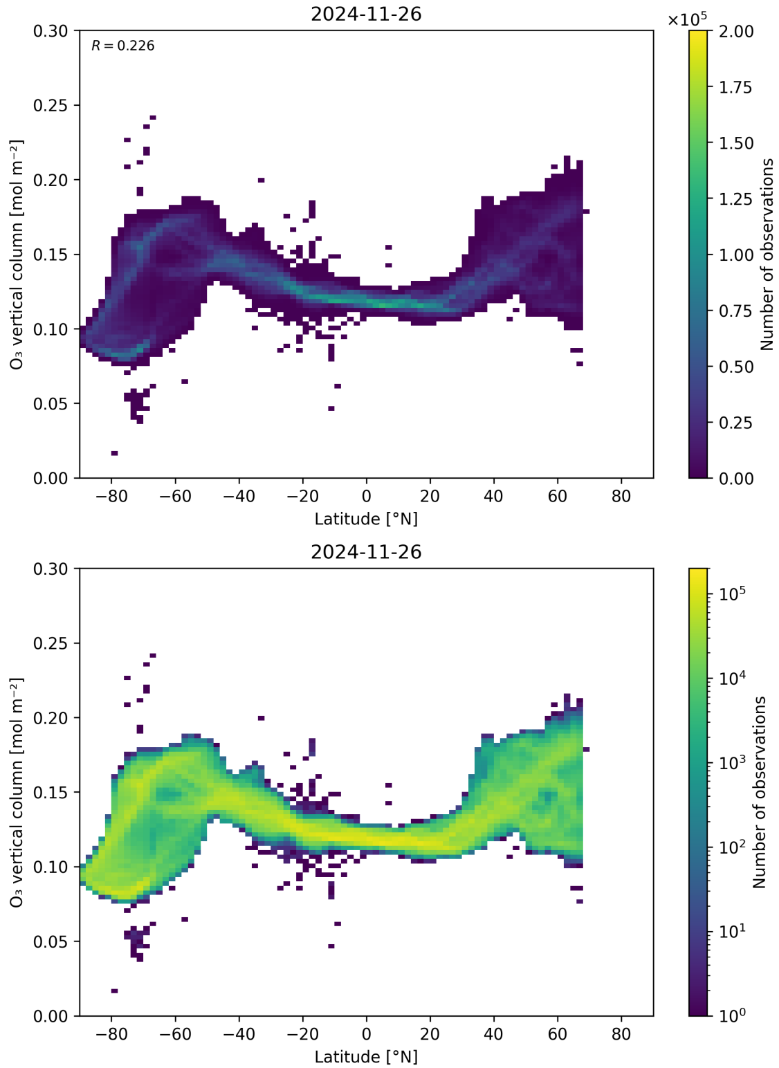
Figure 36: Scatter density plot of “Latitude” against “O 3 vertical column” for 2024-11-25 to 2024-11-27.
