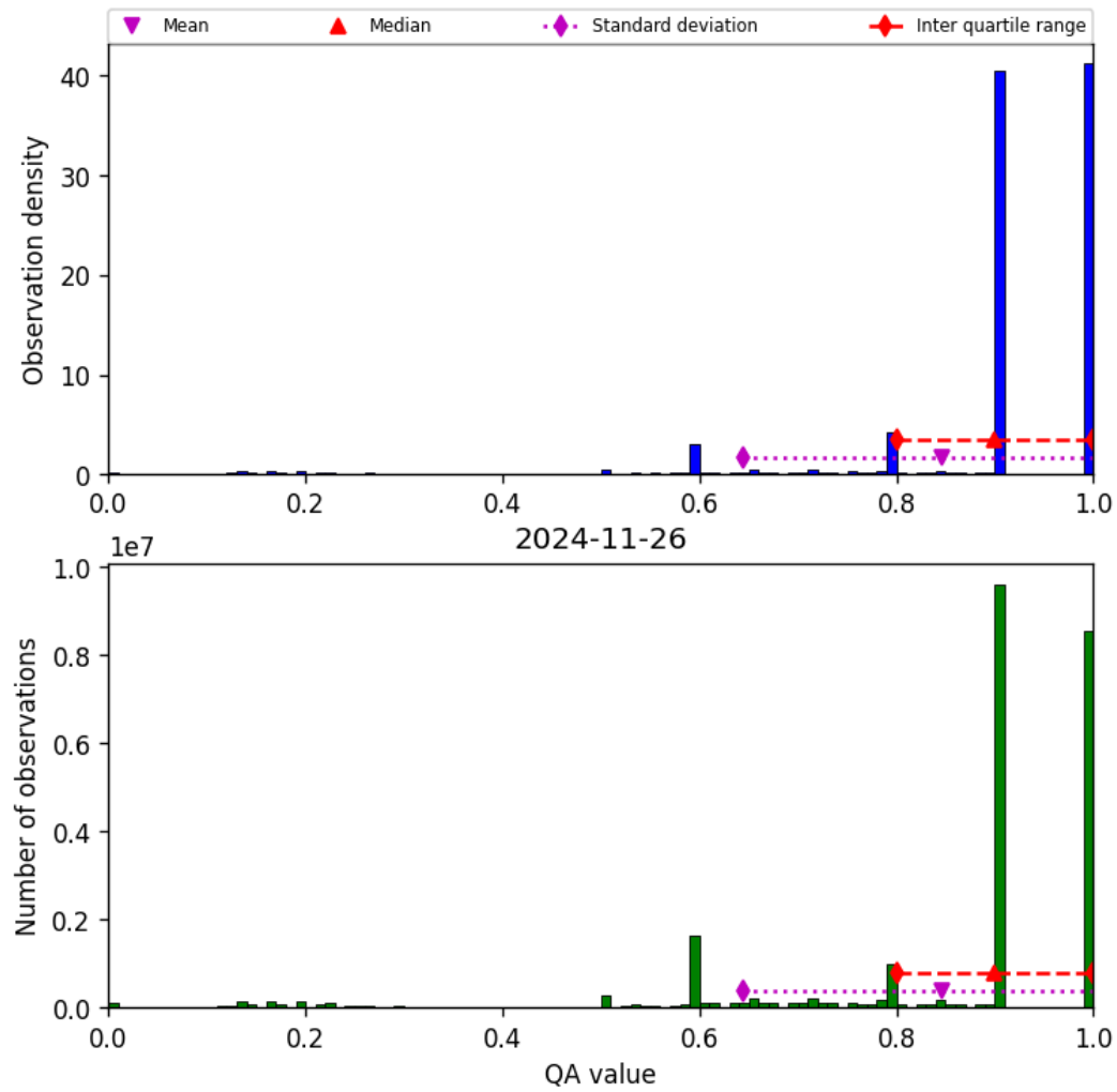
Figure 20: Histogram of “QA value” for 2024-11-25 to 2024-11-27
