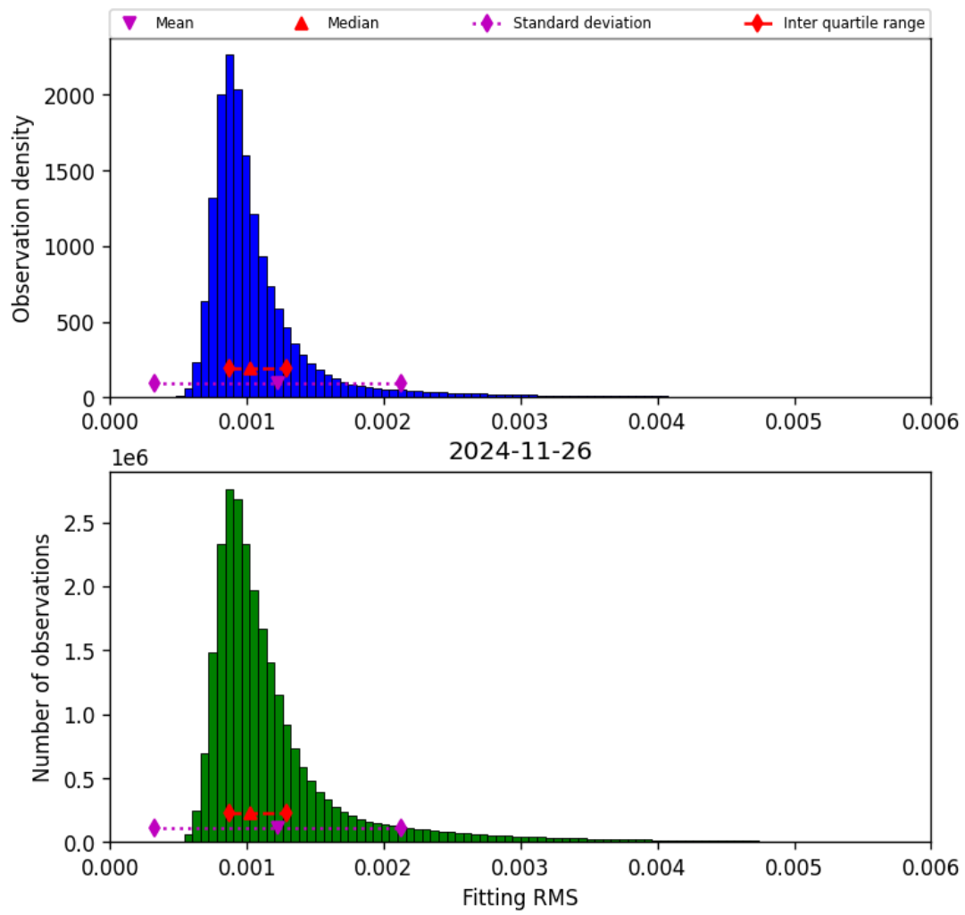
Figure 23: Histogram of “Fitting RMS” for 2024-11-25 to 2024-11-27
