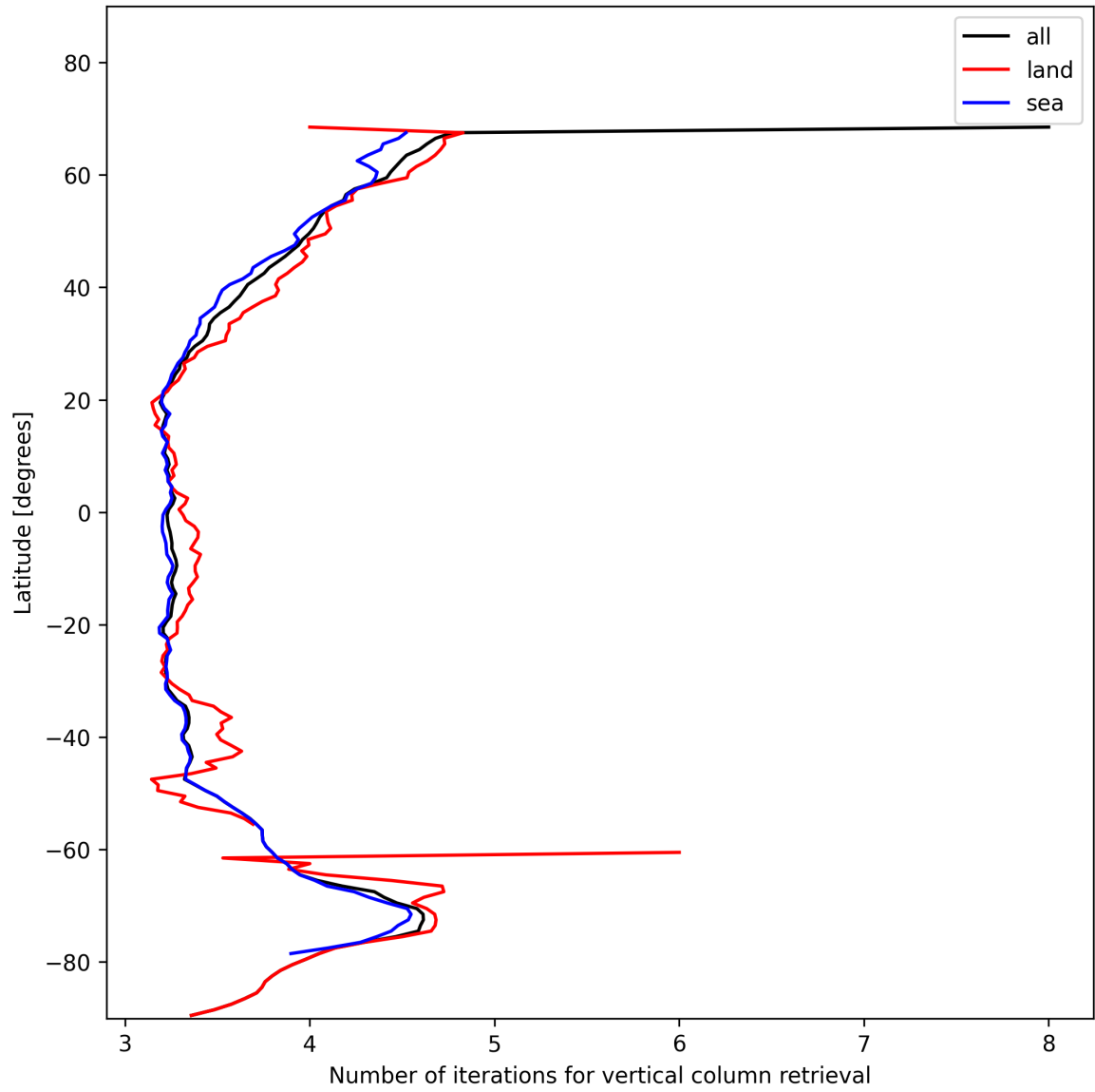
Figure 19: Zonal average of “Number of iterations for vertical column retrieval” for 2024-11-25 to 2024-11-27.
