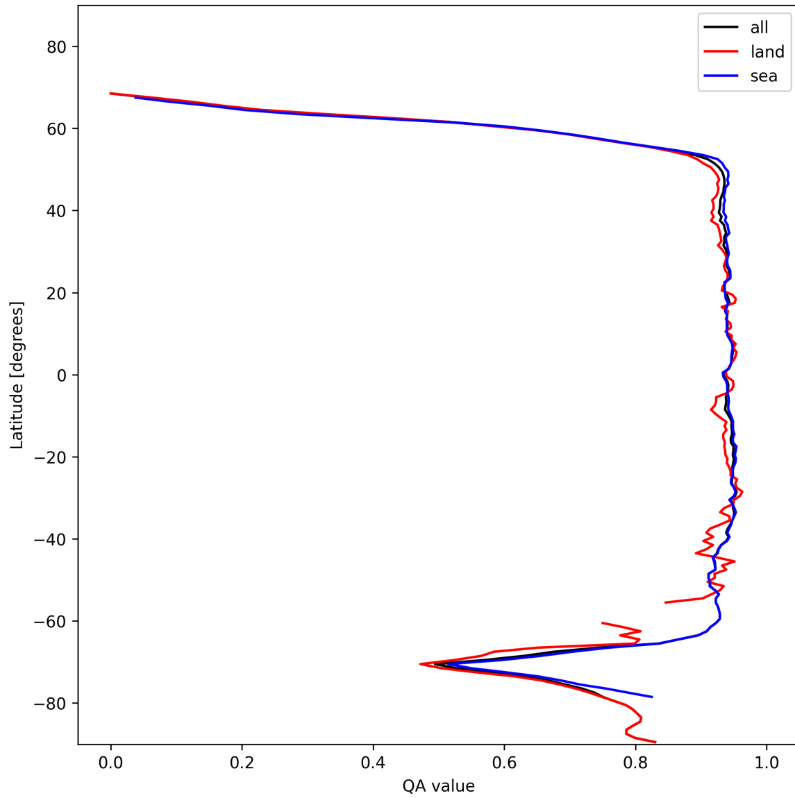
Figure 13: Zonal average of “QA value” for 2024-11-25 to 2024-11-27.
