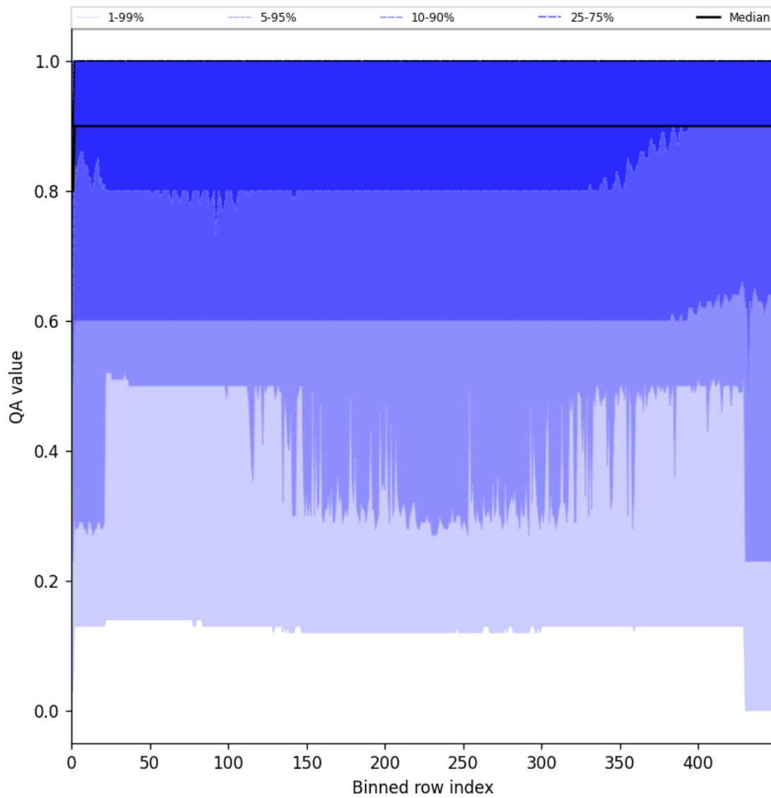
Figure 27: Along track statistics of “QA value” for 2024-11-25 to 2024-11-27
