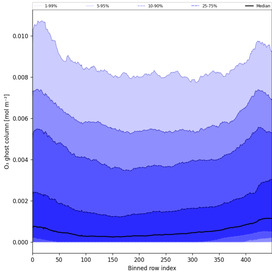
Figure 32: Along track statistics of “O 3 ghost column” for 2024-11-25 to 2024-11-27
