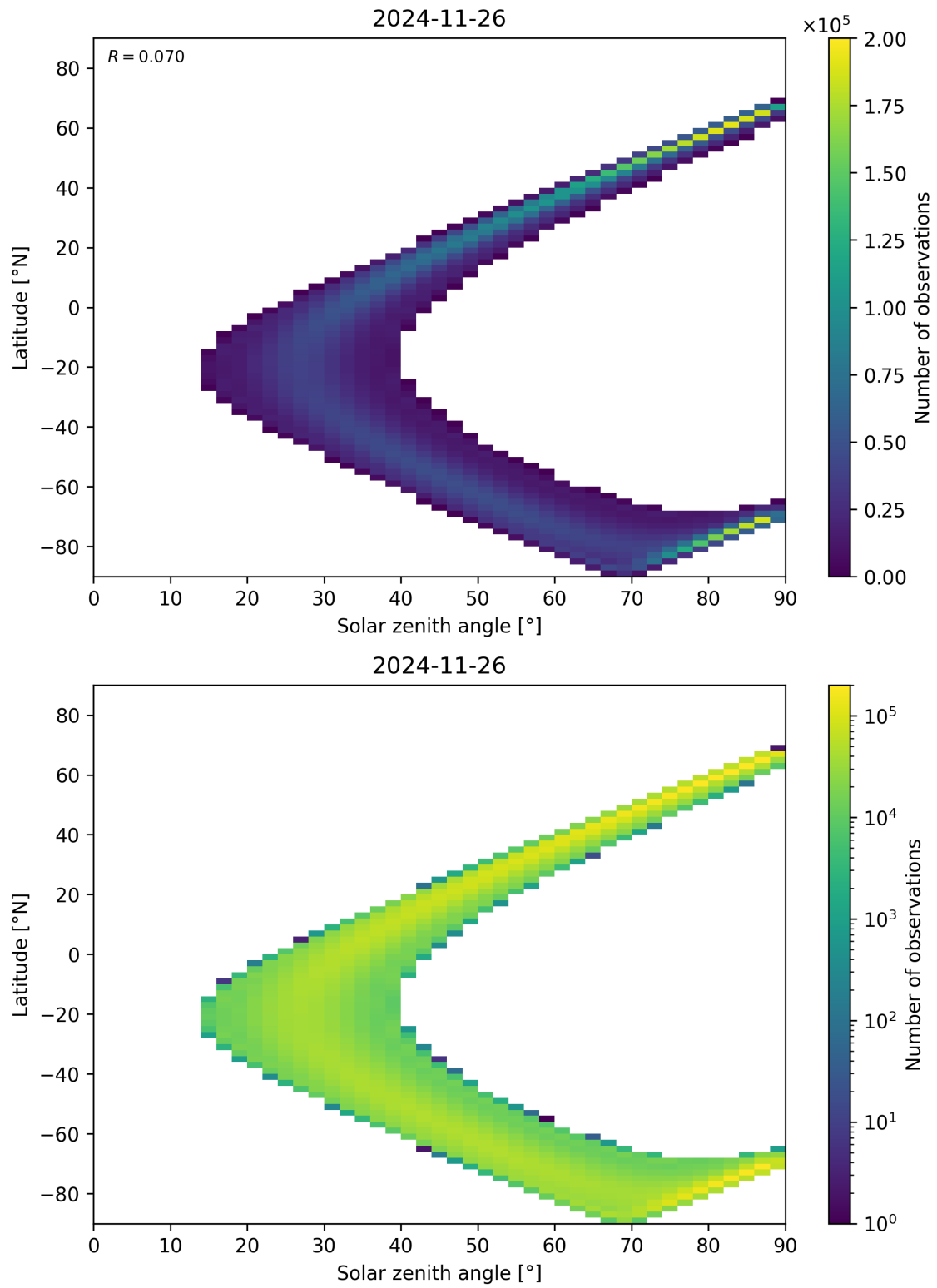
Figure 44: Scatter density plot of “Solar zenith angle” against “Latitude” for 2024-11-25 to 2024-11-27.
