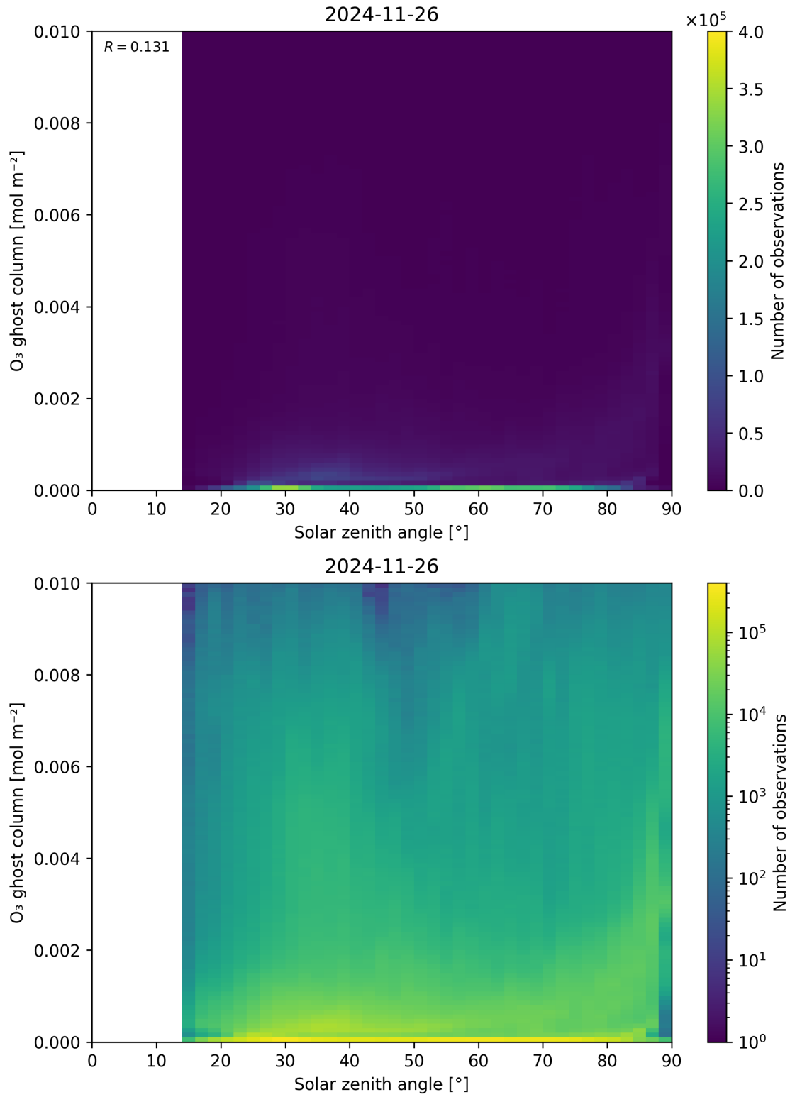
Figure 46: Scatter density plot of “Solar zenith angle” against “O 3 ghost column” for 2024-11-25 to 2024-11-27.
