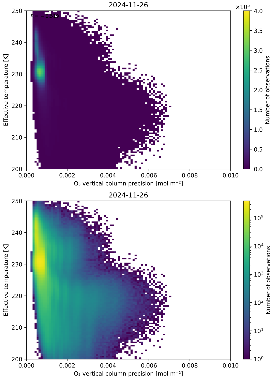
Figure 42: Scatter density plot of “O 3 vertical column precision” against “Effective temperature” for 2024-11-25 to 2024-11-27.
