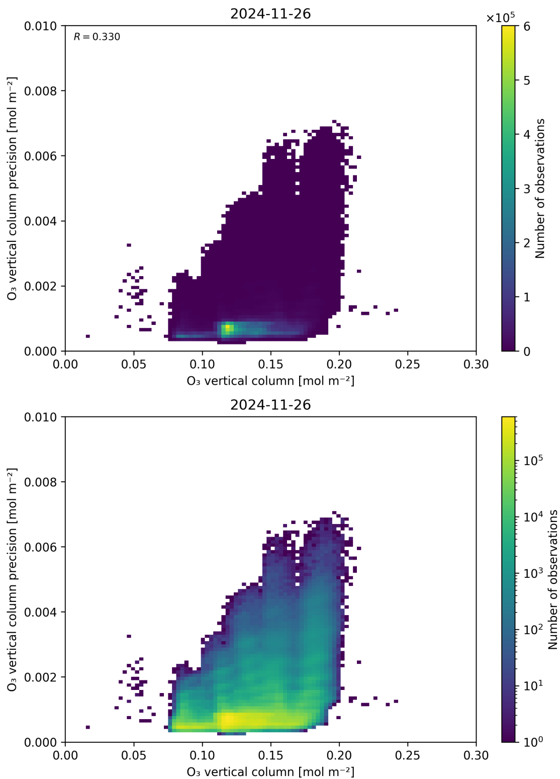
Figure 41: Scatter density plot of “O 3 vertical column” against “O 3 vertical column precision” for 2024-11-25 to 2024-11-27.
