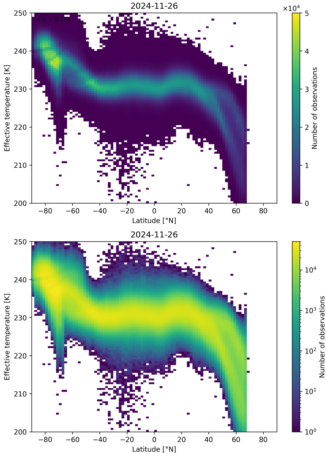
Figure 34: Scatter density plot of “Latitude” against “Effective temperature” for 2024-11-25 to 2024-11-27.
