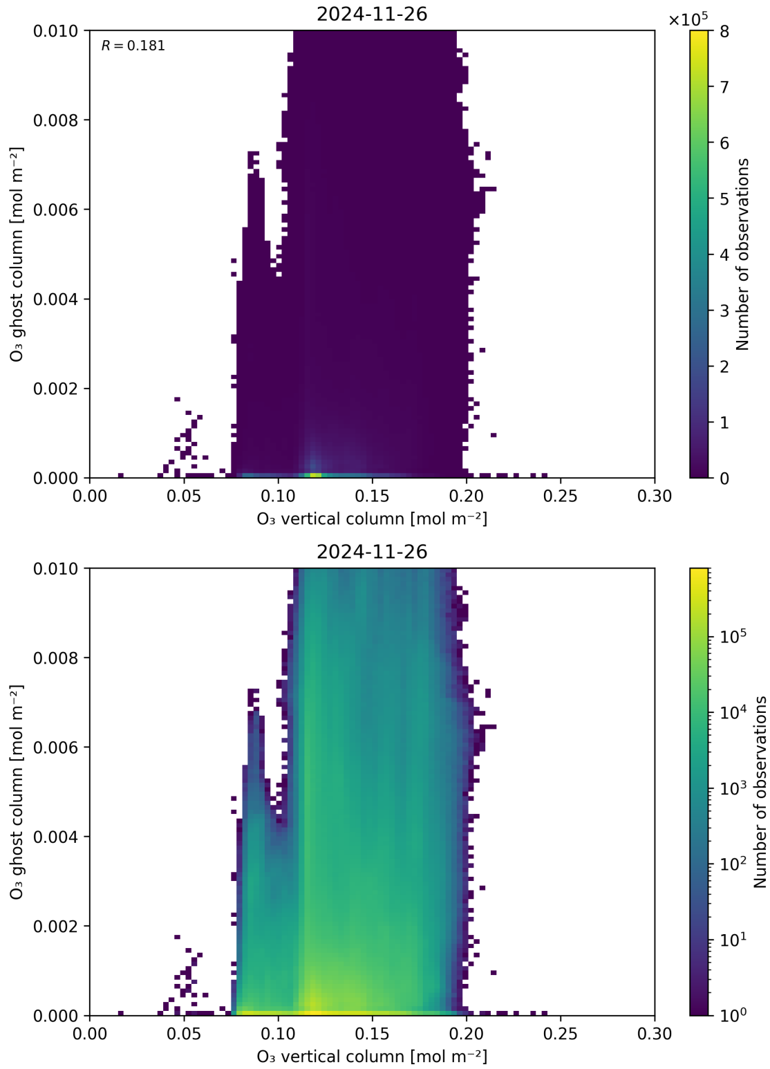
Figure 40: Scatter density plot of “O 3 vertical column” against “O 3 ghost column” for 2024-11-25 to 2024-11-27.
