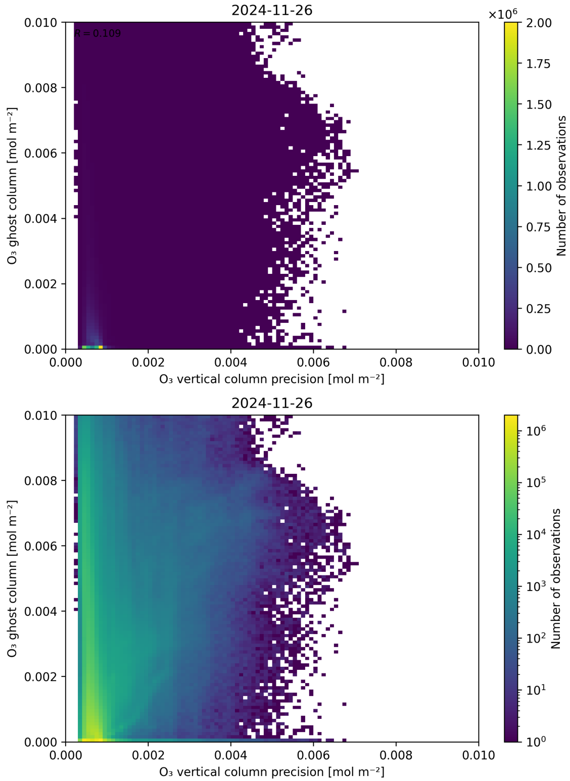
Figure 43: Scatter density plot of “ \text{O}_3 vertical column precision” against “ \text{O}_3 ghost column” for 2024-11-25 to 2024-11-27.
