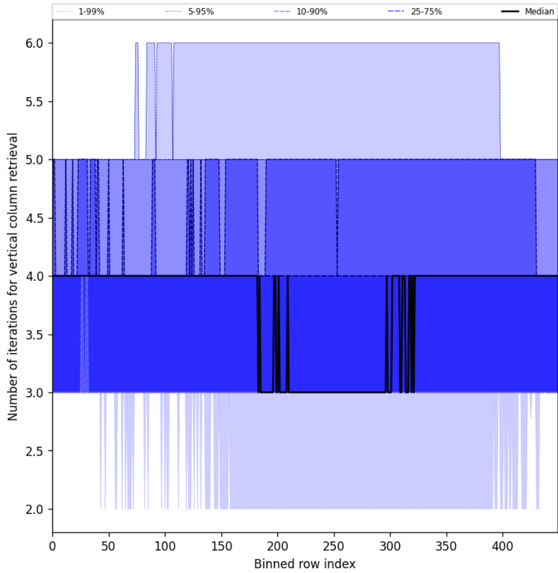
Figure 33: Along track statistics of “Number of iterations for vertical column retrieval” for 2024-11-25 to 2024-11-27
