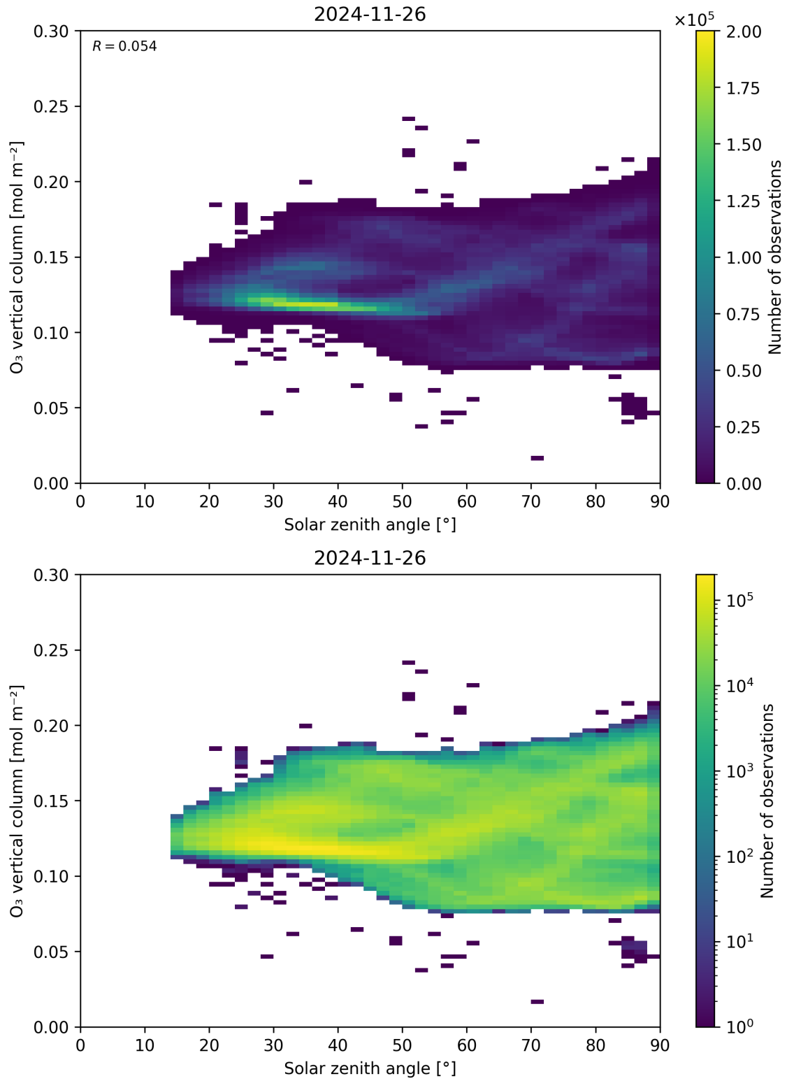
Figure 47: Scatter density plot of “Solar zenith angle” against “O 3 vertical column” for 2024-11-25 to 2024-11-27.
