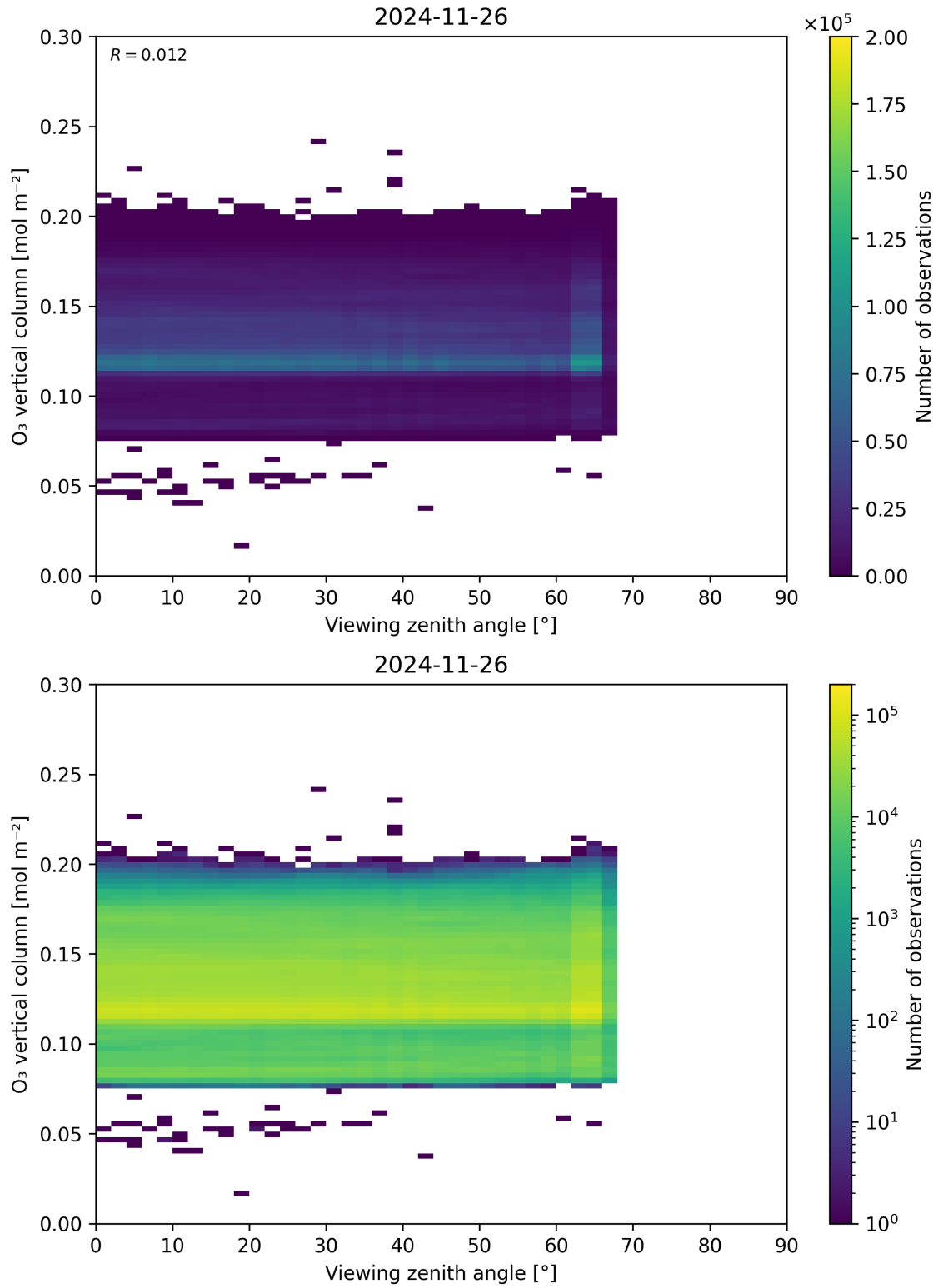
Figure 52: Scatter density plot of “Viewing zenith angle” against “O 3 vertical column” for 2024-11-25 to 2024-11-27.
