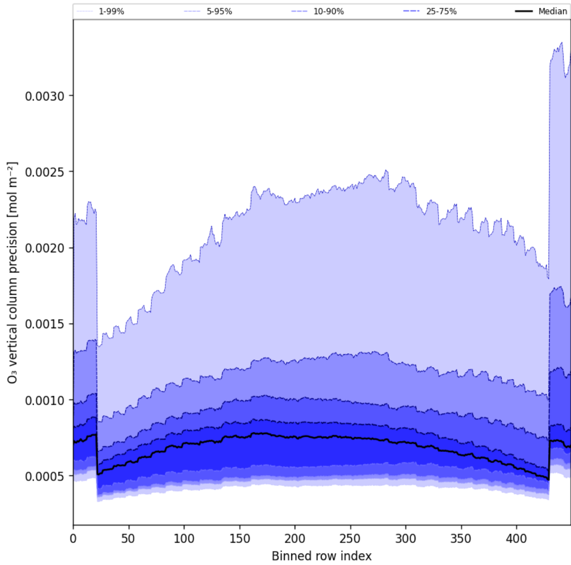
Figure 29: Along track statistics of “O 3 vertical column precision” for 2024-11-25 to 2024-11-27
