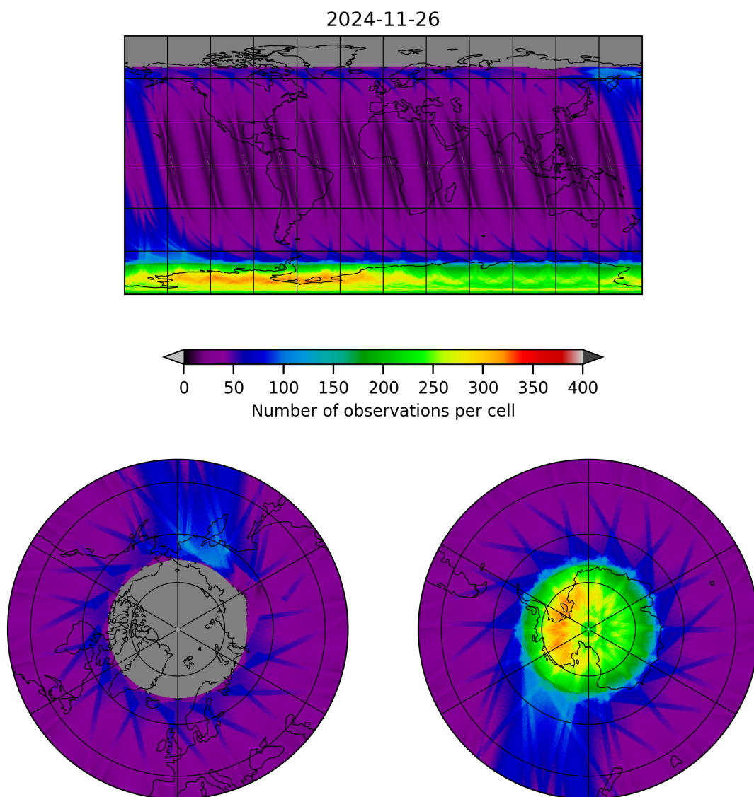
Figure 12: Map of the number of observations for 2024-11-25 to 2024-11-27
