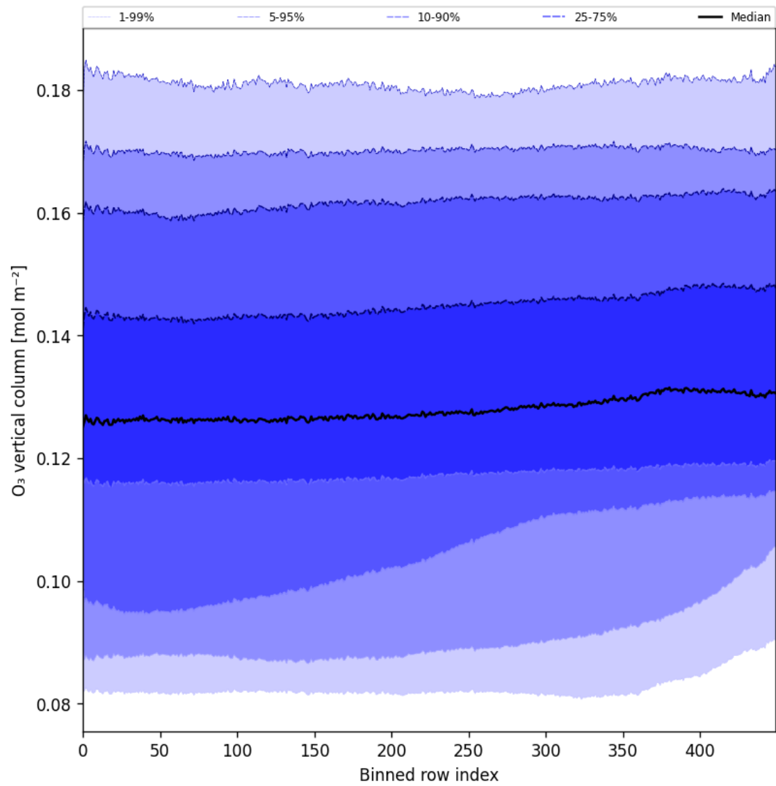
Figure 28: Along track statistics of “O 3 vertical column” for 2024-11-25 to 2024-11-27
