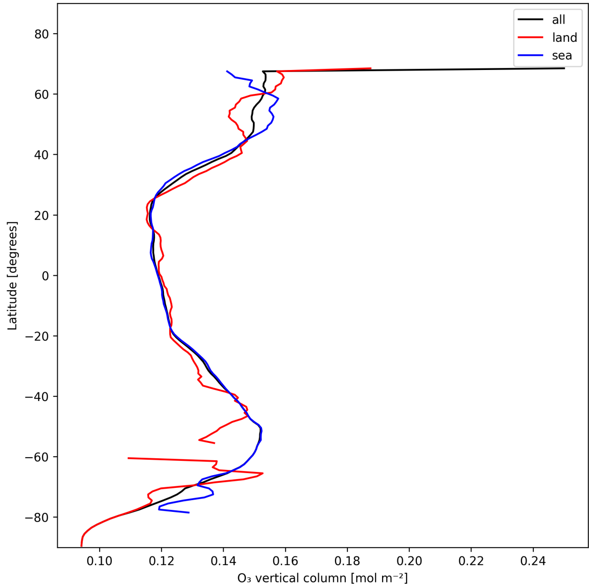
Figure 14: Zonal average of “O 3 vertical column” for 2024-11-25 to 2024-11-27.
