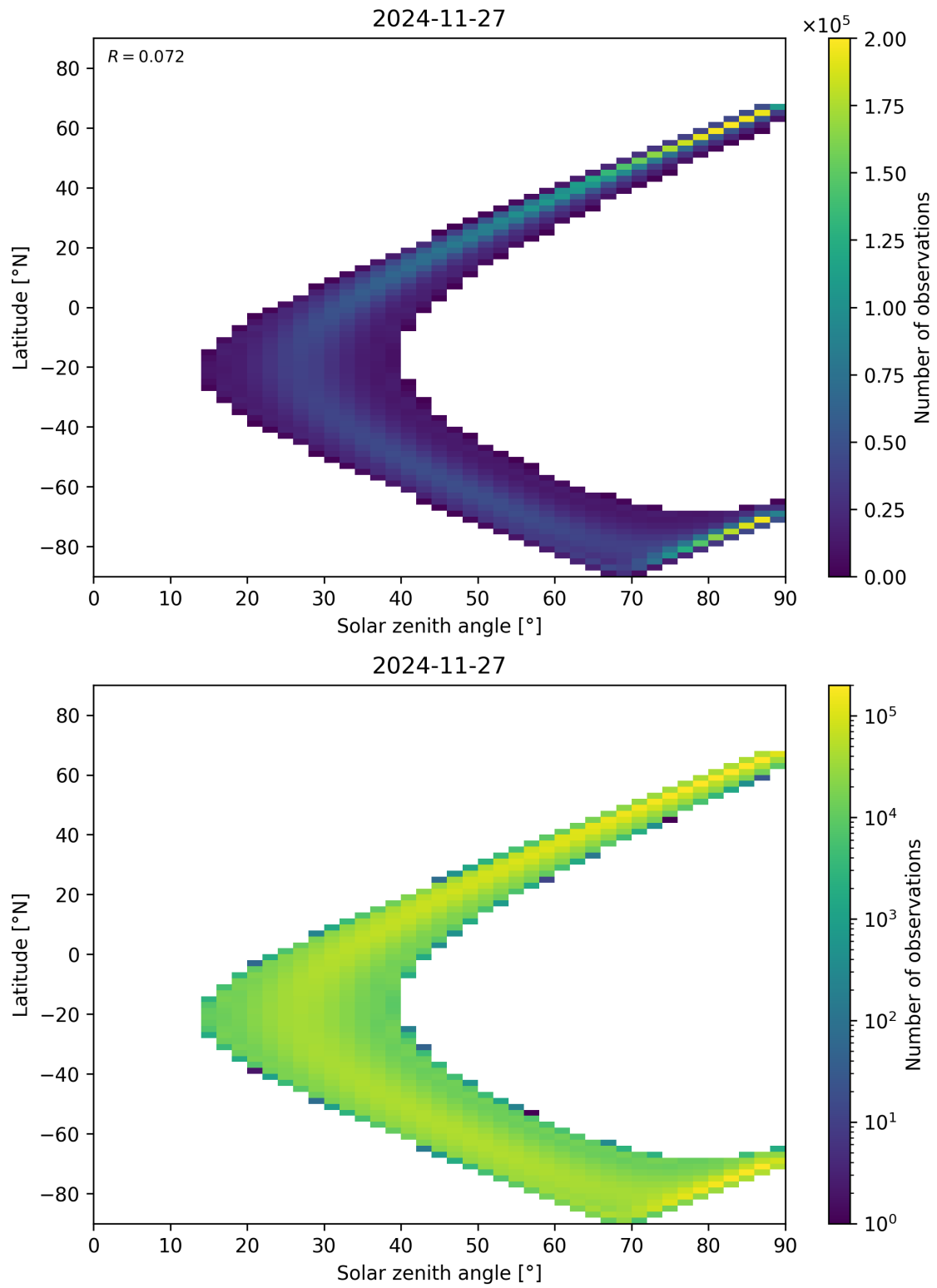
Figure 44: Scatter density plot of “Solar zenith angle” against “Latitude” for 2024-11-26 to 2024-11-28.
