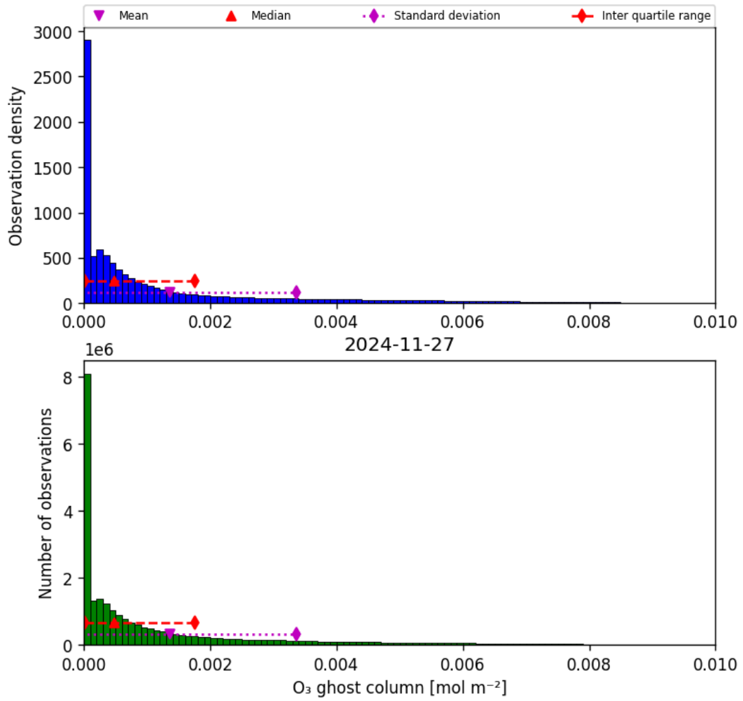
Figure 25: Histogram of “O 3 ghost column” for 2024-11-26 to 2024-11-28
