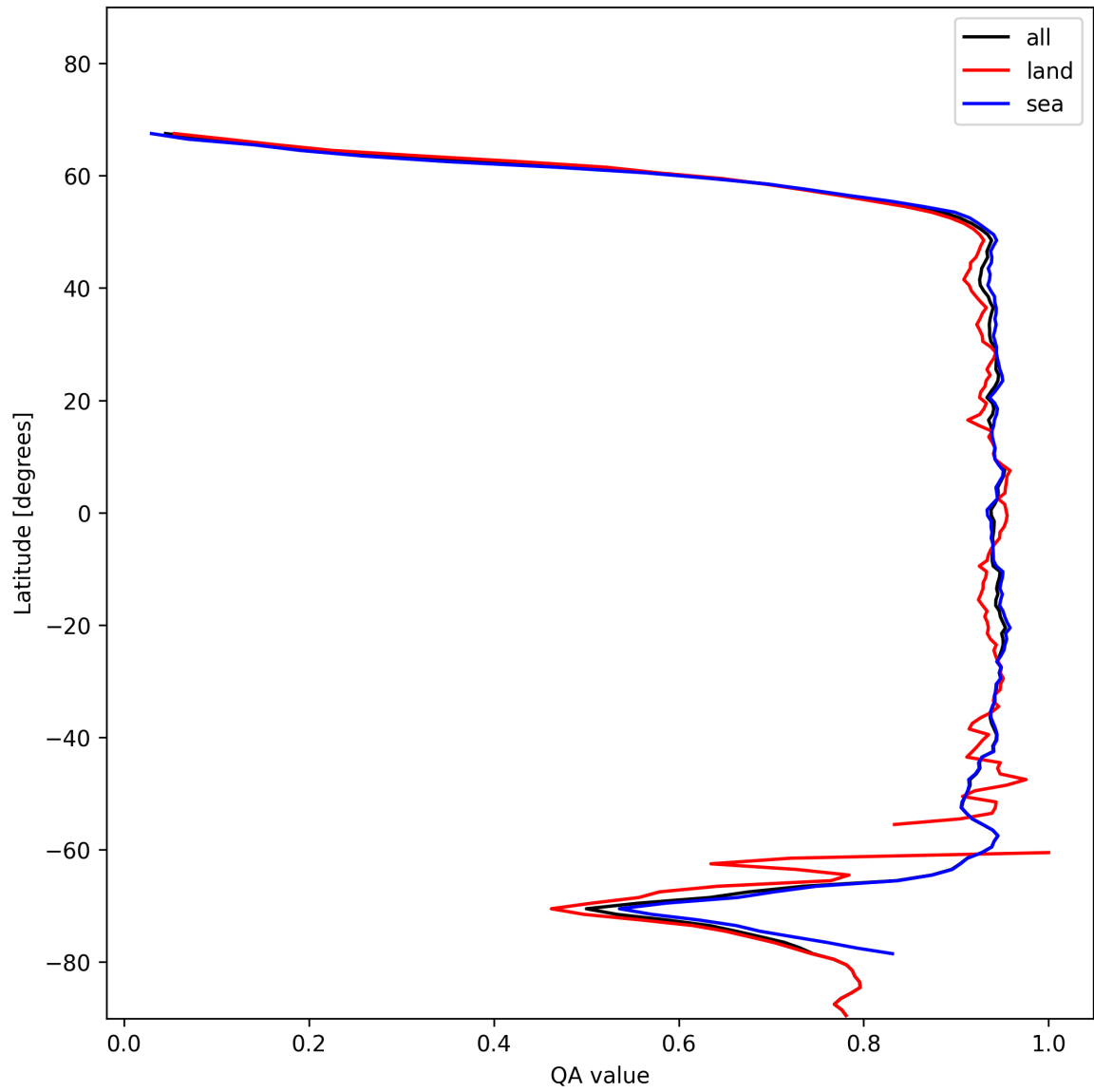
Figure 13: Zonal average of “QA value” for 2024-11-26 to 2024-11-28.
