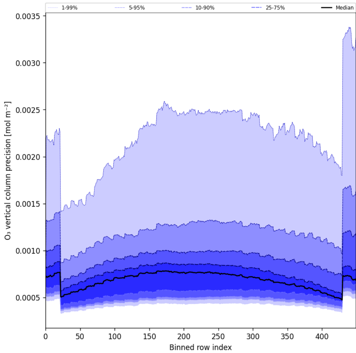
Figure 29: Along track statistics of “O 3 vertical column precision” for 2024-11-26 to 2024-11-28
