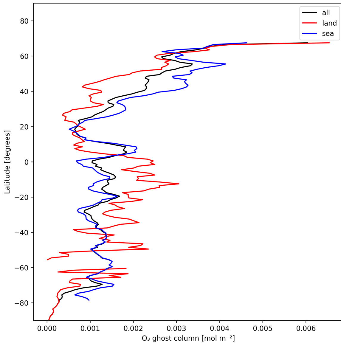
Figure 18: Zonal average of “O 3 ghost column” for 2024-11-26 to 2024-11-28.
