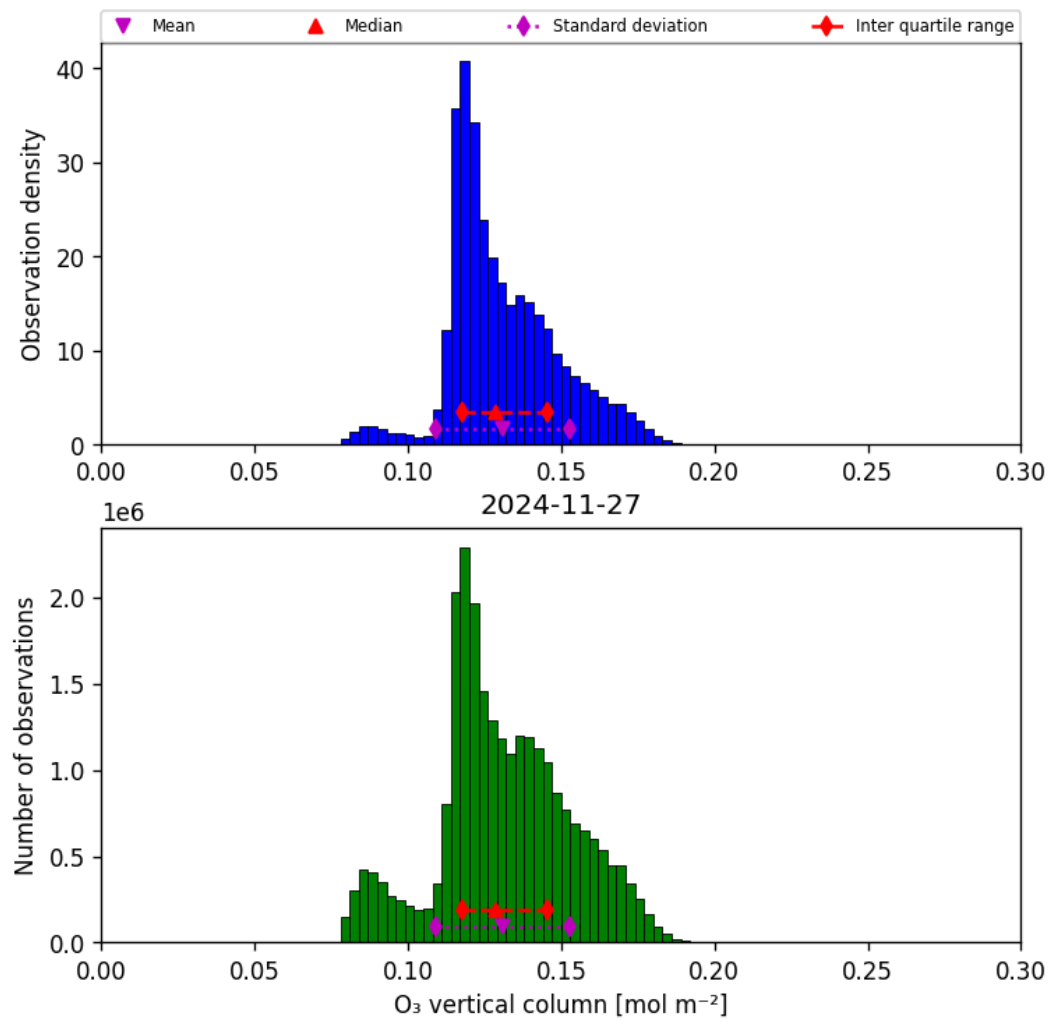
Figure 21: Histogram of “O 3 vertical column” for 2024-11-26 to 2024-11-28
