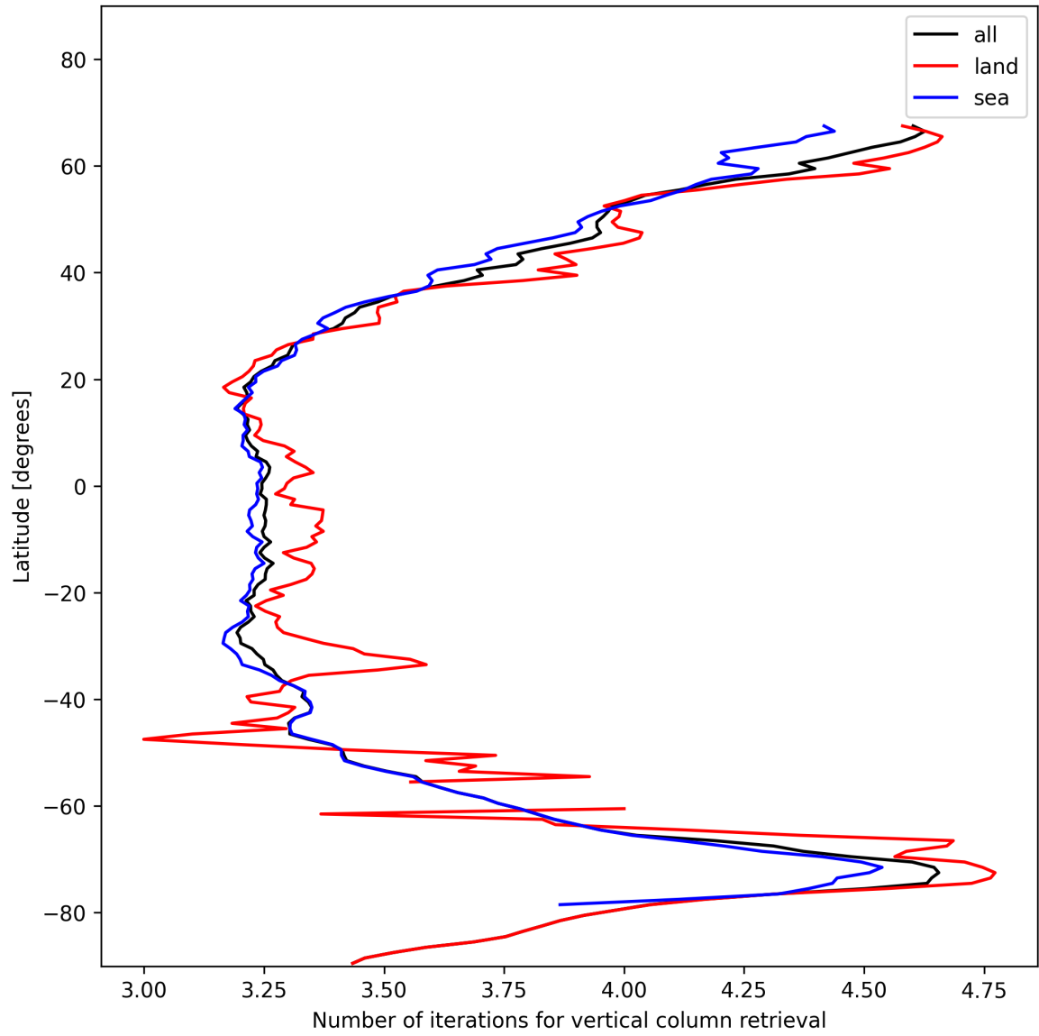
Figure 19: Zonal average of “Number of iterations for vertical column retrieval” for 2024-11-26 to 2024-11-28.
