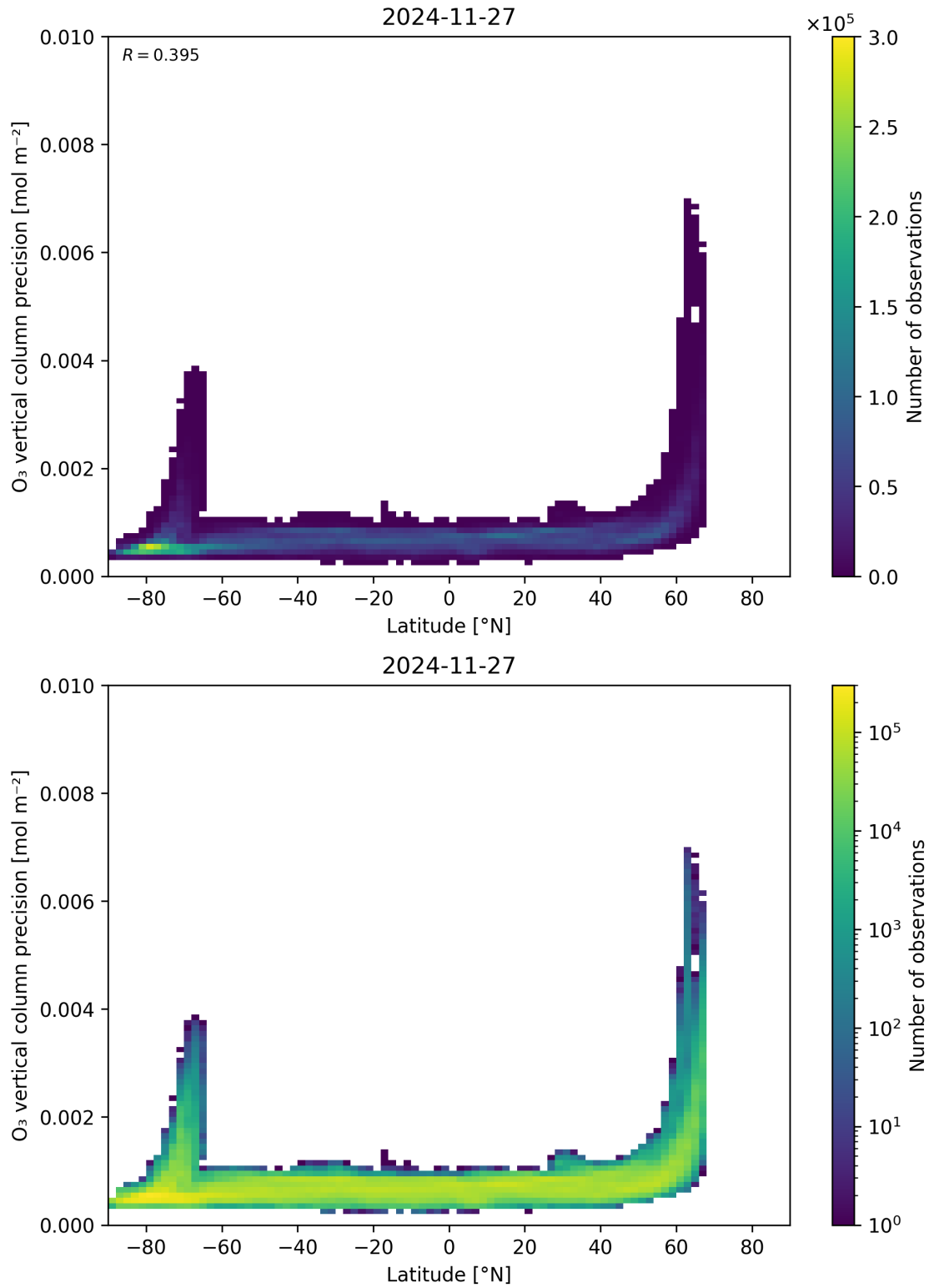
Figure 37: Scatter density plot of “Latitude” against “O 3 vertical column precision” for 2024-11-26 to 2024-11-28.
