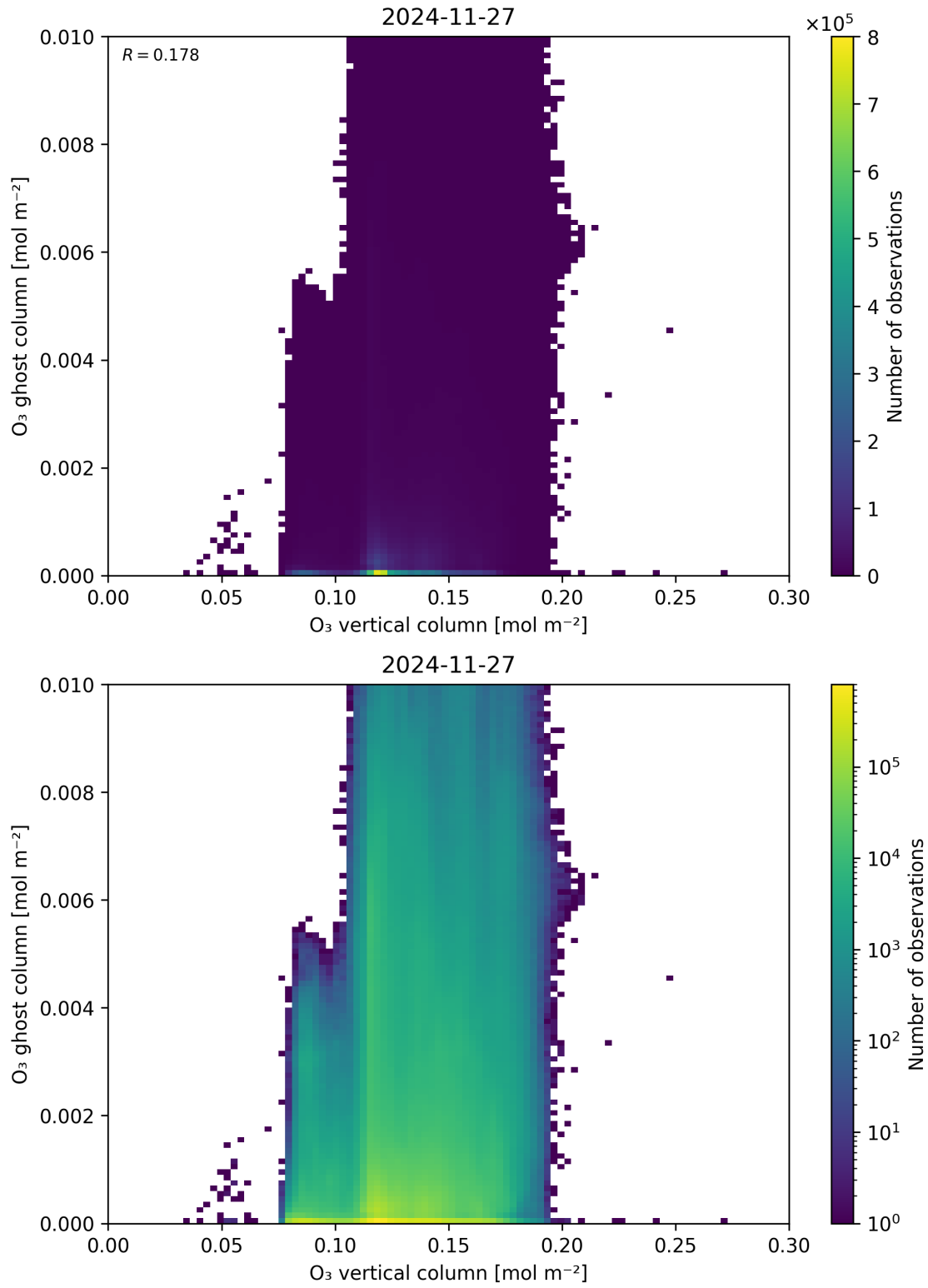
Figure 40: Scatter density plot of “O 3 vertical column” against “O 3 ghost column” for 2024-11-26 to 2024-11-28.
