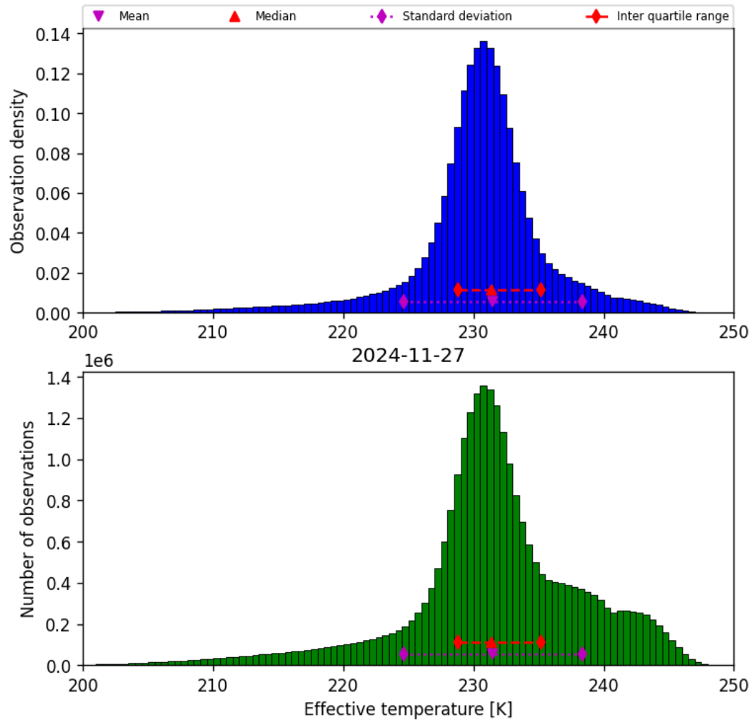
Figure 24: Histogram of “Effective temperature” for 2024-11-26 to 2024-11-28
