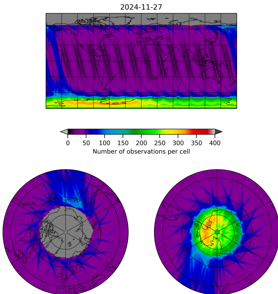
Figure 12: Map of the number of observations for 2024-11-26 to 2024-11-28
