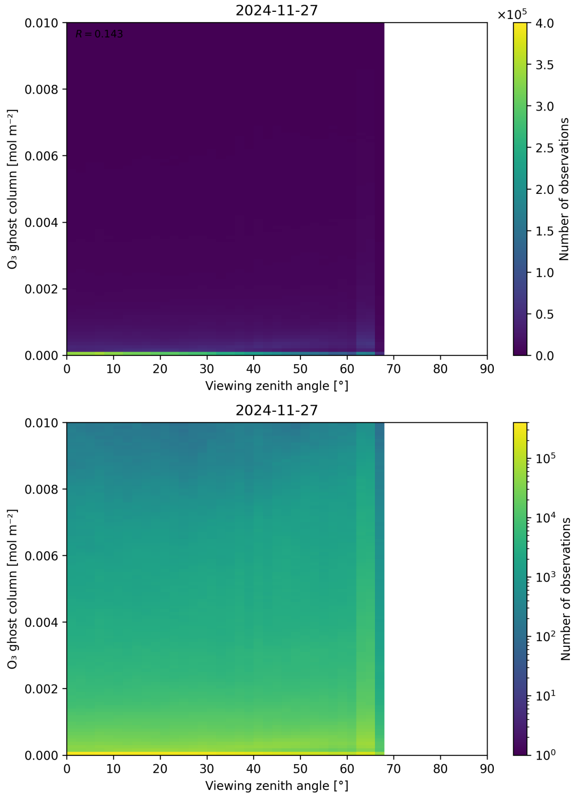
Figure 51: Scatter density plot of “Viewing zenith angle” against “O 3 ghost column” for 2024-11-26 to 2024-11-28.
