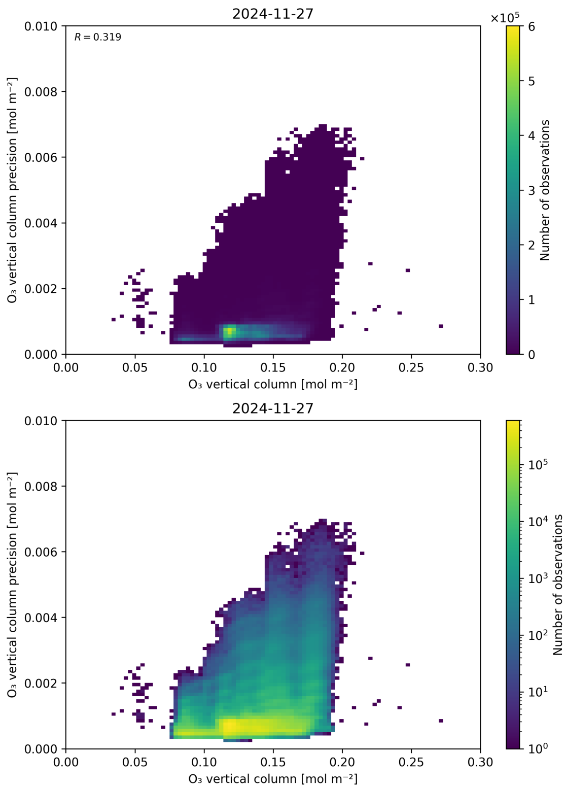
Figure 41: Scatter density plot of “O 3 vertical column” against “O 3 vertical column precision” for 2024-11-26 to 2024-11-28.
