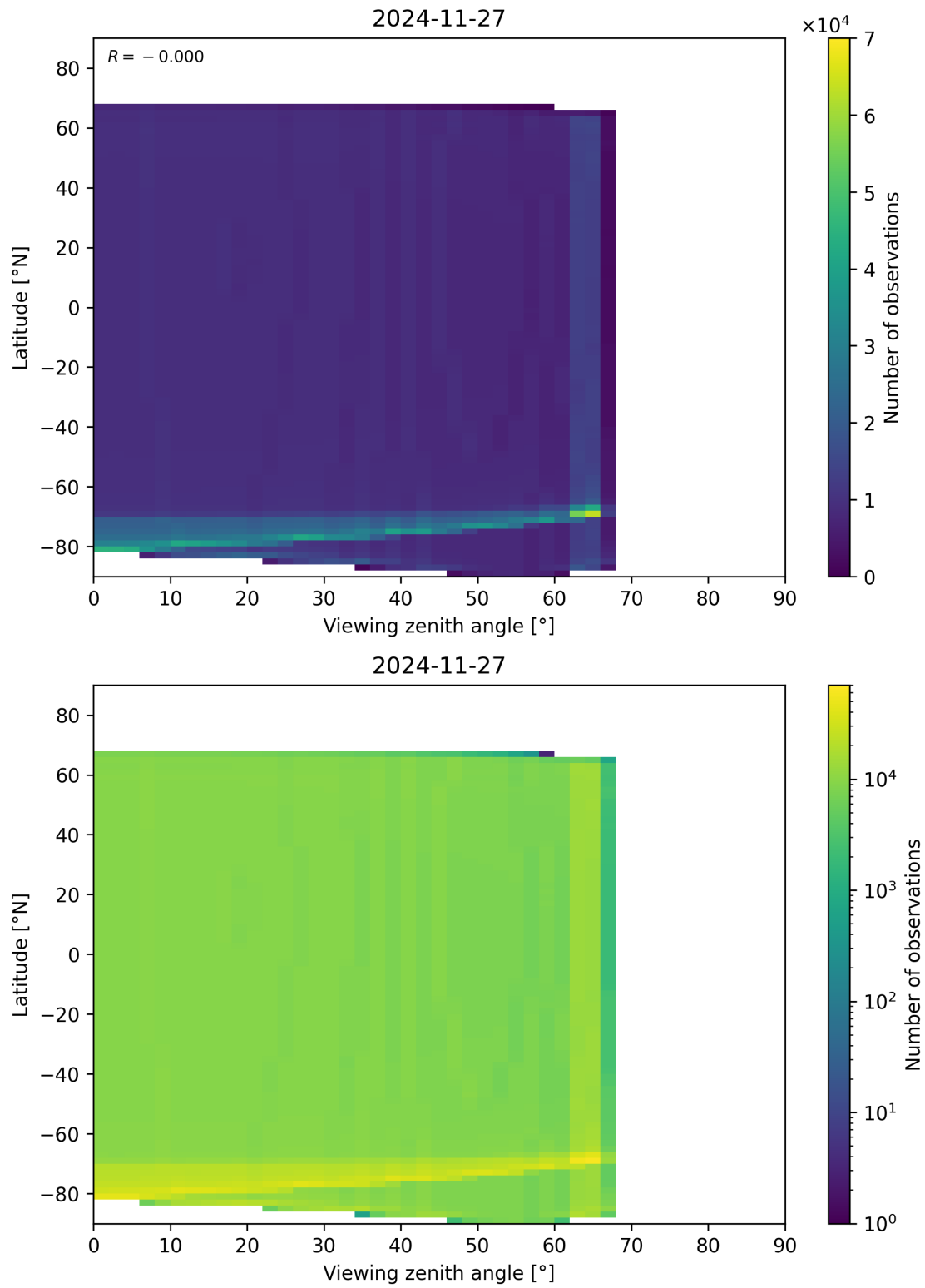
Figure 49: Scatter density plot of “Viewing zenith angle” against “Latitude” for 2024-11-26 to 2024-11-28.
