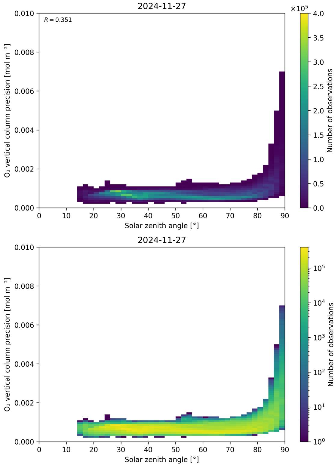
Figure 48: Scatter density plot of “Solar zenith angle” against “O 3 vertical column precision” for 2024-11-26 to 2024-11-28.
