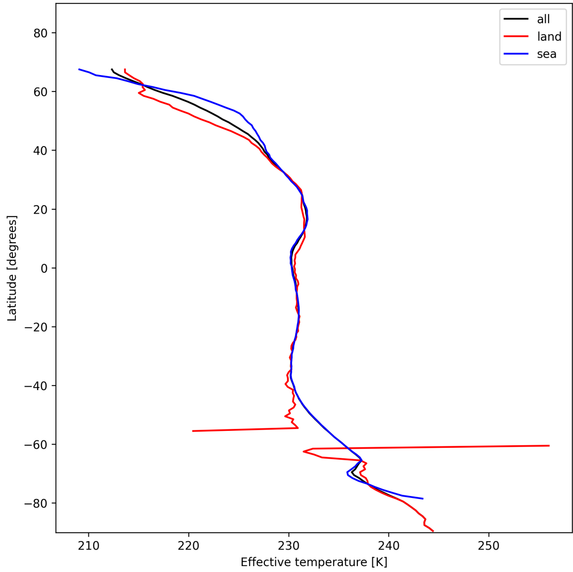
Figure 17: Zonal average of “Effective temperature” for 2024-11-26 to 2024-11-28.
