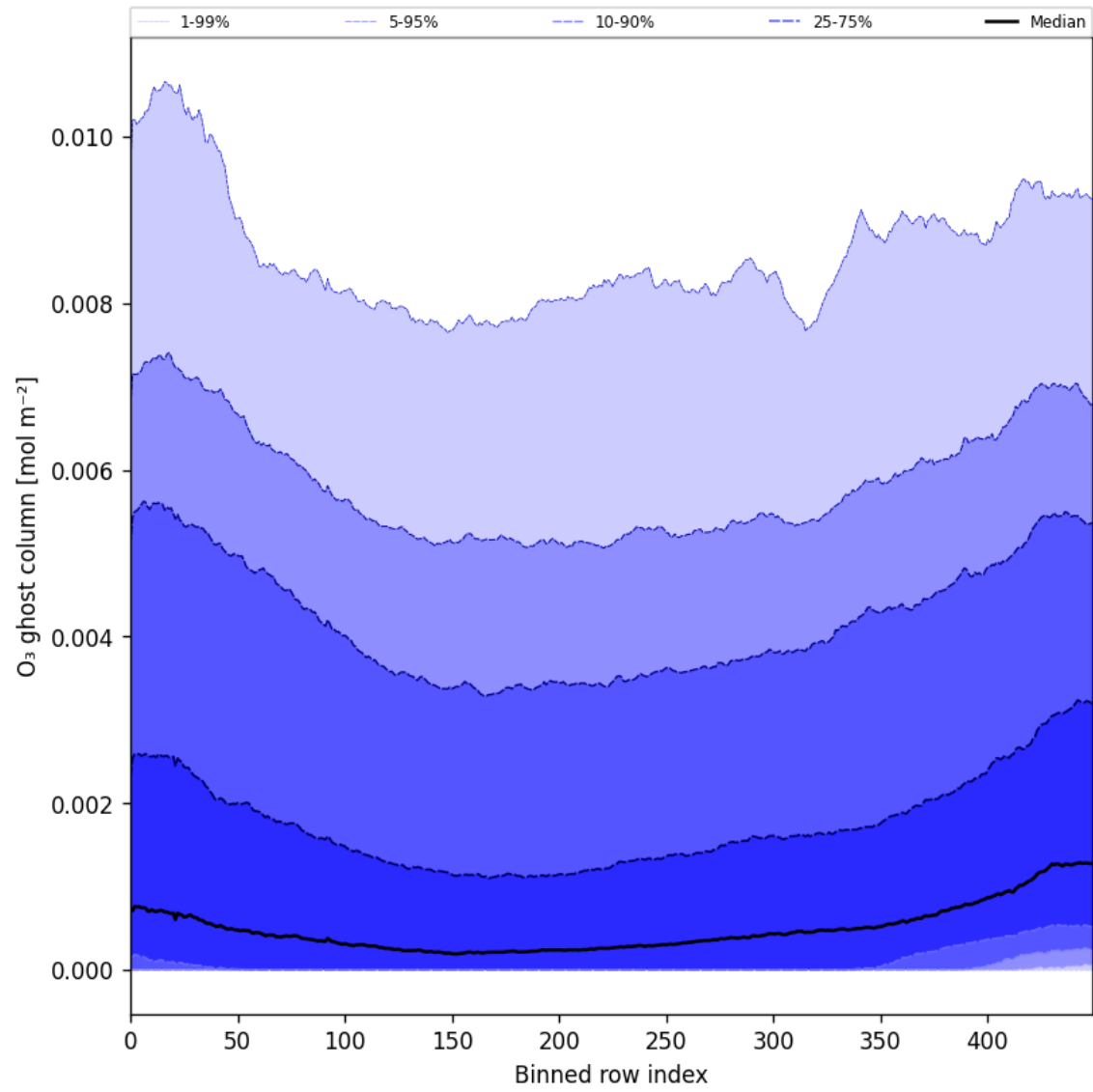
Figure 32: Along track statistics of “O 3 ghost column” for 2024-11-26 to 2024-11-28
