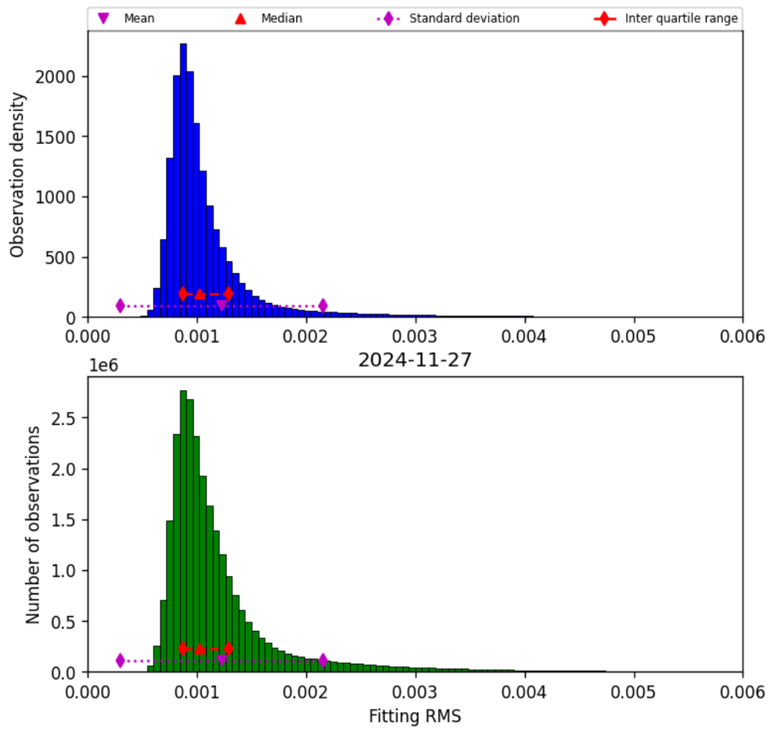
Figure 23: Histogram of “Fitting RMS” for 2024-11-26 to 2024-11-28
