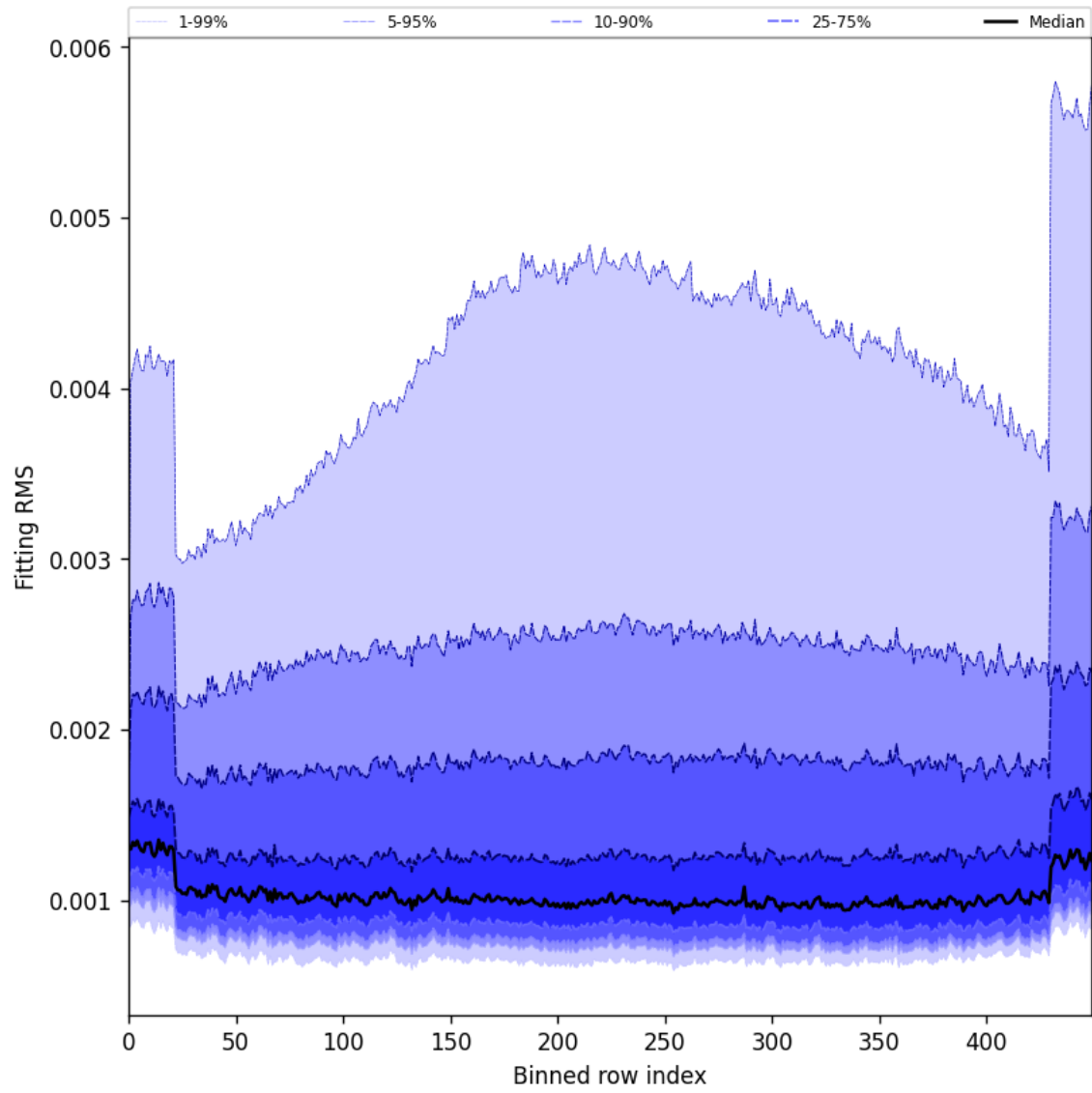
Figure 30: Along track statistics of “Fitting RMS” for 2024-11-26 to 2024-11-28
