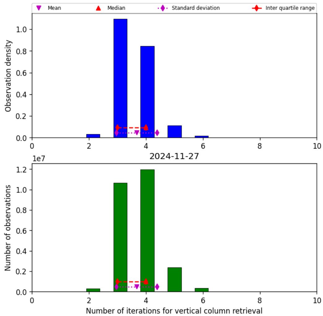
Figure 26: Histogram of “Number of iterations for vertical column retrieval” for 2024-11-26 to 2024-11-28
