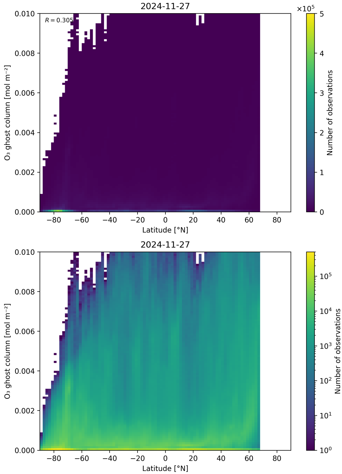
Figure 35: Scatter density plot of “Latitude” against “O 3 ghost column” for 2024-11-26 to 2024-11-28.
