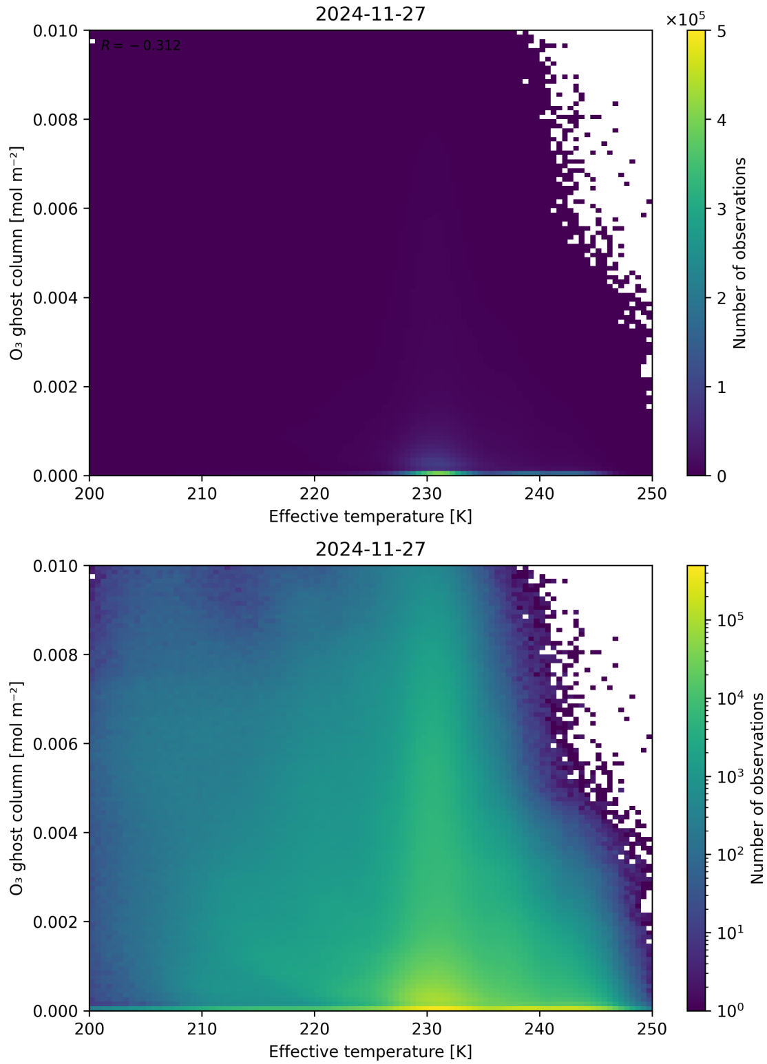
Figure 38: Scatter density plot of “Effective temperature” against “O 3 ghost column” for 2024-11-26 to 2024-11-28.
