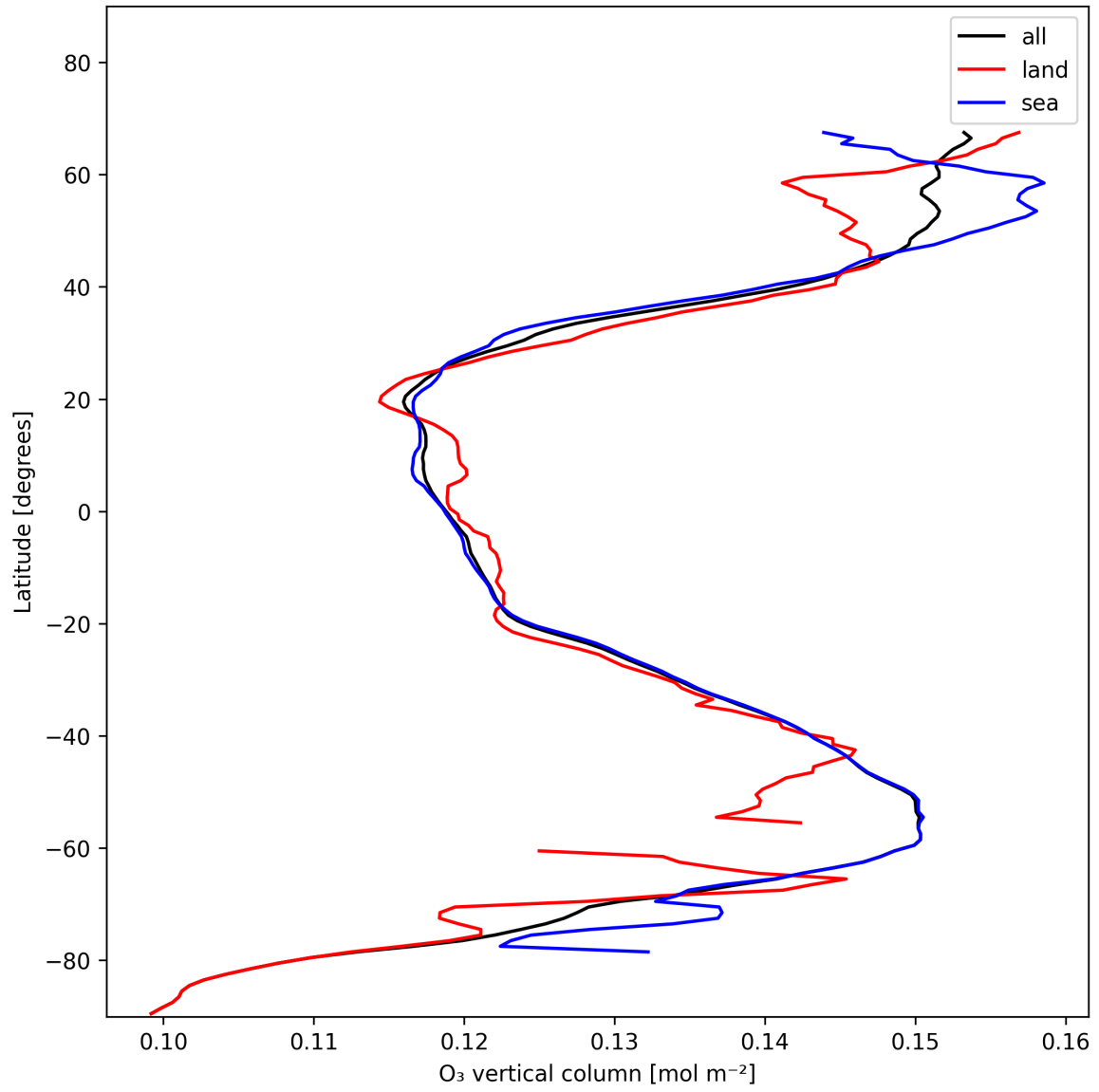
Figure 14: Zonal average of “O 3 vertical column” for 2024-11-26 to 2024-11-28.
