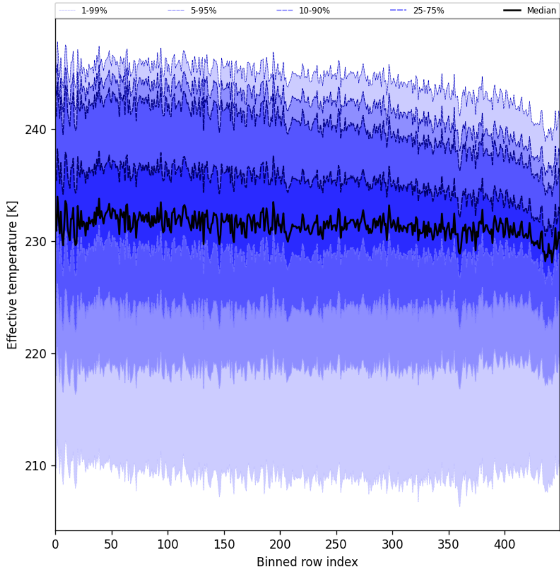
Figure 31: Along track statistics of “Effective temperature” for 2024-11-26 to 2024-11-28
