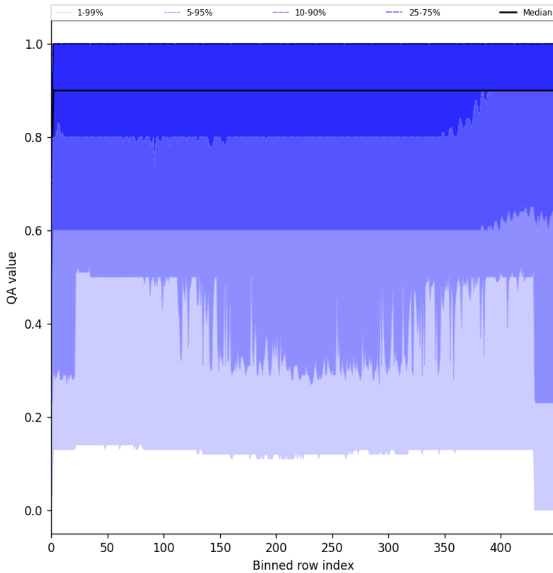
Figure 27: Along track statistics of “QA value” for 2024-11-26 to 2024-11-28
