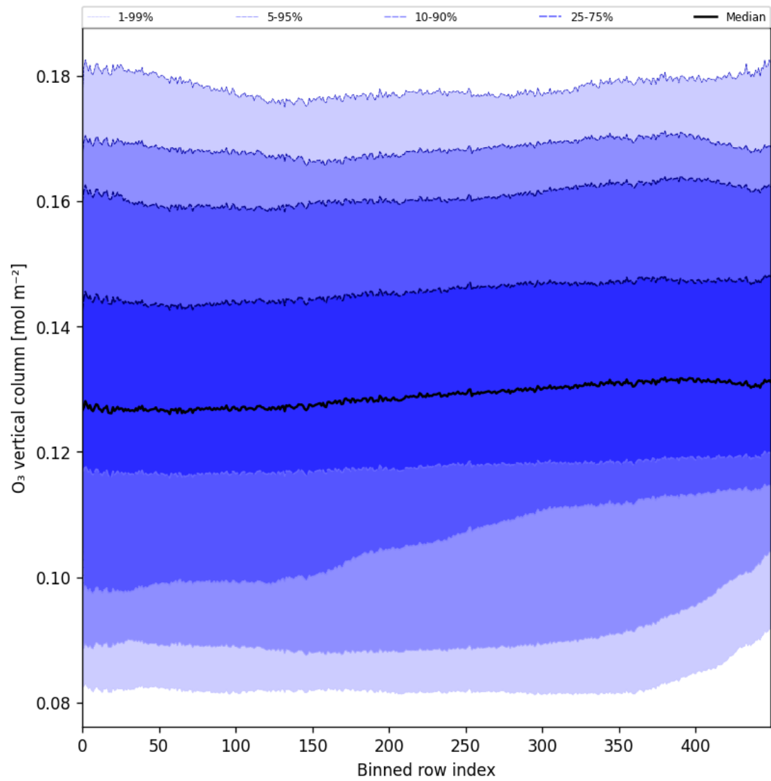
Figure 28: Along track statistics of “O 3 vertical column” for 2024-11-26 to 2024-11-28
