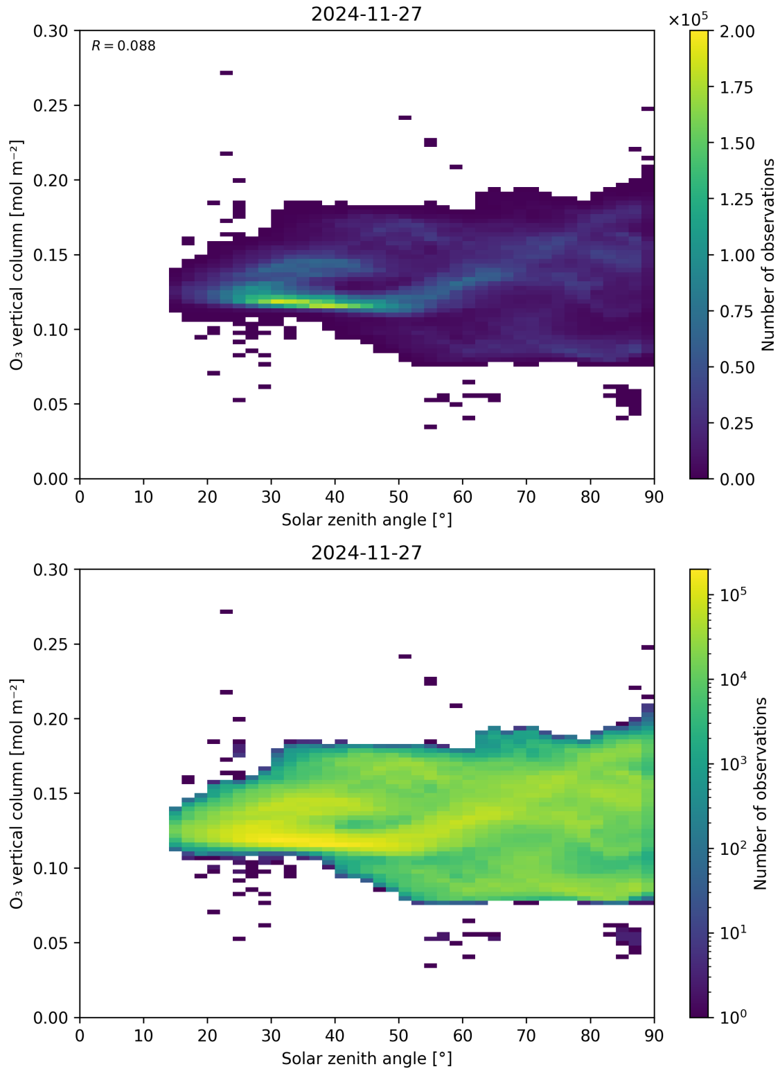
Figure 47: Scatter density plot of “Solar zenith angle” against “O 3 vertical column” for 2024-11-26 to 2024-11-28.
