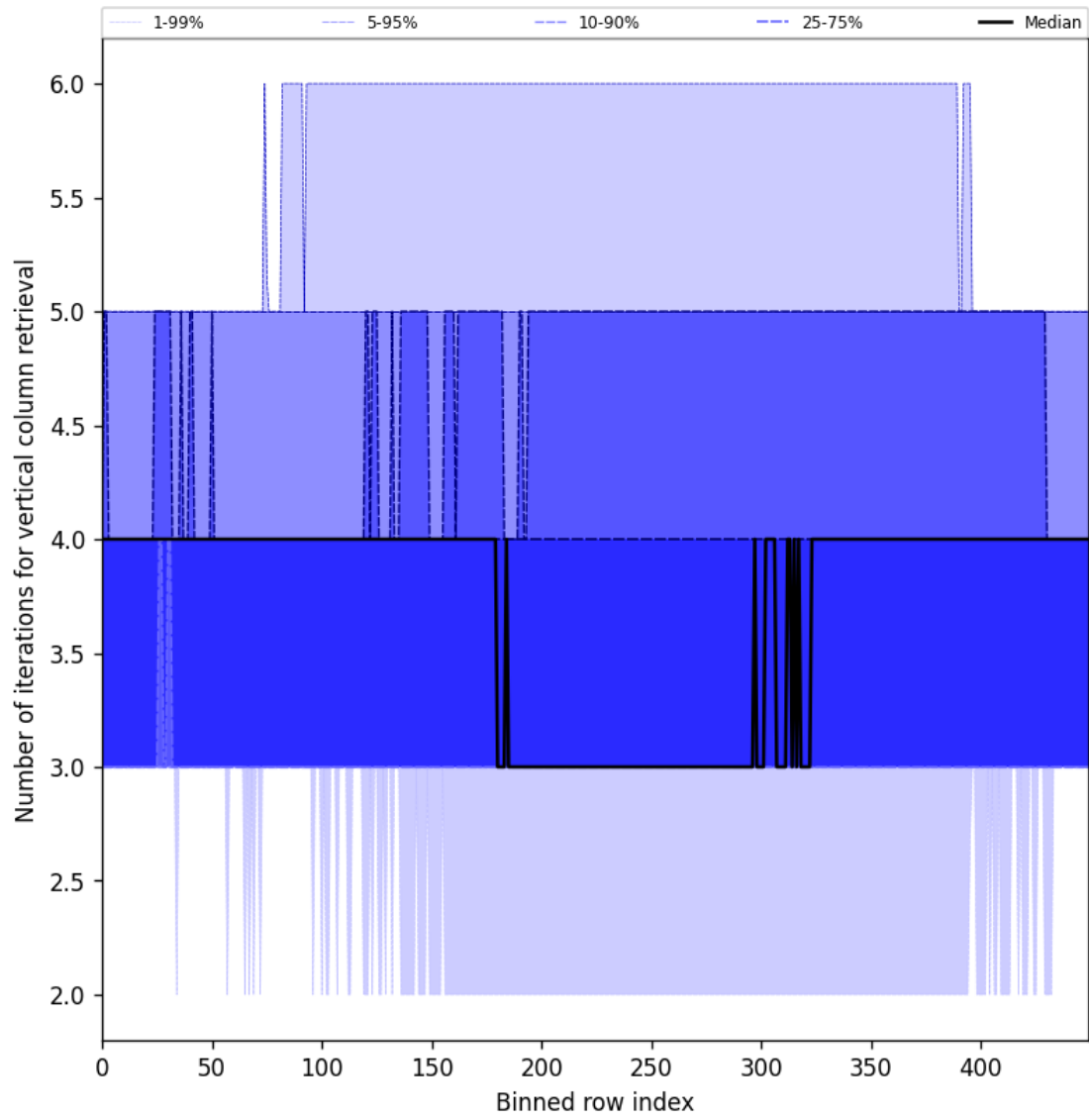
Figure 33: Along track statistics of “Number of iterations for vertical column retrieval” for 2024-11-26 to 2024-11-28
