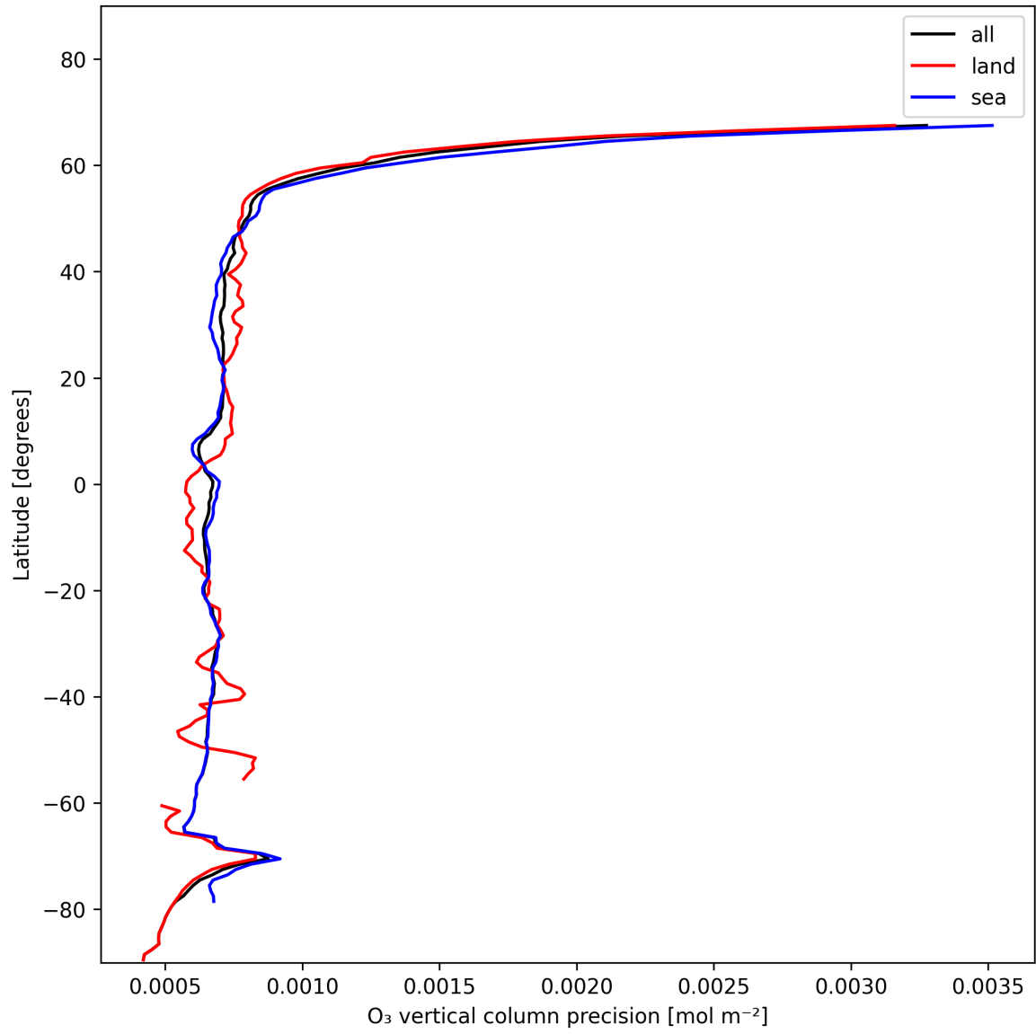
Figure 15: Zonal average of “O 3 vertical column precision” for 2024-11-26 to 2024-11-28.
