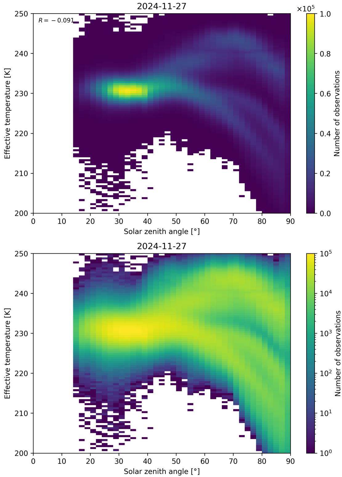
Figure 45: Scatter density plot of “Solar zenith angle” against “Effective temperature” for 2024-11-26 to 2024-11-28.
