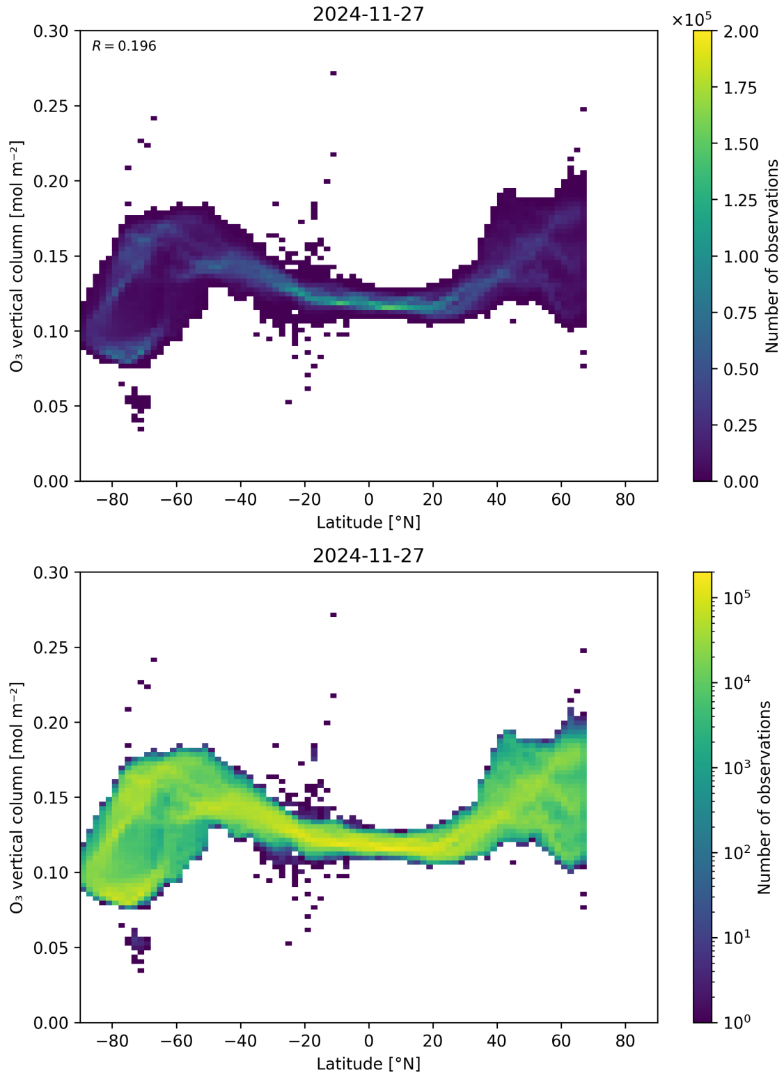
Figure 36: Scatter density plot of “Latitude” against “O 3 vertical column” for 2024-11-26 to 2024-11-28.
