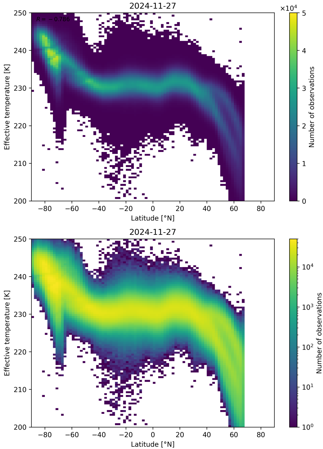
Figure 34: Scatter density plot of “Latitude” against “Effective temperature” for 2024-11-26 to 2024-11-28.
