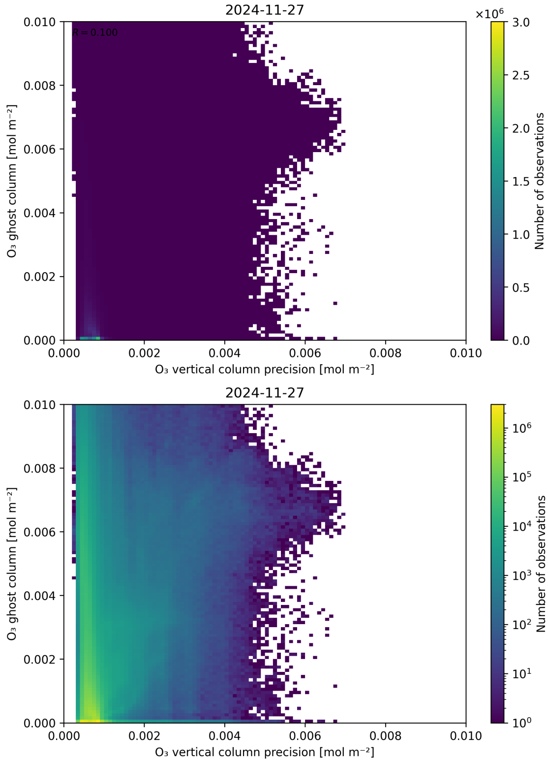
Figure 43: Scatter density plot of “O 3 vertical column precision” against “O 3 ghost column” for 2024-11-26 to 2024-11-28.
