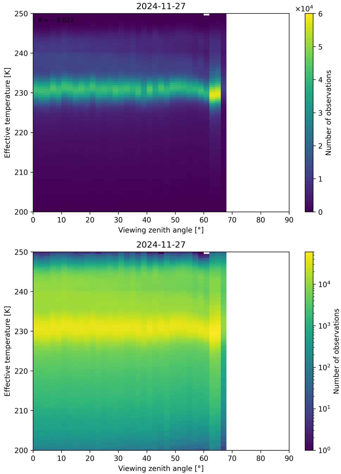
Figure 50: Scatter density plot of “Viewing zenith angle” against “Effective temperature” for 2024-11-26 to 2024-11-28.
