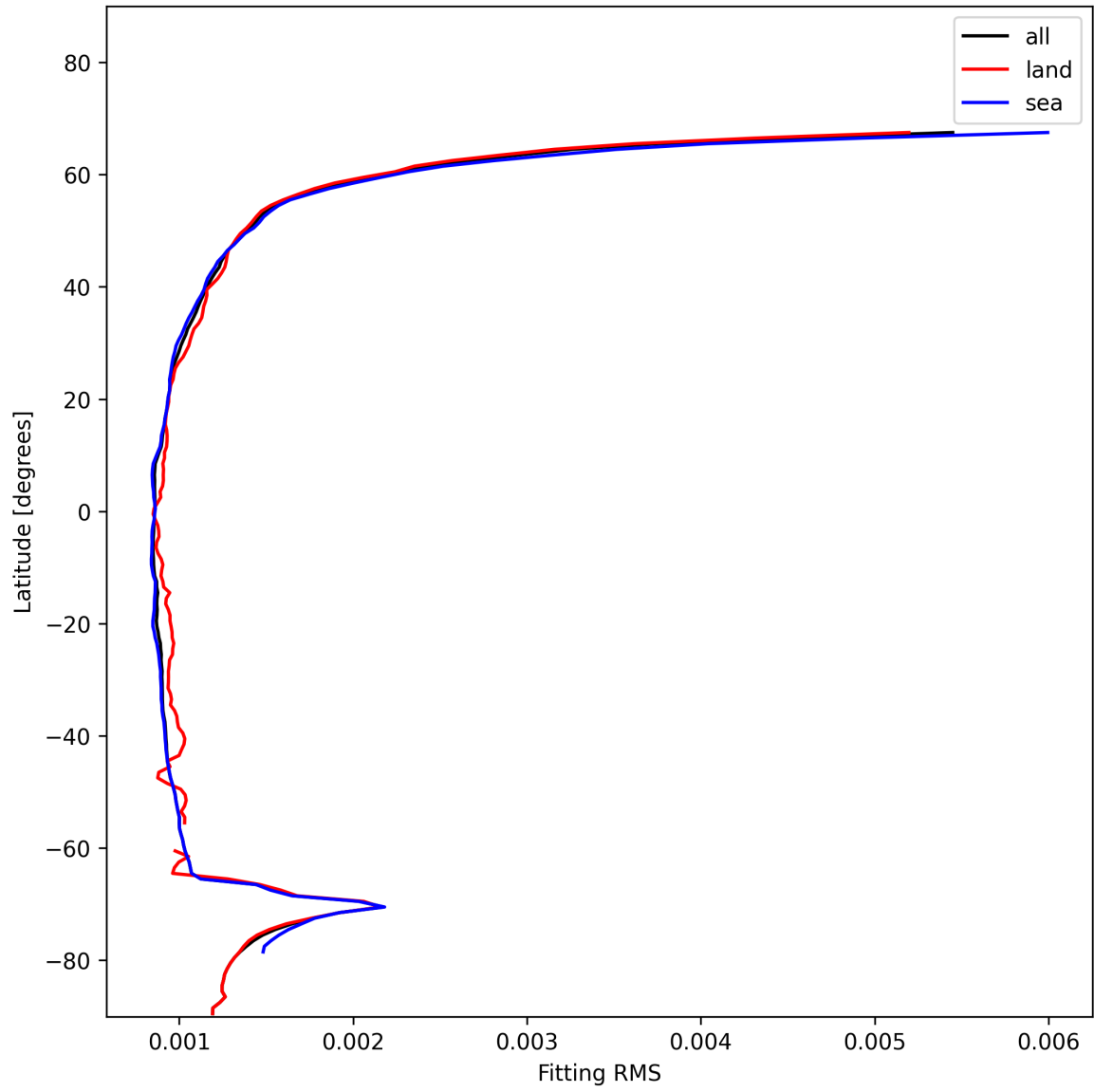
Figure 16: Zonal average of “Fitting RMS” for 2024-11-26 to 2024-11-28.
