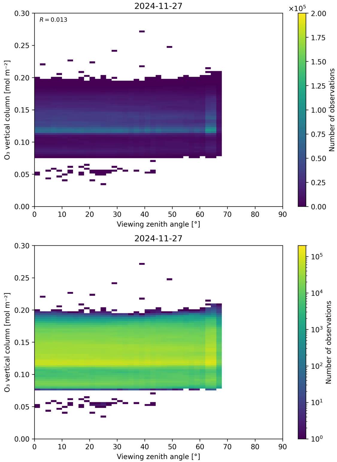
Figure 52: Scatter density plot of “Viewing zenith angle” against “O 3 vertical column” for 2024-11-26 to 2024-11-28.
