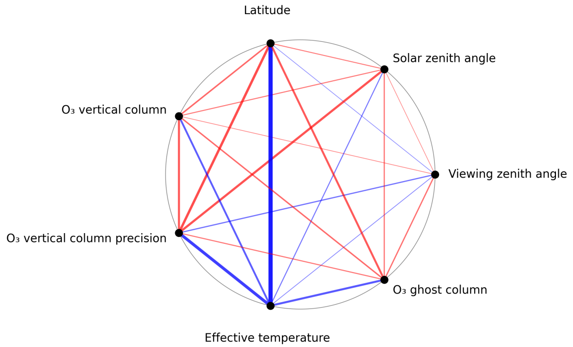
Figure 1: Map of correlation graph for 2024-11-26 to 2024-11-28.
