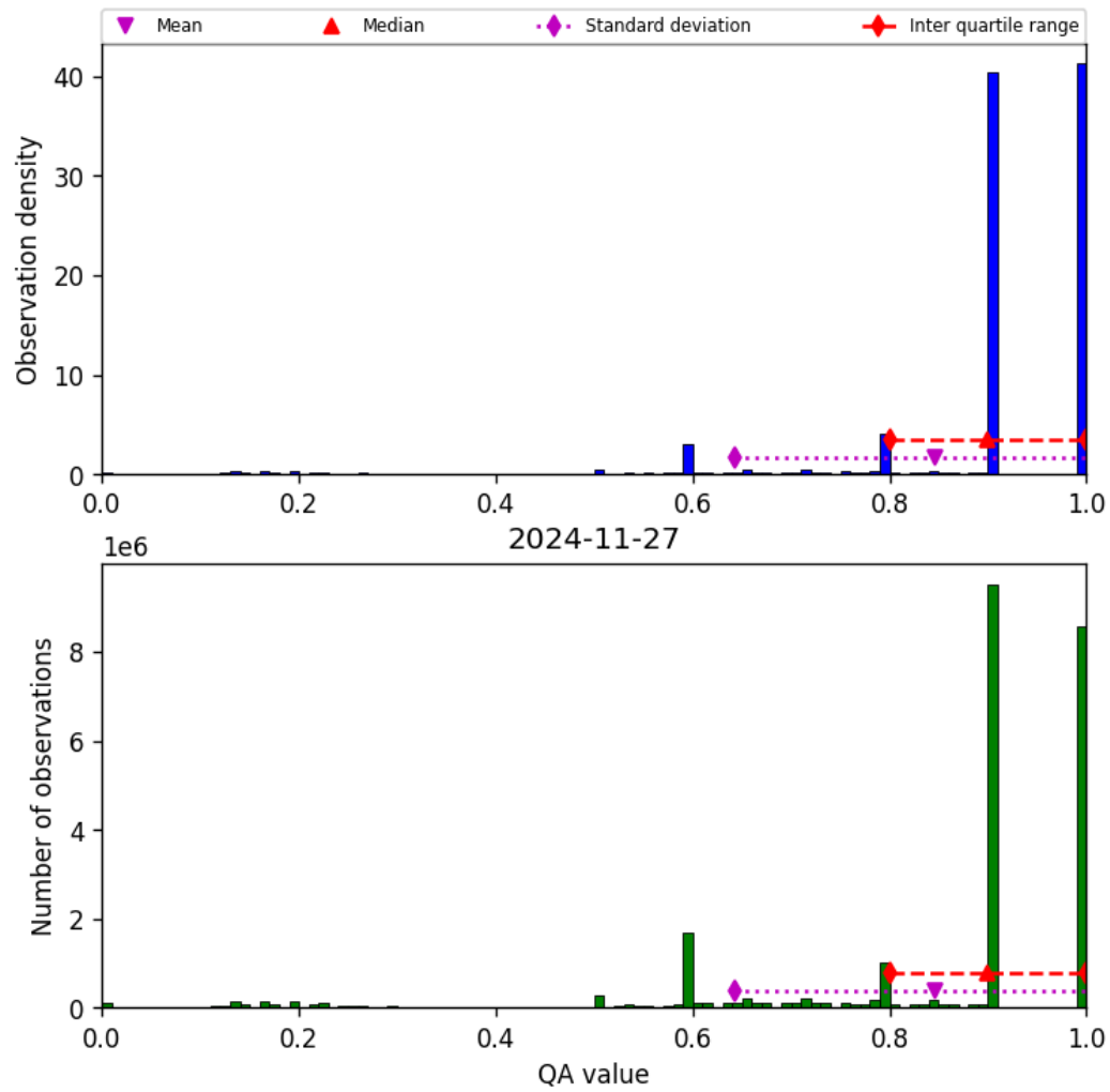
Figure 20: Histogram of “QA value” for 2024-11-26 to 2024-11-28
