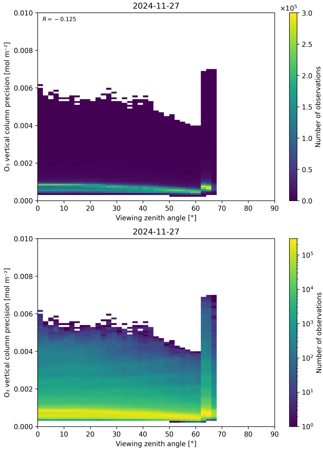
Figure 53: Scatter density plot of “Viewing zenith angle” against “O 3 vertical column precision” for 2024-11-26 to 2024-11-28.
