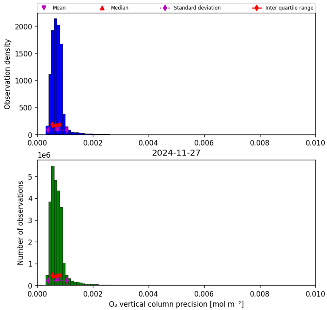
Figure 22: Histogram of “O 3 vertical column precision” for 2024-11-26 to 2024-11-28
