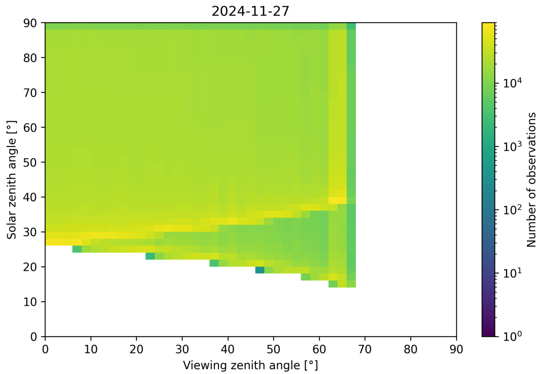
Figure 54: Scatter density plot of “Viewing zenith angle” against “Solar zenith angle” for 2024-11-26 to 2024-11-28.
