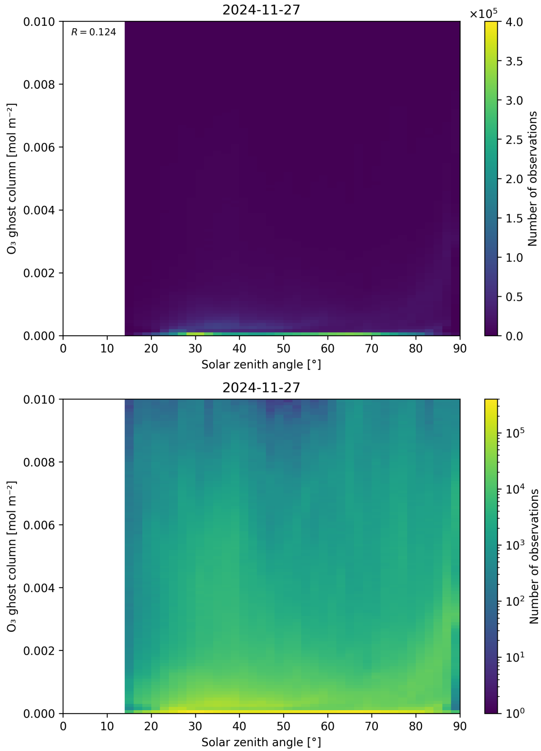
Figure 46: Scatter density plot of “Solar zenith angle” against “O 3 ghost column” for 2024-11-26 to 2024-11-28.
