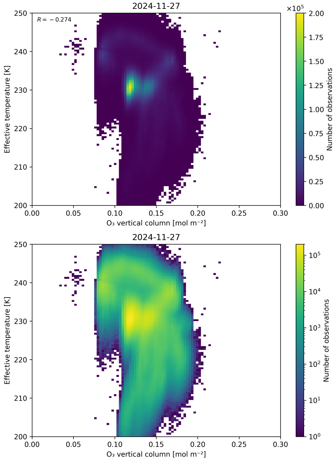
Figure 39: Scatter density plot of “O 3 vertical column” against “Effective temperature” for 2024-11-26 to 2024-11-28.
