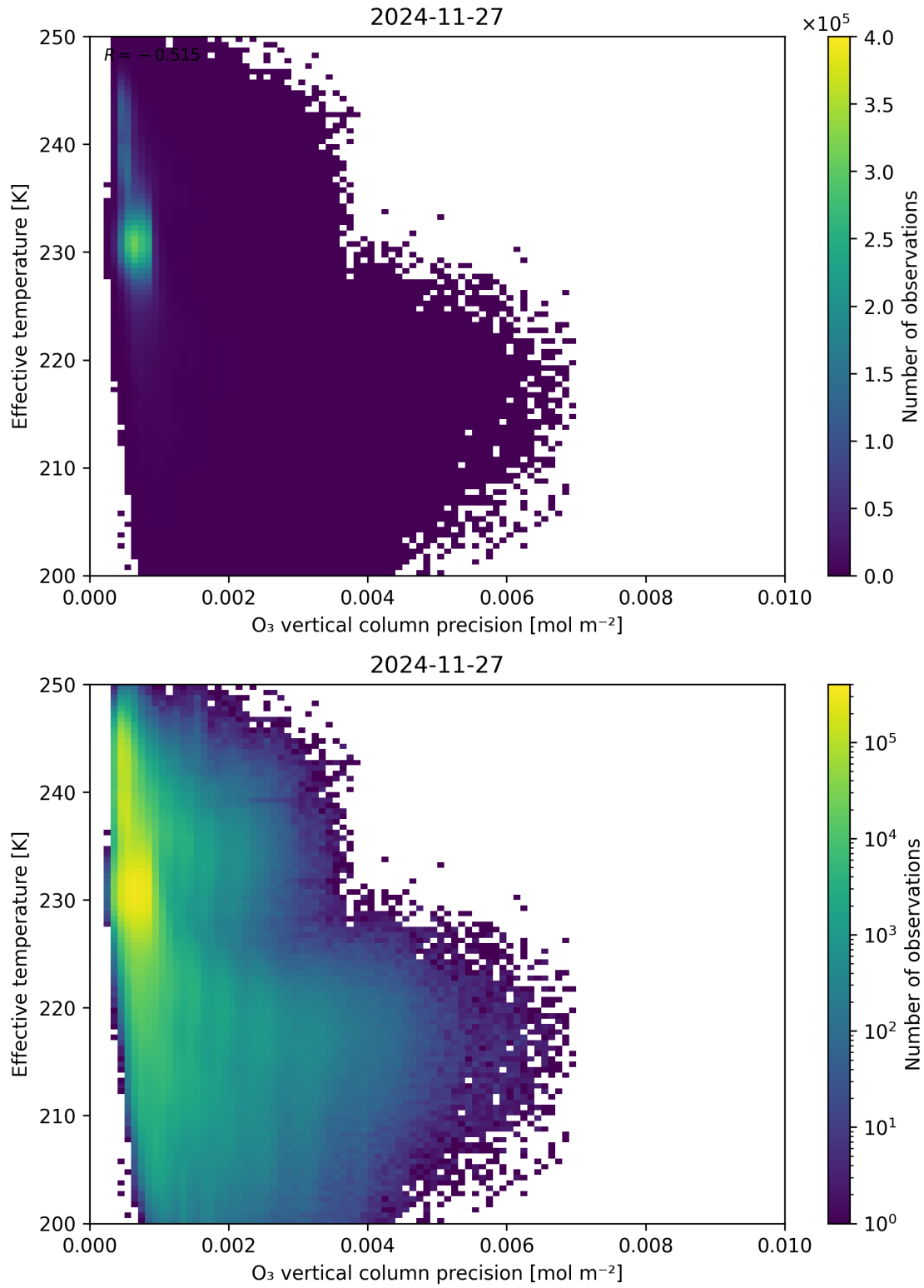
Figure 42: Scatter density plot of “O 3 vertical column precision” against “Effective temperature” for 2024-11-26 to 2024-11-28.
