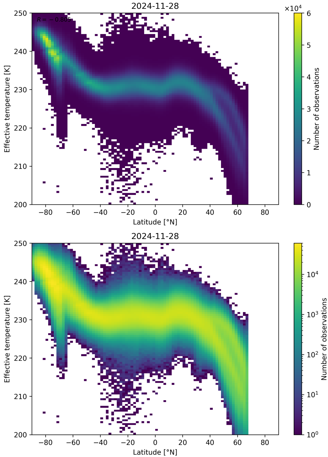
Figure 34: Scatter density plot of “Latitude” against “Effective temperature” for 2024-11-27 to 2024-11-29.
