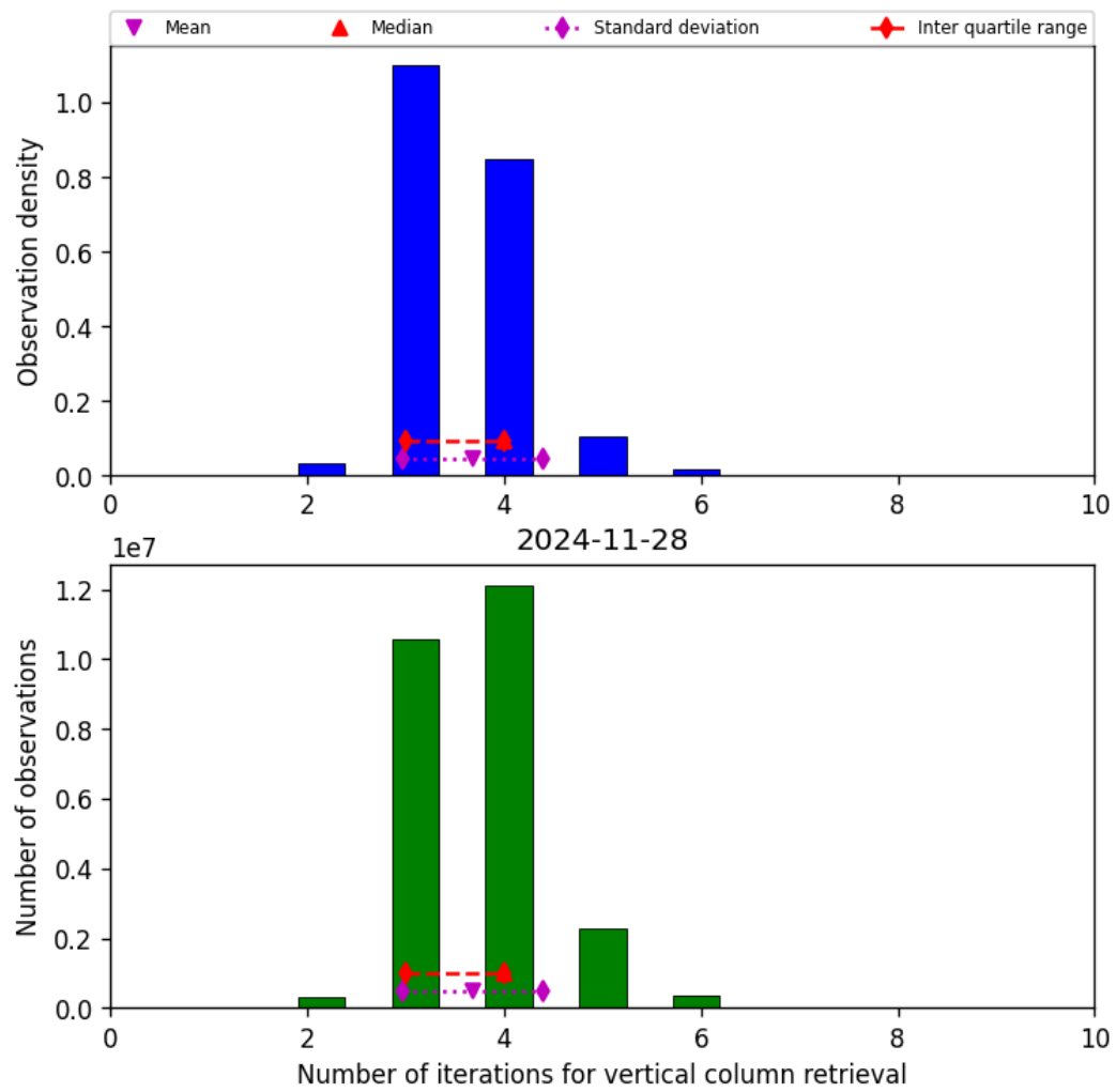
Figure 26: Histogram of “Number of iterations for vertical column retrieval” for 2024-11-27 to 2024-11-29
