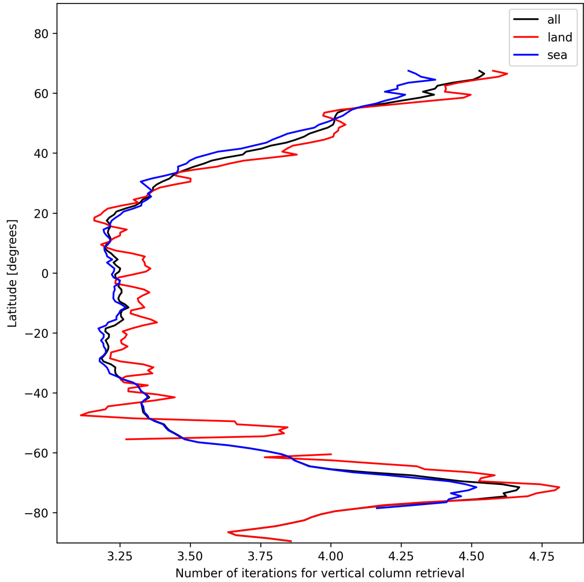
Figure 19: Zonal average of “Number of iterations for vertical column retrieval” for 2024-11-27 to 2024-11-29.
