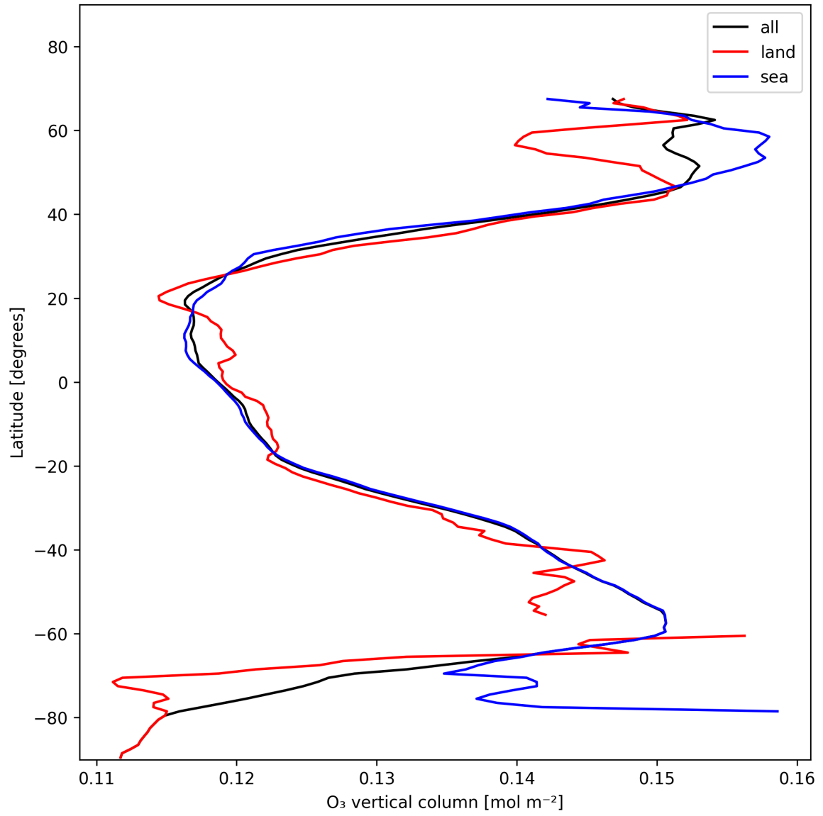
Figure 14: Zonal average of “O 3 vertical column” for 2024-11-27 to 2024-11-29.
