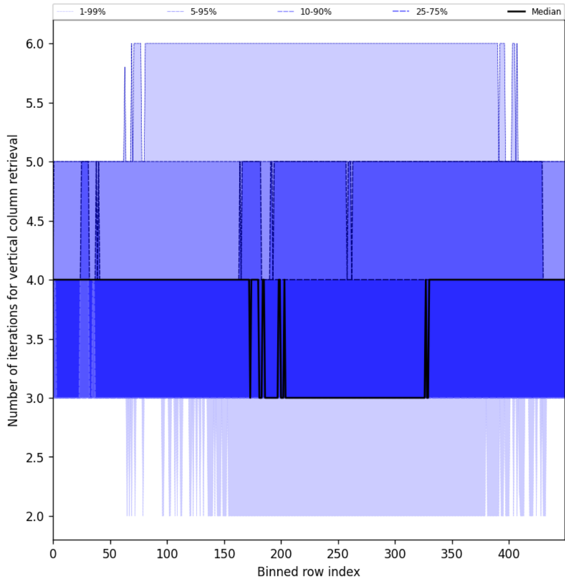
Figure 33: Along track statistics of “Number of iterations for vertical column retrieval” for 2024-11-27 to 2024-11-29
