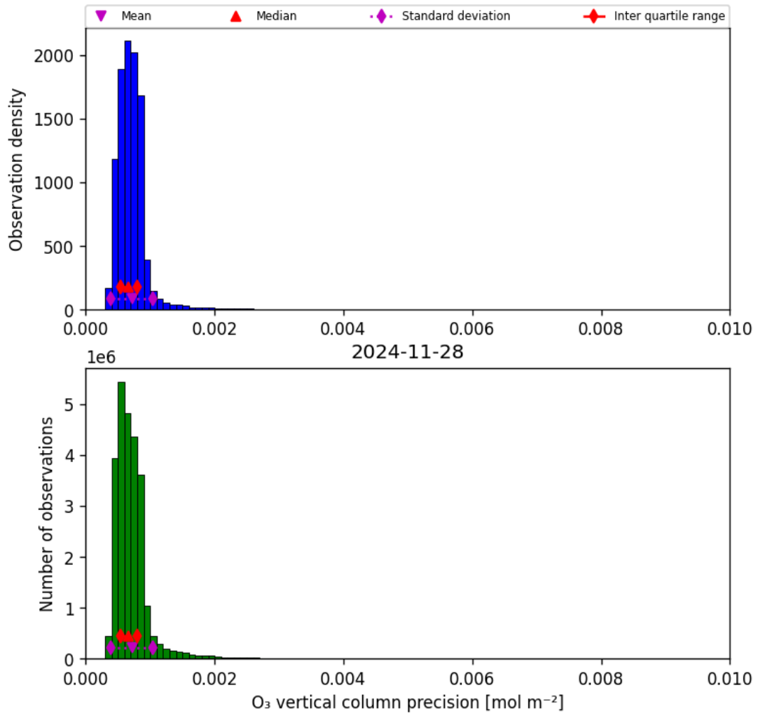
Figure 22: Histogram of “O 3 vertical column precision” for 2024-11-27 to 2024-11-29
