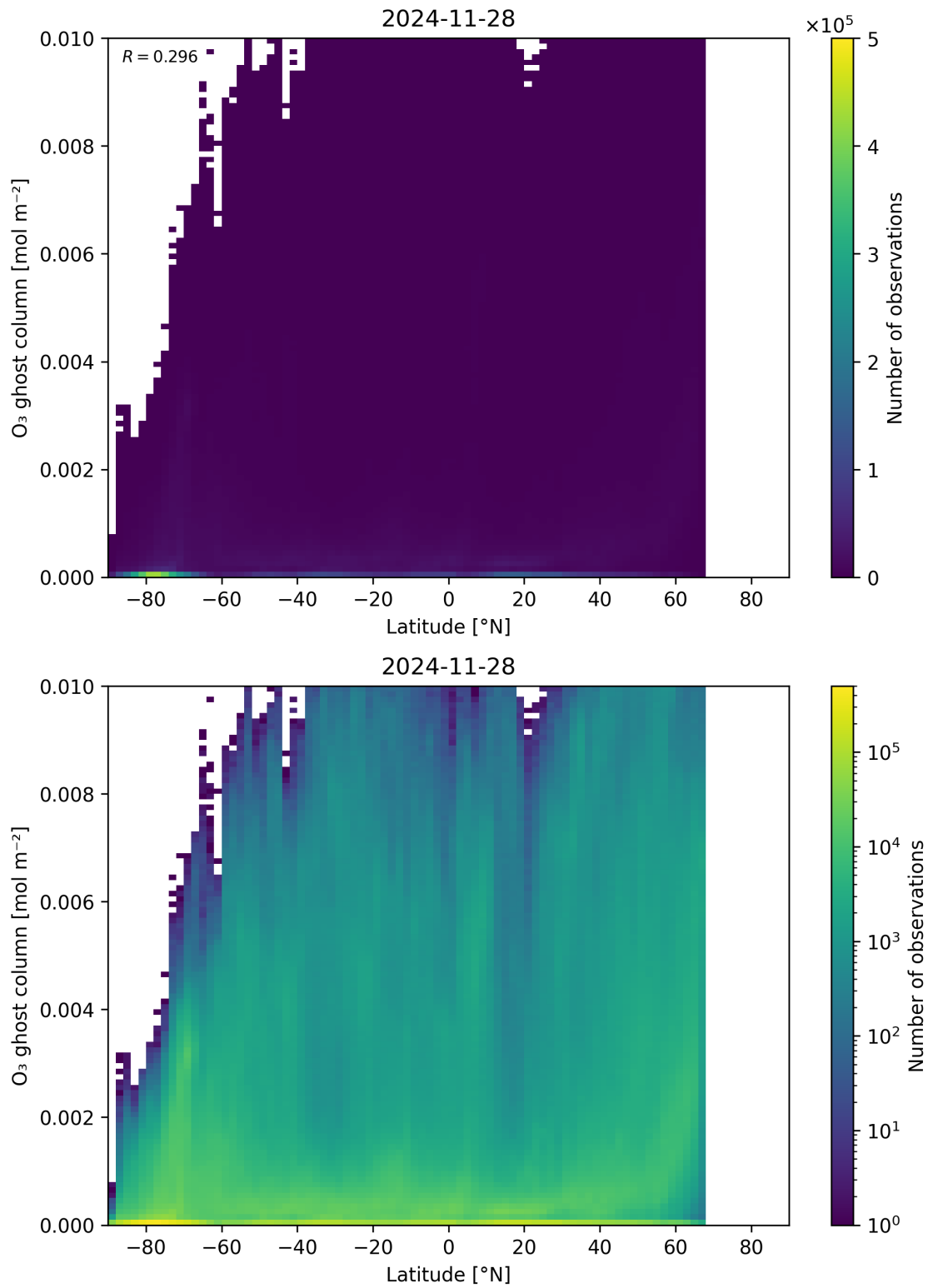
Figure 35: Scatter density plot of “Latitude” against “O 3 ghost column” for 2024-11-27 to 2024-11-29.
