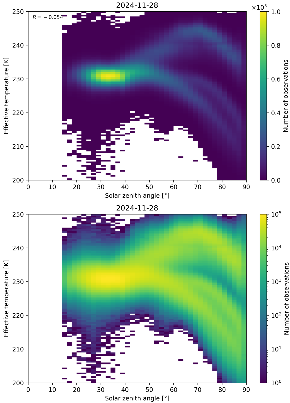
Figure 45: Scatter density plot of “Solar zenith angle” against “Effective temperature” for 2024-11-27 to 2024-11-29.
