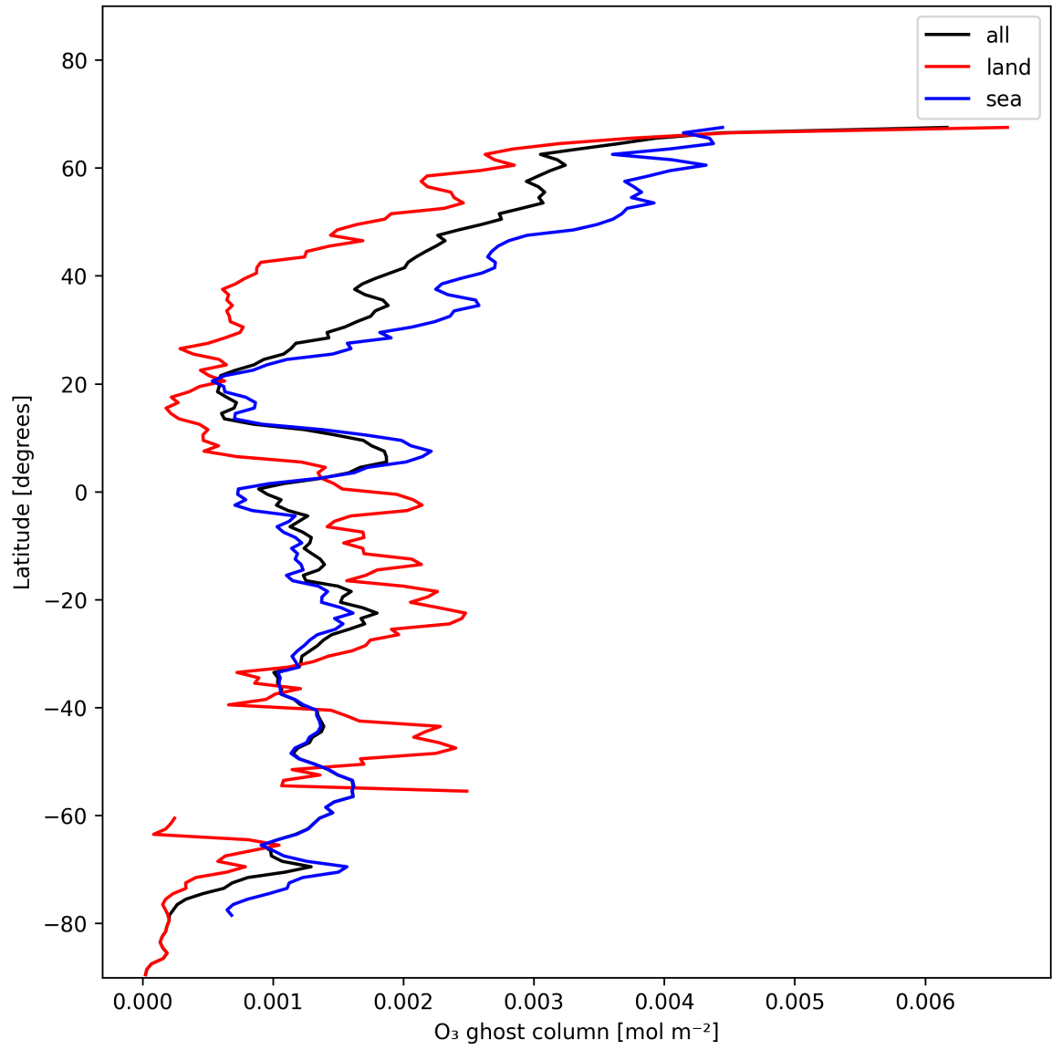
Figure 18: Zonal average of “O 3 ghost column” for 2024-11-27 to 2024-11-29.
