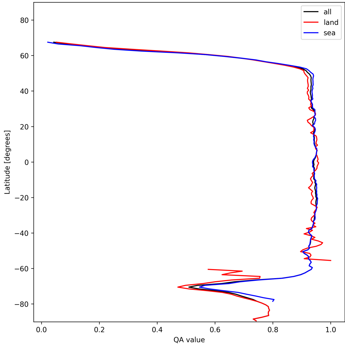
Figure 13: Zonal average of “QA value” for 2024-11-27 to 2024-11-29.
