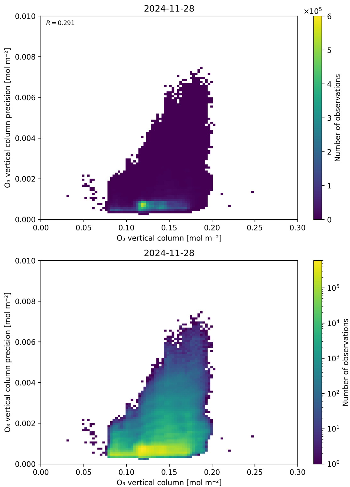
Figure 41: Scatter density plot of “O 3 vertical column” against “O 3 vertical column precision” for 2024-11-27 to 2024-11-29.
