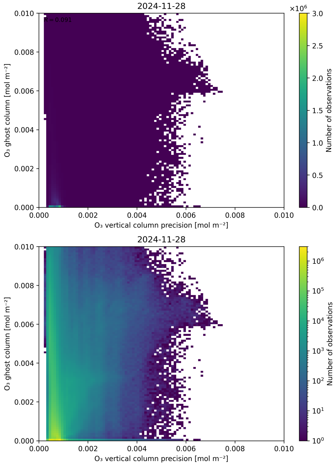
Figure 43: Scatter density plot of “ \text{O}_3 vertical column precision” against “ \text{O}_3 ghost column” for 2024-11-27 to 2024-11-29.
