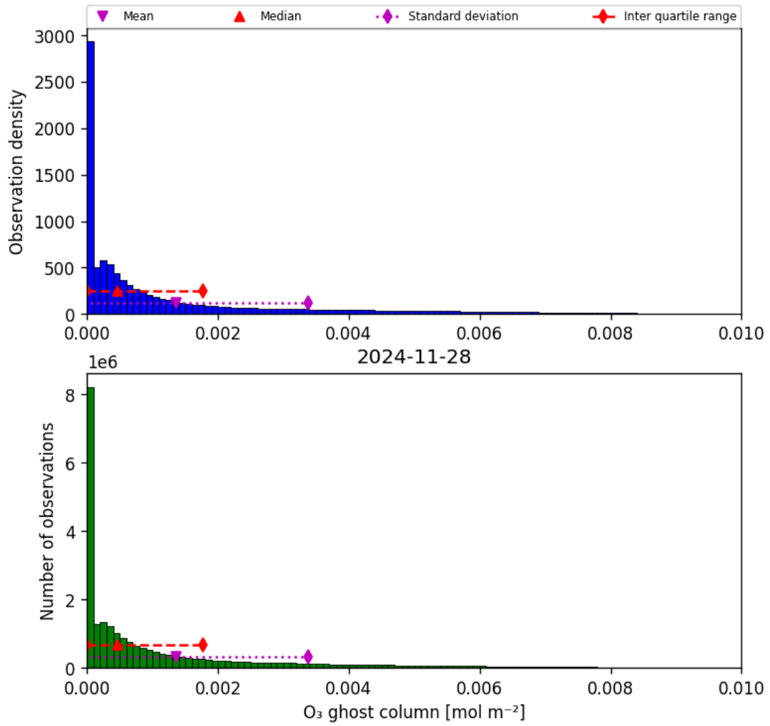
Figure 25: Histogram of “O 3 ghost column” for 2024-11-27 to 2024-11-29
