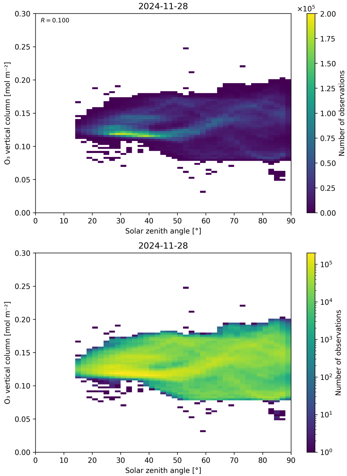
Figure 47: Scatter density plot of “Solar zenith angle” against “O 3 vertical column” for 2024-11-27 to 2024-11-29.
