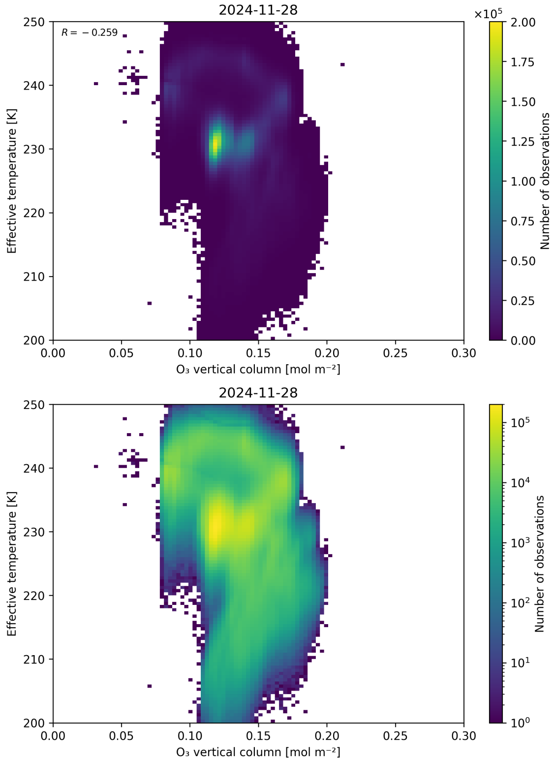
Figure 39: Scatter density plot of “O 3 vertical column” against “Effective temperature” for 2024-11-27 to 2024-11-29.
