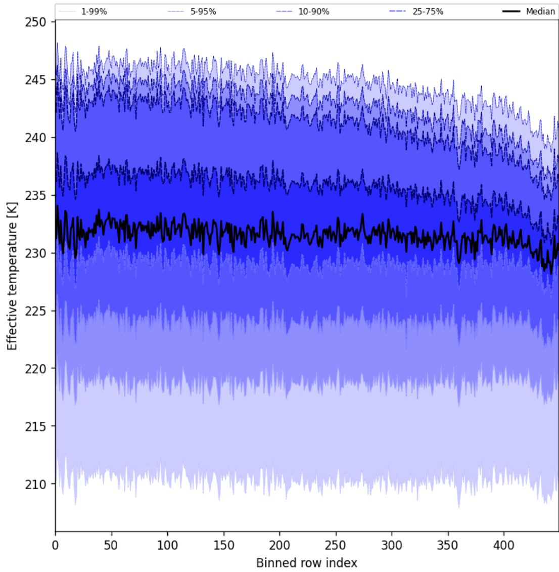
Figure 31: Along track statistics of “Effective temperature” for 2024-11-27 to 2024-11-29
