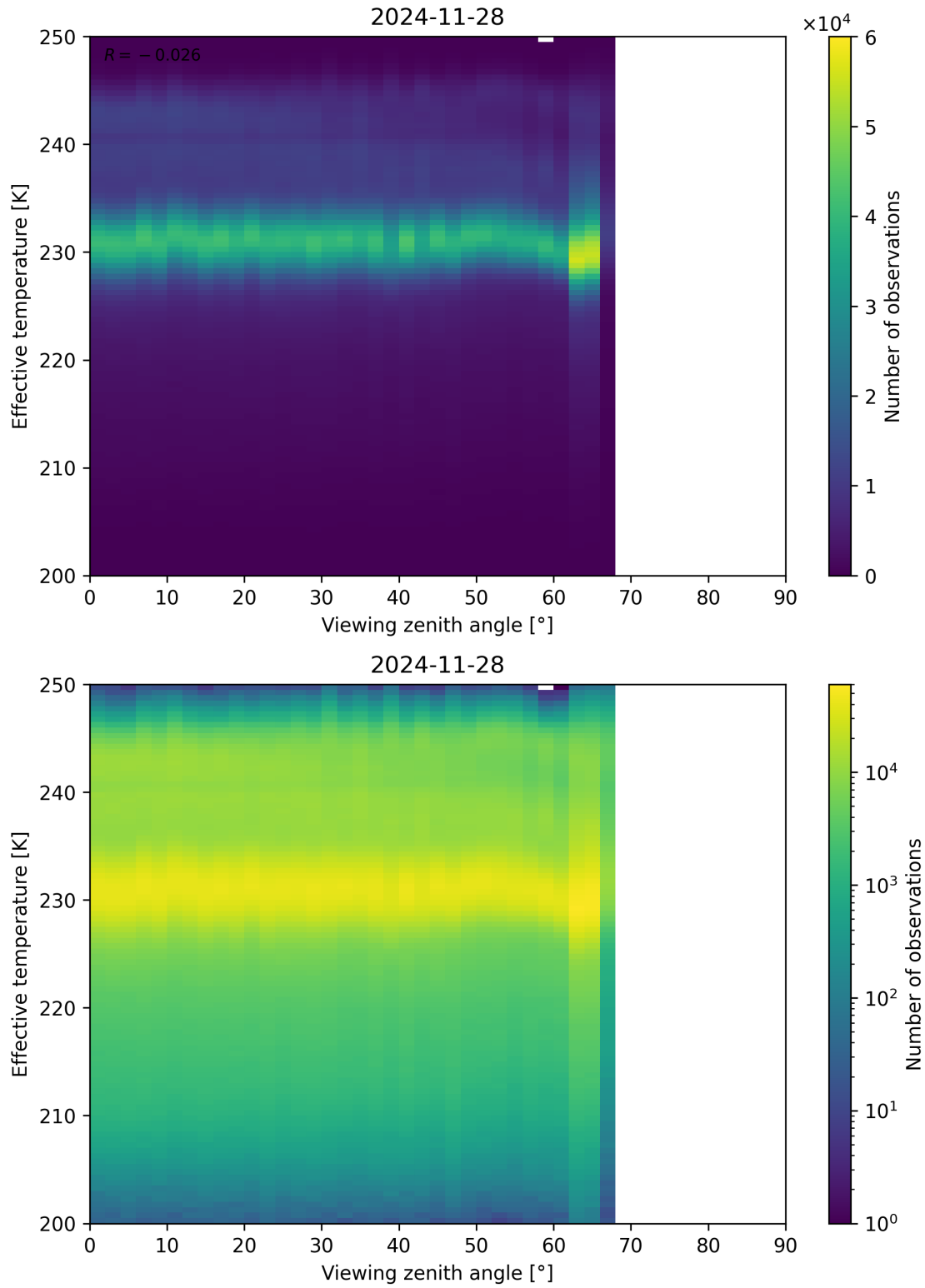
Figure 50: Scatter density plot of “Viewing zenith angle” against “Effective temperature” for 2024-11-27 to 2024-11-29.
