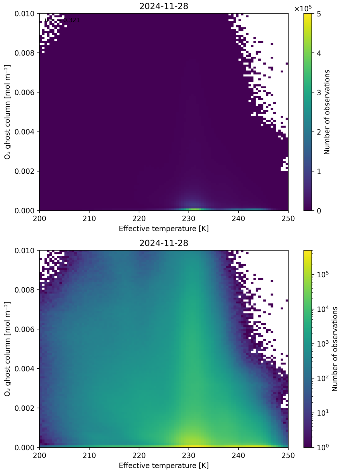
Figure 38: Scatter density plot of “Effective temperature” against “O 3 ghost column” for 2024-11-27 to 2024-11-29.
