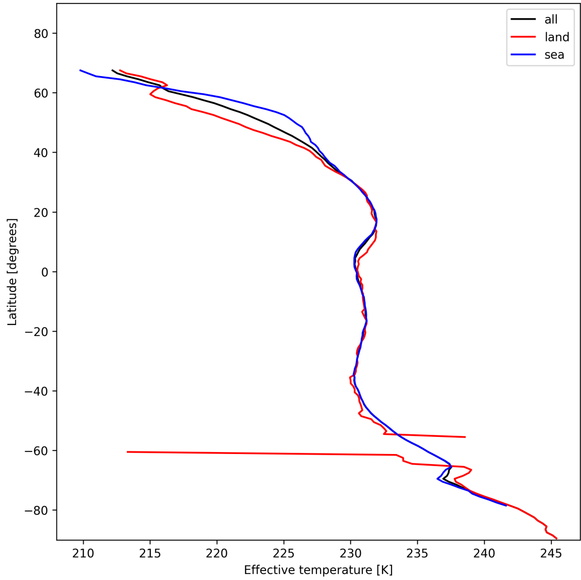
Figure 17: Zonal average of “Effective temperature” for 2024-11-27 to 2024-11-29.
