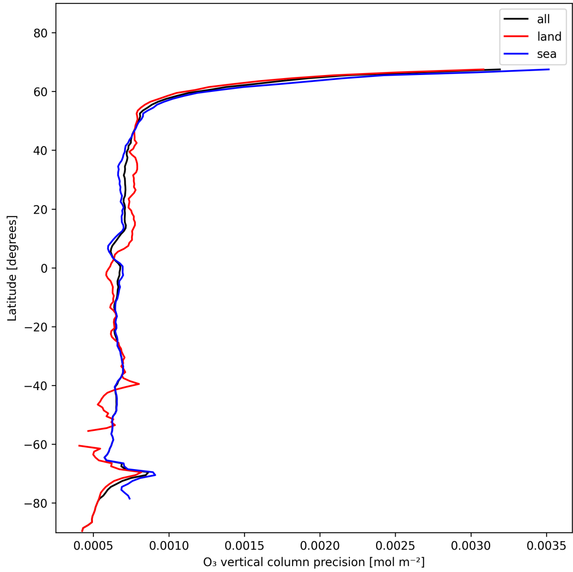
Figure 15: Zonal average of “O 3 vertical column precision” for 2024-11-27 to 2024-11-29.
