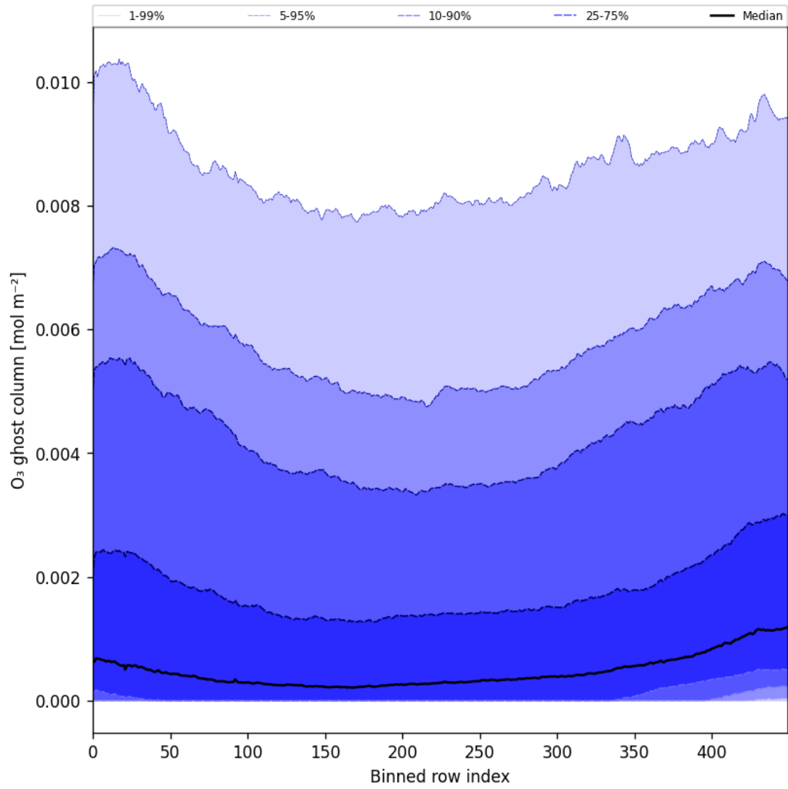
Figure 32: Along track statistics of “O 3 ghost column” for 2024-11-27 to 2024-11-29
