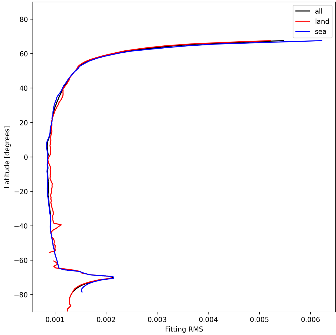
Figure 16: Zonal average of “Fitting RMS” for 2024-11-27 to 2024-11-29.
