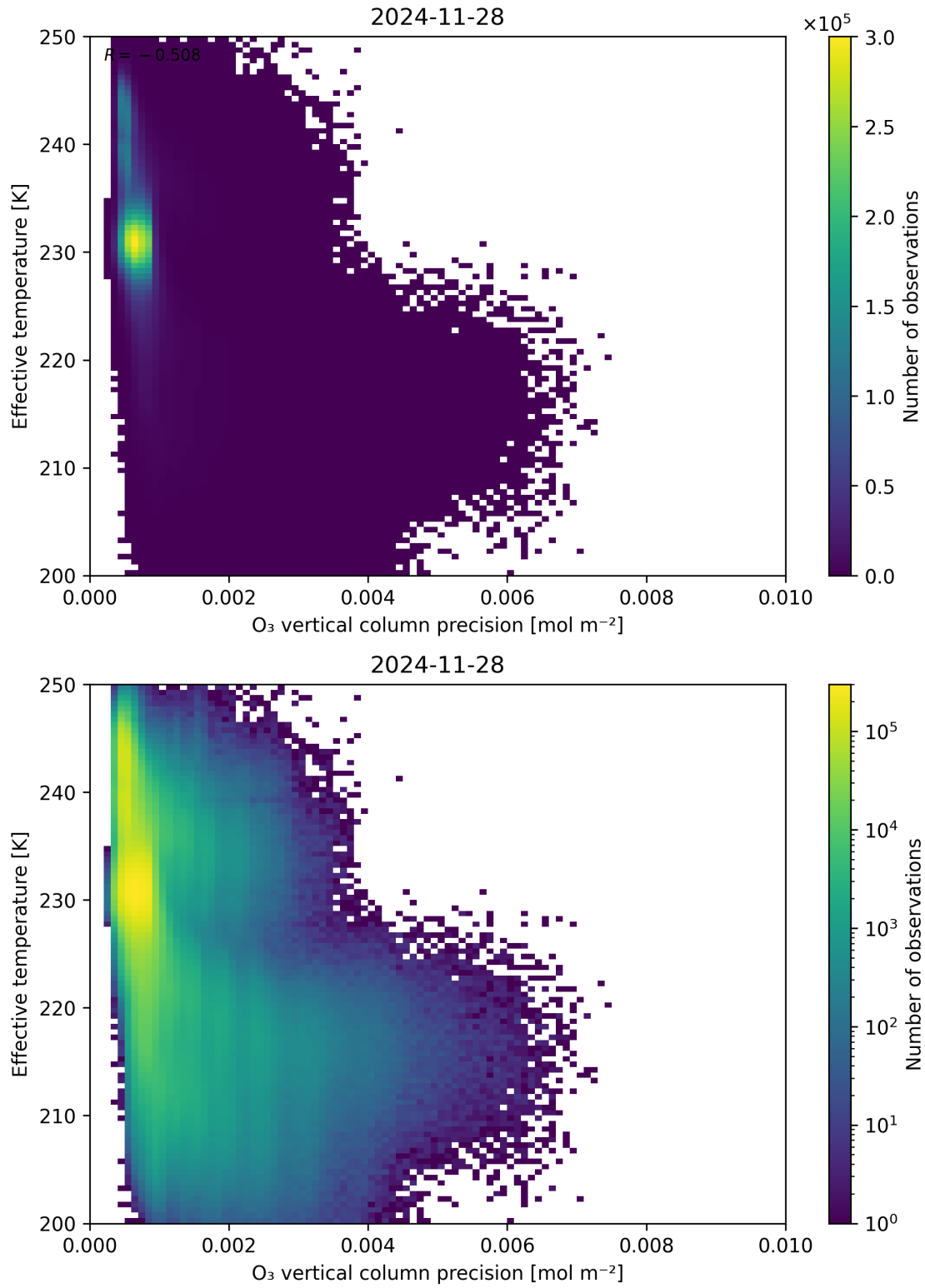
Figure 42: Scatter density plot of “O 3 vertical column precision” against “Effective temperature” for 2024-11-27 to 2024-11-29.
