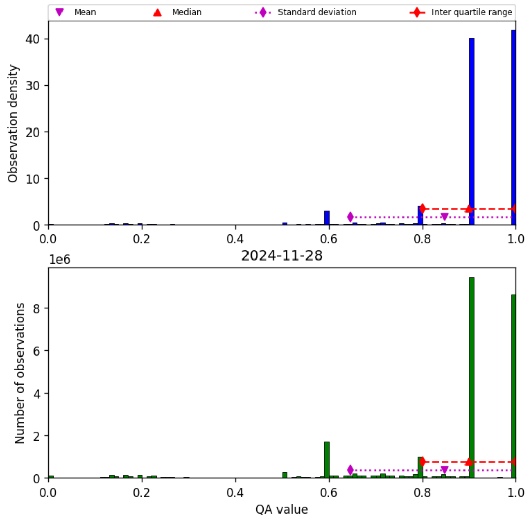
Figure 20: Histogram of “QA value” for 2024-11-27 to 2024-11-29
