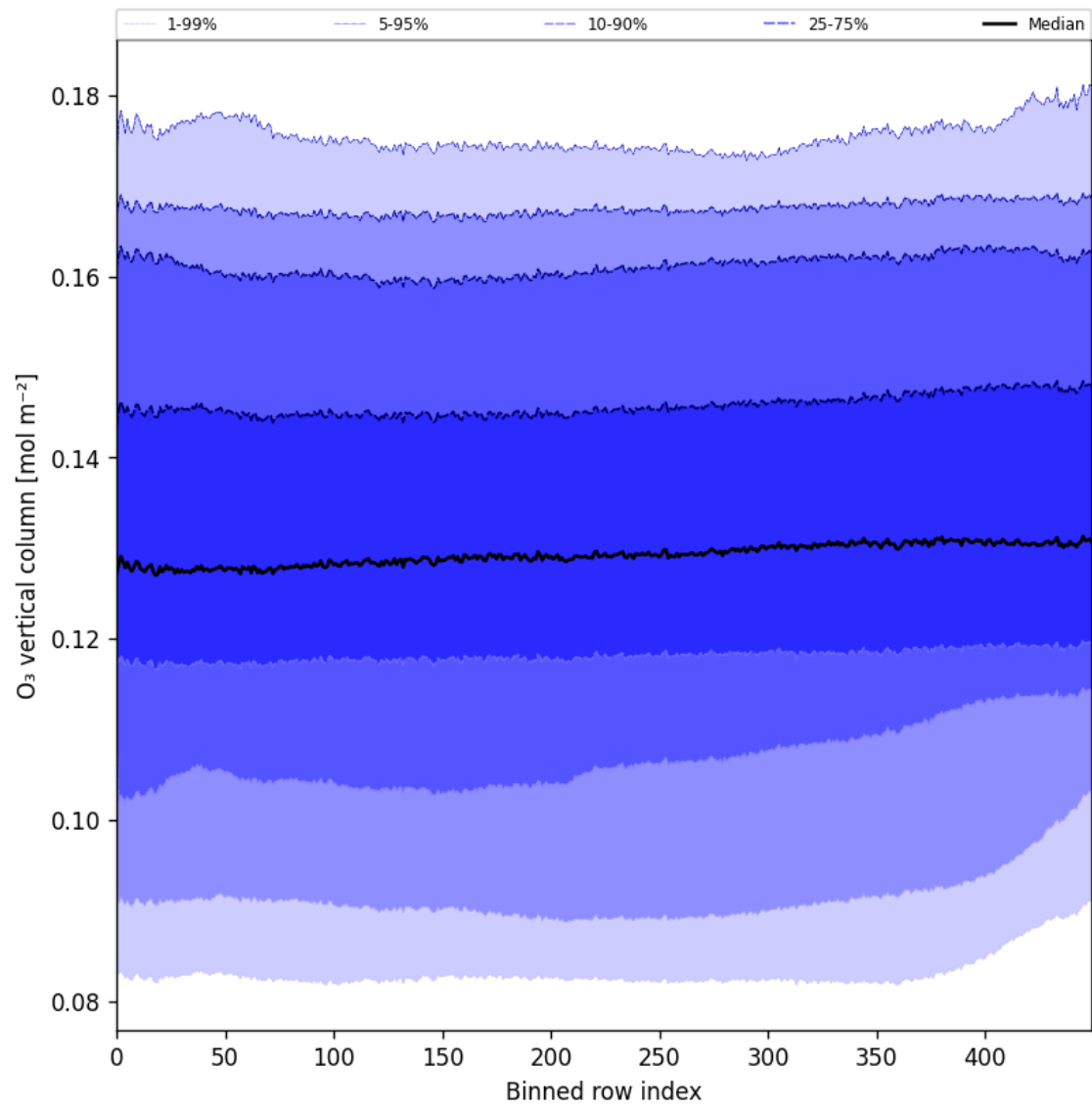
Figure 28: Along track statistics of “O 3 vertical column” for 2024-11-27 to 2024-11-29
