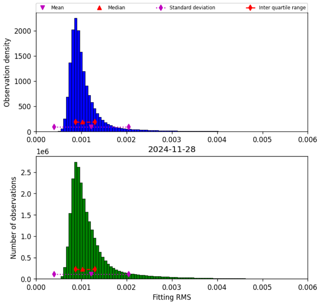
Figure 23: Histogram of “Fitting RMS” for 2024-11-27 to 2024-11-29
