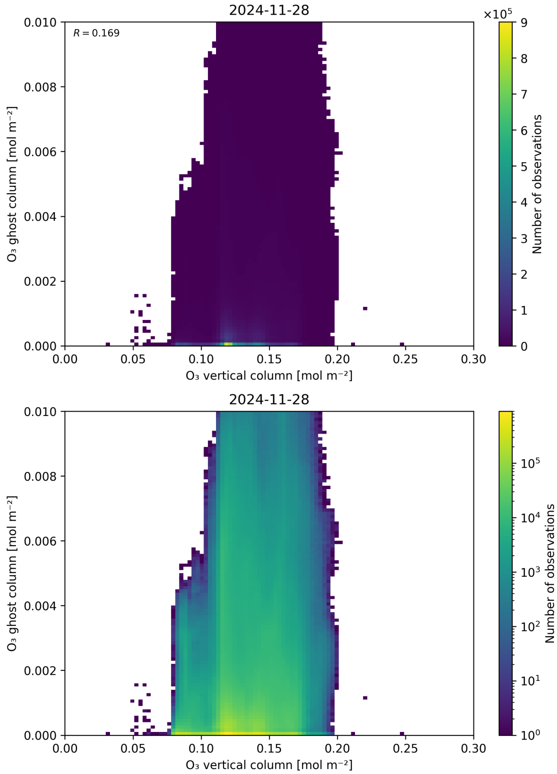
Figure 40: Scatter density plot of “O 3 vertical column” against “O 3 ghost column” for 2024-11-27 to 2024-11-29.
