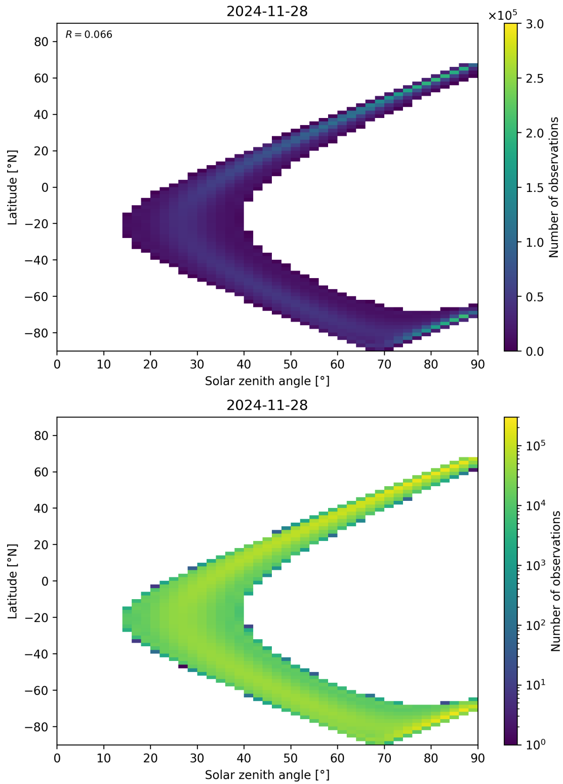
Figure 44: Scatter density plot of “Solar zenith angle” against “Latitude” for 2024-11-27 to 2024-11-29.
