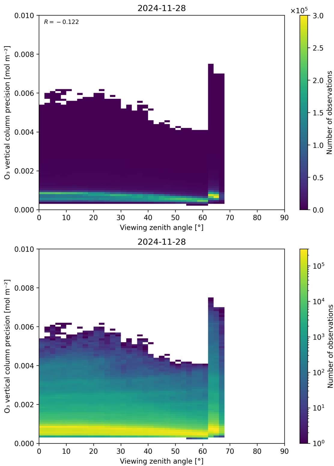
Figure 53: Scatter density plot of “Viewing zenith angle” against “O 3 vertical column precision” for 2024-11-27 to 2024-11-29.
