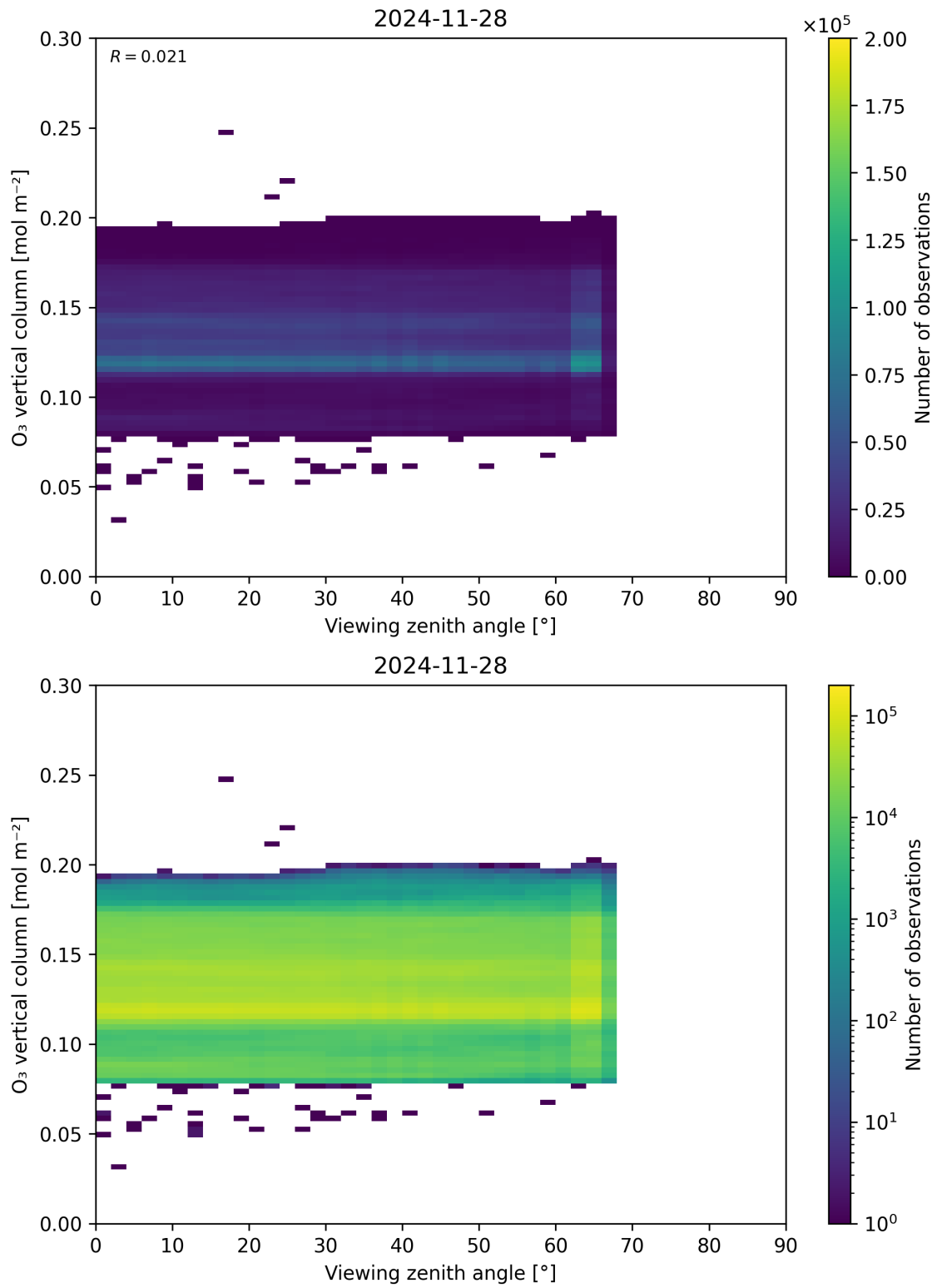
Figure 52: Scatter density plot of “Viewing zenith angle” against “O 3 vertical column” for 2024-11-27 to 2024-11-29.
