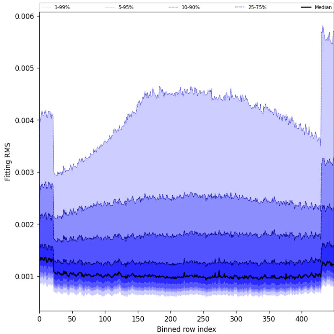
Figure 30: Along track statistics of “Fitting RMS” for 2024-11-27 to 2024-11-29
