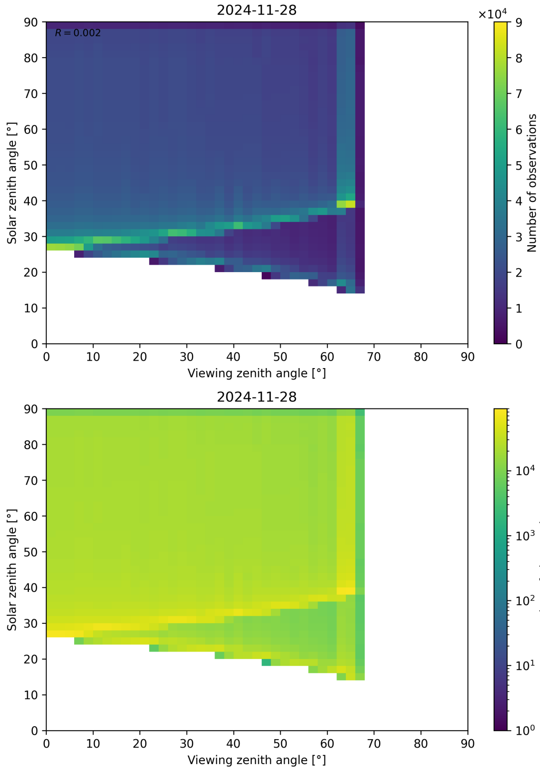
Figure 54: Scatter density plot of “Viewing zenith angle” against “Solar zenith angle” for 2024-11-27 to 2024-11-29.
