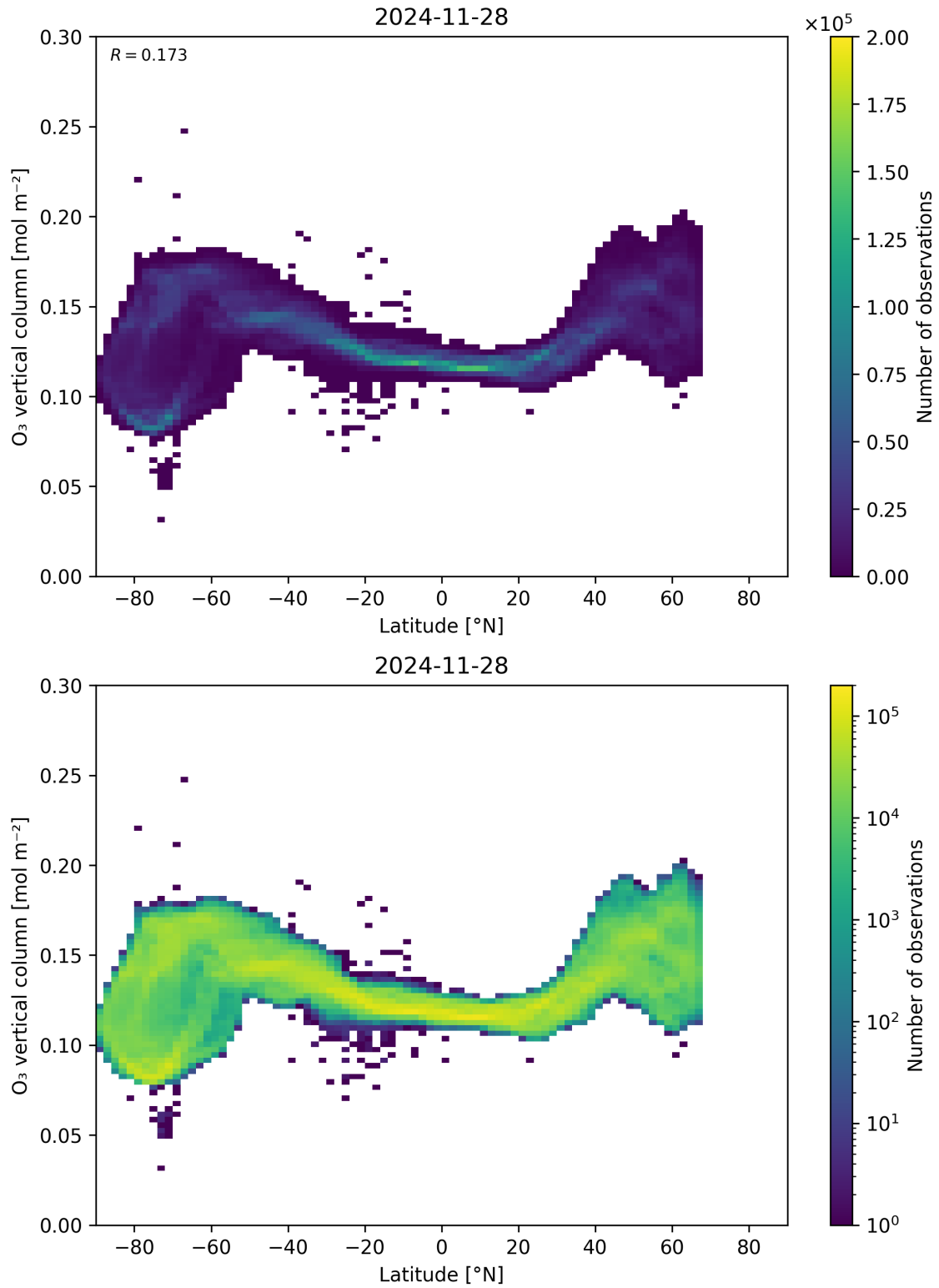
Figure 36: Scatter density plot of “Latitude” against “O 3 vertical column” for 2024-11-27 to 2024-11-29.
