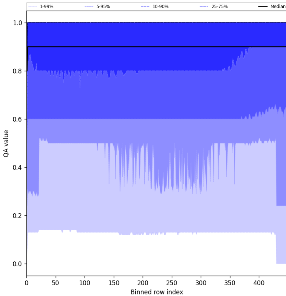
Figure 27: Along track statistics of “QA value” for 2024-11-27 to 2024-11-29
