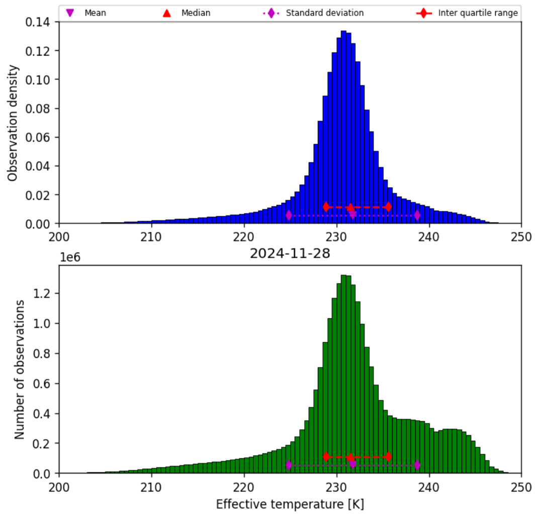
Figure 24: Histogram of “Effective temperature” for 2024-11-27 to 2024-11-29
