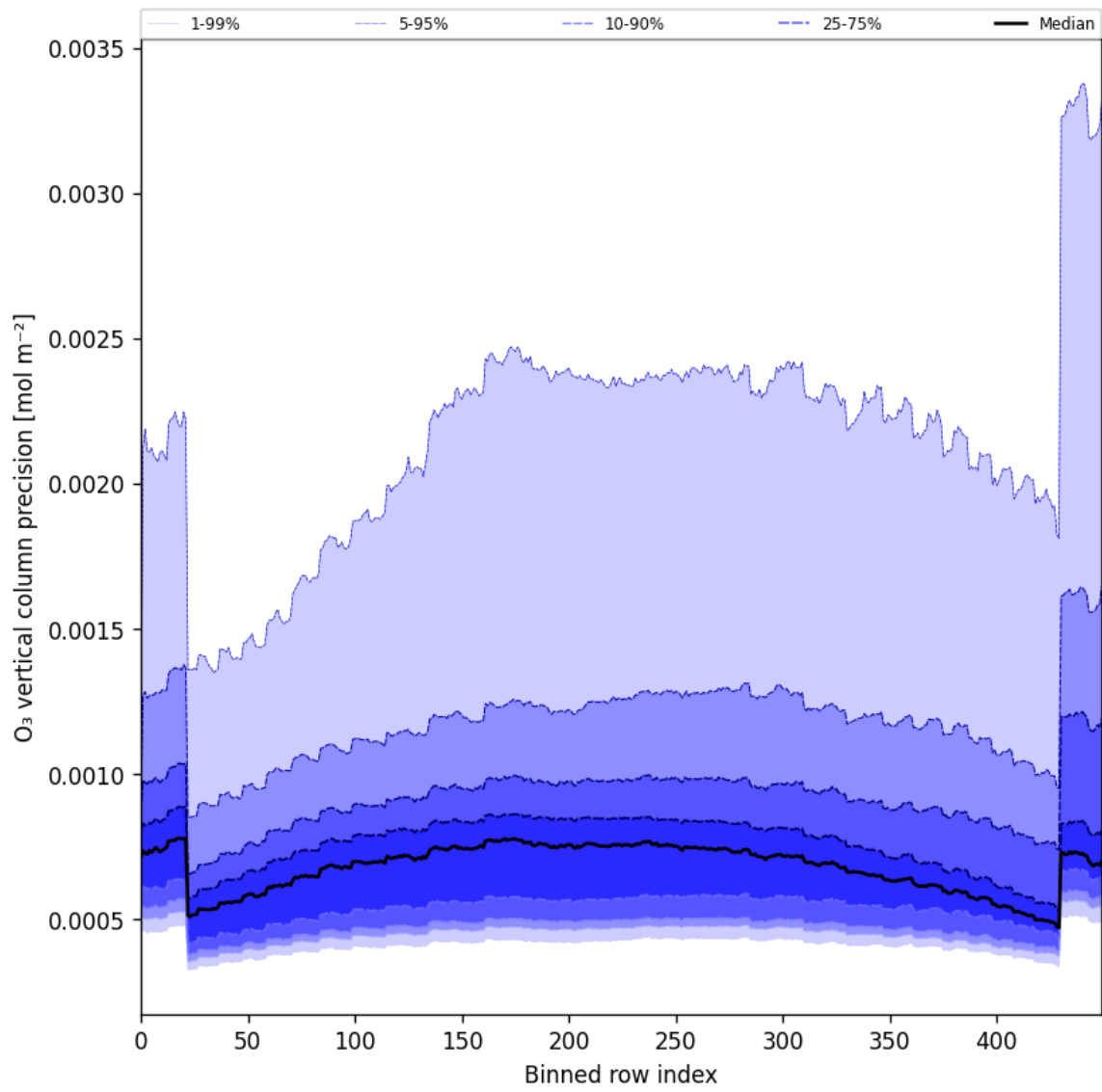
Figure 29: Along track statistics of “O 3 vertical column precision” for 2024-11-27 to 2024-11-29
