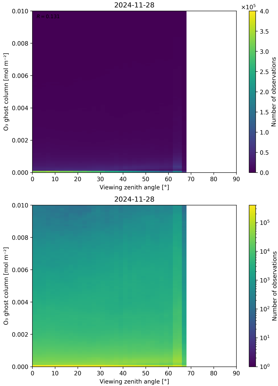
Figure 51: Scatter density plot of “Viewing zenith angle” against “O 3 ghost column” for 2024-11-27 to 2024-11-29.
