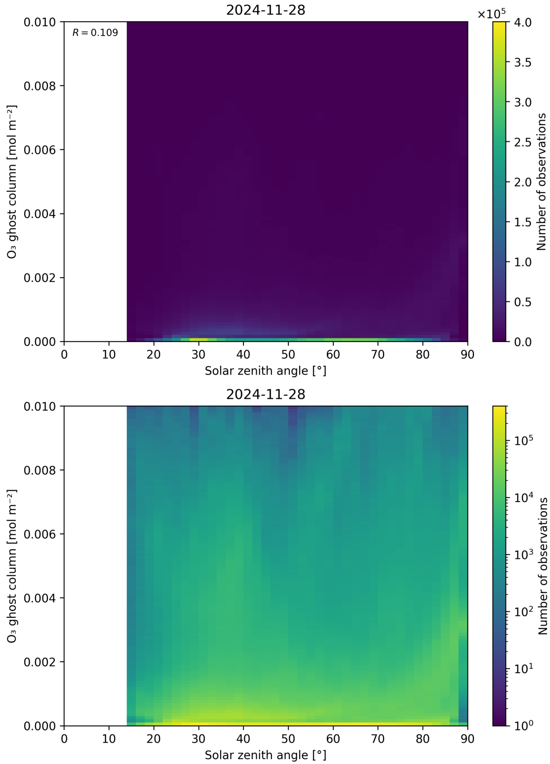
Figure 46: Scatter density plot of “Solar zenith angle” against “O 3 ghost column” for 2024-11-27 to 2024-11-29.
