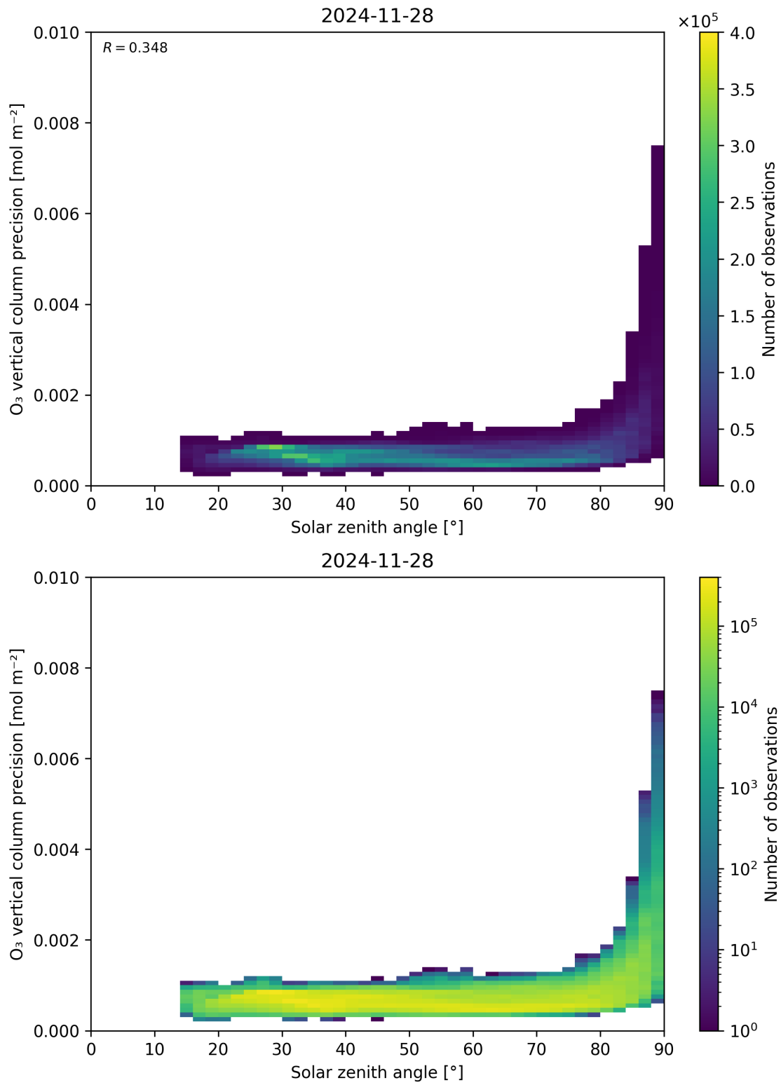
Figure 48: Scatter density plot of “Solar zenith angle” against “O 3 vertical column precision” for 2024-11-27 to 2024-11-29.
