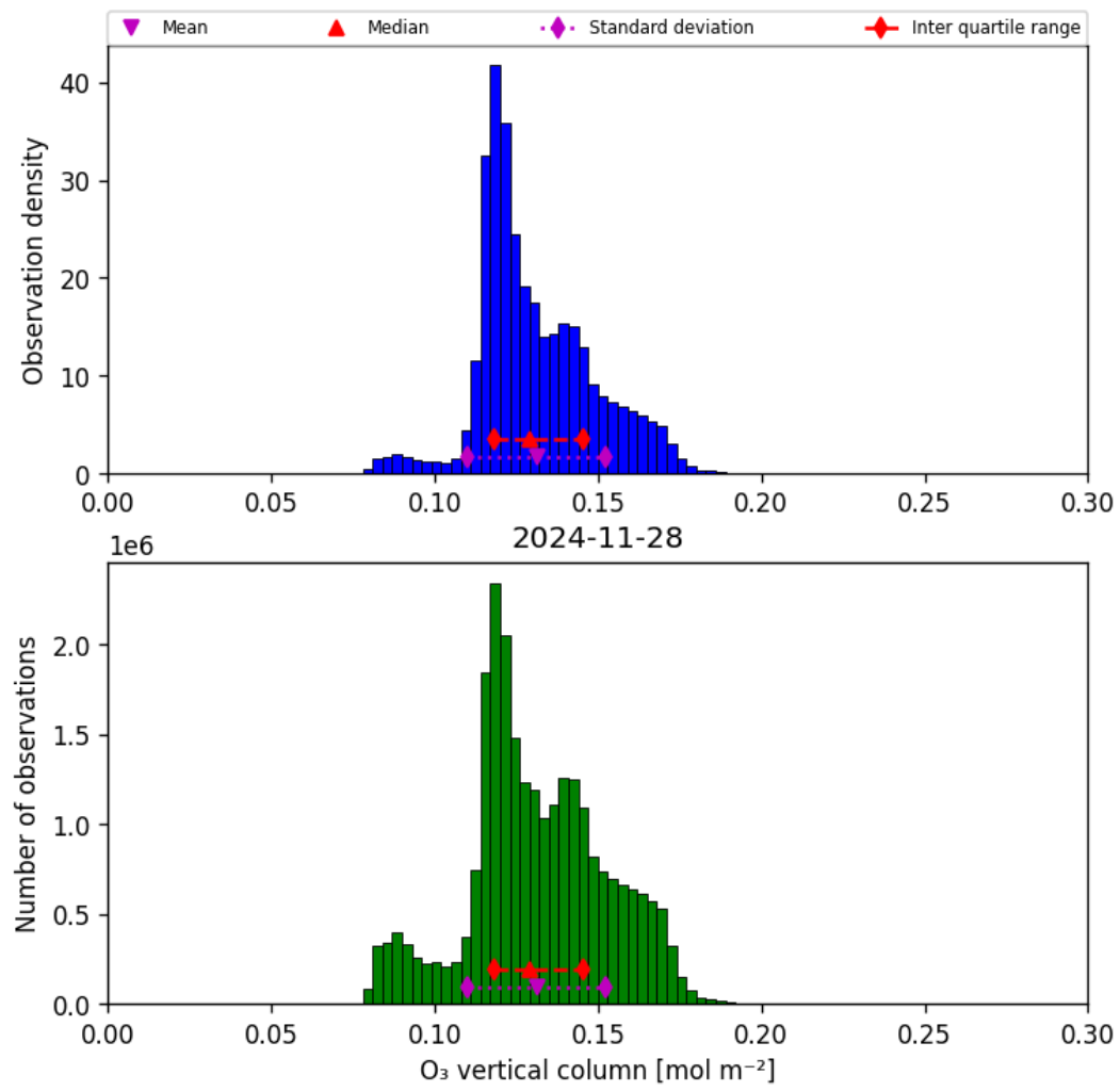
Figure 21: Histogram of “O 3 vertical column” for 2024-11-27 to 2024-11-29
