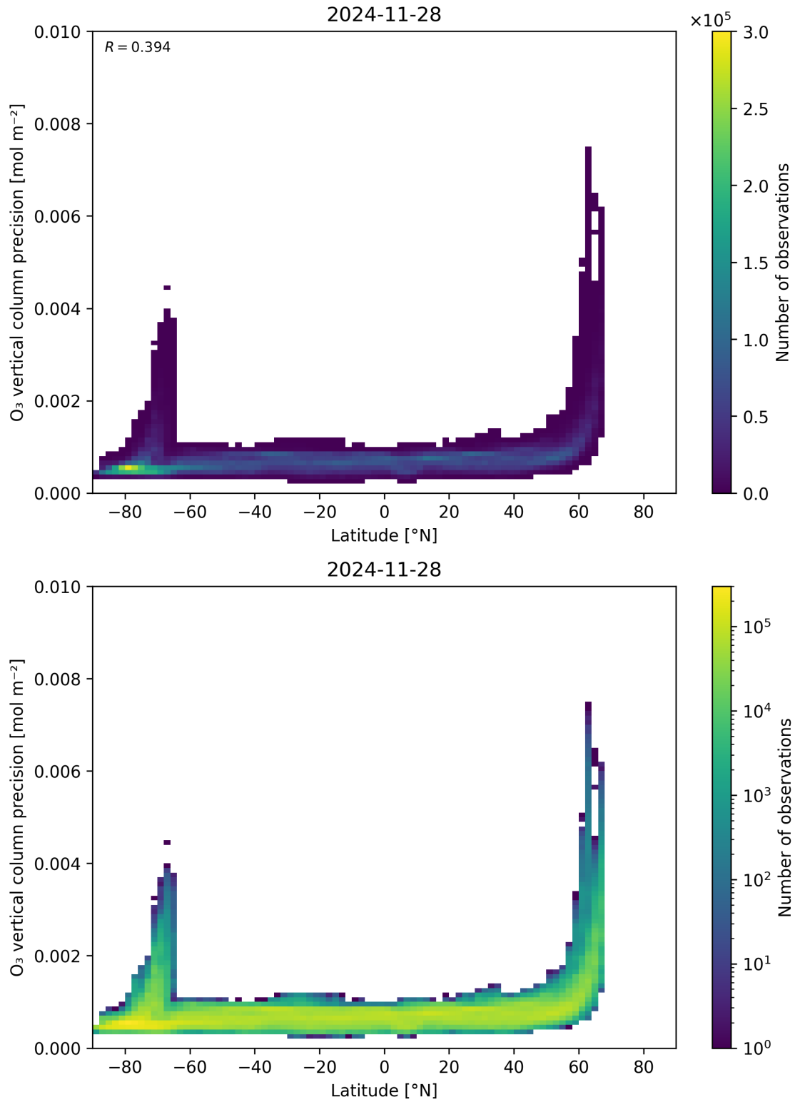
Figure 37: Scatter density plot of “Latitude” against “O 3 vertical column precision” for 2024-11-27 to 2024-11-29.
