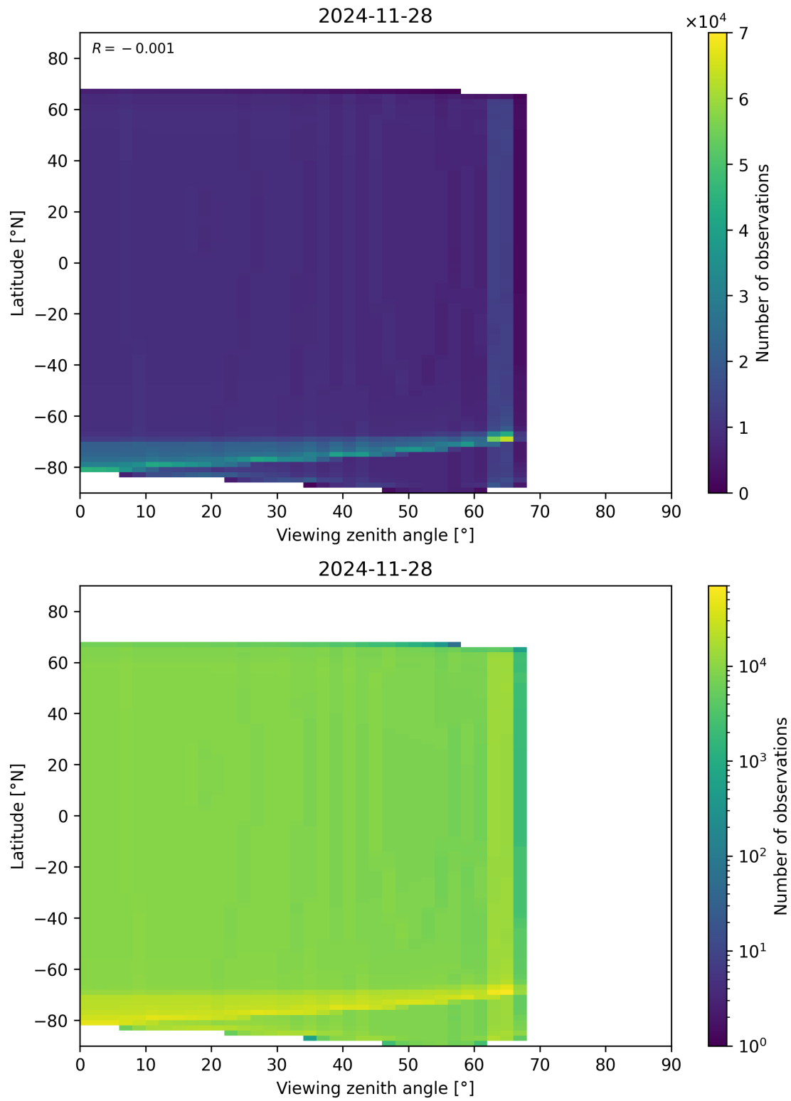
Figure 49: Scatter density plot of “Viewing zenith angle” against “Latitude” for 2024-11-27 to 2024-11-29.
