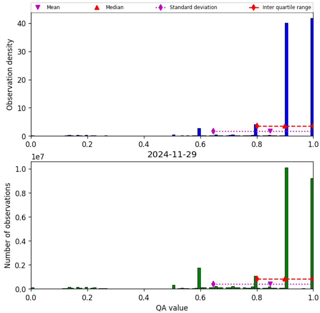
Figure 20: Histogram of “QA value” for 2024-11-28 to 2024-11-30
