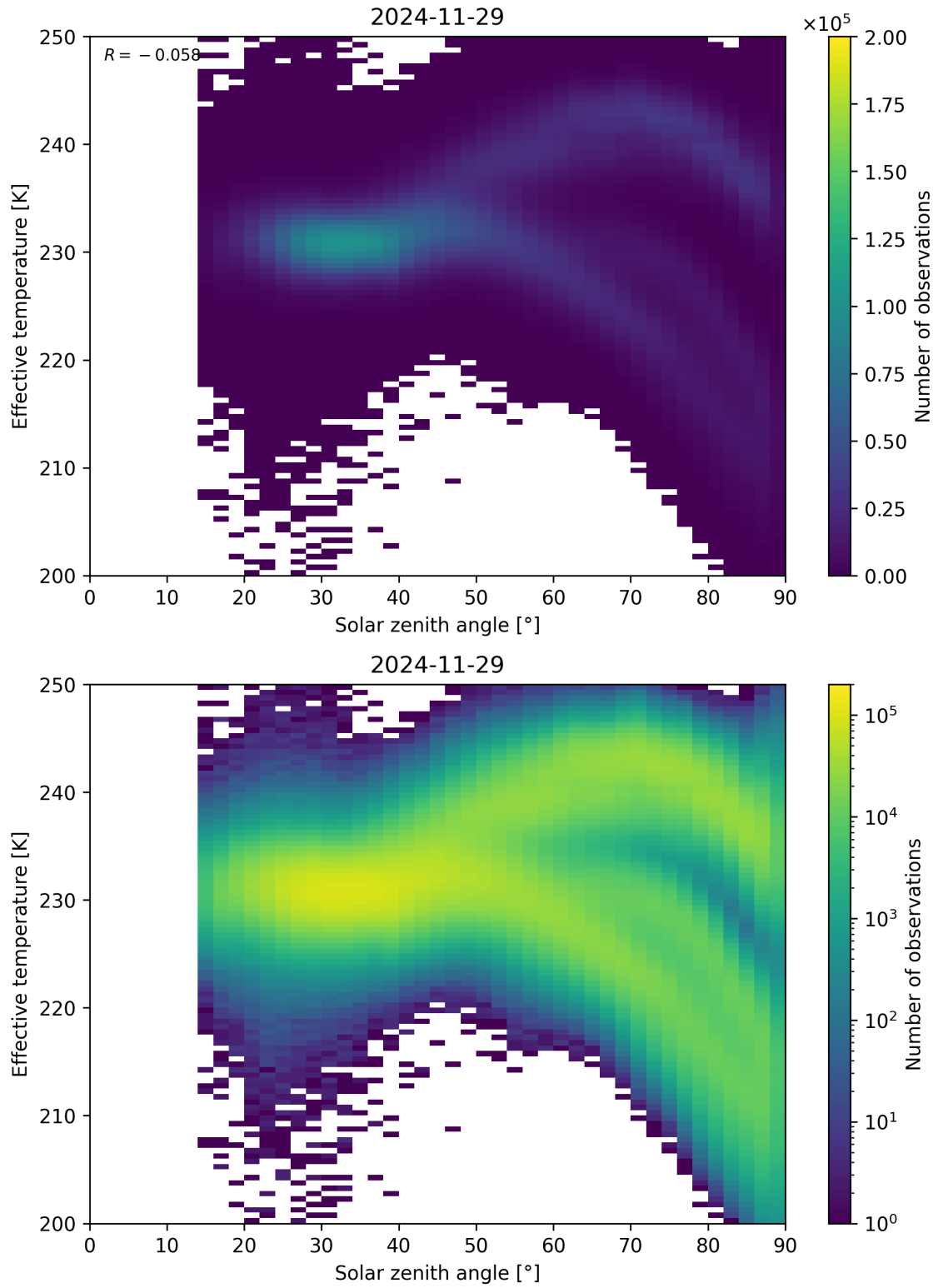
Figure 45: Scatter density plot of “Solar zenith angle” against “Effective temperature” for 2024-11-28 to 2024-11-30.
