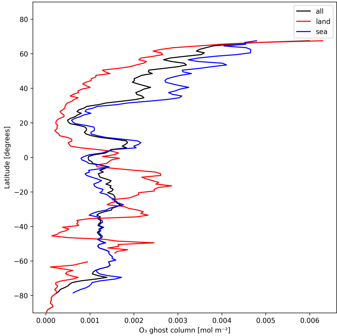
Figure 18: Zonal average of “O 3 ghost column” for 2024-11-28 to 2024-11-30.
