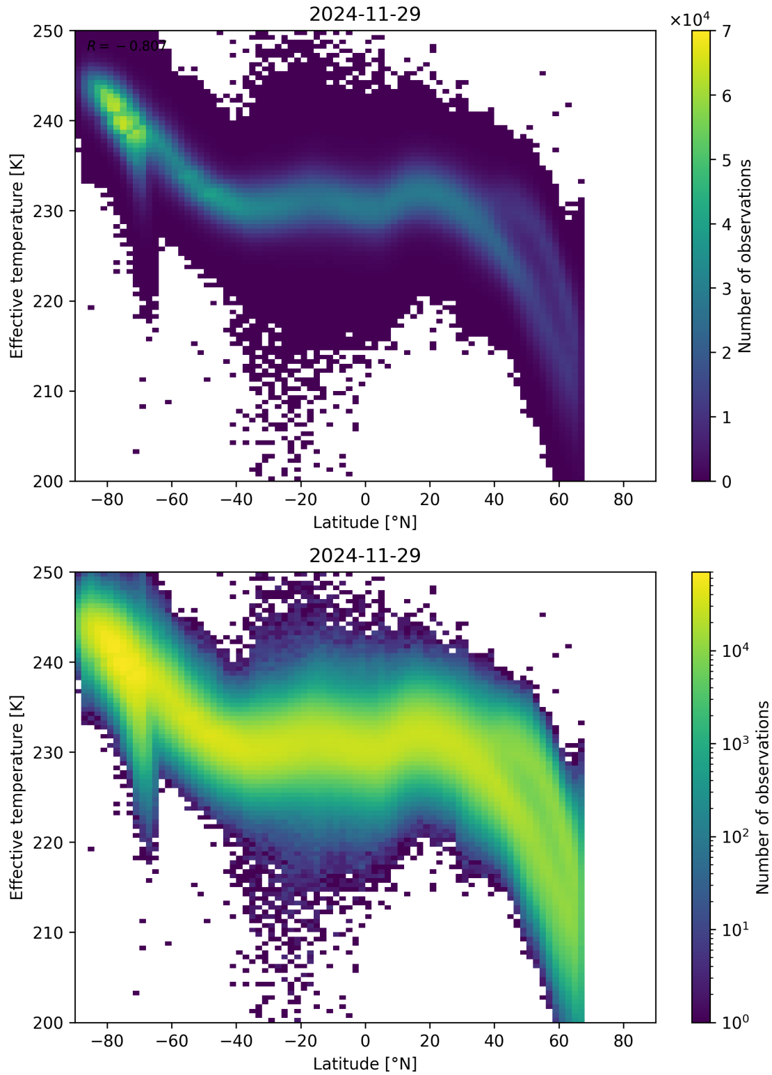
Figure 34: Scatter density plot of “Latitude” against “Effective temperature” for 2024-11-28 to 2024-11-30.
