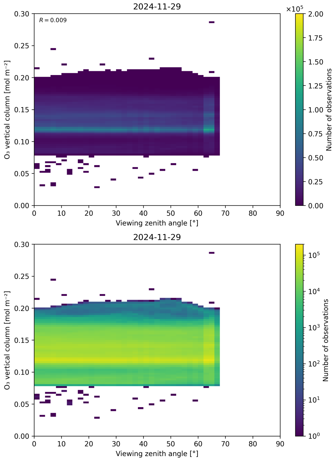
Figure 52: Scatter density plot of “Viewing zenith angle” against “O 3 vertical column” for 2024-11-28 to 2024-11-30.
