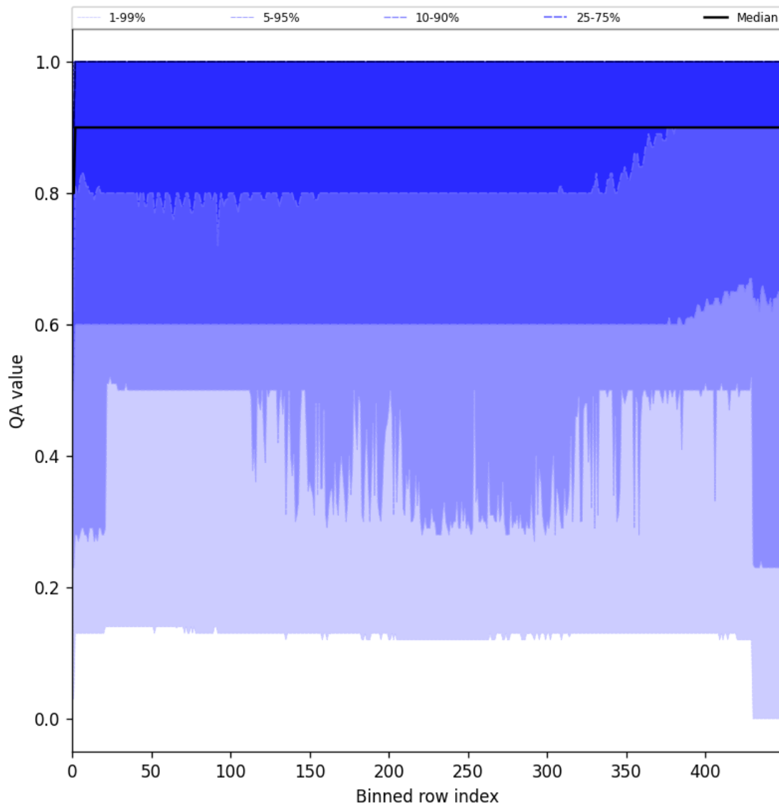
Figure 27: Along track statistics of “QA value” for 2024-11-28 to 2024-11-30
