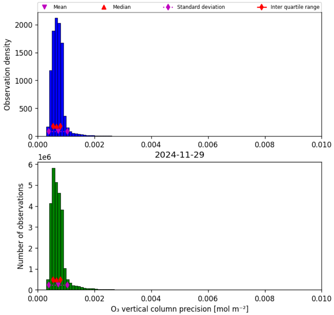
Figure 22: Histogram of “O 3 vertical column precision” for 2024-11-28 to 2024-11-30
