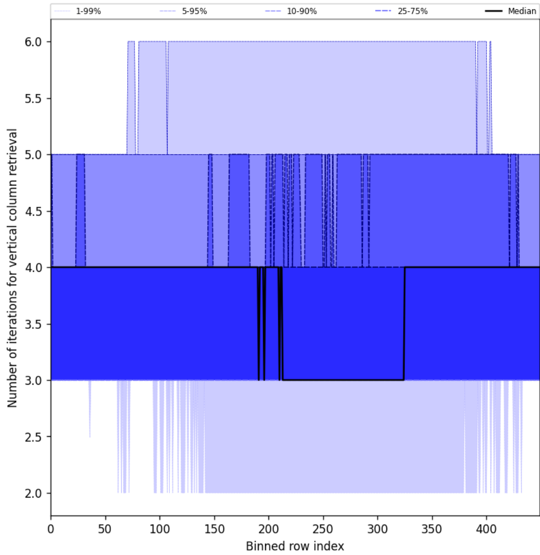
Figure 33: Along track statistics of “Number of iterations for vertical column retrieval” for 2024-11-28 to 2024-11-30
