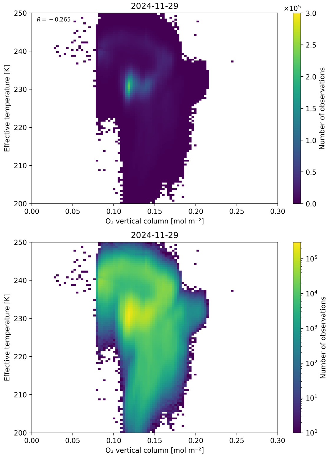
Figure 39: Scatter density plot of “O 3 vertical column” against “Effective temperature” for 2024-11-28 to 2024-11-30.
