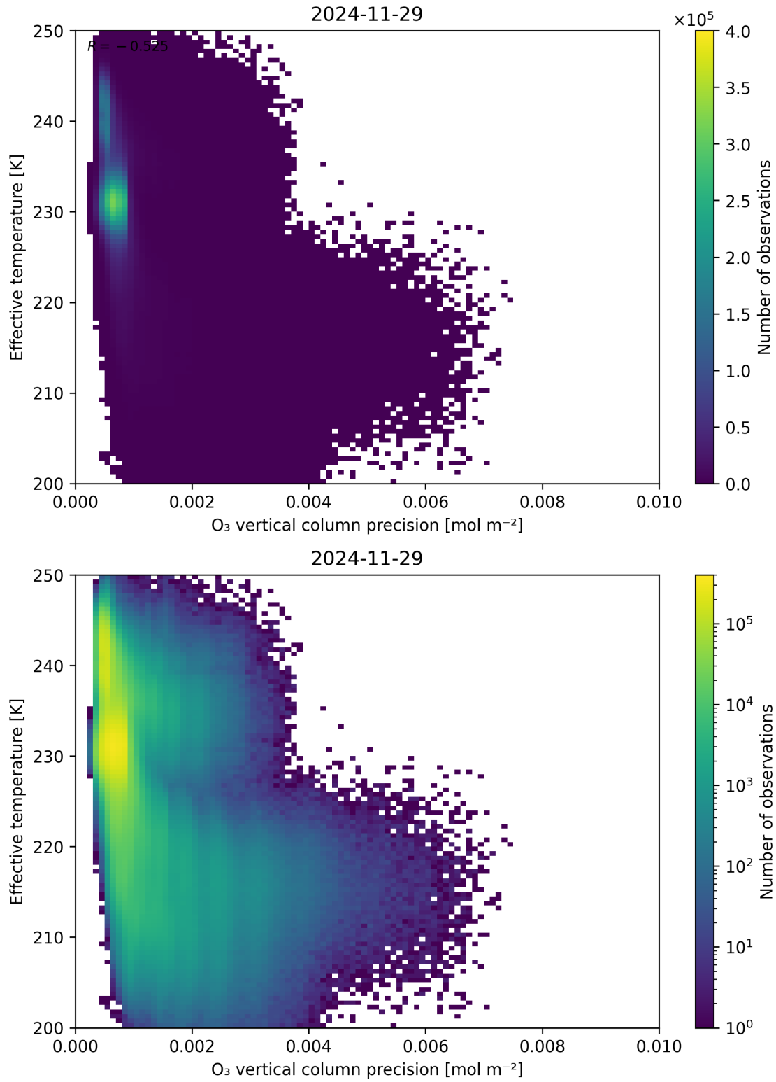
Figure 42: Scatter density plot of “O 3 vertical column precision” against “Effective temperature” for 2024-11-28 to 2024-11-30.
