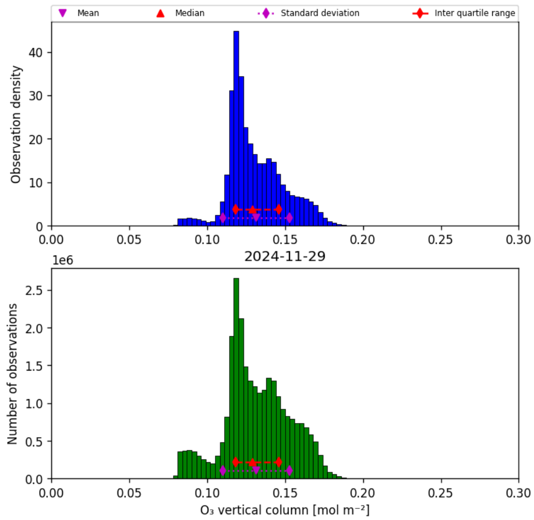
Figure 21: Histogram of “O 3 vertical column” for 2024-11-28 to 2024-11-30
