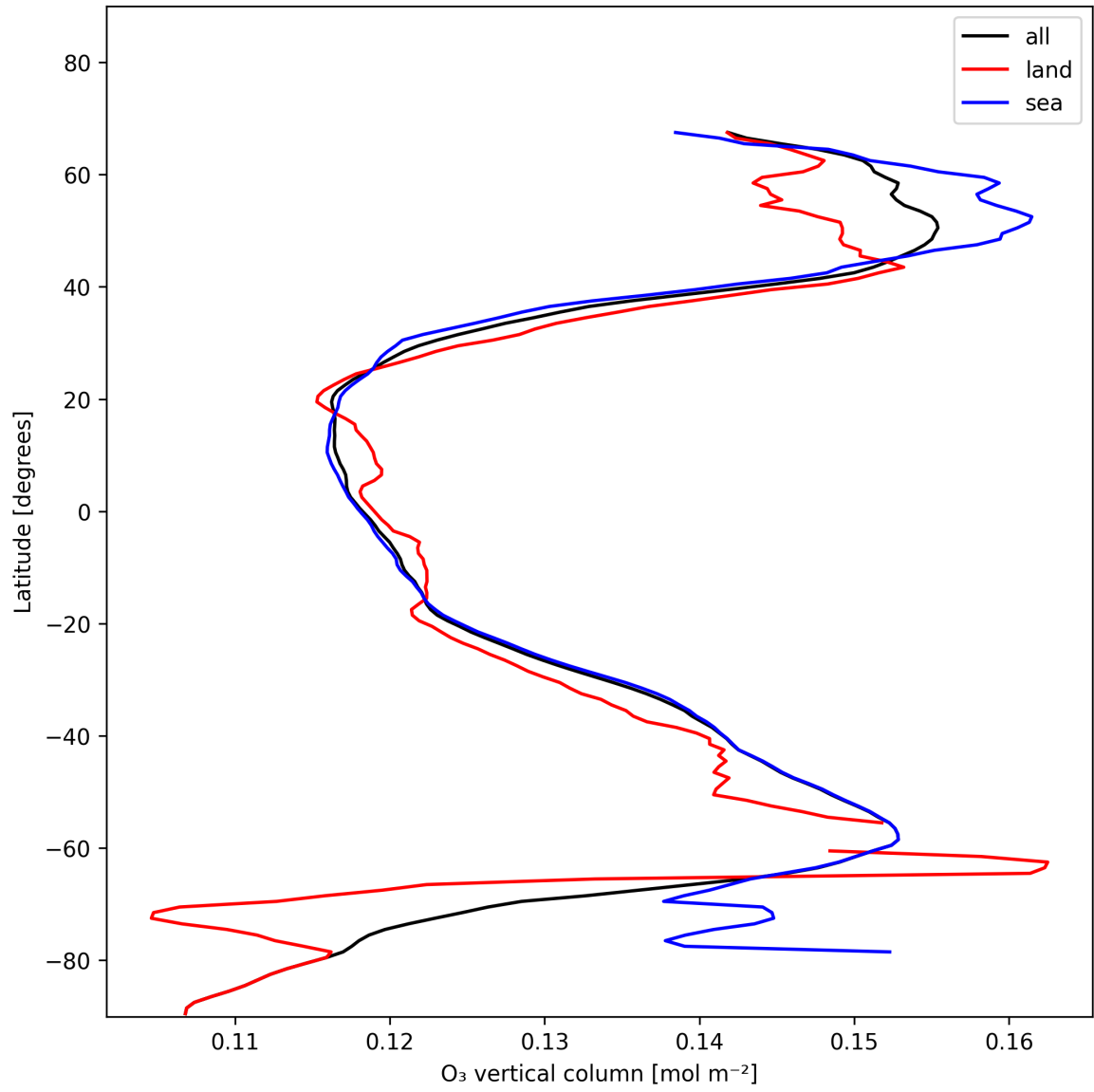
Figure 14: Zonal average of “O 3 vertical column” for 2024-11-28 to 2024-11-30.
