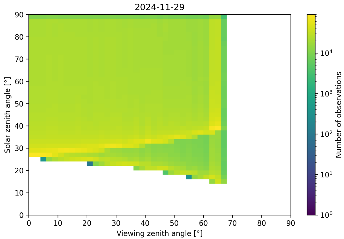
Figure 54: Scatter density plot of “Viewing zenith angle” against “Solar zenith angle” for 2024-11-28 to 2024-11-30.
