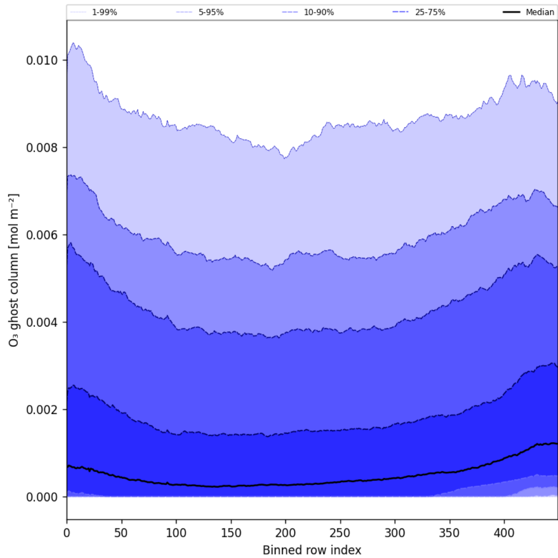
Figure 32: Along track statistics of “O 3 ghost column” for 2024-11-28 to 2024-11-30
