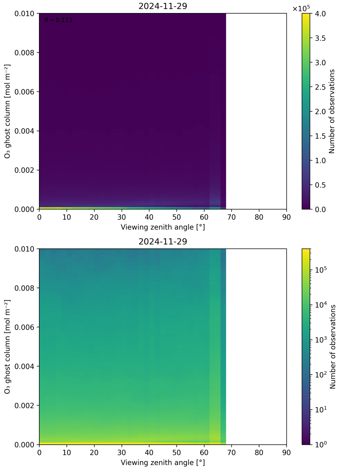
Figure 51: Scatter density plot of “Viewing zenith angle” against “O 3 ghost column” for 2024-11-28 to 2024-11-30.
