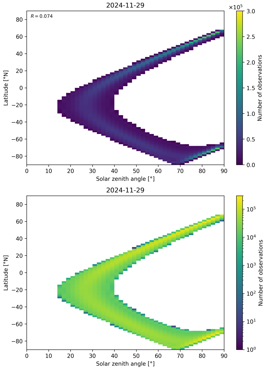
Figure 44: Scatter density plot of “Solar zenith angle” against “Latitude” for 2024-11-28 to 2024-11-30.
