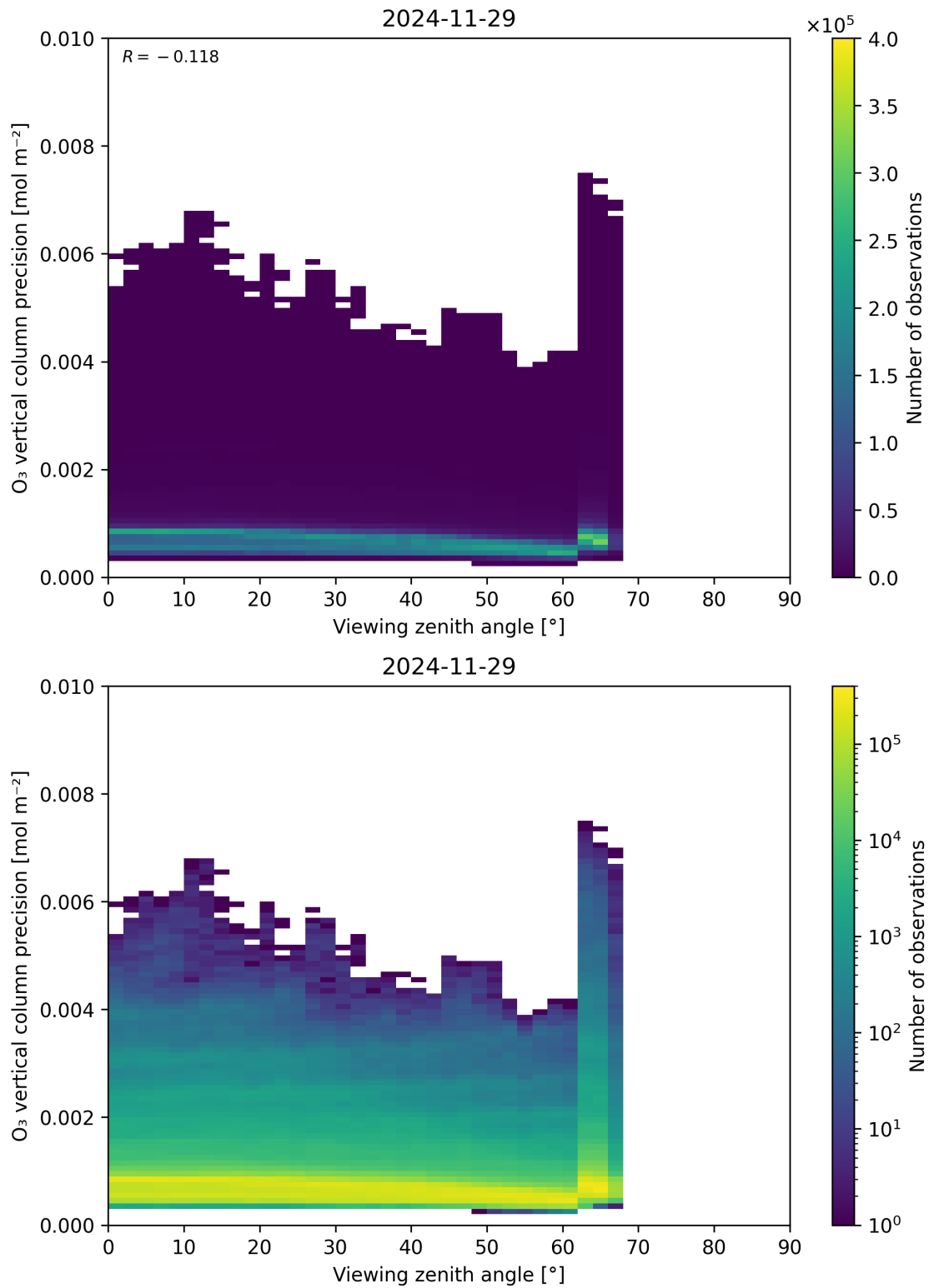
Figure 53: Scatter density plot of “Viewing zenith angle” against “O 3 vertical column precision” for 2024-11-28 to 2024-11-30.
