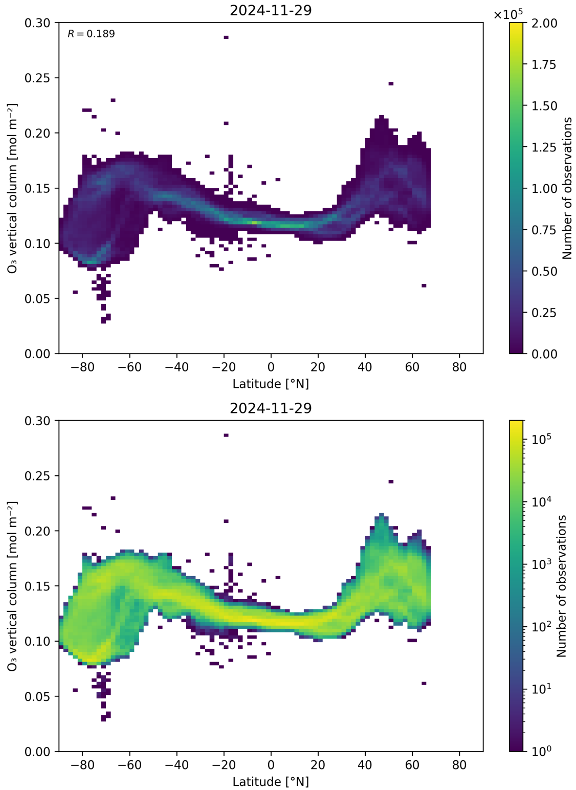
Figure 36: Scatter density plot of “Latitude” against “O 3 vertical column” for 2024-11-28 to 2024-11-30.
