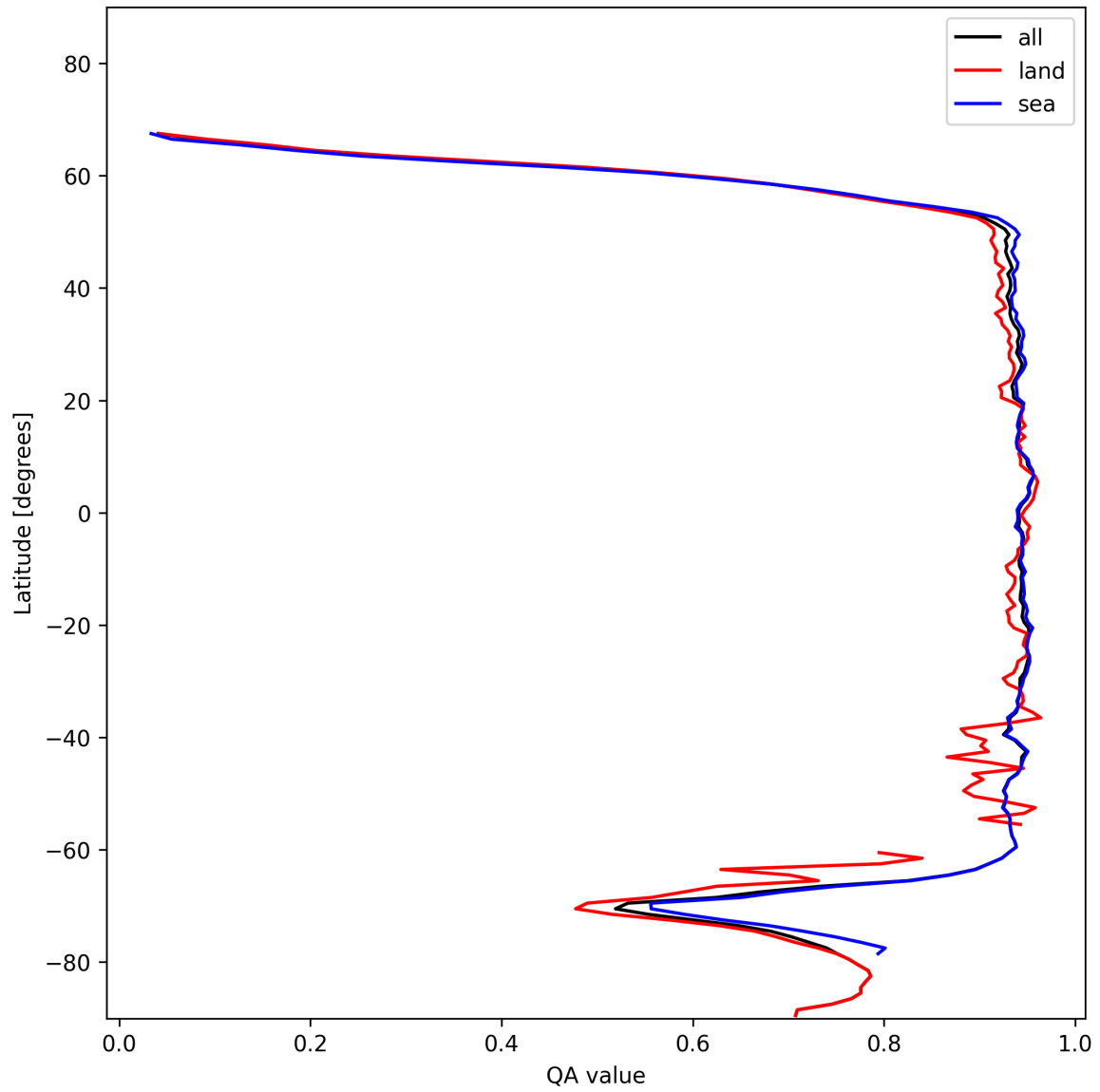
Figure 13: Zonal average of “QA value” for 2024-11-28 to 2024-11-30.
