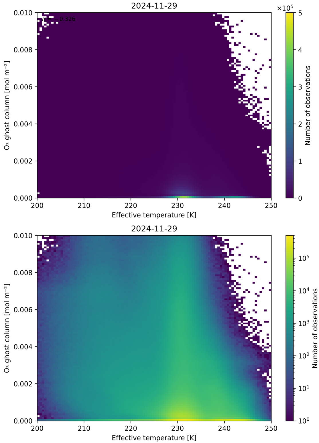
Figure 38: Scatter density plot of “Effective temperature” against “O 3 ghost column” for 2024-11-28 to 2024-11-30.
