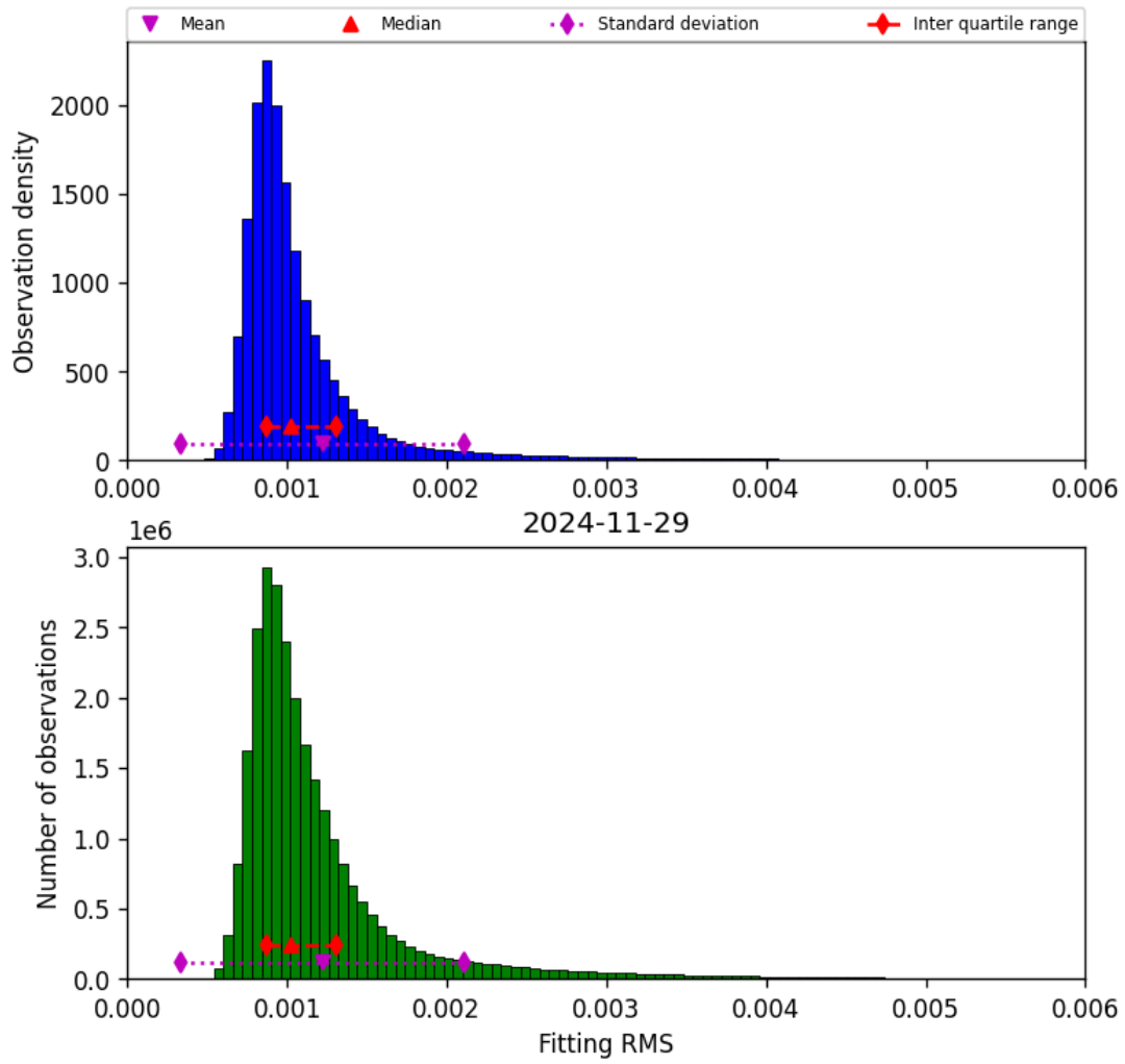
Figure 23: Histogram of “Fitting RMS” for 2024-11-28 to 2024-11-30
