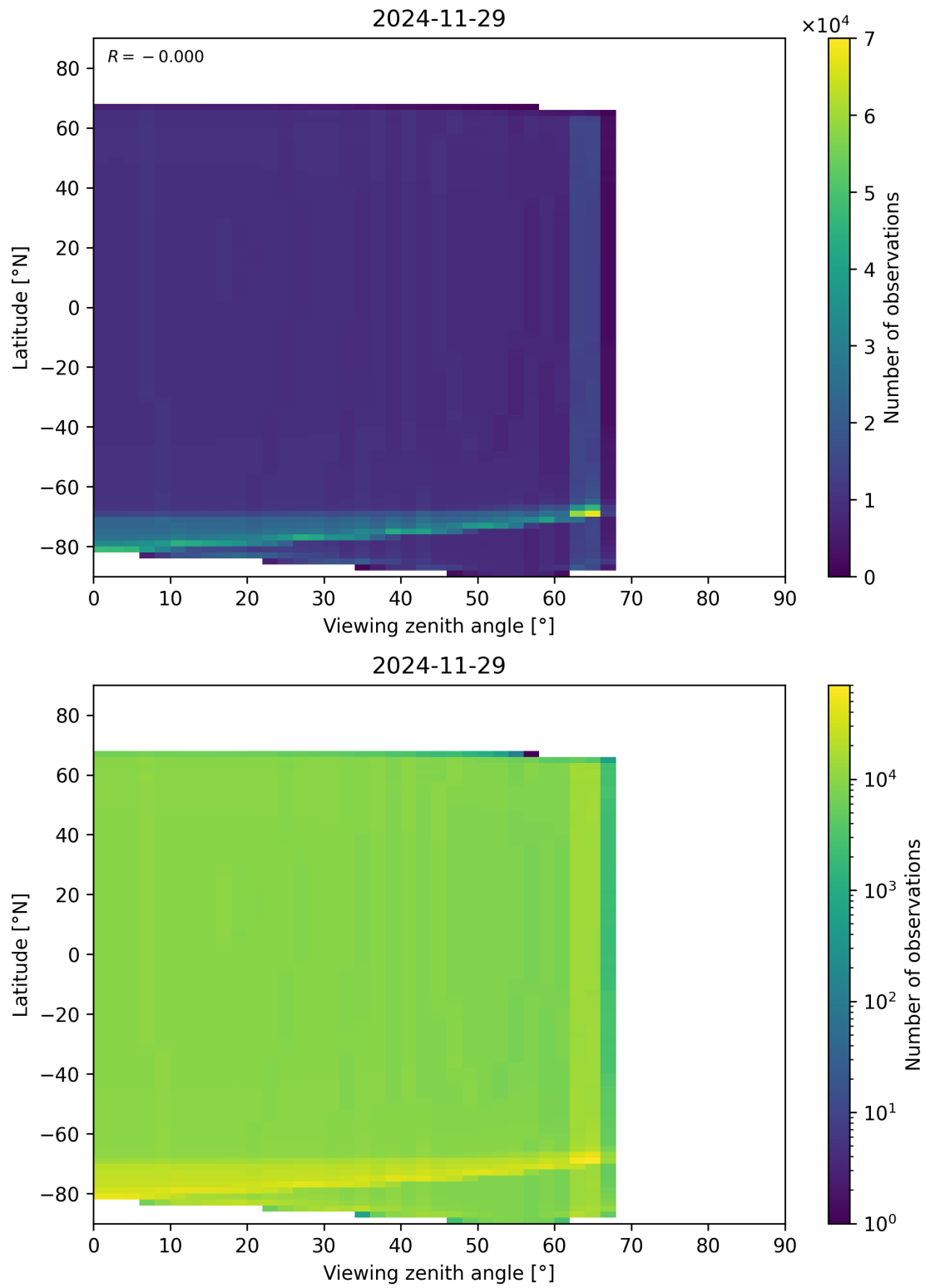
Figure 49: Scatter density plot of “Viewing zenith angle” against “Latitude” for 2024-11-28 to 2024-11-30.
