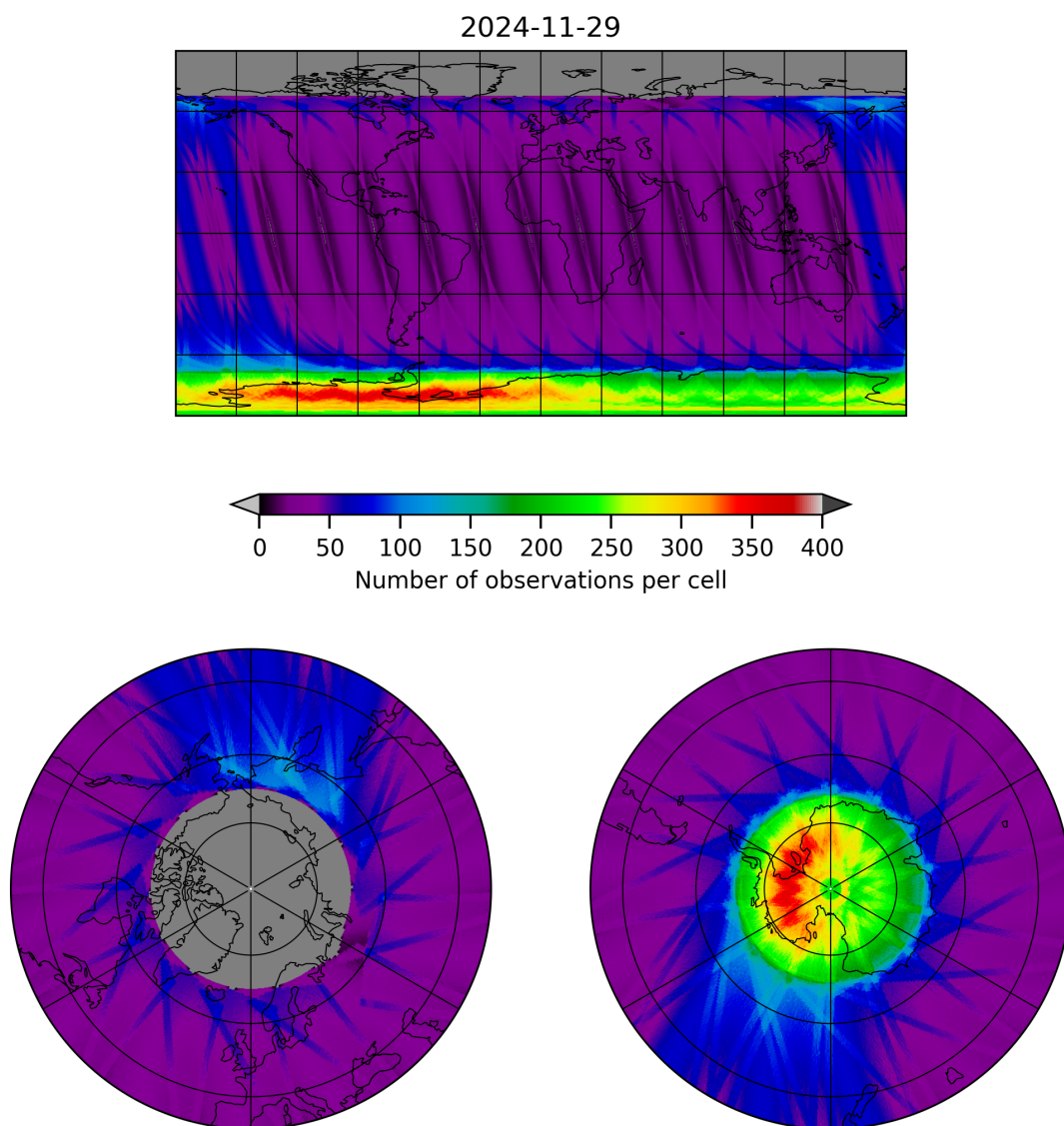
Figure 12: Map of the number of observations for 2024-11-28 to 2024-11-30
