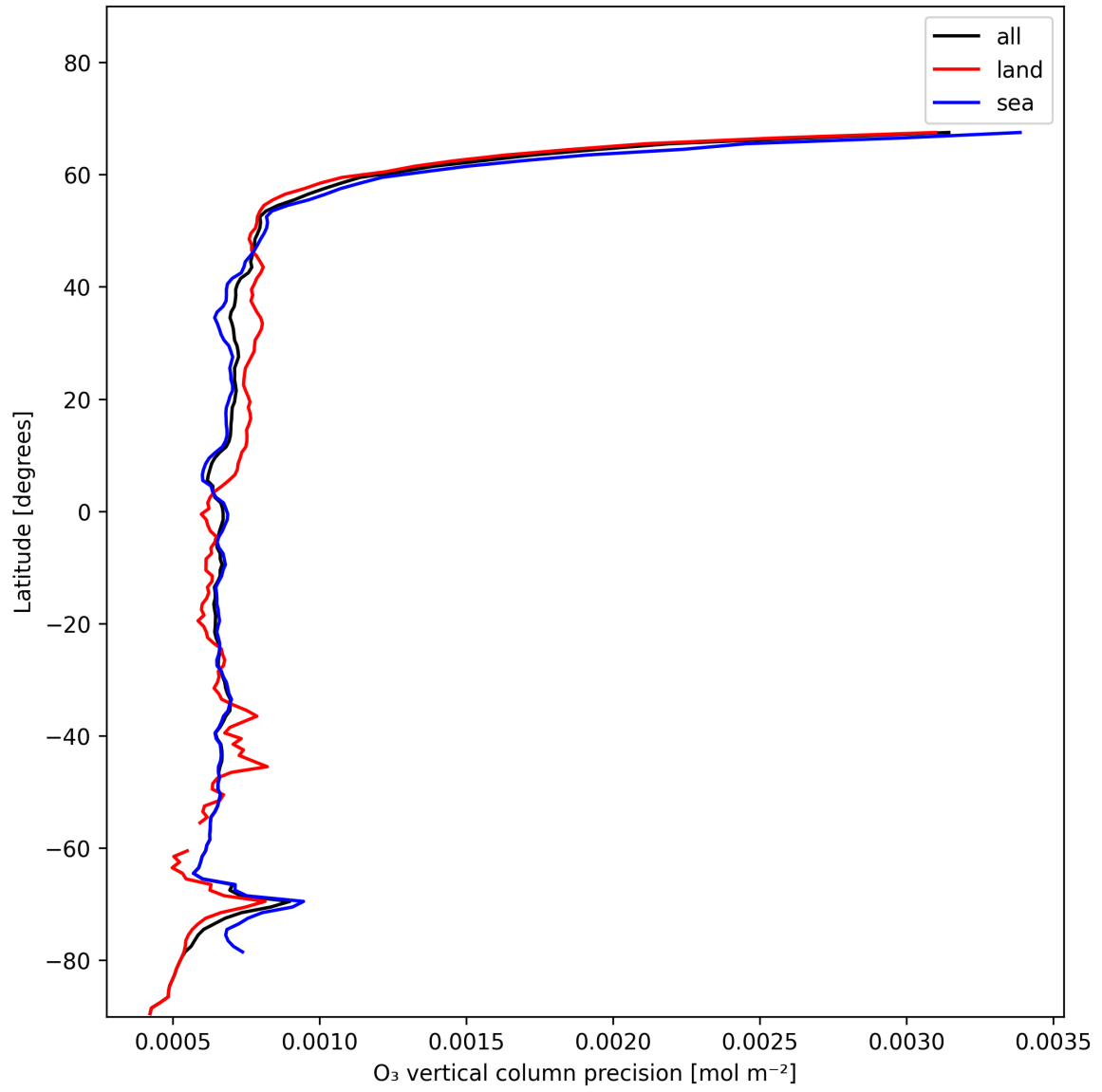
Figure 15: Zonal average of “O 3 vertical column precision” for 2024-11-28 to 2024-11-30.
