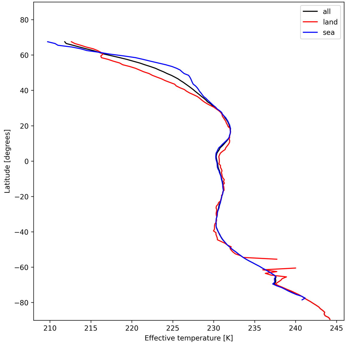
Figure 17: Zonal average of “Effective temperature” for 2024-11-28 to 2024-11-30.
