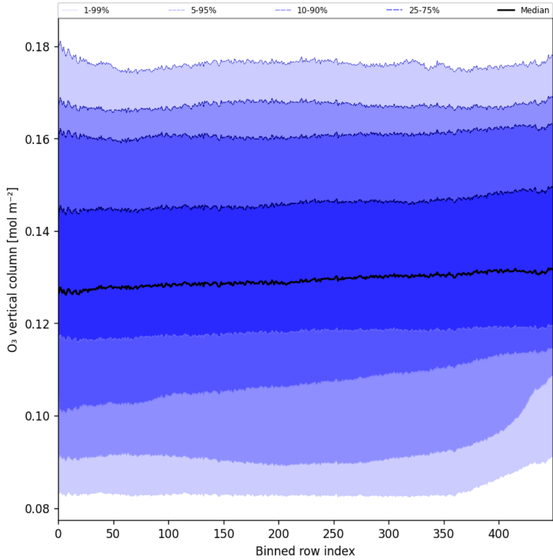
Figure 28: Along track statistics of “O 3 vertical column” for 2024-11-28 to 2024-11-30
