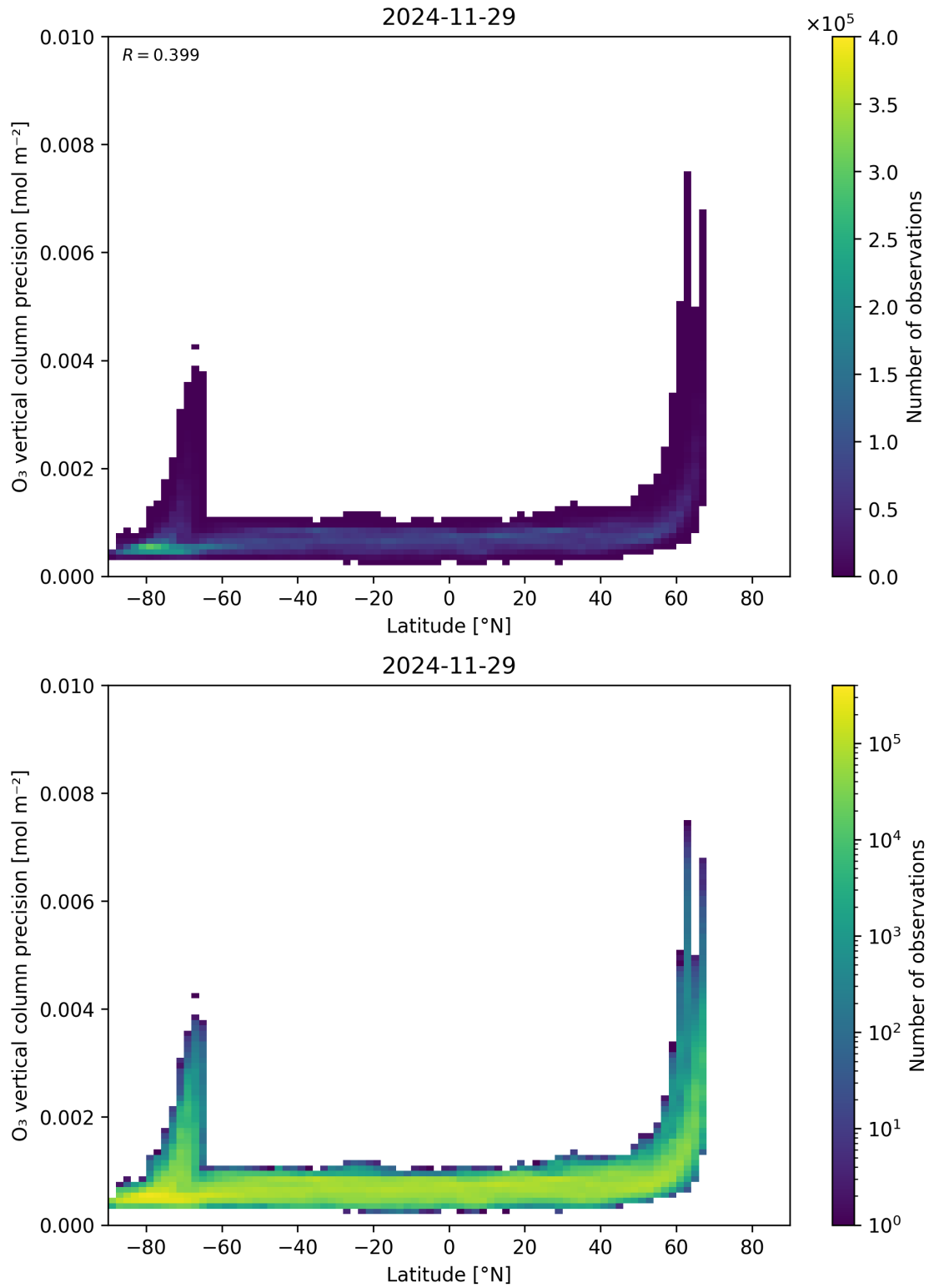
Figure 37: Scatter density plot of “Latitude” against “O 3 vertical column precision” for 2024-11-28 to 2024-11-30.
