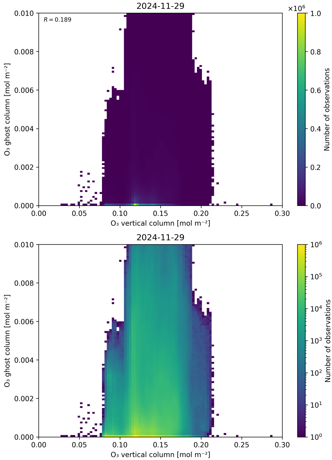
Figure 40: Scatter density plot of “O 3 vertical column” against “O 3 ghost column” for 2024-11-28 to 2024-11-30.
