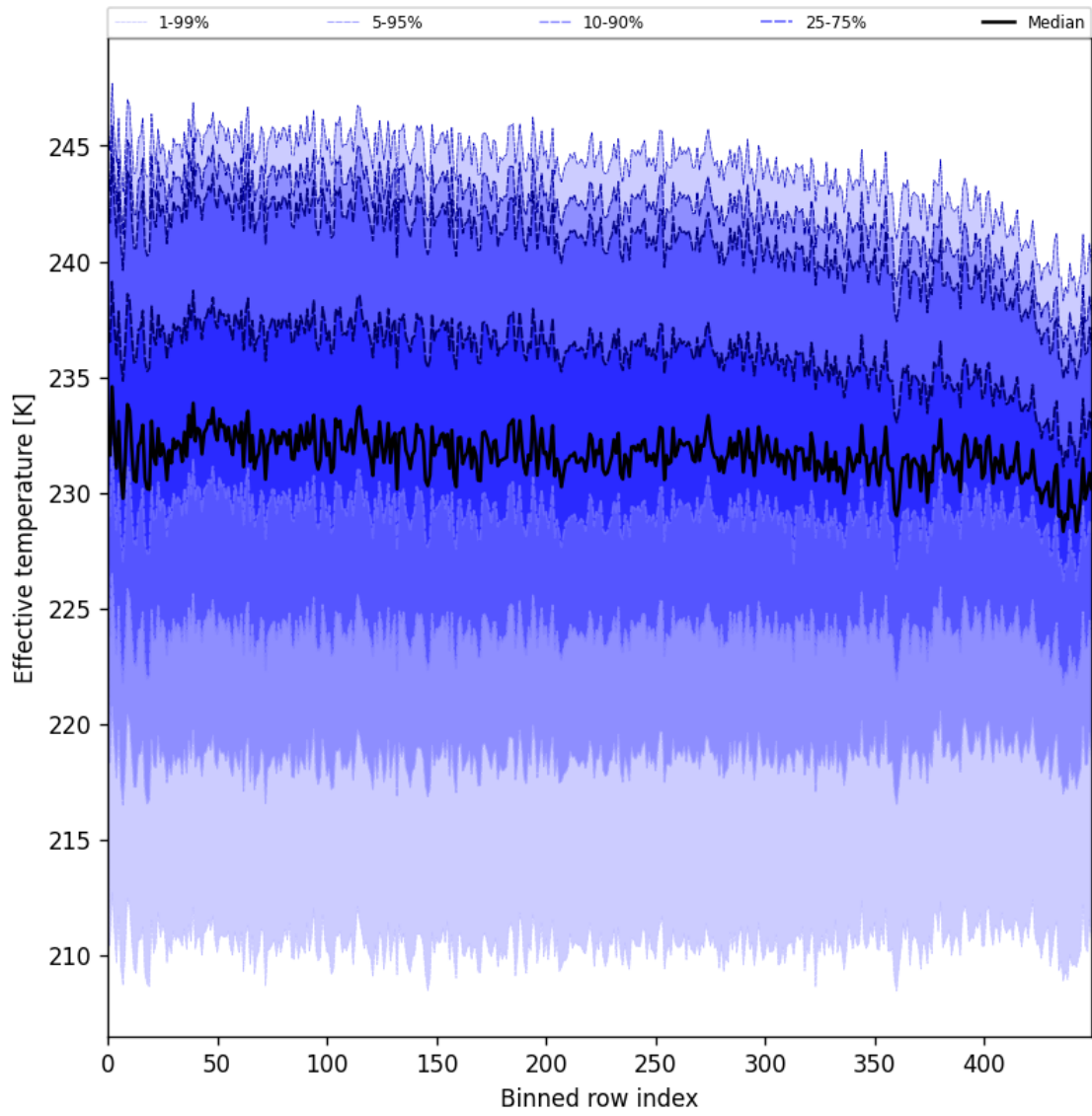
Figure 31: Along track statistics of “Effective temperature” for 2024-11-28 to 2024-11-30
