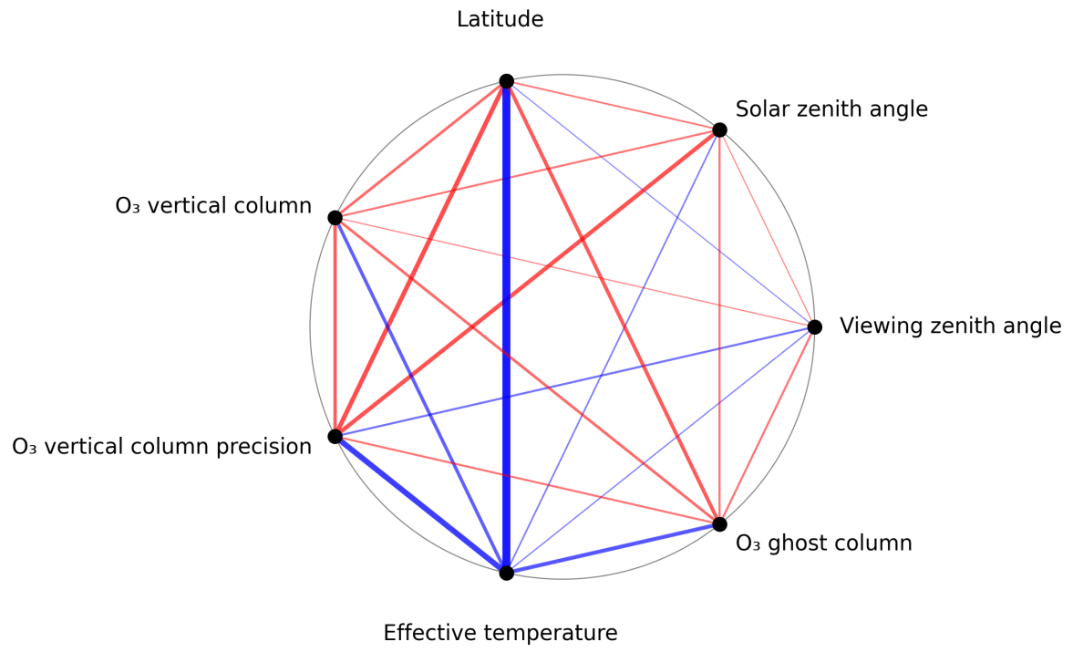
Figure 1: Map of correlation graph for 2024-11-28 to 2024-11-30.
