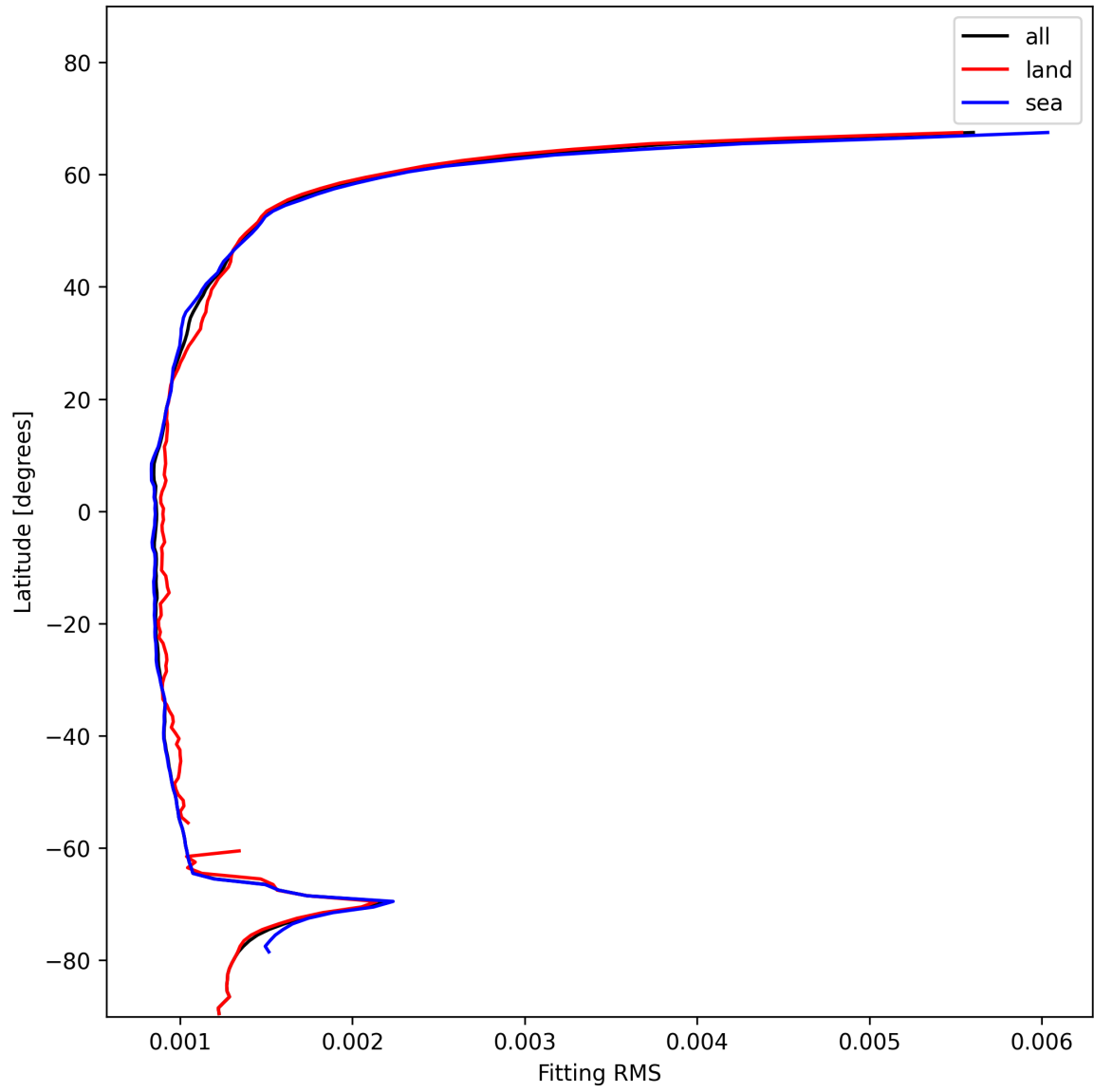
Figure 16: Zonal average of “Fitting RMS” for 2024-11-28 to 2024-11-30.
