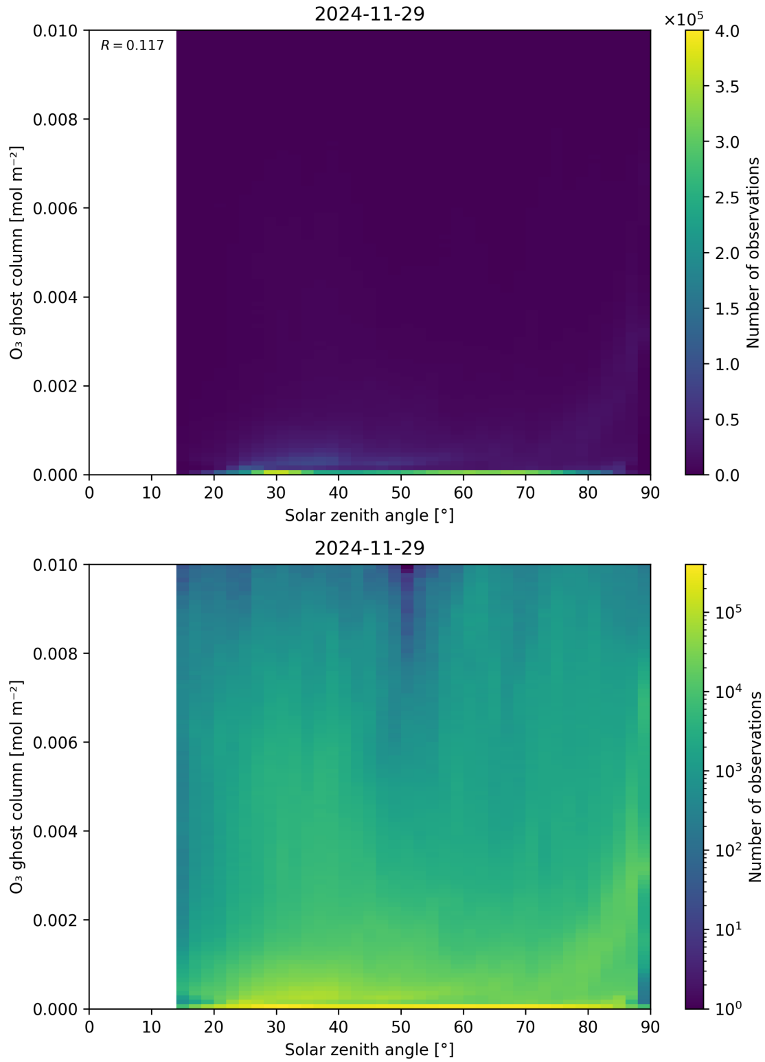
Figure 46: Scatter density plot of “Solar zenith angle” against “O 3 ghost column” for 2024-11-28 to 2024-11-30.
