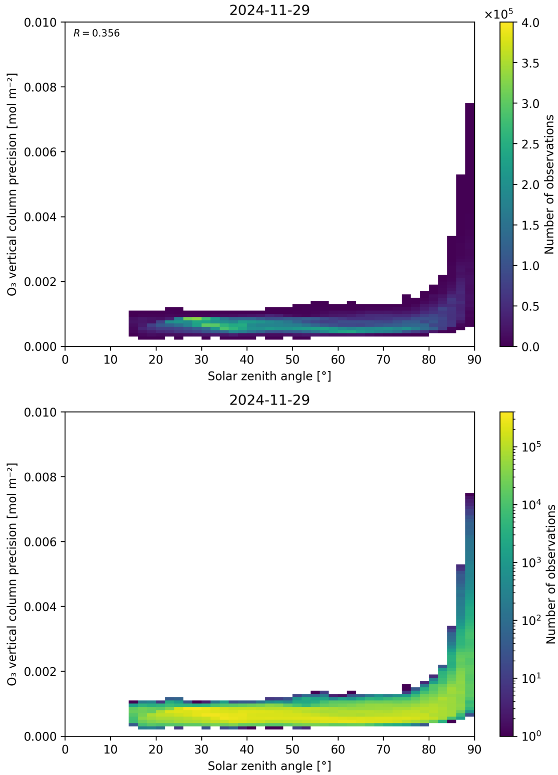
Figure 48: Scatter density plot of “Solar zenith angle” against “O 3 vertical column precision” for 2024-11-28 to 2024-11-30.
