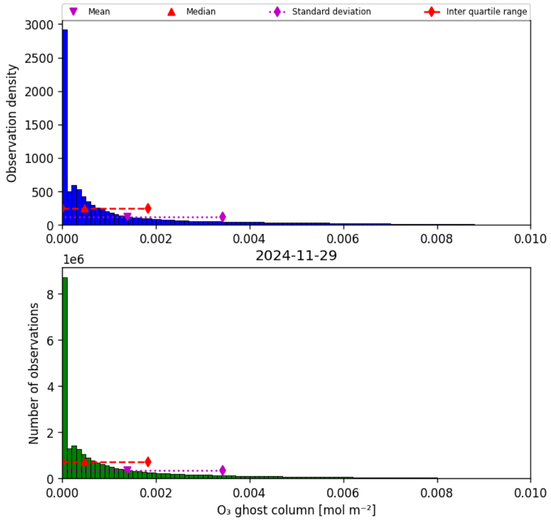
Figure 25: Histogram of “O 3 ghost column” for 2024-11-28 to 2024-11-30
