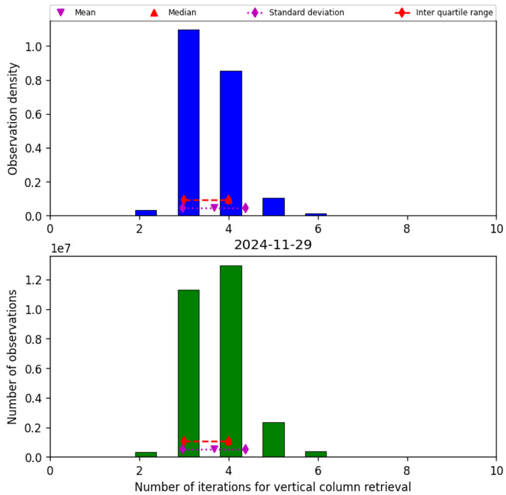
Figure 26: Histogram of “Number of iterations for vertical column retrieval” for 2024-11-28 to 2024-11-30
