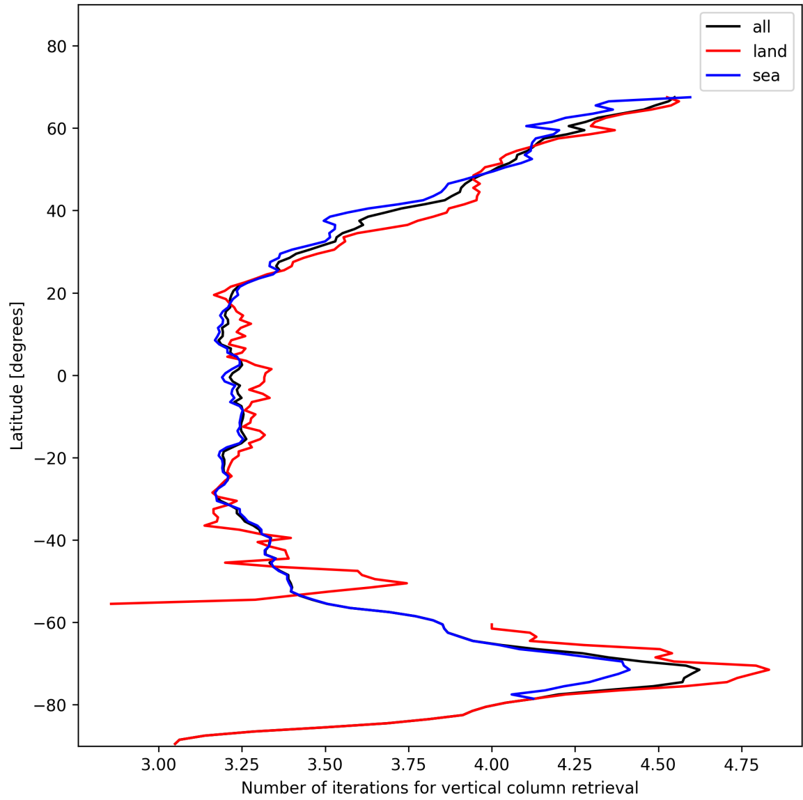
Figure 19: Zonal average of “Number of iterations for vertical column retrieval” for 2024-11-28 to 2024-11-30.
