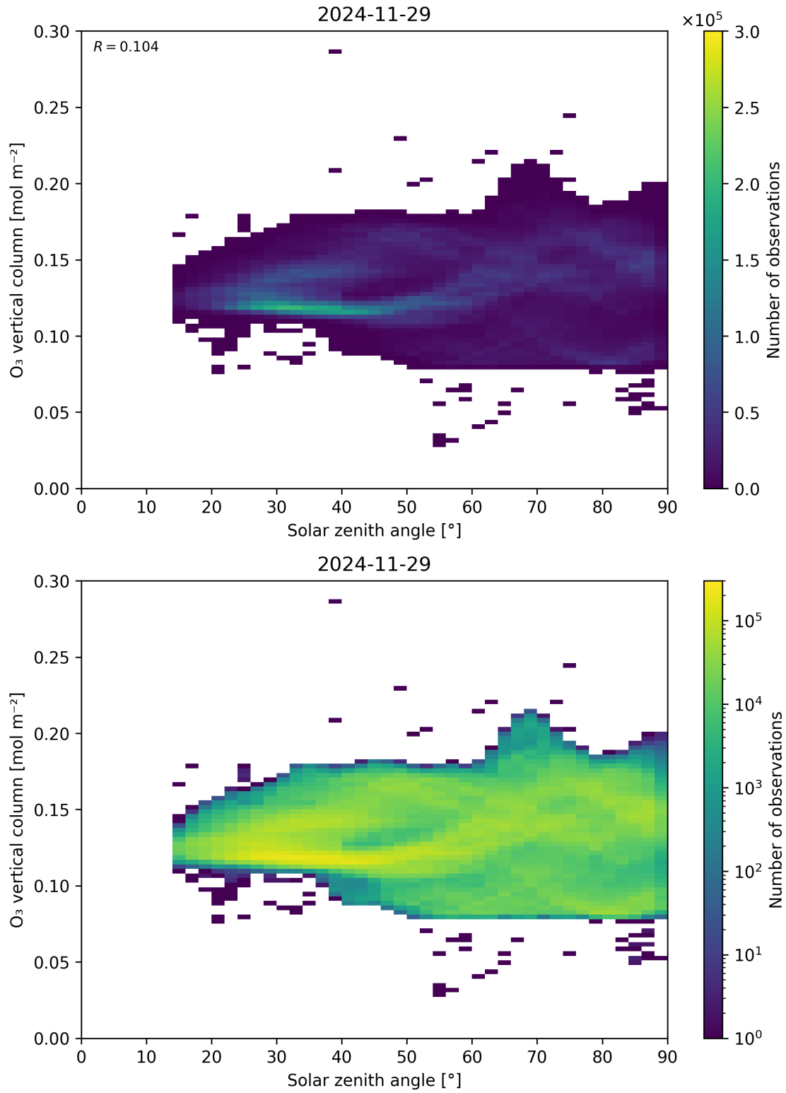
Figure 47: Scatter density plot of “Solar zenith angle” against “O 3 vertical column” for 2024-11-28 to 2024-11-30.
