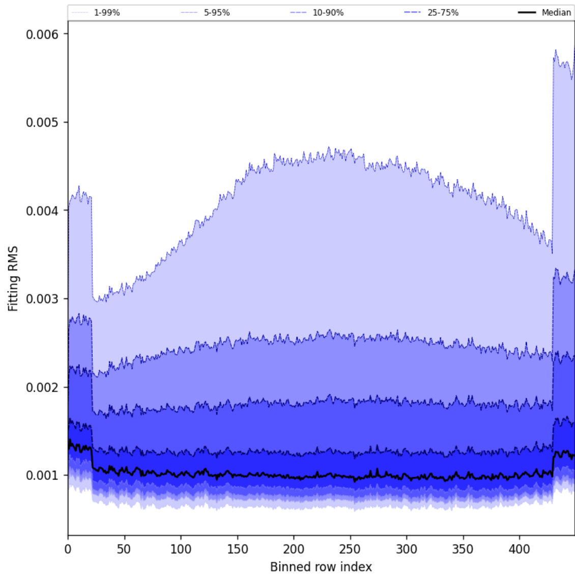
Figure 30: Along track statistics of “Fitting RMS” for 2024-11-28 to 2024-11-30
