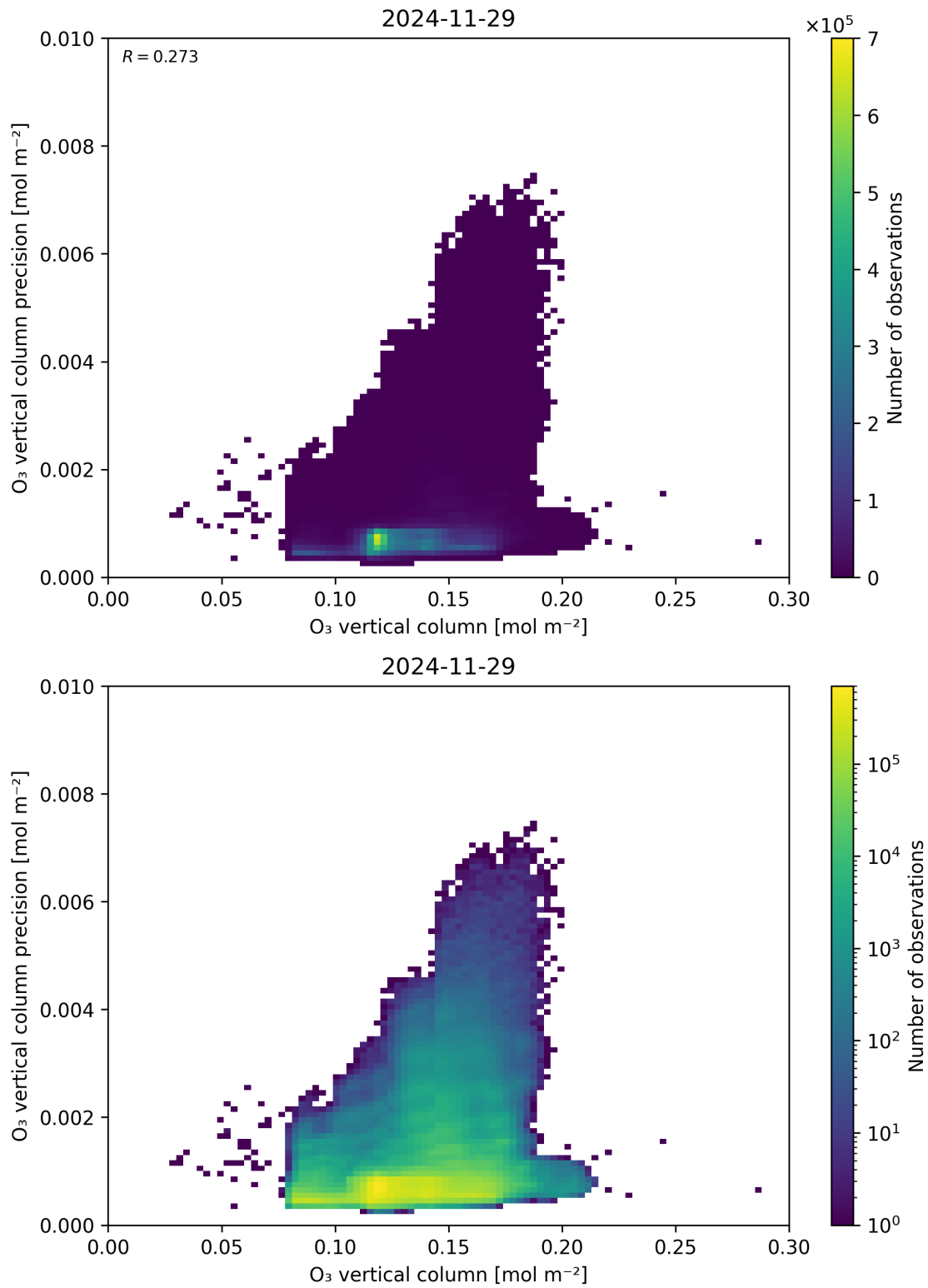
Figure 41: Scatter density plot of “O 3 vertical column” against “O 3 vertical column precision” for 2024-11-28 to 2024-11-30.
