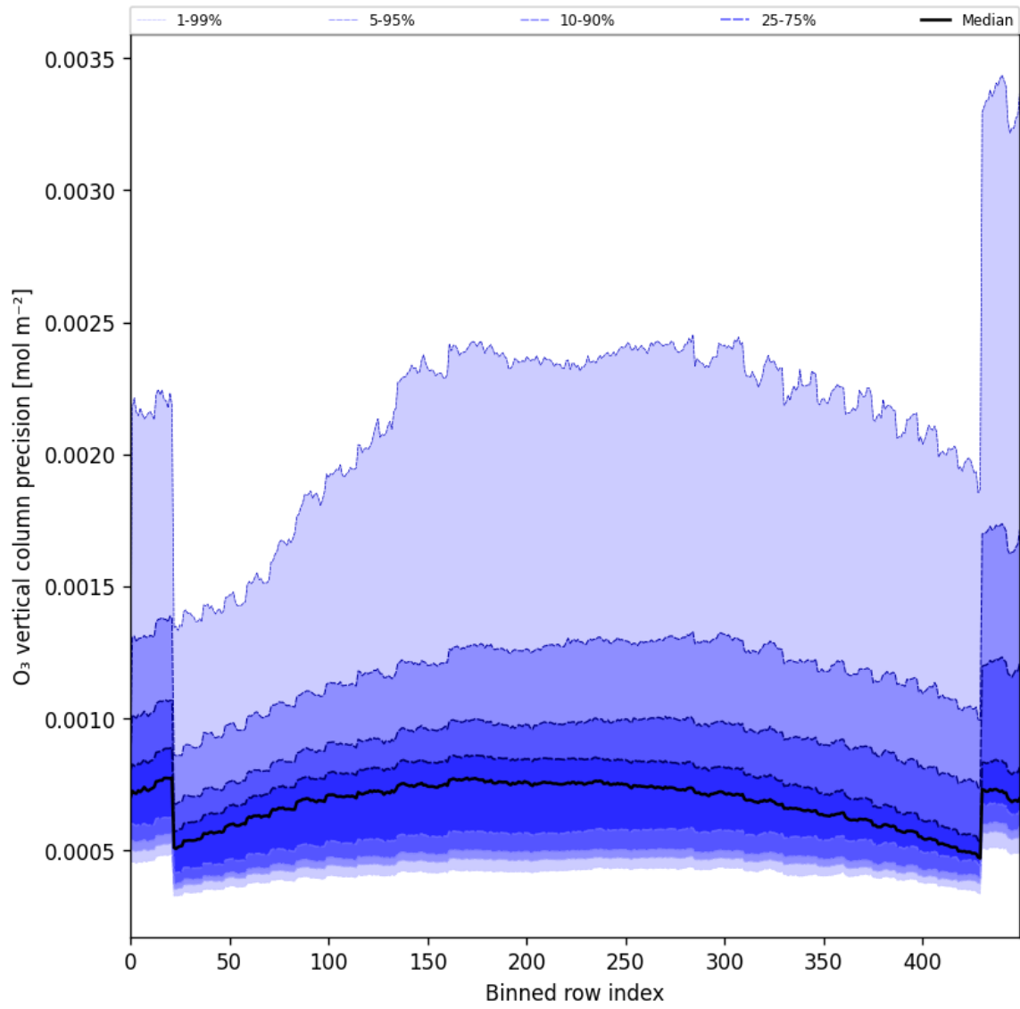
Figure 29: Along track statistics of “O 3 vertical column precision” for 2024-11-28 to 2024-11-30
