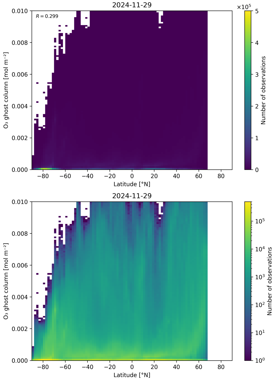
Figure 35: Scatter density plot of “Latitude” against “O 3 ghost column” for 2024-11-28 to 2024-11-30.
