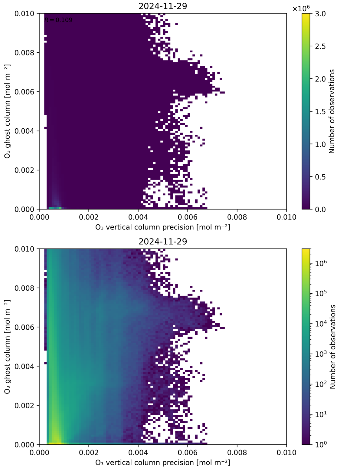
Figure 43: Scatter density plot of “ O_3 vertical column precision” against “ O_3 ghost column” for 2024-11-28 to 2024-11-30.
