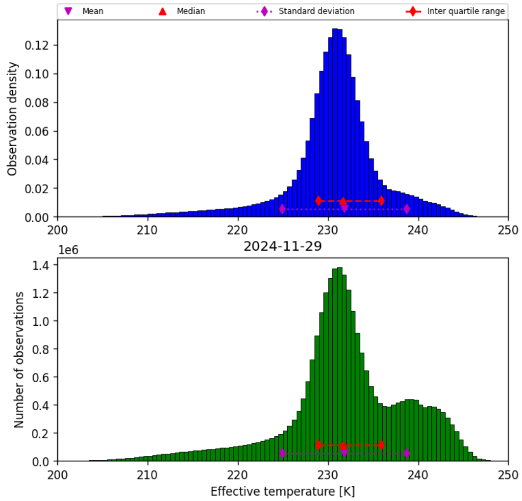
Figure 24: Histogram of “Effective temperature” for 2024-11-28 to 2024-11-30
