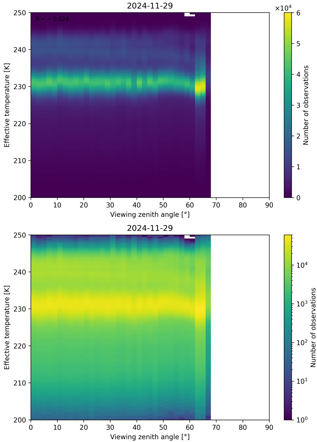
Figure 50: Scatter density plot of “Viewing zenith angle” against “Effective temperature” for 2024-11-28 to 2024-11-30.
