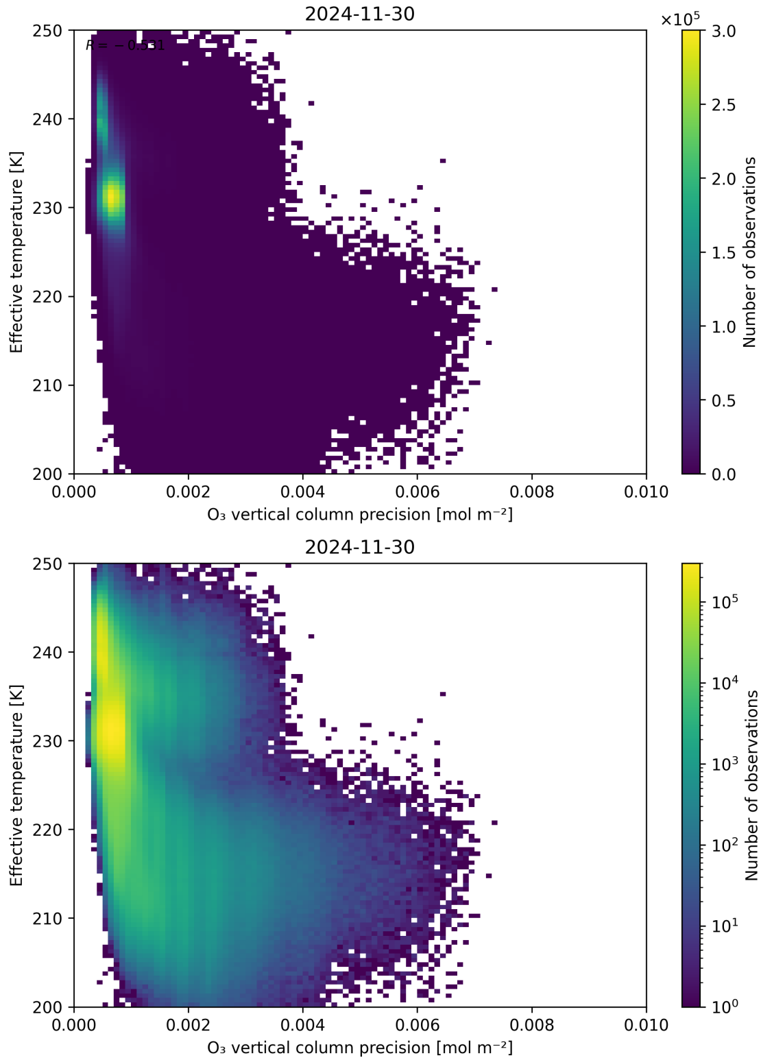
Figure 42: Scatter density plot of “O 3 vertical column precision” against “Effective temperature” for 2024-11-30 to 2024-12-01.
