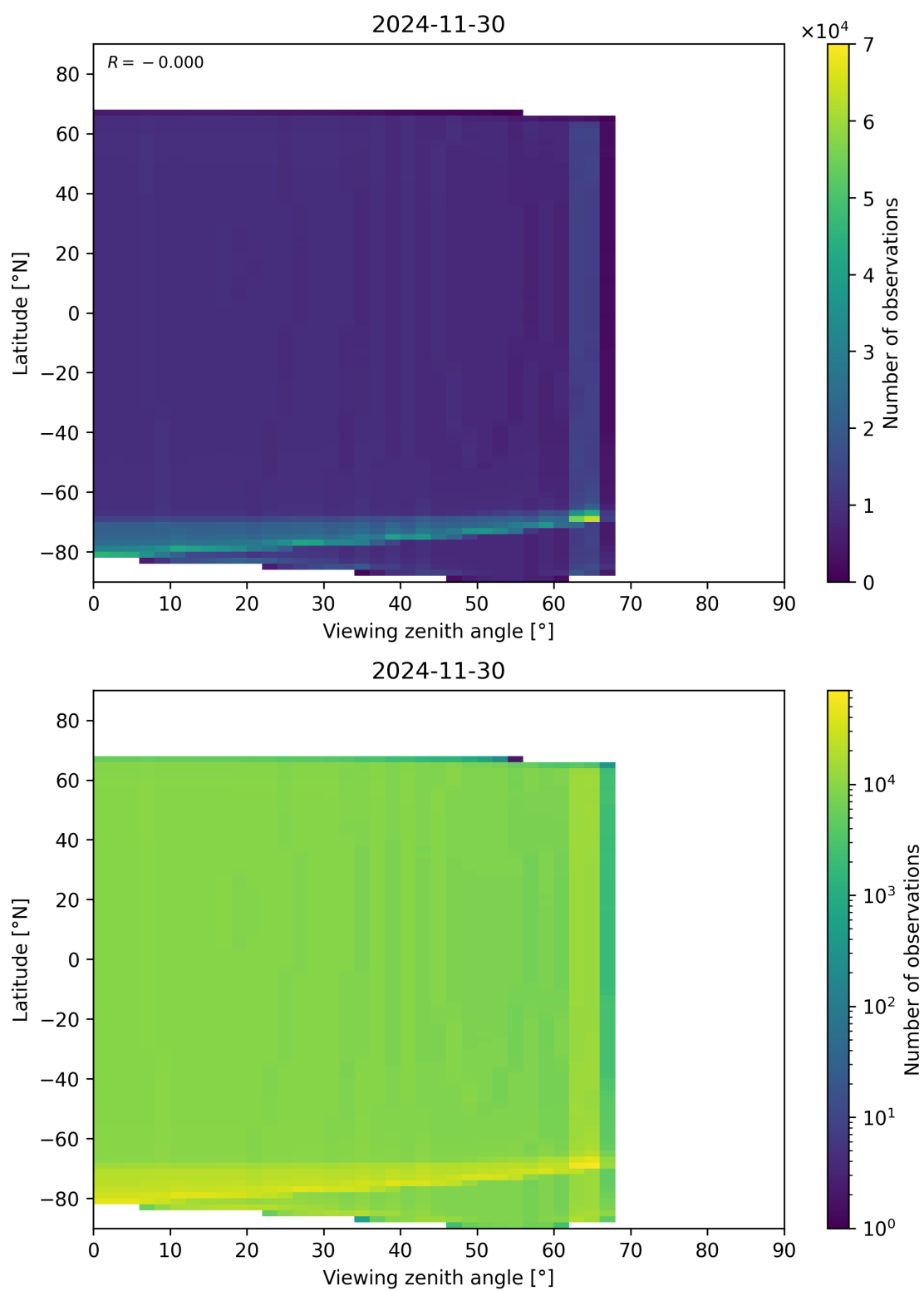
Figure 49: Scatter density plot of “Viewing zenith angle” against “Latitude” for 2024-11-30 to 2024-12-01.
