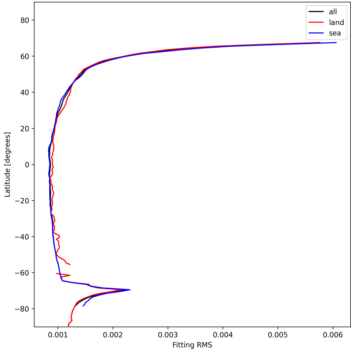
Figure 16: Zonal average of “Fitting RMS” for 2024-11-30 to 2024-12-01.
