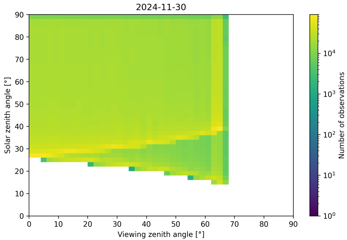
Figure 54: Scatter density plot of “Viewing zenith angle” against “Solar zenith angle” for 2024-11-30 to 2024-12-01.
