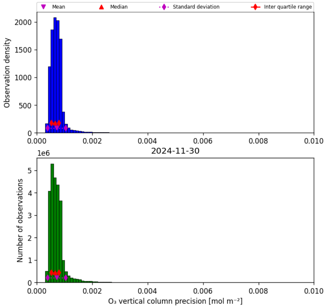
Figure 22: Histogram of “O 3 vertical column precision” for 2024-11-30 to 2024-12-01
