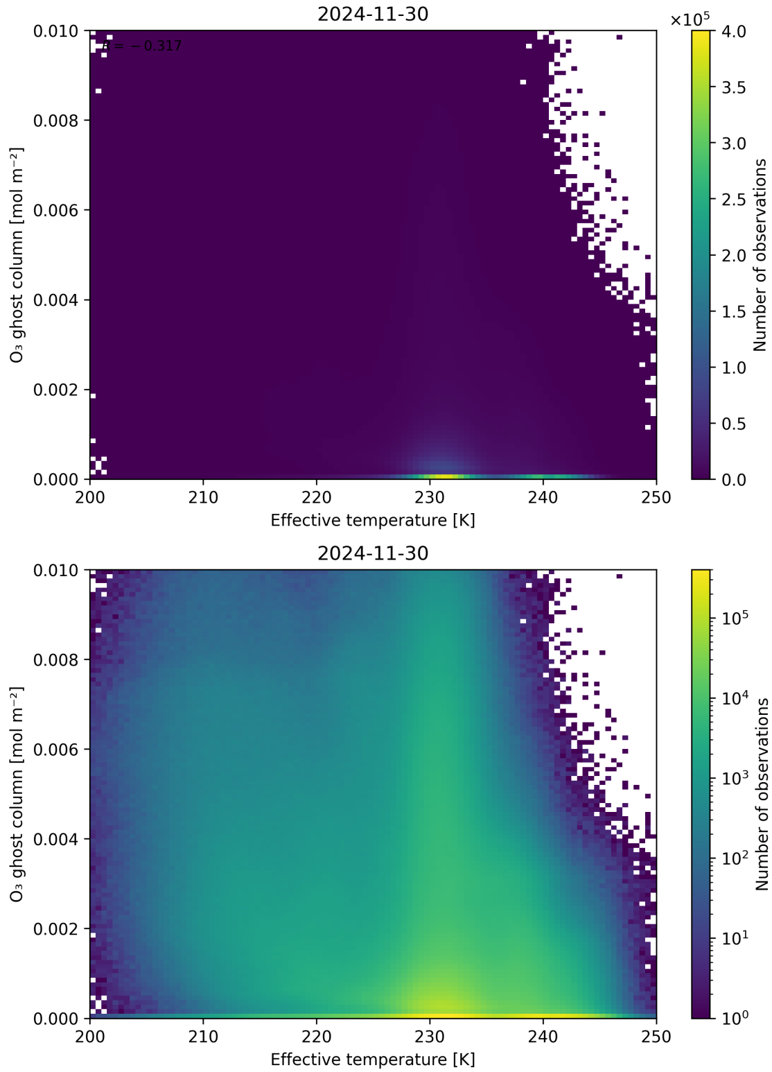
Figure 38: Scatter density plot of “Effective temperature” against “O 3 ghost column” for 2024-11-30 to 2024-12-01.
