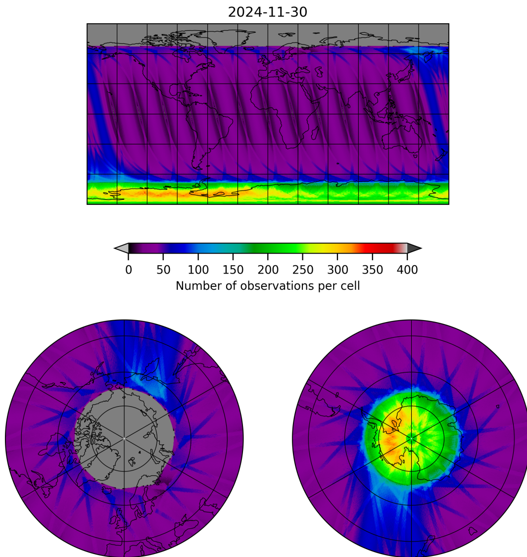
Figure 12: Map of the number of observations for 2024-11-30 to 2024-12-01
