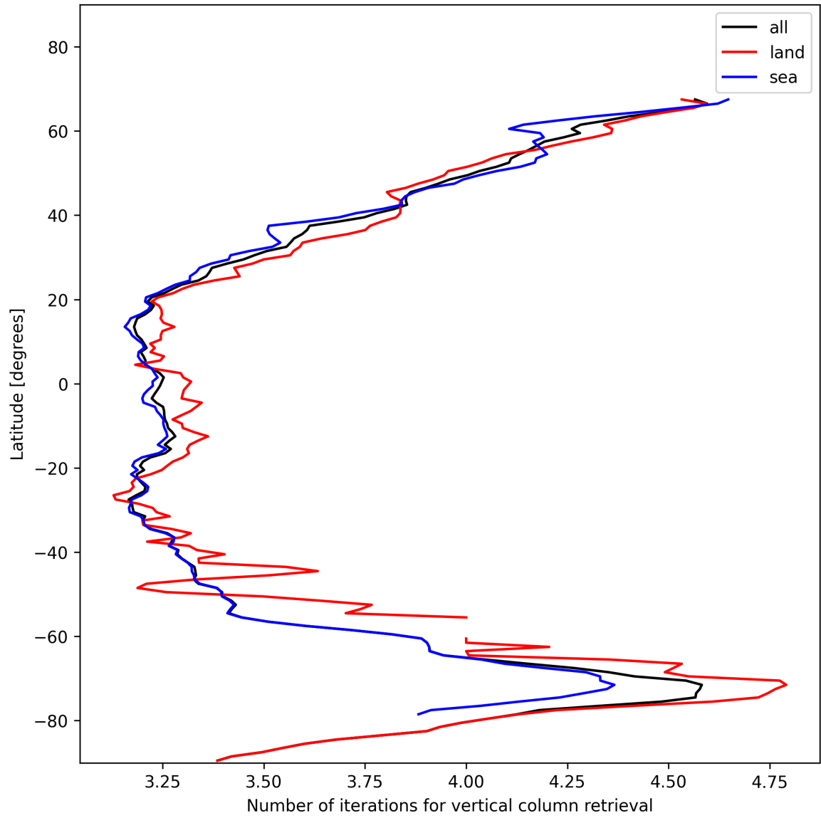
Figure 19: Zonal average of “Number of iterations for vertical column retrieval” for 2024-11-30 to 2024-12-01.
