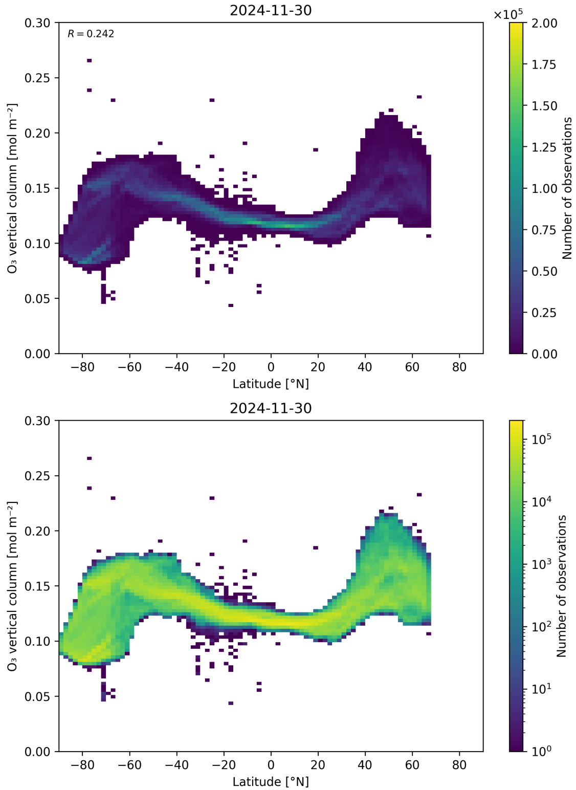
Figure 36: Scatter density plot of “Latitude” against “O 3 vertical column” for 2024-11-30 to 2024-12-01.
