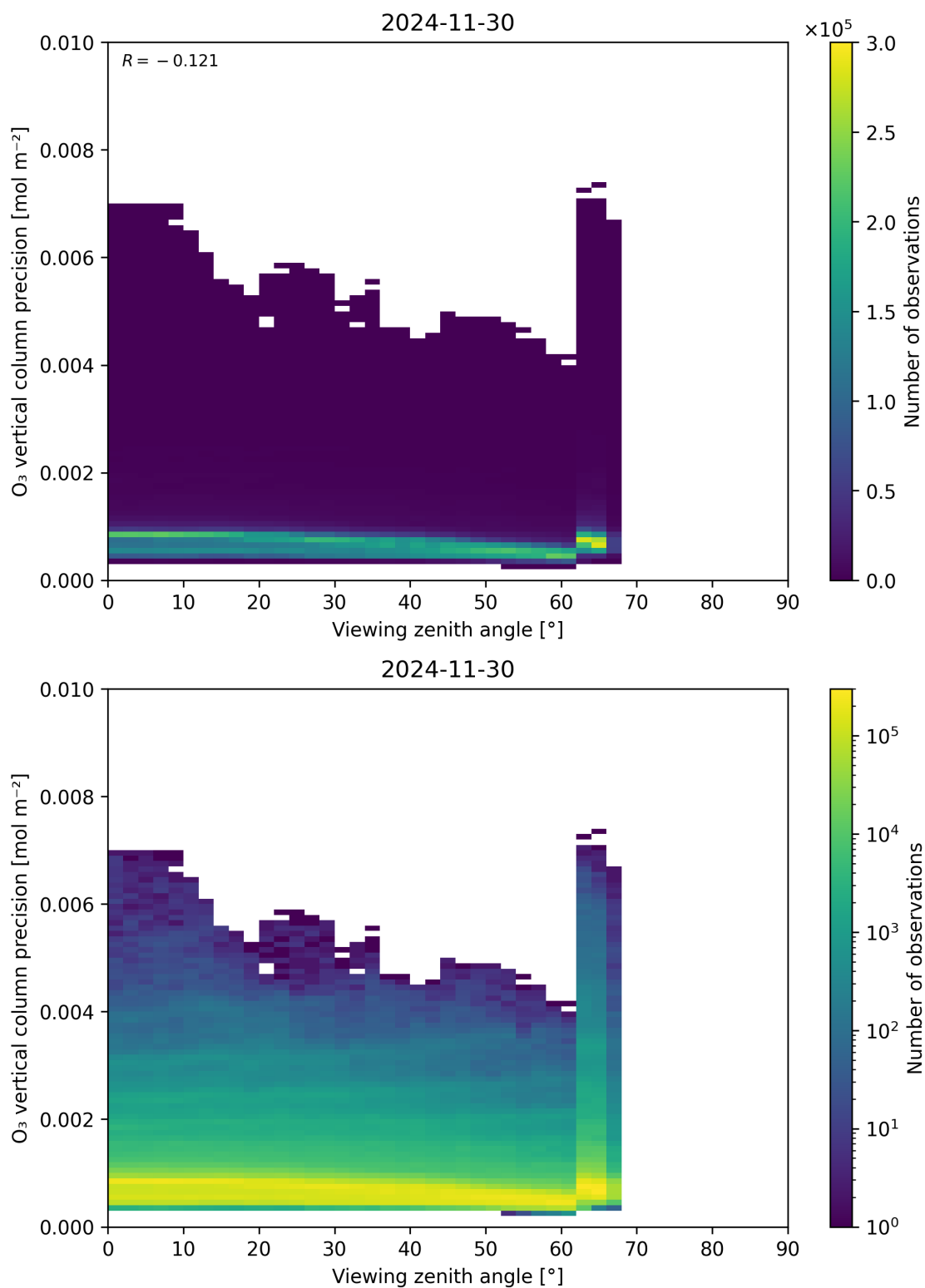
Figure 53: Scatter density plot of “Viewing zenith angle” against “O 3 vertical column precision” for 2024-11-30 to 2024-12-01.
