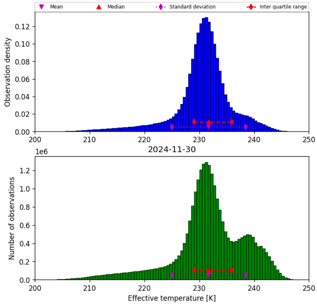
Figure 24: Histogram of “Effective temperature” for 2024-11-30 to 2024-12-01
