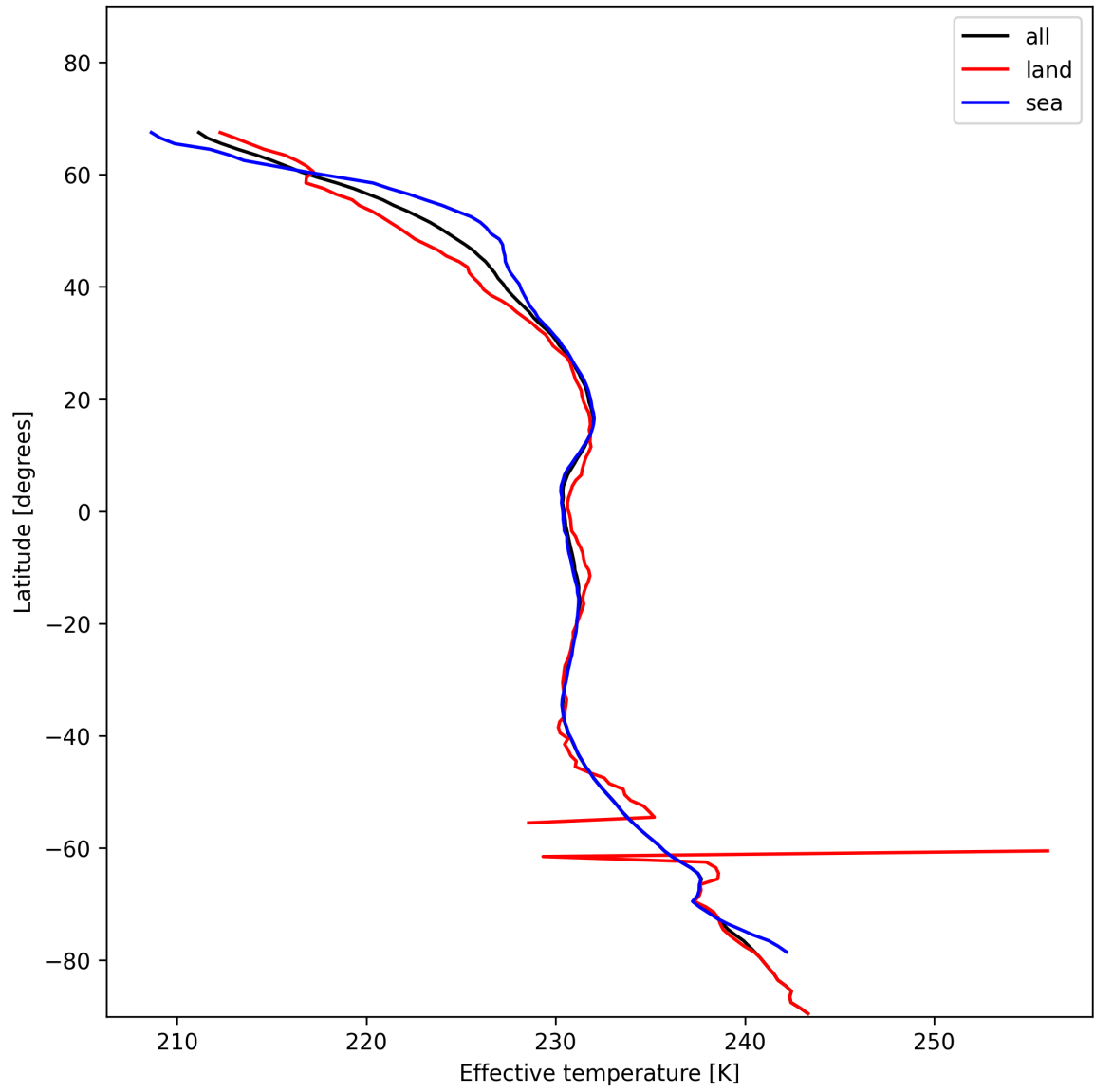
Figure 17: Zonal average of “Effective temperature” for 2024-11-30 to 2024-12-01.
