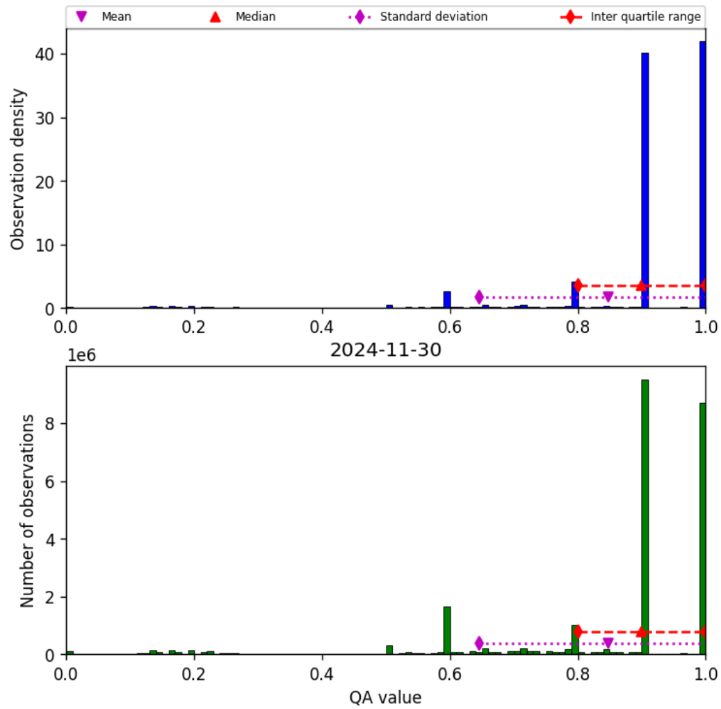
Figure 20: Histogram of “QA value” for 2024-11-30 to 2024-12-01
