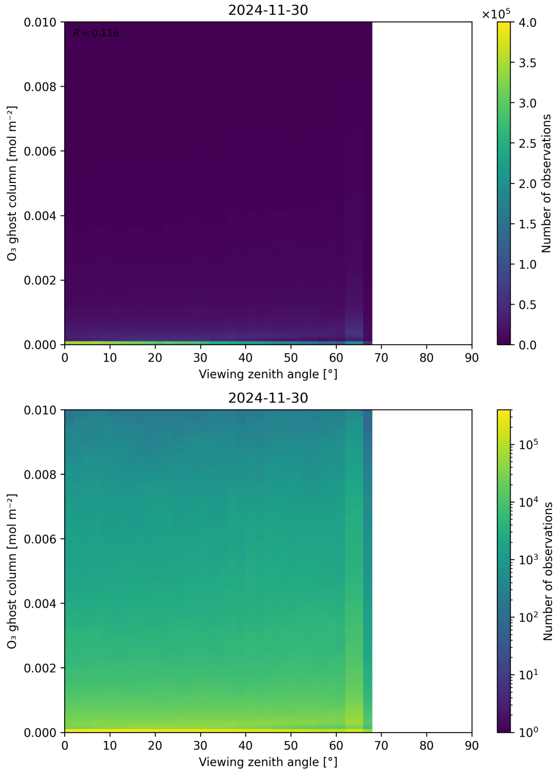
Figure 51: Scatter density plot of “Viewing zenith angle” against “O 3 ghost column” for 2024-11-30 to 2024-12-01.
