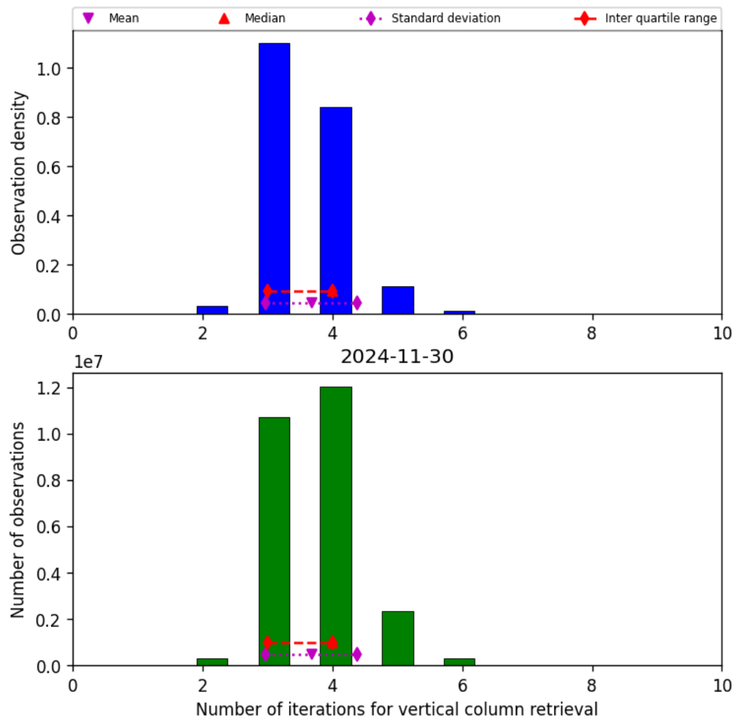
Figure 26: Histogram of “Number of iterations for vertical column retrieval” for 2024-11-30 to 2024-12-01
