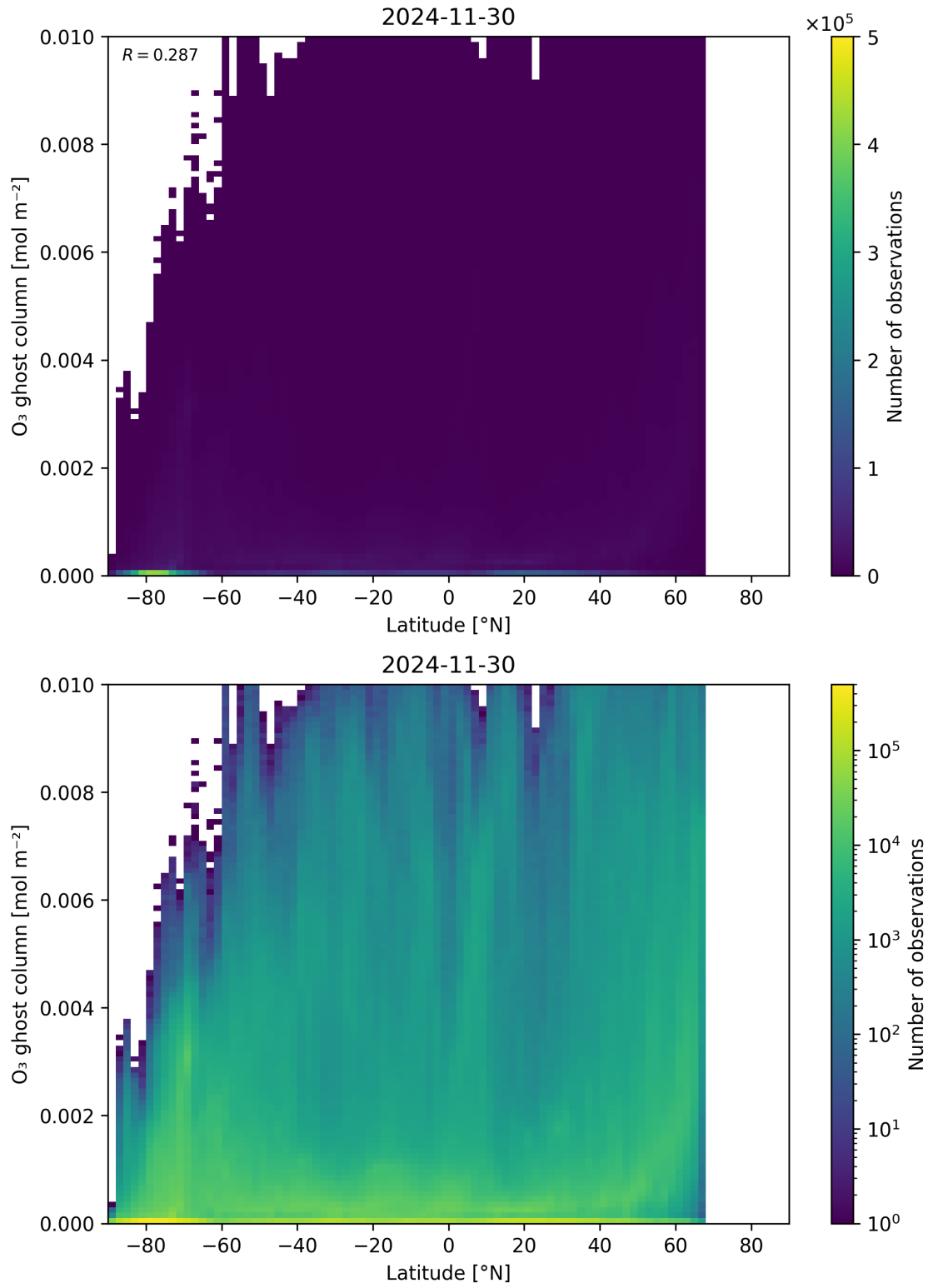
Figure 35: Scatter density plot of “Latitude” against “O 3 ghost column” for 2024-11-30 to 2024-12-01.
