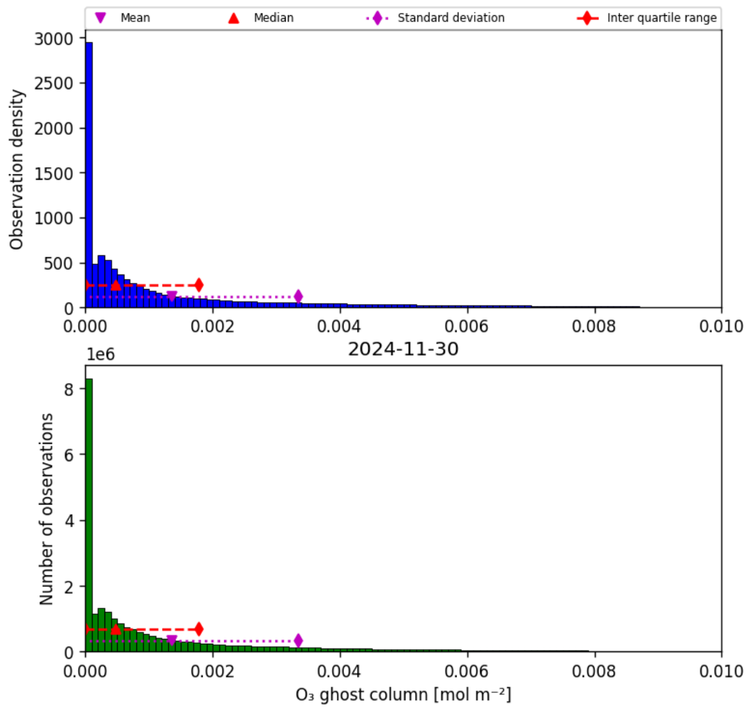
Figure 25: Histogram of “O 3 ghost column” for 2024-11-30 to 2024-12-01
