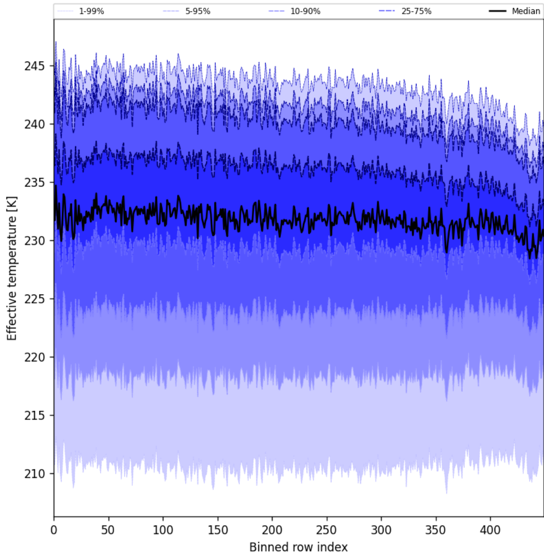
Figure 31: Along track statistics of “Effective temperature” for 2024-11-30 to 2024-12-01
