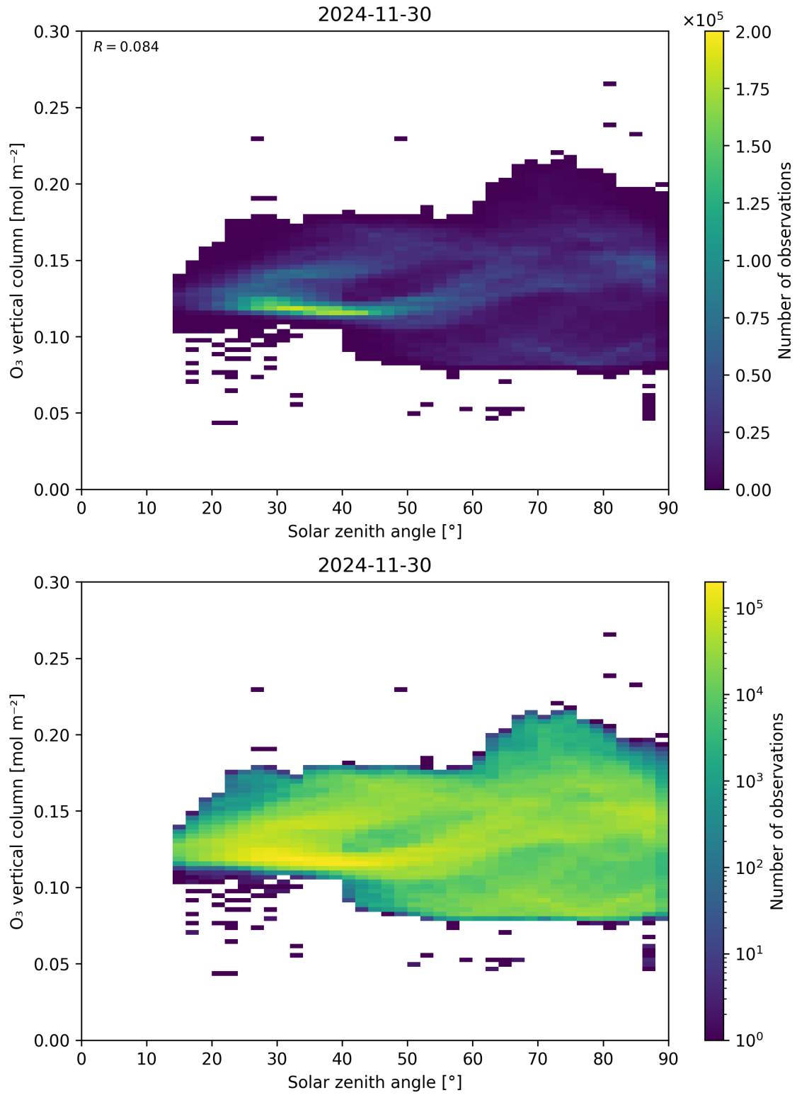
Figure 47: Scatter density plot of “Solar zenith angle” against “O 3 vertical column” for 2024-11-30 to 2024-12-01.
