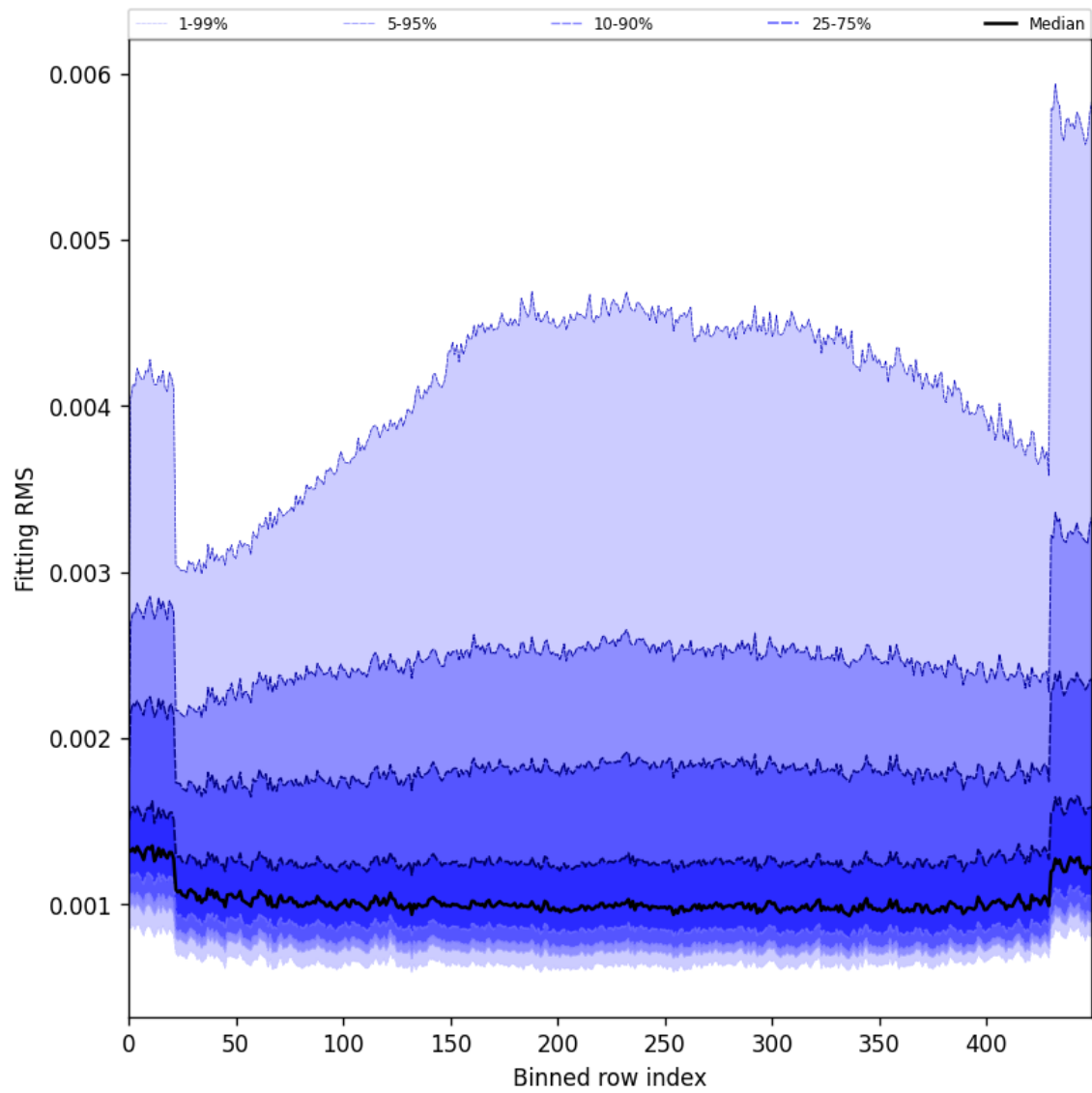
Figure 30: Along track statistics of “Fitting RMS” for 2024-11-30 to 2024-12-01
