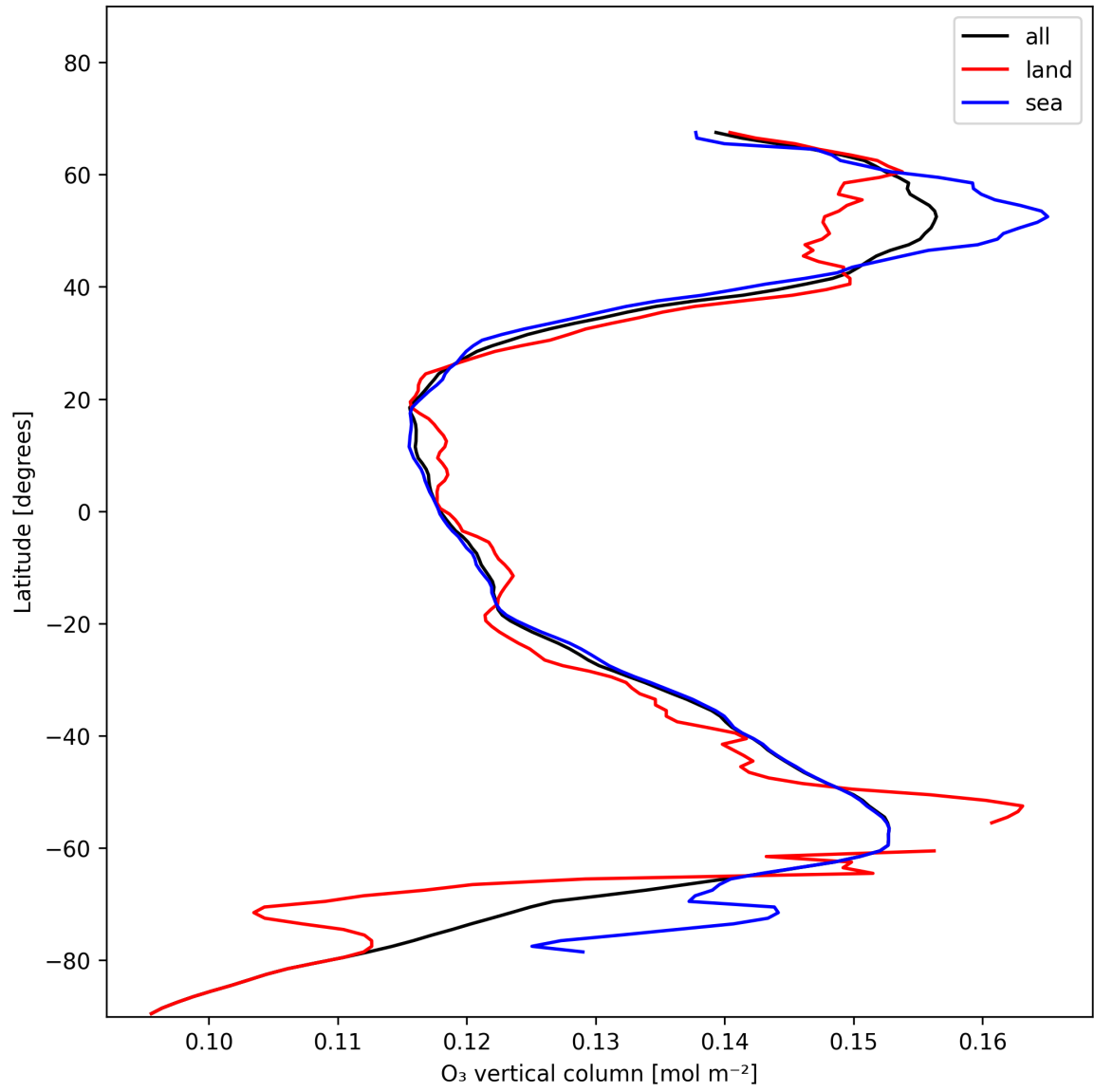
Figure 14: Zonal average of “O 3 vertical column” for 2024-11-30 to 2024-12-01.
