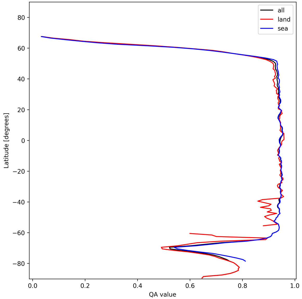
Figure 13: Zonal average of “QA value” for 2024-11-30 to 2024-12-01.
