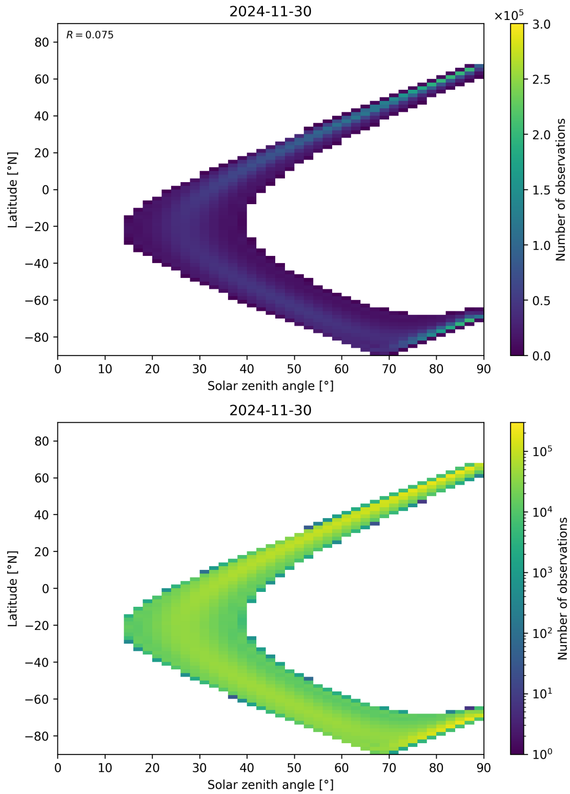
Figure 44: Scatter density plot of “Solar zenith angle” against “Latitude” for 2024-11-30 to 2024-12-01.
