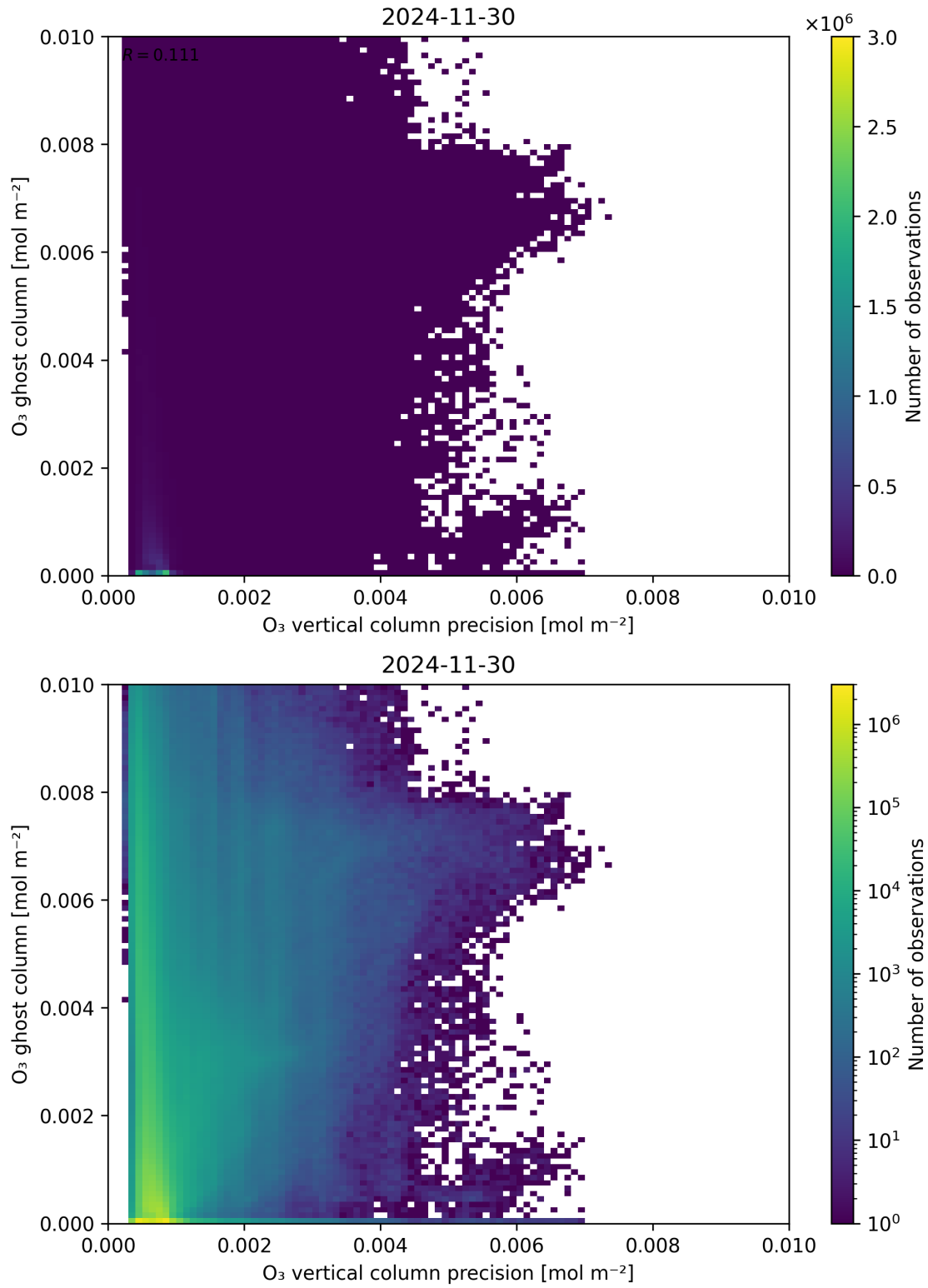
Figure 43: Scatter density plot of “O 3 vertical column precision” against “O 3 ghost column” for 2024-11-30 to 2024-12-01.
