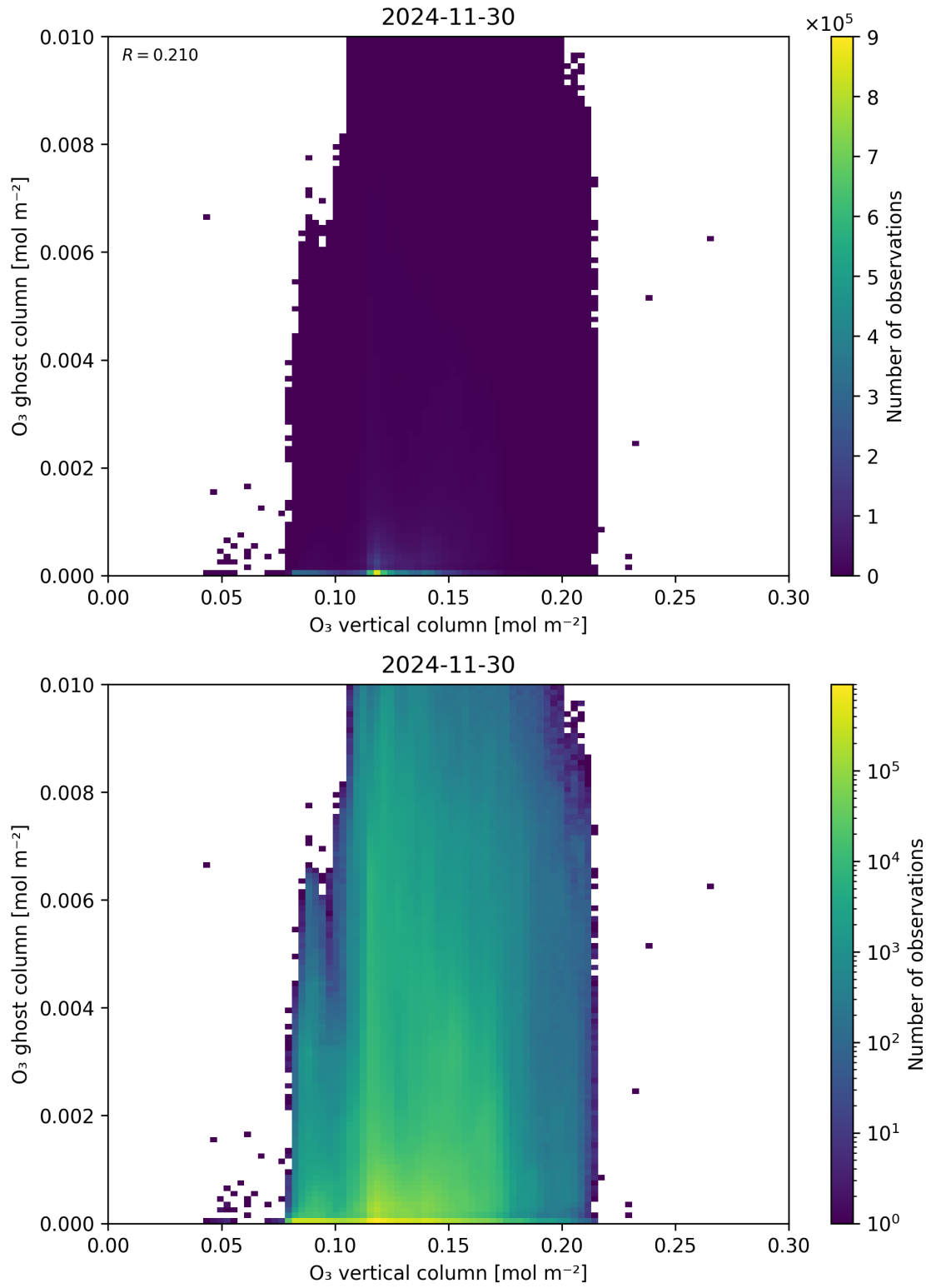
Figure 40: Scatter density plot of “O 3 vertical column” against “O 3 ghost column” for 2024-11-30 to 2024-12-01.
