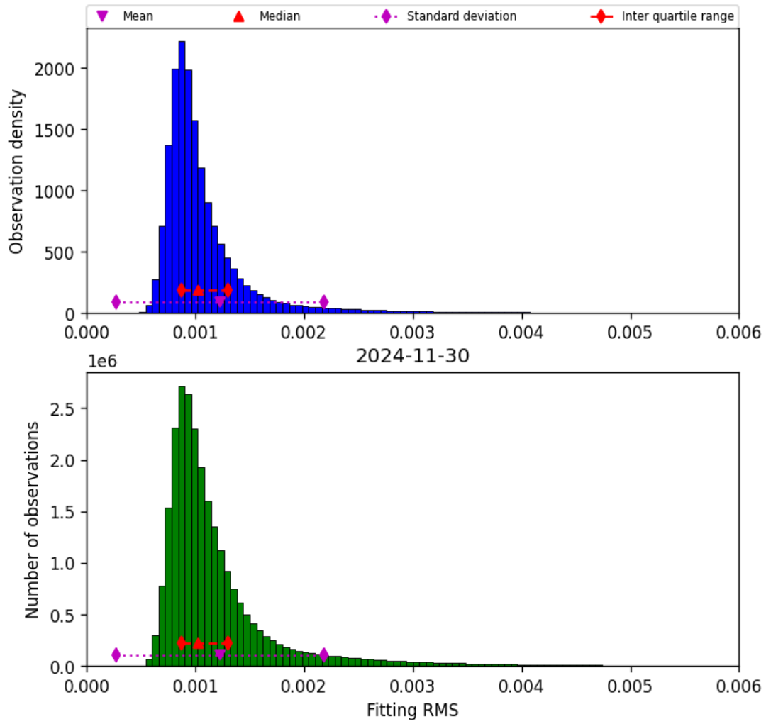
Figure 23: Histogram of “Fitting RMS” for 2024-11-30 to 2024-12-01
