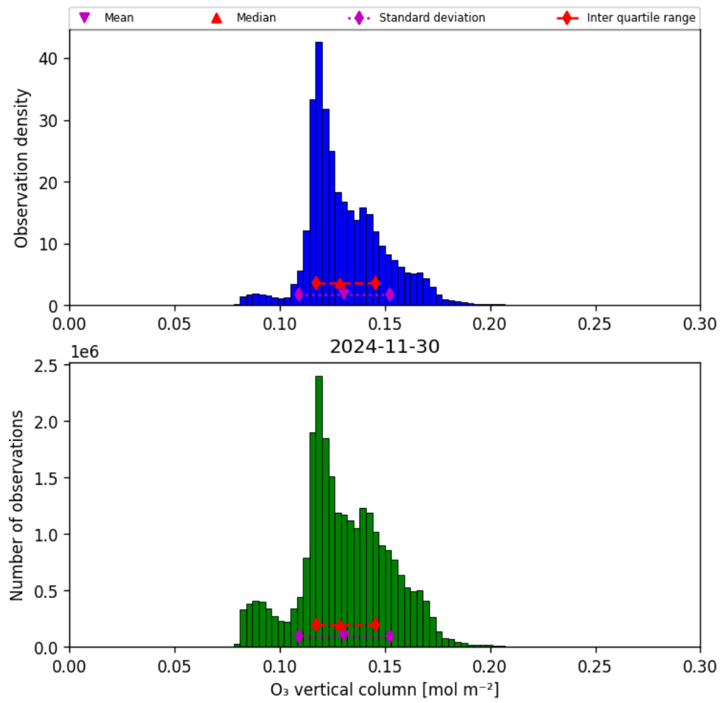
Figure 21: Histogram of “O 3 vertical column” for 2024-11-30 to 2024-12-01
