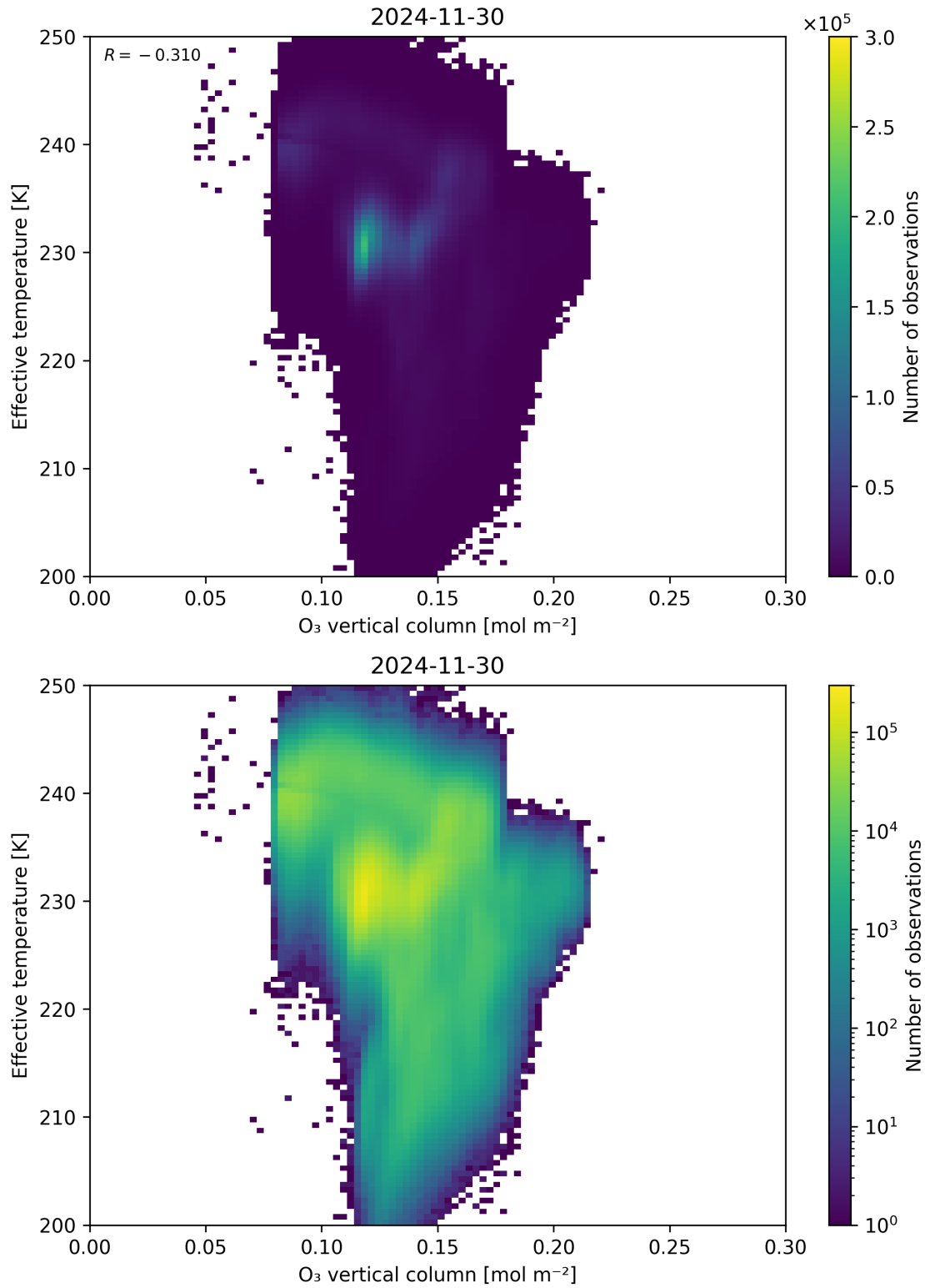
Figure 39: Scatter density plot of “O 3 vertical column” against “Effective temperature” for 2024-11-30 to 2024-12-01.
