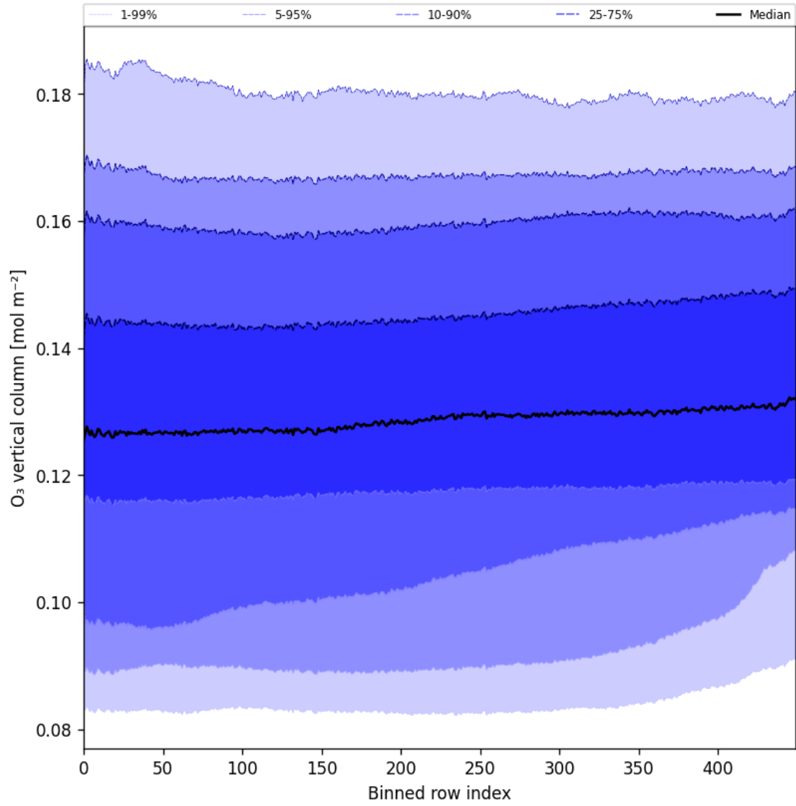
Figure 28: Along track statistics of "O 3 vertical column" for 2024-11-30 to 2024-12-01
