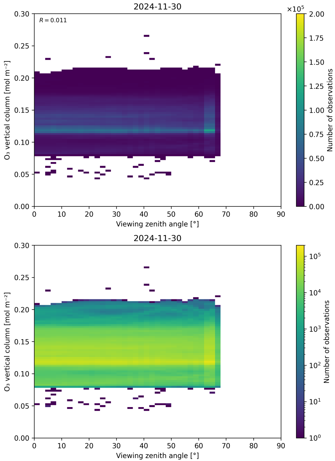
Figure 52: Scatter density plot of “Viewing zenith angle” against “O 3 vertical column” for 2024-11-30 to 2024-12-01.
