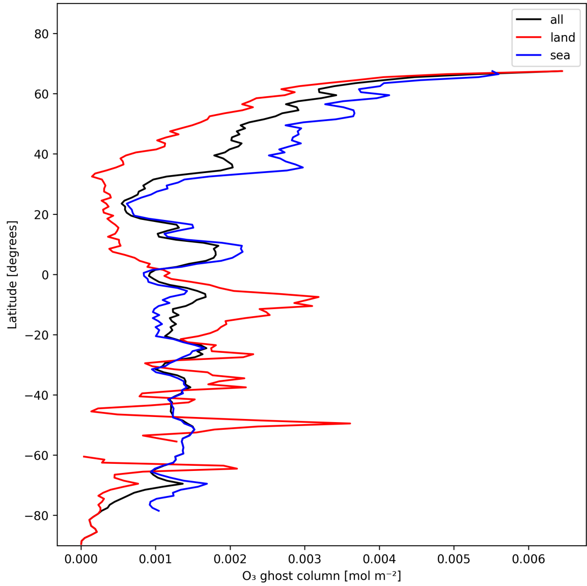
Figure 18: Zonal average of “O 3 ghost column” for 2024-11-30 to 2024-12-01.
