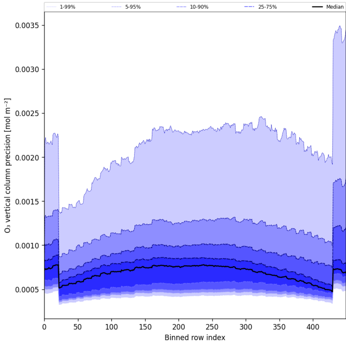
Figure 29: Along track statistics of “O 3 vertical column precision” for 2024-11-30 to 2024-12-01
