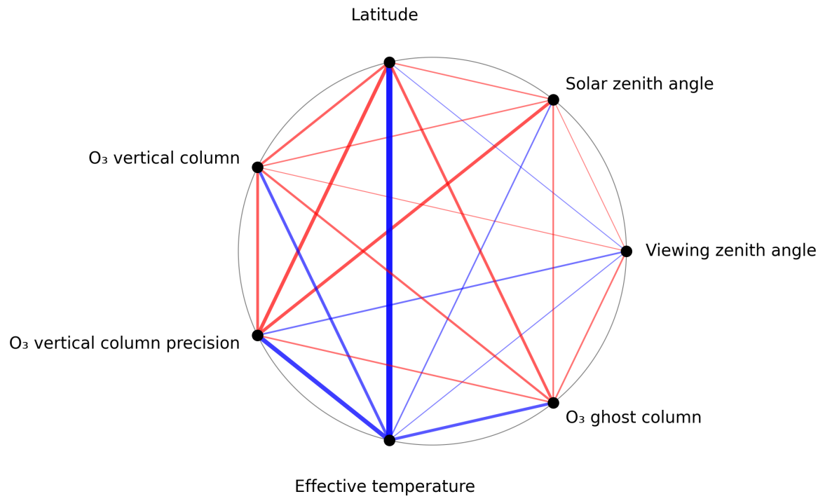
Figure 1: Map of correlation graph for 2024-11-30 to 2024-12-01.
