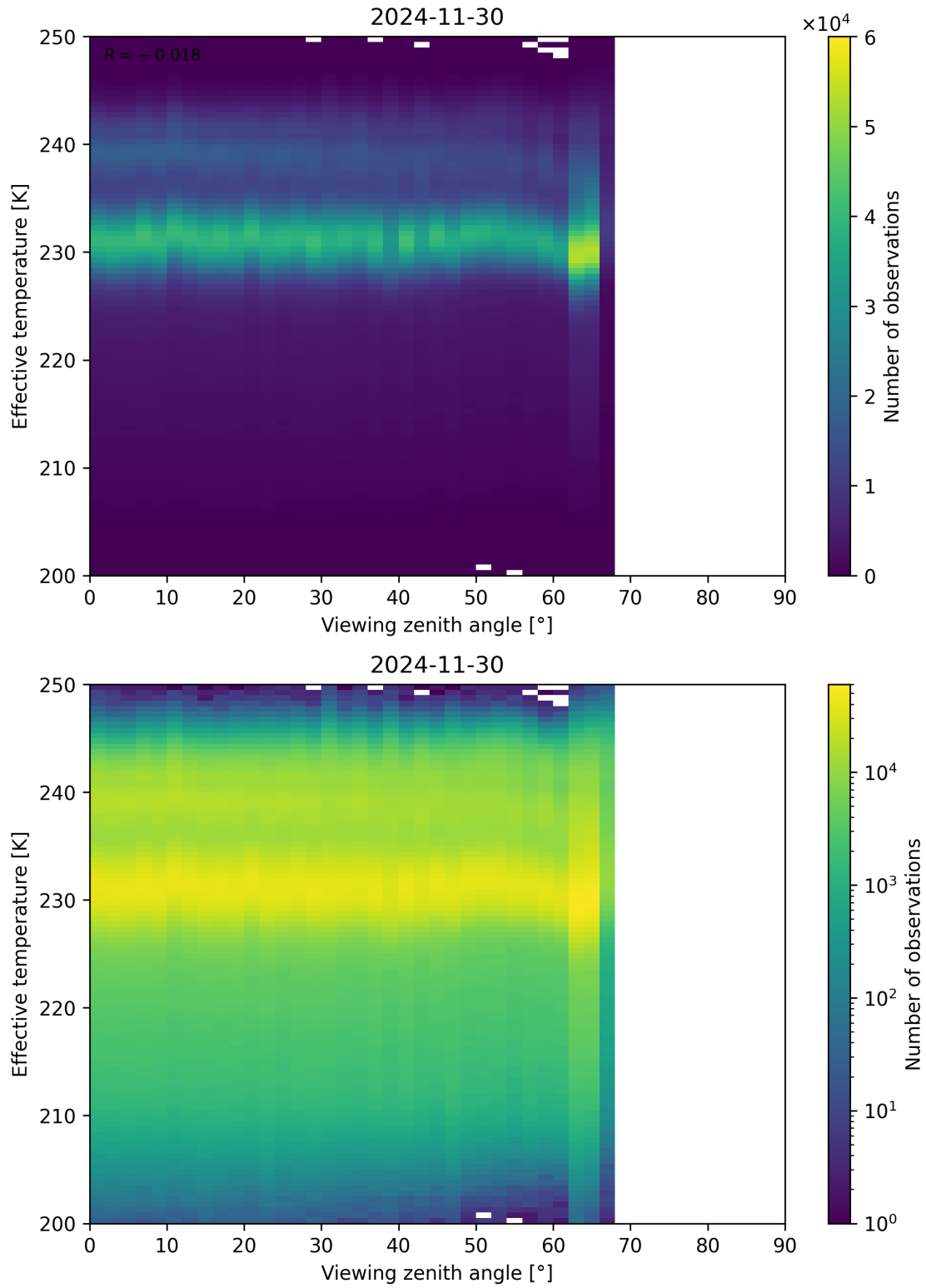
Figure 50: Scatter density plot of “Viewing zenith angle” against “Effective temperature” for 2024-11-30 to 2024-12-01.
