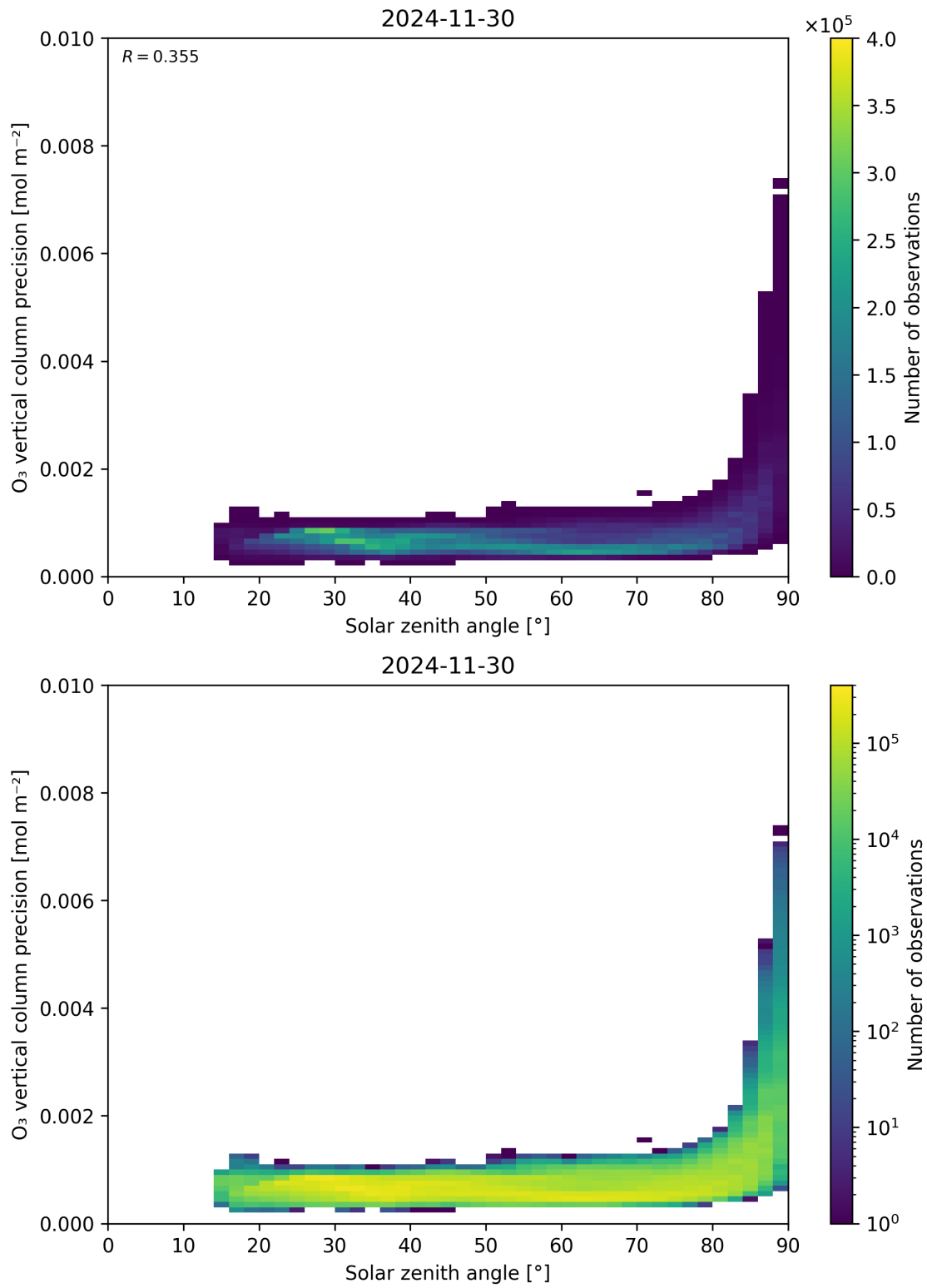
Figure 48: Scatter density plot of “Solar zenith angle” against “O 3 vertical column precision” for 2024-11-30 to 2024-12-01.
