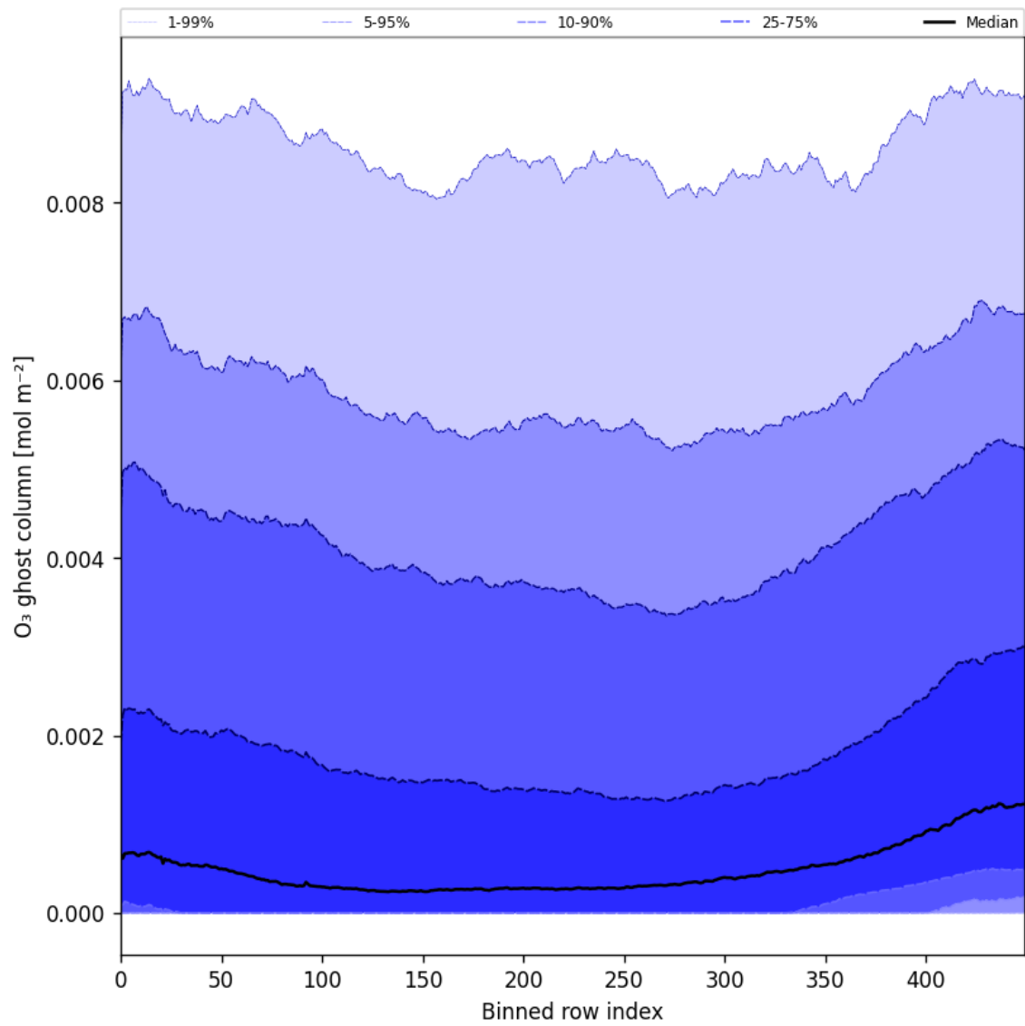
Figure 32: Along track statistics of “O 3 ghost column” for 2024-11-30 to 2024-12-01
