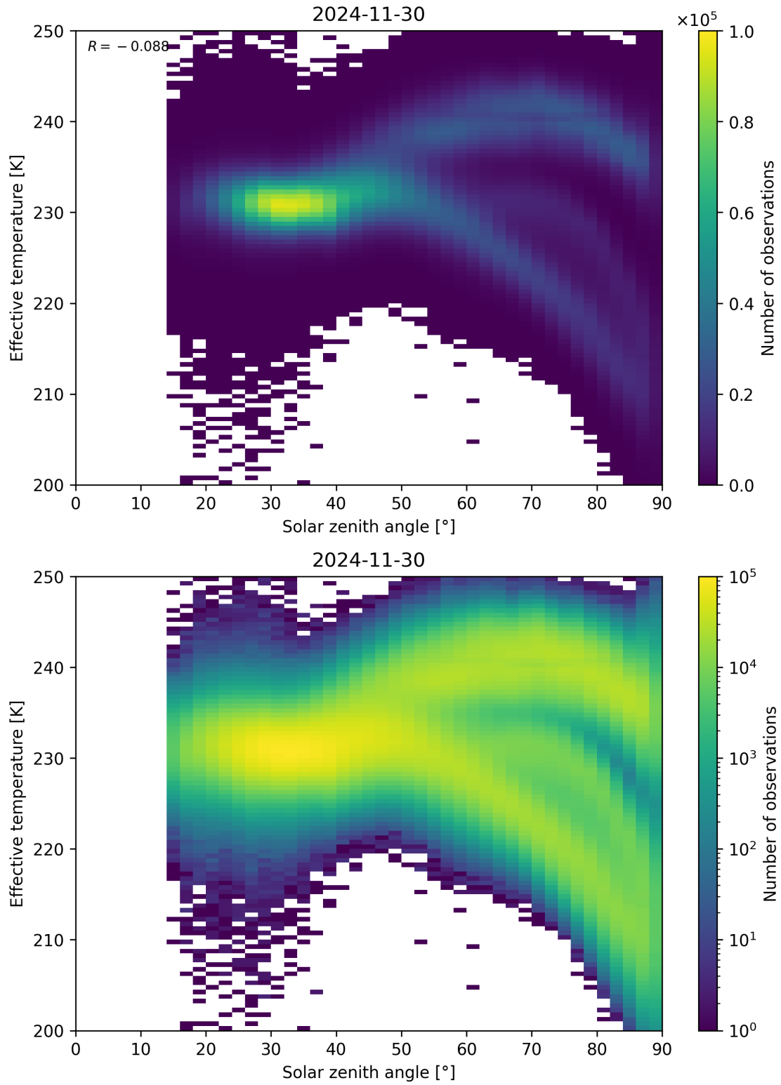
Figure 45: Scatter density plot of “Solar zenith angle” against “Effective temperature” for 2024-11-30 to 2024-12-01.
