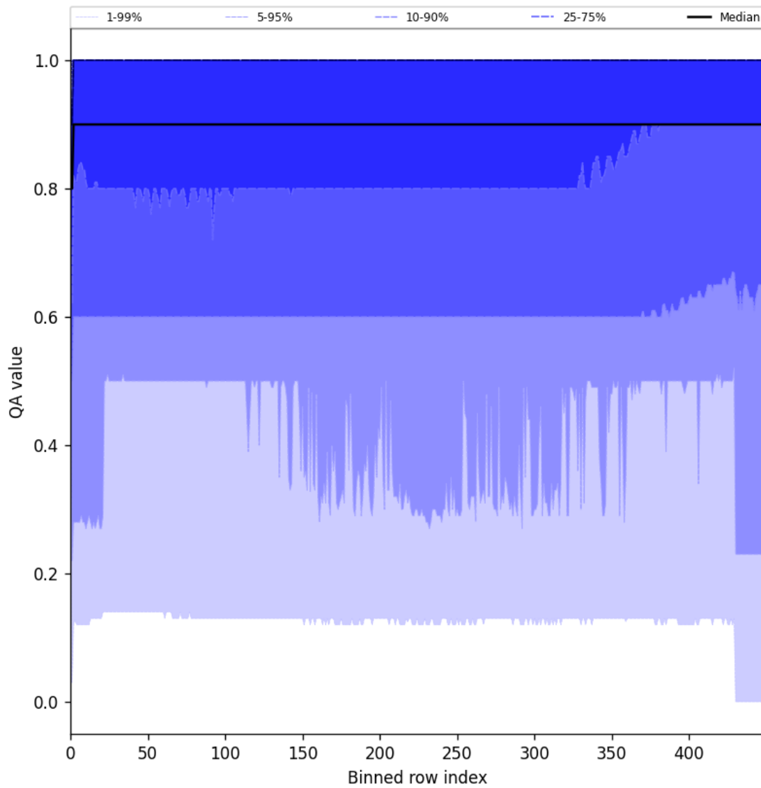
Figure 27: Along track statistics of “QA value” for 2024-11-30 to 2024-12-01
