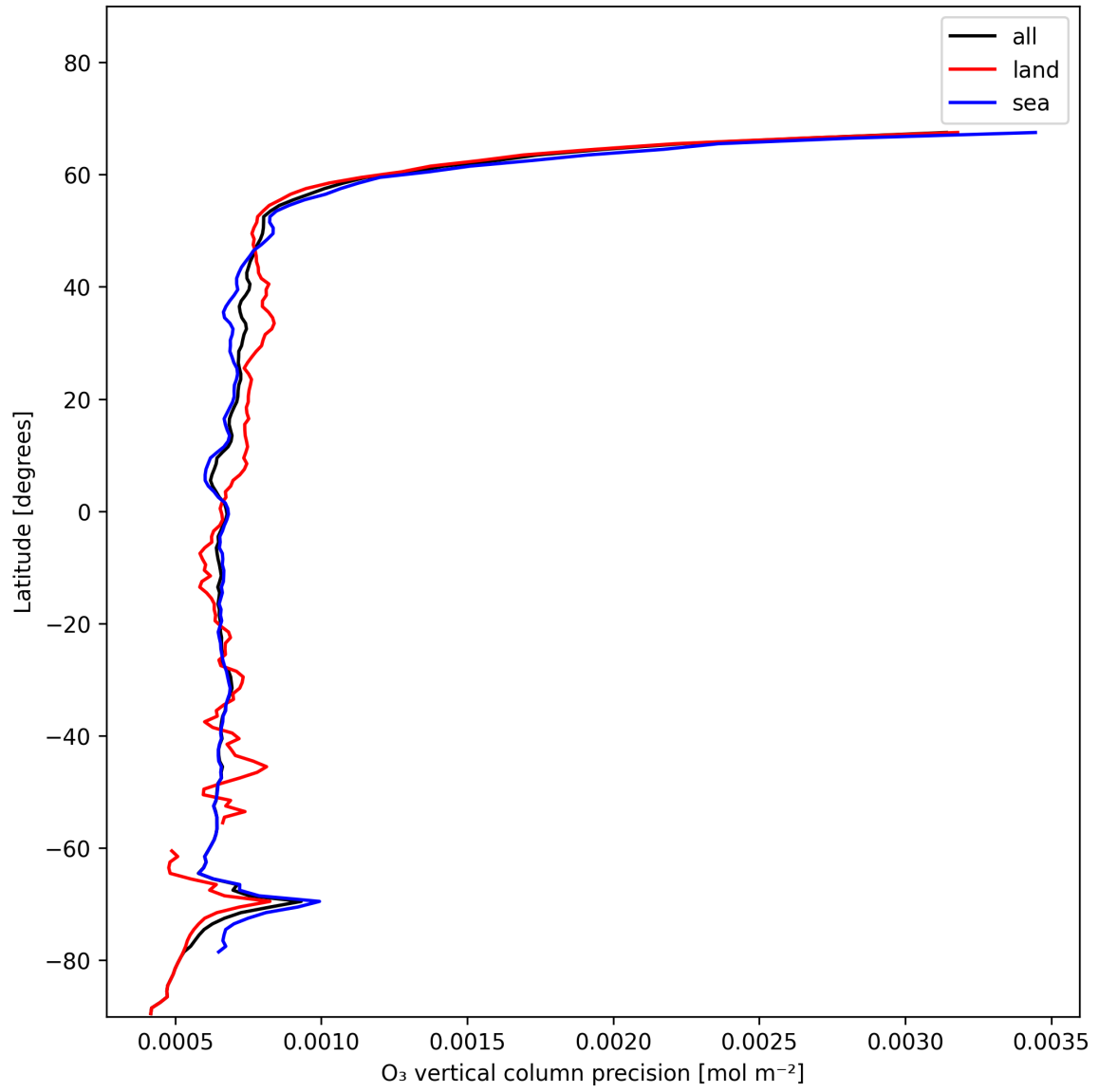
Figure 15: Zonal average of “O 3 vertical column precision” for 2024-11-30 to 2024-12-01.
