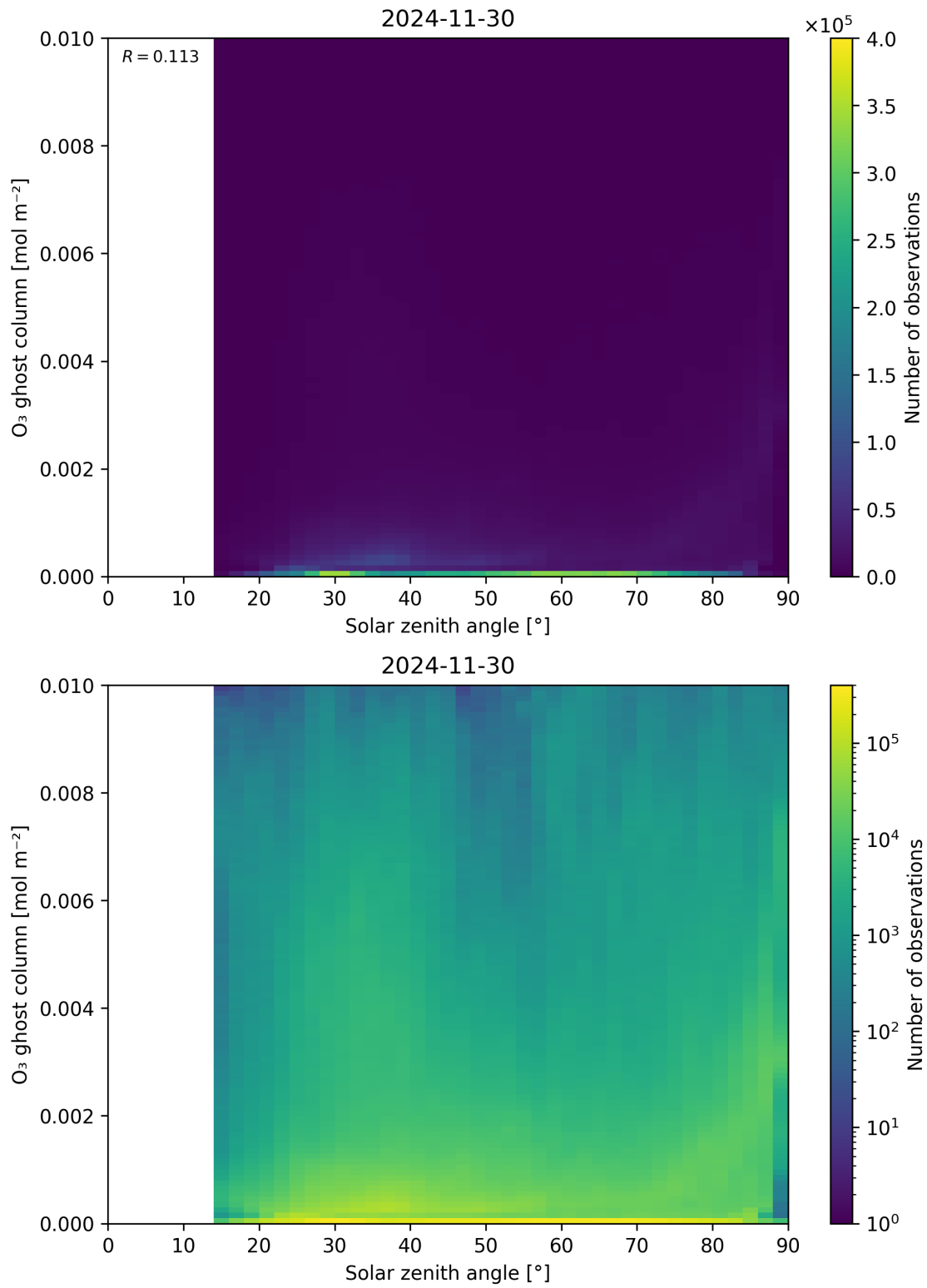
Figure 46: Scatter density plot of “Solar zenith angle” against “O 3 ghost column” for 2024-11-30 to 2024-12-01.
