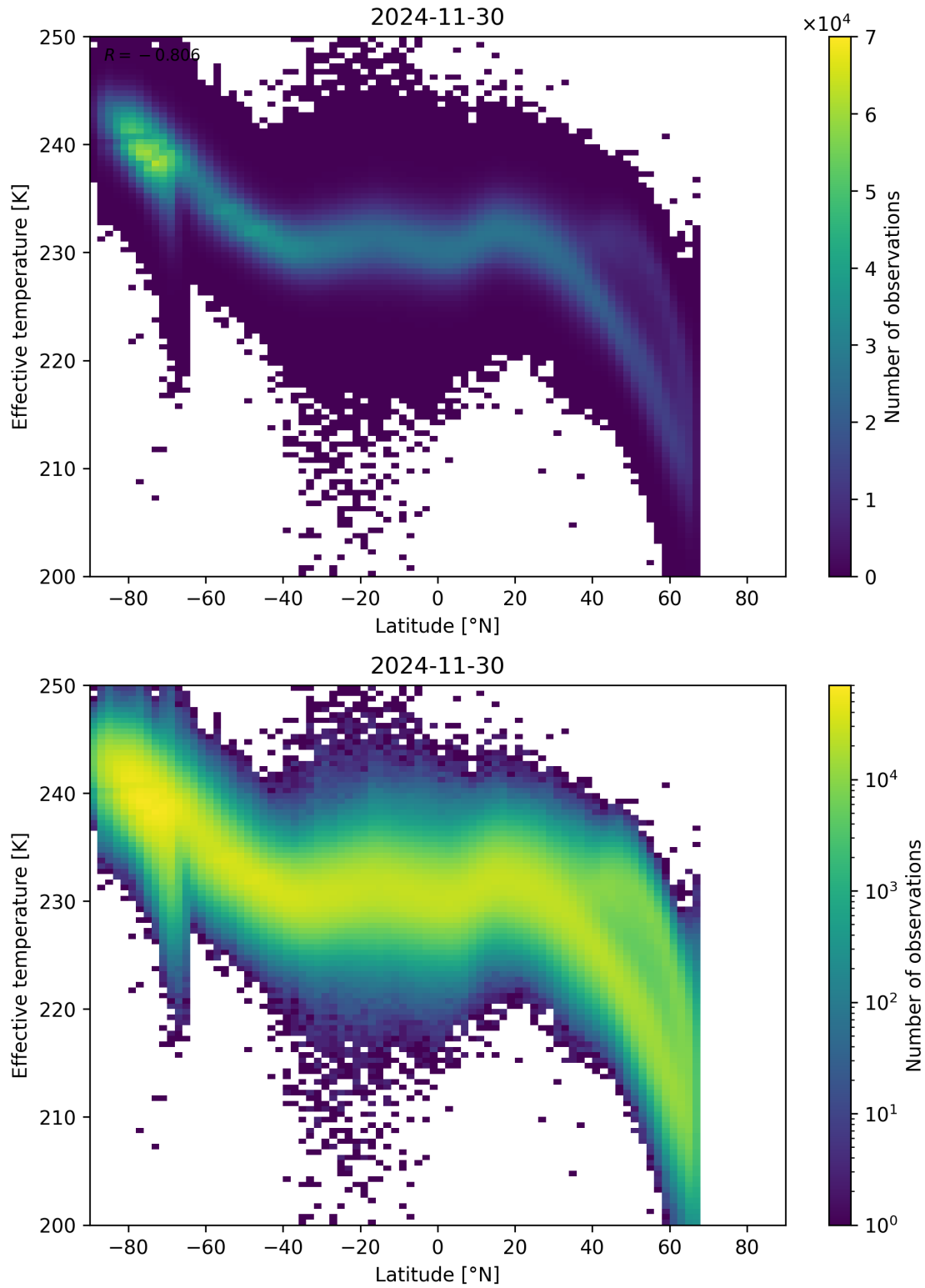
Figure 34: Scatter density plot of “Latitude” against “Effective temperature” for 2024-11-30 to 2024-12-01.
