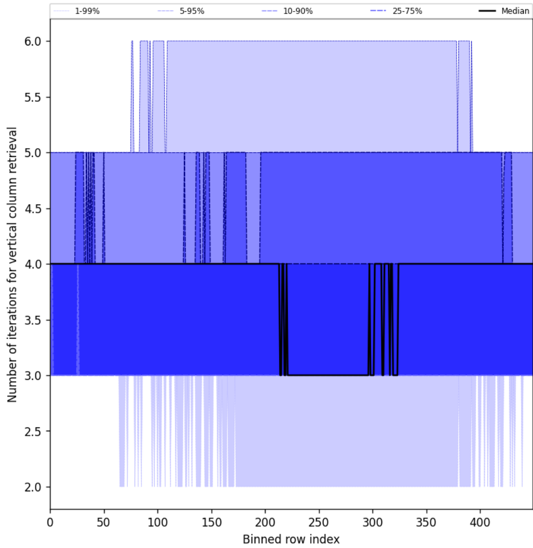
Figure 33: Along track statistics of “Number of iterations for vertical column retrieval” for 2024-11-30 to 2024-12-01
