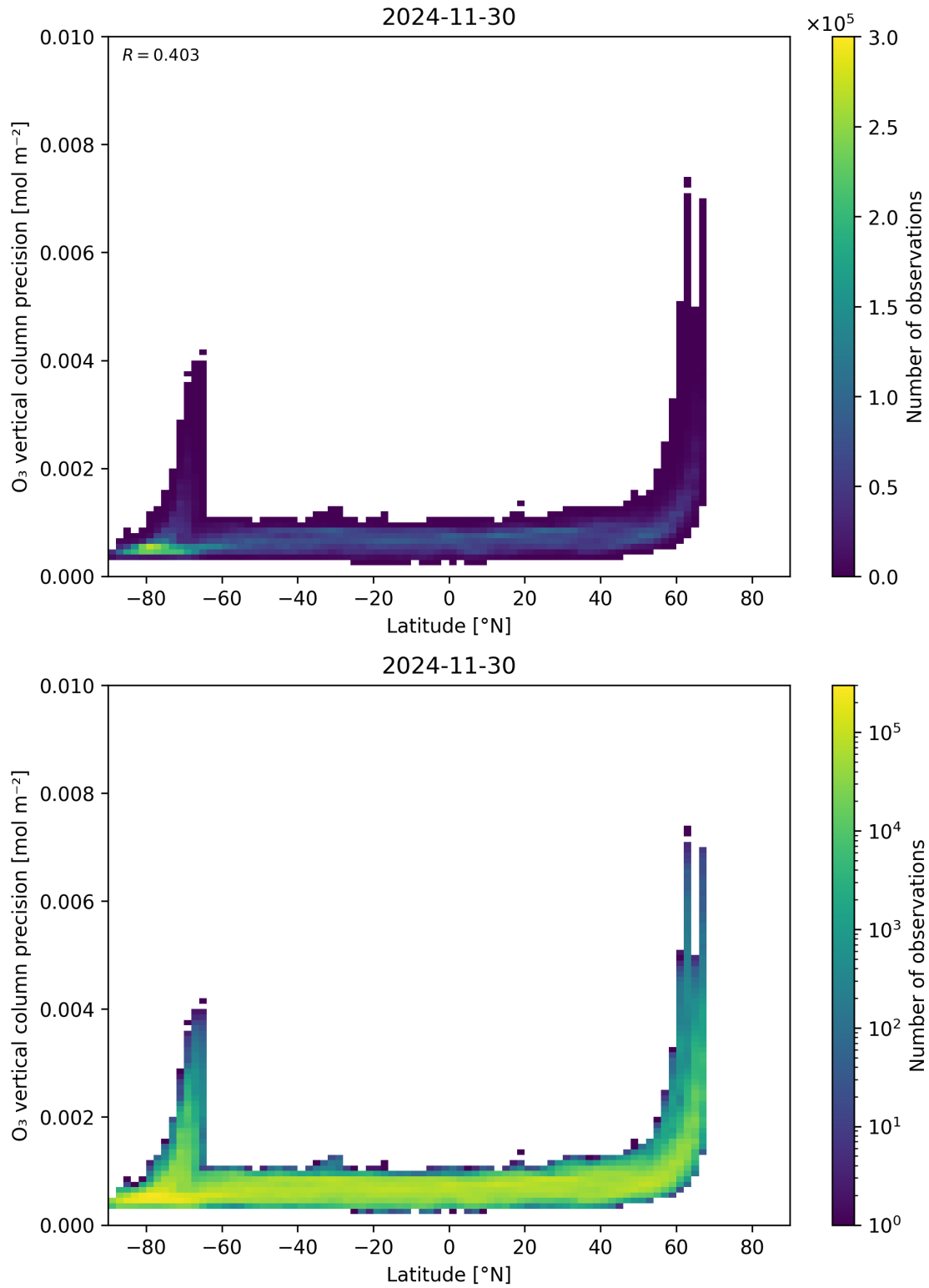
Figure 37: Scatter density plot of “Latitude” against “O 3 vertical column precision” for 2024-11-30 to 2024-12-01.
