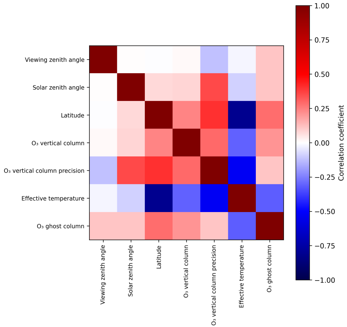
Figure 2: Map of correlation matrix for 2024-11-30 to 2024-12-01.
