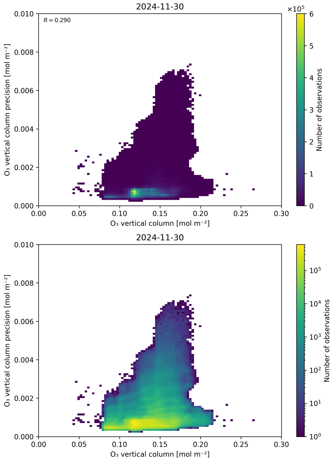
Figure 41: Scatter density plot of “O 3 vertical column” against “O 3 vertical column precision” for 2024-11-30 to 2024-12-01.
