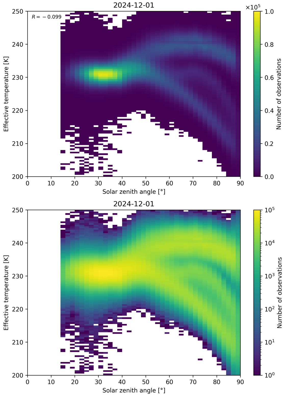
Figure 45: Scatter density plot of “Solar zenith angle” against “Effective temperature” for 2024-11-30 to 2024-12-02.
