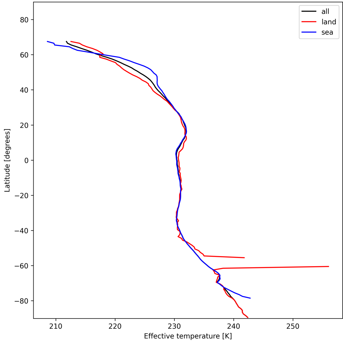
Figure 17: Zonal average of “Effective temperature” for 2024-11-30 to 2024-12-02.
