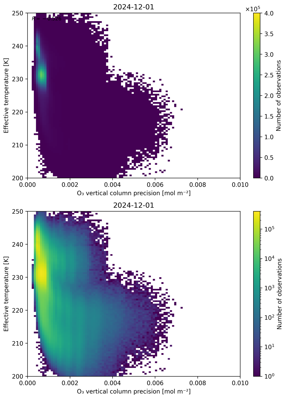
Figure 42: Scatter density plot of “O 3 vertical column precision” against “Effective temperature” for 2024-11-30 to 2024-12-02.
