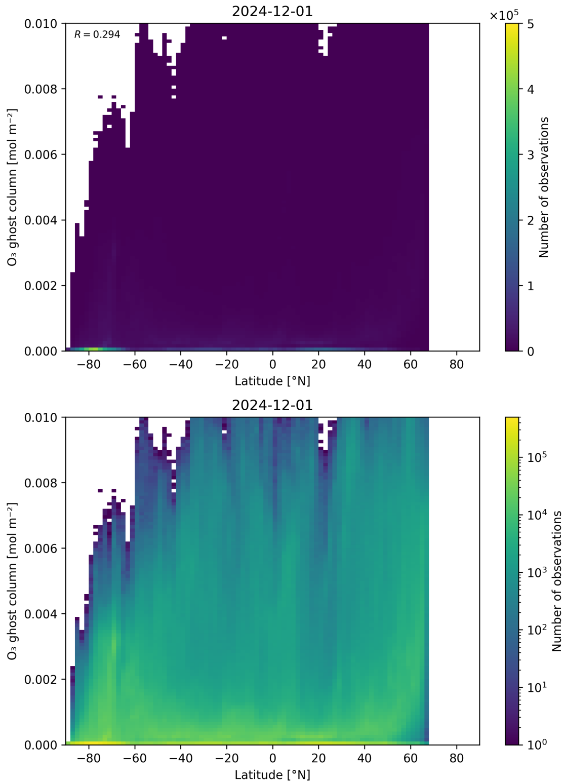
Figure 35: Scatter density plot of “Latitude” against “O 3 ghost column” for 2024-11-30 to 2024-12-02.
