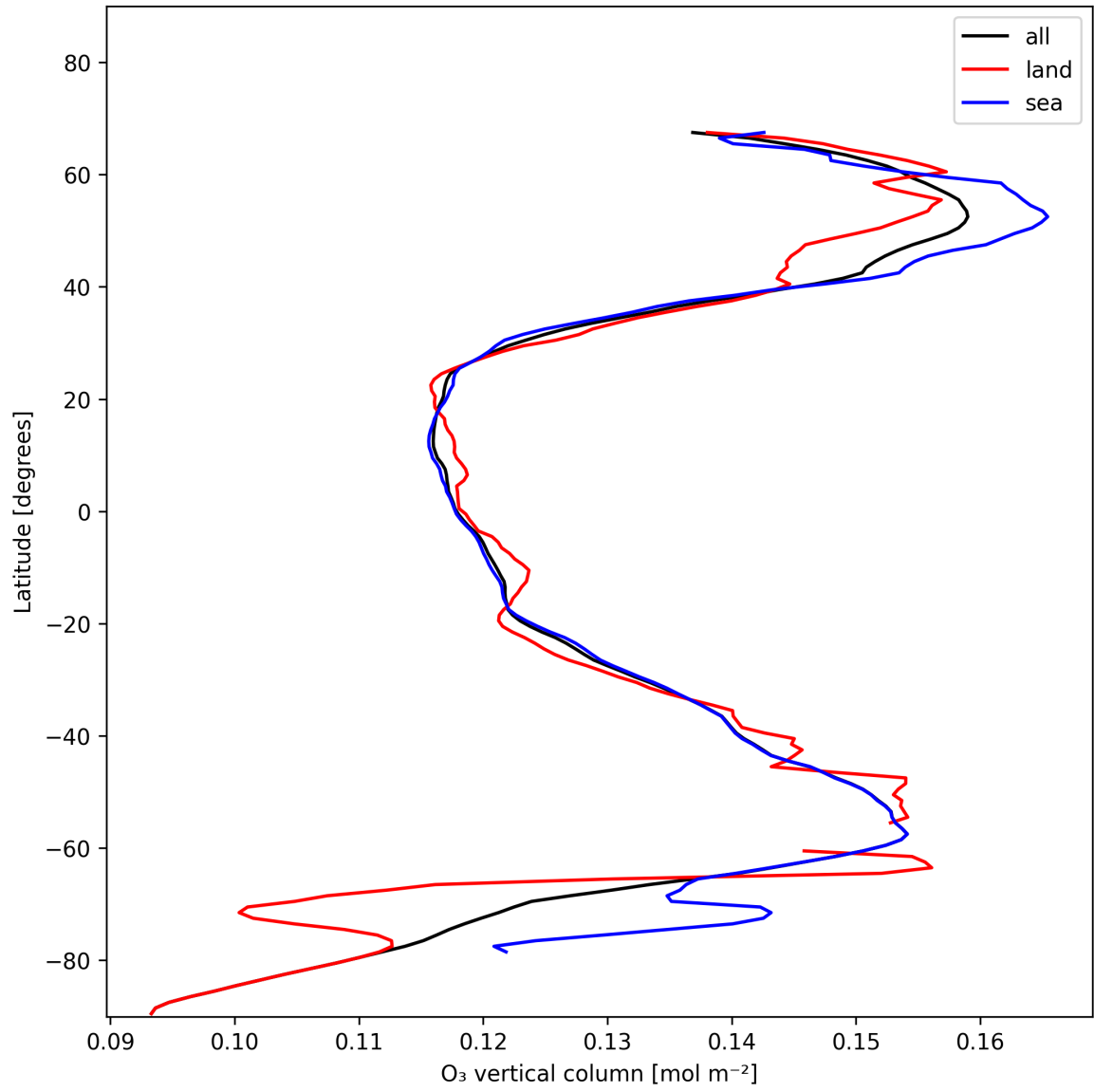
Figure 14: Zonal average of “O 3 vertical column” for 2024-11-30 to 2024-12-02.
