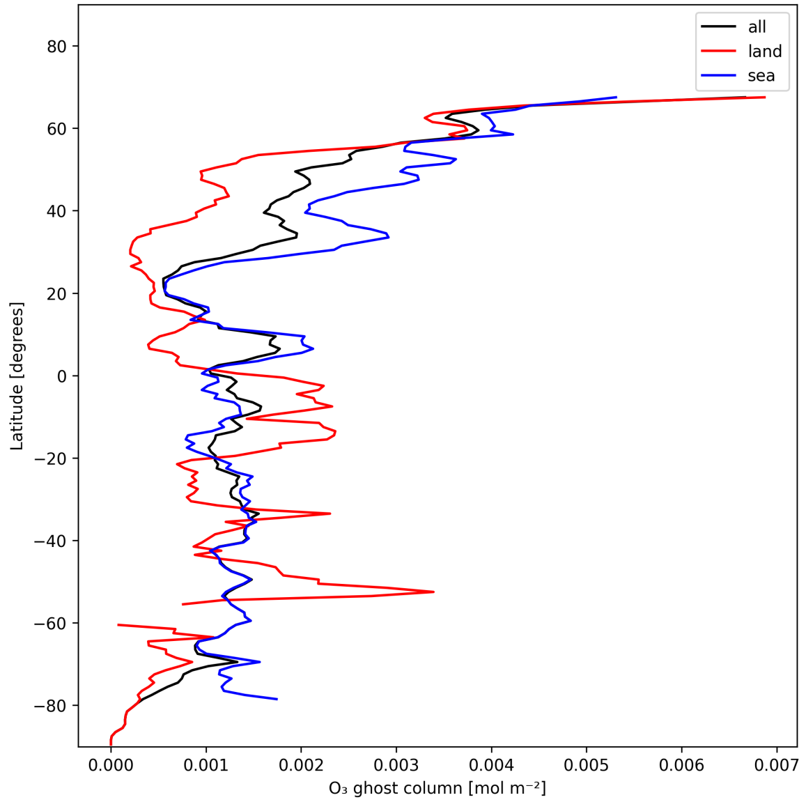
Figure 18: Zonal average of “O 3 ghost column” for 2024-11-30 to 2024-12-02.
