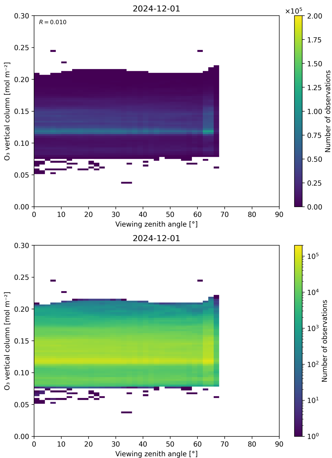
Figure 52: Scatter density plot of “Viewing zenith angle” against “O 3 vertical column” for 2024-11-30 to 2024-12-02.
