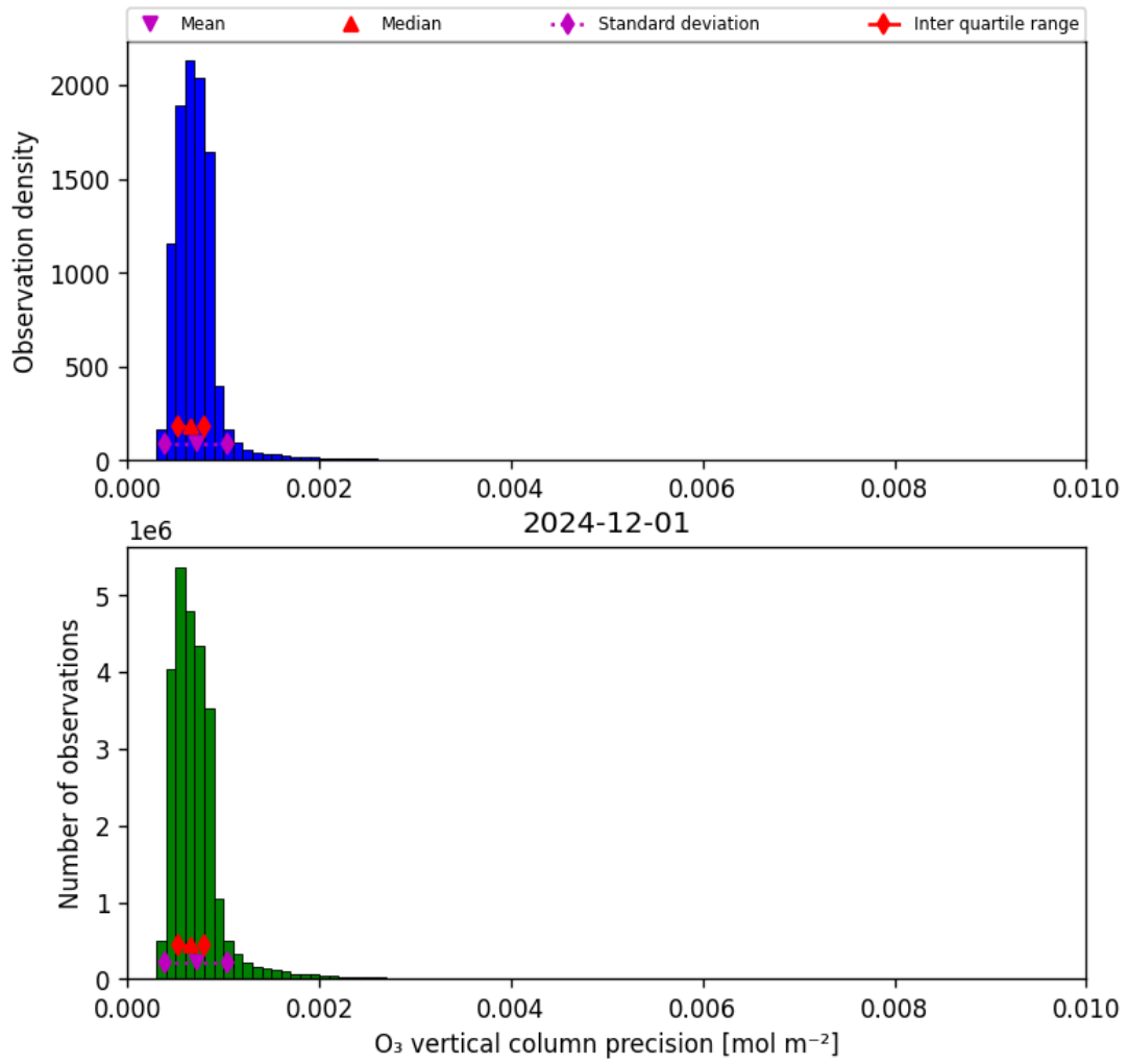
Figure 22: Histogram of “O 3 vertical column precision” for 2024-11-30 to 2024-12-02
