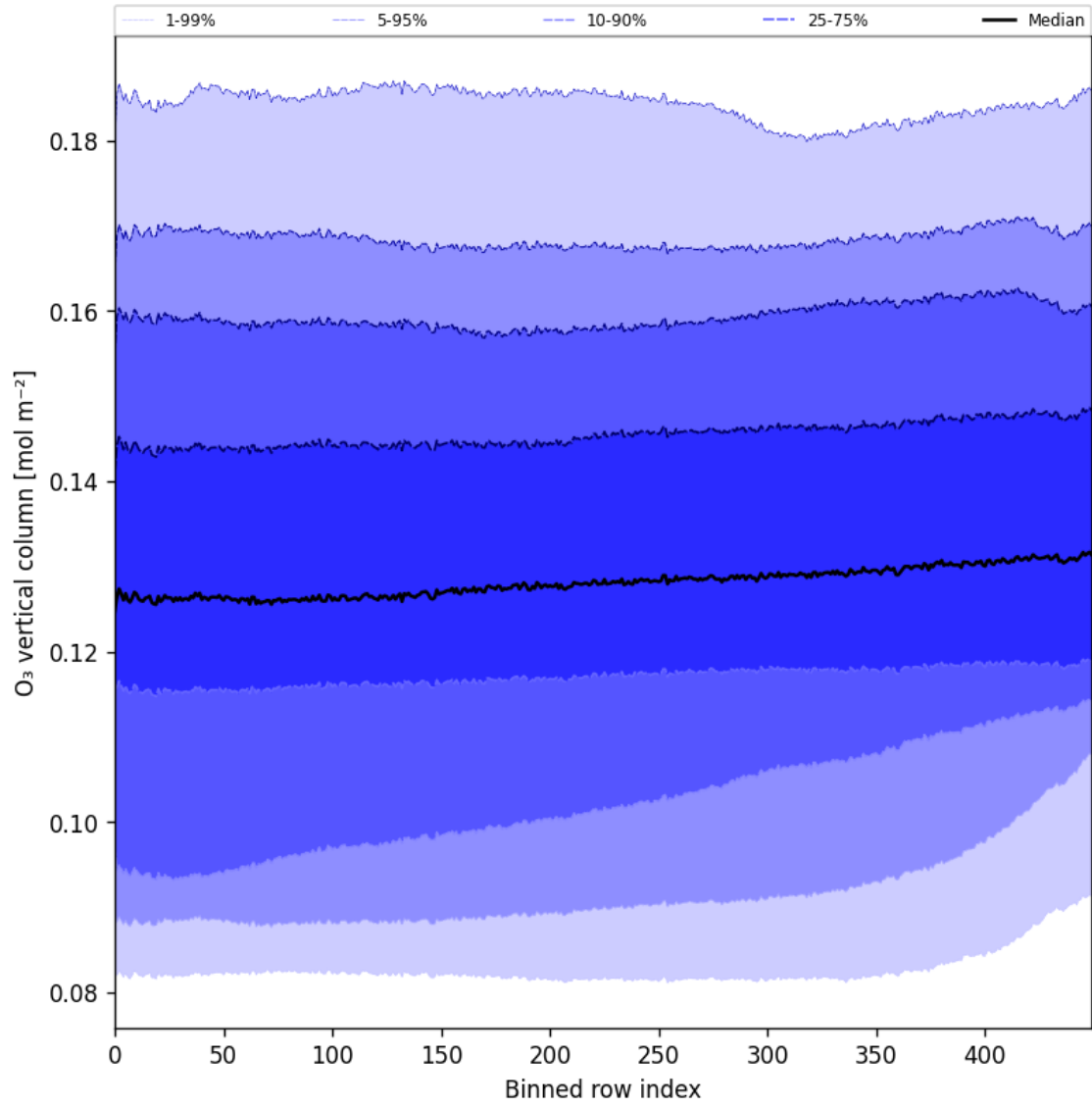
Figure 28: Along track statistics of “O 3 vertical column” for 2024-11-30 to 2024-12-02
