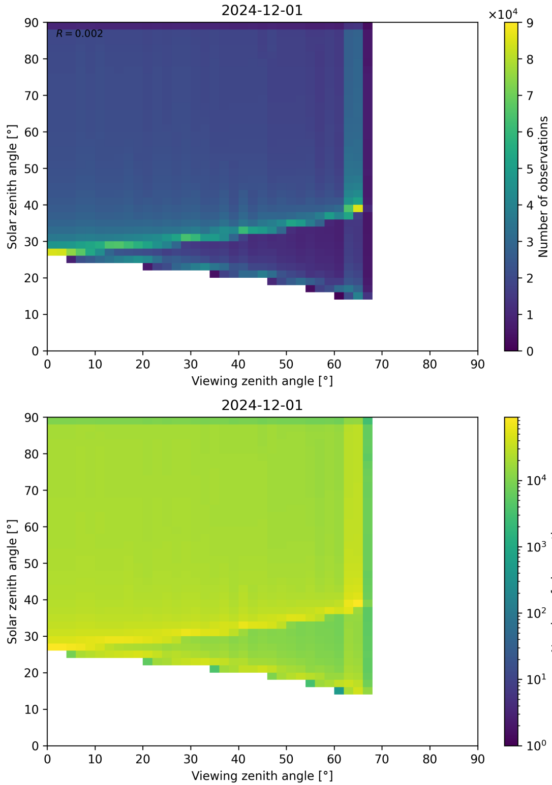
Figure 54: Scatter density plot of “Viewing zenith angle” against “Solar zenith angle” for 2024-11-30 to 2024-12-02.
