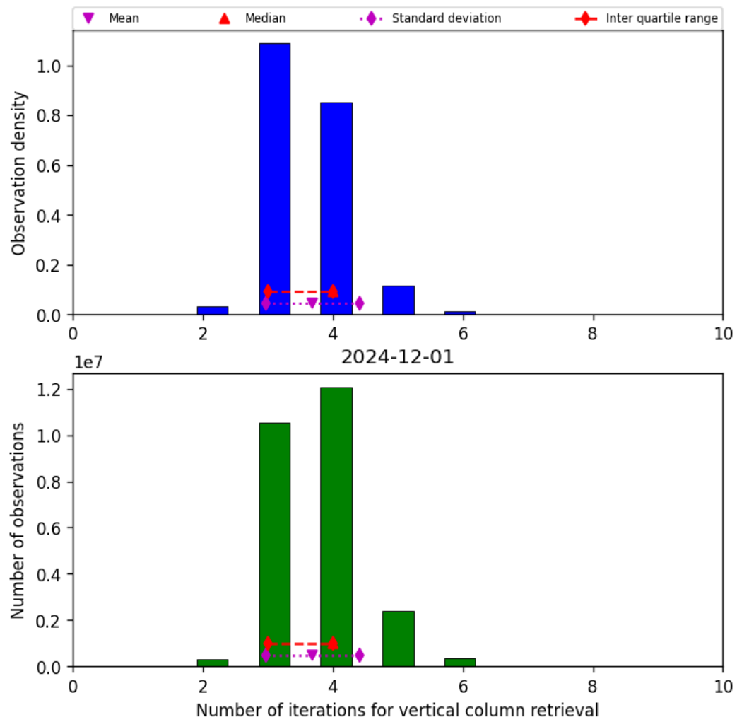
Figure 26: Histogram of “Number of iterations for vertical column retrieval” for 2024-11-30 to 2024-12-02
