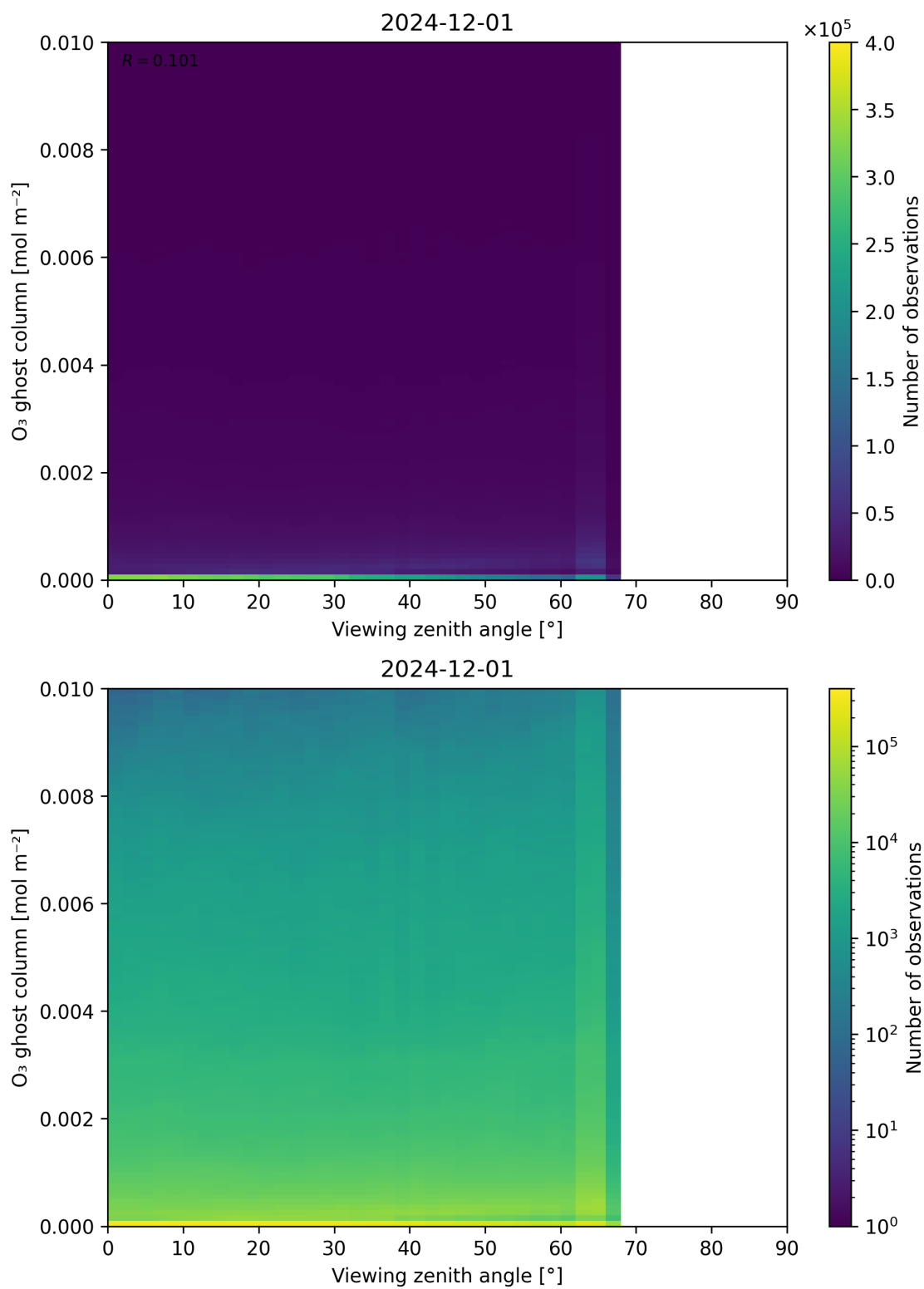
Figure 51: Scatter density plot of “Viewing zenith angle” against “O 3 ghost column” for 2024-11-30 to 2024-12-02.
