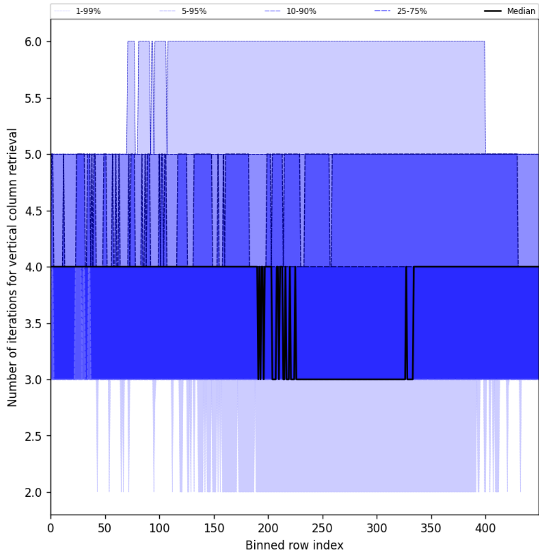
Figure 33: Along track statistics of “Number of iterations for vertical column retrieval” for 2024-11-30 to 2024-12-02
