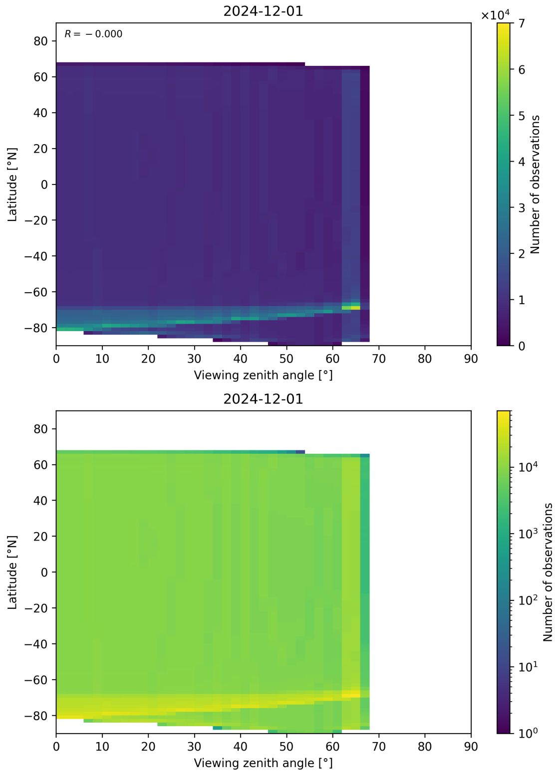
Figure 49: Scatter density plot of “Viewing zenith angle” against “Latitude” for 2024-11-30 to 2024-12-02.
