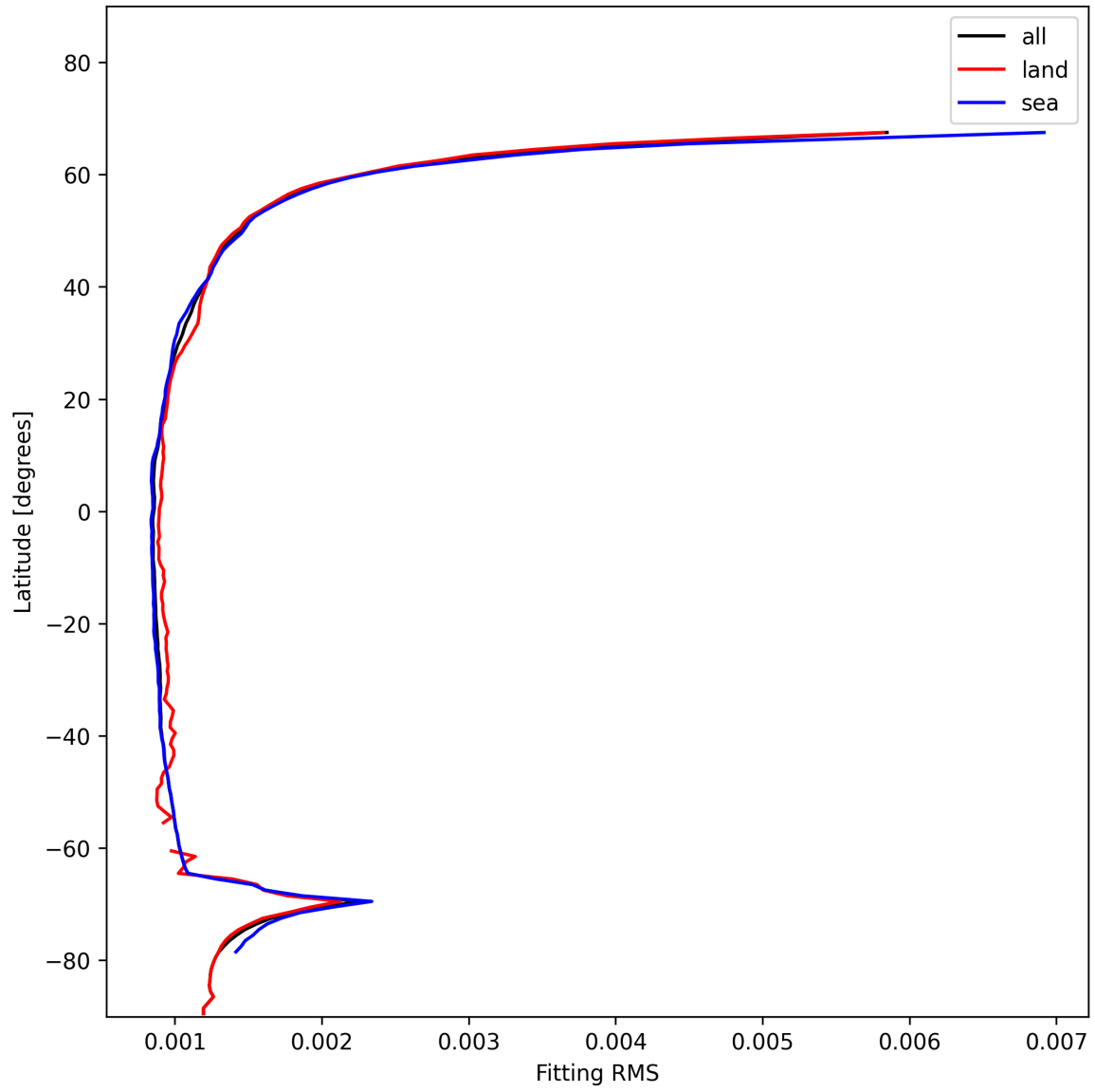
Figure 16: Zonal average of “Fitting RMS” for 2024-11-30 to 2024-12-02.
