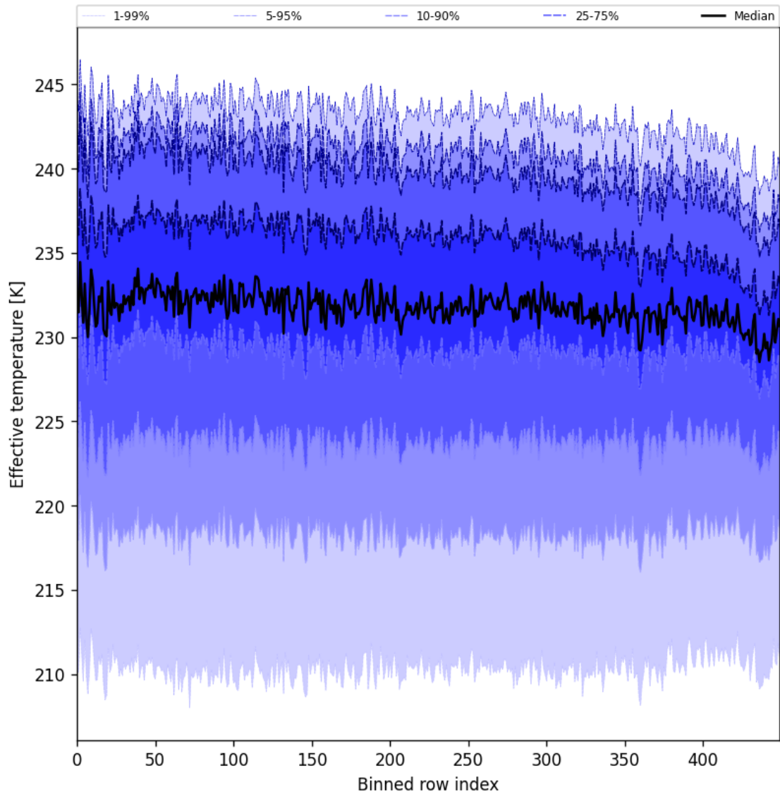
Figure 31: Along track statistics of “Effective temperature” for 2024-11-30 to 2024-12-02
