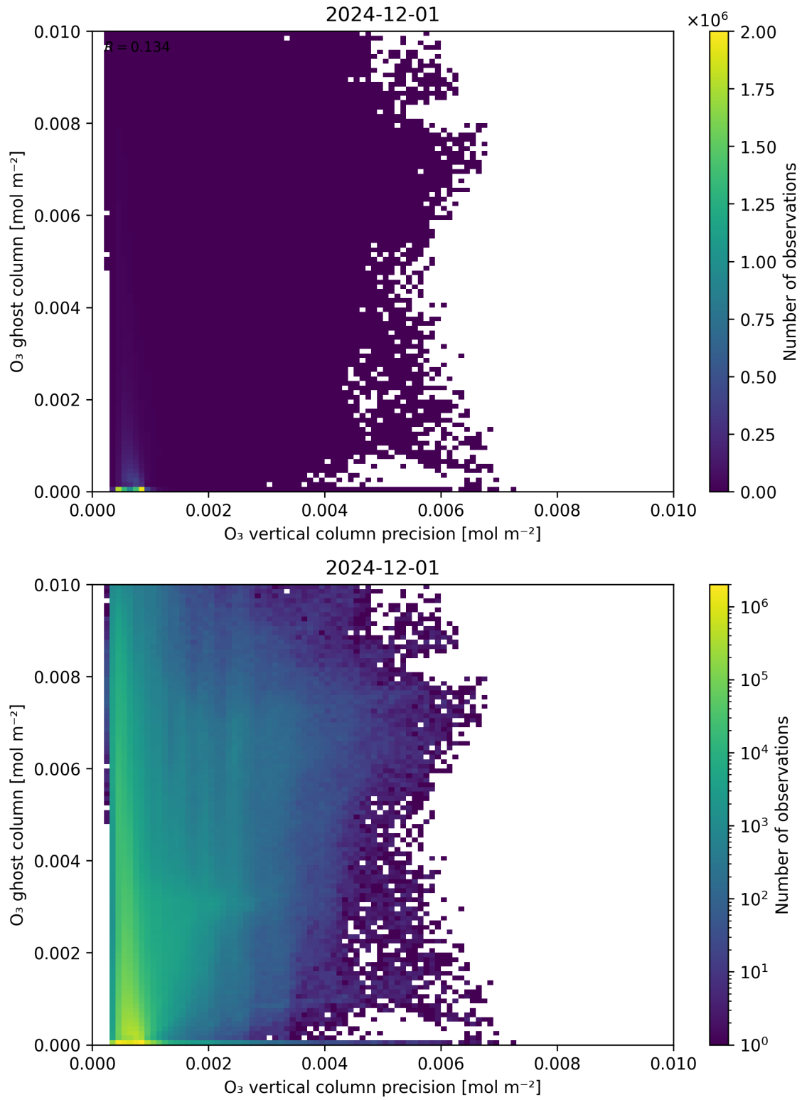
Figure 43: Scatter density plot of “O 3 vertical column precision” against “O 3 ghost column” for 2024-11-30 to 2024-12-02.
