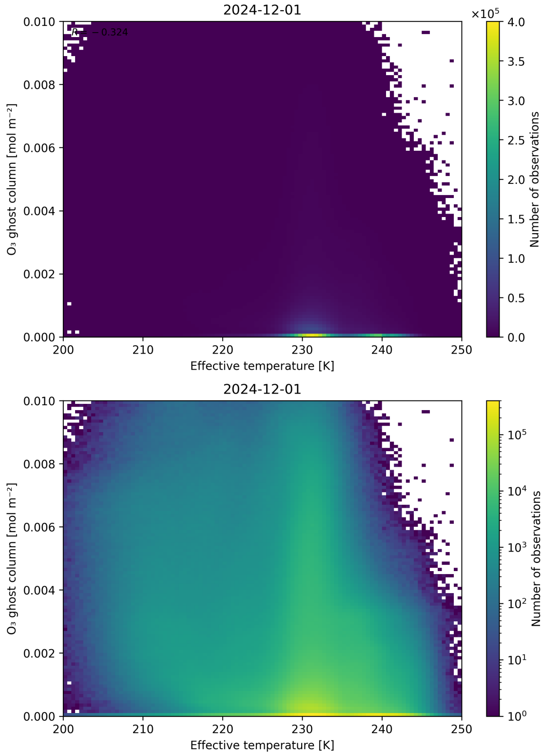
Figure 38: Scatter density plot of “Effective temperature” against “O 3 ghost column” for 2024-11-30 to 2024-12-02.
