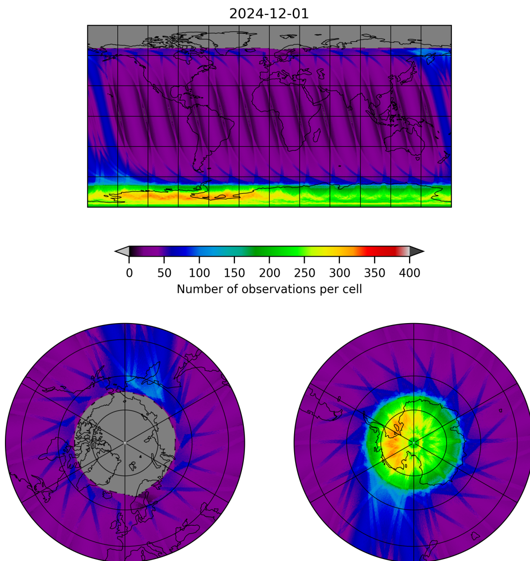
Figure 12: Map of the number of observations for 2024-11-30 to 2024-12-02
