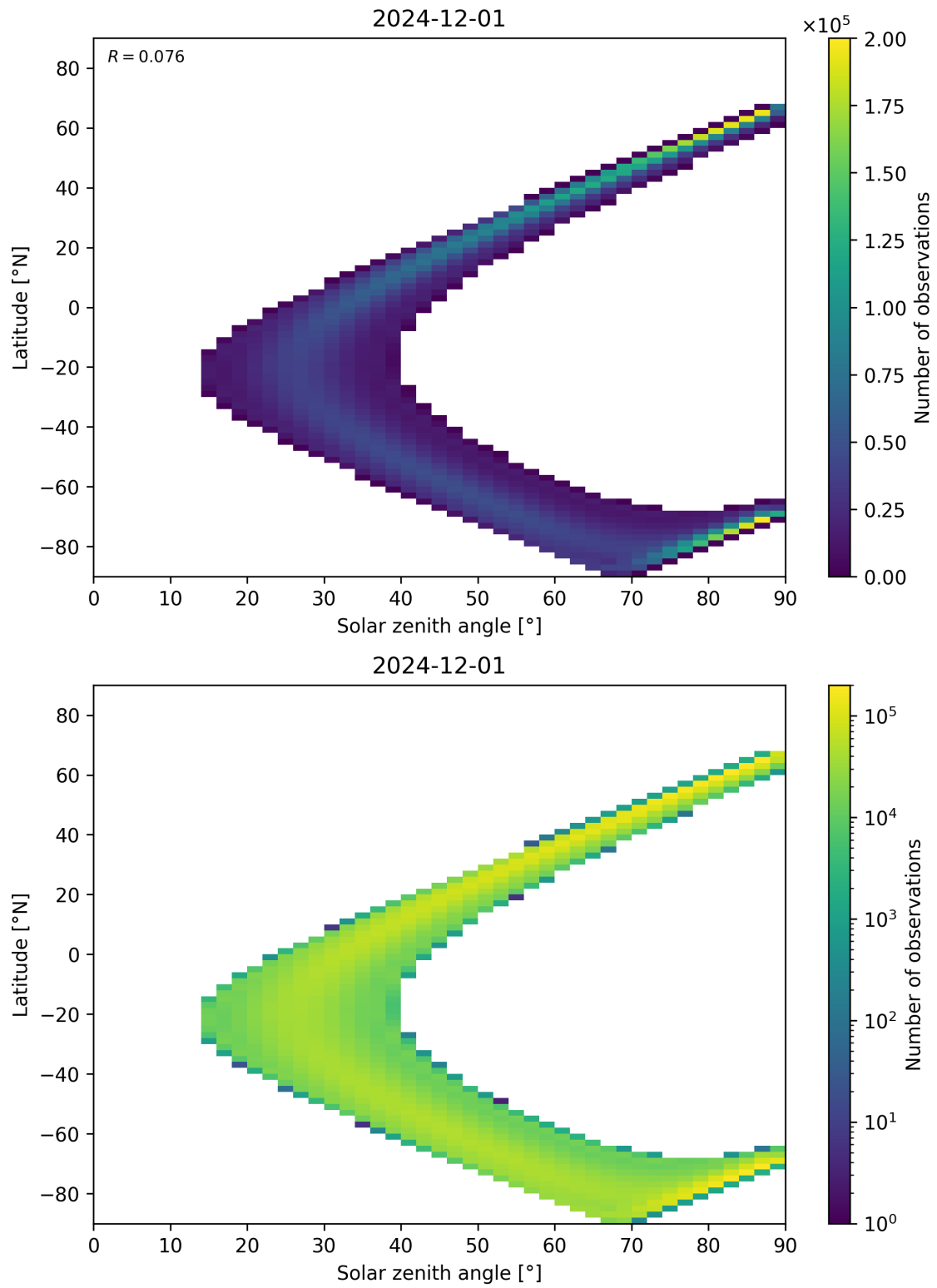
Figure 44: Scatter density plot of “Solar zenith angle” against “Latitude” for 2024-11-30 to 2024-12-02.
