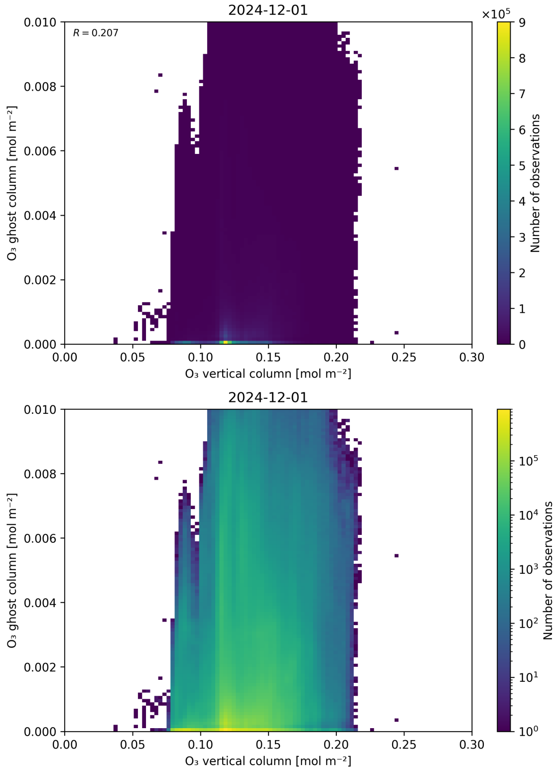
Figure 40: Scatter density plot of “O 3 vertical column” against “O 3 ghost column” for 2024-11-30 to 2024-12-02.
