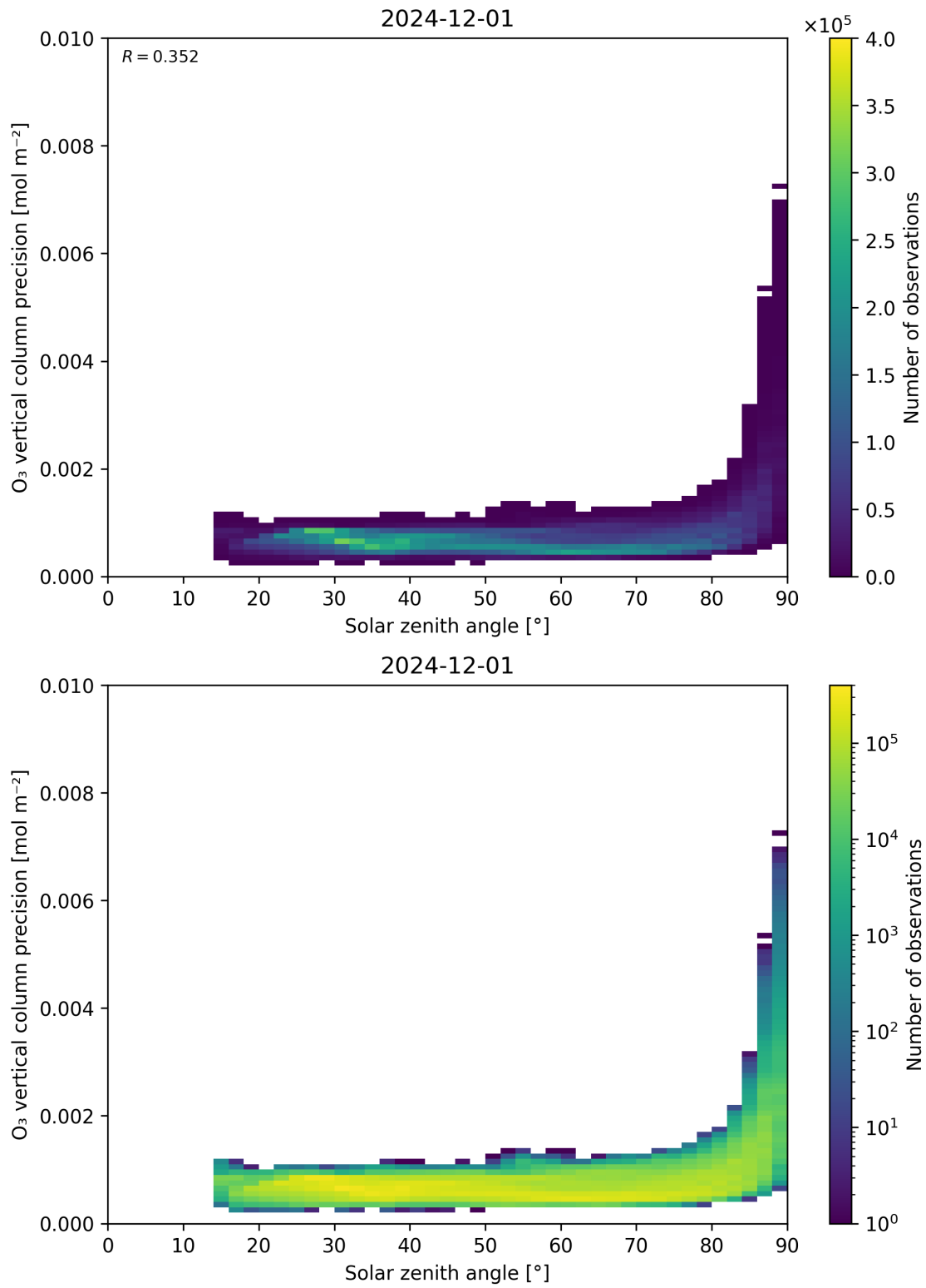
Figure 48: Scatter density plot of “Solar zenith angle” against “O 3 vertical column precision” for 2024-11-30 to 2024-12-02.
