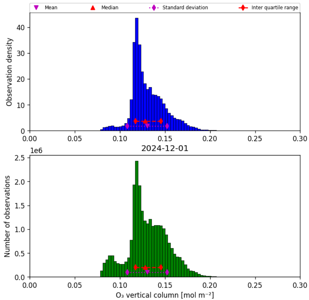
Figure 21: Histogram of “O 3 vertical column” for 2024-11-30 to 2024-12-02
