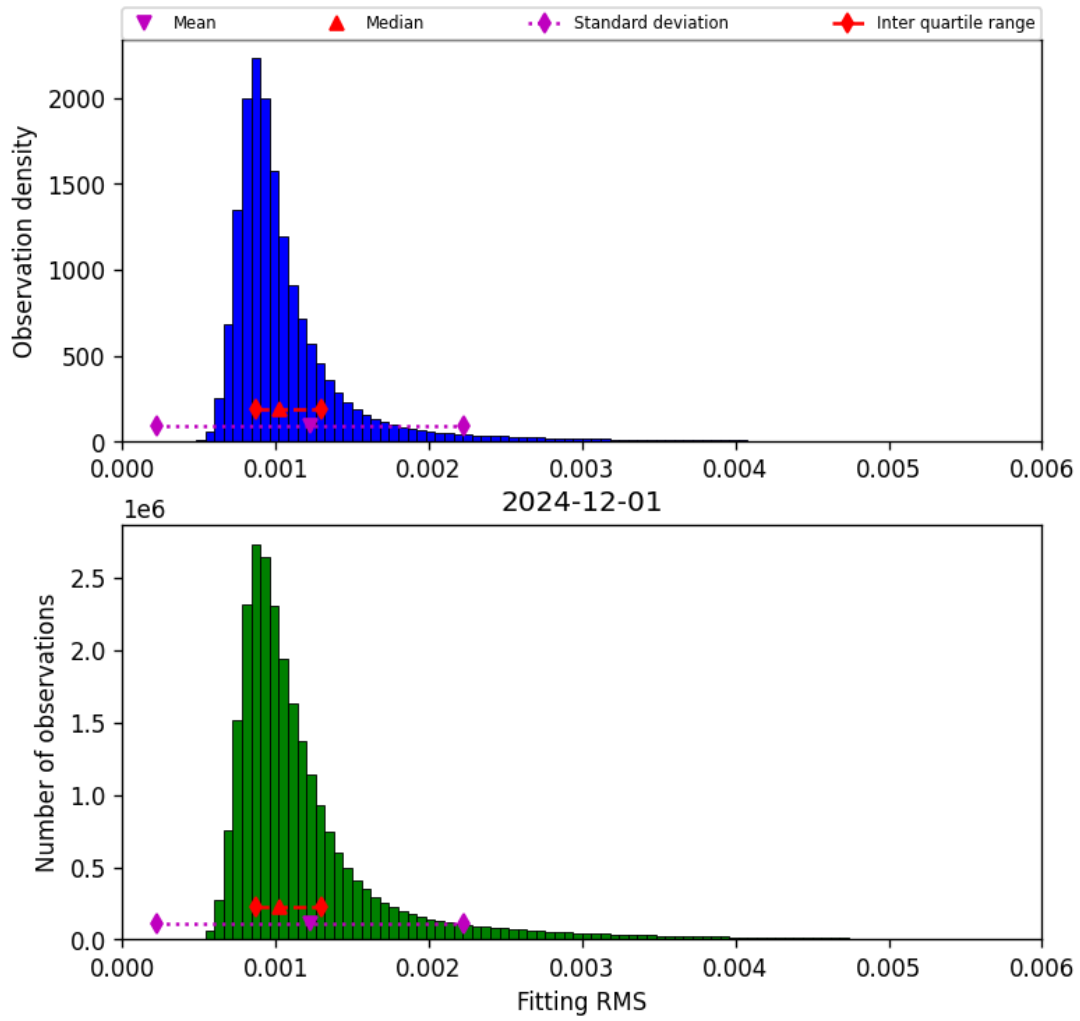
Figure 23: Histogram of “Fitting RMS” for 2024-11-30 to 2024-12-02
