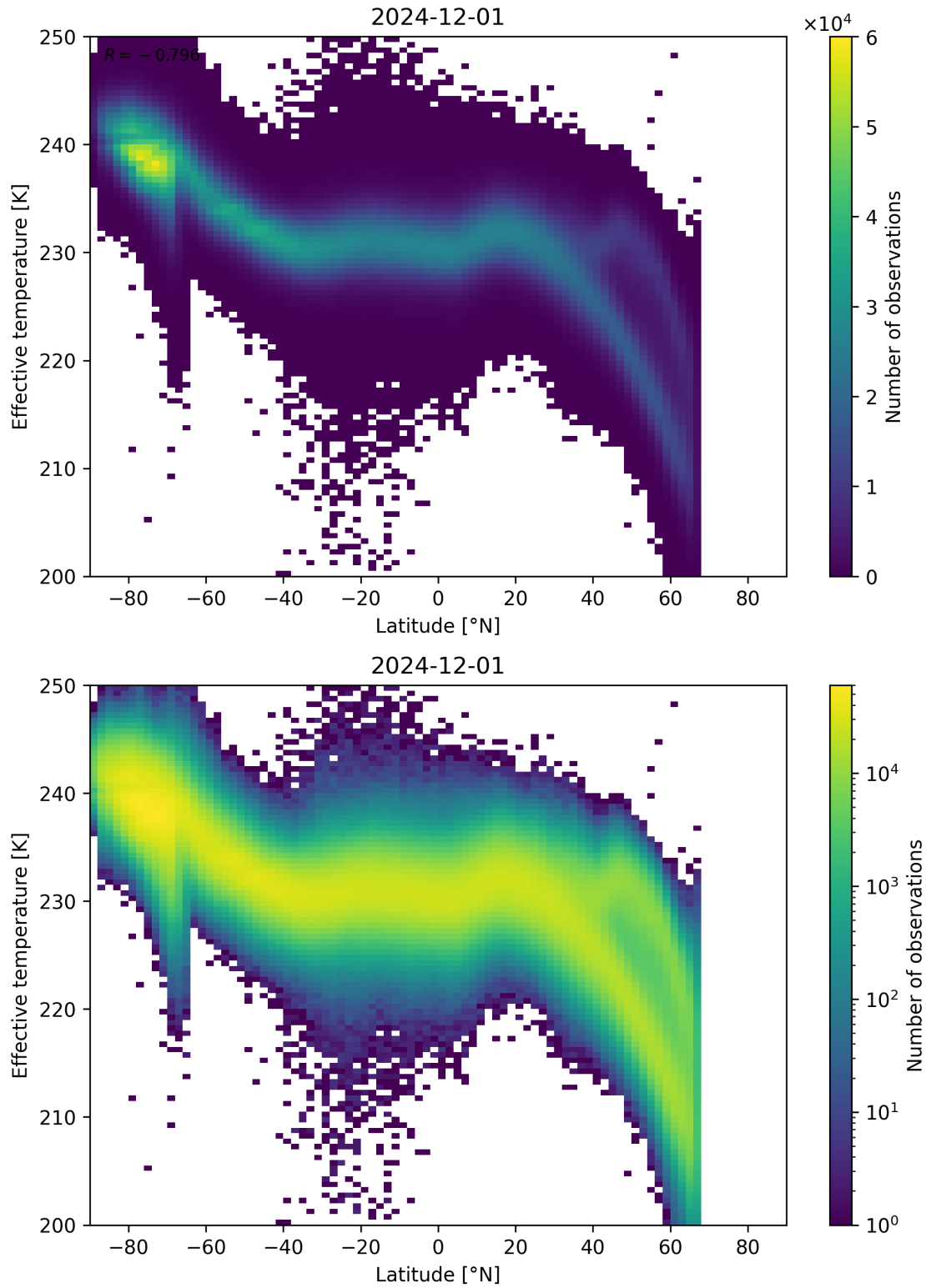
Figure 34: Scatter density plot of “Latitude” against “Effective temperature” for 2024-11-30 to 2024-12-02.
