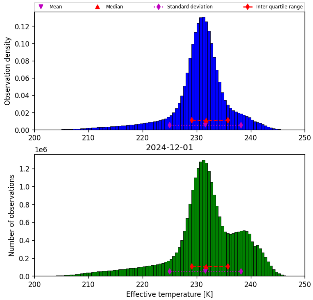
Figure 24: Histogram of “Effective temperature” for 2024-11-30 to 2024-12-02
