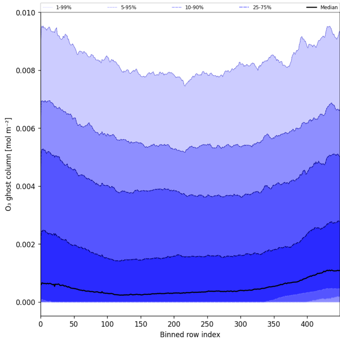
Figure 32: Along track statistics of “O 3 ghost column” for 2024-11-30 to 2024-12-02
