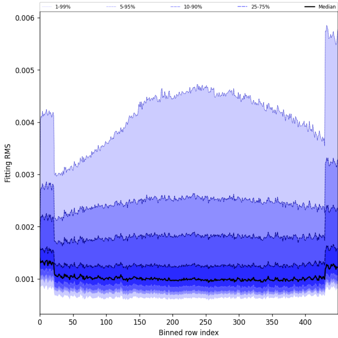
Figure 30: Along track statistics of “Fitting RMS” for 2024-11-30 to 2024-12-02
