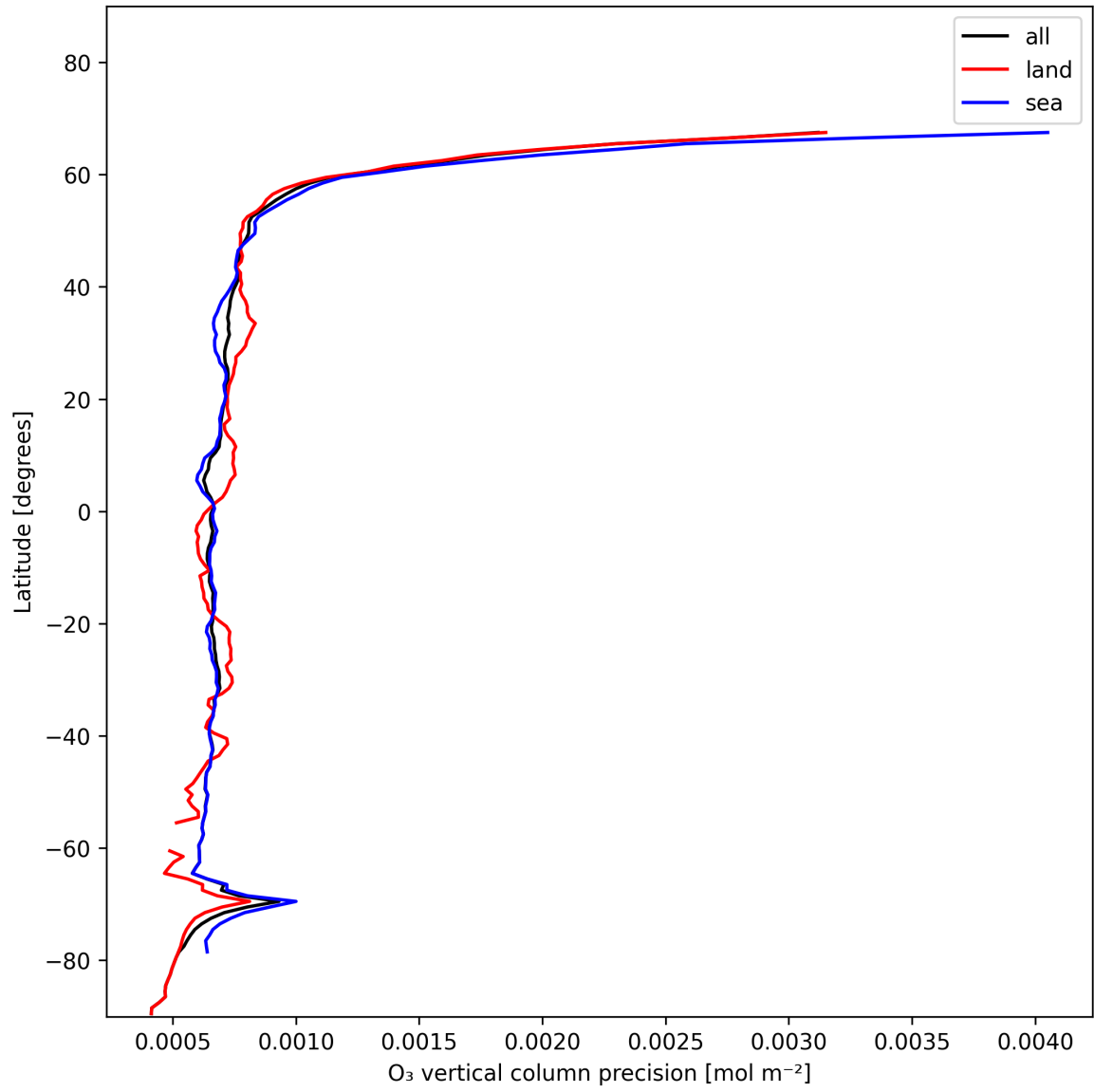
Figure 15: Zonal average of “O 3 vertical column precision” for 2024-11-30 to 2024-12-02.
