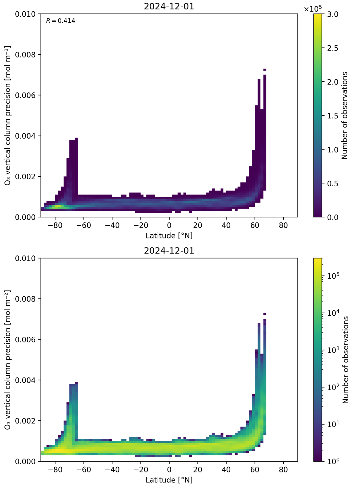
Figure 37: Scatter density plot of “Latitude” against “O 3 vertical column precision” for 2024-11-30 to 2024-12-02.
