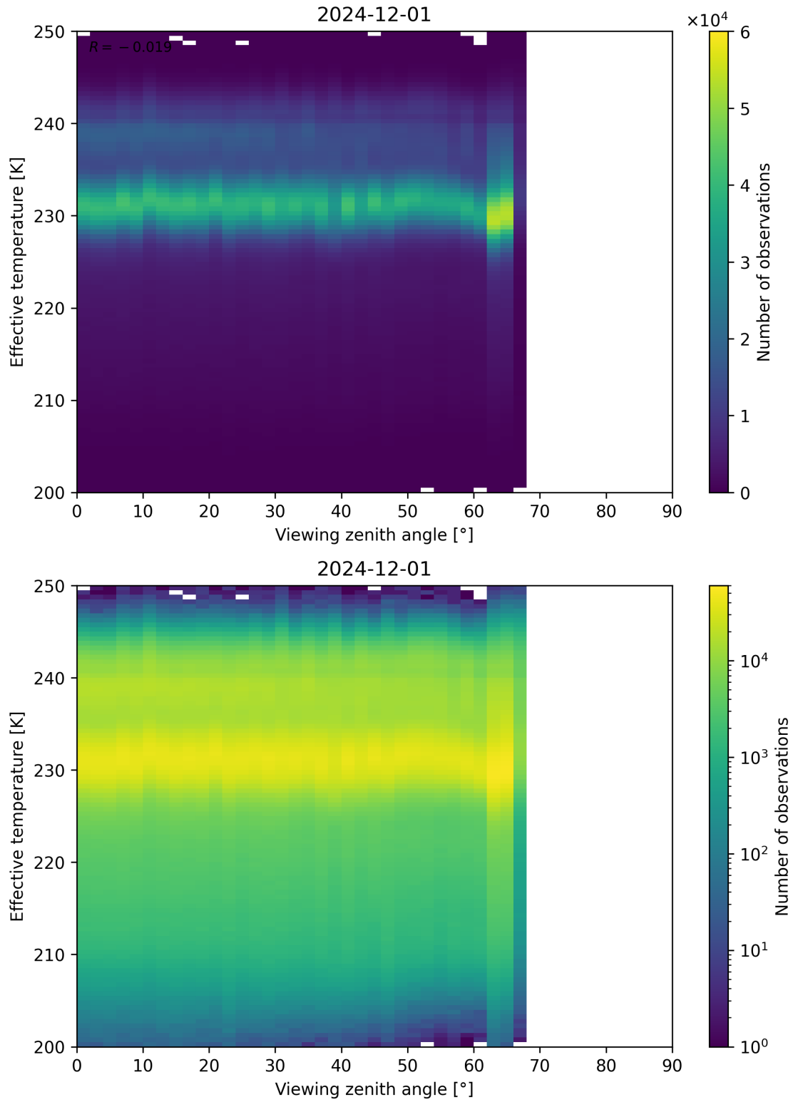
Figure 50: Scatter density plot of “Viewing zenith angle” against “Effective temperature” for 2024-11-30 to 2024-12-02.
