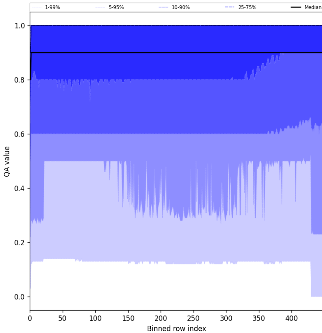
Figure 27: Along track statistics of “QA value” for 2024-11-30 to 2024-12-02
