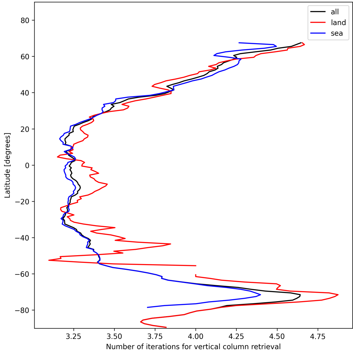
Figure 19: Zonal average of “Number of iterations for vertical column retrieval” for 2024-11-30 to 2024-12-02.
