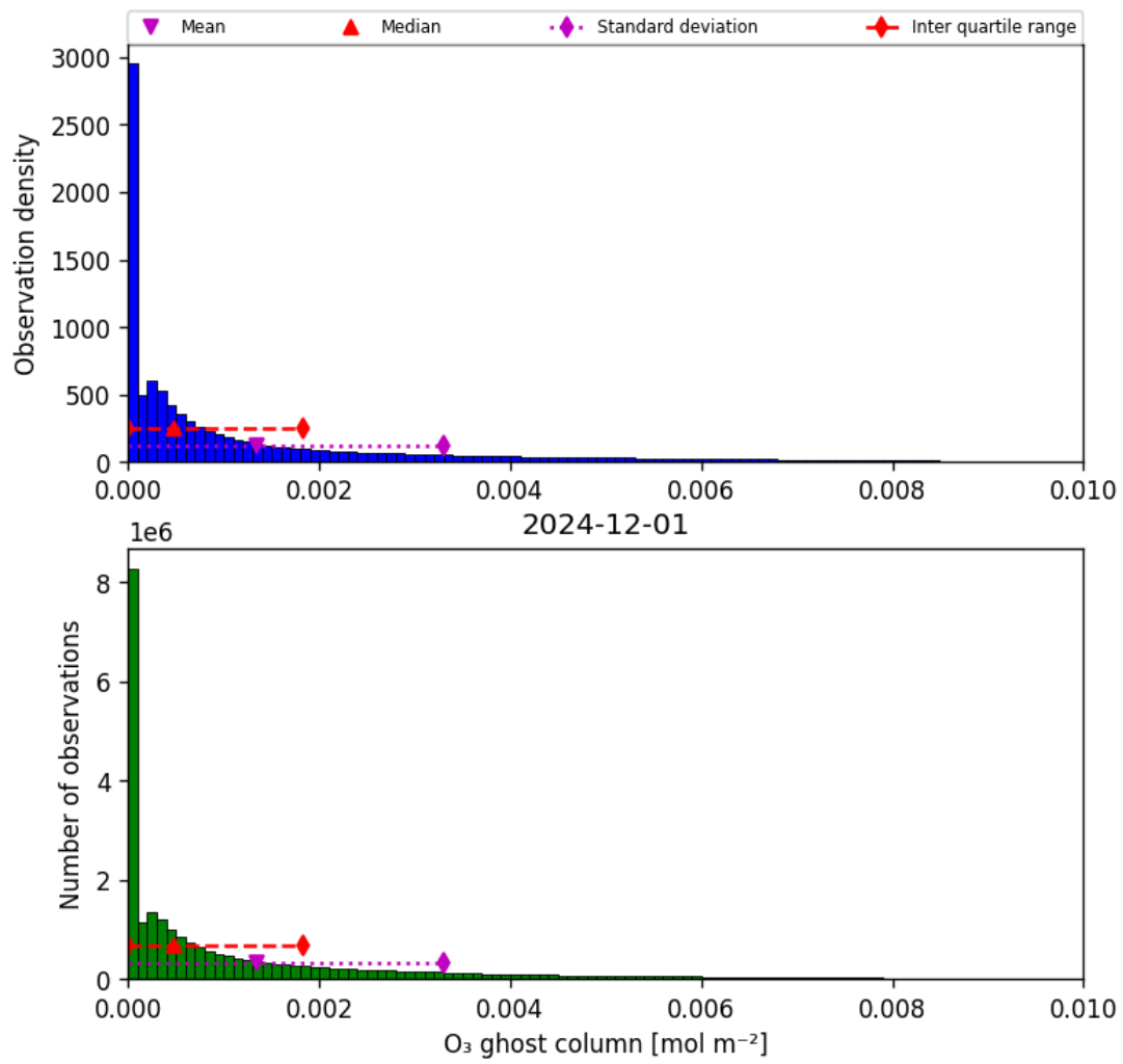
Figure 25: Histogram of “O 3 ghost column” for 2024-11-30 to 2024-12-02
