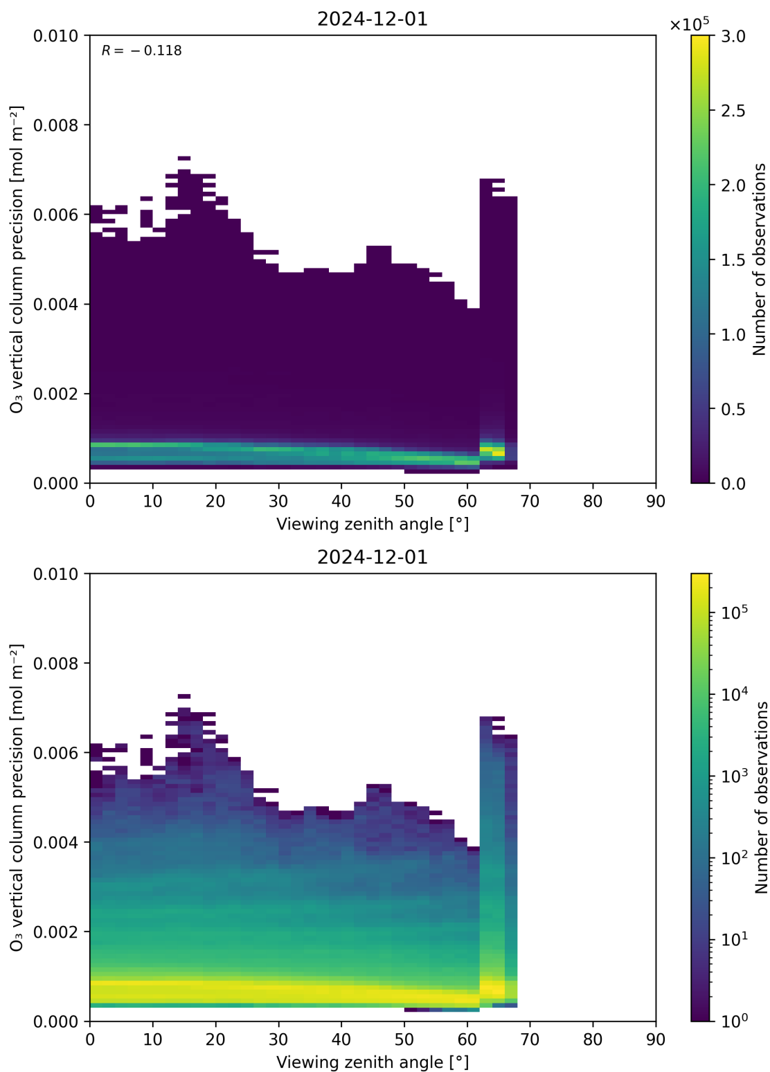
Figure 53: Scatter density plot of “Viewing zenith angle” against “O 3 vertical column precision” for 2024-11-30 to 2024-12-02.
