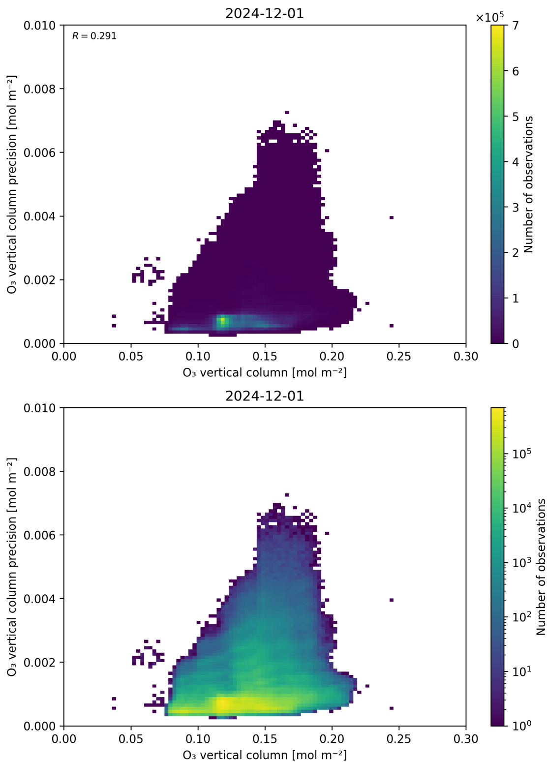
Figure 41: Scatter density plot of “O 3 vertical column” against “O 3 vertical column precision” for 2024-11-30 to 2024-12-02.
