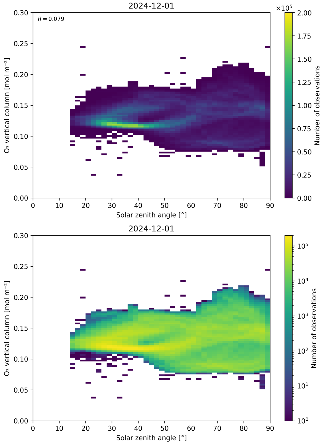
Figure 47: Scatter density plot of “Solar zenith angle” against “O 3 vertical column” for 2024-11-30 to 2024-12-02.
