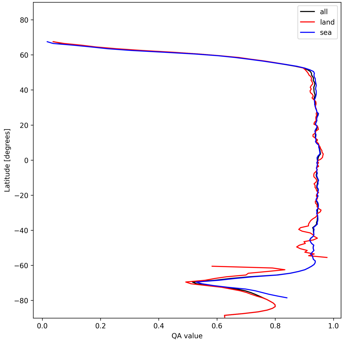
Figure 13: Zonal average of “QA value” for 2024-11-30 to 2024-12-02.
