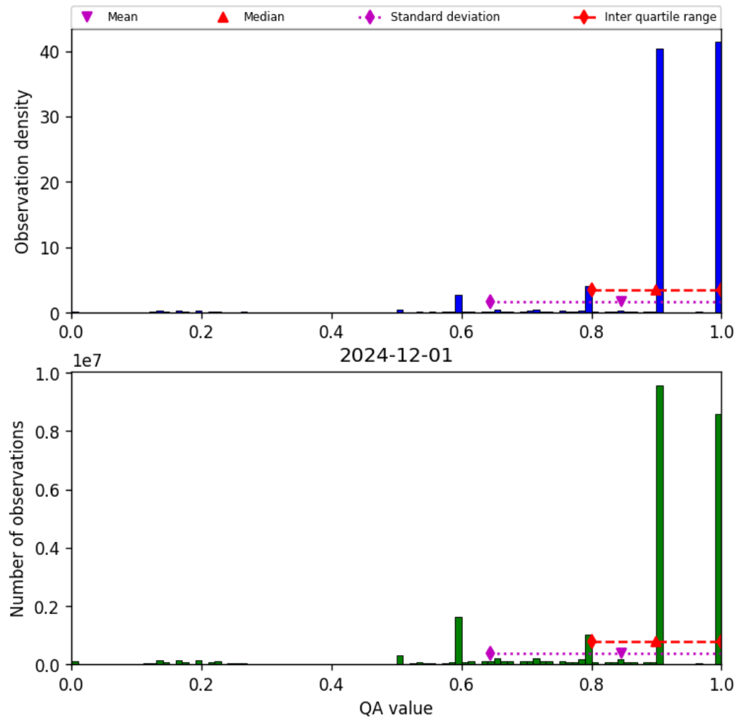
Figure 20: Histogram of “QA value” for 2024-11-30 to 2024-12-02
