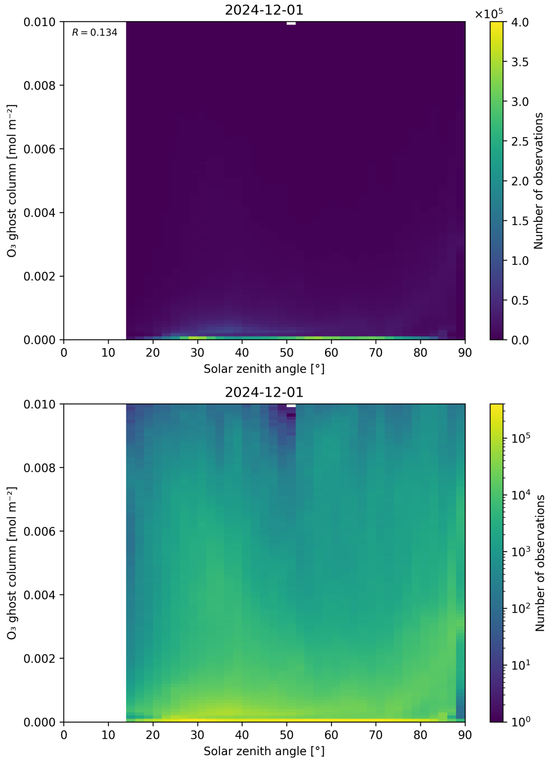
Figure 46: Scatter density plot of “Solar zenith angle” against “O 3 ghost column” for 2024-11-30 to 2024-12-02.
