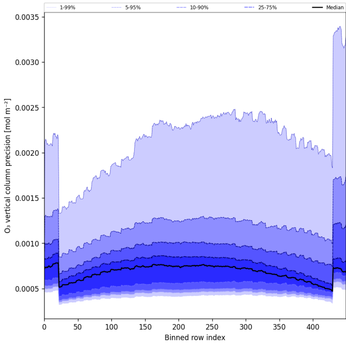
Figure 29: Along track statistics of “O 3 vertical column precision” for 2024-11-30 to 2024-12-02
