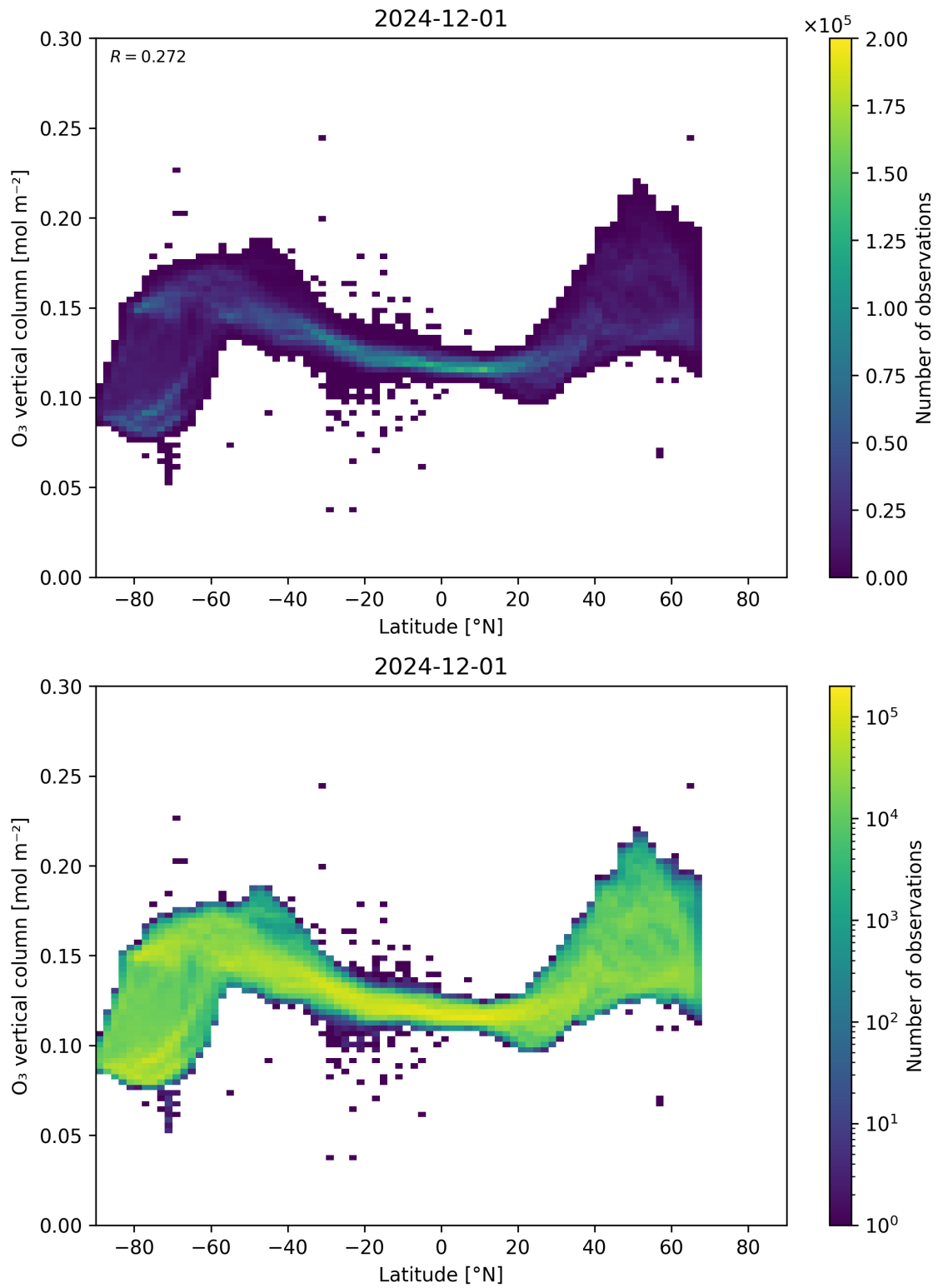
Figure 36: Scatter density plot of “Latitude” against “O 3 vertical column” for 2024-11-30 to 2024-12-02.
