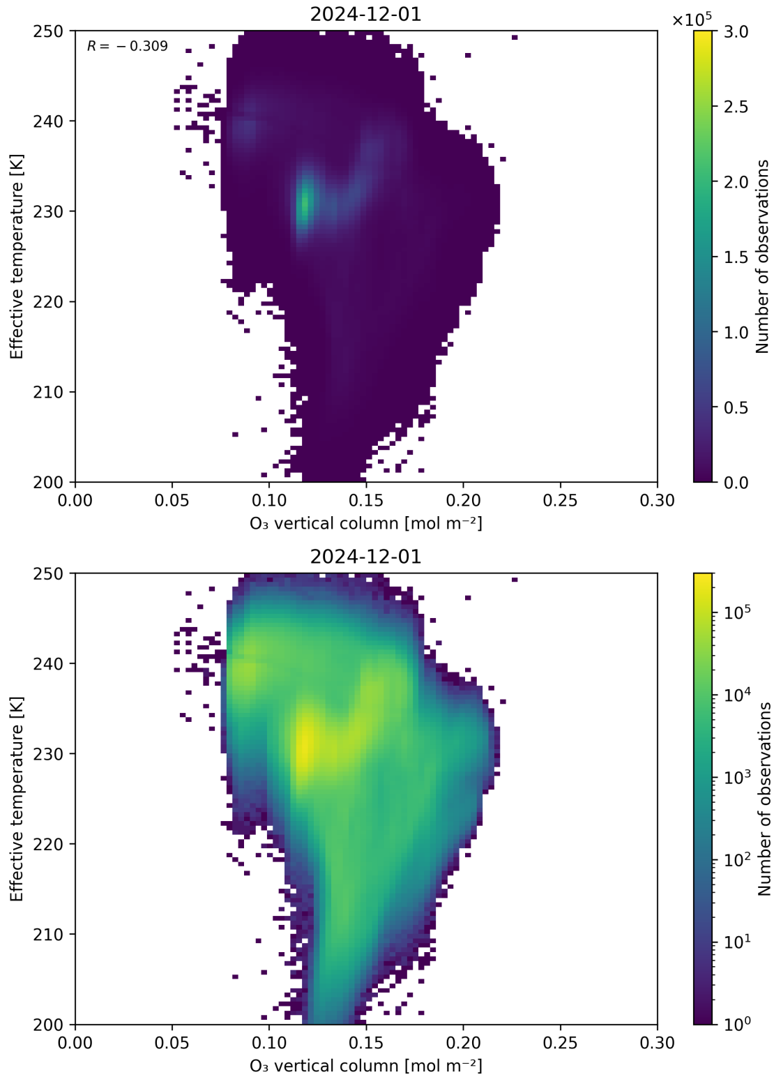
Figure 39: Scatter density plot of “O 3 vertical column” against “Effective temperature” for 2024-11-30 to 2024-12-02.
