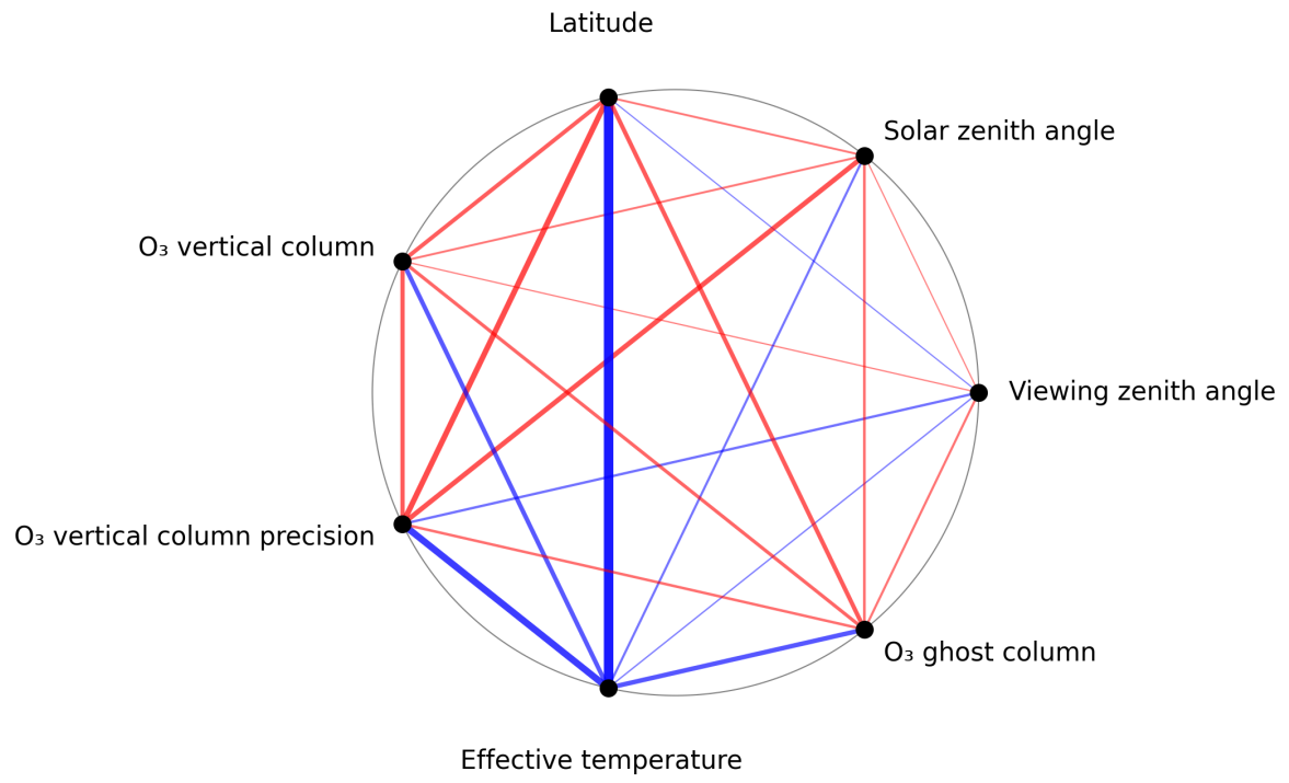
Figure 1: Map of correlation graph for 2024-11-30 to 2024-12-02.
