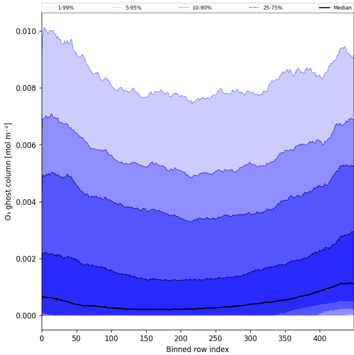
Figure 32: Along track statistics of “O 3 ghost column” for 2024-12-02 to 2024-12-04
