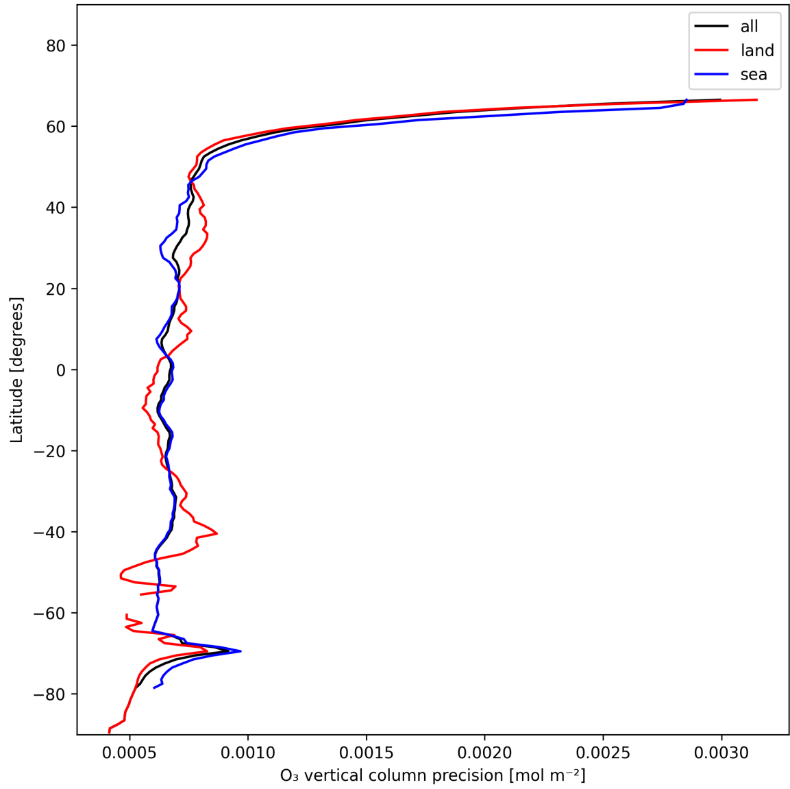
Figure 15: Zonal average of “O 3 vertical column precision” for 2024-12-02 to 2024-12-04.
