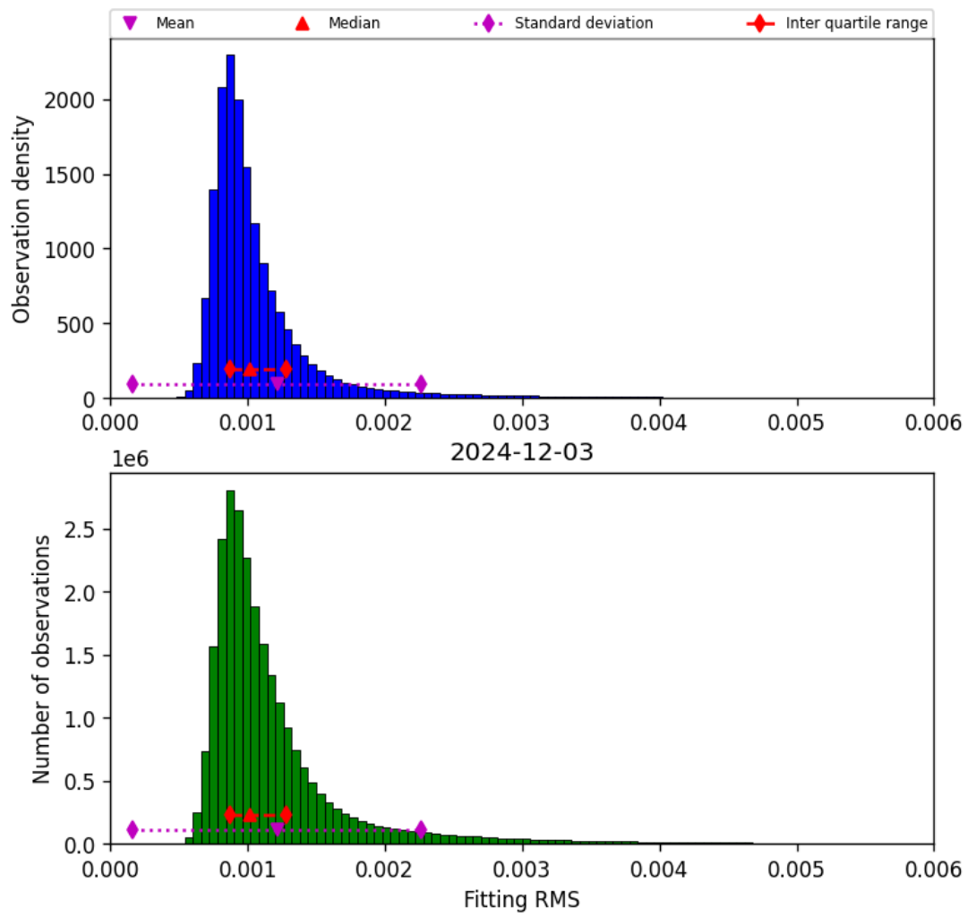
Figure 23: Histogram of “Fitting RMS” for 2024-12-02 to 2024-12-04
