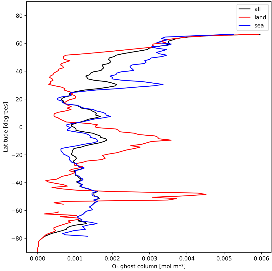
Figure 18: Zonal average of “O 3 ghost column” for 2024-12-02 to 2024-12-04.
