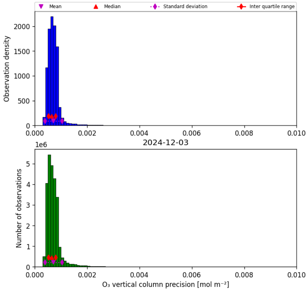
Figure 22: Histogram of "O 3 vertical column precision" for 2024-12-02 to 2024-12-04
