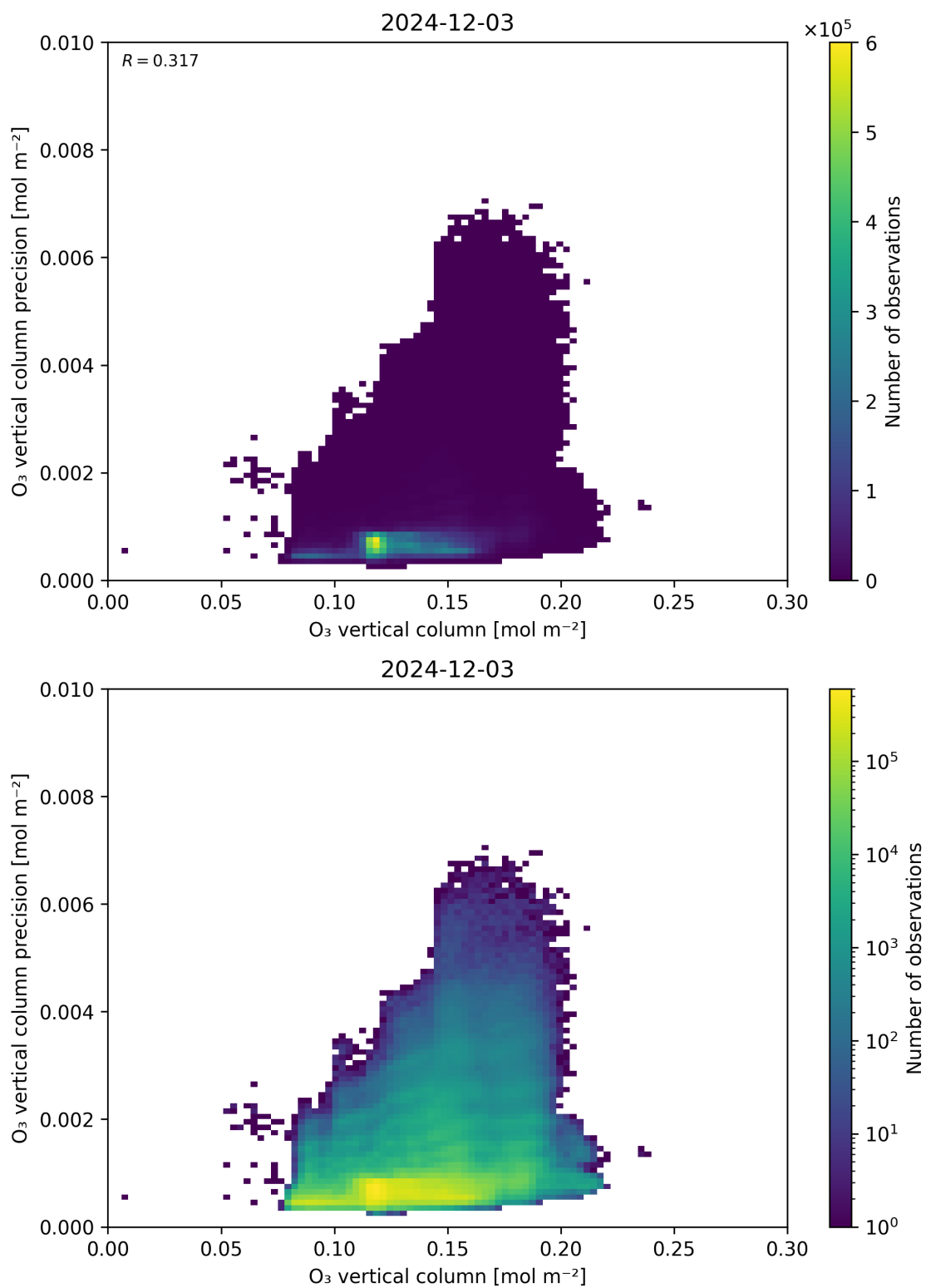
Figure 41: Scatter density plot of “O 3 vertical column” against “O 3 vertical column precision” for 2024-12-02 to 2024-12-04.
