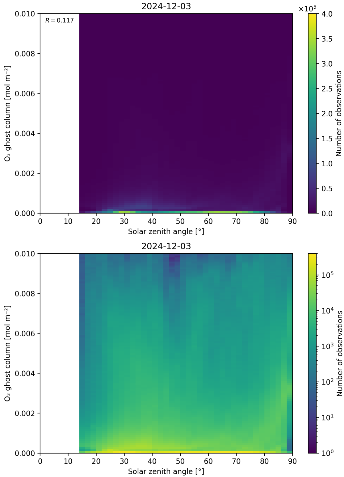
Figure 46: Scatter density plot of “Solar zenith angle” against “O 3 ghost column” for 2024-12-02 to 2024-12-04.
