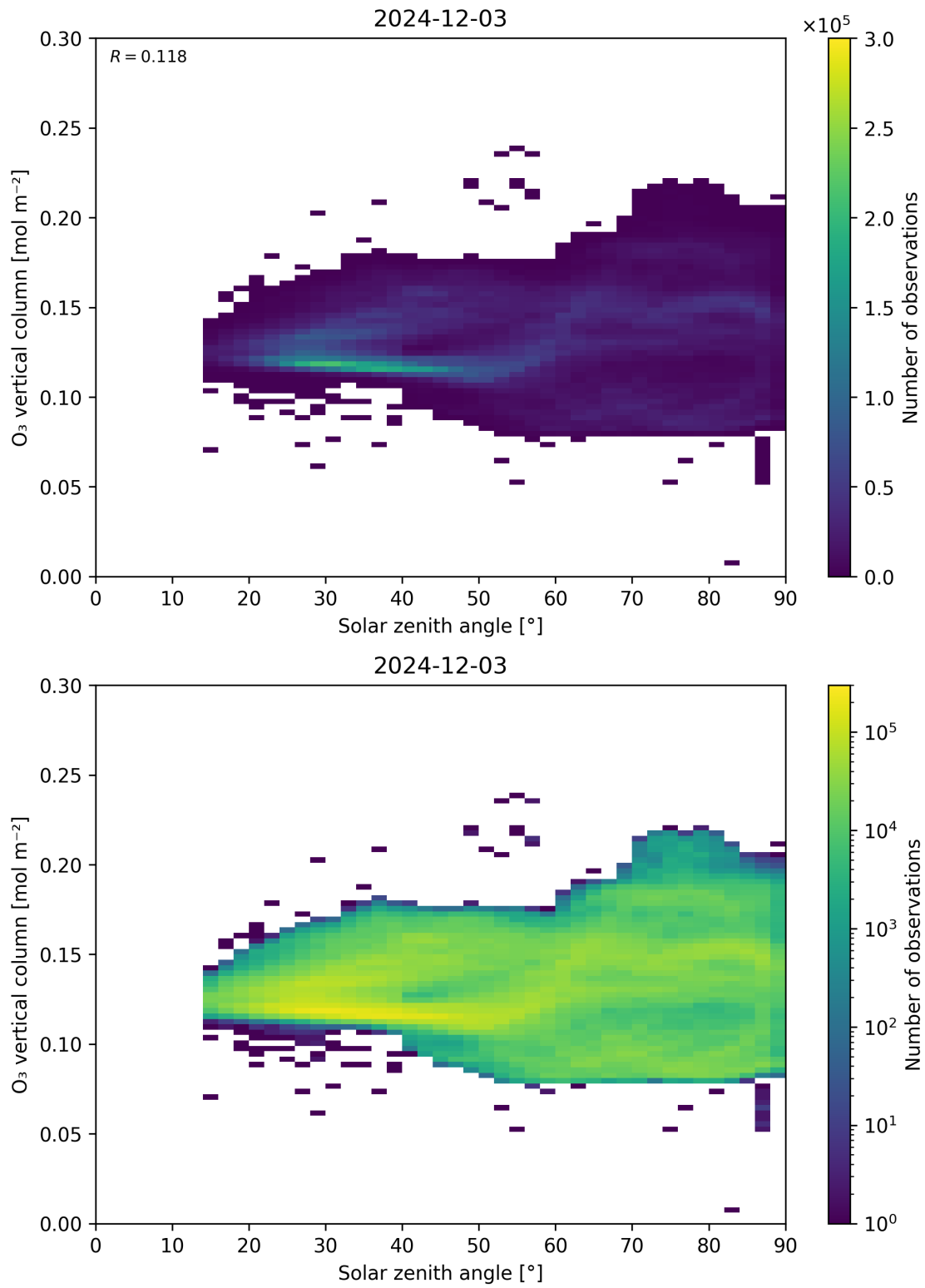
Figure 47: Scatter density plot of “Solar zenith angle” against “O 3 vertical column” for 2024-12-02 to 2024-12-04.
