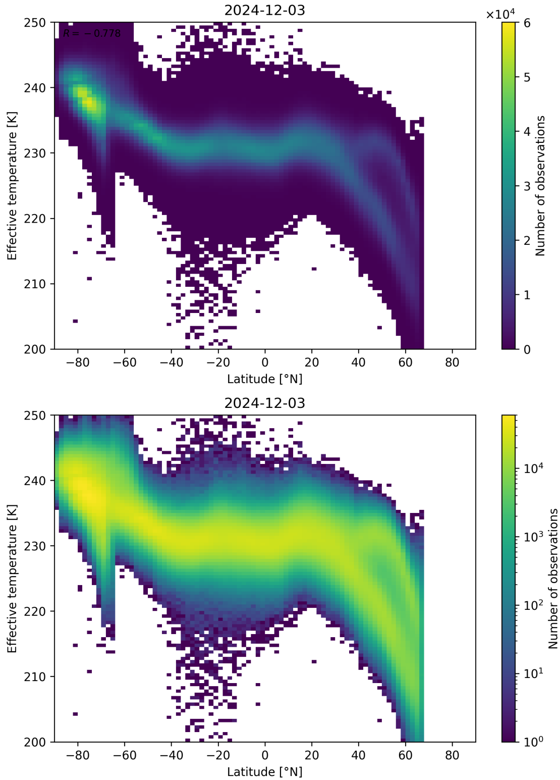
Figure 34: Scatter density plot of “Latitude” against “Effective temperature” for 2024-12-02 to 2024-12-04.
