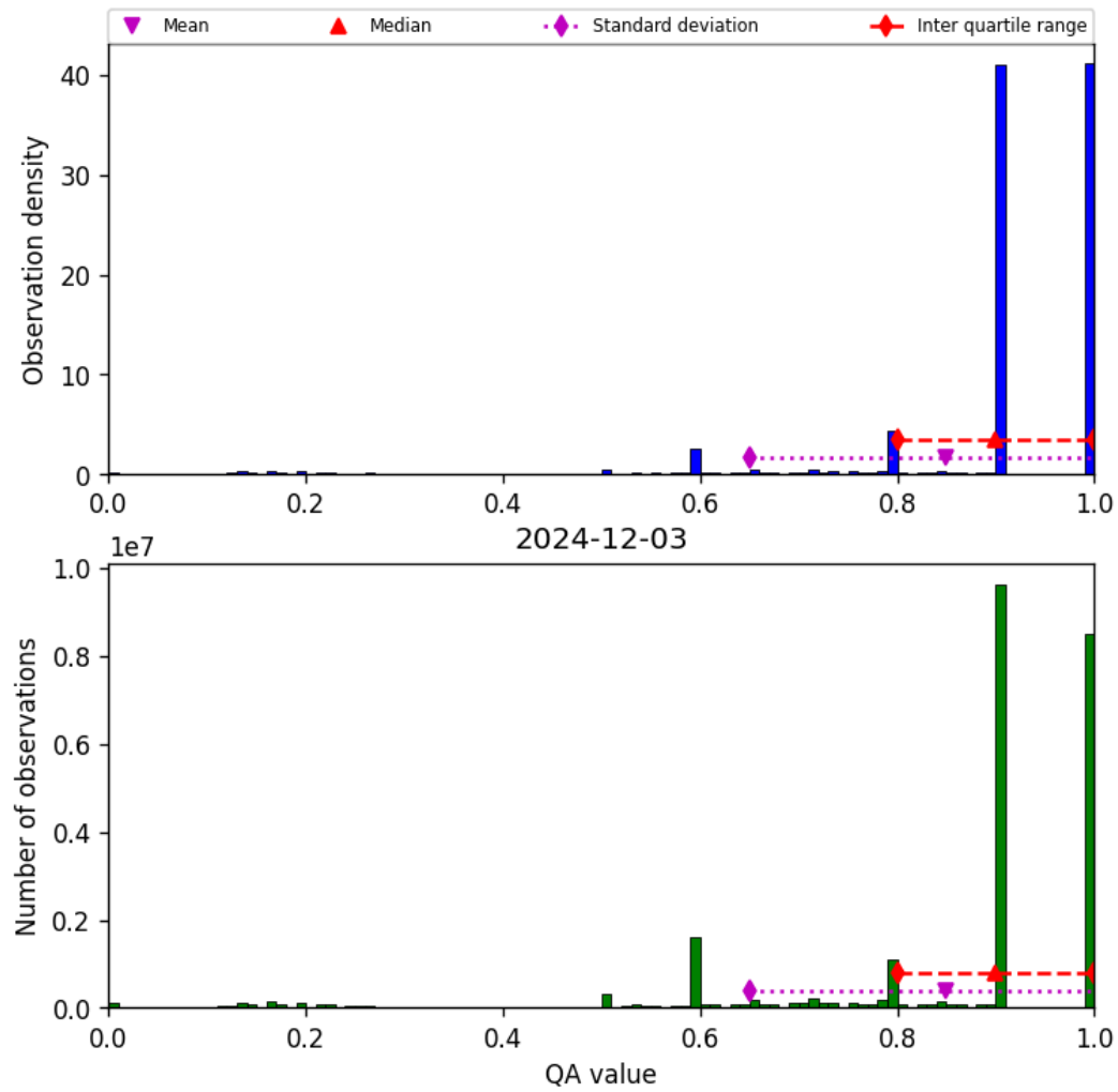
Figure 20: Histogram of “QA value” for 2024-12-02 to 2024-12-04
