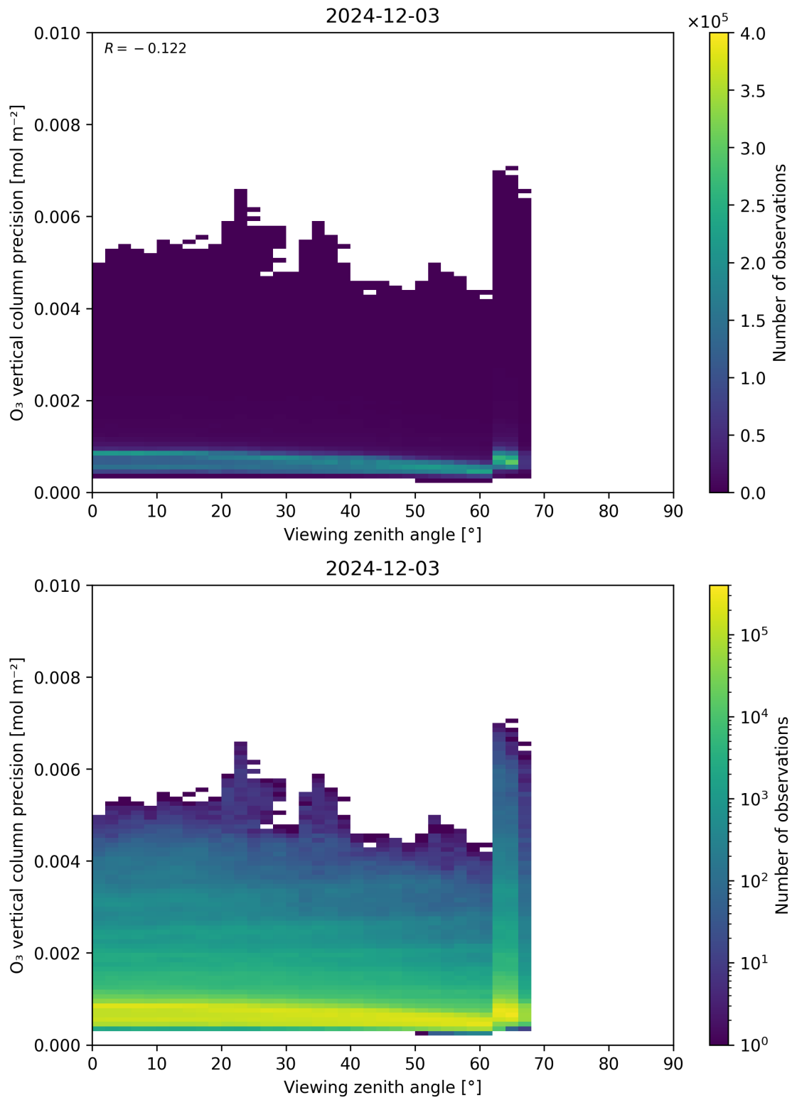
Figure 53: Scatter density plot of “Viewing zenith angle” against “O 3 vertical column precision” for 2024-12-02 to 2024-12-04.
