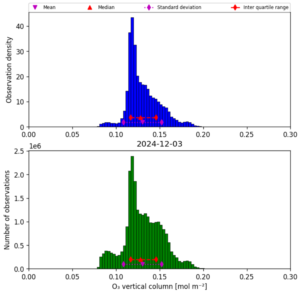
Figure 21: Histogram of “O 3 vertical column” for 2024-12-02 to 2024-12-04
