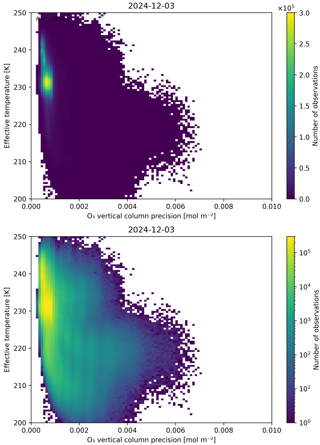
Figure 42: Scatter density plot of “O 3 vertical column precision” against “Effective temperature” for 2024-12-02 to 2024-12-04.
