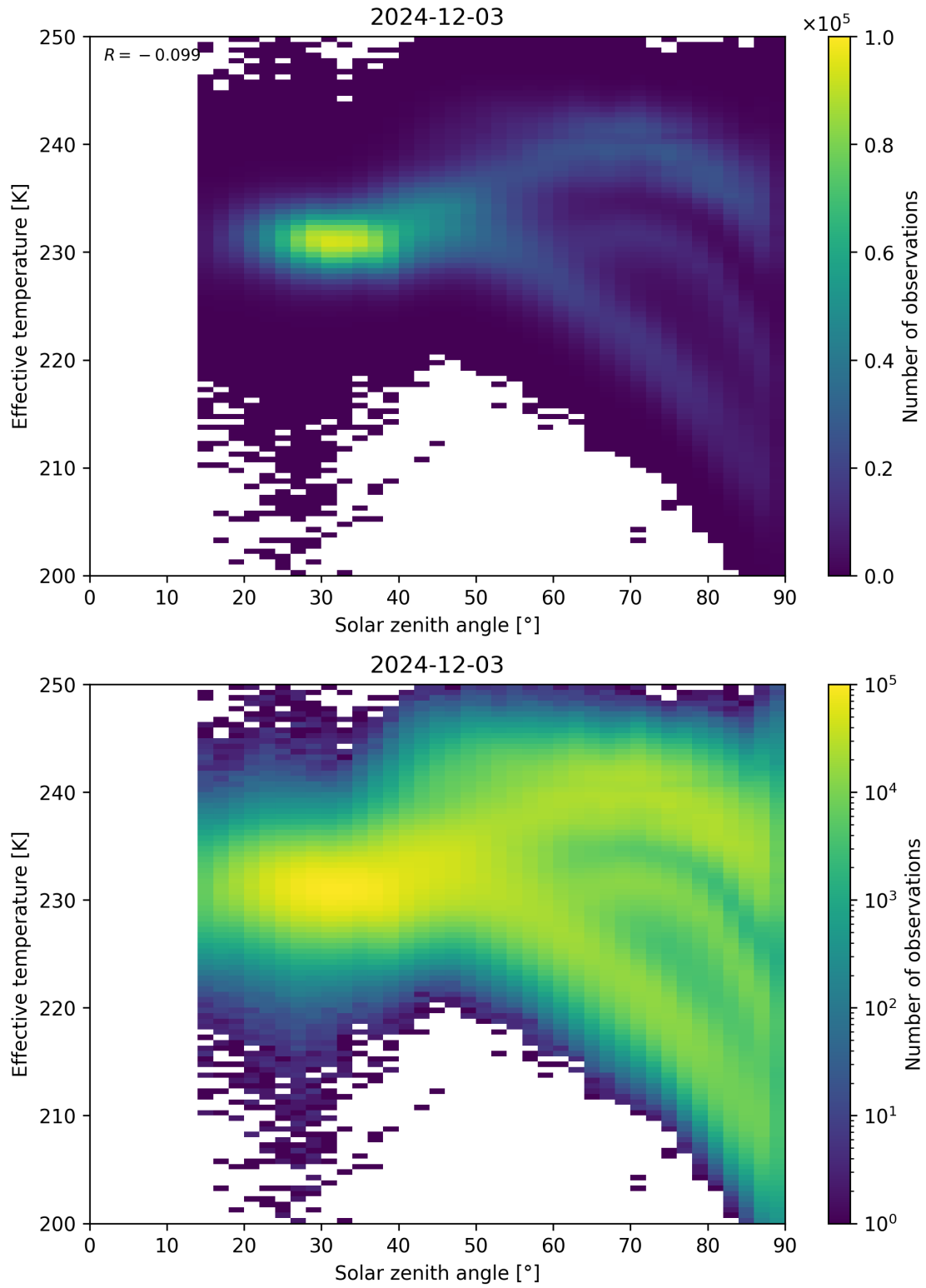
Figure 45: Scatter density plot of “Solar zenith angle” against “Effective temperature” for 2024-12-02 to 2024-12-04.
