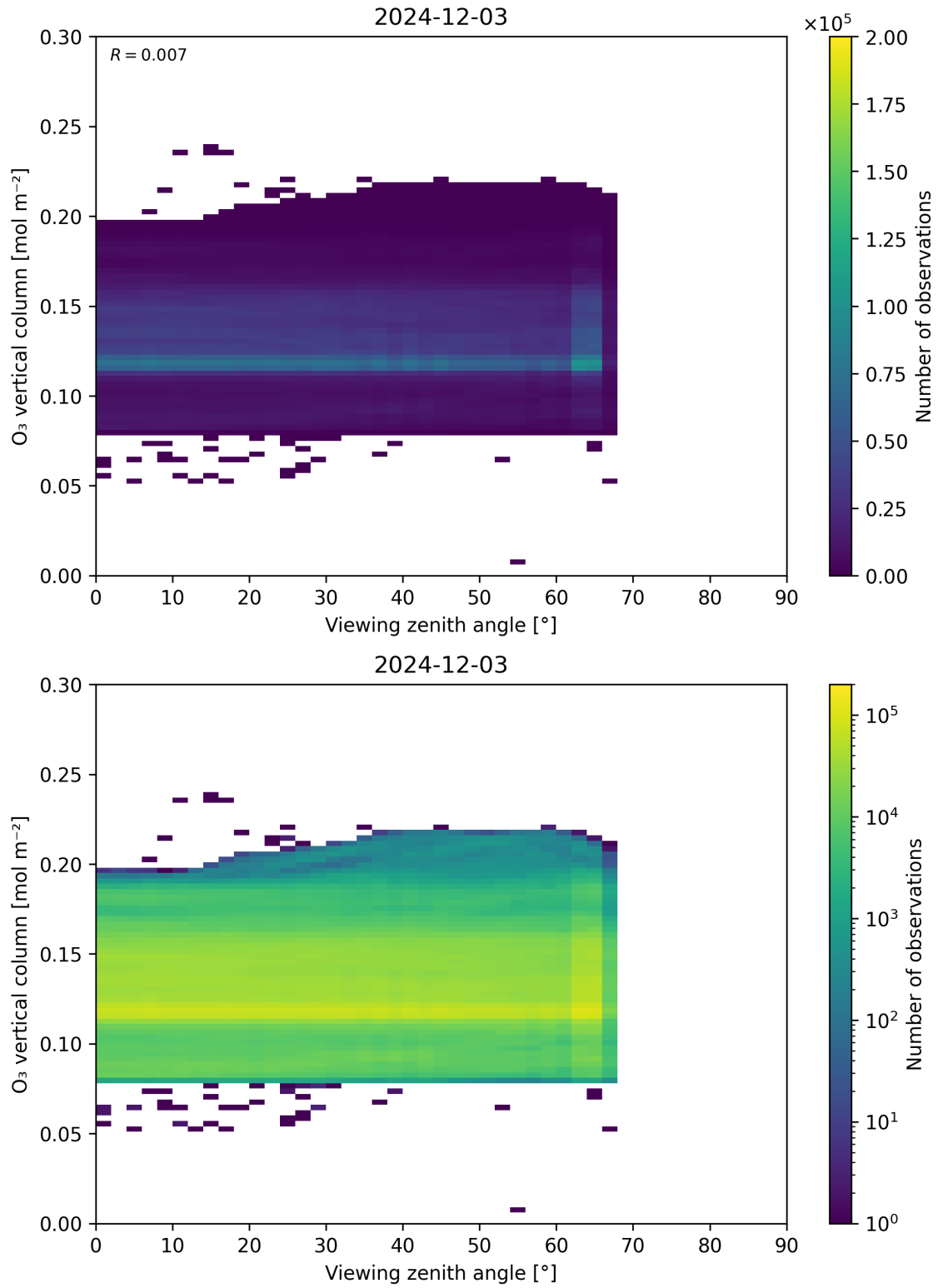
Figure 52: Scatter density plot of “Viewing zenith angle” against “O 3 vertical column” for 2024-12-02 to 2024-12-04.
