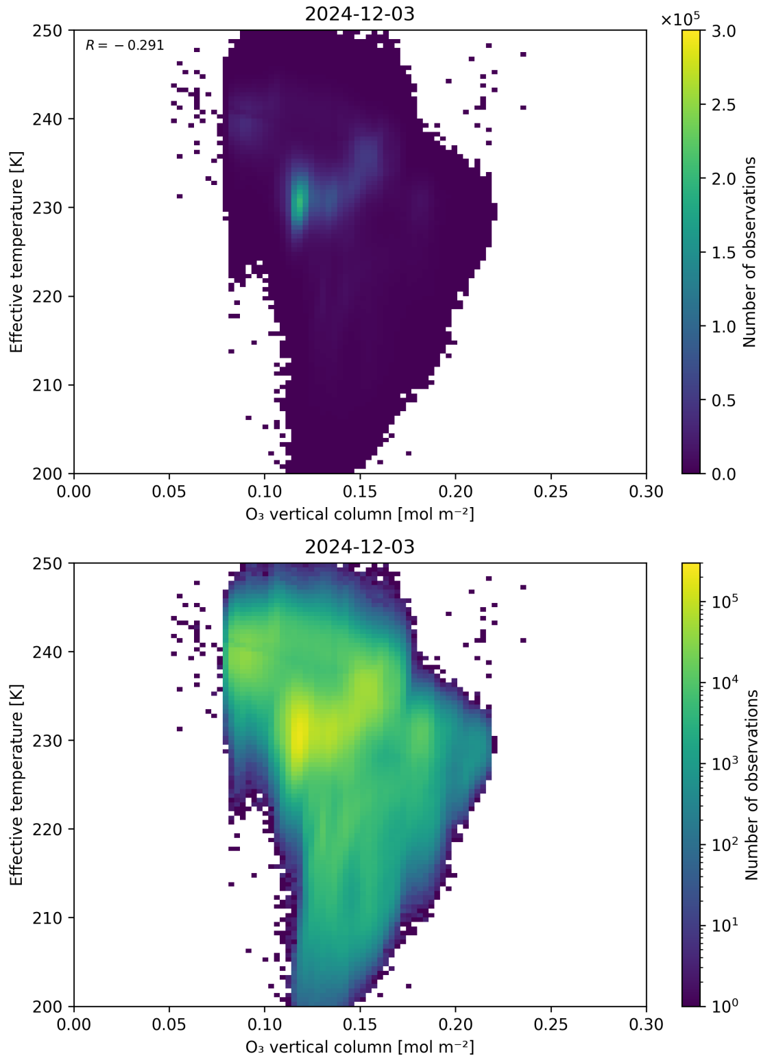
Figure 39: Scatter density plot of “O 3 vertical column” against “Effective temperature” for 2024-12-02 to 2024-12-04.
