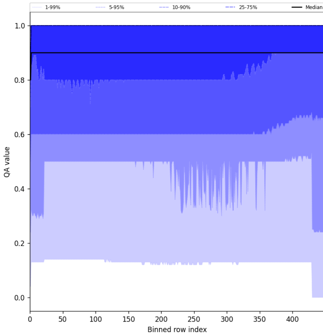
Figure 27: Along track statistics of “QA value” for 2024-12-02 to 2024-12-04
