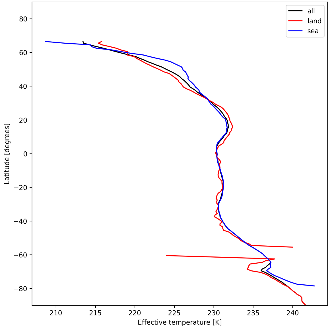
Figure 17: Zonal average of “Effective temperature” for 2024-12-02 to 2024-12-04.
