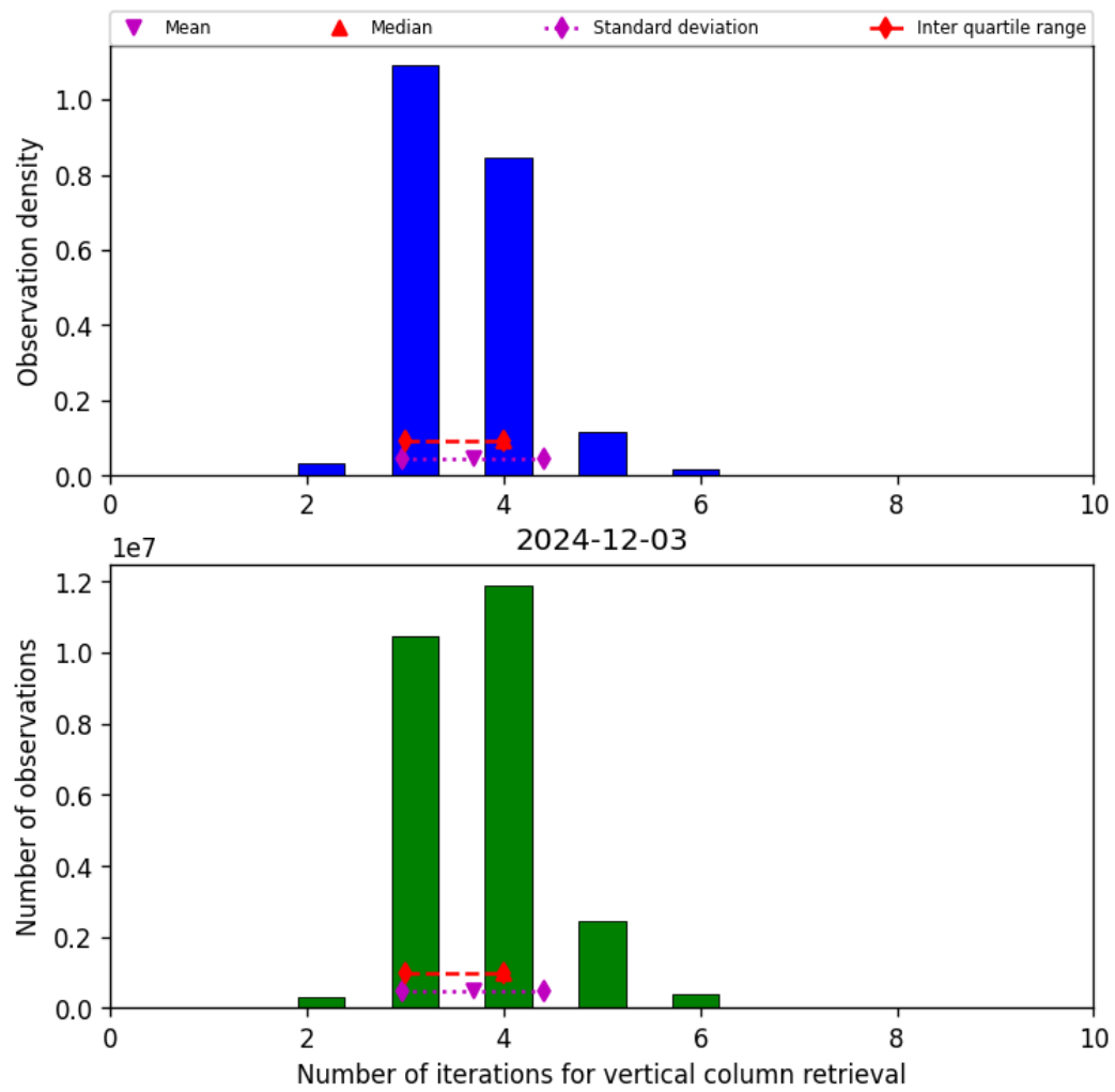
Figure 26: Histogram of “Number of iterations for vertical column retrieval” for 2024-12-02 to 2024-12-04
