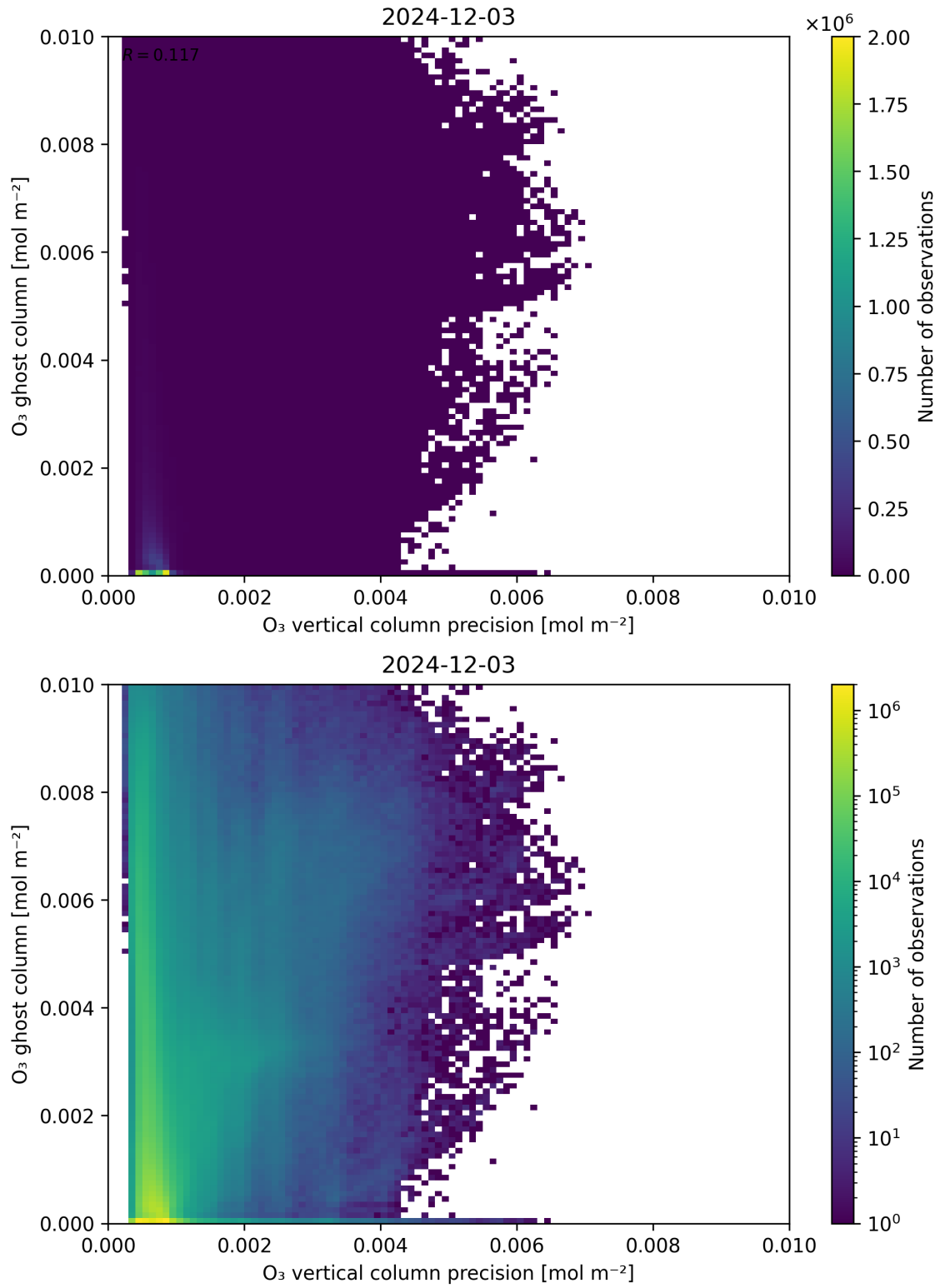
Figure 43: Scatter density plot of “O 3 vertical column precision” against “O 3 ghost column” for 2024-12-02 to 2024-12-04.
