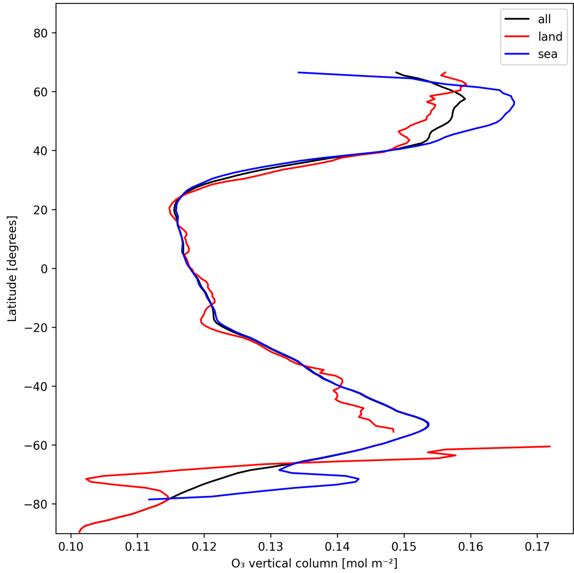
Figure 14: Zonal average of “O 3 vertical column” for 2024-12-02 to 2024-12-04.
