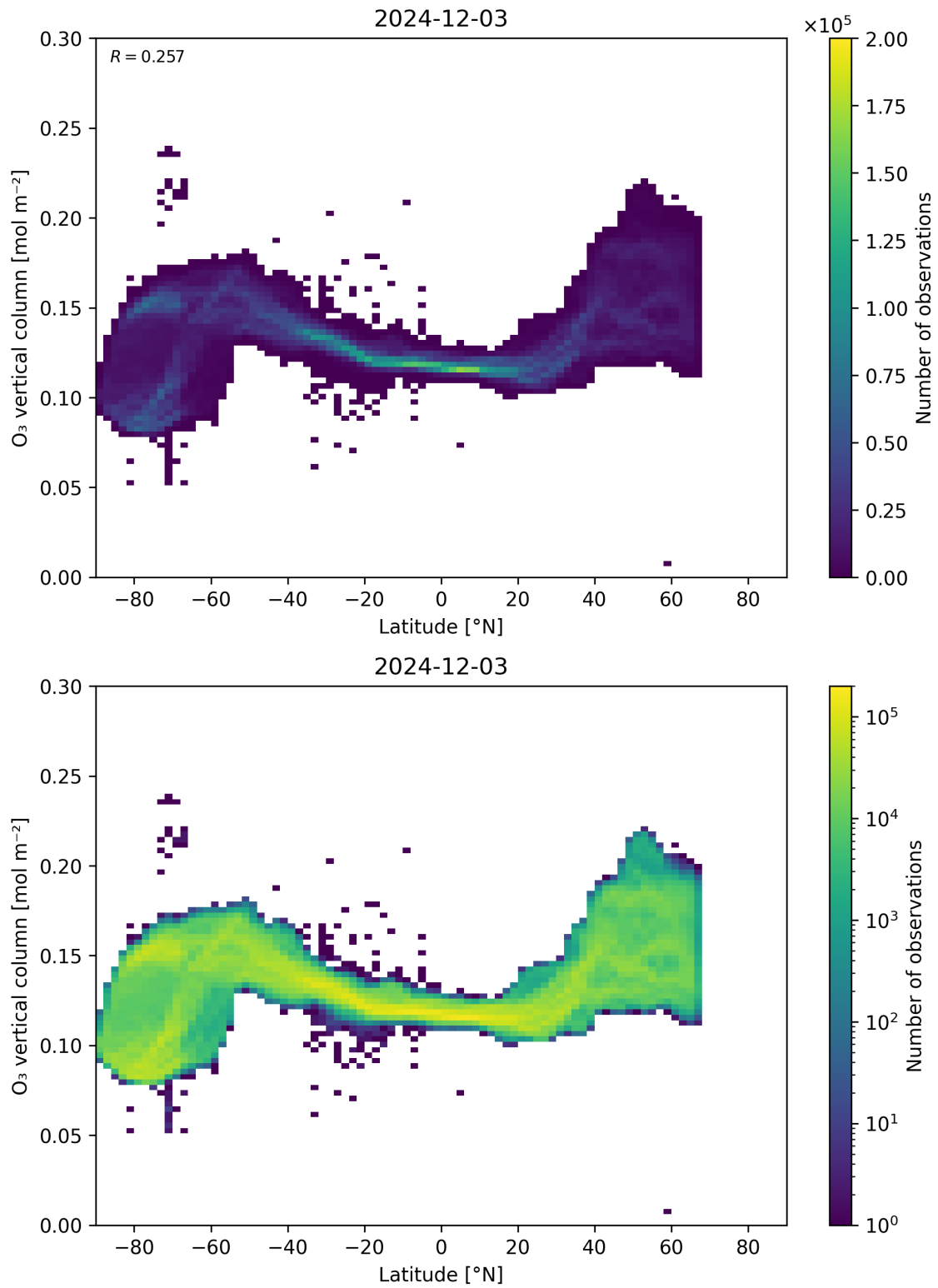
Figure 36: Scatter density plot of “Latitude” against “O 3 vertical column” for 2024-12-02 to 2024-12-04.
