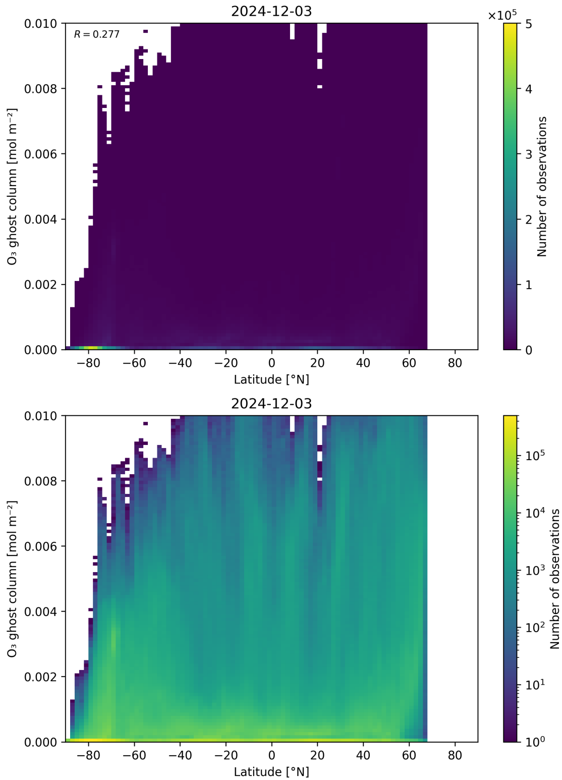
Figure 35: Scatter density plot of “Latitude” against “O 3 ghost column” for 2024-12-02 to 2024-12-04.
