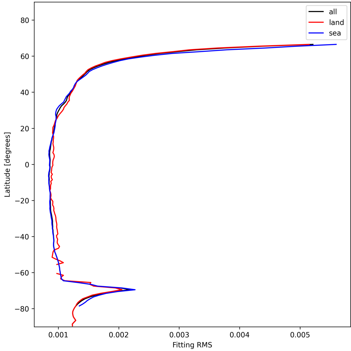
Figure 16: Zonal average of “Fitting RMS” for 2024-12-02 to 2024-12-04.
