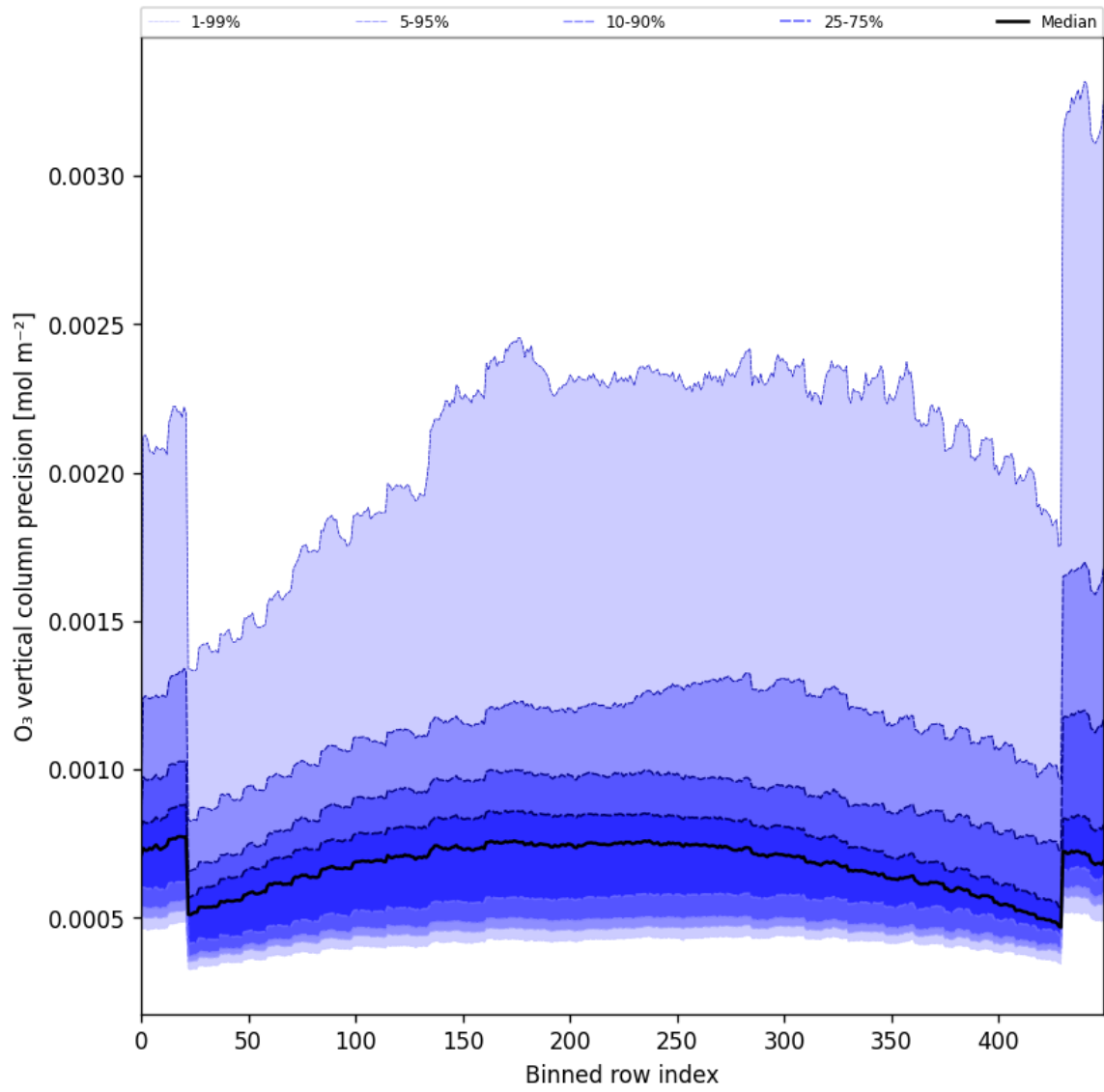
Figure 29: Along track statistics of “O 3 vertical column precision” for 2024-12-02 to 2024-12-04
