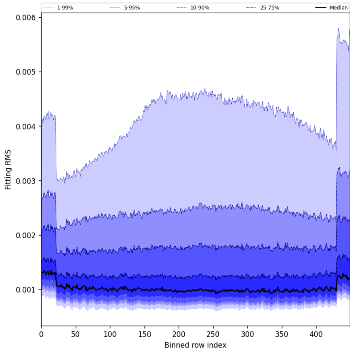
Figure 30: Along track statistics of “Fitting RMS” for 2024-12-02 to 2024-12-04
