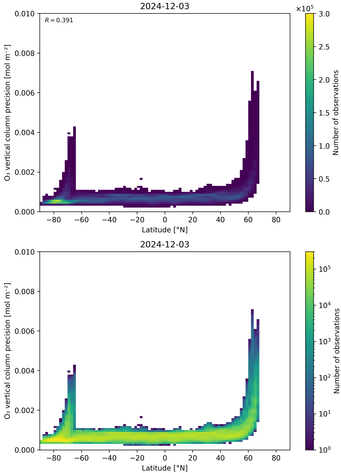
Figure 37: Scatter density plot of “Latitude” against “O 3 vertical column precision” for 2024-12-02 to 2024-12-04.
