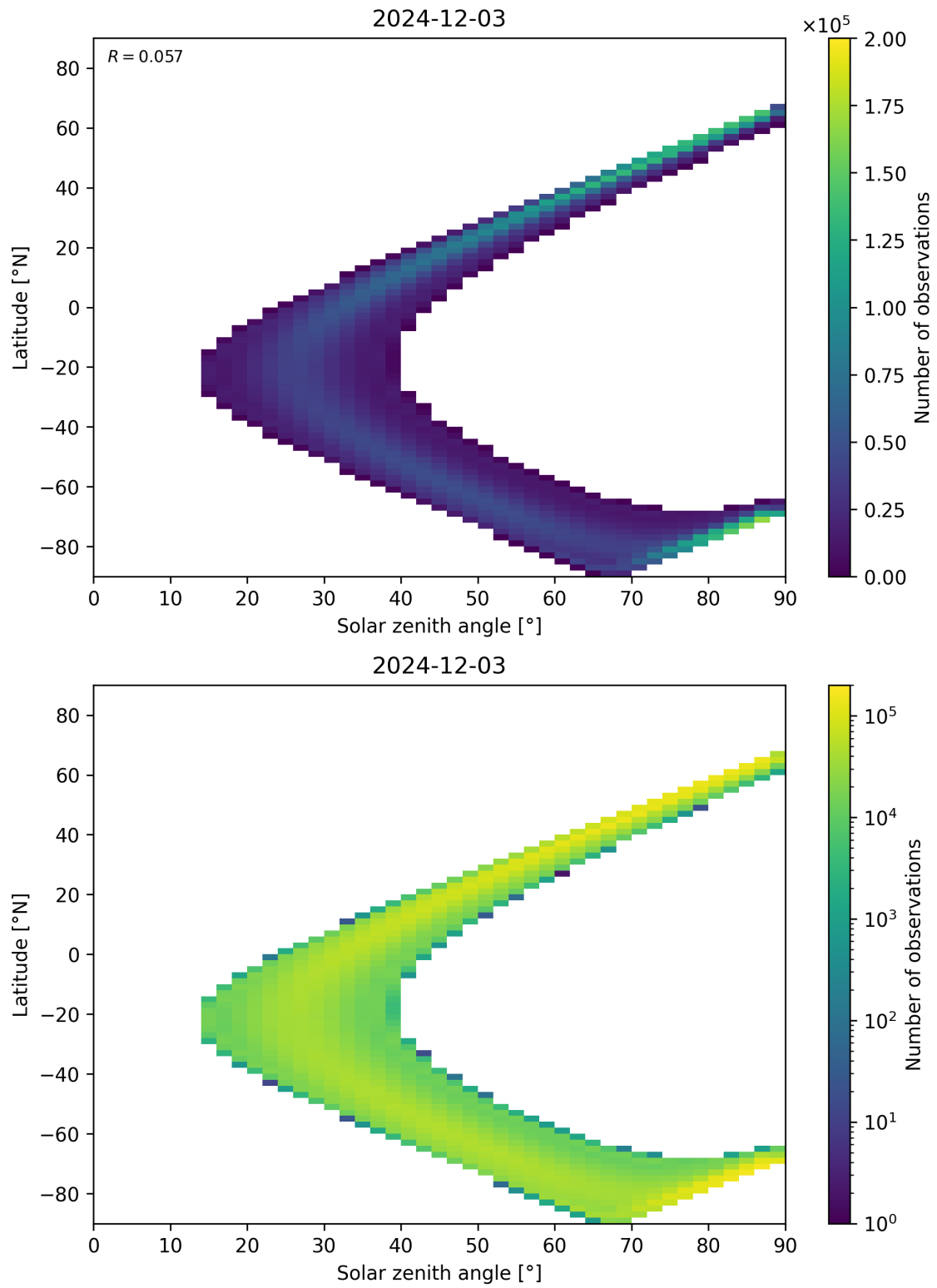
Figure 44: Scatter density plot of “Solar zenith angle” against “Latitude” for 2024-12-02 to 2024-12-04.
