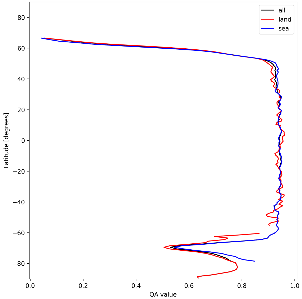
Figure 13: Zonal average of “QA value” for 2024-12-02 to 2024-12-04.
