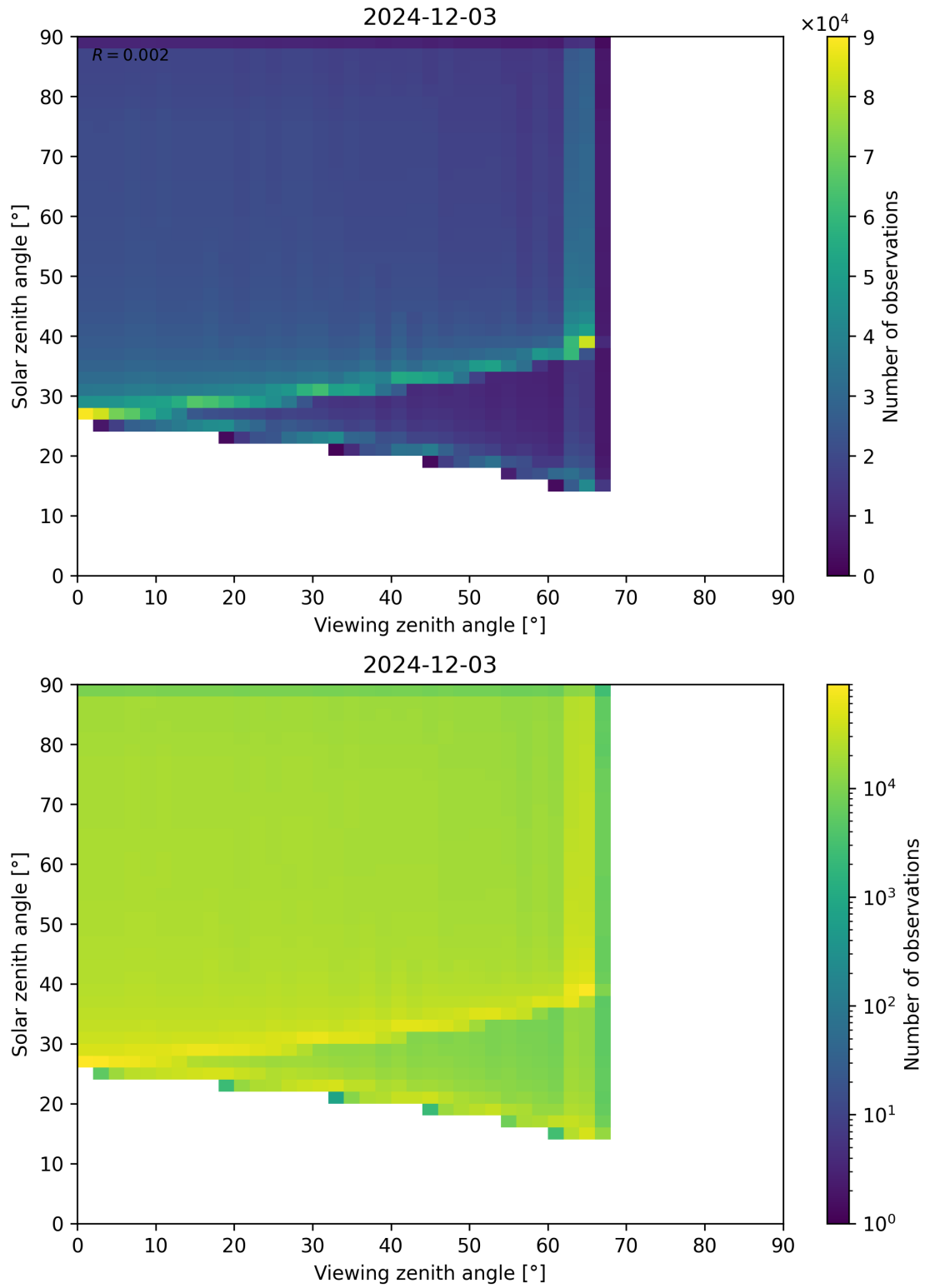
Figure 54: Scatter density plot of “Viewing zenith angle” against “Solar zenith angle” for 2024-12-02 to 2024-12-04.
