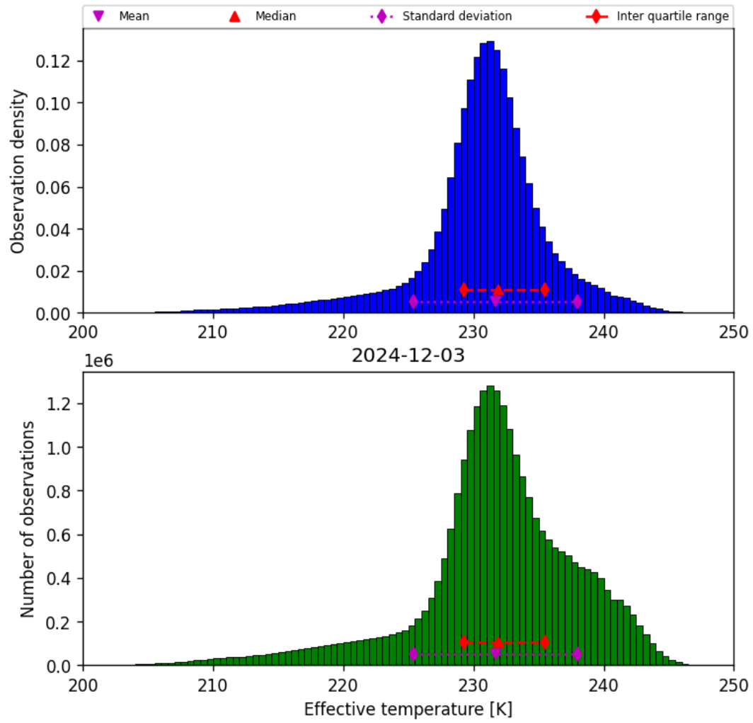
Figure 24: Histogram of “Effective temperature” for 2024-12-02 to 2024-12-04
