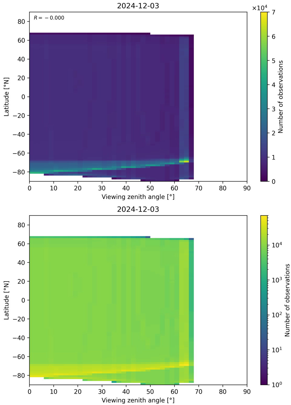
Figure 49: Scatter density plot of “Viewing zenith angle” against “Latitude” for 2024-12-02 to 2024-12-04.
