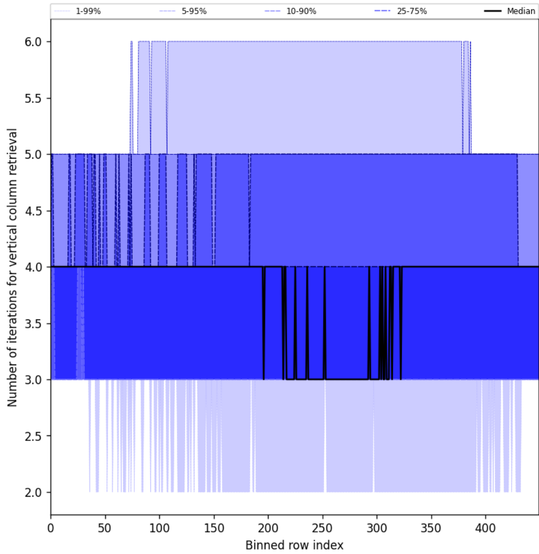
Figure 33: Along track statistics of “Number of iterations for vertical column retrieval” for 2024-12-02 to 2024-12-04
