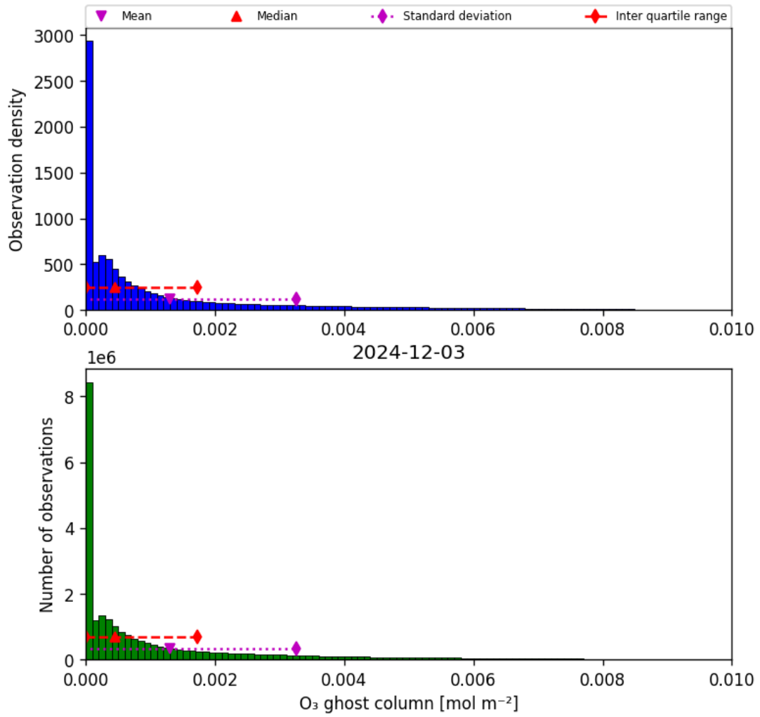
Figure 25: Histogram of “O 3 ghost column” for 2024-12-02 to 2024-12-04
