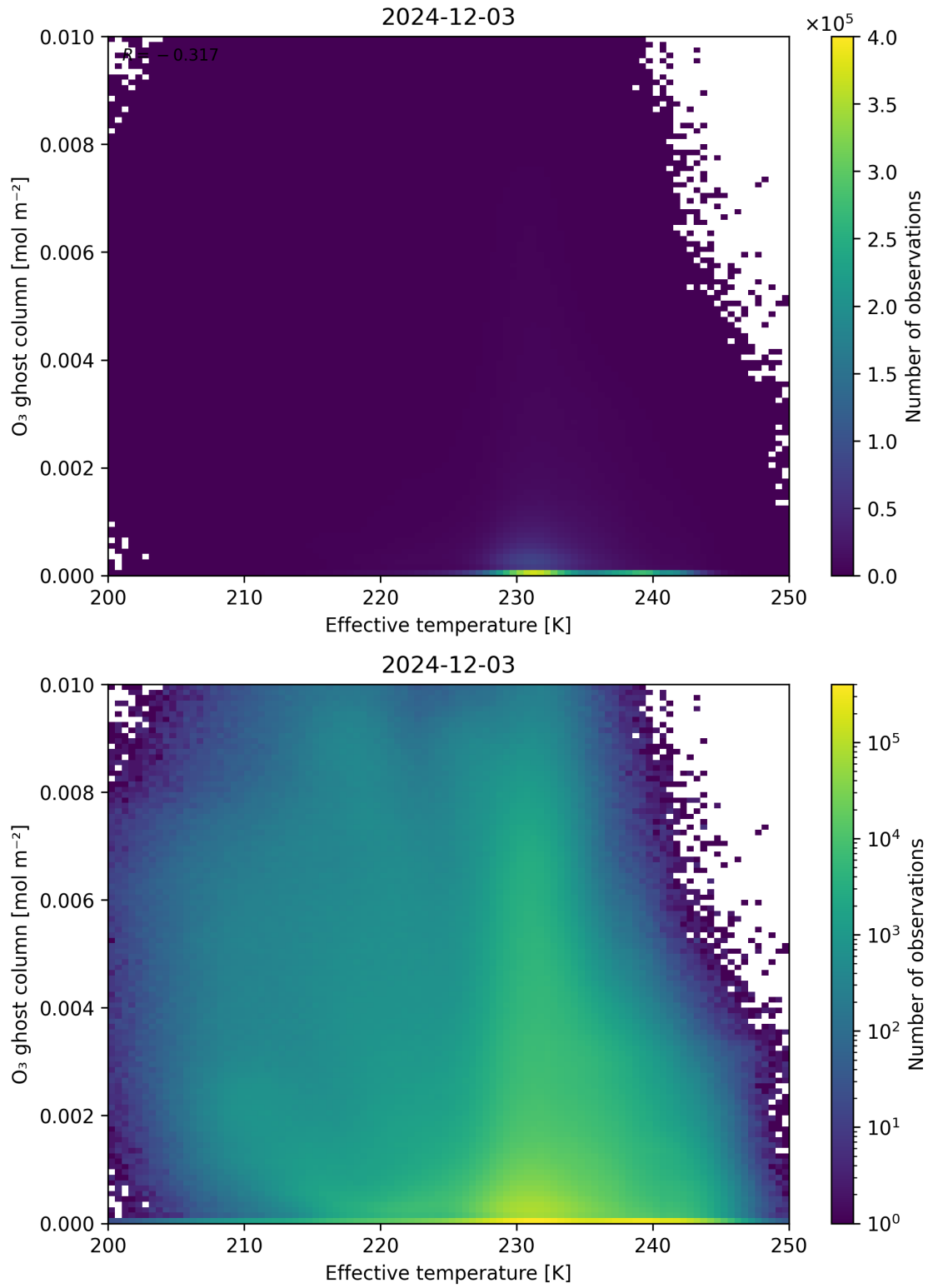
Figure 38: Scatter density plot of “Effective temperature” against “O 3 ghost column” for 2024-12-02 to 2024-12-04.
