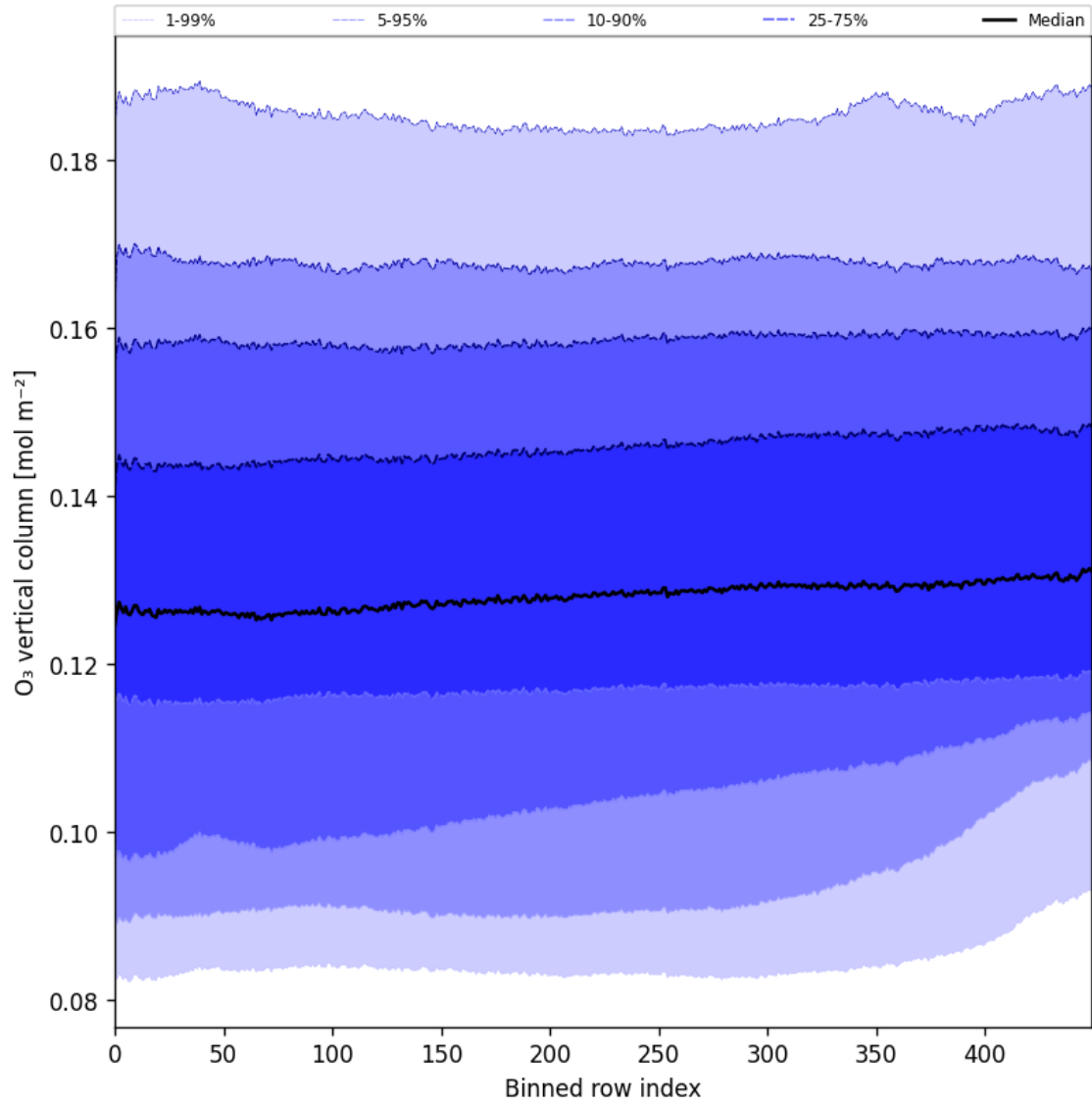
Figure 28: Along track statistics of “O 3 vertical column” for 2024-12-02 to 2024-12-04
