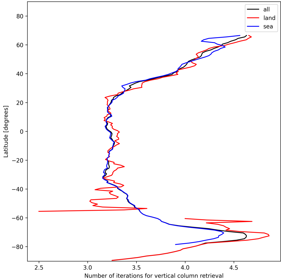
Figure 19: Zonal average of “Number of iterations for vertical column retrieval” for 2024-12-02 to 2024-12-04.
