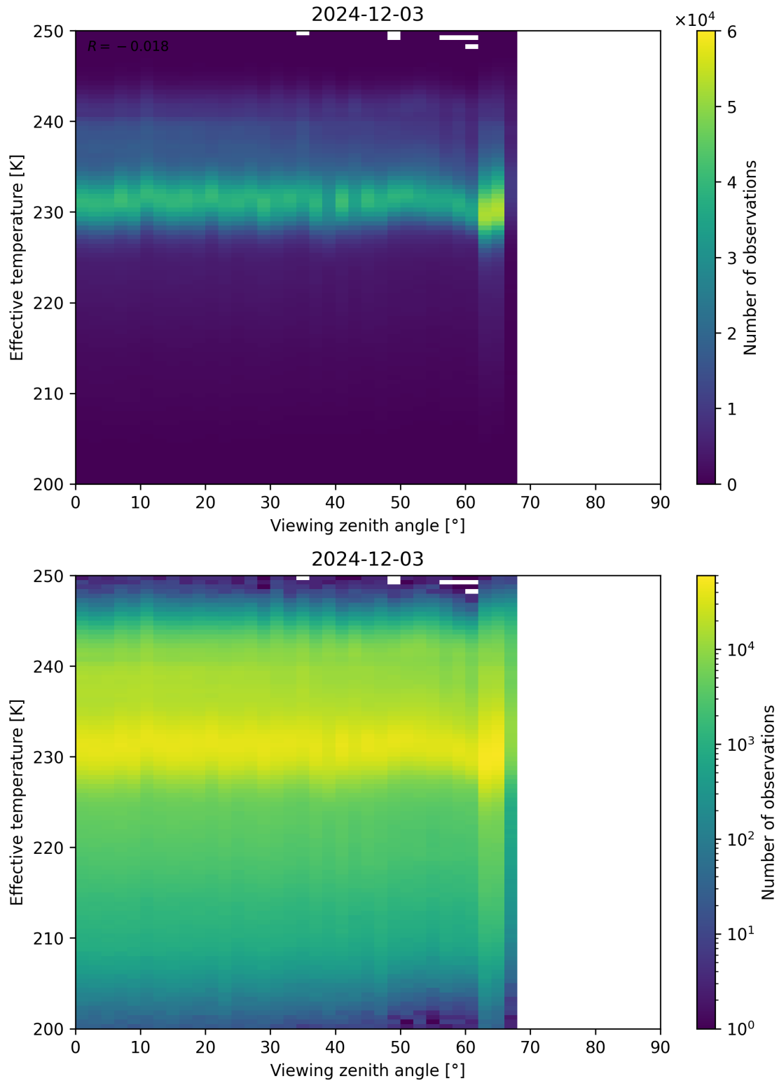
Figure 50: Scatter density plot of “Viewing zenith angle” against “Effective temperature” for 2024-12-02 to 2024-12-04.
