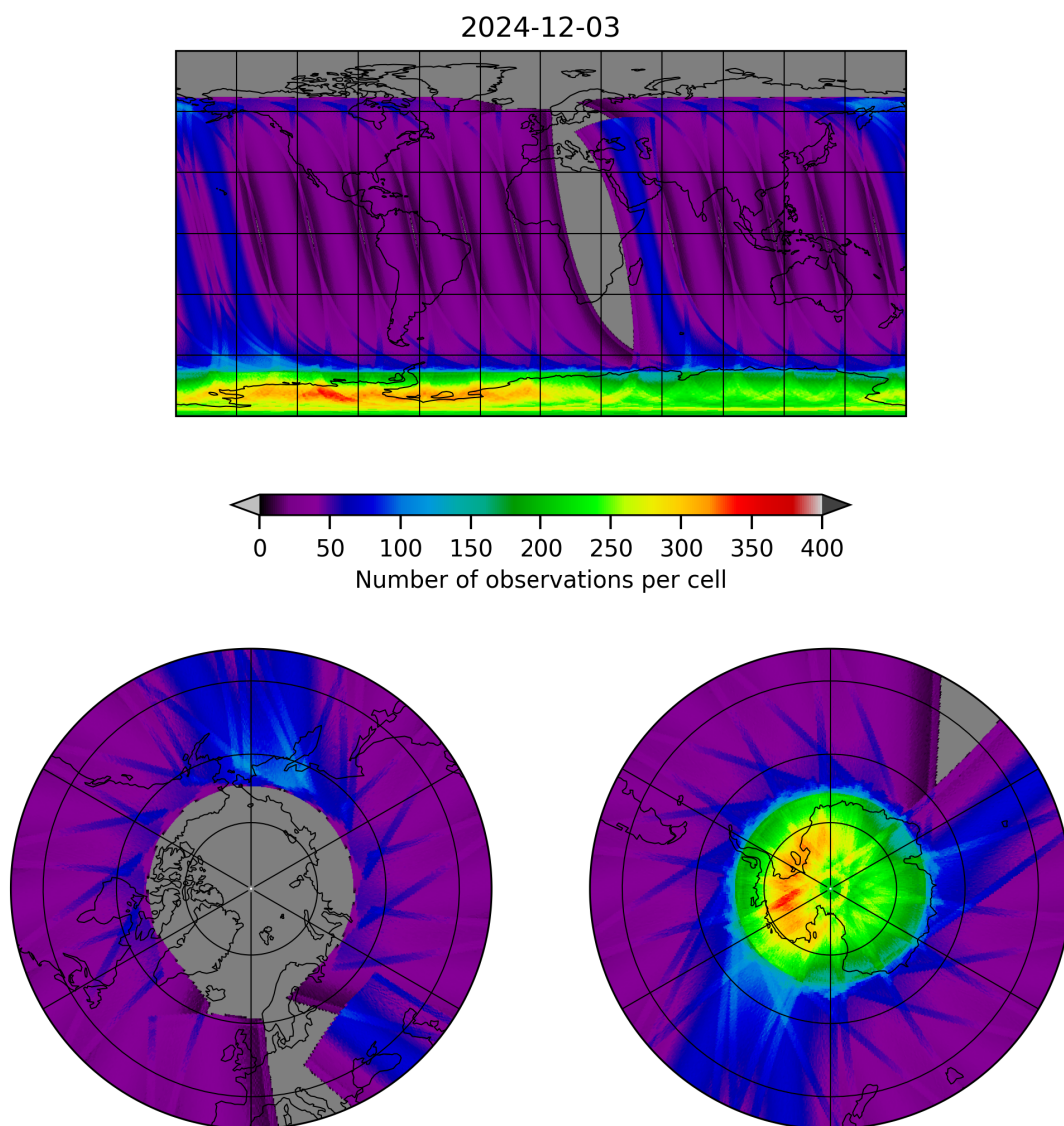
Figure 12: Map of the number of observations for 2024-12-02 to 2024-12-04
