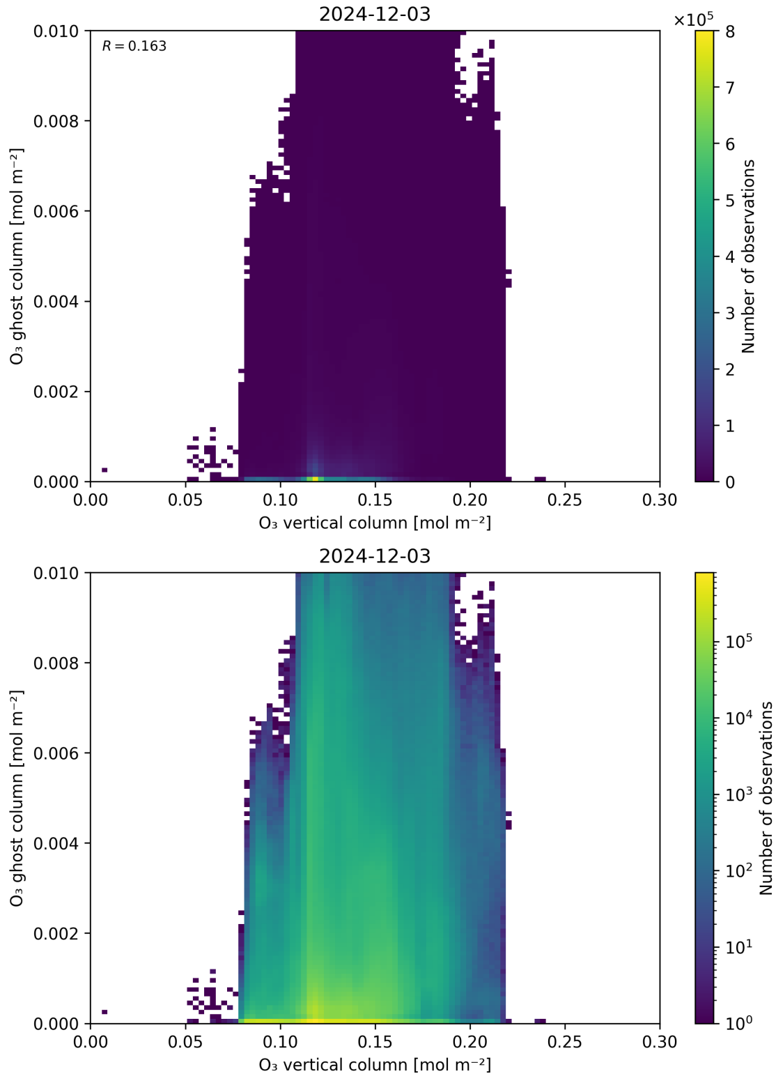
Figure 40: Scatter density plot of “O 3 vertical column” against “O 3 ghost column” for 2024-12-02 to 2024-12-04.
