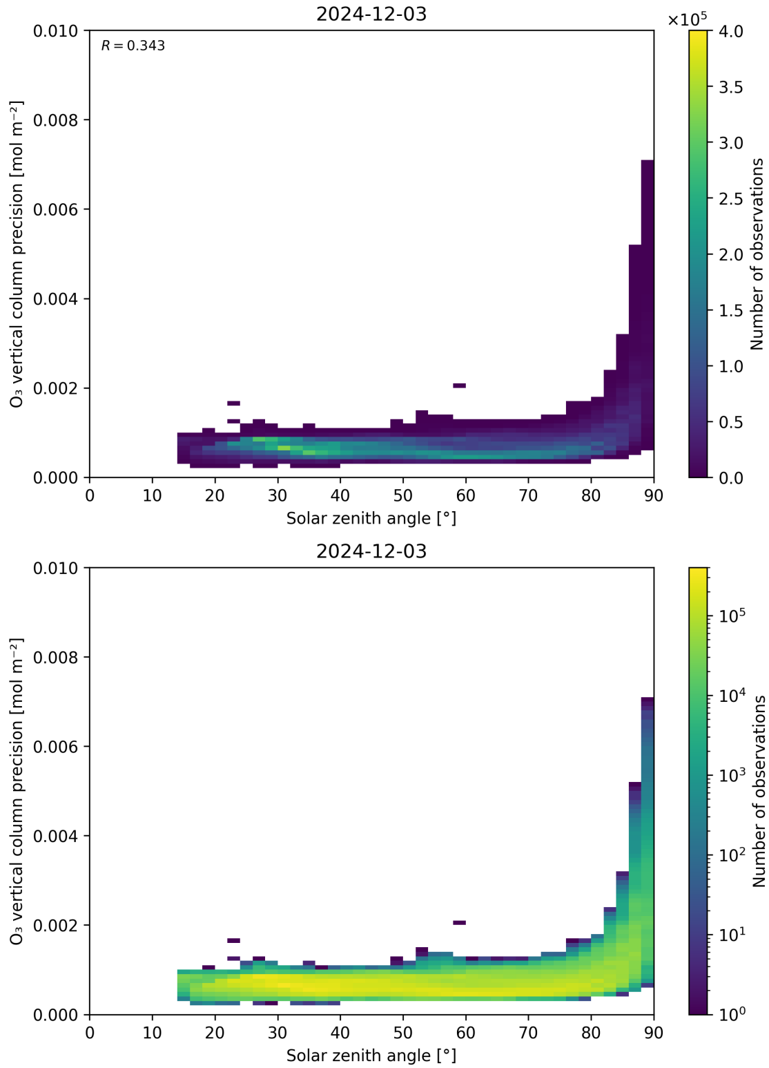
Figure 48: Scatter density plot of “Solar zenith angle” against “O 3 vertical column precision” for 2024-12-02 to 2024-12-04.
