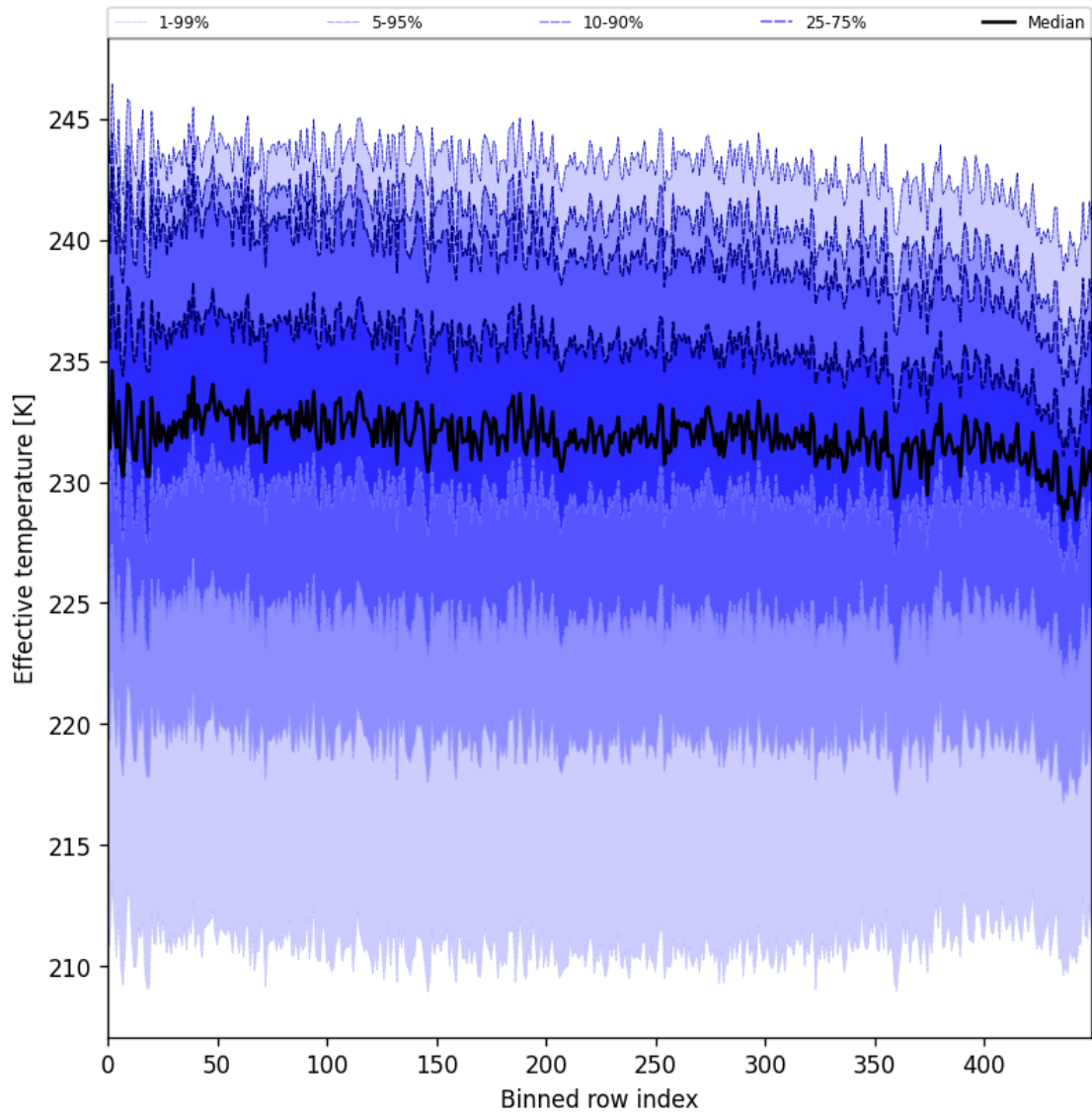
Figure 31: Along track statistics of “Effective temperature” for 2024-12-02 to 2024-12-04
