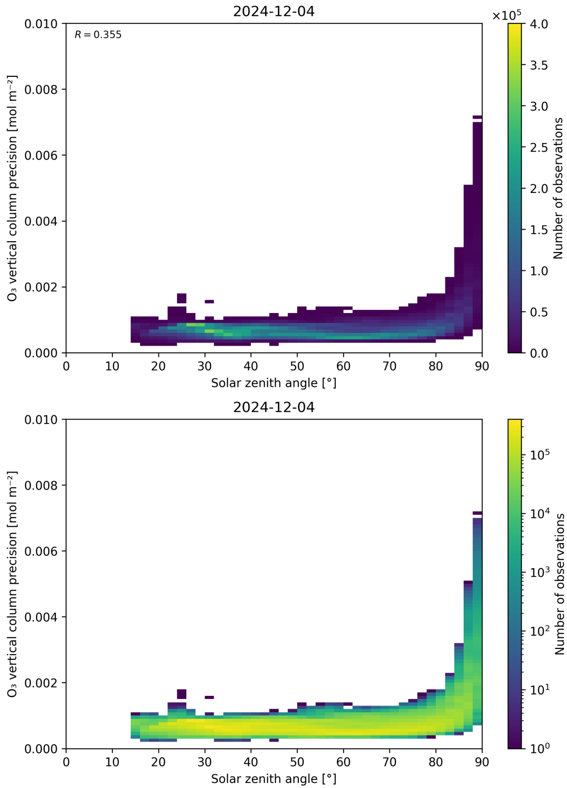
Figure 48: Scatter density plot of “Solar zenith angle” against “O 3 vertical column precision” for 2024-12-03 to 2024-12-05.
