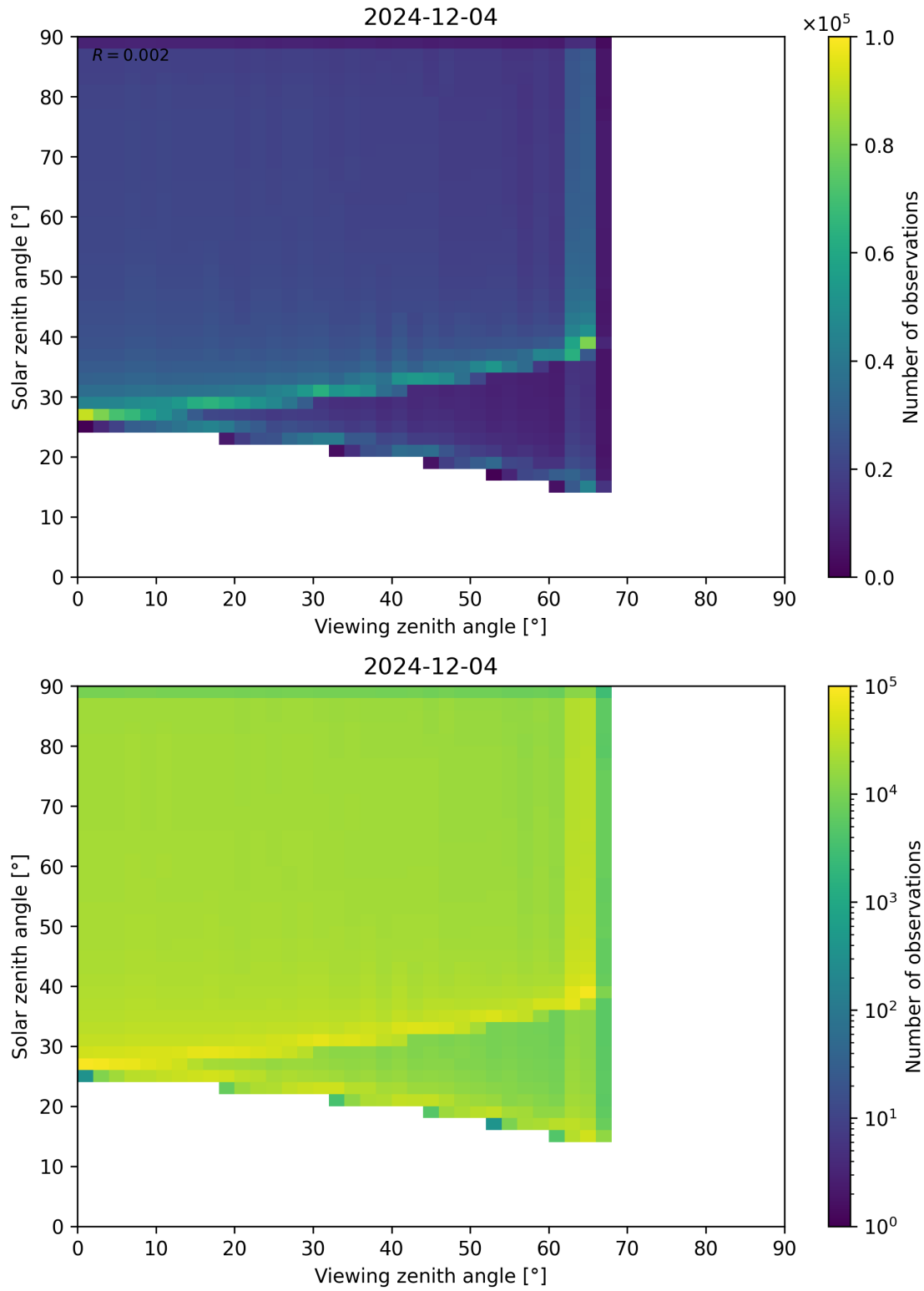
Figure 54: Scatter density plot of “Viewing zenith angle” against “Solar zenith angle” for 2024-12-03 to 2024-12-05.
