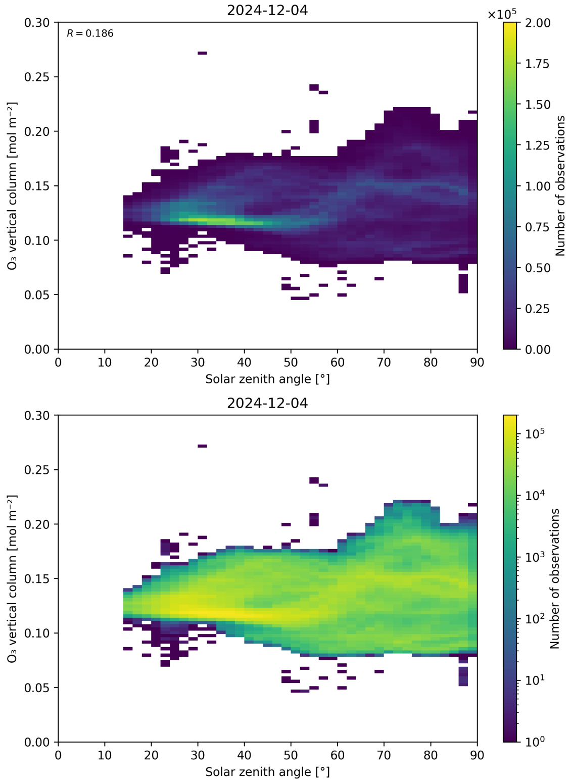
Figure 47: Scatter density plot of “Solar zenith angle” against “O 3 vertical column” for 2024-12-03 to 2024-12-05.
