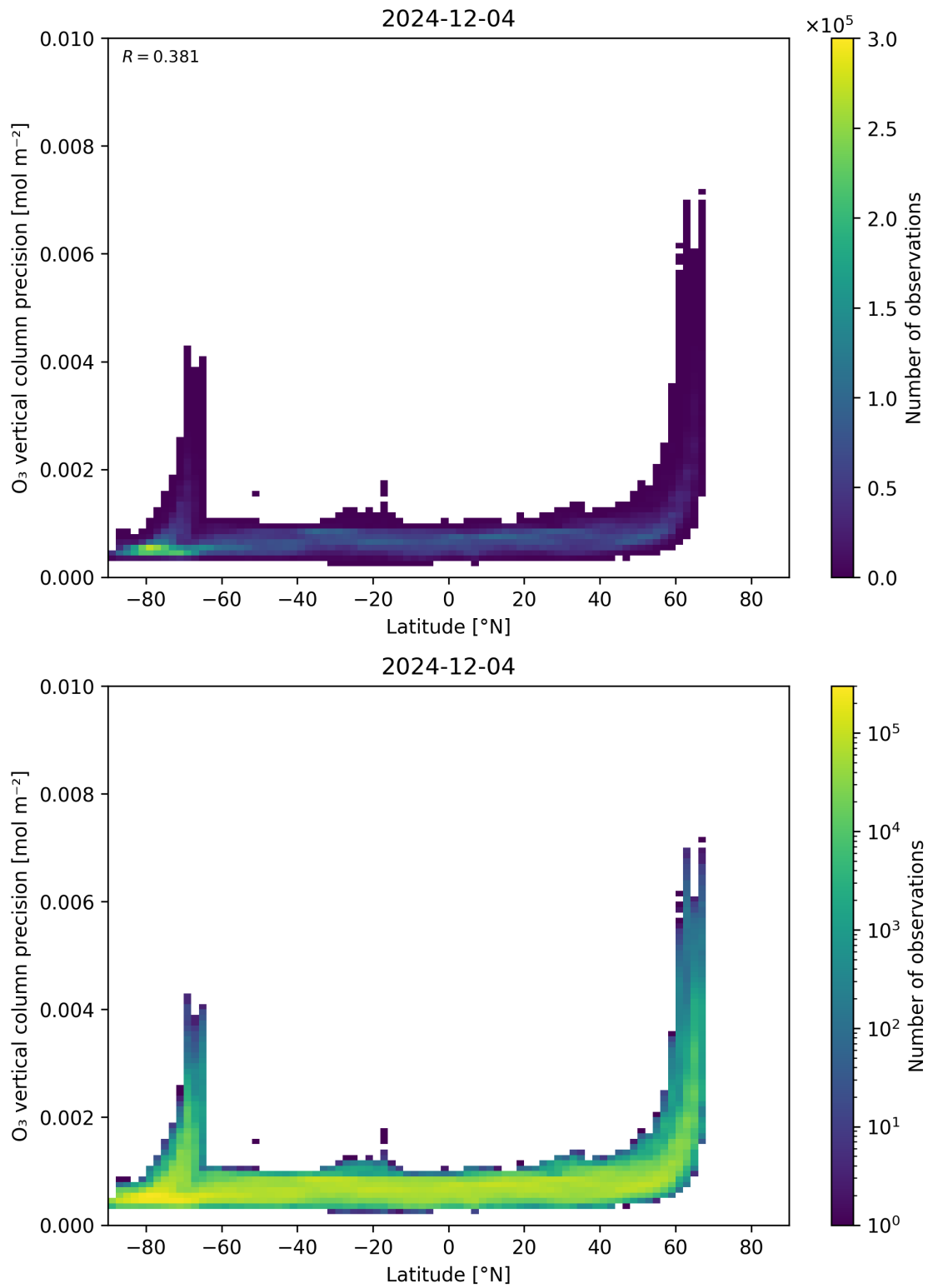
Figure 37: Scatter density plot of “Latitude” against “O 3 vertical column precision” for 2024-12-03 to 2024-12-05.
