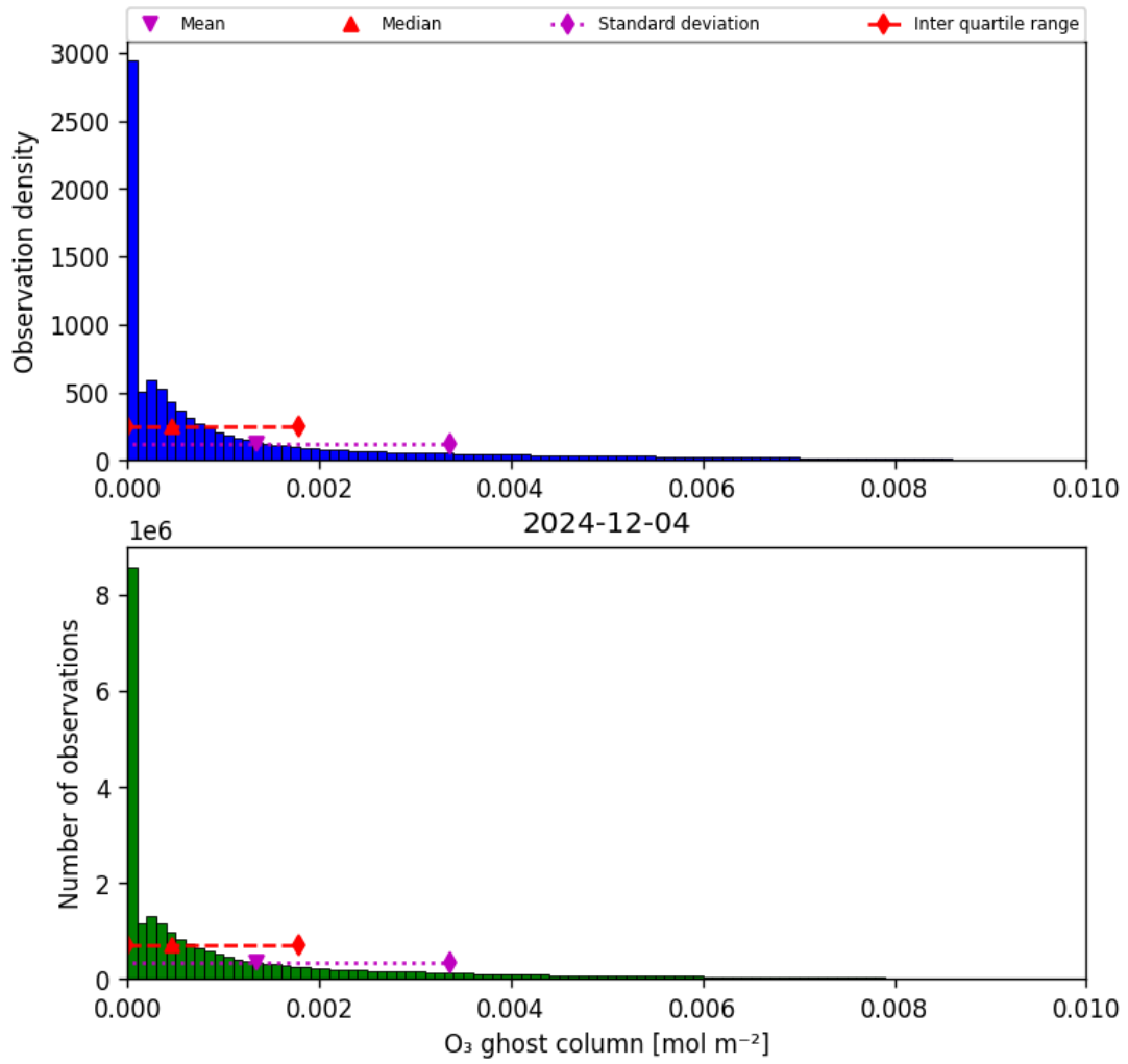
Figure 25: Histogram of “O 3 ghost column” for 2024-12-03 to 2024-12-05
