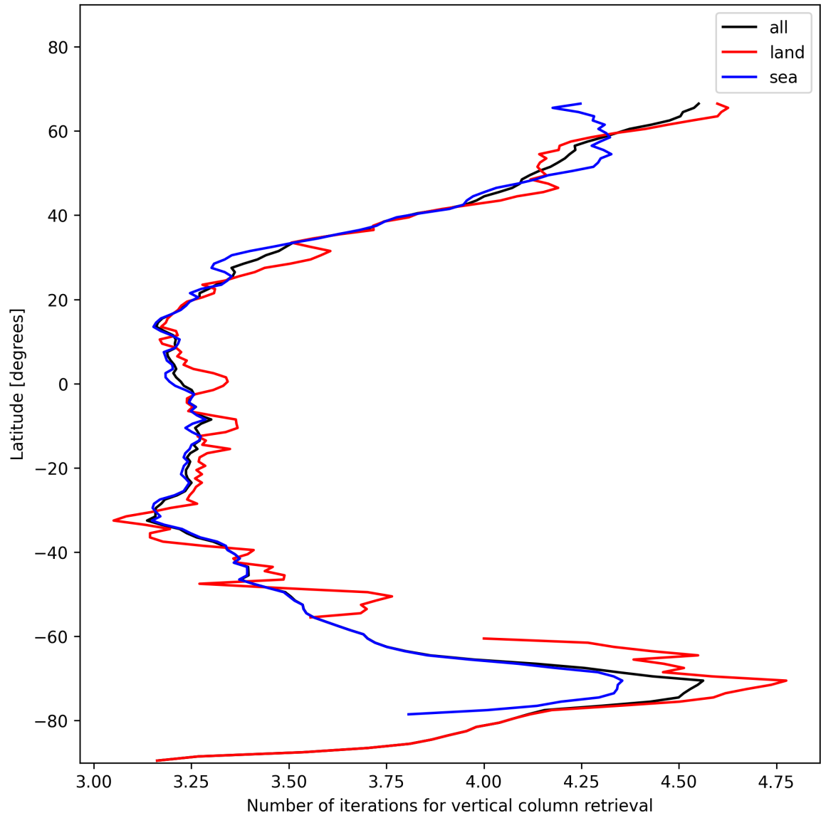
Figure 19: Zonal average of “Number of iterations for vertical column retrieval” for 2024-12-03 to 2024-12-05.
