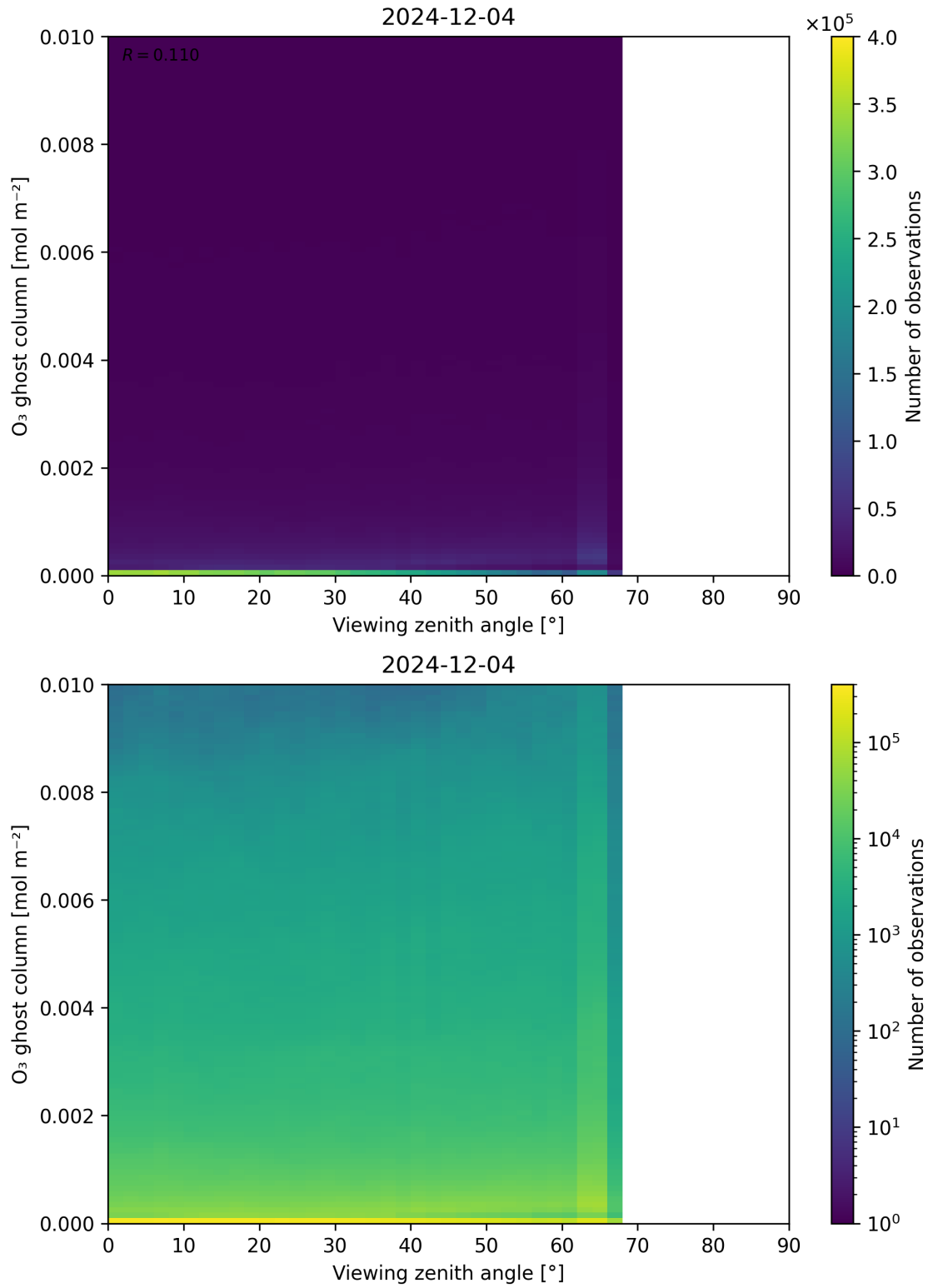
Figure 51: Scatter density plot of “Viewing zenith angle” against “O 3 ghost column” for 2024-12-03 to 2024-12-05.
