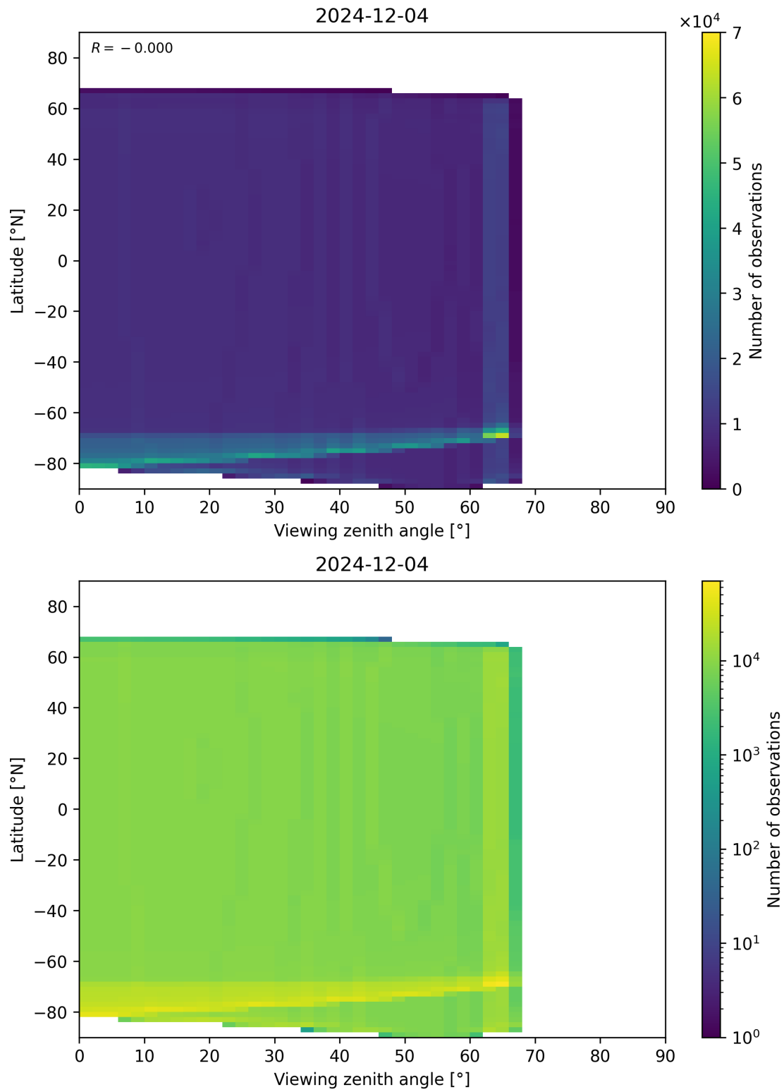
Figure 49: Scatter density plot of “Viewing zenith angle” against “Latitude” for 2024-12-03 to 2024-12-05.
