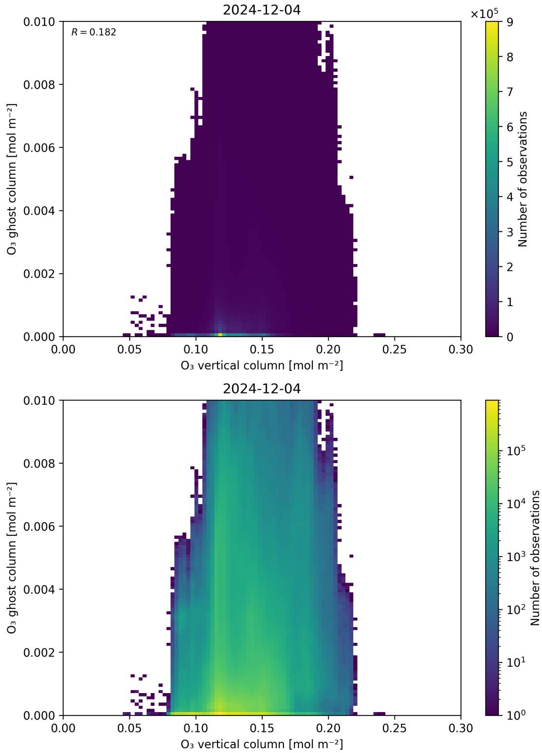
Figure 40: Scatter density plot of “O 3 vertical column” against “O 3 ghost column” for 2024-12-03 to 2024-12-05.
