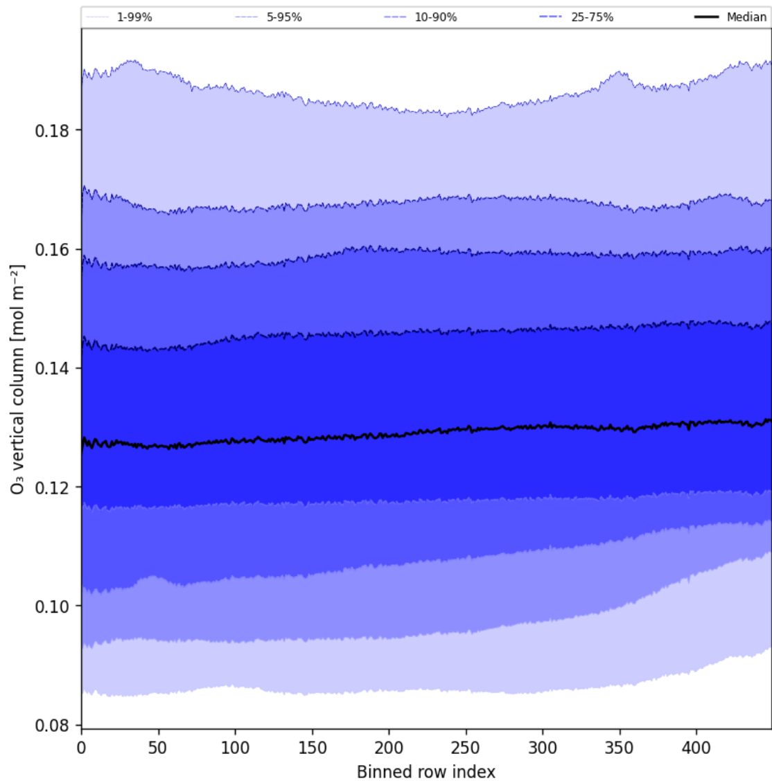
Figure 28: Along track statistics of “O 3 vertical column” for 2024-12-03 to 2024-12-05
