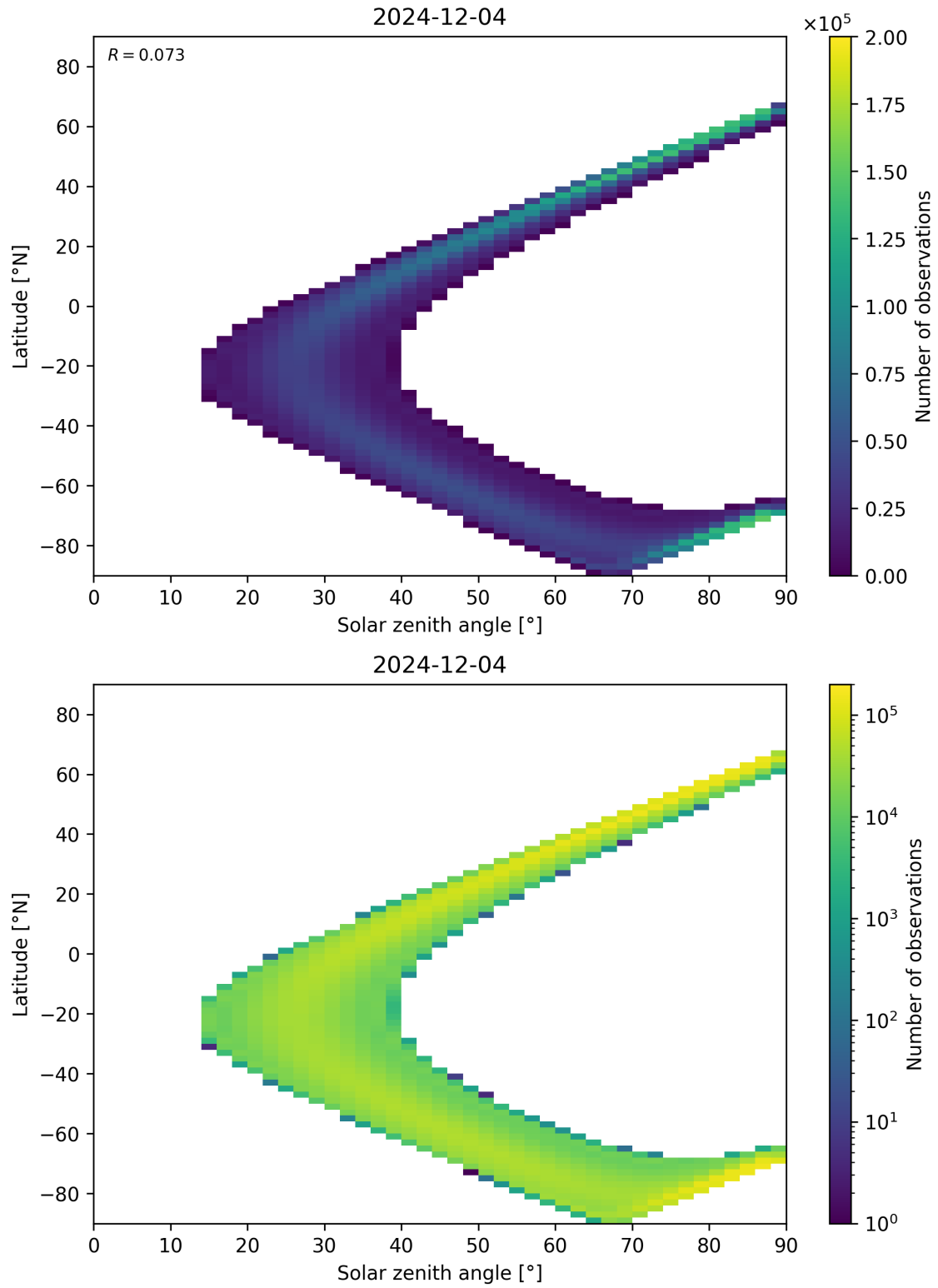
Figure 44: Scatter density plot of “Solar zenith angle” against “Latitude” for 2024-12-03 to 2024-12-05.
