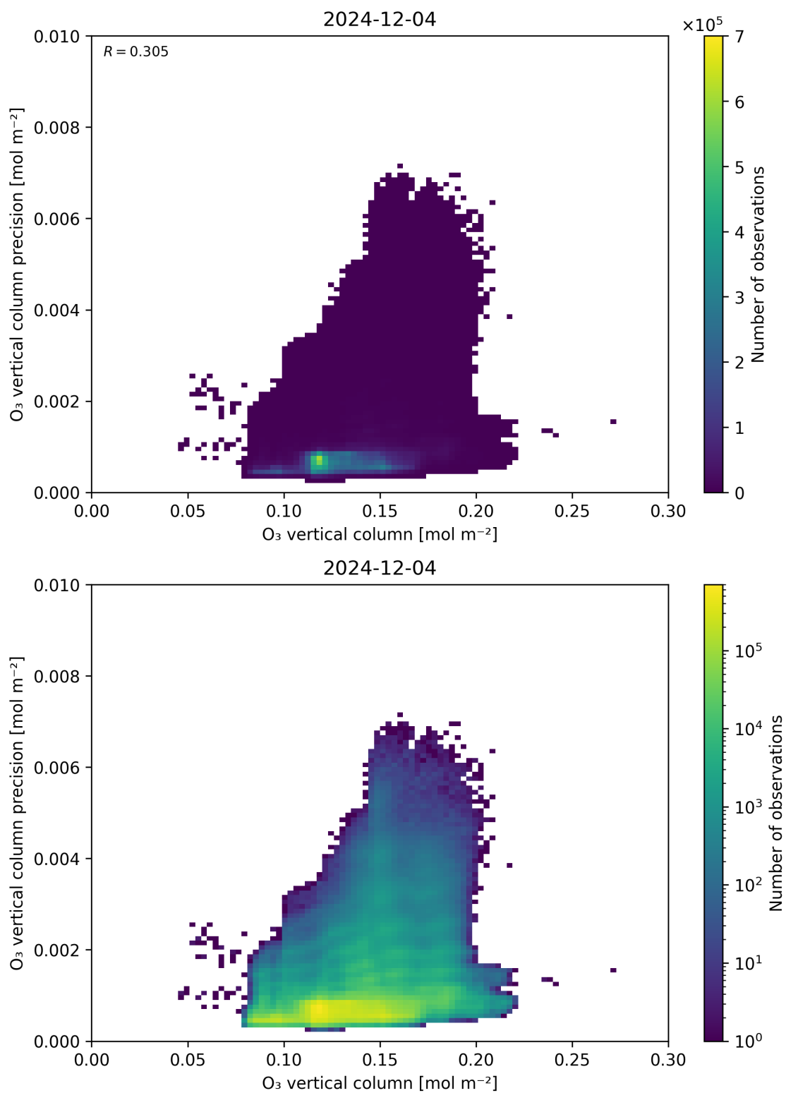
Figure 41: Scatter density plot of “O 3 vertical column” against “O 3 vertical column precision” for 2024-12-03 to 2024-12-05.
