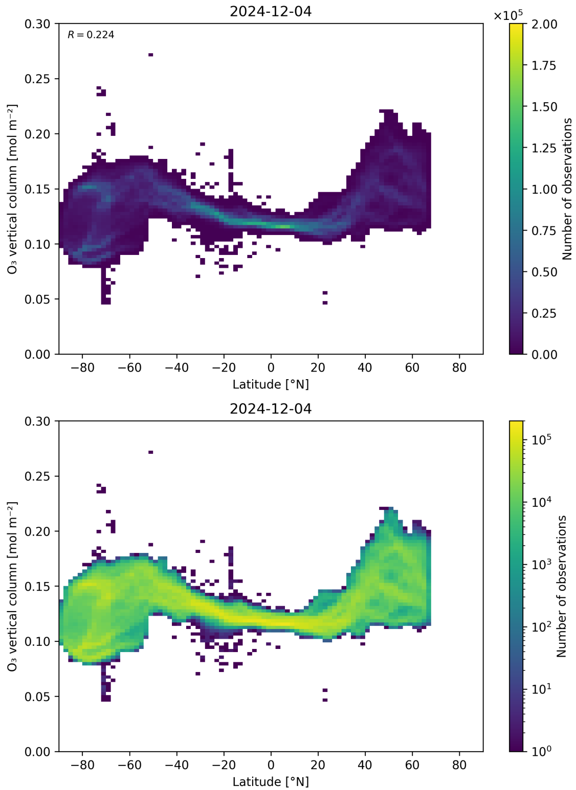
Figure 36: Scatter density plot of “Latitude” against “O 3 vertical column” for 2024-12-03 to 2024-12-05.
