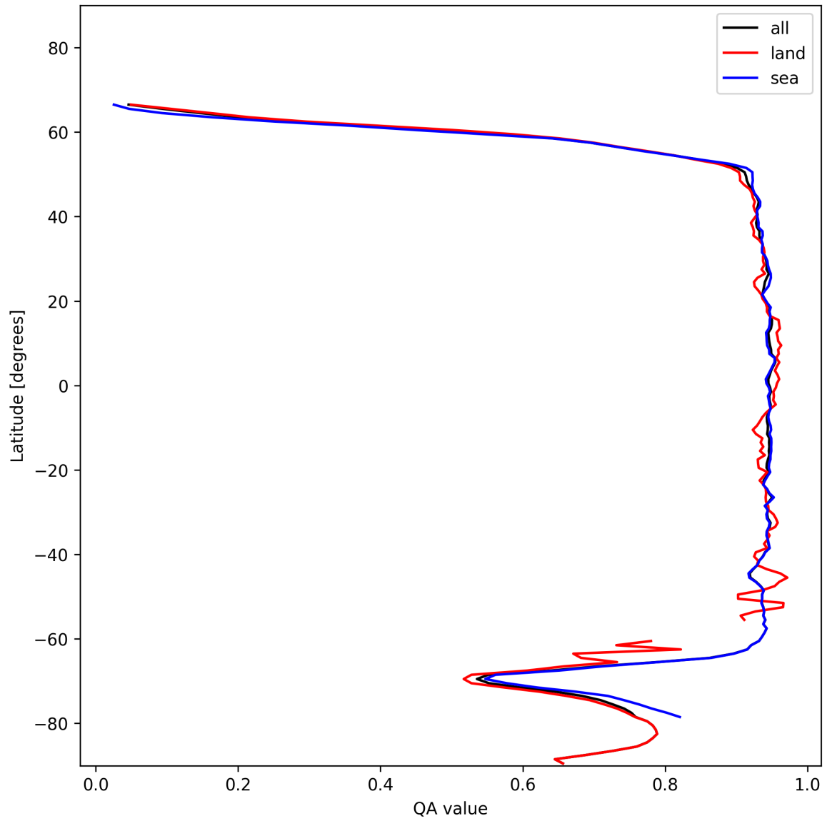
Figure 13: Zonal average of “QA value” for 2024-12-03 to 2024-12-05.
