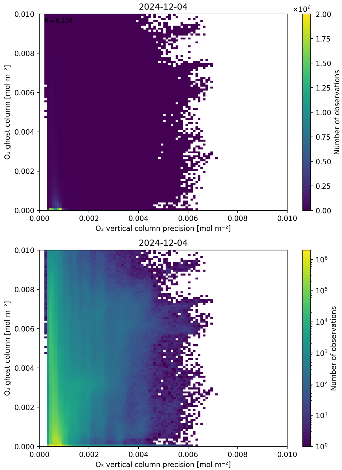
Figure 43: Scatter density plot of “ \text{O}_3 vertical column precision” against “ \text{O}_3 ghost column” for 2024-12-03 to 2024-12-05.
