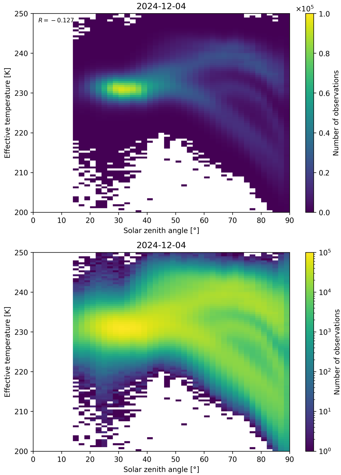
Figure 45: Scatter density plot of “Solar zenith angle” against “Effective temperature” for 2024-12-03 to 2024-12-05.
