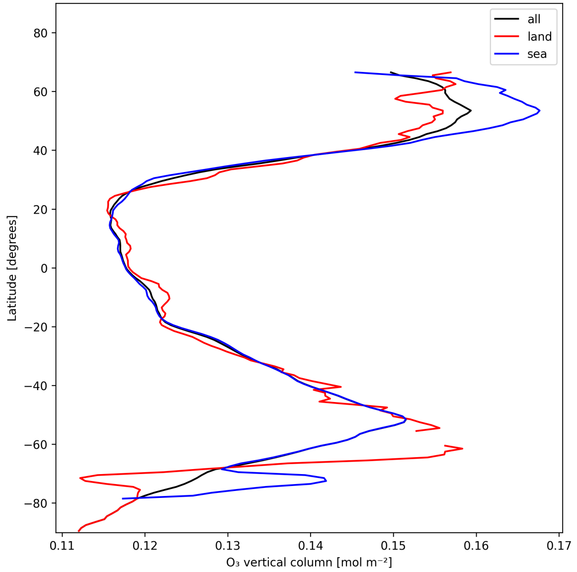
Figure 14: Zonal average of “O 3 vertical column” for 2024-12-03 to 2024-12-05.
