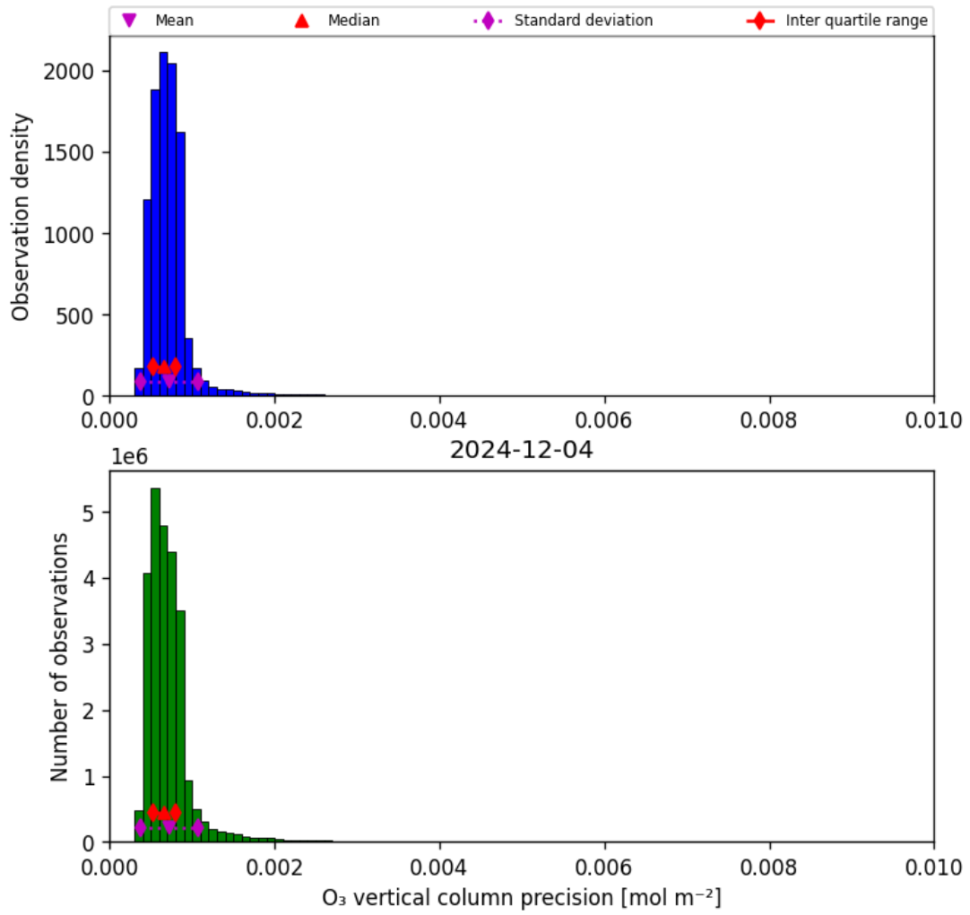
Figure 22: Histogram of “O 3 vertical column precision” for 2024-12-03 to 2024-12-05
