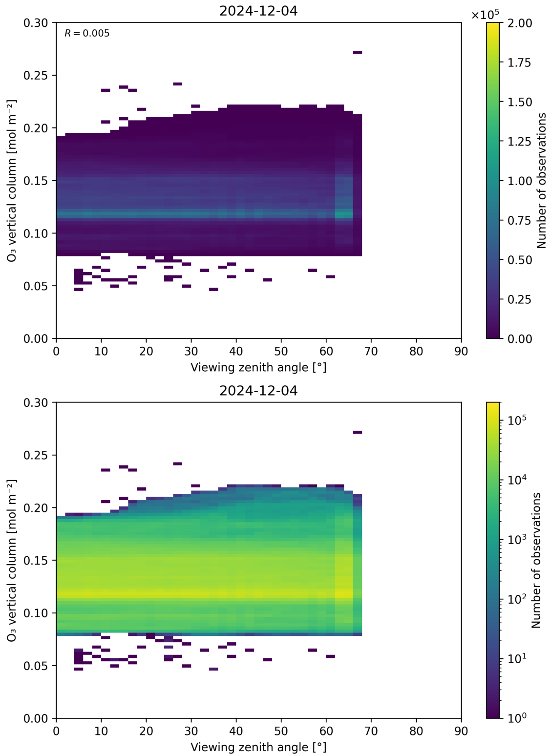
Figure 52: Scatter density plot of “Viewing zenith angle” against “O 3 vertical column” for 2024-12-03 to 2024-12-05.
