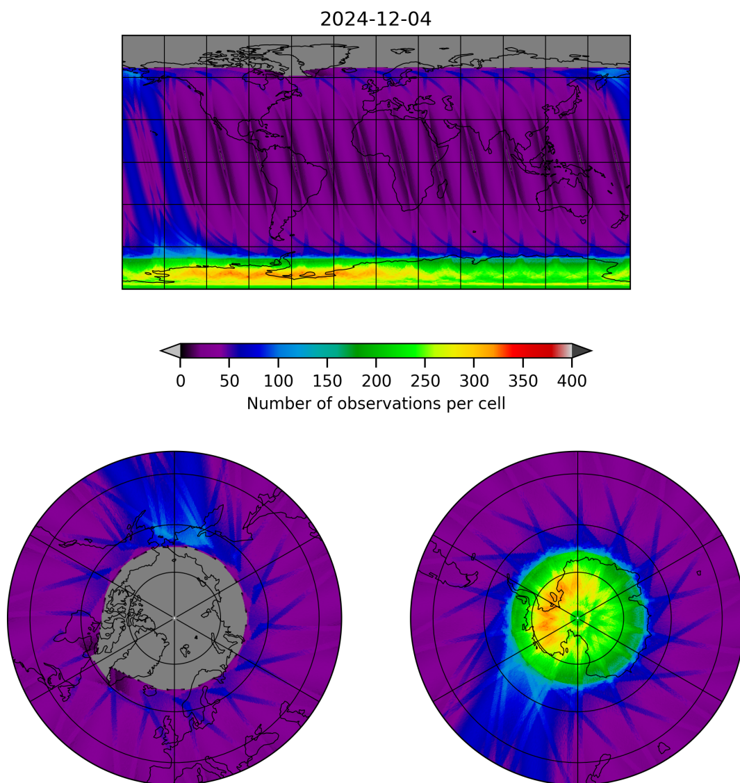
Figure 12: Map of the number of observations for 2024-12-03 to 2024-12-05
