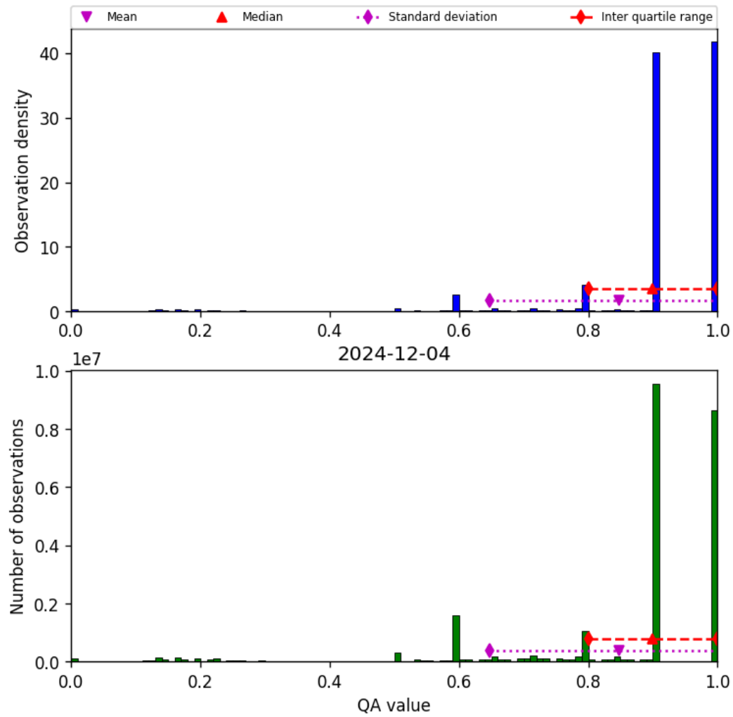
Figure 20: Histogram of “QA value” for 2024-12-03 to 2024-12-05
