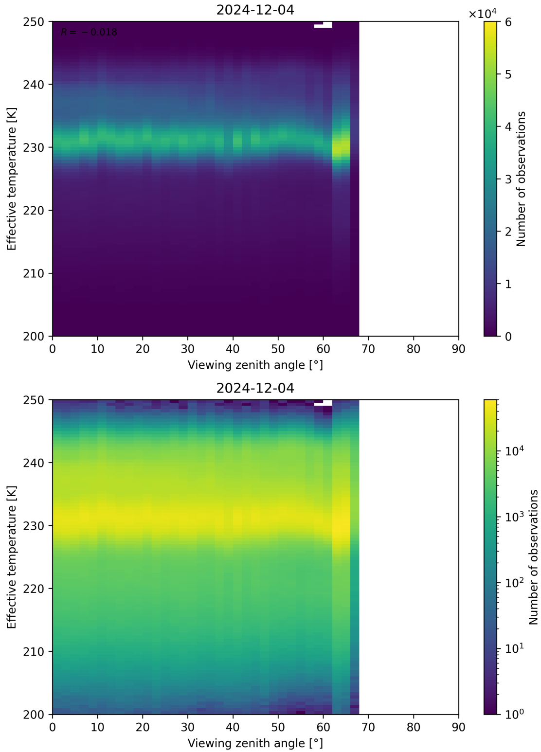
Figure 50: Scatter density plot of “Viewing zenith angle” against “Effective temperature” for 2024-12-03 to 2024-12-05.
