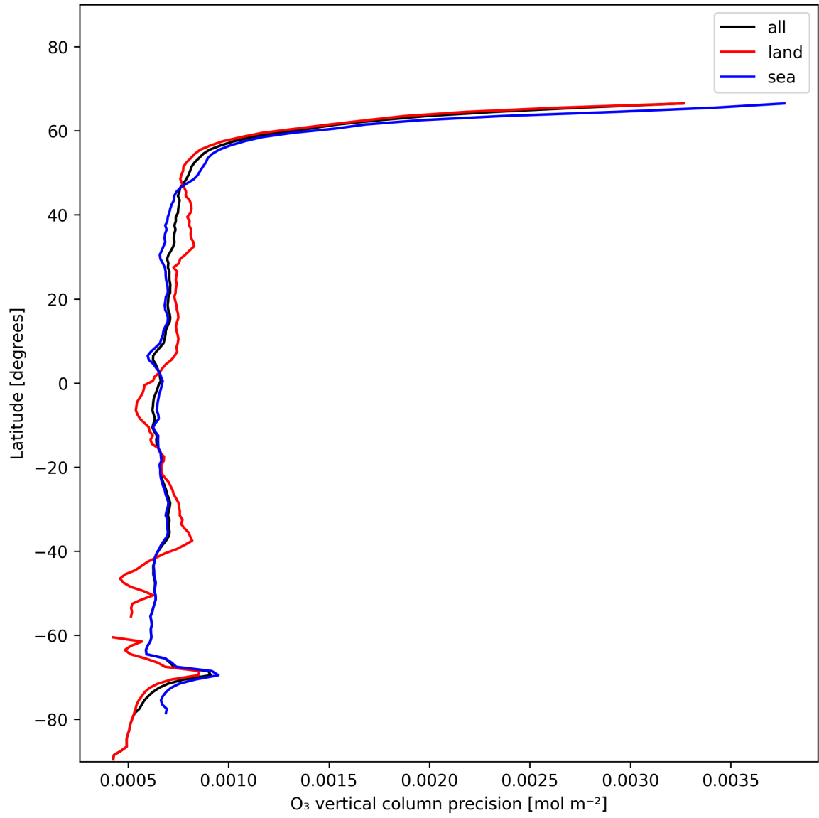
Figure 15: Zonal average of “O 3 vertical column precision” for 2024-12-03 to 2024-12-05.
