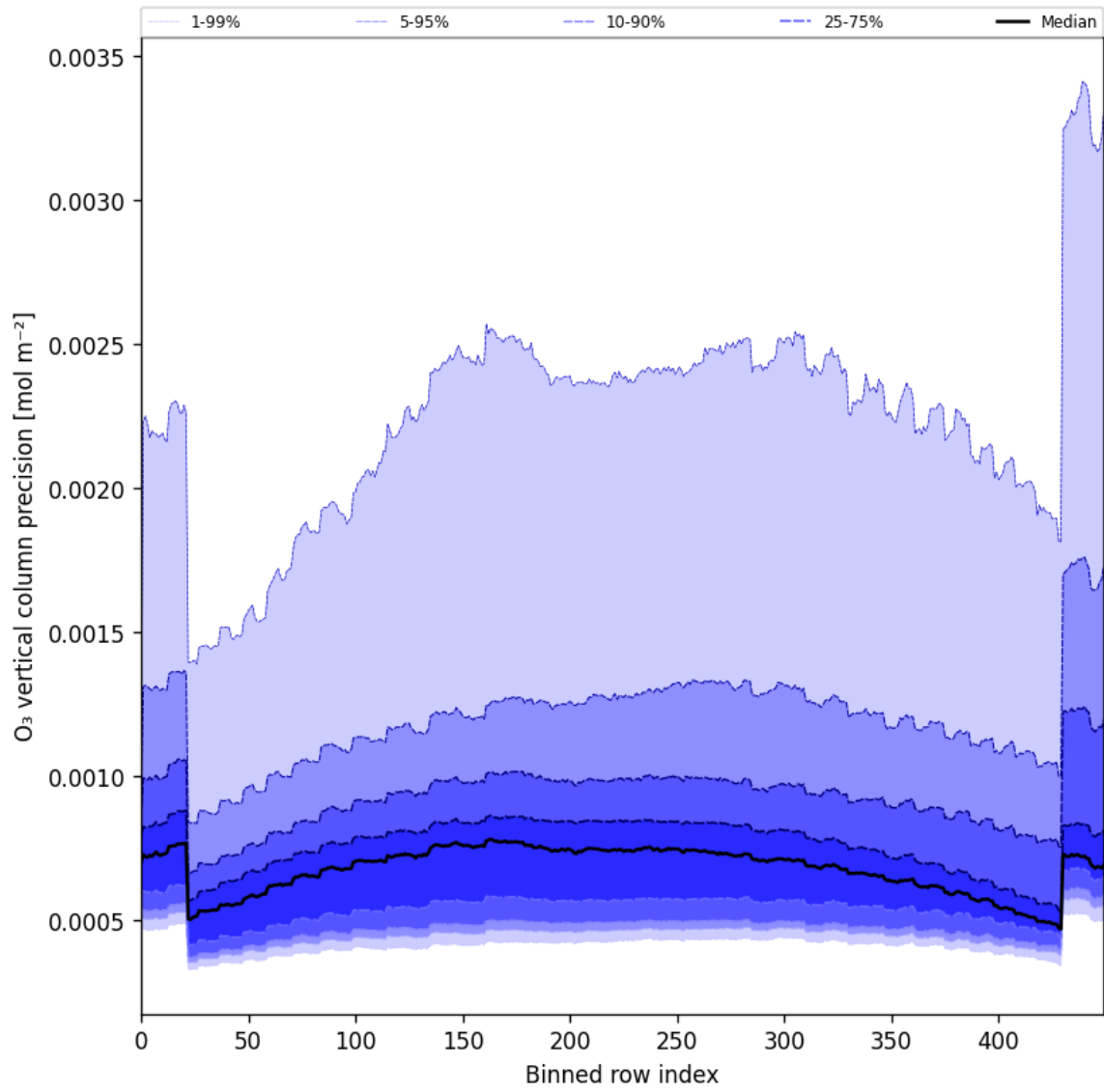
Figure 29: Along track statistics of “O 3 vertical column precision” for 2024-12-03 to 2024-12-05
