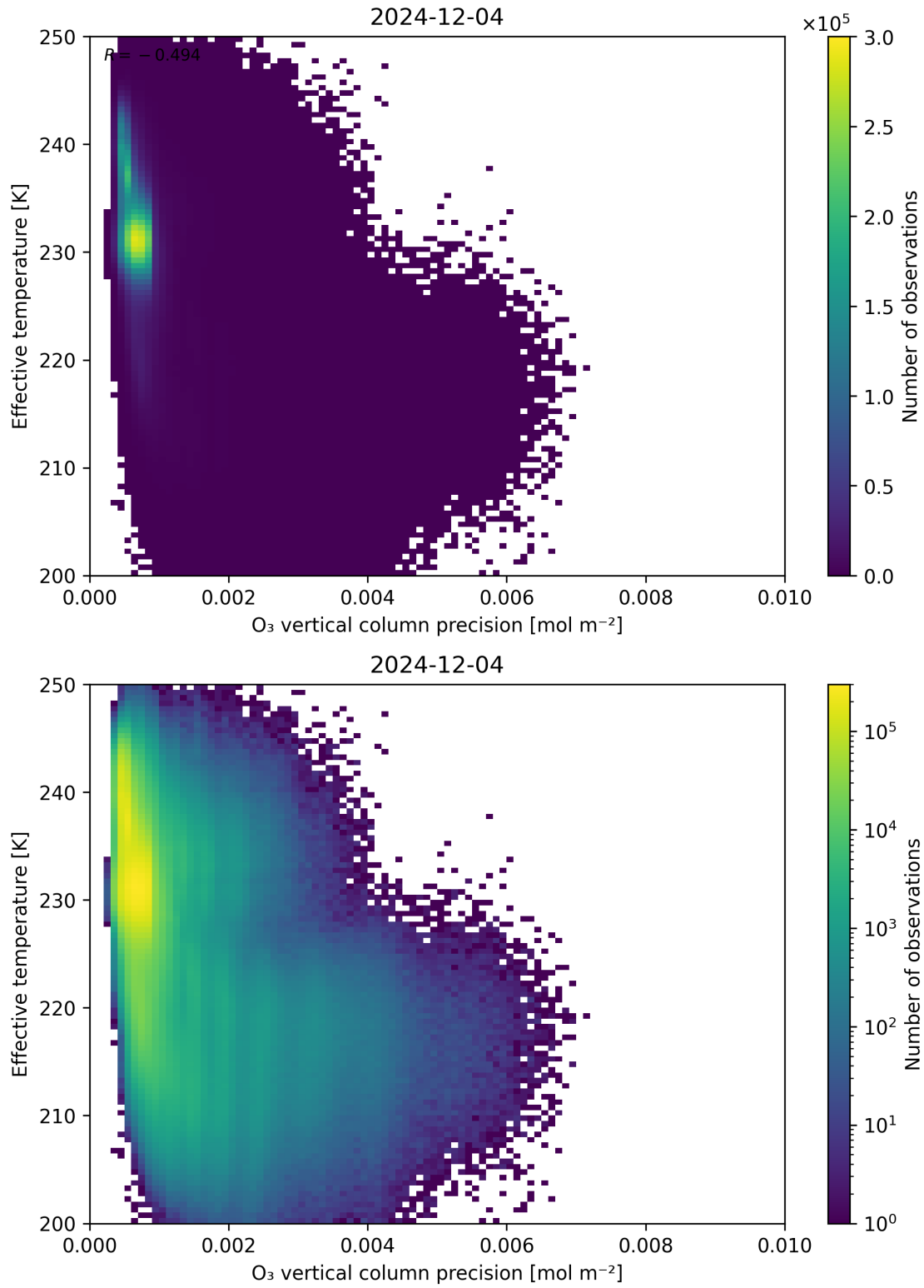
Figure 42: Scatter density plot of “O 3 vertical column precision” against “Effective temperature” for 2024-12-03 to 2024-12-05.
