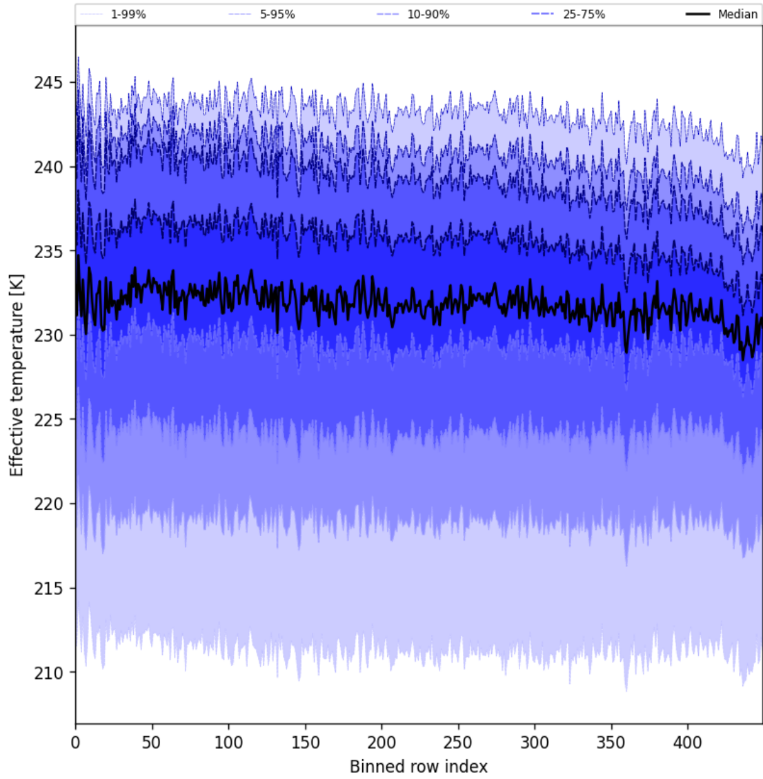
Figure 31: Along track statistics of “Effective temperature” for 2024-12-03 to 2024-12-05
