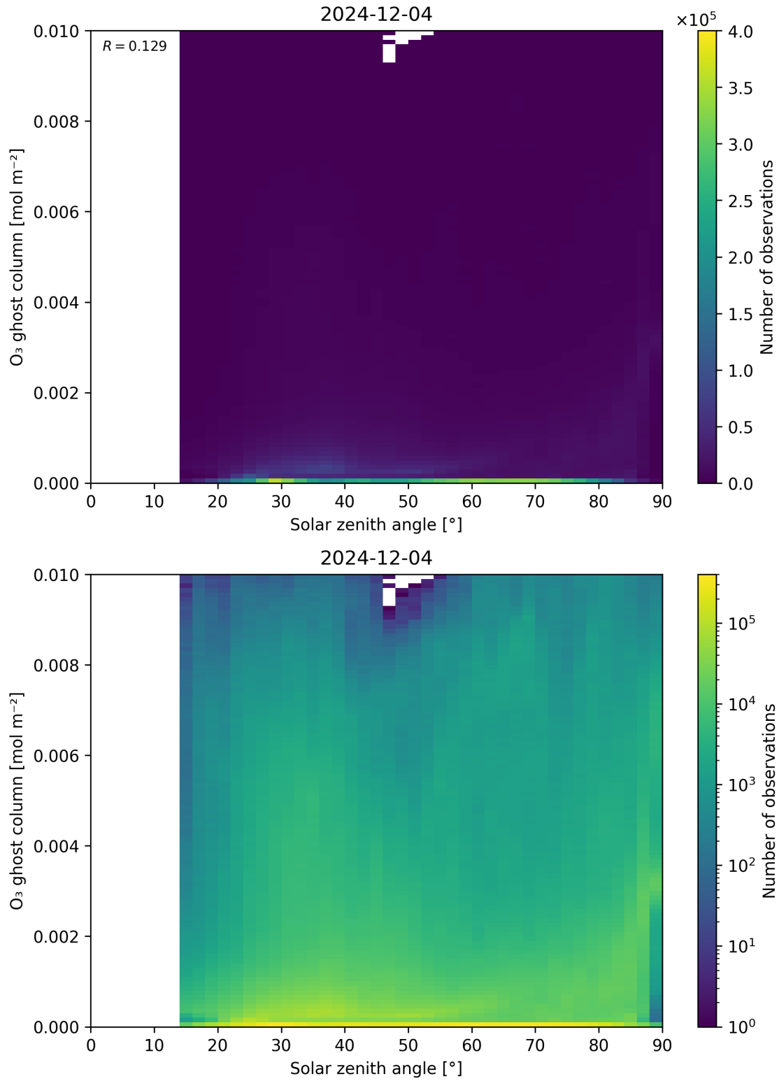
Figure 46: Scatter density plot of “Solar zenith angle” against “O 3 ghost column” for 2024-12-03 to 2024-12-05.
