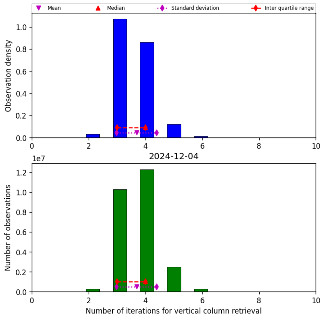
Figure 26: Histogram of “Number of iterations for vertical column retrieval” for 2024-12-03 to 2024-12-05
