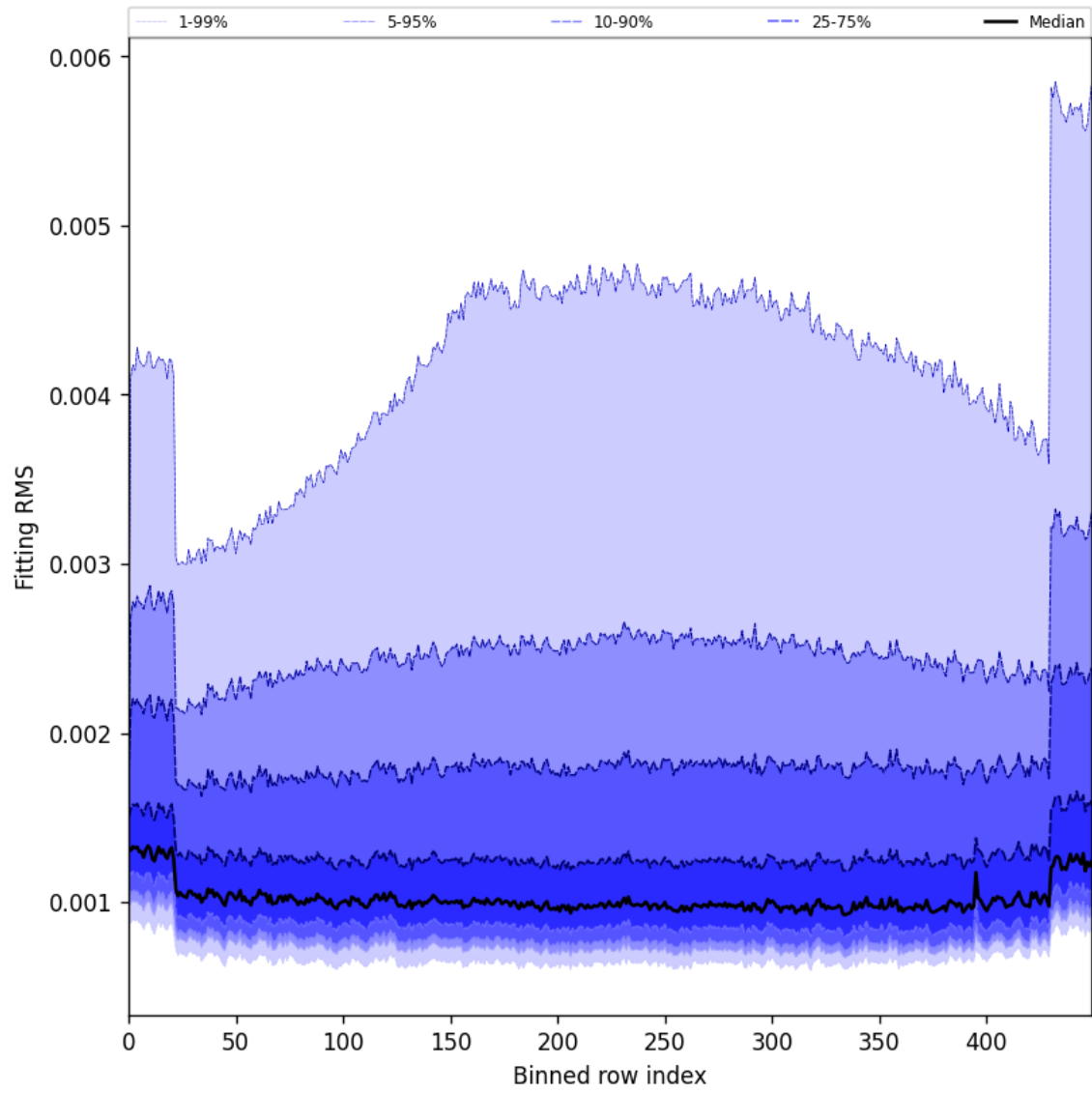
Figure 30: Along track statistics of “Fitting RMS” for 2024-12-03 to 2024-12-05
