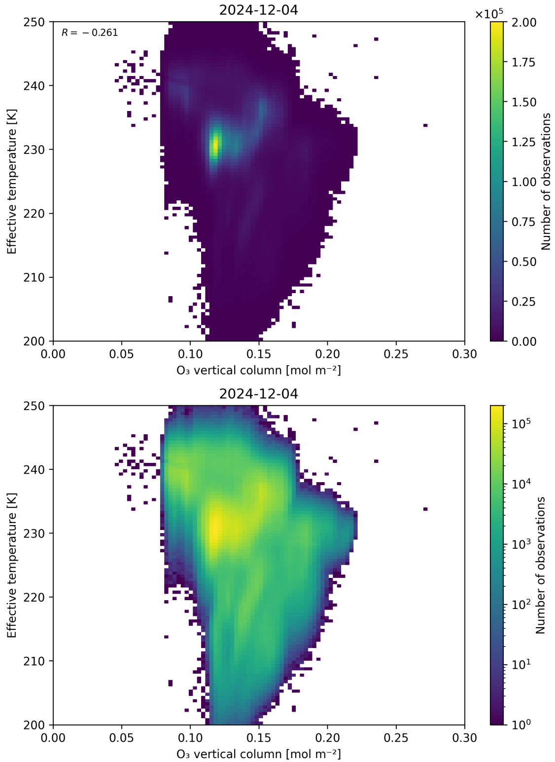
Figure 39: Scatter density plot of “O 3 vertical column” against “Effective temperature” for 2024-12-03 to 2024-12-05.
