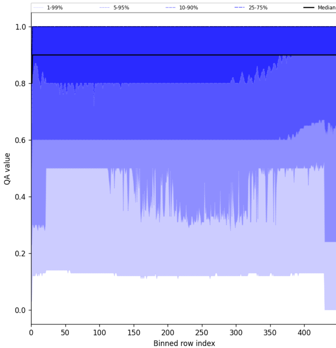
Figure 27: Along track statistics of “QA value” for 2024-12-03 to 2024-12-05
