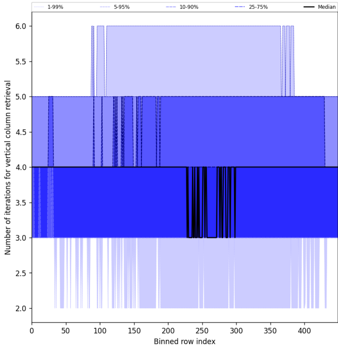
Figure 33: Along track statistics of “Number of iterations for vertical column retrieval” for 2024-12-03 to 2024-12-05
