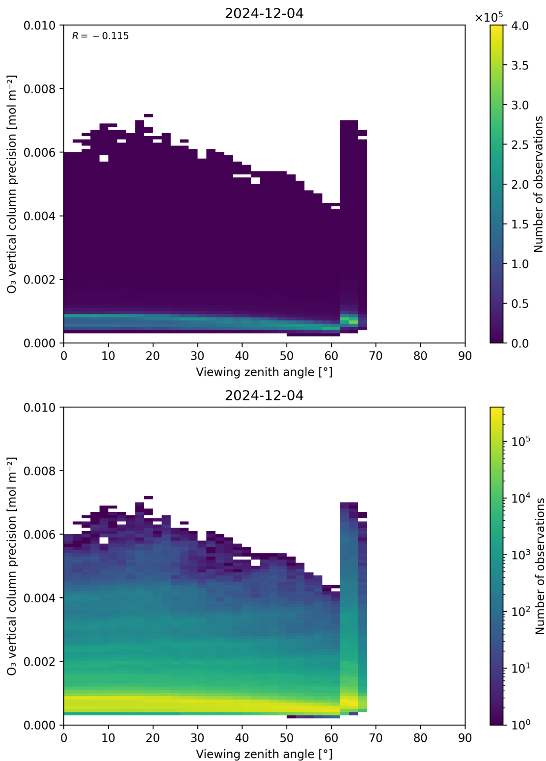
Figure 53: Scatter density plot of “Viewing zenith angle” against “O 3 vertical column precision” for 2024-12-03 to 2024-12-05.
