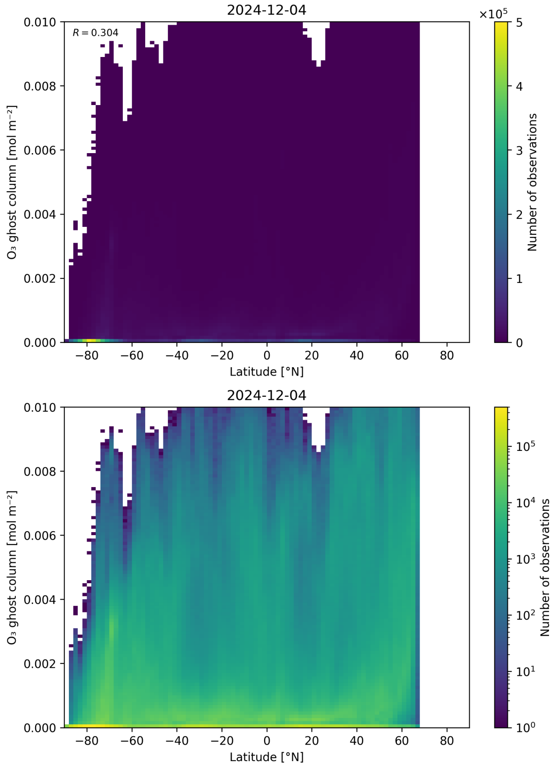
Figure 35: Scatter density plot of “Latitude” against “O 3 ghost column” for 2024-12-03 to 2024-12-05.
