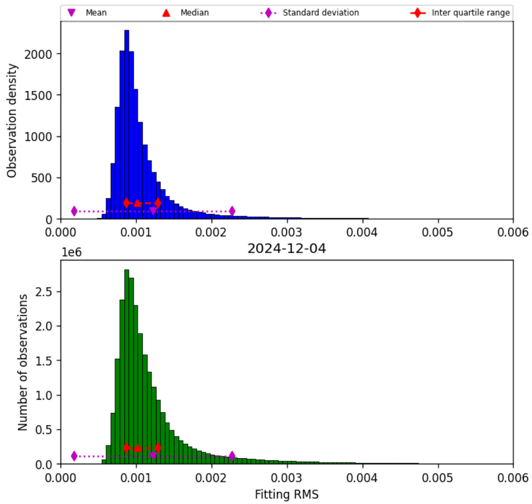
Figure 23: Histogram of “Fitting RMS” for 2024-12-03 to 2024-12-05
