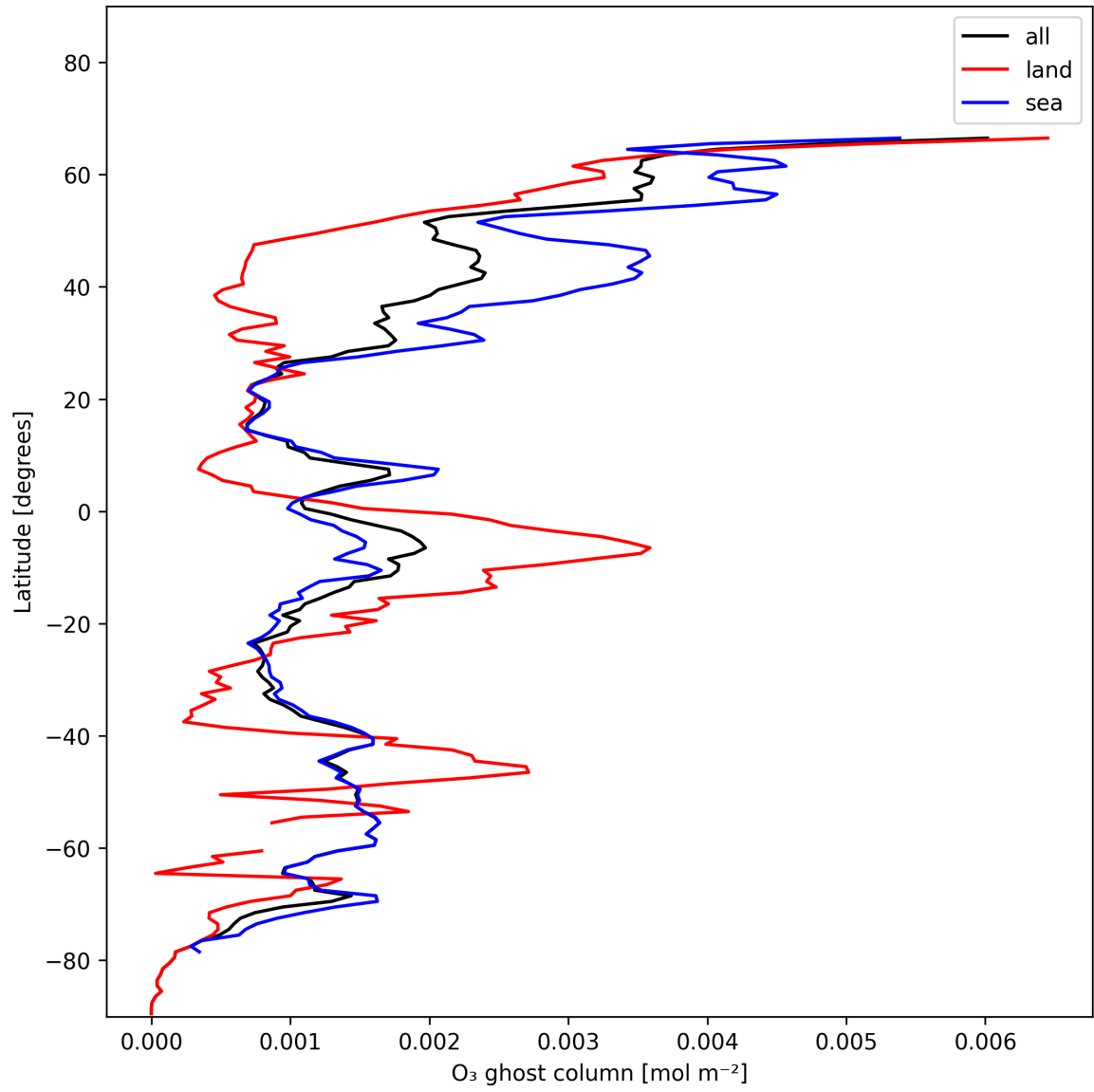
Figure 18: Zonal average of “O 3 ghost column” for 2024-12-03 to 2024-12-05.
