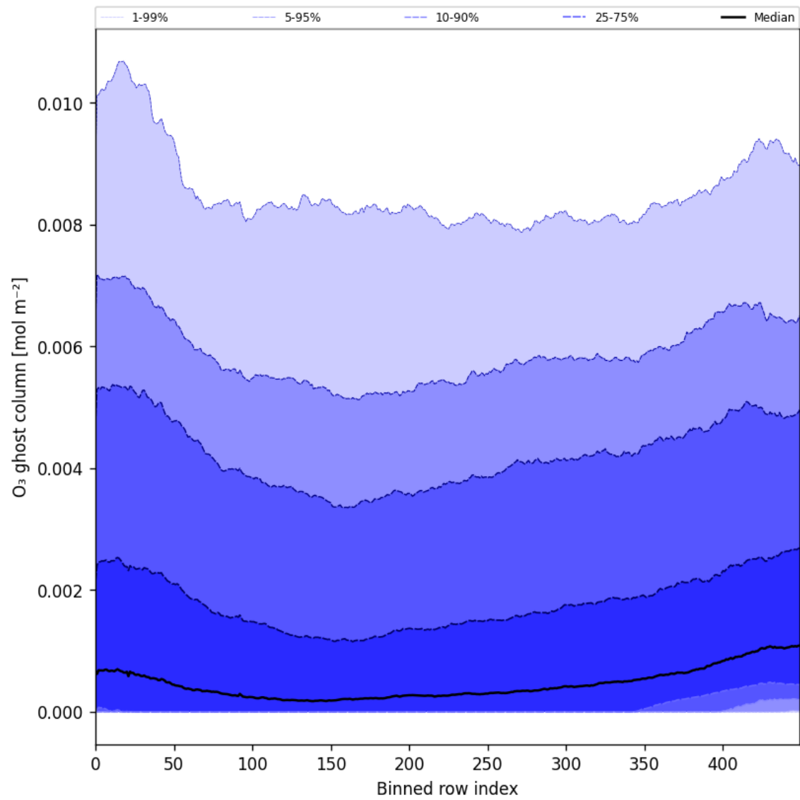
Figure 32: Along track statistics of “O 3 ghost column” for 2024-12-03 to 2024-12-05
