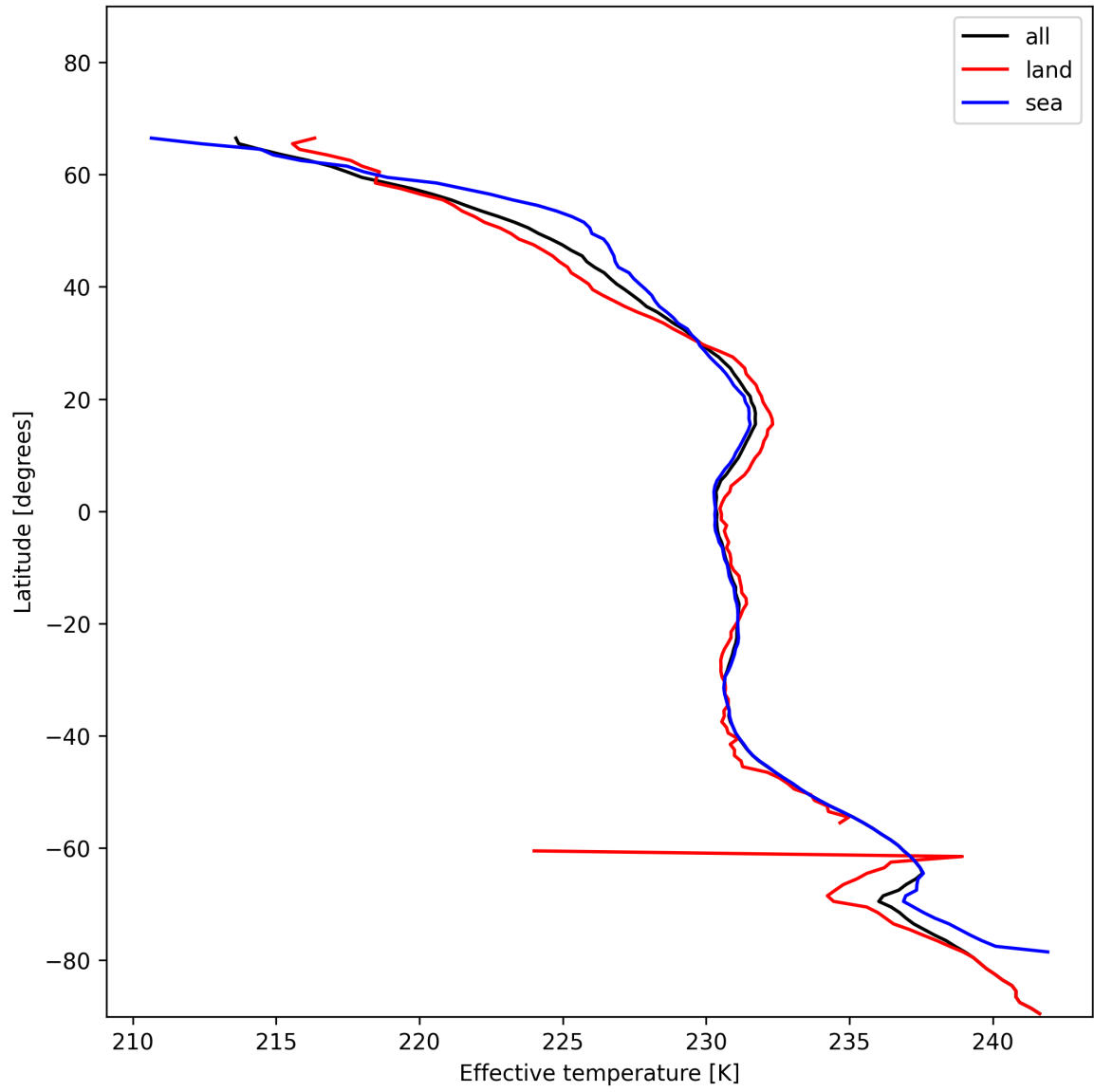
Figure 17: Zonal average of “Effective temperature” for 2024-12-03 to 2024-12-05.
