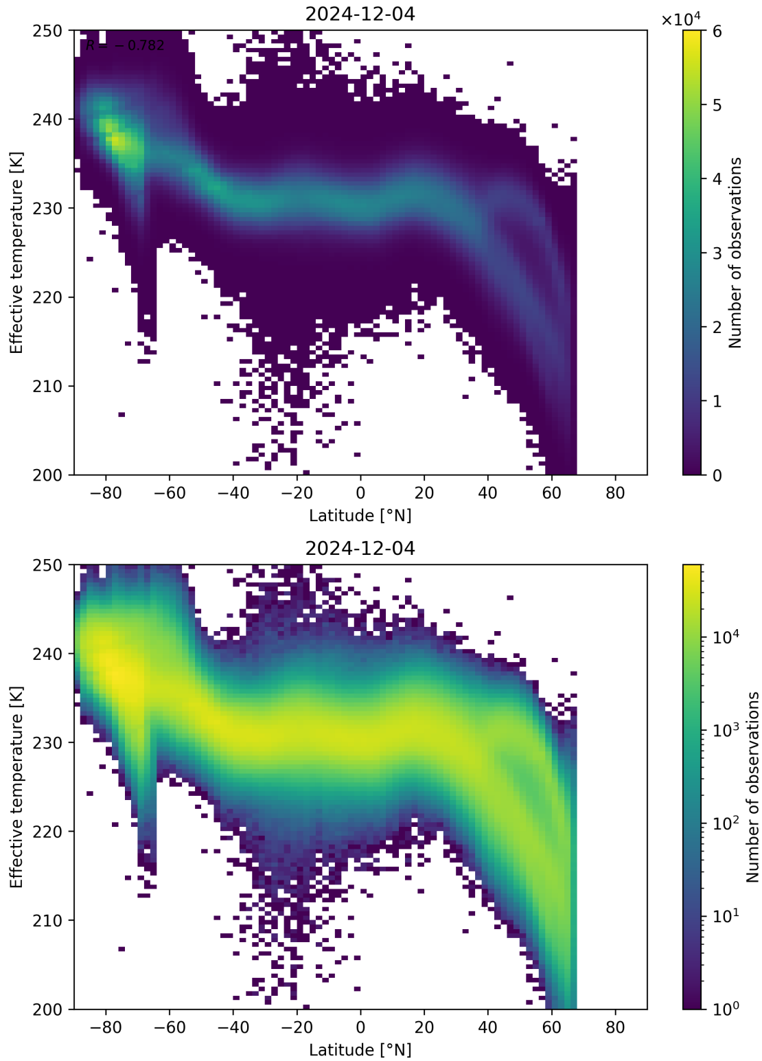
Figure 34: Scatter density plot of “Latitude” against “Effective temperature” for 2024-12-03 to 2024-12-05.
