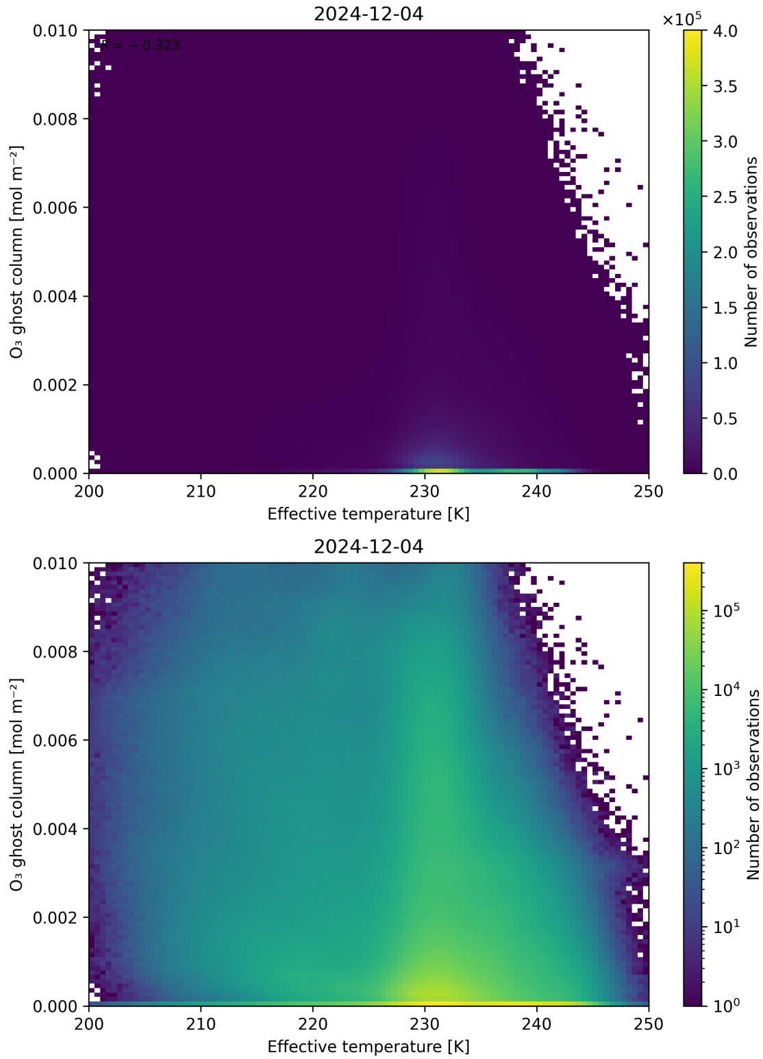
Figure 38: Scatter density plot of “Effective temperature” against “O 3 ghost column” for 2024-12-03 to 2024-12-05.
