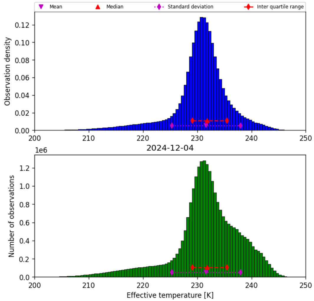
Figure 24: Histogram of “Effective temperature” for 2024-12-03 to 2024-12-05
