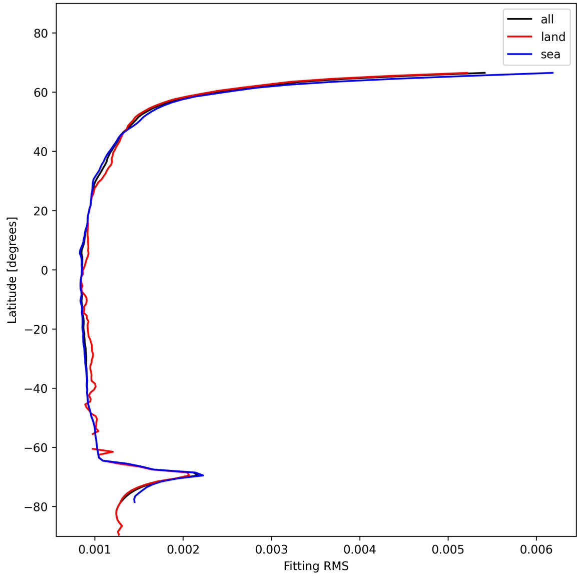
Figure 16: Zonal average of “Fitting RMS” for 2024-12-03 to 2024-12-05.
