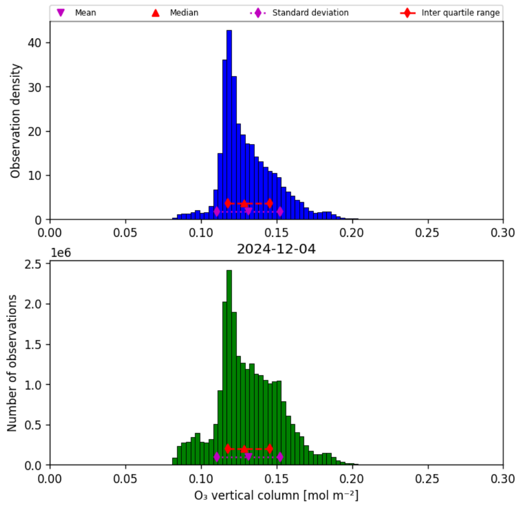
Figure 21: Histogram of “O 3 vertical column” for 2024-12-03 to 2024-12-05
