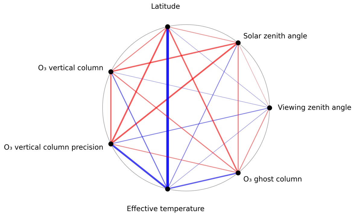
Figure 1: Map of correlation graph for 2024-12-04 to 2024-12-06.
