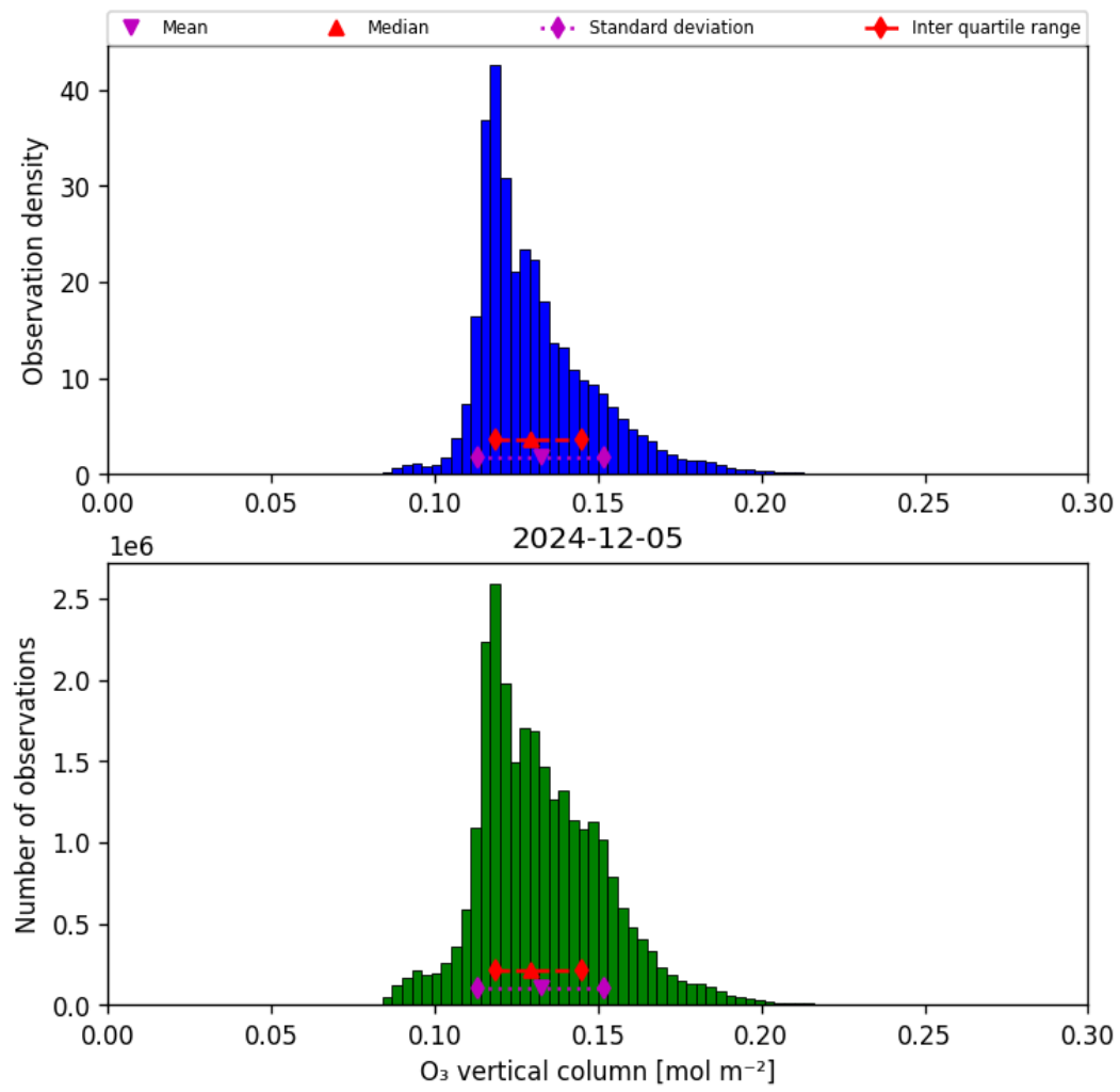
Figure 21: Histogram of “O 3 vertical column” for 2024-12-04 to 2024-12-06
