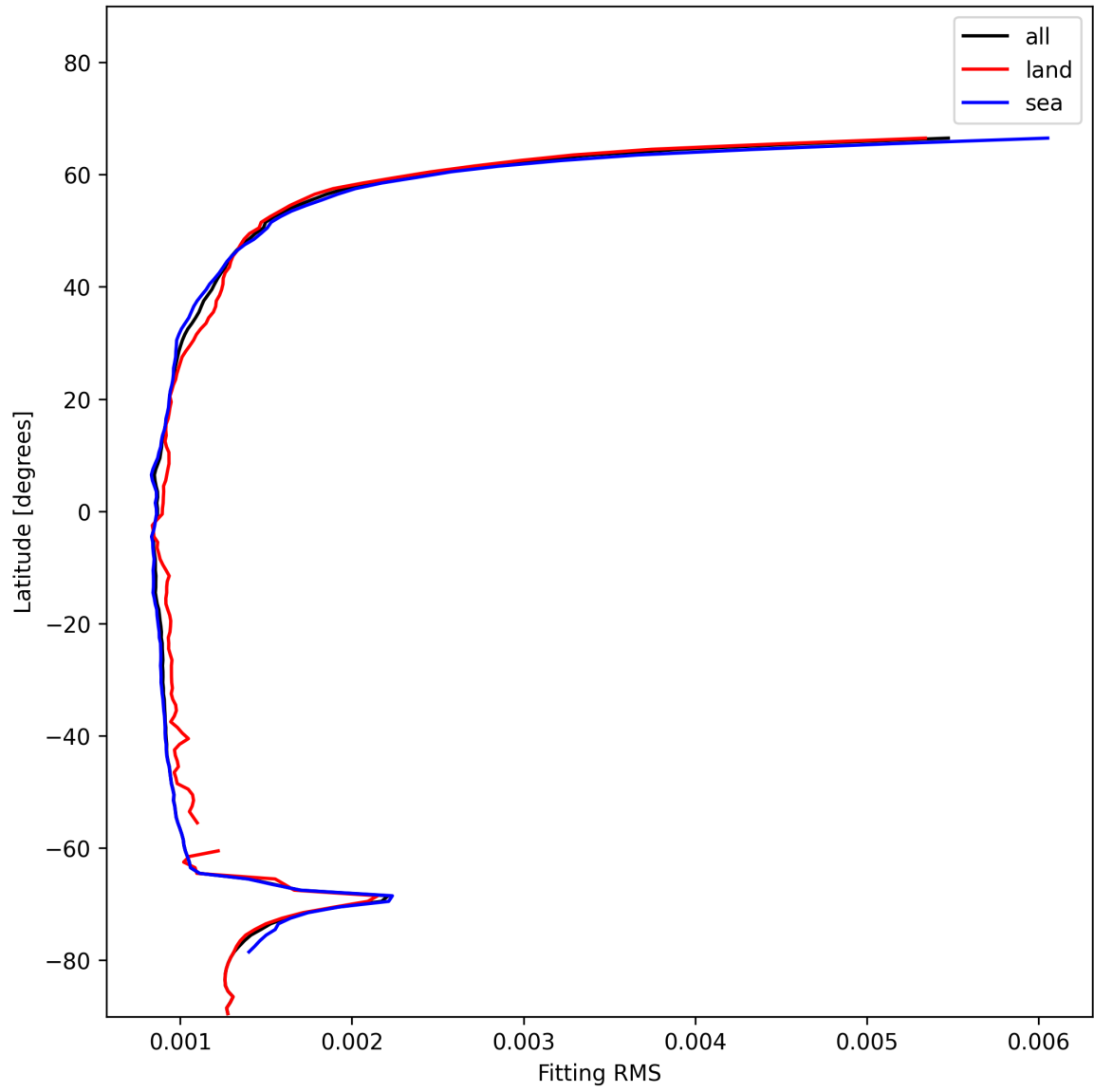
Figure 16: Zonal average of “Fitting RMS” for 2024-12-04 to 2024-12-06.
