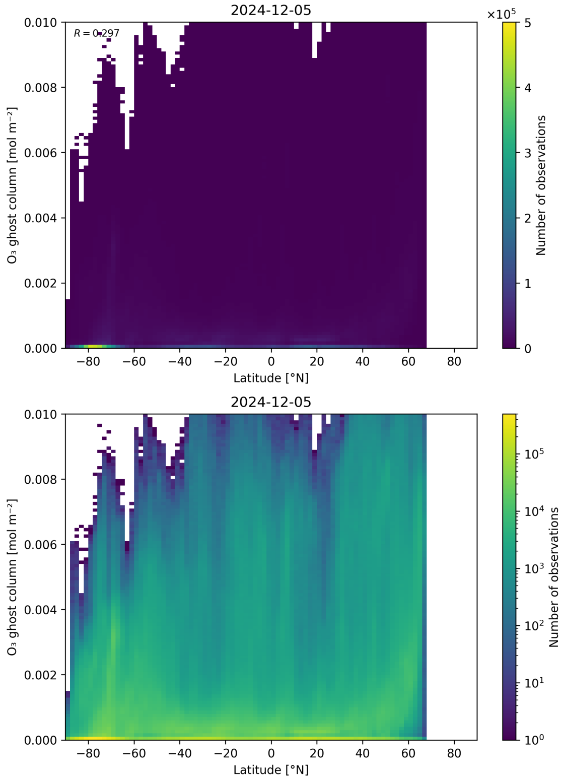
Figure 35: Scatter density plot of “Latitude” against “O 3 ghost column” for 2024-12-04 to 2024-12-06.
