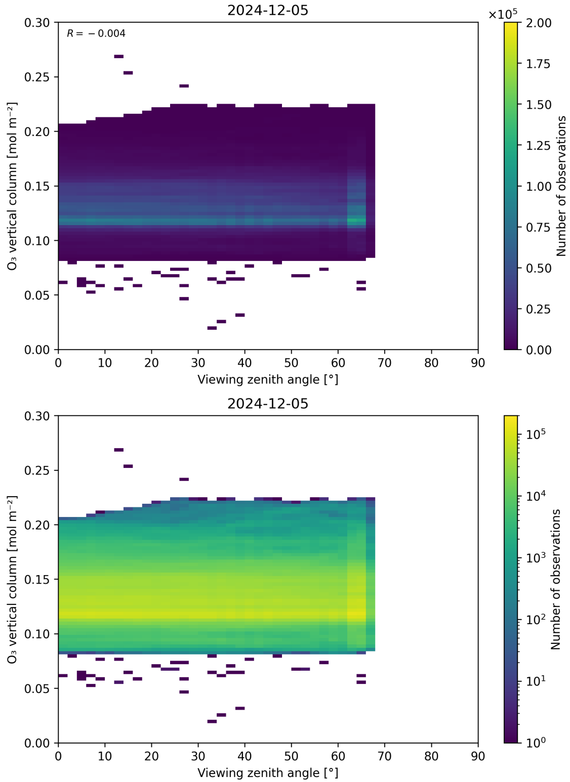
Figure 52: Scatter density plot of “Viewing zenith angle” against “O 3 vertical column” for 2024-12-04 to 2024-12-06.
