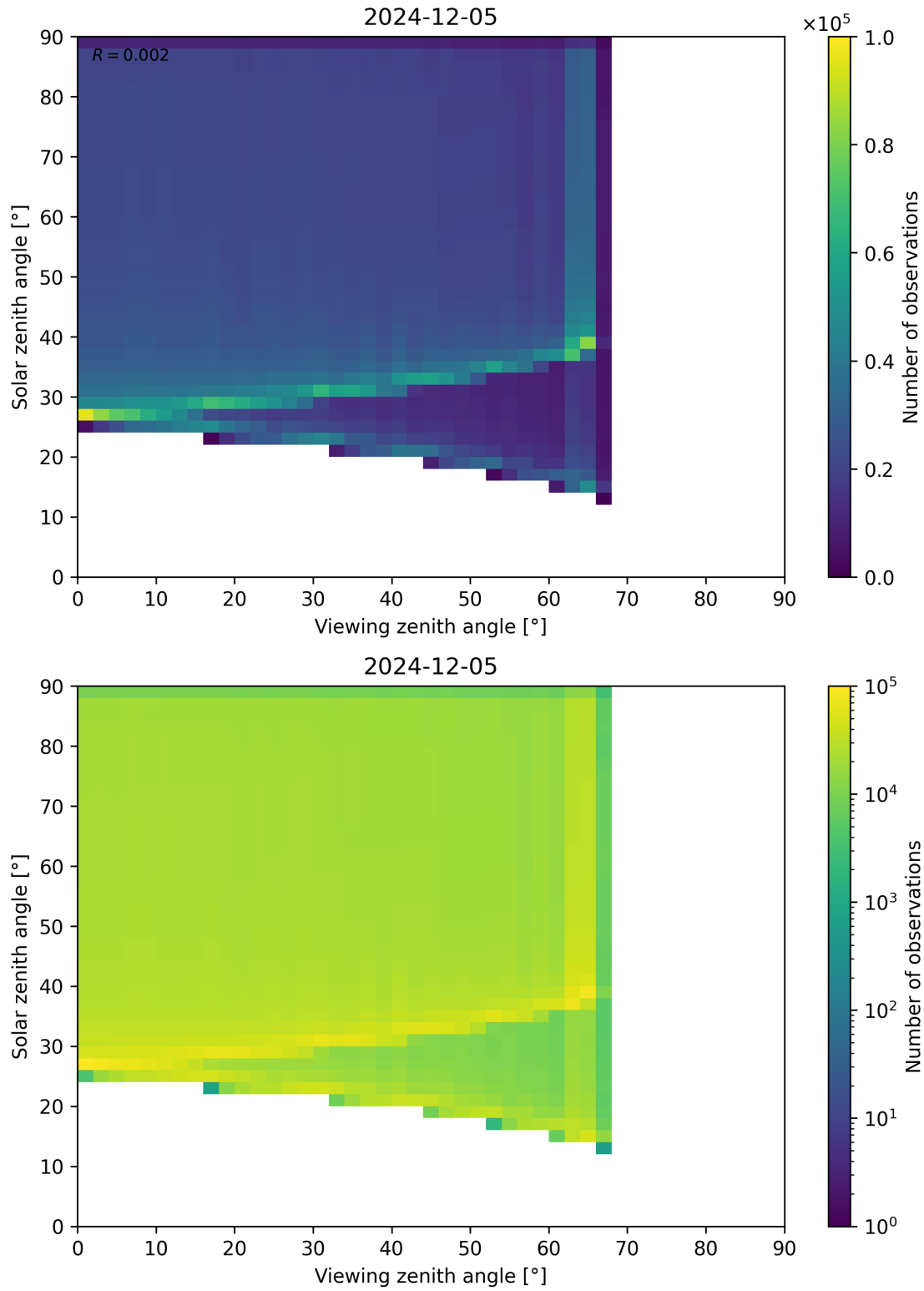
Figure 54: Scatter density plot of “Viewing zenith angle” against “Solar zenith angle” for 2024-12-04 to 2024-12-06.
