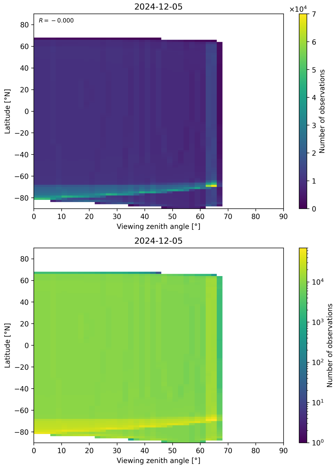
Figure 49: Scatter density plot of “Viewing zenith angle” against “Latitude” for 2024-12-04 to 2024-12-06.
