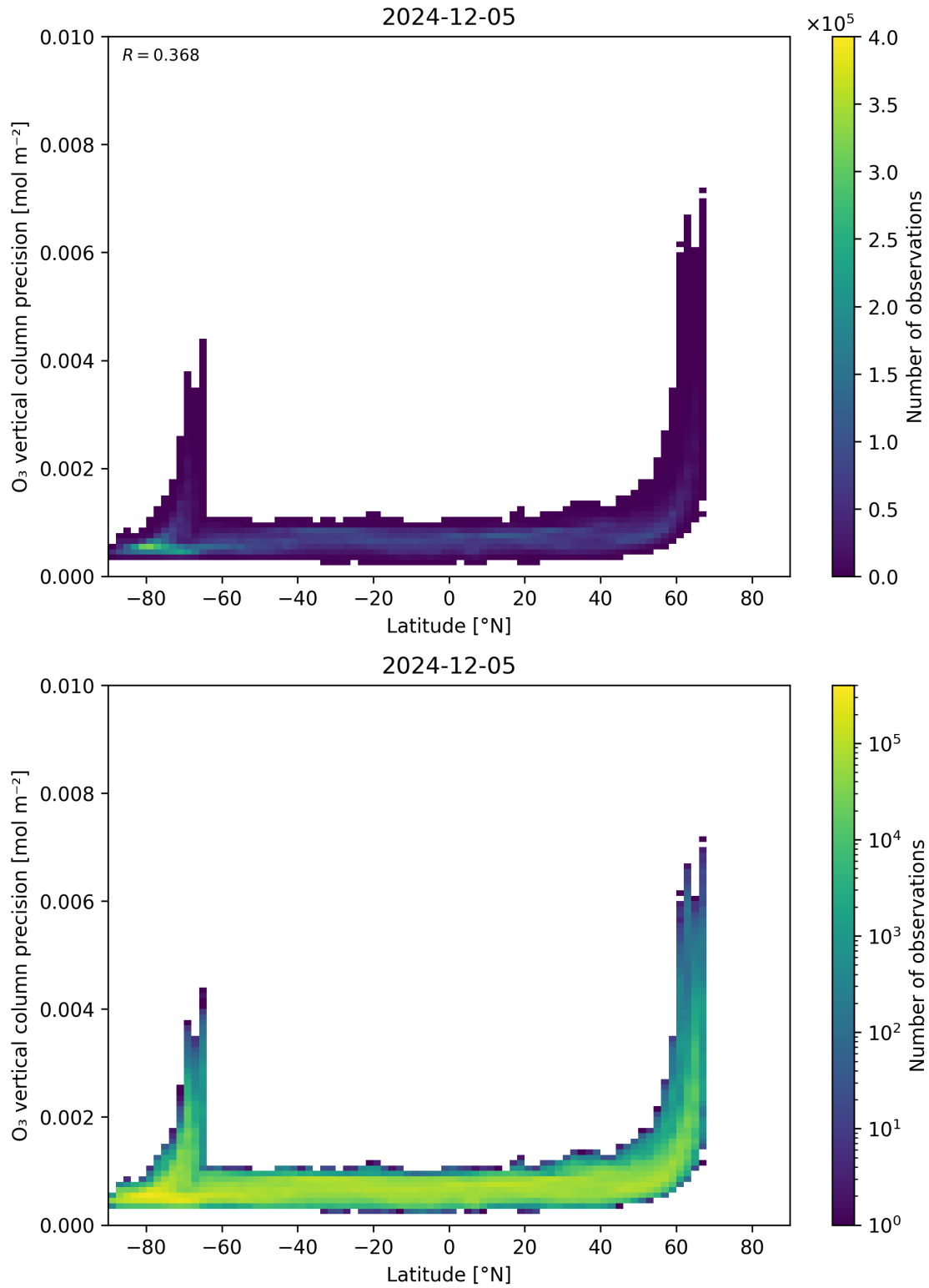
Figure 37: Scatter density plot of “Latitude” against “O 3 vertical column precision” for 2024-12-04 to 2024-12-06.
