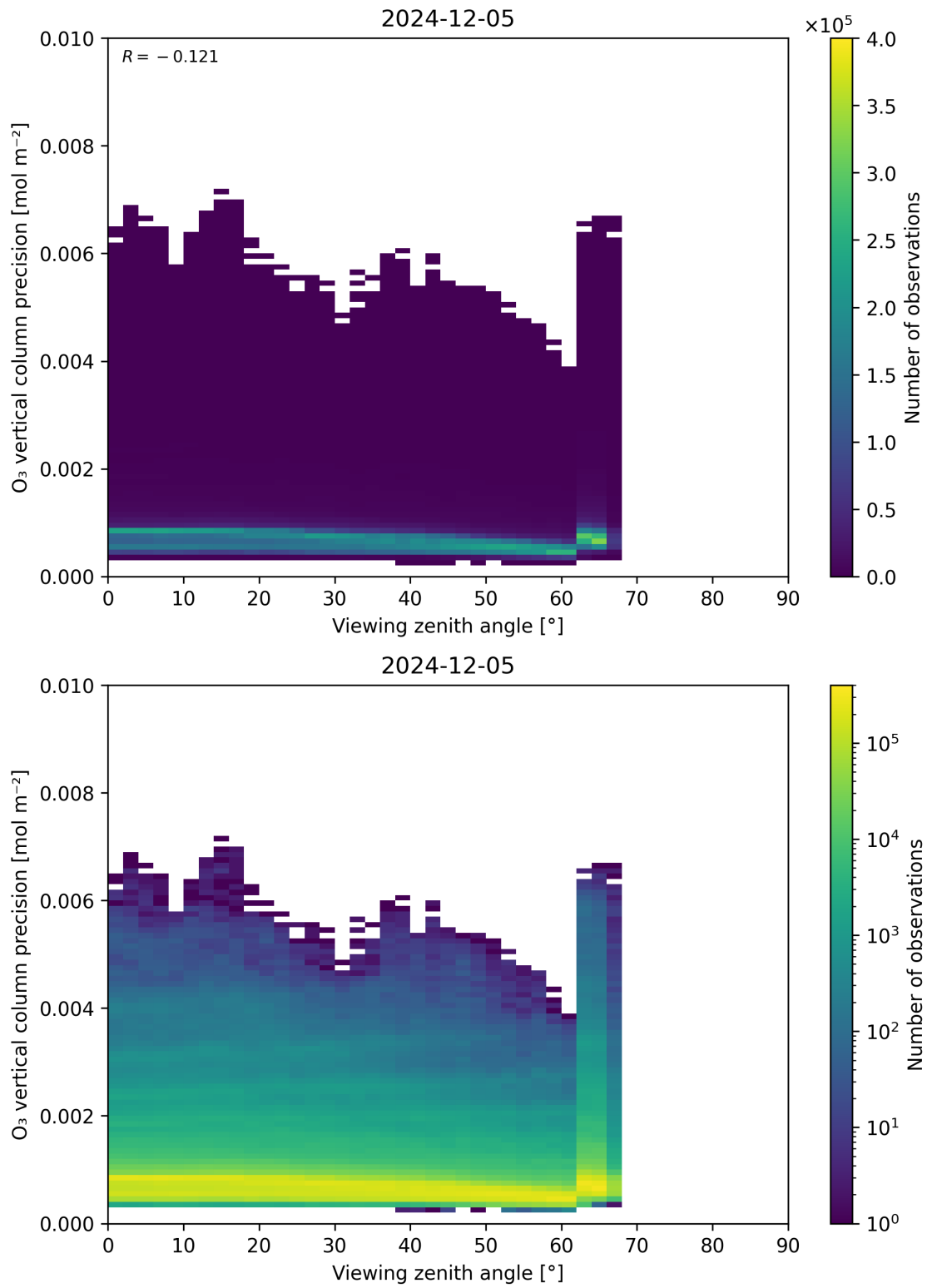
Figure 53: Scatter density plot of “Viewing zenith angle” against “O 3 vertical column precision” for 2024-12-04 to 2024-12-06.
