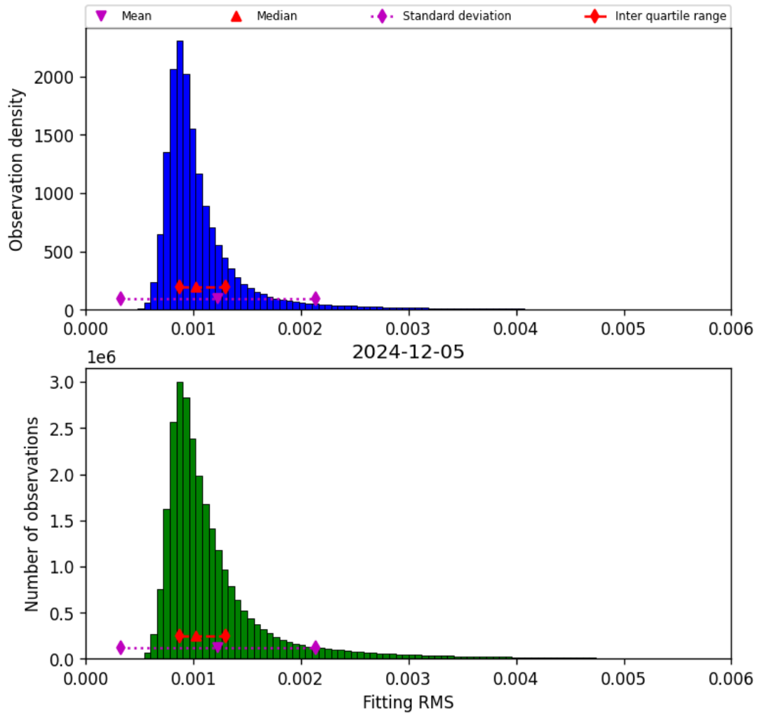
Figure 23: Histogram of “Fitting RMS” for 2024-12-04 to 2024-12-06
