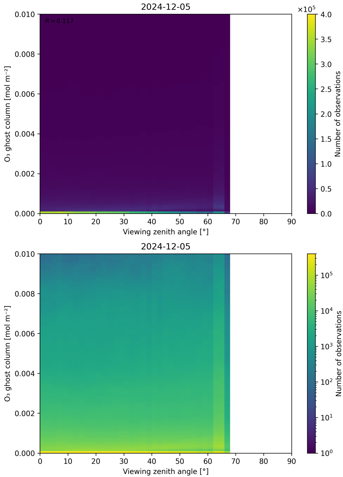
Figure 51: Scatter density plot of “Viewing zenith angle” against “O 3 ghost column” for 2024-12-04 to 2024-12-06.
