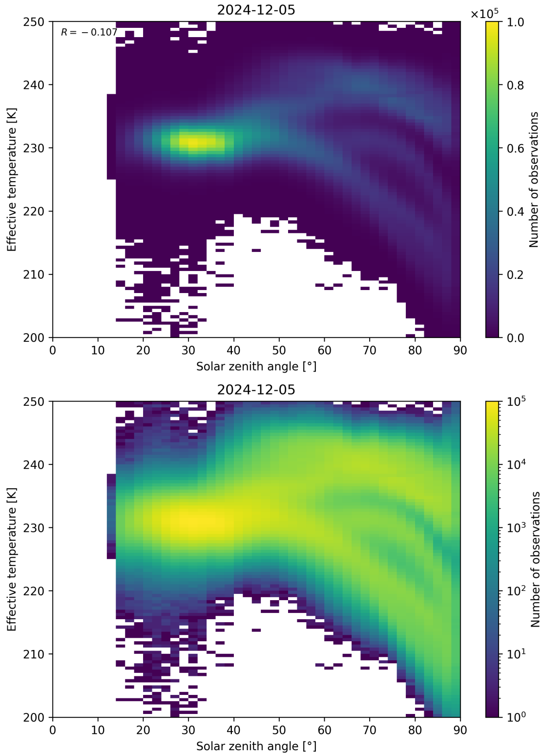
Figure 45: Scatter density plot of “Solar zenith angle” against “Effective temperature” for 2024-12-04 to 2024-12-06.
