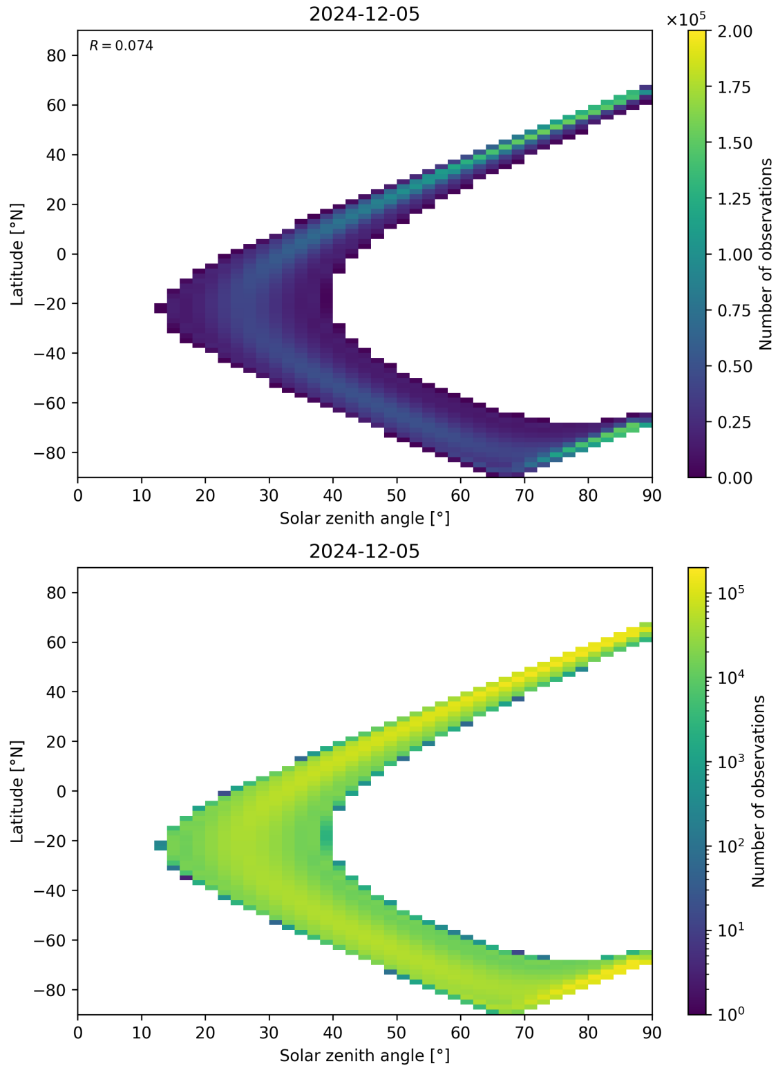
Figure 44: Scatter density plot of “Solar zenith angle” against “Latitude” for 2024-12-04 to 2024-12-06.
