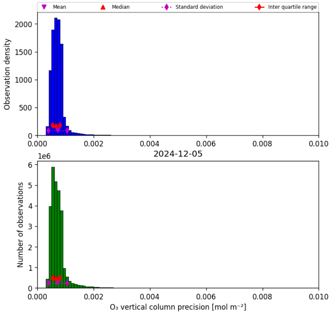
Figure 22: Histogram of “O 3 vertical column precision” for 2024-12-04 to 2024-12-06
