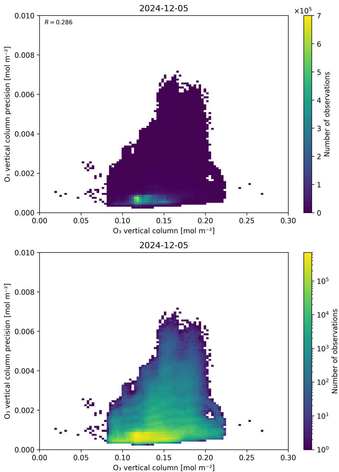
Figure 41: Scatter density plot of “O 3 vertical column” against “O 3 vertical column precision” for 2024-12-04 to 2024-12-06.
