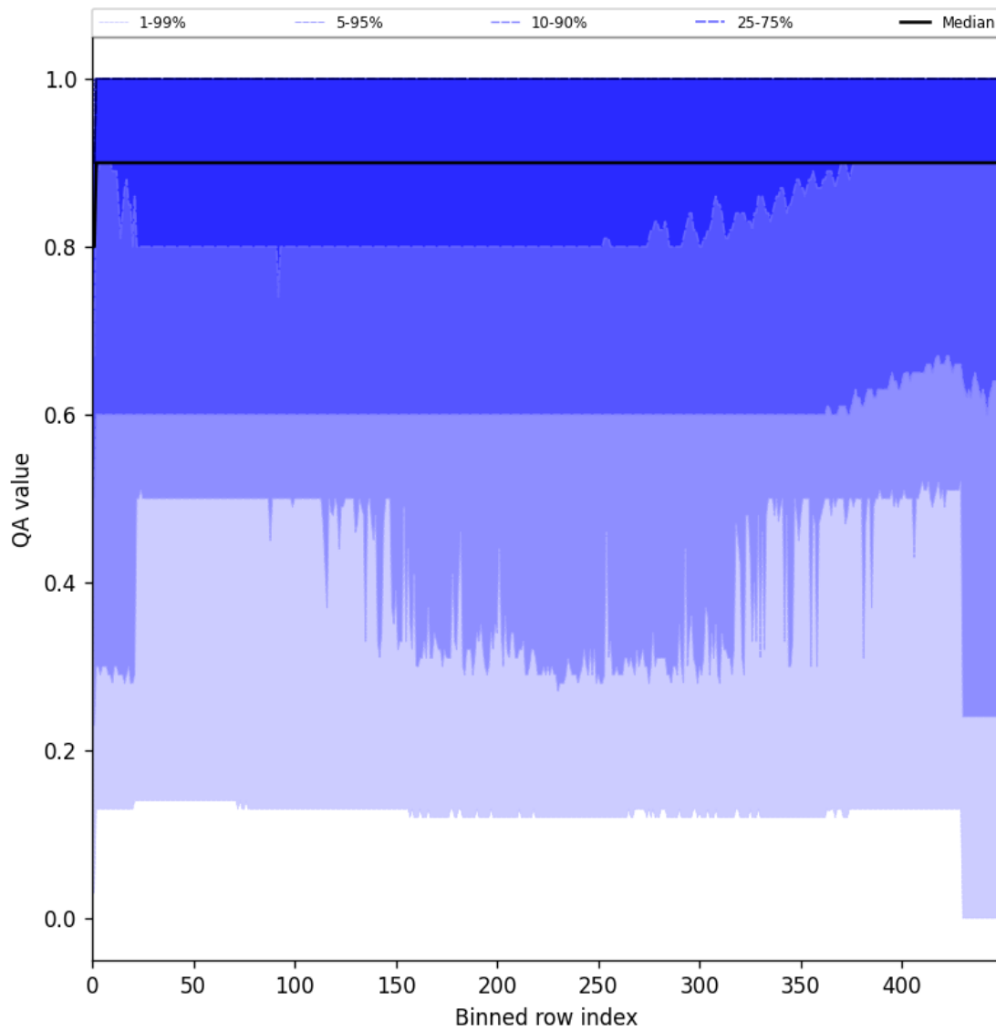
Figure 27: Along track statistics of “QA value” for 2024-12-04 to 2024-12-06
