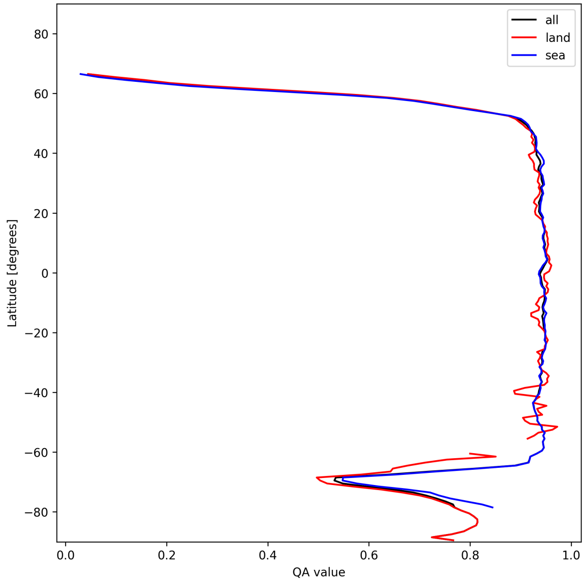
Figure 13: Zonal average of “QA value” for 2024-12-04 to 2024-12-06.
