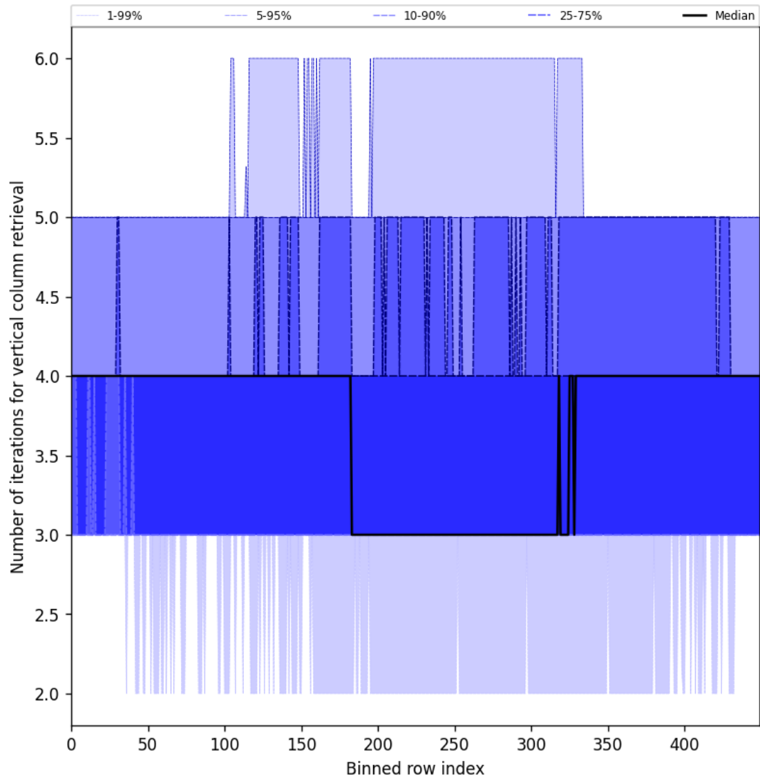
Figure 33: Along track statistics of “Number of iterations for vertical column retrieval” for 2024-12-04 to 2024-12-06
