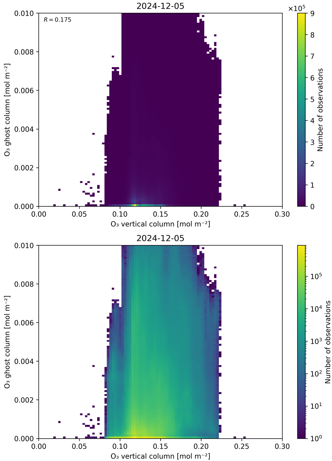
Figure 40: Scatter density plot of “O 3 vertical column” against “O 3 ghost column” for 2024-12-04 to 2024-12-06.
