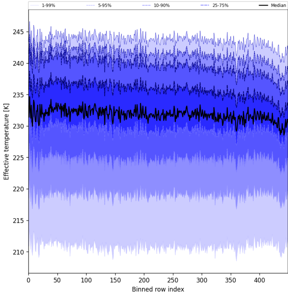
Figure 31: Along track statistics of “Effective temperature” for 2024-12-04 to 2024-12-06
