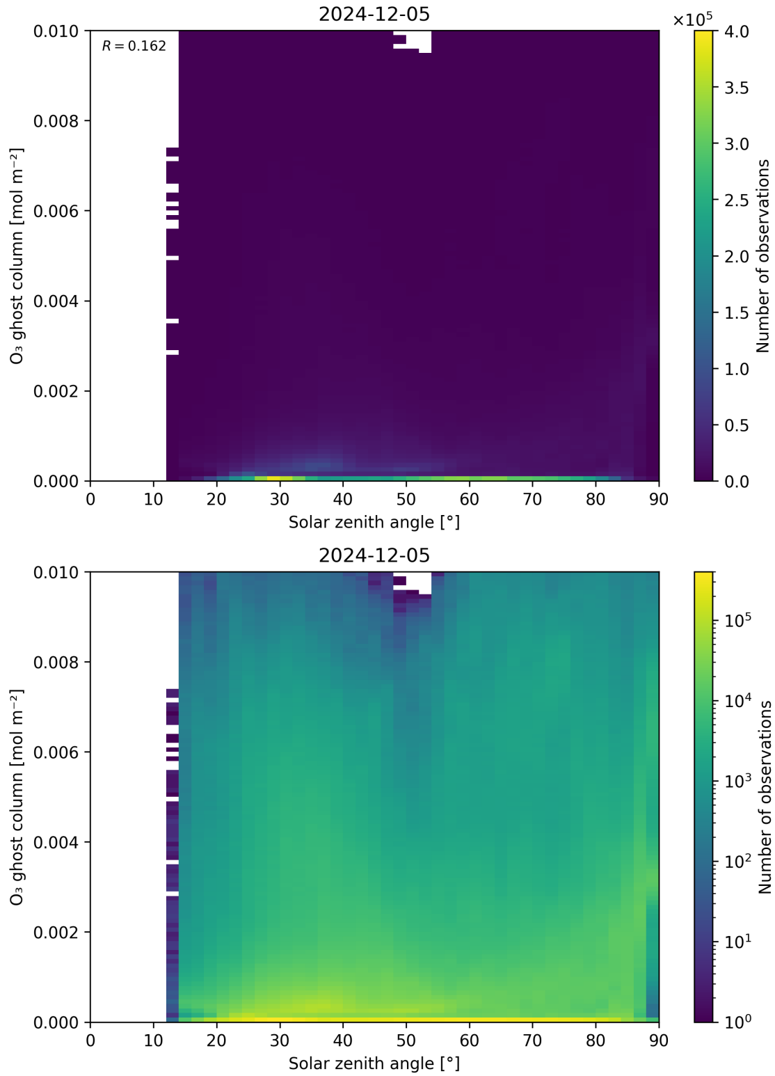
Figure 46: Scatter density plot of “Solar zenith angle” against “O 3 ghost column” for 2024-12-04 to 2024-12-06.
