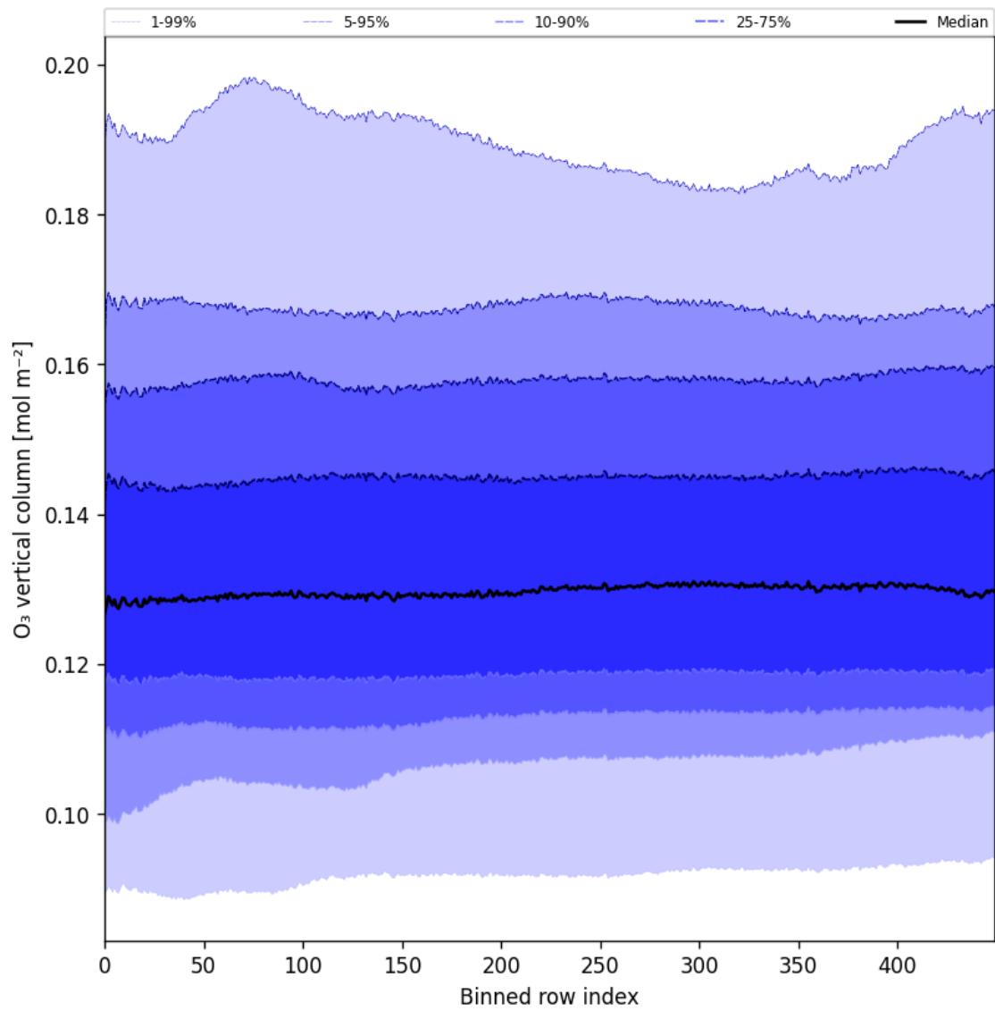
Figure 28: Along track statistics of “O 3 vertical column” for 2024-12-04 to 2024-12-06
