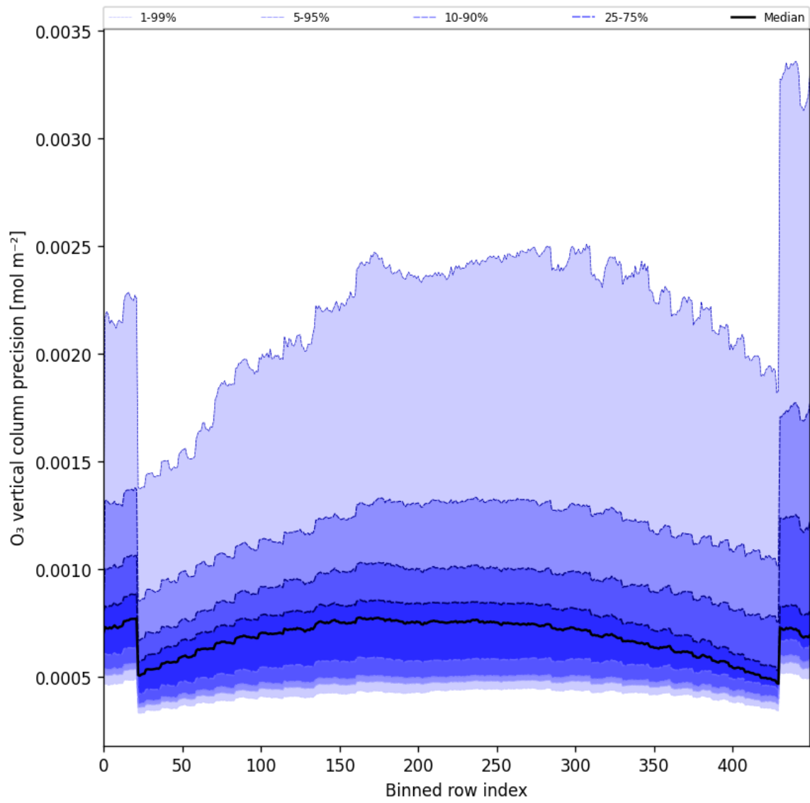
Figure 29: Along track statistics of “O 3 vertical column precision” for 2024-12-04 to 2024-12-06
