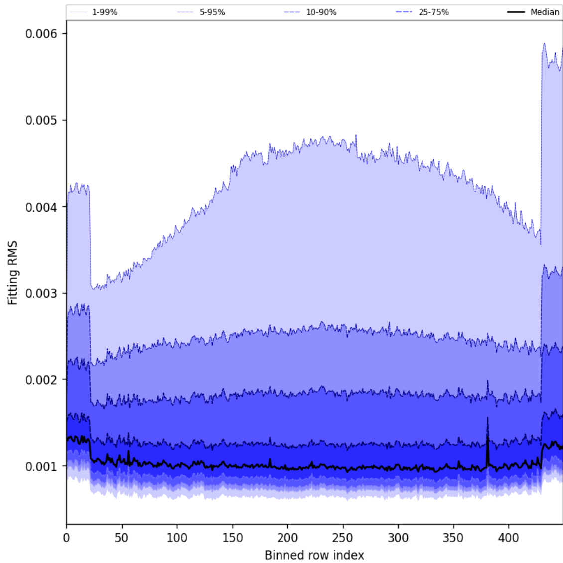
Figure 30: Along track statistics of “Fitting RMS” for 2024-12-04 to 2024-12-06
