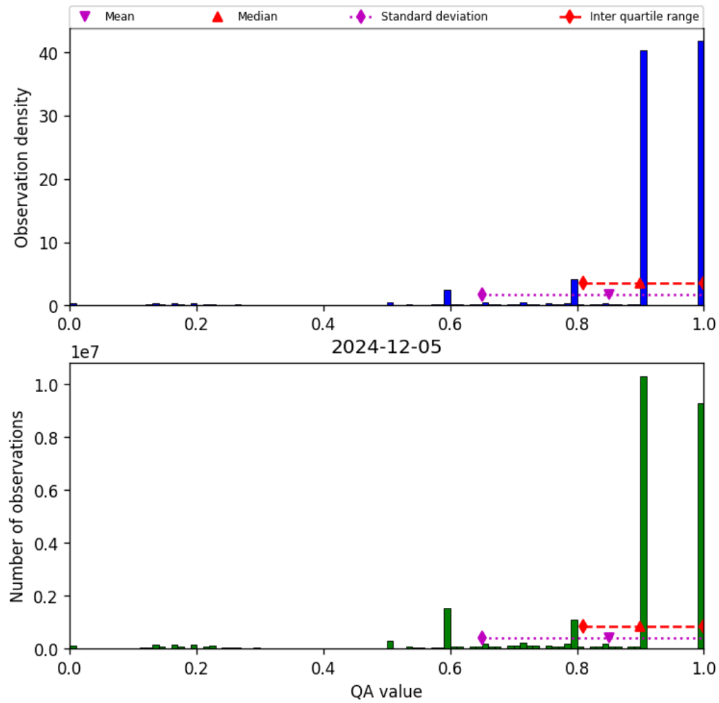
Figure 20: Histogram of “QA value” for 2024-12-04 to 2024-12-06
