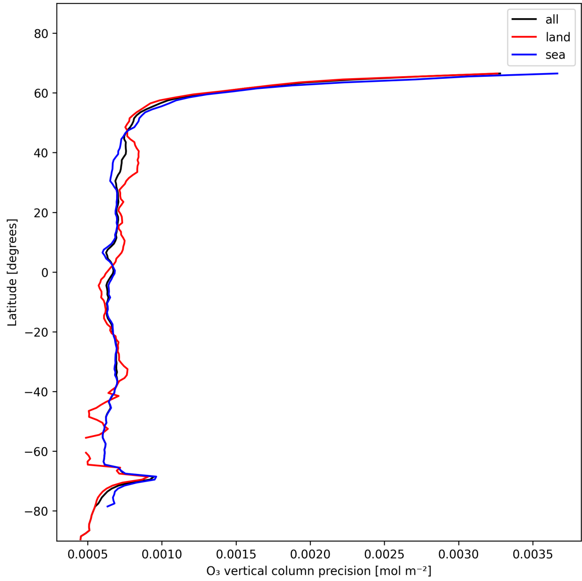
Figure 15: Zonal average of “O 3 vertical column precision” for 2024-12-04 to 2024-12-06.
