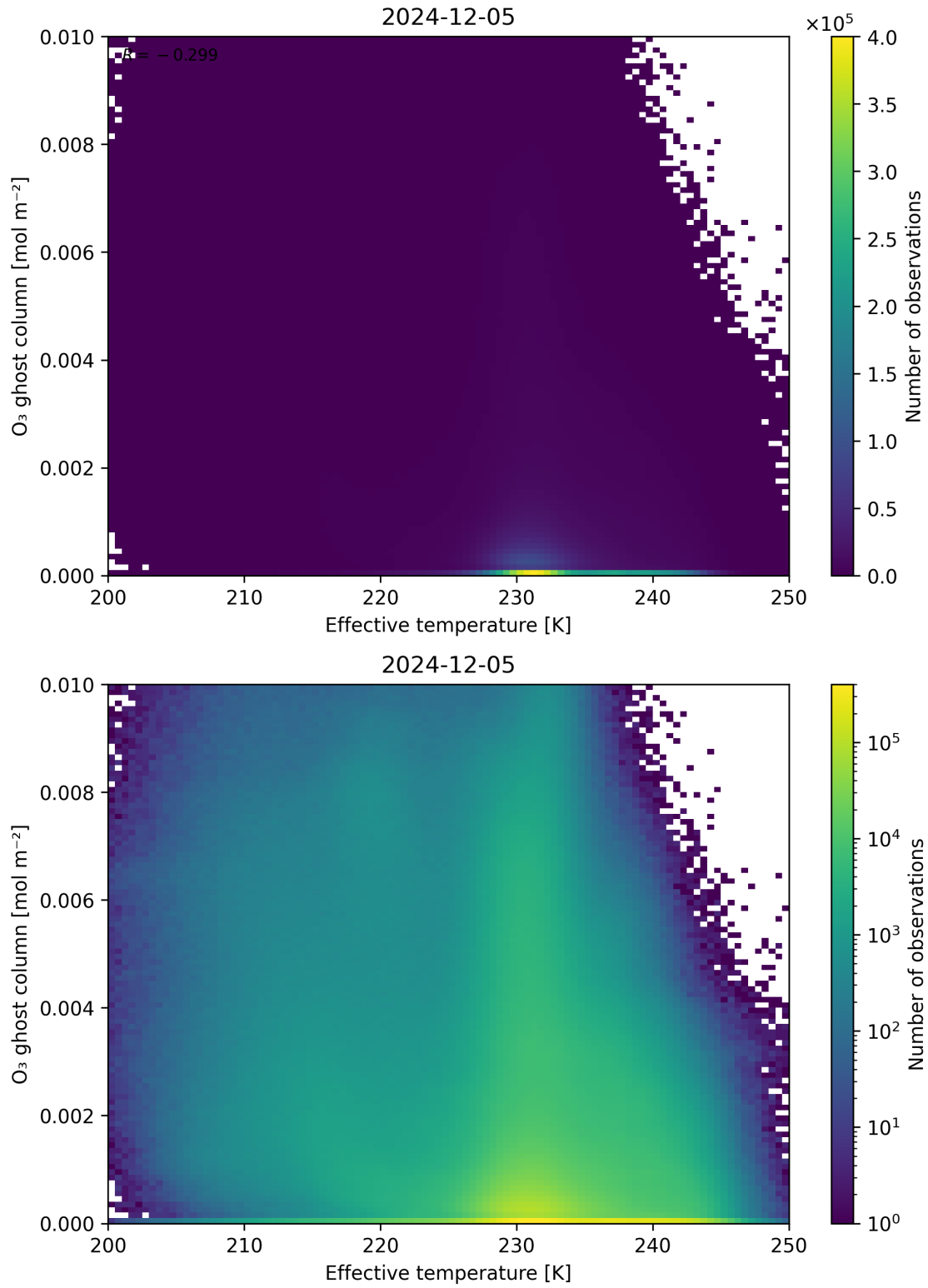
Figure 38: Scatter density plot of “Effective temperature” against “O 3 ghost column” for 2024-12-04 to 2024-12-06.
