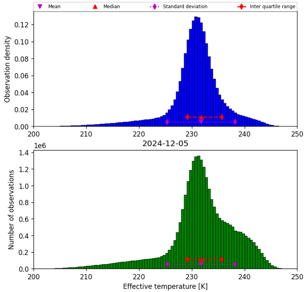
Figure 24: Histogram of “Effective temperature” for 2024-12-04 to 2024-12-06
