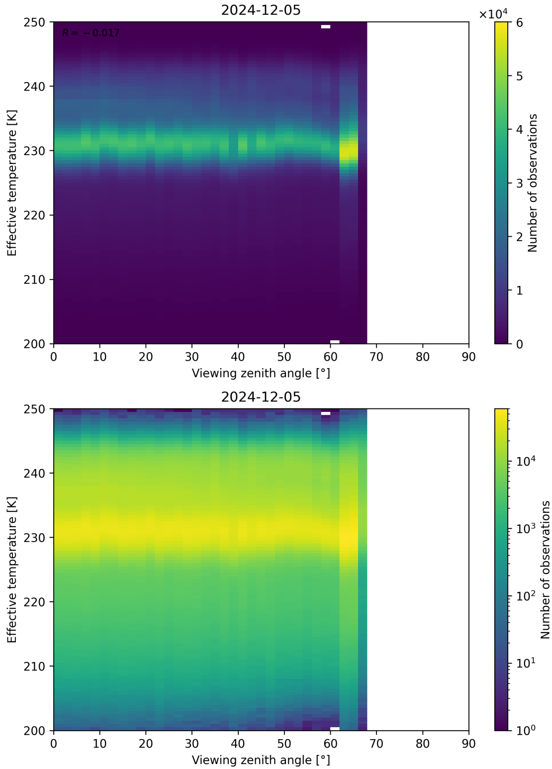
Figure 50: Scatter density plot of “Viewing zenith angle” against “Effective temperature” for 2024-12-04 to 2024-12-06.
