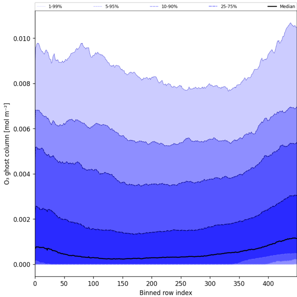
Figure 32: Along track statistics of “O 3 ghost column” for 2024-12-04 to 2024-12-06
