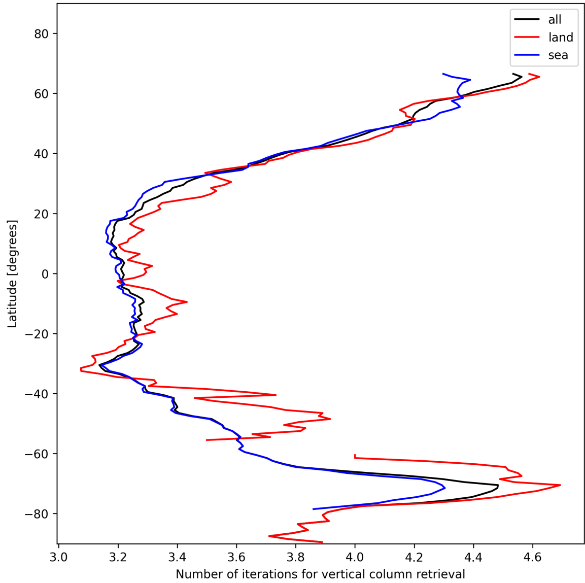
Figure 19: Zonal average of “Number of iterations for vertical column retrieval” for 2024-12-04 to 2024-12-06.
