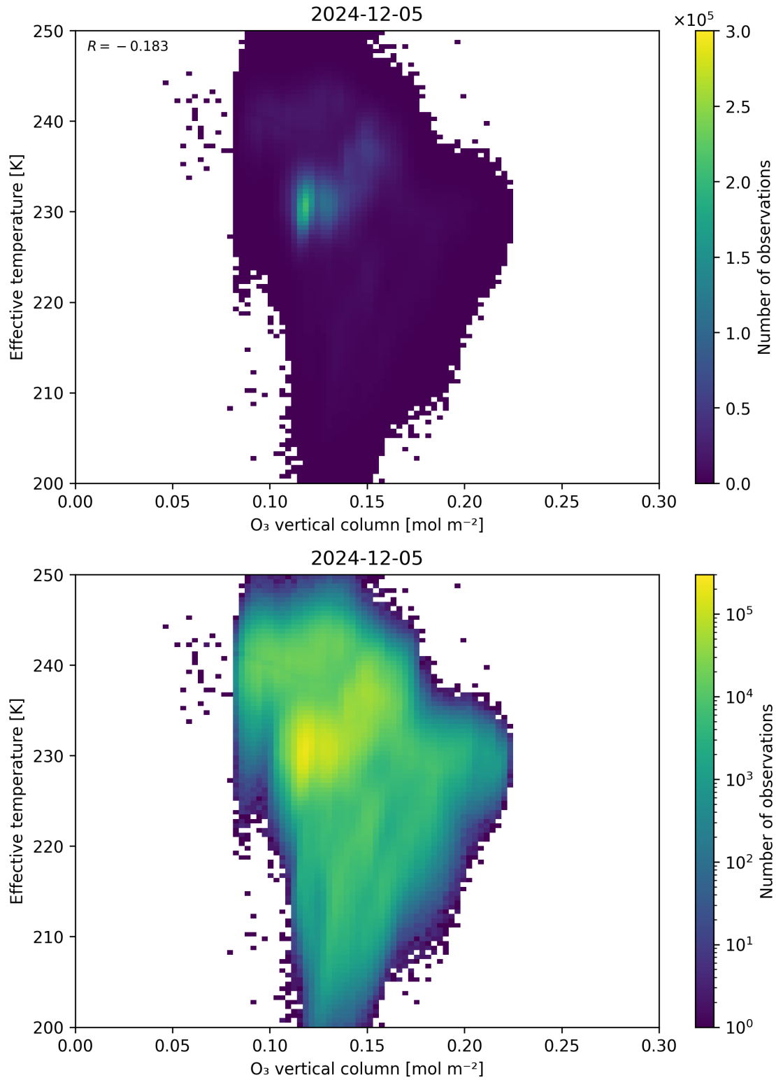
Figure 39: Scatter density plot of “O 3 vertical column” against “Effective temperature” for 2024-12-04 to 2024-12-06.
