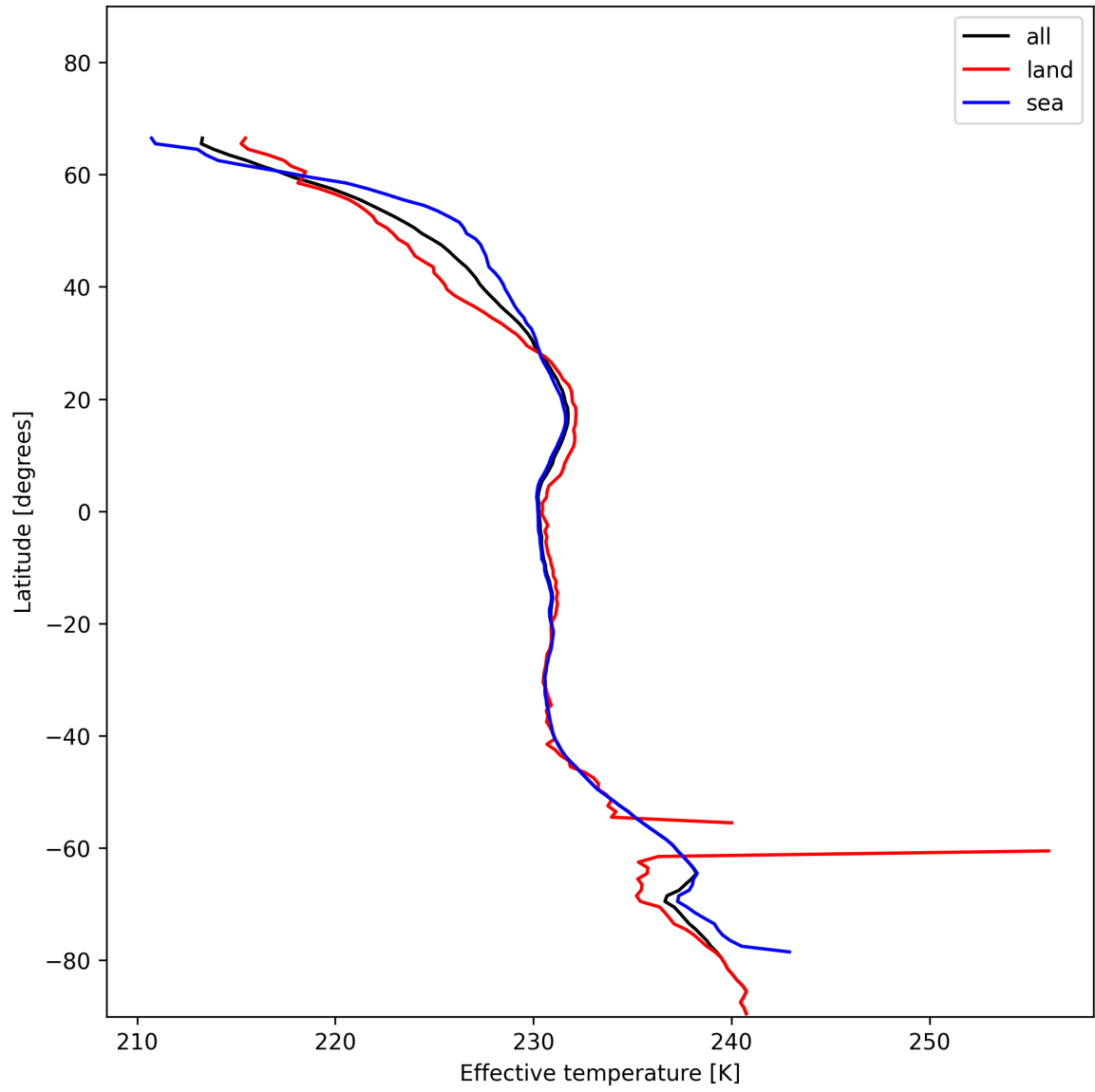
Figure 17: Zonal average of “Effective temperature” for 2024-12-04 to 2024-12-06.
