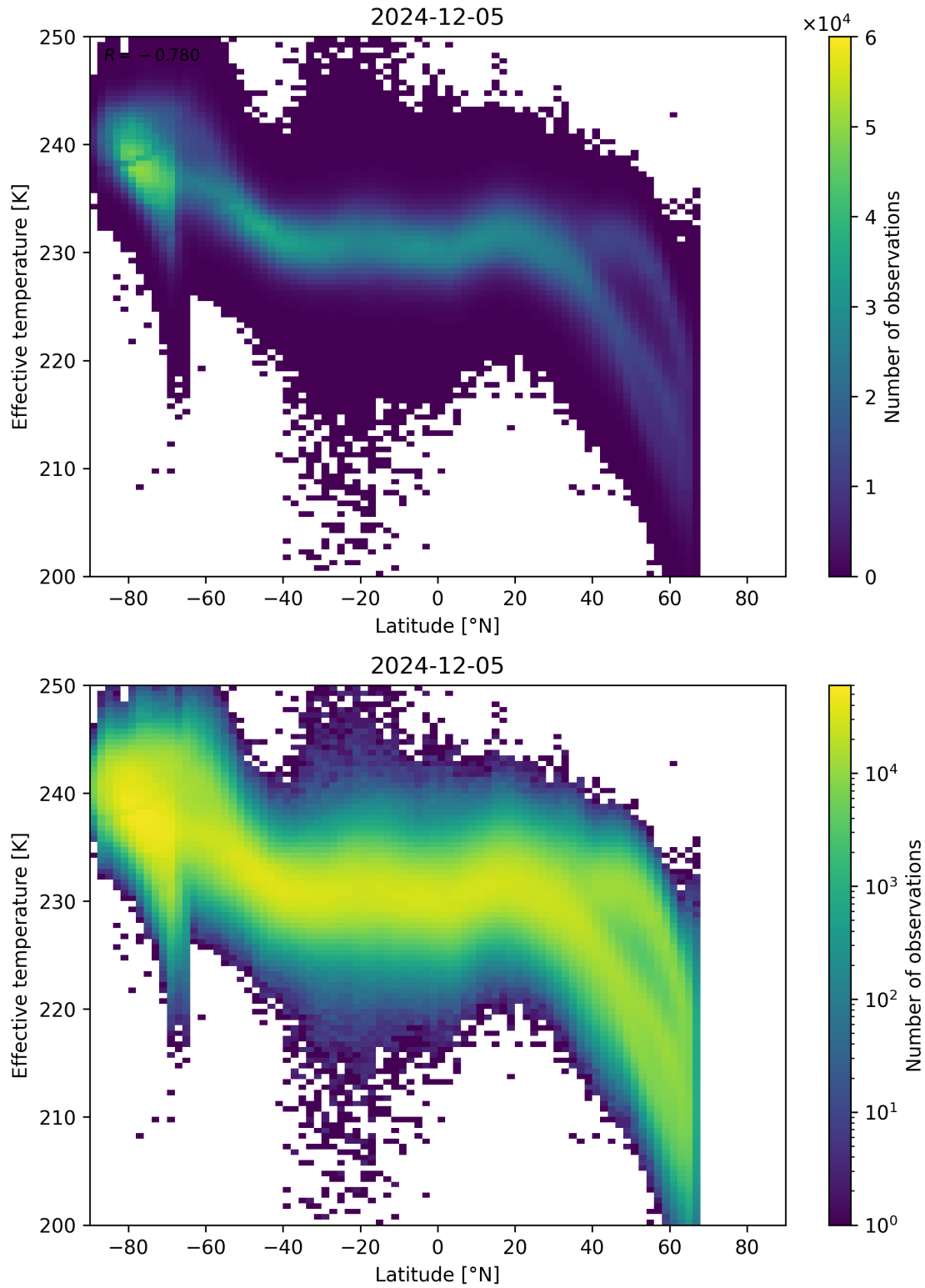
Figure 34: Scatter density plot of “Latitude” against “Effective temperature” for 2024-12-04 to 2024-12-06.
