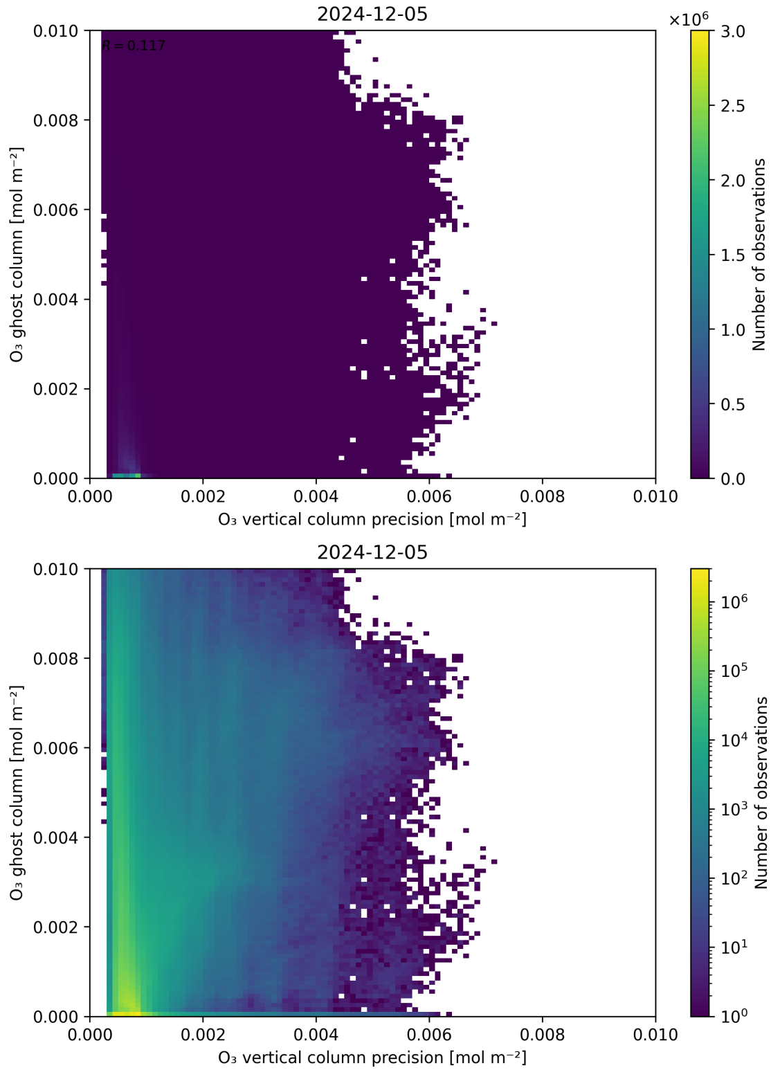
Figure 43: Scatter density plot of “ \text{O}_3 vertical column precision” against “ \text{O}_3 ghost column” for 2024-12-04 to 2024-12-06.
