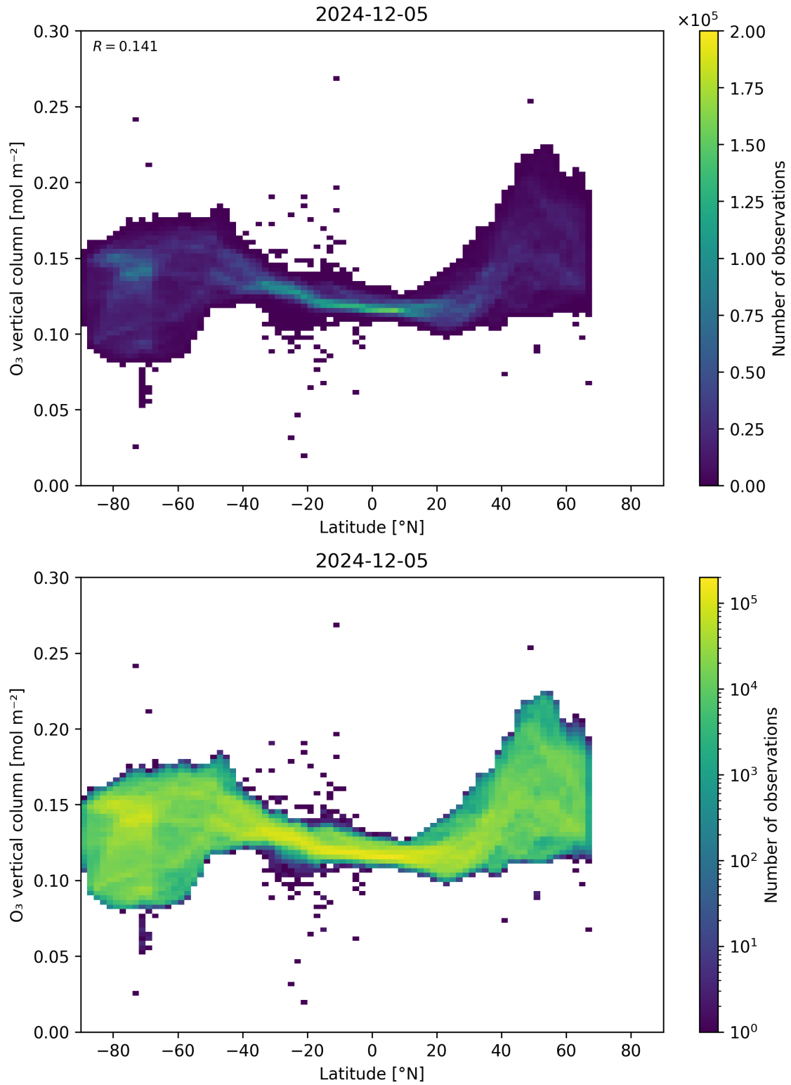
Figure 36: Scatter density plot of “Latitude” against “O 3 vertical column” for 2024-12-04 to 2024-12-06.
