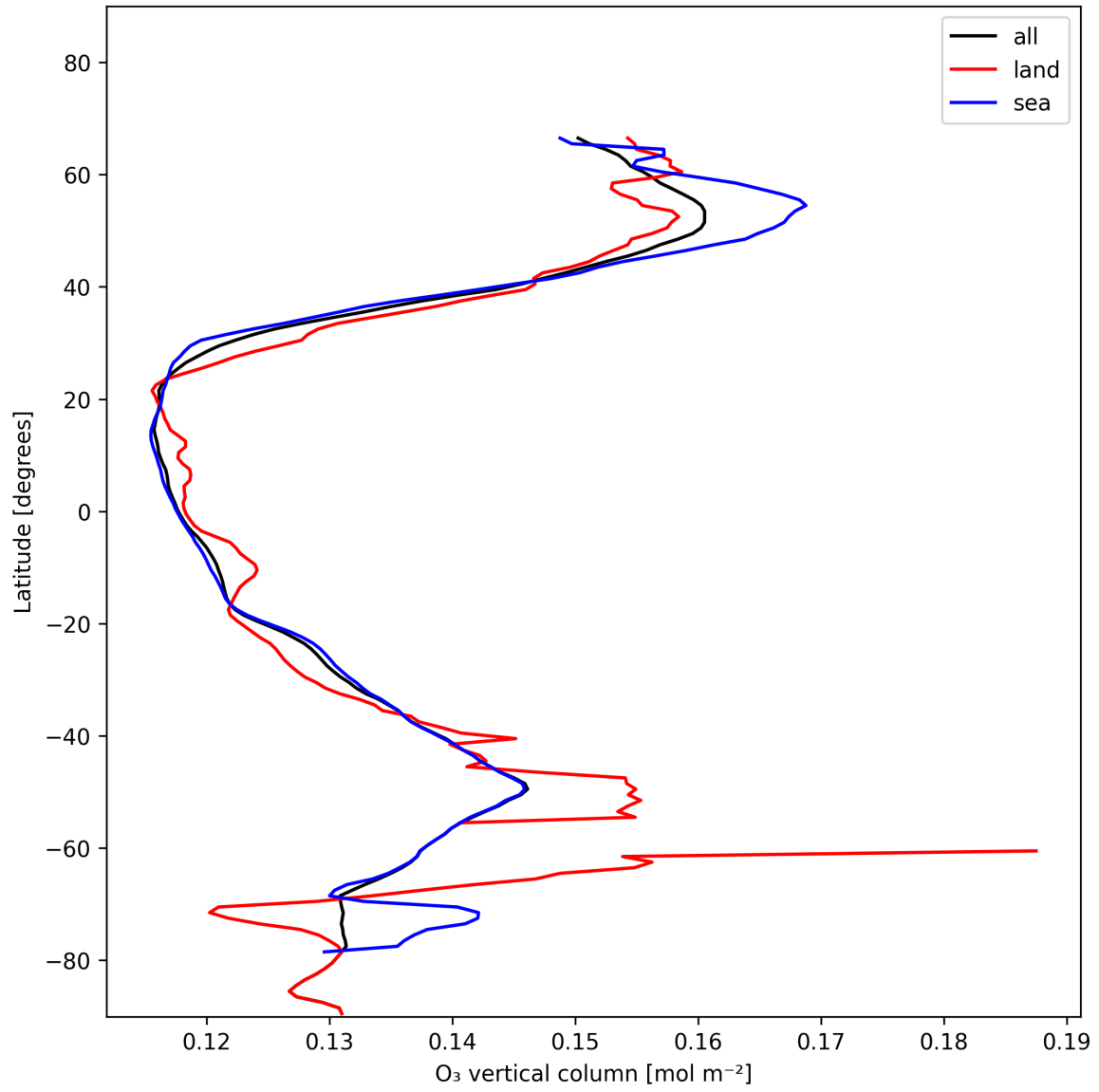
Figure 14: Zonal average of “O 3 vertical column” for 2024-12-04 to 2024-12-06.
