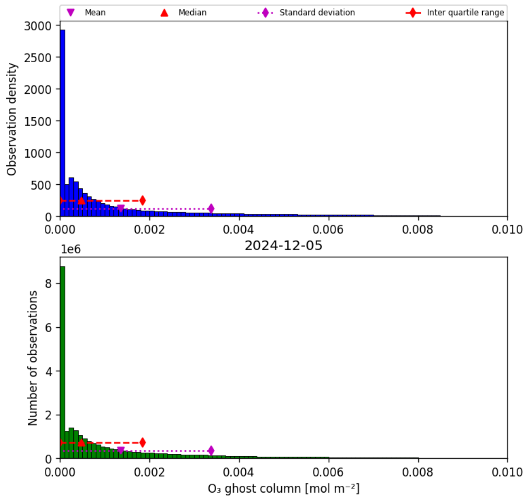
Figure 25: Histogram of “O 3 ghost column” for 2024-12-04 to 2024-12-06
