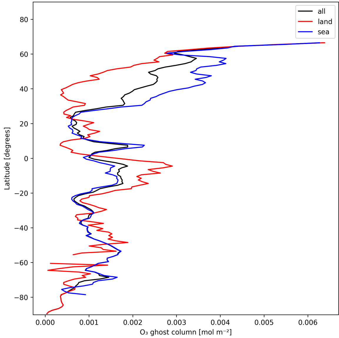
Figure 18: Zonal average of “O 3 ghost column” for 2024-12-04 to 2024-12-06.
