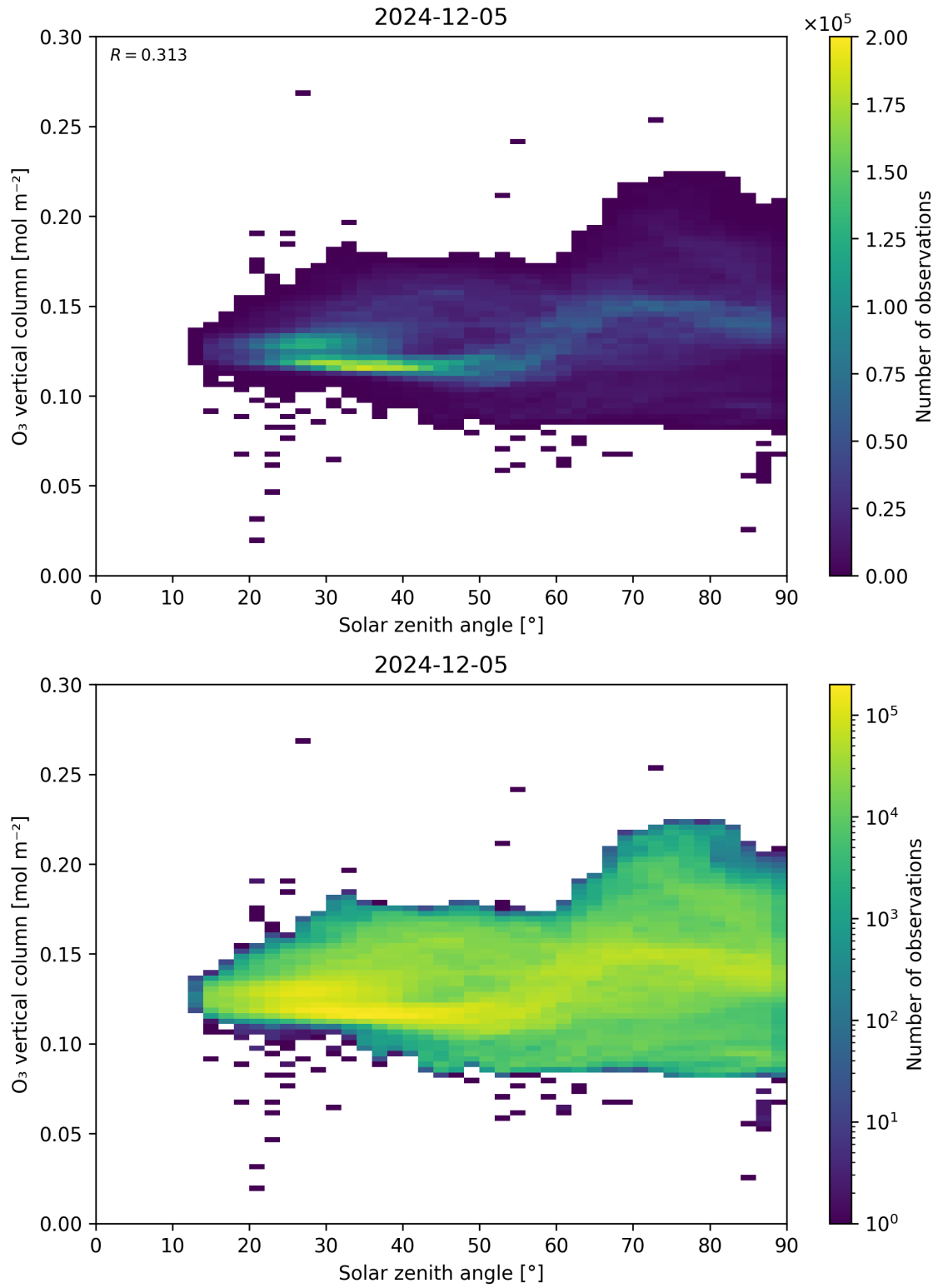
Figure 47: Scatter density plot of “Solar zenith angle” against “O 3 vertical column” for 2024-12-04 to 2024-12-06.
