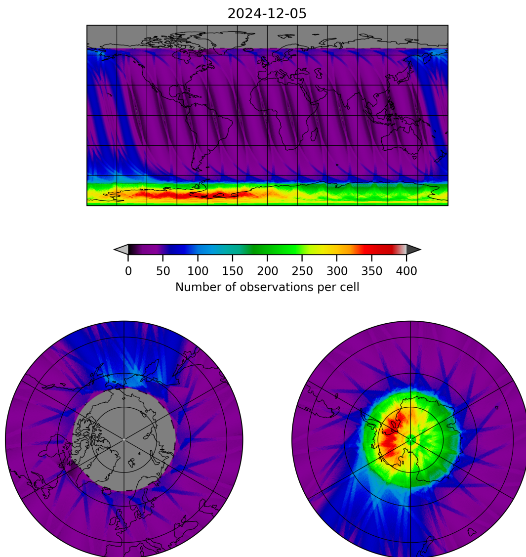
Figure 12: Map of the number of observations for 2024-12-04 to 2024-12-06
