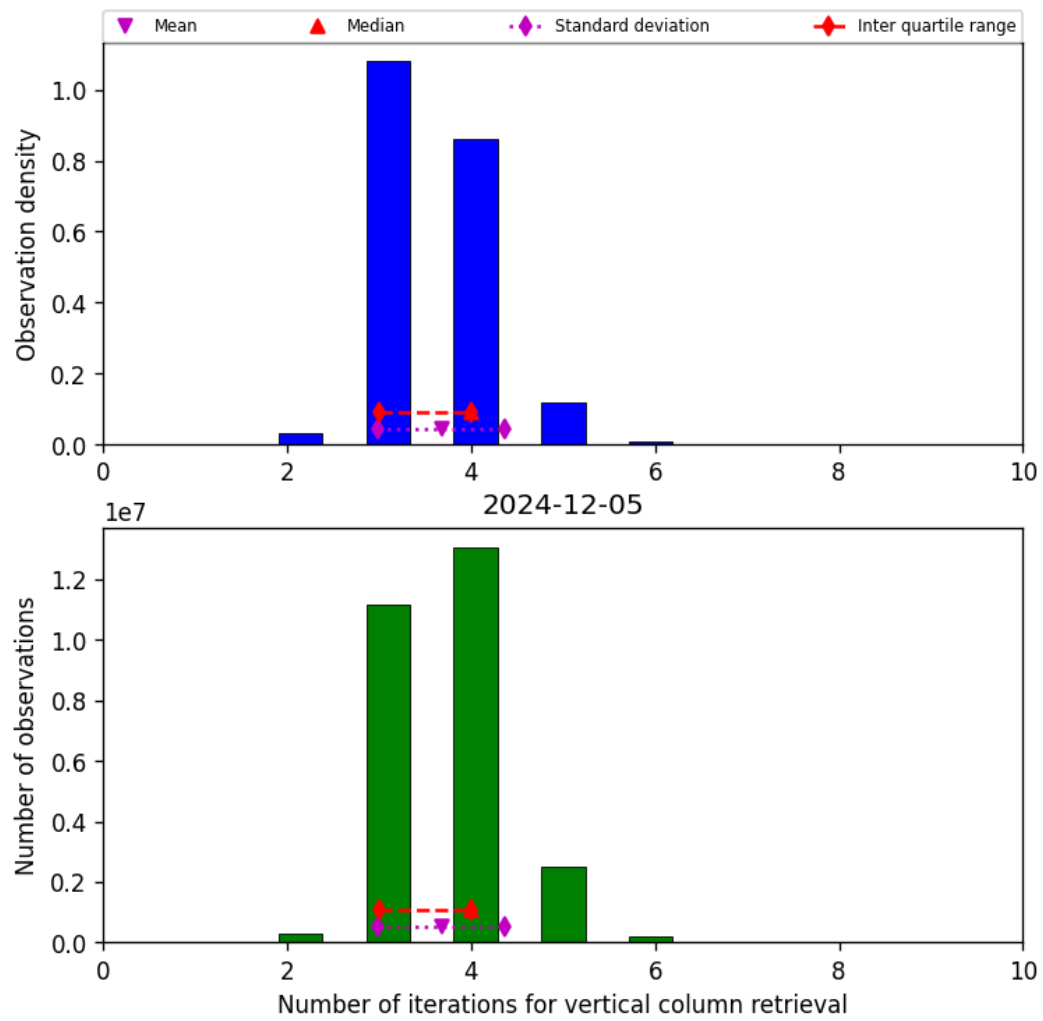
Figure 26: Histogram of “Number of iterations for vertical column retrieval” for 2024-12-04 to 2024-12-06
