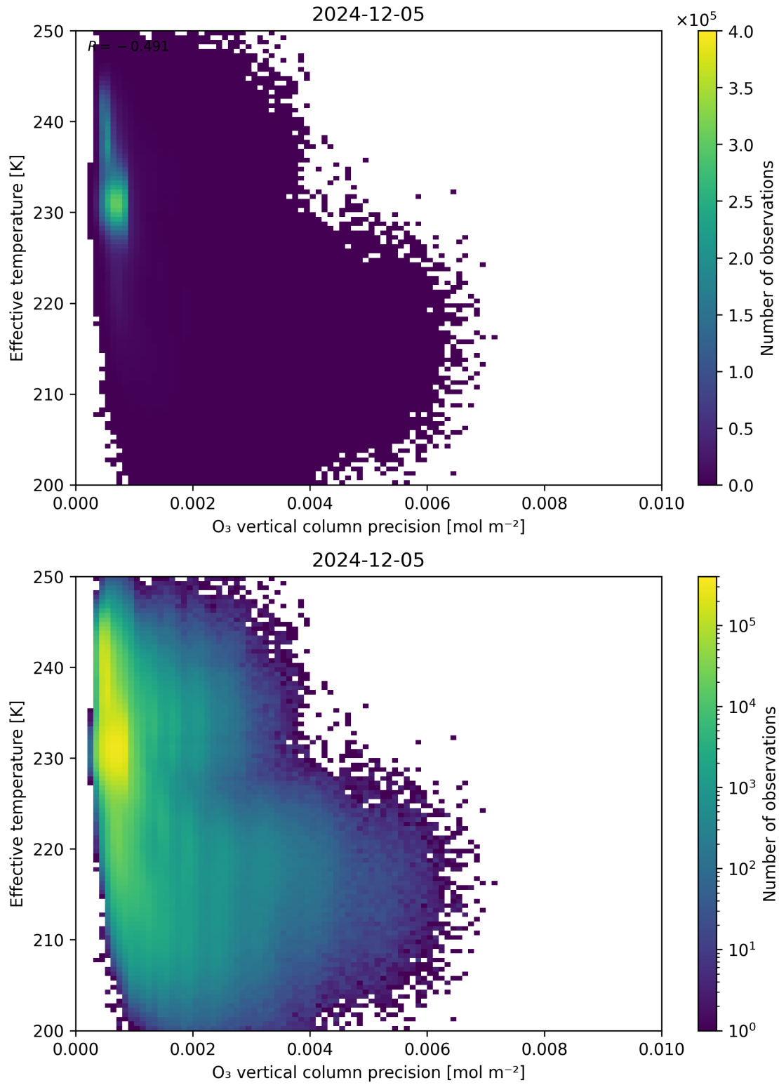
Figure 42: Scatter density plot of “O 3 vertical column precision” against “Effective temperature” for 2024-12-04 to 2024-12-06.
