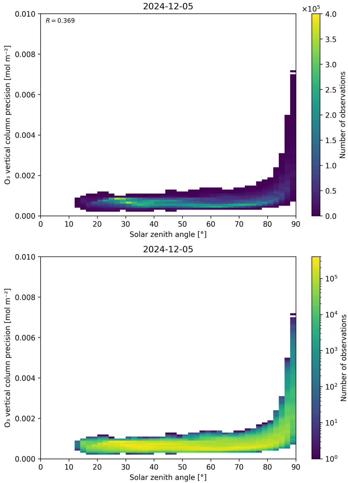
Figure 48: Scatter density plot of “Solar zenith angle” against “O 3 vertical column precision” for 2024-12-04 to 2024-12-06.
