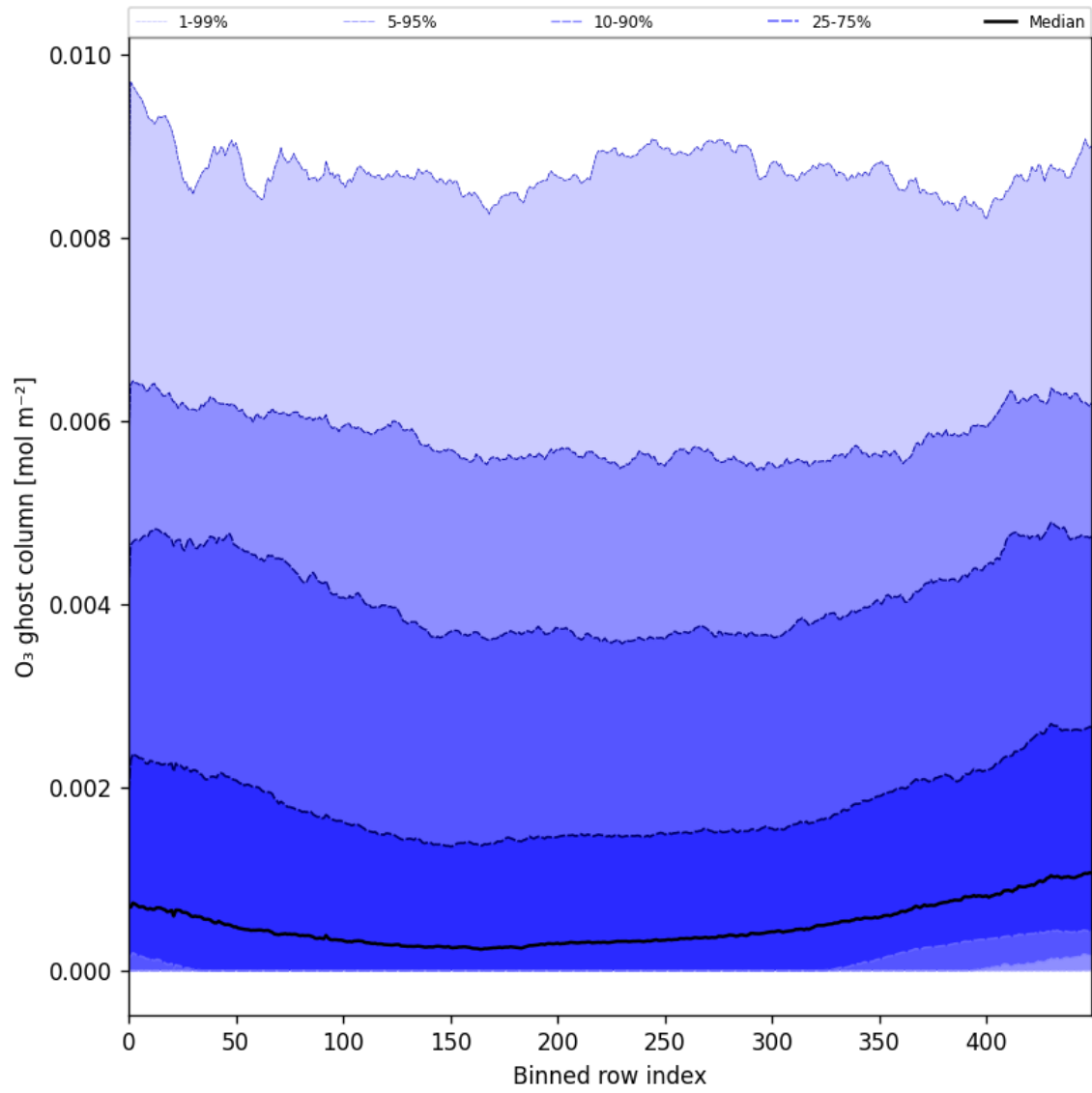
Figure 32: Along track statistics of “O 3 ghost column” for 2024-12-06 to 2024-12-07
