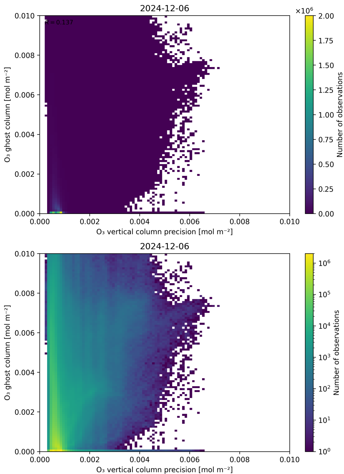
Figure 43: Scatter density plot of “O 3 vertical column precision” against “O 3 ghost column” for 2024-12-06 to 2024-12-07.
