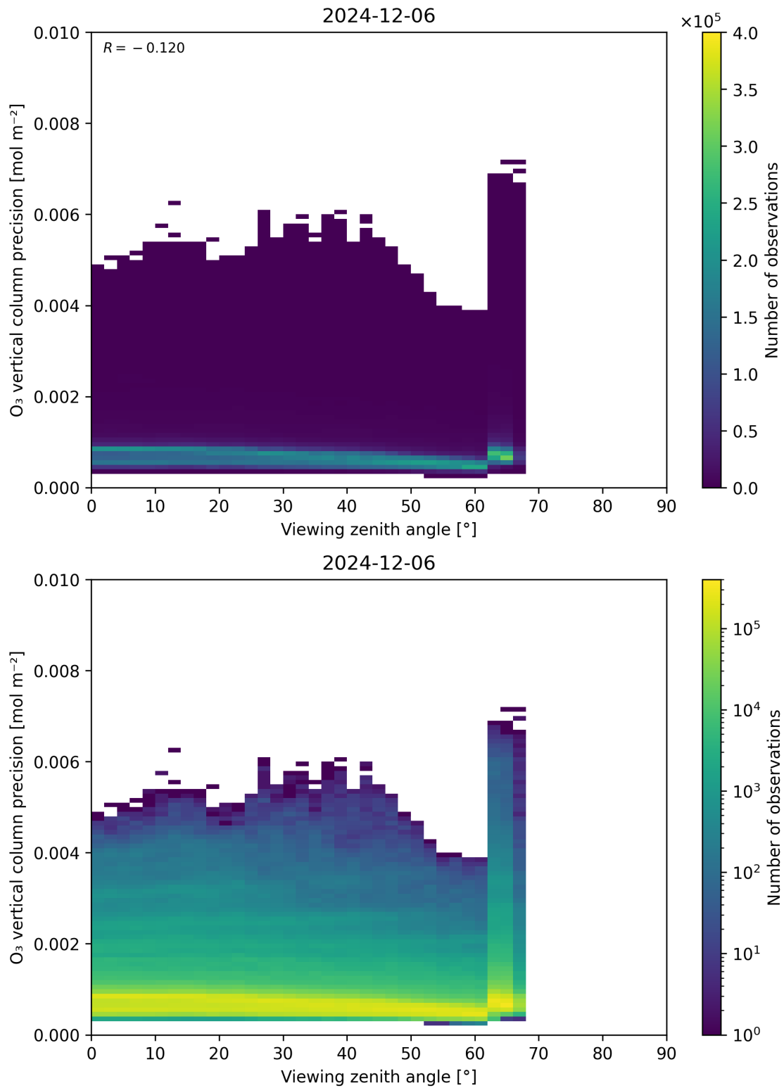
Figure 53: Scatter density plot of “Viewing zenith angle” against “O 3 vertical column precision” for 2024-12-06 to 2024-12-07.
