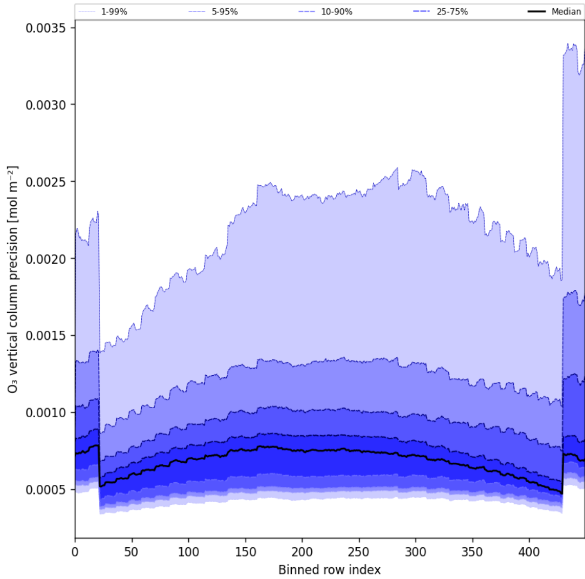
Figure 29: Along track statistics of “O 3 vertical column precision” for 2024-12-06 to 2024-12-07
