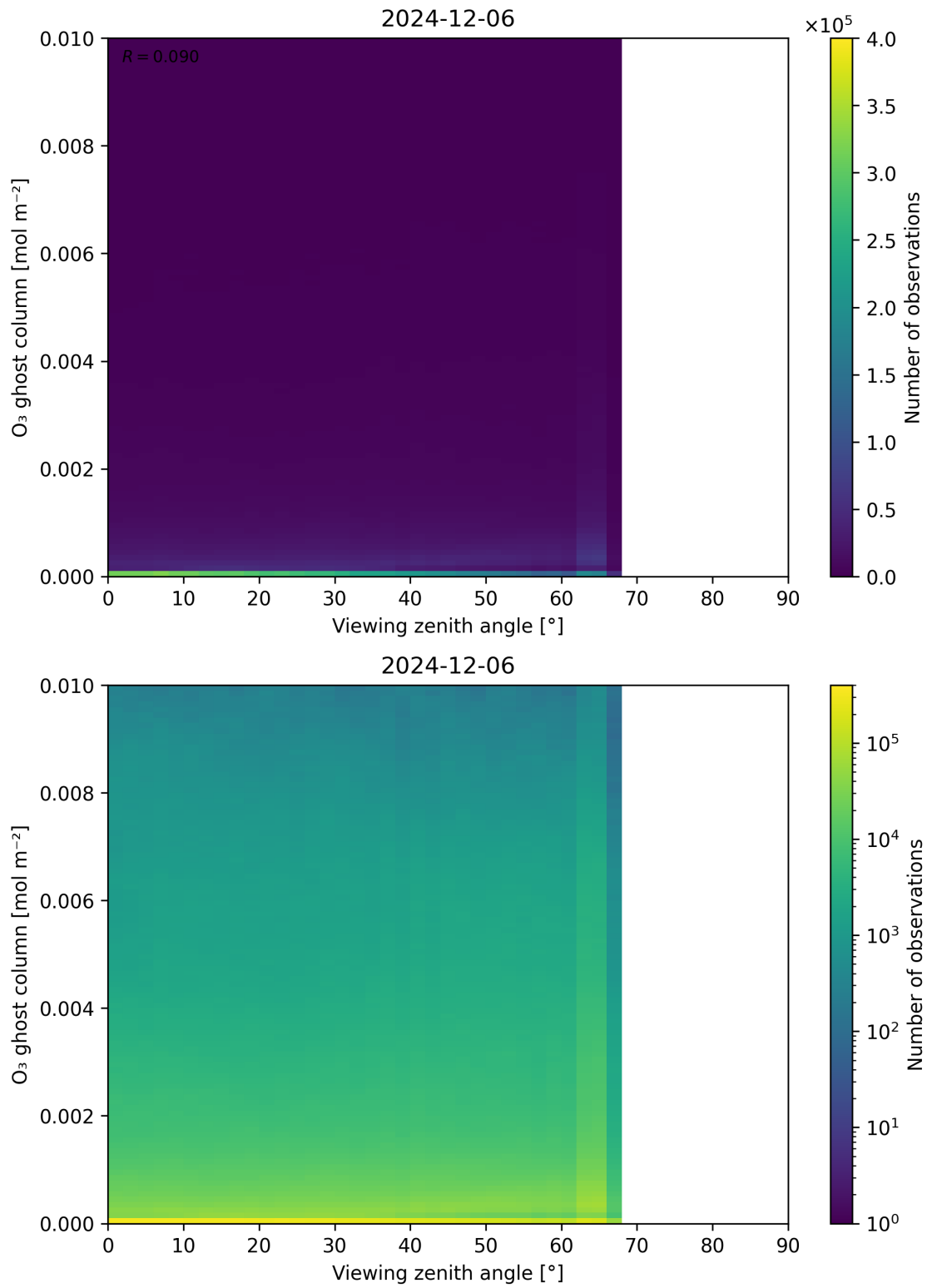
Figure 51: Scatter density plot of “Viewing zenith angle” against “O 3 ghost column” for 2024-12-06 to 2024-12-07.
