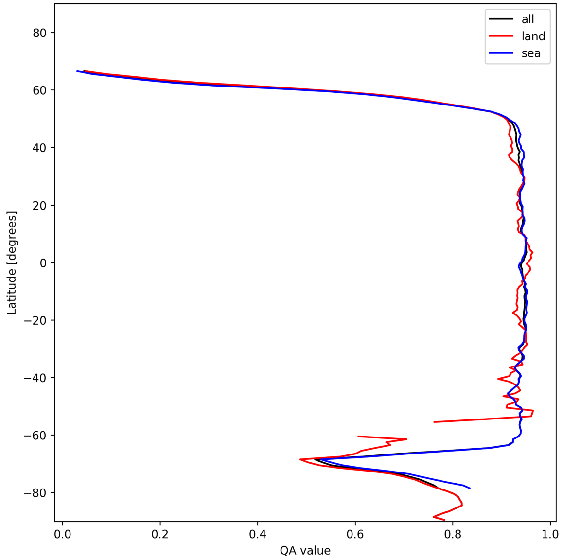
Figure 13: Zonal average of “QA value” for 2024-12-06 to 2024-12-07.
