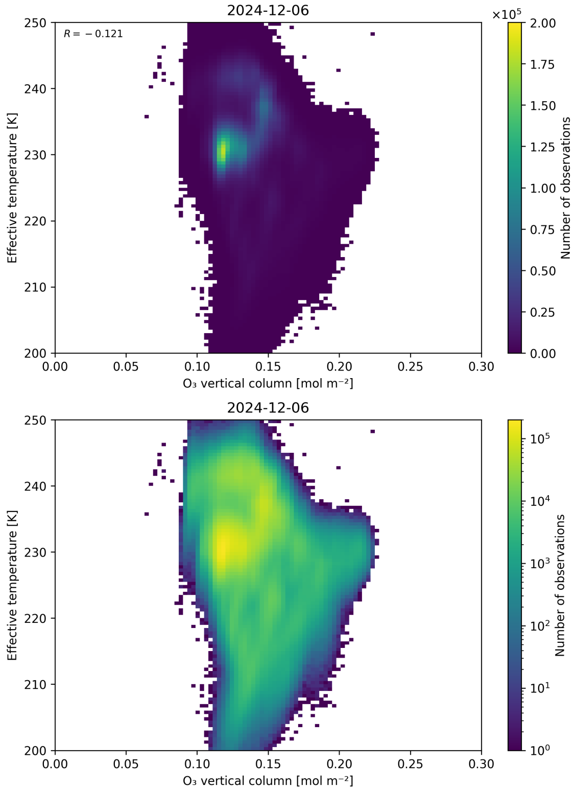
Figure 39: Scatter density plot of “O 3 vertical column” against “Effective temperature” for 2024-12-06 to 2024-12-07.
