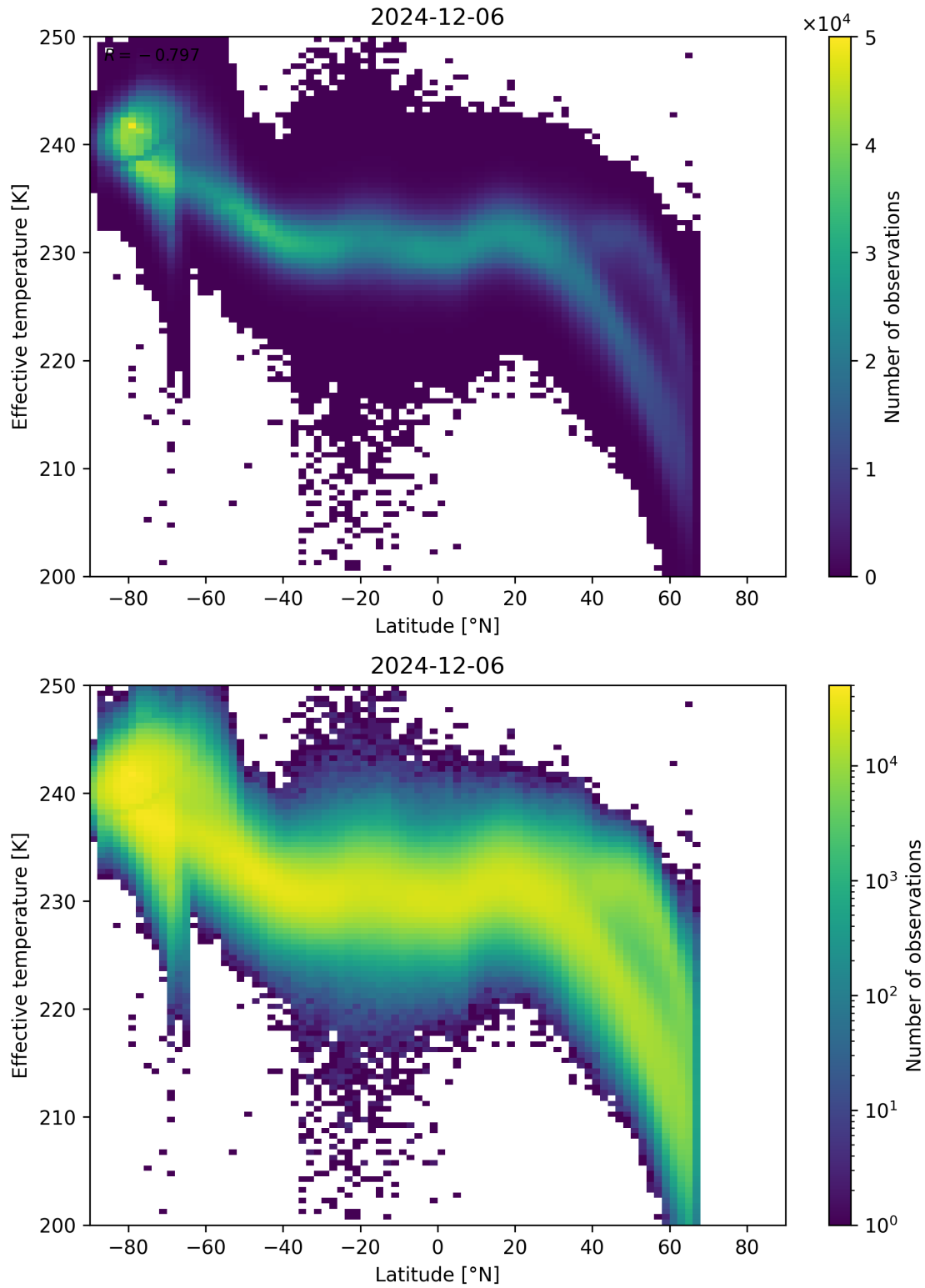
Figure 34: Scatter density plot of “Latitude” against “Effective temperature” for 2024-12-06 to 2024-12-07.
