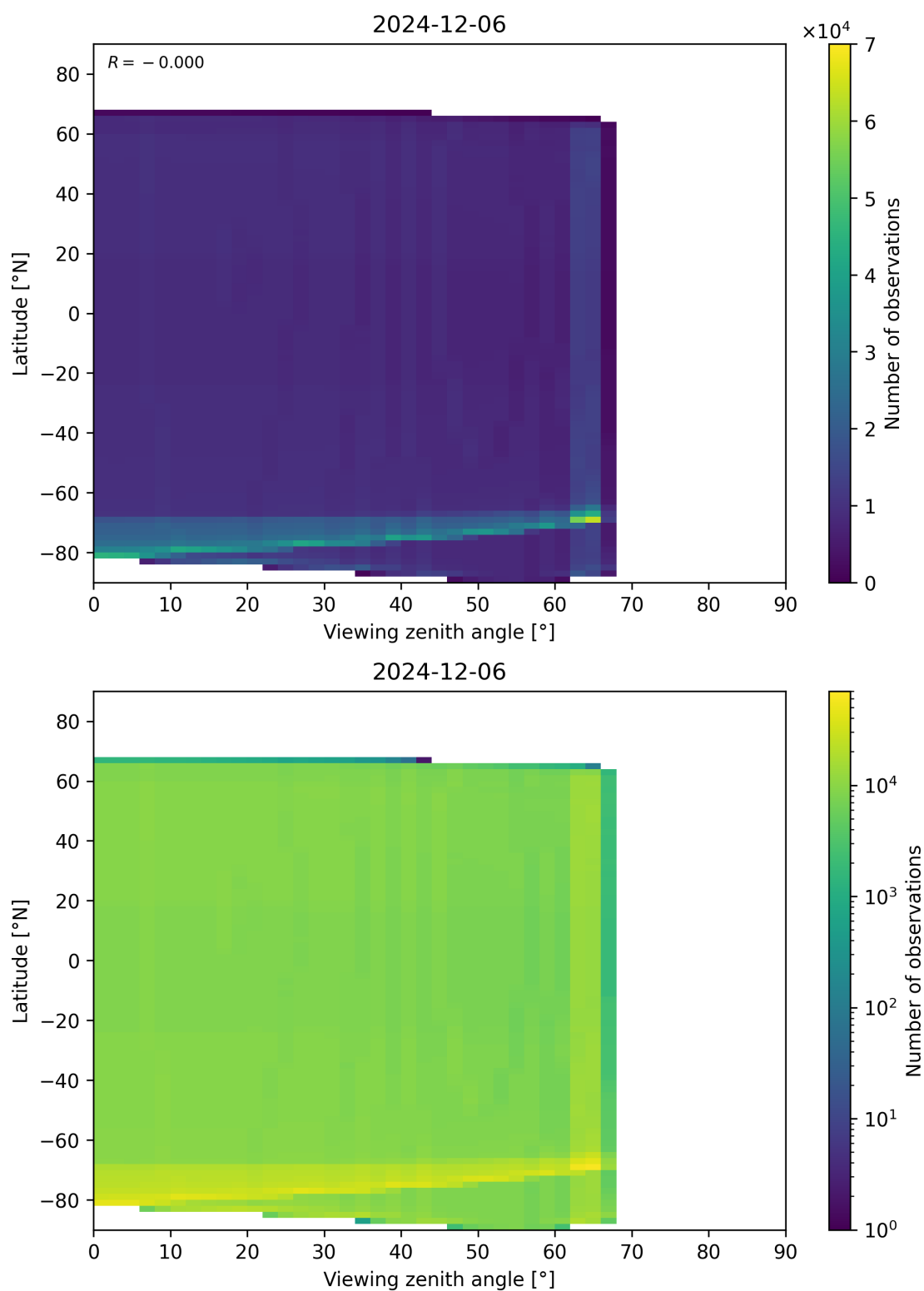
Figure 49: Scatter density plot of “Viewing zenith angle” against “Latitude” for 2024-12-06 to 2024-12-07.
