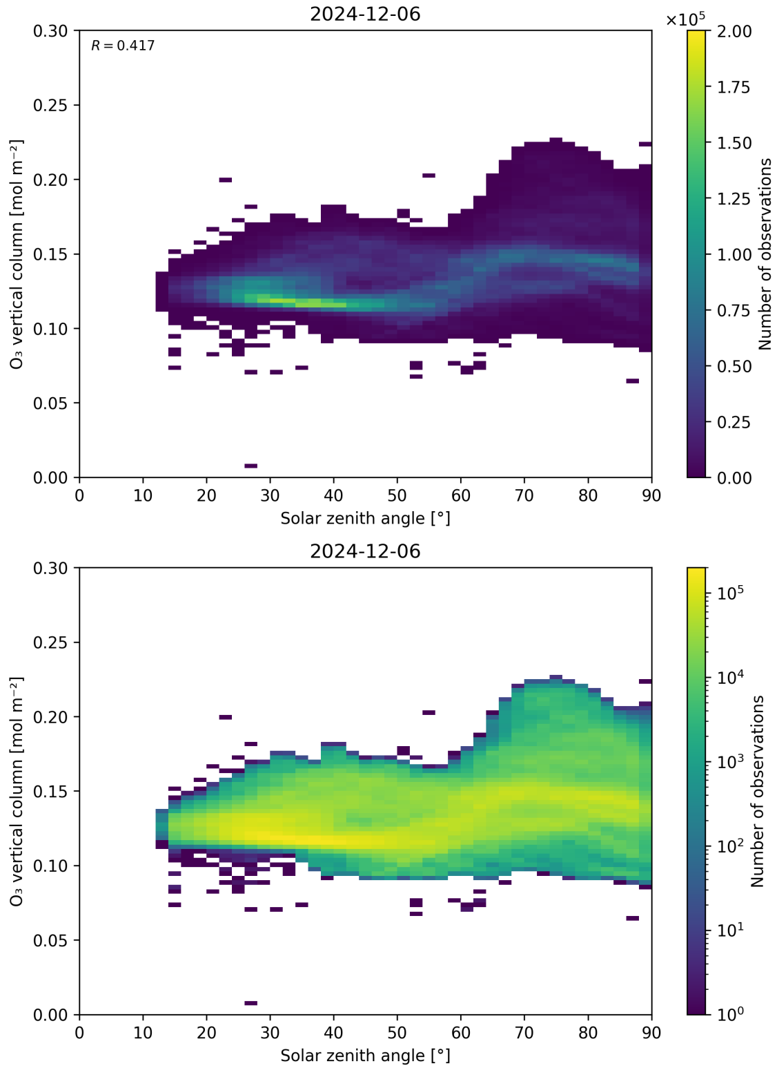
Figure 47: Scatter density plot of “Solar zenith angle” against “O 3 vertical column” for 2024-12-06 to 2024-12-07.
