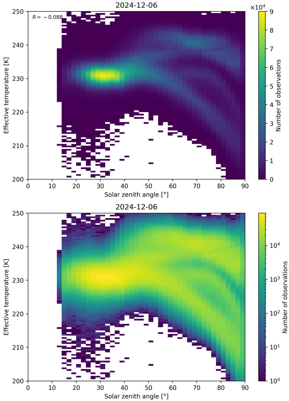
Figure 45: Scatter density plot of “Solar zenith angle” against “Effective temperature” for 2024-12-06 to 2024-12-07.
