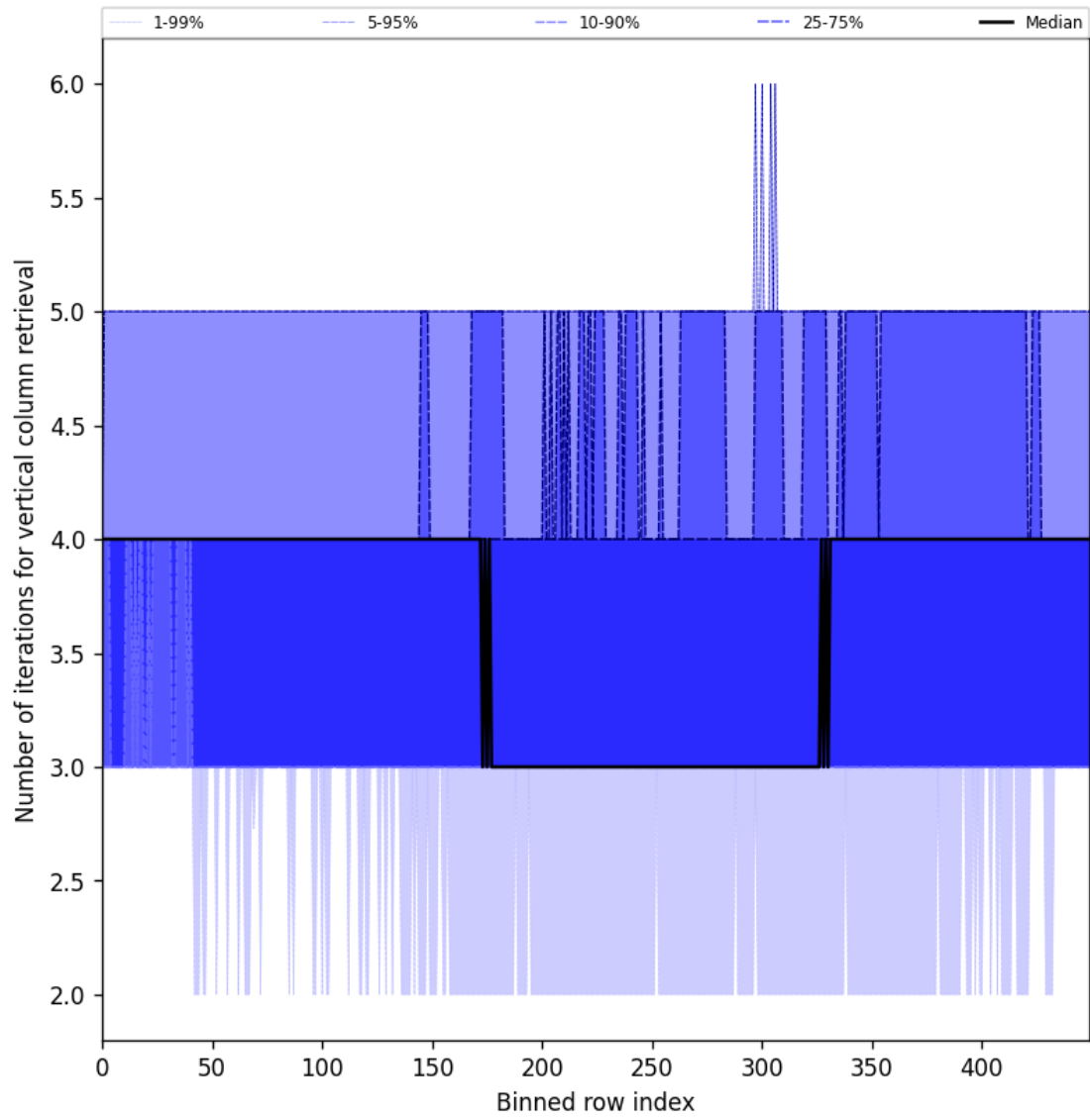
Figure 33: Along track statistics of “Number of iterations for vertical column retrieval” for 2024-12-06 to 2024-12-07
