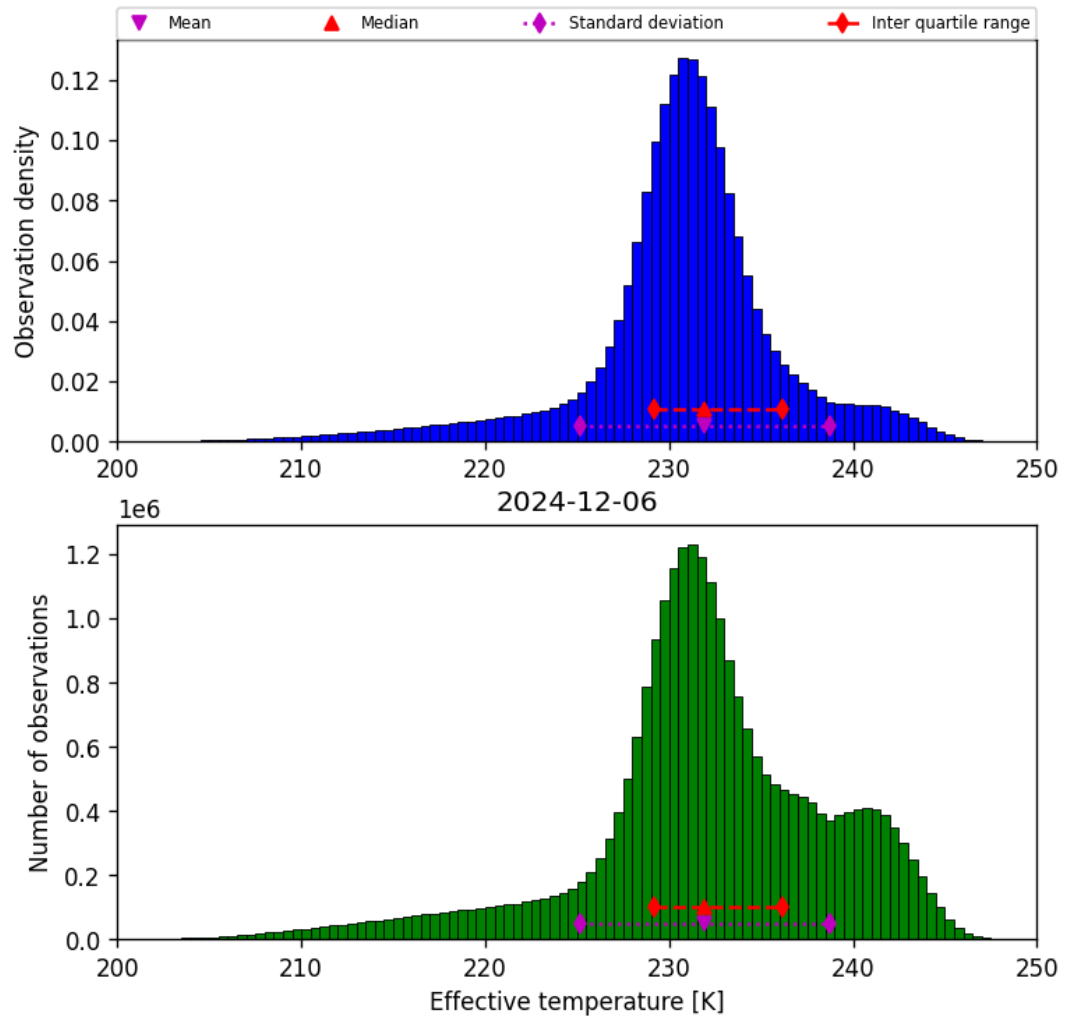
Figure 24: Histogram of “Effective temperature” for 2024-12-06 to 2024-12-07
