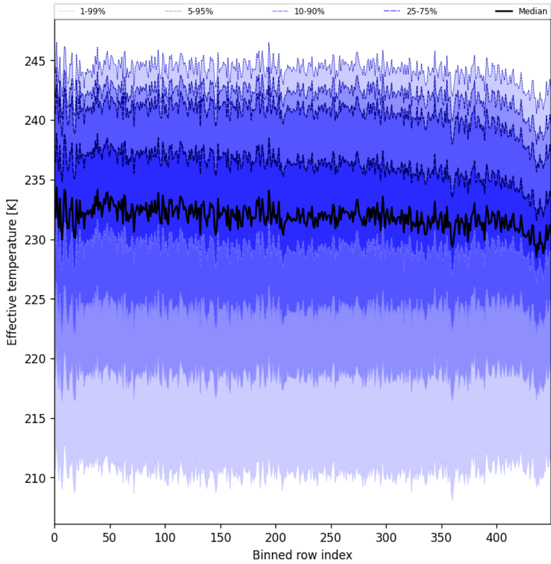
Figure 31: Along track statistics of “Effective temperature” for 2024-12-06 to 2024-12-07
