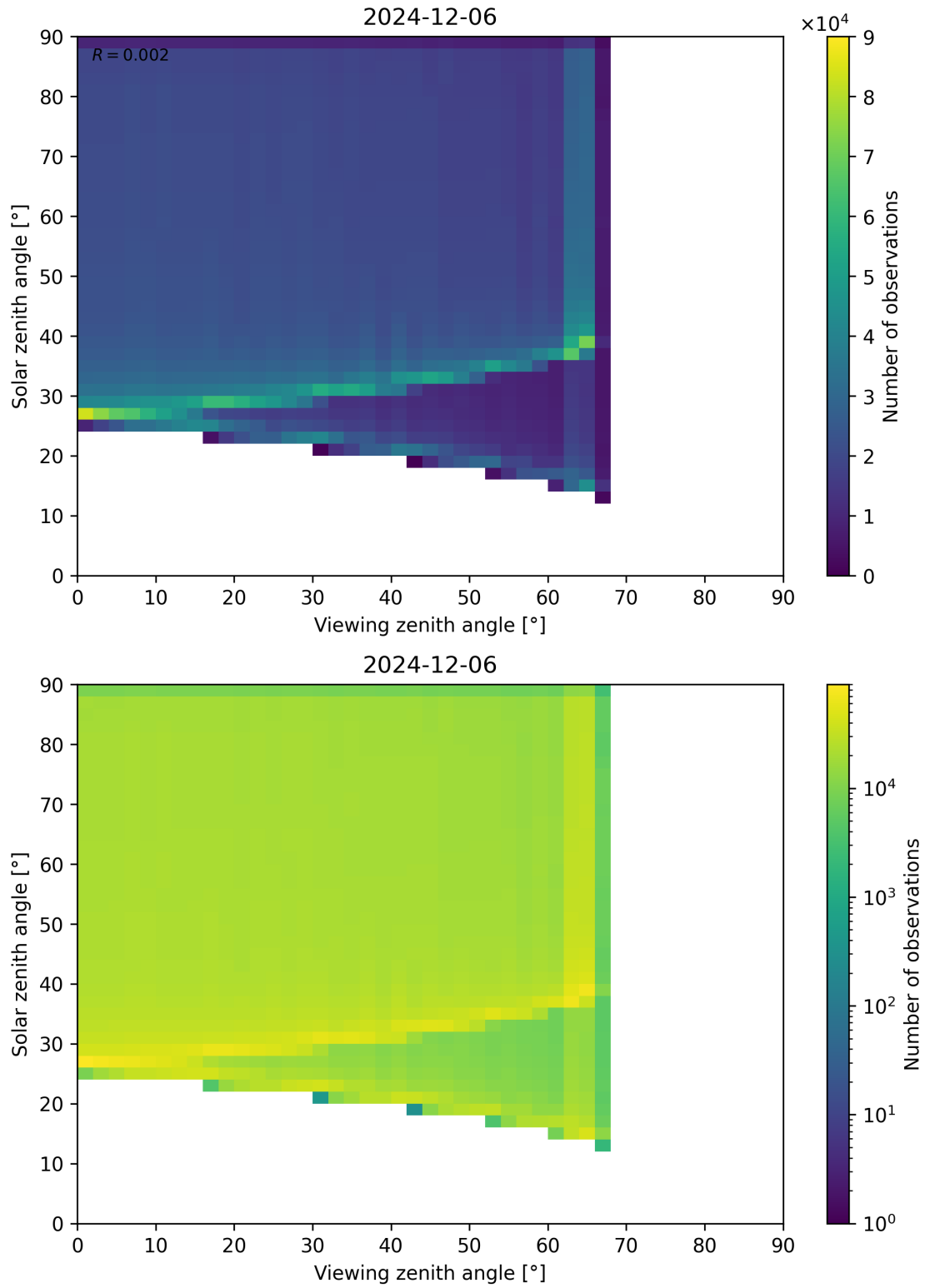
Figure 54: Scatter density plot of “Viewing zenith angle” against “Solar zenith angle” for 2024-12-06 to 2024-12-07.
