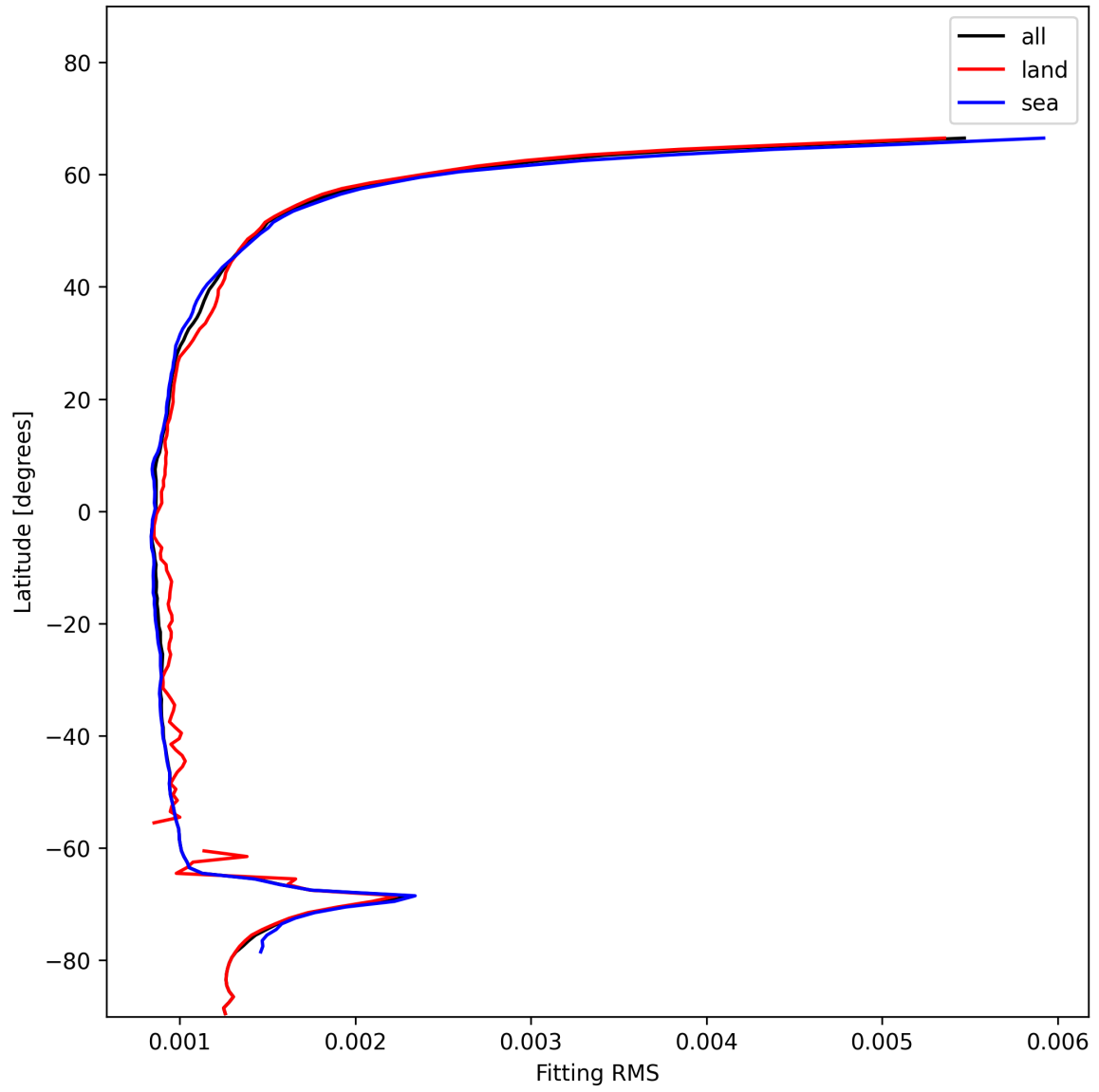
Figure 16: Zonal average of “Fitting RMS” for 2024-12-06 to 2024-12-07.
