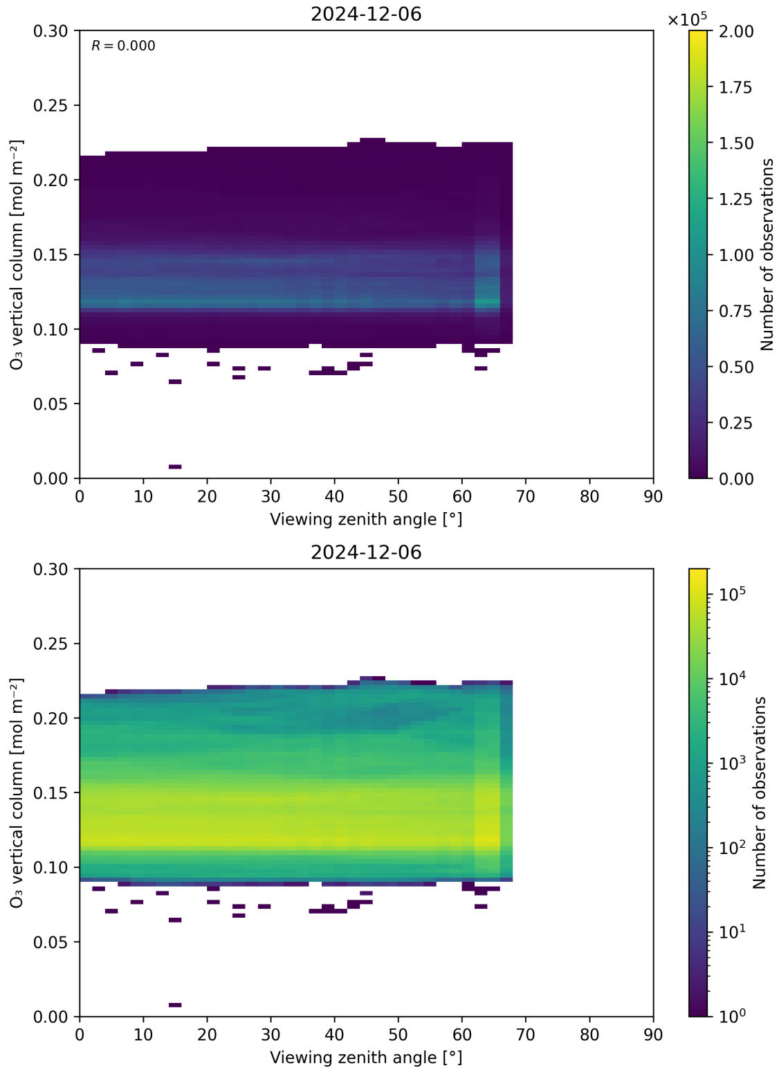
Figure 52: Scatter density plot of “Viewing zenith angle” against “O 3 vertical column” for 2024-12-06 to 2024-12-07.
