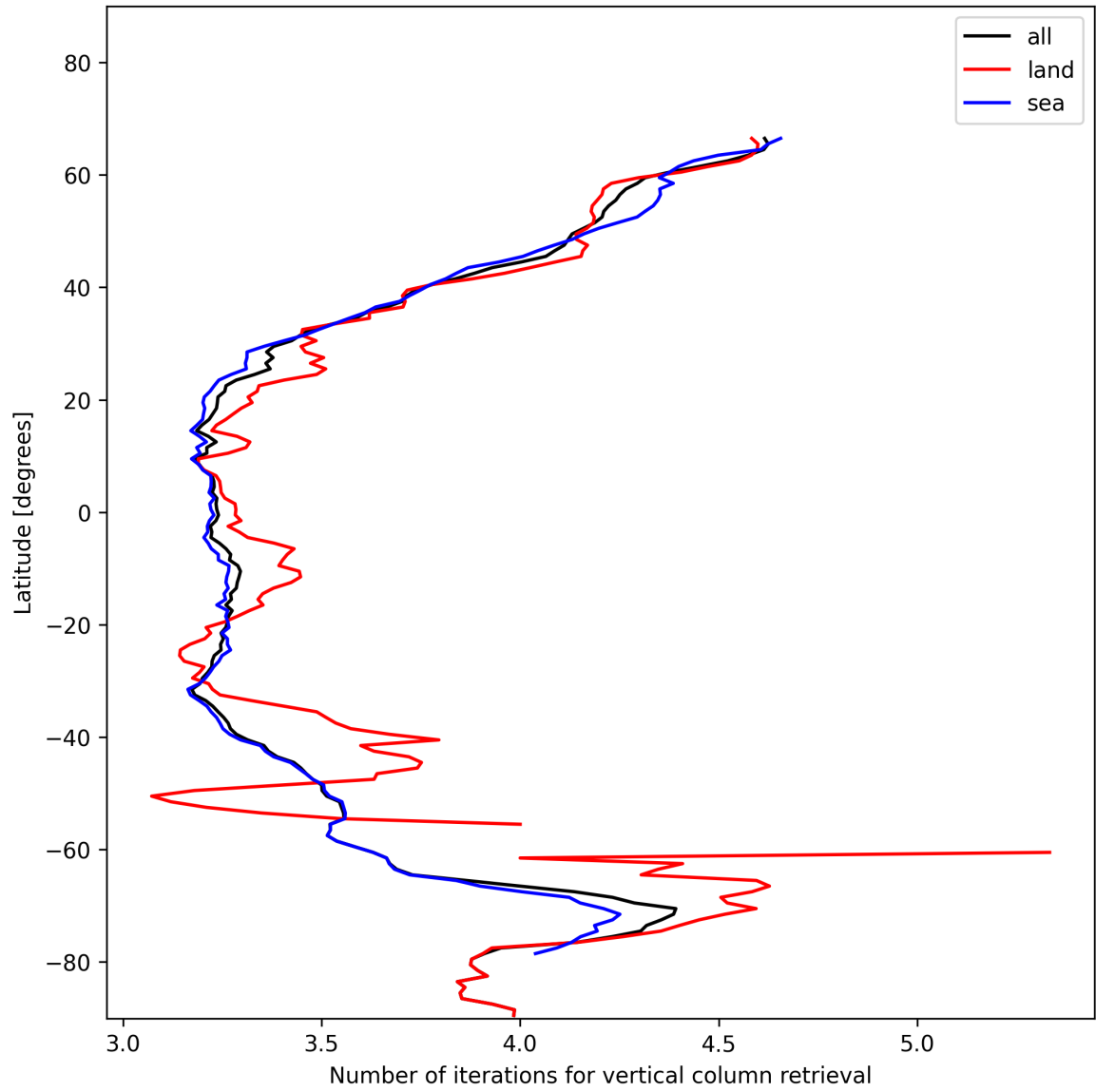
Figure 19: Zonal average of “Number of iterations for vertical column retrieval” for 2024-12-06 to 2024-12-07.
