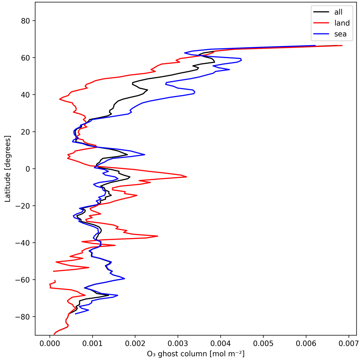
Figure 18: Zonal average of “O 3 ghost column” for 2024-12-06 to 2024-12-07.
