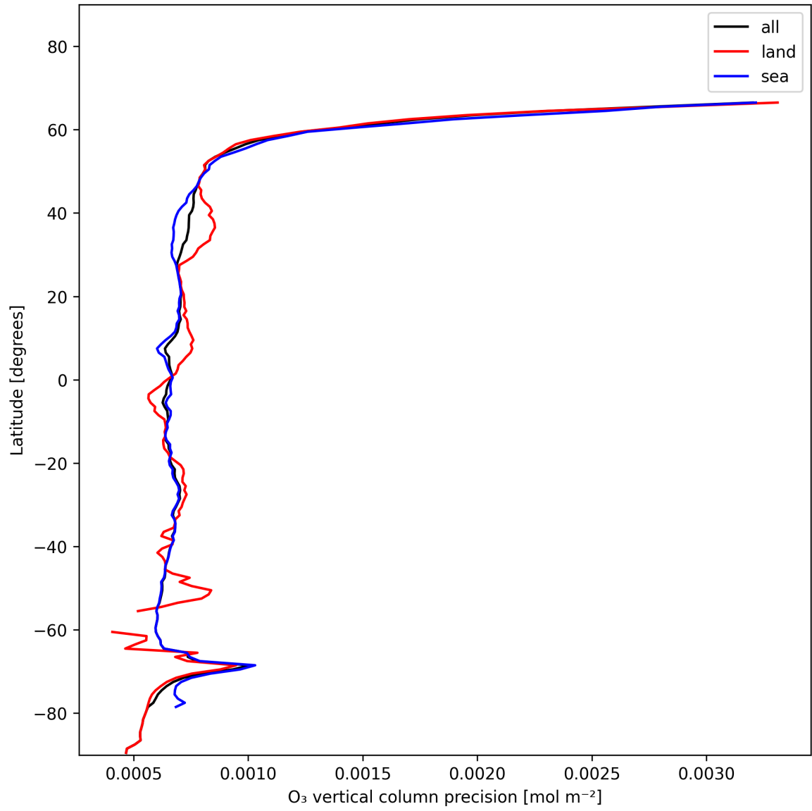
Figure 15: Zonal average of “O 3 vertical column precision” for 2024-12-06 to 2024-12-07.
