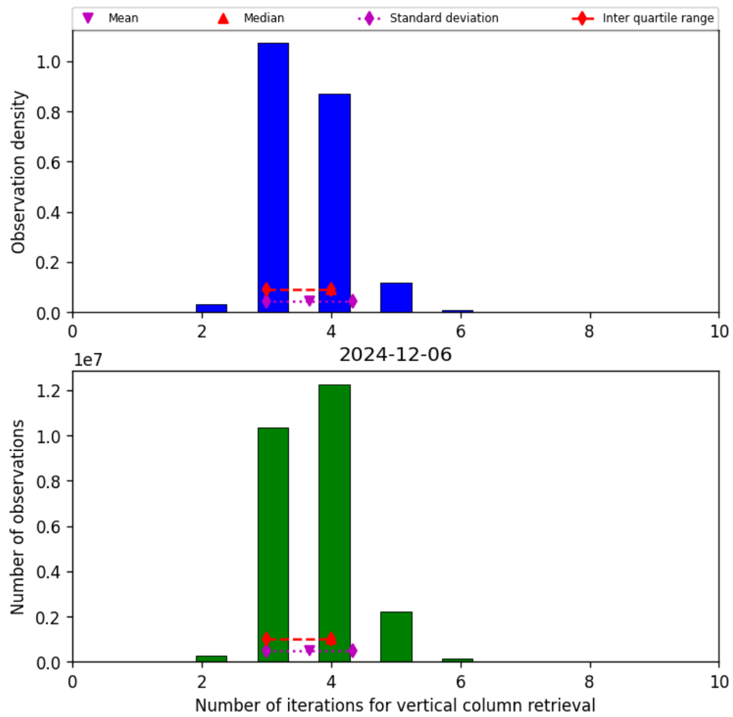
Figure 26: Histogram of “Number of iterations for vertical column retrieval” for 2024-12-06 to 2024-12-07
