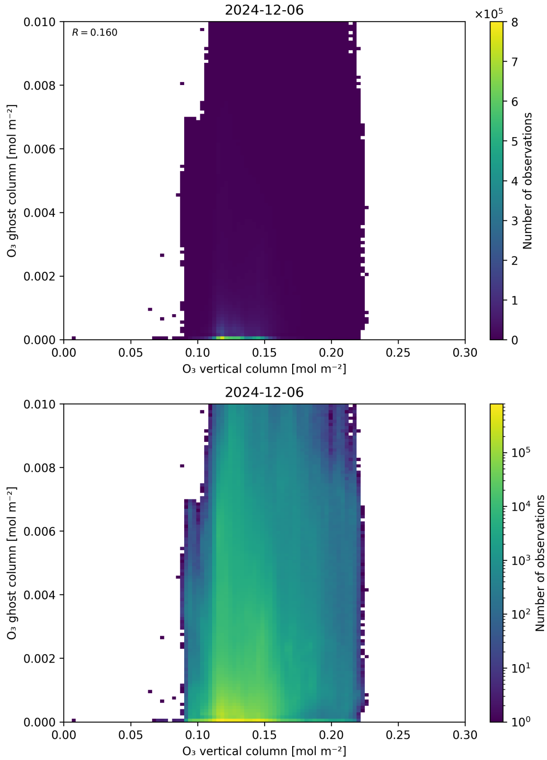
Figure 40: Scatter density plot of “O 3 vertical column” against “O 3 ghost column” for 2024-12-06 to 2024-12-07.
