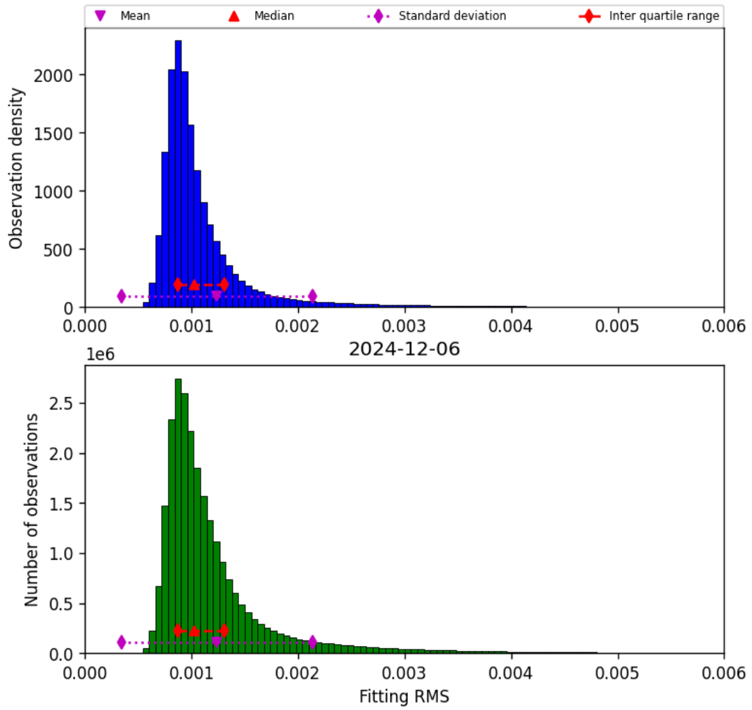
Figure 23: Histogram of “Fitting RMS” for 2024-12-06 to 2024-12-07
