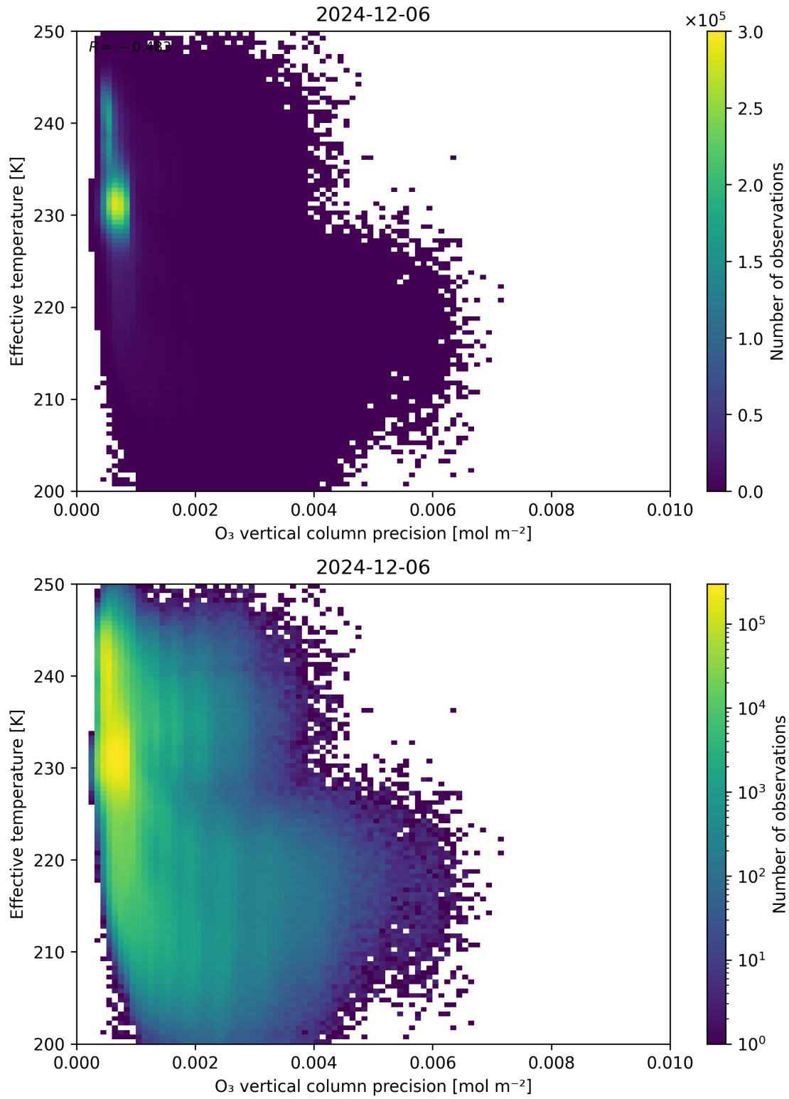
Figure 42: Scatter density plot of “O 3 vertical column precision” against “Effective temperature” for 2024-12-06 to 2024-12-07.
