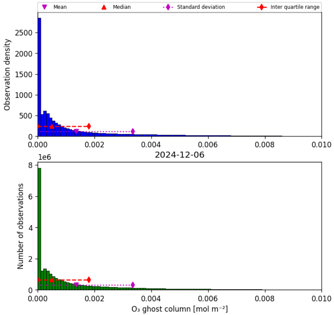
Figure 25: Histogram of “O 3 ghost column” for 2024-12-06 to 2024-12-07
