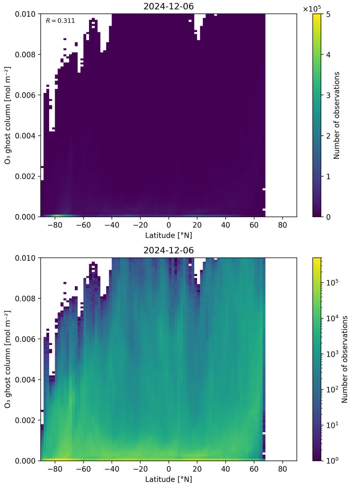
Figure 35: Scatter density plot of “Latitude” against “O 3 ghost column” for 2024-12-06 to 2024-12-07.
