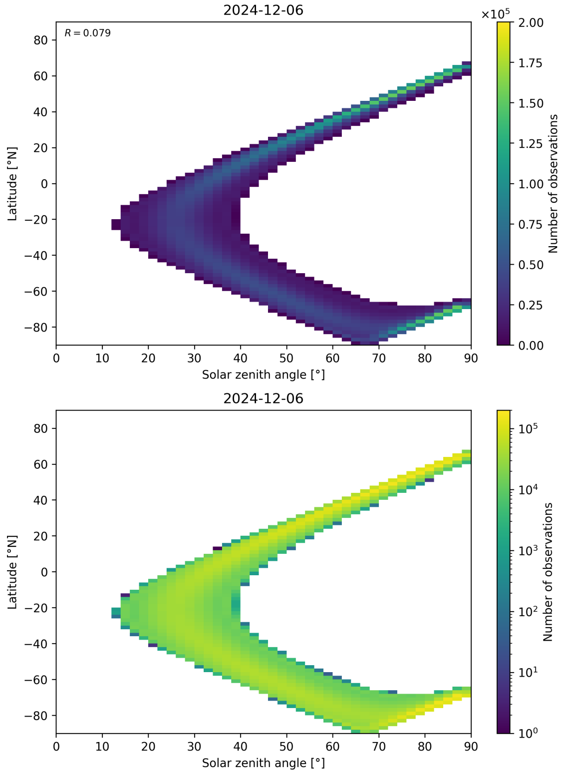
Figure 44: Scatter density plot of “Solar zenith angle” against “Latitude” for 2024-12-06 to 2024-12-07.
