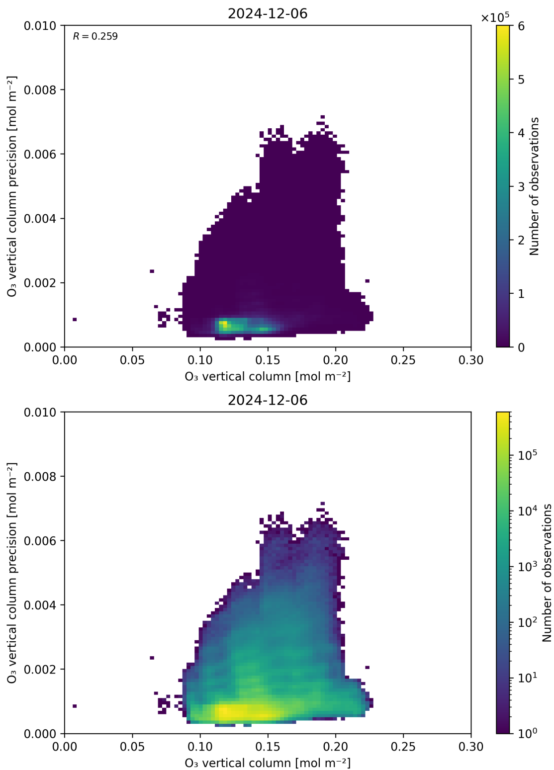
Figure 41: Scatter density plot of “O 3 vertical column” against “O 3 vertical column precision” for 2024-12-06 to 2024-12-07.
