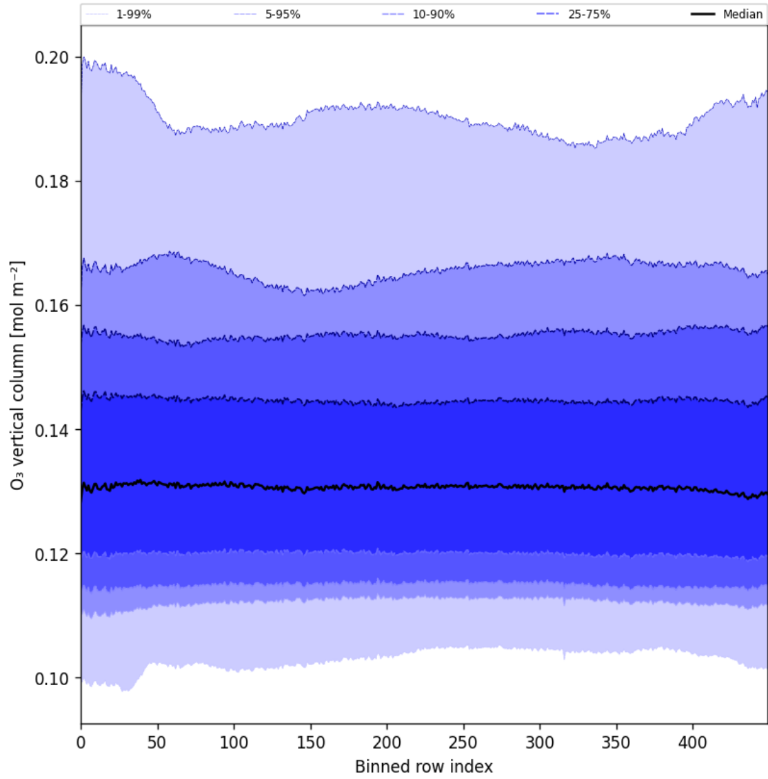
Figure 28: Along track statistics of “O 3 vertical column” for 2024-12-06 to 2024-12-07
