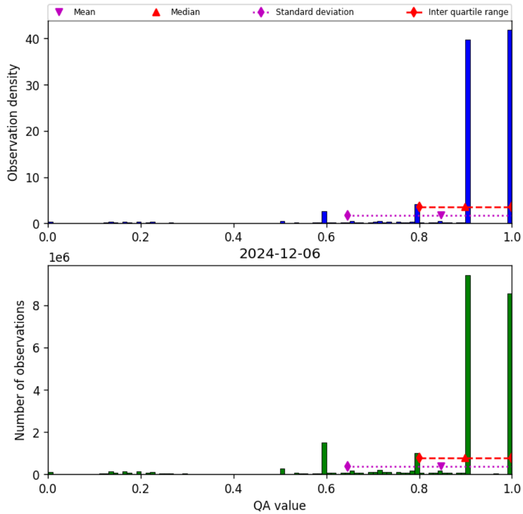
Figure 20: Histogram of “QA value” for 2024-12-06 to 2024-12-07
