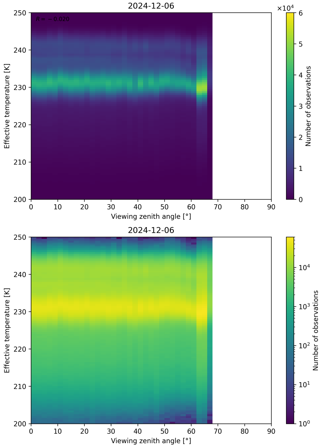
Figure 50: Scatter density plot of “Viewing zenith angle” against “Effective temperature” for 2024-12-06 to 2024-12-07.
