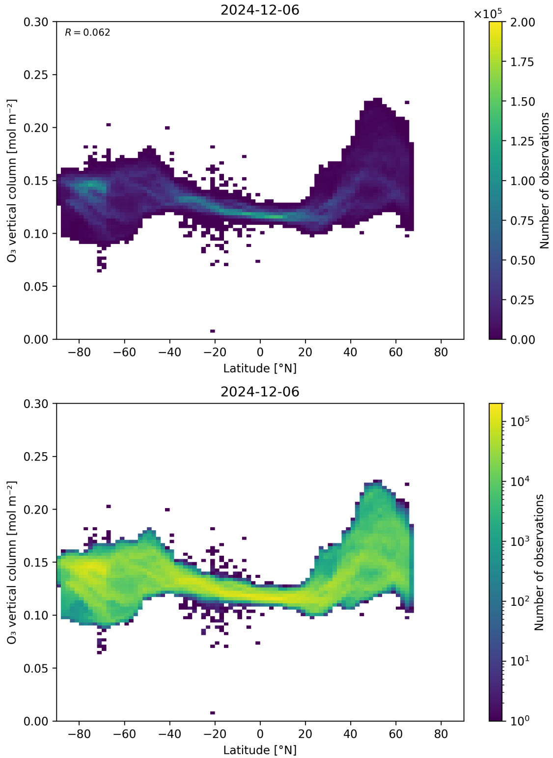
Figure 36: Scatter density plot of “Latitude” against “O 3 vertical column” for 2024-12-06 to 2024-12-07.
