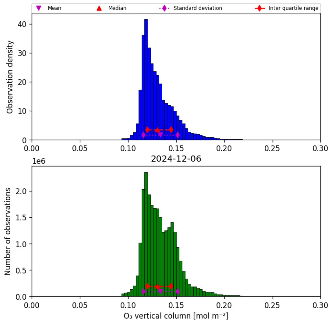
Figure 21: Histogram of “O 3 vertical column” for 2024-12-06 to 2024-12-07
