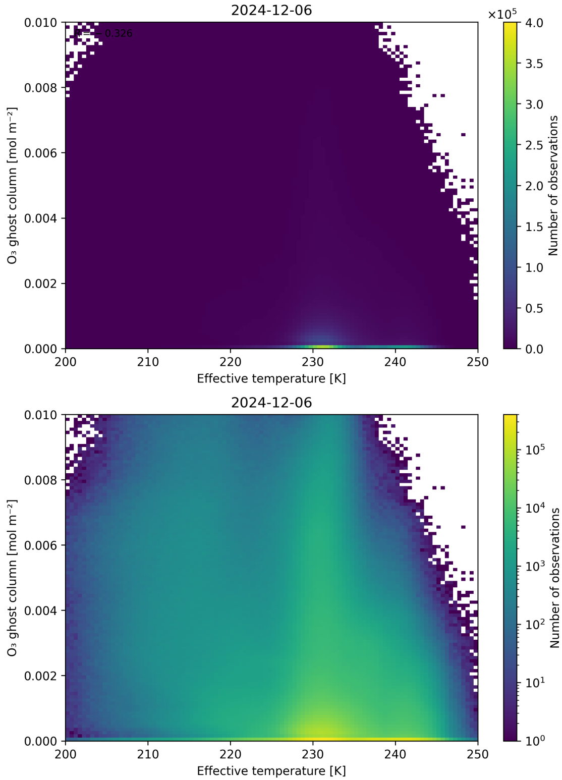
Figure 38: Scatter density plot of “Effective temperature” against “O 3 ghost column” for 2024-12-06 to 2024-12-07.
