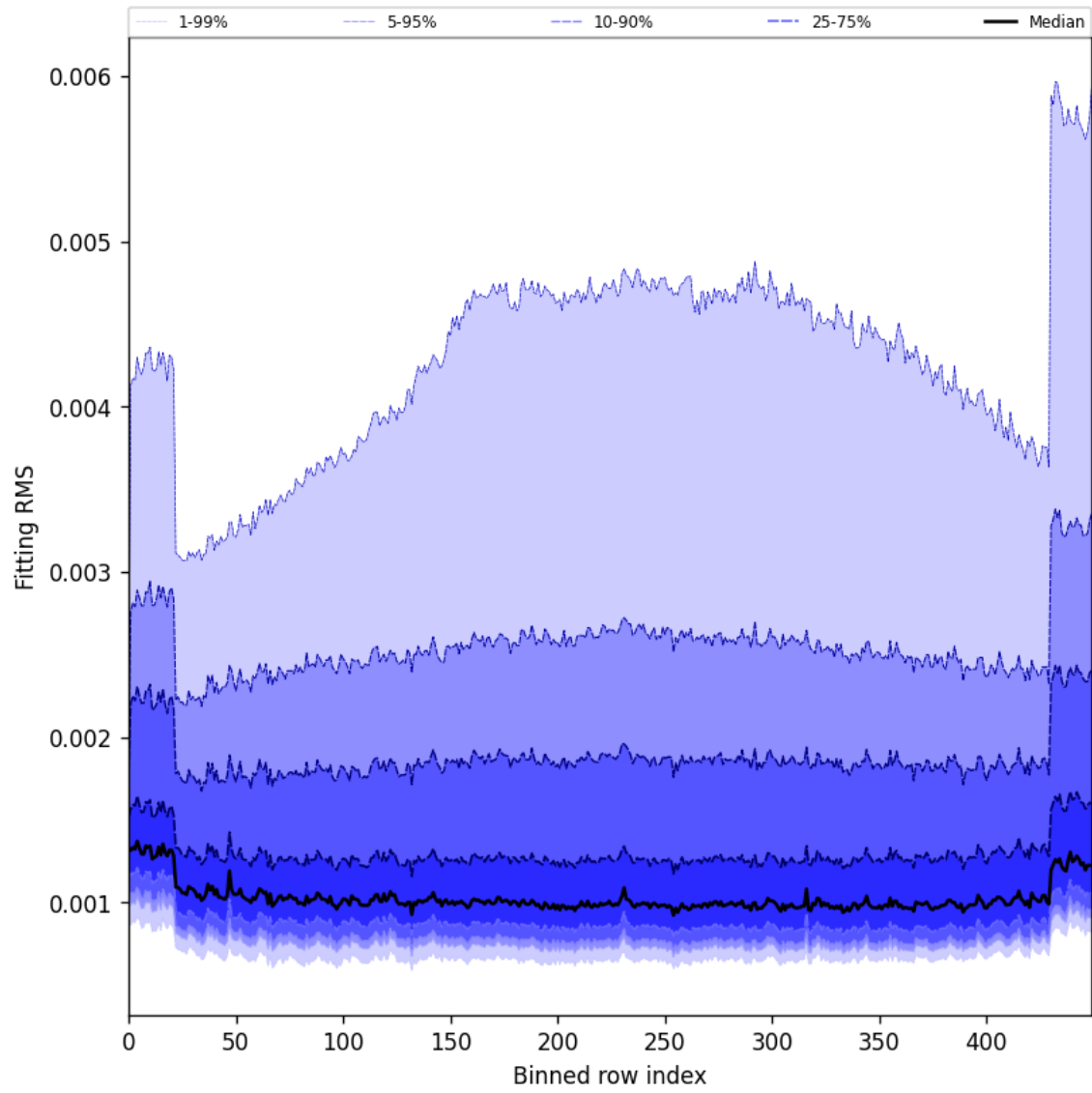
Figure 30: Along track statistics of “Fitting RMS” for 2024-12-06 to 2024-12-07
