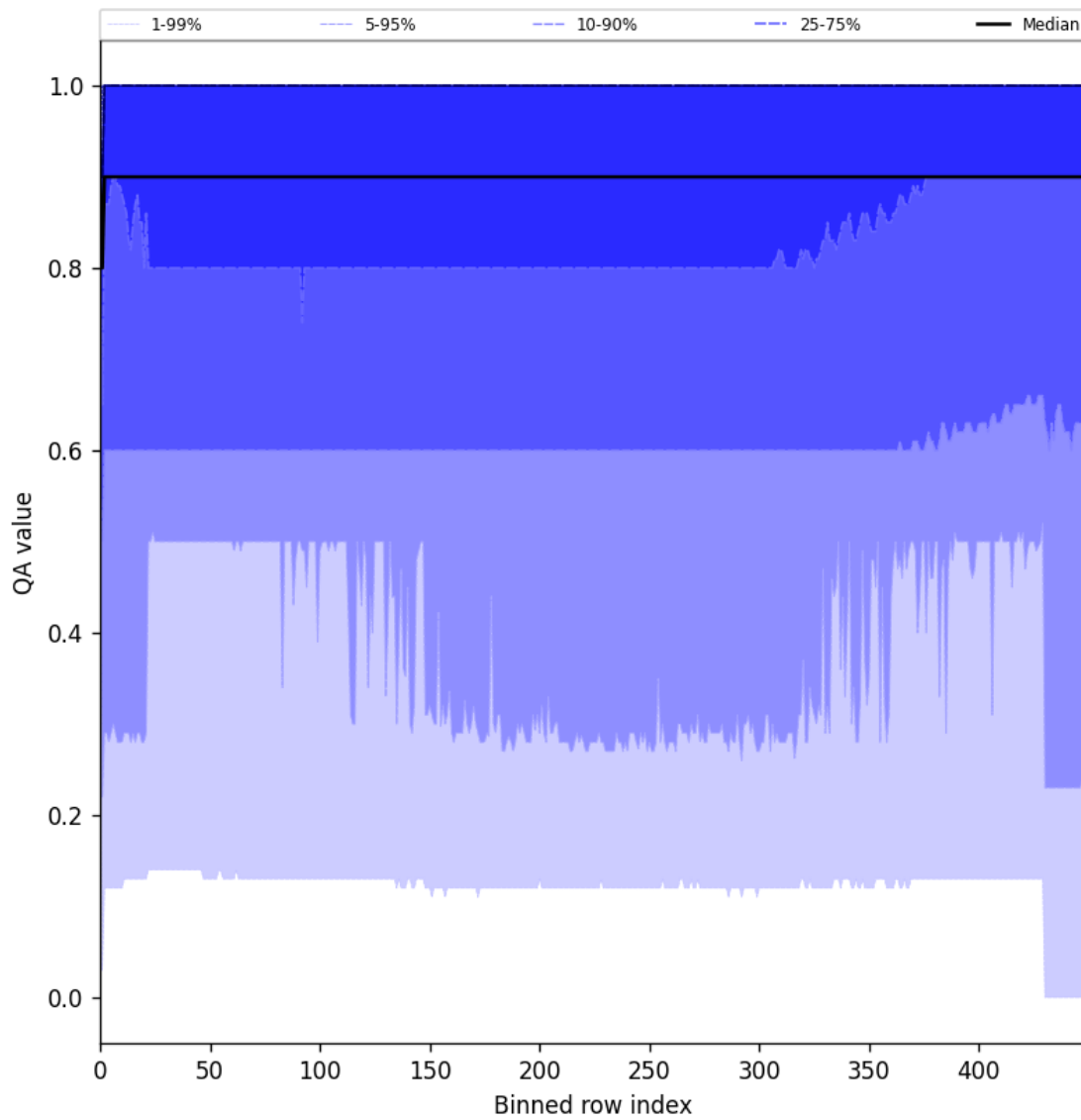
Figure 27: Along track statistics of “QA value” for 2024-12-06 to 2024-12-07
