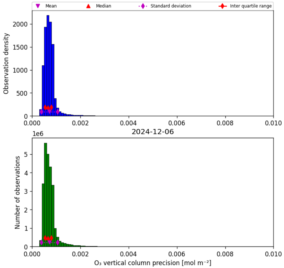
Figure 22: Histogram of “O 3 vertical column precision” for 2024-12-06 to 2024-12-07
