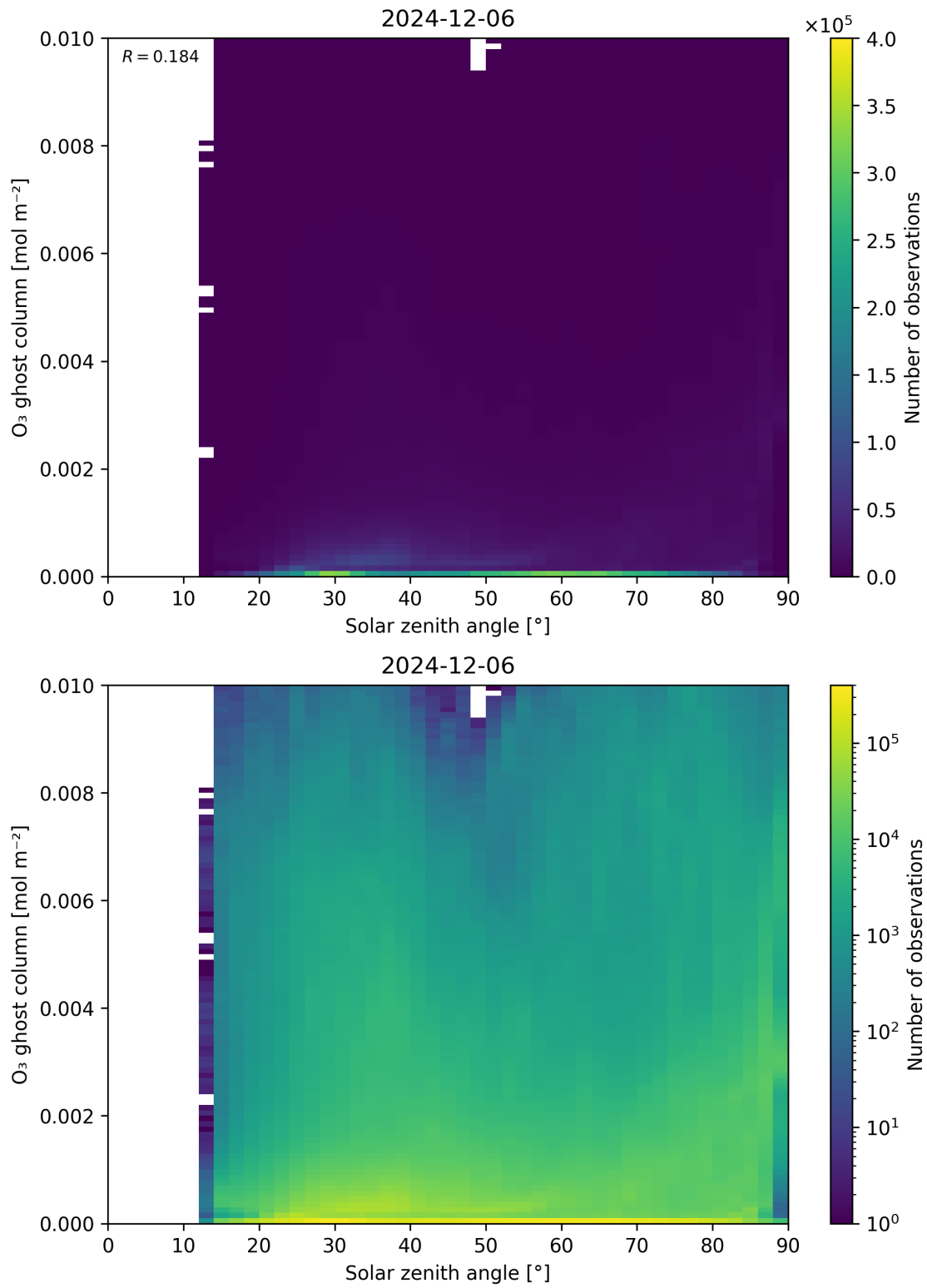
Figure 46: Scatter density plot of “Solar zenith angle” against “O 3 ghost column” for 2024-12-06 to 2024-12-07.
