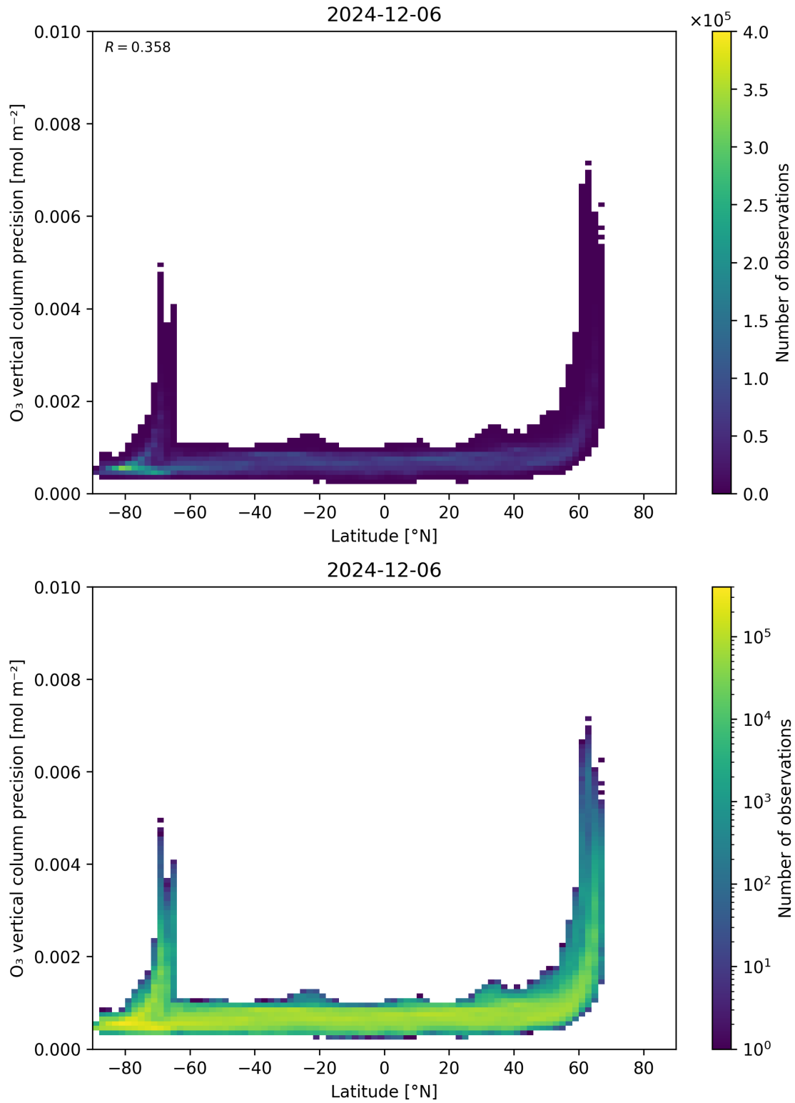
Figure 37: Scatter density plot of “Latitude” against “O 3 vertical column precision” for 2024-12-06 to 2024-12-07.
