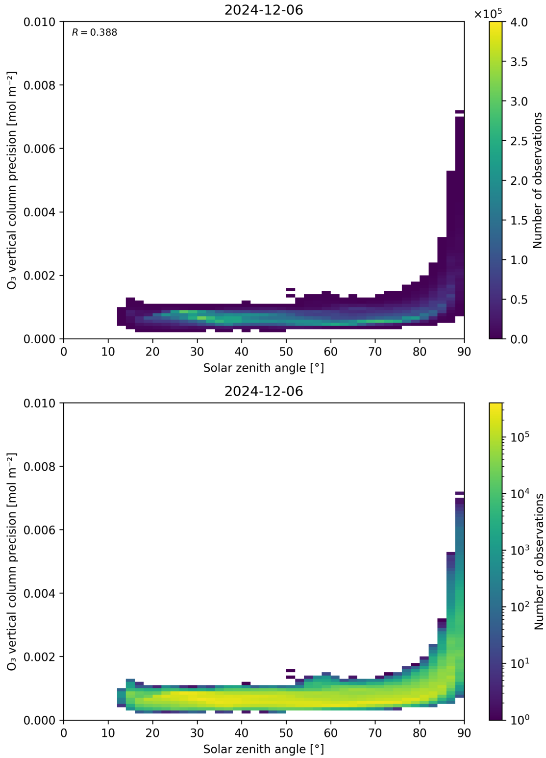
Figure 48: Scatter density plot of “Solar zenith angle” against “O 3 vertical column precision” for 2024-12-06 to 2024-12-07.
