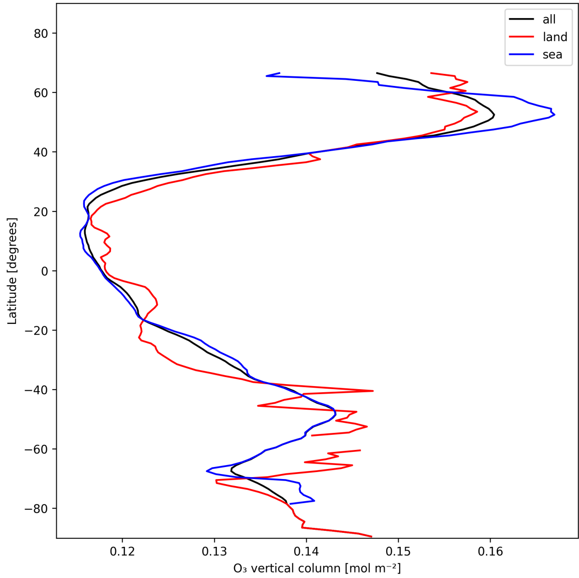
Figure 14: Zonal average of “O 3 vertical column” for 2024-12-06 to 2024-12-07.
