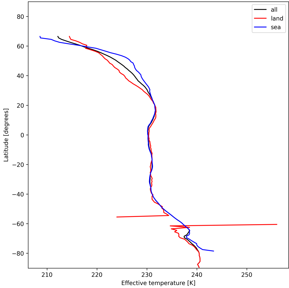
Figure 17: Zonal average of “Effective temperature” for 2024-12-06 to 2024-12-07.
