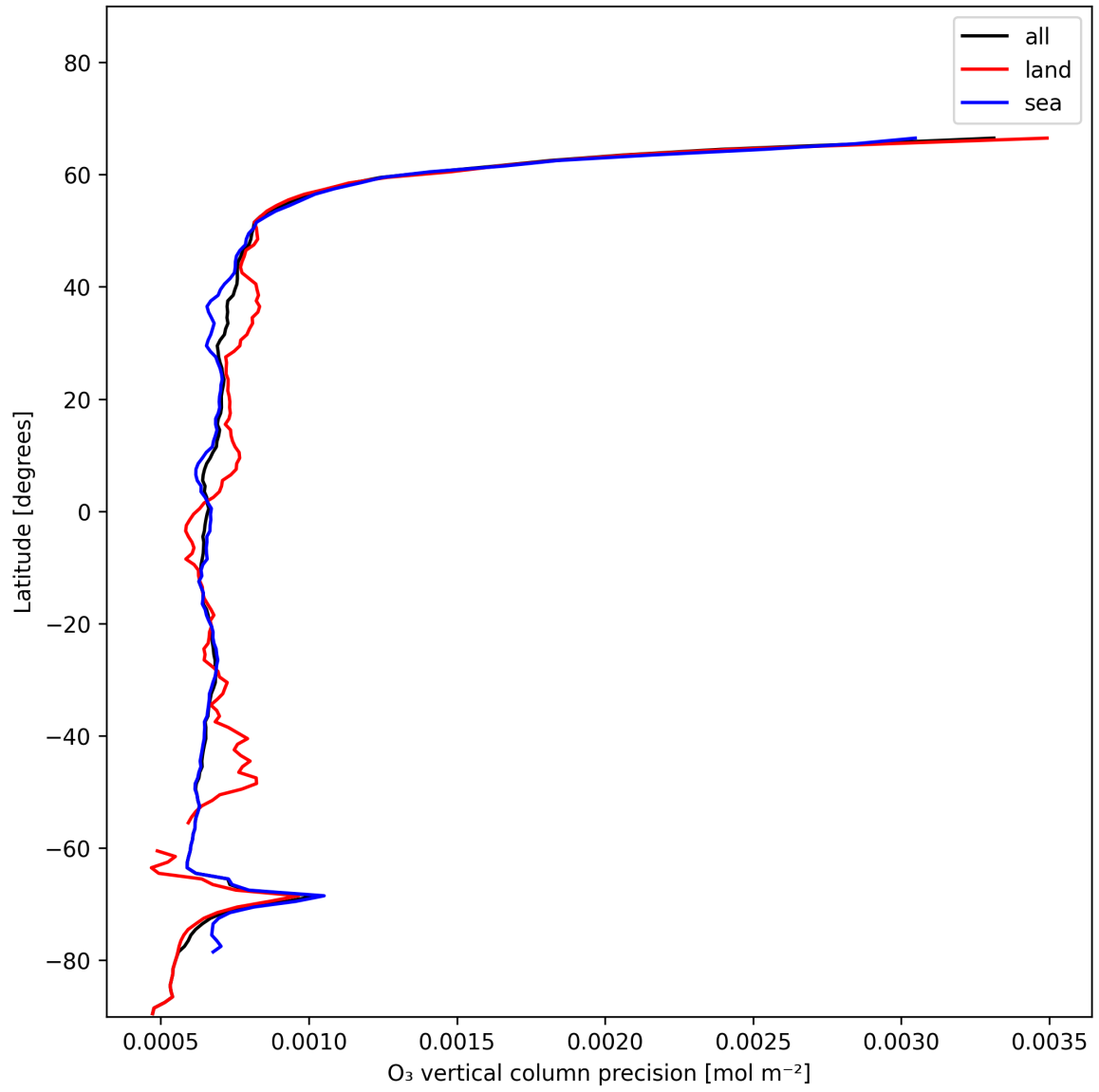
Figure 15: Zonal average of “O 3 vertical column precision” for 2024-12-06 to 2024-12-08.
