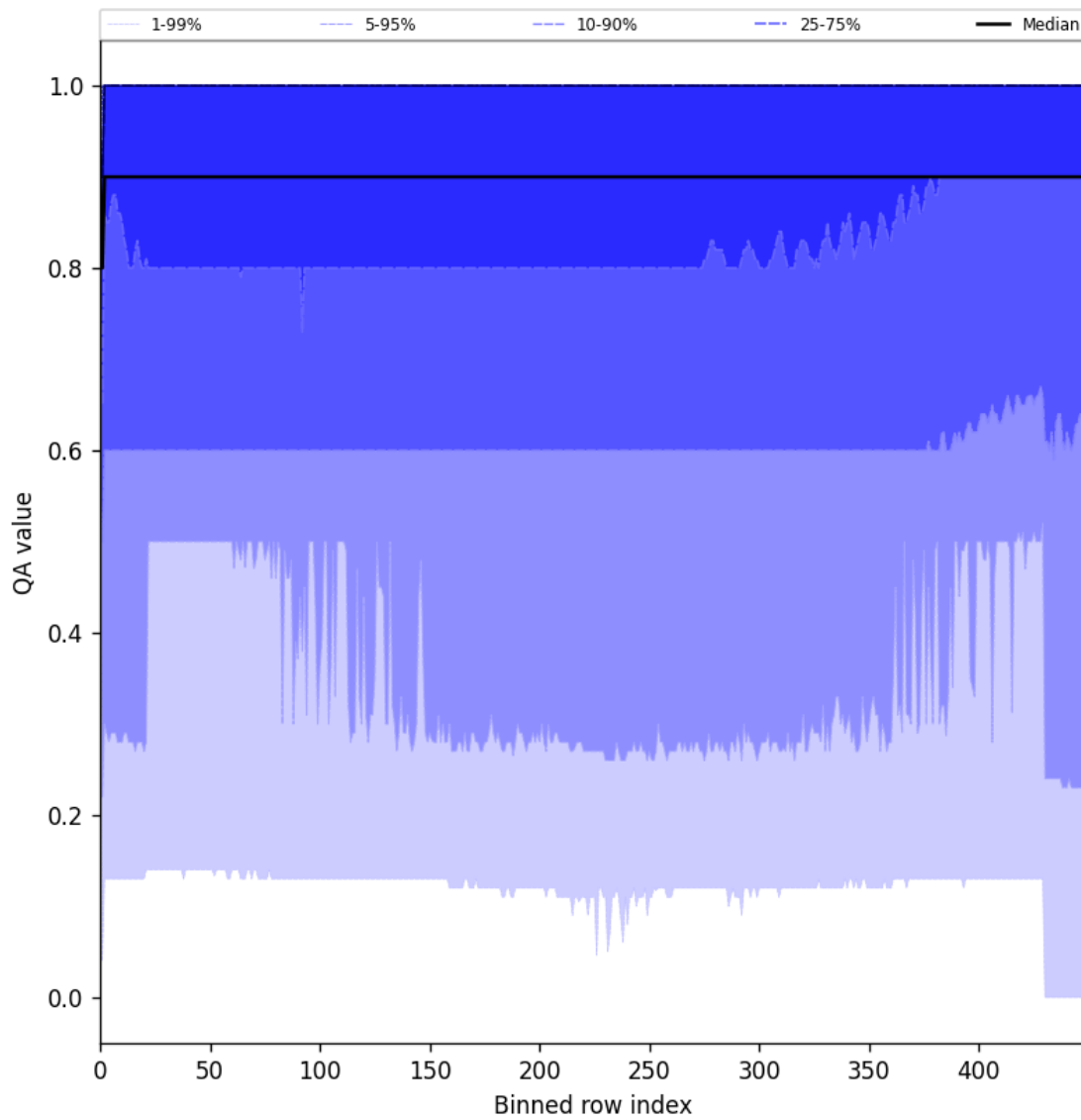
Figure 27: Along track statistics of “QA value” for 2024-12-06 to 2024-12-08
