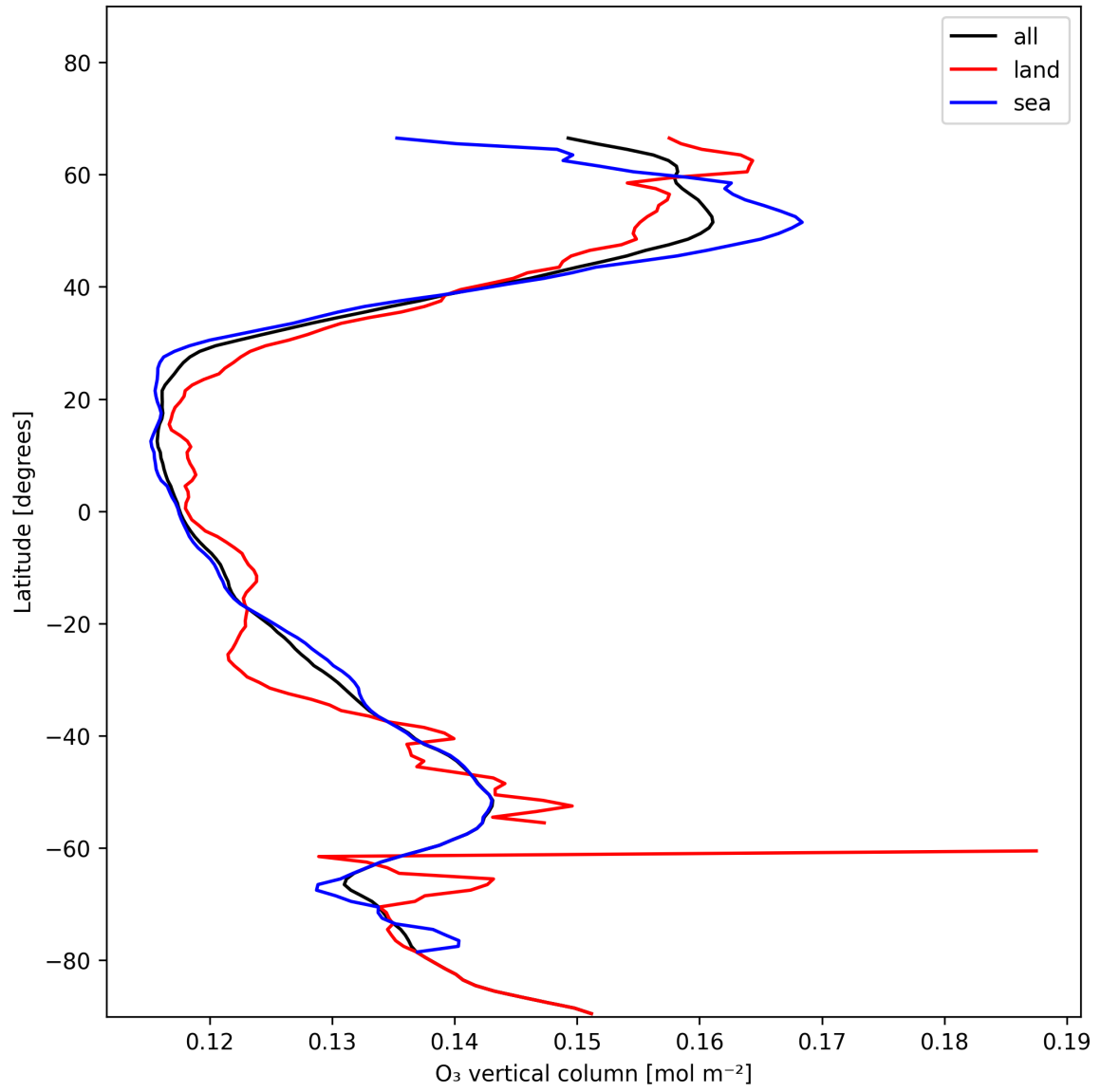
Figure 14: Zonal average of “O 3 vertical column” for 2024-12-06 to 2024-12-08.
