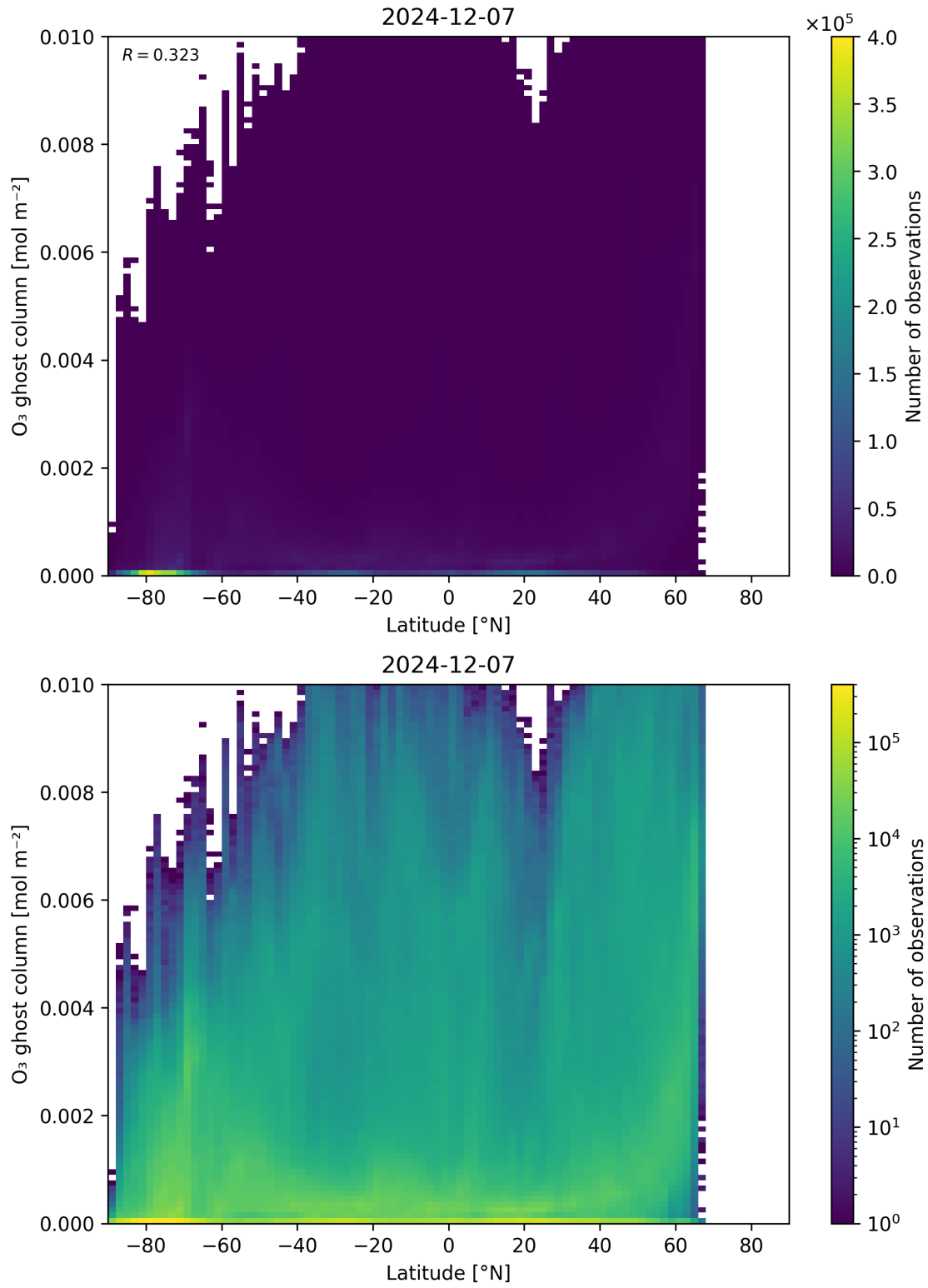
Figure 35: Scatter density plot of “Latitude” against “O 3 ghost column” for 2024-12-06 to 2024-12-08.
