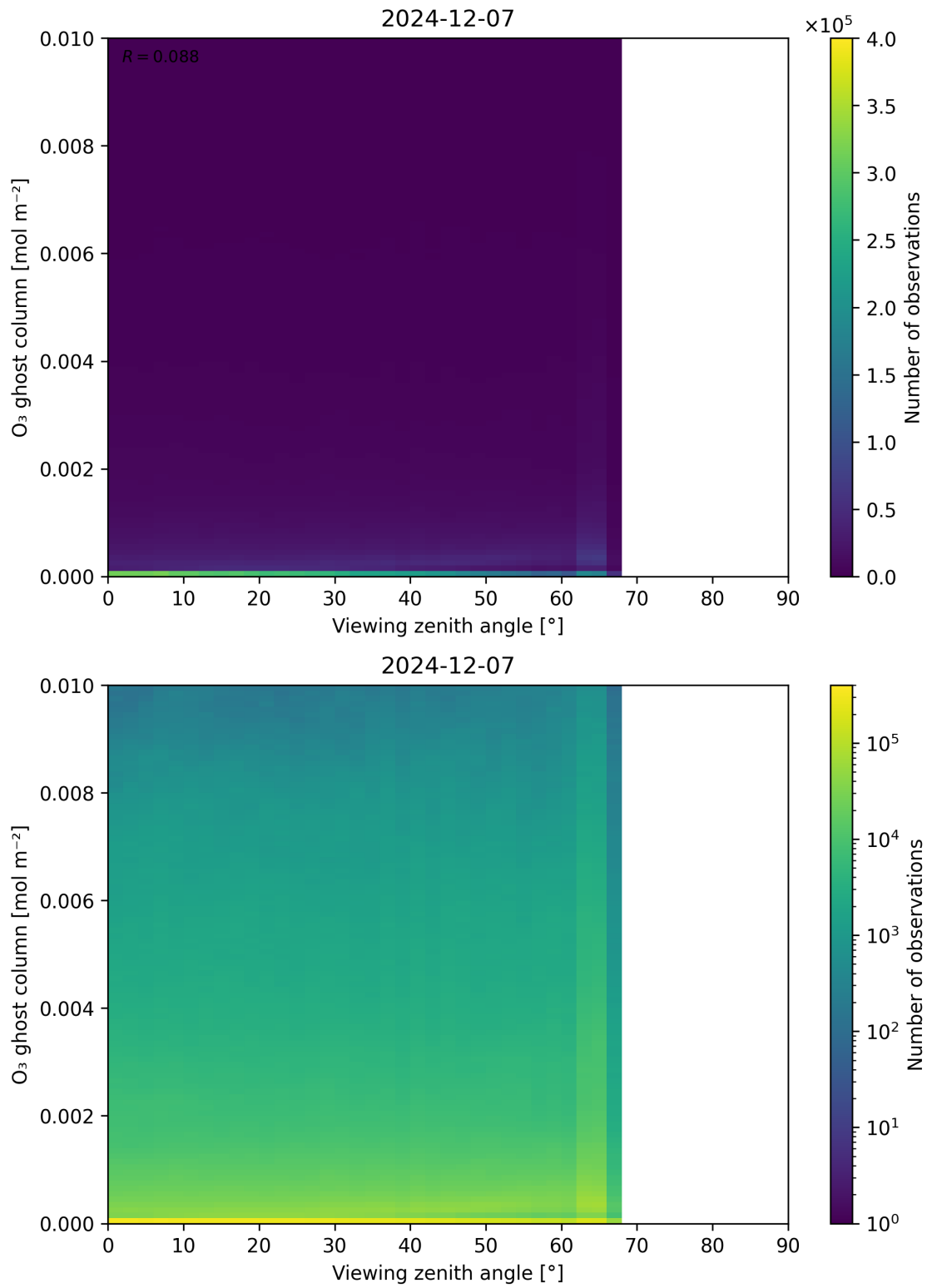
Figure 51: Scatter density plot of “Viewing zenith angle” against “O 3 ghost column” for 2024-12-06 to 2024-12-08.
