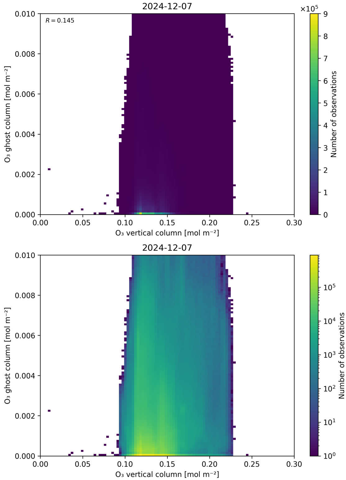
Figure 40: Scatter density plot of “O 3 vertical column” against “O 3 ghost column” for 2024-12-06 to 2024-12-08.
