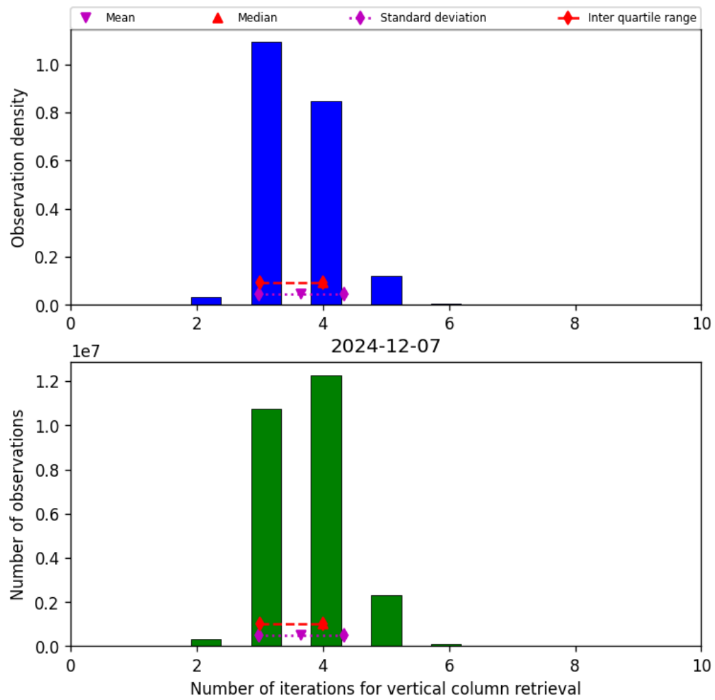
Figure 26: Histogram of “Number of iterations for vertical column retrieval” for 2024-12-06 to 2024-12-08
