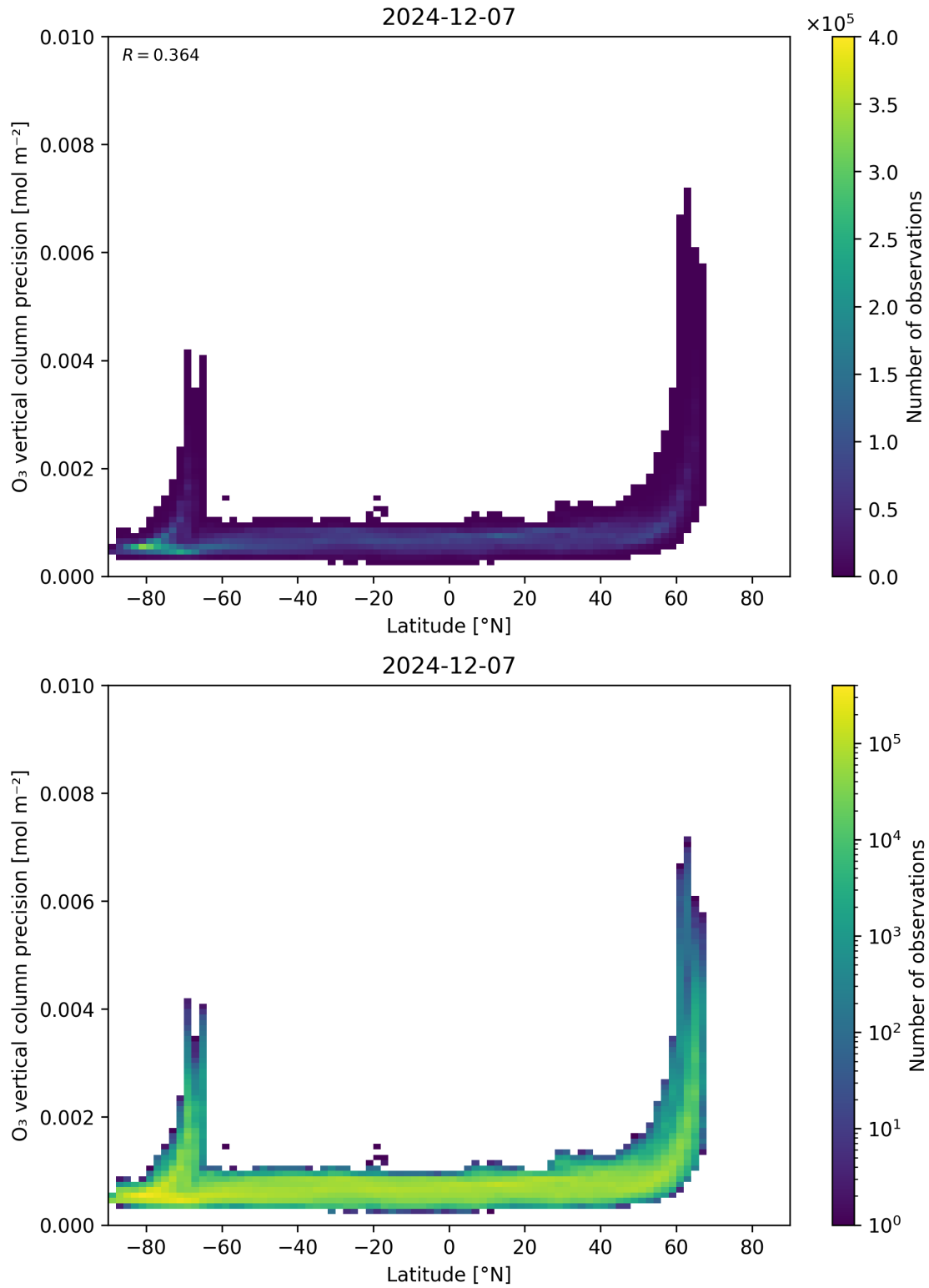
Figure 37: Scatter density plot of “Latitude” against “O 3 vertical column precision” for 2024-12-06 to 2024-12-08.
