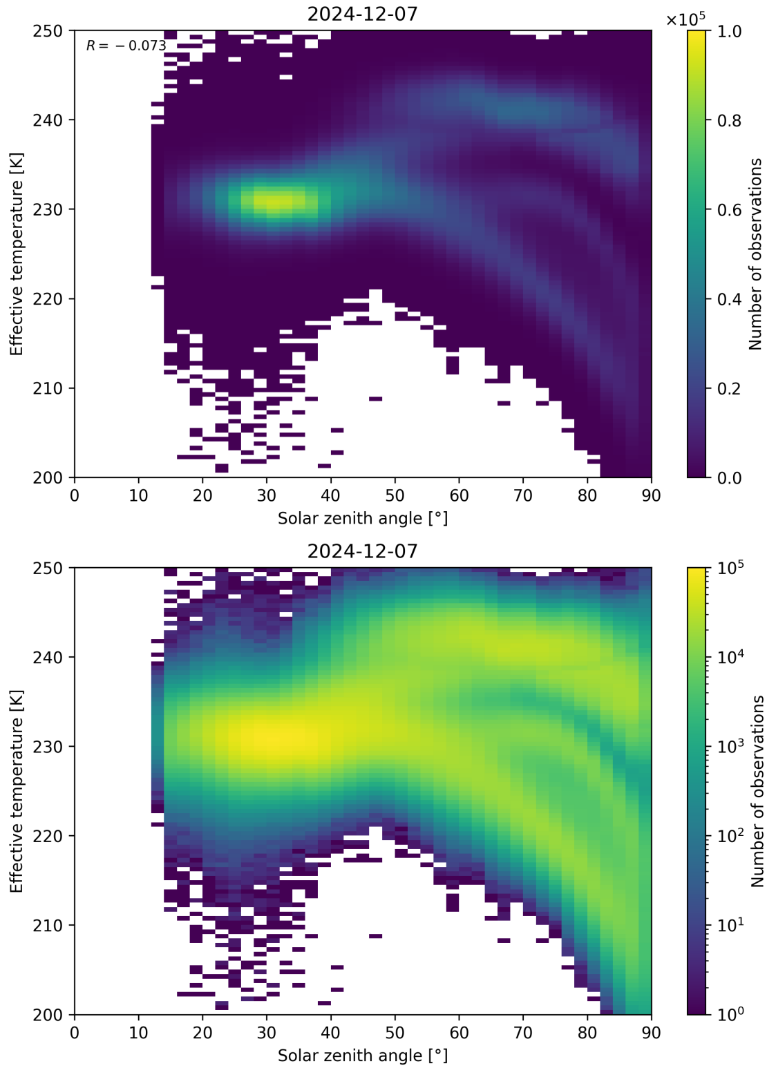
Figure 45: Scatter density plot of “Solar zenith angle” against “Effective temperature” for 2024-12-06 to 2024-12-08.
