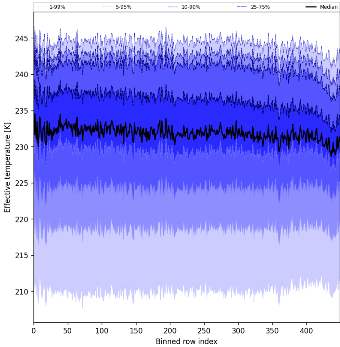
Figure 31: Along track statistics of “Effective temperature” for 2024-12-06 to 2024-12-08
