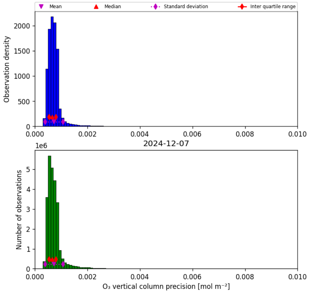
Figure 22: Histogram of “O 3 vertical column precision” for 2024-12-06 to 2024-12-08
