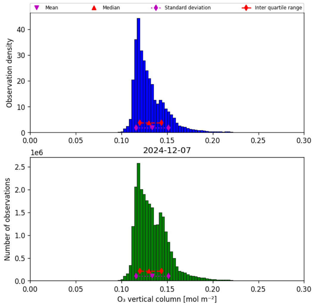
Figure 21: Histogram of “O 3 vertical column” for 2024-12-06 to 2024-12-08
