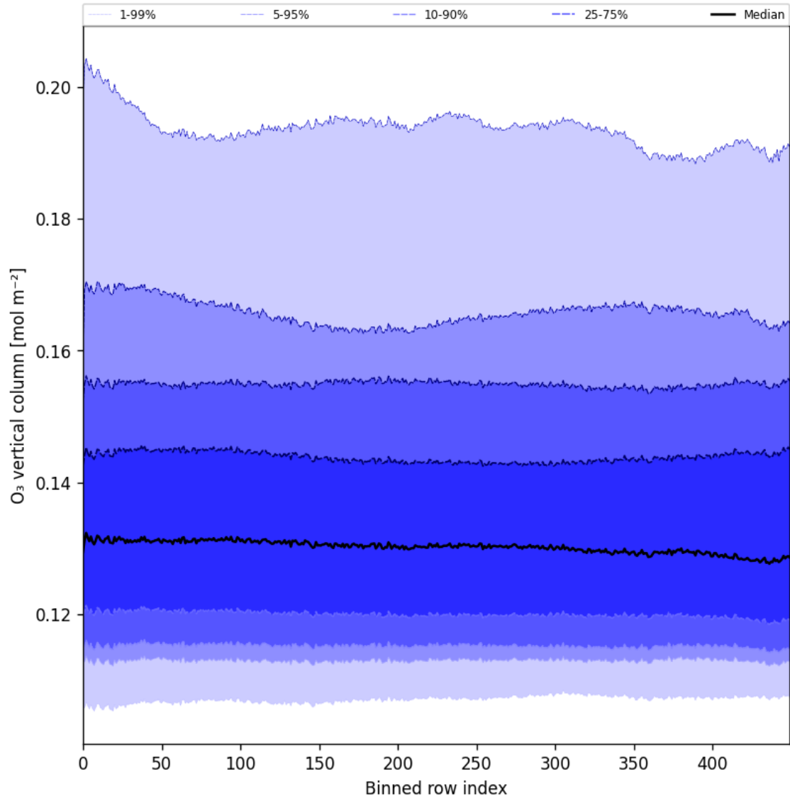
Figure 28: Along track statistics of “O 3 vertical column” for 2024-12-06 to 2024-12-08
