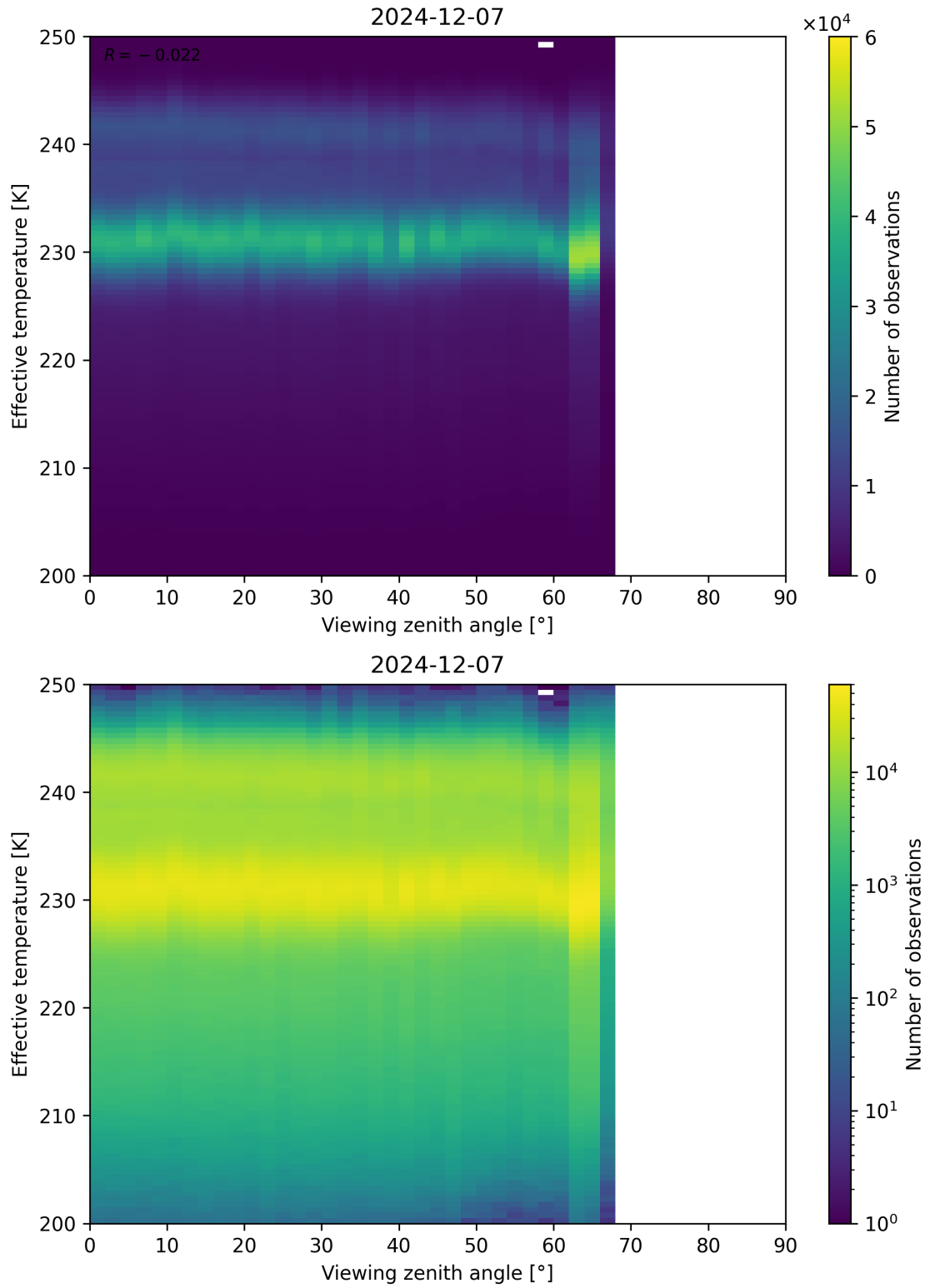
Figure 50: Scatter density plot of “Viewing zenith angle” against “Effective temperature” for 2024-12-06 to 2024-12-08.
