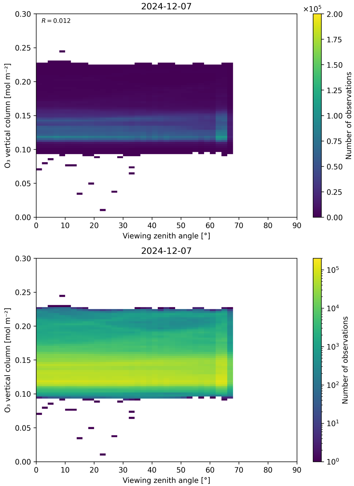
Figure 52: Scatter density plot of “Viewing zenith angle” against “O 3 vertical column” for 2024-12-06 to 2024-12-08.
