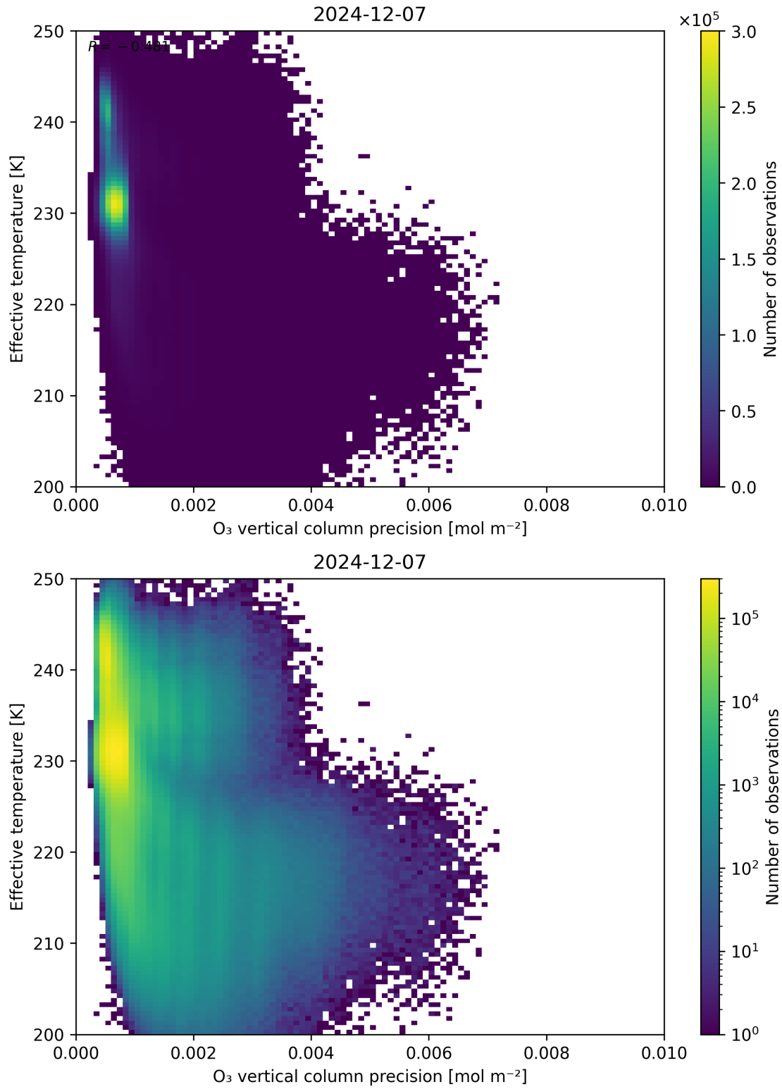
Figure 42: Scatter density plot of “O 3 vertical column precision” against “Effective temperature” for 2024-12-06 to 2024-12-08.
