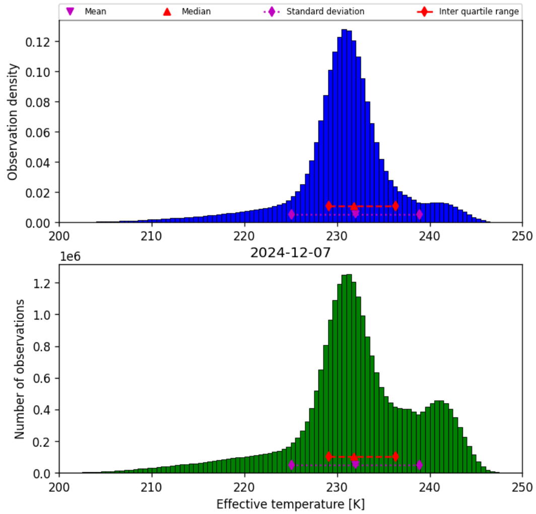
Figure 24: Histogram of “Effective temperature” for 2024-12-06 to 2024-12-08
