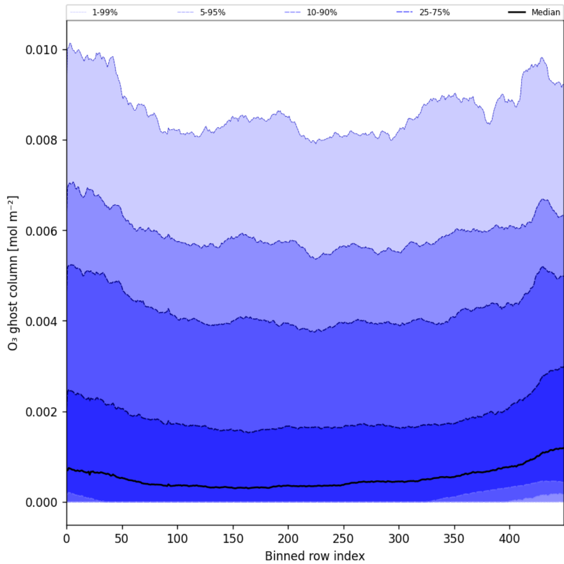
Figure 32: Along track statistics of “O 3 ghost column” for 2024-12-06 to 2024-12-08
