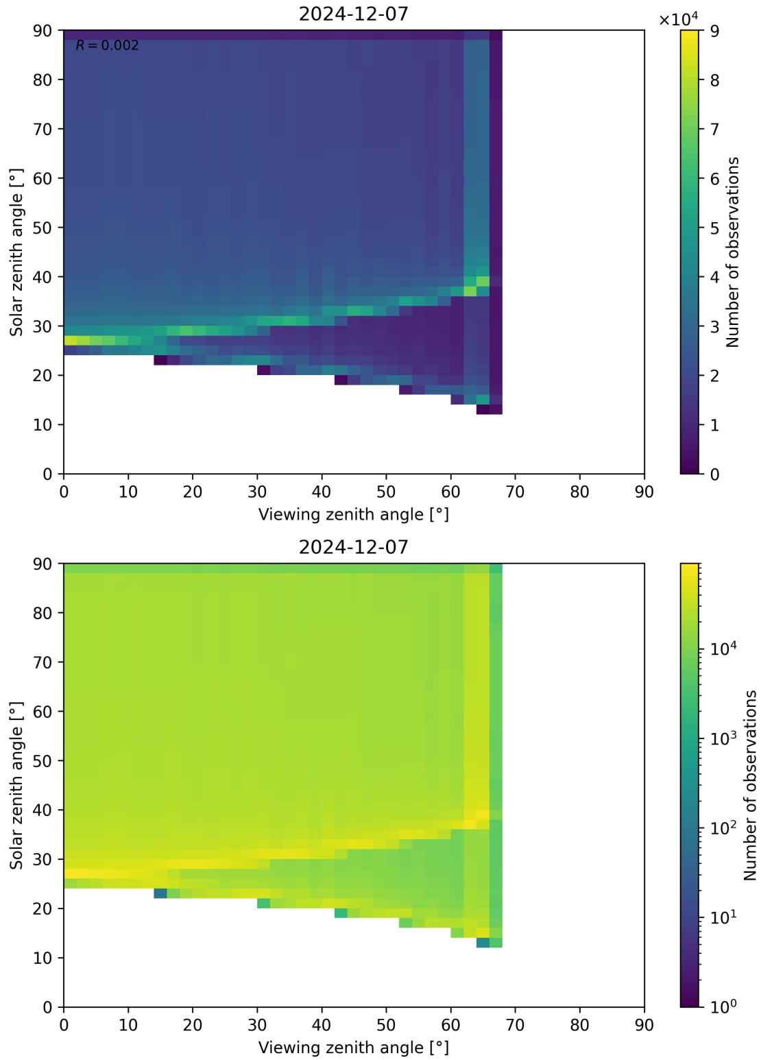
Figure 54: Scatter density plot of “Viewing zenith angle” against “Solar zenith angle” for 2024-12-06 to 2024-12-08.
