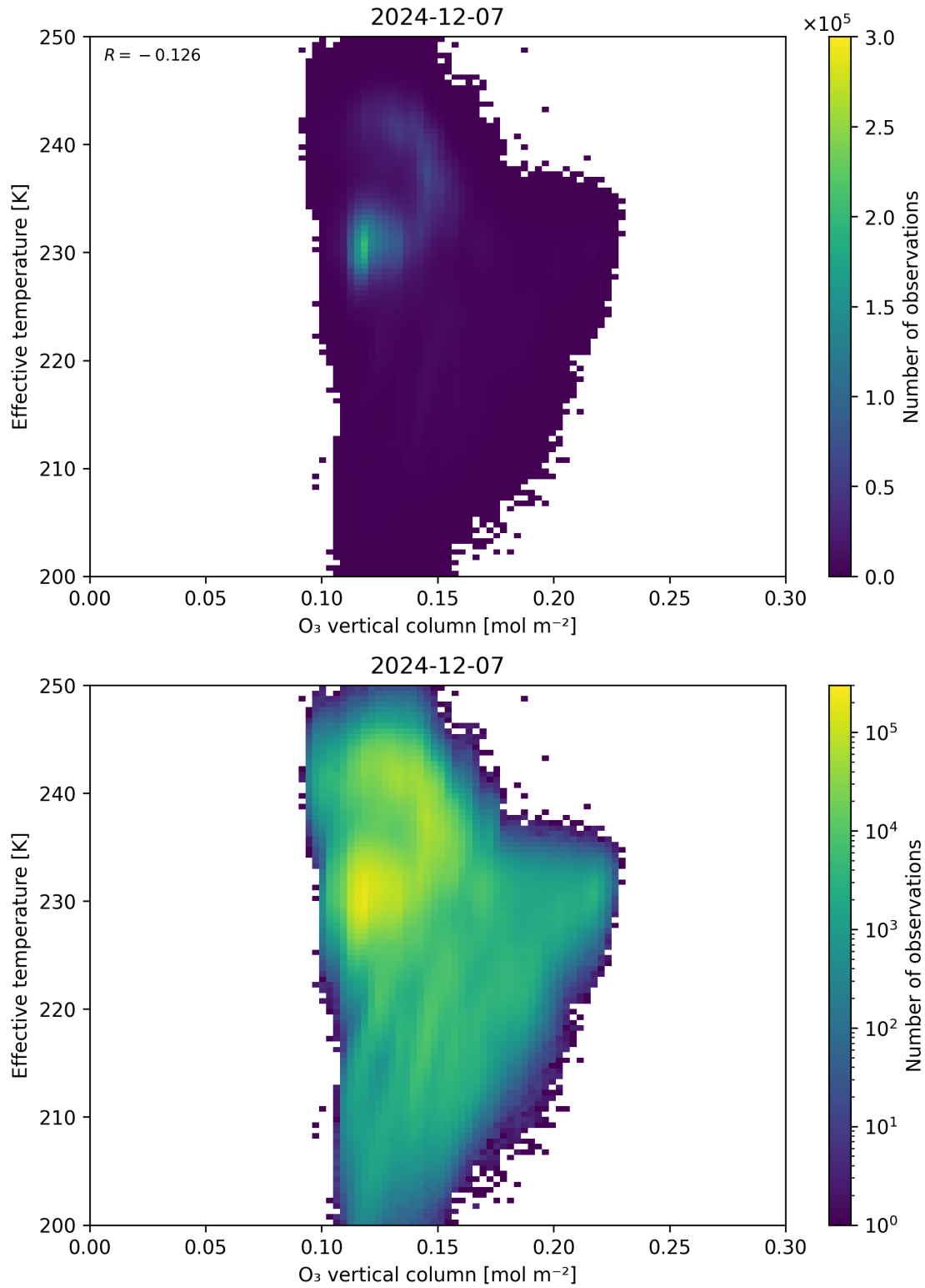
Figure 39: Scatter density plot of “O 3 vertical column” against “Effective temperature” for 2024-12-06 to 2024-12-08.
