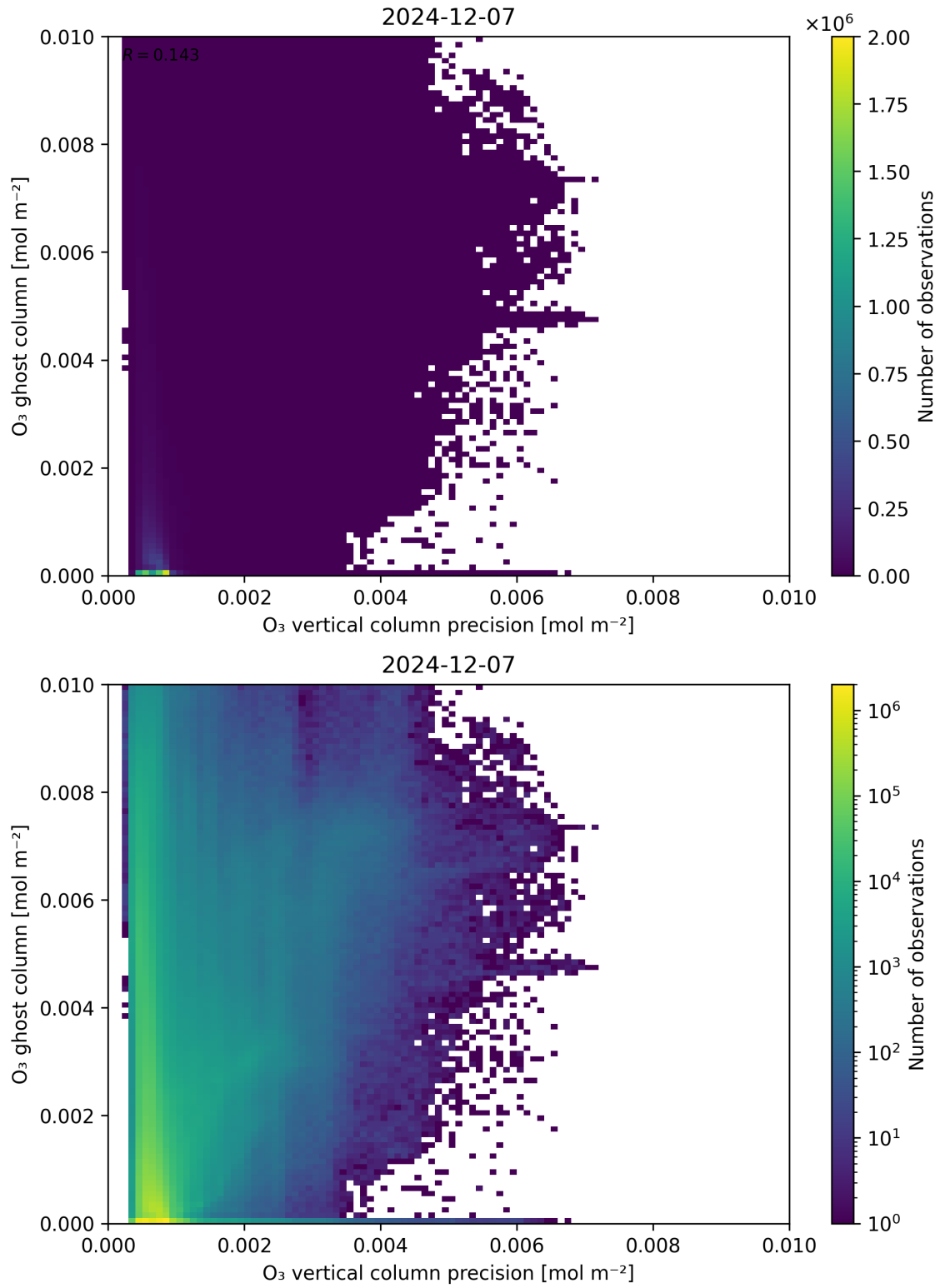
Figure 43: Scatter density plot of “ \text{O}_3 vertical column precision” against “ \text{O}_3 ghost column” for 2024-12-06 to 2024-12-08.
