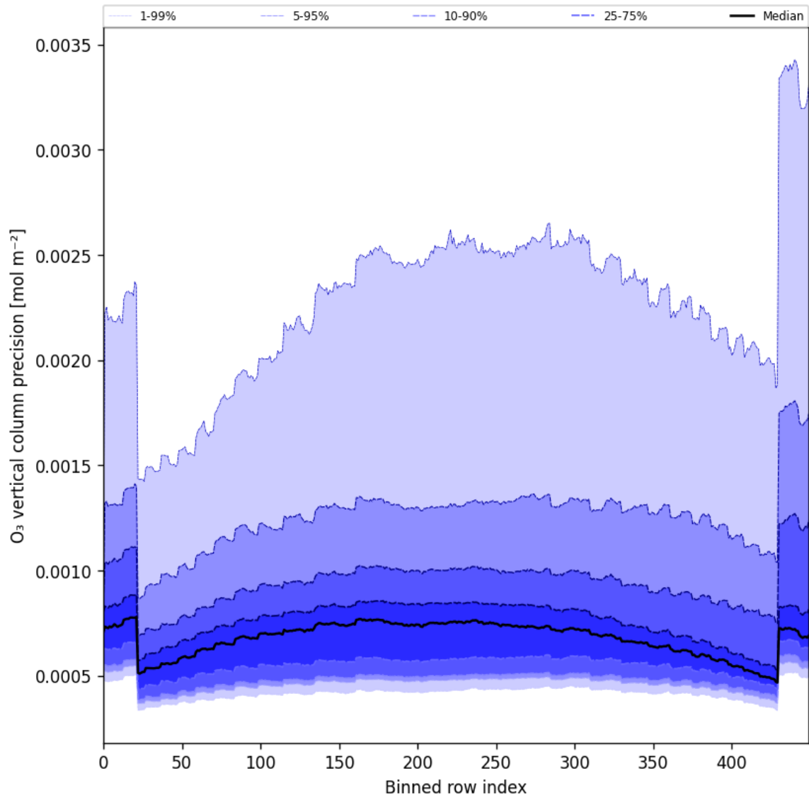
Figure 29: Along track statistics of “O 3 vertical column precision” for 2024-12-06 to 2024-12-08
