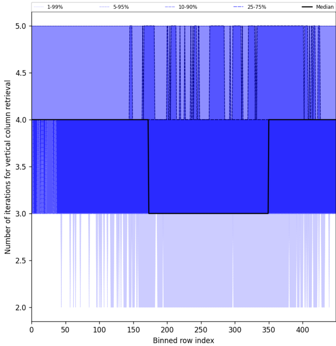
Figure 33: Along track statistics of “Number of iterations for vertical column retrieval” for 2024-12-06 to 2024-12-08
