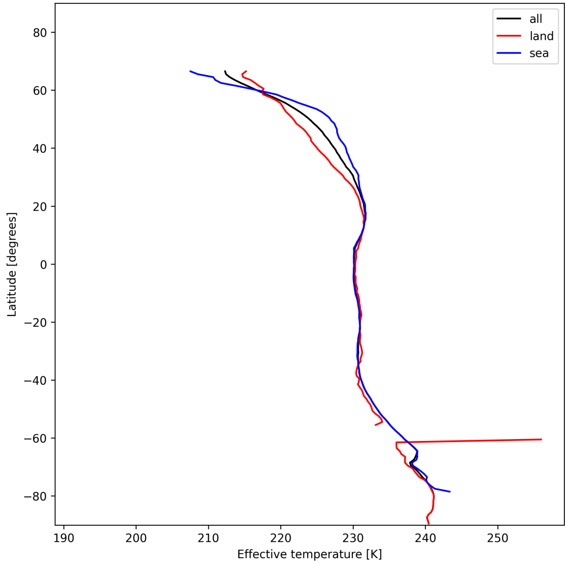
Figure 17: Zonal average of "Effective temperature" for 2024-12-06 to 2024-12-08.
