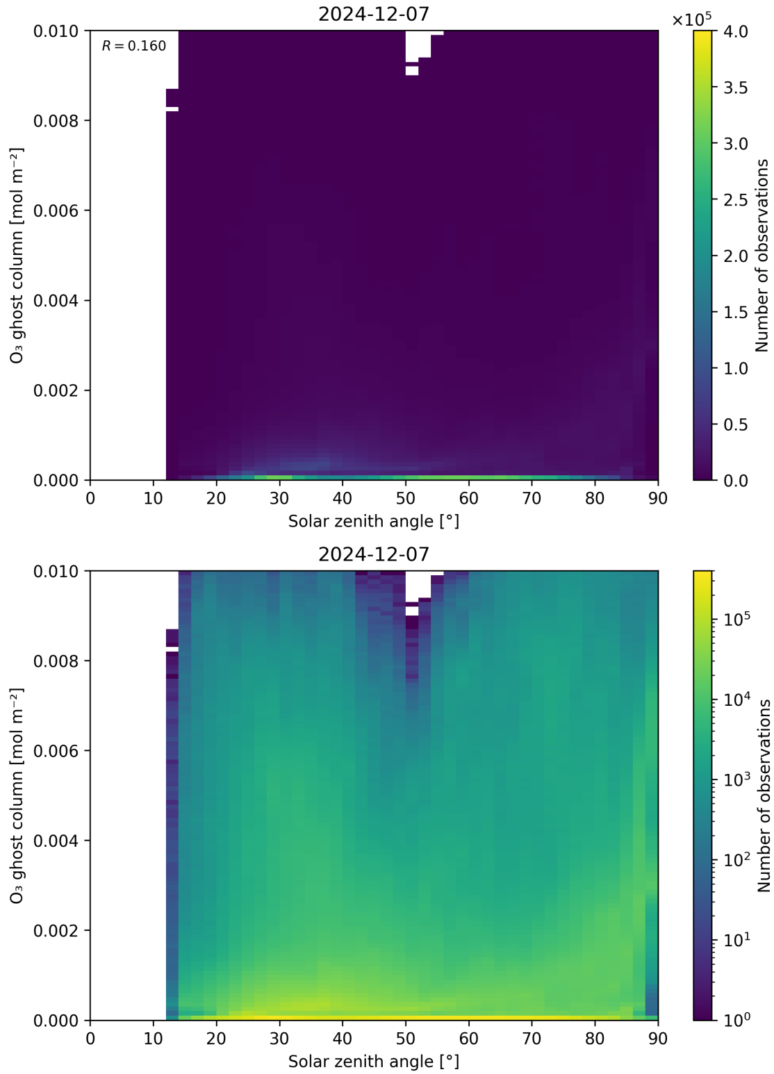
Figure 46: Scatter density plot of “Solar zenith angle” against “O 3 ghost column” for 2024-12-06 to 2024-12-08.
