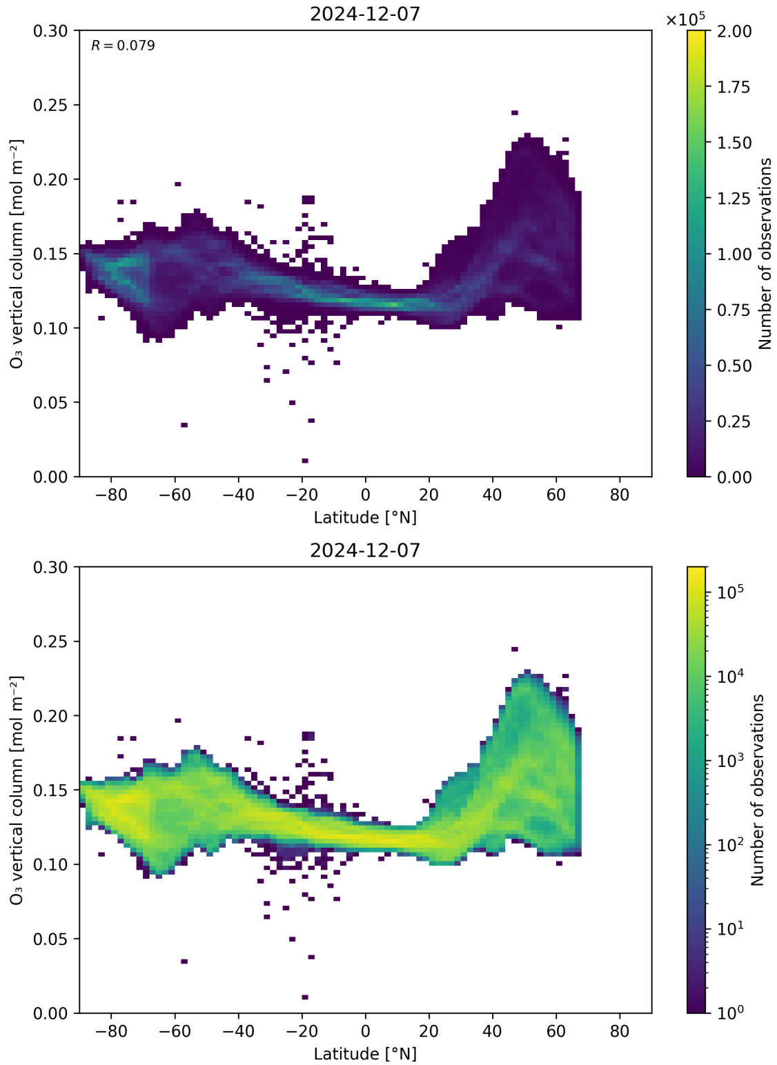
Figure 36: Scatter density plot of “Latitude” against “O 3 vertical column” for 2024-12-06 to 2024-12-08.
