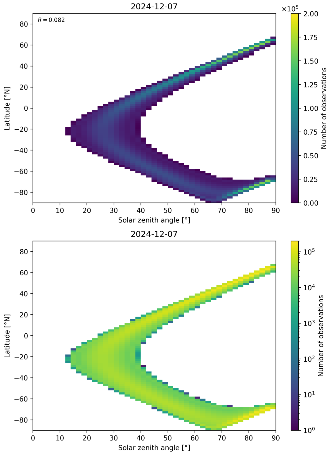
Figure 44: Scatter density plot of “Solar zenith angle” against “Latitude” for 2024-12-06 to 2024-12-08.
