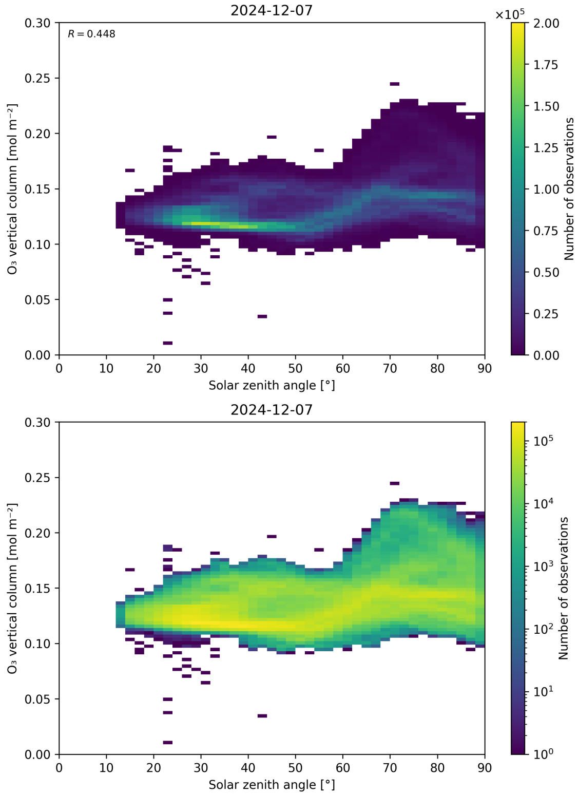
Figure 47: Scatter density plot of “Solar zenith angle” against “O 3 vertical column” for 2024-12-06 to 2024-12-08.
