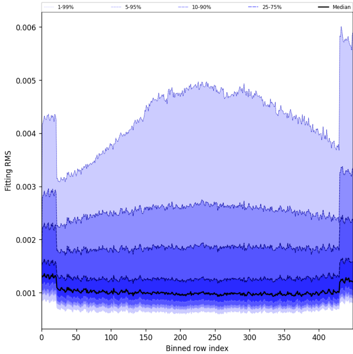
Figure 30: Along track statistics of “Fitting RMS” for 2024-12-06 to 2024-12-08
