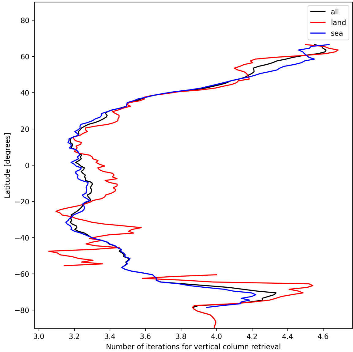
Figure 19: Zonal average of “Number of iterations for vertical column retrieval” for 2024-12-06 to 2024-12-08.
