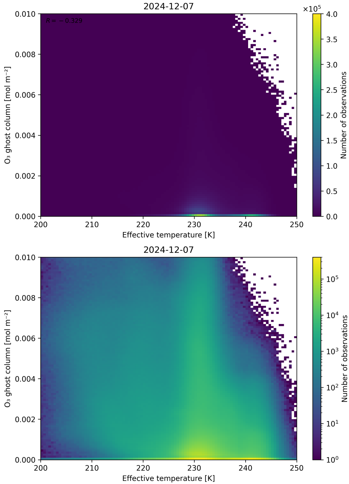
Figure 38: Scatter density plot of “Effective temperature” against “O 3 ghost column” for 2024-12-06 to 2024-12-08.
