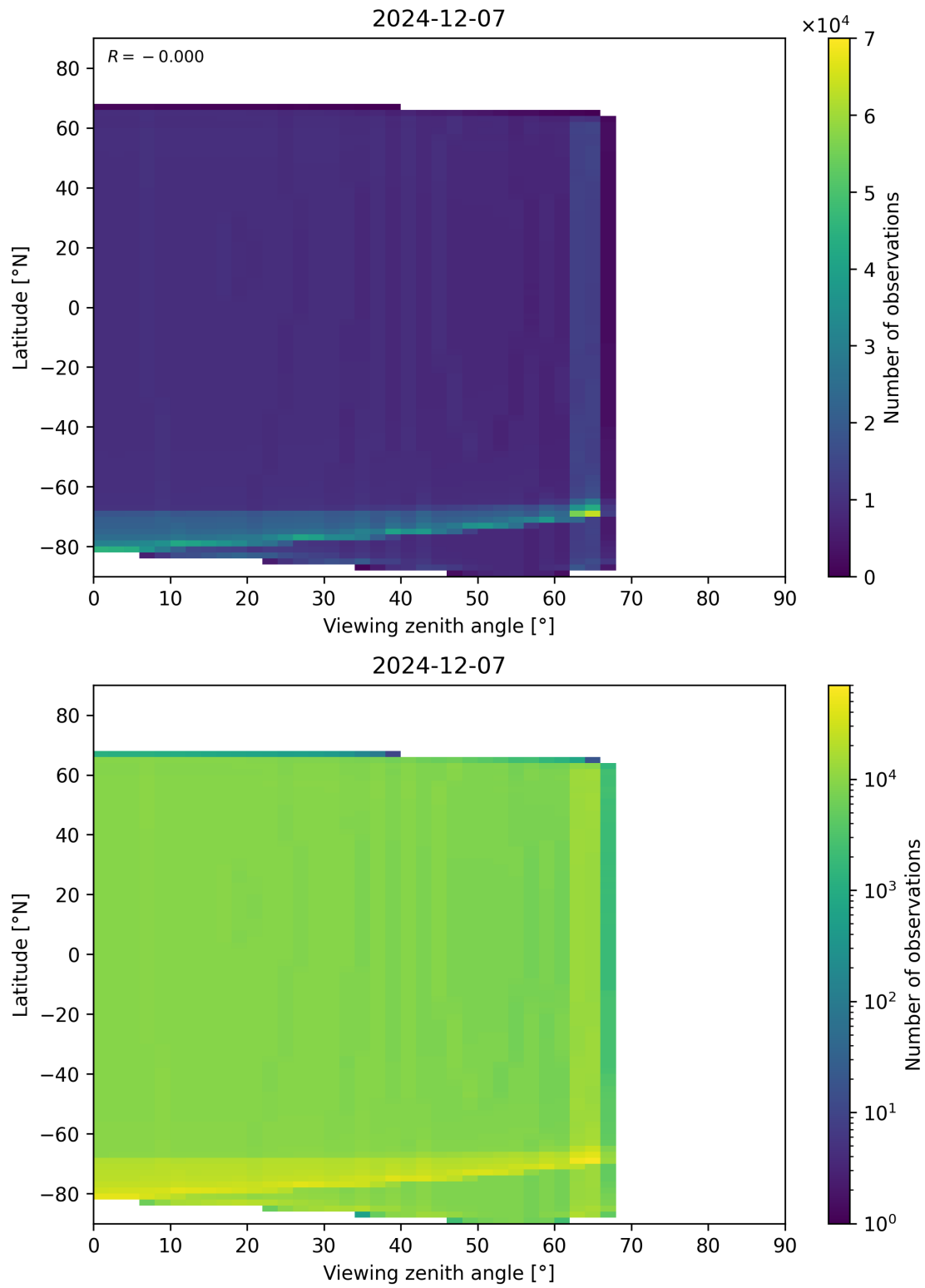
Figure 49: Scatter density plot of “Viewing zenith angle” against “Latitude” for 2024-12-06 to 2024-12-08.
