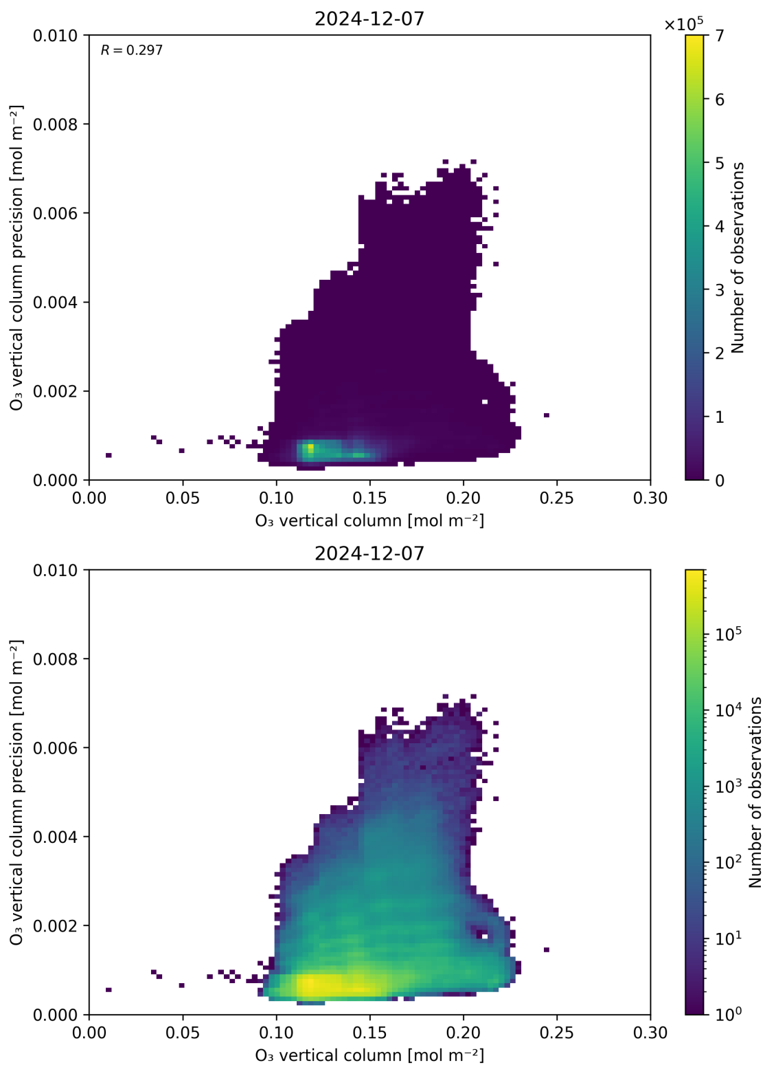
Figure 41: Scatter density plot of “O 3 vertical column” against “O 3 vertical column precision” for 2024-12-06 to 2024-12-08.
