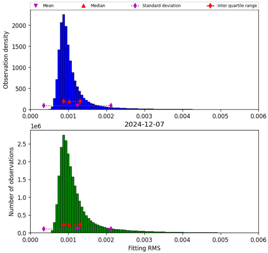
Figure 23: Histogram of “Fitting RMS” for 2024-12-06 to 2024-12-08
