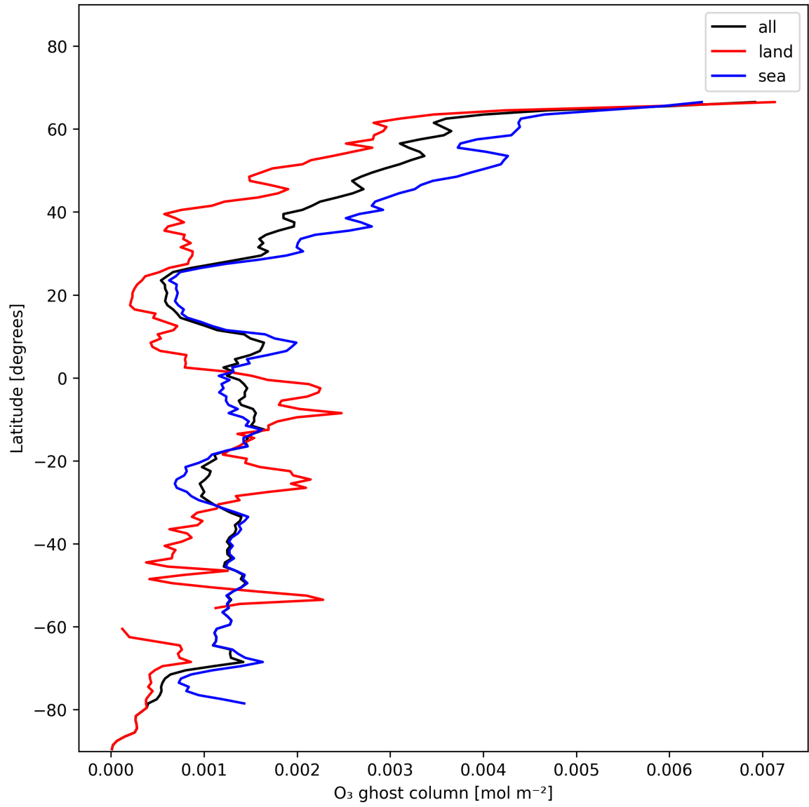
Figure 18: Zonal average of “O 3 ghost column” for 2024-12-06 to 2024-12-08.
