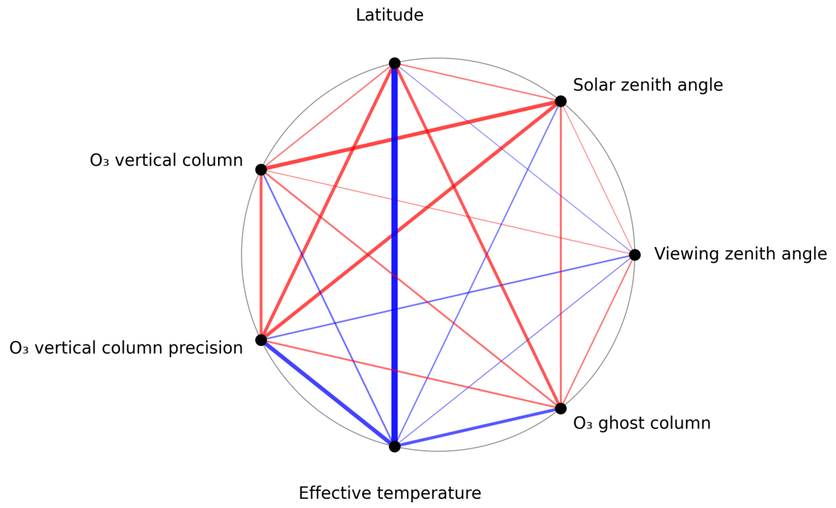
Figure 1: Map of correlation graph for 2024-12-06 to 2024-12-08.
