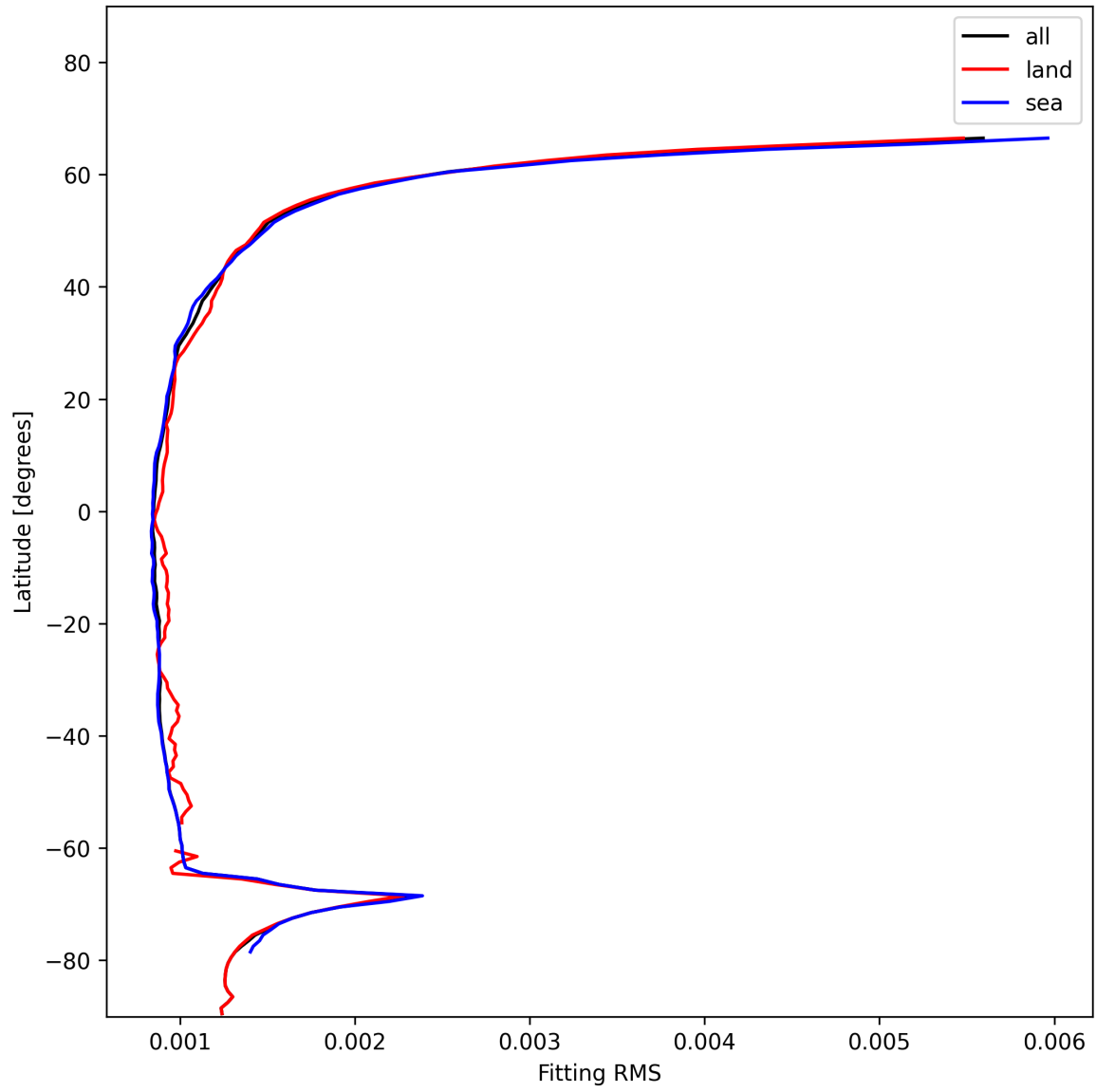
Figure 16: Zonal average of “Fitting RMS” for 2024-12-06 to 2024-12-08.
