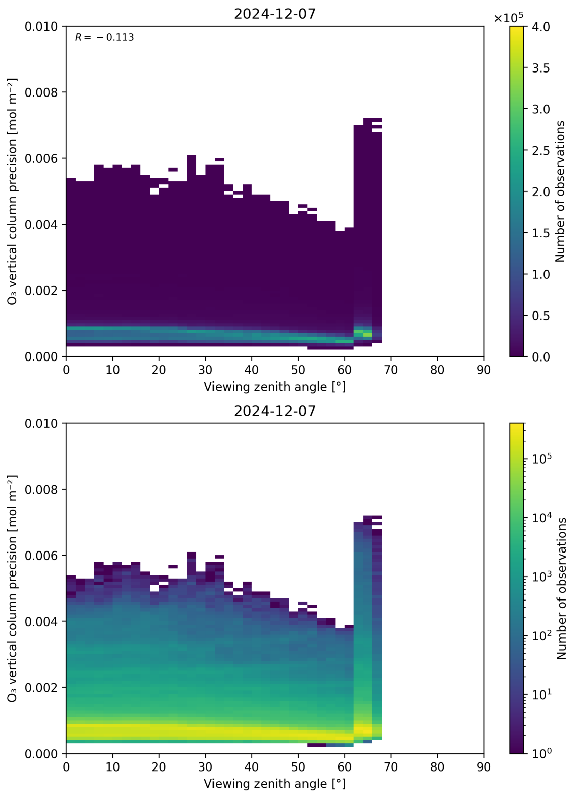
Figure 53: Scatter density plot of “Viewing zenith angle” against “O 3 vertical column precision” for 2024-12-06 to 2024-12-08.
