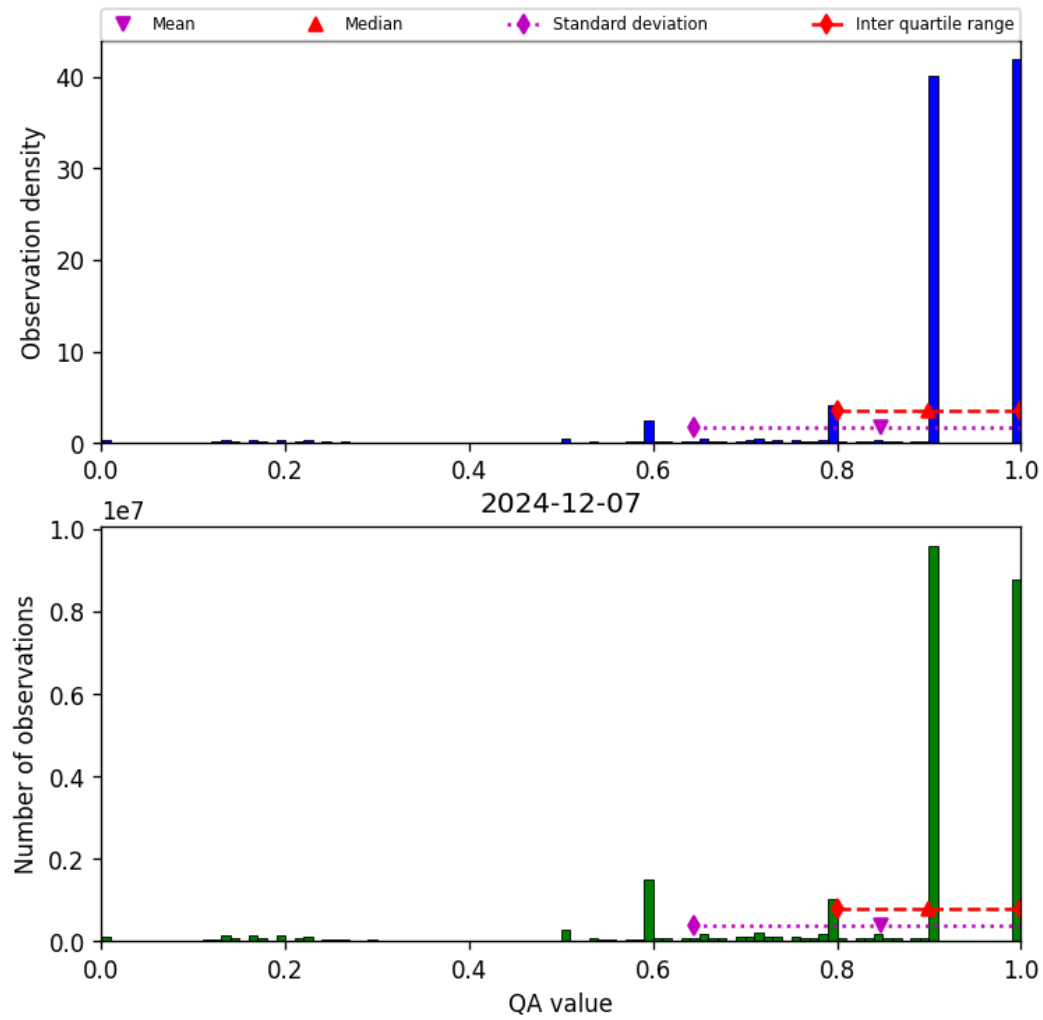
Figure 20: Histogram of “QA value” for 2024-12-06 to 2024-12-08
