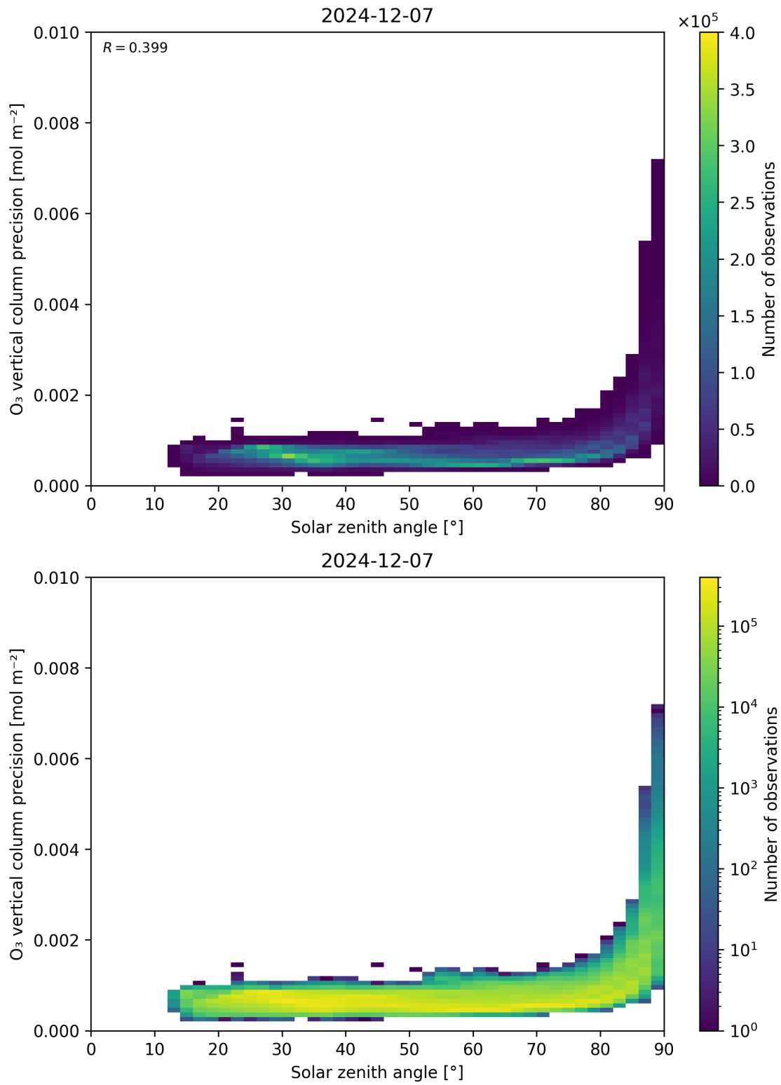
Figure 48: Scatter density plot of “Solar zenith angle” against “O 3 vertical column precision” for 2024-12-06 to 2024-12-08.
