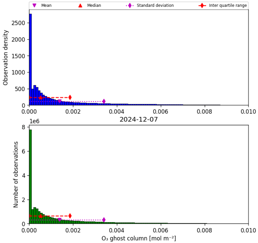
Figure 25: Histogram of “O 3 ghost column” for 2024-12-06 to 2024-12-08
