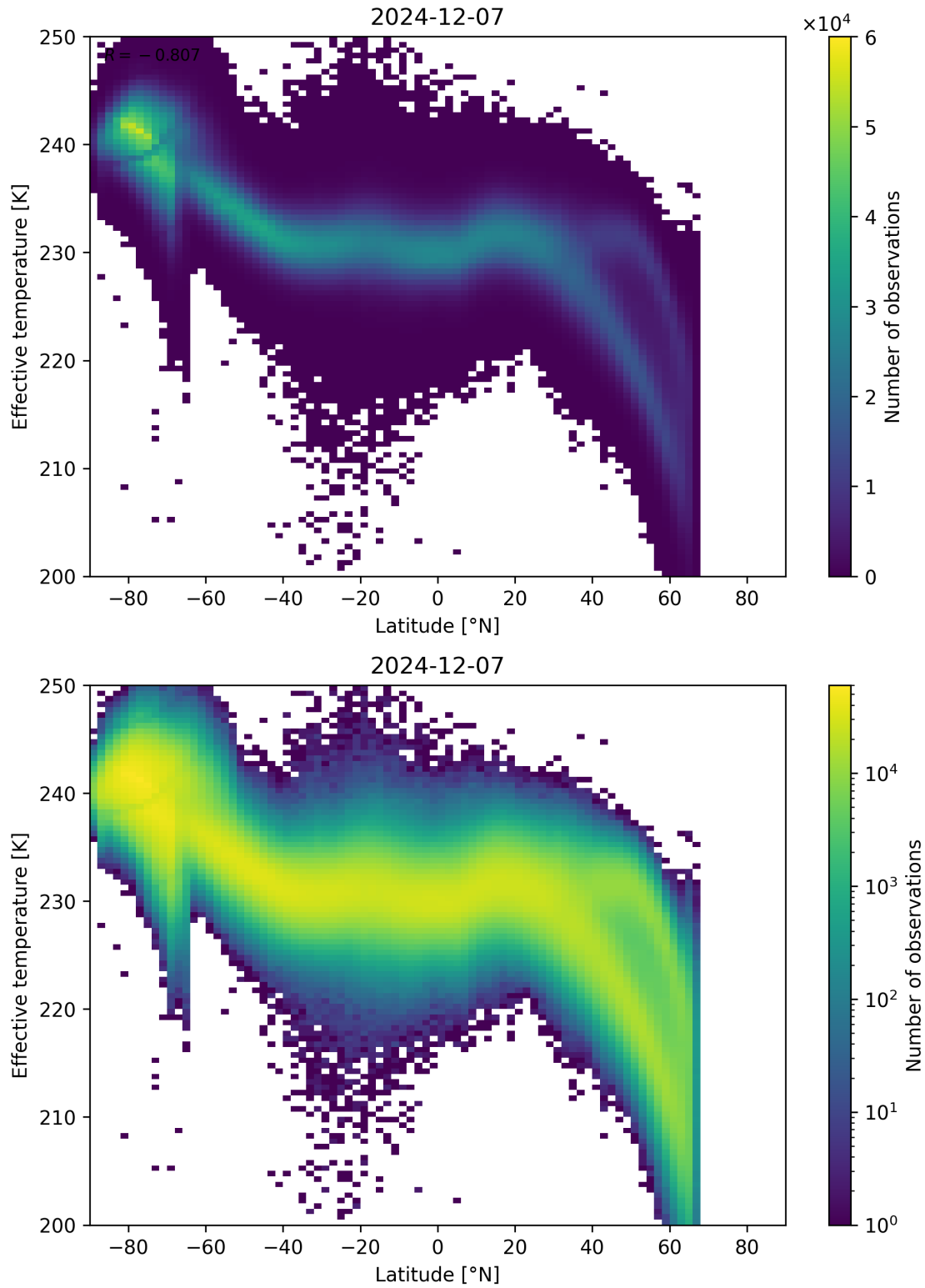
Figure 34: Scatter density plot of “Latitude” against “Effective temperature” for 2024-12-06 to 2024-12-08.
