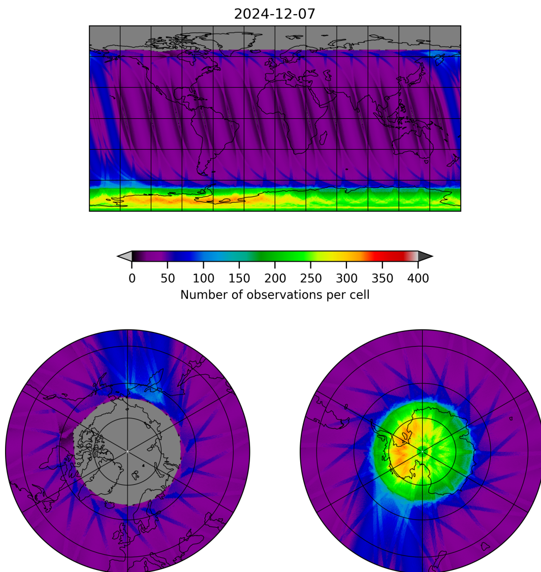
Figure 12: Map of the number of observations for 2024-12-06 to 2024-12-08
