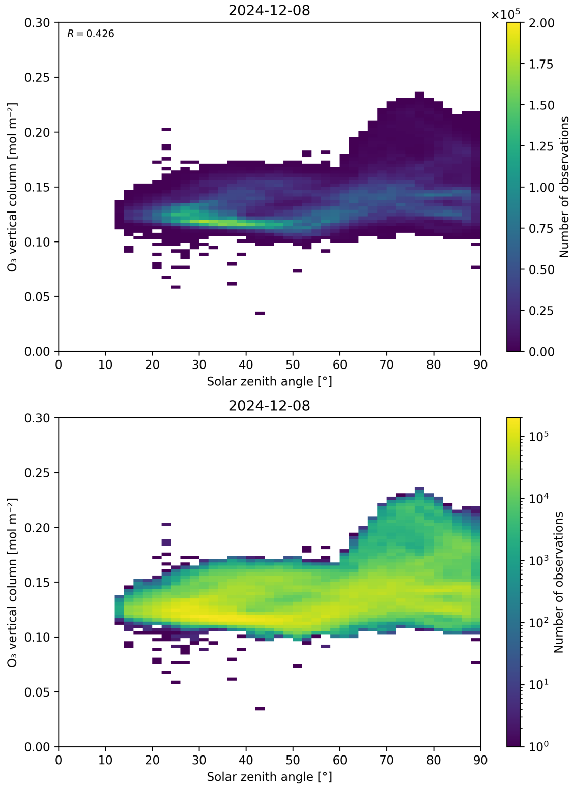
Figure 47: Scatter density plot of “Solar zenith angle” against “O 3 vertical column” for 2024-12-07 to 2024-12-09.
