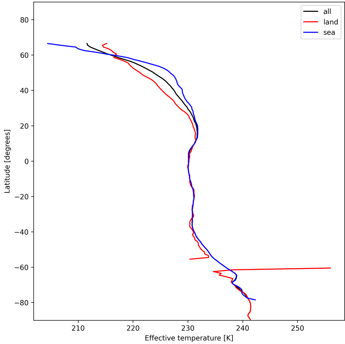
Figure 17: Zonal average of “Effective temperature” for 2024-12-07 to 2024-12-09.
