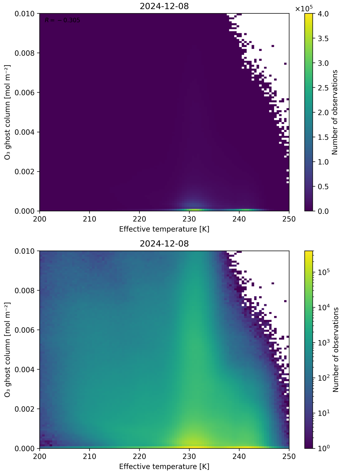
Figure 38: Scatter density plot of “Effective temperature” against “O 3 ghost column” for 2024-12-07 to 2024-12-09.
