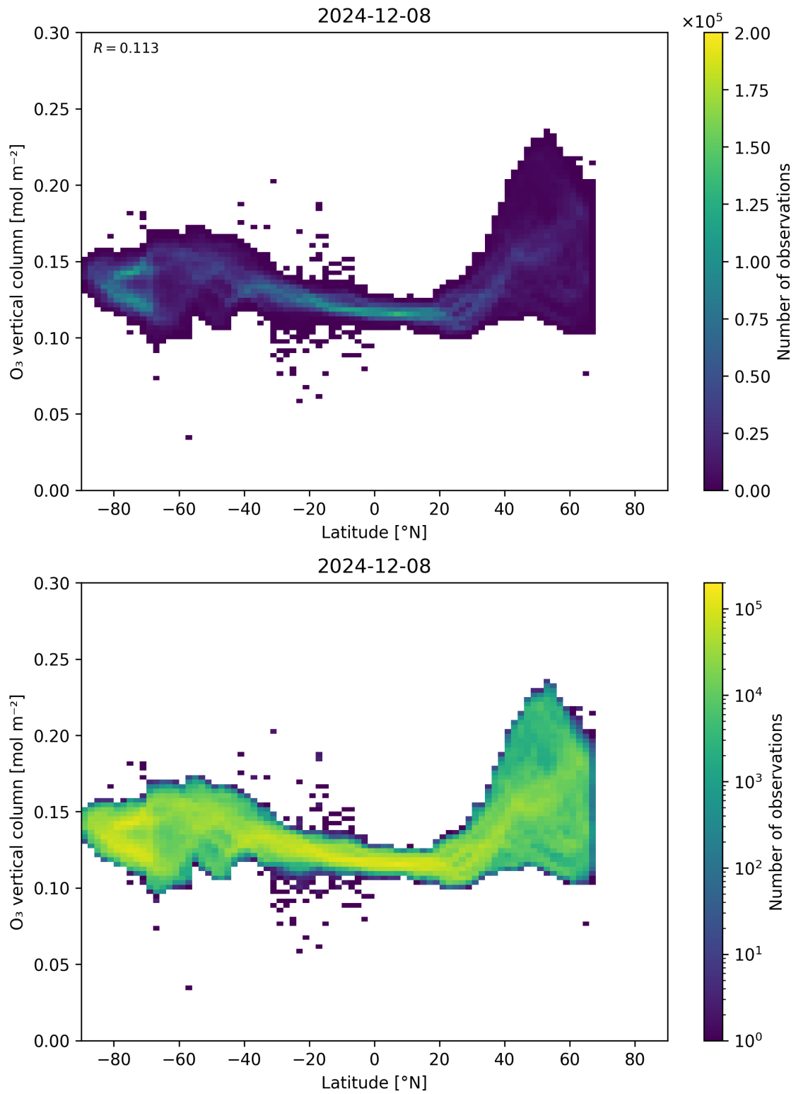
Figure 36: Scatter density plot of “Latitude” against “O 3 vertical column” for 2024-12-07 to 2024-12-09.
