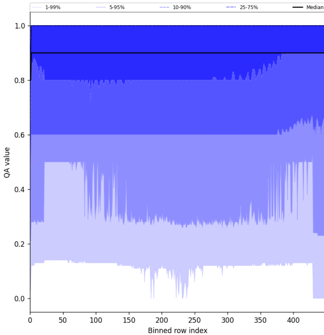
Figure 27: Along track statistics of “QA value” for 2024-12-07 to 2024-12-09
