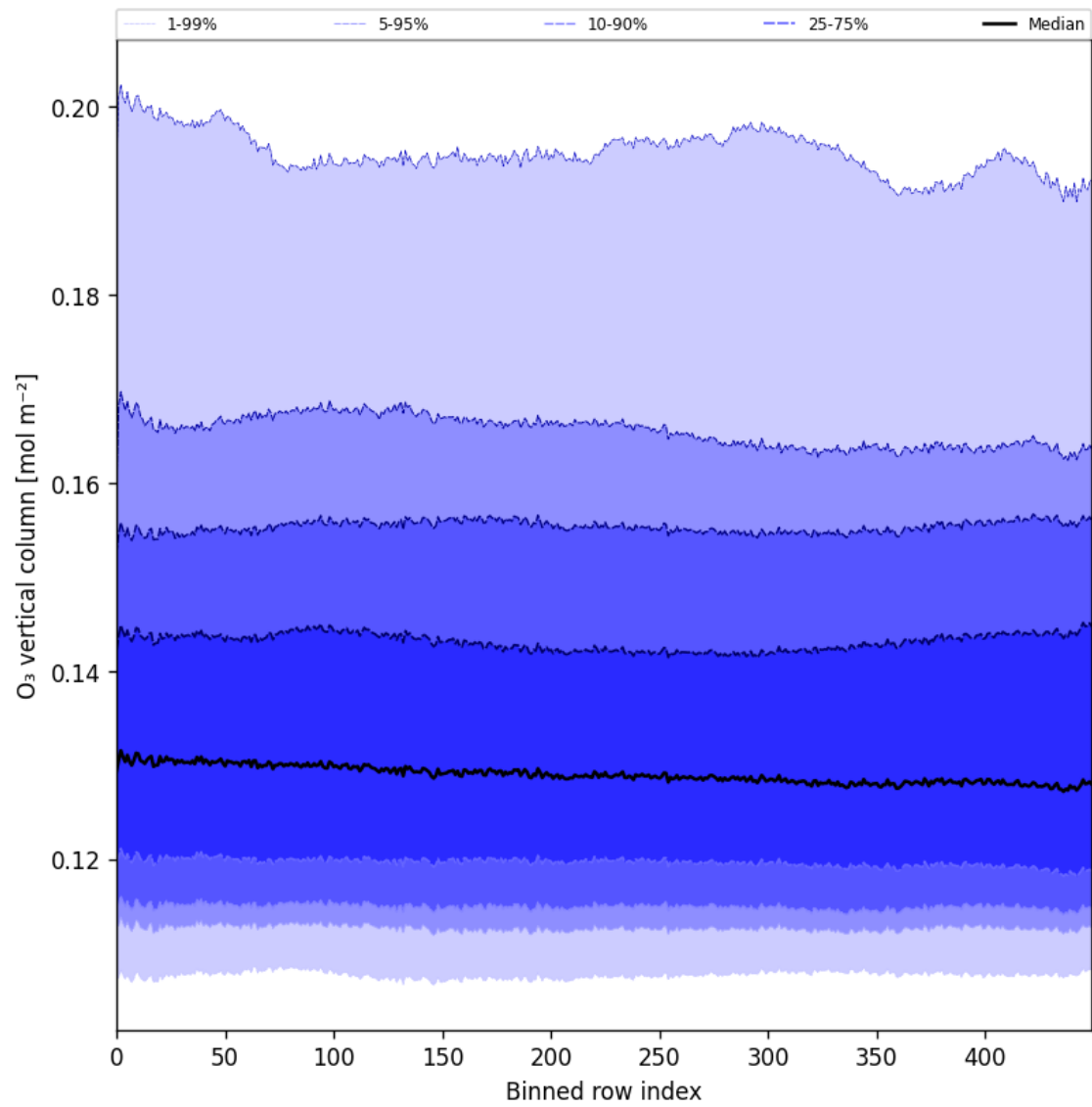
Figure 28: Along track statistics of “O 3 vertical column” for 2024-12-07 to 2024-12-09
