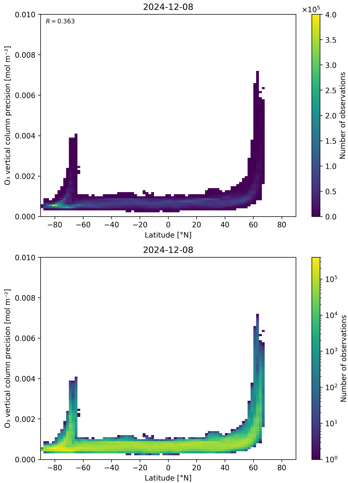
Figure 37: Scatter density plot of “Latitude” against “O 3 vertical column precision” for 2024-12-07 to 2024-12-09.
