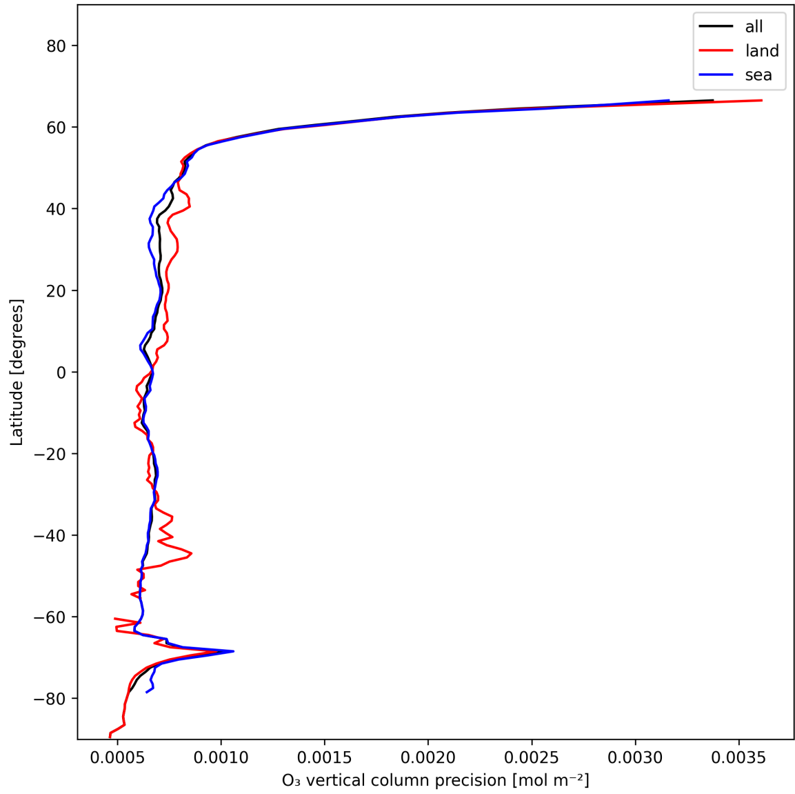
Figure 15: Zonal average of “O 3 vertical column precision” for 2024-12-07 to 2024-12-09.
