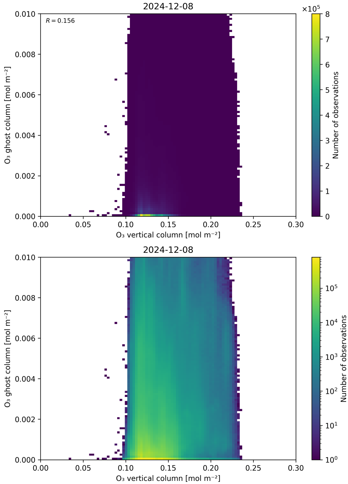
Figure 40: Scatter density plot of “O 3 vertical column” against “O 3 ghost column” for 2024-12-07 to 2024-12-09.
