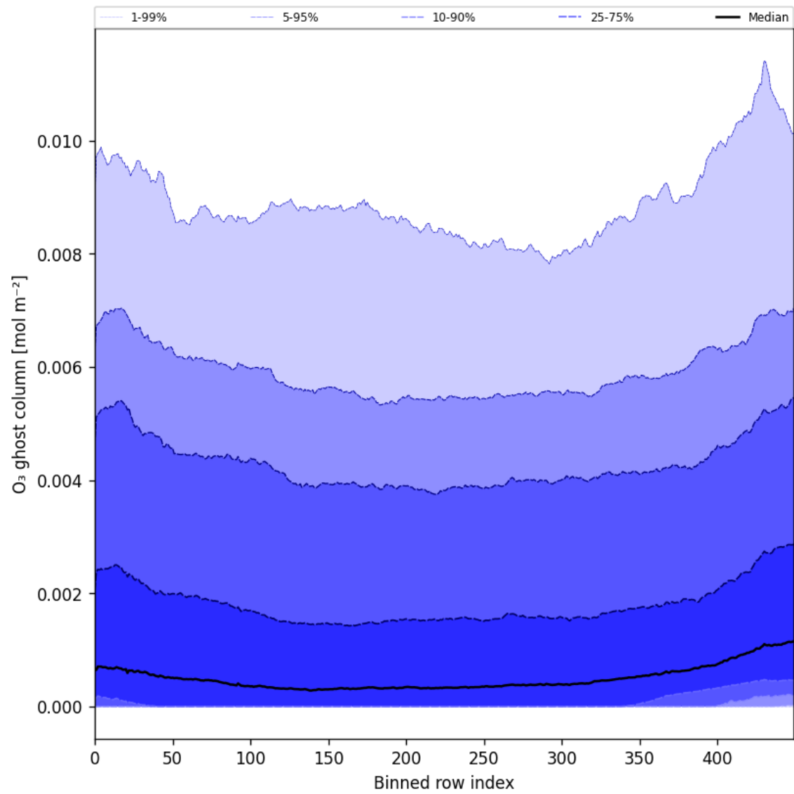
Figure 32: Along track statistics of “O 3 ghost column” for 2024-12-07 to 2024-12-09
