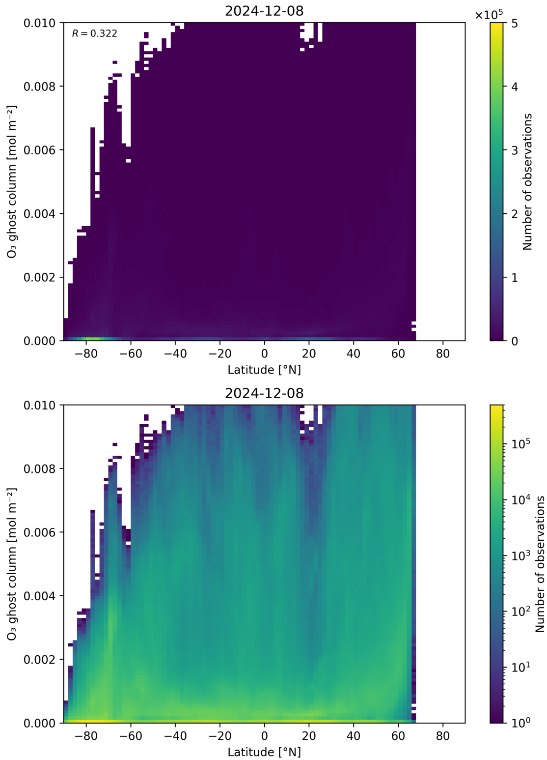
Figure 35: Scatter density plot of “Latitude” against “O 3 ghost column” for 2024-12-07 to 2024-12-09.
