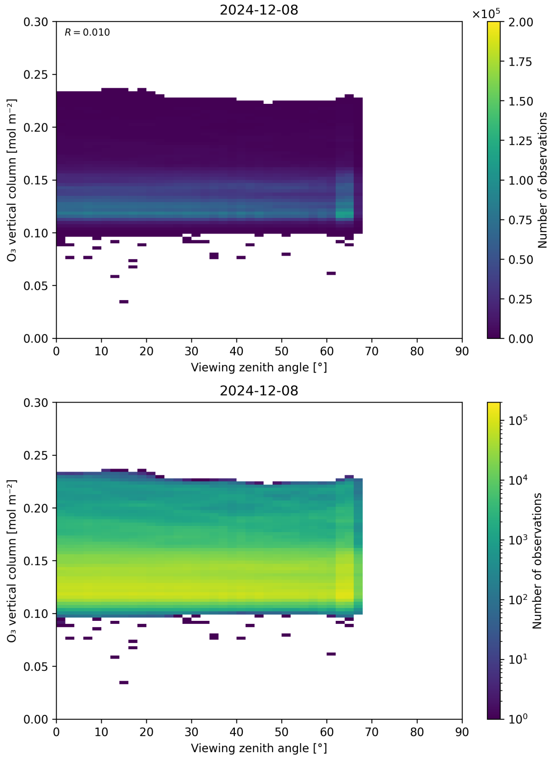
Figure 52: Scatter density plot of “Viewing zenith angle” against “O 3 vertical column” for 2024-12-07 to 2024-12-09.
