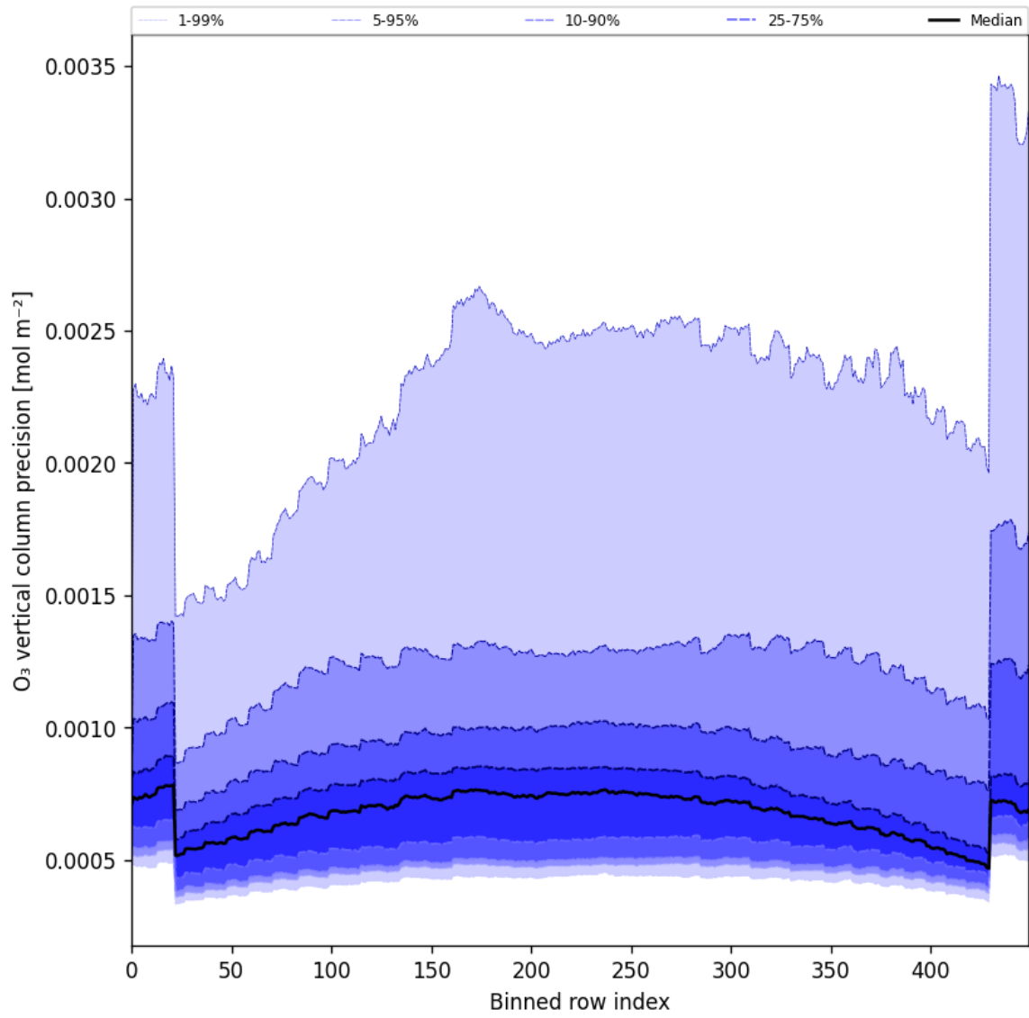
Figure 29: Along track statistics of “O 3 vertical column precision” for 2024-12-07 to 2024-12-09
