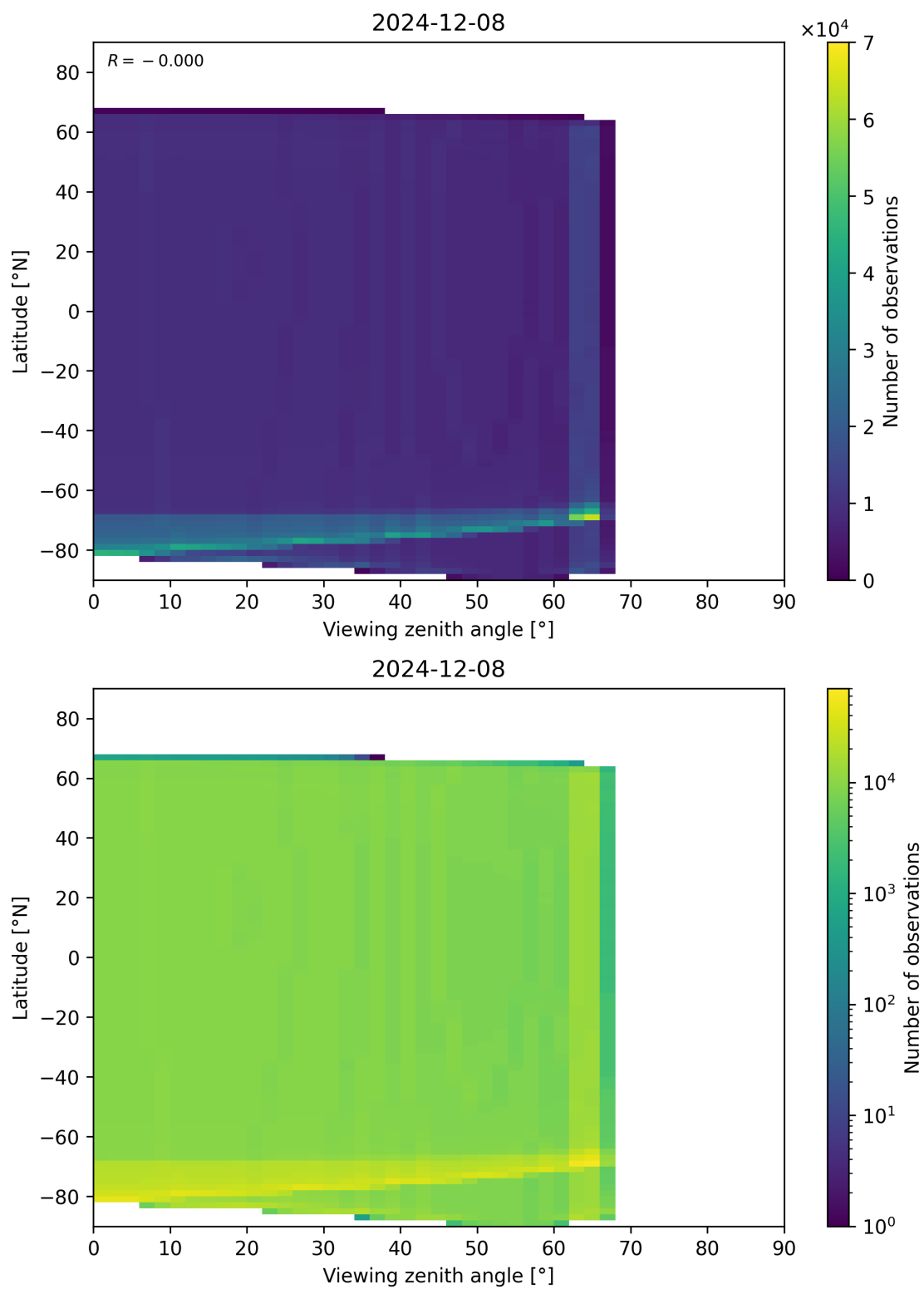
Figure 49: Scatter density plot of “Viewing zenith angle” against “Latitude” for 2024-12-07 to 2024-12-09.
