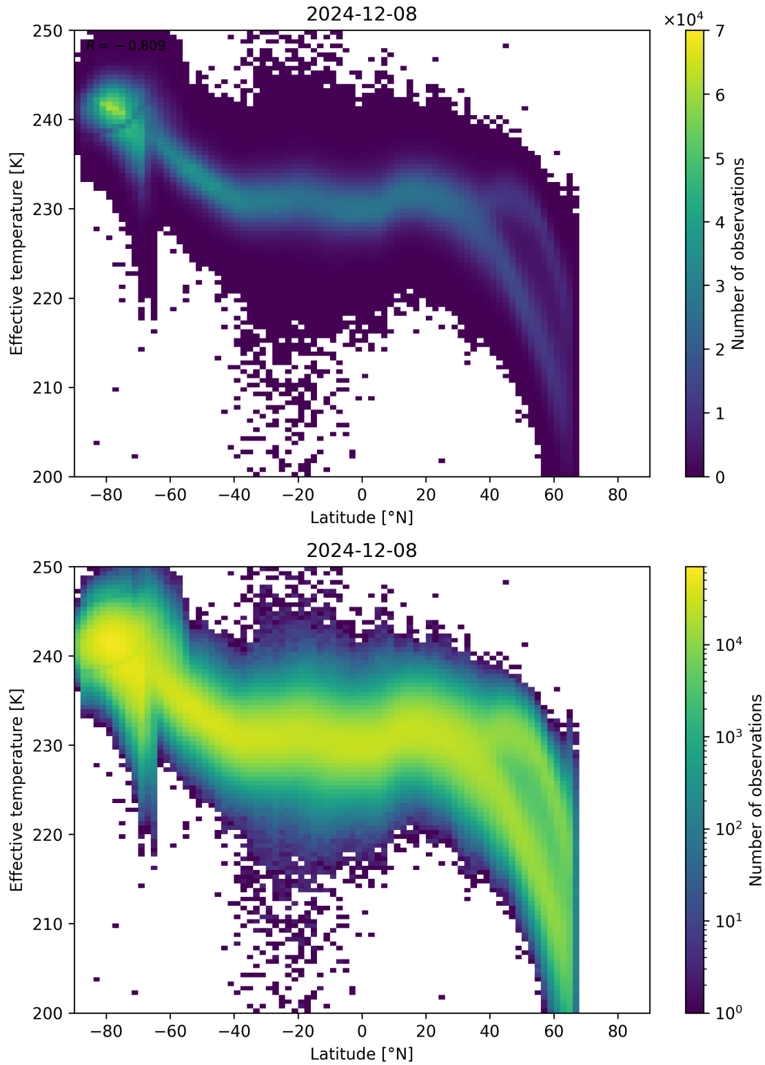
Figure 34: Scatter density plot of “Latitude” against “Effective temperature” for 2024-12-07 to 2024-12-09.
