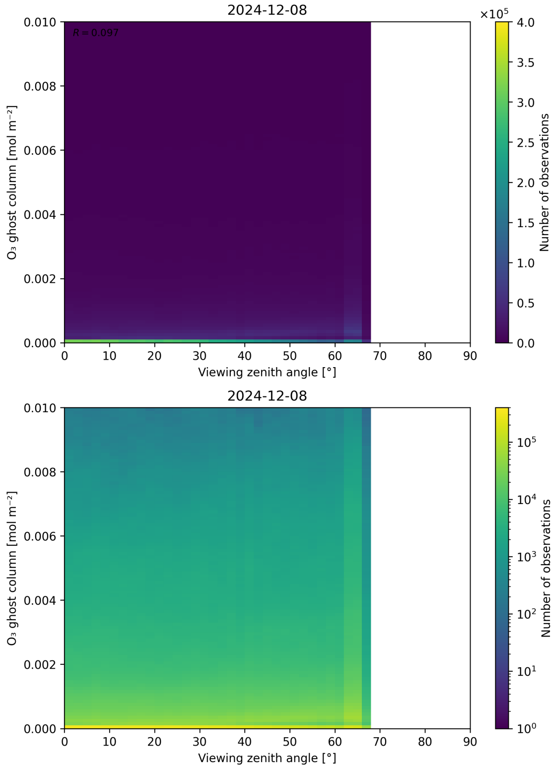
Figure 51: Scatter density plot of “Viewing zenith angle” against “O 3 ghost column” for 2024-12-07 to 2024-12-09.
