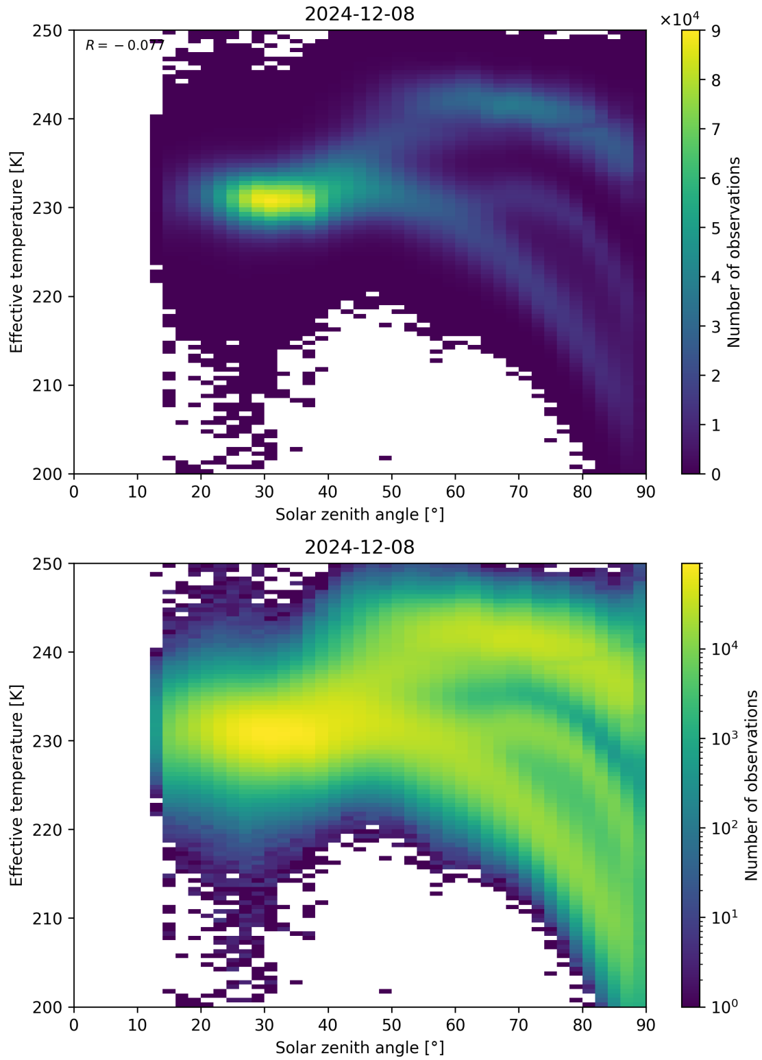
Figure 45: Scatter density plot of “Solar zenith angle” against “Effective temperature” for 2024-12-07 to 2024-12-09.
