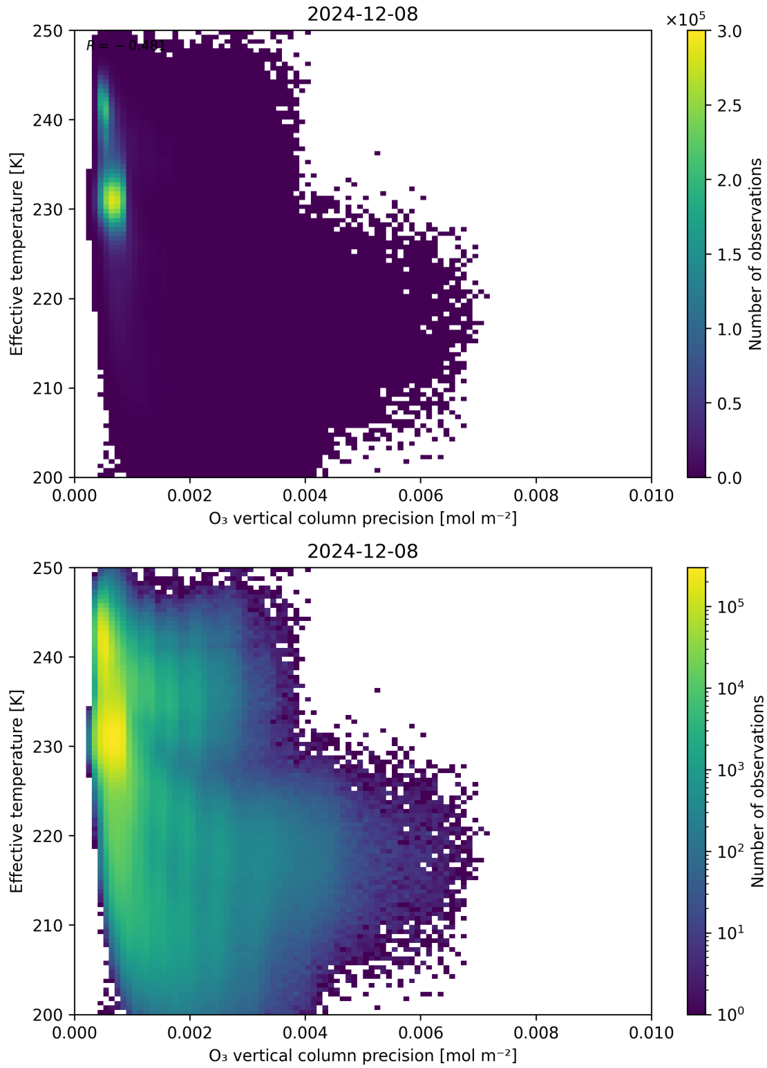
Figure 42: Scatter density plot of “O 3 vertical column precision” against “Effective temperature” for 2024-12-07 to 2024-12-09.
