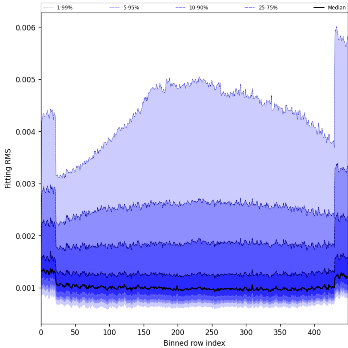
Figure 30: Along track statistics of “Fitting RMS” for 2024-12-07 to 2024-12-09
