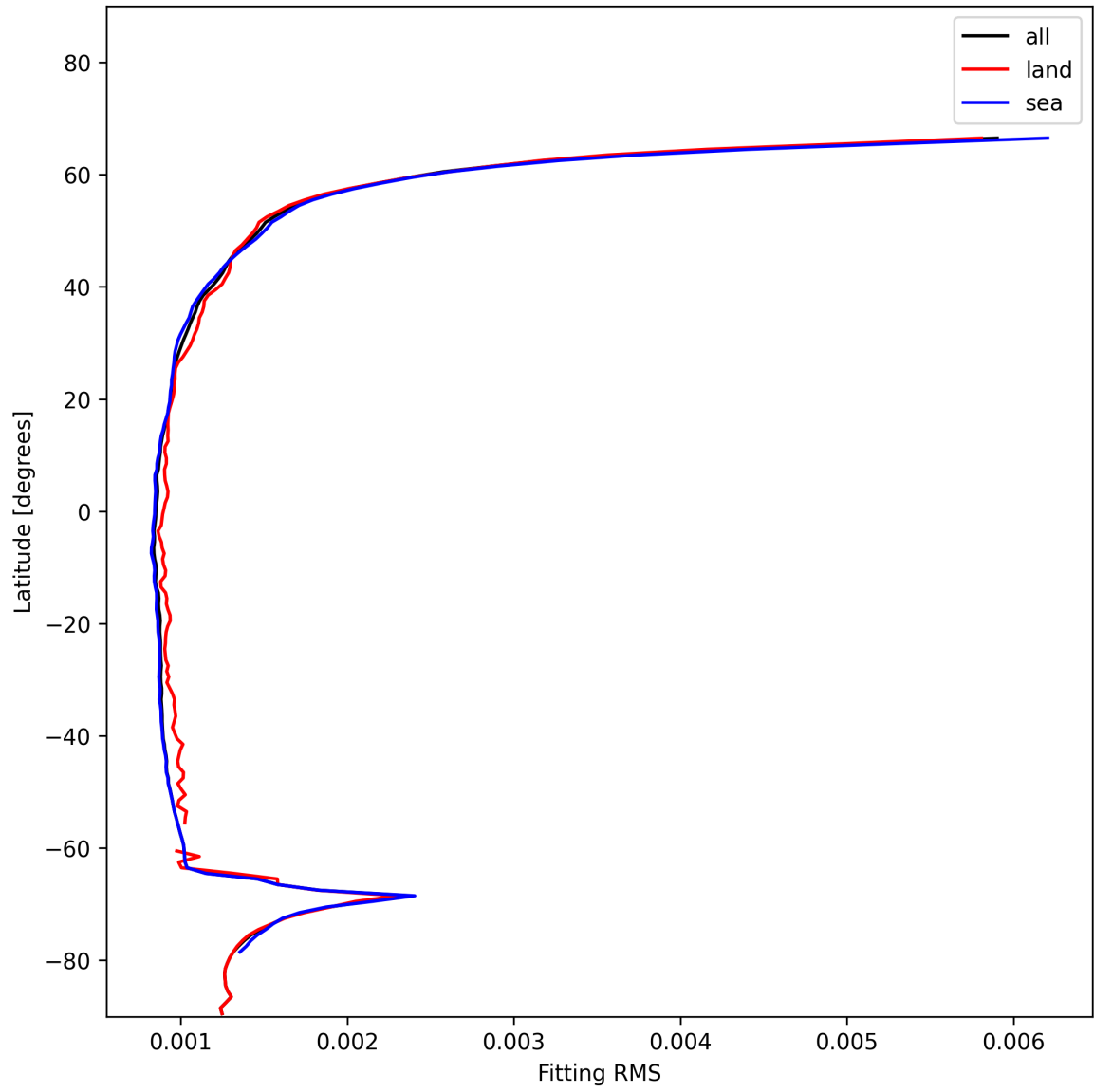
Figure 16: Zonal average of “Fitting RMS” for 2024-12-07 to 2024-12-09.
