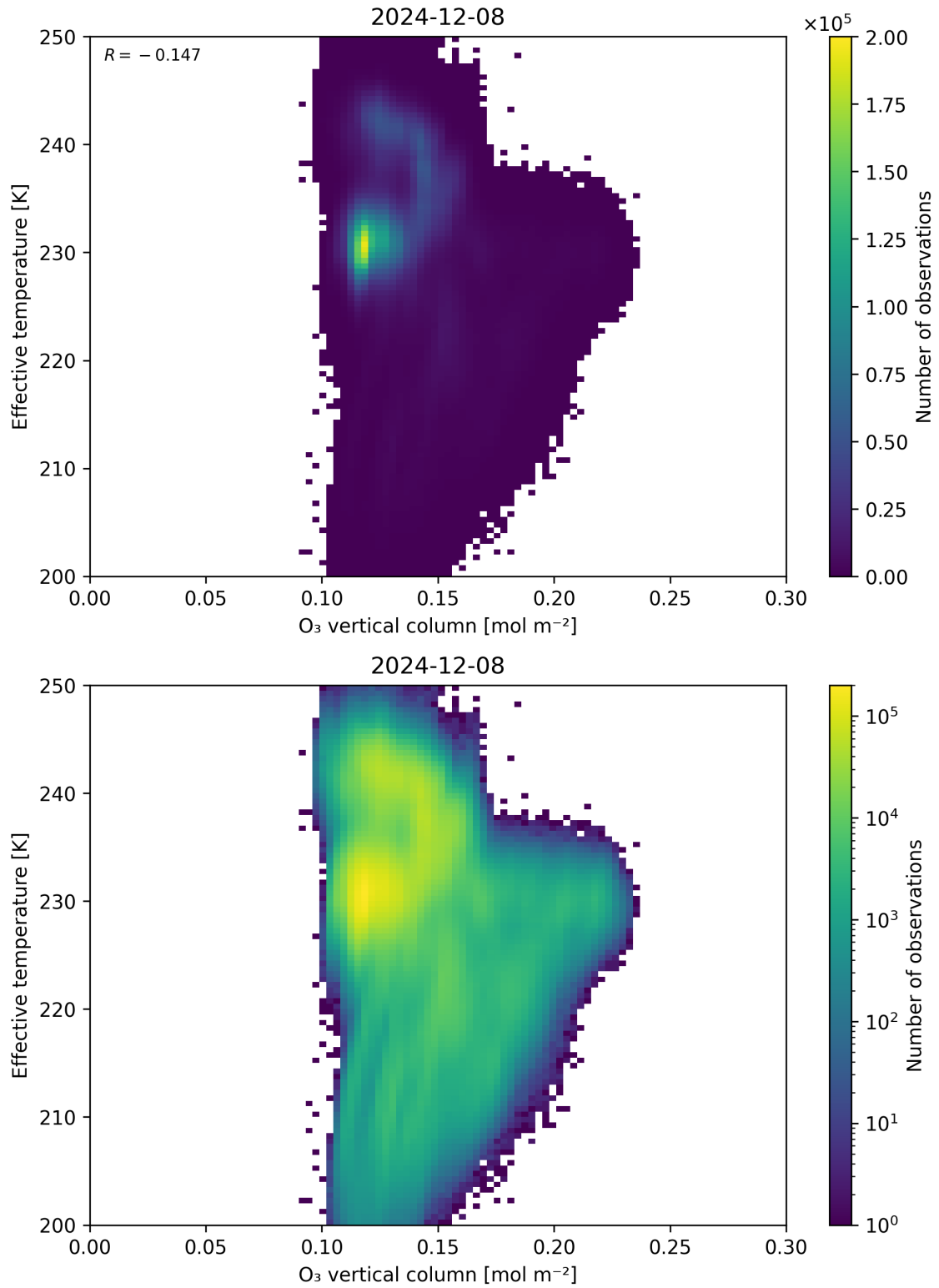
Figure 39: Scatter density plot of “O 3 vertical column” against “Effective temperature” for 2024-12-07 to 2024-12-09.
