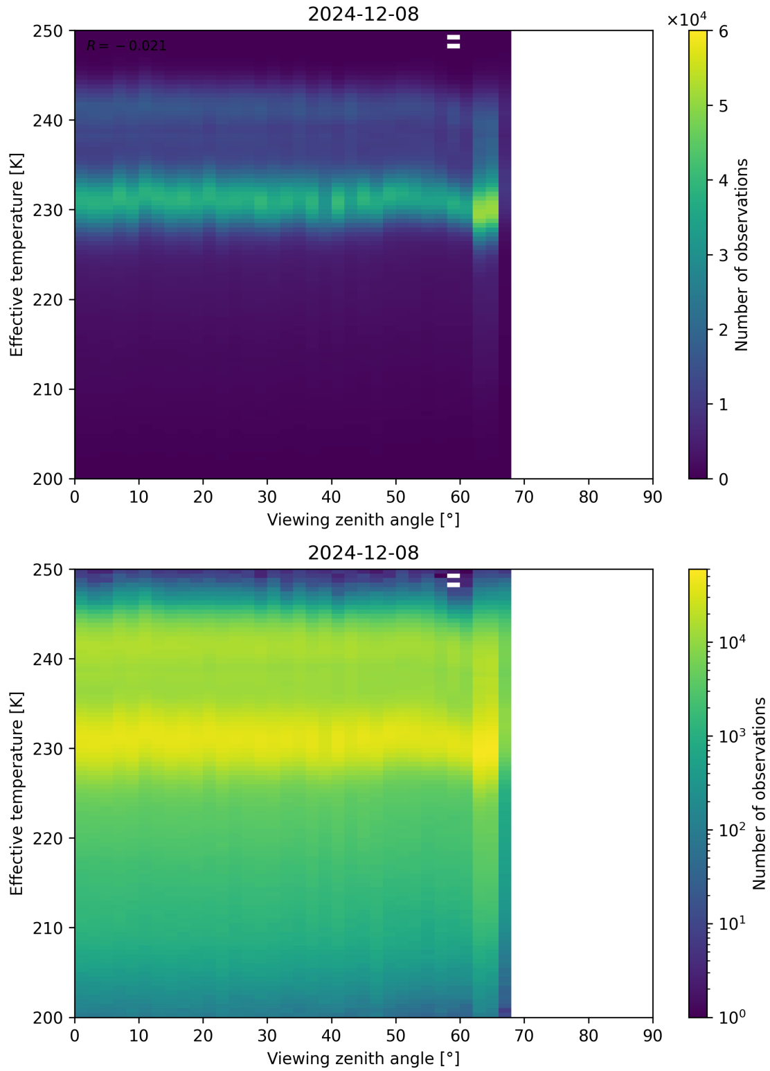
Figure 50: Scatter density plot of “Viewing zenith angle” against “Effective temperature” for 2024-12-07 to 2024-12-09.
