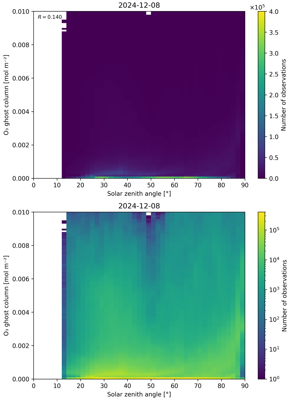
Figure 46: Scatter density plot of “Solar zenith angle” against “O 3 ghost column” for 2024-12-07 to 2024-12-09.
