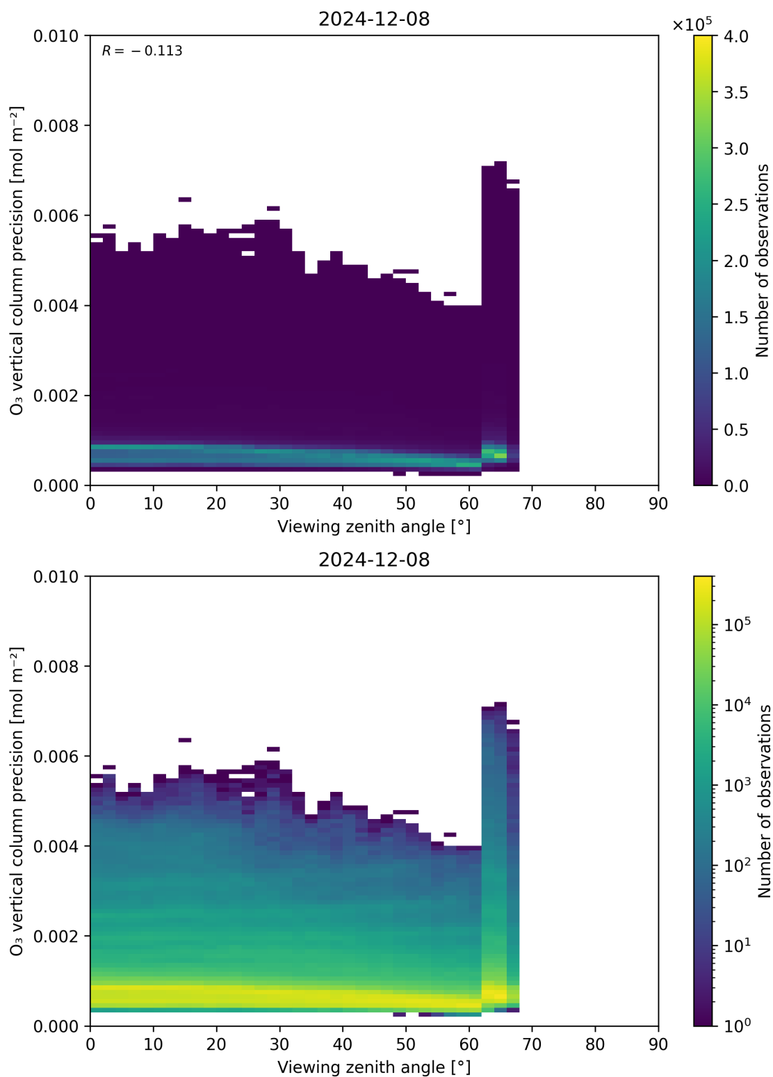
Figure 53: Scatter density plot of “Viewing zenith angle” against “O 3 vertical column precision” for 2024-12-07 to 2024-12-09.
