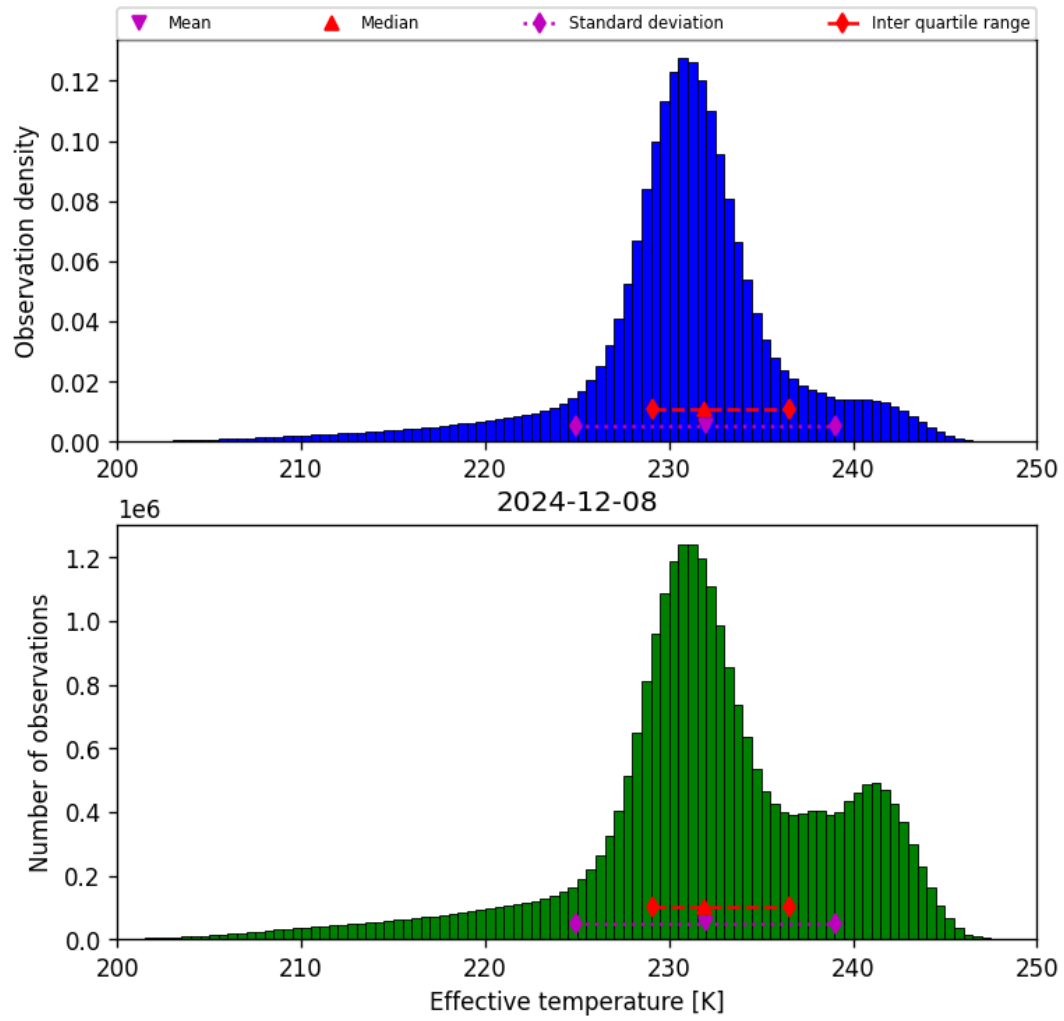
Figure 24: Histogram of “Effective temperature” for 2024-12-07 to 2024-12-09
