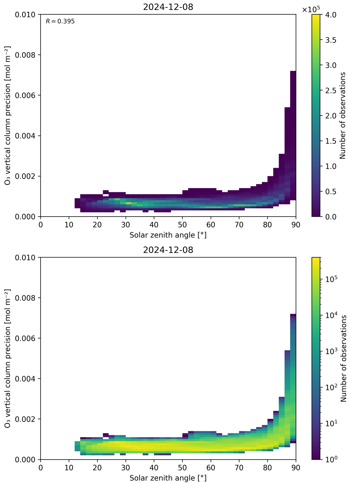
Figure 48: Scatter density plot of “Solar zenith angle” against “O 3 vertical column precision” for 2024-12-07 to 2024-12-09.
