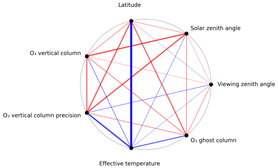
Figure 1: Map of correlation graph for 2024-12-07 to 2024-12-09.
