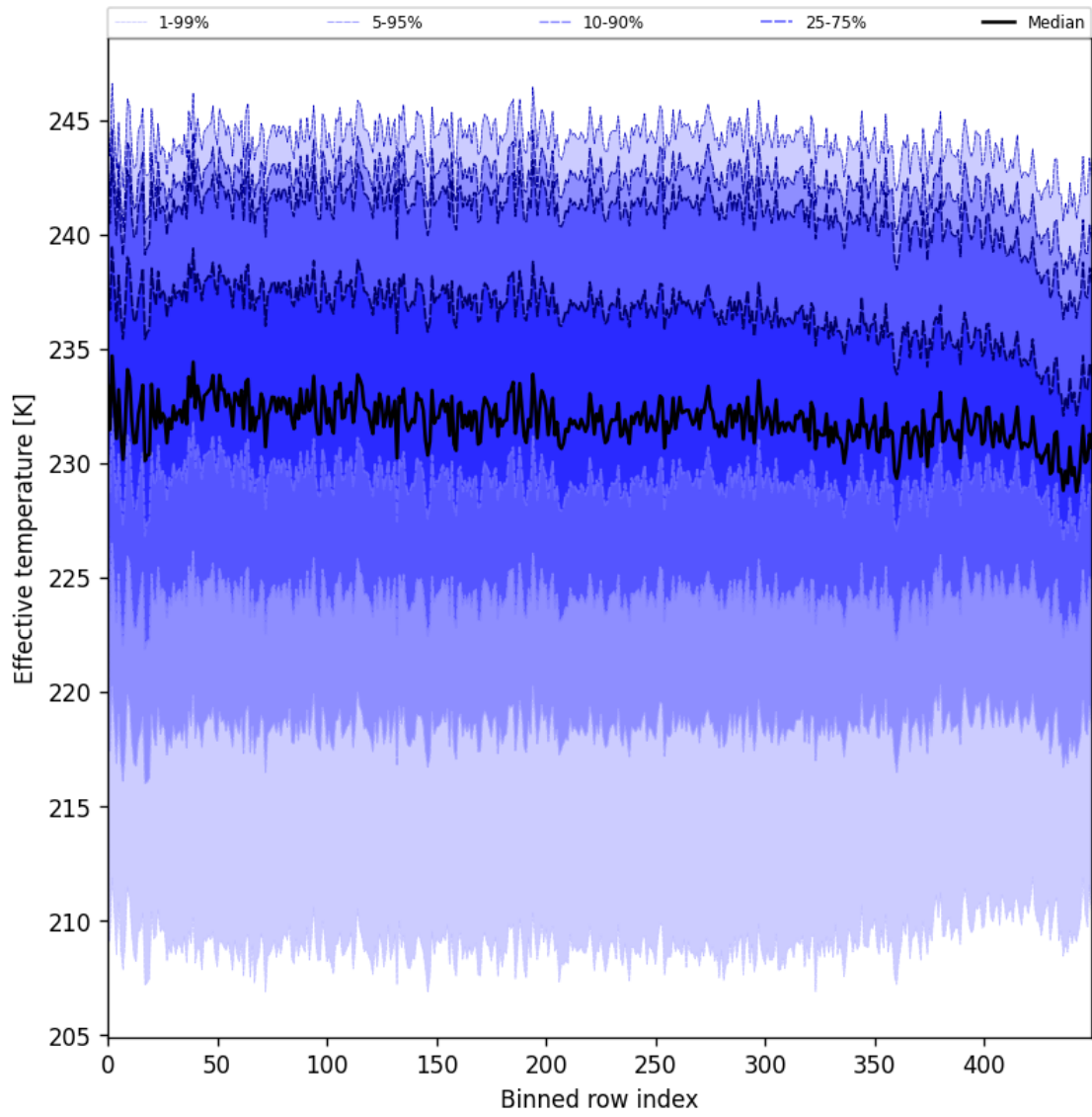
Figure 31: Along track statistics of “Effective temperature” for 2024-12-07 to 2024-12-09
