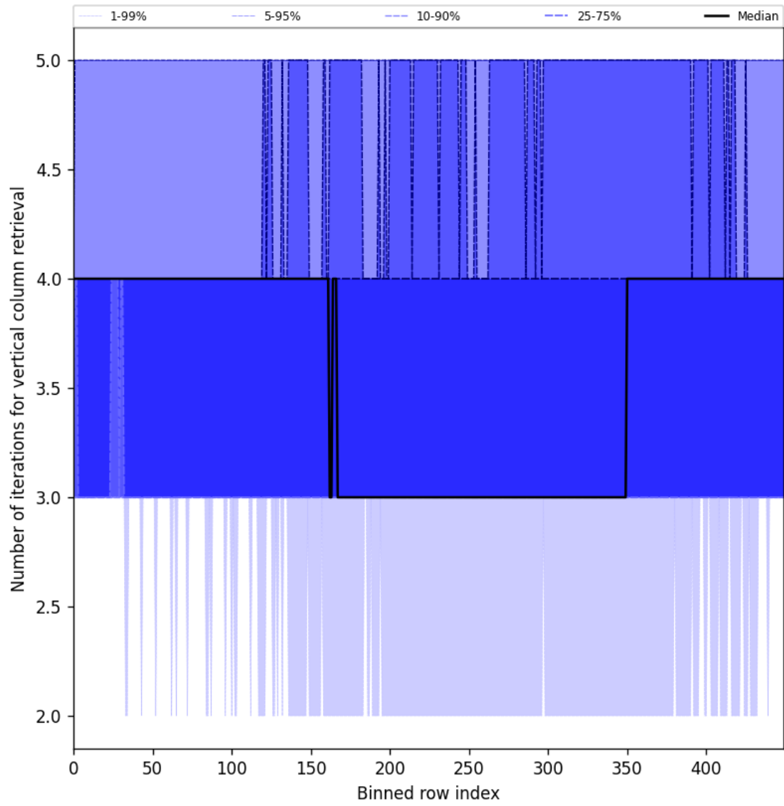
Figure 33: Along track statistics of “Number of iterations for vertical column retrieval” for 2024-12-07 to 2024-12-09
