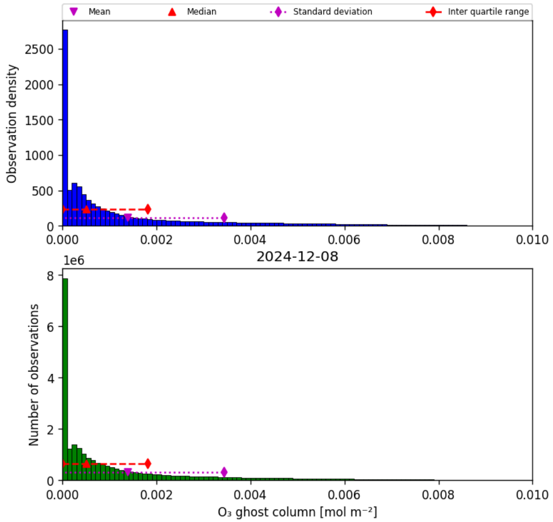
Figure 25: Histogram of “O 3 ghost column” for 2024-12-07 to 2024-12-09
