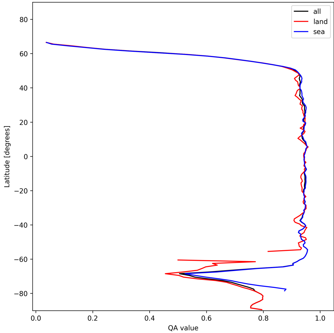
Figure 13: Zonal average of “QA value” for 2024-12-07 to 2024-12-09.
