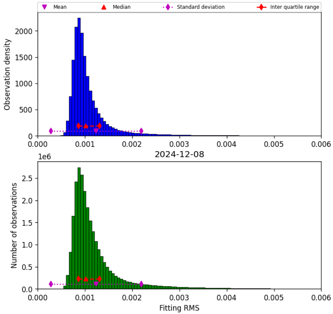
Figure 23: Histogram of “Fitting RMS” for 2024-12-07 to 2024-12-09
