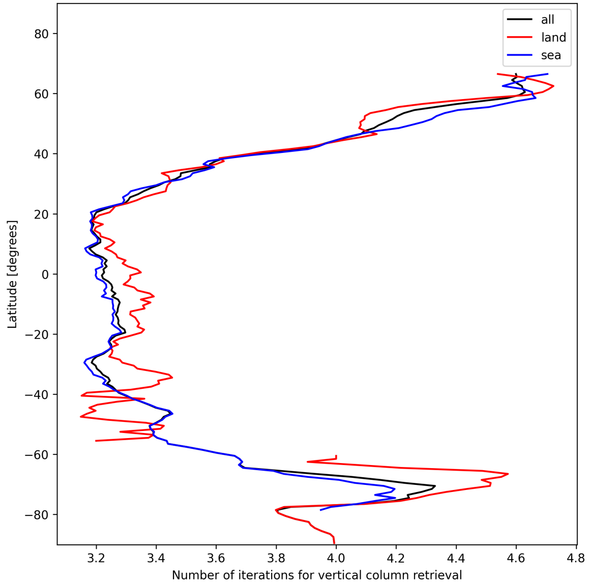
Figure 19: Zonal average of “Number of iterations for vertical column retrieval” for 2024-12-07 to 2024-12-09.
