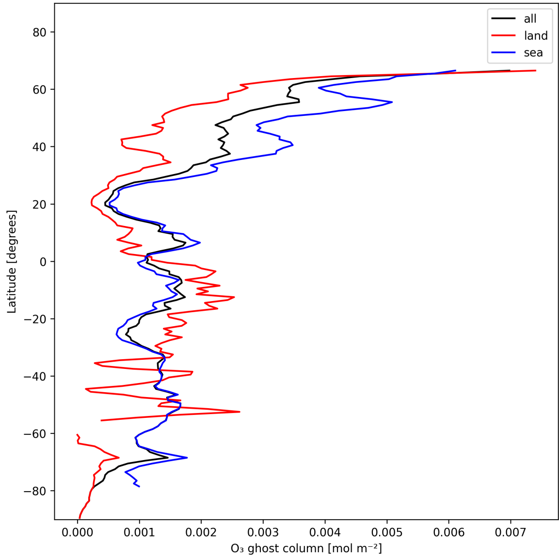
Figure 18: Zonal average of “O 3 ghost column” for 2024-12-07 to 2024-12-09.
