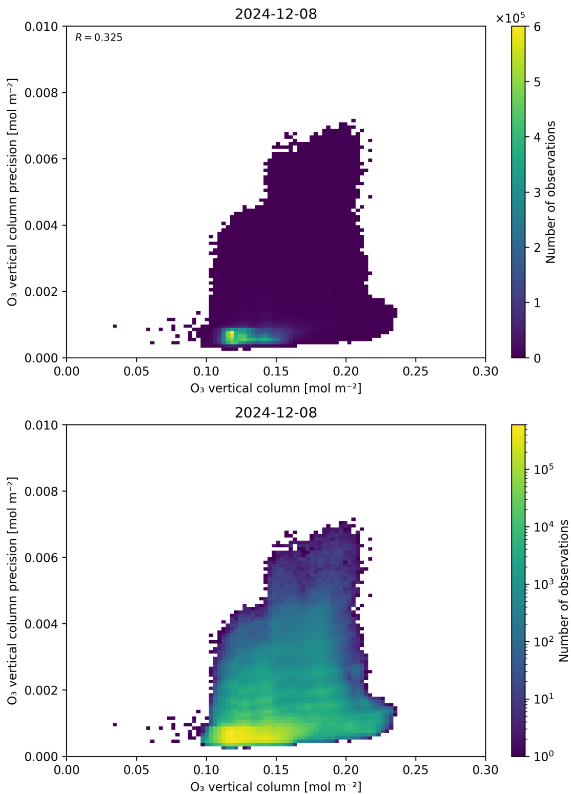
Figure 41: Scatter density plot of “O 3 vertical column” against “O 3 vertical column precision” for 2024-12-07 to 2024-12-09.
