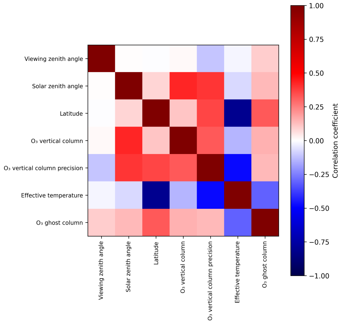
Figure 2: Map of correlation matrix for 2024-12-07 to 2024-12-09.
