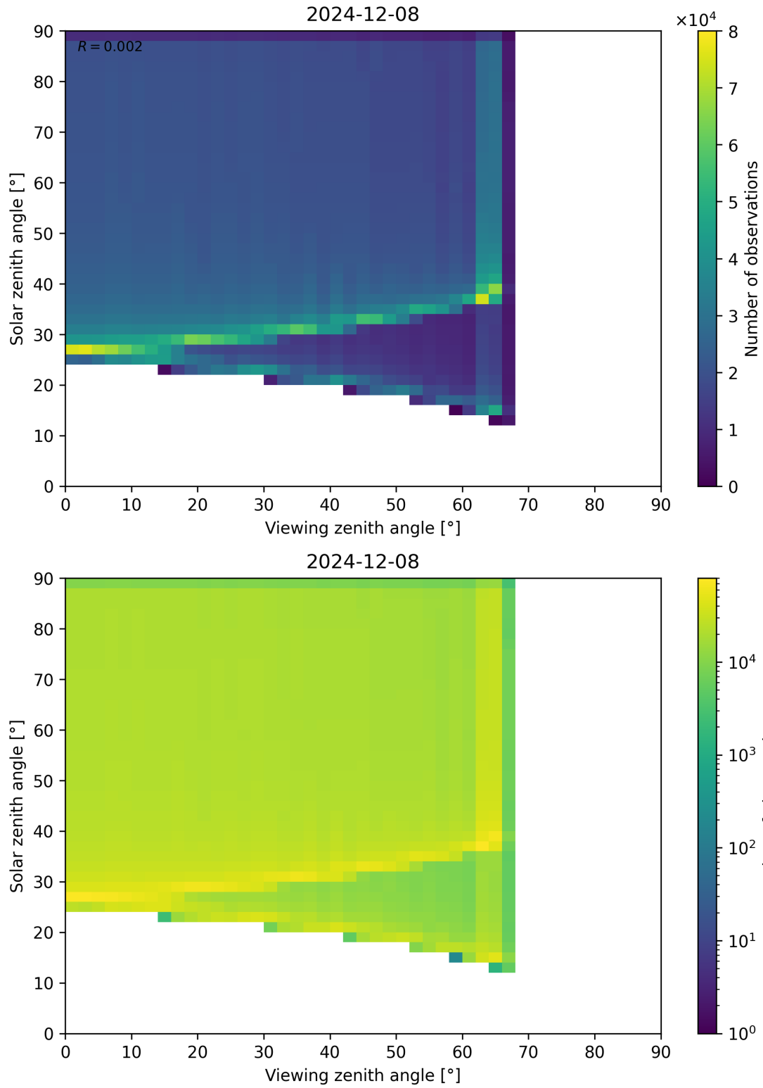
Figure 54: Scatter density plot of “Viewing zenith angle” against “Solar zenith angle” for 2024-12-07 to 2024-12-09.
