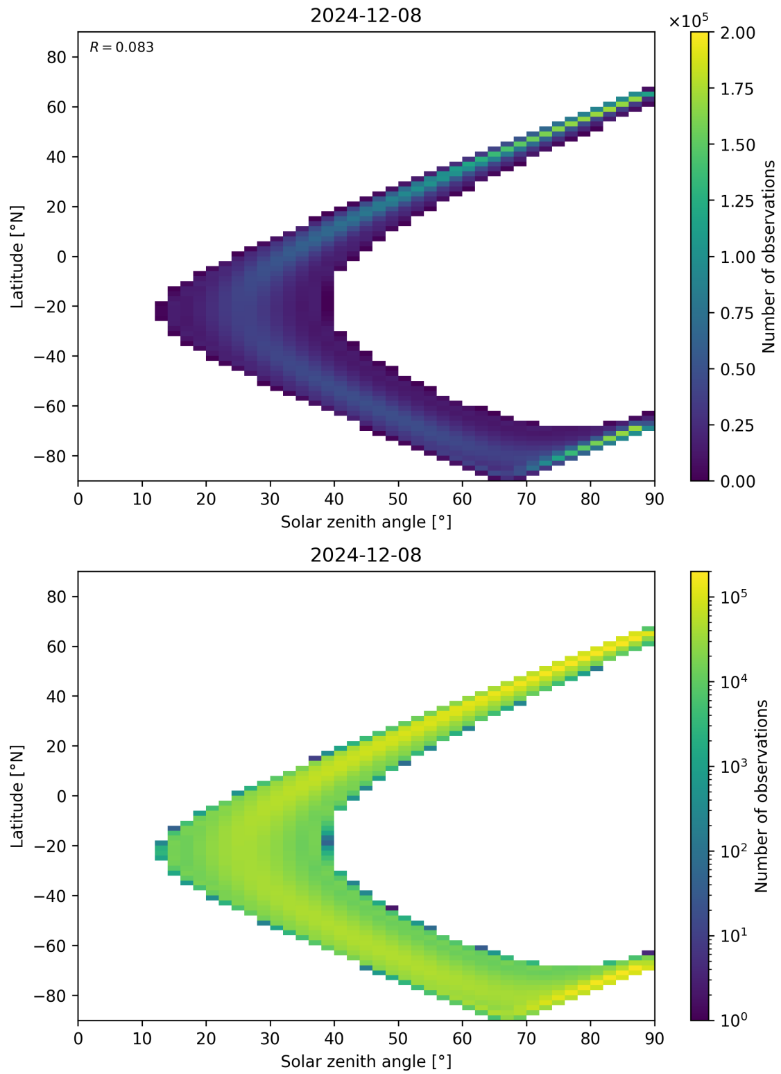
Figure 44: Scatter density plot of “Solar zenith angle” against “Latitude” for 2024-12-07 to 2024-12-09.
