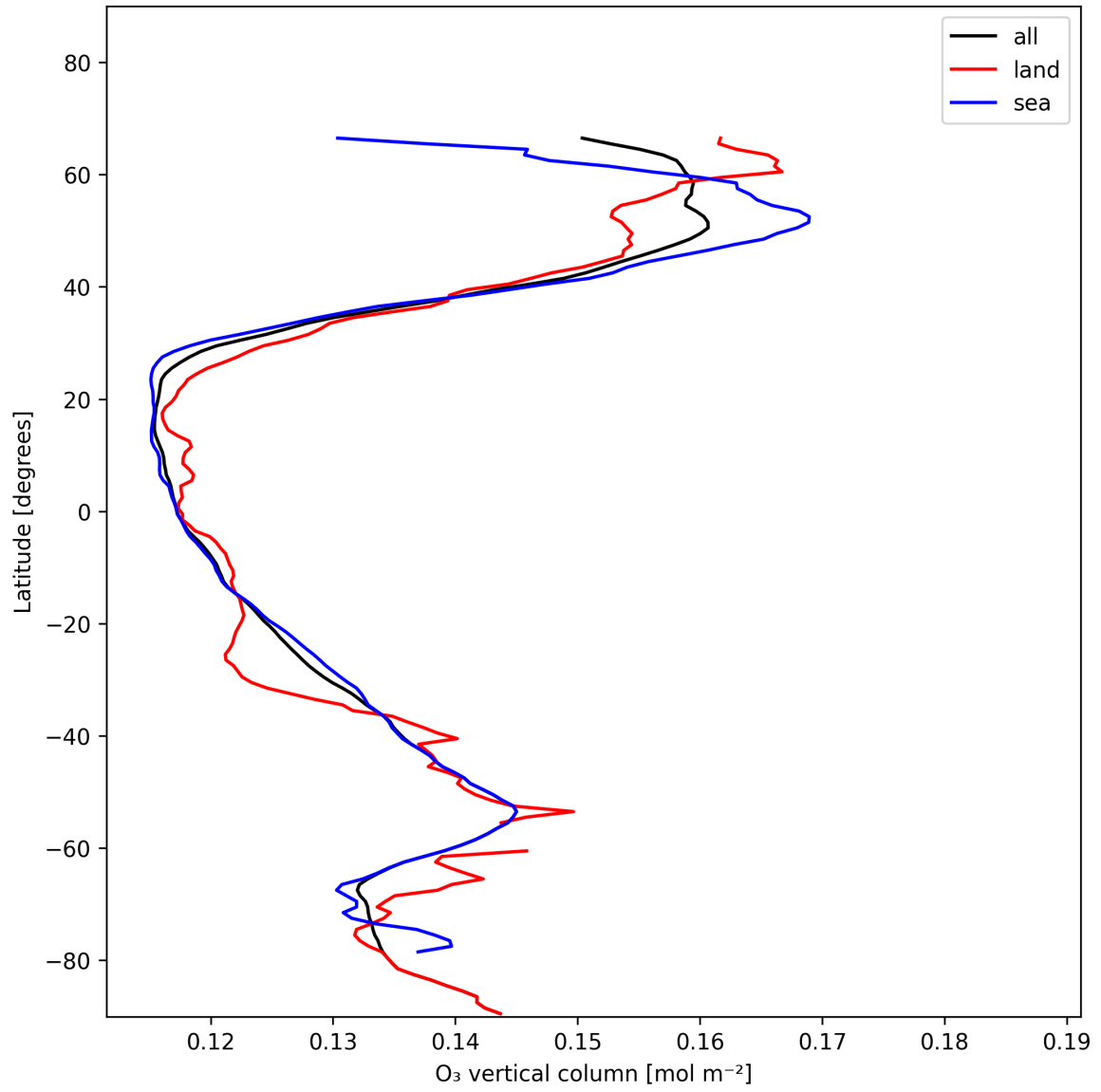
Figure 14: Zonal average of “O 3 vertical column” for 2024-12-07 to 2024-12-09.
