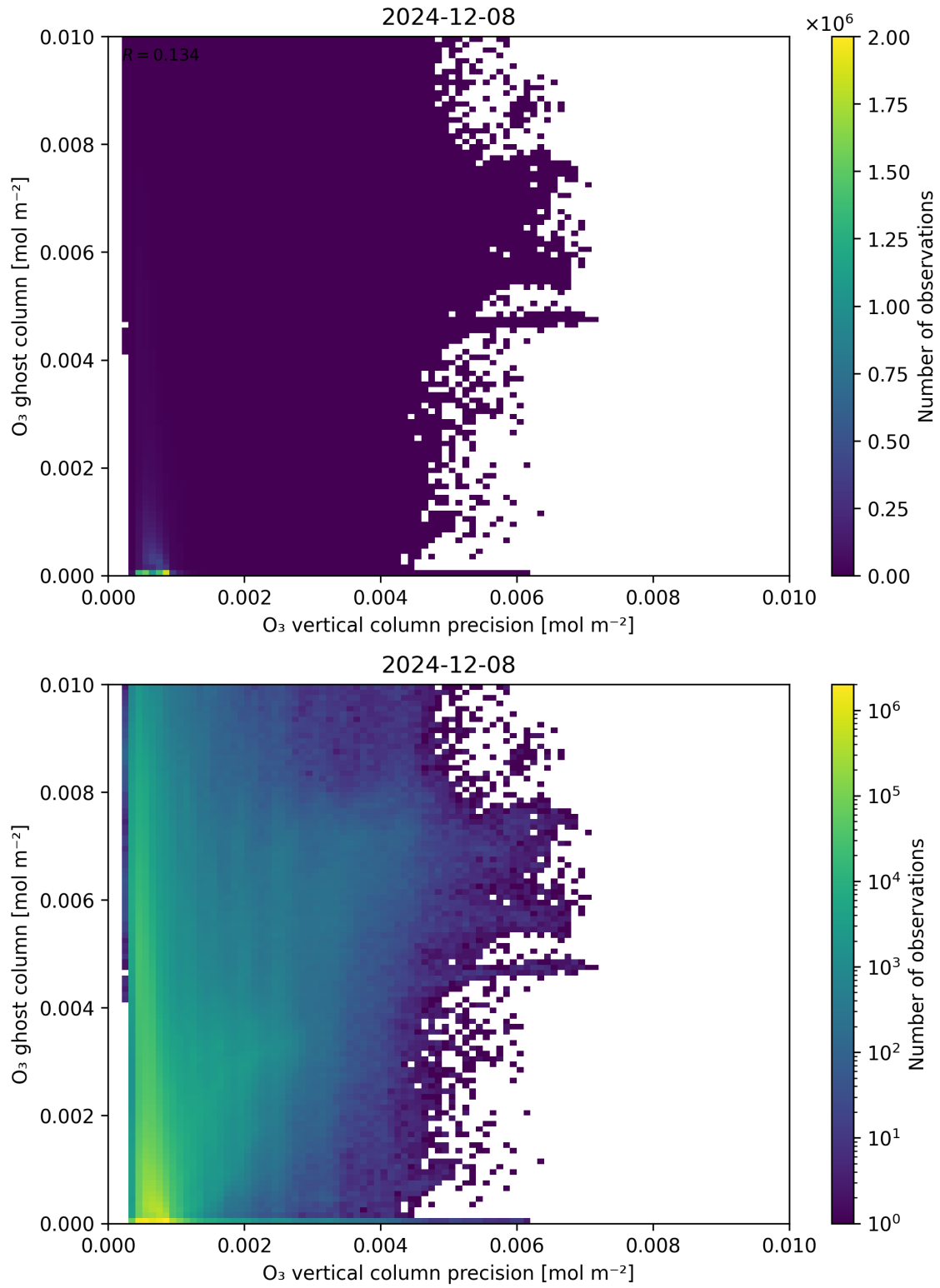
Figure 43: Scatter density plot of “ \text{O}_3 vertical column precision” against “ \text{O}_3 ghost column” for 2024-12-07 to 2024-12-09.
