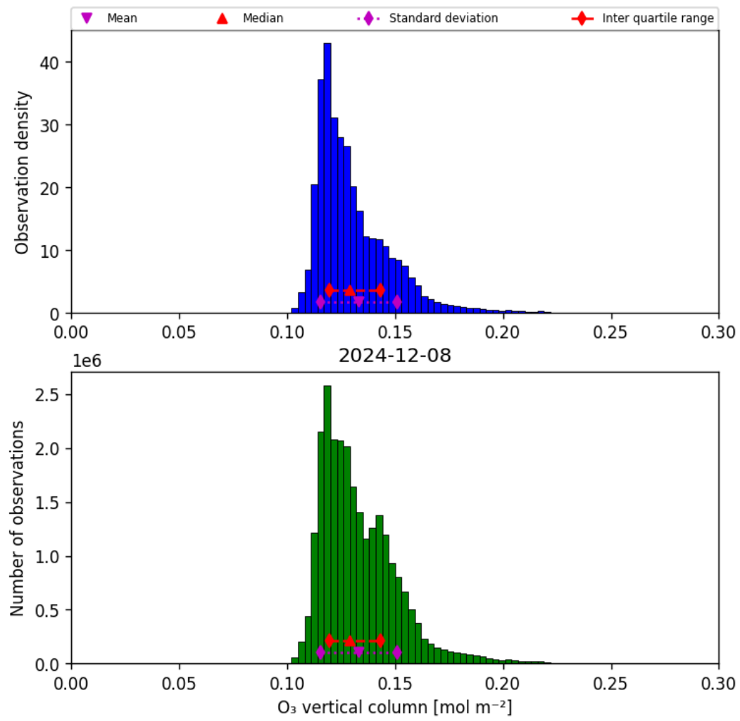
Figure 21: Histogram of “O 3 vertical column” for 2024-12-07 to 2024-12-09
