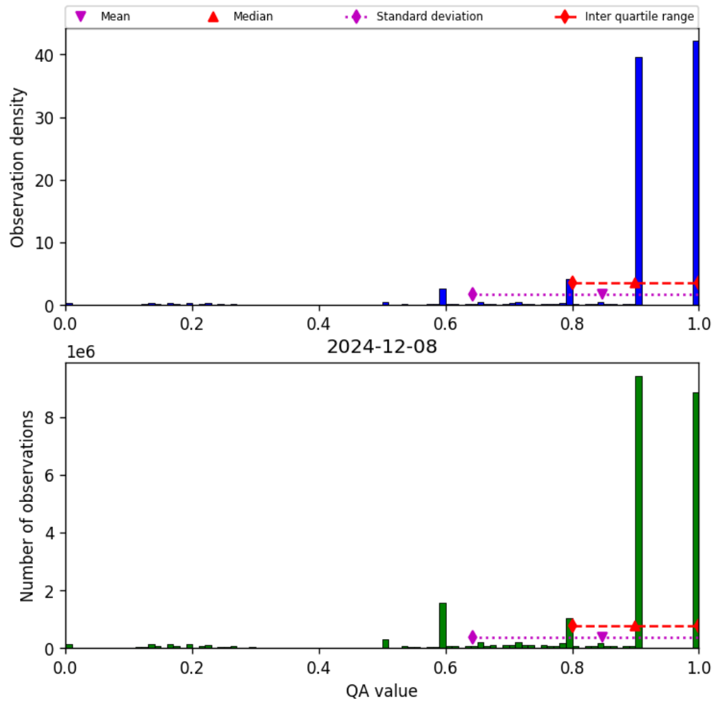
Figure 20: Histogram of “QA value” for 2024-12-07 to 2024-12-09
