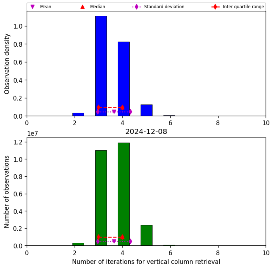
Figure 26: Histogram of “Number of iterations for vertical column retrieval” for 2024-12-07 to 2024-12-09
