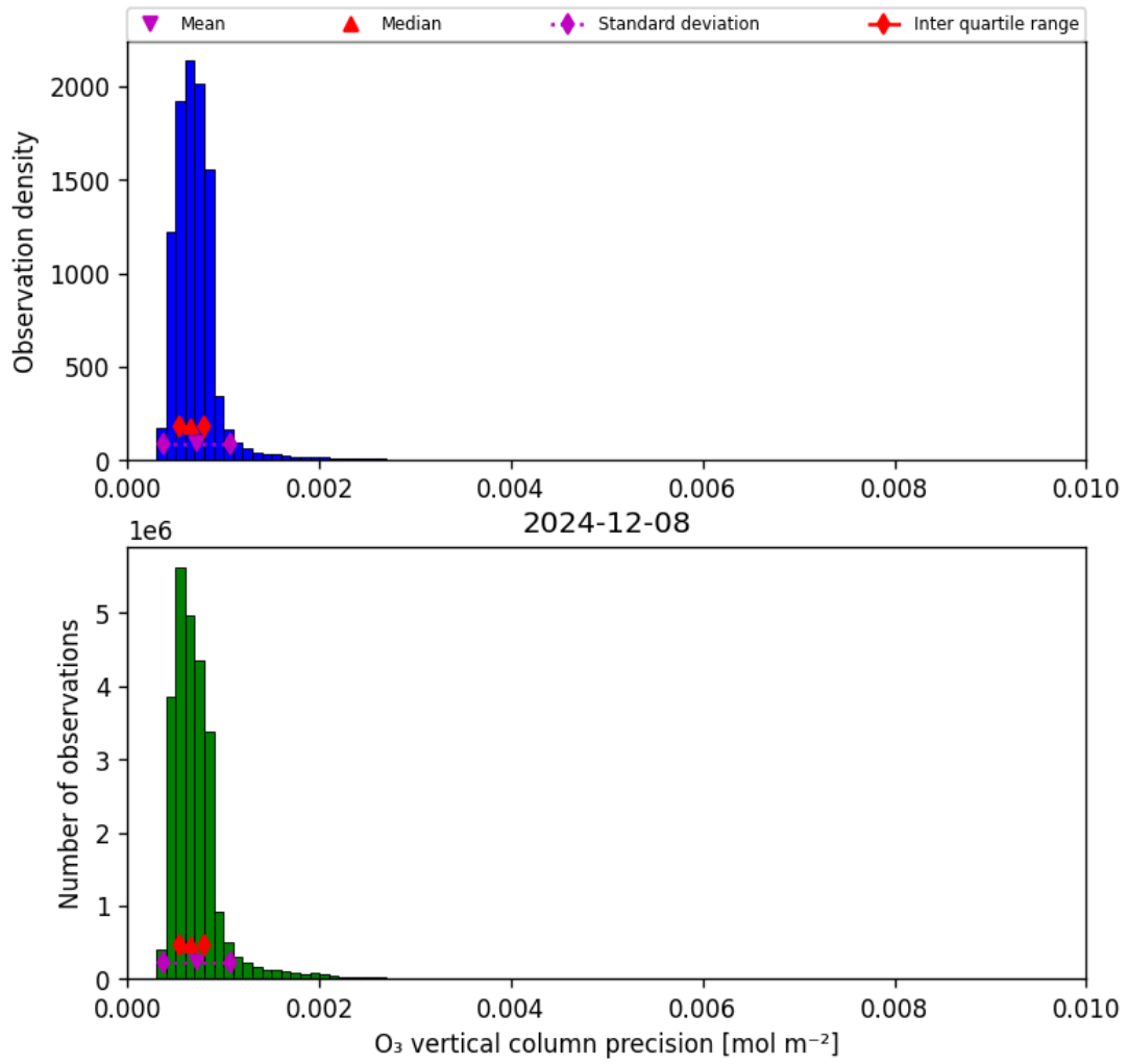
Figure 22: Histogram of “O 3 vertical column precision” for 2024-12-07 to 2024-12-09
