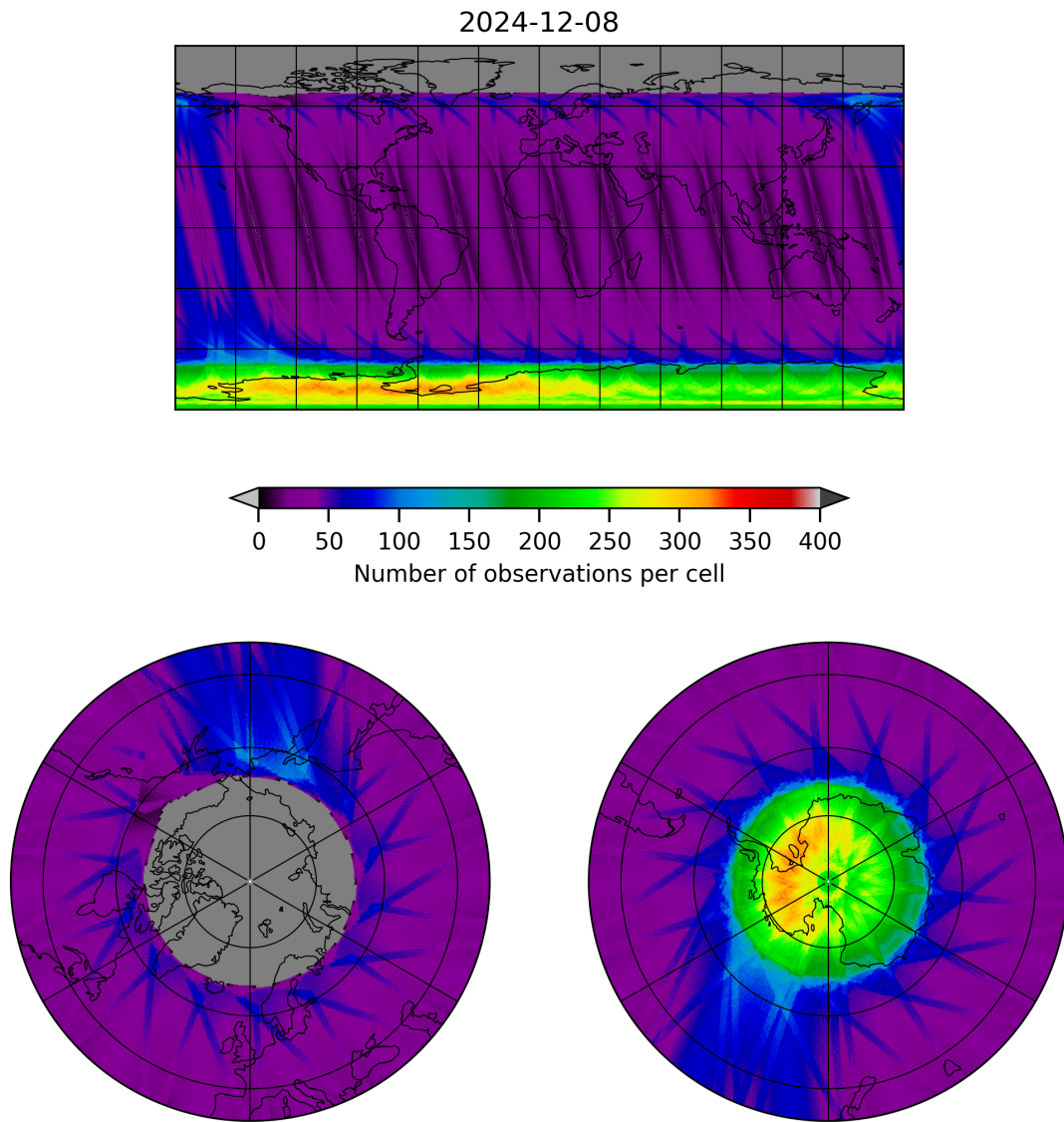
Figure 12: Map of the number of observations for 2024-12-07 to 2024-12-09
