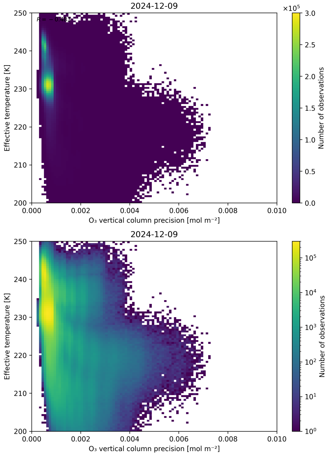
Figure 42: Scatter density plot of “O 3 vertical column precision” against “Effective temperature” for 2024-12-08 to 2024-12-10.
