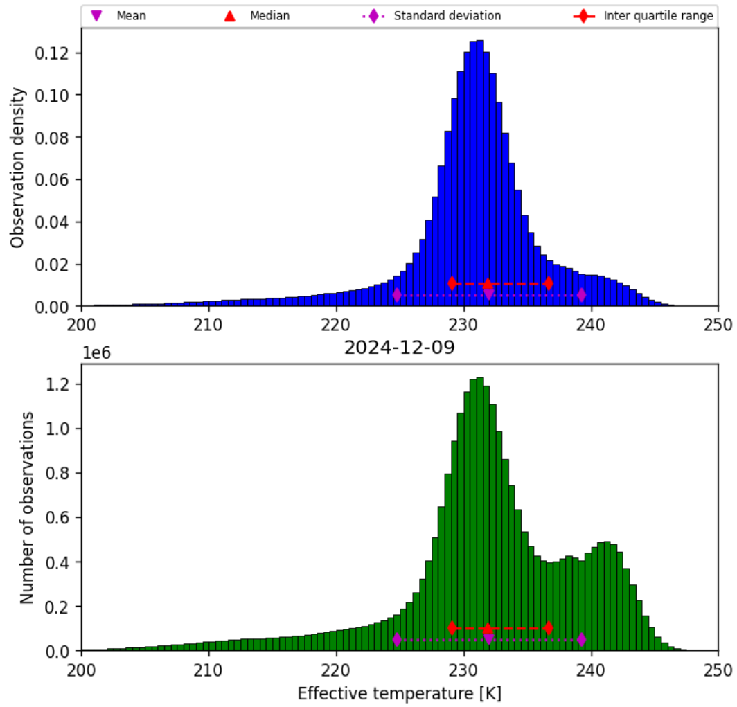
Figure 24: Histogram of “Effective temperature” for 2024-12-08 to 2024-12-10
