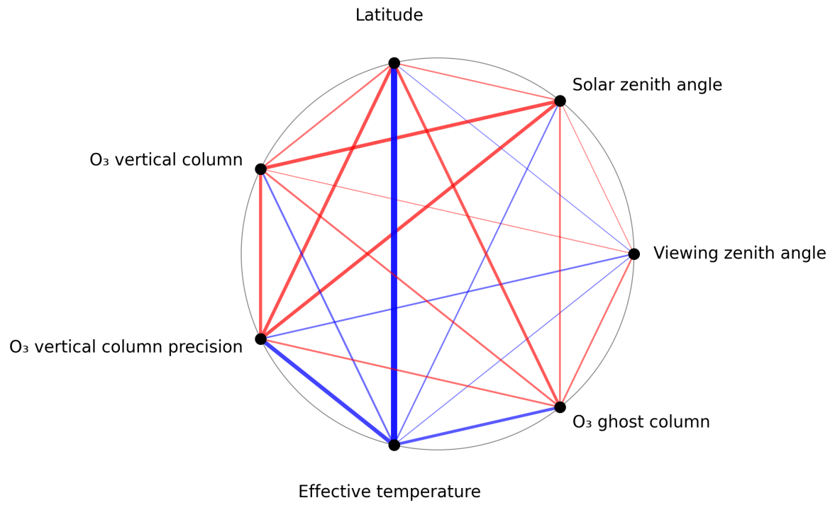
Figure 1: Map of correlation graph for 2024-12-08 to 2024-12-10.
