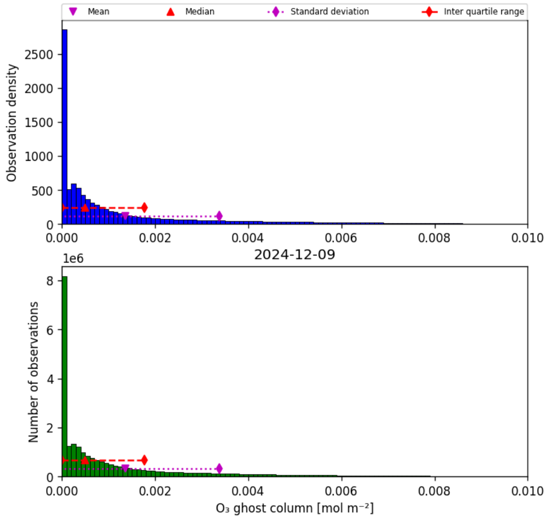
Figure 25: Histogram of “O 3 ghost column” for 2024-12-08 to 2024-12-10
