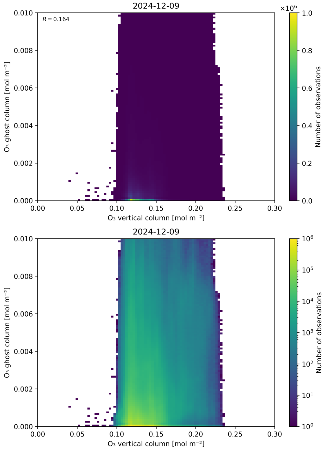
Figure 40: Scatter density plot of “O 3 vertical column” against “O 3 ghost column” for 2024-12-08 to 2024-12-10.
