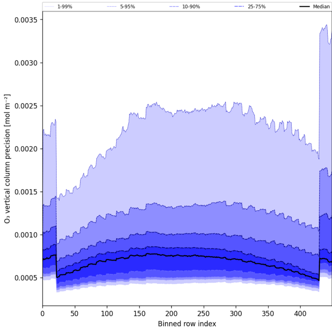
Figure 29: Along track statistics of “O 3 vertical column precision” for 2024-12-08 to 2024-12-10
