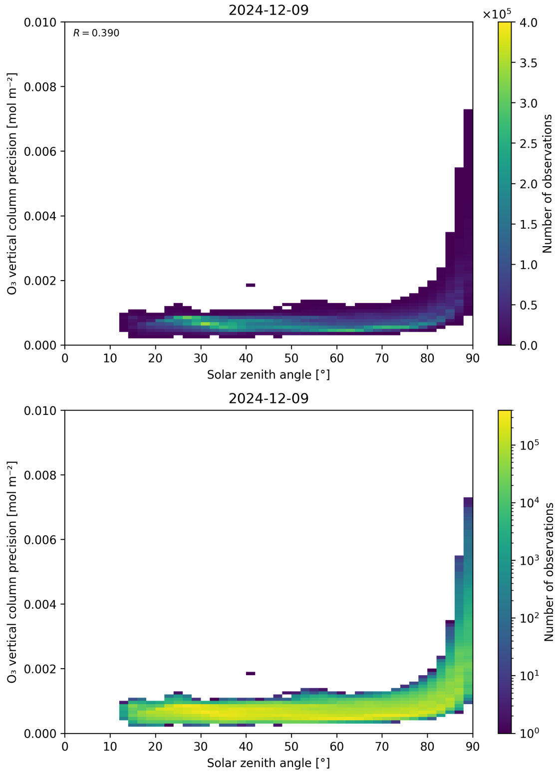
Figure 48: Scatter density plot of “Solar zenith angle” against “O 3 vertical column precision” for 2024-12-08 to 2024-12-10.
