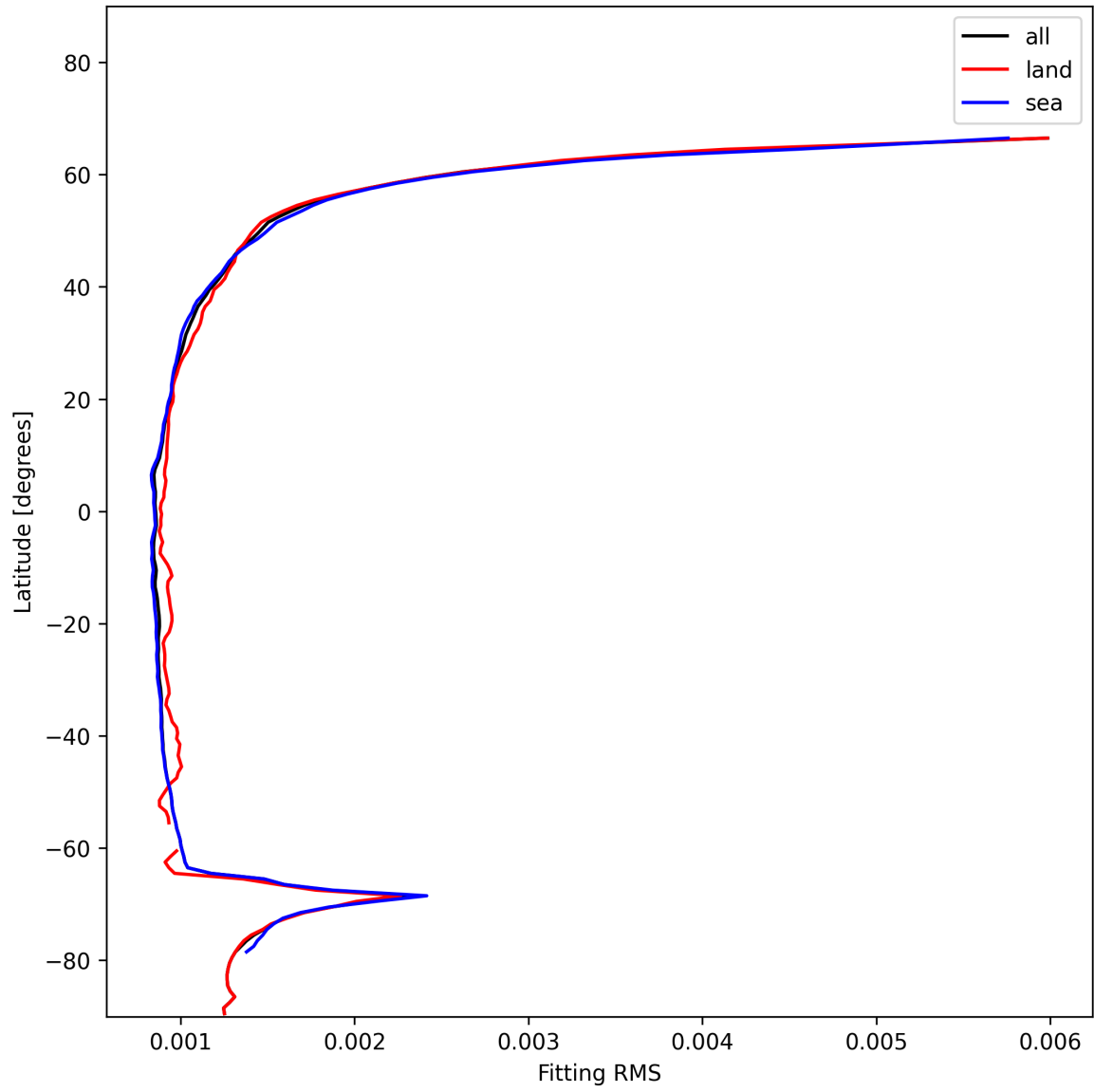
Figure 16: Zonal average of “Fitting RMS” for 2024-12-08 to 2024-12-10.
