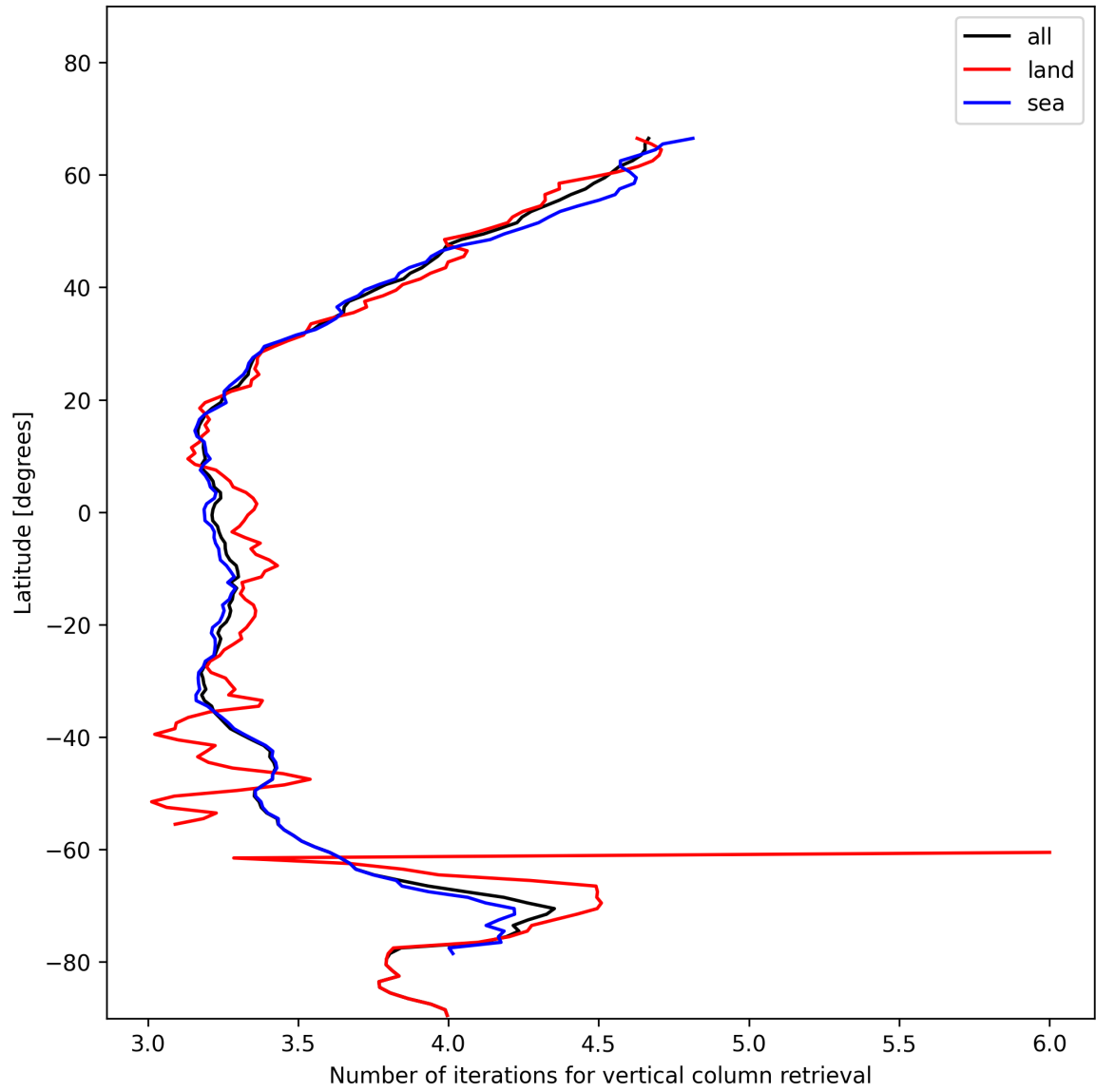
Figure 19: Zonal average of “Number of iterations for vertical column retrieval” for 2024-12-08 to 2024-12-10.
