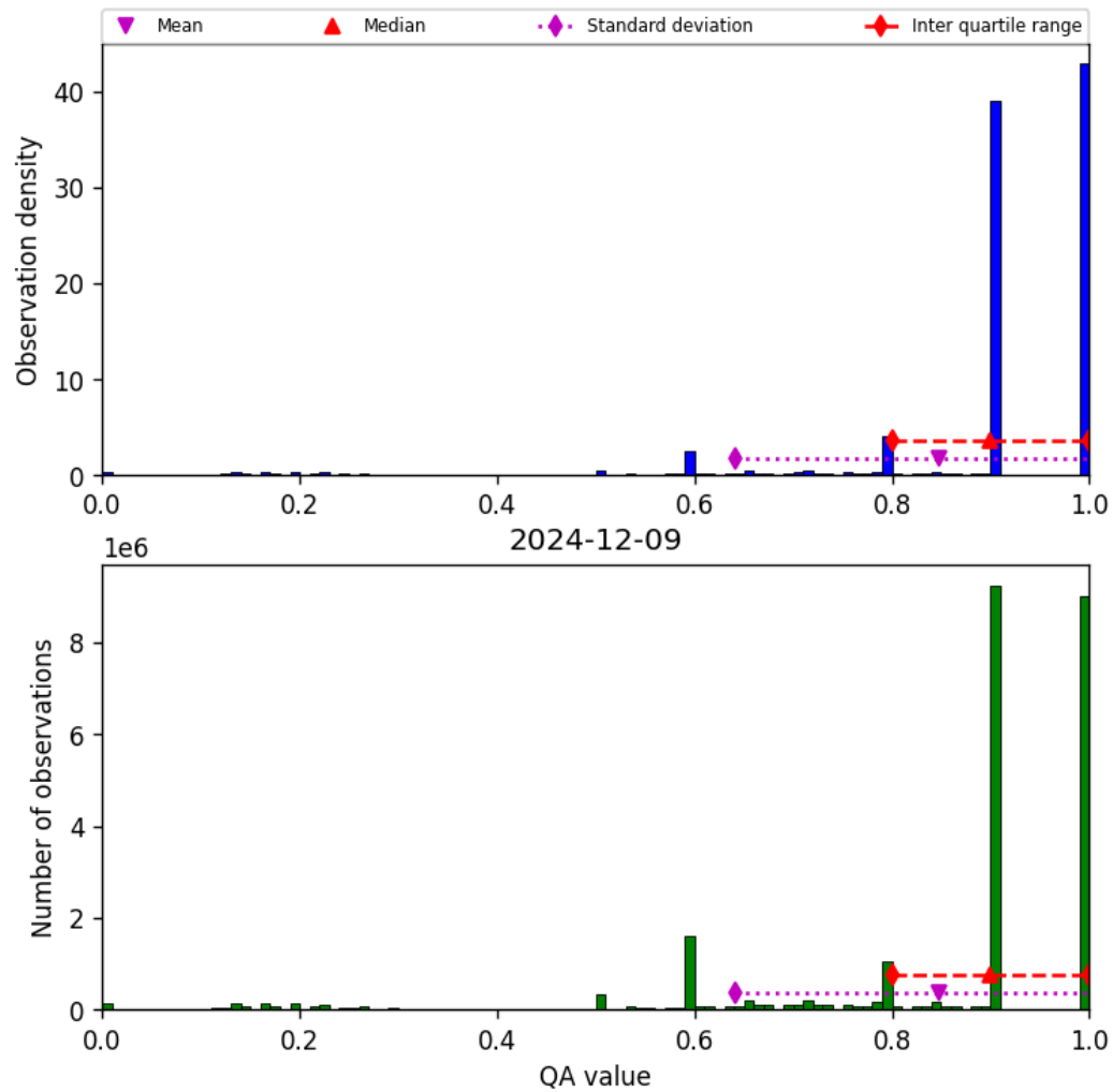
Figure 20: Histogram of “QA value” for 2024-12-08 to 2024-12-10
