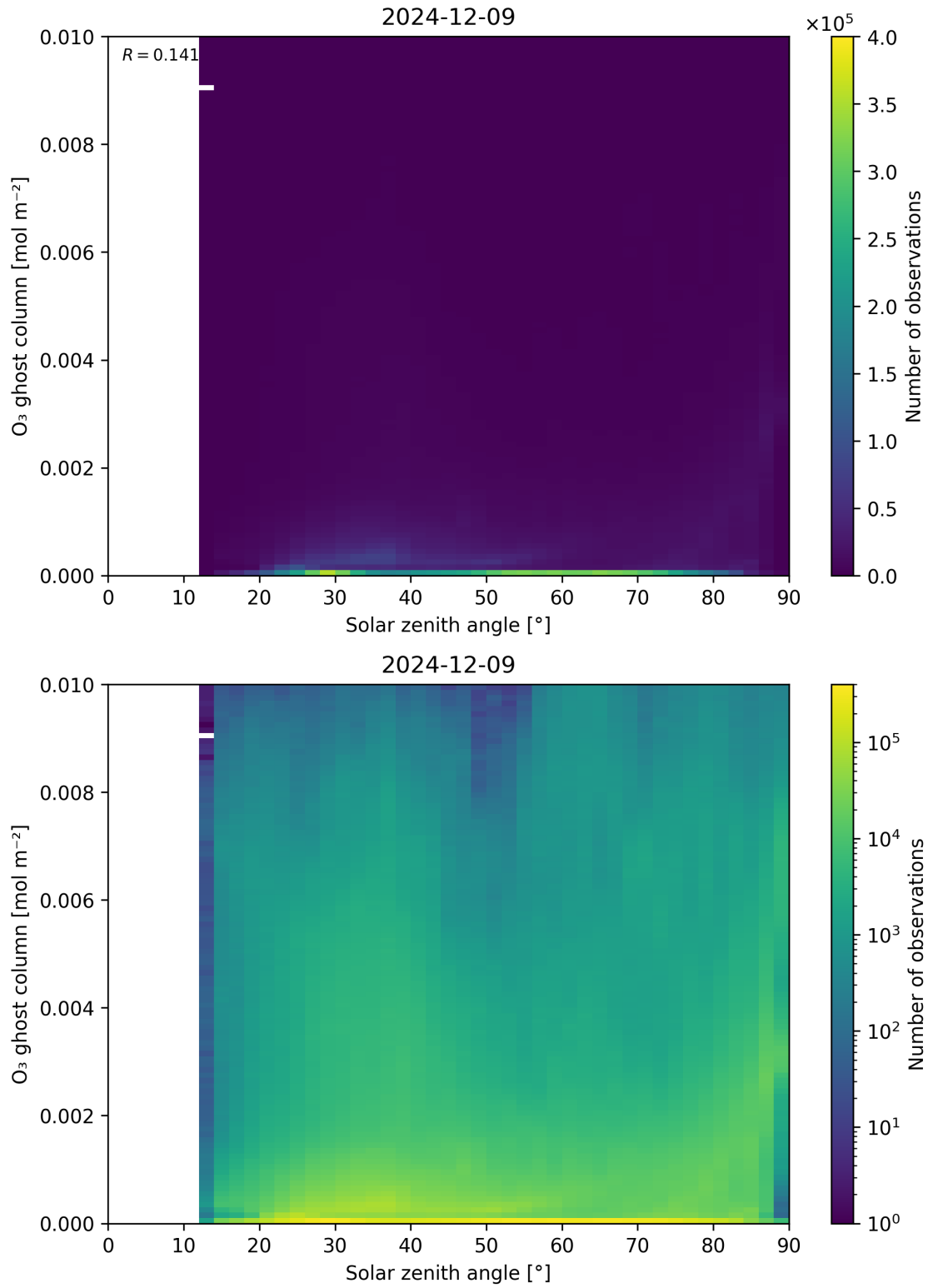
Figure 46: Scatter density plot of “Solar zenith angle” against “O 3 ghost column” for 2024-12-08 to 2024-12-10.
