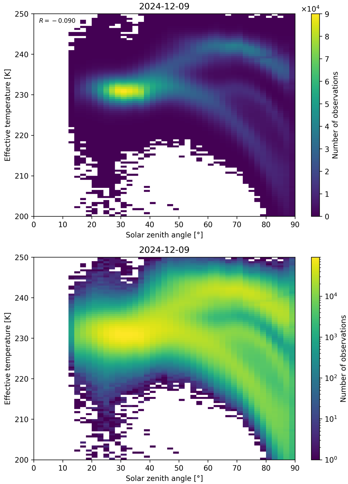
Figure 45: Scatter density plot of “Solar zenith angle” against “Effective temperature” for 2024-12-08 to 2024-12-10.
