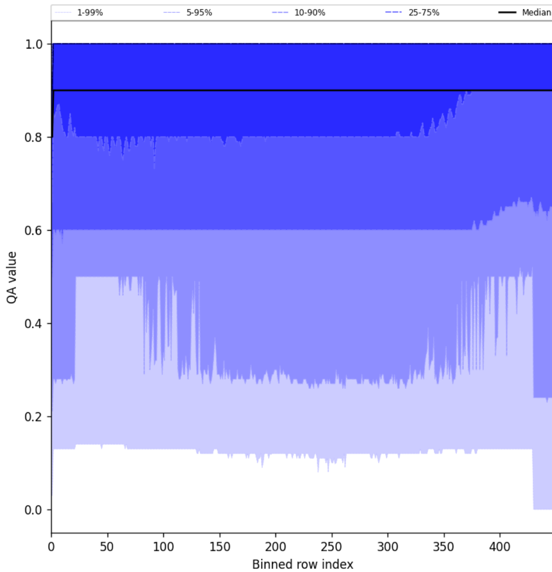
Figure 27: Along track statistics of “QA value” for 2024-12-08 to 2024-12-10
