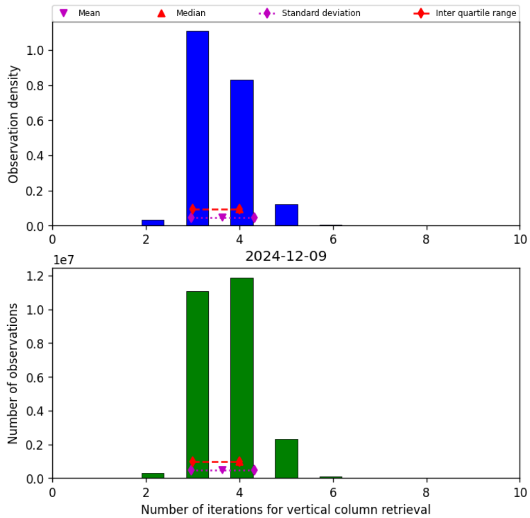
Figure 26: Histogram of “Number of iterations for vertical column retrieval” for 2024-12-08 to 2024-12-10
