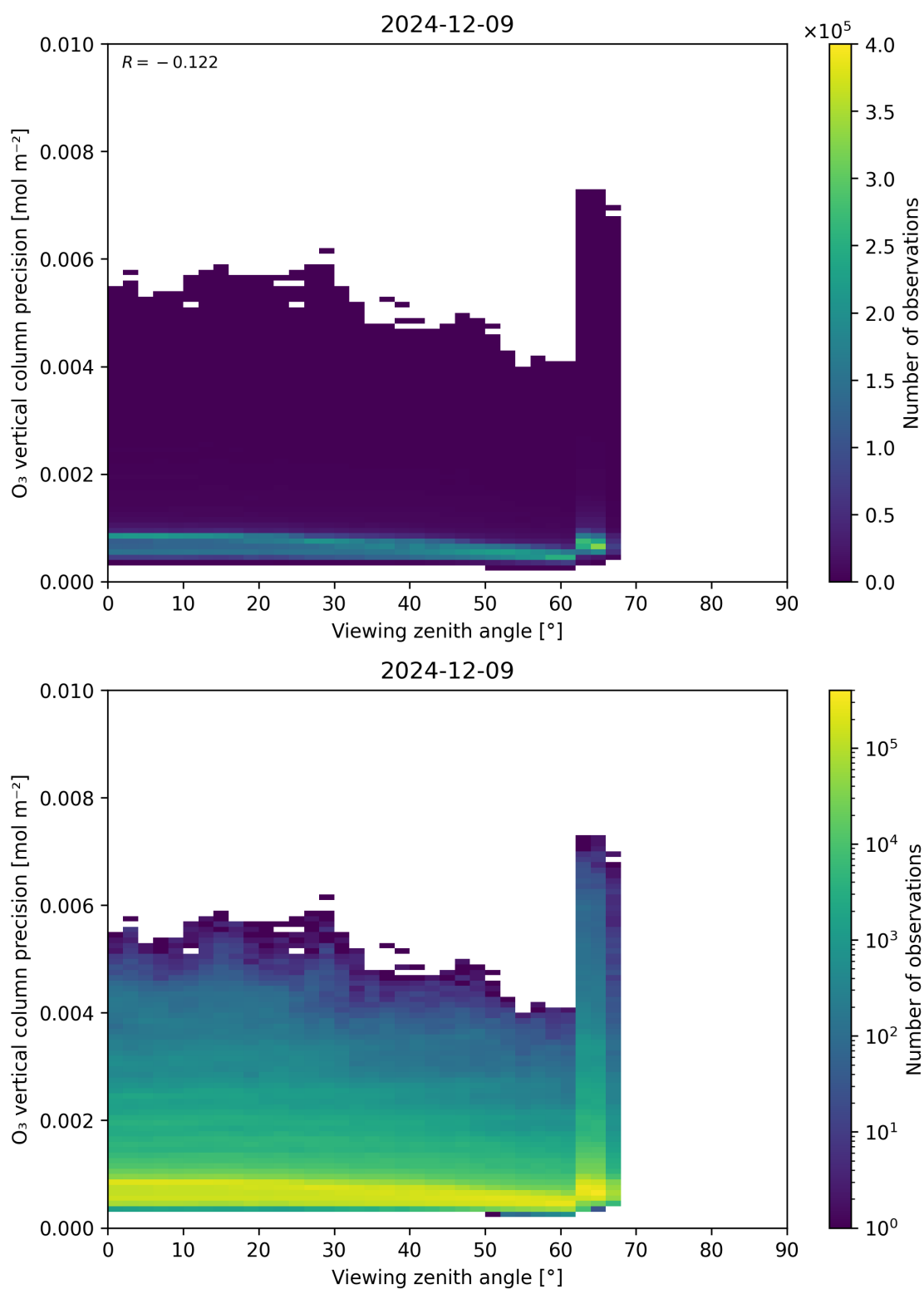
Figure 53: Scatter density plot of “Viewing zenith angle” against “O 3 vertical column precision” for 2024-12-08 to 2024-12-10.
