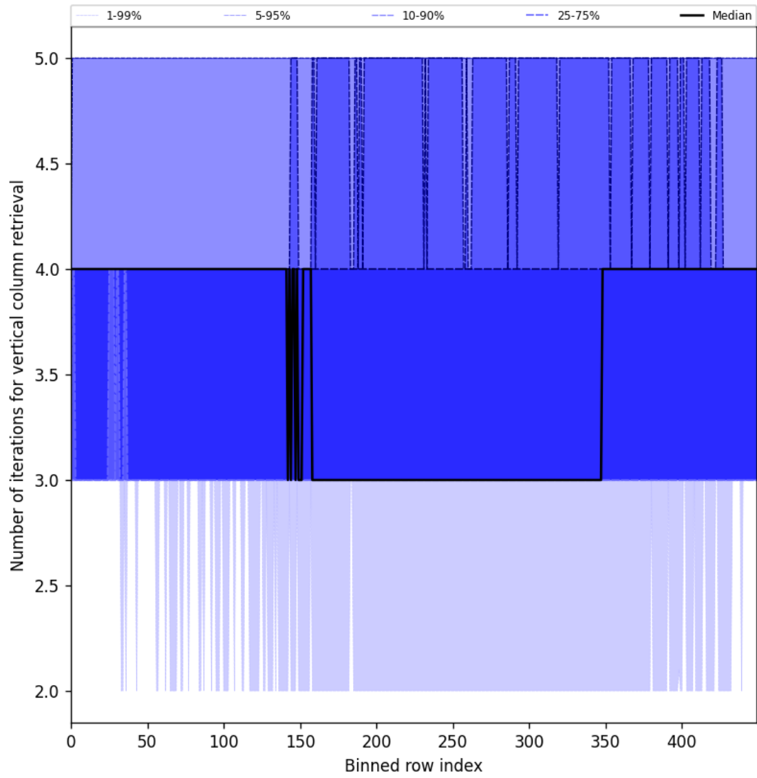
Figure 33: Along track statistics of “Number of iterations for vertical column retrieval” for 2024-12-08 to 2024-12-10
