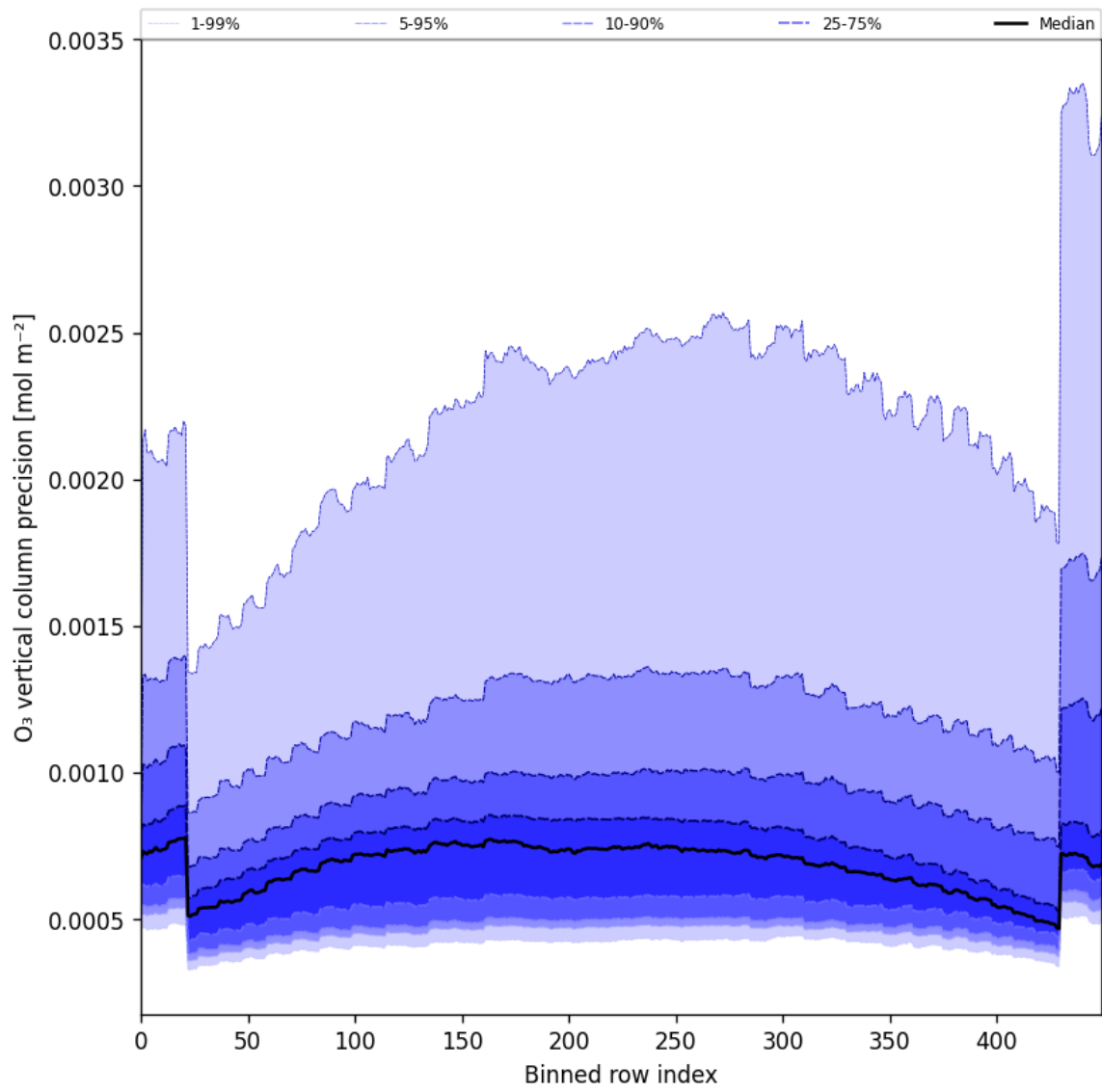
Figure 29: Along track statistics of “O 3 vertical column precision” for 2024-12-09 to 2024-12-11
