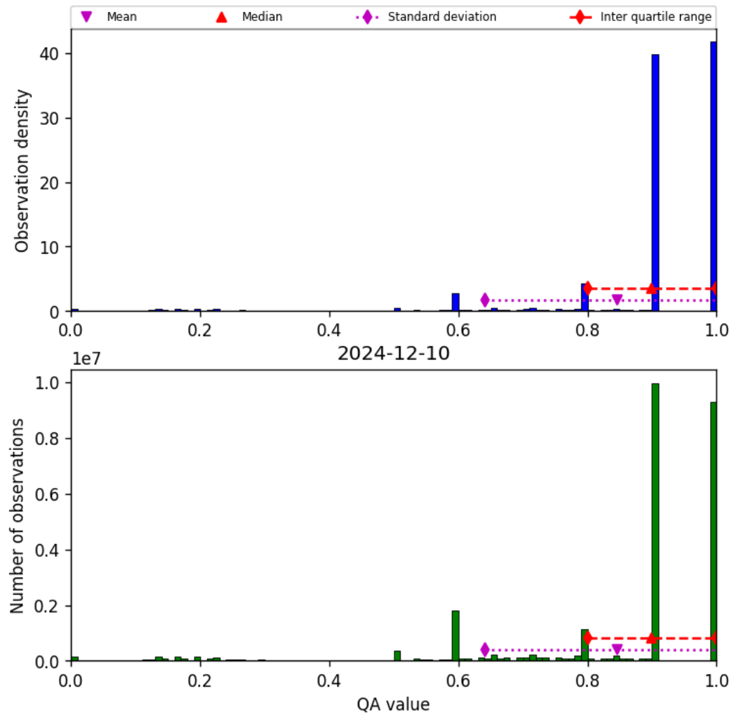
Figure 20: Histogram of “QA value” for 2024-12-09 to 2024-12-11
