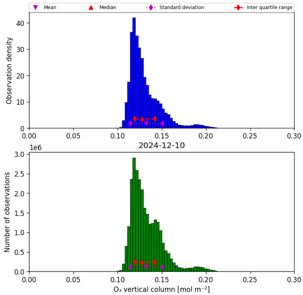
Figure 21: Histogram of “O 3 vertical column” for 2024-12-09 to 2024-12-11
