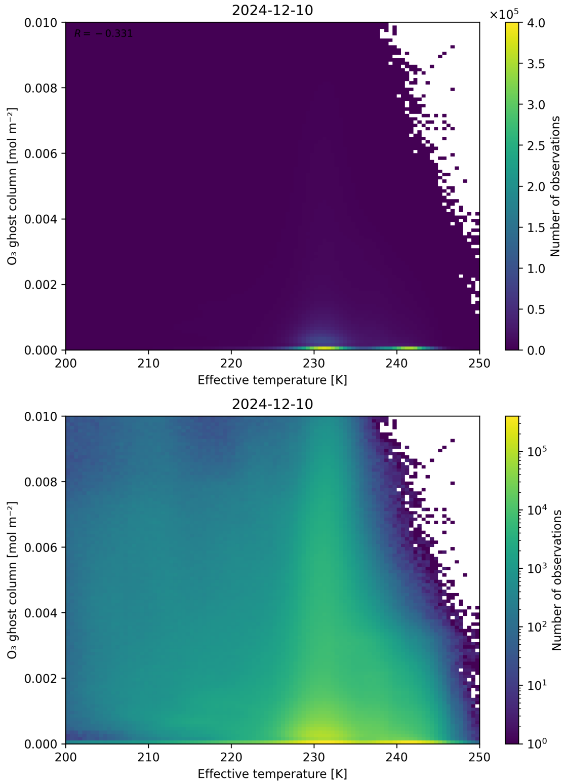
Figure 38: Scatter density plot of “Effective temperature” against “O 3 ghost column” for 2024-12-09 to 2024-12-11.
