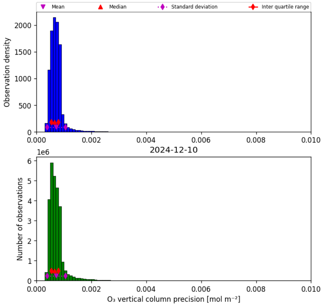
Figure 22: Histogram of “O 3 vertical column precision” for 2024-12-09 to 2024-12-11
