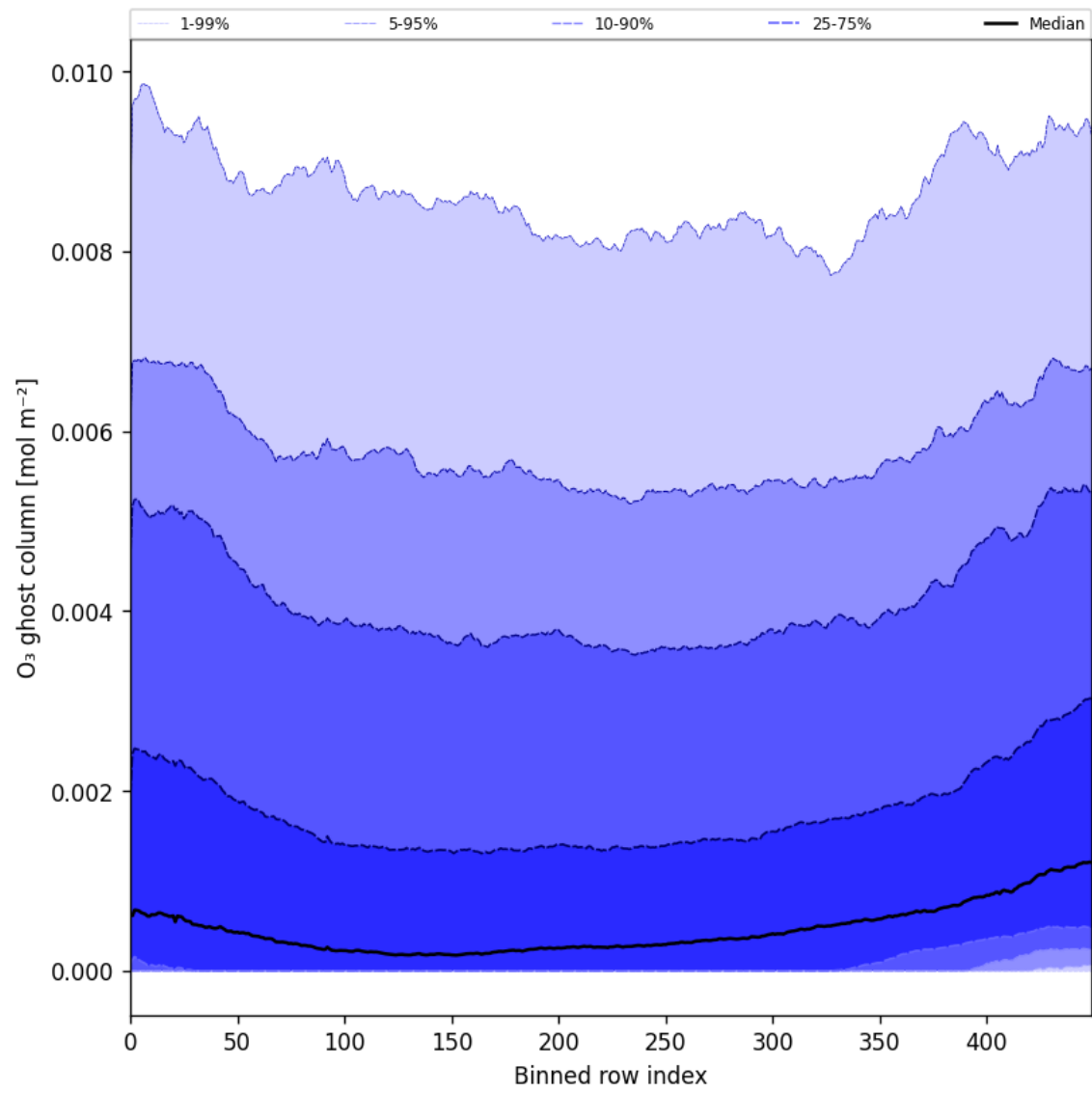
Figure 32: Along track statistics of "O 3 ghost column" for 2024-12-09 to 2024-12-11
