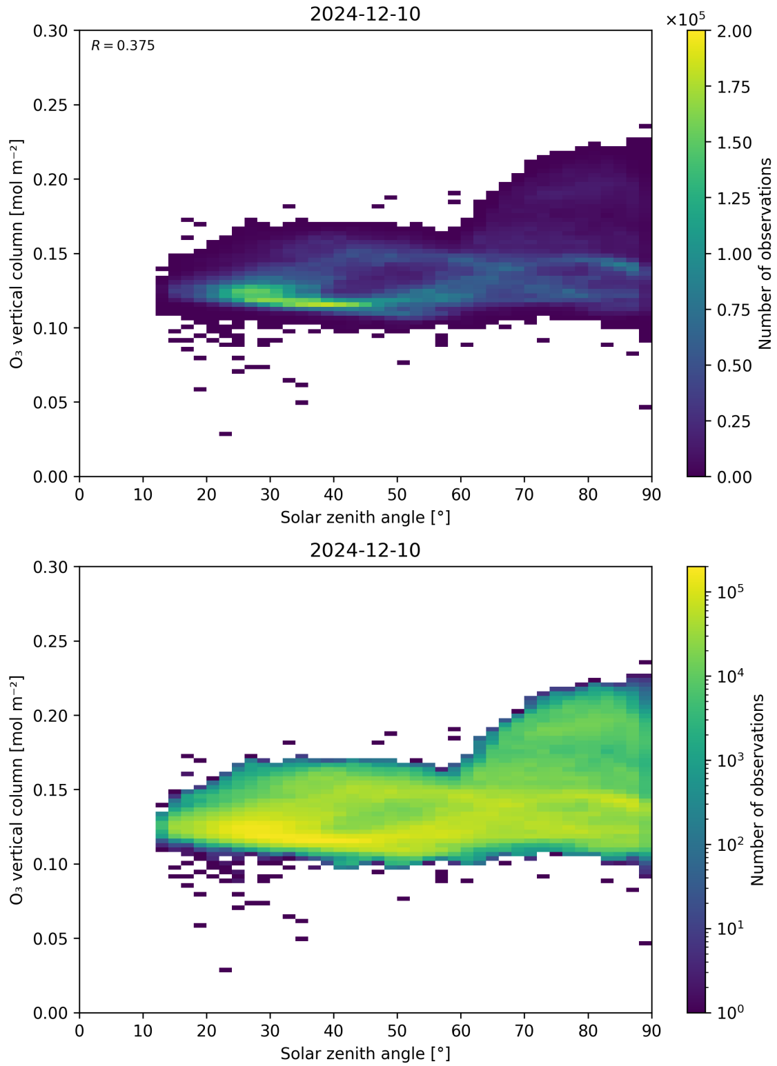
Figure 47: Scatter density plot of “Solar zenith angle” against “O 3 vertical column” for 2024-12-09 to 2024-12-11.
