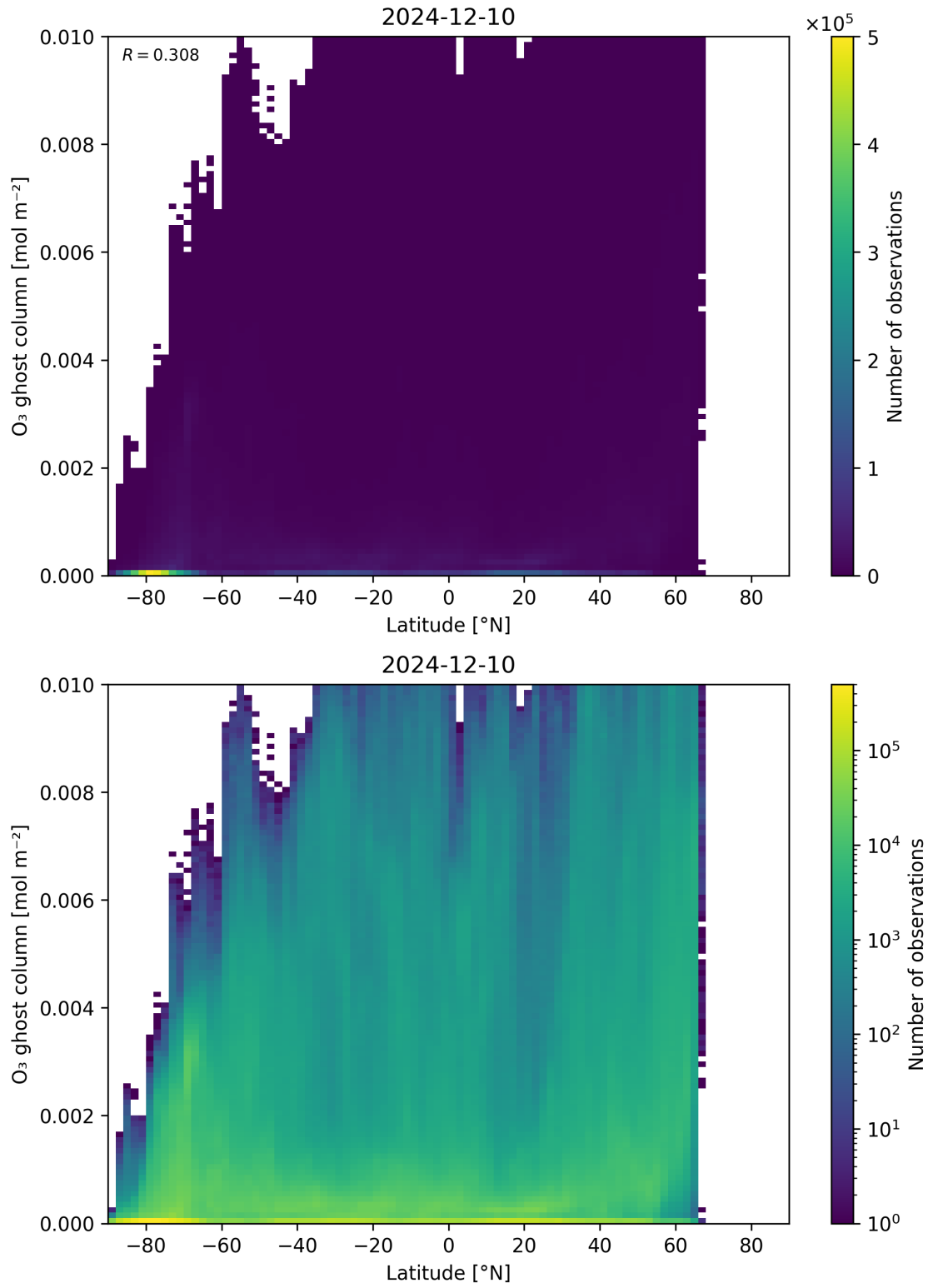
Figure 35: Scatter density plot of “Latitude” against “O 3 ghost column” for 2024-12-09 to 2024-12-11.
