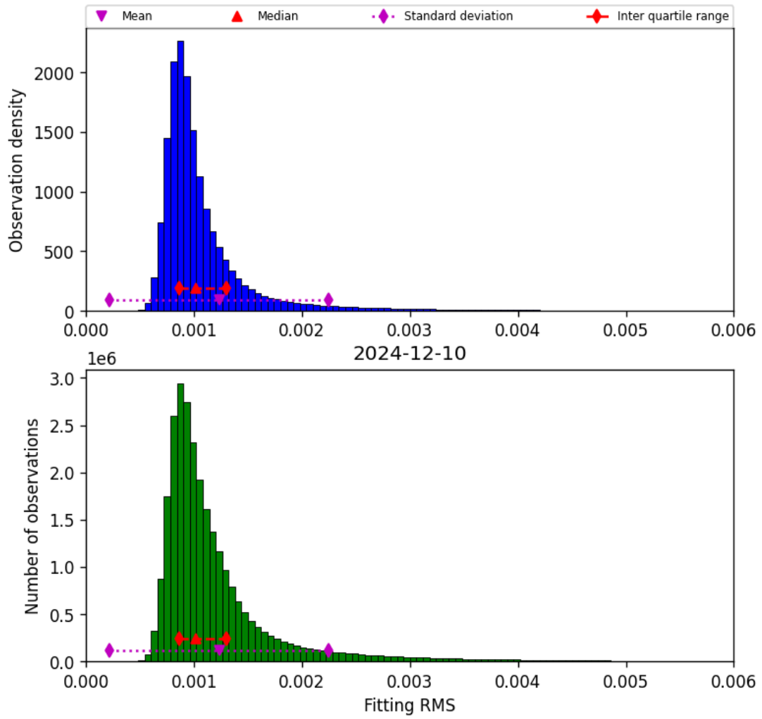
Figure 23: Histogram of “Fitting RMS” for 2024-12-09 to 2024-12-11
