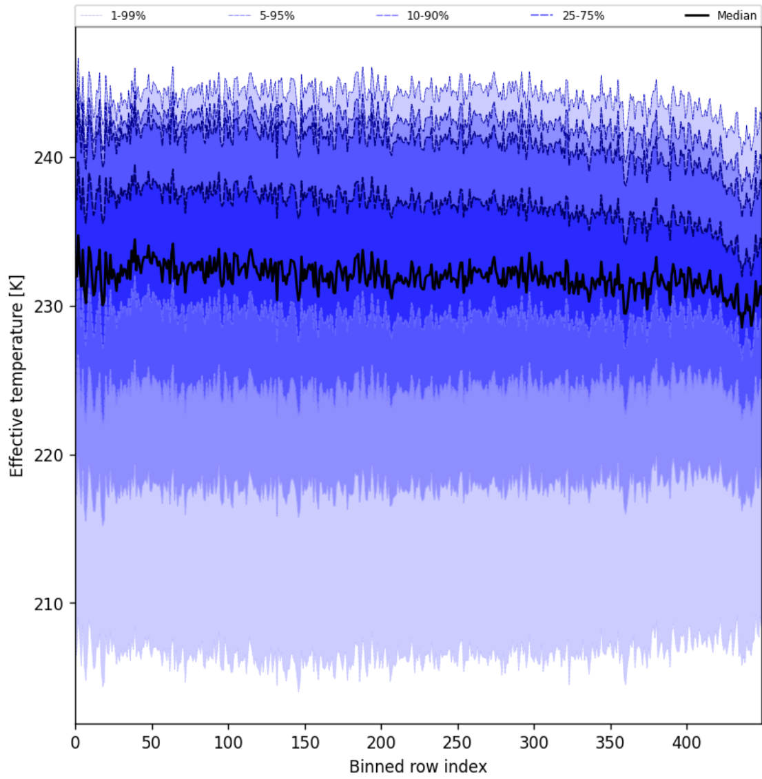
Figure 31: Along track statistics of "Effective temperature" for 2024-12-09 to 2024-12-11
