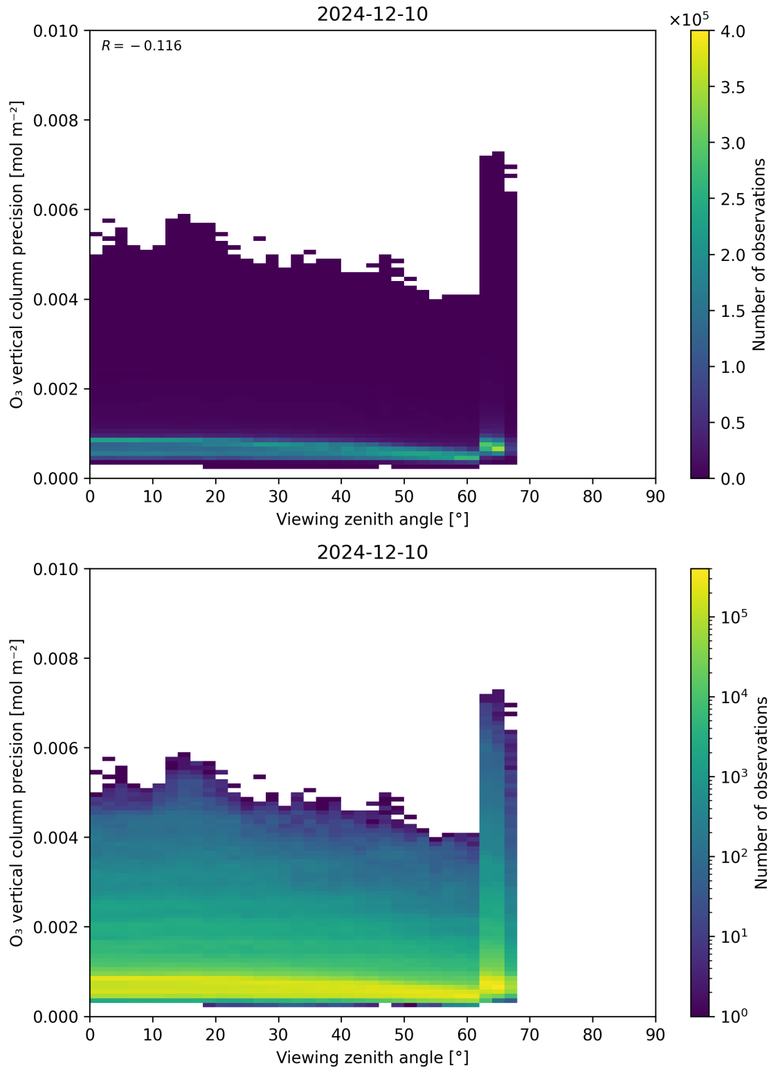
Figure 53: Scatter density plot of “Viewing zenith angle” against “O 3 vertical column precision” for 2024-12-09 to 2024-12-11.
