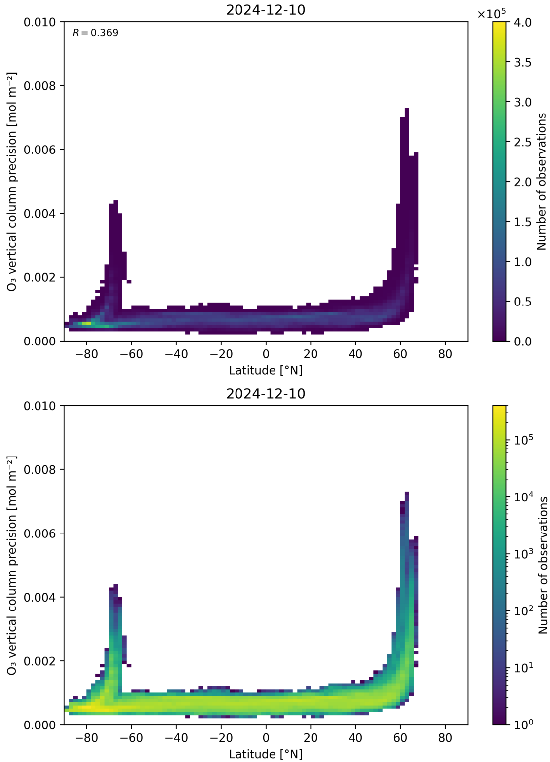
Figure 37: Scatter density plot of “Latitude” against “O 3 vertical column precision” for 2024-12-09 to 2024-12-11.
