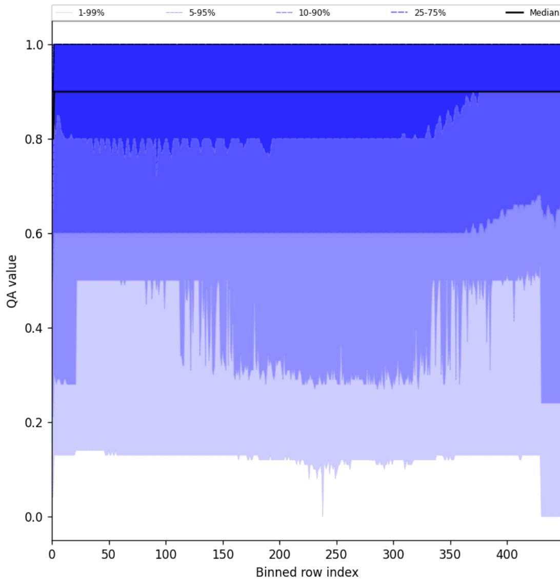
Figure 27: Along track statistics of “QA value” for 2024-12-09 to 2024-12-11
