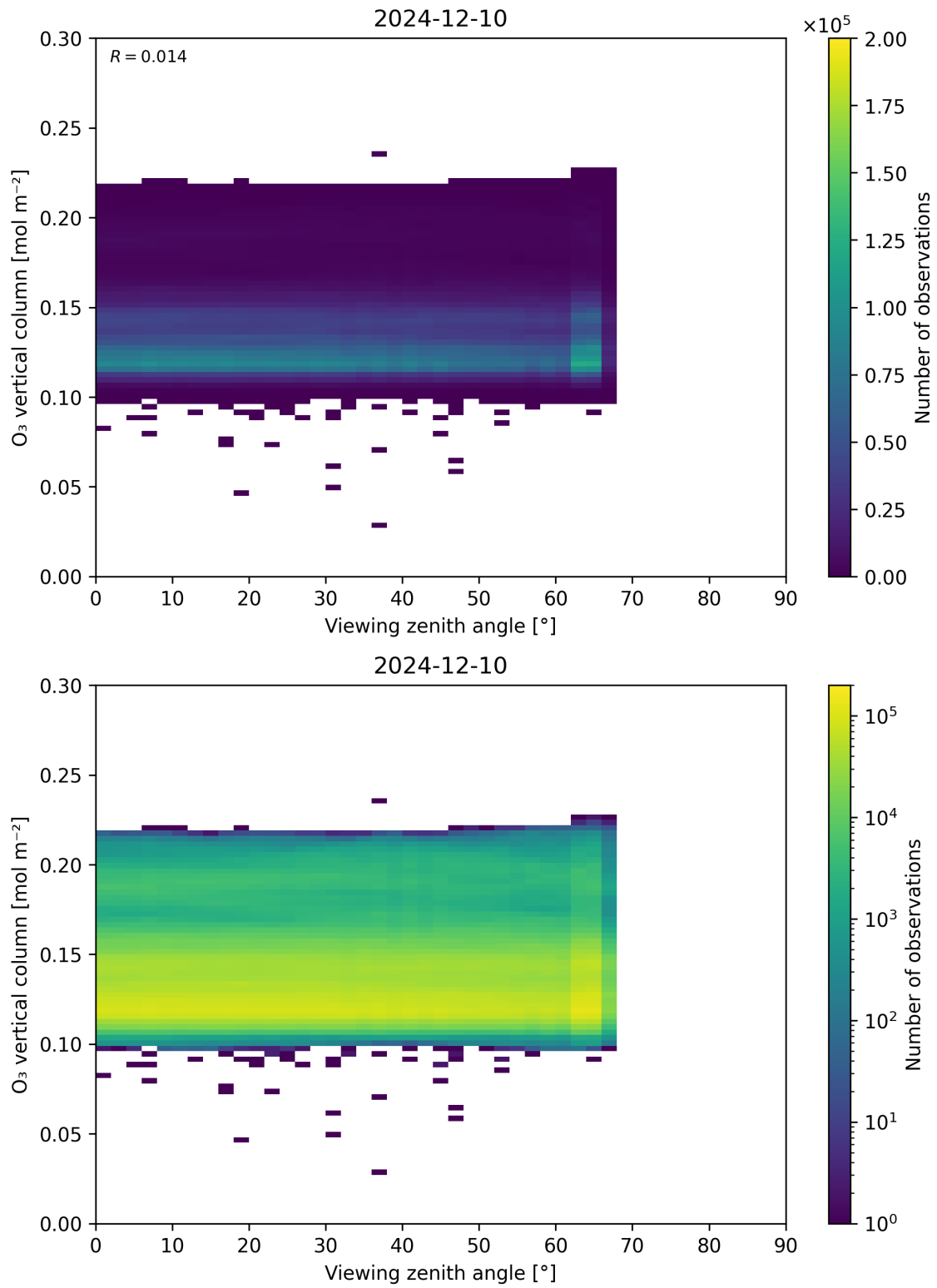
Figure 52: Scatter density plot of “Viewing zenith angle” against “O 3 vertical column” for 2024-12-09 to 2024-12-11.
