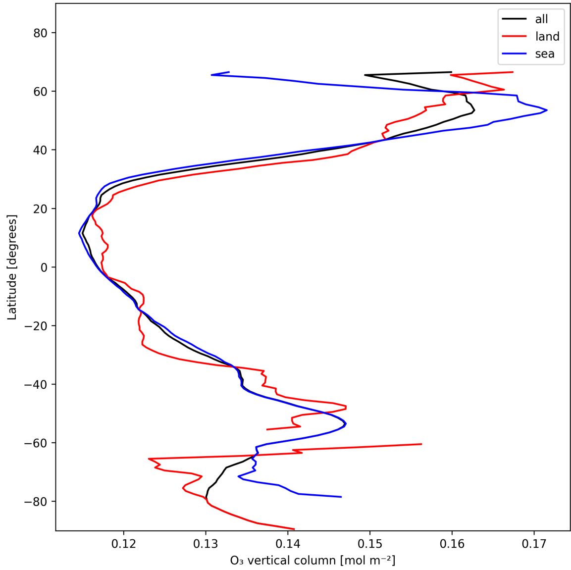
Figure 14: Zonal average of “O 3 vertical column” for 2024-12-09 to 2024-12-11.
