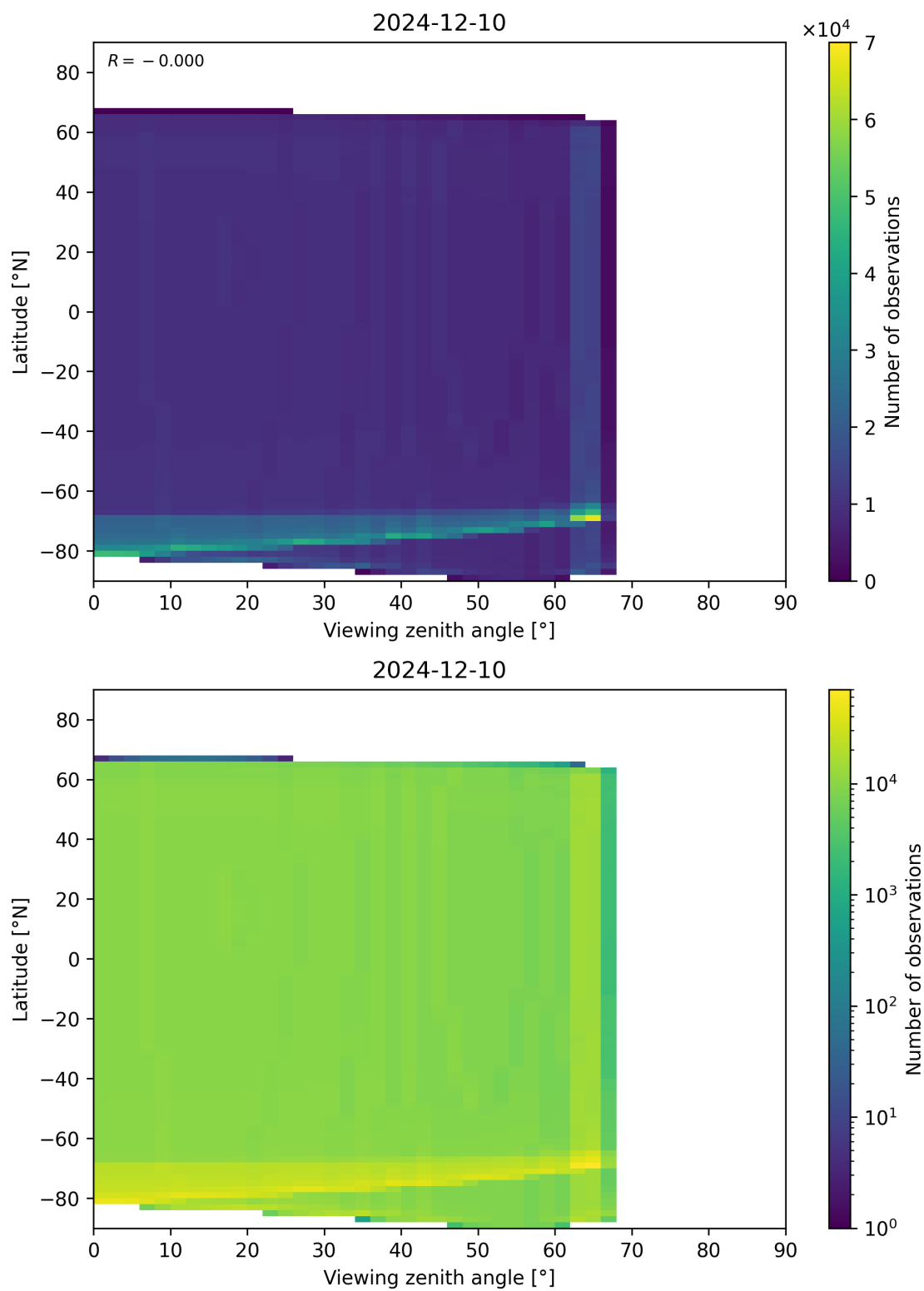
Figure 49: Scatter density plot of “Viewing zenith angle” against “Latitude” for 2024-12-09 to 2024-12-11.
