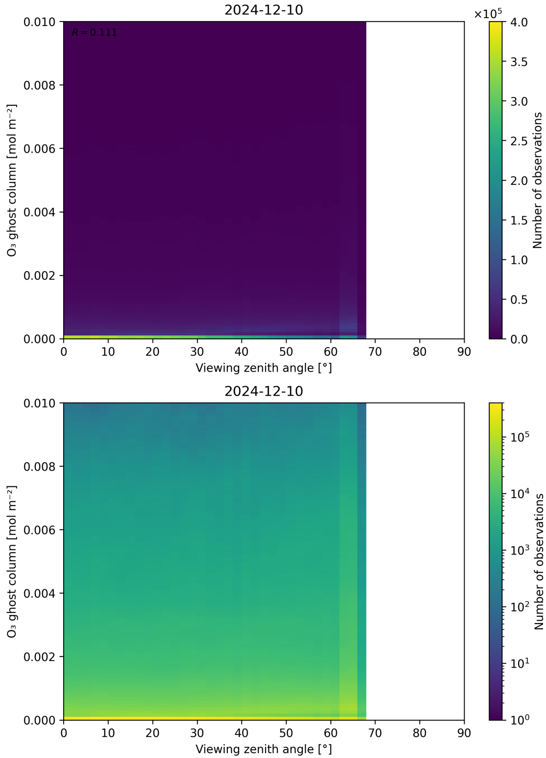
Figure 51: Scatter density plot of “Viewing zenith angle” against “O 3 ghost column” for 2024-12-09 to 2024-12-11.
