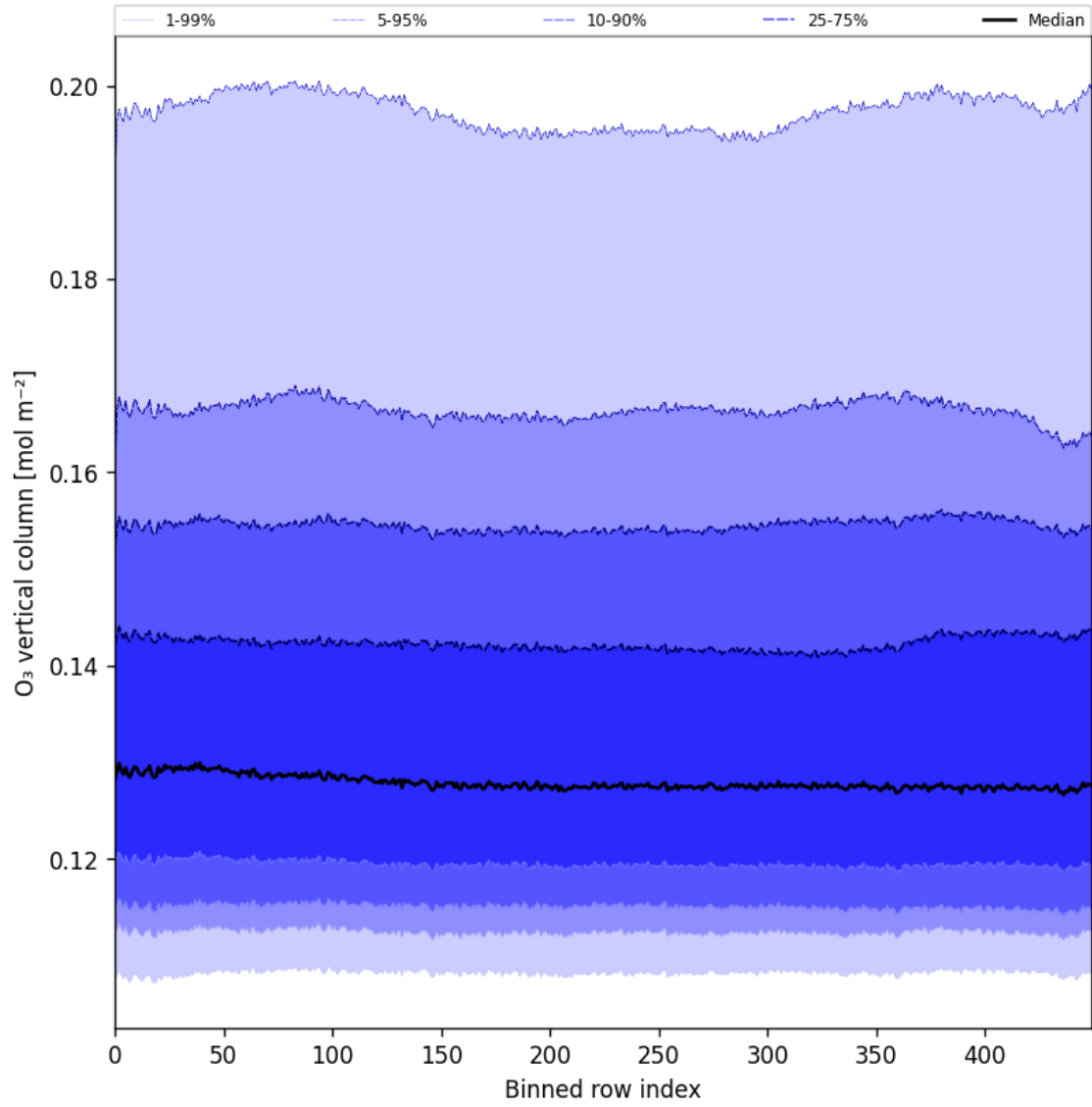
Figure 28: Along track statistics of “O 3 vertical column” for 2024-12-09 to 2024-12-11
