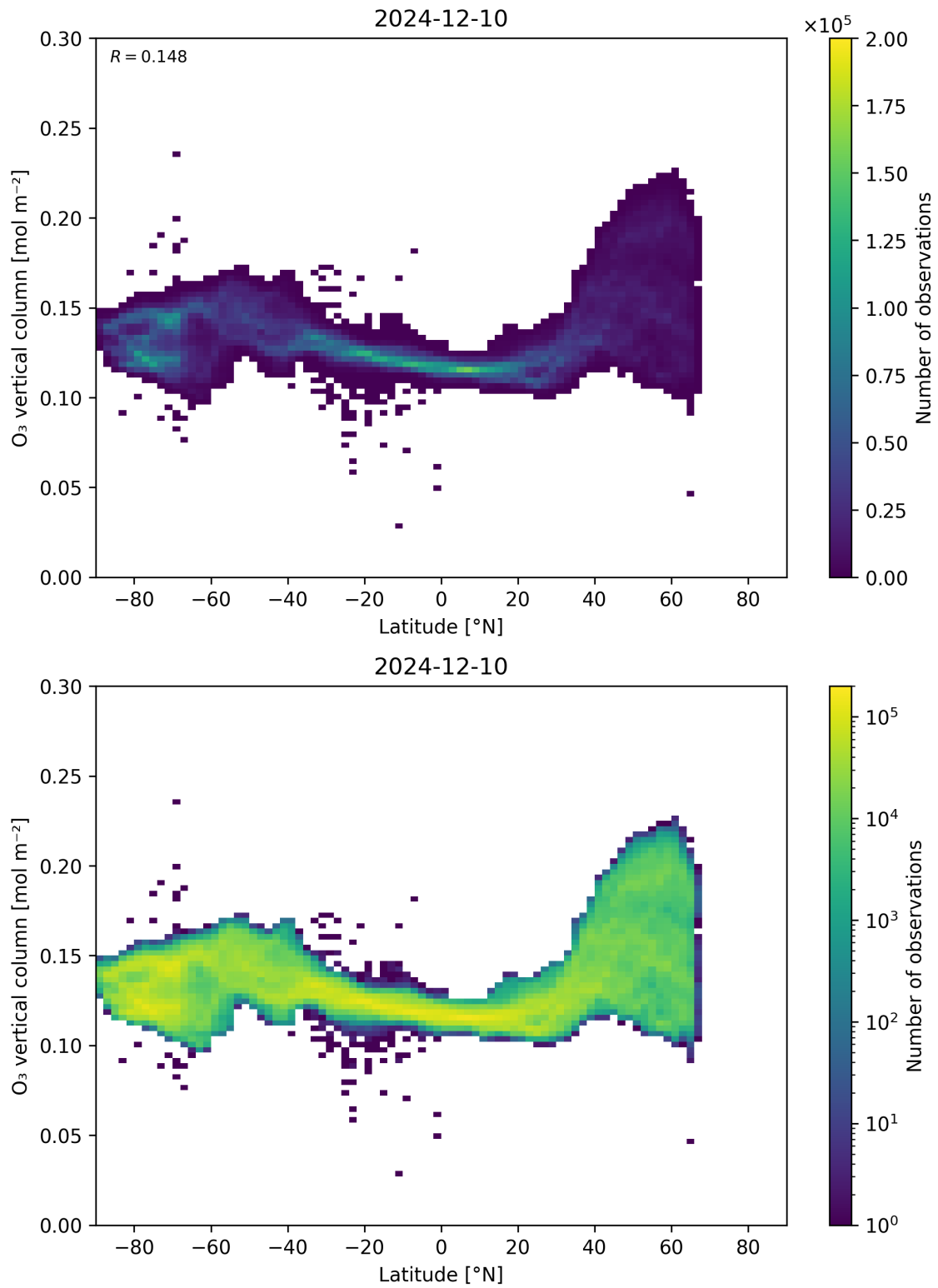
Figure 36: Scatter density plot of “Latitude” against “O 3 vertical column” for 2024-12-09 to 2024-12-11.
