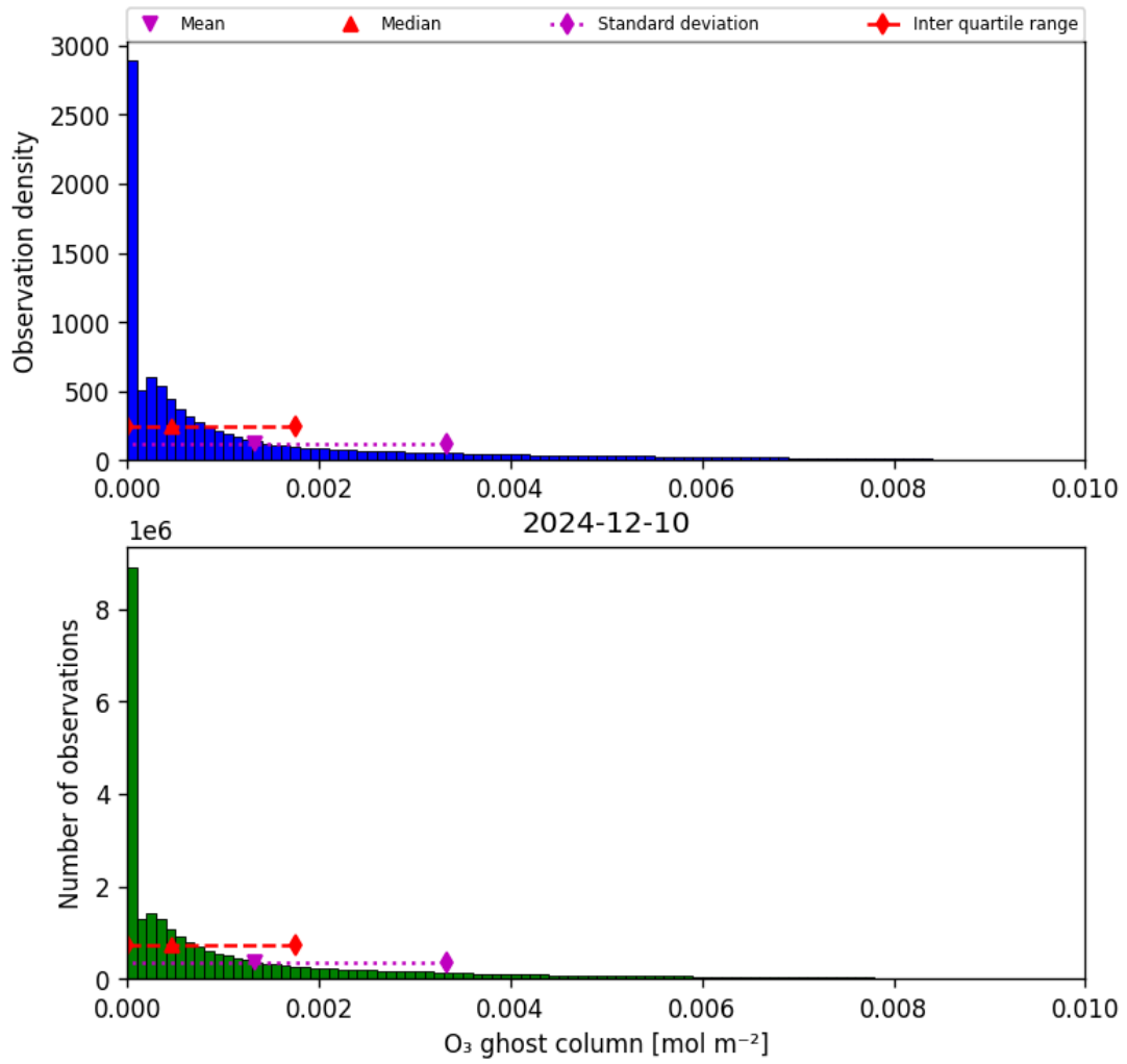
Figure 25: Histogram of “O 3 ghost column” for 2024-12-09 to 2024-12-11
