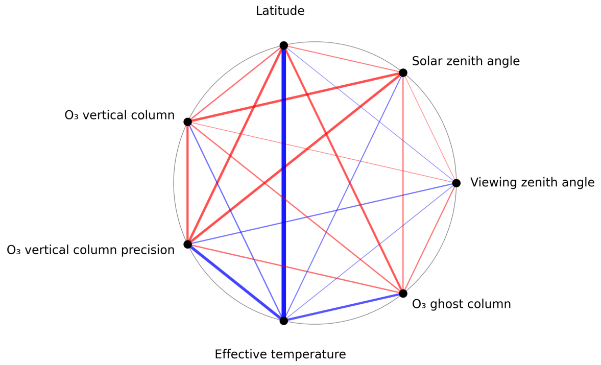
Figure 1: Map of correlation graph for 2024-12-09 to 2024-12-11.
