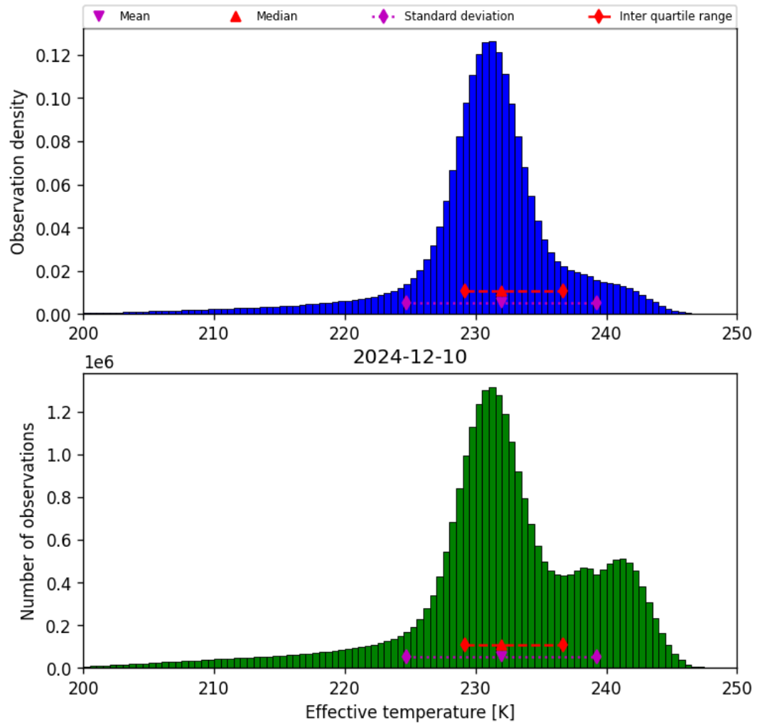
Figure 24: Histogram of “Effective temperature” for 2024-12-09 to 2024-12-11
