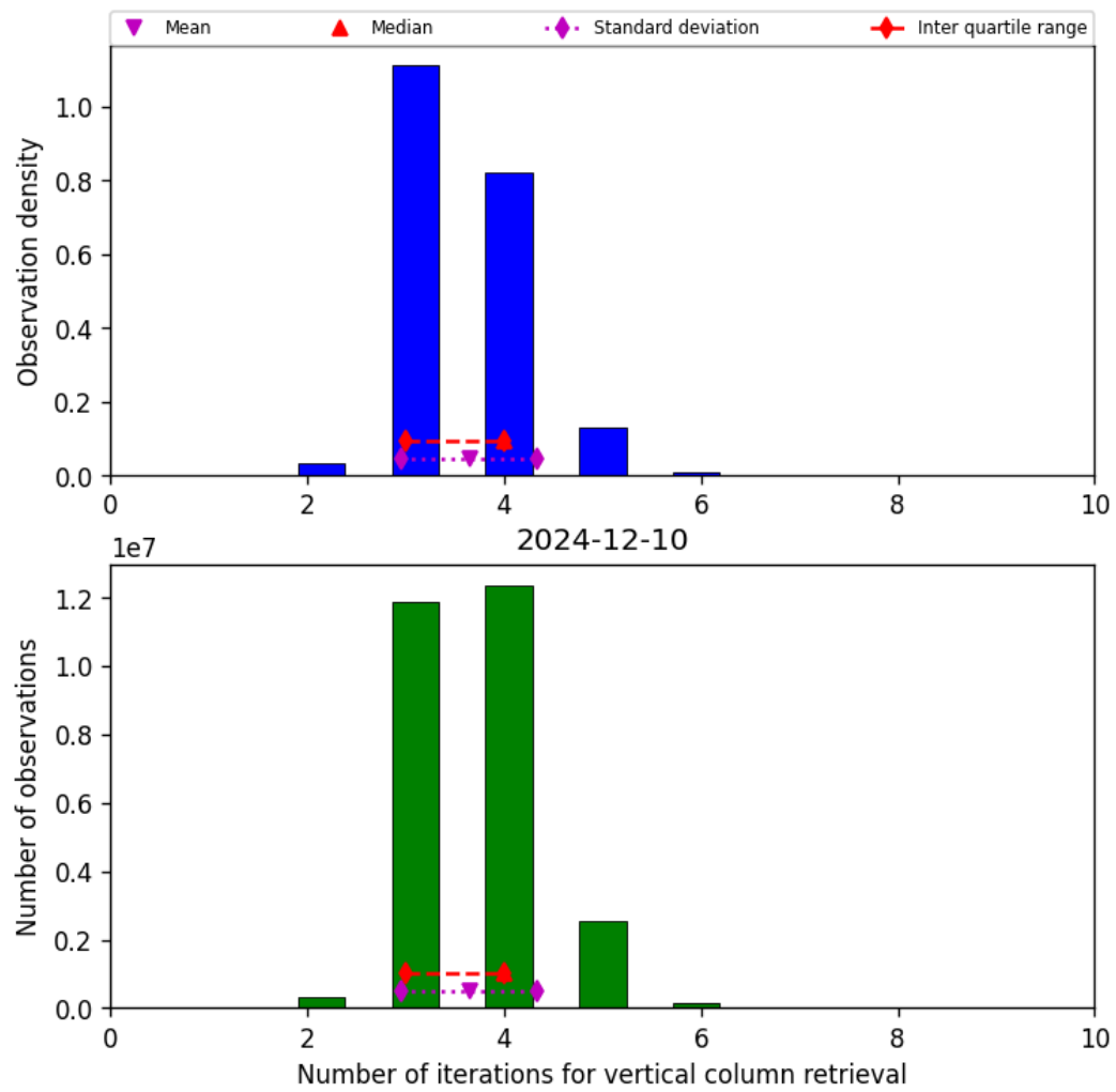
Figure 26: Histogram of “Number of iterations for vertical column retrieval” for 2024-12-09 to 2024-12-11
