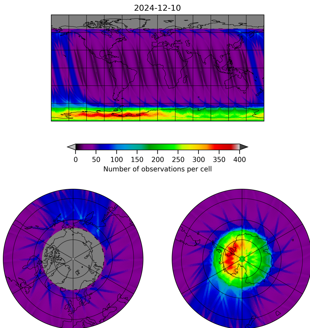
Figure 12: Map of the number of observations for 2024-12-09 to 2024-12-11
