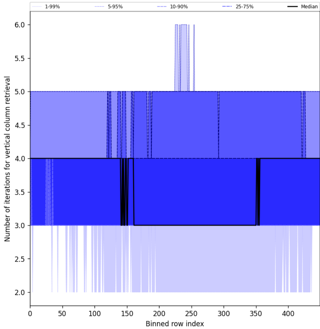
Figure 33: Along track statistics of “Number of iterations for vertical column retrieval” for 2024-12-09 to 2024-12-11
