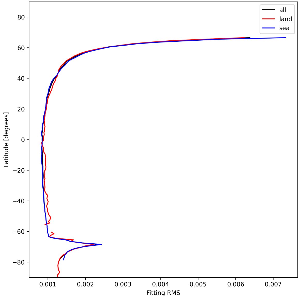
Figure 16: Zonal average of “Fitting RMS” for 2024-12-09 to 2024-12-11.
