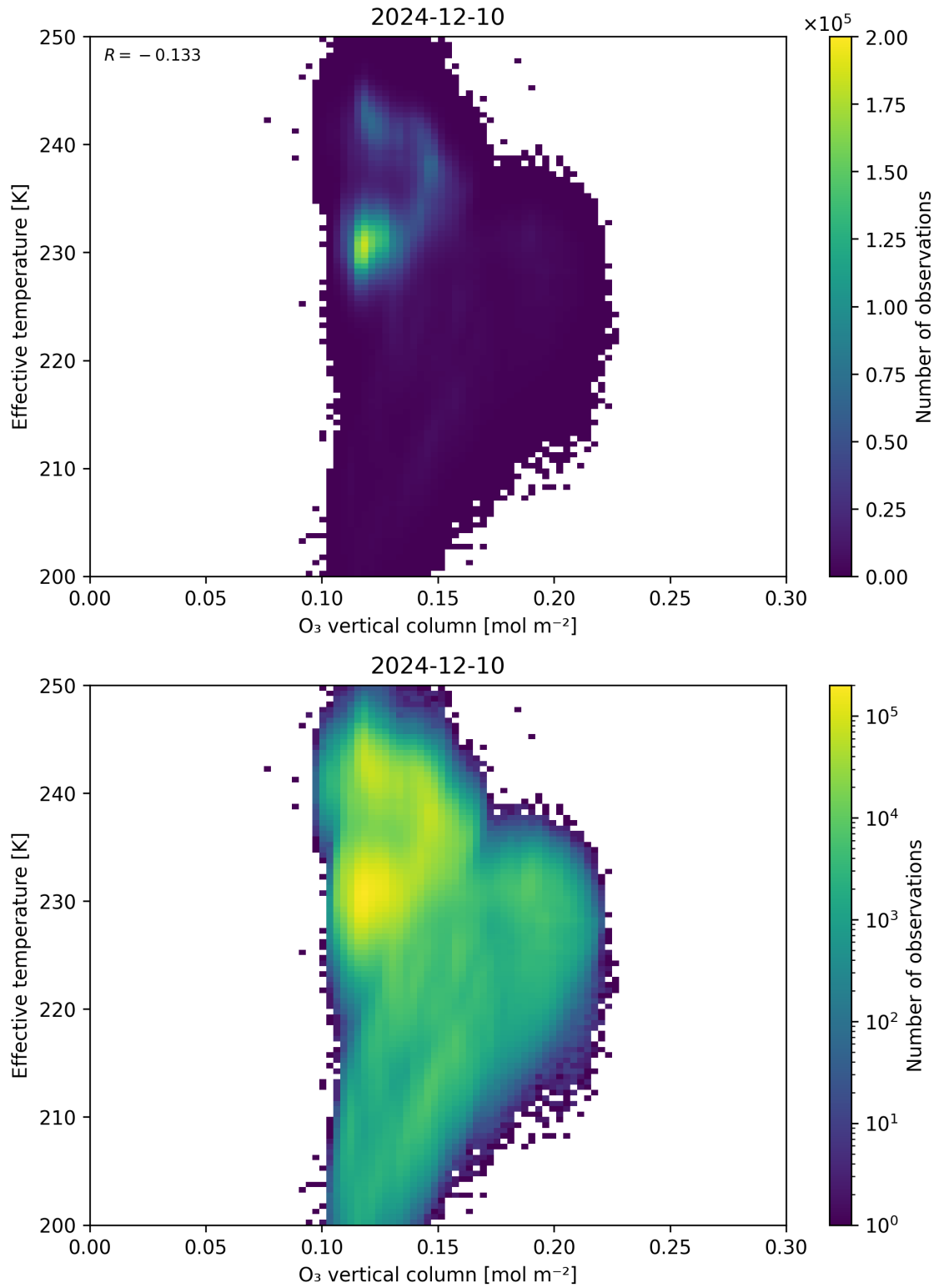
Figure 39: Scatter density plot of “O 3 vertical column” against “Effective temperature” for 2024-12-09 to 2024-12-11.
