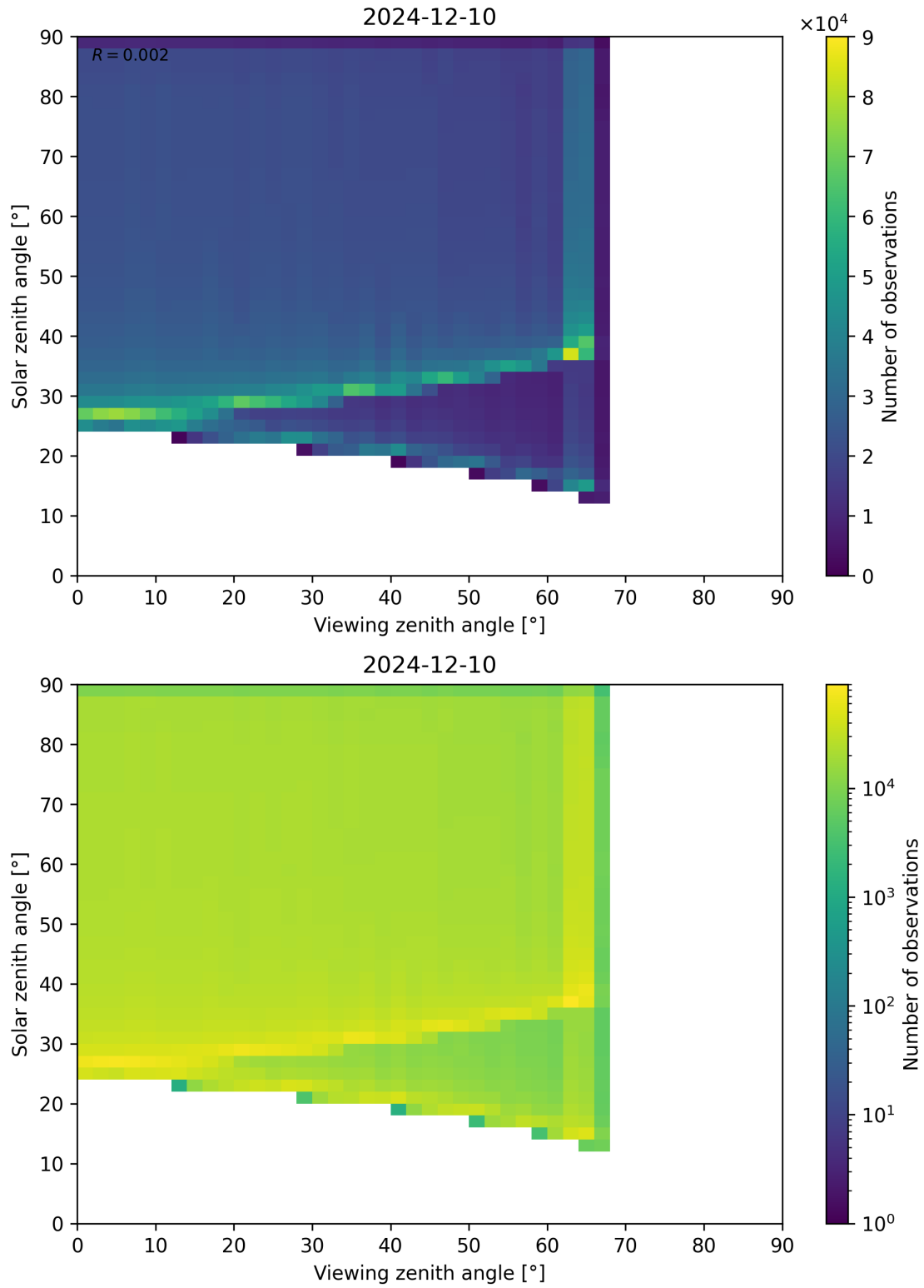
Figure 54: Scatter density plot of “Viewing zenith angle” against “Solar zenith angle” for 2024-12-09 to 2024-12-11.
