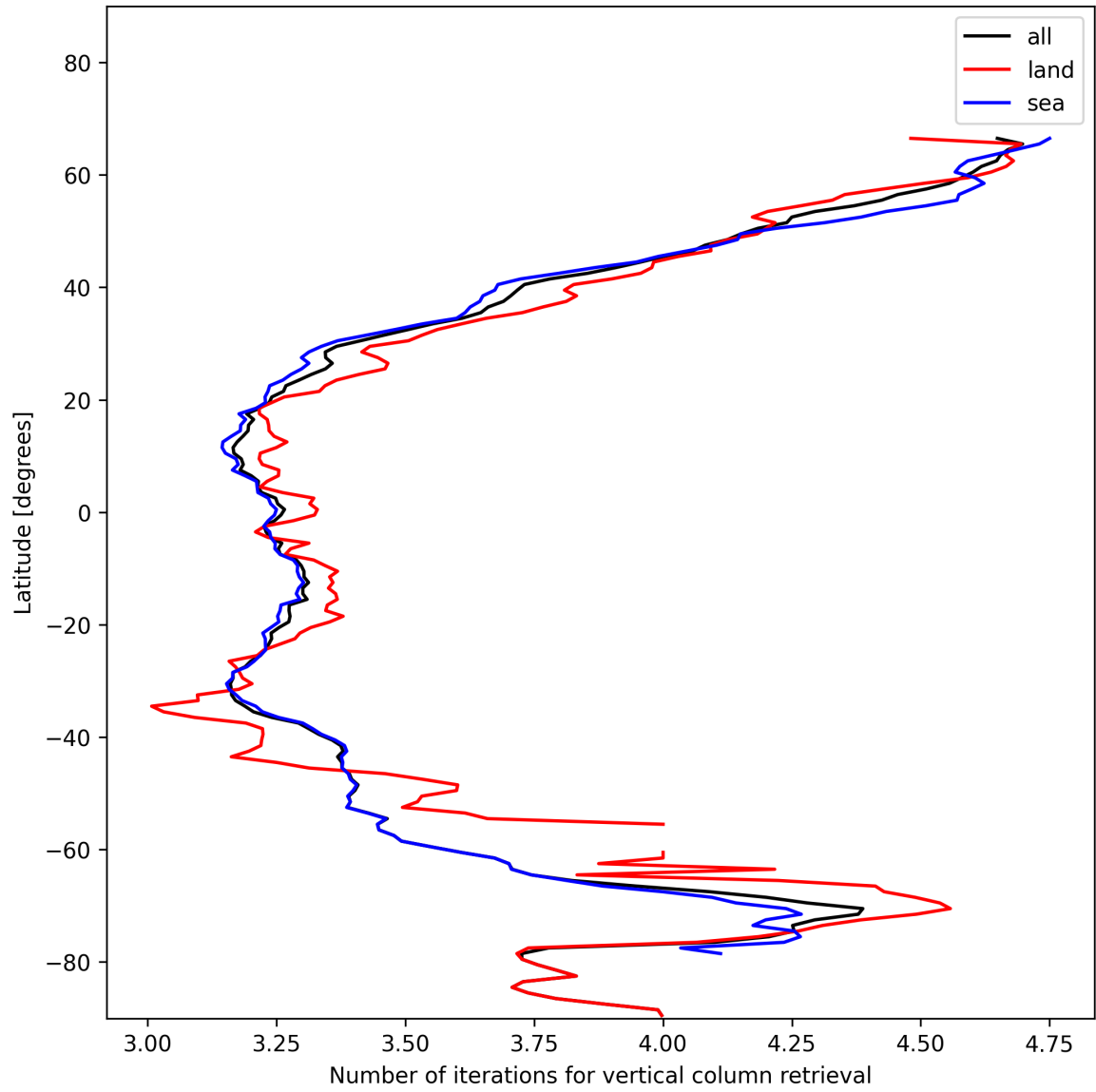
Figure 19: Zonal average of “Number of iterations for vertical column retrieval” for 2024-12-09 to 2024-12-11.
