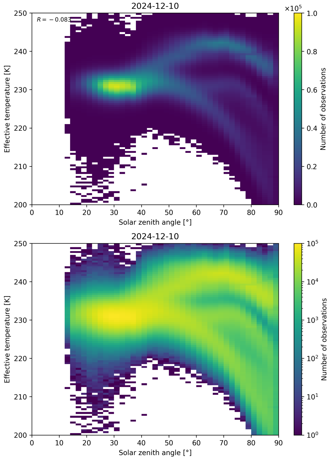
Figure 45: Scatter density plot of “Solar zenith angle” against “Effective temperature” for 2024-12-09 to 2024-12-11.
