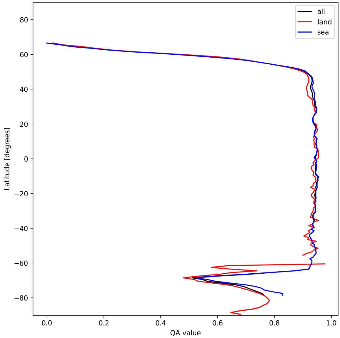
Figure 13: Zonal average of “QA value” for 2024-12-09 to 2024-12-11.
