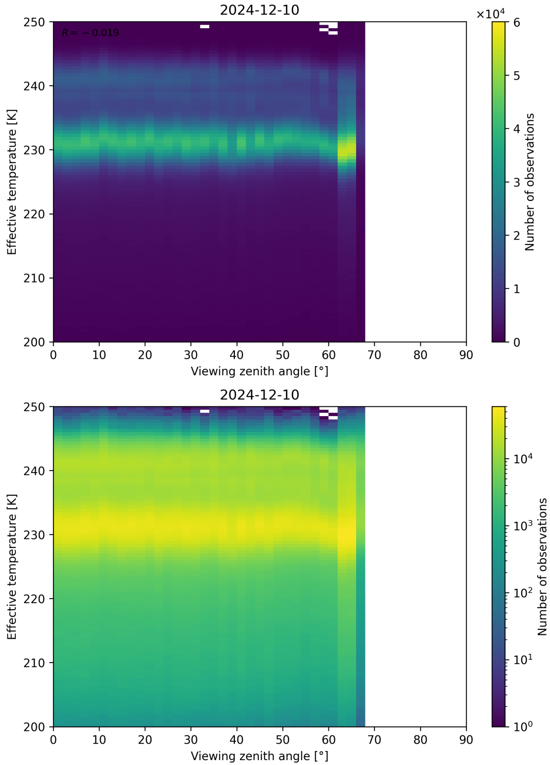
Figure 50: Scatter density plot of “Viewing zenith angle” against “Effective temperature” for 2024-12-09 to 2024-12-11.
