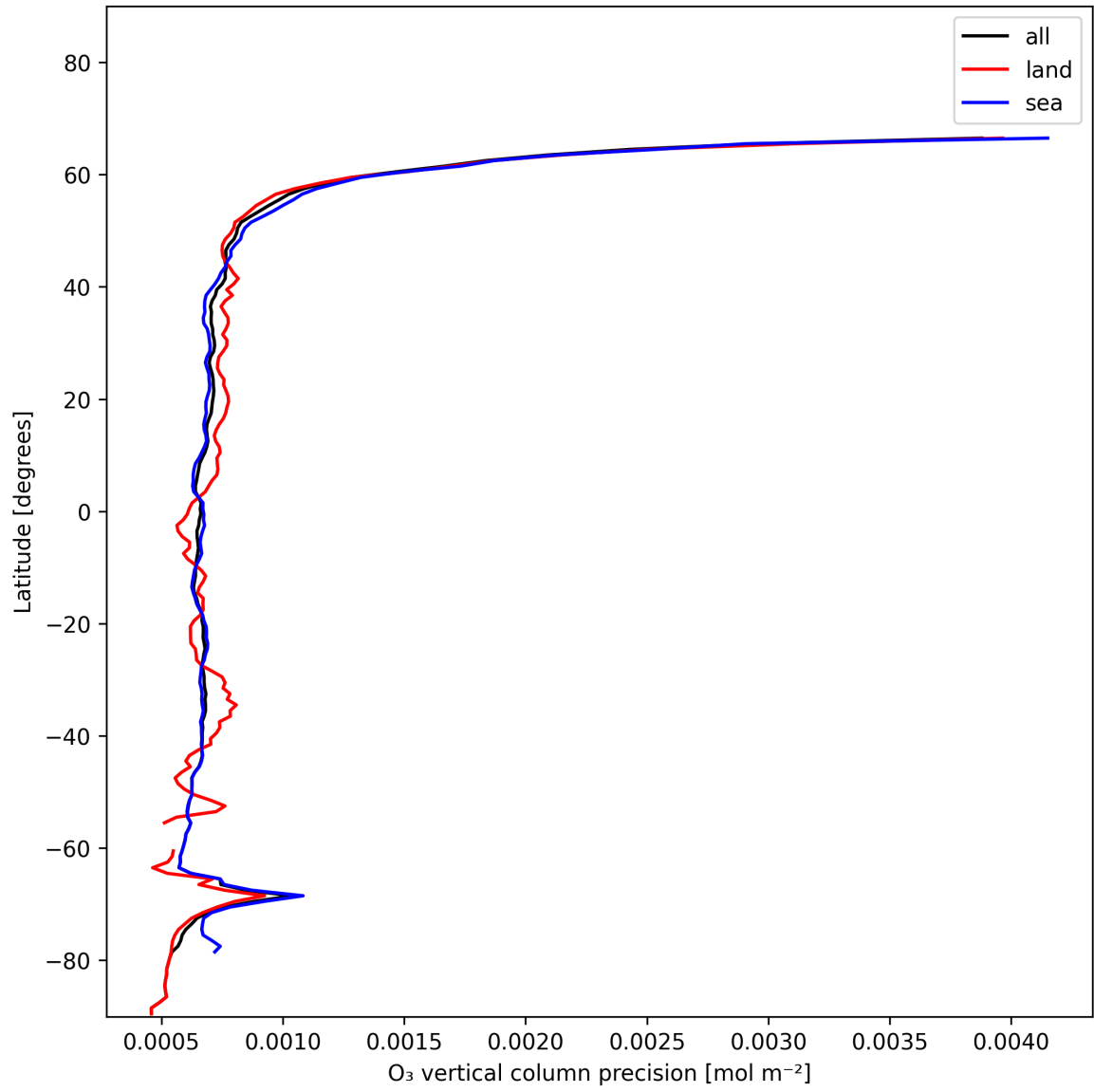
Figure 15: Zonal average of “O 3 vertical column precision” for 2024-12-09 to 2024-12-11.
