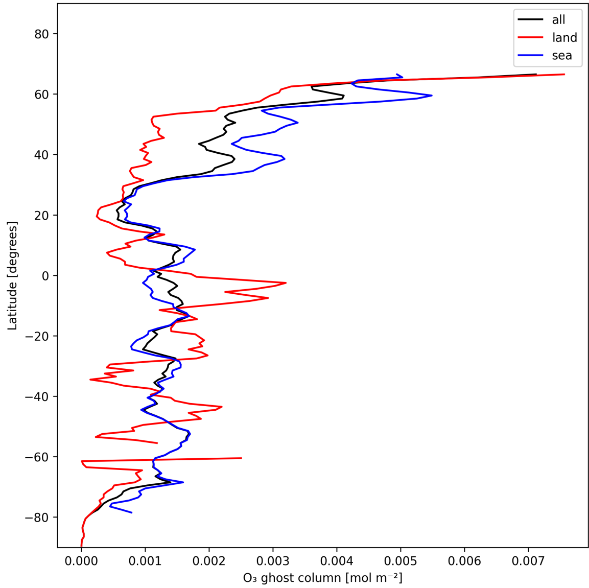
Figure 18: Zonal average of “O 3 ghost column” for 2024-12-09 to 2024-12-11.
