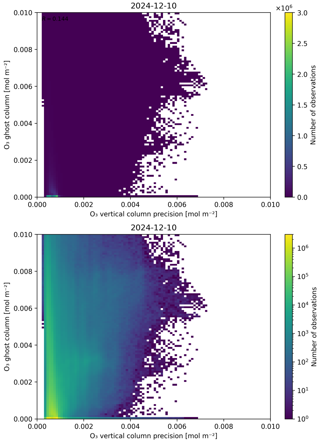
Figure 43: Scatter density plot of “ \text{O}_3 vertical column precision” against “ \text{O}_3 ghost column” for 2024-12-09 to 2024-12-11.
