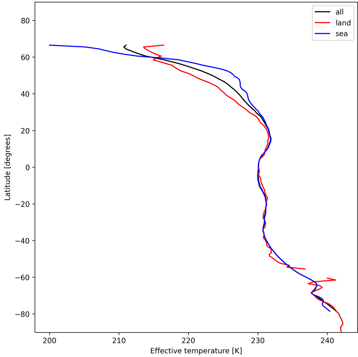
Figure 17: Zonal average of "Effective temperature" for 2024-12-09 to 2024-12-11.
