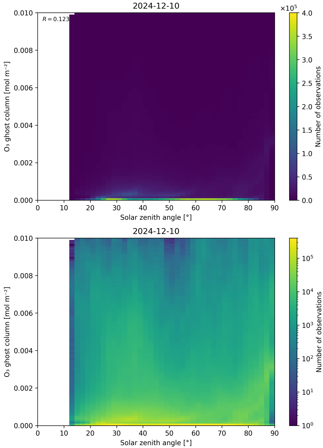
Figure 46: Scatter density plot of “Solar zenith angle” against “O 3 ghost column” for 2024-12-09 to 2024-12-11.
