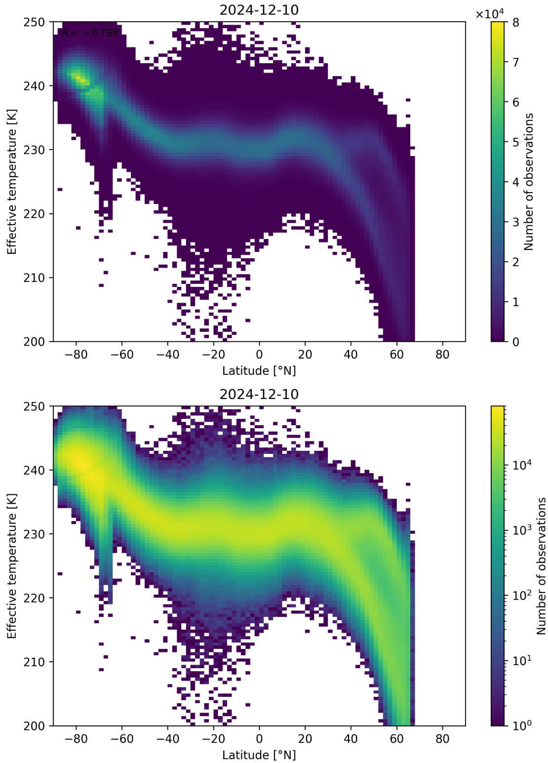
Figure 34: Scatter density plot of “Latitude” against “Effective temperature” for 2024-12-09 to 2024-12-11.
