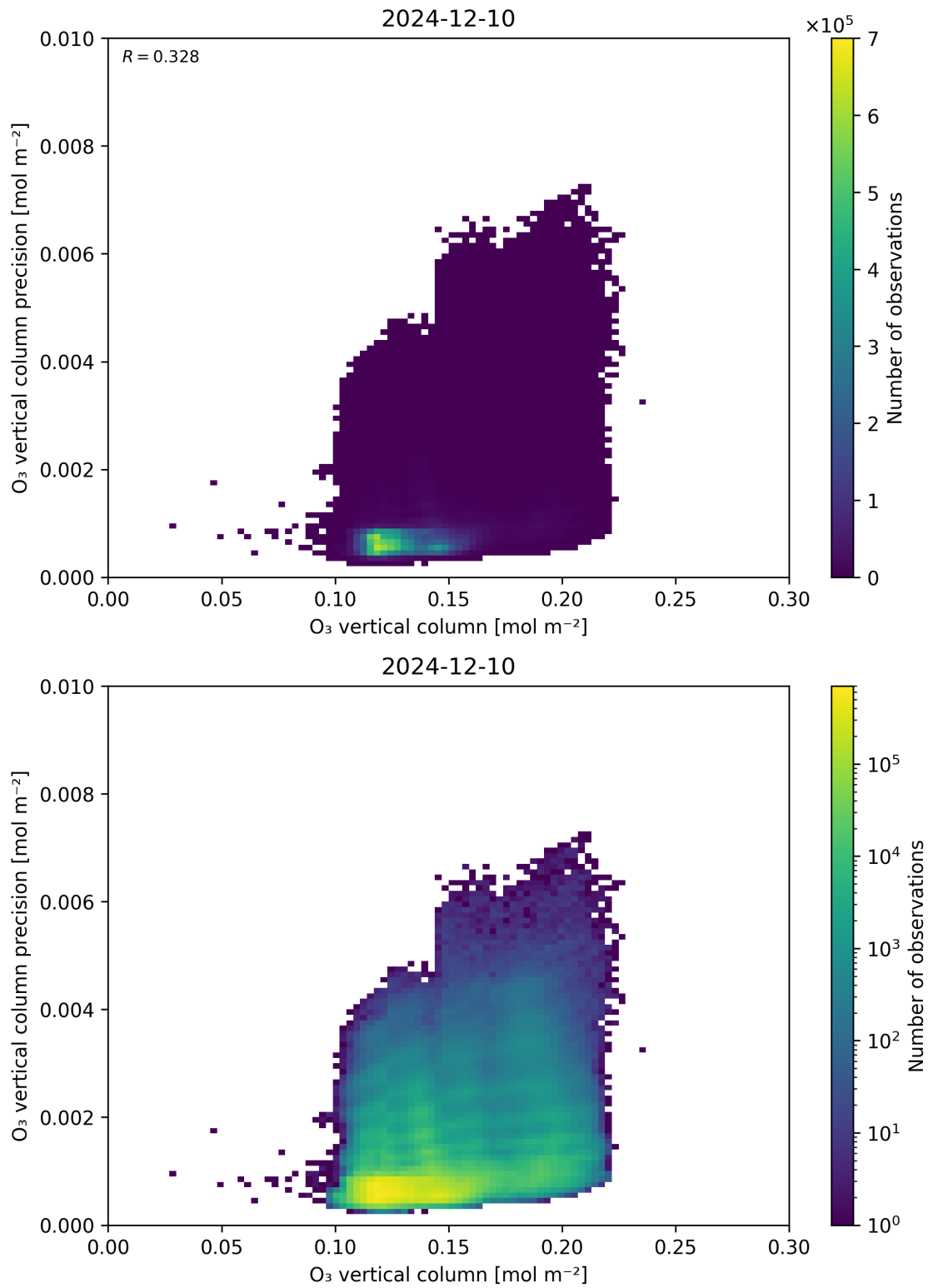
Figure 41: Scatter density plot of “O 3 vertical column” against “O 3 vertical column precision” for 2024-12-09 to 2024-12-11.
