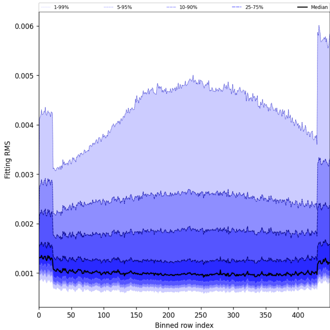
Figure 30: Along track statistics of “Fitting RMS” for 2024-12-09 to 2024-12-11
