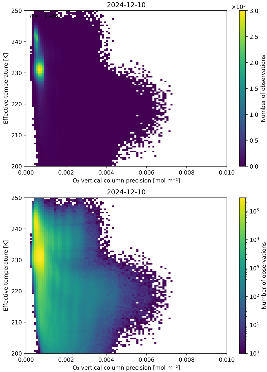
Figure 42: Scatter density plot of “O 3 vertical column precision” against “Effective temperature” for 2024-12-09 to 2024-12-11.
