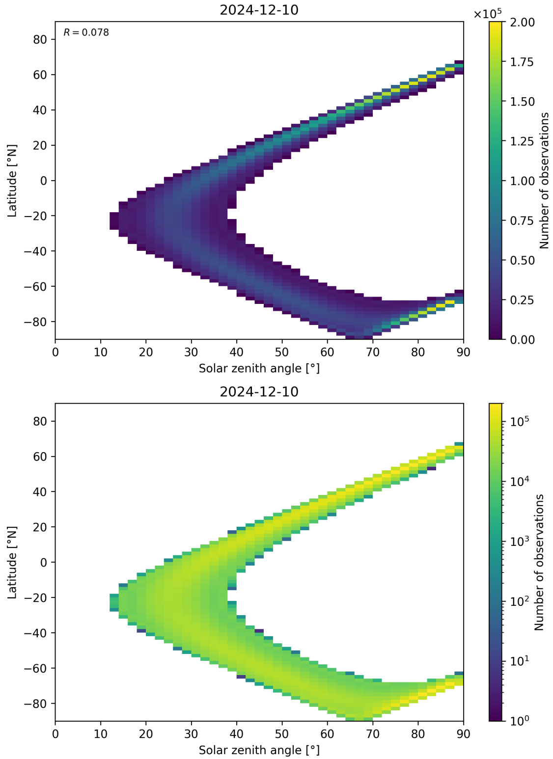
Figure 44: Scatter density plot of “Solar zenith angle” against “Latitude” for 2024-12-09 to 2024-12-11.
