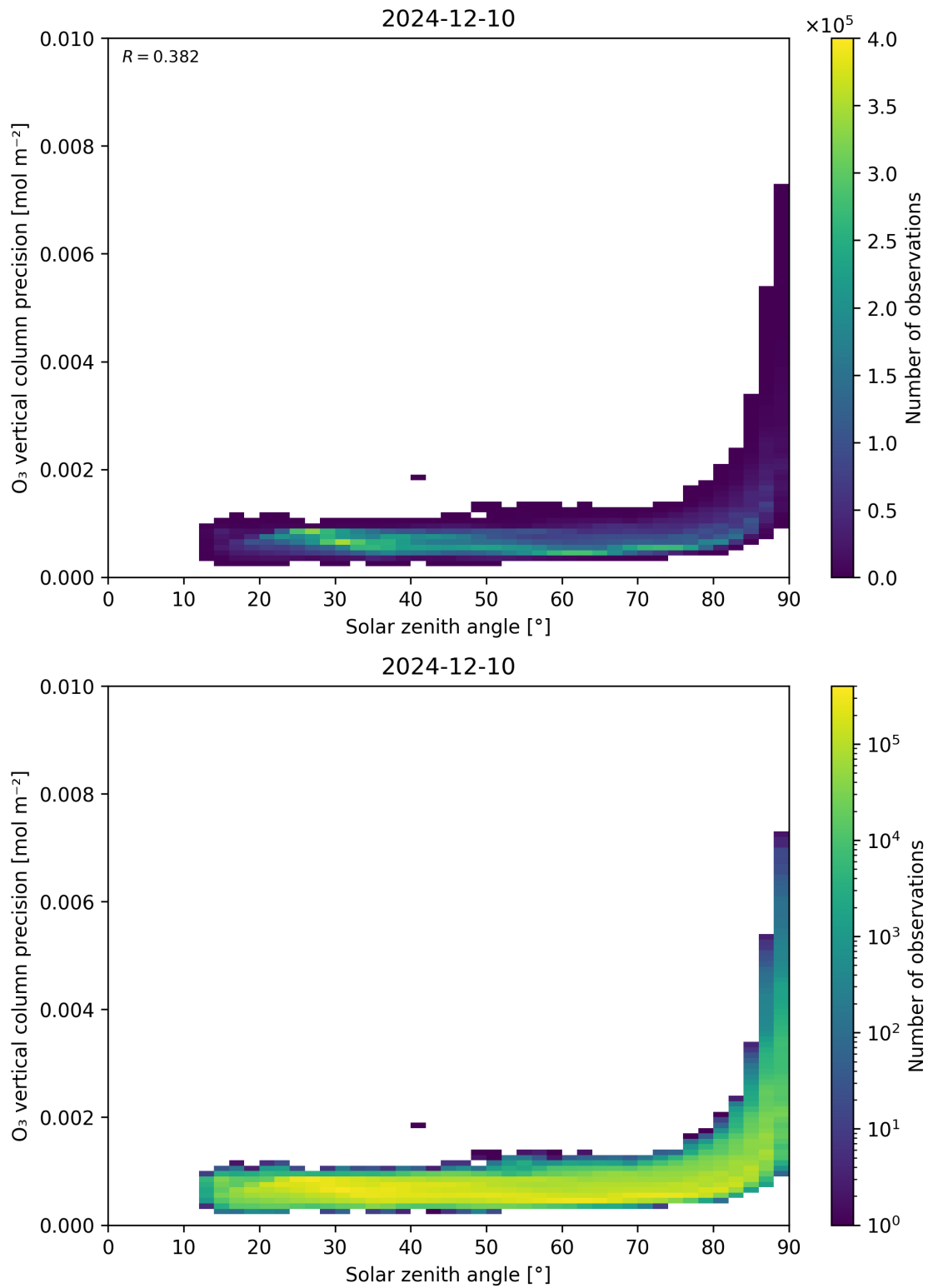
Figure 48: Scatter density plot of “Solar zenith angle” against “O 3 vertical column precision” for 2024-12-09 to 2024-12-11.
