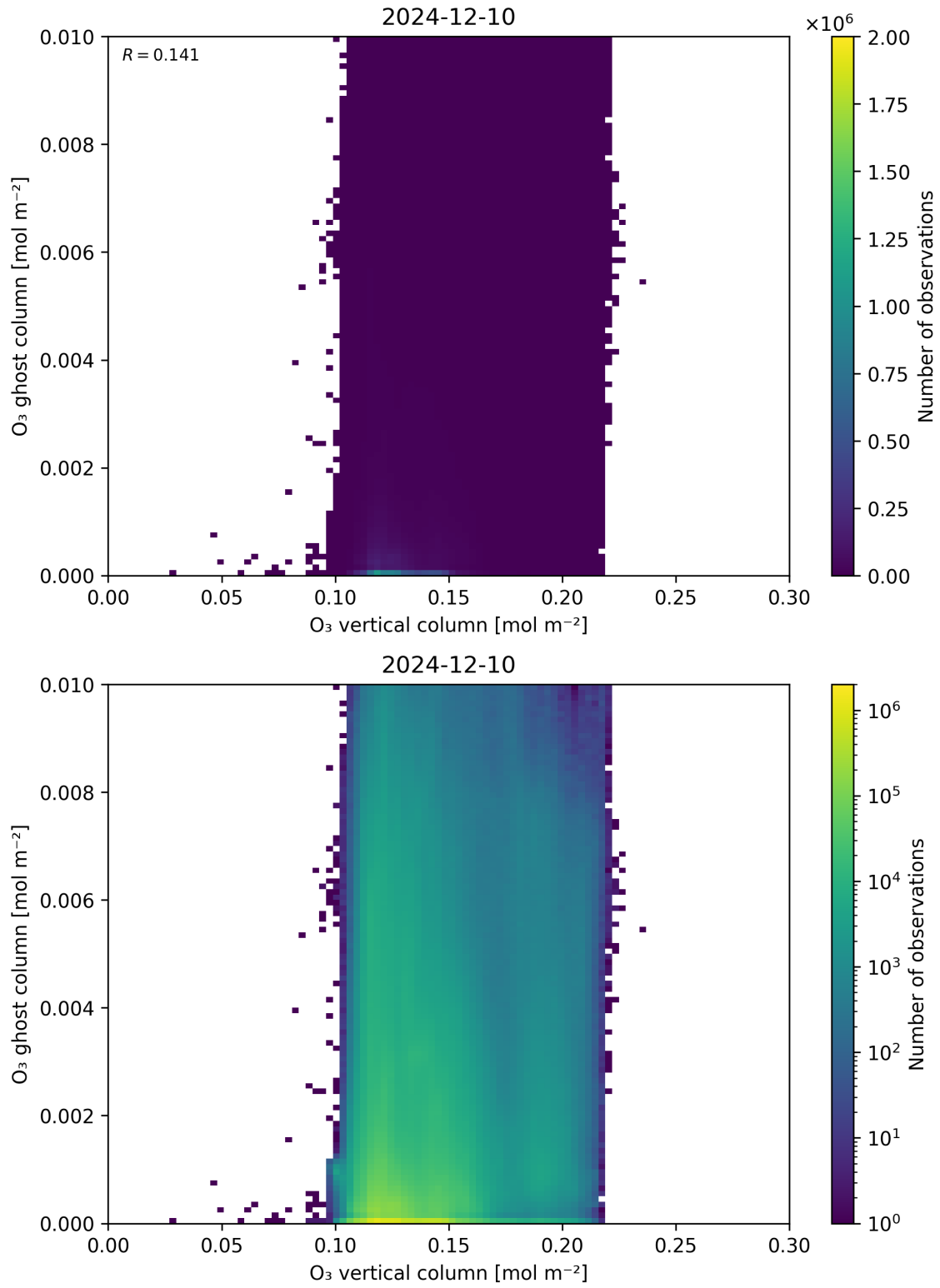
Figure 40: Scatter density plot of “O 3 vertical column” against “O 3 ghost column” for 2024-12-09 to 2024-12-11.
