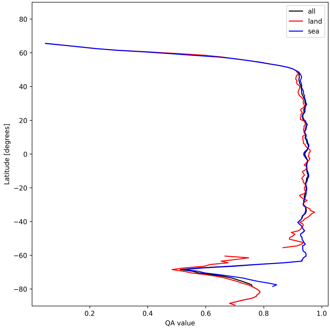
Figure 13: Zonal average of “QA value” for 2024-12-11 to 2024-12-12.
