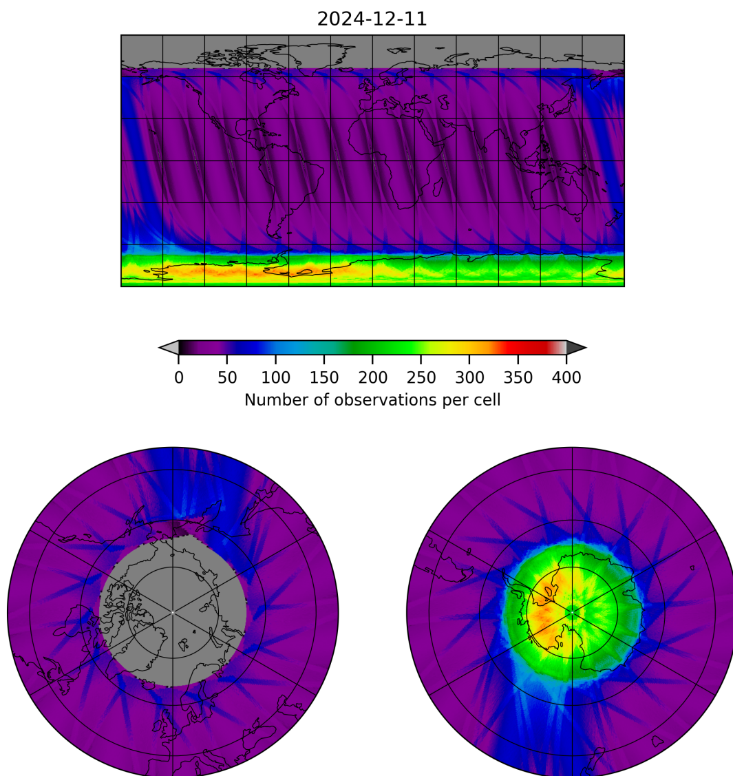
Figure 12: Map of the number of observations for 2024-12-11 to 2024-12-12
