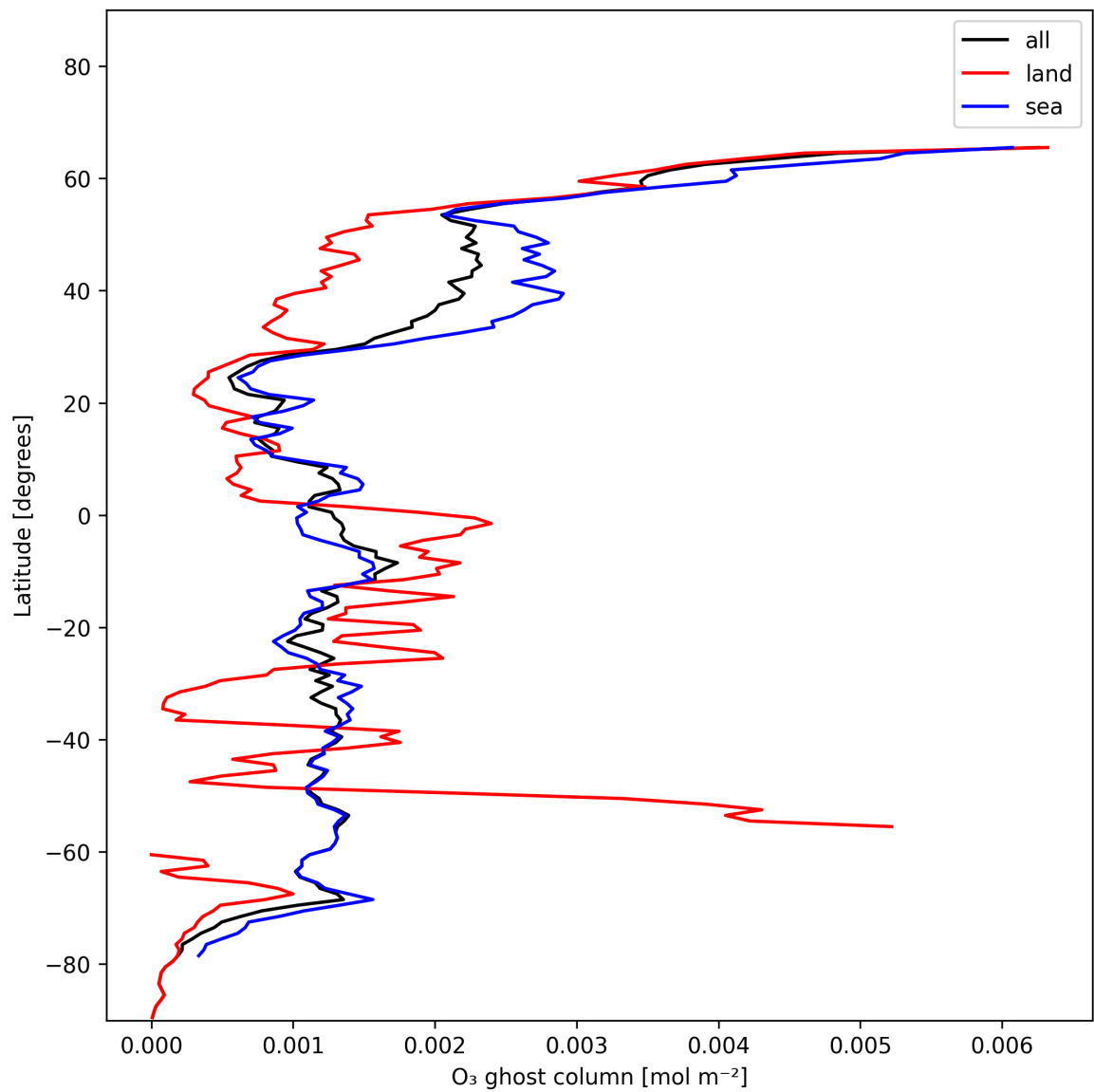
Figure 18: Zonal average of “O 3 ghost column” for 2024-12-11 to 2024-12-12.
