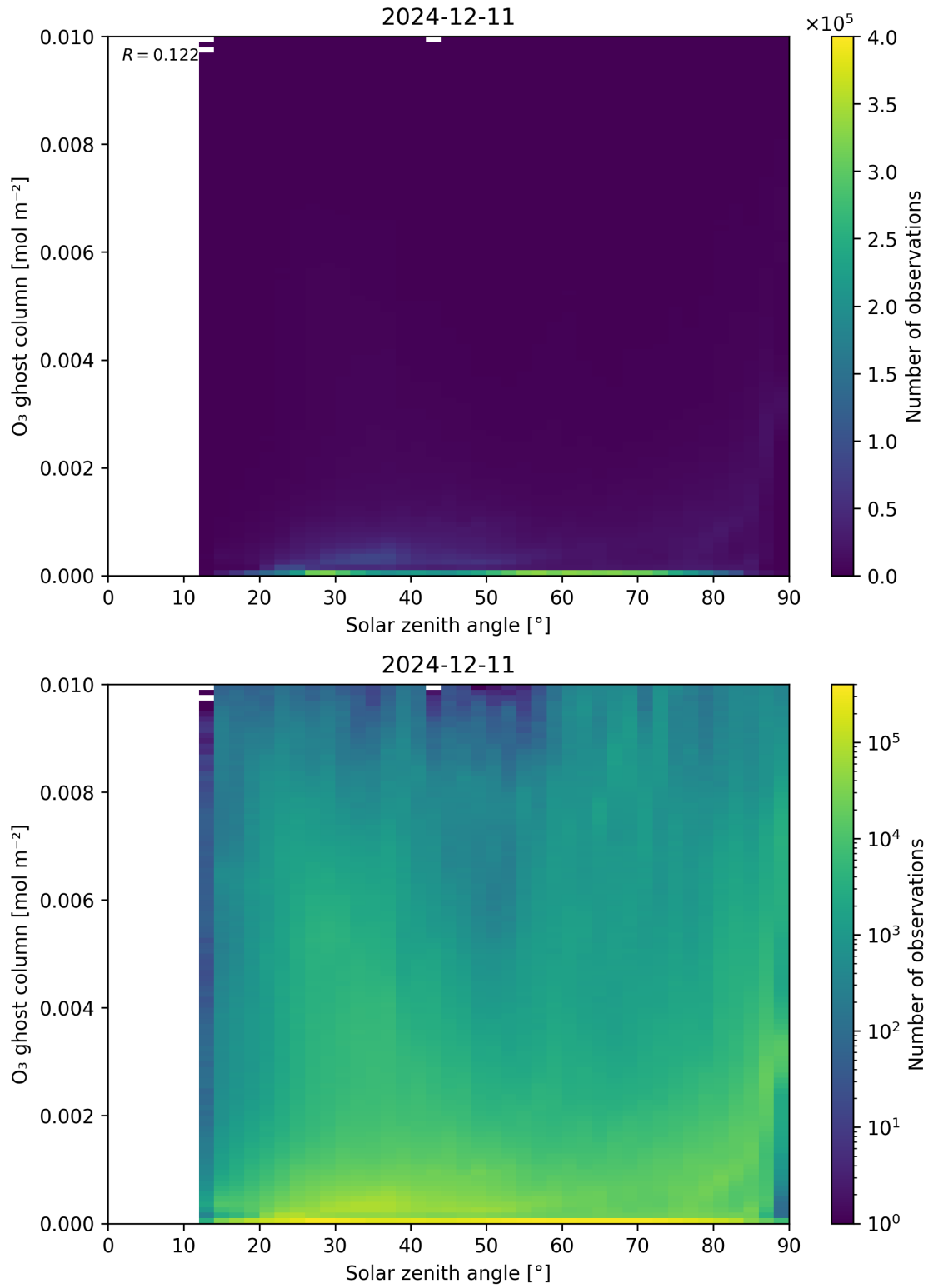
Figure 46: Scatter density plot of “Solar zenith angle” against “O 3 ghost column” for 2024-12-11 to 2024-12-12.
