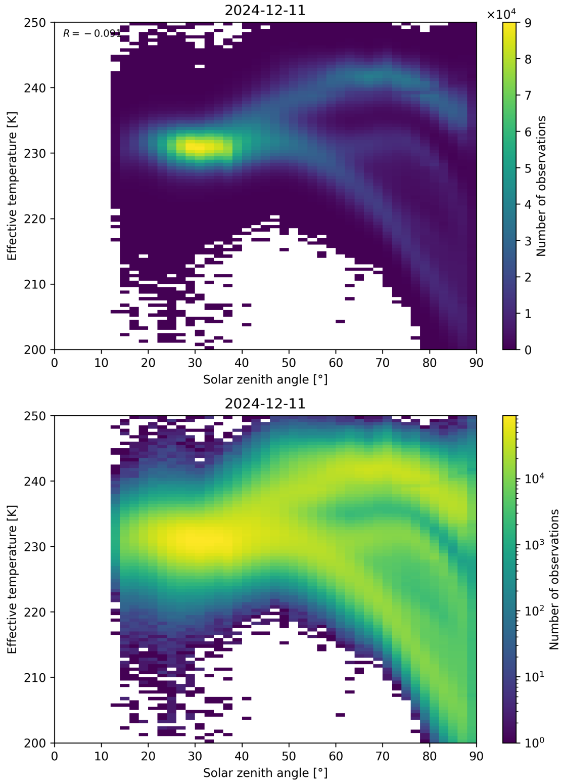
Figure 45: Scatter density plot of “Solar zenith angle” against “Effective temperature” for 2024-12-11 to 2024-12-12.
