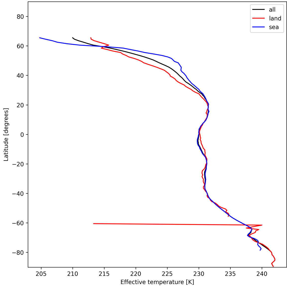
Figure 17: Zonal average of “Effective temperature” for 2024-12-11 to 2024-12-12.
