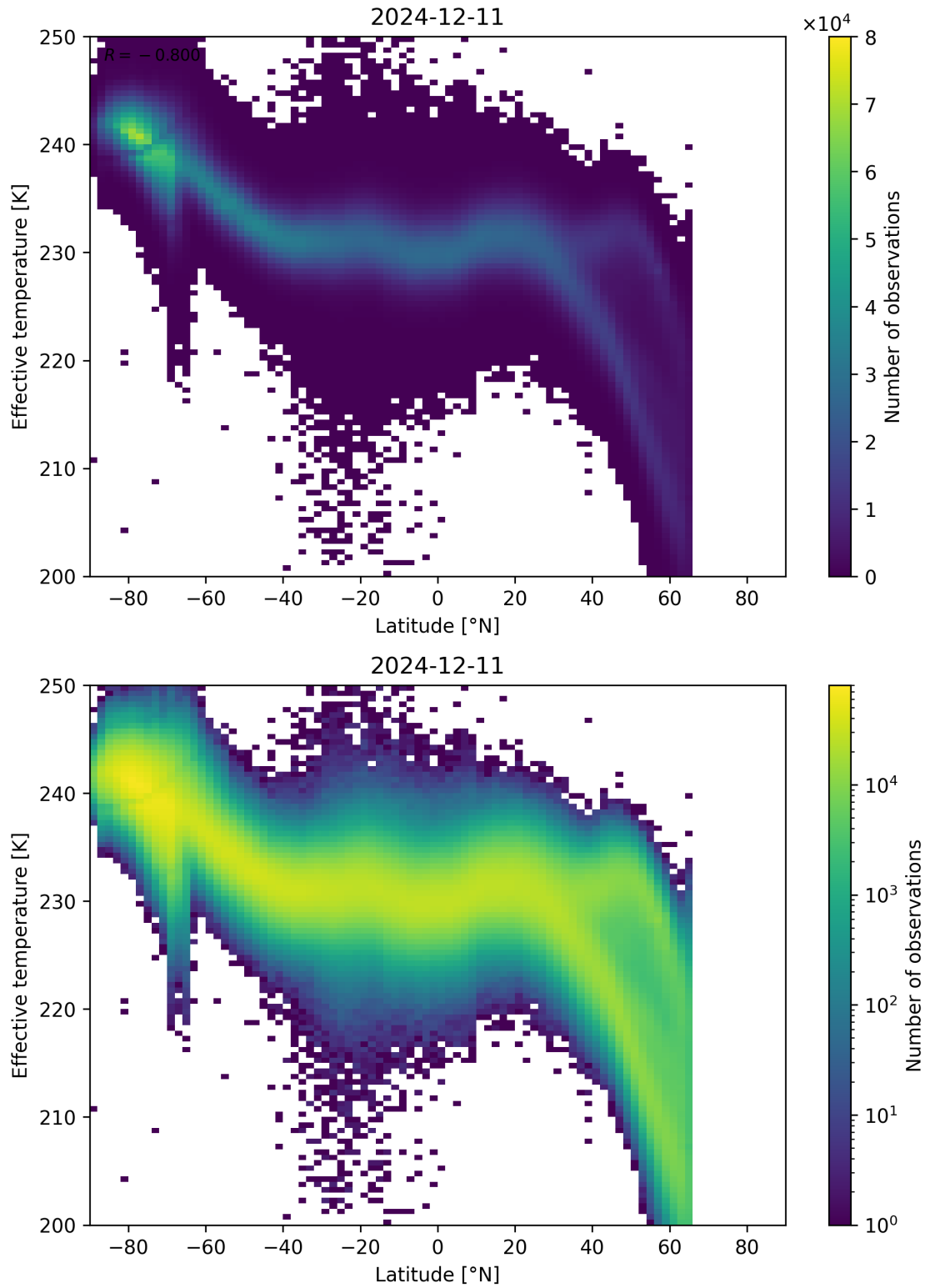
Figure 34: Scatter density plot of “Latitude” against “Effective temperature” for 2024-12-11 to 2024-12-12.
