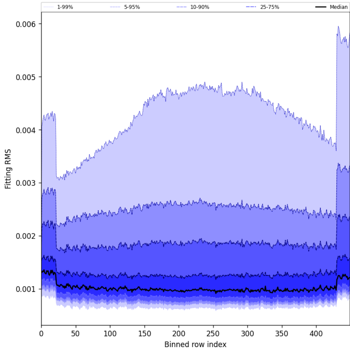
Figure 30: Along track statistics of “Fitting RMS” for 2024-12-11 to 2024-12-12
