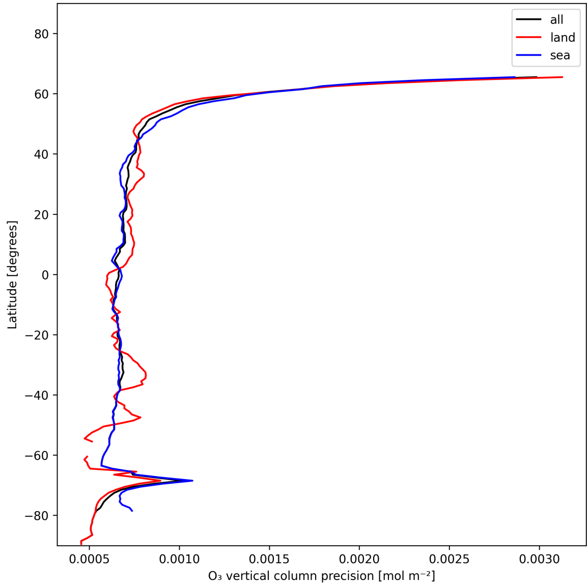
Figure 15: Zonal average of “O 3 vertical column precision” for 2024-12-11 to 2024-12-12.
