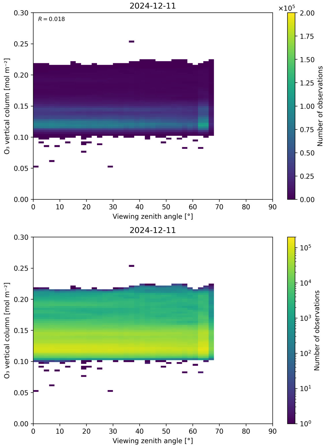
Figure 52: Scatter density plot of “Viewing zenith angle” against “O 3 vertical column” for 2024-12-11 to 2024-12-12.
