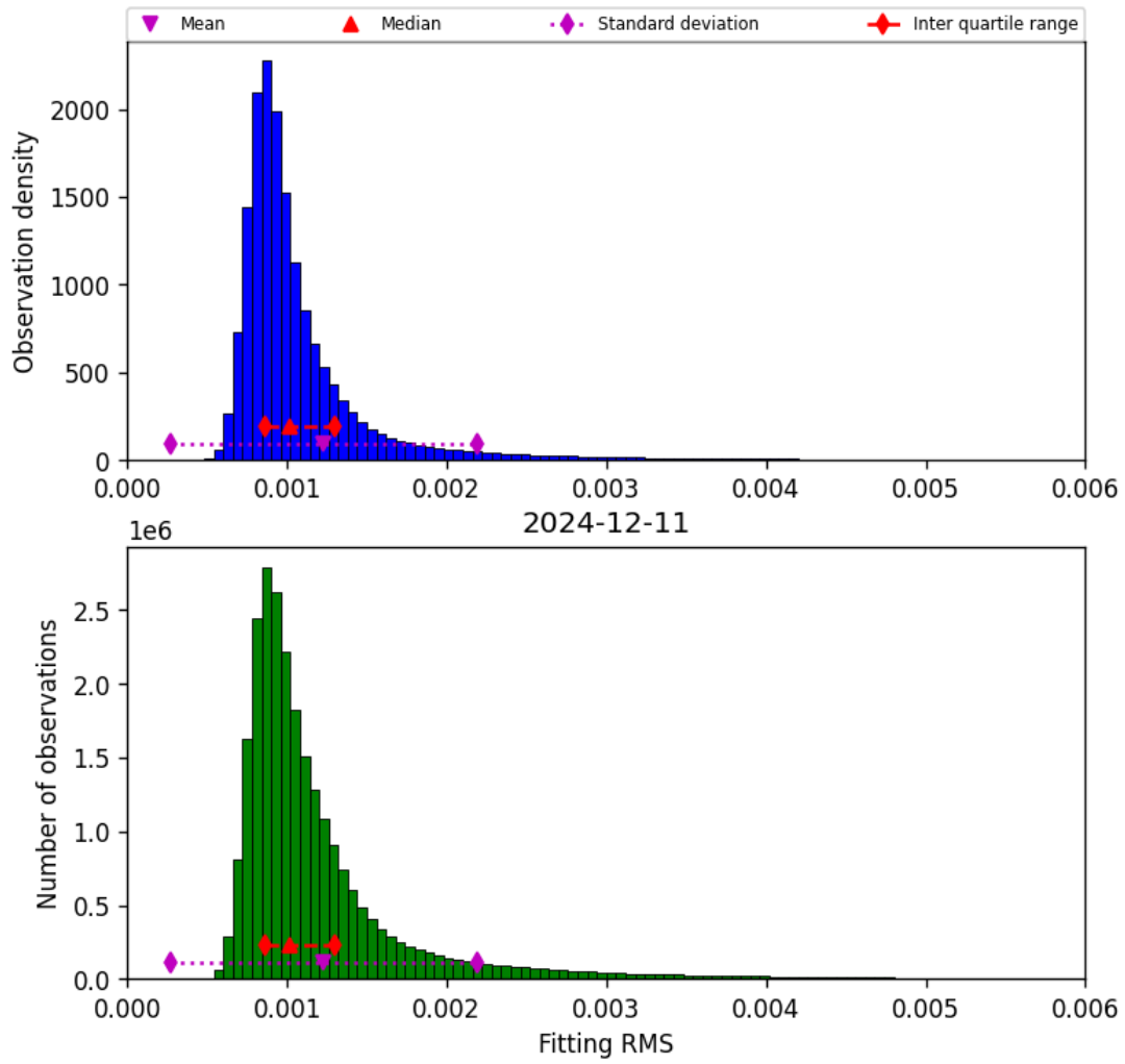
Figure 23: Histogram of “Fitting RMS” for 2024-12-11 to 2024-12-12
