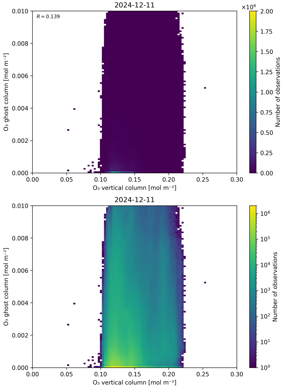
Figure 40: Scatter density plot of “O 3 vertical column” against “O 3 ghost column” for 2024-12-11 to 2024-12-12.
