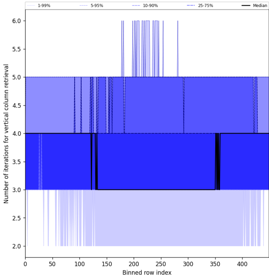
Figure 33: Along track statistics of “Number of iterations for vertical column retrieval” for 2024-12-11 to 2024-12-12
