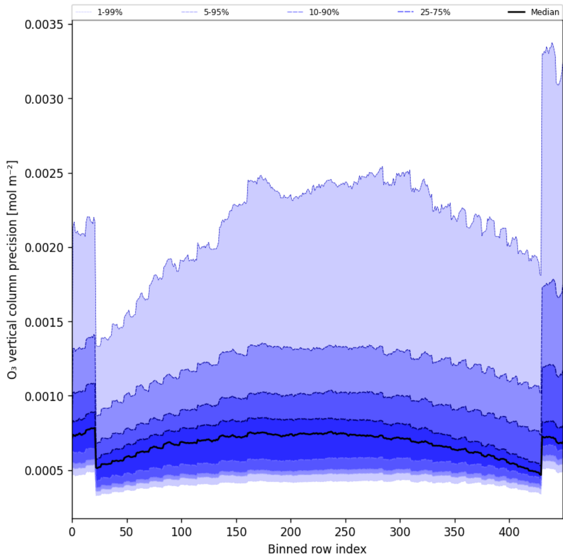
Figure 29: Along track statistics of “O 3 vertical column precision” for 2024-12-11 to 2024-12-12
