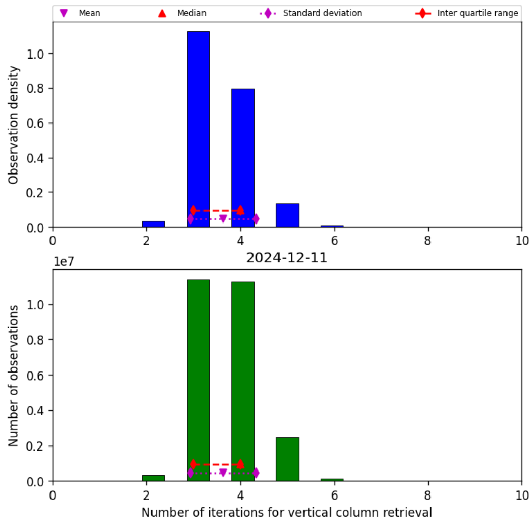
Figure 26: Histogram of “Number of iterations for vertical column retrieval” for 2024-12-11 to 2024-12-12
