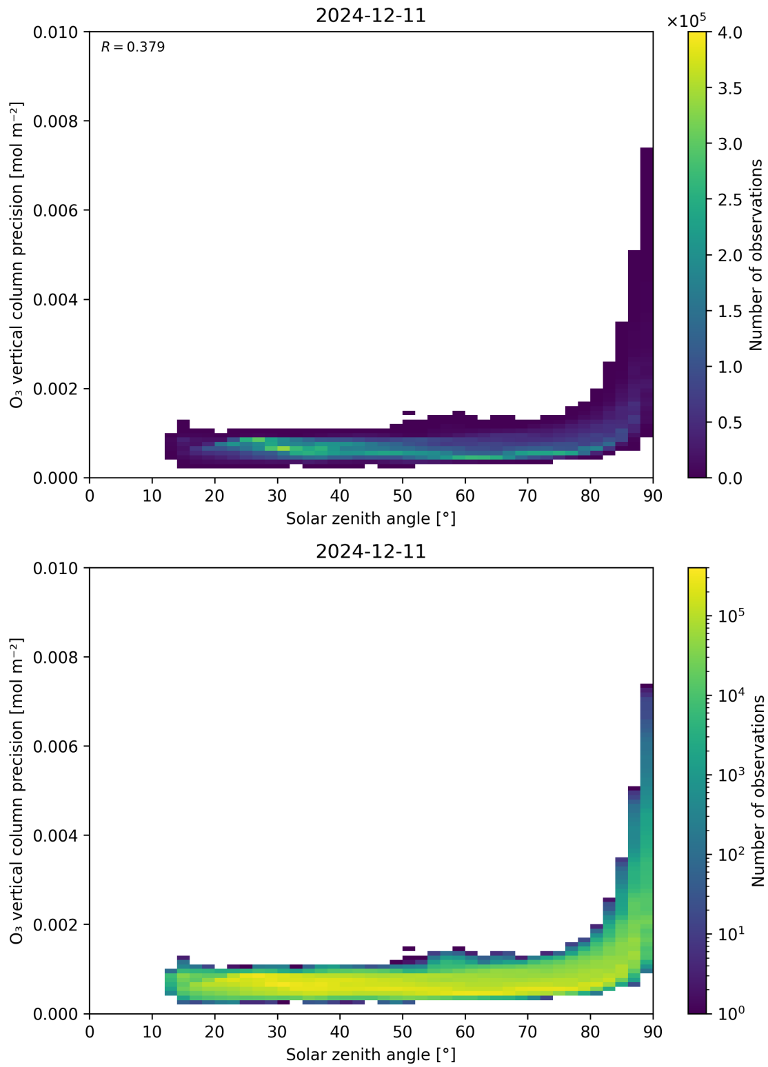
Figure 48: Scatter density plot of “Solar zenith angle” against “O 3 vertical column precision” for 2024-12-11 to 2024-12-12.
