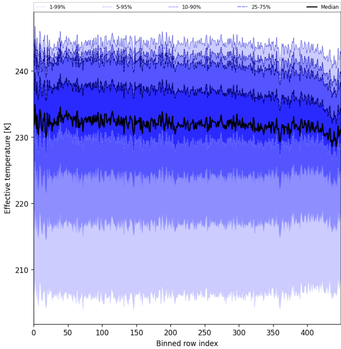
Figure 31: Along track statistics of “Effective temperature” for 2024-12-11 to 2024-12-12
