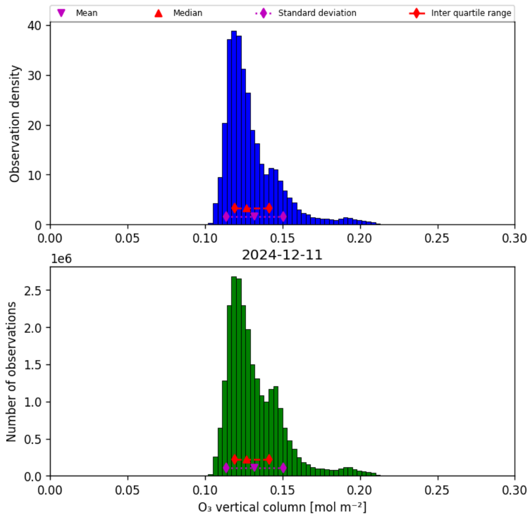
Figure 21: Histogram of “O 3 vertical column” for 2024-12-11 to 2024-12-12
