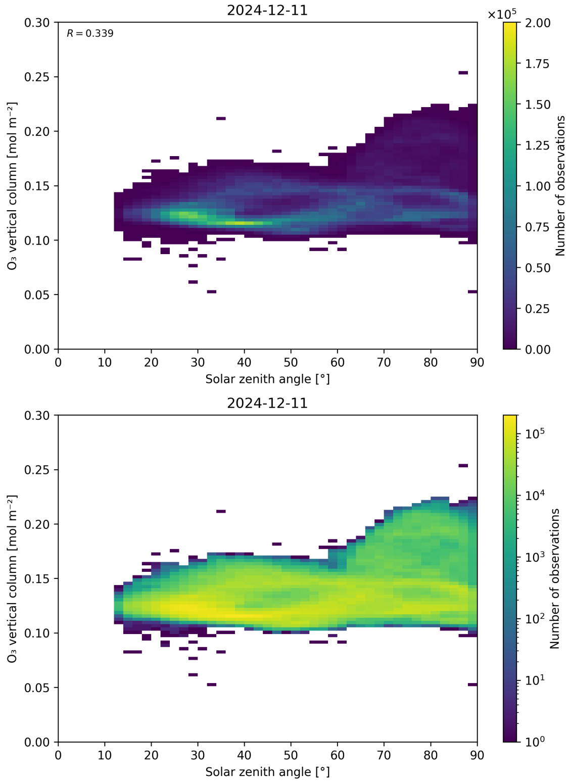
Figure 47: Scatter density plot of “Solar zenith angle” against “O 3 vertical column” for 2024-12-11 to 2024-12-12.
