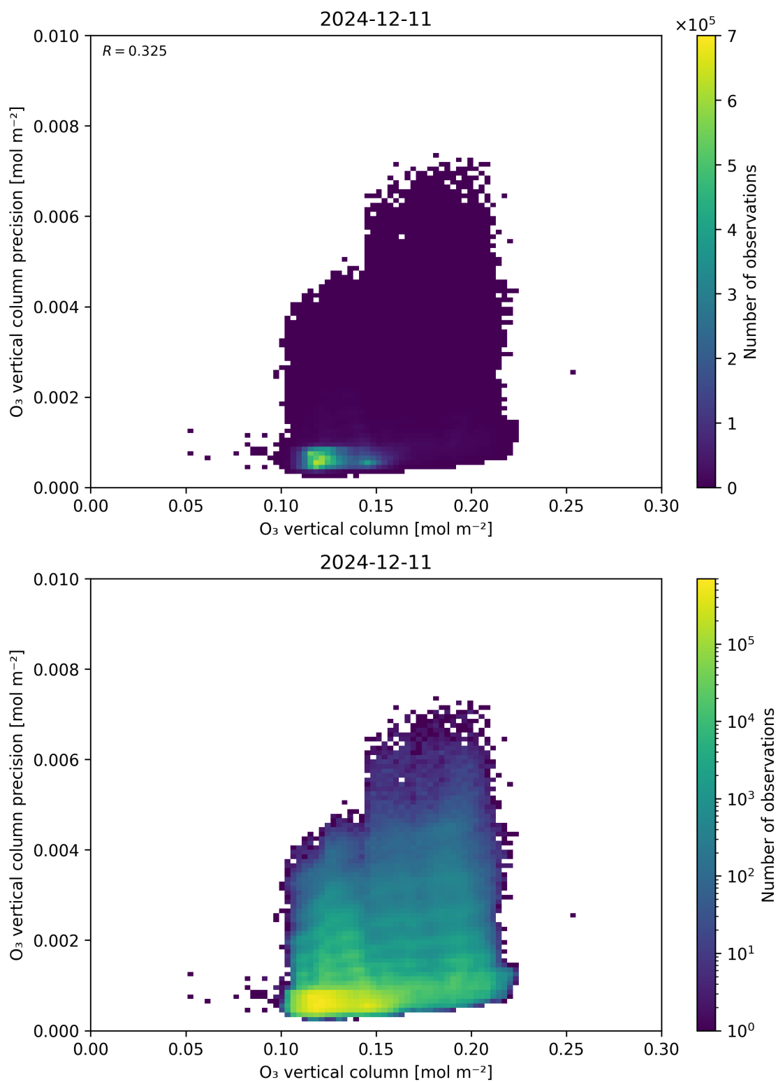
Figure 41: Scatter density plot of “O 3 vertical column” against “O 3 vertical column precision” for 2024-12-11 to 2024-12-12.
