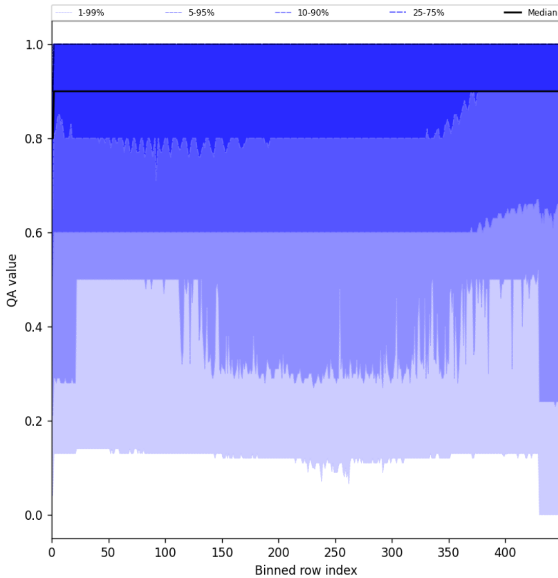
Figure 27: Along track statistics of “QA value” for 2024-12-11 to 2024-12-12
