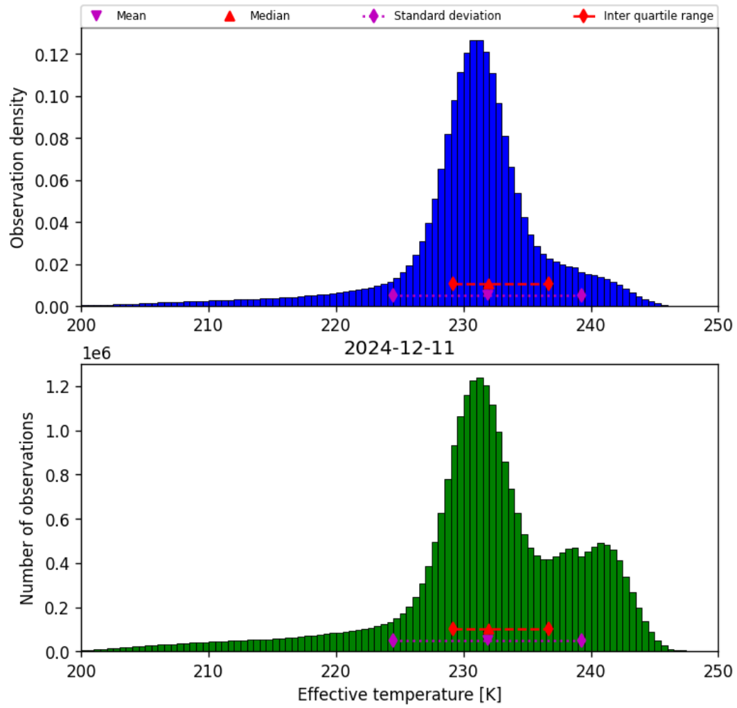
Figure 24: Histogram of “Effective temperature” for 2024-12-11 to 2024-12-12
