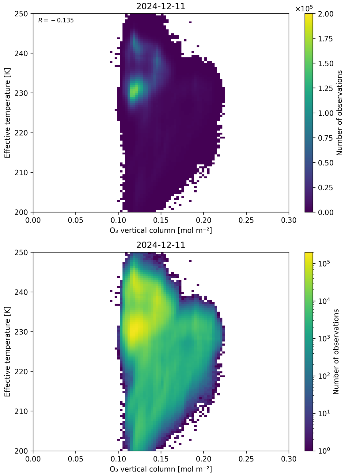
Figure 39: Scatter density plot of “O 3 vertical column” against “Effective temperature” for 2024-12-11 to 2024-12-12.
