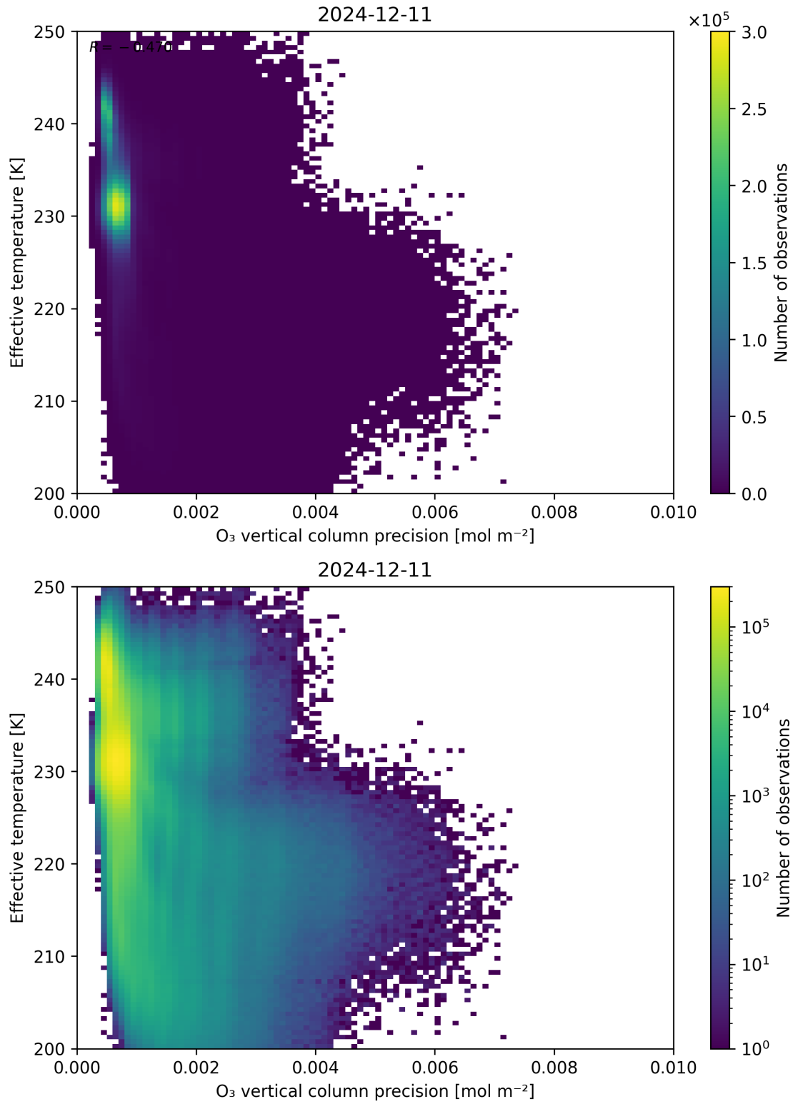
Figure 42: Scatter density plot of “O 3 vertical column precision” against “Effective temperature” for 2024-12-11 to 2024-12-12.
