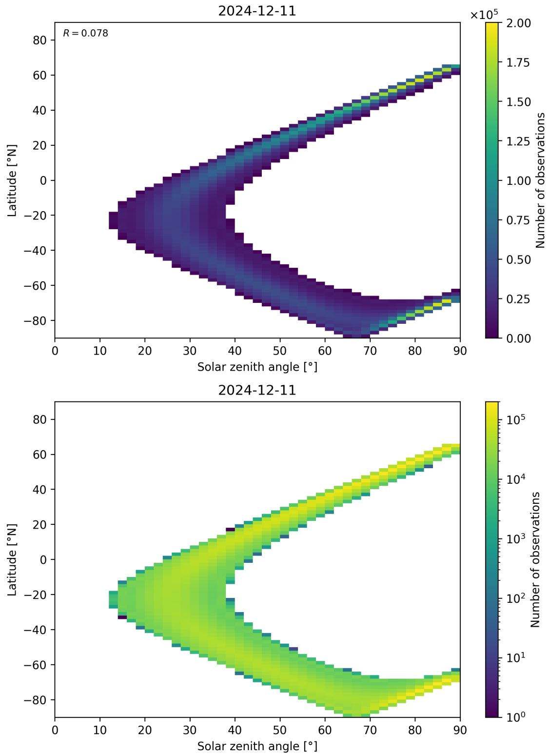
Figure 44: Scatter density plot of “Solar zenith angle” against “Latitude” for 2024-12-11 to 2024-12-12.
