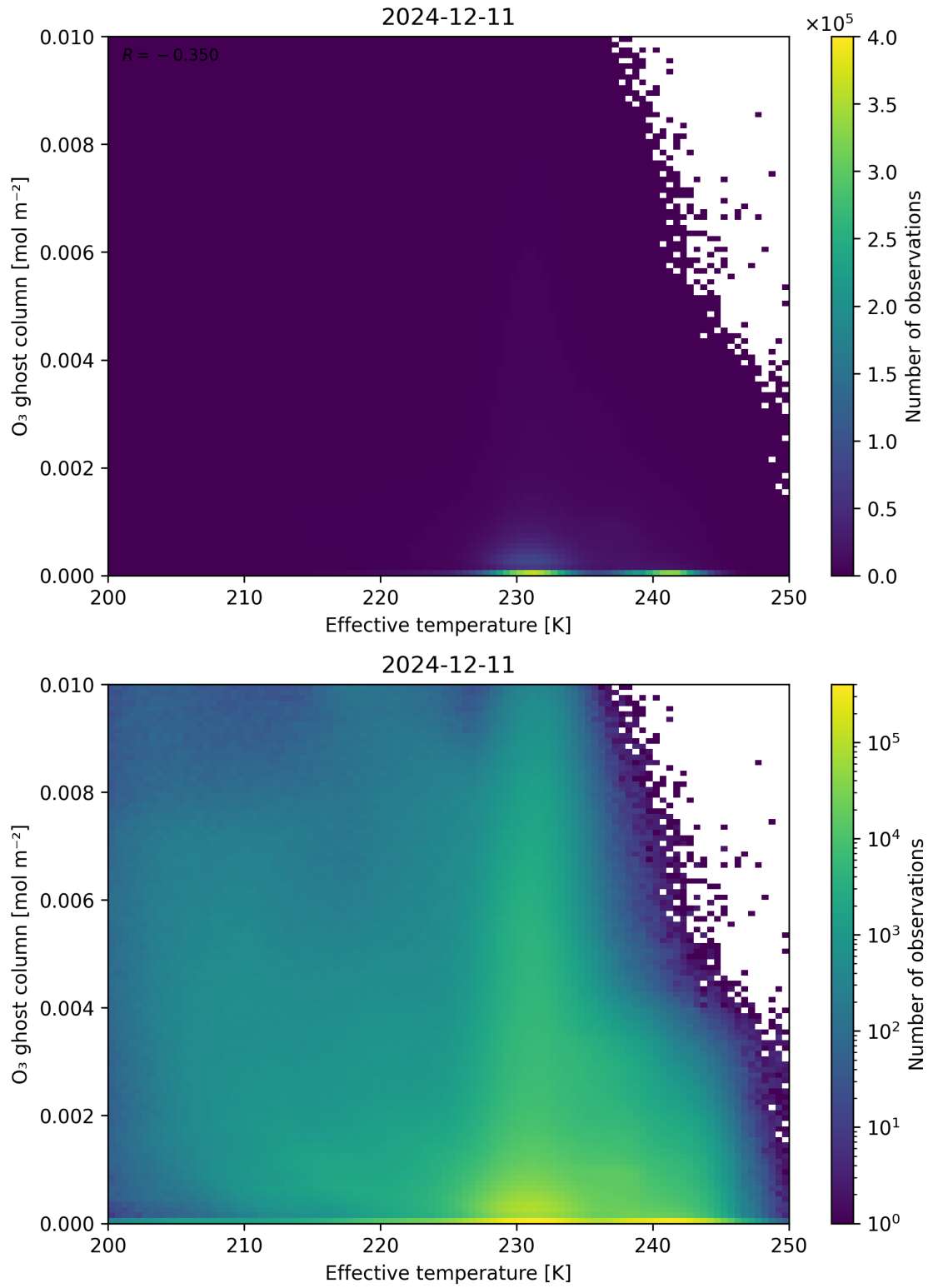
Figure 38: Scatter density plot of “Effective temperature” against “O 3 ghost column” for 2024-12-11 to 2024-12-12.
