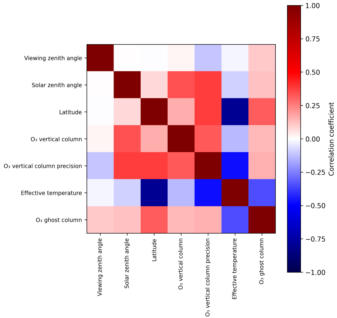
Figure 2: Map of correlation matrix for 2024-12-11 to 2024-12-12.
