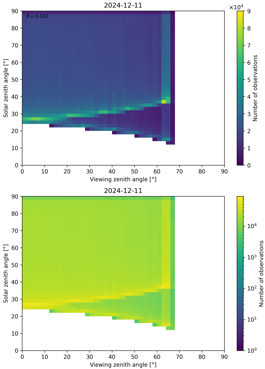
Figure 54: Scatter density plot of “Viewing zenith angle” against “Solar zenith angle” for 2024-12-11 to 2024-12-12.
