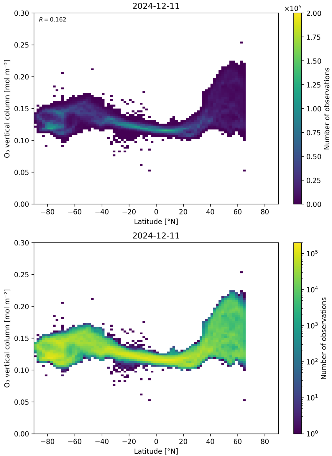
Figure 36: Scatter density plot of “Latitude” against “O 3 vertical column” for 2024-12-11 to 2024-12-12.
