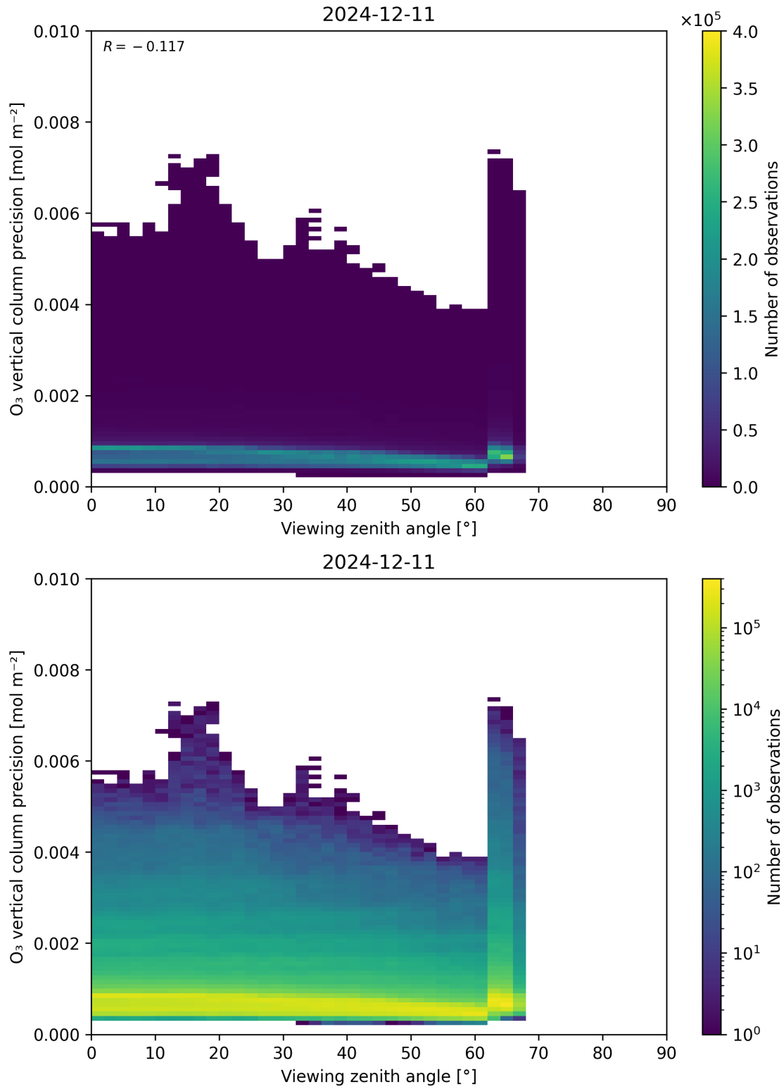
Figure 53: Scatter density plot of “Viewing zenith angle” against “O 3 vertical column precision” for 2024-12-11 to 2024-12-12.
