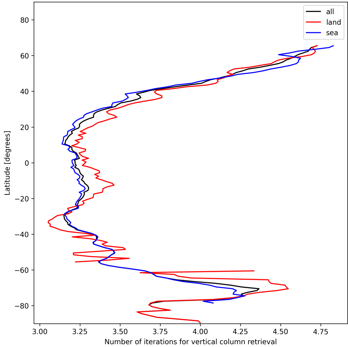
Figure 19: Zonal average of “Number of iterations for vertical column retrieval” for 2024-12-11 to 2024-12-12.
