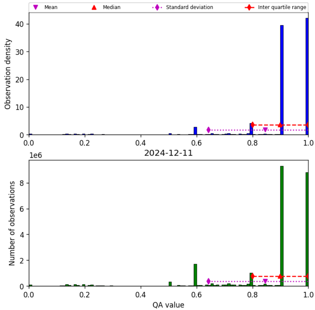
Figure 20: Histogram of “QA value” for 2024-12-11 to 2024-12-12
