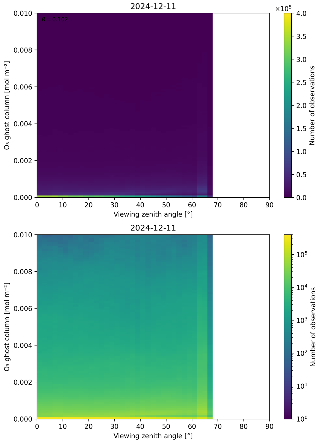
Figure 51: Scatter density plot of “Viewing zenith angle” against “O 3 ghost column” for 2024-12-11 to 2024-12-12.
