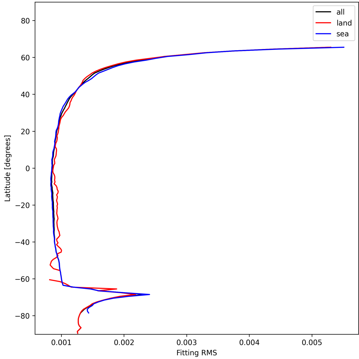
Figure 16: Zonal average of “Fitting RMS” for 2024-12-11 to 2024-12-12.
