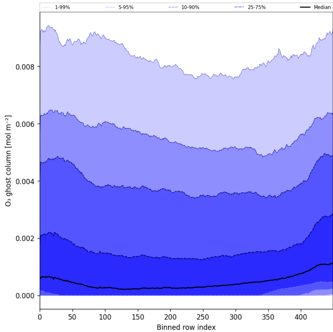
Figure 32: Along track statistics of “O 3 ghost column” for 2024-12-11 to 2024-12-12
