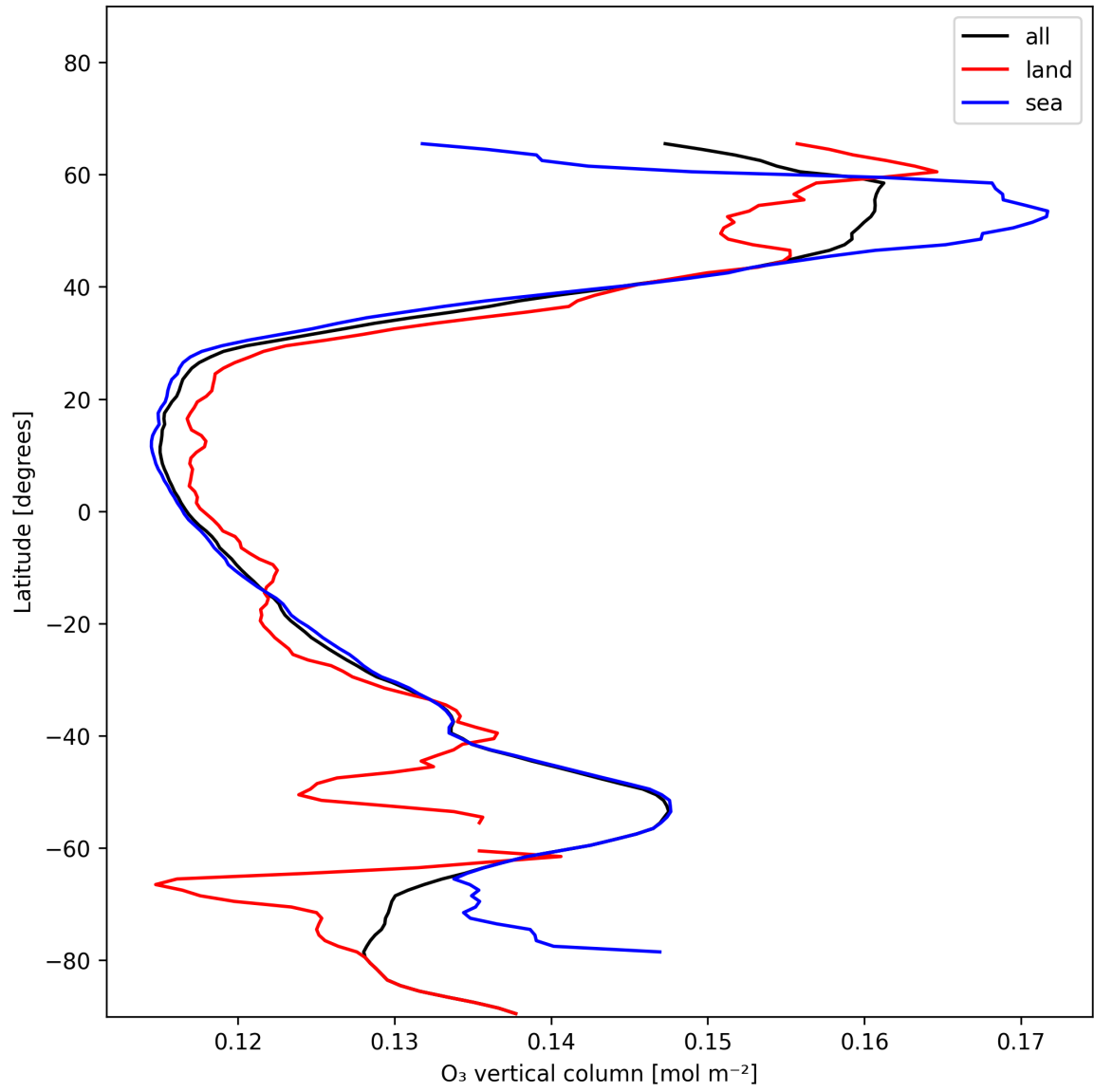
Figure 14: Zonal average of “O 3 vertical column” for 2024-12-11 to 2024-12-12.
