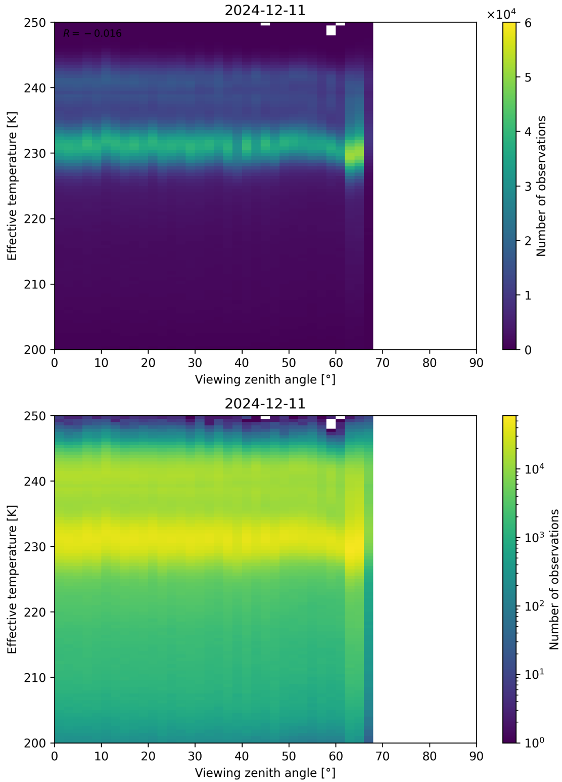
Figure 50: Scatter density plot of “Viewing zenith angle” against “Effective temperature” for 2024-12-11 to 2024-12-12.
