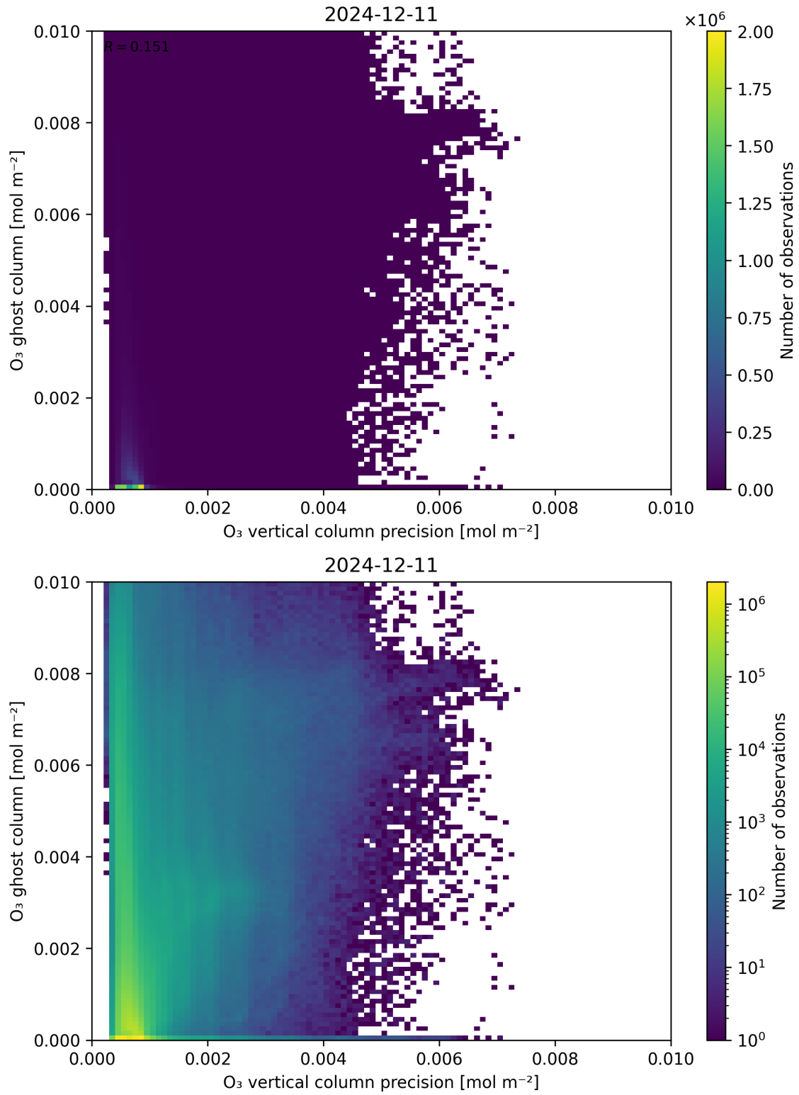
Figure 43: Scatter density plot of “ O_3 vertical column precision” against “ O_3 ghost column” for 2024-12-11 to 2024-12-12.
