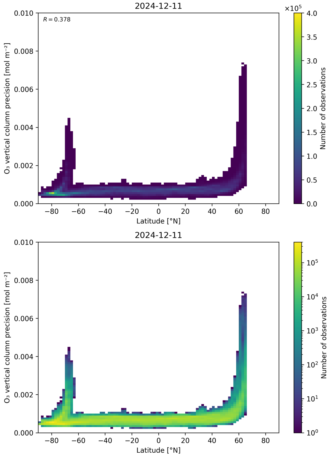
Figure 37: Scatter density plot of “Latitude” against “O 3 vertical column precision” for 2024-12-11 to 2024-12-12.
