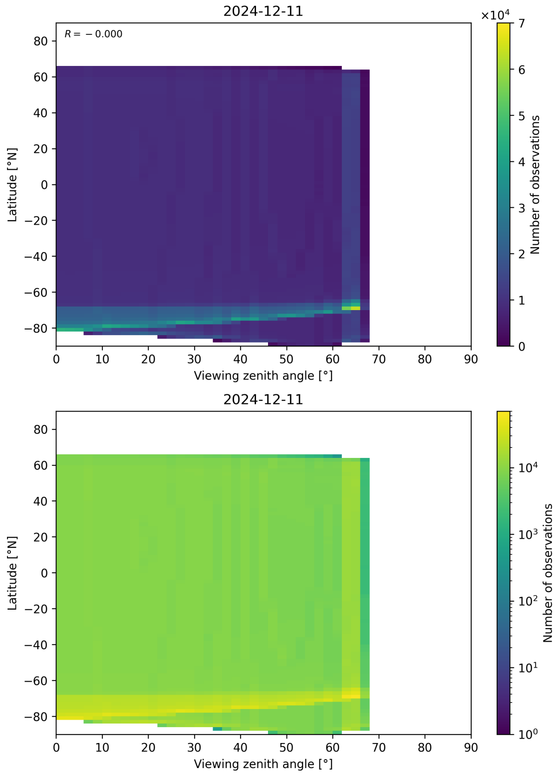
Figure 49: Scatter density plot of “Viewing zenith angle” against “Latitude” for 2024-12-11 to 2024-12-12.
