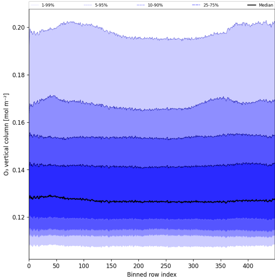
Figure 28: Along track statistics of “O 3 vertical column” for 2024-12-11 to 2024-12-12
