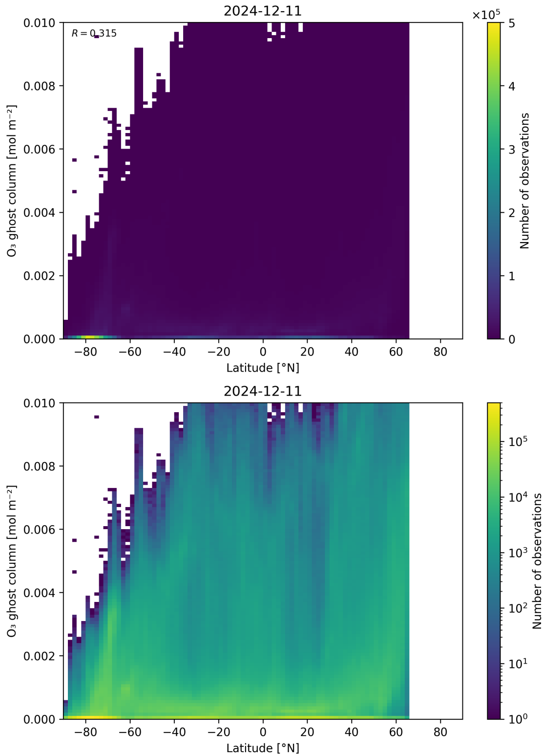
Figure 35: Scatter density plot of “Latitude” against “O 3 ghost column” for 2024-12-11 to 2024-12-12.
