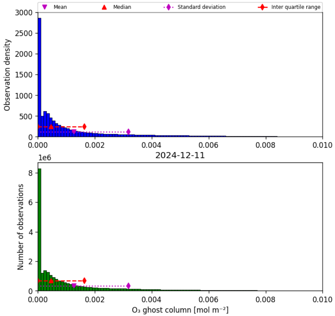
Figure 25: Histogram of “O 3 ghost column” for 2024-12-11 to 2024-12-12
