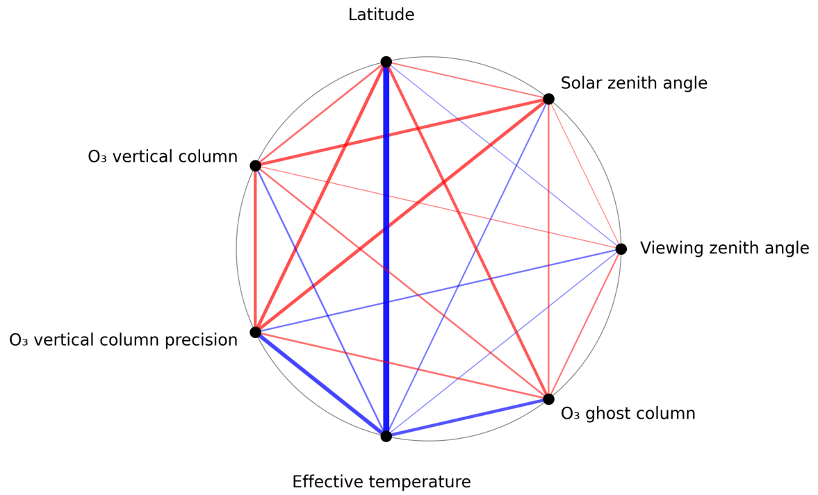
Figure 1: Map of correlation graph for 2024-12-11 to 2024-12-12.
