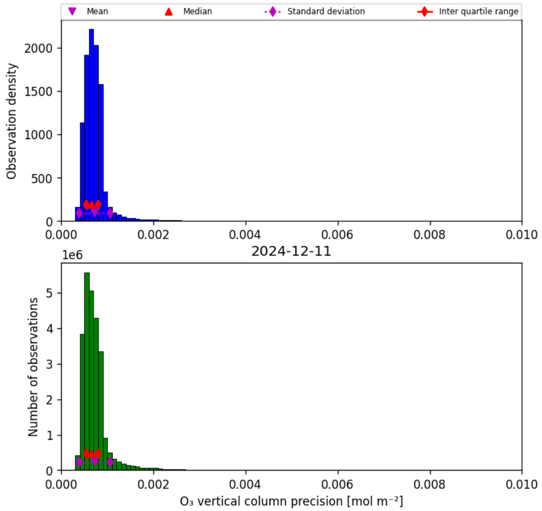
Figure 22: Histogram of “O 3 vertical column precision” for 2024-12-11 to 2024-12-12
