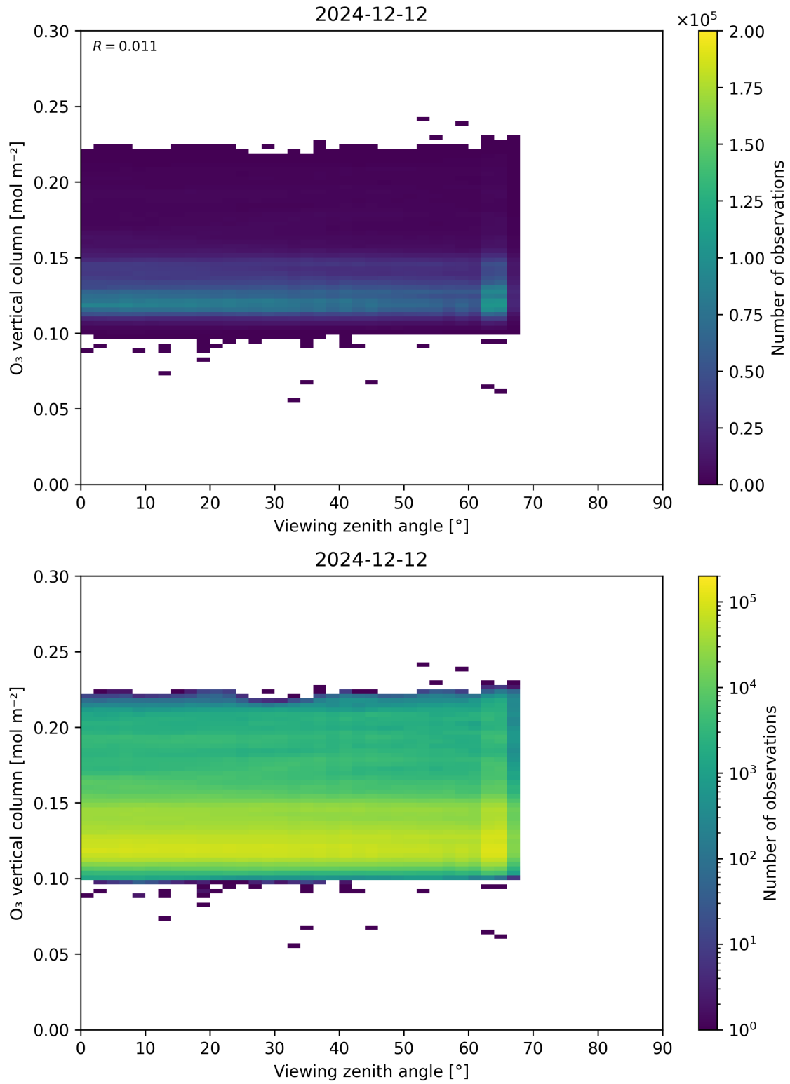
Figure 52: Scatter density plot of “Viewing zenith angle” against “O 3 vertical column” for 2024-12-11 to 2024-12-13.
