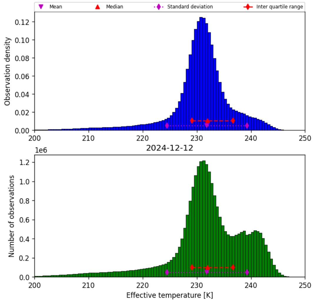
Figure 24: Histogram of “Effective temperature” for 2024-12-11 to 2024-12-13
