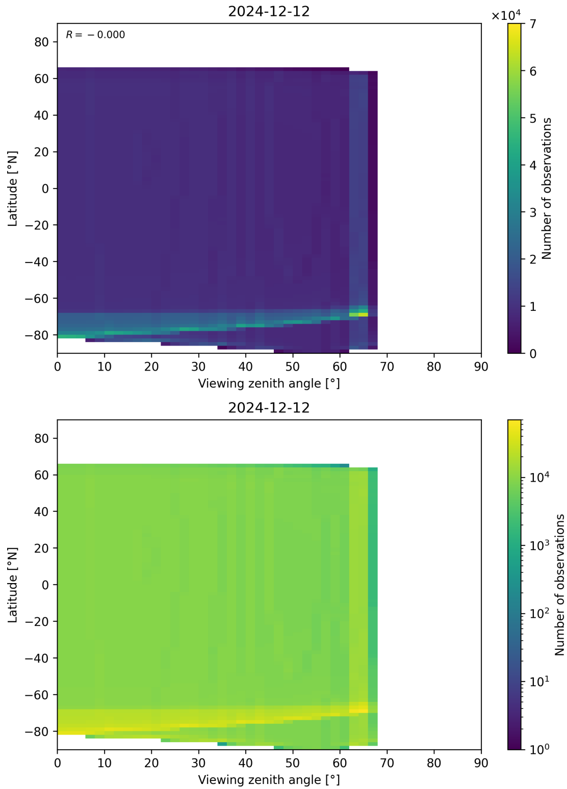
Figure 49: Scatter density plot of “Viewing zenith angle” against “Latitude” for 2024-12-11 to 2024-12-13.
