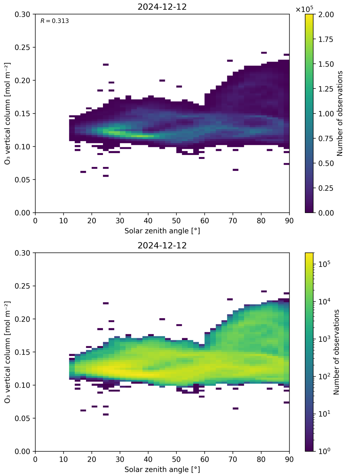
Figure 47: Scatter density plot of “Solar zenith angle” against “O 3 vertical column” for 2024-12-11 to 2024-12-13.
