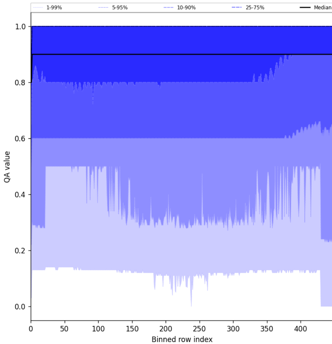
Figure 27: Along track statistics of “QA value” for 2024-12-11 to 2024-12-13
