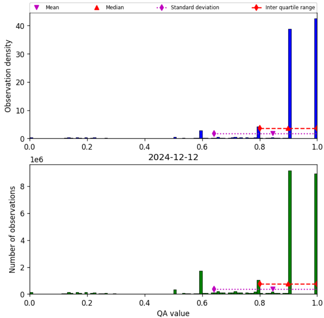
Figure 20: Histogram of “QA value” for 2024-12-11 to 2024-12-13
