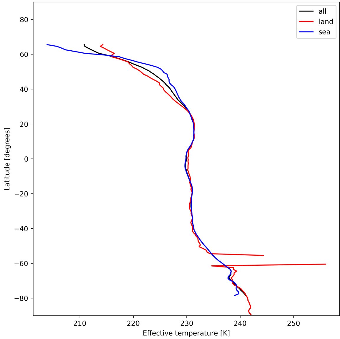
Figure 17: Zonal average of “Effective temperature” for 2024-12-11 to 2024-12-13.
