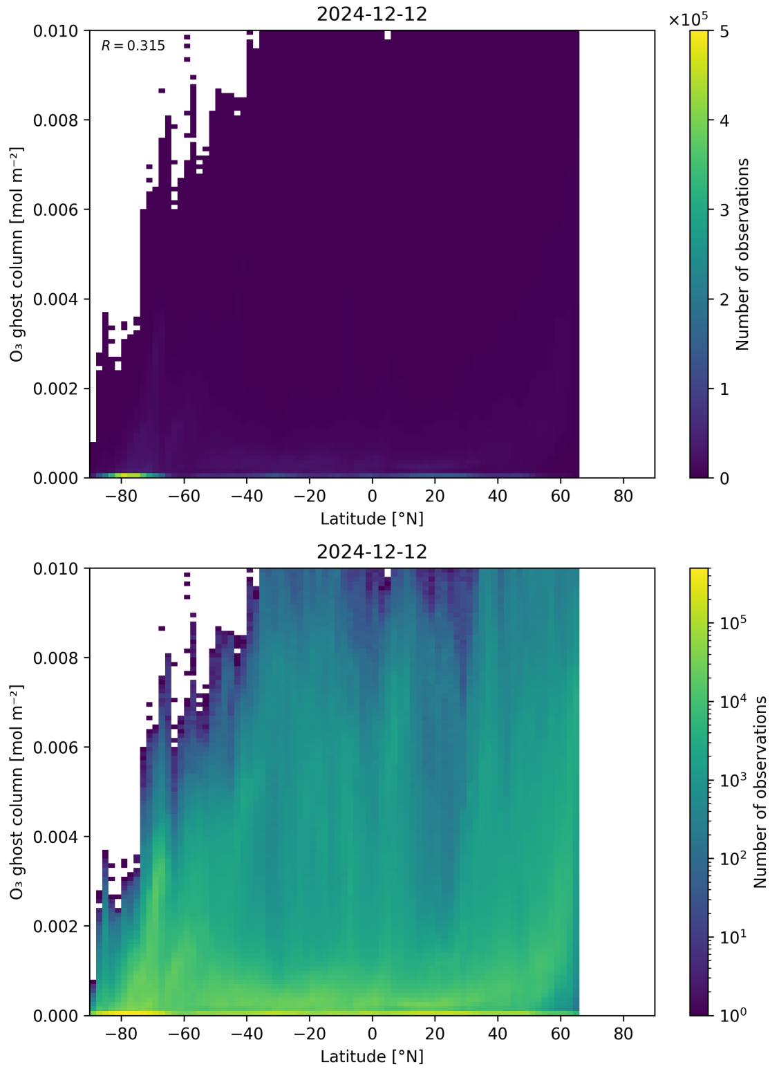
Figure 35: Scatter density plot of “Latitude” against “O 3 ghost column” for 2024-12-11 to 2024-12-13.
