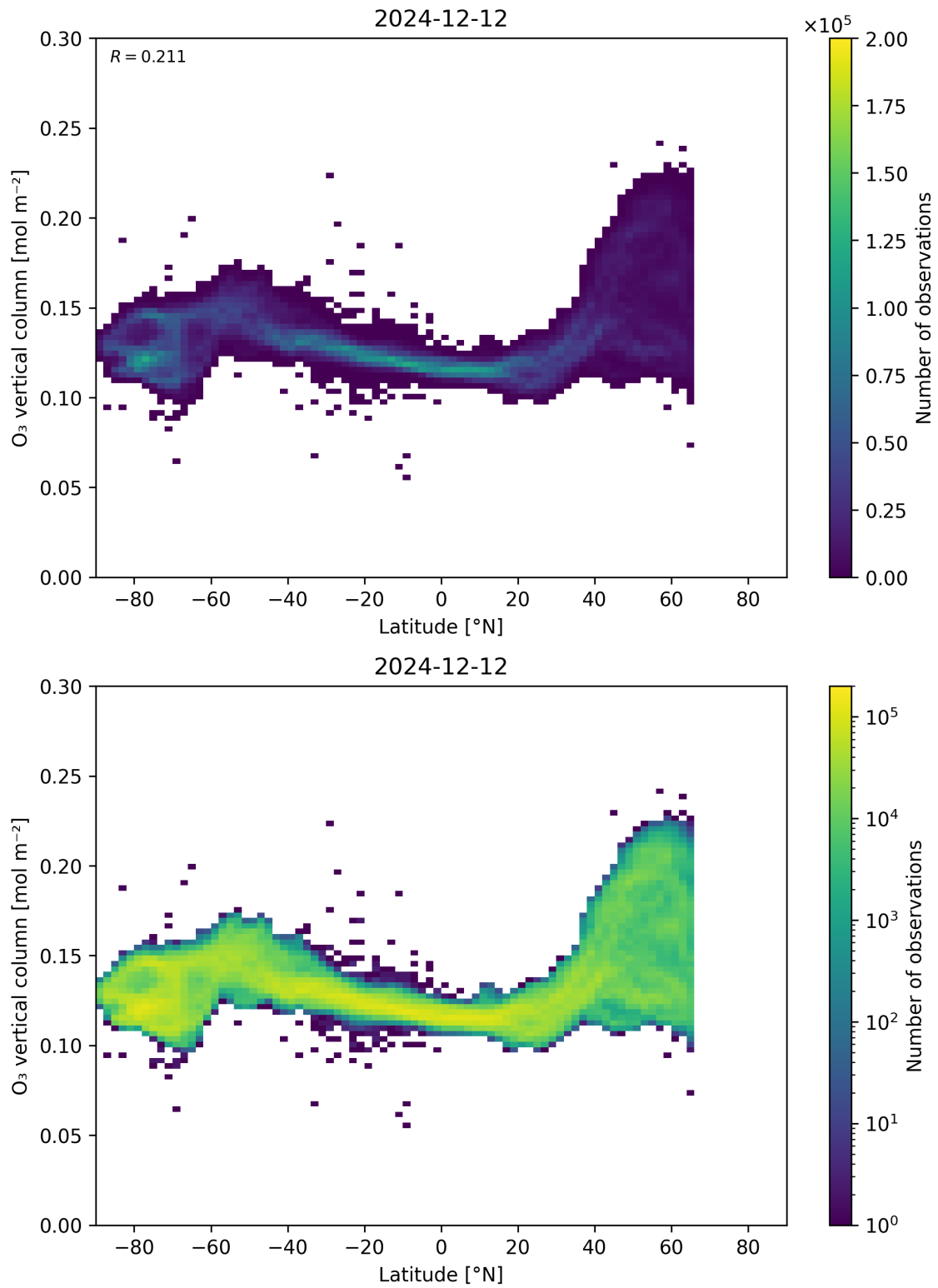
Figure 36: Scatter density plot of “Latitude” against “O 3 vertical column” for 2024-12-11 to 2024-12-13.
