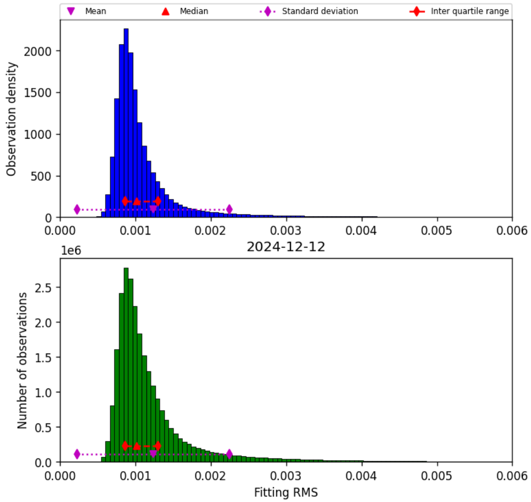
Figure 23: Histogram of “Fitting RMS” for 2024-12-11 to 2024-12-13
