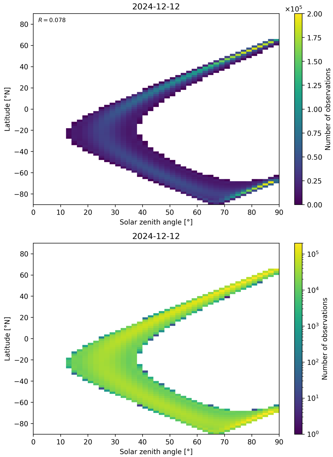
Figure 44: Scatter density plot of “Solar zenith angle” against “Latitude” for 2024-12-11 to 2024-12-13.
