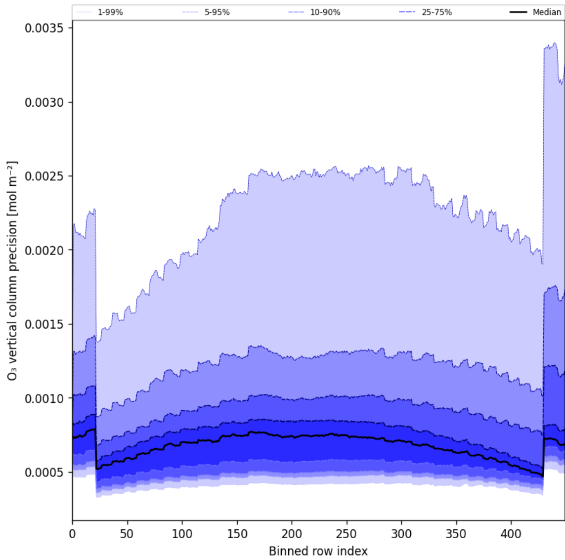
Figure 29: Along track statistics of “O 3 vertical column precision” for 2024-12-11 to 2024-12-13
