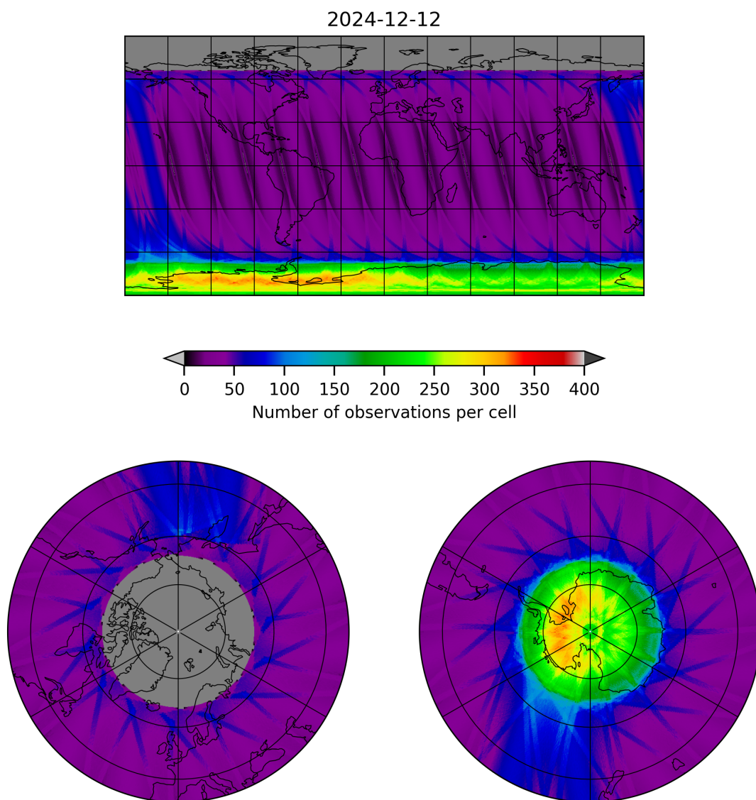
Figure 12: Map of the number of observations for 2024-12-11 to 2024-12-13
