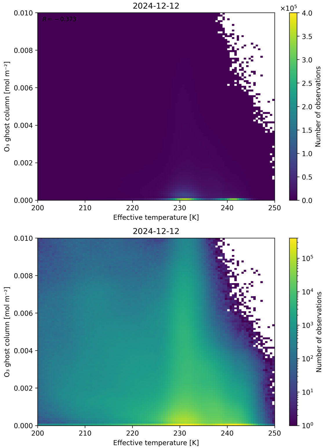
Figure 38: Scatter density plot of “Effective temperature” against “O 3 ghost column” for 2024-12-11 to 2024-12-13.
