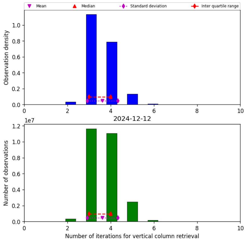
Figure 26: Histogram of “Number of iterations for vertical column retrieval” for 2024-12-11 to 2024-12-13
