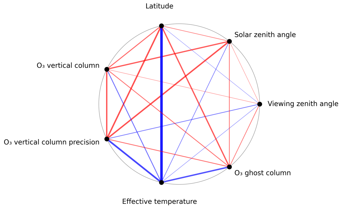
Figure 1: Map of correlation graph for 2024-12-11 to 2024-12-13.
