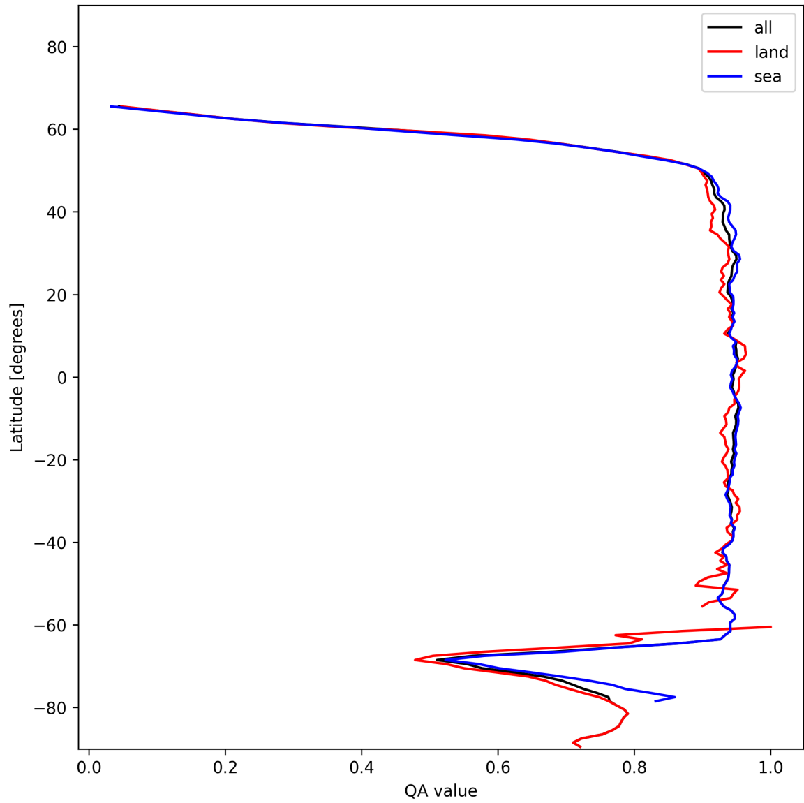
Figure 13: Zonal average of “QA value” for 2024-12-11 to 2024-12-13.
