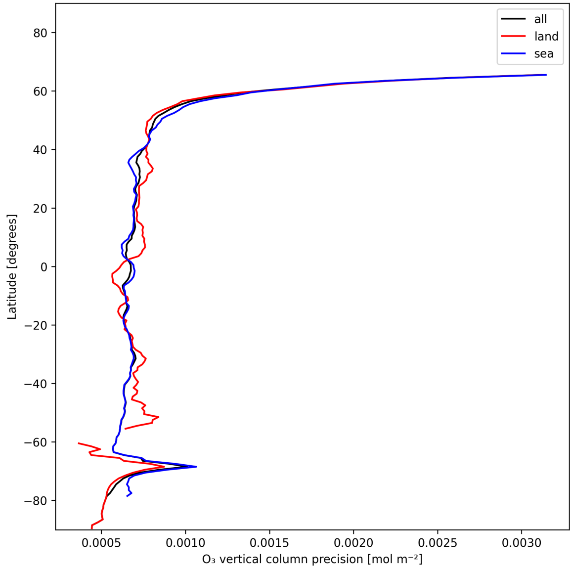
Figure 15: Zonal average of “O 3 vertical column precision” for 2024-12-11 to 2024-12-13.
