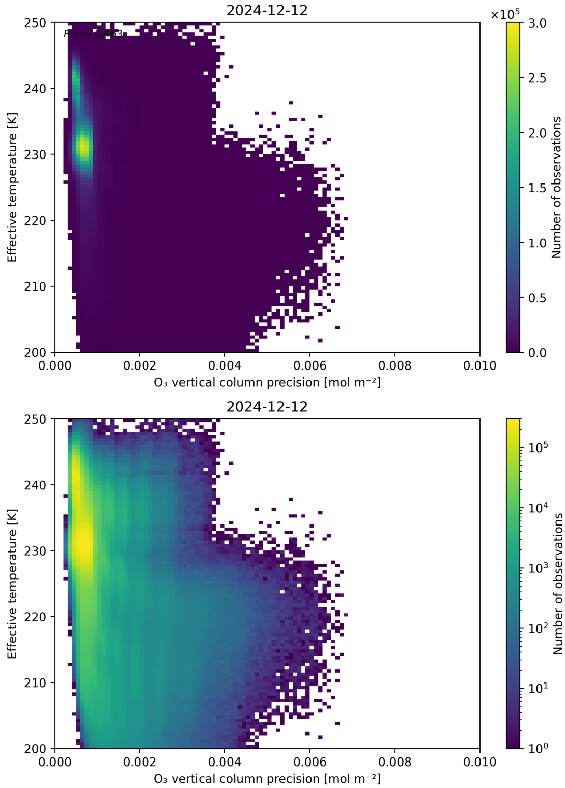
Figure 42: Scatter density plot of “O 3 vertical column precision” against “Effective temperature” for 2024-12-11 to 2024-12-13.
