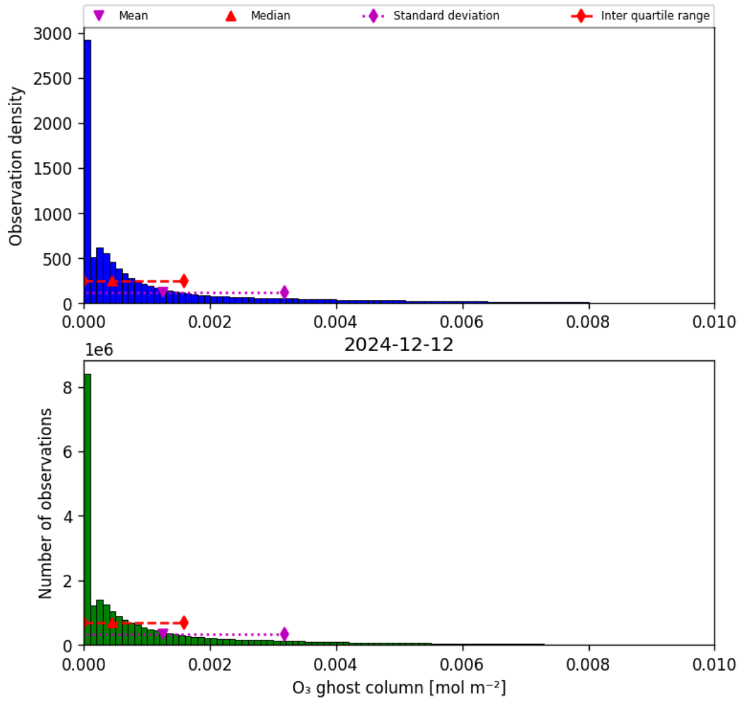
Figure 25: Histogram of “O 3 ghost column” for 2024-12-11 to 2024-12-13
