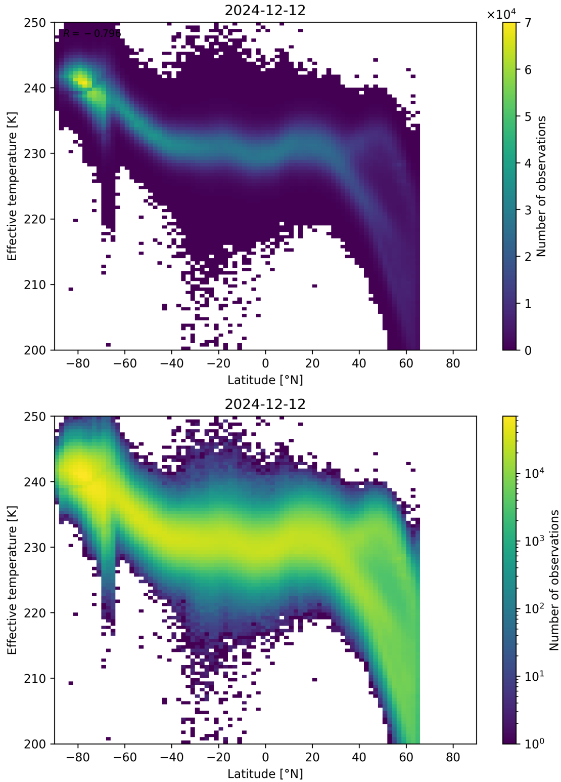
Figure 34: Scatter density plot of “Latitude” against “Effective temperature” for 2024-12-11 to 2024-12-13.
