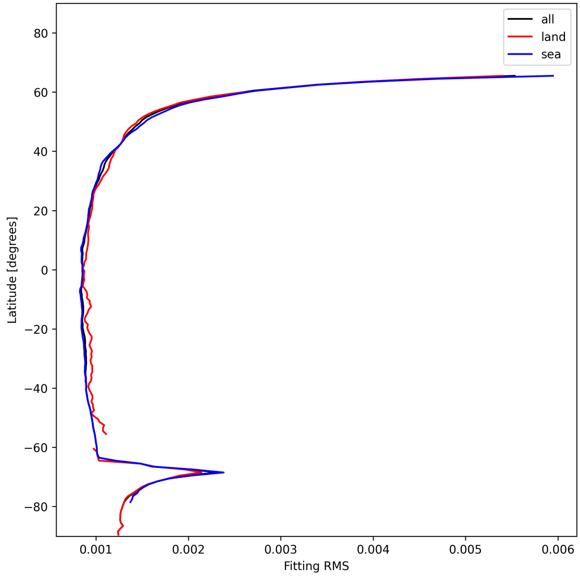
Figure 16: Zonal average of “Fitting RMS” for 2024-12-11 to 2024-12-13.
