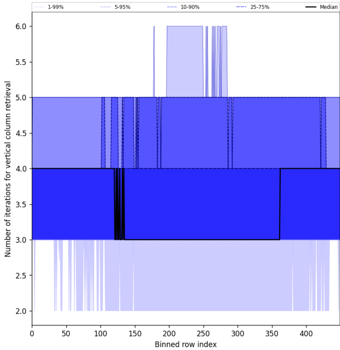
Figure 33: Along track statistics of “Number of iterations for vertical column retrieval” for 2024-12-11 to 2024-12-13
