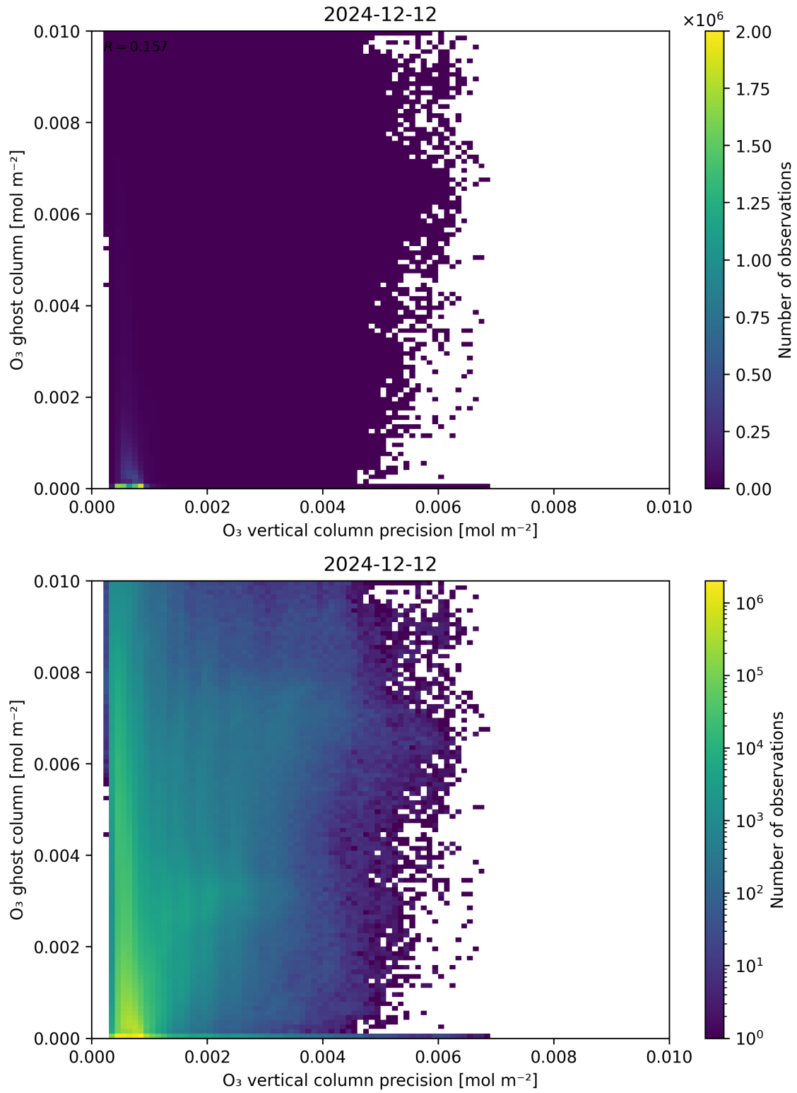
Figure 43: Scatter density plot of “ \text{O}_3 vertical column precision” against “ \text{O}_3 ghost column” for 2024-12-11 to 2024-12-13.
