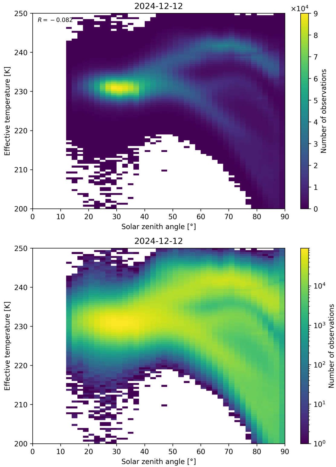
Figure 45: Scatter density plot of “Solar zenith angle” against “Effective temperature” for 2024-12-11 to 2024-12-13.
