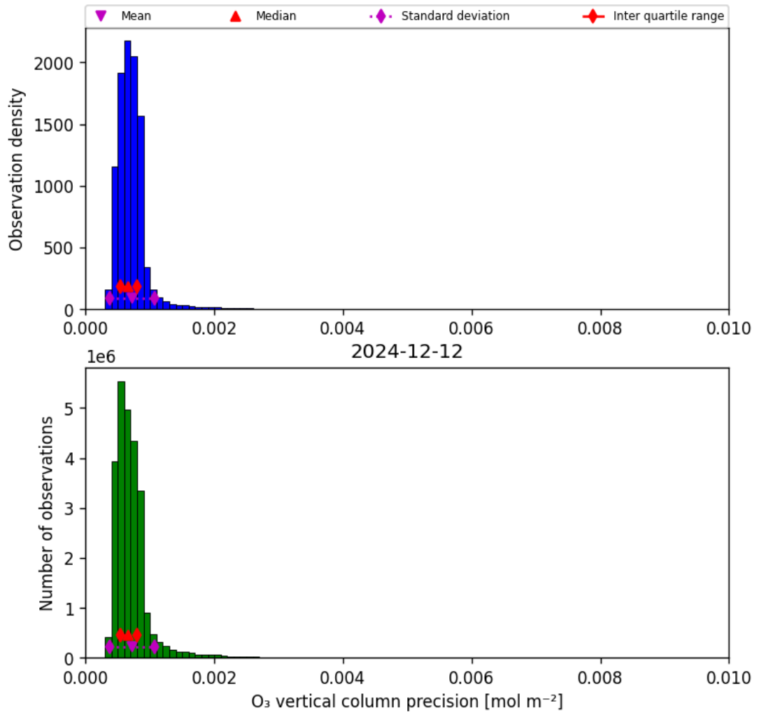
Figure 22: Histogram of “O 3 vertical column precision” for 2024-12-11 to 2024-12-13
