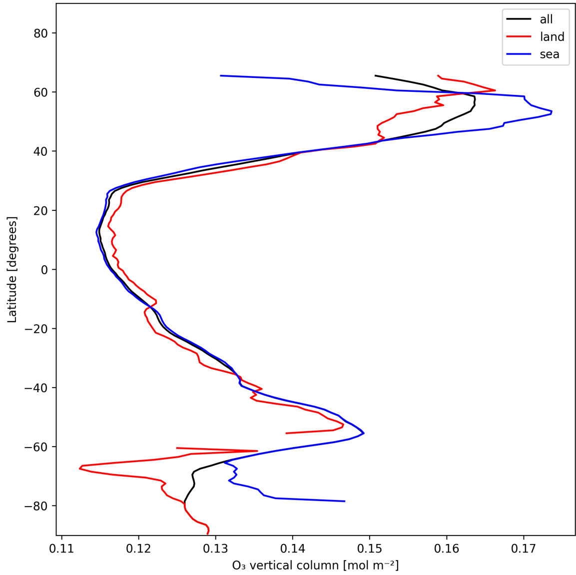
Figure 14: Zonal average of “O 3 vertical column” for 2024-12-11 to 2024-12-13.
