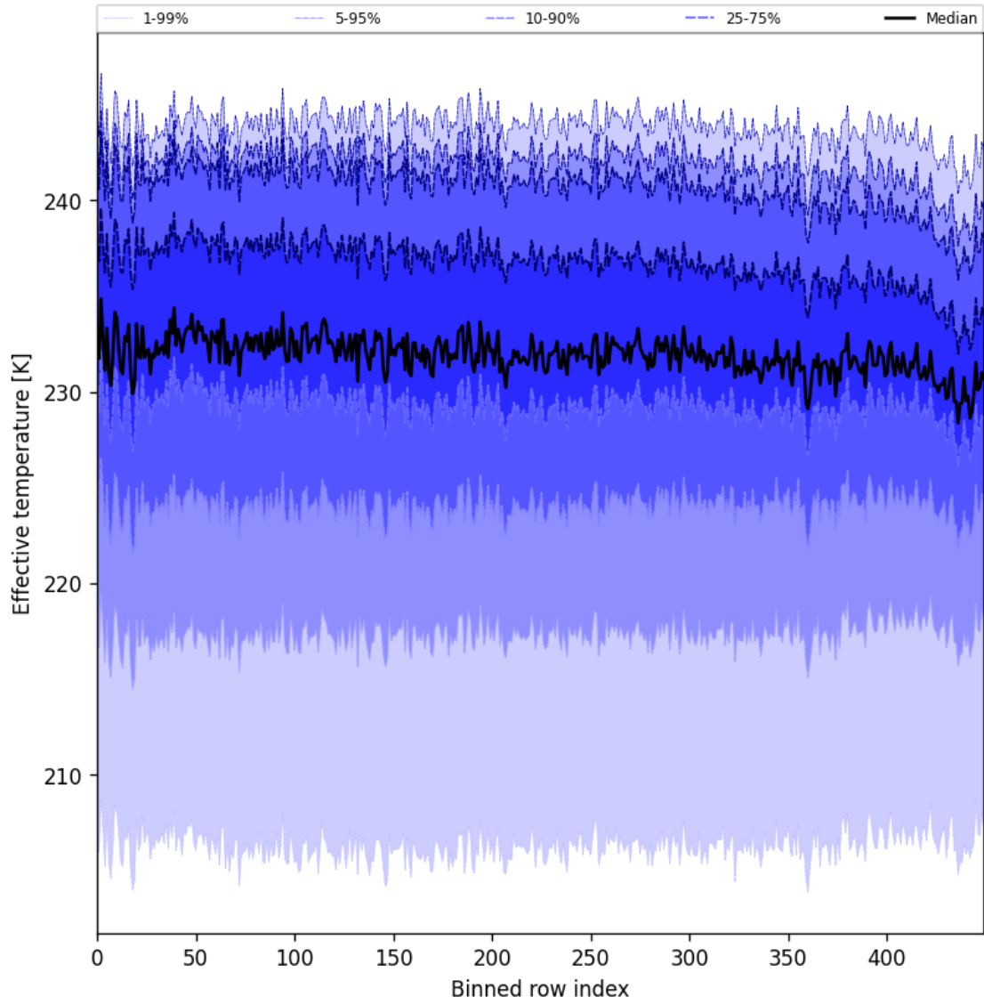
Figure 31: Along track statistics of “Effective temperature” for 2024-12-11 to 2024-12-13
