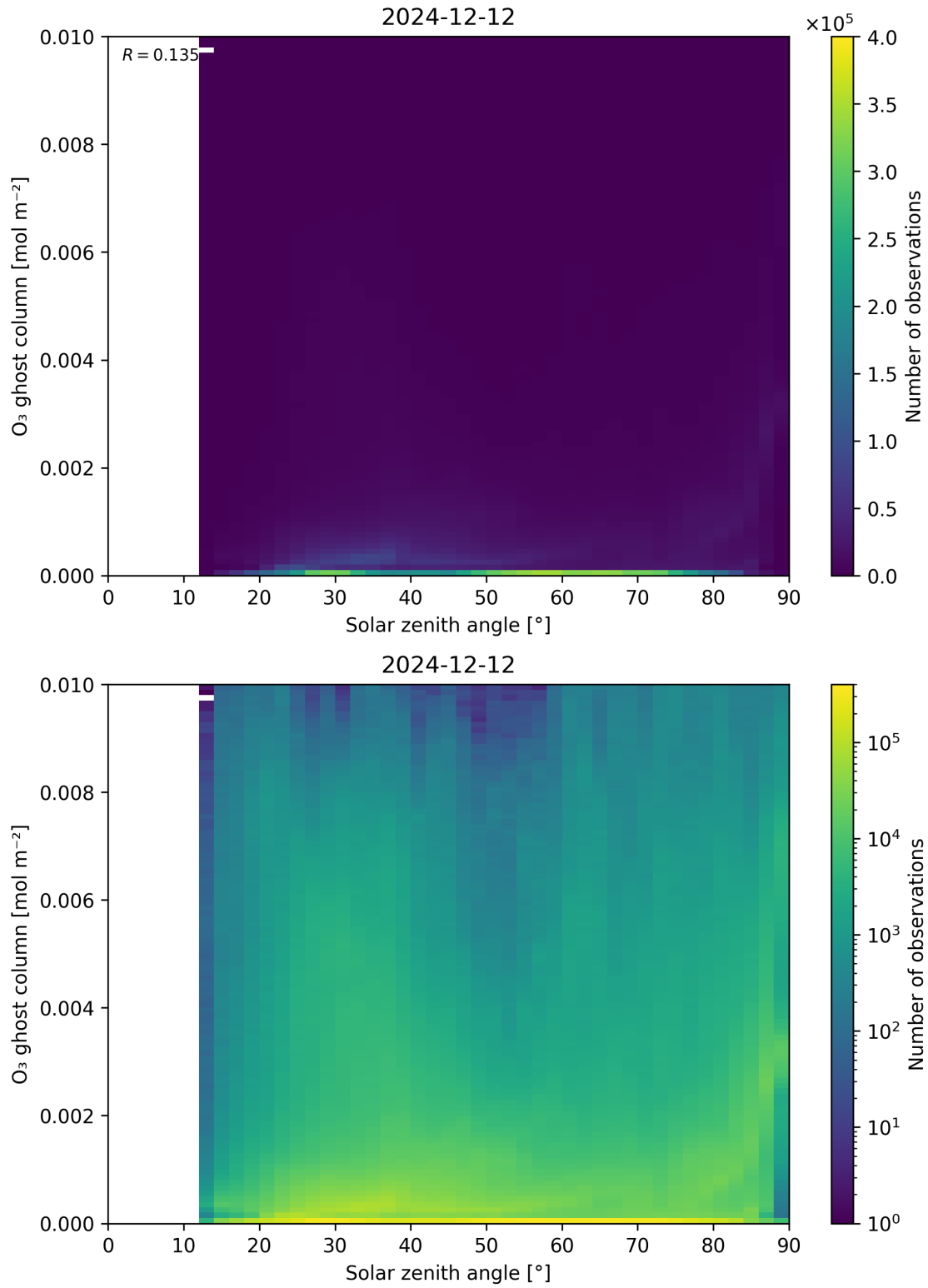
Figure 46: Scatter density plot of “Solar zenith angle” against “O 3 ghost column” for 2024-12-11 to 2024-12-13.
