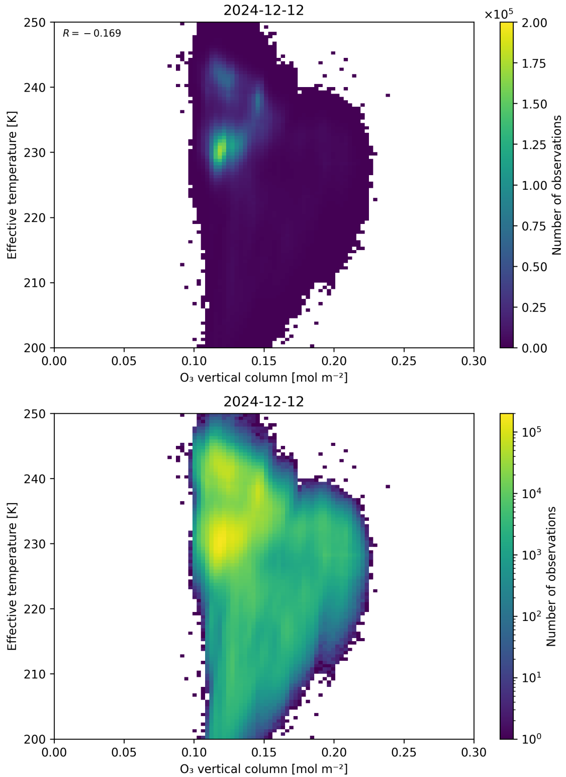
Figure 39: Scatter density plot of “O 3 vertical column” against “Effective temperature” for 2024-12-11 to 2024-12-13.
