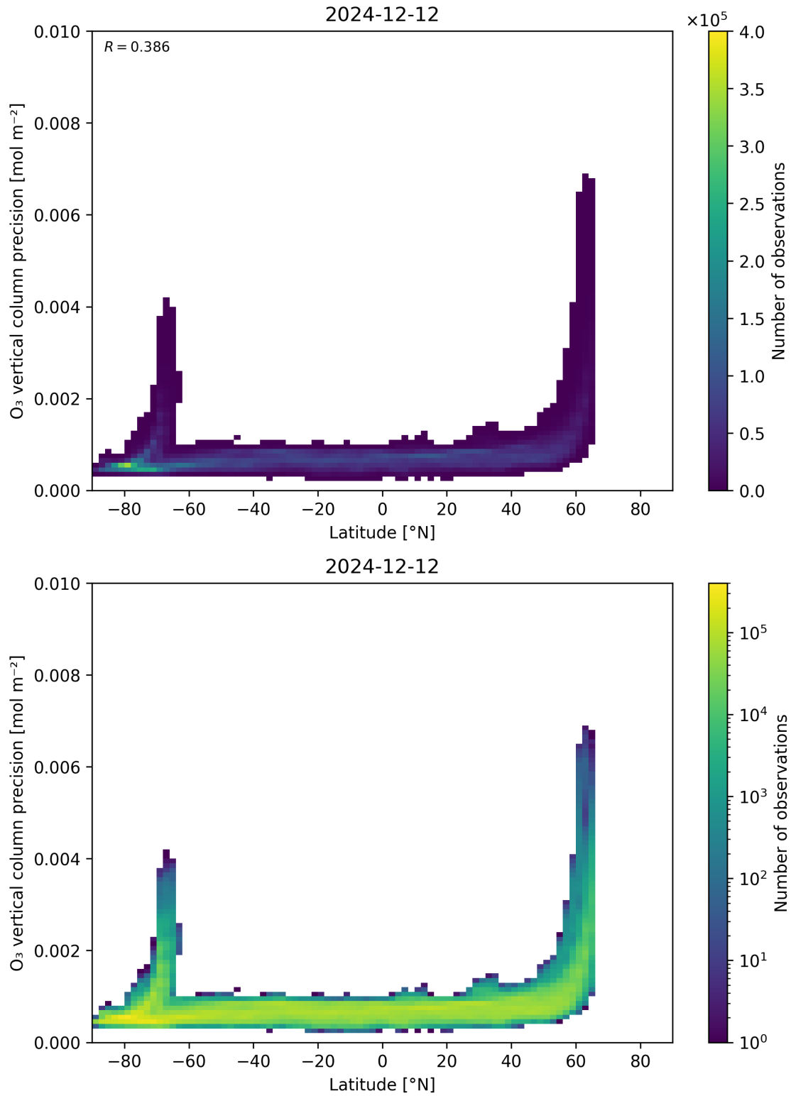
Figure 37: Scatter density plot of “Latitude” against “O 3 vertical column precision” for 2024-12-11 to 2024-12-13.
