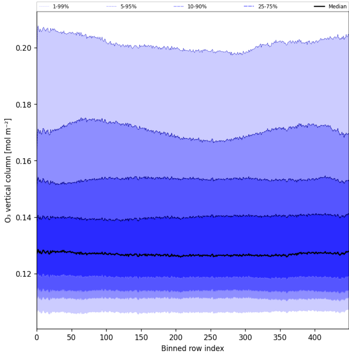
Figure 28: Along track statistics of “O 3 vertical column” for 2024-12-11 to 2024-12-13
