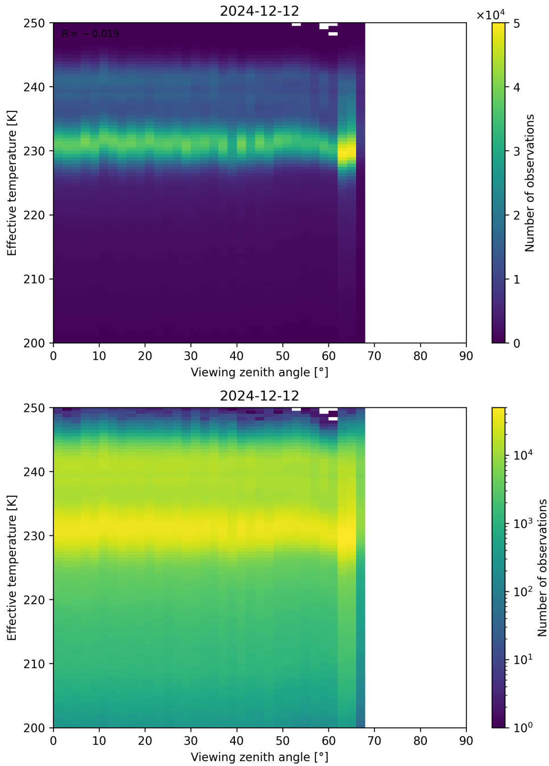
Figure 50: Scatter density plot of “Viewing zenith angle” against “Effective temperature” for 2024-12-11 to 2024-12-13.
