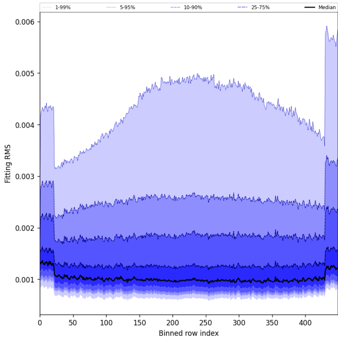
Figure 30: Along track statistics of “Fitting RMS” for 2024-12-11 to 2024-12-13
