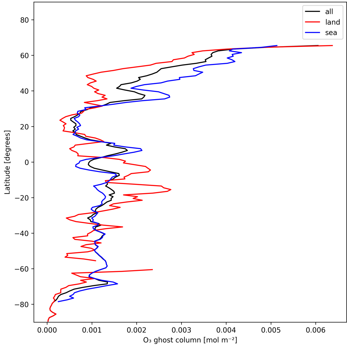
Figure 18: Zonal average of "O 3 ghost column" for 2024-12-11 to 2024-12-13.
