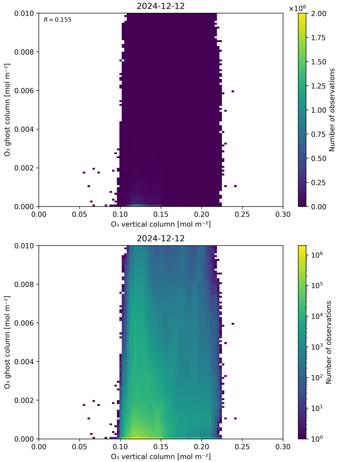
Figure 40: Scatter density plot of “O 3 vertical column” against “O 3 ghost column” for 2024-12-11 to 2024-12-13.
