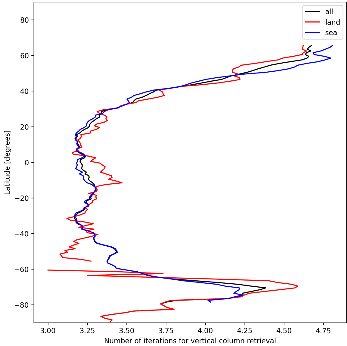
Figure 19: Zonal average of “Number of iterations for vertical column retrieval” for 2024-12-11 to 2024-12-13.
