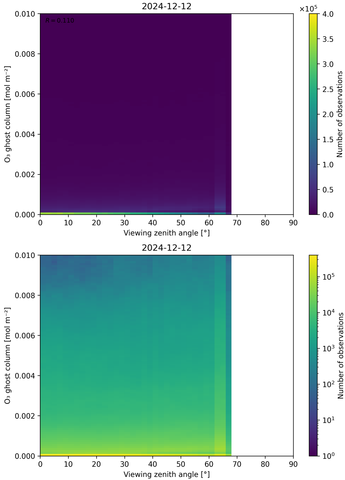
Figure 51: Scatter density plot of “Viewing zenith angle” against “O 3 ghost column” for 2024-12-11 to 2024-12-13.
