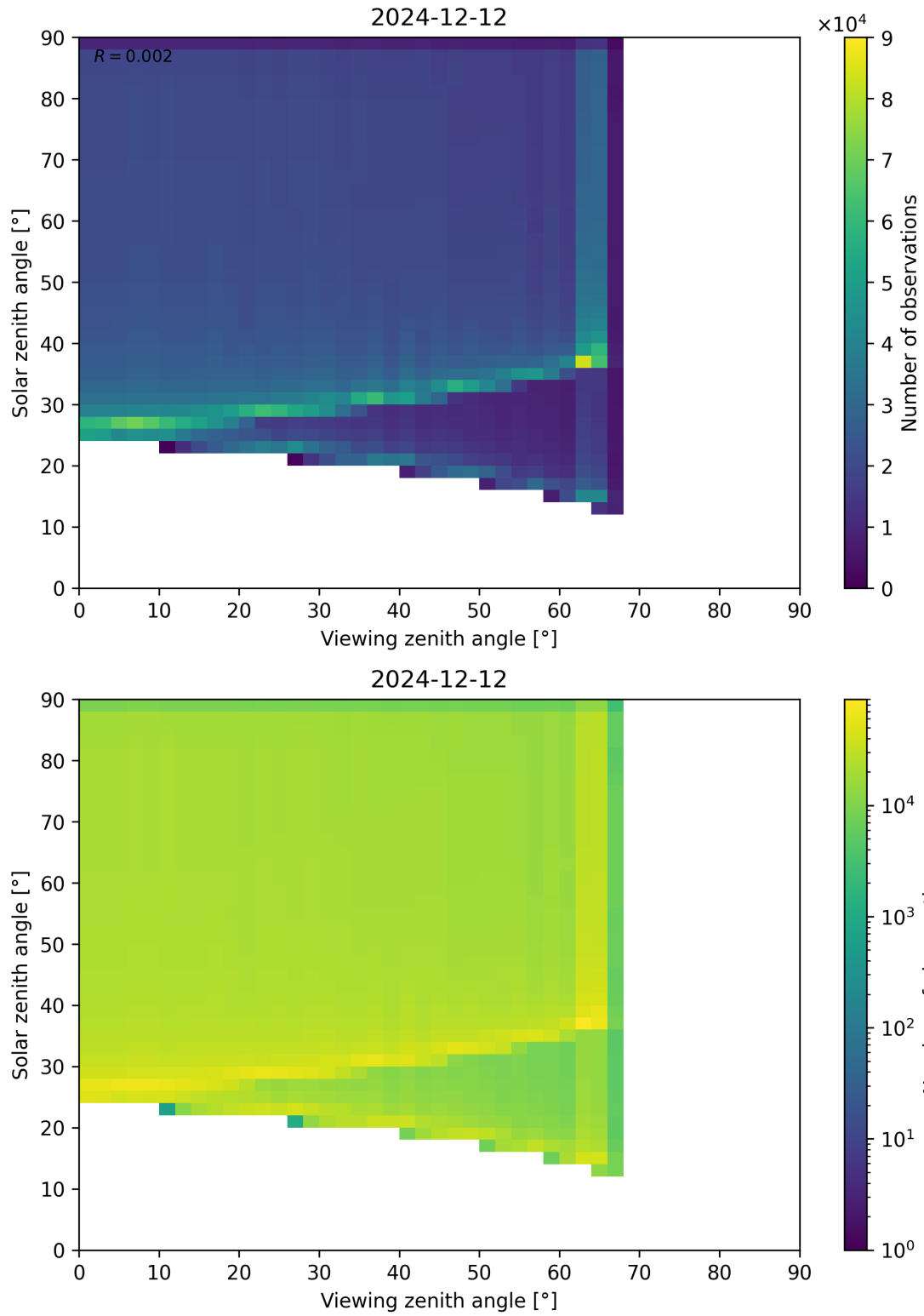
Figure 54: Scatter density plot of “Viewing zenith angle” against “Solar zenith angle” for 2024-12-11 to 2024-12-13.
