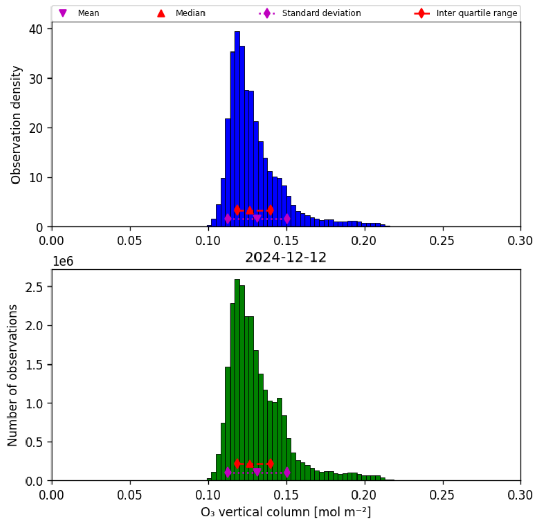
Figure 21: Histogram of “O 3 vertical column” for 2024-12-11 to 2024-12-13
