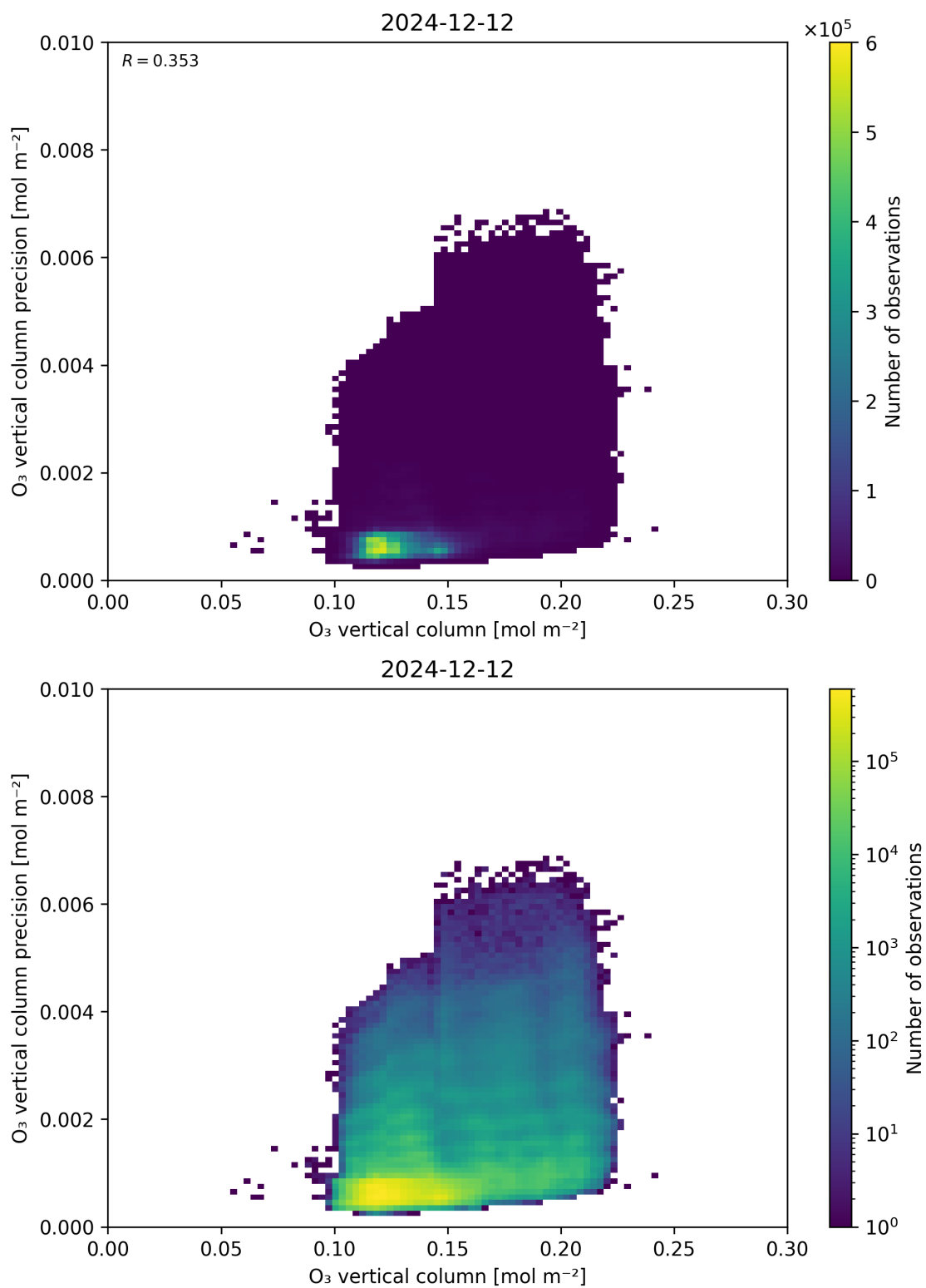
Figure 41: Scatter density plot of “O 3 vertical column” against “O 3 vertical column precision” for 2024-12-11 to 2024-12-13.
