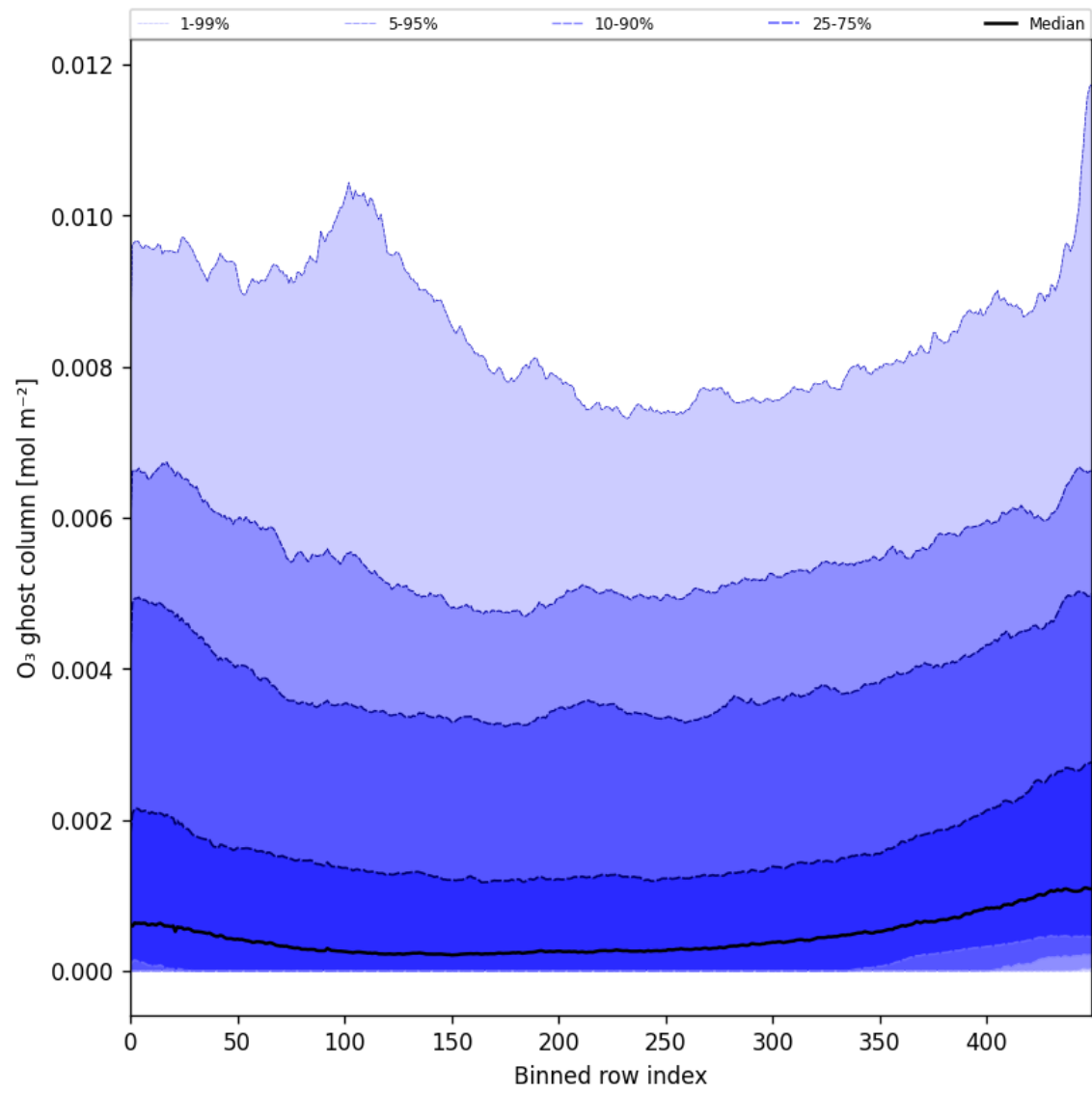
Figure 32: Along track statistics of "O 3 ghost column" for 2024-12-11 to 2024-12-13
