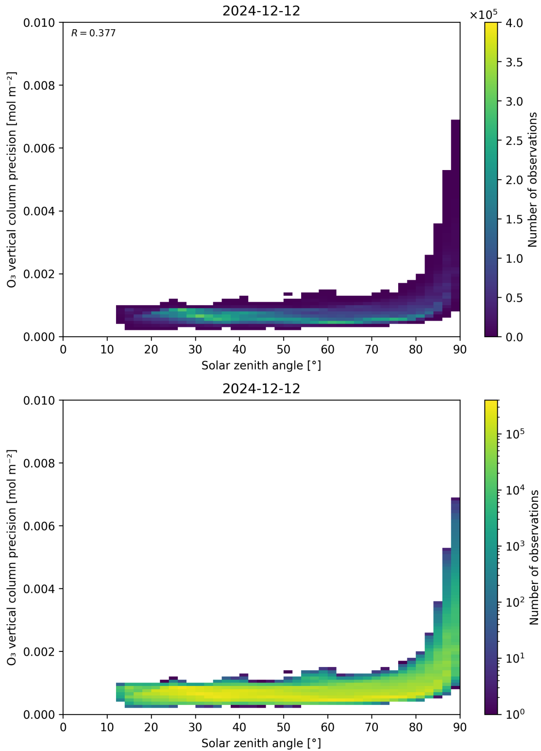
Figure 48: Scatter density plot of “Solar zenith angle” against “O 3 vertical column precision” for 2024-12-11 to 2024-12-13.
