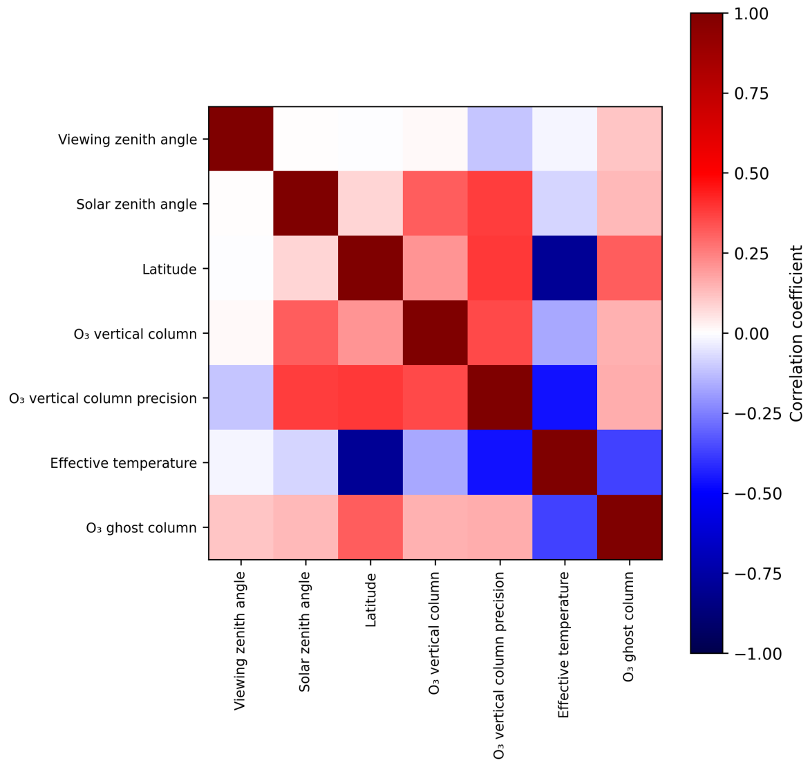
Figure 2: Map of correlation matrix for 2024-12-11 to 2024-12-13.
