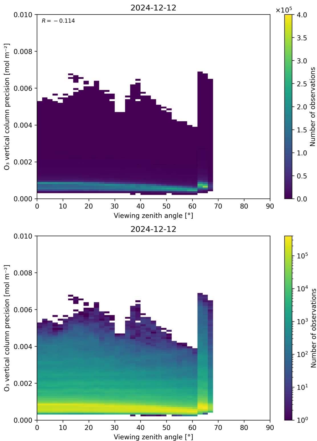
Figure 53: Scatter density plot of “Viewing zenith angle” against “O 3 vertical column precision” for 2024-12-11 to 2024-12-13.
