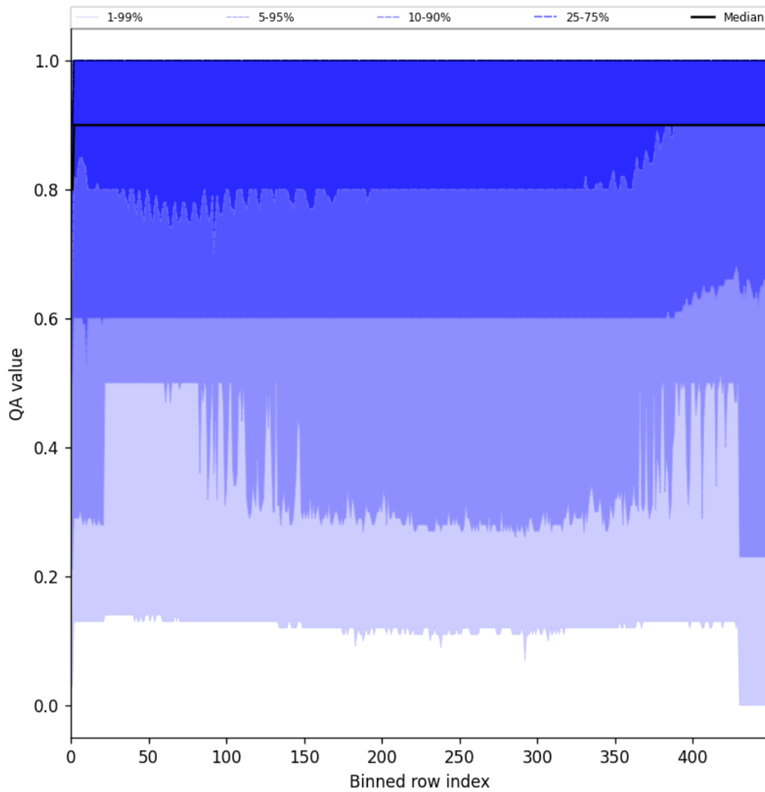
Figure 27: Along track statistics of “QA value” for 2024-12-13 to 2024-12-15
