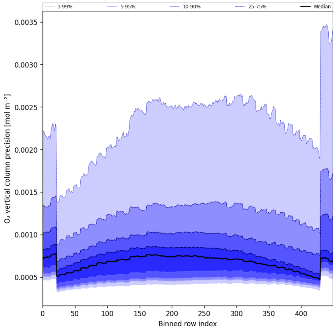
Figure 29: Along track statistics of “O 3 vertical column precision” for 2024-12-13 to 2024-12-15
