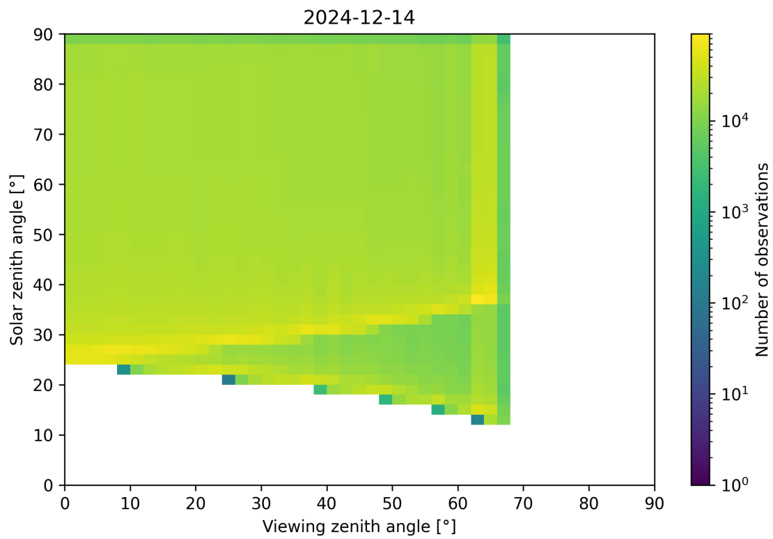
Figure 54: Scatter density plot of “Viewing zenith angle” against “Solar zenith angle” for 2024-12-13 to 2024-12-15.
