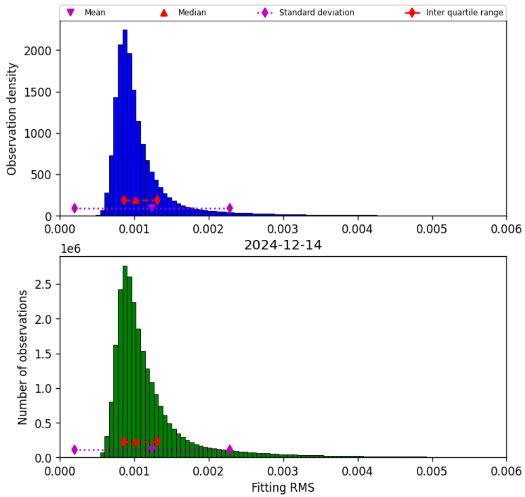
Figure 23: Histogram of “Fitting RMS” for 2024-12-13 to 2024-12-15
