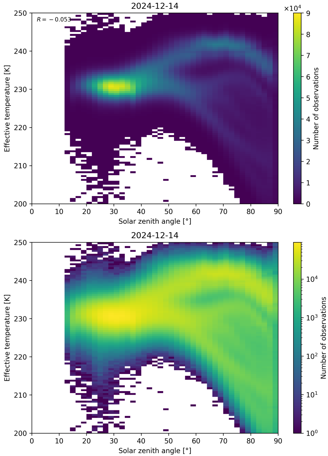
Figure 45: Scatter density plot of “Solar zenith angle” against “Effective temperature” for 2024-12-13 to 2024-12-15.
