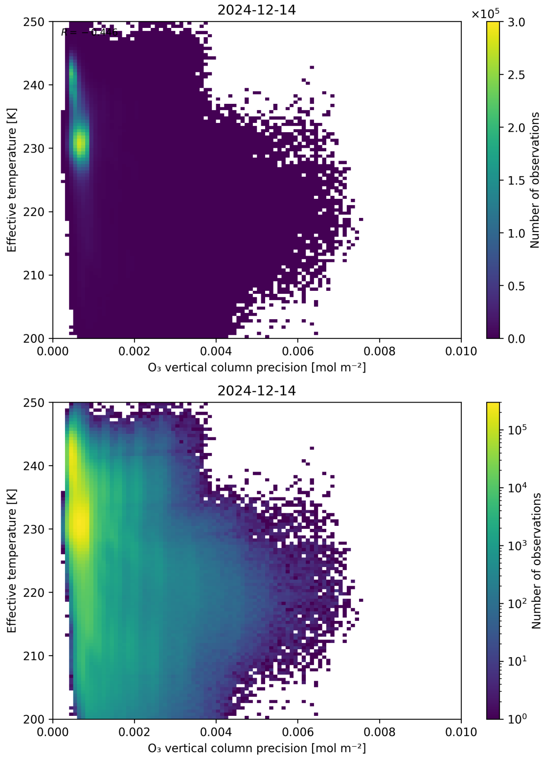
Figure 42: Scatter density plot of “O 3 vertical column precision” against “Effective temperature” for 2024-12-13 to 2024-12-15.
