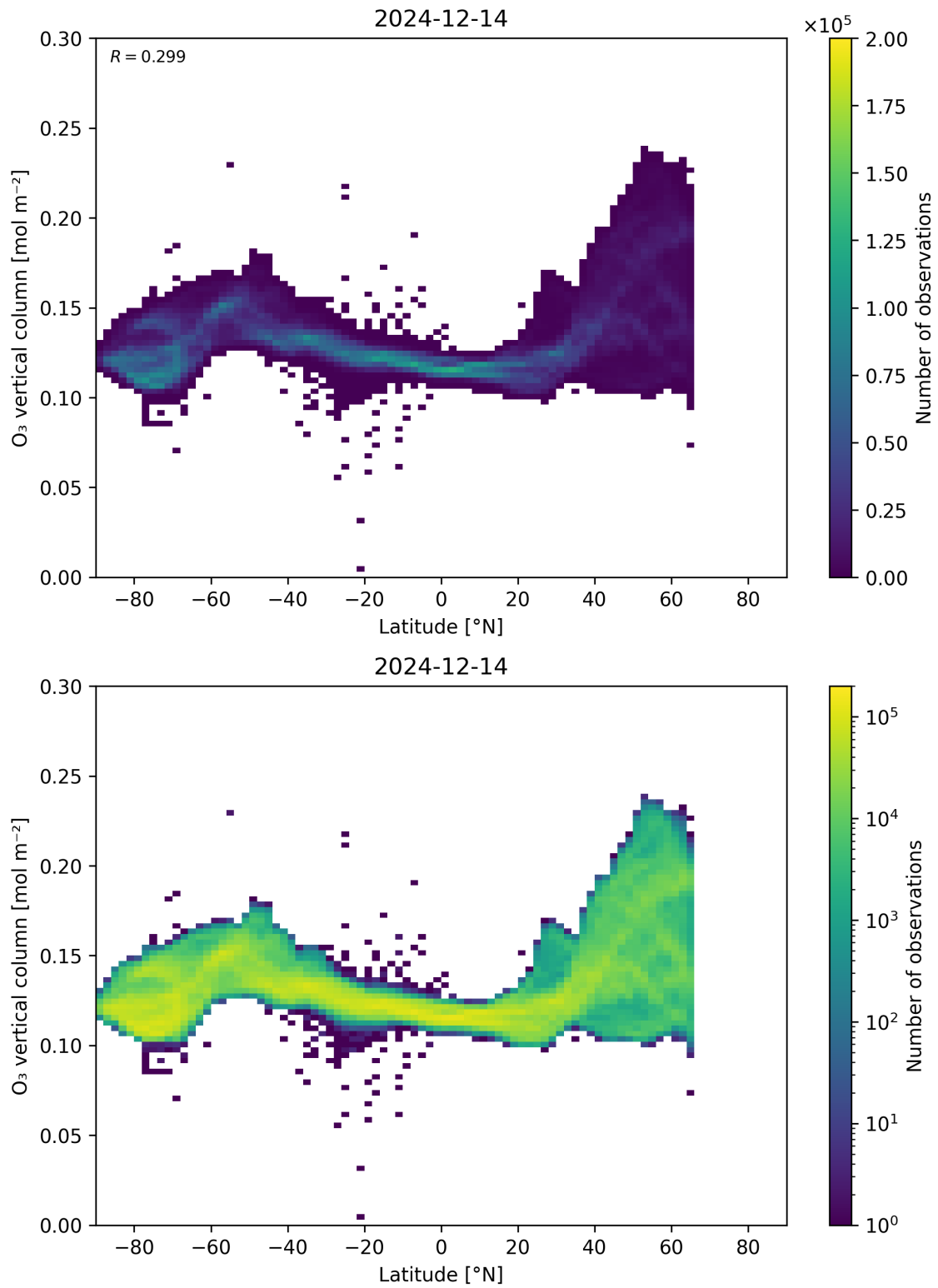
Figure 36: Scatter density plot of “Latitude” against “O 3 vertical column” for 2024-12-13 to 2024-12-15.
