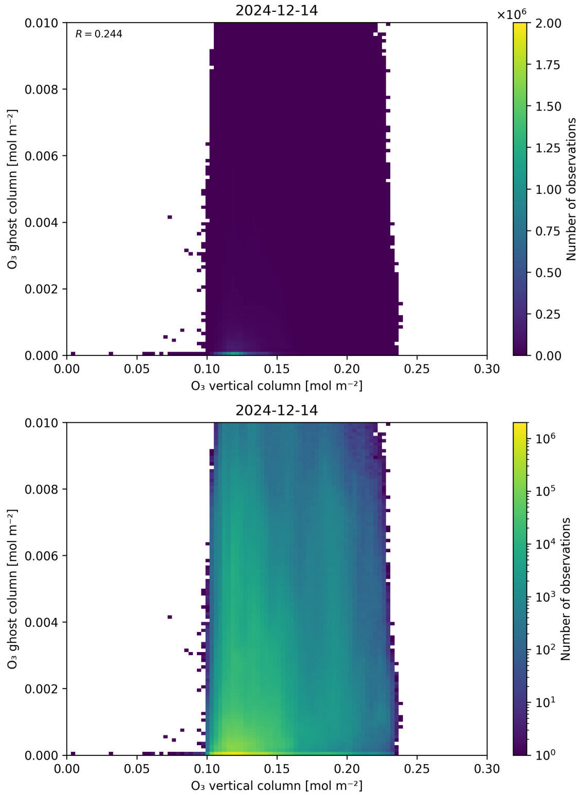
Figure 40: Scatter density plot of “O 3 vertical column” against “O 3 ghost column” for 2024-12-13 to 2024-12-15.
