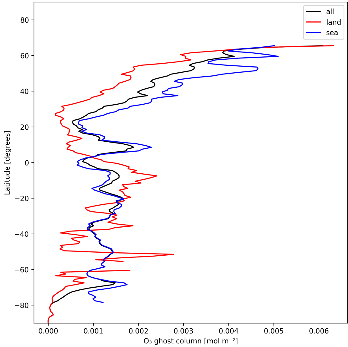
Figure 18: Zonal average of "O 3 ghost column" for 2024-12-13 to 2024-12-15.
