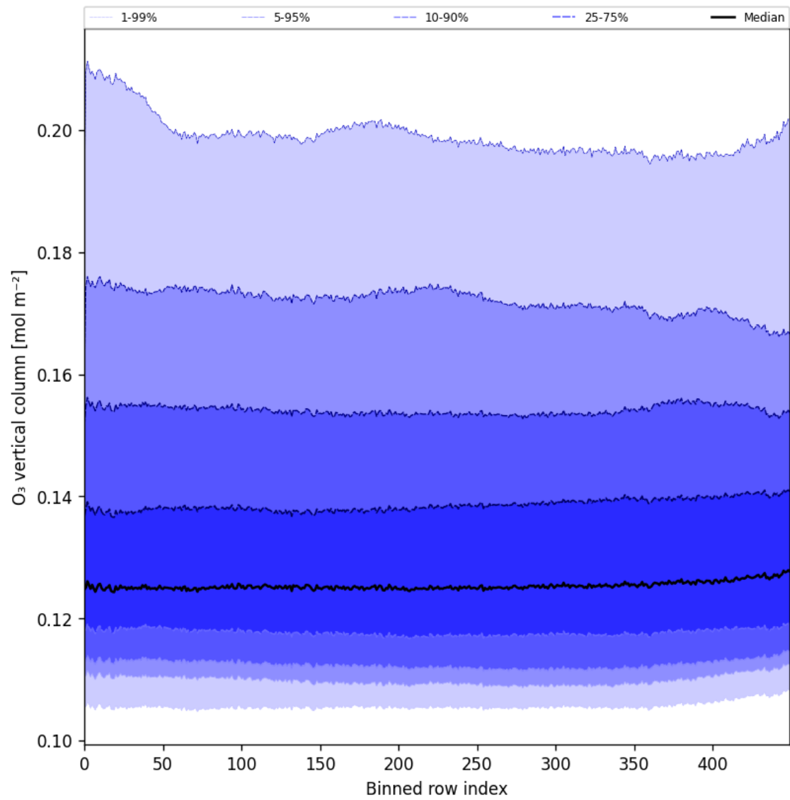
Figure 28: Along track statistics of “O 3 vertical column” for 2024-12-13 to 2024-12-15
