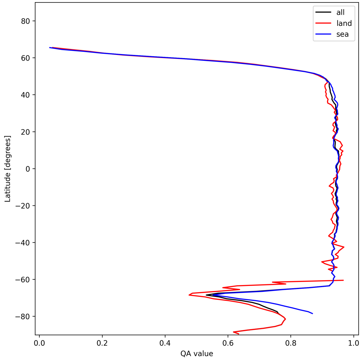
Figure 13: Zonal average of “QA value” for 2024-12-13 to 2024-12-15.
