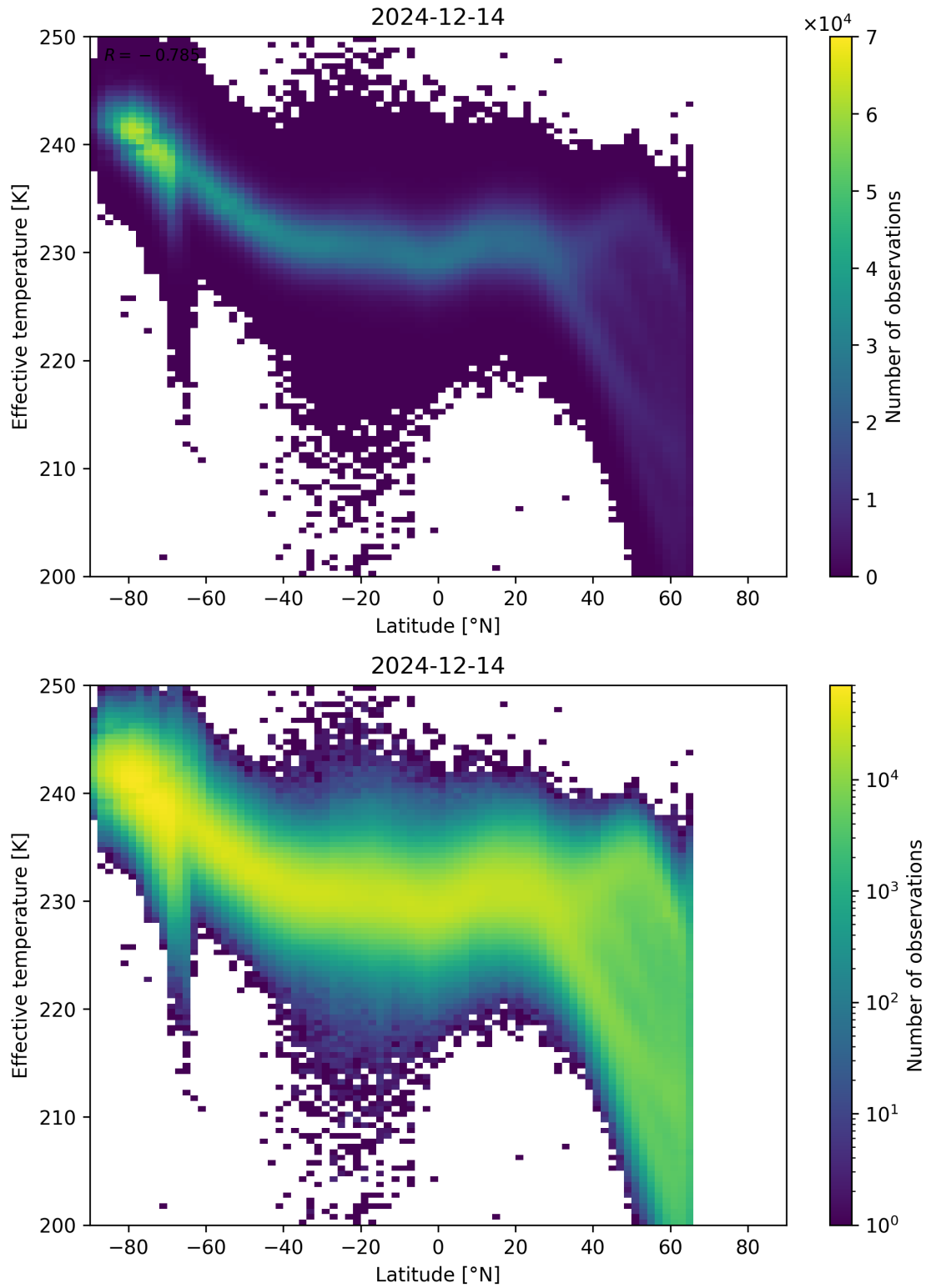
Figure 34: Scatter density plot of “Latitude” against “Effective temperature” for 2024-12-13 to 2024-12-15.
