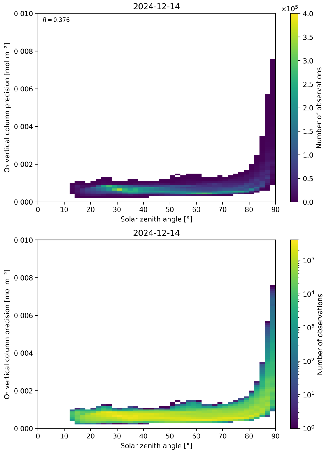
Figure 48: Scatter density plot of “Solar zenith angle” against “O 3 vertical column precision” for 2024-12-13 to 2024-12-15.
