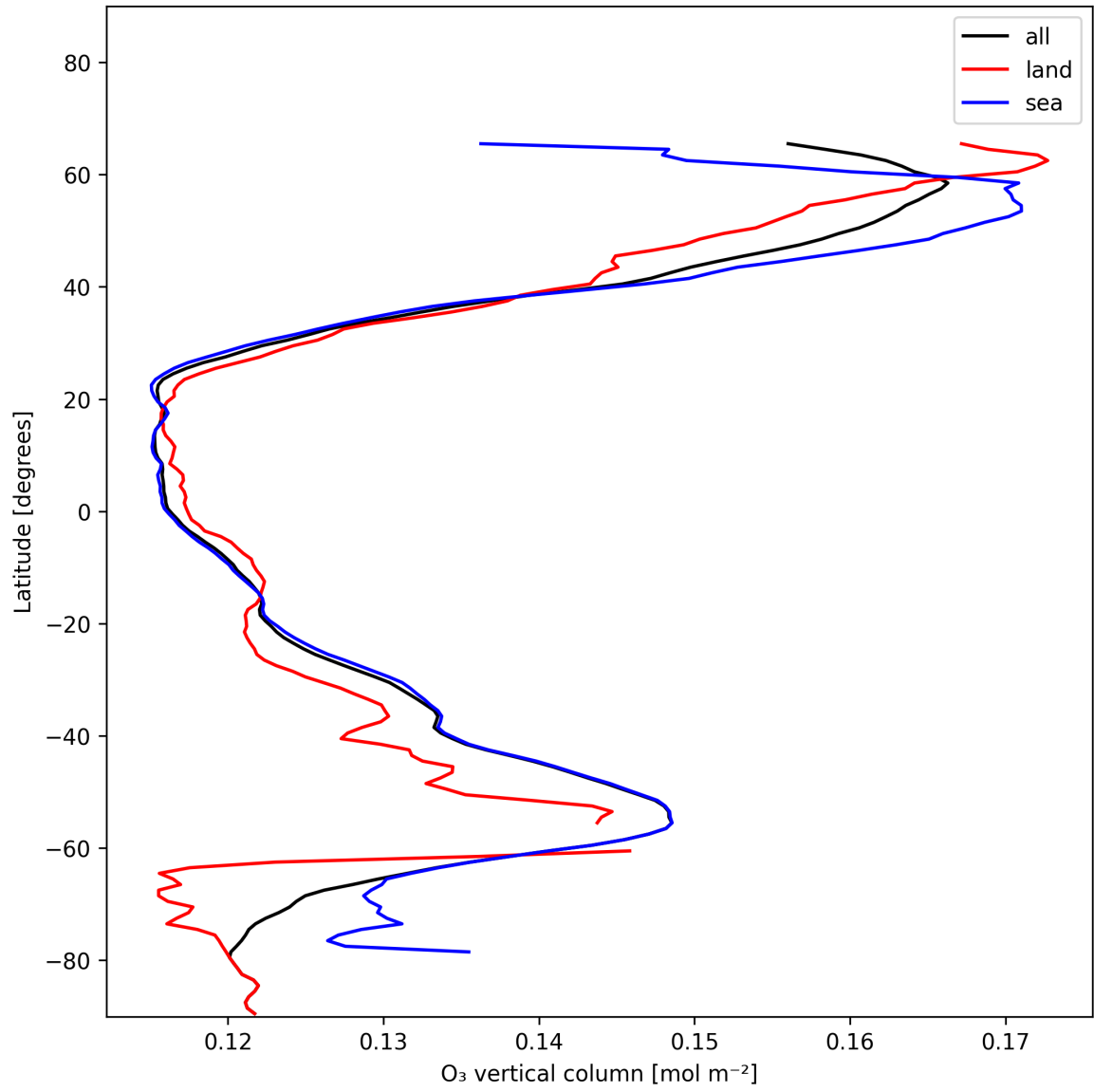
Figure 14: Zonal average of “O 3 vertical column” for 2024-12-13 to 2024-12-15.
