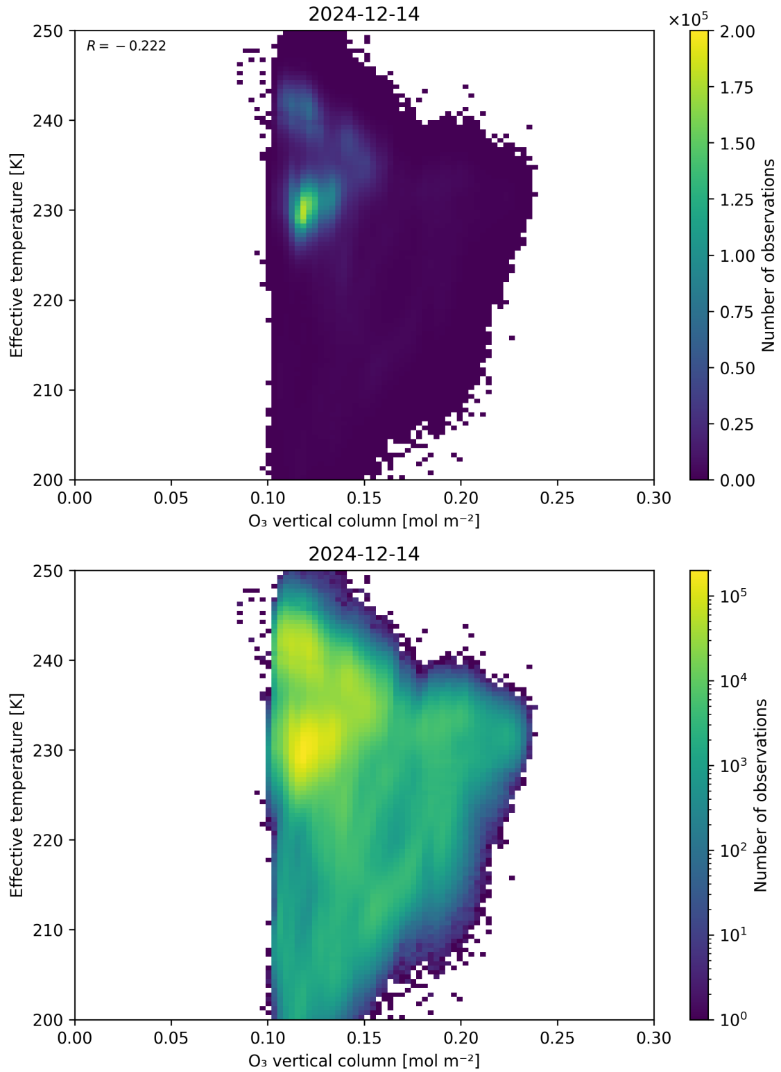
Figure 39: Scatter density plot of “O 3 vertical column” against “Effective temperature” for 2024-12-13 to 2024-12-15.
