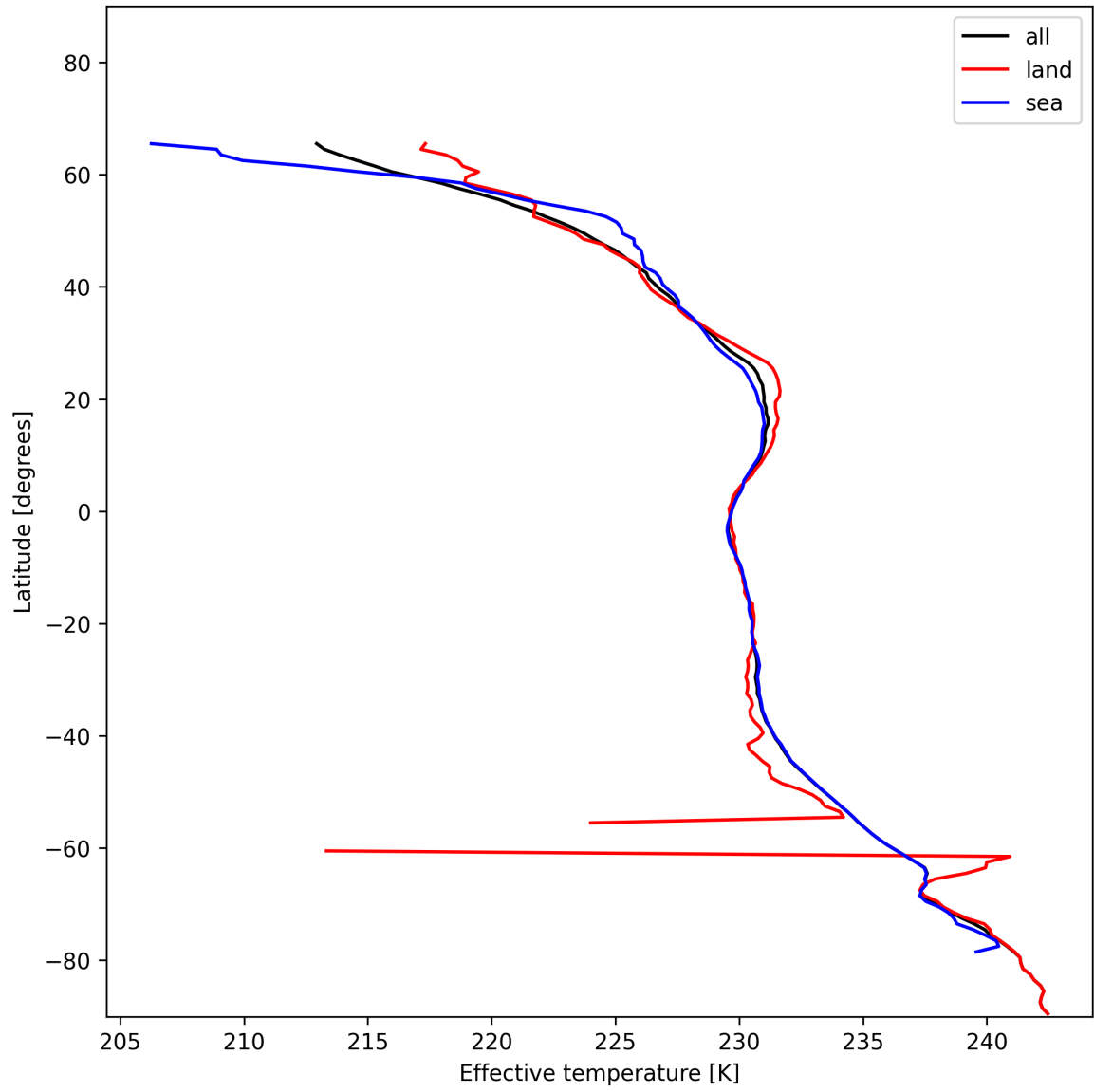
Figure 17: Zonal average of “Effective temperature” for 2024-12-13 to 2024-12-15.
