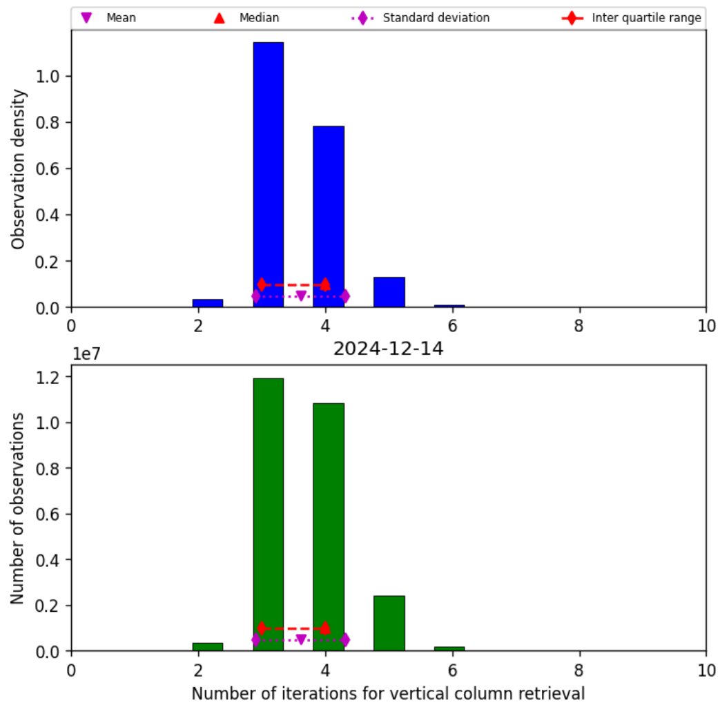
Figure 26: Histogram of “Number of iterations for vertical column retrieval” for 2024-12-13 to 2024-12-15
