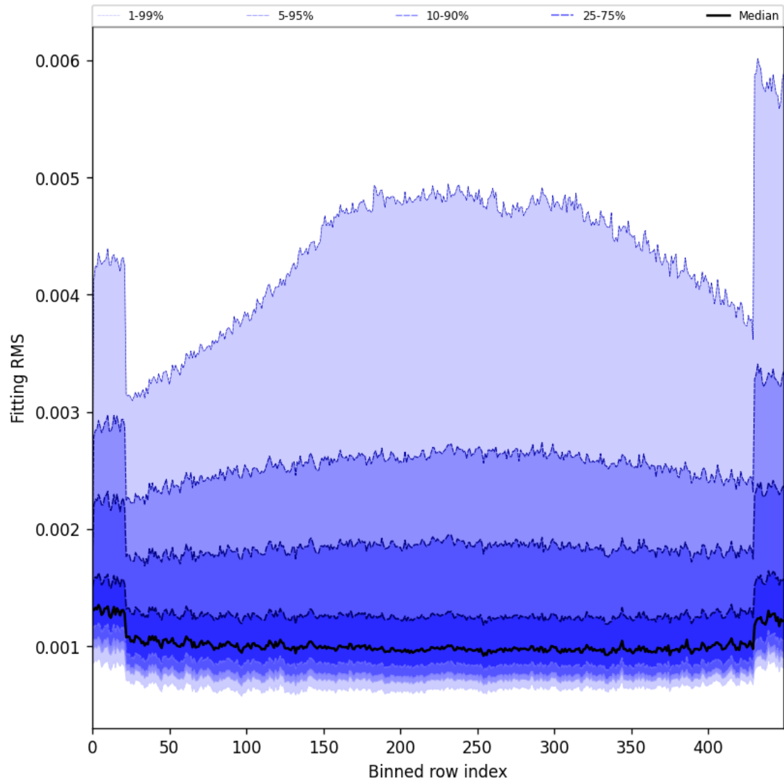
Figure 30: Along track statistics of “Fitting RMS” for 2024-12-13 to 2024-12-15
