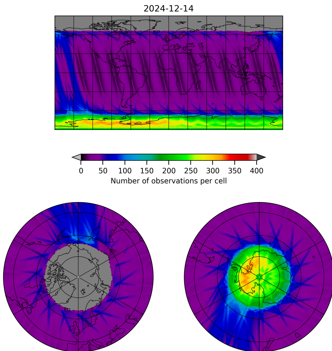
Figure 12: Map of the number of observations for 2024-12-13 to 2024-12-15
