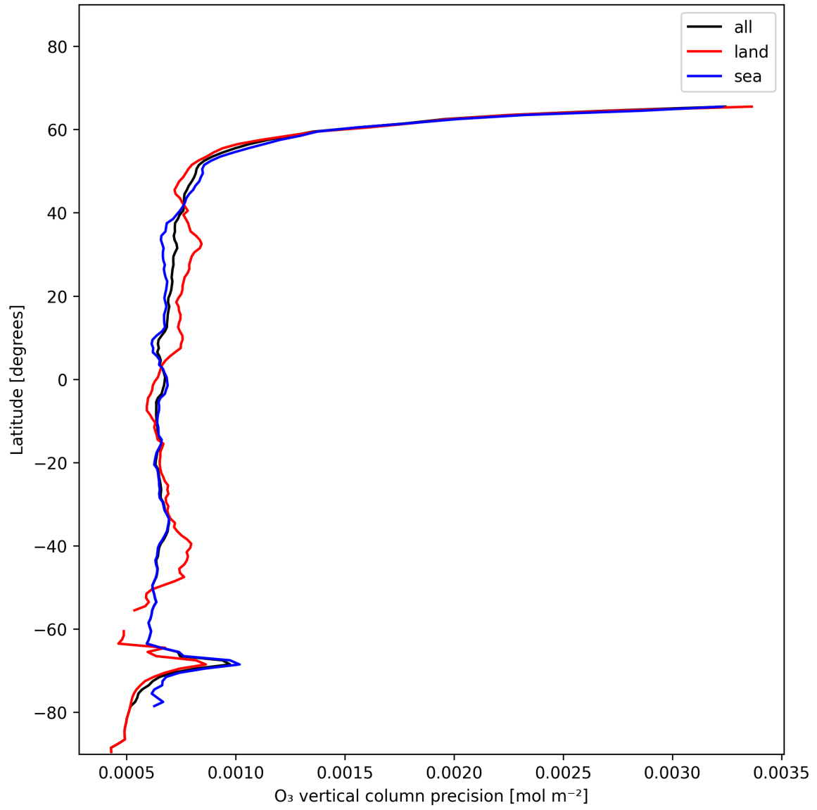
Figure 15: Zonal average of “O 3 vertical column precision” for 2024-12-13 to 2024-12-15.
