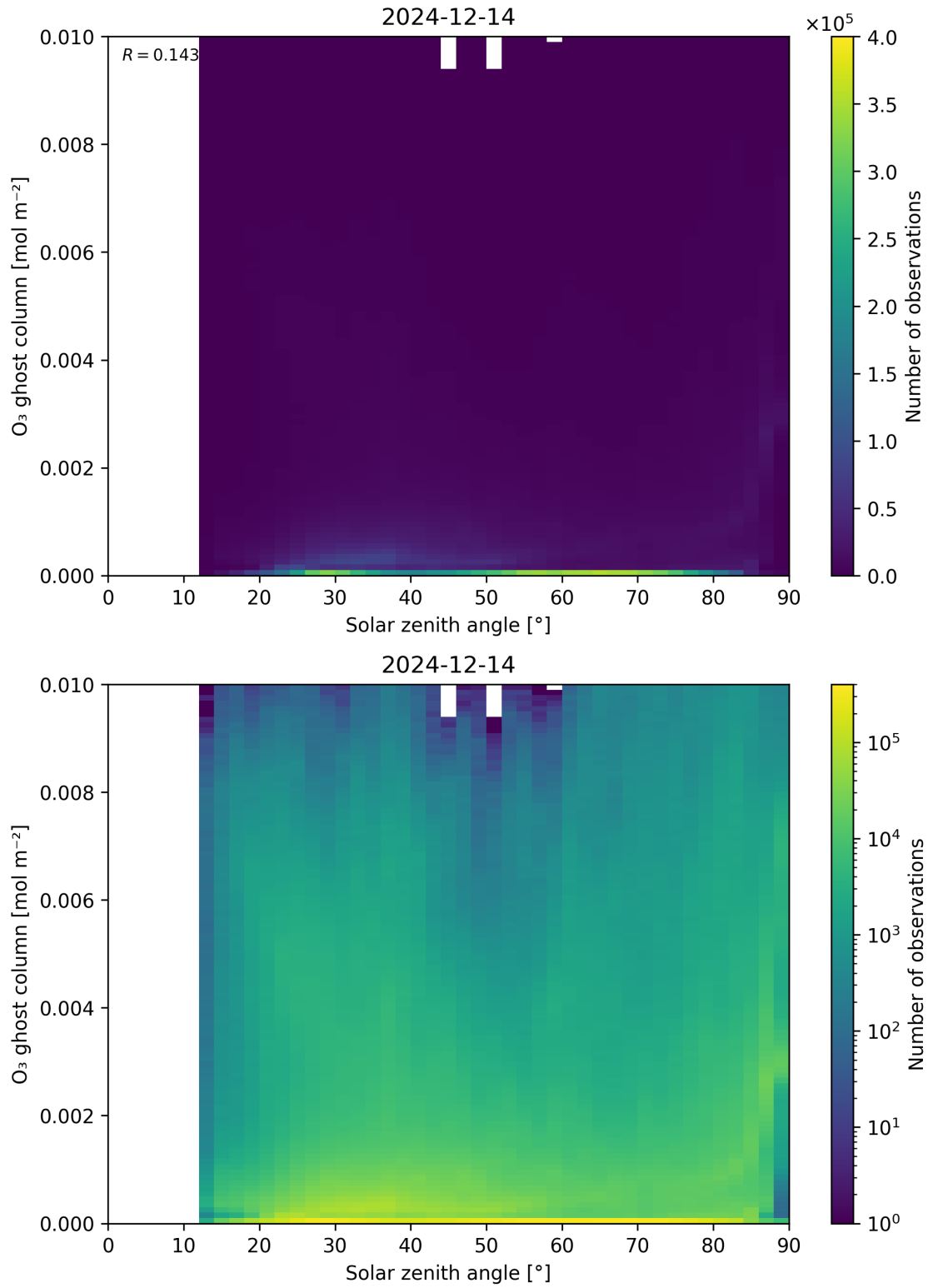
Figure 46: Scatter density plot of “Solar zenith angle” against “O 3 ghost column” for 2024-12-13 to 2024-12-15.
