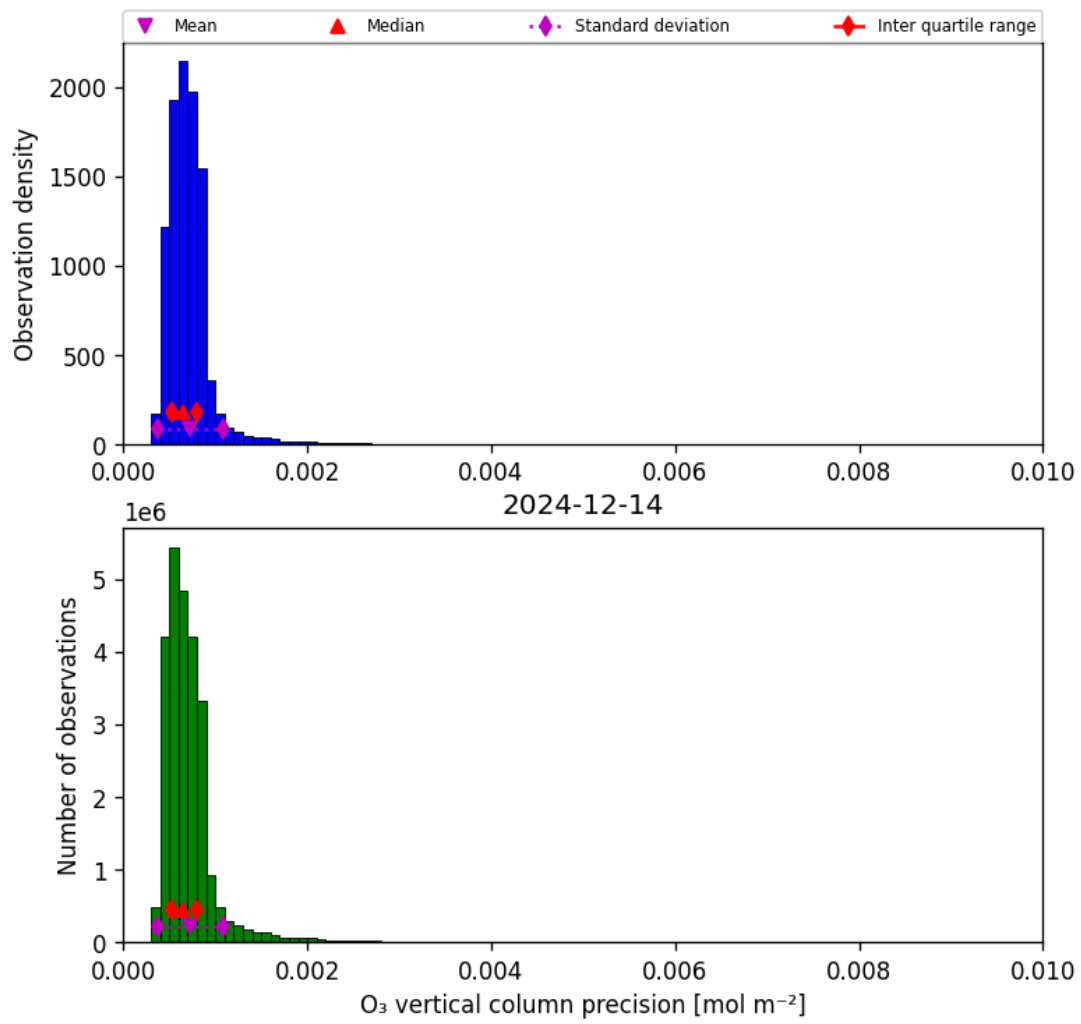
Figure 22: Histogram of “O 3 vertical column precision” for 2024-12-13 to 2024-12-15
