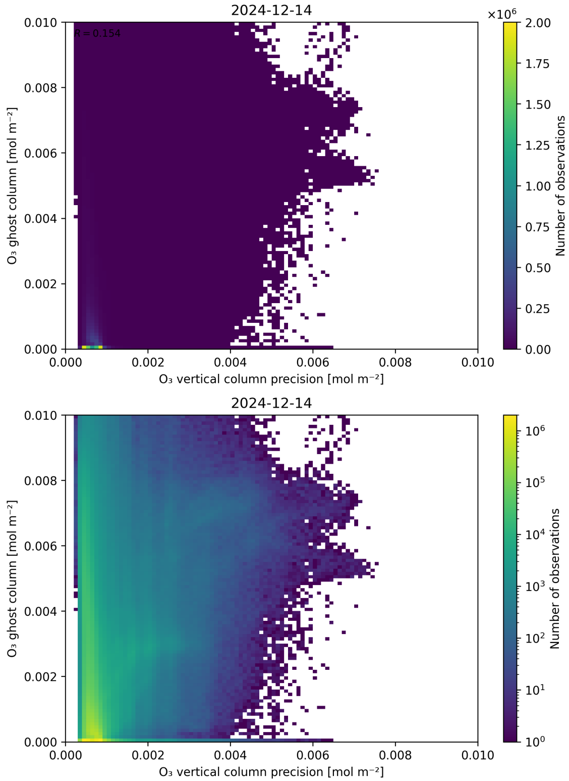
Figure 43: Scatter density plot of “ \text{O}_3 vertical column precision” against “ \text{O}_3 ghost column” for 2024-12-13 to 2024-12-15.
