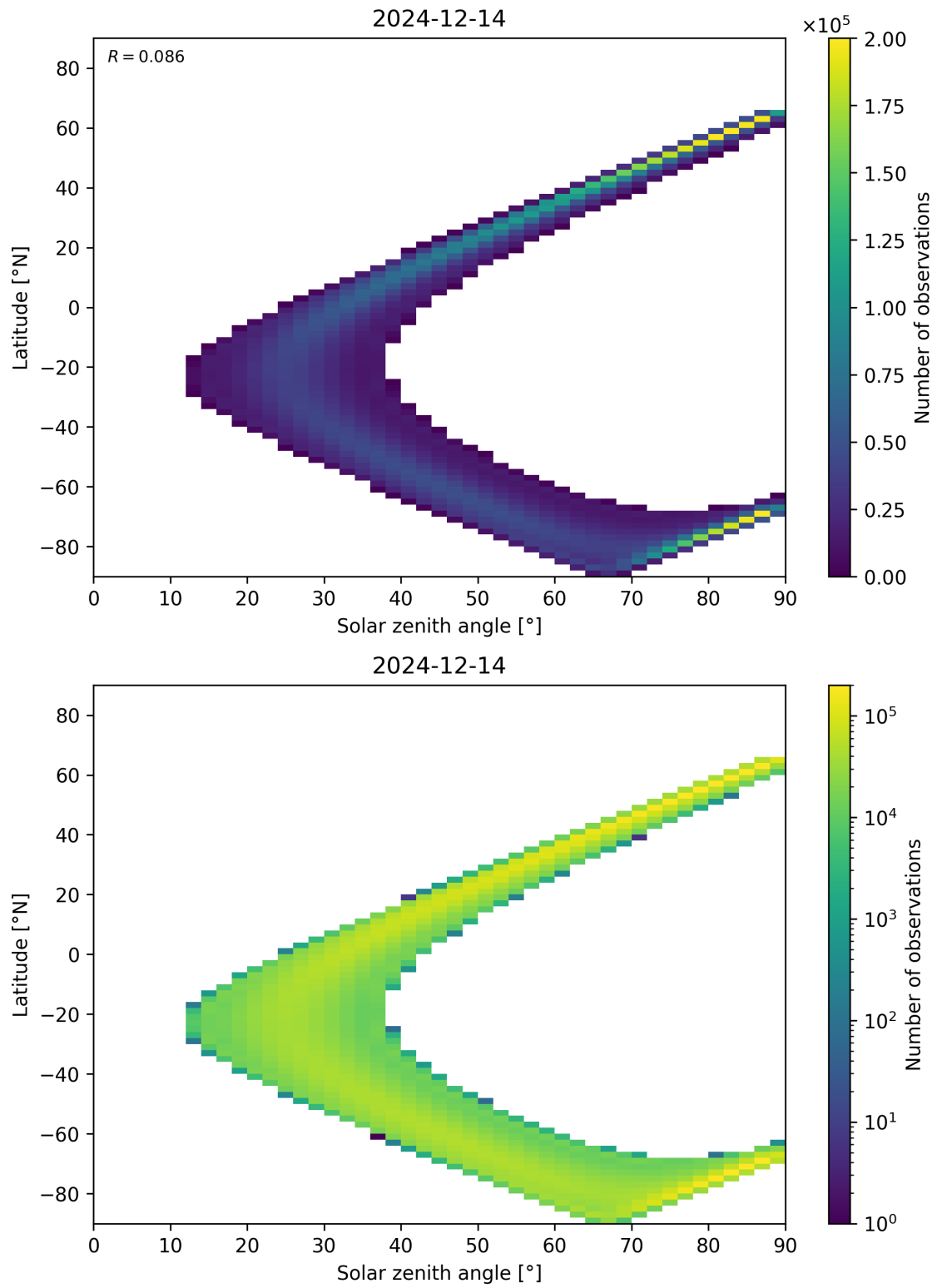
Figure 44: Scatter density plot of “Solar zenith angle” against “Latitude” for 2024-12-13 to 2024-12-15.
