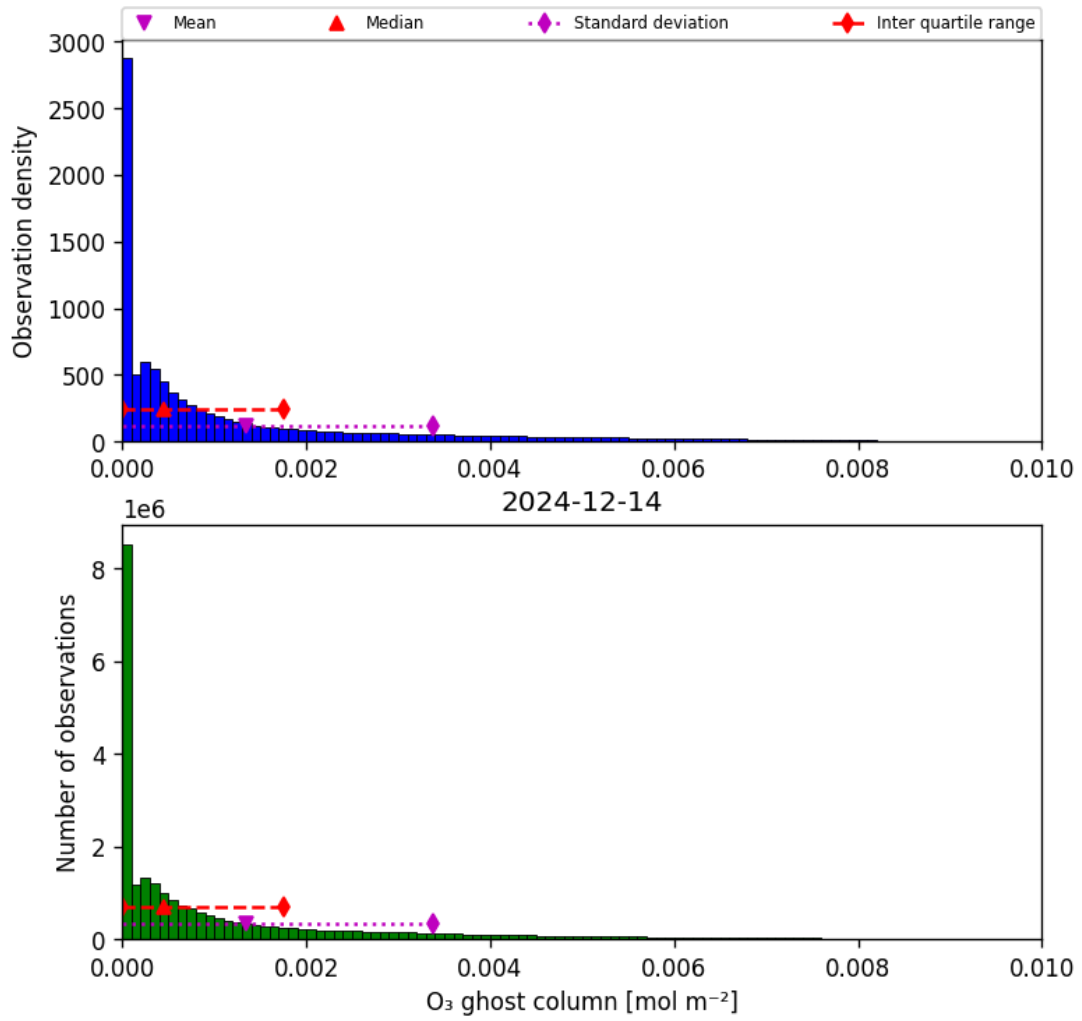
Figure 25: Histogram of “O 3 ghost column” for 2024-12-13 to 2024-12-15
