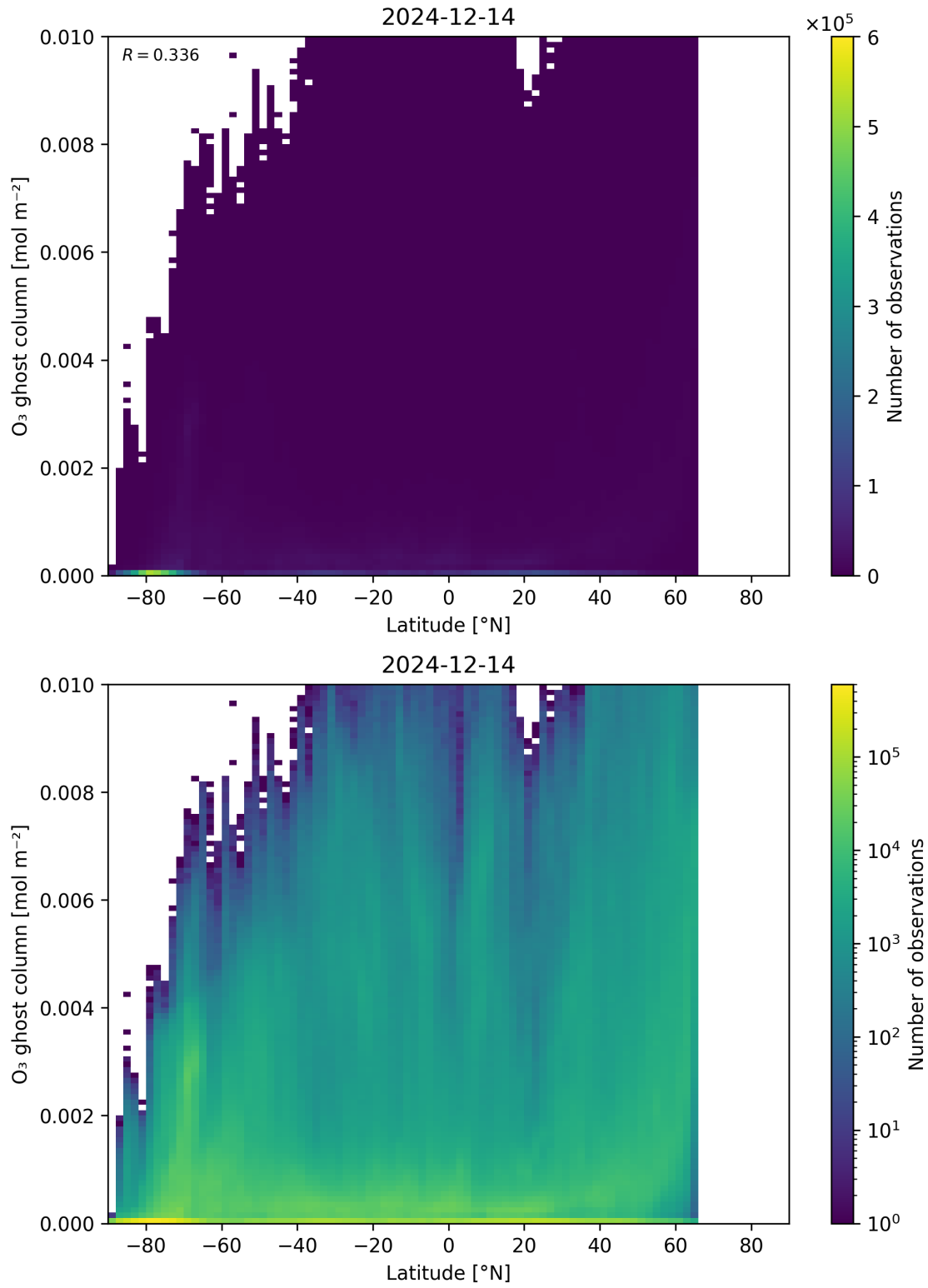
Figure 35: Scatter density plot of “Latitude” against “O 3 ghost column” for 2024-12-13 to 2024-12-15.
