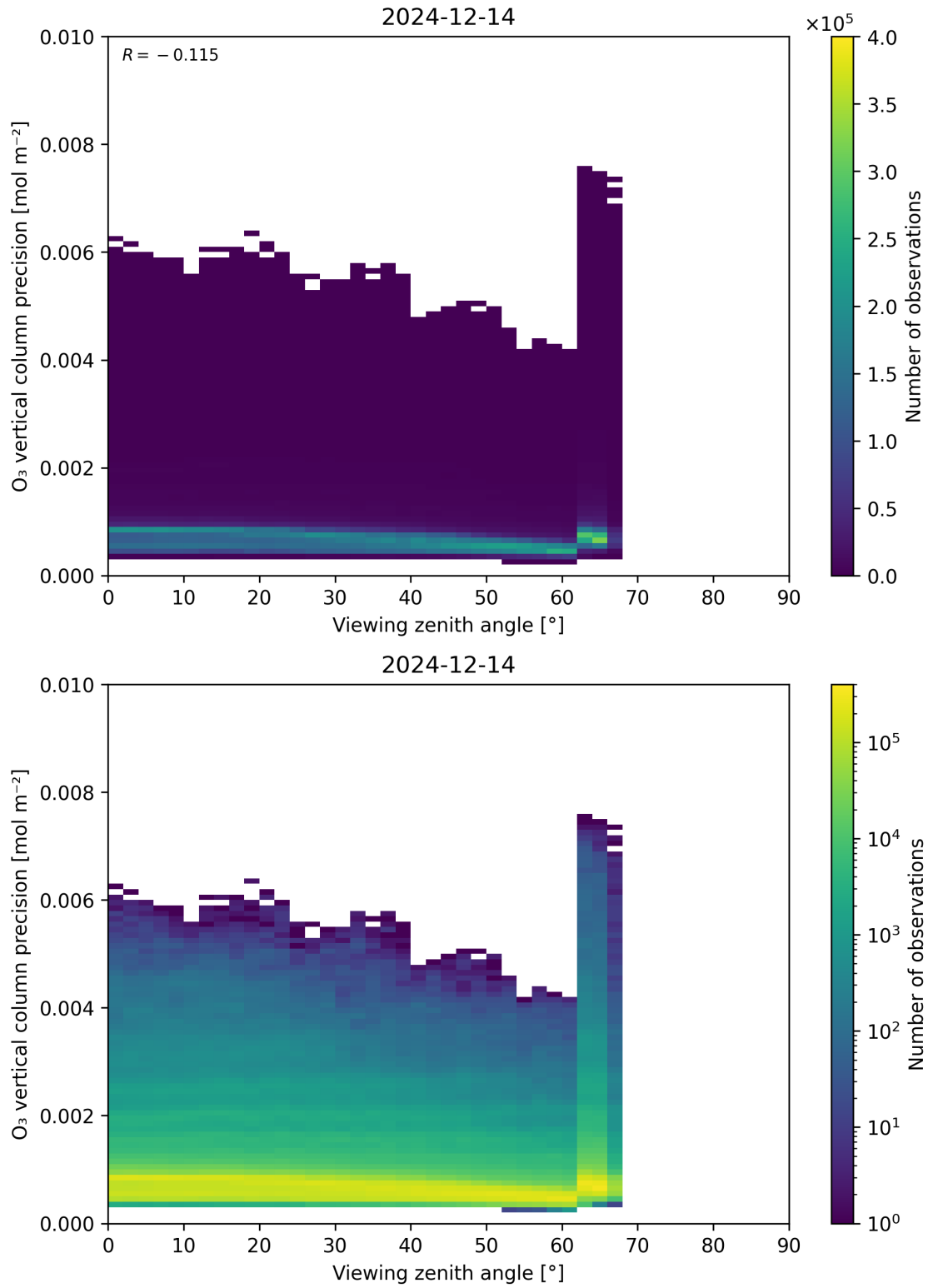
Figure 53: Scatter density plot of “Viewing zenith angle” against “O 3 vertical column precision” for 2024-12-13 to 2024-12-15.
