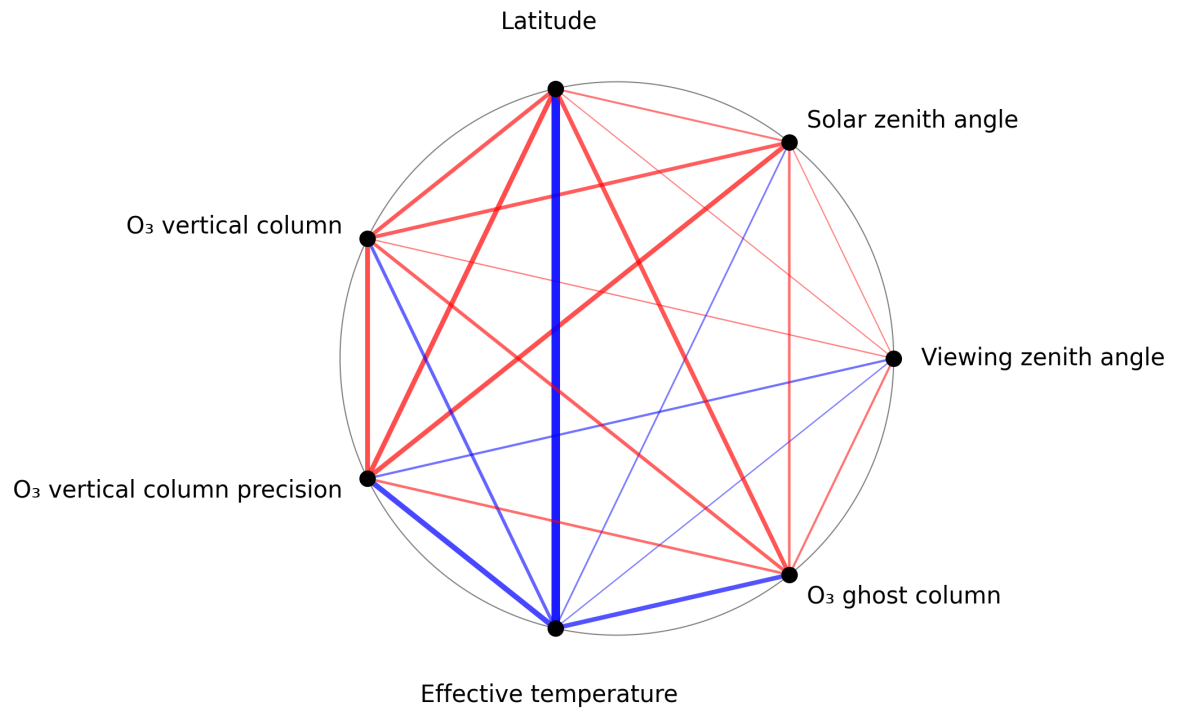
Figure 1: Map of correlation graph for 2024-12-13 to 2024-12-15.
