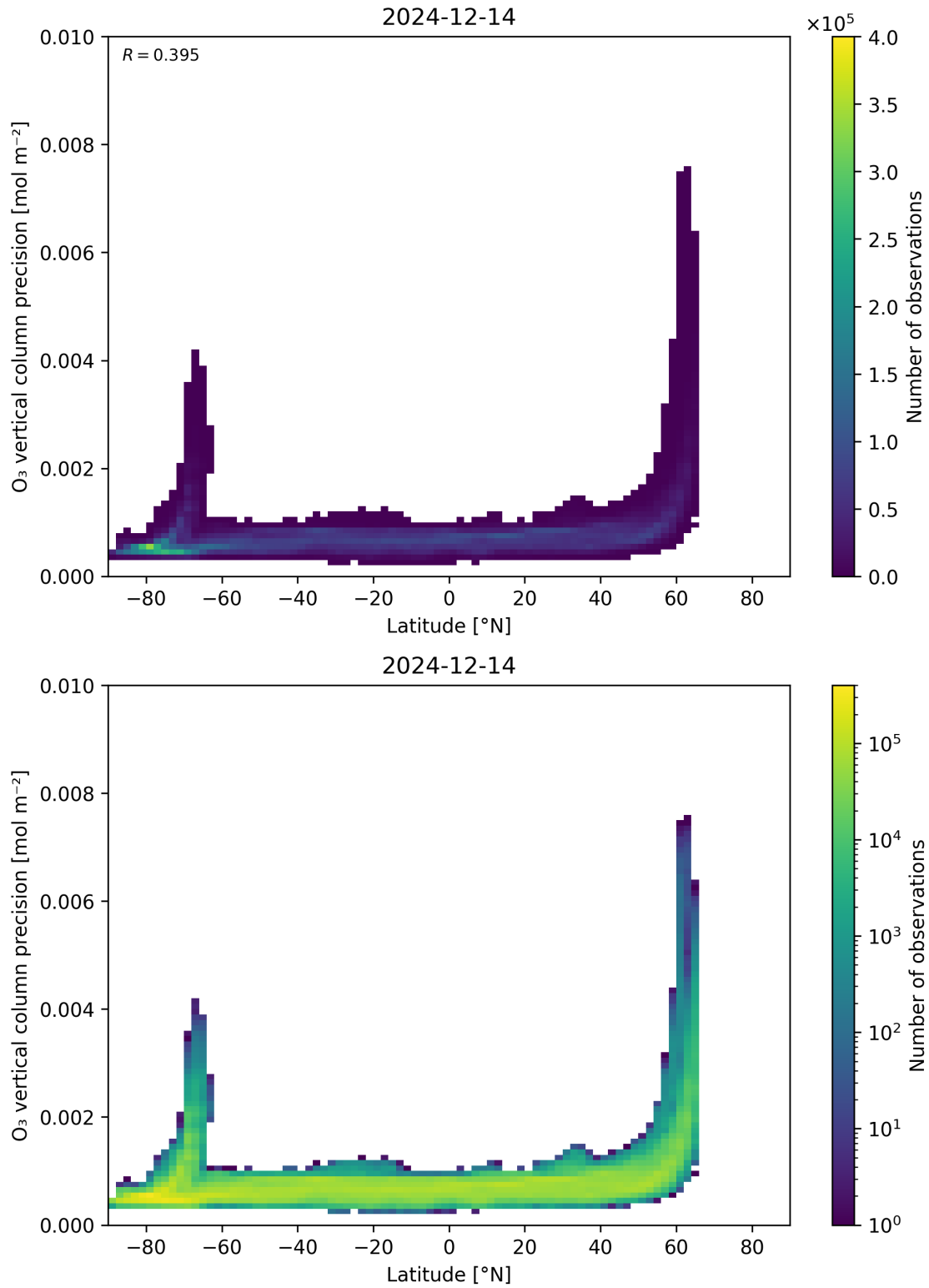
Figure 37: Scatter density plot of “Latitude” against “O 3 vertical column precision” for 2024-12-13 to 2024-12-15.
