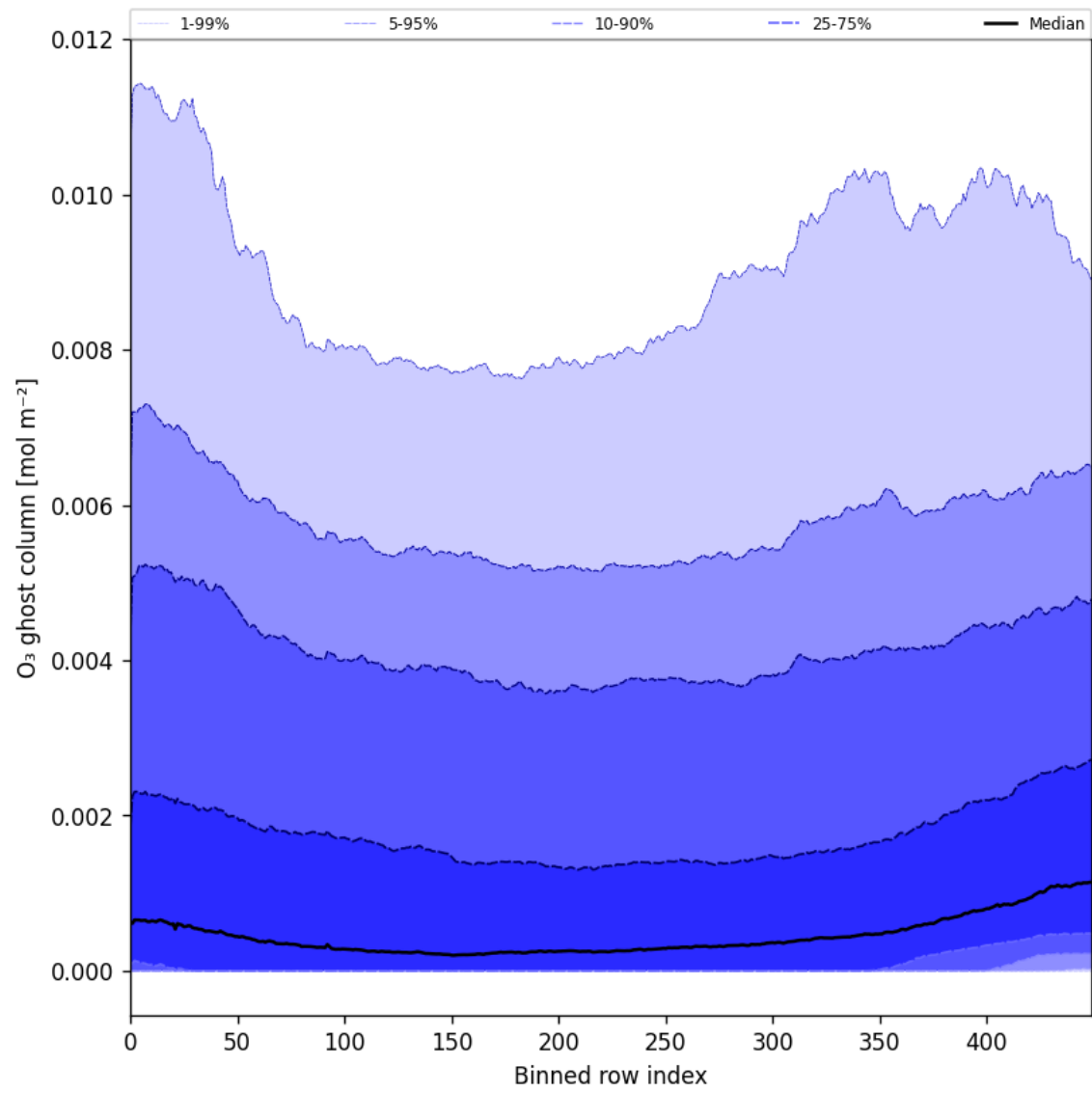
Figure 32: Along track statistics of “O 3 ghost column” for 2024-12-13 to 2024-12-15
