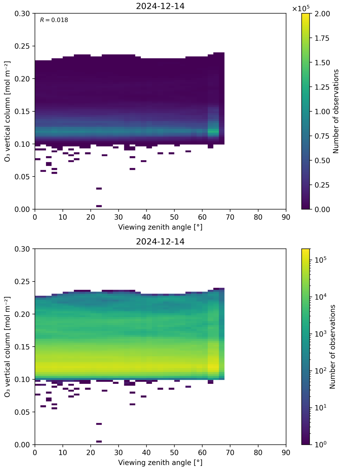
Figure 52: Scatter density plot of “Viewing zenith angle” against “O 3 vertical column” for 2024-12-13 to 2024-12-15.
