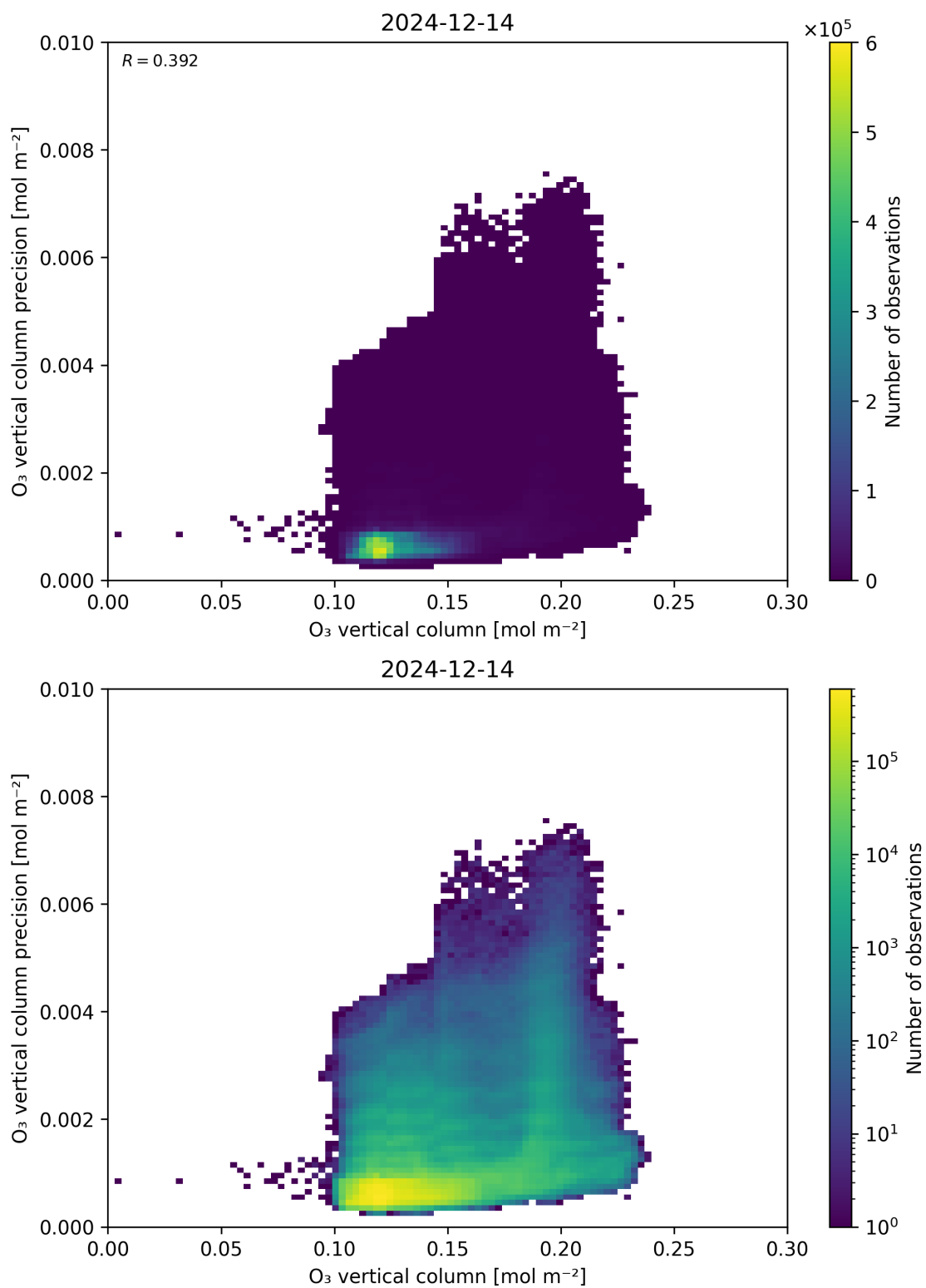
Figure 41: Scatter density plot of “O 3 vertical column” against “O 3 vertical column precision” for 2024-12-13 to 2024-12-15.
