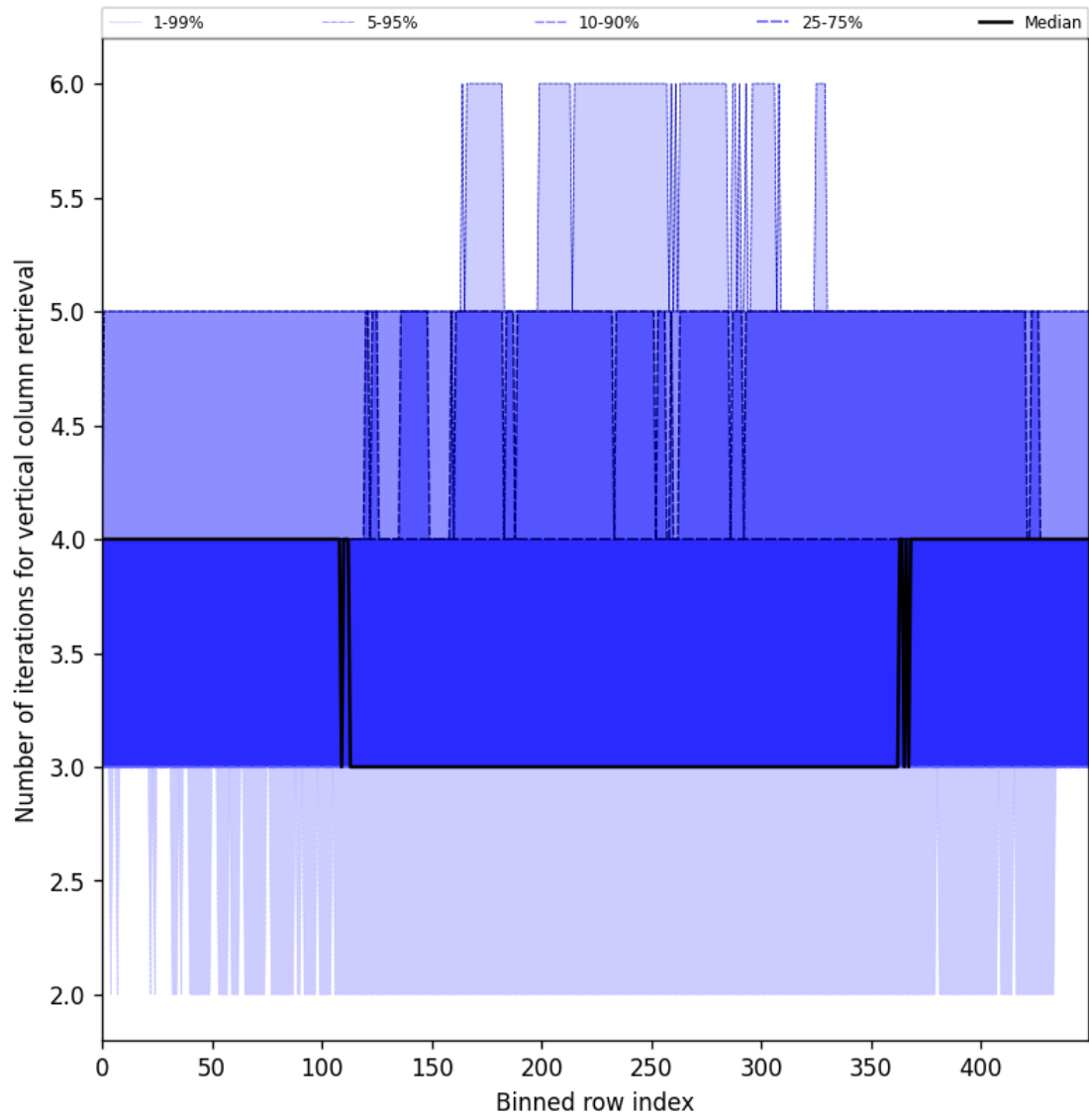
Figure 33: Along track statistics of “Number of iterations for vertical column retrieval” for 2024-12-13 to 2024-12-15
