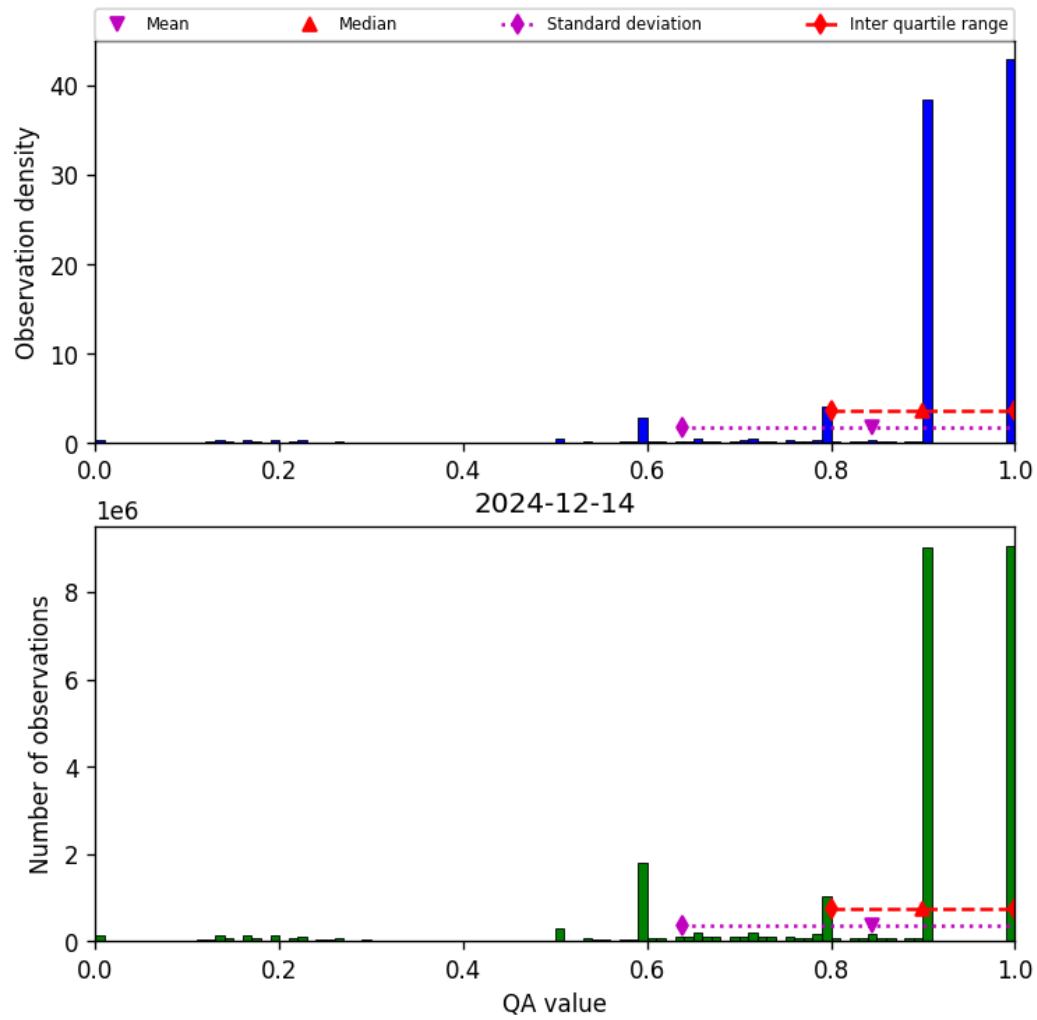
Figure 20: Histogram of “QA value” for 2024-12-13 to 2024-12-15
