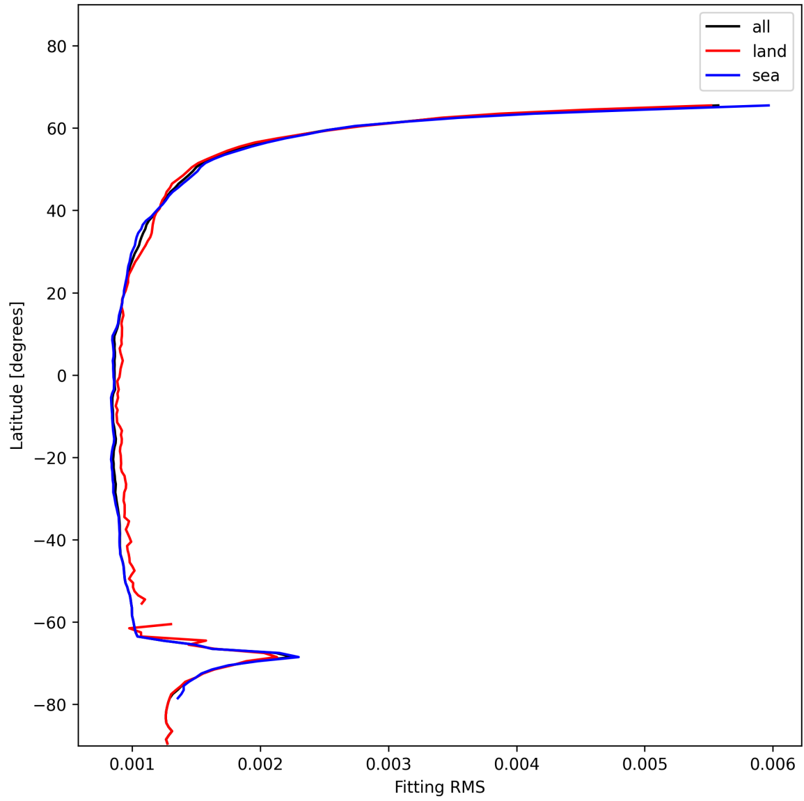
Figure 16: Zonal average of “Fitting RMS” for 2024-12-13 to 2024-12-15.
