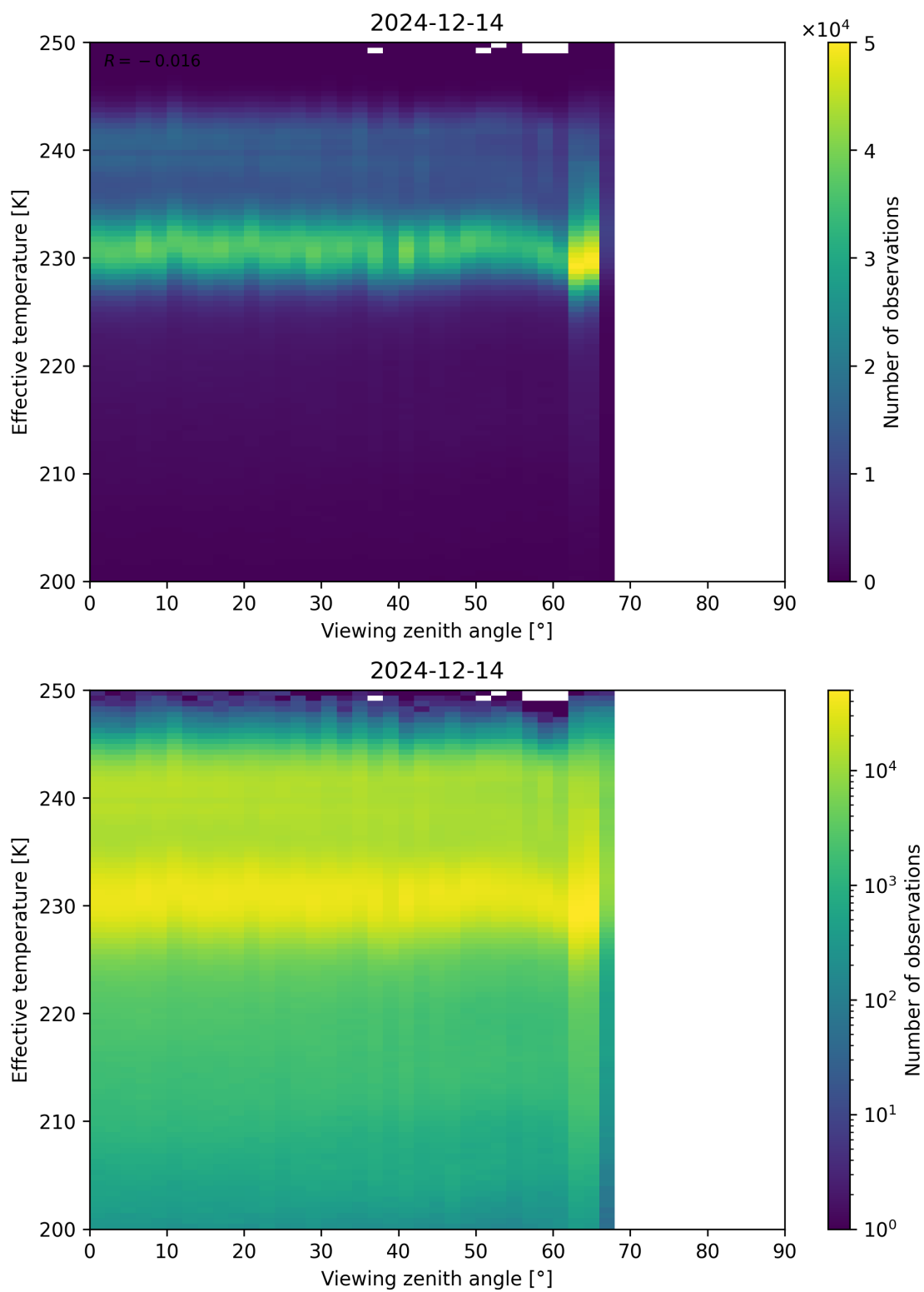
Figure 50: Scatter density plot of “Viewing zenith angle” against “Effective temperature” for 2024-12-13 to 2024-12-15.
