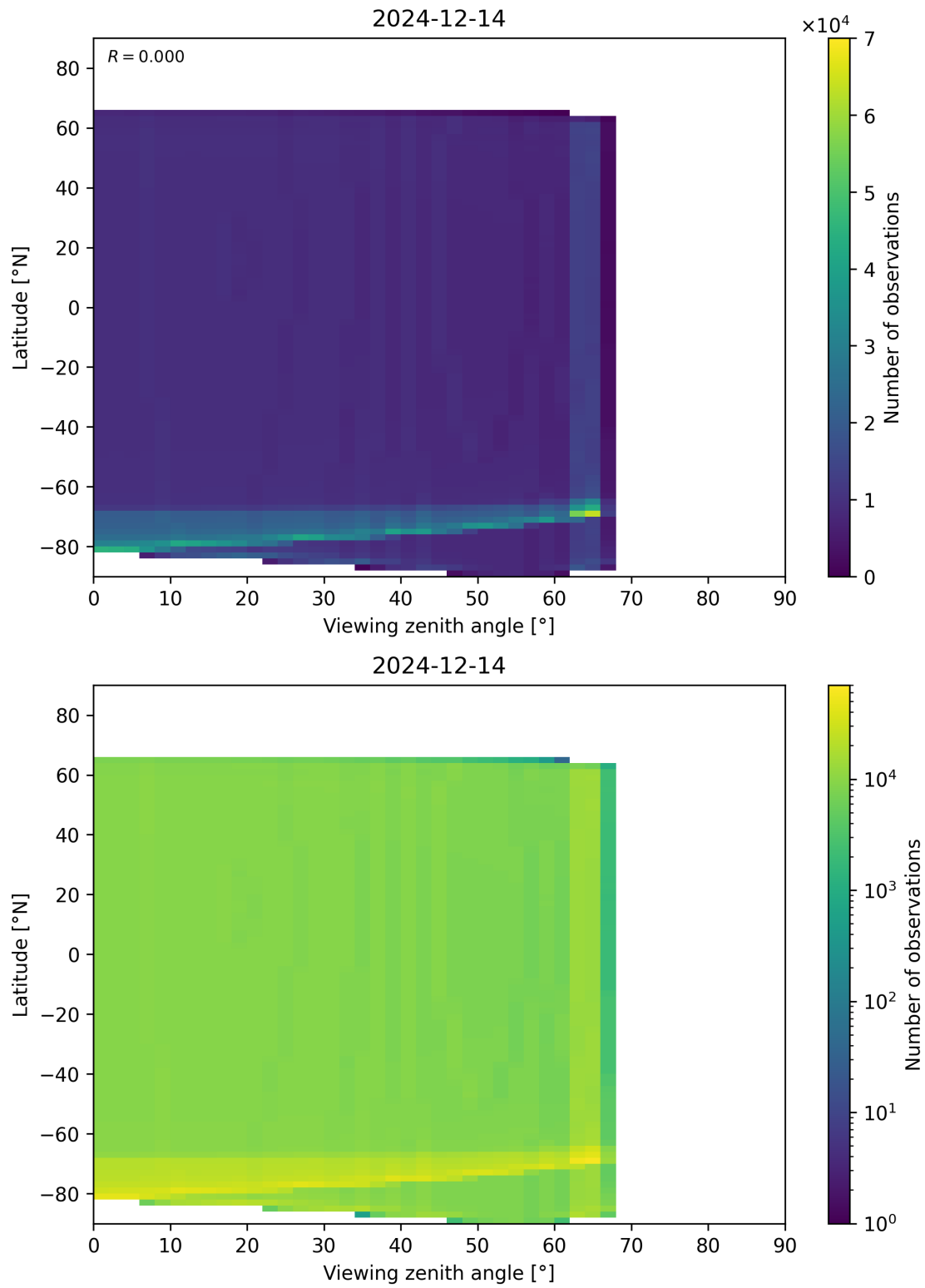
Figure 49: Scatter density plot of “Viewing zenith angle” against “Latitude” for 2024-12-13 to 2024-12-15.
