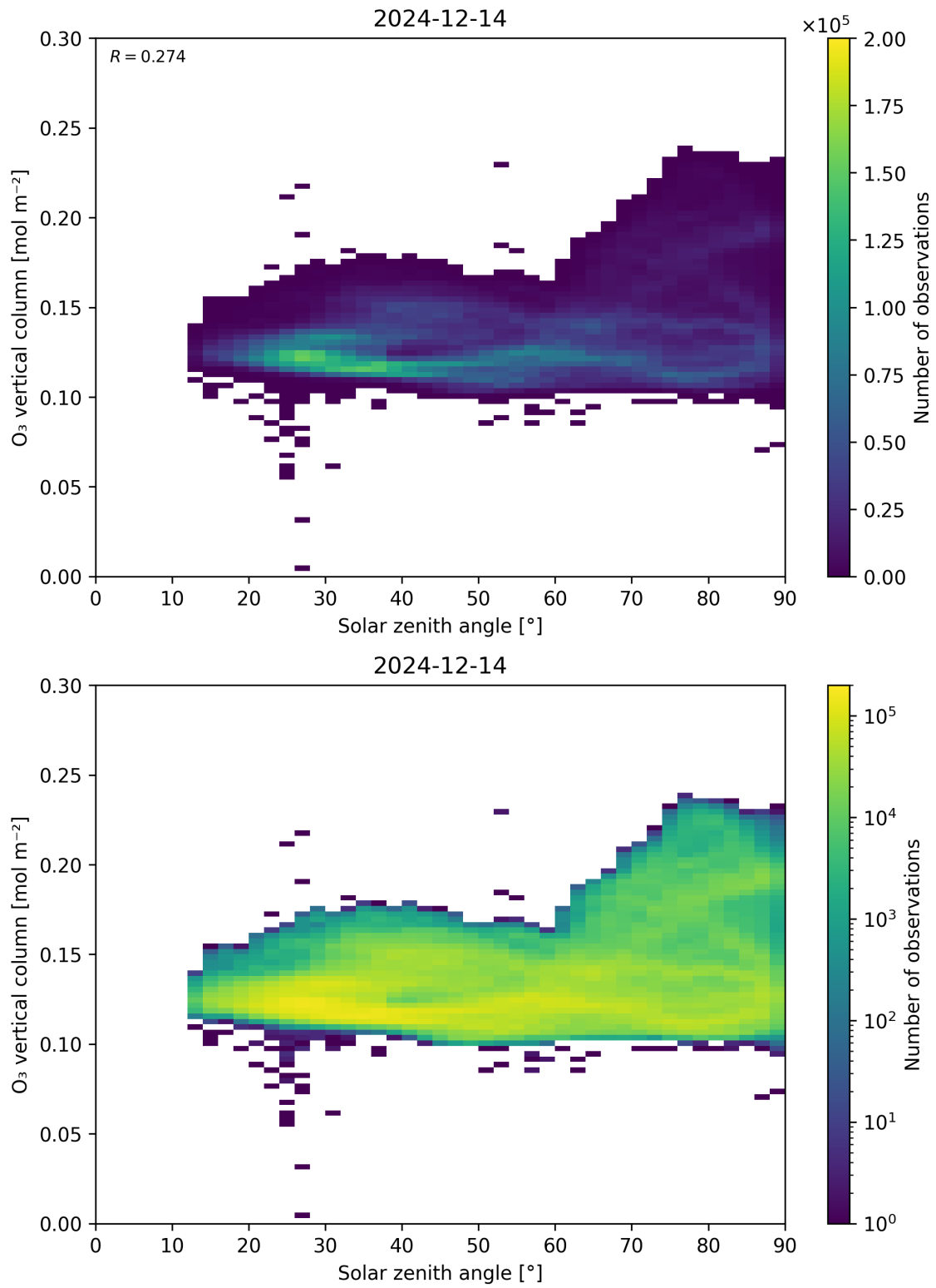
Figure 47: Scatter density plot of “Solar zenith angle” against “O 3 vertical column” for 2024-12-13 to 2024-12-15.
