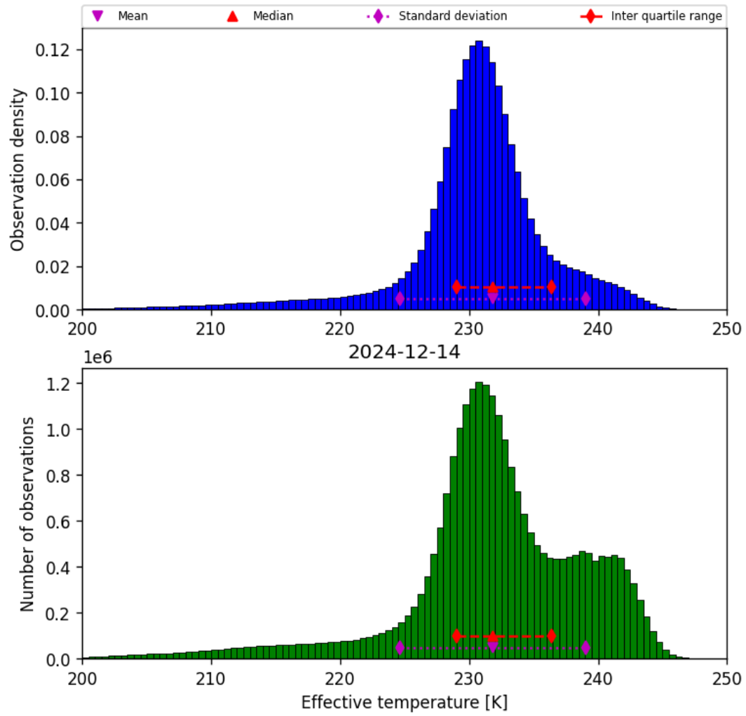
Figure 24: Histogram of “Effective temperature” for 2024-12-13 to 2024-12-15
