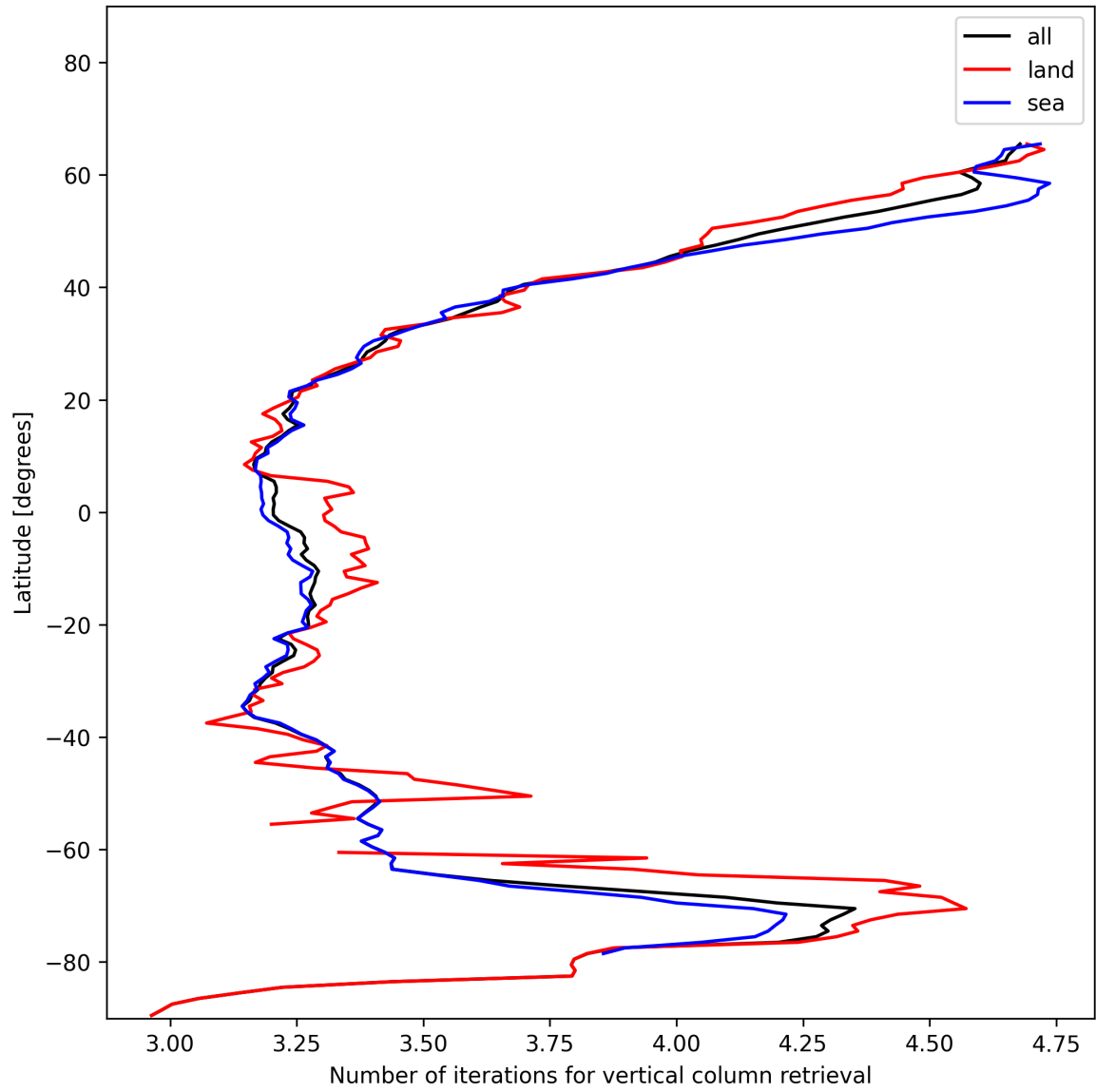
Figure 19: Zonal average of “Number of iterations for vertical column retrieval” for 2024-12-13 to 2024-12-15.
