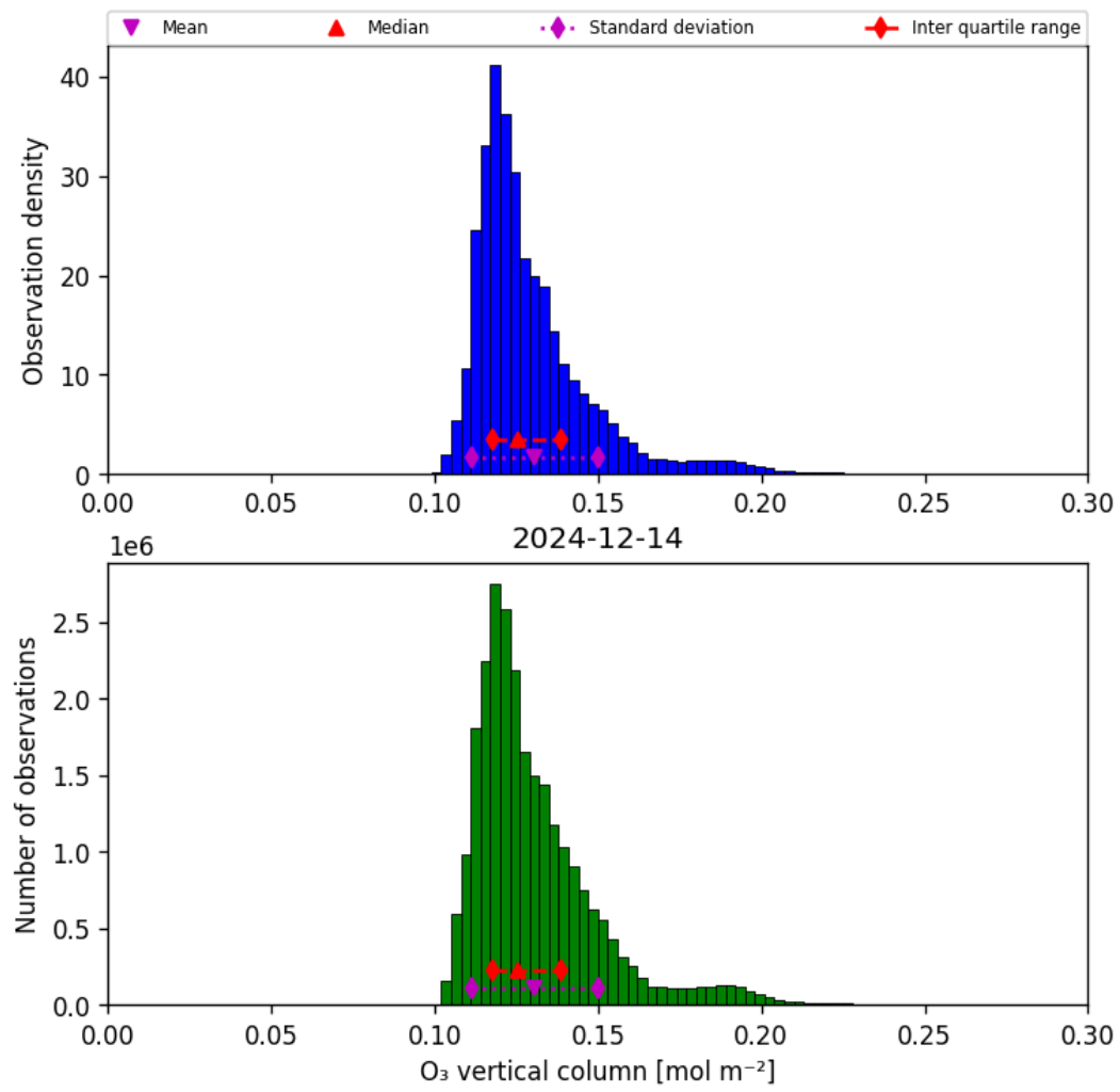
Figure 21: Histogram of “O 3 vertical column” for 2024-12-13 to 2024-12-15
