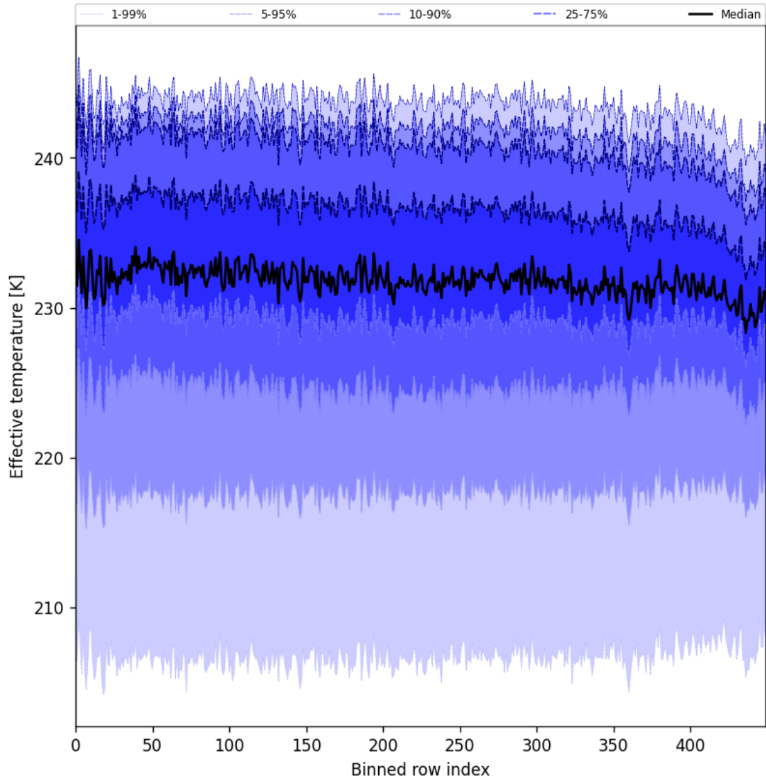
Figure 31: Along track statistics of "Effective temperature" for 2024-12-13 to 2024-12-15
