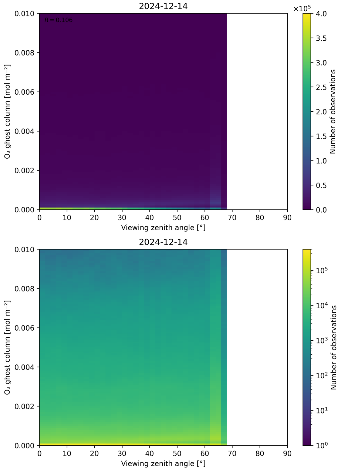
Figure 51: Scatter density plot of “Viewing zenith angle” against “O 3 ghost column” for 2024-12-13 to 2024-12-15.
