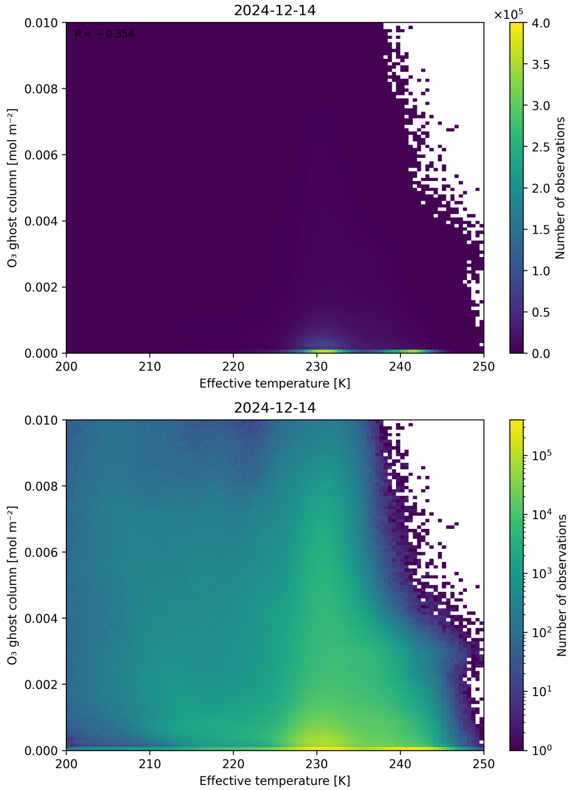
Figure 38: Scatter density plot of “Effective temperature” against “O 3 ghost column” for 2024-12-13 to 2024-12-15.
